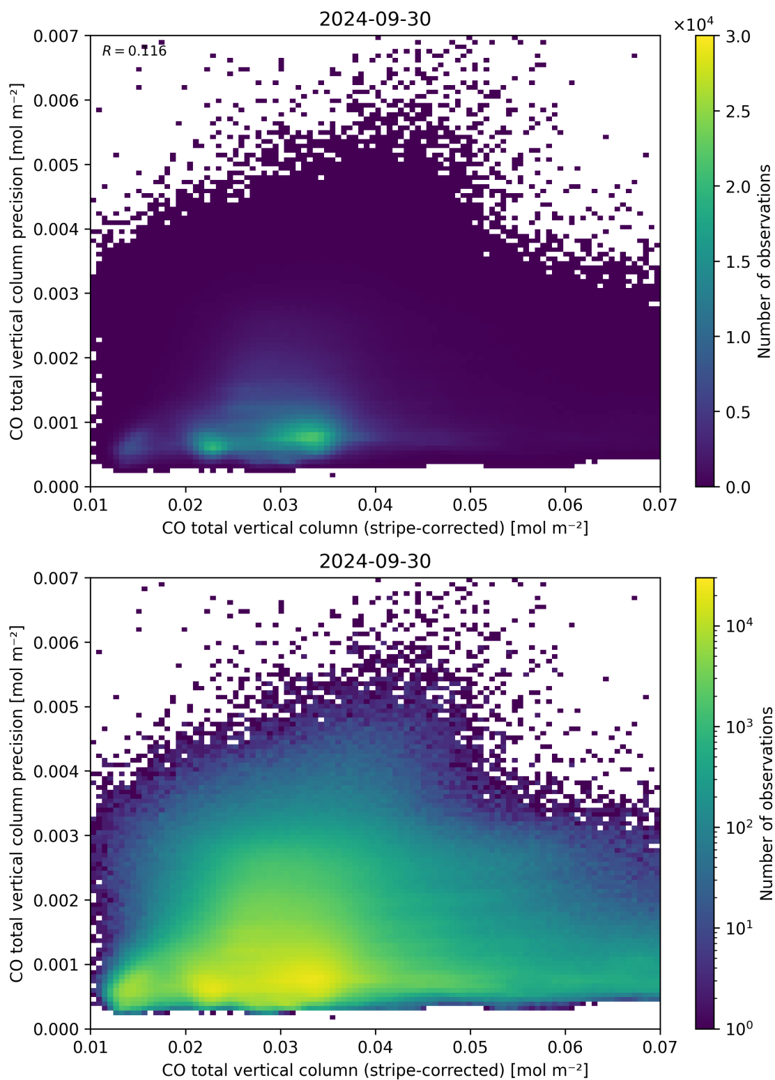
Figure 36: Scatter density plot of “CO total vertical column (stripe-corrected)” against “CO total vertical column precision” for 2024-09-29 to 2024-10-01.
