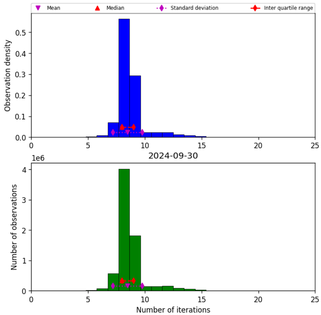
Figure 24: Histogram of “Number of iterations” for 2024-09-29 to 2024-10-01
