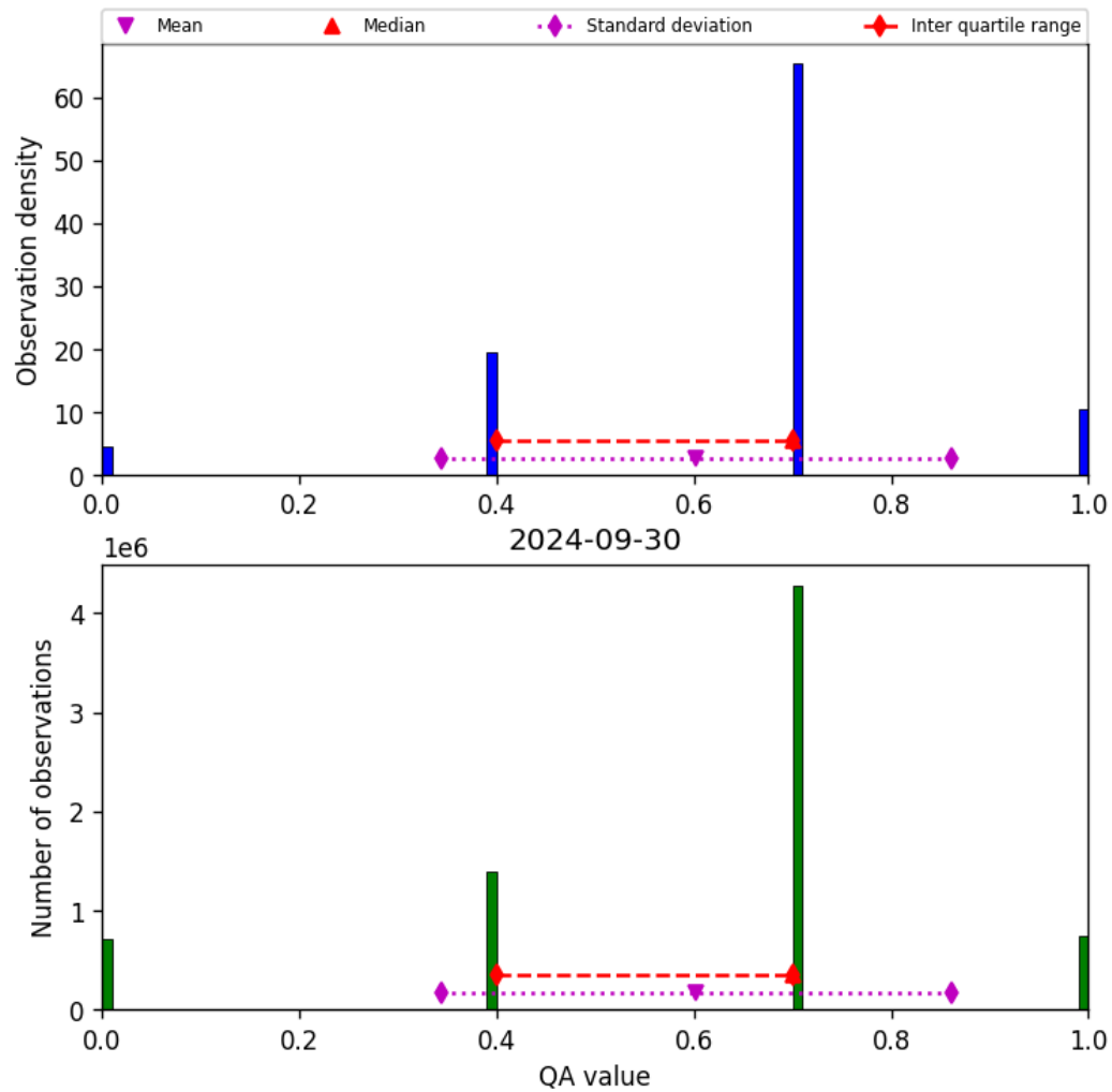
Figure 17: Histogram of “QA value” for 2024-09-29 to 2024-10-01
