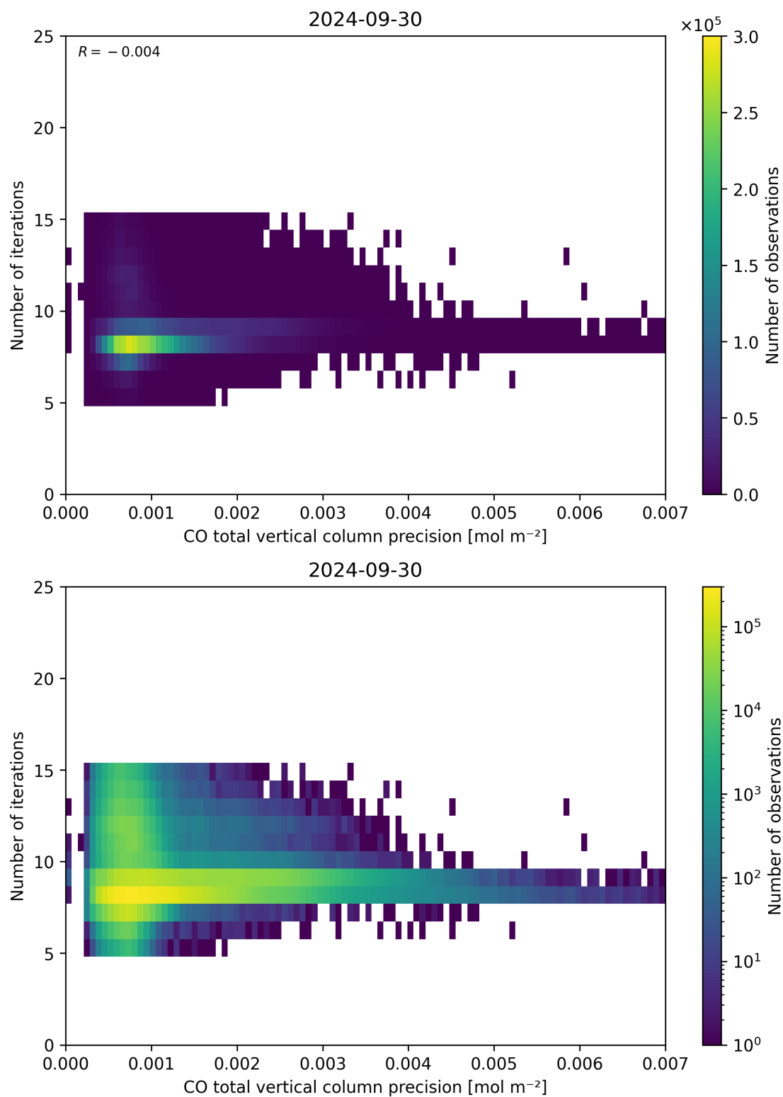
Figure 46: Scatter density plot of “CO total vertical column precision” against “Number of iterations” for 2024-09-29 to 2024-10-01.
