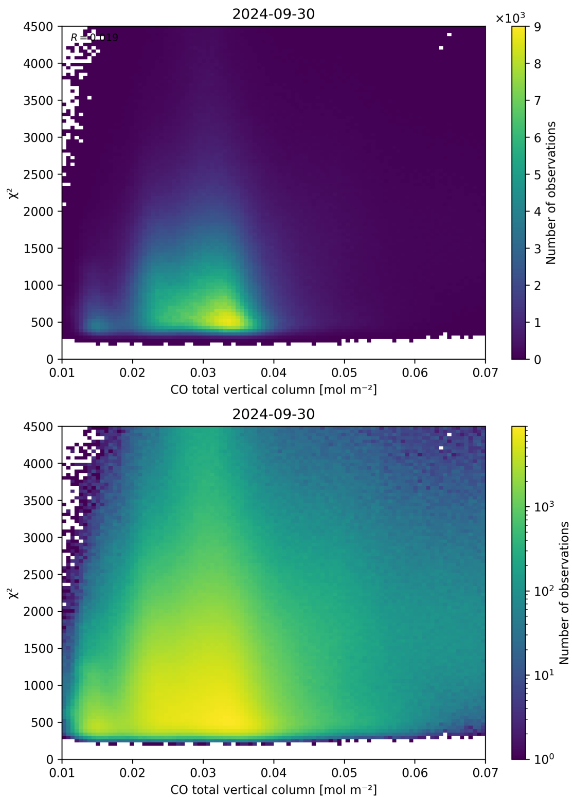
Figure 35: Scatter density plot of “CO total vertical column” against “ \chi^2 ” for 2024-09-29 to 2024-10-01.
