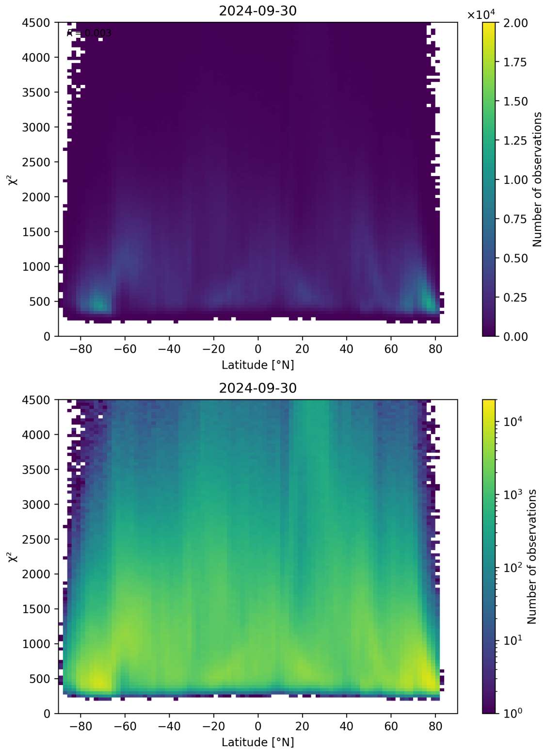
Figure 54: Scatter density plot of “Latitude” against “ \chi^2 ” for 2024-09-29 to 2024-10-01.
