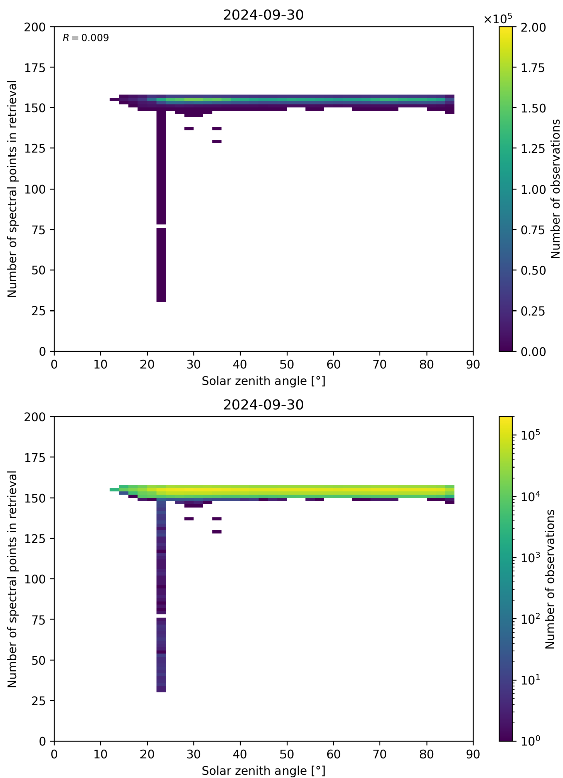
Figure 68: Scatter density plot of “Solar zenith angle” against “Number of spectral points in retrieval” for 2024-09-29 to 2024-10-01.
