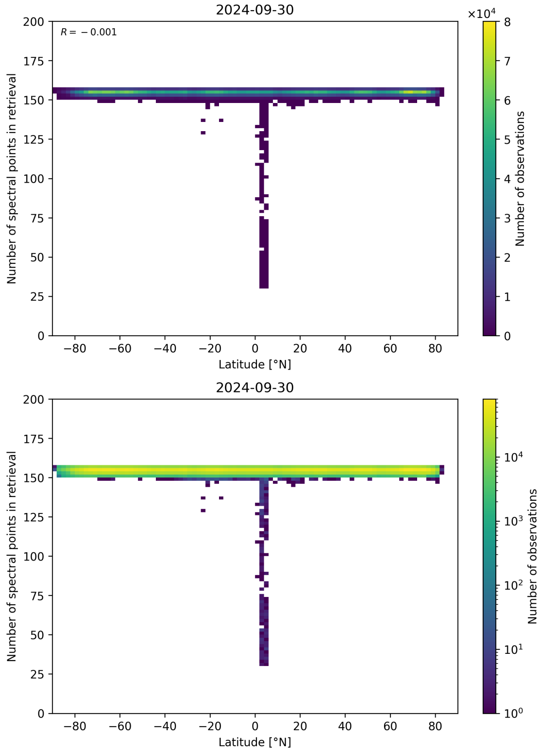
Figure 57: Scatter density plot of “Latitude” against “Number of spectral points in retrieval” for 2024-09-29 to 2024-10-01.
