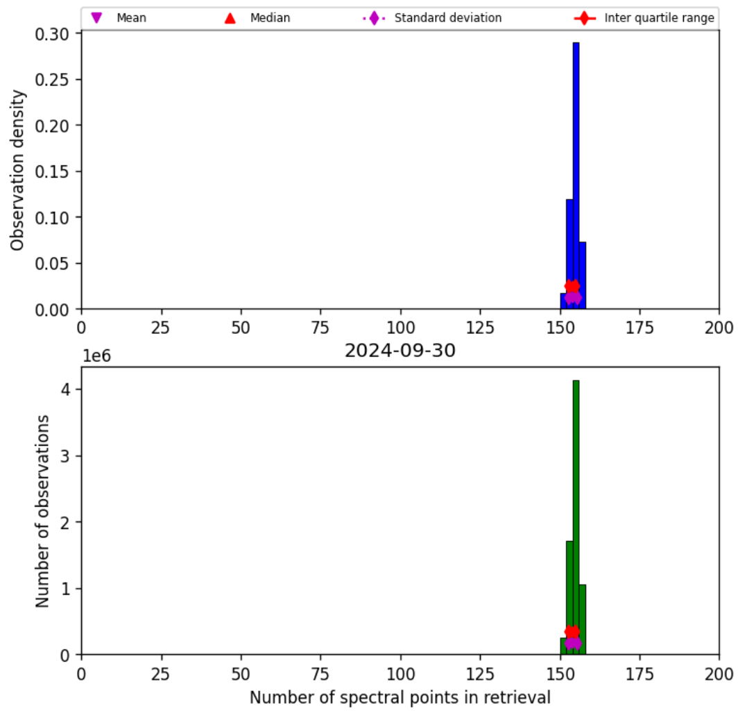
Figure 21: Histogram of “Number of spectral points in retrieval” for 2024-09-29 to 2024-10-01
