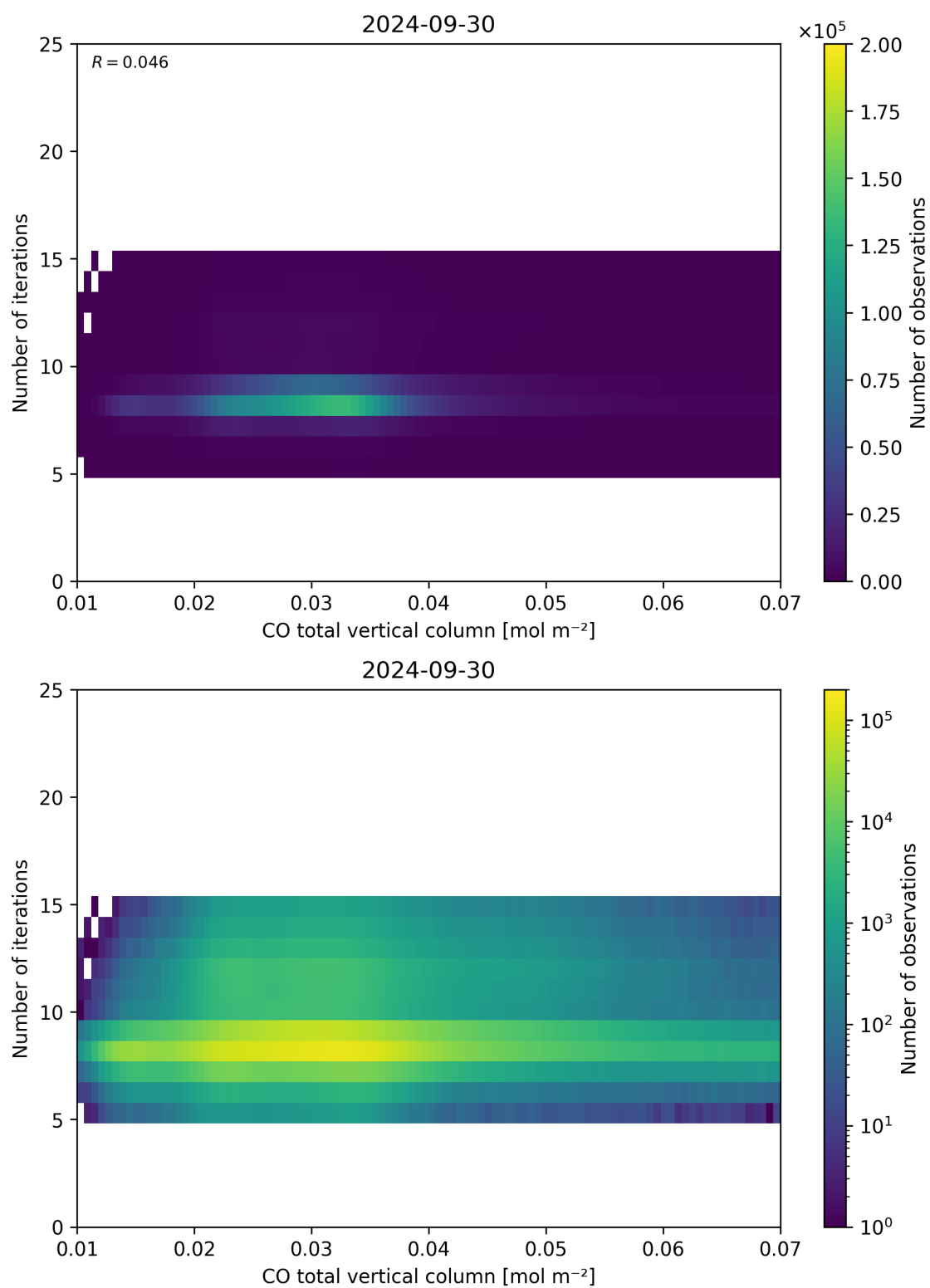
Figure 42: Scatter density plot of “CO total vertical column” against “Number of iterations” for 2024-09-29 to 2024-10-01.
