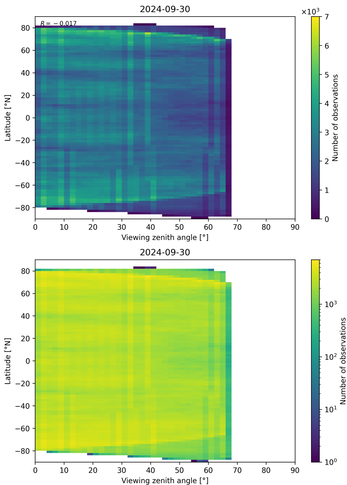
Figure 74: Scatter density plot of “Viewing zenith angle” against “Latitude” for 2024-09-29 to 2024-10-01.
