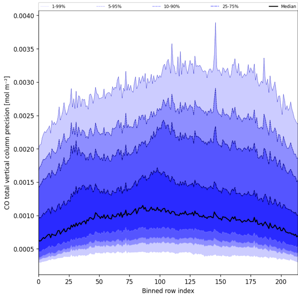
Figure 28: Along track statistics of "CO total vertical column precision" for 2024-09-29 to 2024-10-01
