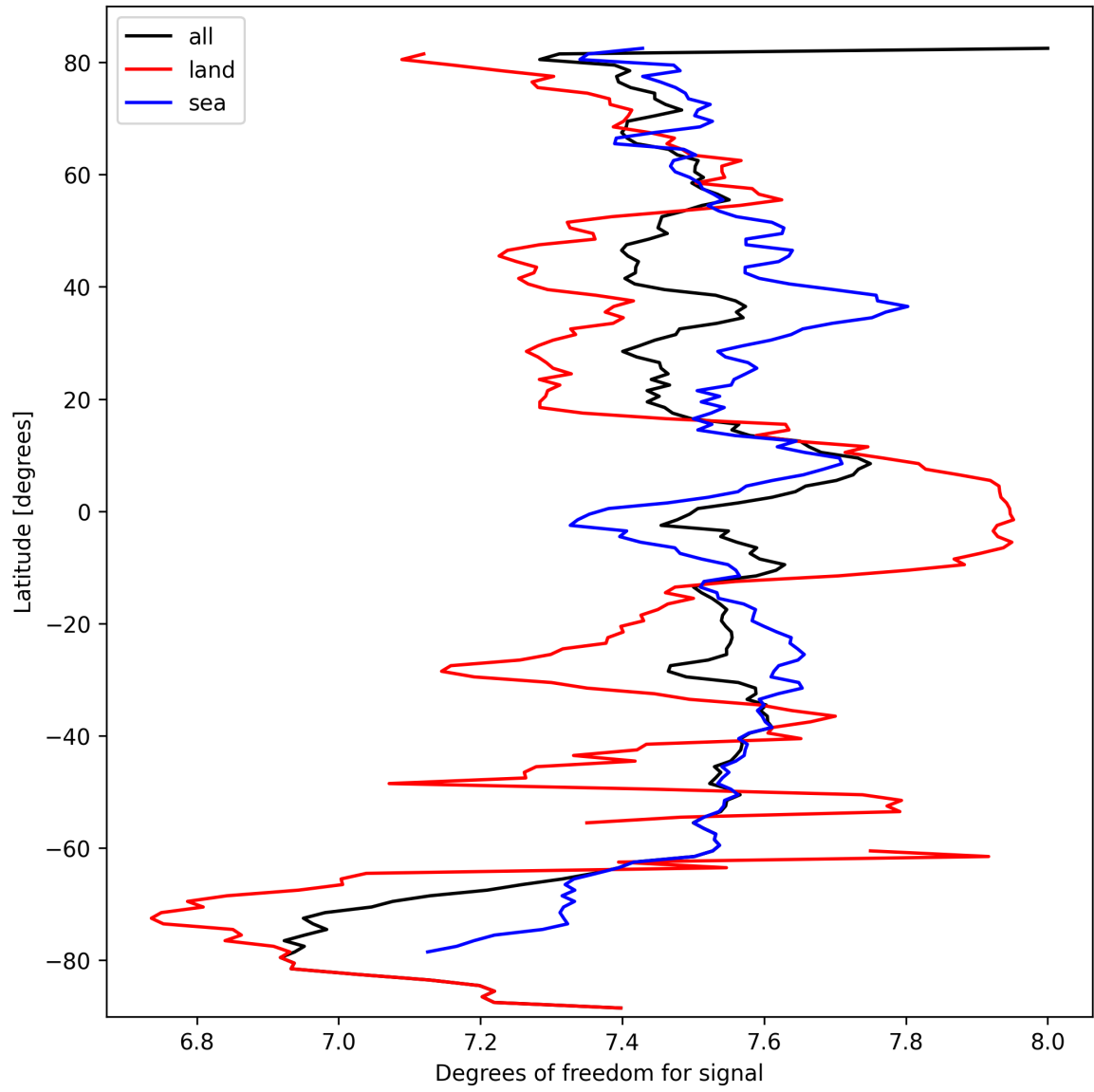
Figure 15: Zonal average of “Degrees of freedom for signal” for 2024-09-29 to 2024-10-01.
