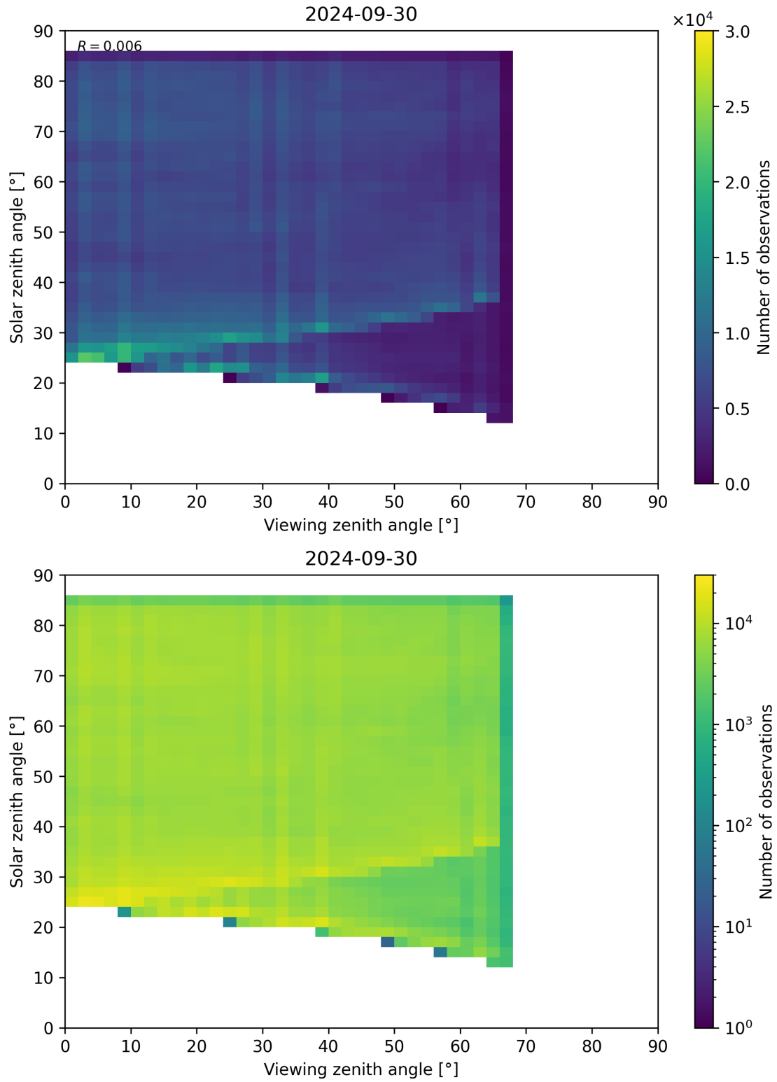
Figure 77: Scatter density plot of “Viewing zenith angle” against “Solar zenith angle” for 2024-09-29 to 2024-10-01.
