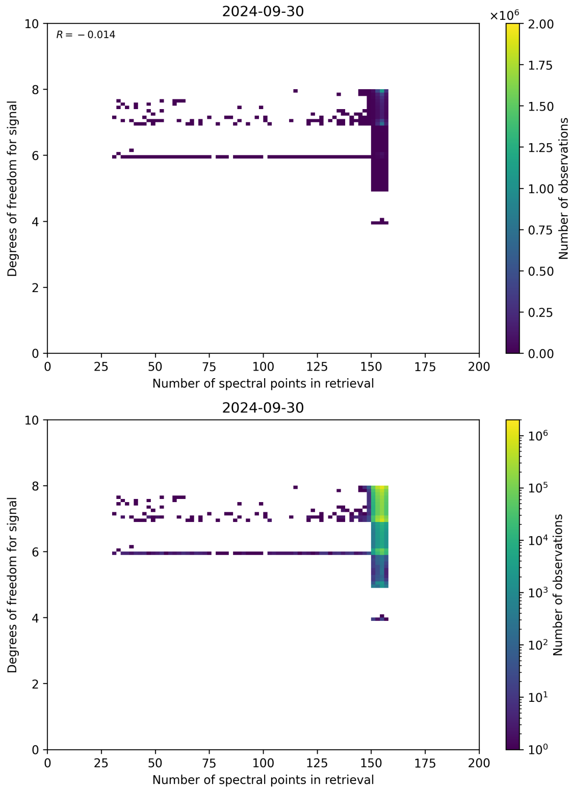
Figure 59: Scatter density plot of “Number of spectral points in retrieval” against “Degrees of freedom for signal” for 2024-09-29 to 2024-10-01.
