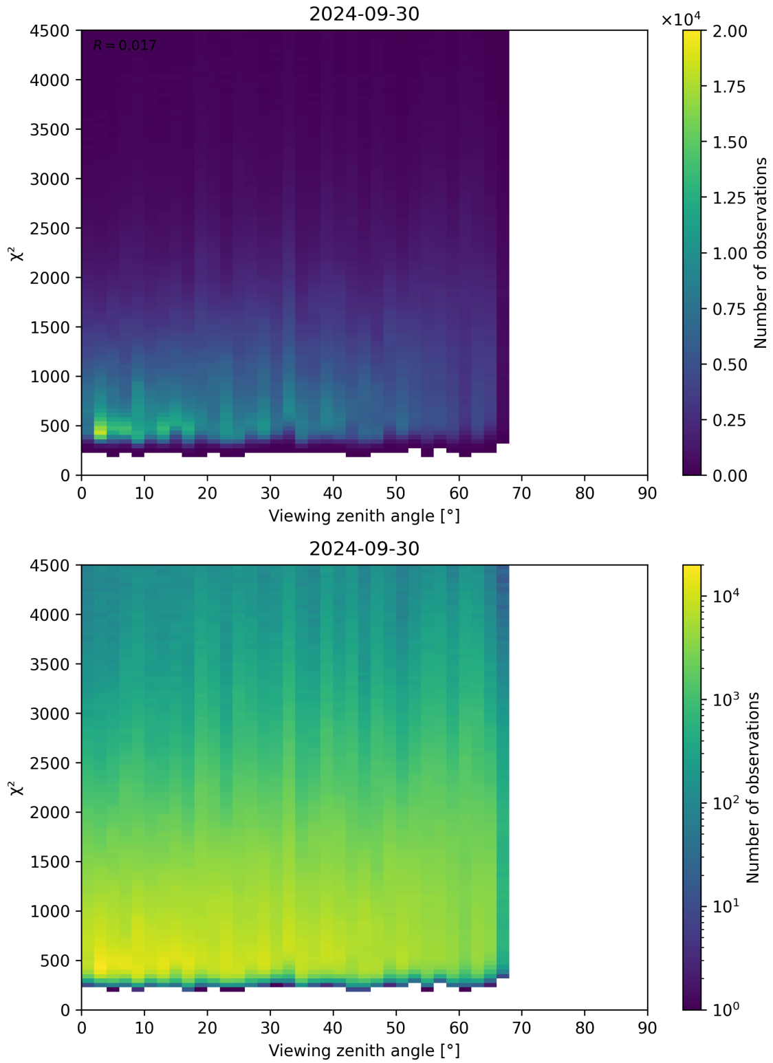
Figure 72: Scatter density plot of “Viewing zenith angle” against “ \chi^2 ” for 2024-09-29 to 2024-10-01.
