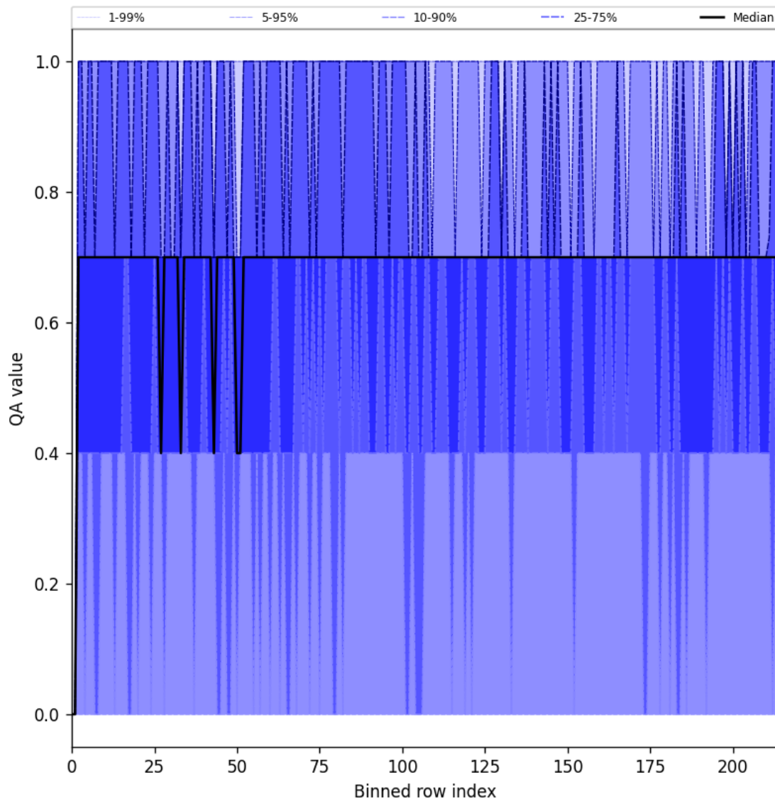
Figure 25: Along track statistics of “QA value” for 2024-09-29 to 2024-10-01
