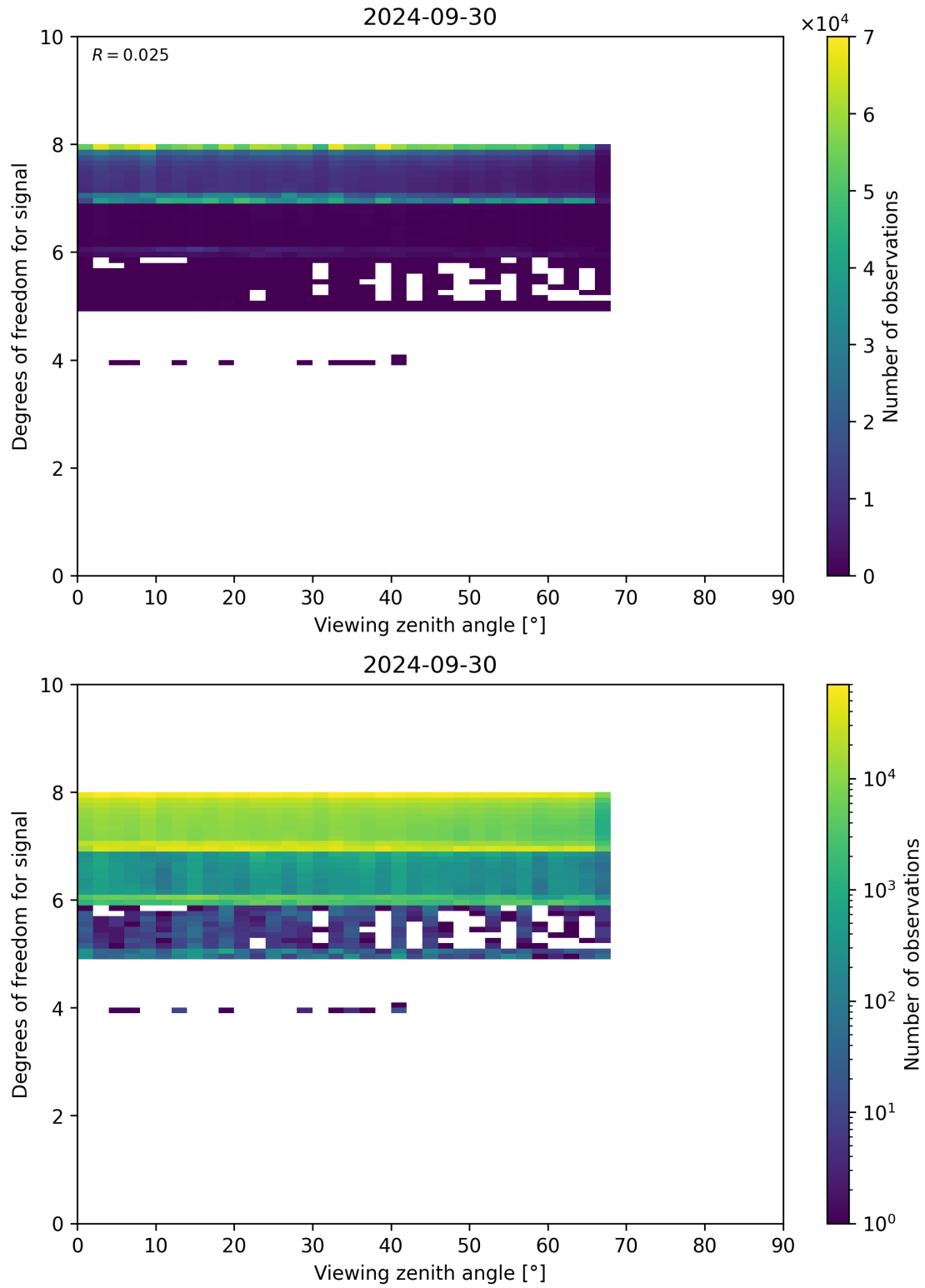
Figure 73: Scatter density plot of “Viewing zenith angle” against “Degrees of freedom for signal” for 2024-09-29 to 2024-10-01.
