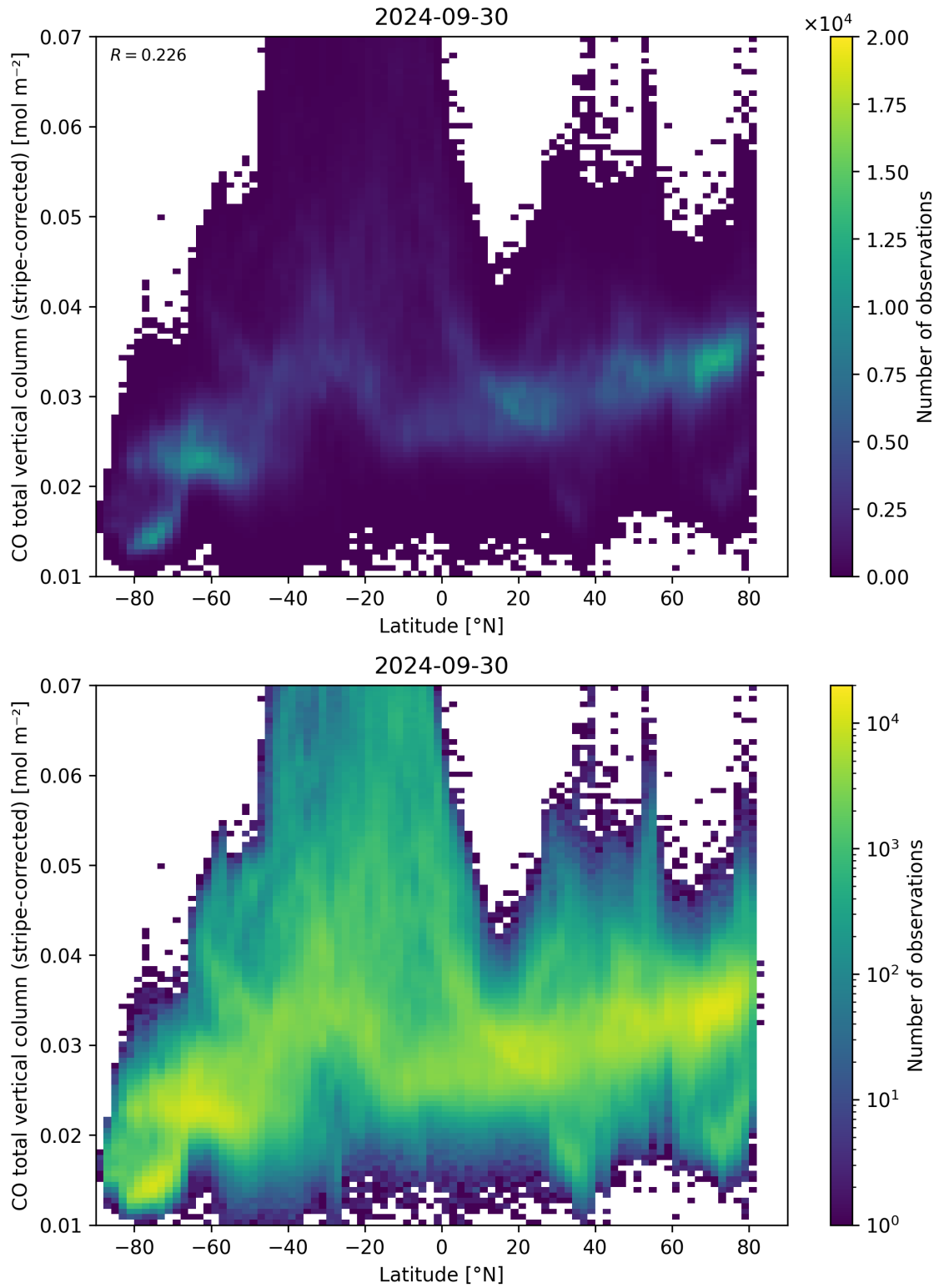
Figure 52: Scatter density plot of “Latitude” against “CO total vertical column (stripe-corrected)” for 2024-09-29 to 2024-10-01.
