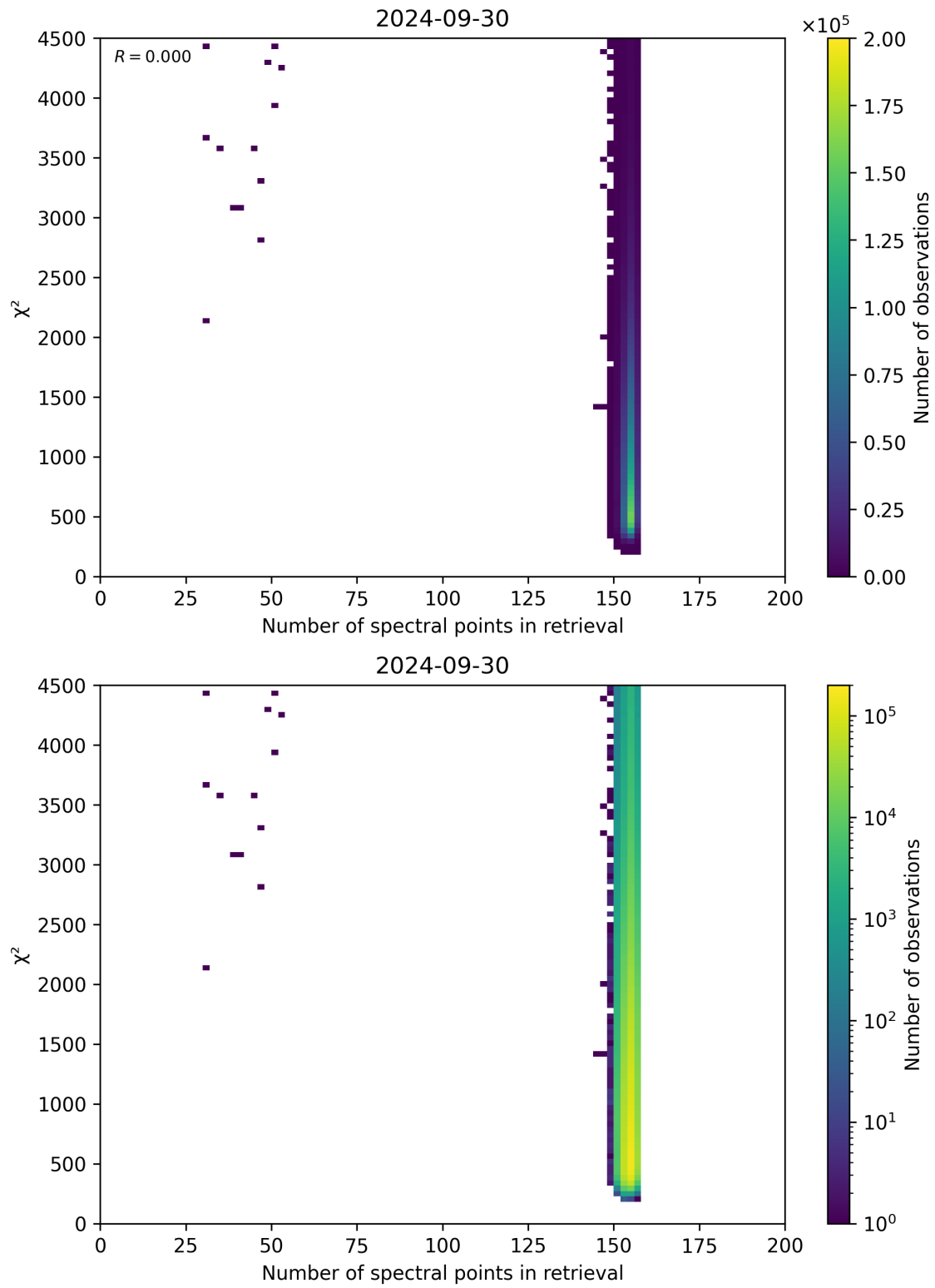
Figure 58: Scatter density plot of “Number of spectral points in retrieval” against “ \chi^2 ” for 2024-09-29 to 2024-10-01.
