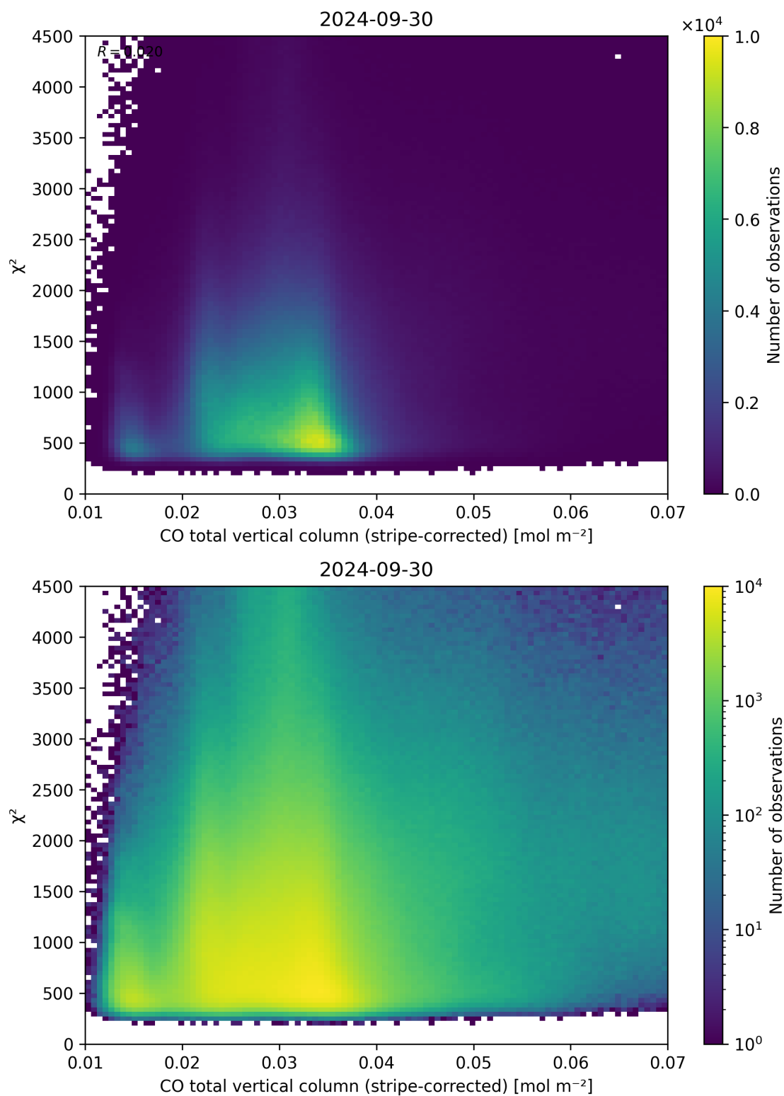
Figure 37: Scatter density plot of “CO total vertical column (stripe-corrected)” against “ \chi^2 ” for 2024-09-29 to 2024-10-01.
