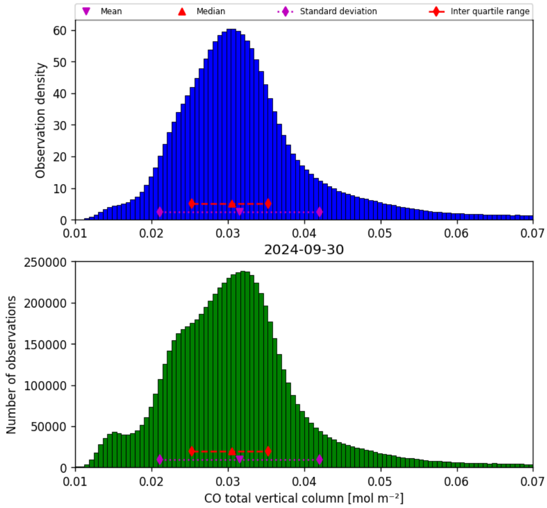
Figure 18: Histogram of “CO total vertical column” for 2024-09-29 to 2024-10-01
