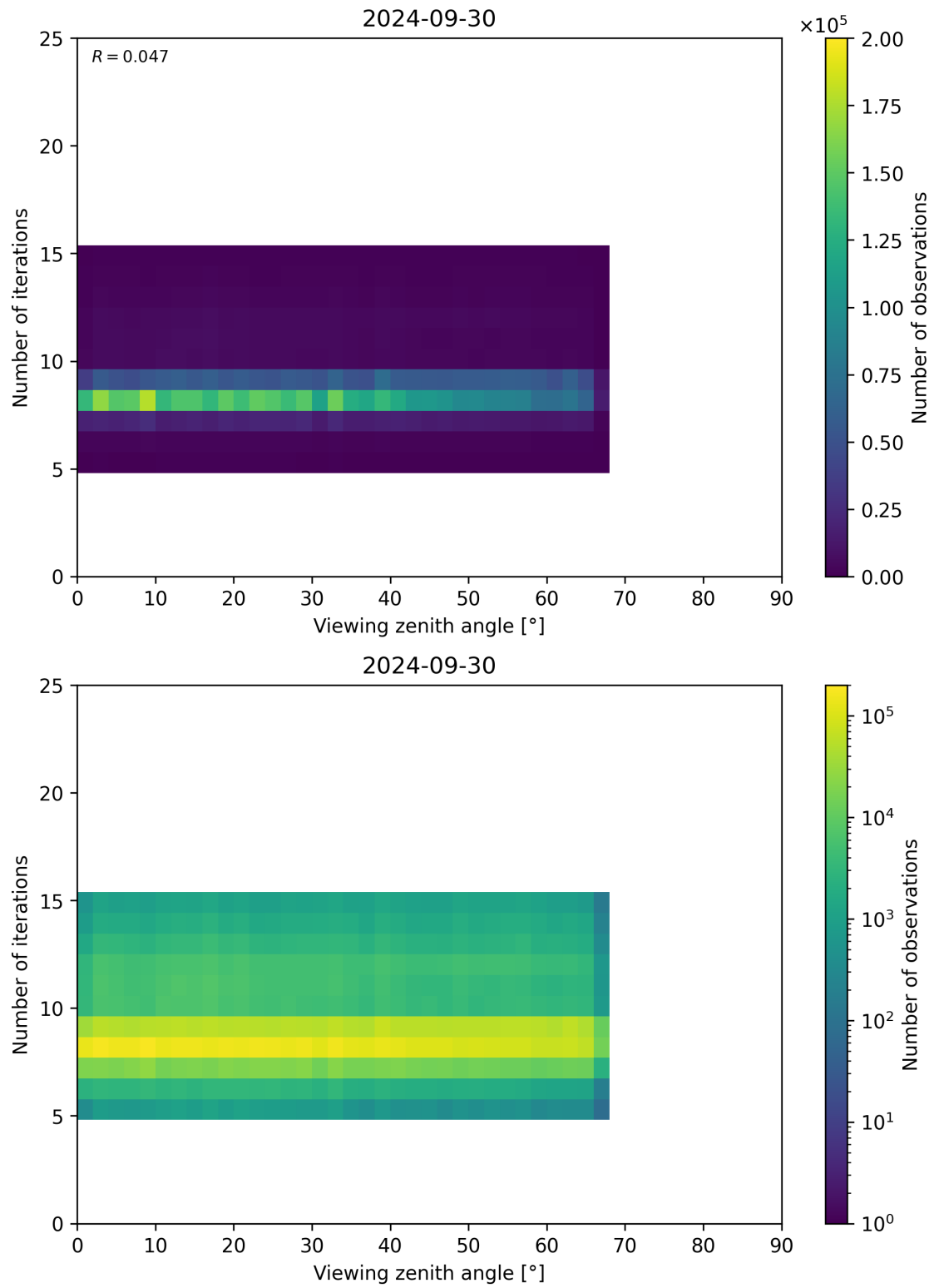
Figure 75: Scatter density plot of “Viewing zenith angle” against “Number of iterations” for 2024-09-29 to 2024-10-01.
