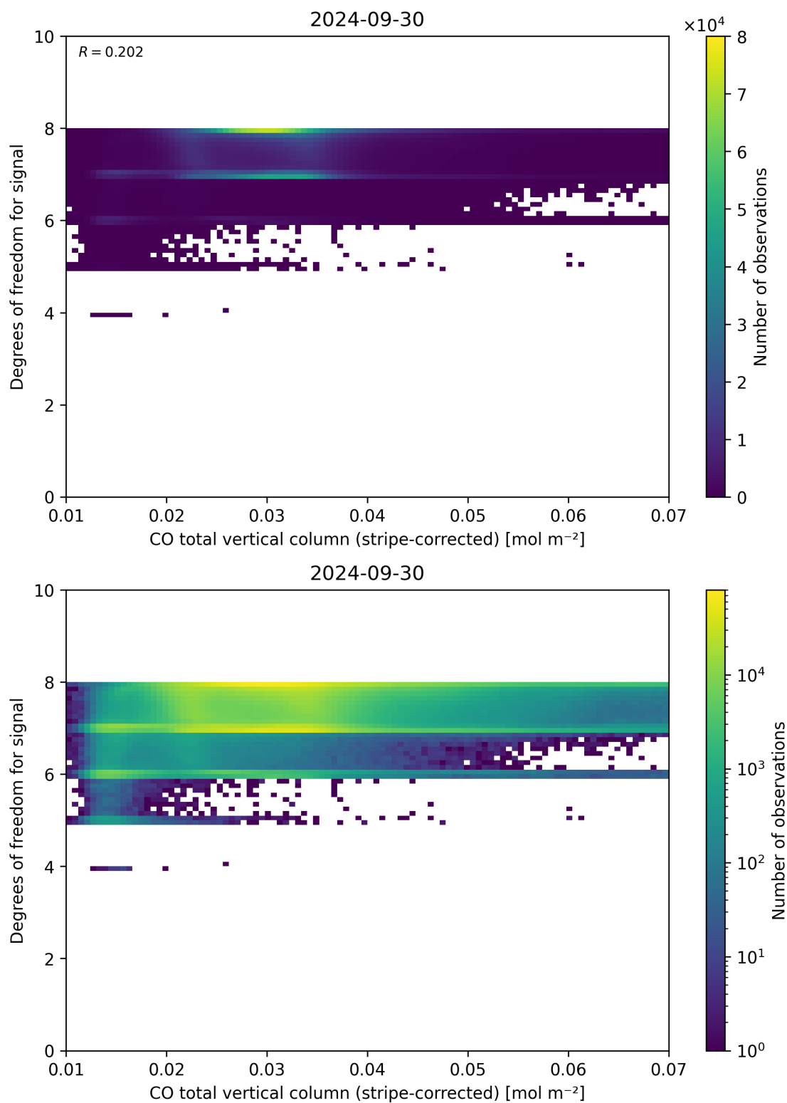
Figure 38: Scatter density plot of “CO total vertical column (stripe-corrected)” against “Degrees of freedom for signal” for 2024-09-29 to 2024-10-01.
