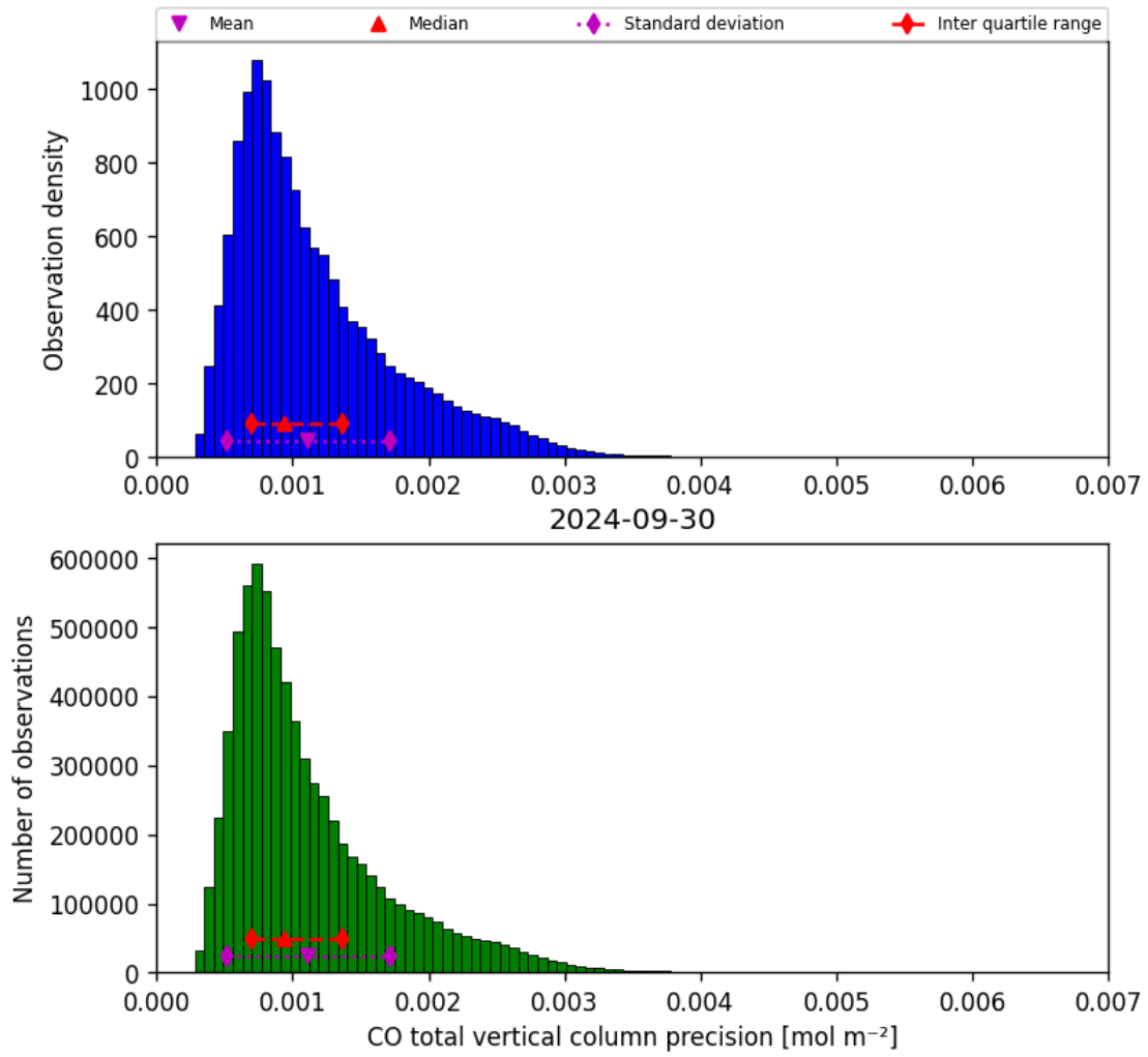
Figure 20: Histogram of “CO total vertical column precision” for 2024-09-29 to 2024-10-01
