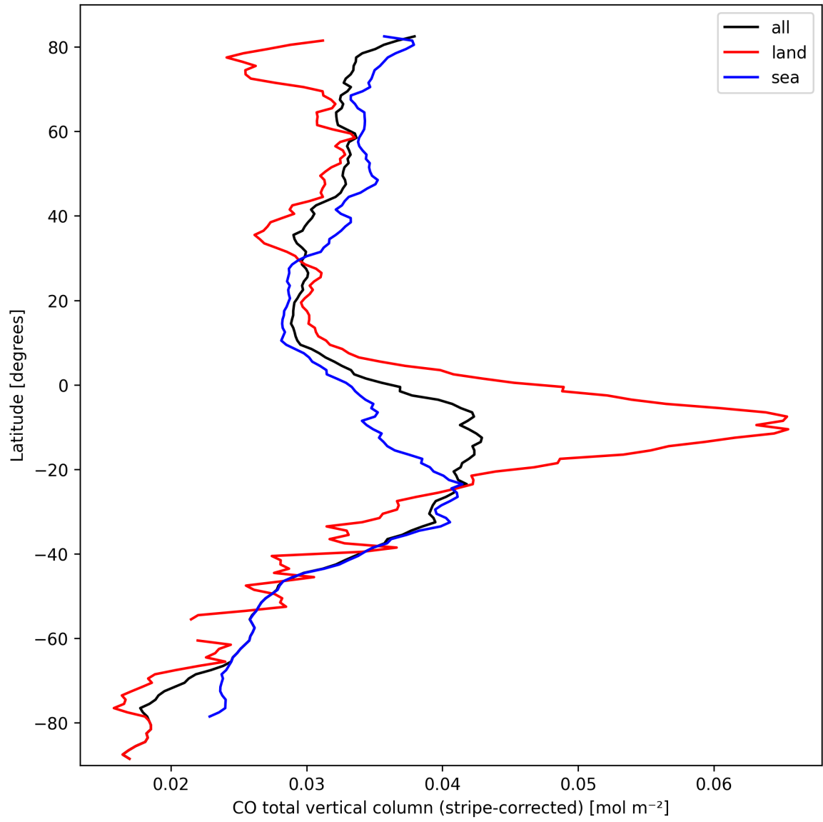
Figure 11: Zonal average of “CO total vertical column (stripe-corrected)” for 2024-09-29 to 2024-10-01.
