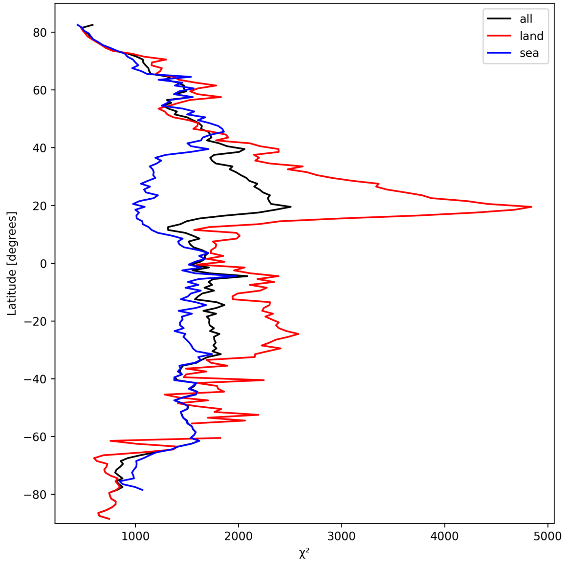
Figure 14: Zonal average of “ \chi^2 ” for 2024-09-29 to 2024-10-01.
