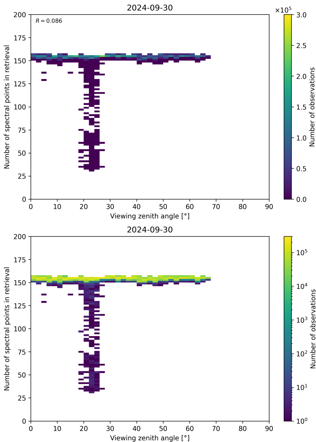
Figure 76: Scatter density plot of “Viewing zenith angle” against “Number of spectral points in retrieval” for 2024-09-29 to 2024-10-01.
