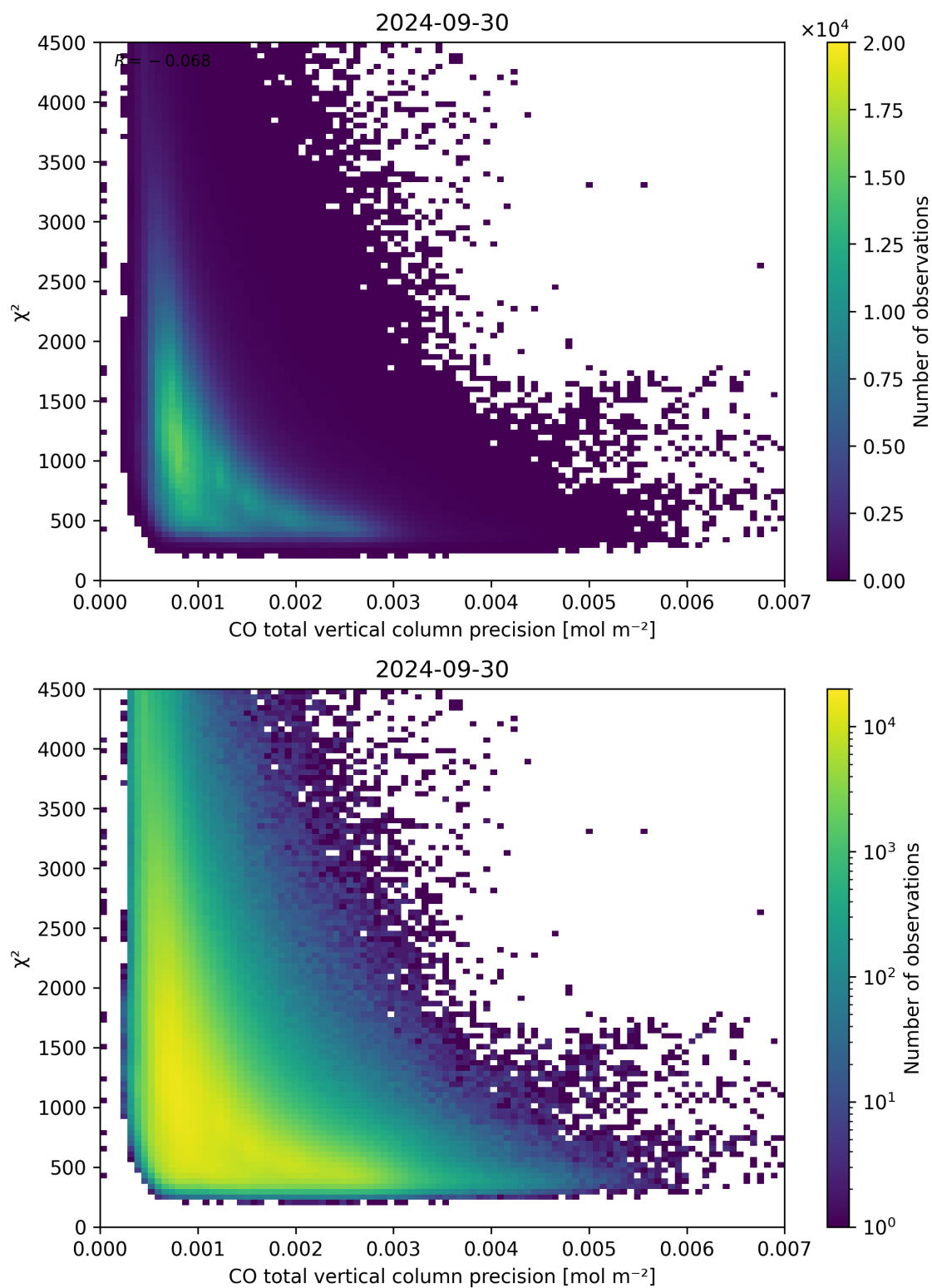
Figure 44: Scatter density plot of “CO total vertical column precision” against “ \chi^2 ” for 2024-09-29 to 2024-10-01.
