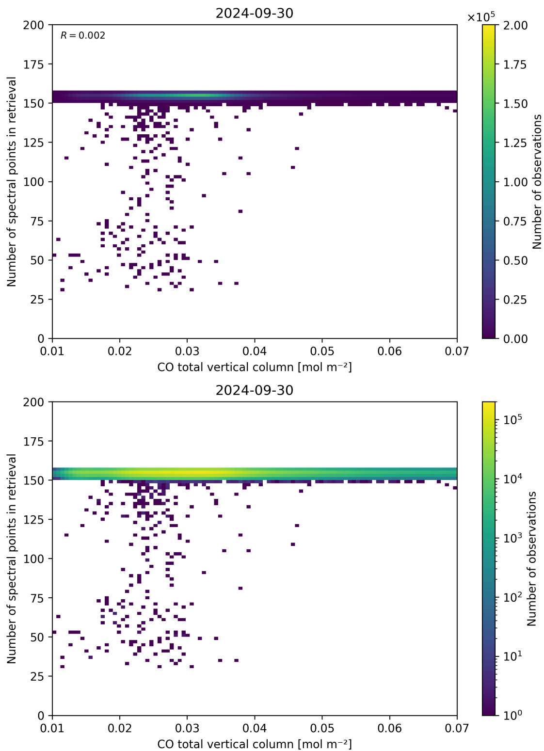
Figure 43: Scatter density plot of “CO total vertical column” against “Number of spectral points in retrieval” for 2024-09-29 to 2024-10-01.
