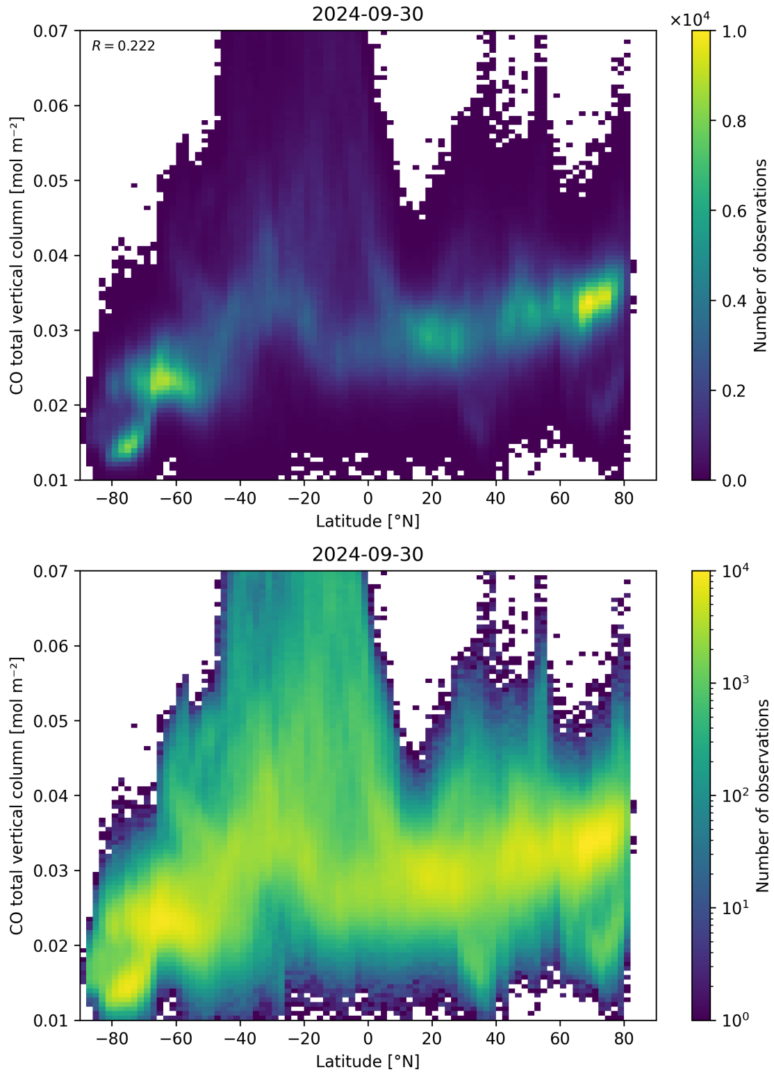
Figure 51: Scatter density plot of “Latitude” against “CO total vertical column” for 2024-09-29 to 2024-10-01.
