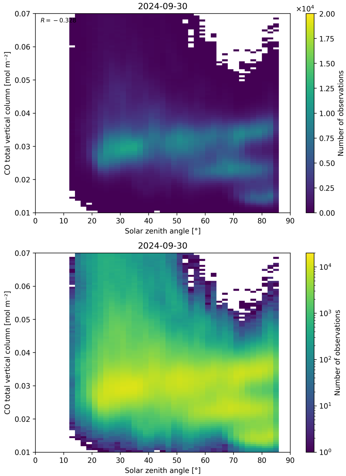
Figure 61: Scatter density plot of “Solar zenith angle” against “CO total vertical column” for 2024-09-29 to 2024-10-01.
