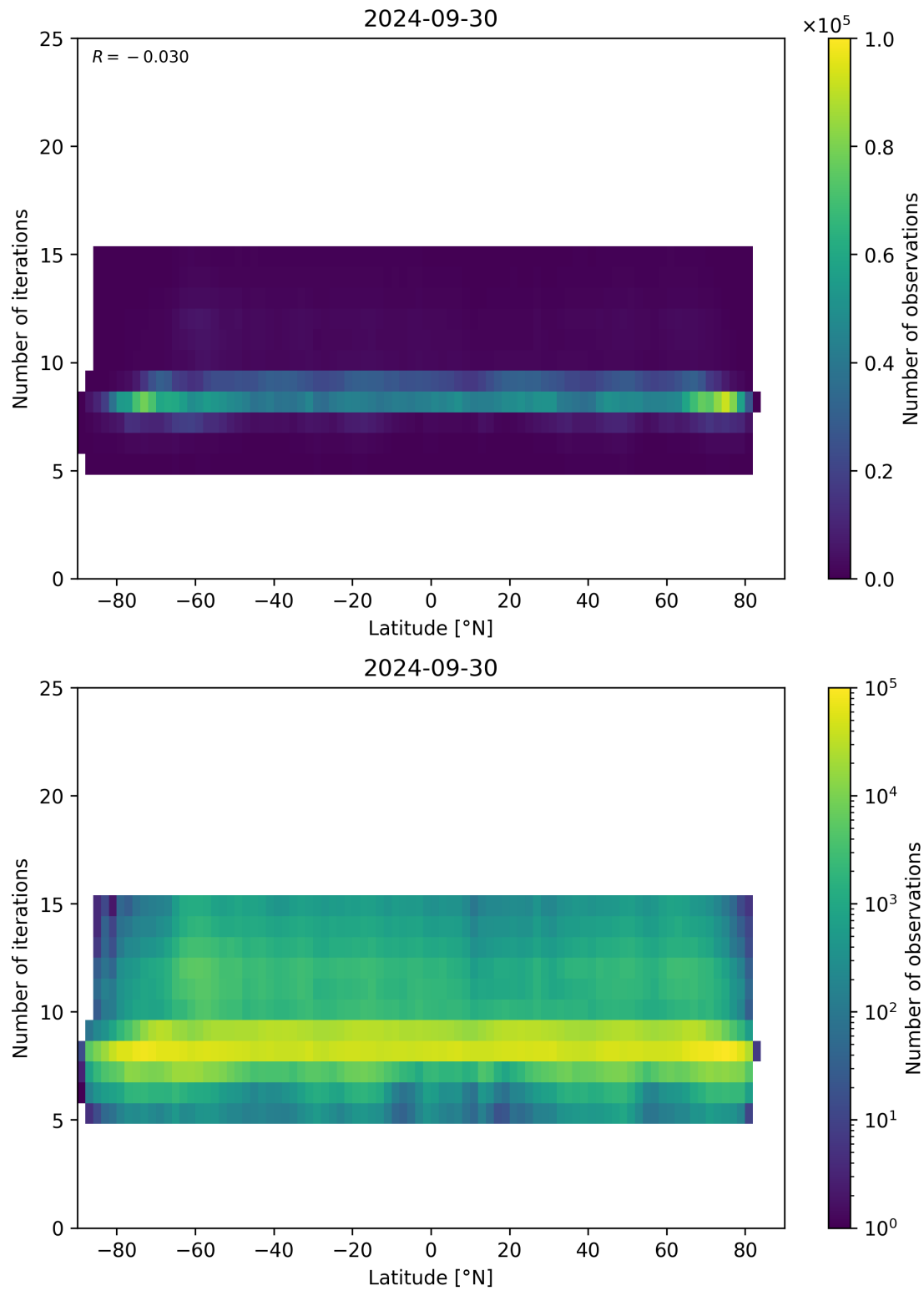
Figure 56: Scatter density plot of “Latitude” against “Number of iterations” for 2024-09-29 to 2024-10-01.
