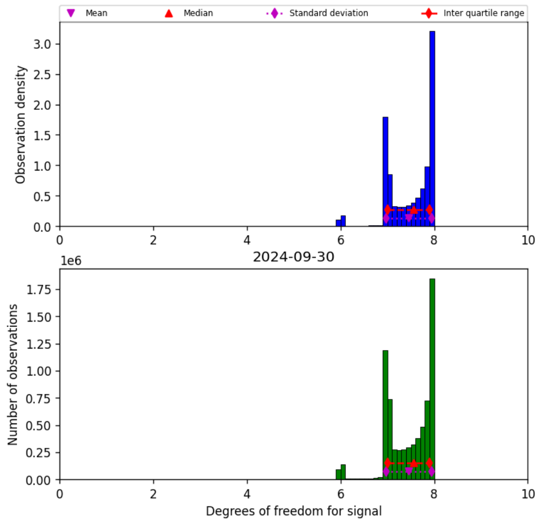
Figure 23: Histogram of “Degrees of freedom for signal” for 2024-09-29 to 2024-10-01
