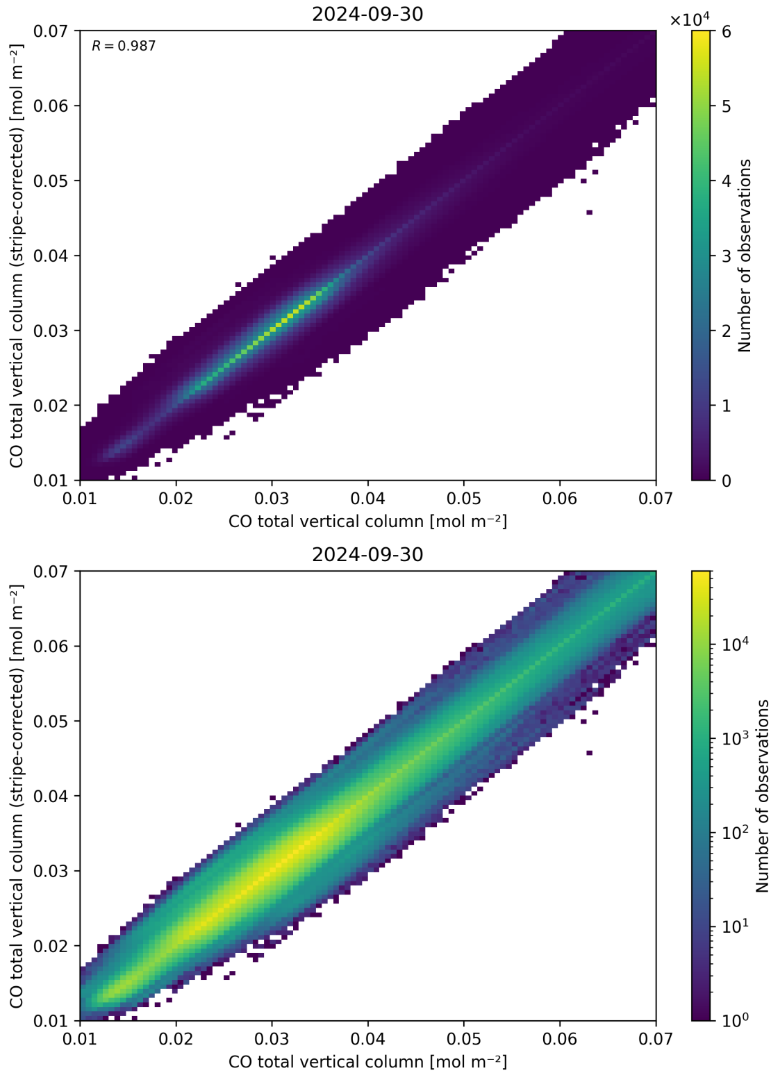
Figure 33: Scatter density plot of “CO total vertical column” against “CO total vertical column (stripe-corrected)” for 2024-09-29 to 2024-10-01.
