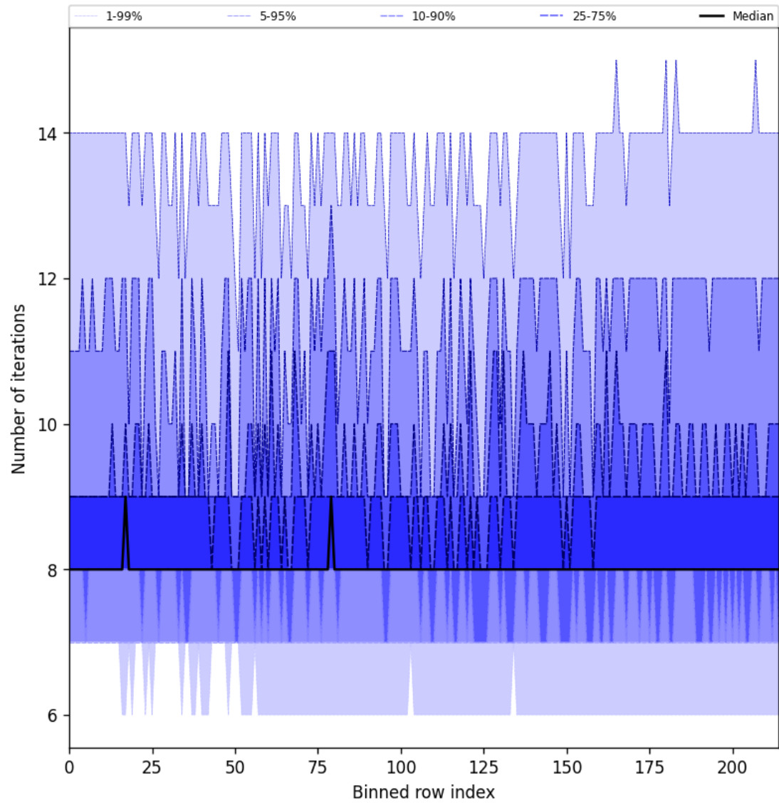
Figure 32: Along track statistics of “Number of iterations” for 2024-09-29 to 2024-10-01
