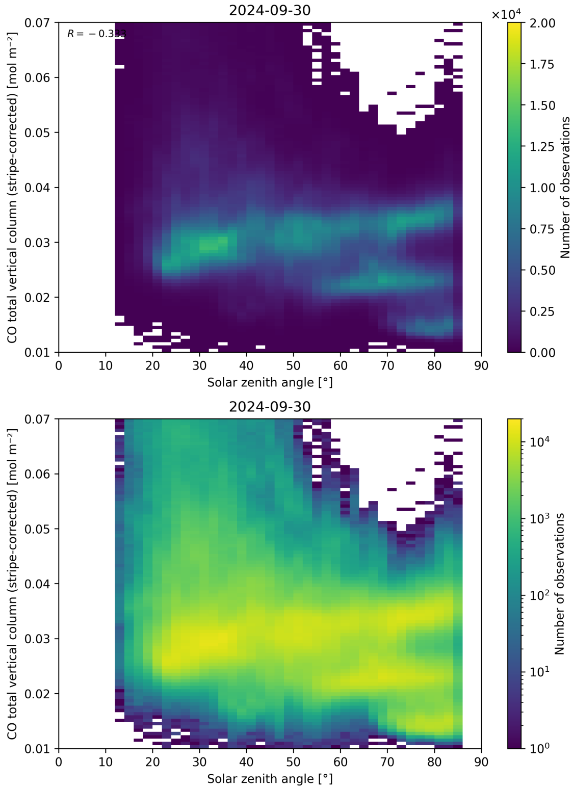
Figure 62: Scatter density plot of “Solar zenith angle” against “CO total vertical column (stripe-corrected)” for 2024-09-29 to 2024-10-01.
