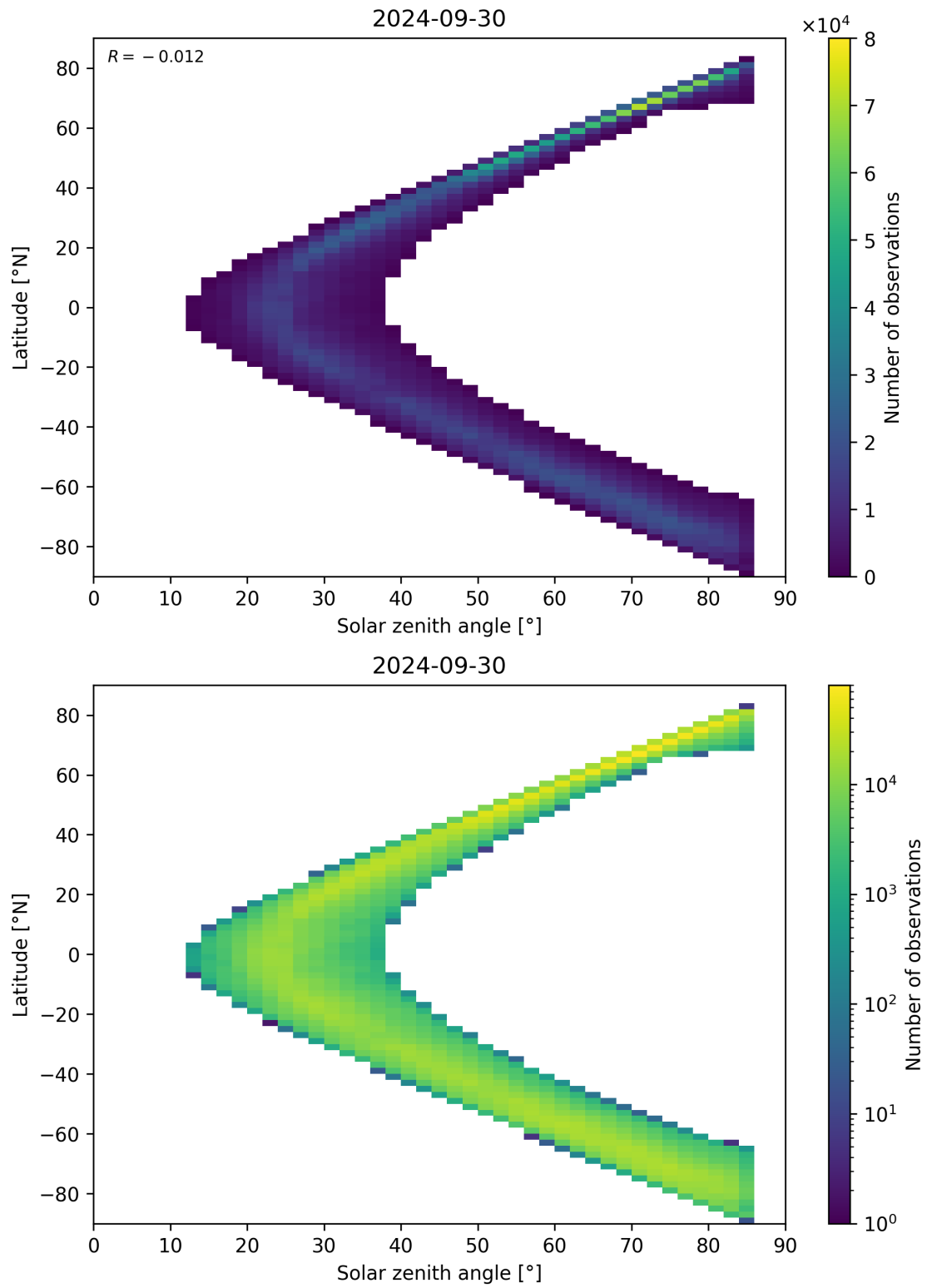
Figure 66: Scatter density plot of “Solar zenith angle” against “Latitude” for 2024-09-29 to 2024-10-01.
