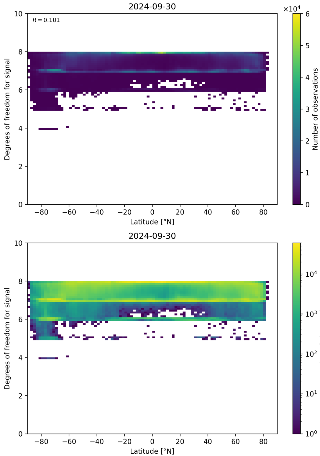
Figure 55: Scatter density plot of “Latitude” against “Degrees of freedom for signal” for 2024-09-29 to 2024-10-01.
