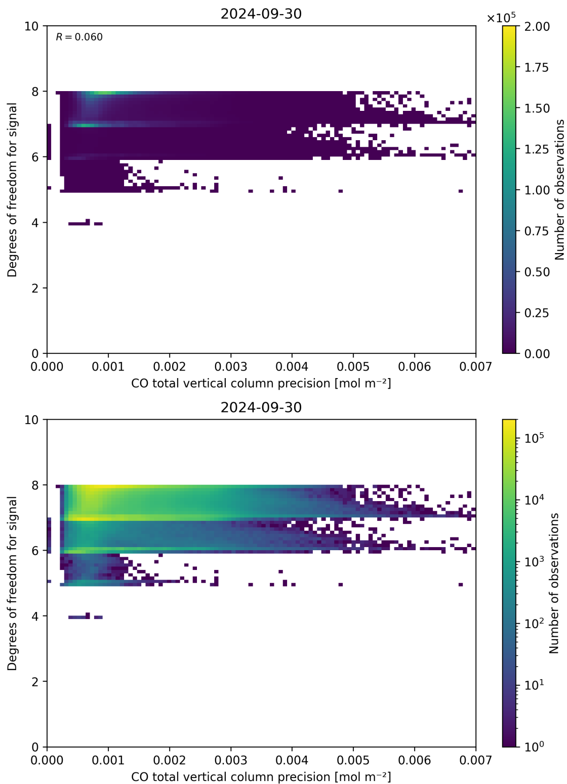
Figure 45: Scatter density plot of “CO total vertical column precision” against “Degrees of freedom for signal” for 2024-09-29 to 2024-10-01.
