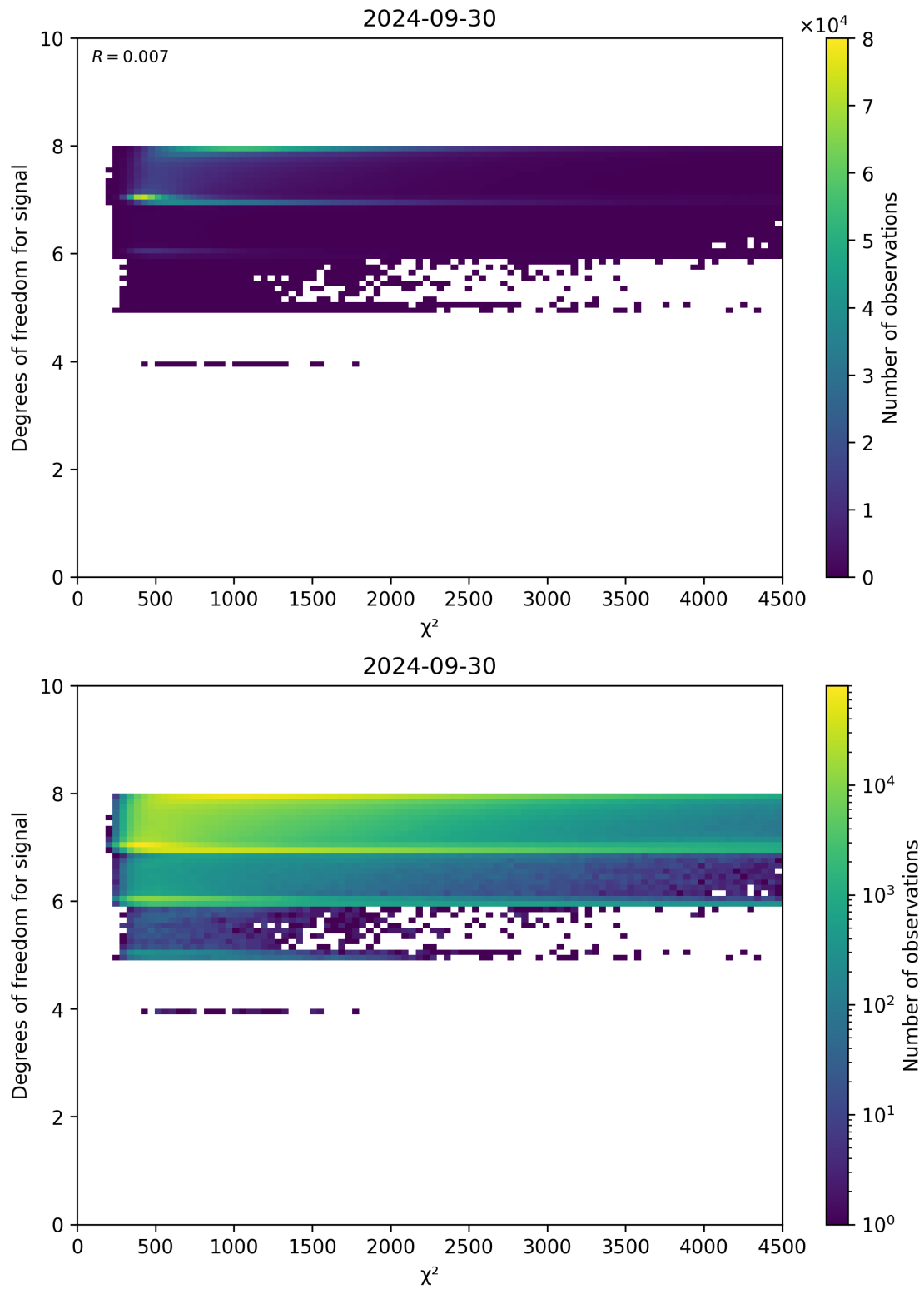
Figure 48: Scatter density plot of " \chi^2 " against "Degrees of freedom for signal" for 2024-09-29 to 2024-10-01.
