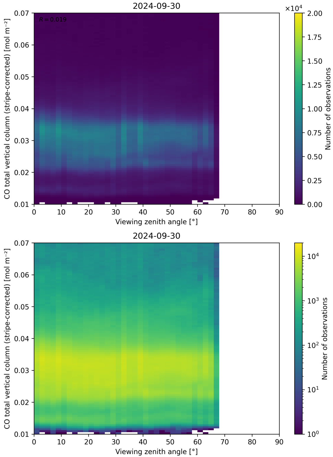
Figure 70: Scatter density plot of “Viewing zenith angle” against “CO total vertical column (stripe-corrected)” for 2024-09-29 to 2024-10-01.
