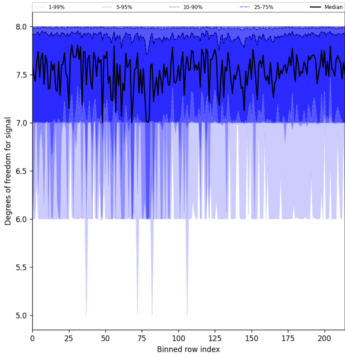
Figure 31: Along track statistics of “Degrees of freedom for signal” for 2024-09-29 to 2024-10-01
