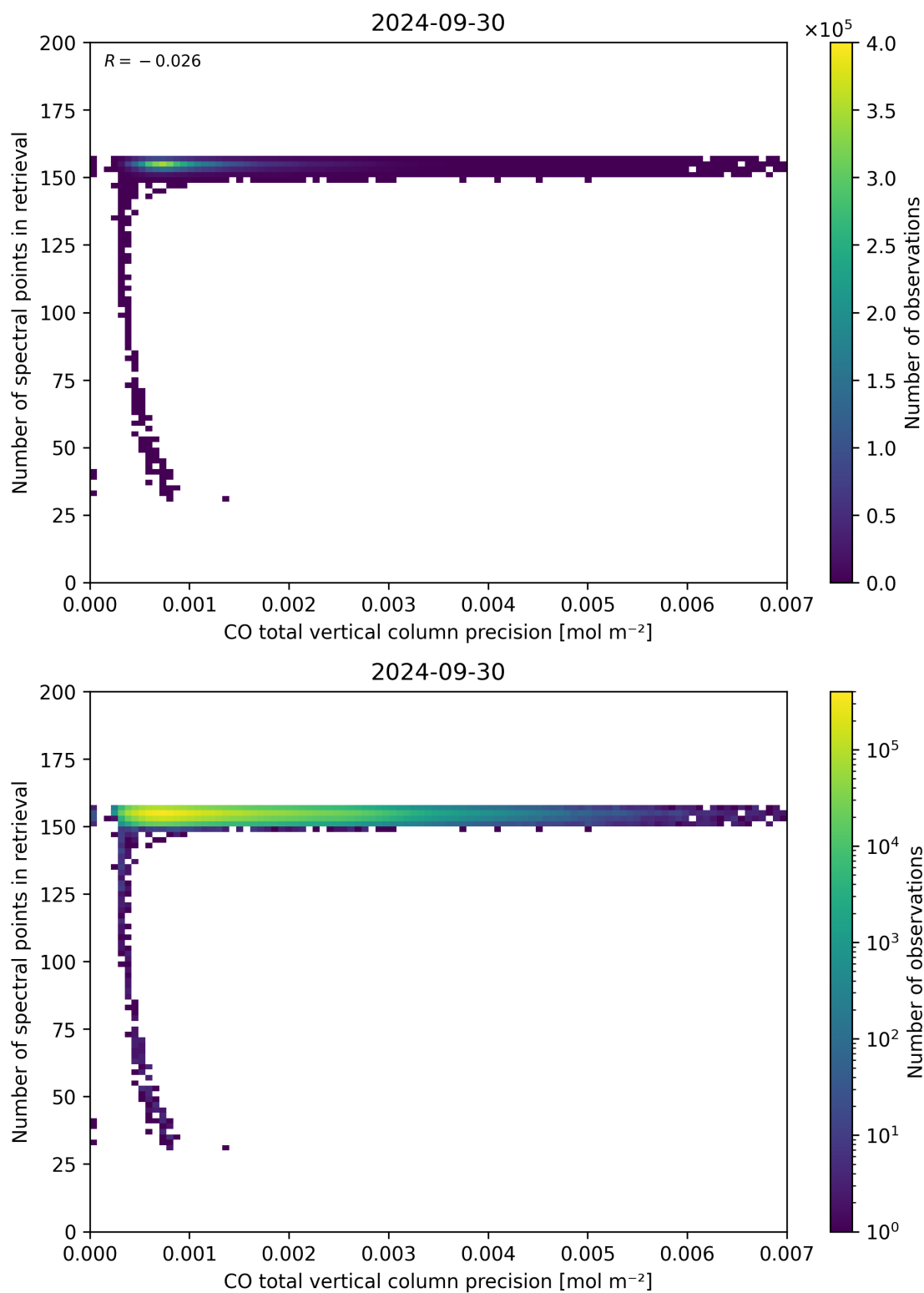
Figure 47: Scatter density plot of “CO total vertical column precision” against “Number of spectral points in retrieval” for 2024-09-29 to 2024-10-01.
