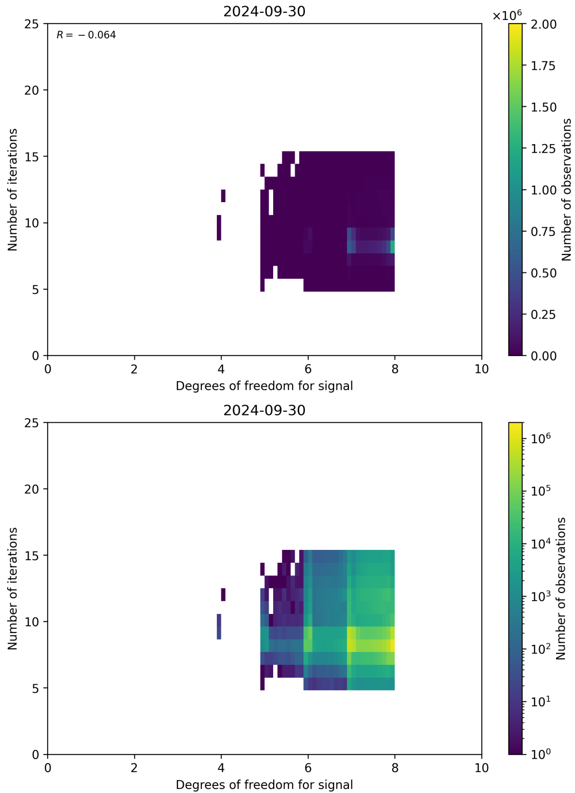
Figure 50: Scatter density plot of “Degrees of freedom for signal” against “Number of iterations” for 2024-09-29 to 2024-10-01.
