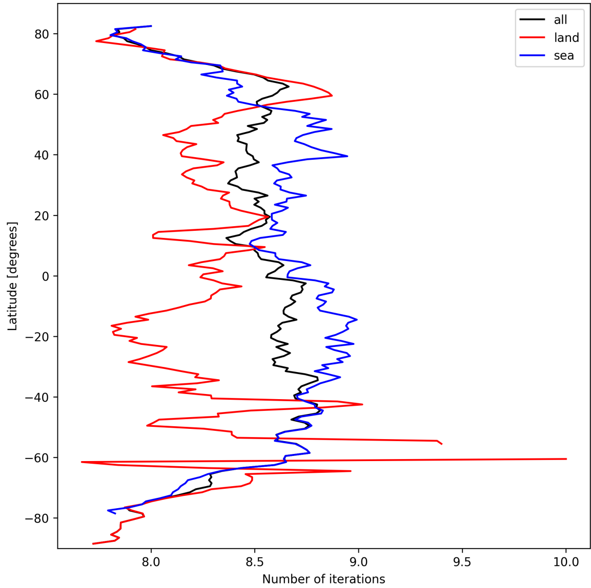
Figure 16: Zonal average of “Number of iterations” for 2024-09-29 to 2024-10-01.
