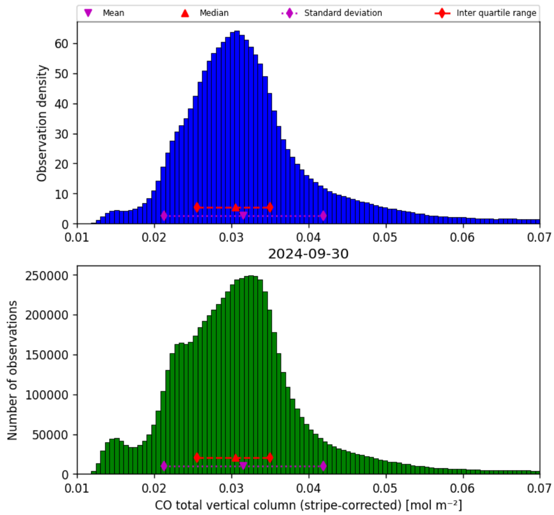
Figure 19: Histogram of “CO total vertical column (stripe-corrected)” for 2024-09-29 to 2024-10-01
