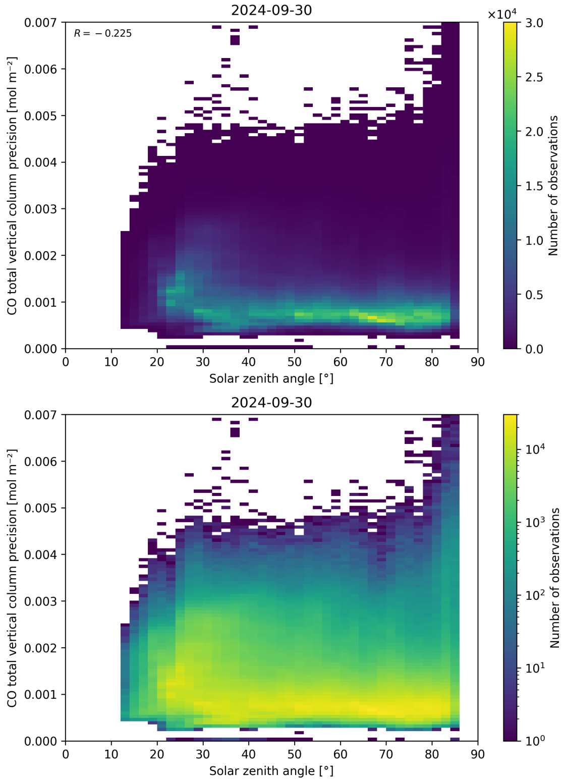
Figure 63: Scatter density plot of “Solar zenith angle” against “CO total vertical column precision” for 2024-09-29 to 2024-10-01.
