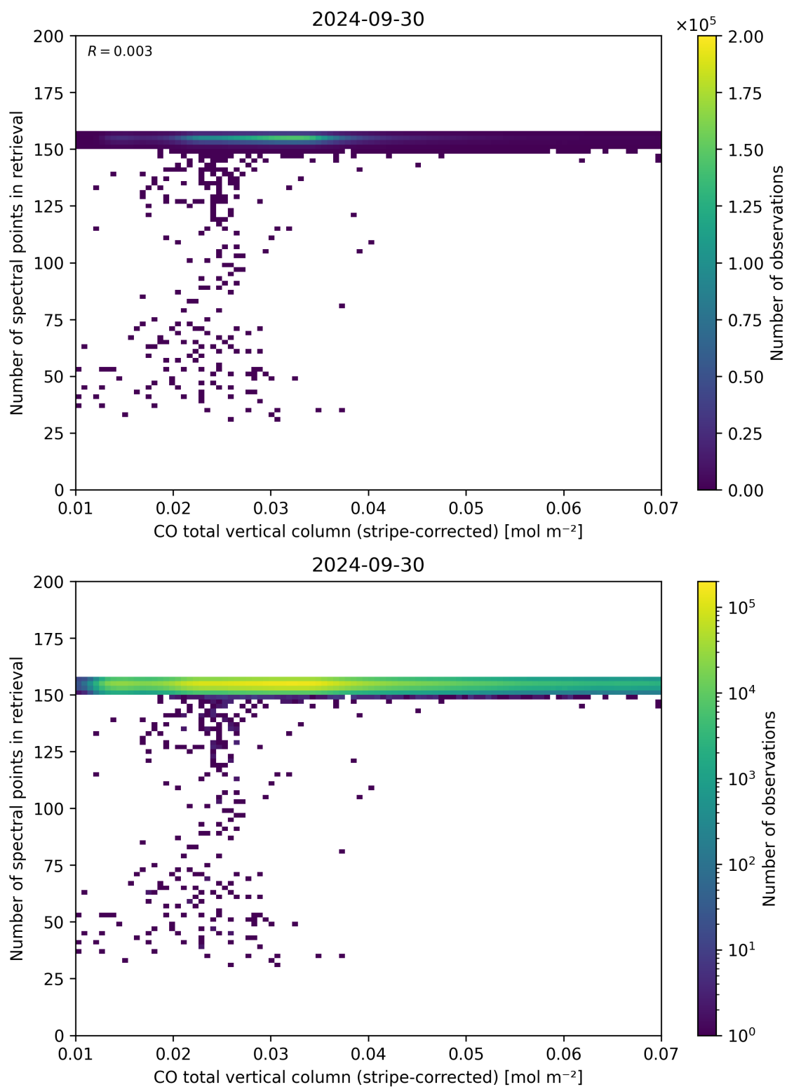
Figure 40: Scatter density plot of “CO total vertical column (stripe-corrected)” against “Number of spectral points in retrieval” for 2024-09-29 to 2024-10-01.
