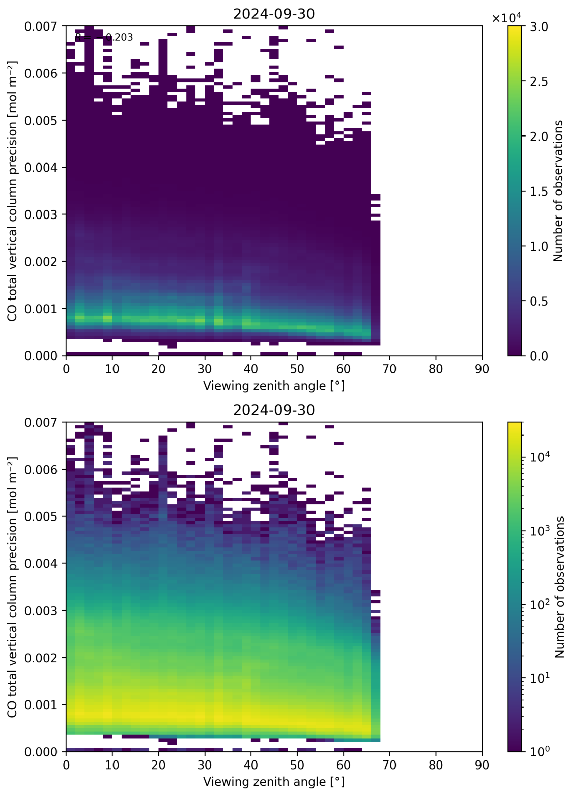
Figure 71: Scatter density plot of “Viewing zenith angle” against “CO total vertical column precision” for 2024-09-29 to 2024-10-01.
