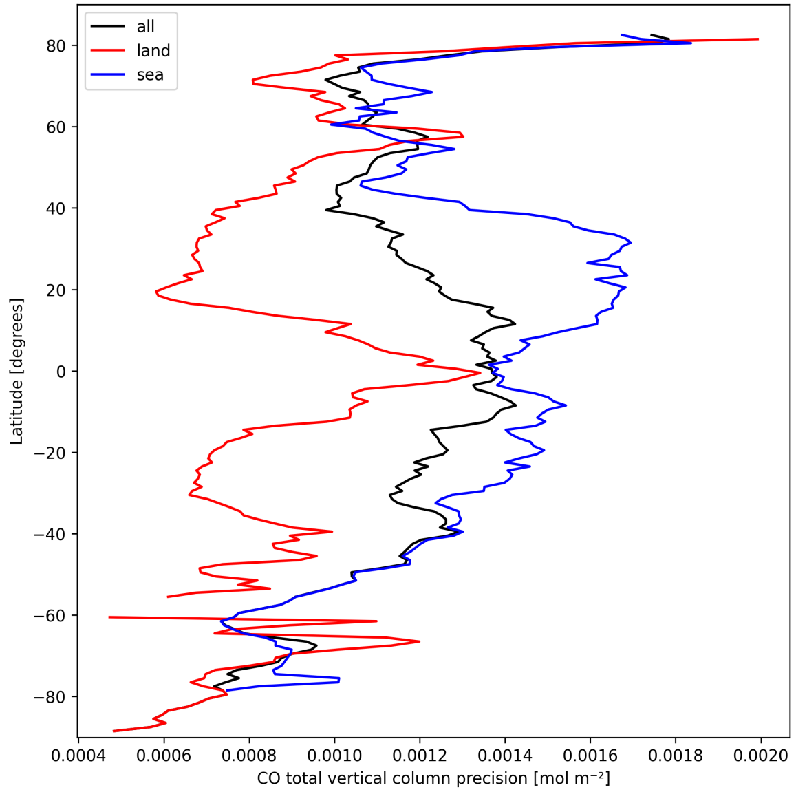
Figure 12: Zonal average of “CO total vertical column precision” for 2024-09-29 to 2024-10-01.
