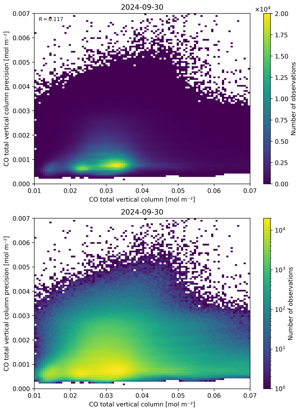
Figure 34: Scatter density plot of “CO total vertical column” against “CO total vertical column precision” for 2024-09-29 to 2024-10-01.
