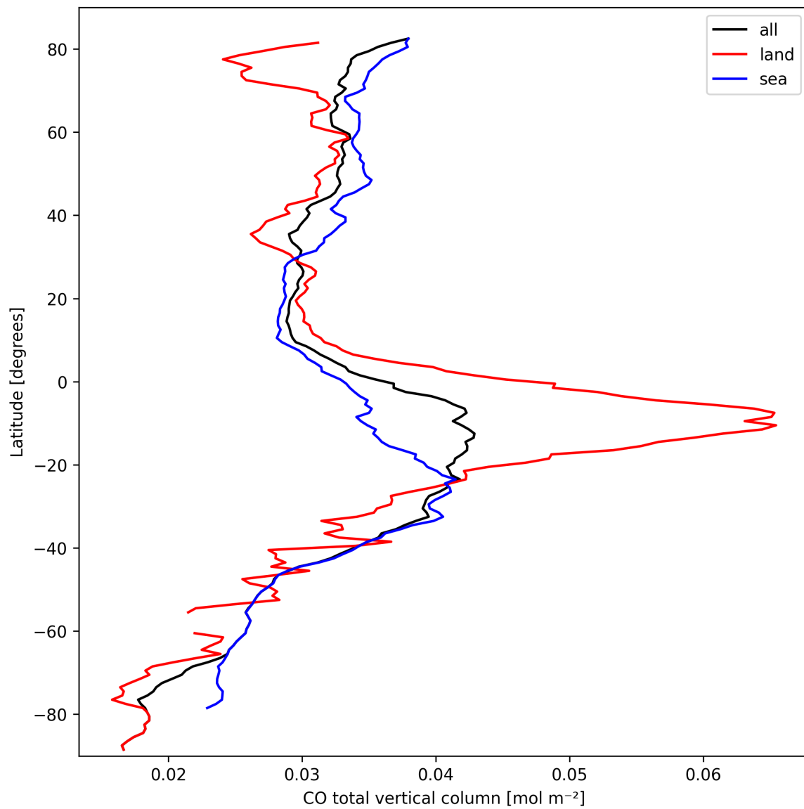
Figure 10: Zonal average of “CO total vertical column” for 2024-09-29 to 2024-10-01.
