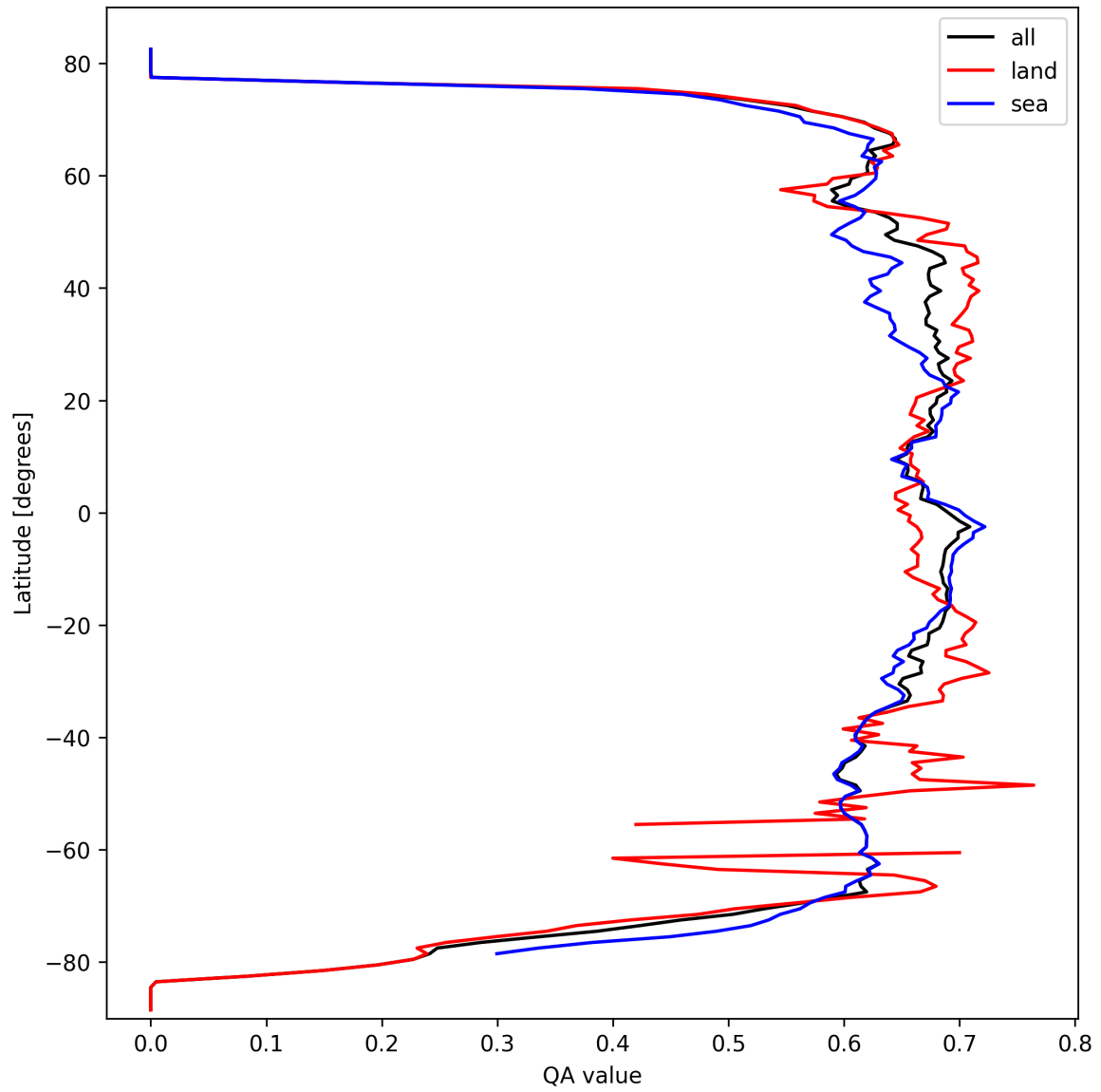
Figure 9: Zonal average of “QA value” for 2024-09-29 to 2024-10-01.
