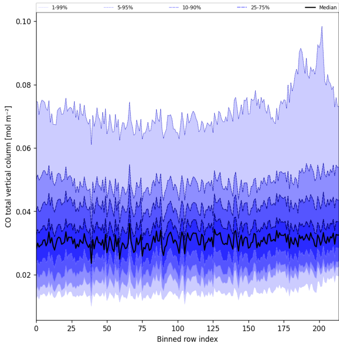
Figure 26: Along track statistics of “CO total vertical column” for 2024-09-29 to 2024-10-01
