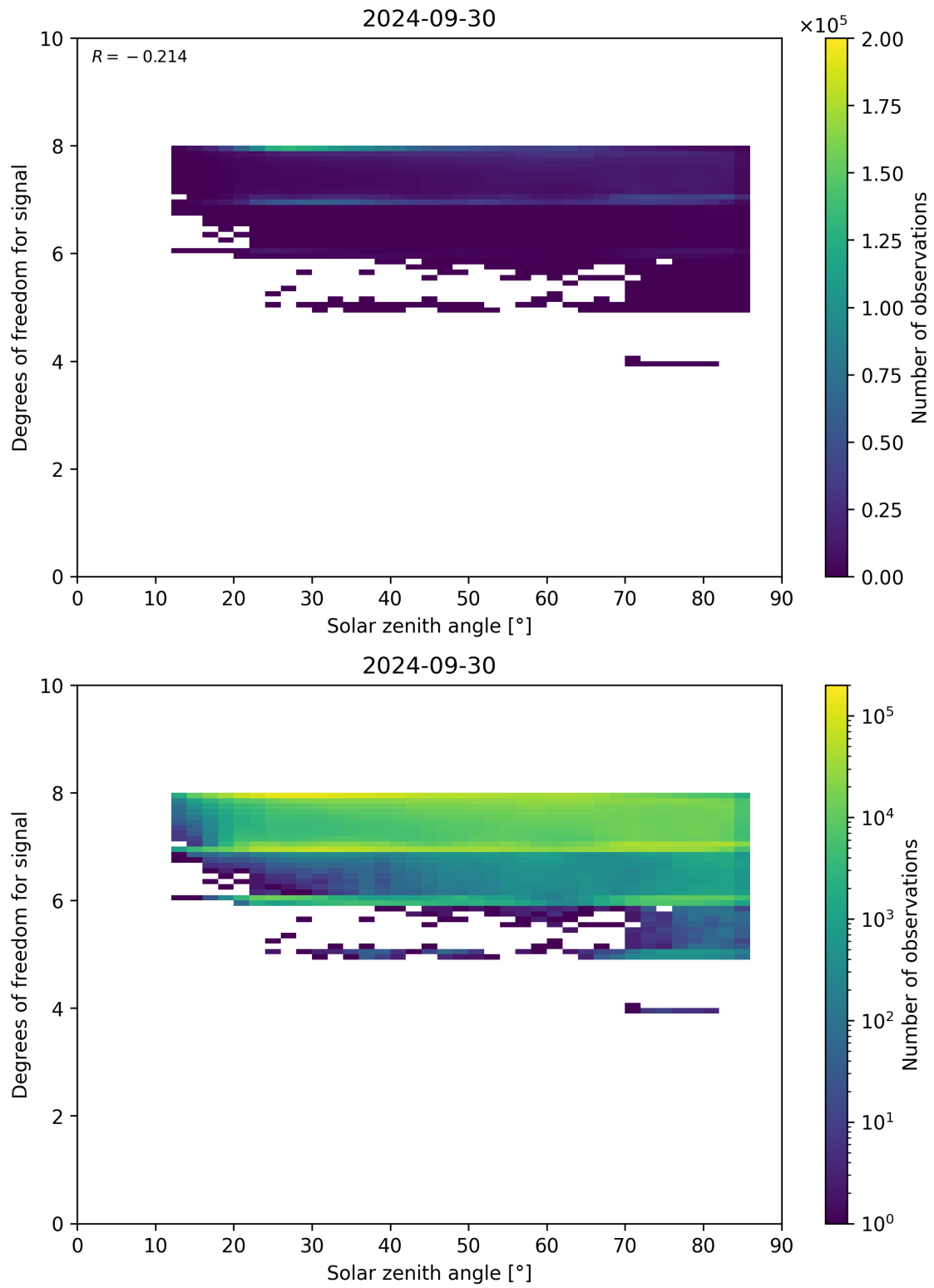
Figure 65: Scatter density plot of “Solar zenith angle” against “Degrees of freedom for signal” for 2024-09-29 to 2024-10-01.
