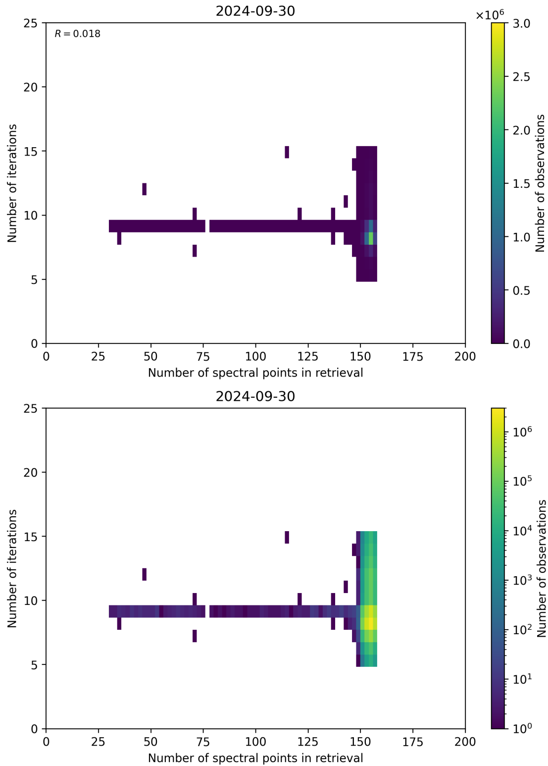
Figure 60: Scatter density plot of “Number of spectral points in retrieval” against “Number of iterations” for 2024-09-29 to 2024-10-01.
