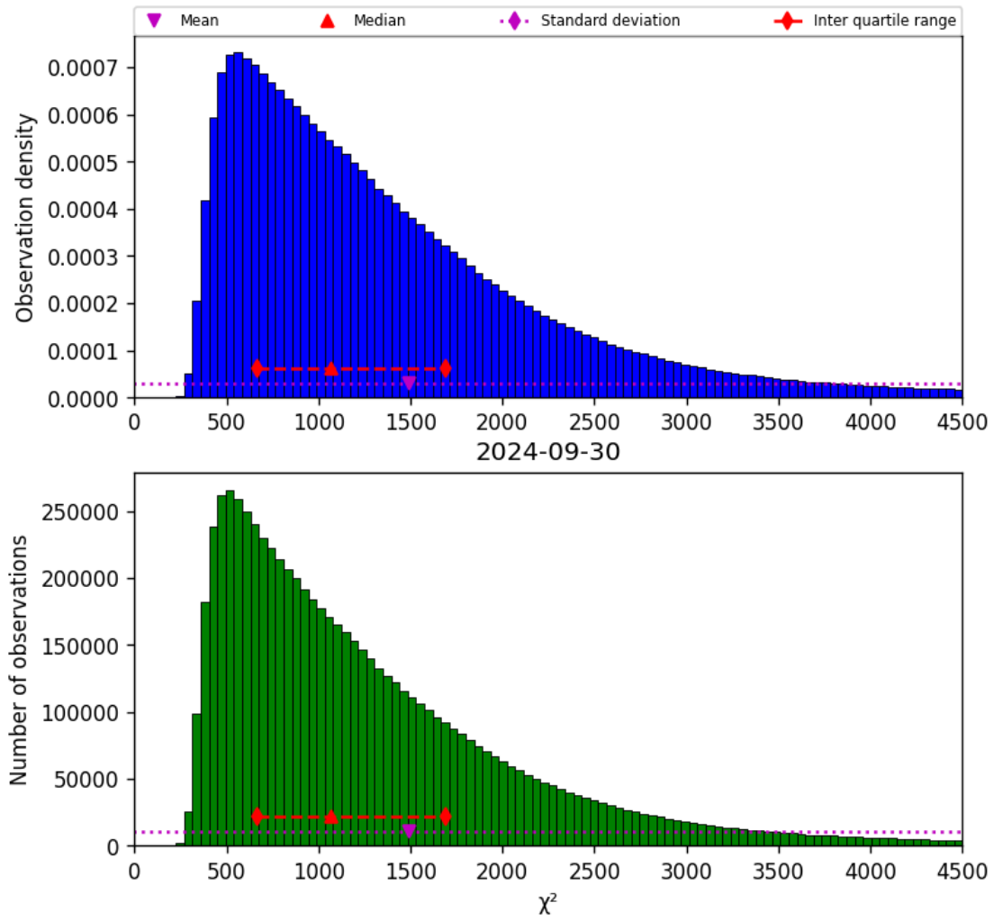
Figure 22: Histogram of “ \chi^2 ” for 2024-09-29 to 2024-10-01
