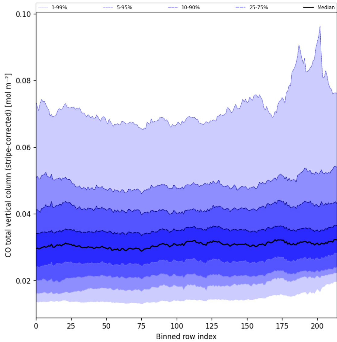
Figure 27: Along track statistics of “CO total vertical column (stripe-corrected)” for 2024-09-29 to 2024-10-01
