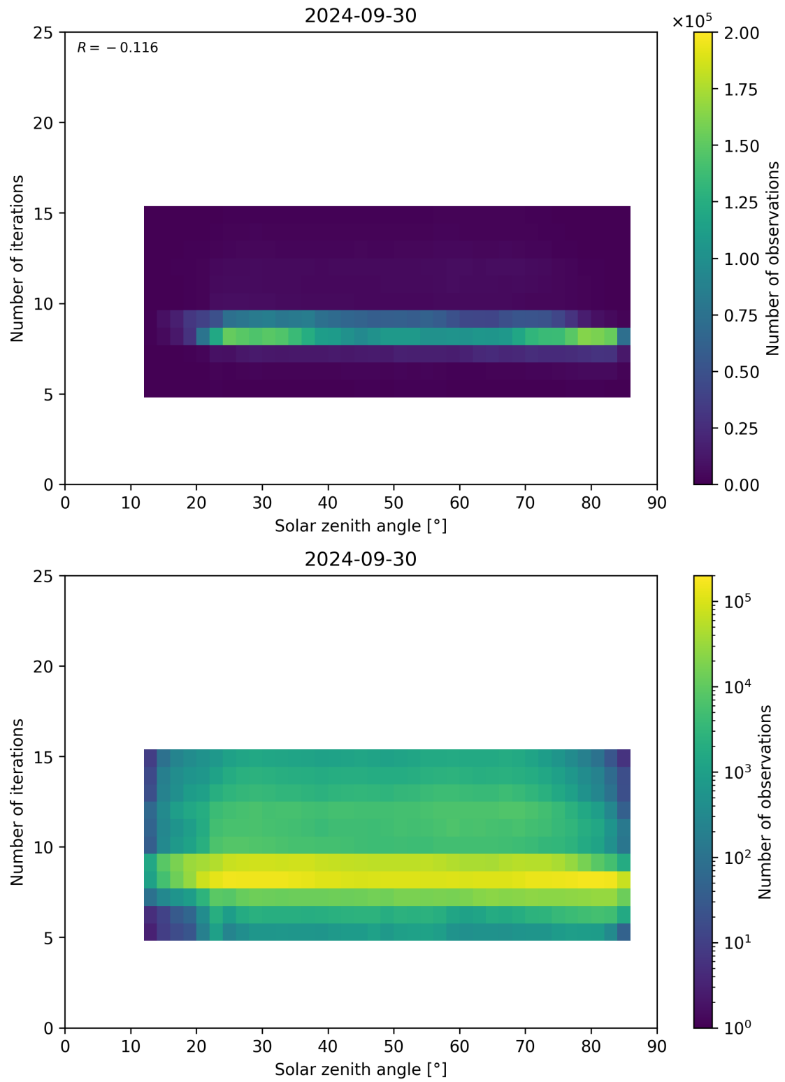
Figure 67: Scatter density plot of “Solar zenith angle” against “Number of iterations” for 2024-09-29 to 2024-10-01.
