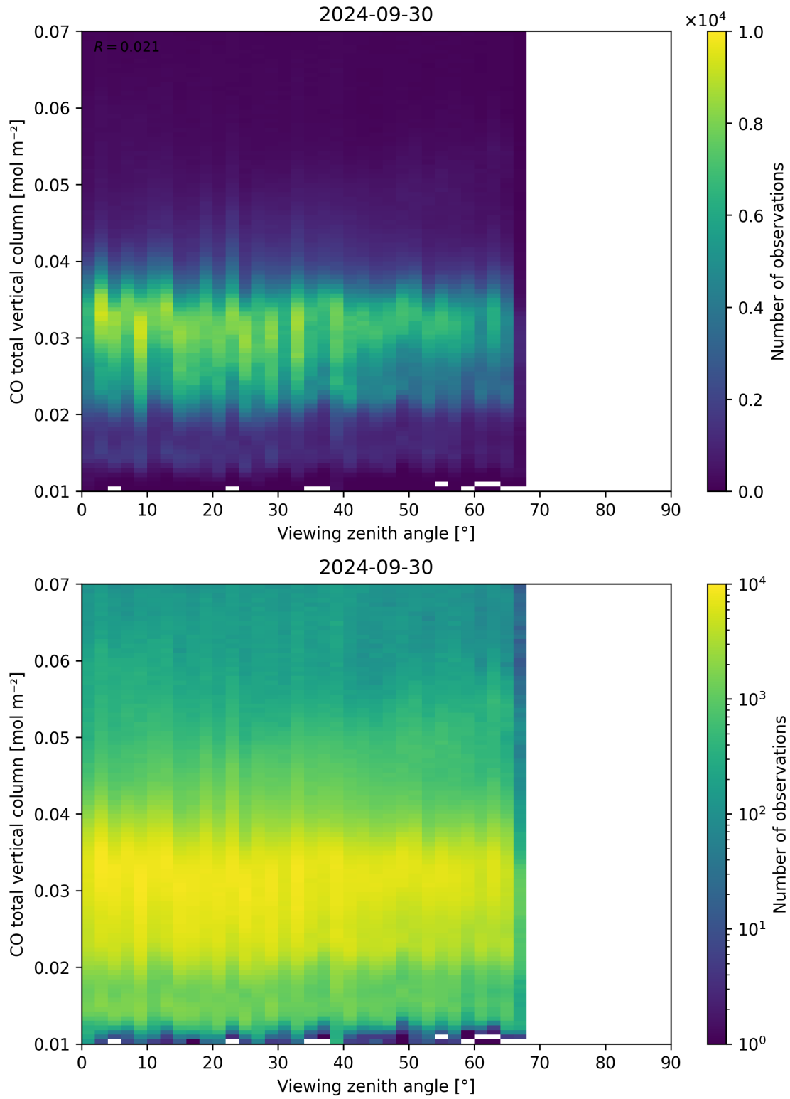
Figure 69: Scatter density plot of “Viewing zenith angle” against “CO total vertical column” for 2024-09-29 to 2024-10-01.
