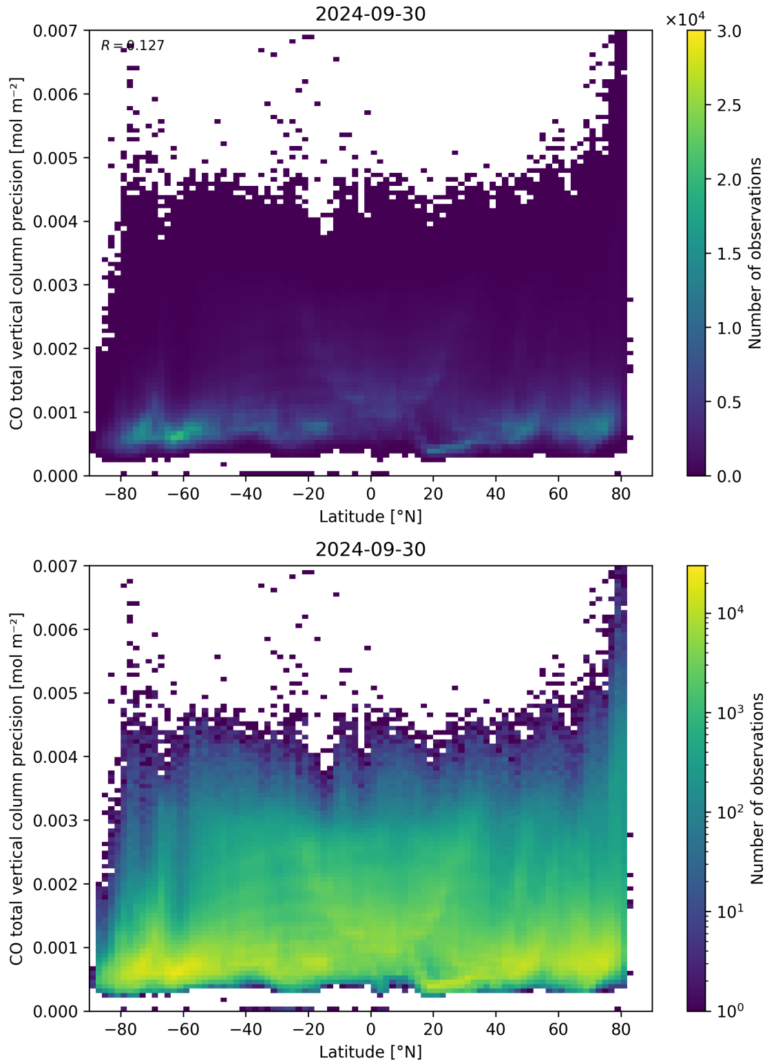
Figure 53: Scatter density plot of “Latitude” against “CO total vertical column precision” for 2024-09-29 to 2024-10-01.
