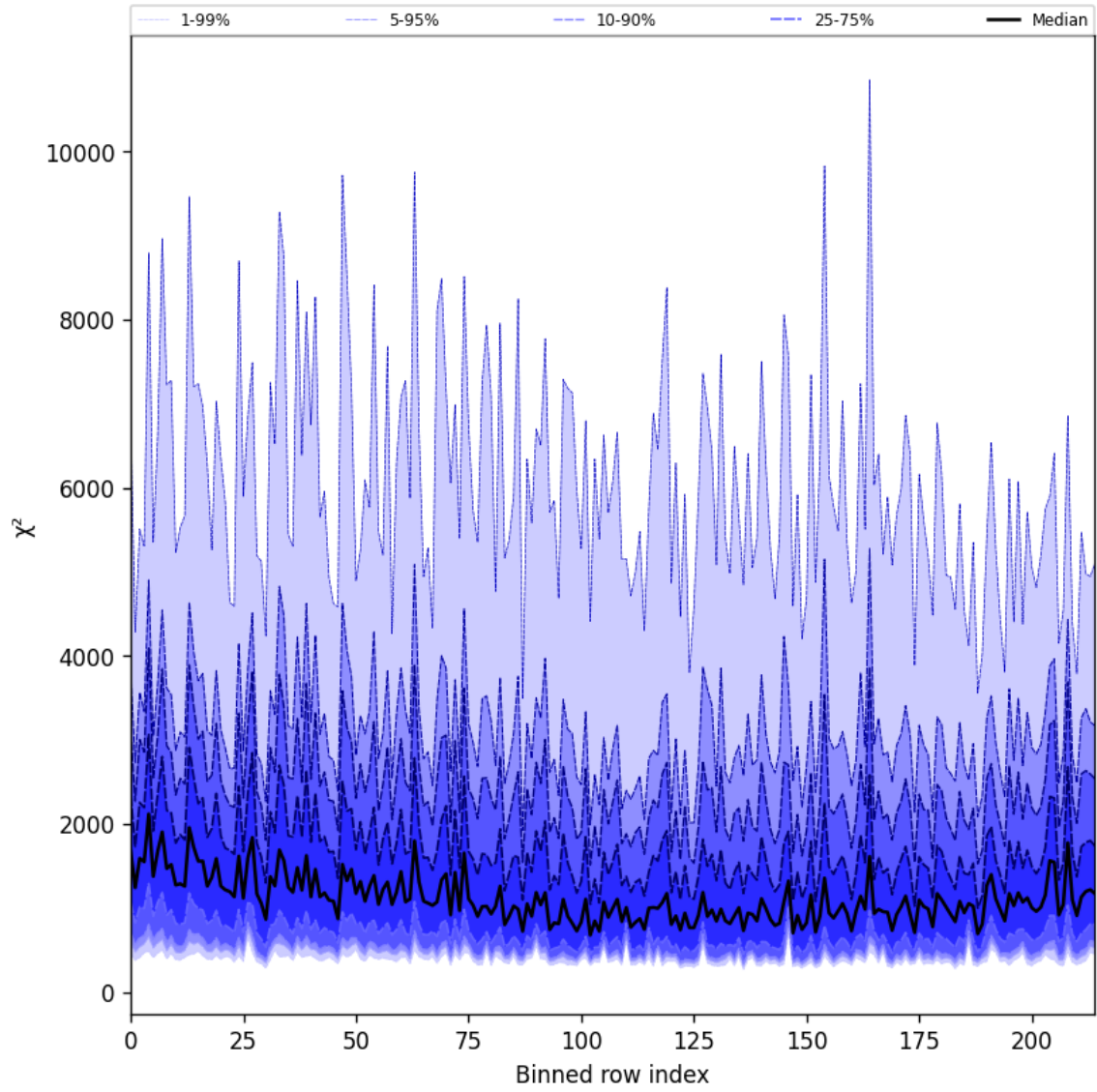
Figure 30: Along track statistics of “ \chi^2 ” for 2024-09-29 to 2024-10-01
