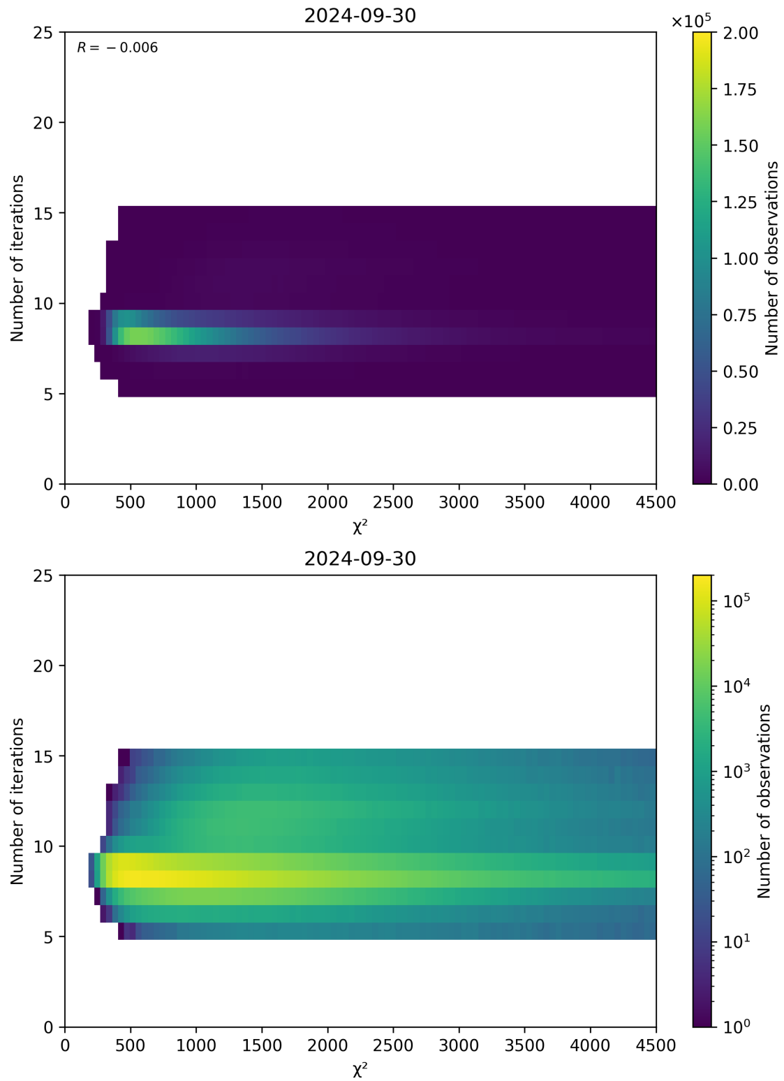
Figure 49: Scatter density plot of “ \chi^2 ” against “Number of iterations” for 2024-09-29 to 2024-10-01.
