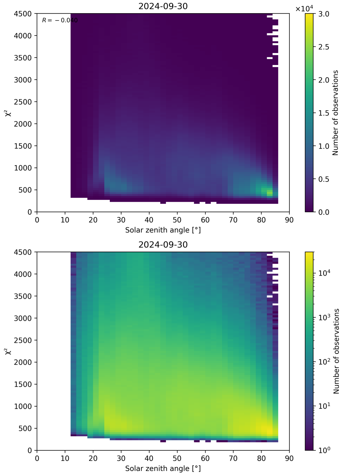
Figure 64: Scatter density plot of “Solar zenith angle” against “ \chi^2 ” for 2024-09-29 to 2024-10-01.
