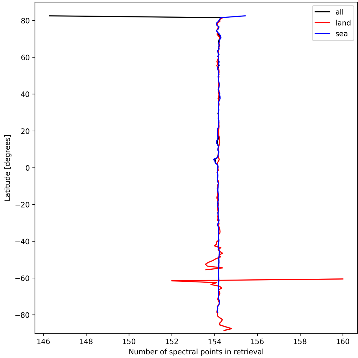
Figure 13: Zonal average of “Number of spectral points in retrieval” for 2024-09-29 to 2024-10-01.
