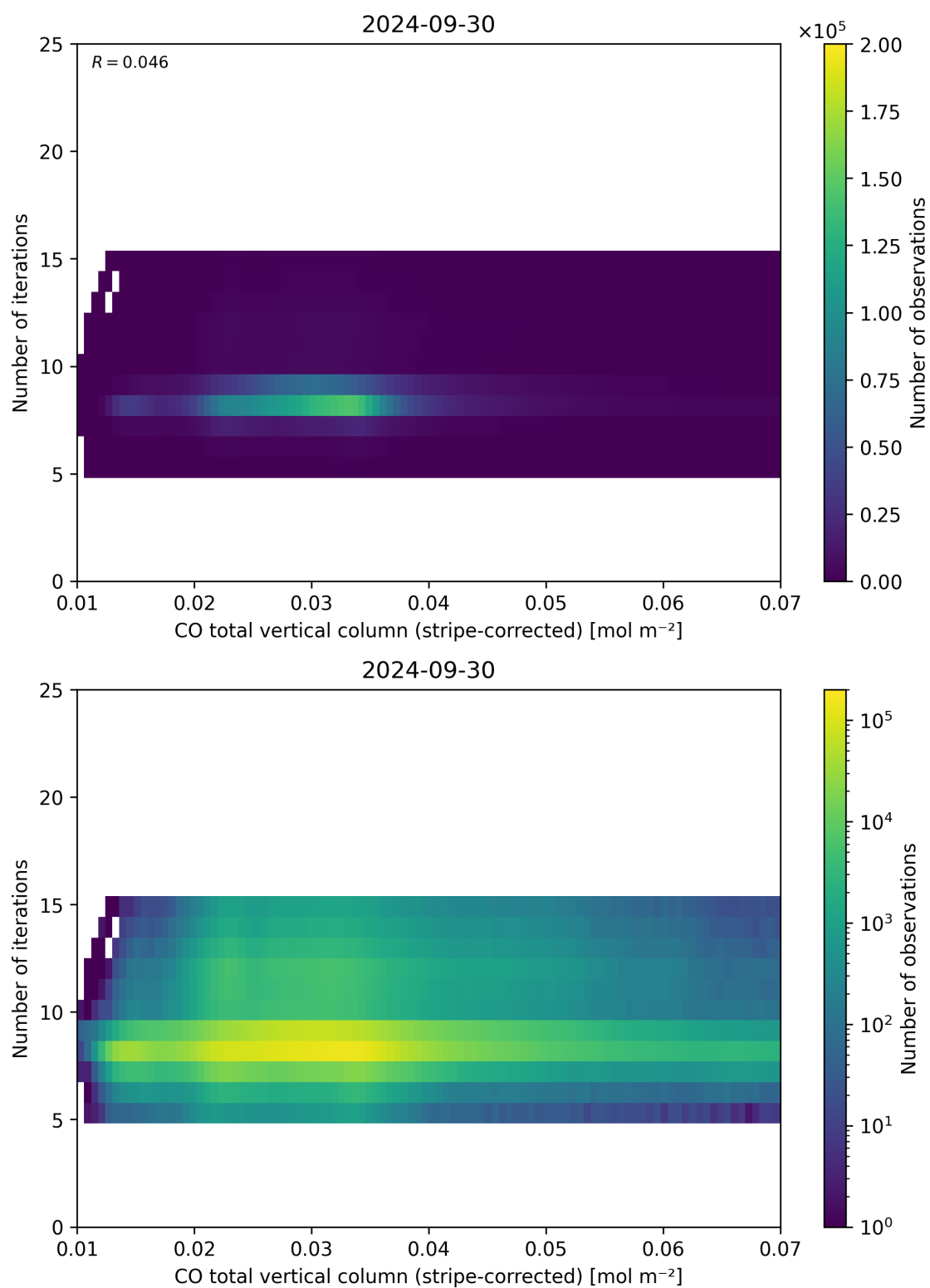
Figure 39: Scatter density plot of “CO total vertical column (stripe-corrected)” against “Number of iterations” for 2024-09-29 to 2024-10-01.
