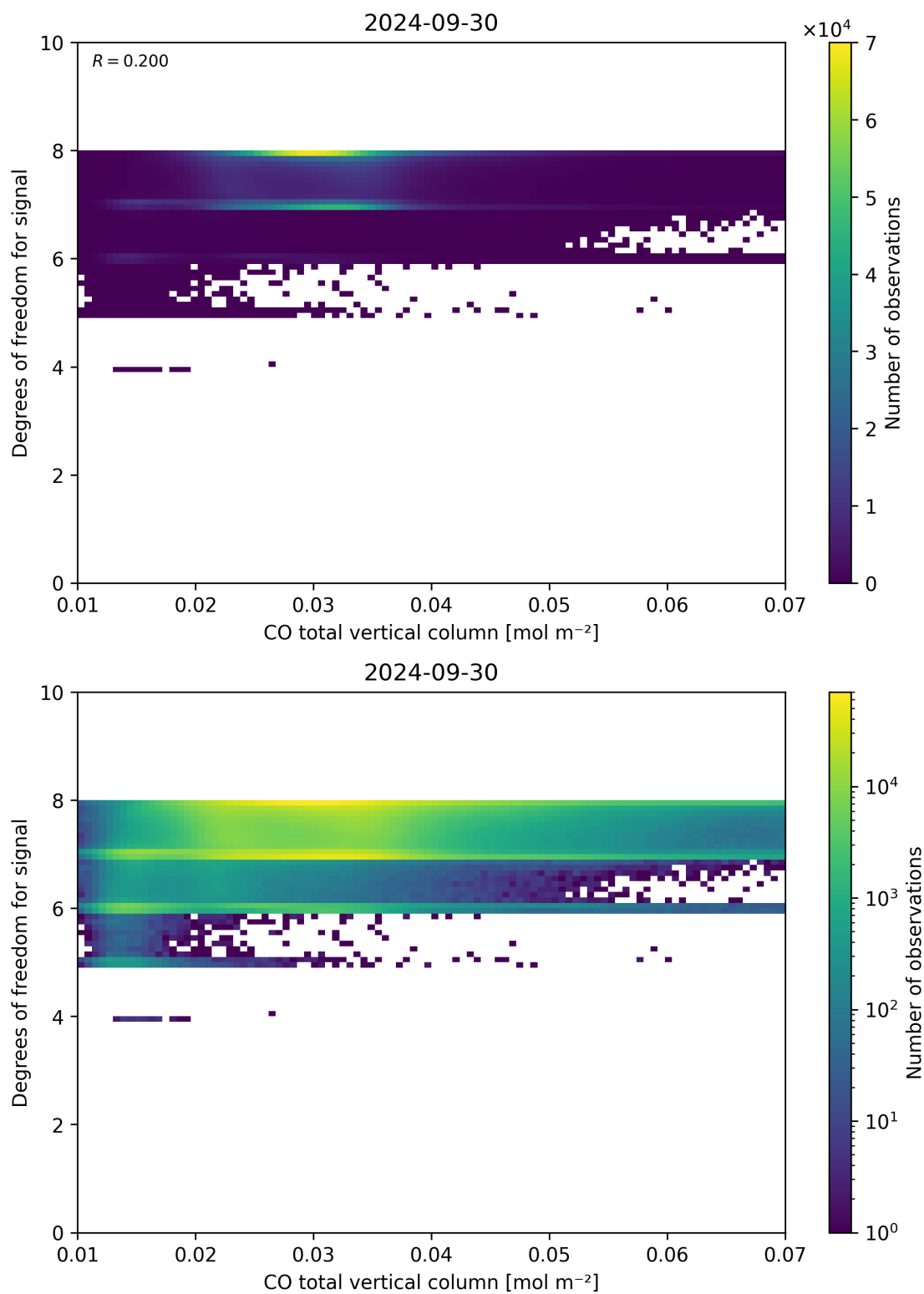
Figure 41: Scatter density plot of “CO total vertical column” against “Degrees of freedom for signal” for 2024-09-29 to 2024-10-01.
