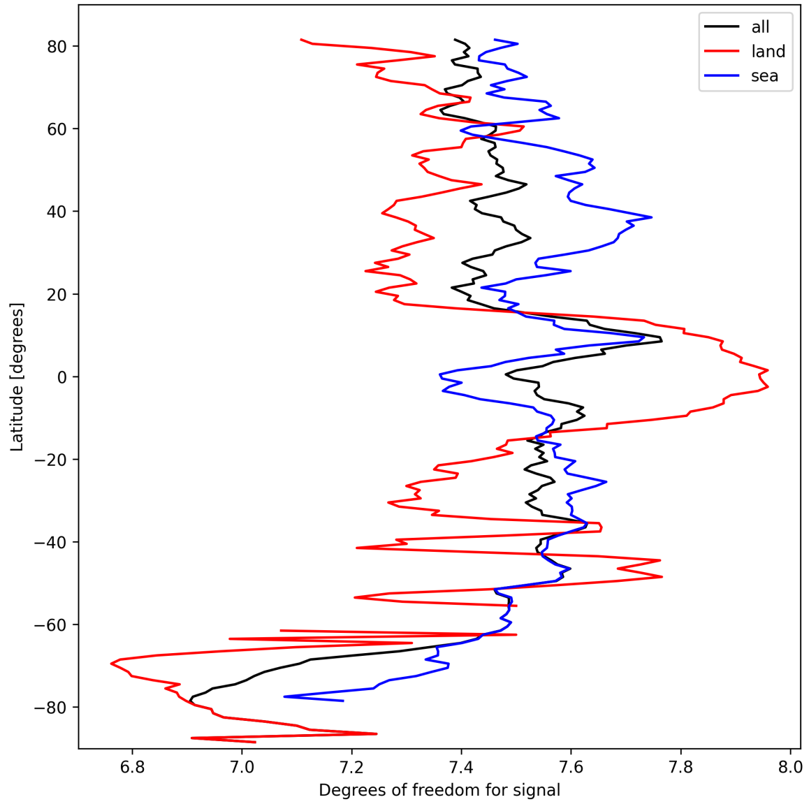
Figure 15: Zonal average of “Degrees of freedom for signal” for 2024-09-30 to 2024-10-02.
