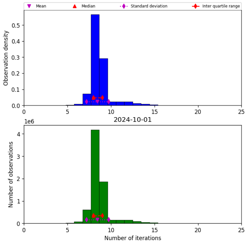
Figure 24: Histogram of “Number of iterations” for 2024-09-30 to 2024-10-02
