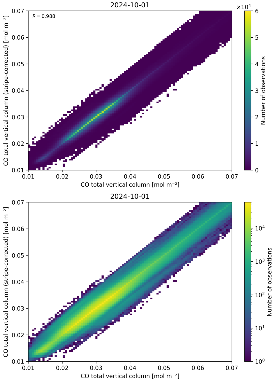
Figure 33: Scatter density plot of “CO total vertical column” against “CO total vertical column (stripe-corrected)” for 2024-09-30 to 2024-10-02.
