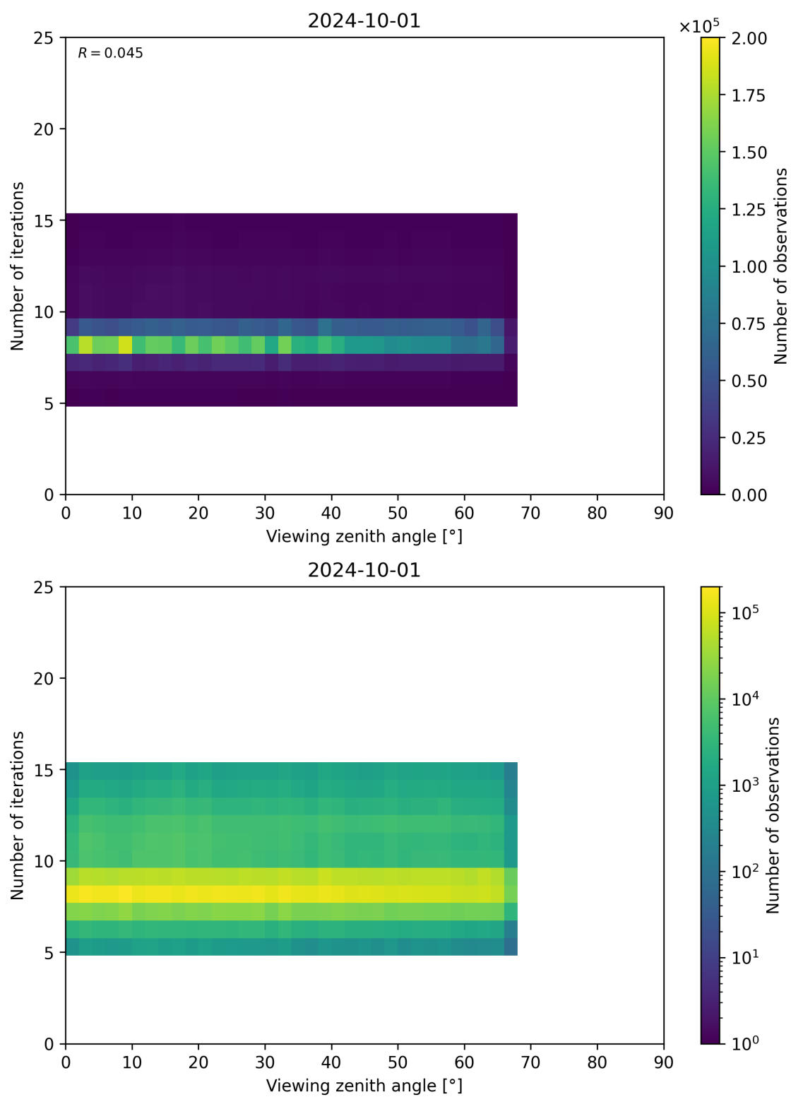
Figure 75: Scatter density plot of “Viewing zenith angle” against “Number of iterations” for 2024-09-30 to 2024-10-02.
