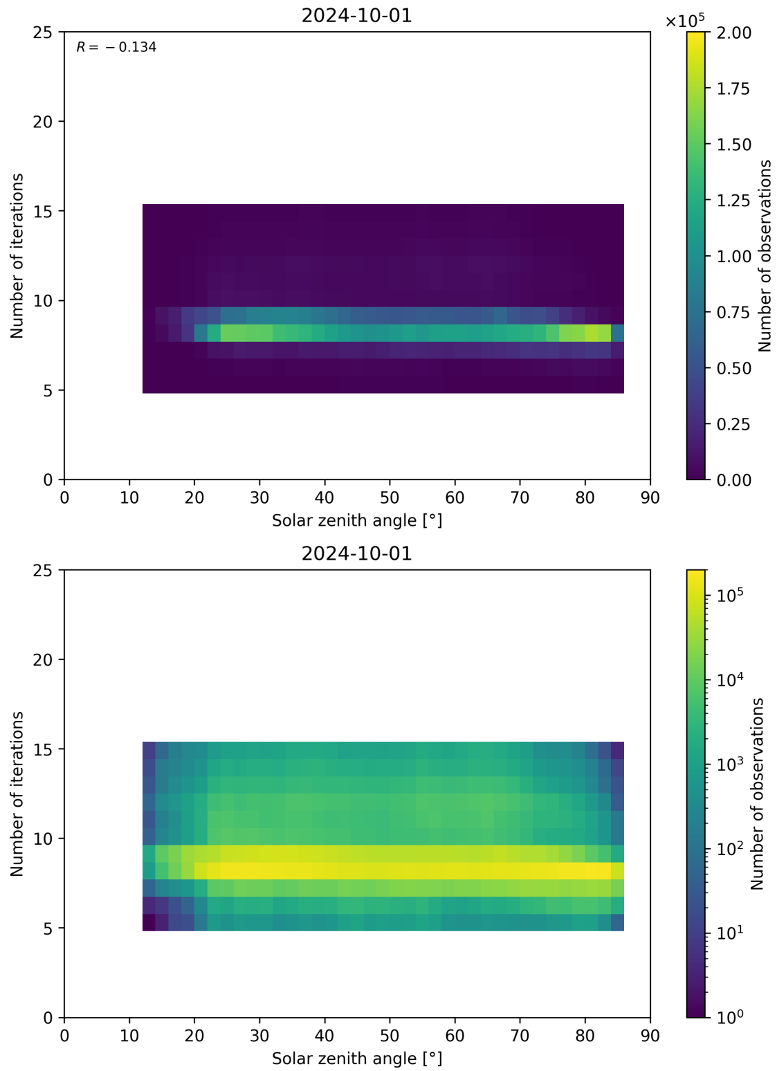
Figure 67: Scatter density plot of “Solar zenith angle” against “Number of iterations” for 2024-09-30 to 2024-10-02.
