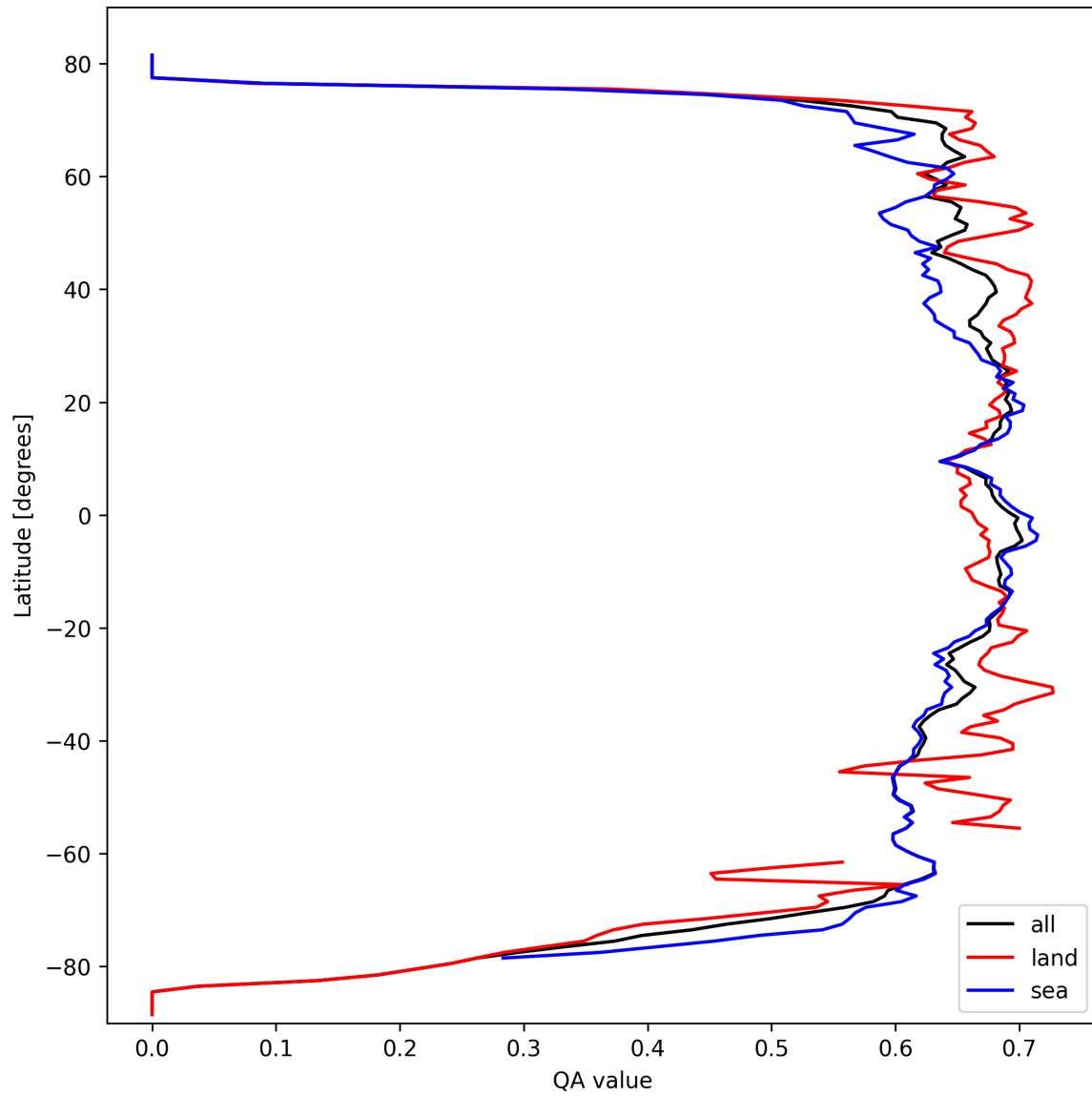
Figure 9: Zonal average of “QA value” for 2024-09-30 to 2024-10-02.
