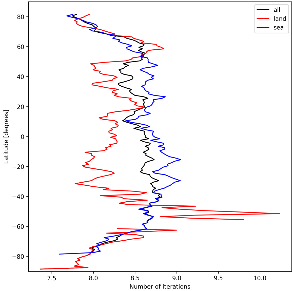
Figure 16: Zonal average of “Number of iterations” for 2024-09-30 to 2024-10-02.
