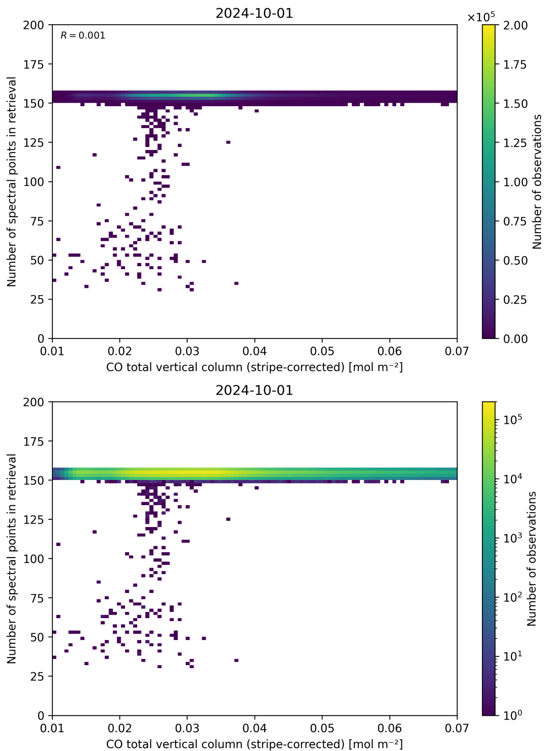
Figure 40: Scatter density plot of “CO total vertical column (stripe-corrected)” against “Number of spectral points in retrieval” for 2024-09-30 to 2024-10-02.
