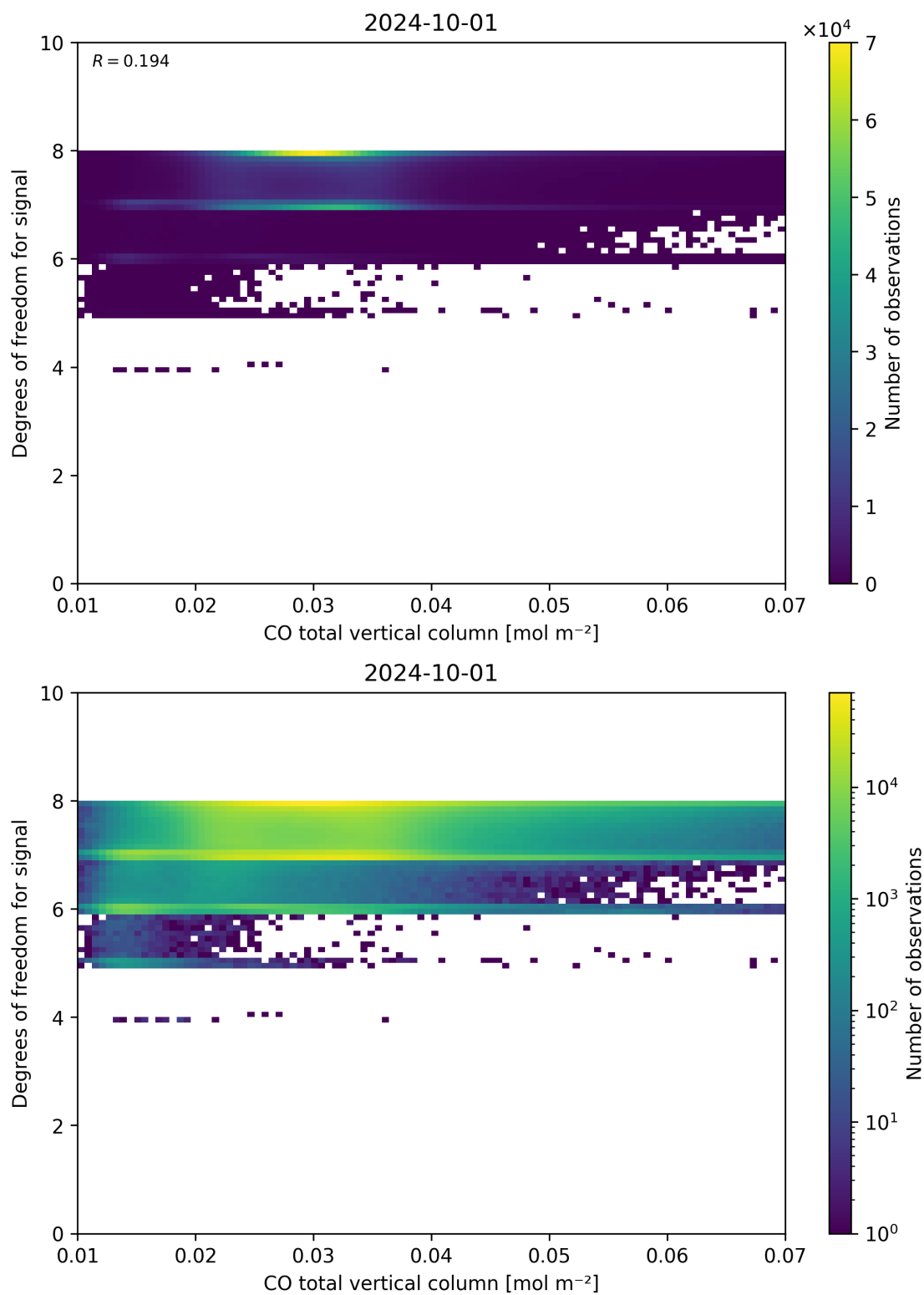
Figure 41: Scatter density plot of “CO total vertical column” against “Degrees of freedom for signal” for 2024-09-30 to 2024-10-02.
