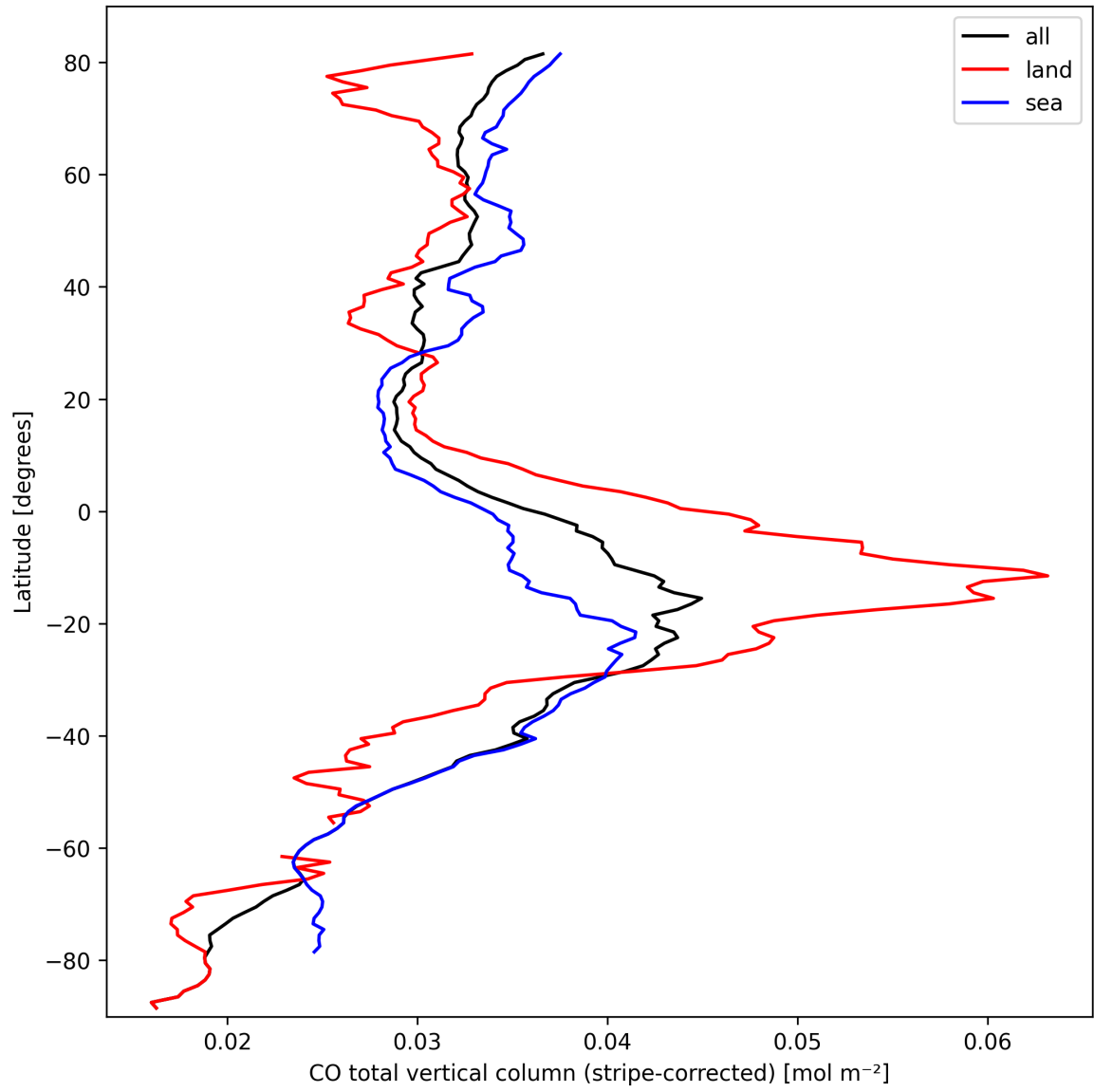
Figure 11: Zonal average of “CO total vertical column (stripe-corrected)” for 2024-09-30 to 2024-10-02.
