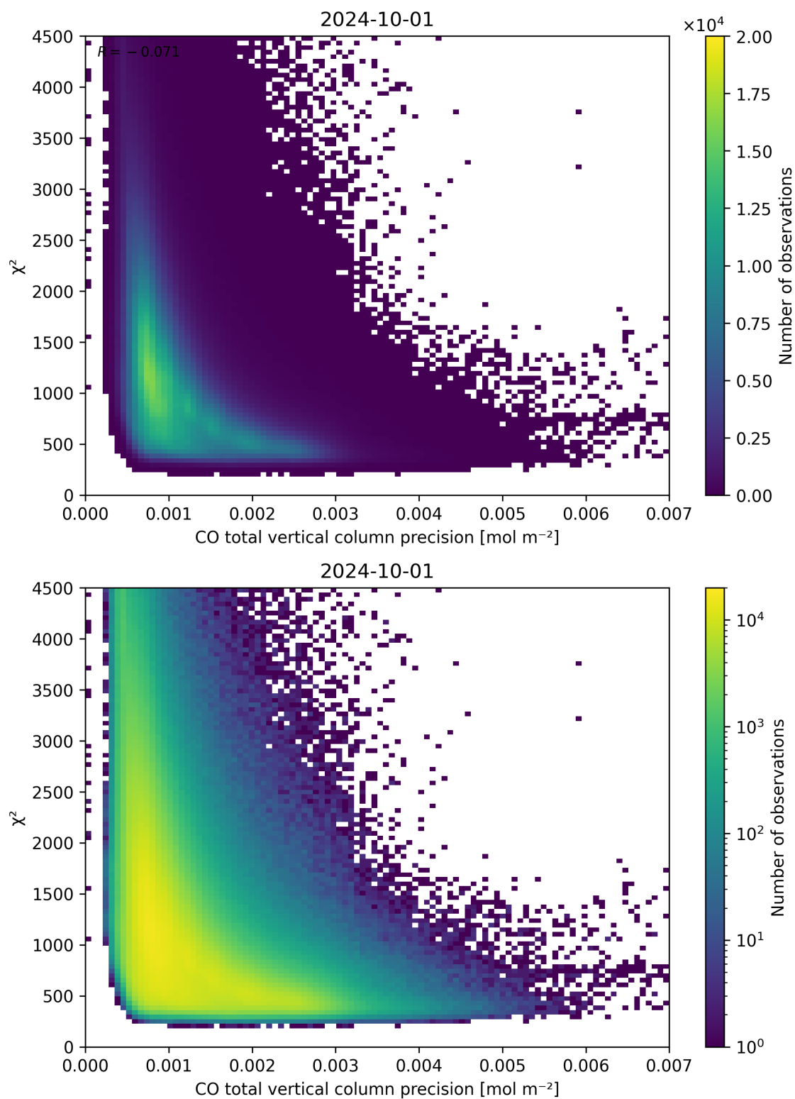
Figure 44: Scatter density plot of “CO total vertical column precision” against “ \chi^2 ” for 2024-09-30 to 2024-10-02.
