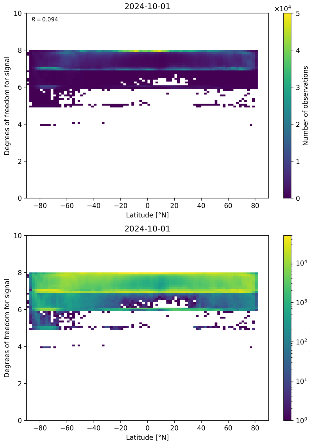
Figure 55: Scatter density plot of “Latitude” against “Degrees of freedom for signal” for 2024-09-30 to 2024-10-02.
