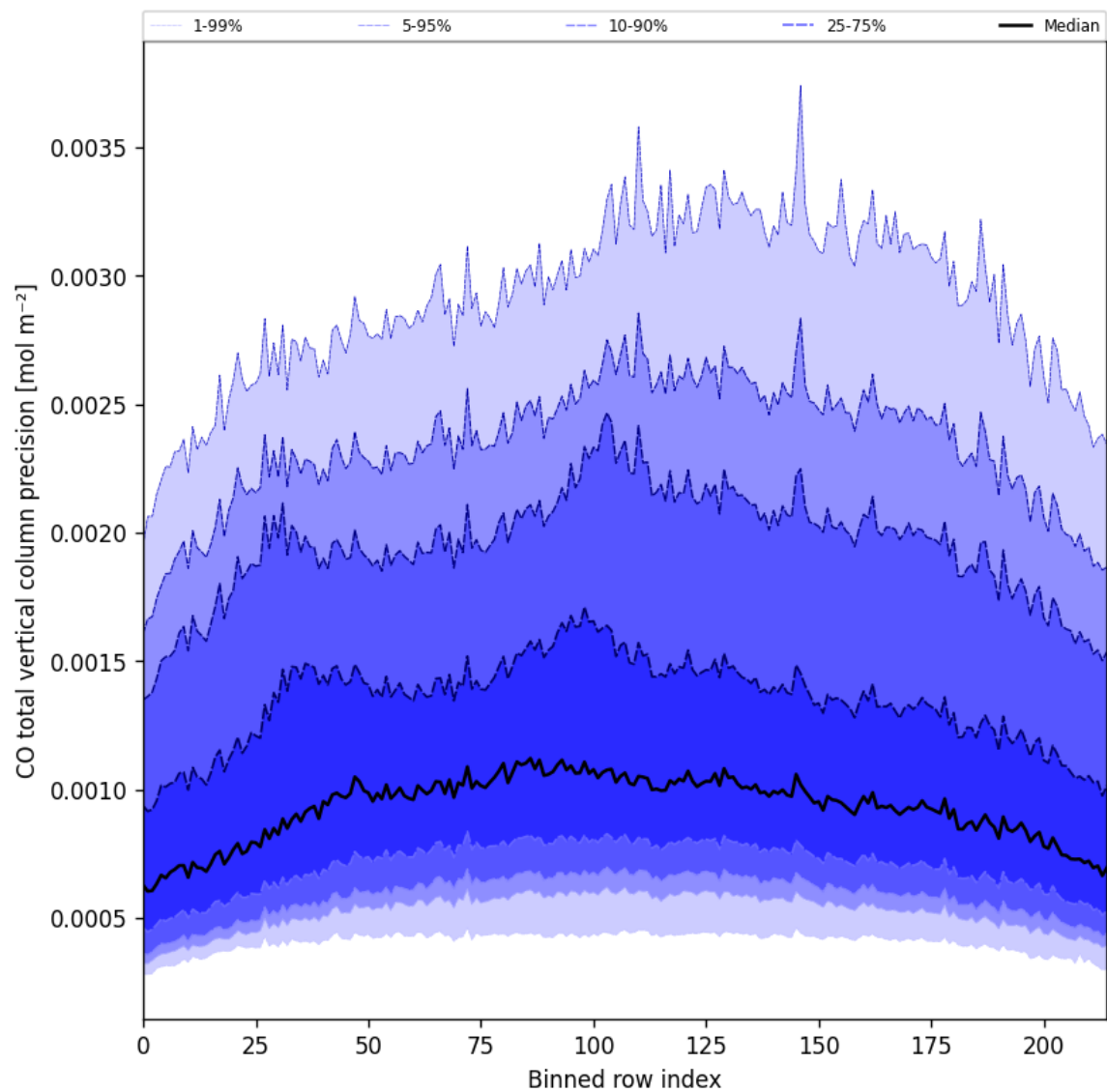
Figure 28: Along track statistics of “CO total vertical column precision” for 2024-09-30 to 2024-10-02
