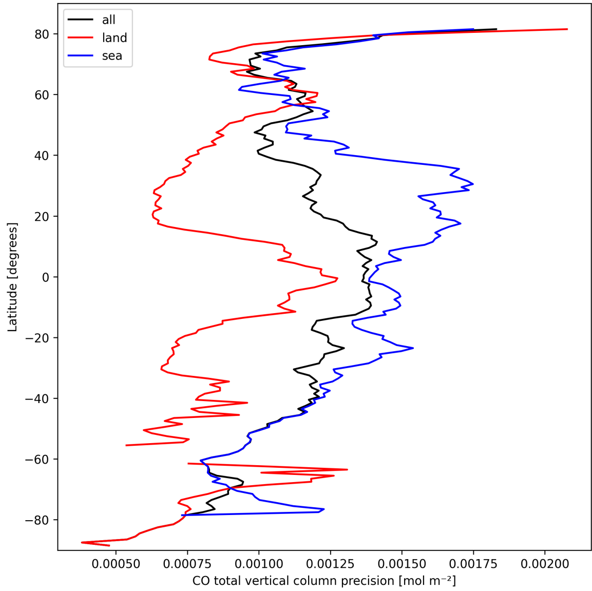
Figure 12: Zonal average of “CO total vertical column precision” for 2024-09-30 to 2024-10-02.
