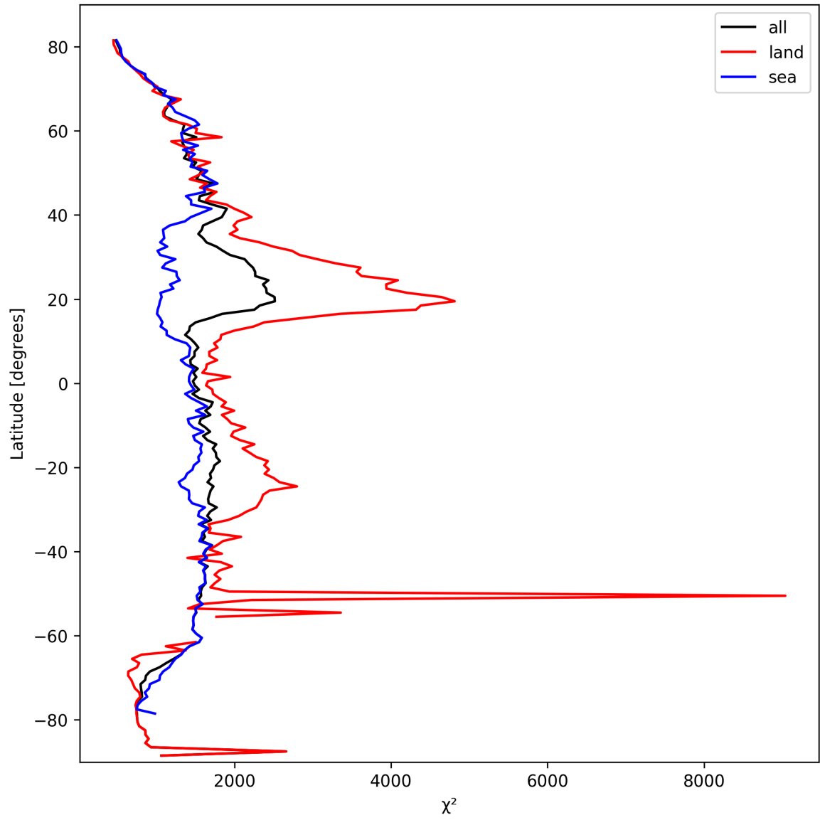
Figure 14: Zonal average of “ \chi^2 ” for 2024-09-30 to 2024-10-02.
