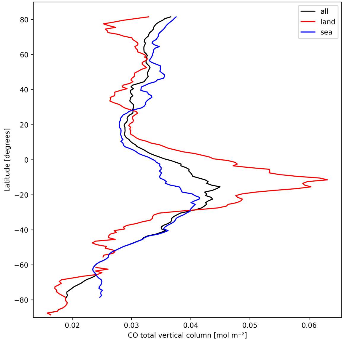
Figure 10: Zonal average of “CO total vertical column” for 2024-09-30 to 2024-10-02.
