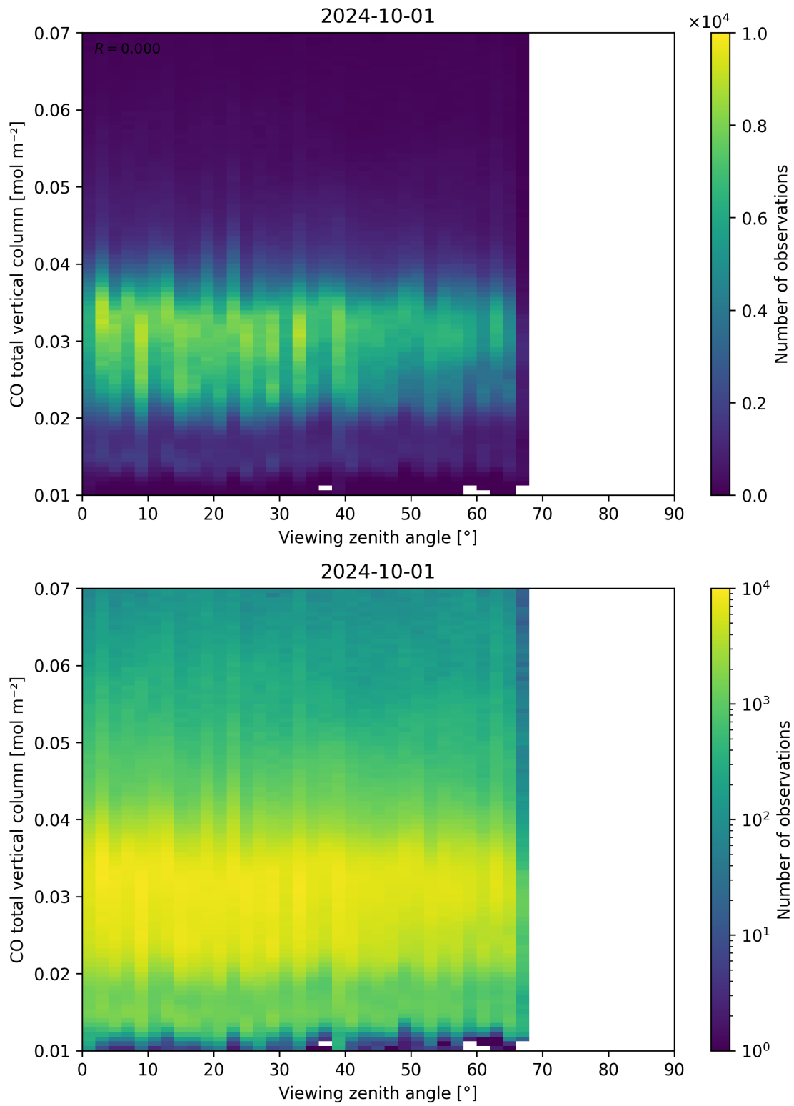
Figure 69: Scatter density plot of “Viewing zenith angle” against “CO total vertical column” for 2024-09-30 to 2024-10-02.
