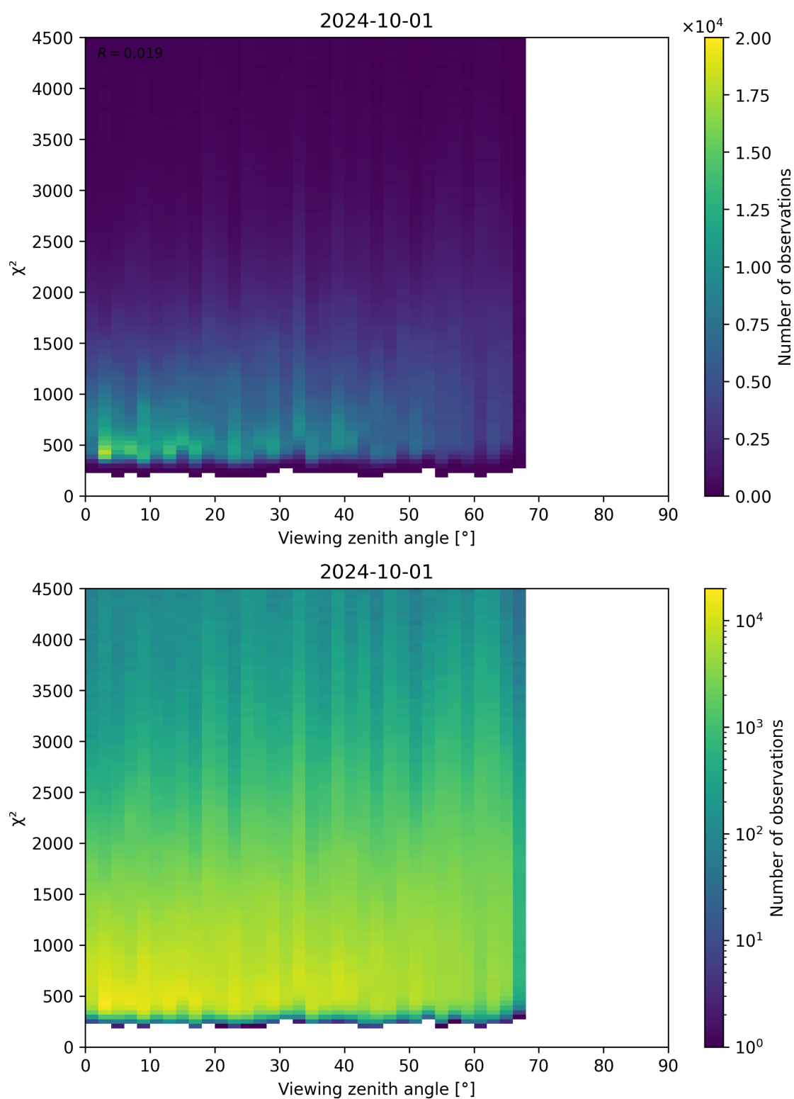
Figure 72: Scatter density plot of “Viewing zenith angle” against “ \chi^2 ” for 2024-09-30 to 2024-10-02.
