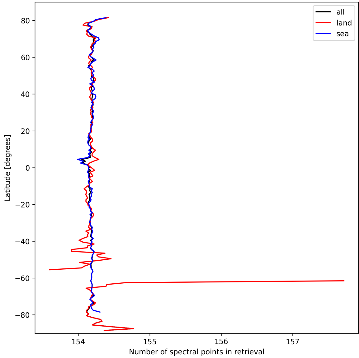
Figure 13: Zonal average of “Number of spectral points in retrieval” for 2024-09-30 to 2024-10-02.
