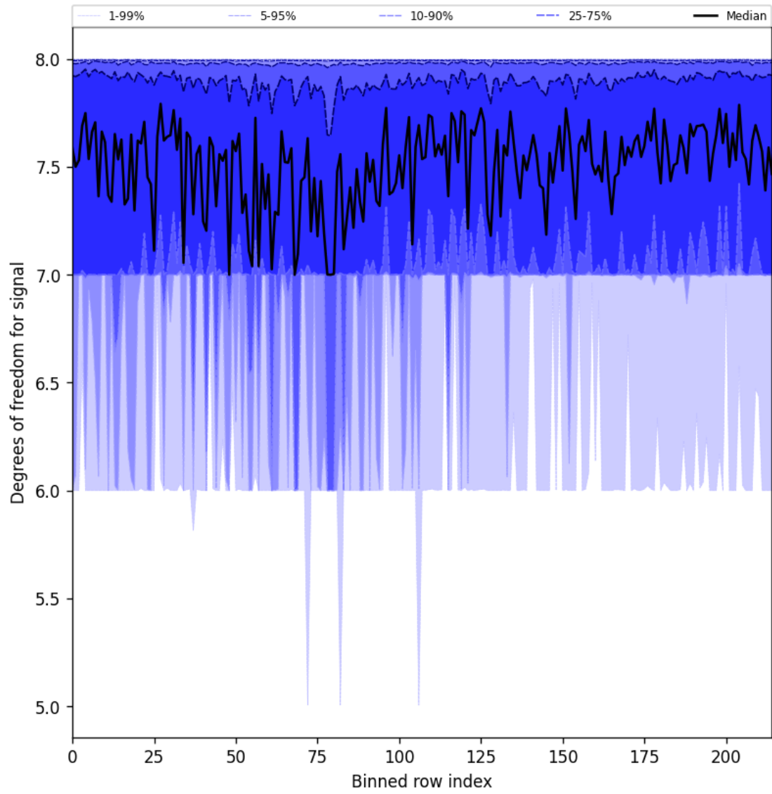
Figure 31: Along track statistics of “Degrees of freedom for signal” for 2024-09-30 to 2024-10-02
