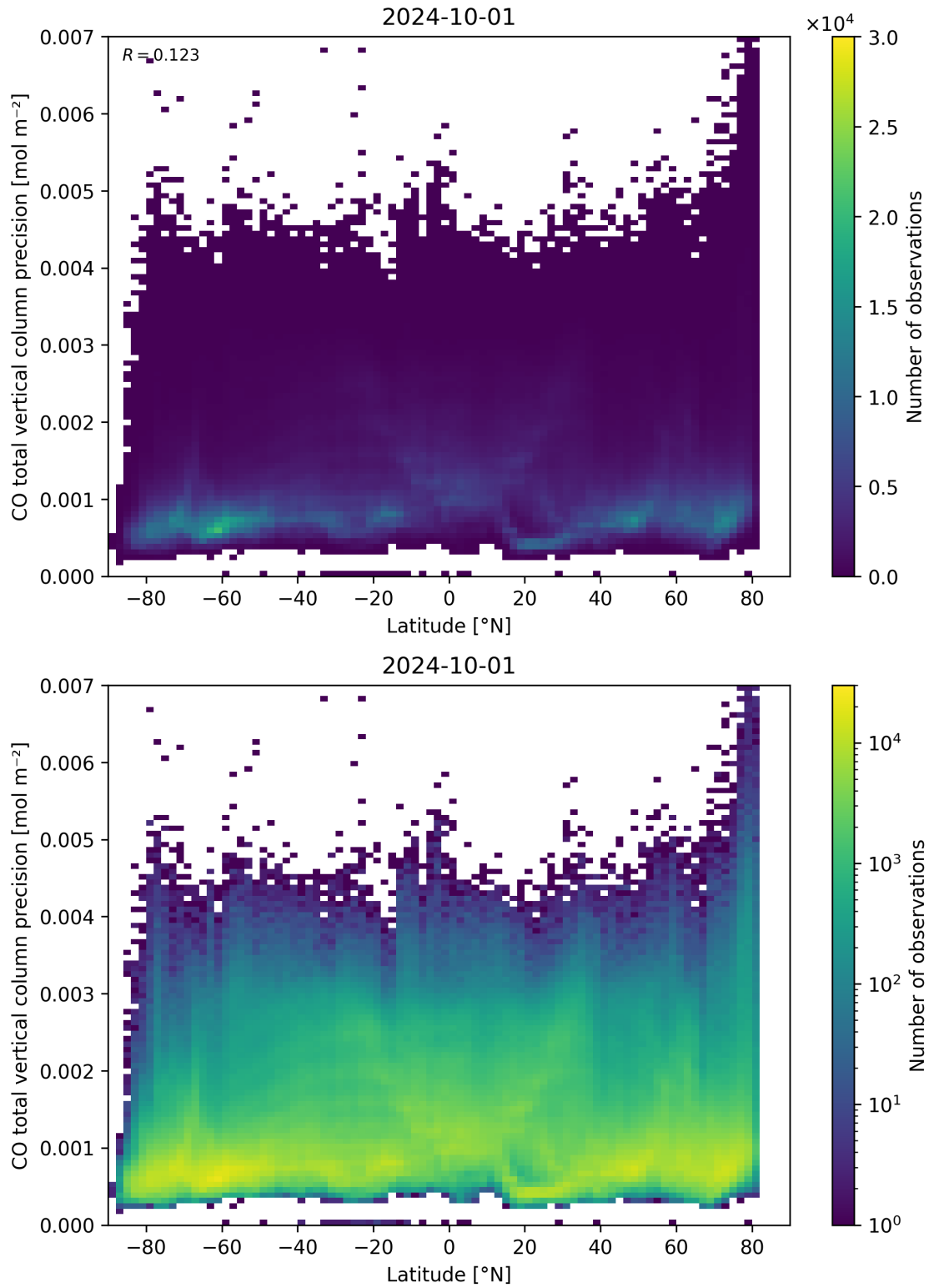
Figure 53: Scatter density plot of “Latitude” against “CO total vertical column precision” for 2024-09-30 to 2024-10-02.
