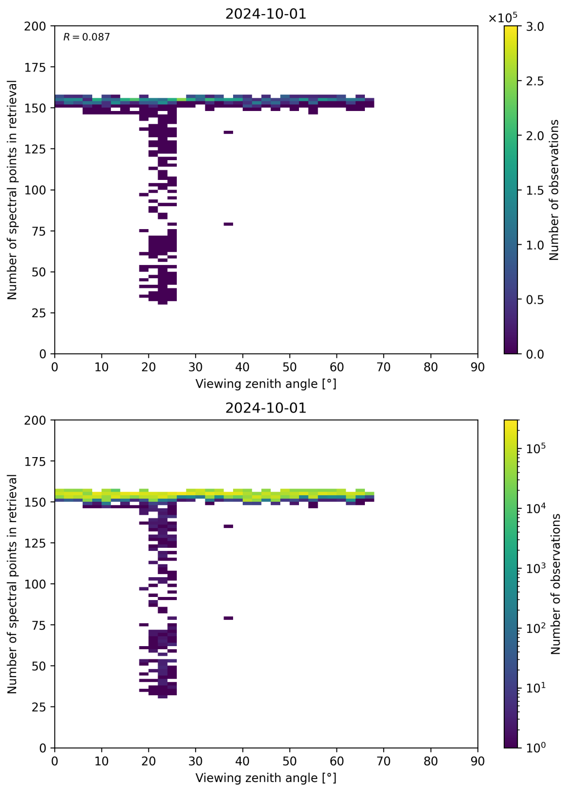
Figure 76: Scatter density plot of “Viewing zenith angle” against “Number of spectral points in retrieval” for 2024-09-30 to 2024-10-02.
