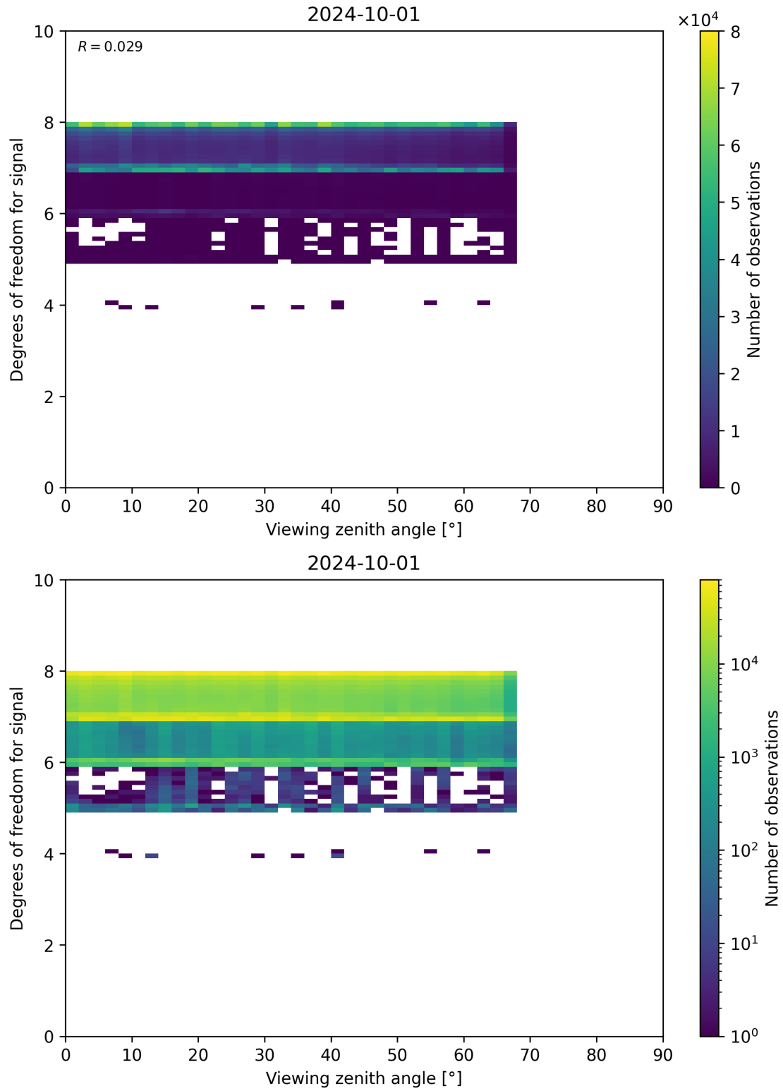
Figure 73: Scatter density plot of “Viewing zenith angle” against “Degrees of freedom for signal” for 2024-09-30 to 2024-10-02.
