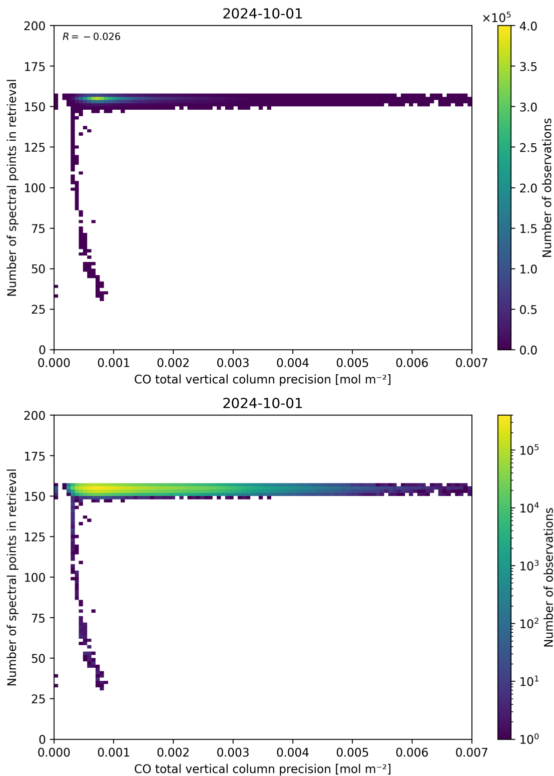
Figure 47: Scatter density plot of “CO total vertical column precision” against “Number of spectral points in retrieval” for 2024-09-30 to 2024-10-02.
