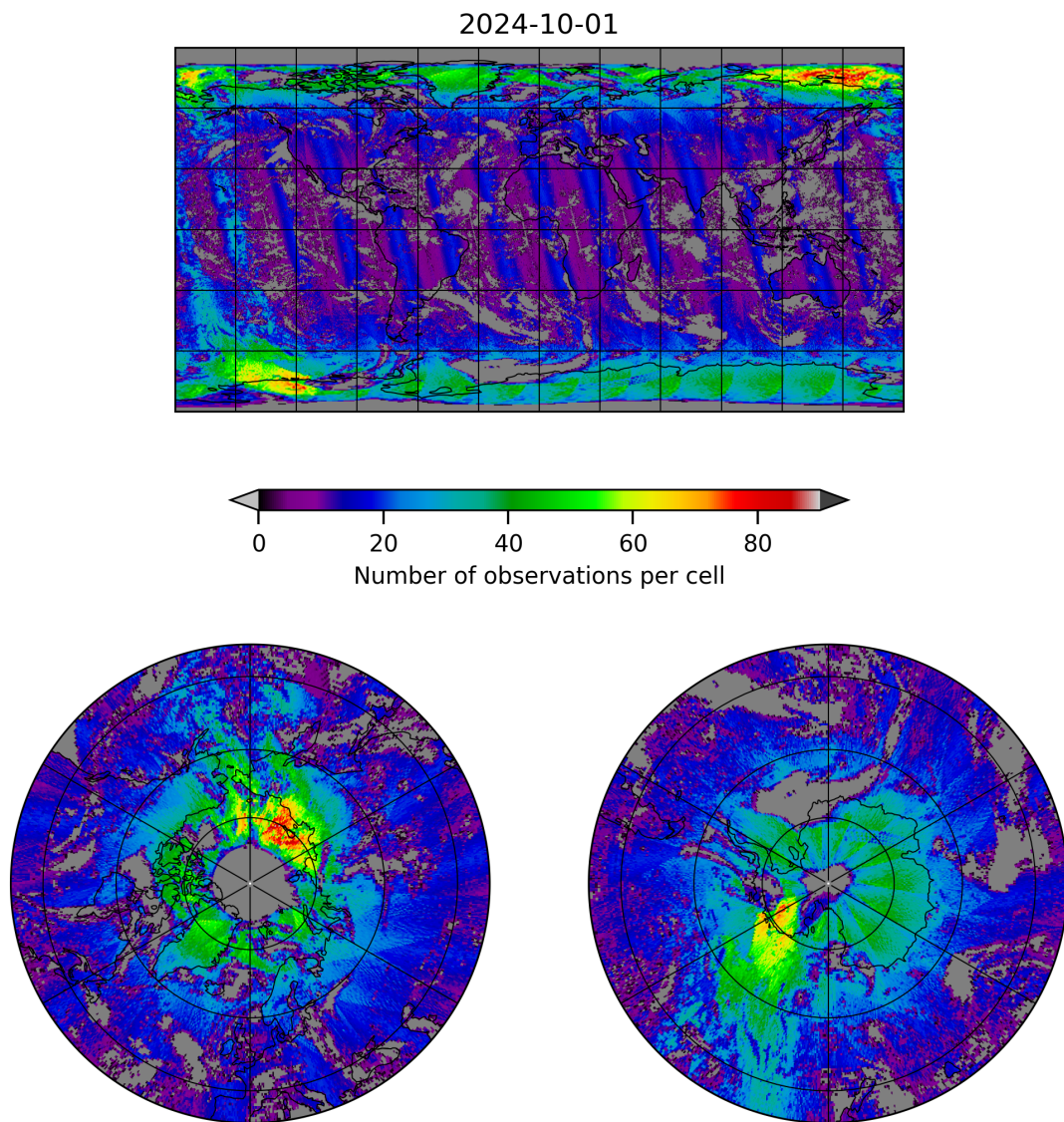
Figure 8: Map of the number of observations for 2024-09-30 to 2024-10-02
