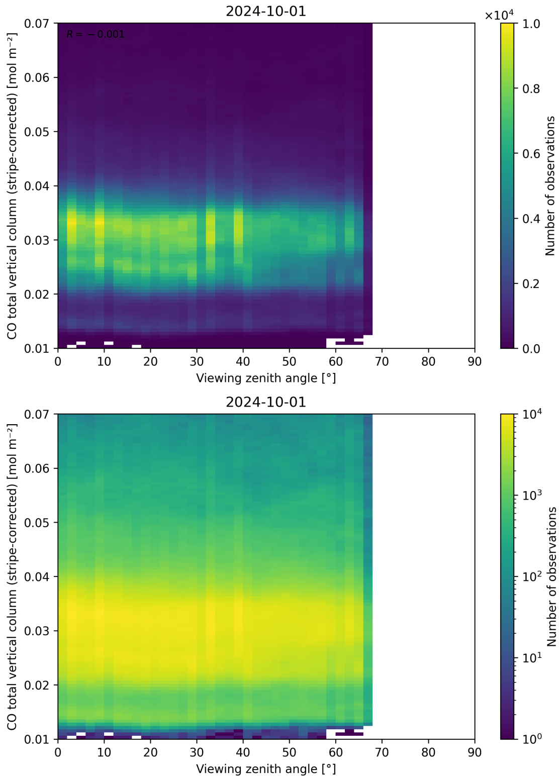
Figure 70: Scatter density plot of “Viewing zenith angle” against “CO total vertical column (stripe-corrected)” for 2024-09-30 to 2024-10-02.
