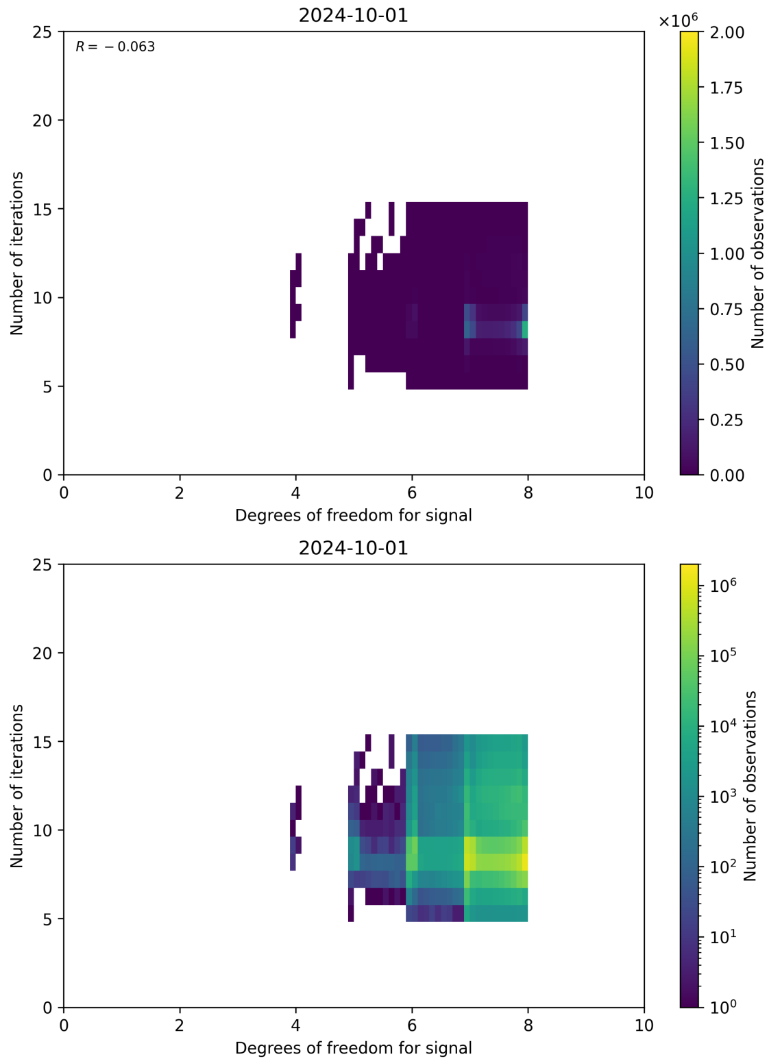
Figure 50: Scatter density plot of “Degrees of freedom for signal” against “Number of iterations” for 2024-09-30 to 2024-10-02.
