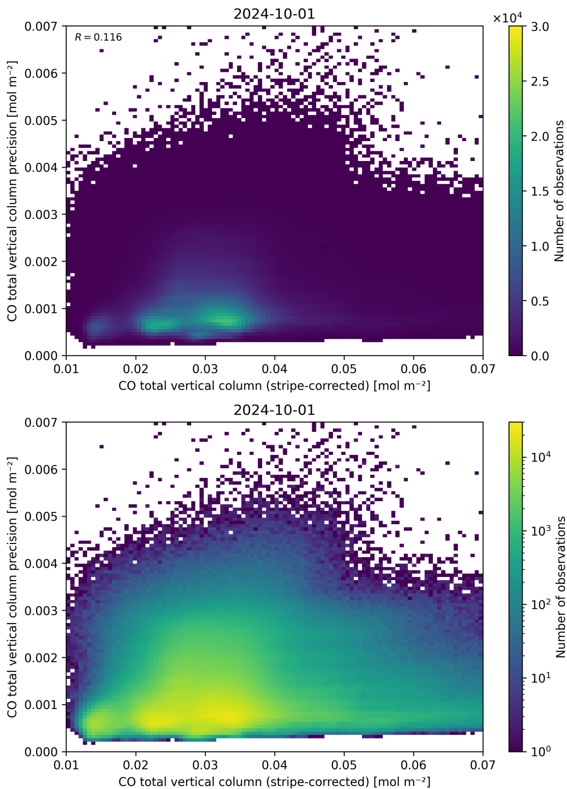
Figure 36: Scatter density plot of “CO total vertical column (stripe-corrected)” against “CO total vertical column precision” for 2024-09-30 to 2024-10-02.
