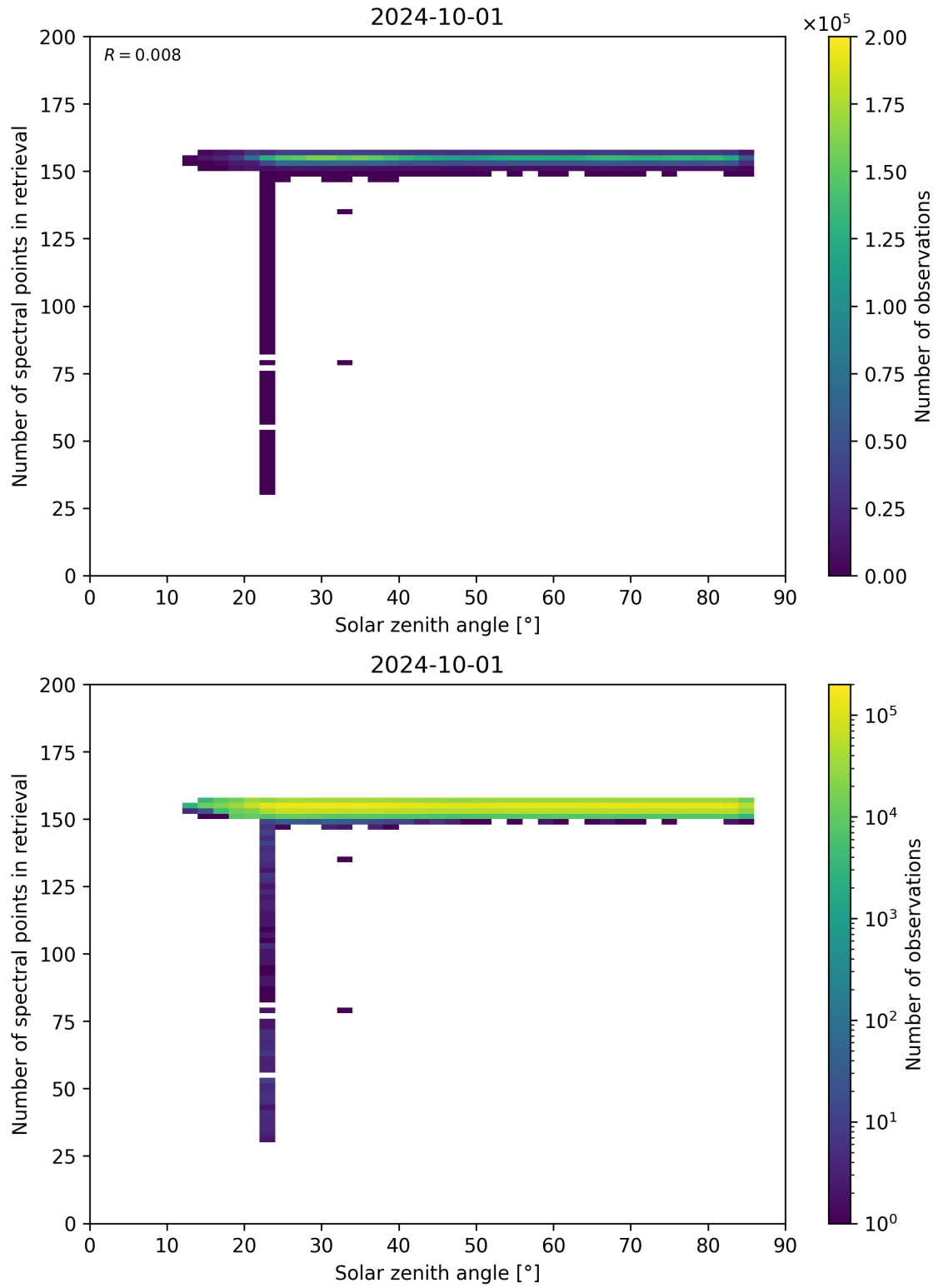
Figure 68: Scatter density plot of “Solar zenith angle” against “Number of spectral points in retrieval” for 2024-09-30 to 2024-10-02.
