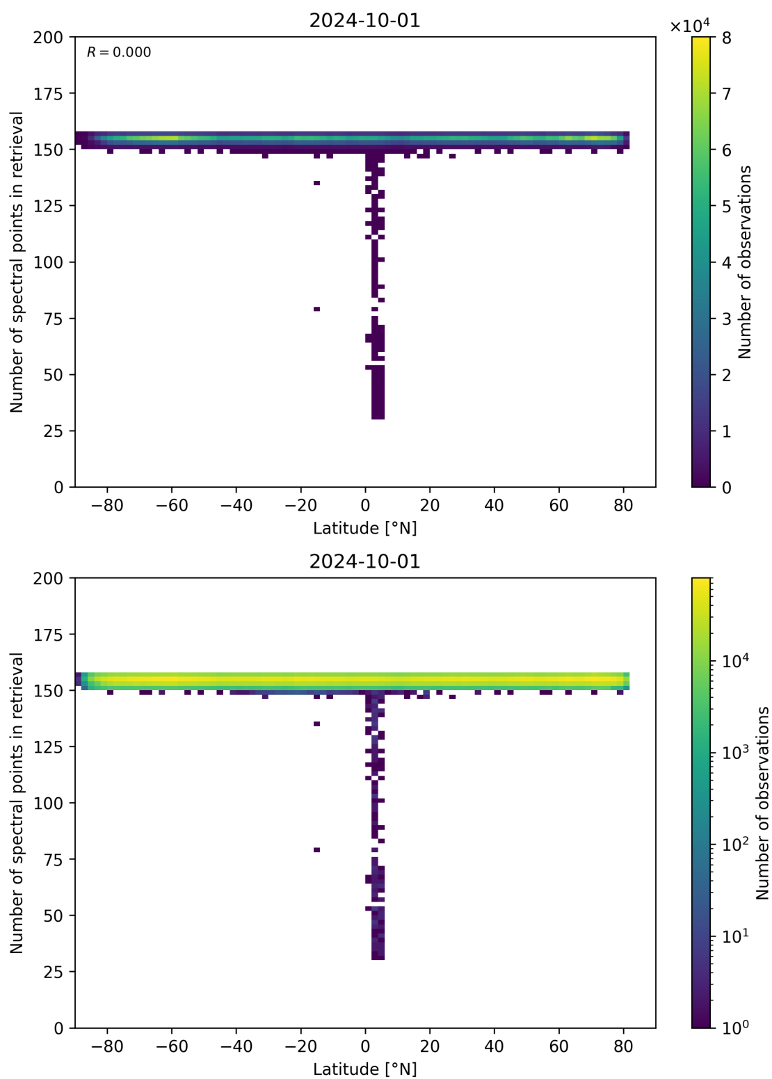
Figure 57: Scatter density plot of “Latitude” against “Number of spectral points in retrieval” for 2024-09-30 to 2024-10-02.
