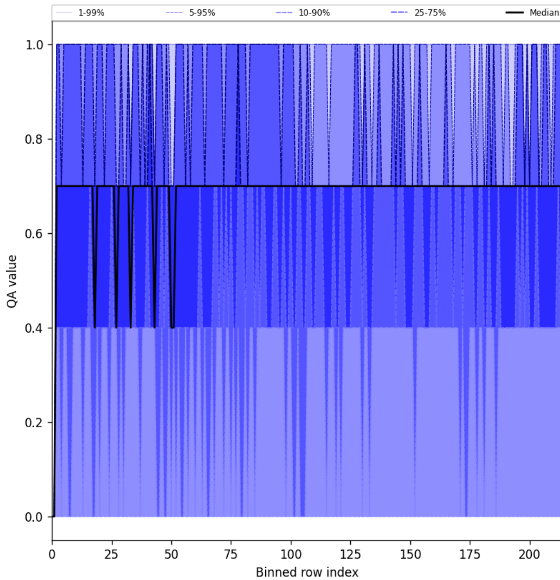
Figure 25: Along track statistics of “QA value” for 2024-09-30 to 2024-10-02
