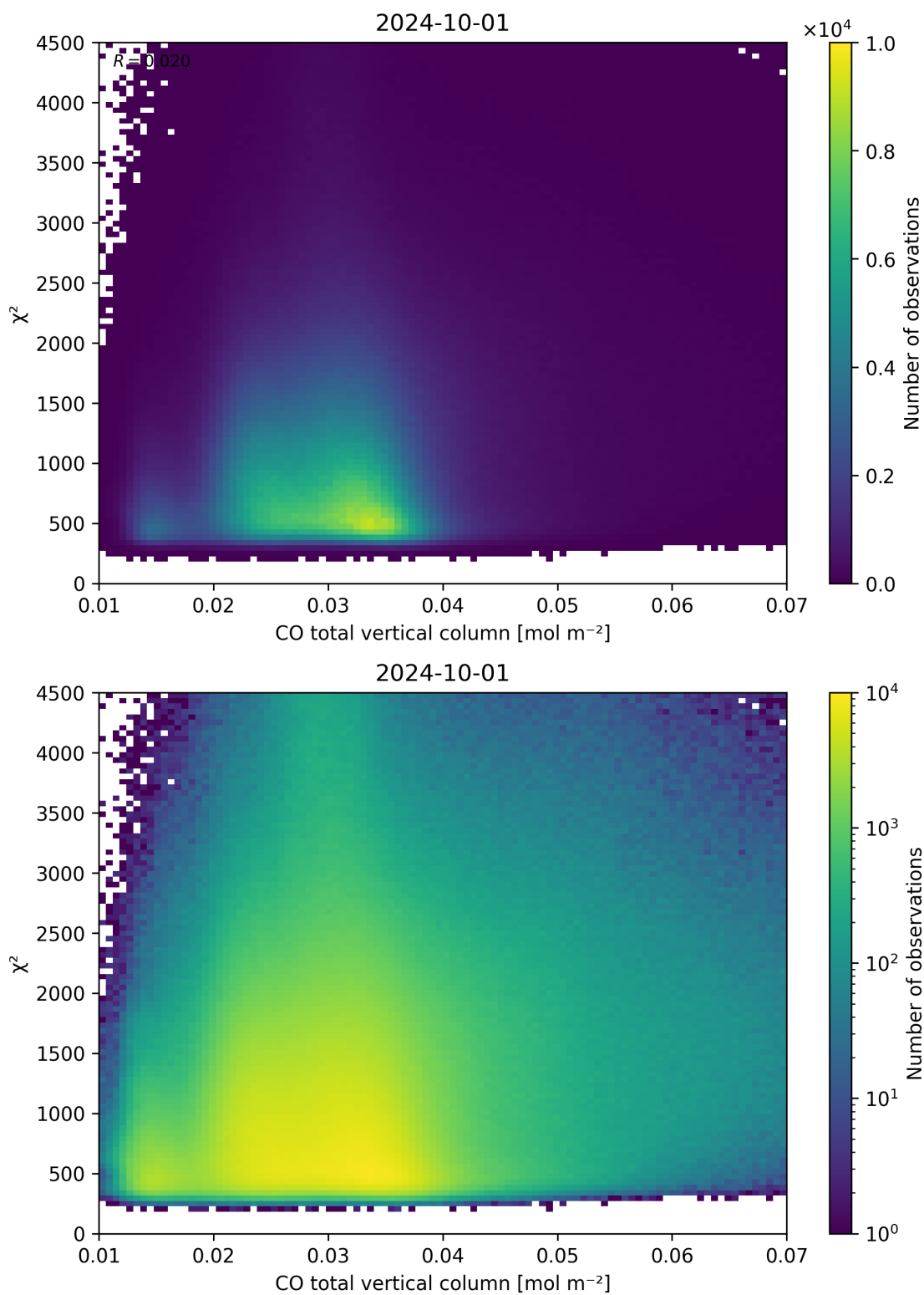
Figure 35: Scatter density plot of “CO total vertical column” against “ \chi^2 ” for 2024-09-30 to 2024-10-02.
