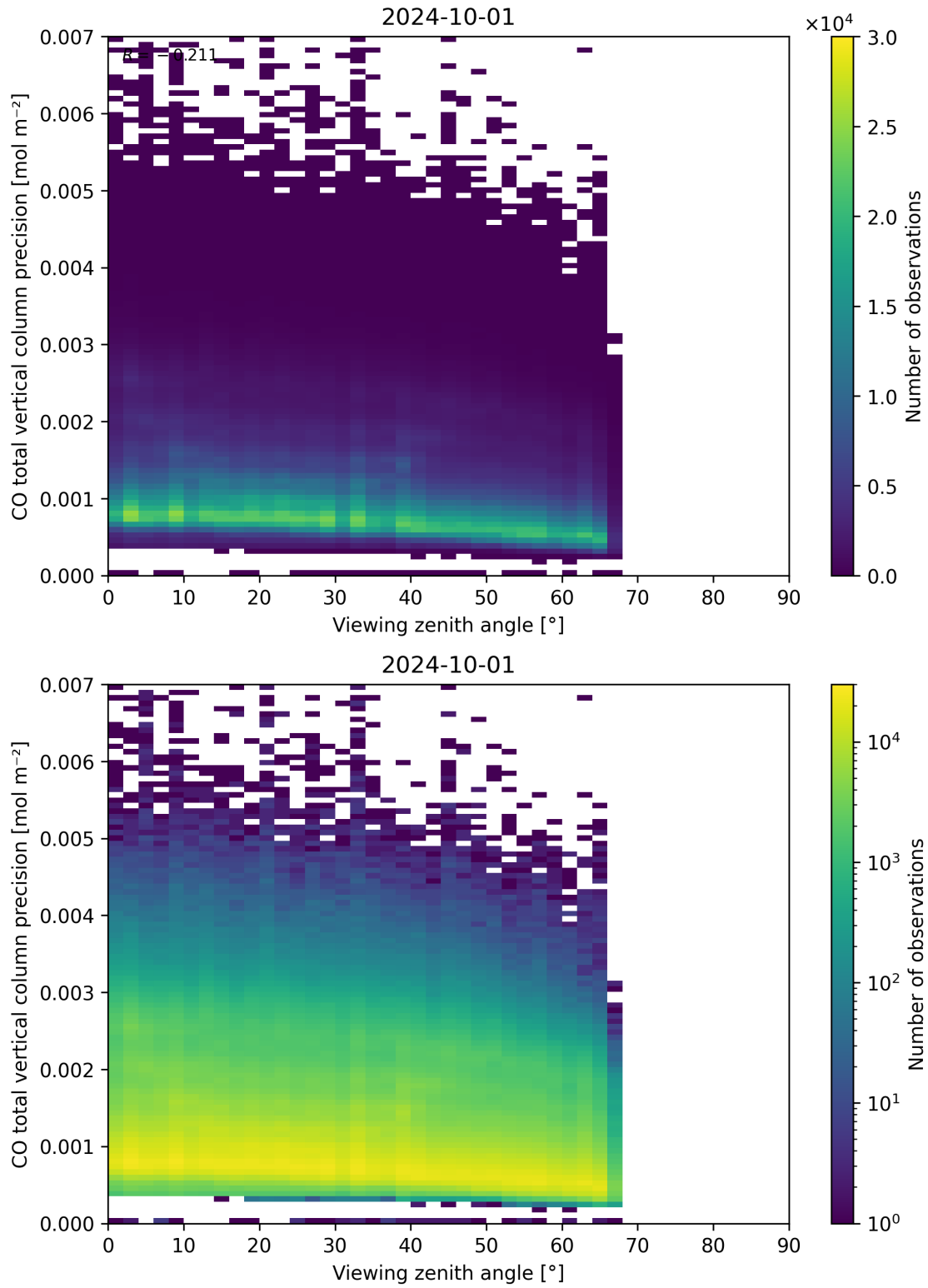
Figure 71: Scatter density plot of “Viewing zenith angle” against “CO total vertical column precision” for 2024-09-30 to 2024-10-02.
