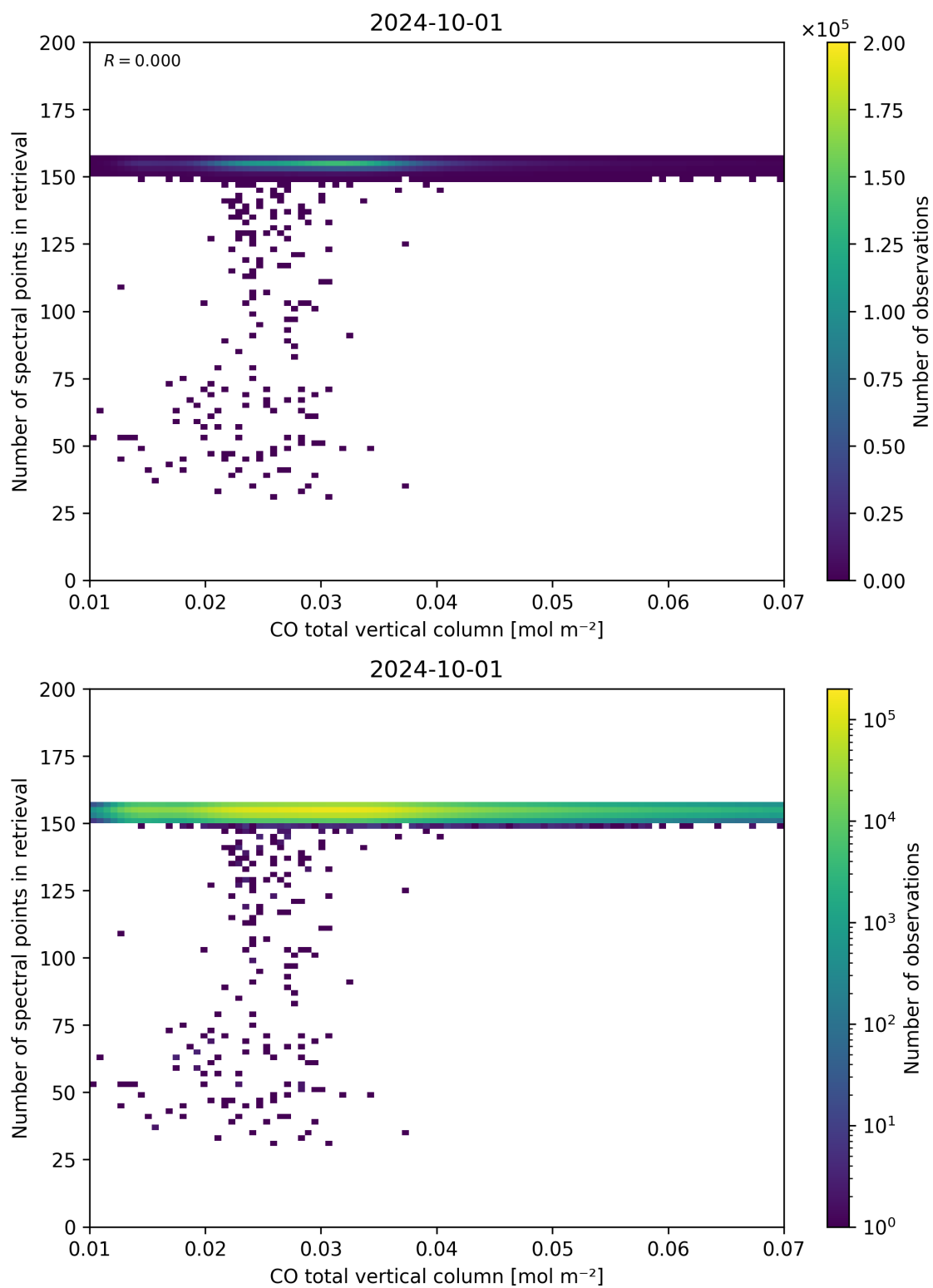
Figure 43: Scatter density plot of “CO total vertical column” against “Number of spectral points in retrieval” for 2024-09-30 to 2024-10-02.
