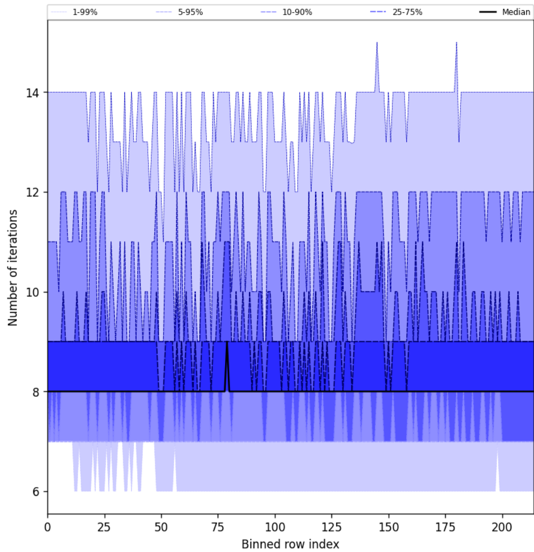
Figure 32: Along track statistics of “Number of iterations” for 2024-09-30 to 2024-10-02
