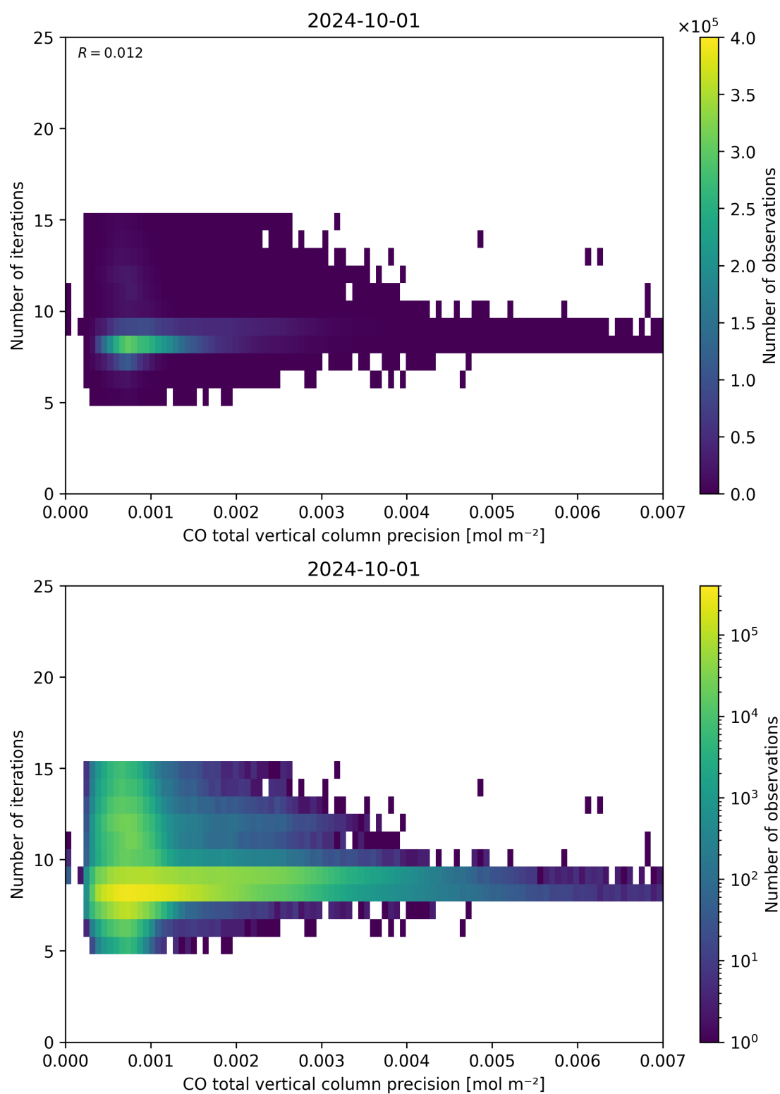
Figure 46: Scatter density plot of “CO total vertical column precision” against “Number of iterations” for 2024-09-30 to 2024-10-02.
