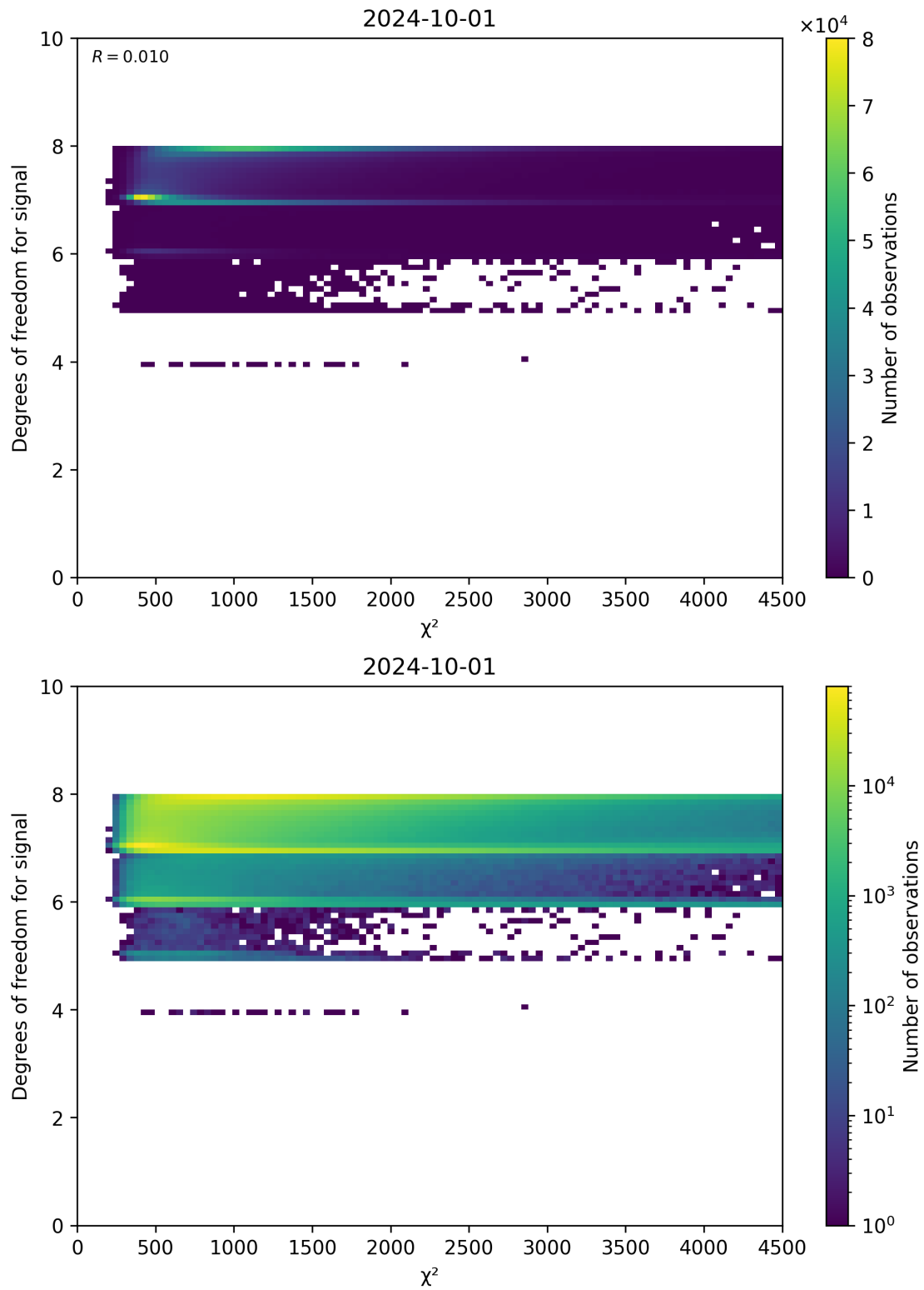
Figure 48: Scatter density plot of “ \chi^2 ” against “Degrees of freedom for signal” for 2024-09-30 to 2024-10-02.
