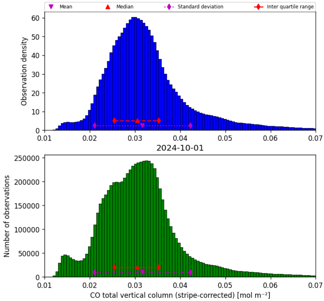
Figure 19: Histogram of “CO total vertical column (stripe-corrected)” for 2024-09-30 to 2024-10-02
