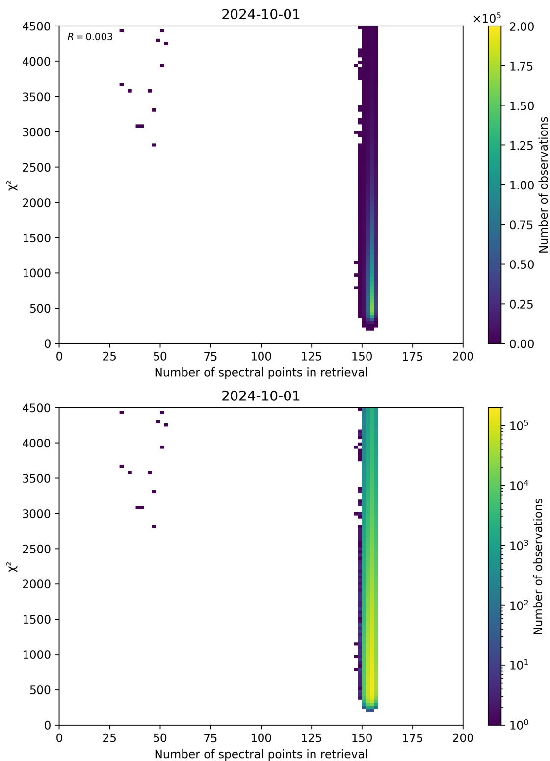
Figure 58: Scatter density plot of “Number of spectral points in retrieval” against “ \chi^2 ” for 2024-09-30 to 2024-10-02.
