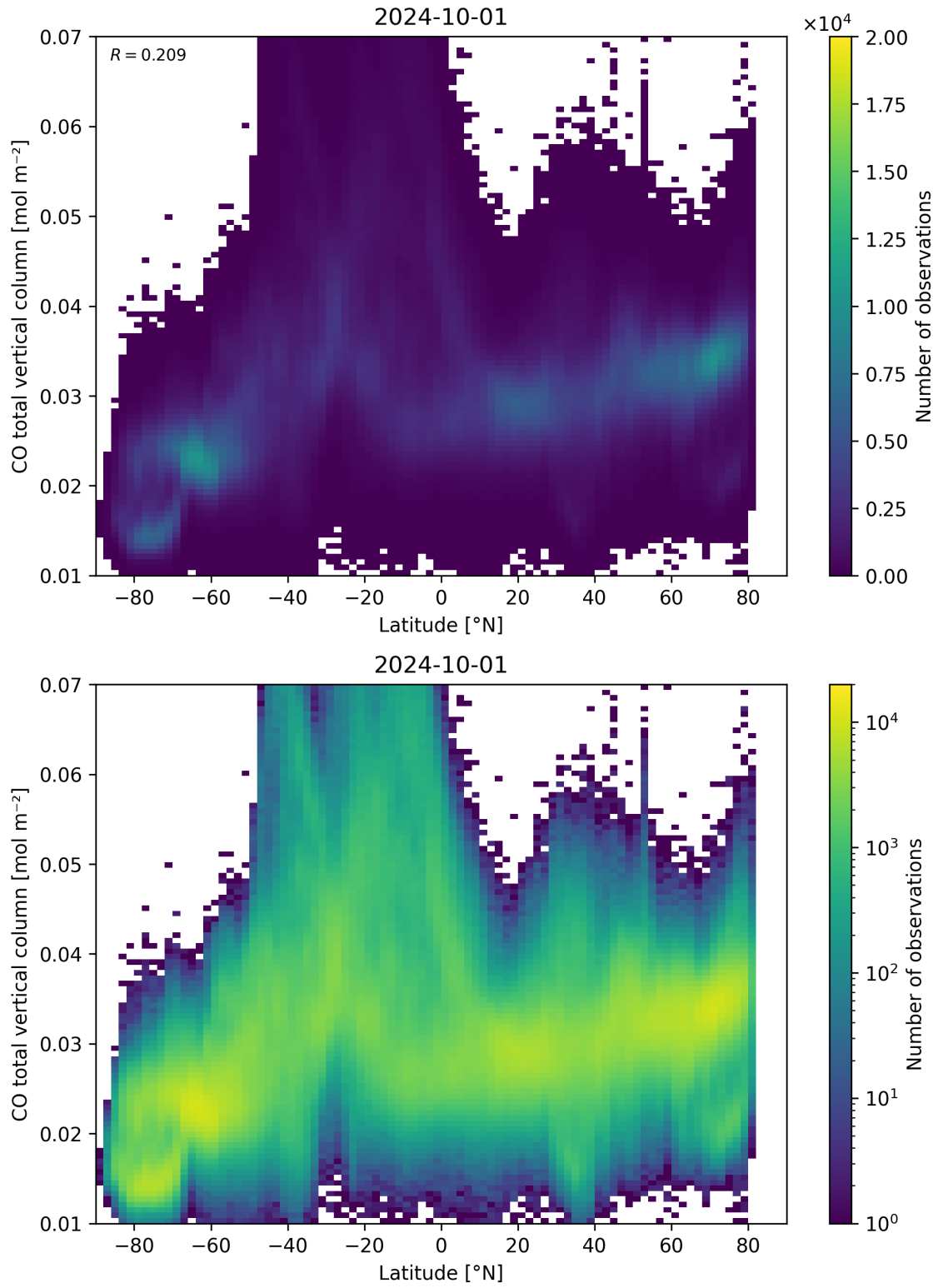
Figure 51: Scatter density plot of “Latitude” against “CO total vertical column” for 2024-09-30 to 2024-10-02.
