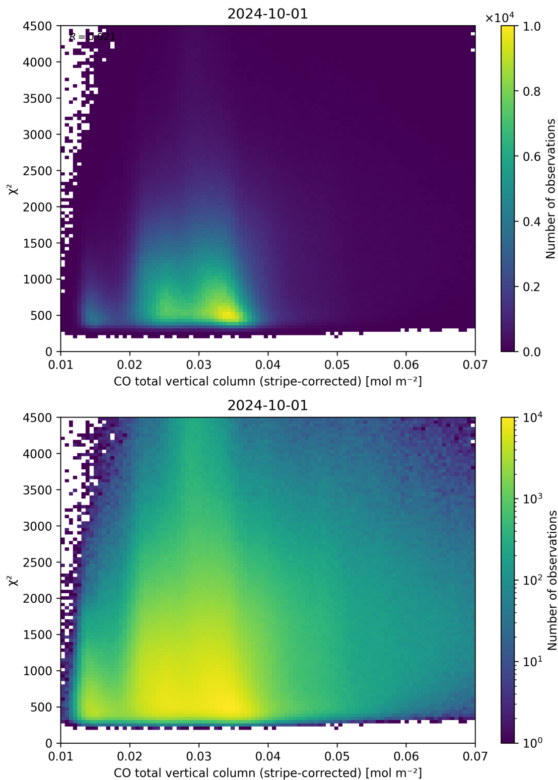
Figure 37: Scatter density plot of “CO total vertical column (stripe-corrected)” against “ \chi^2 ” for 2024-09-30 to 2024-10-02.
