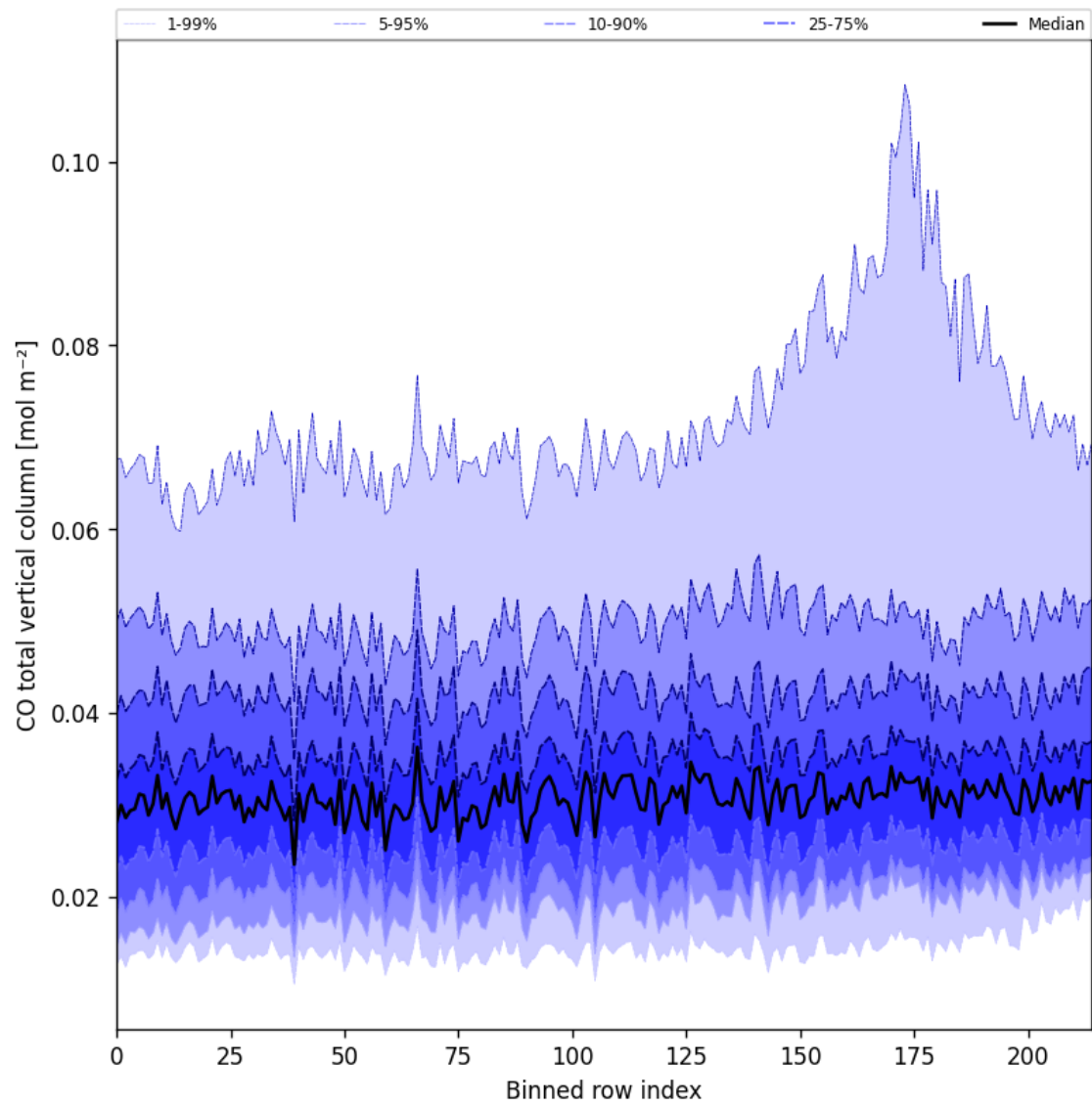
Figure 26: Along track statistics of “CO total vertical column” for 2024-09-30 to 2024-10-02
