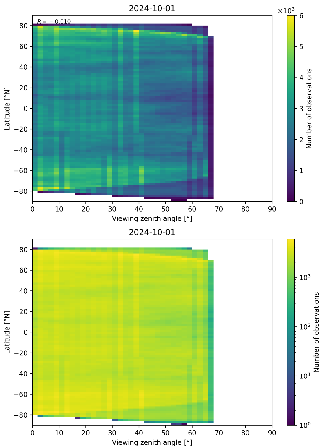
Figure 74: Scatter density plot of “Viewing zenith angle” against “Latitude” for 2024-09-30 to 2024-10-02.
