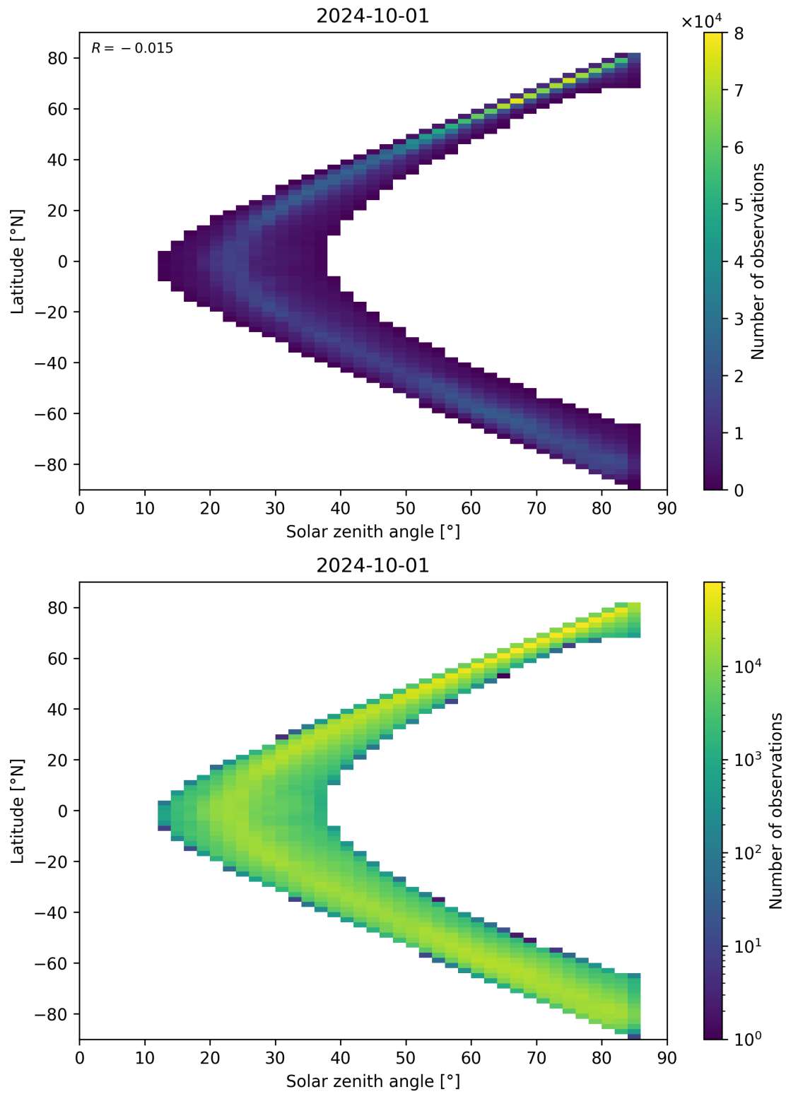
Figure 66: Scatter density plot of “Solar zenith angle” against “Latitude” for 2024-09-30 to 2024-10-02.
