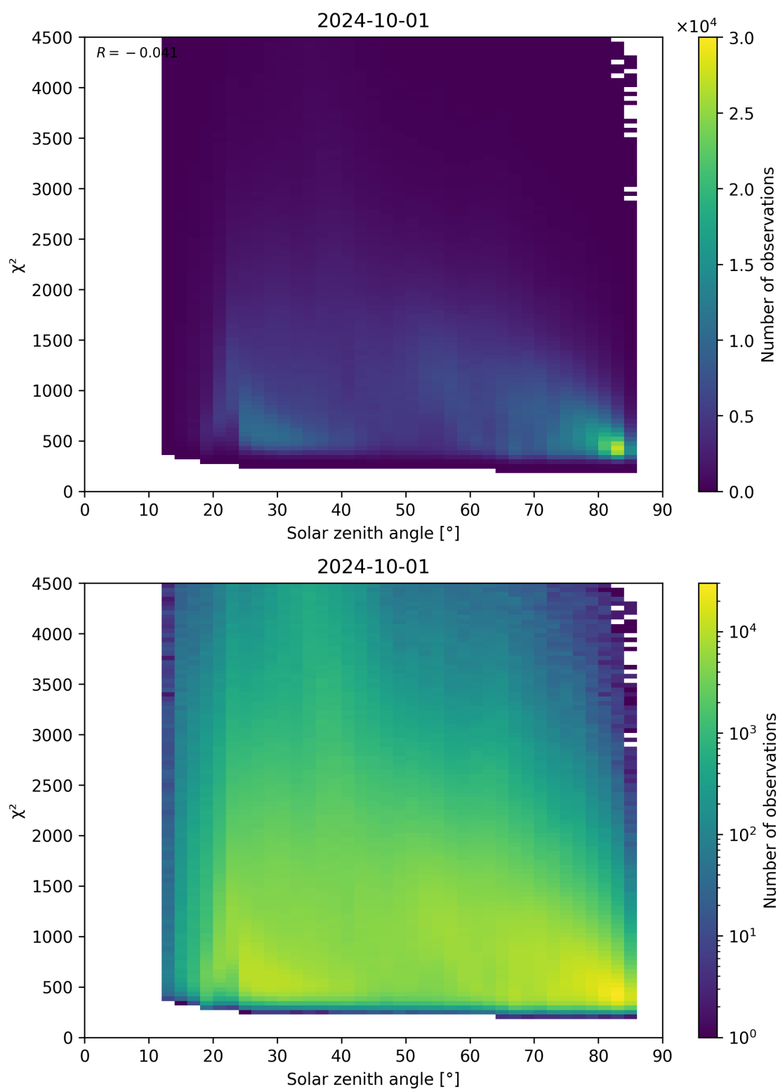
Figure 64: Scatter density plot of “Solar zenith angle” against “ \chi^2 ” for 2024-09-30 to 2024-10-02.
