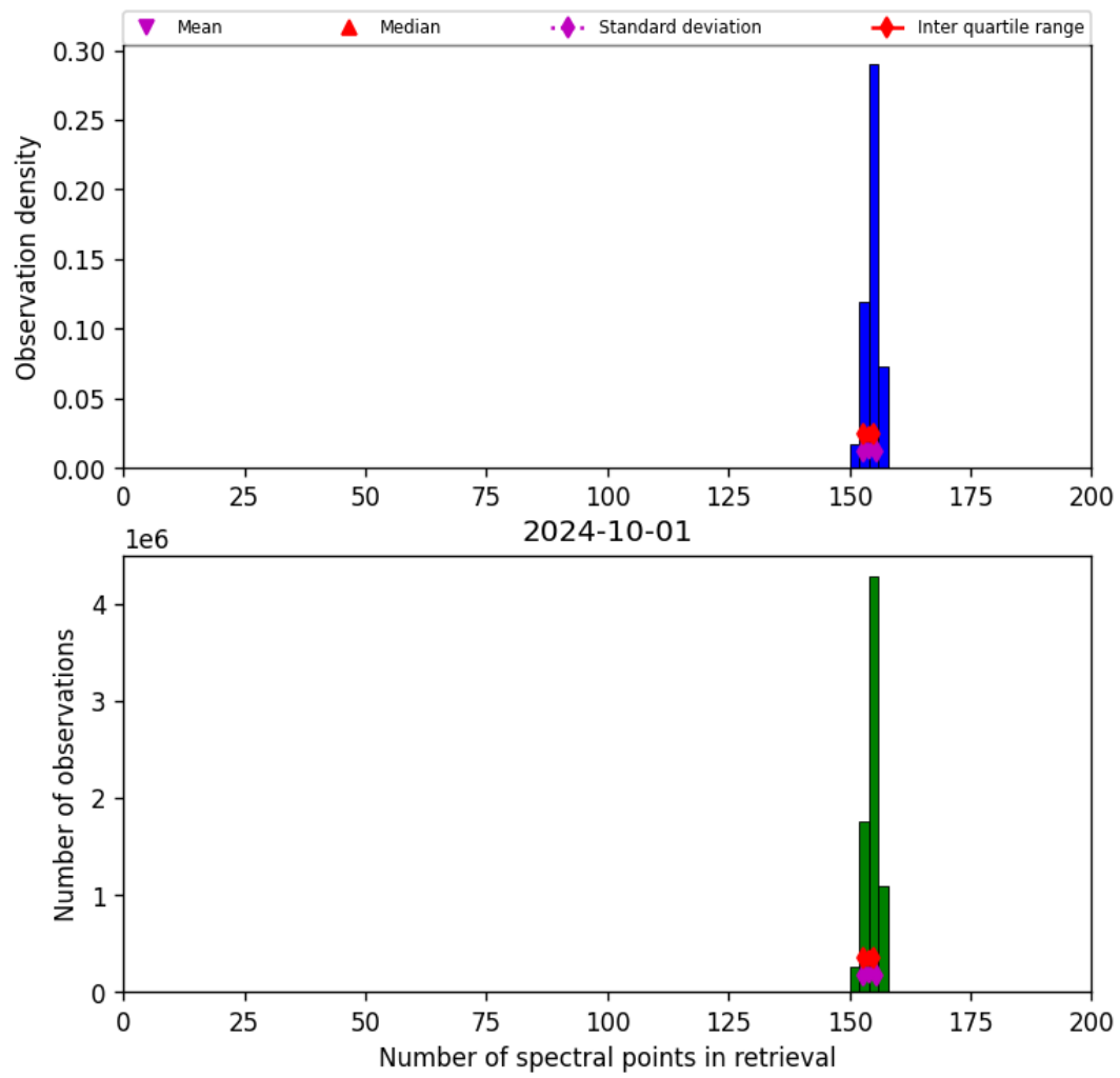
Figure 21: Histogram of "Number of spectral points in retrieval" for 2024-09-30 to 2024-10-02
