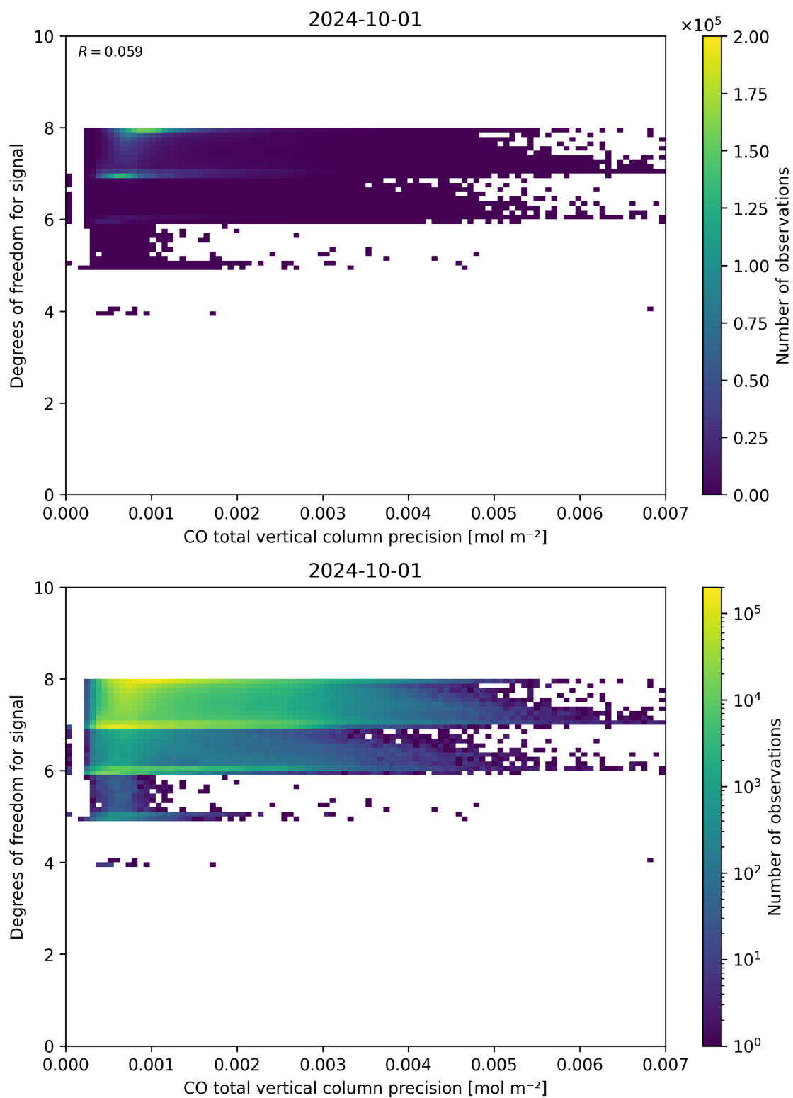
Figure 45: Scatter density plot of “CO total vertical column precision” against “Degrees of freedom for signal” for 2024-09-30 to 2024-10-02.
