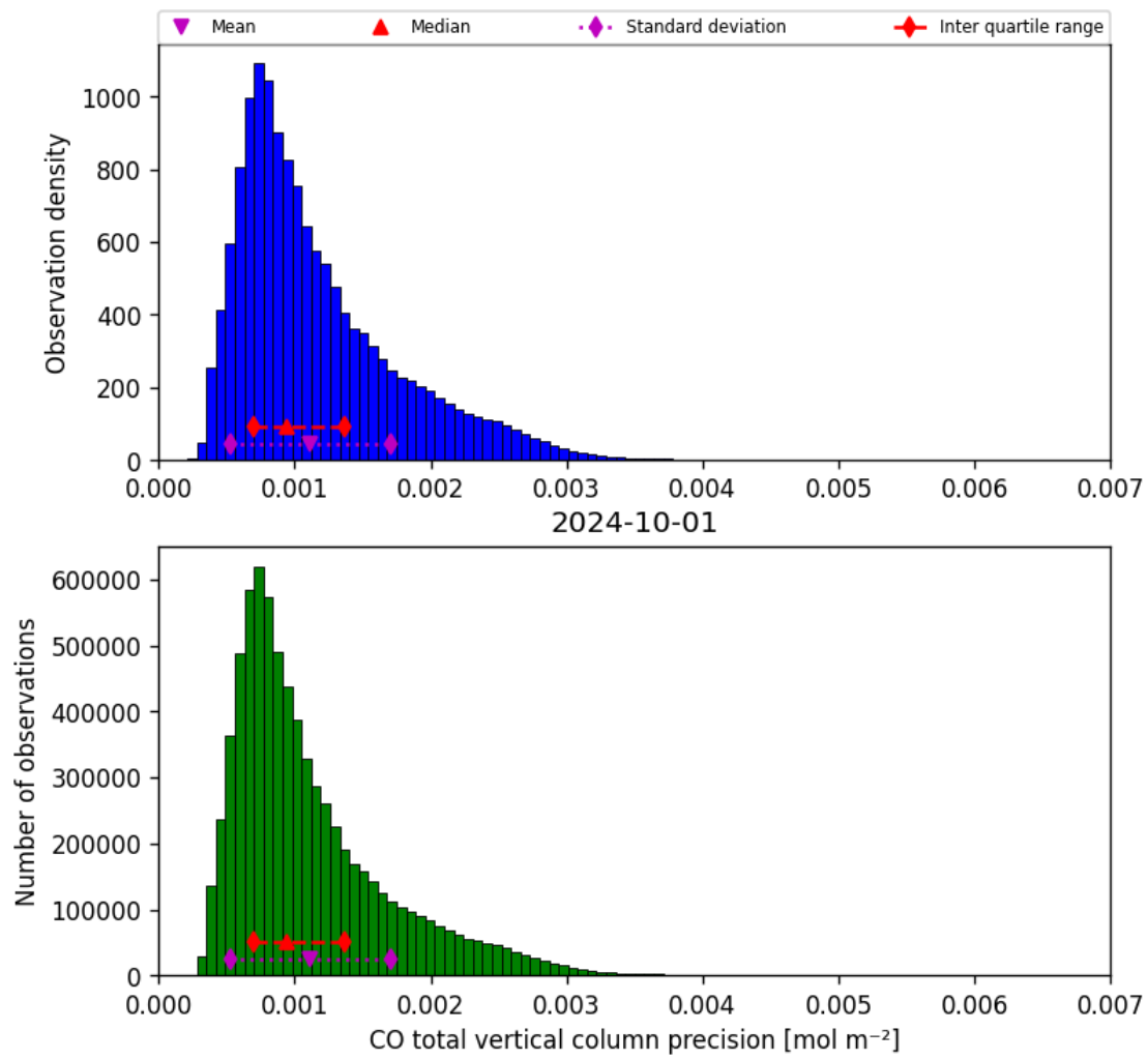
Figure 20: Histogram of “CO total vertical column precision” for 2024-09-30 to 2024-10-02
