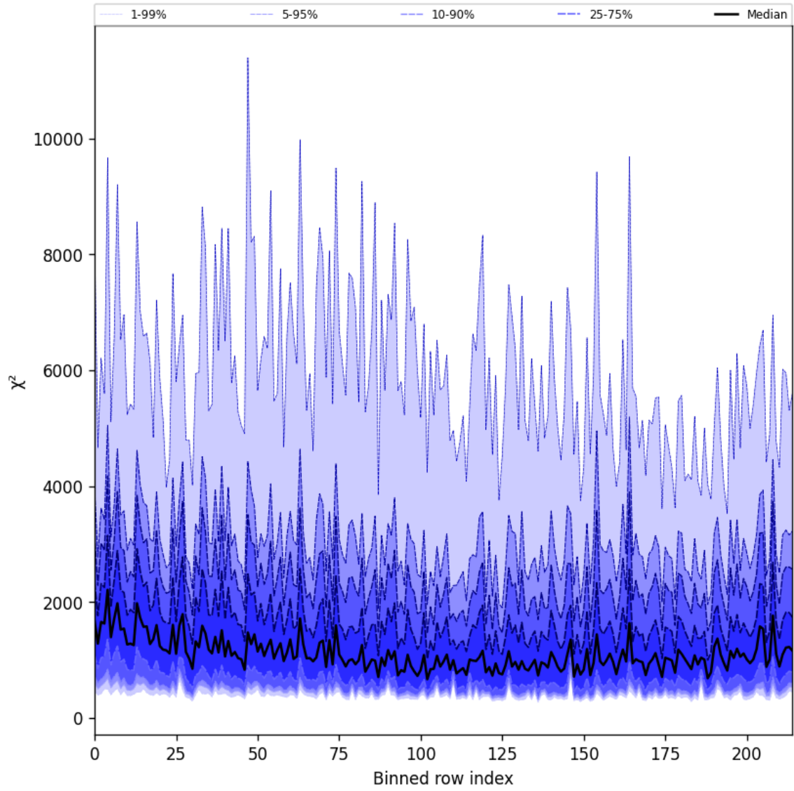
Figure 30: Along track statistics of “ \chi^2 ” for 2024-09-30 to 2024-10-02
