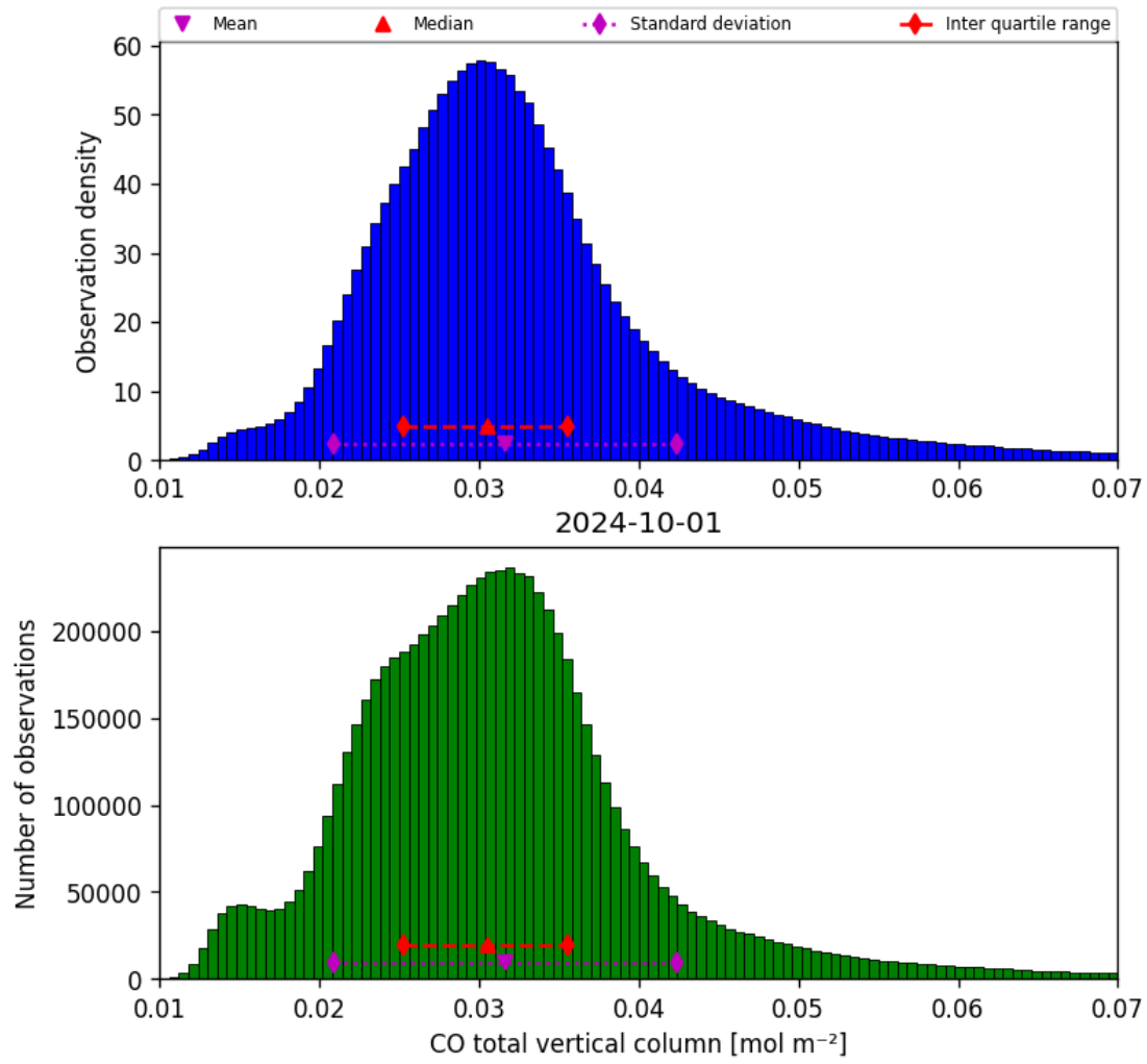
Figure 18: Histogram of “CO total vertical column” for 2024-09-30 to 2024-10-02
