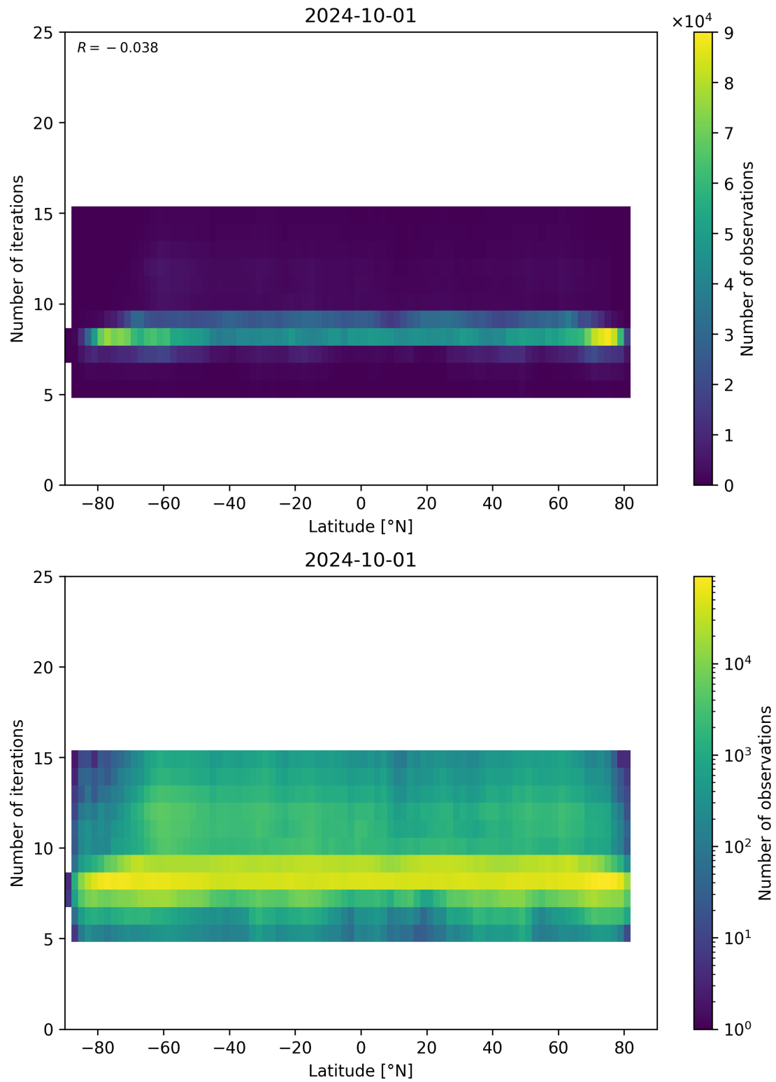
Figure 56: Scatter density plot of “Latitude” against “Number of iterations” for 2024-09-30 to 2024-10-02.
