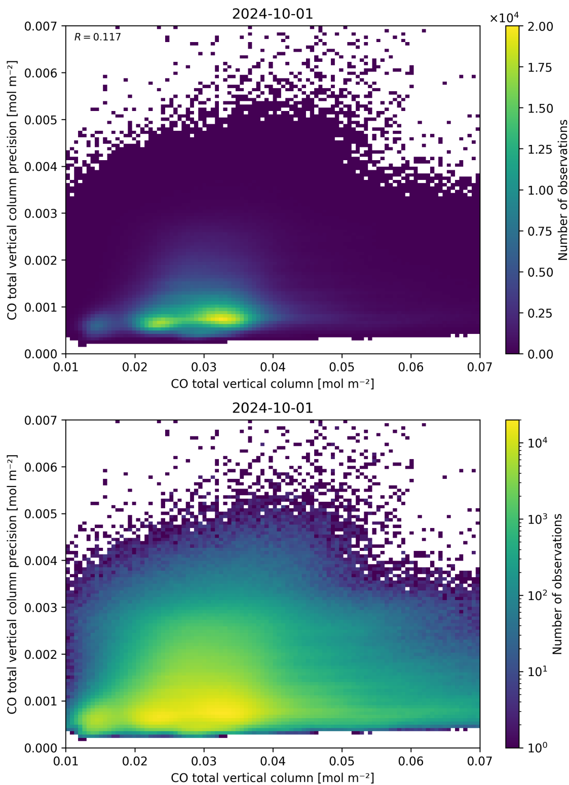
Figure 34: Scatter density plot of “CO total vertical column” against “CO total vertical column precision” for 2024-09-30 to 2024-10-02.
