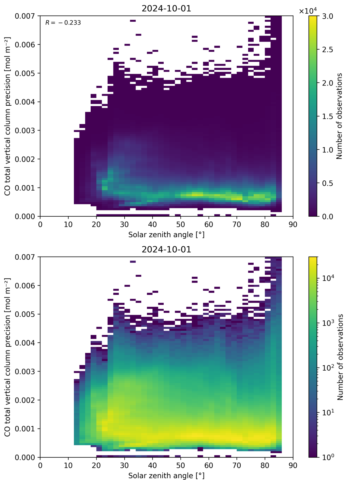
Figure 63: Scatter density plot of “Solar zenith angle” against “CO total vertical column precision” for 2024-09-30 to 2024-10-02.
