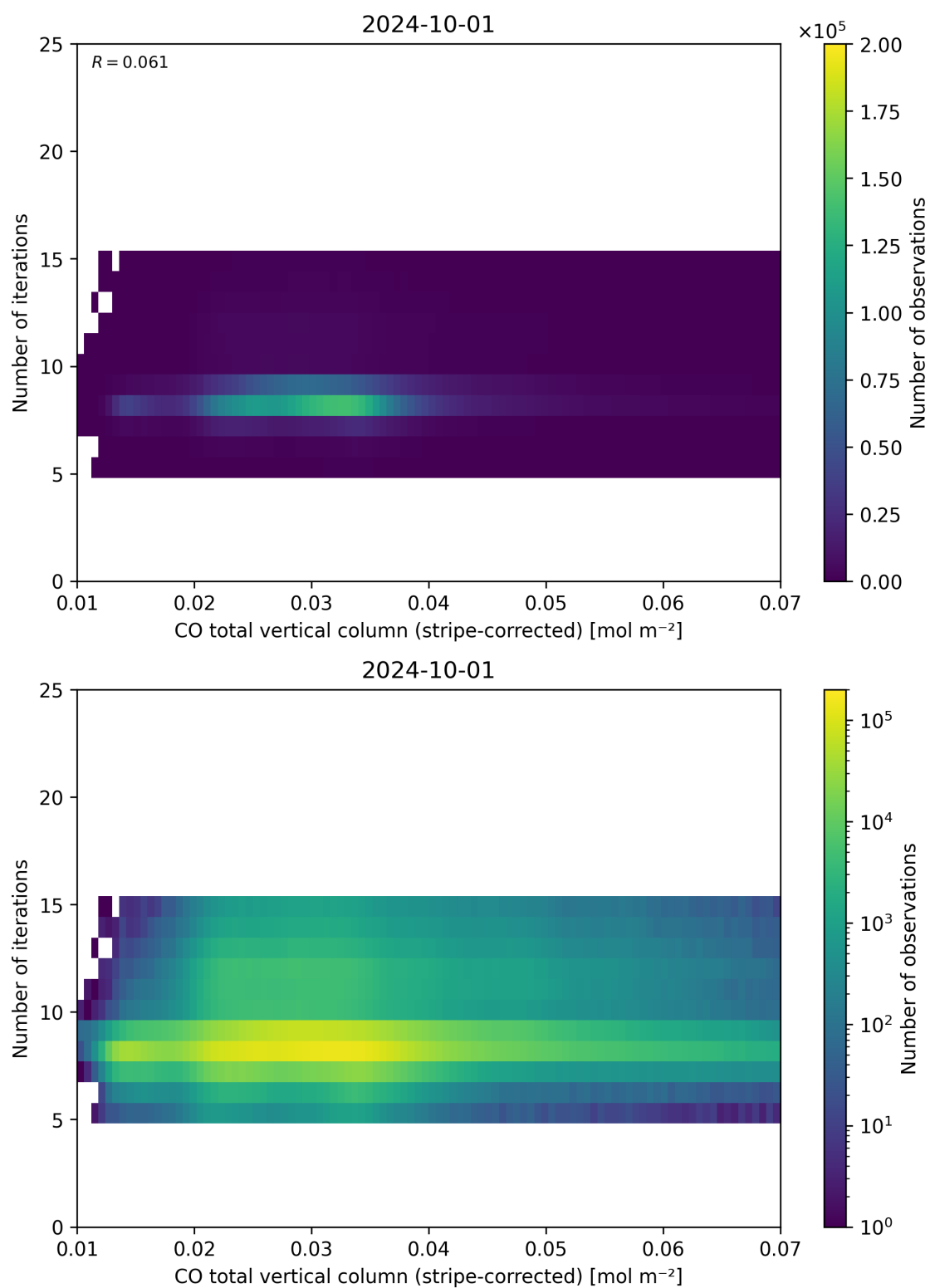
Figure 39: Scatter density plot of “CO total vertical column (stripe-corrected)” against “Number of iterations” for 2024-09-30 to 2024-10-02.
