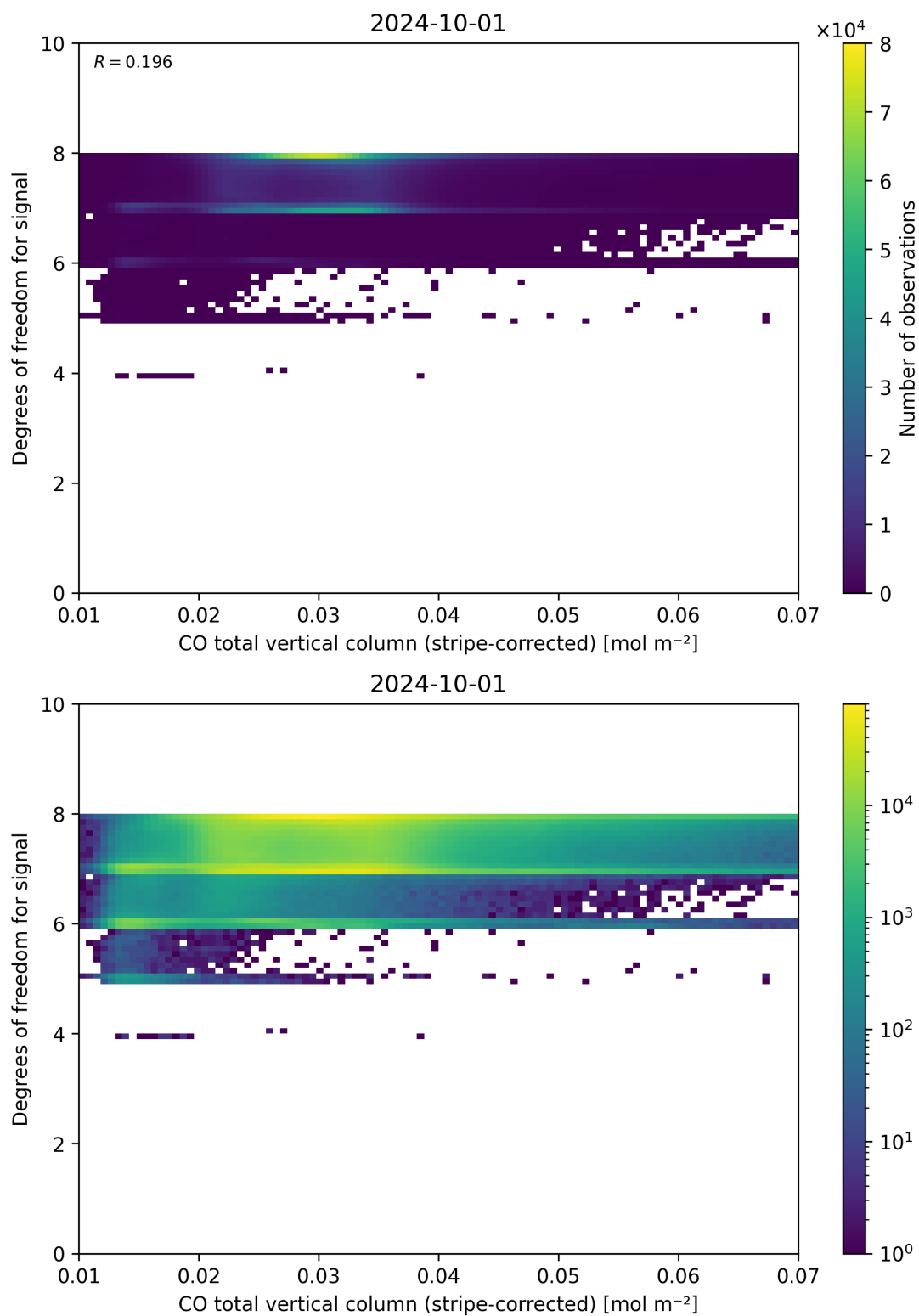
Figure 38: Scatter density plot of “CO total vertical column (stripe-corrected)” against “Degrees of freedom for signal” for 2024-09-30 to 2024-10-02.
