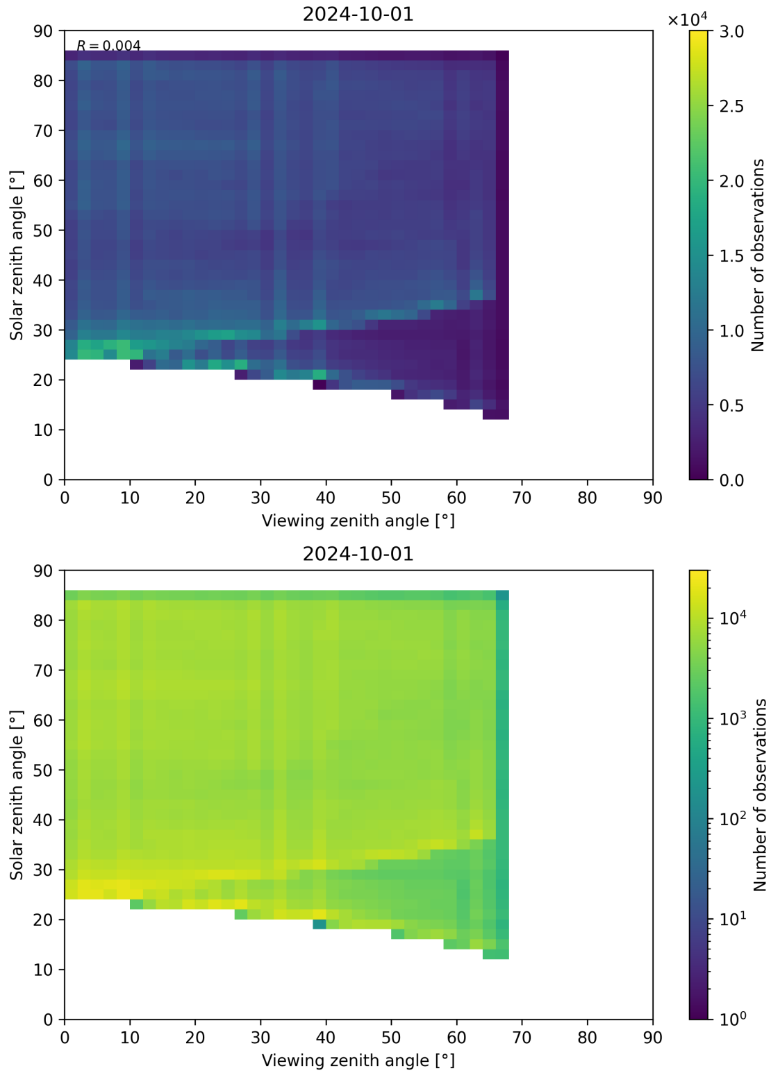
Figure 77: Scatter density plot of “Viewing zenith angle” against “Solar zenith angle” for 2024-09-30 to 2024-10-02.
