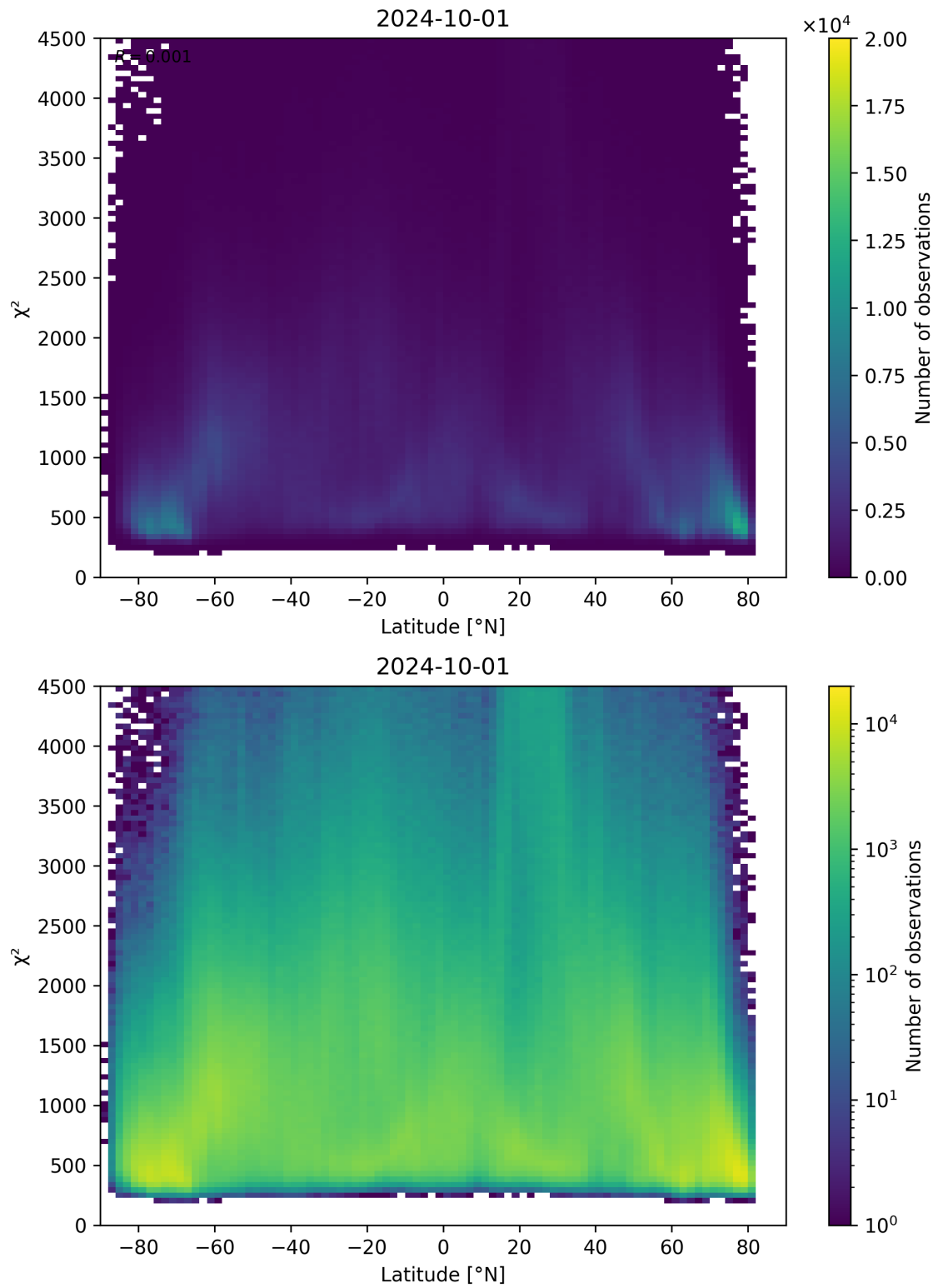
Figure 54: Scatter density plot of “Latitude” against “ \chi^2 ” for 2024-09-30 to 2024-10-02.
