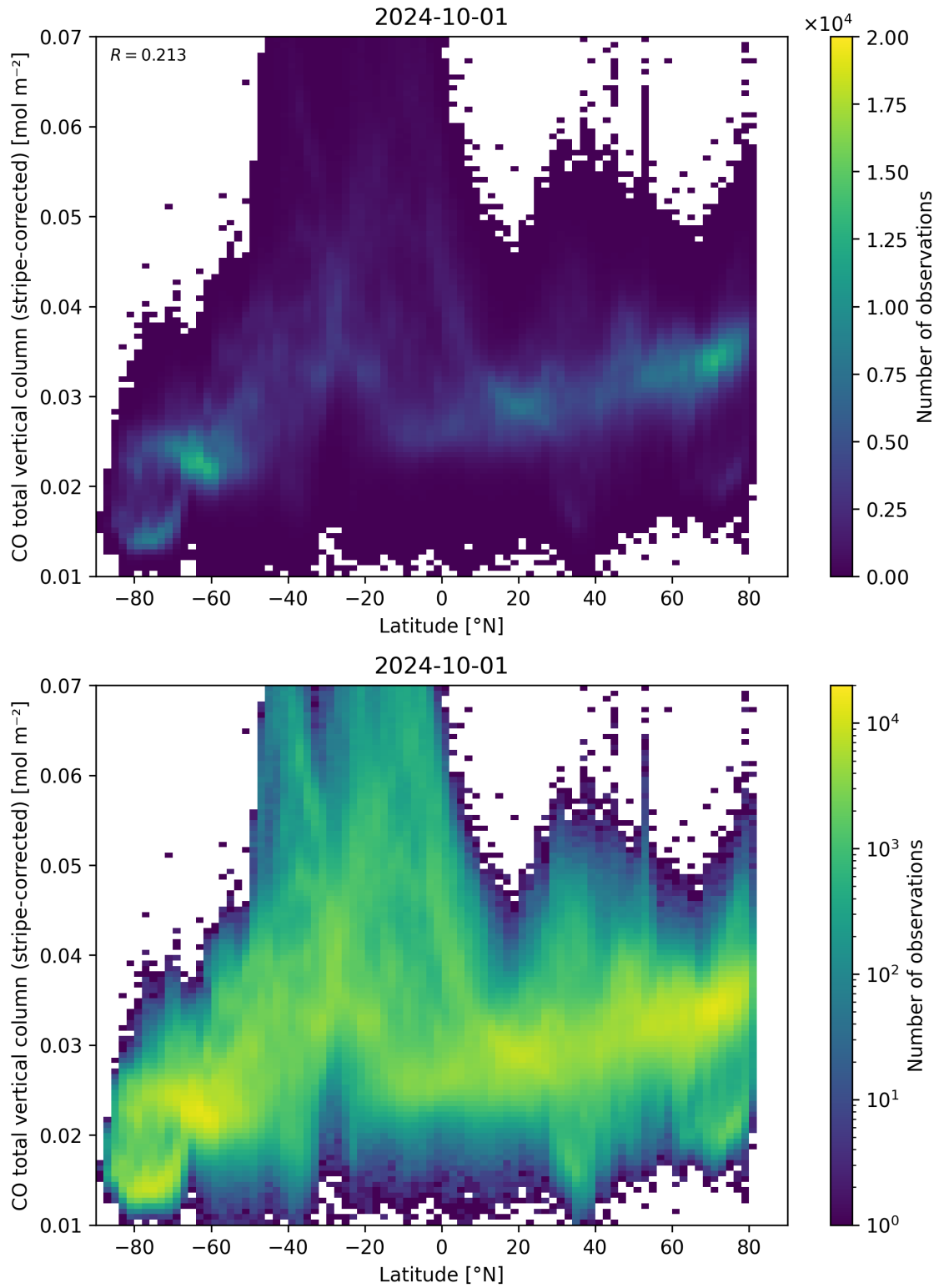
Figure 52: Scatter density plot of “Latitude” against “CO total vertical column (stripe-corrected)” for 2024-09-30 to 2024-10-02.
