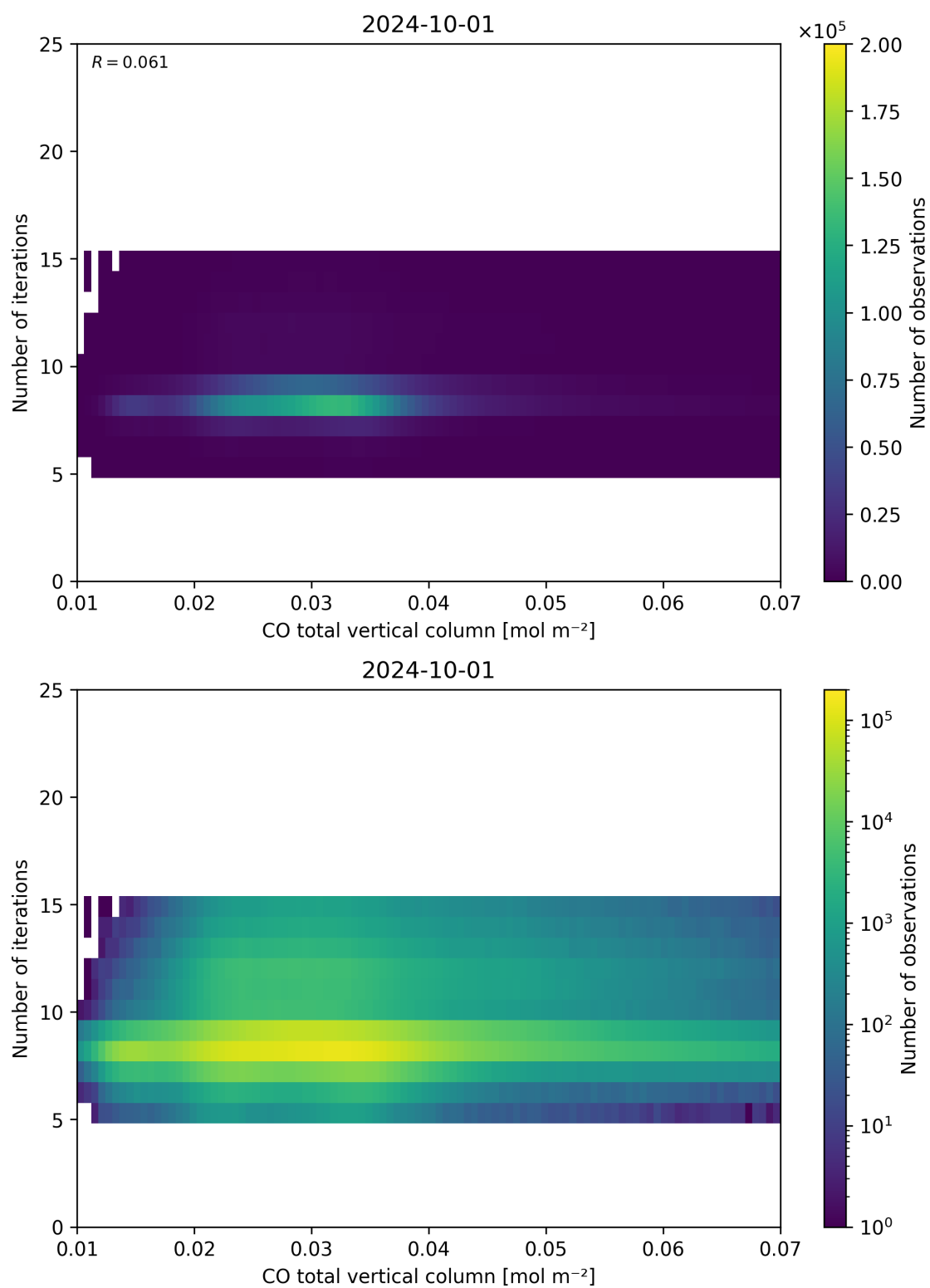
Figure 42: Scatter density plot of “CO total vertical column” against “Number of iterations” for 2024-09-30 to 2024-10-02.
