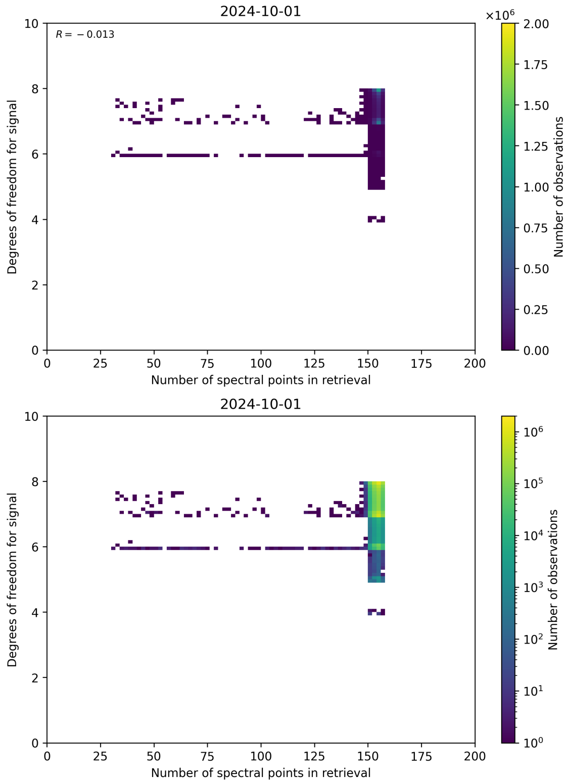
Figure 59: Scatter density plot of “Number of spectral points in retrieval” against “Degrees of freedom for signal” for 2024-09-30 to 2024-10-02.
