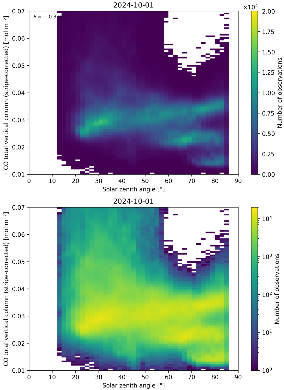
Figure 62: Scatter density plot of “Solar zenith angle” against “CO total vertical column (stripe-corrected)” for 2024-09-30 to 2024-10-02.
