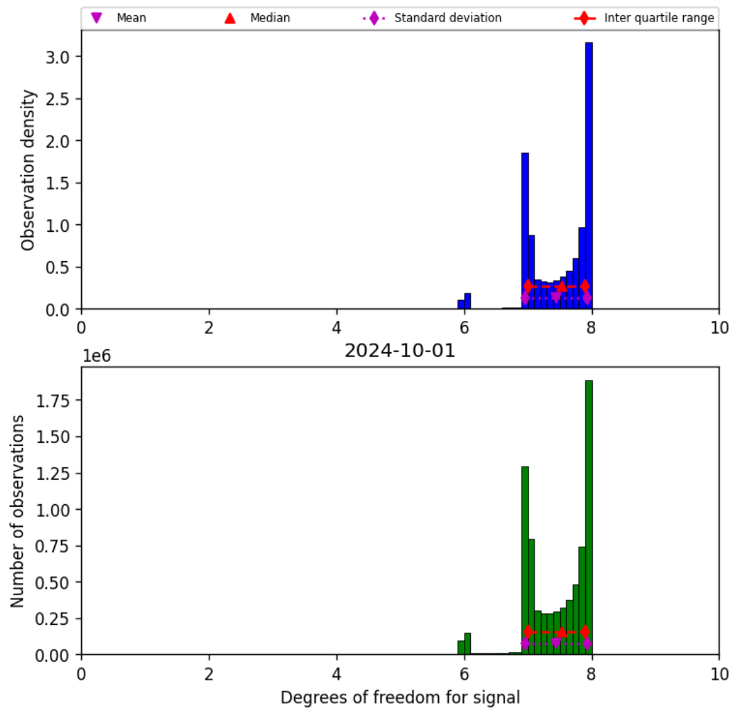
Figure 23: Histogram of “Degrees of freedom for signal” for 2024-09-30 to 2024-10-02
