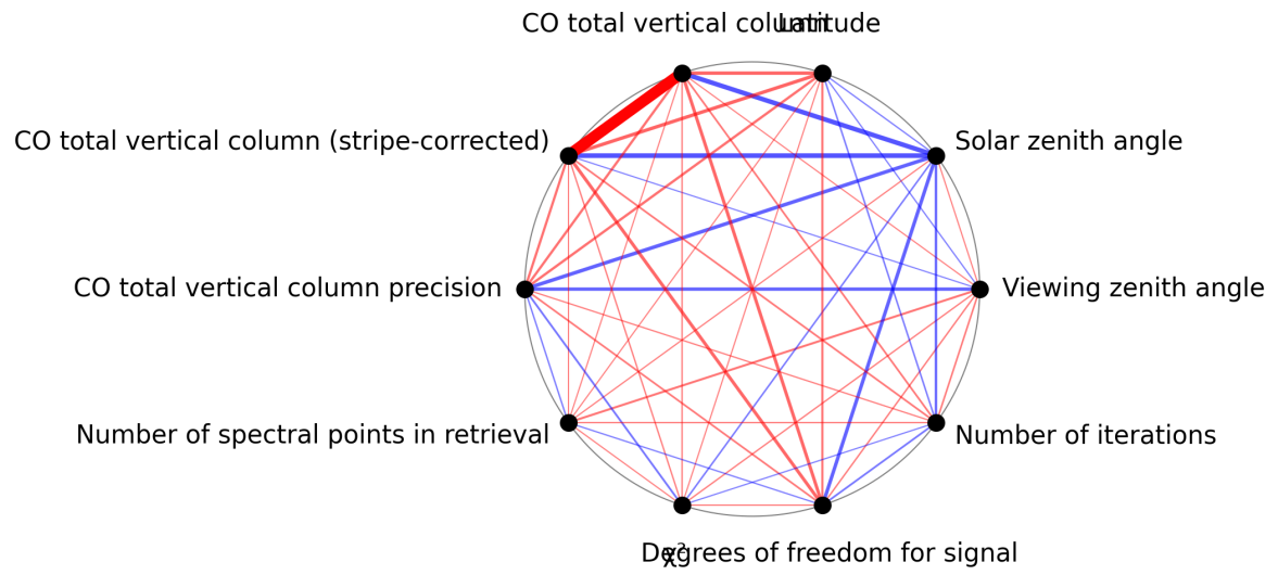
Figure 1: Map of correlation graph for 2024-09-30 to 2024-10-02.
