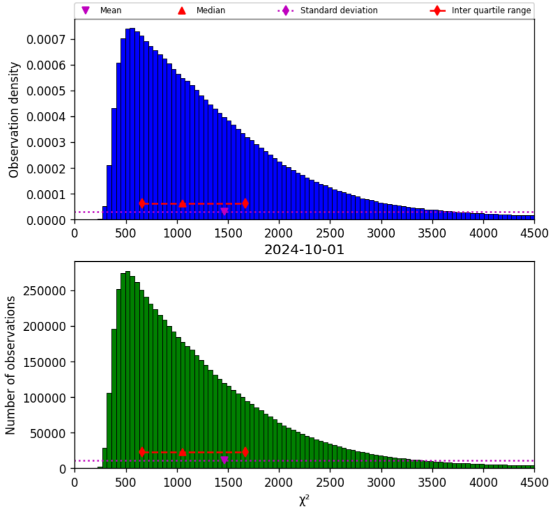
Figure 22: Histogram of “ \chi^2 ” for 2024-09-30 to 2024-10-02
