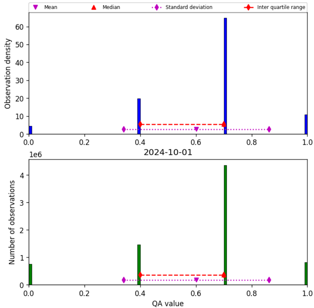
Figure 17: Histogram of “QA value” for 2024-09-30 to 2024-10-02
