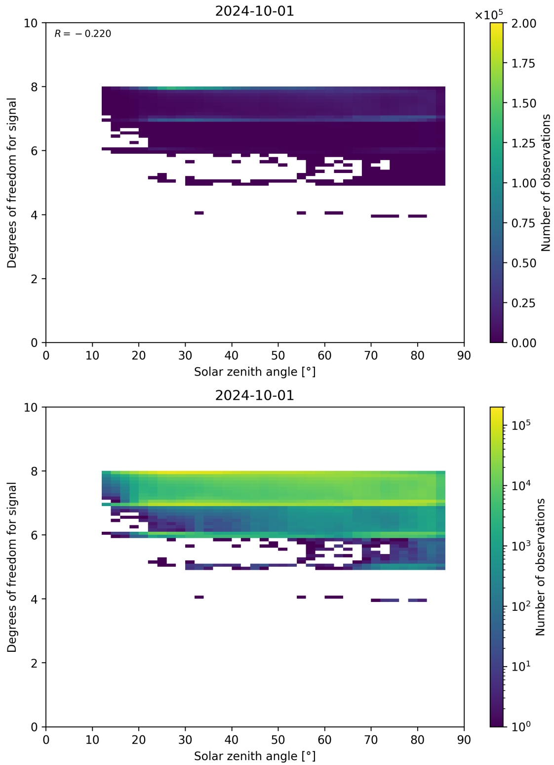
Figure 65: Scatter density plot of “Solar zenith angle” against “Degrees of freedom for signal” for 2024-09-30 to 2024-10-02.
