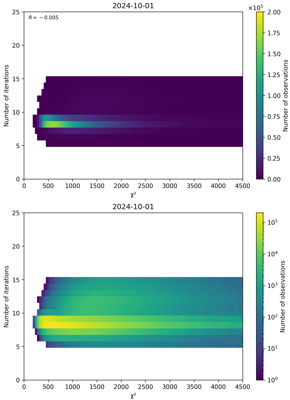
Figure 49: Scatter density plot of “ \chi^2 ” against “Number of iterations” for 2024-09-30 to 2024-10-02.
