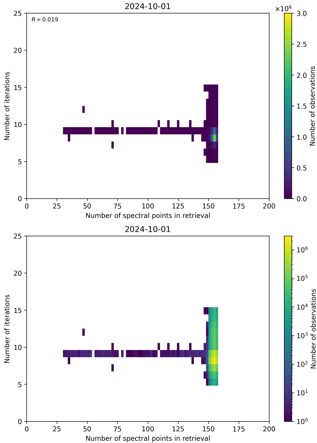
Figure 60: Scatter density plot of “Number of spectral points in retrieval” against “Number of iterations” for 2024-09-30 to 2024-10-02.
