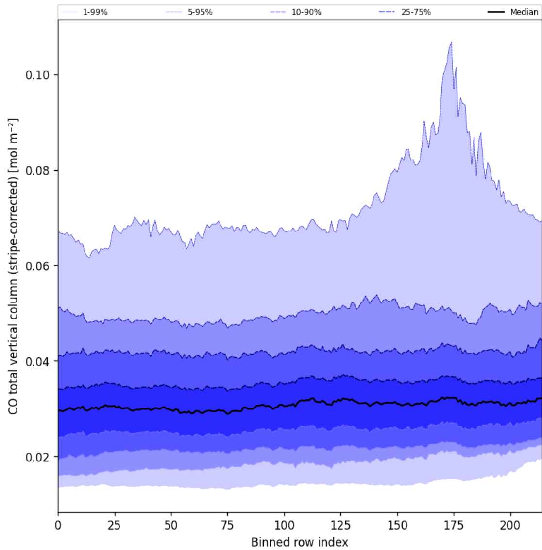
Figure 27: Along track statistics of “CO total vertical column (stripe-corrected)” for 2024-09-30 to 2024-10-02
