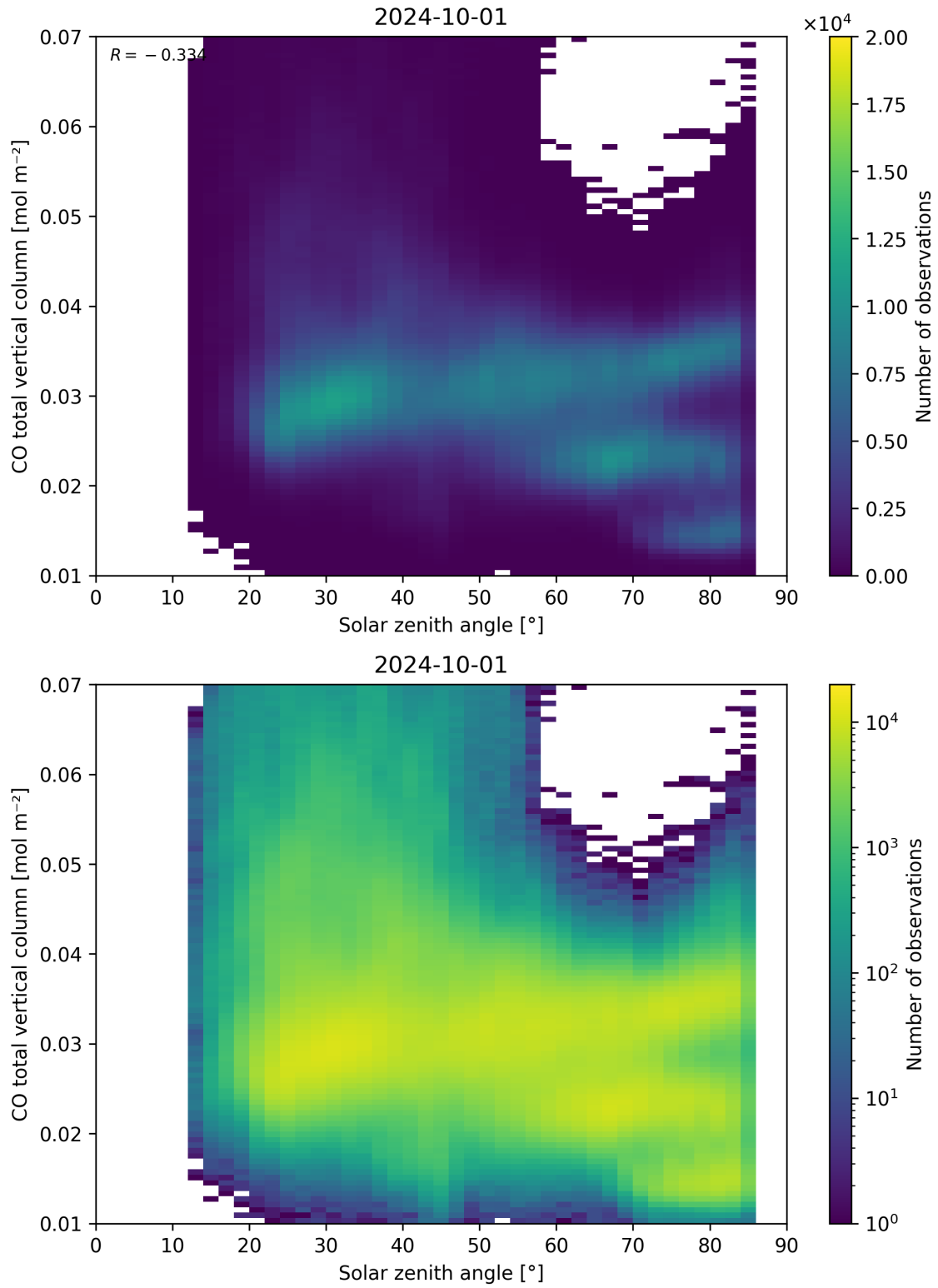
Figure 61: Scatter density plot of “Solar zenith angle” against “CO total vertical column” for 2024-09-30 to 2024-10-02.
