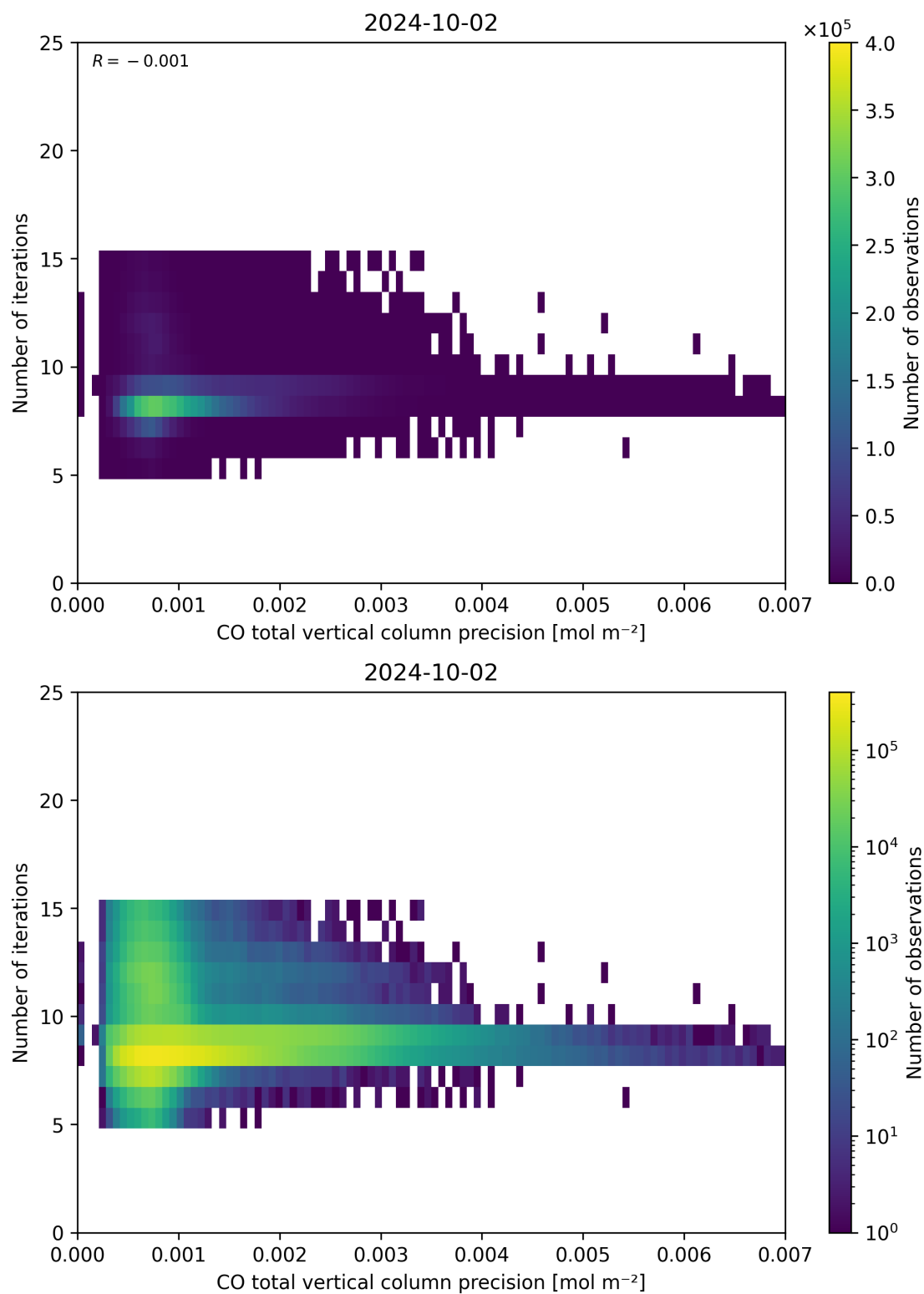
Figure 46: Scatter density plot of “CO total vertical column precision” against “Number of iterations” for 2024-10-01 to 2024-10-03.
