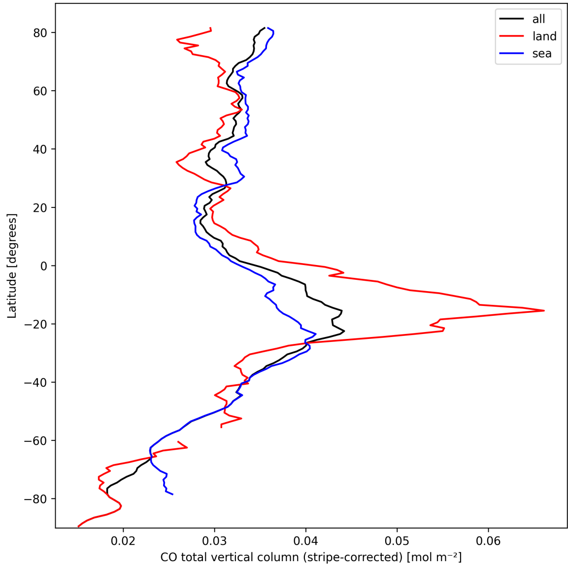
Figure 11: Zonal average of “CO total vertical column (stripe-corrected)” for 2024-10-01 to 2024-10-03.
