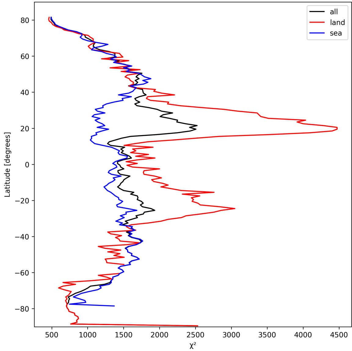
Figure 14: Zonal average of “ \chi^2 ” for 2024-10-01 to 2024-10-03.
