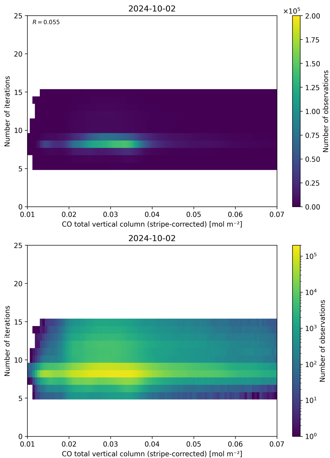
Figure 39: Scatter density plot of “CO total vertical column (stripe-corrected)” against “Number of iterations” for 2024-10-01 to 2024-10-03.
