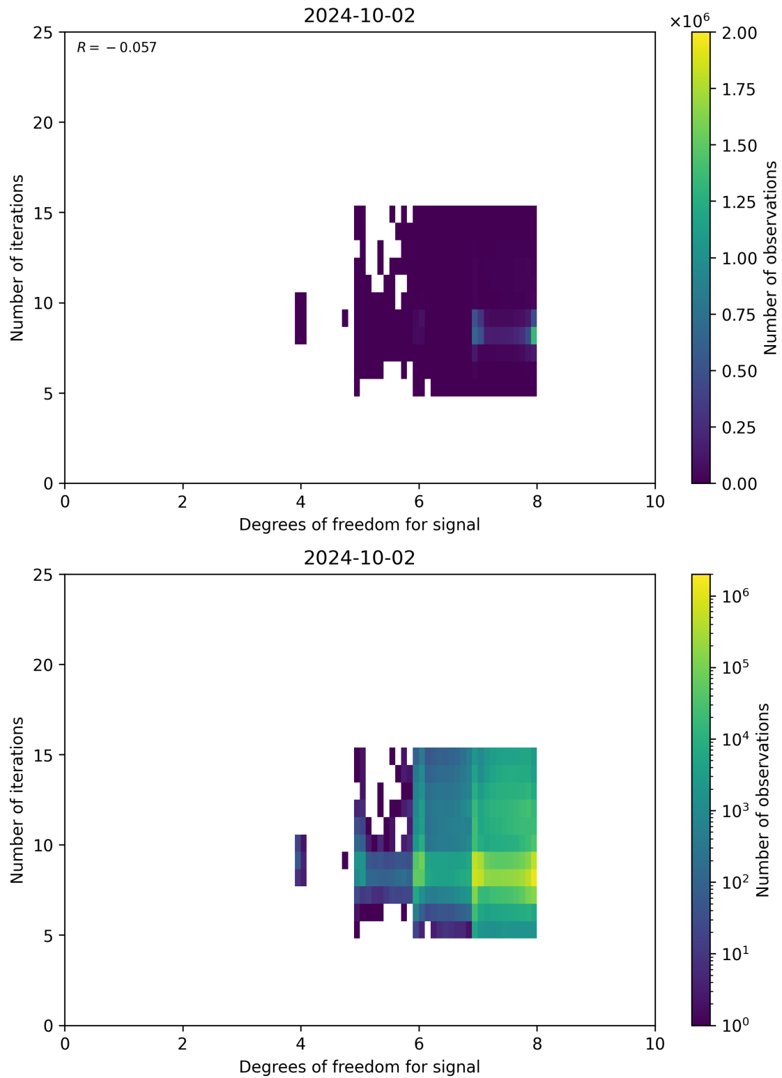
Figure 50: Scatter density plot of “Degrees of freedom for signal” against “Number of iterations” for 2024-10-01 to 2024-10-03.
