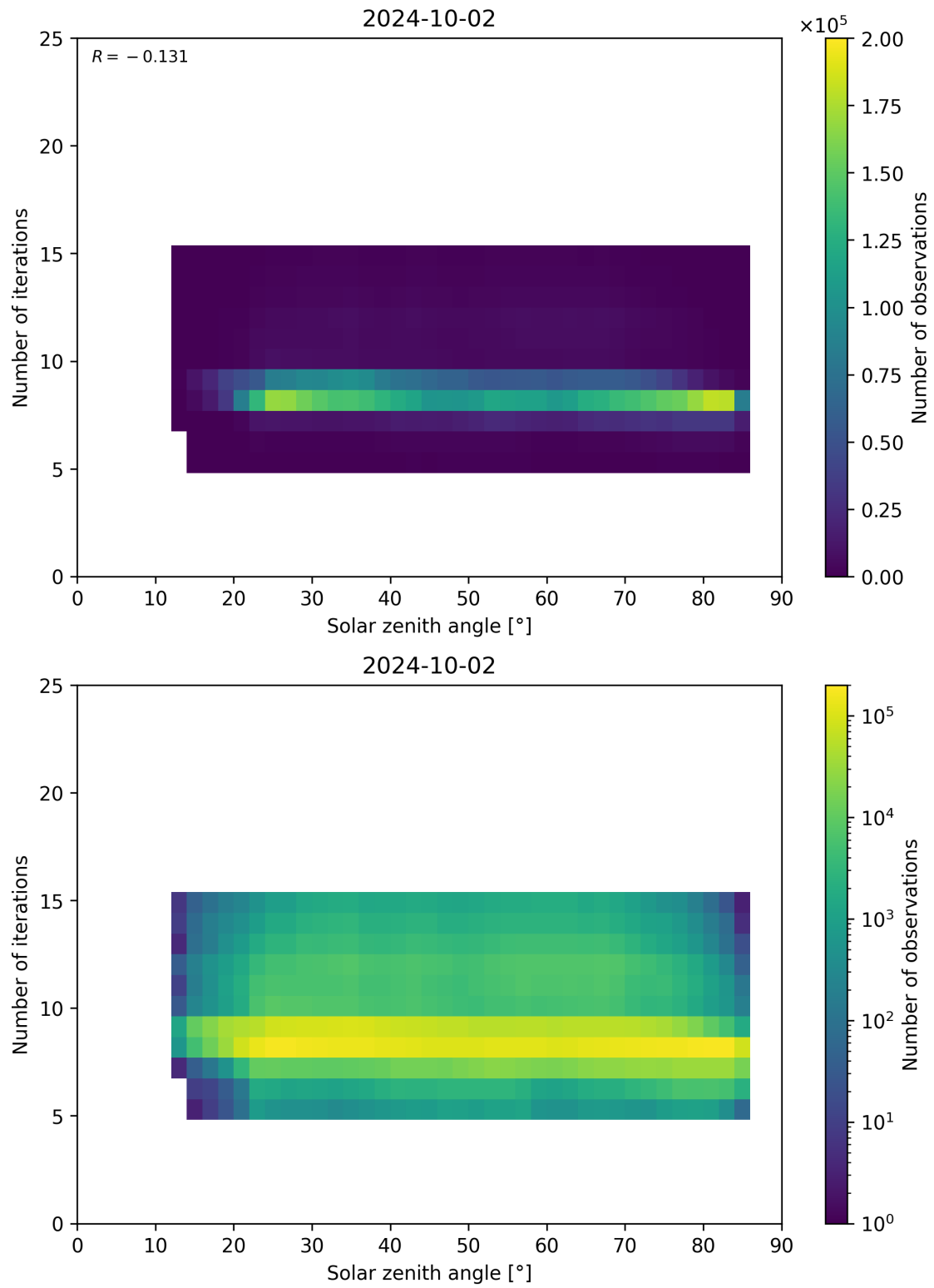
Figure 67: Scatter density plot of “Solar zenith angle” against “Number of iterations” for 2024-10-01 to 2024-10-03.
