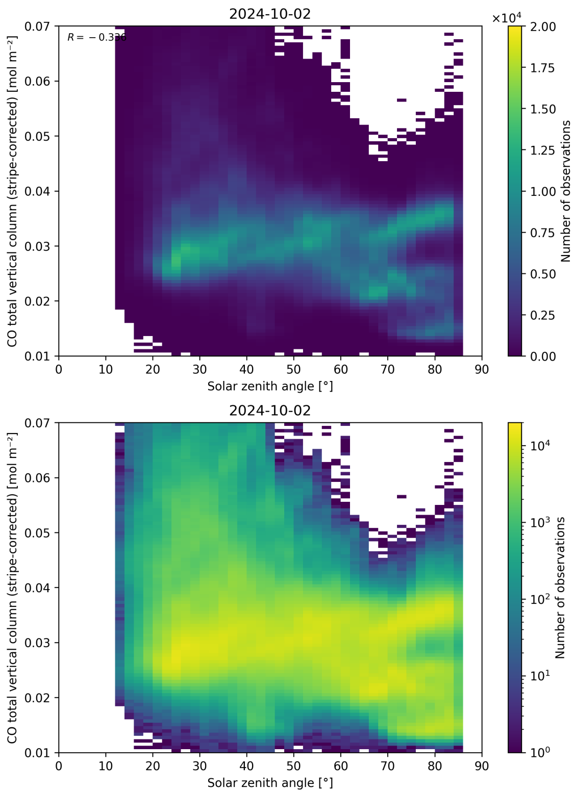
Figure 62: Scatter density plot of “Solar zenith angle” against “CO total vertical column (stripe-corrected)” for 2024-10-01 to 2024-10-03.
