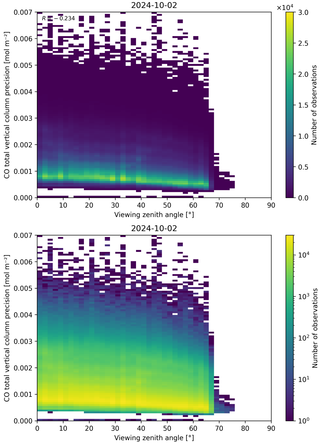
Figure 71: Scatter density plot of “Viewing zenith angle” against “CO total vertical column precision” for 2024-10-01 to 2024-10-03.
