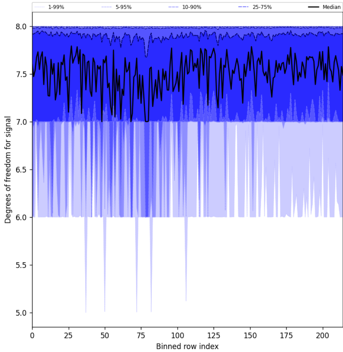
Figure 31: Along track statistics of “Degrees of freedom for signal” for 2024-10-01 to 2024-10-03
