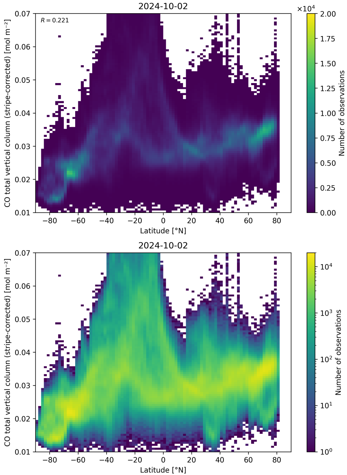
Figure 52: Scatter density plot of “Latitude” against “CO total vertical column (stripe-corrected)” for 2024-10-01 to 2024-10-03.
