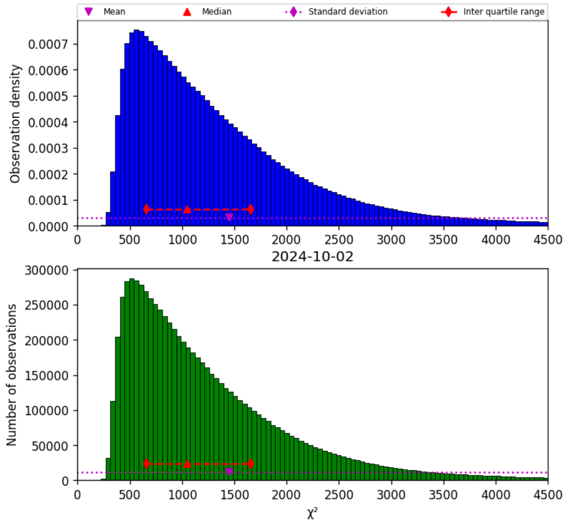
Figure 22: Histogram of " \chi^2 " for 2024-10-01 to 2024-10-03
