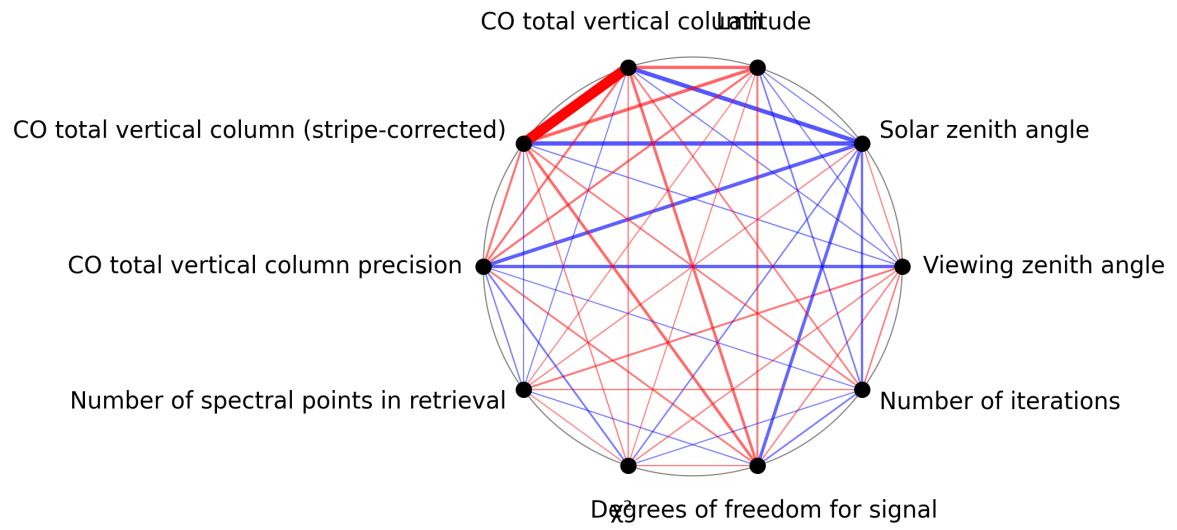
Figure 1: Map of correlation graph for 2024-10-01 to 2024-10-03.
