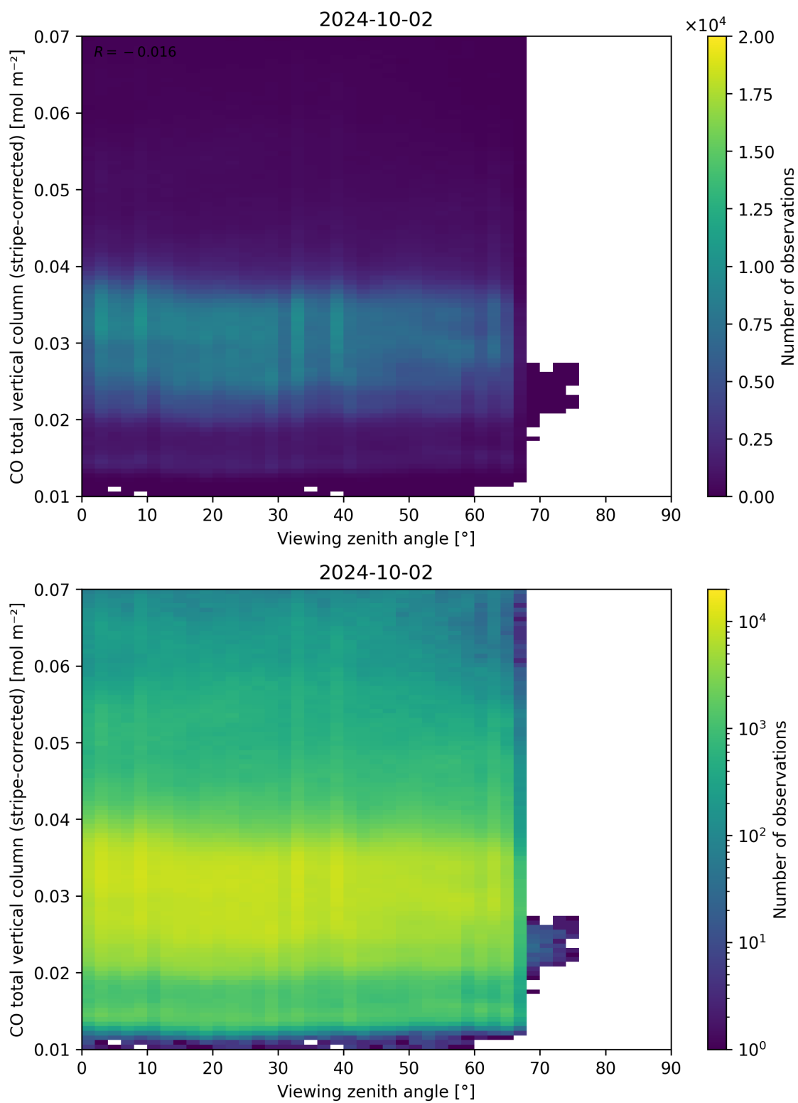
Figure 70: Scatter density plot of “Viewing zenith angle” against “CO total vertical column (stripe-corrected)” for 2024-10-01 to 2024-10-03.
