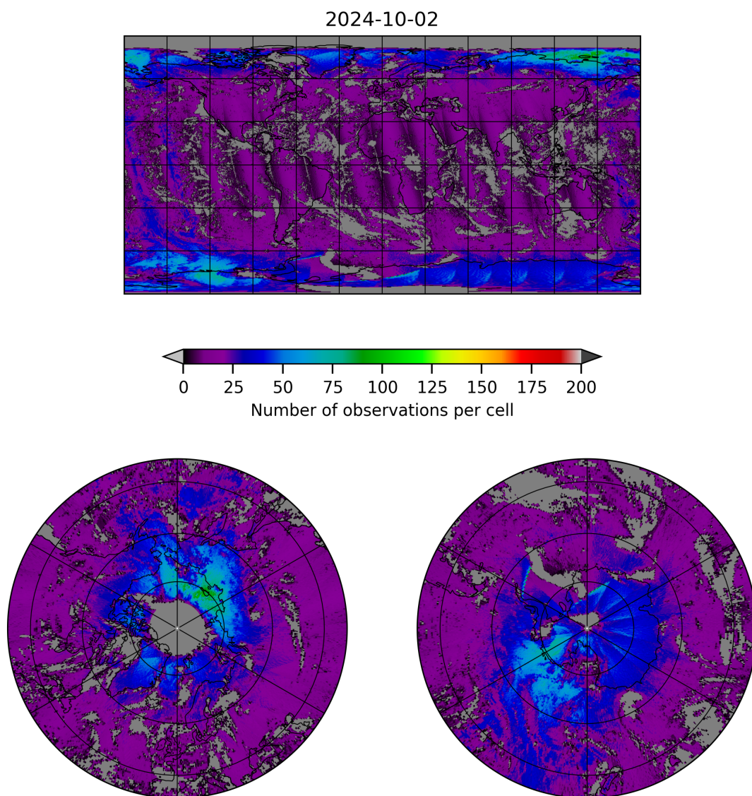
Figure 8: Map of the number of observations for 2024-10-01 to 2024-10-03
