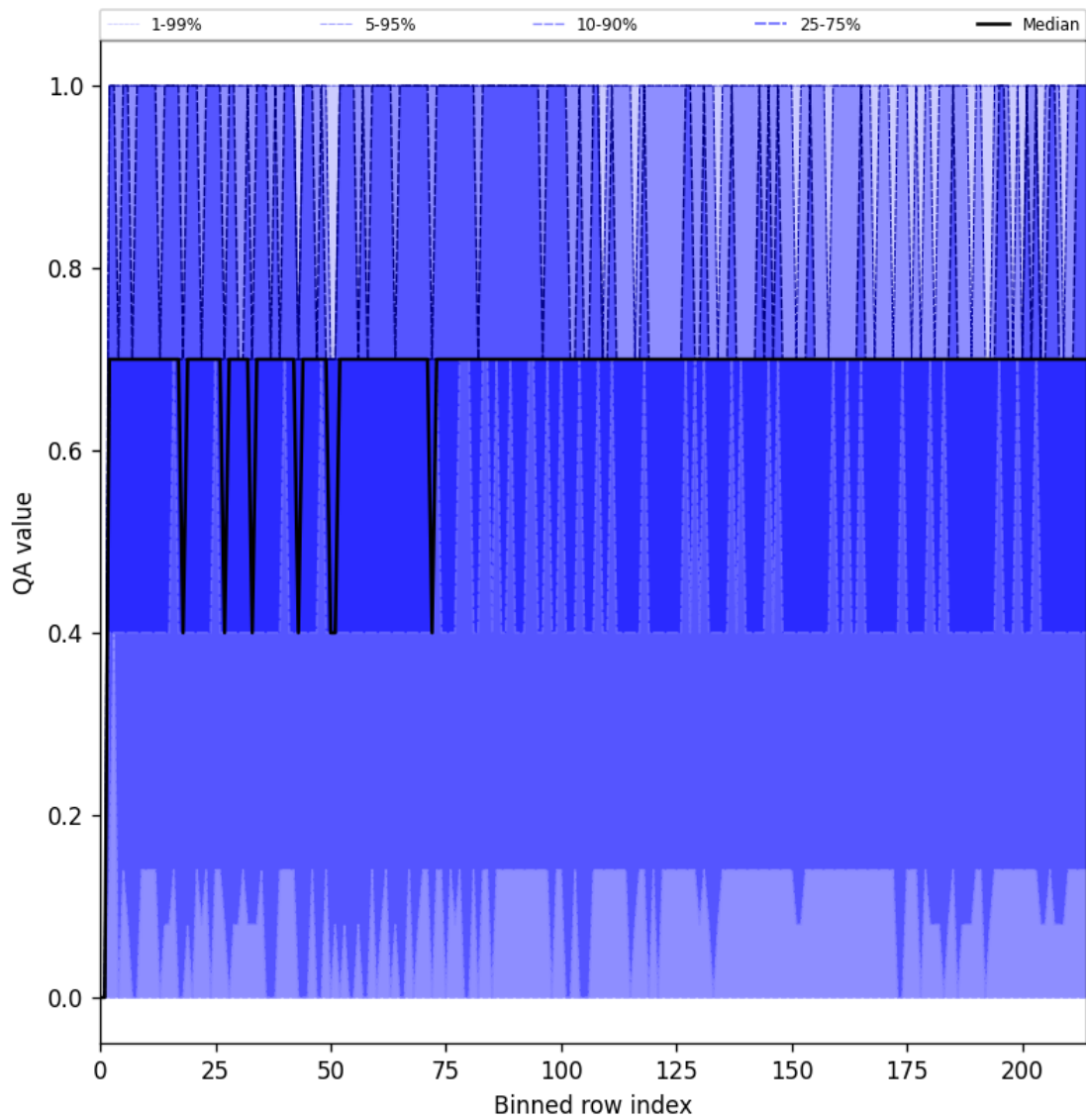
Figure 25: Along track statistics of “QA value” for 2024-10-01 to 2024-10-03
