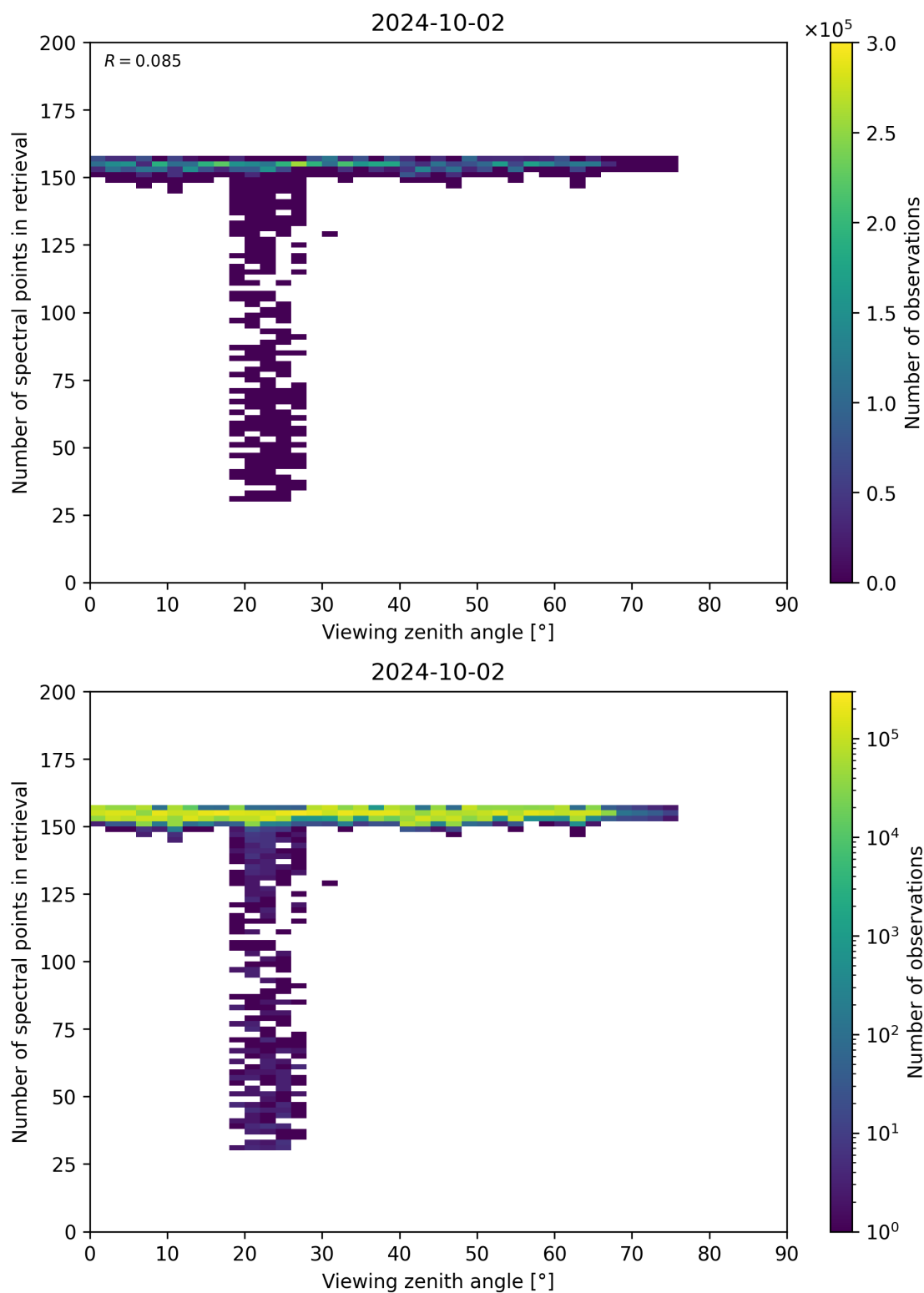
Figure 76: Scatter density plot of “Viewing zenith angle” against “Number of spectral points in retrieval” for 2024-10-01 to 2024-10-03.
