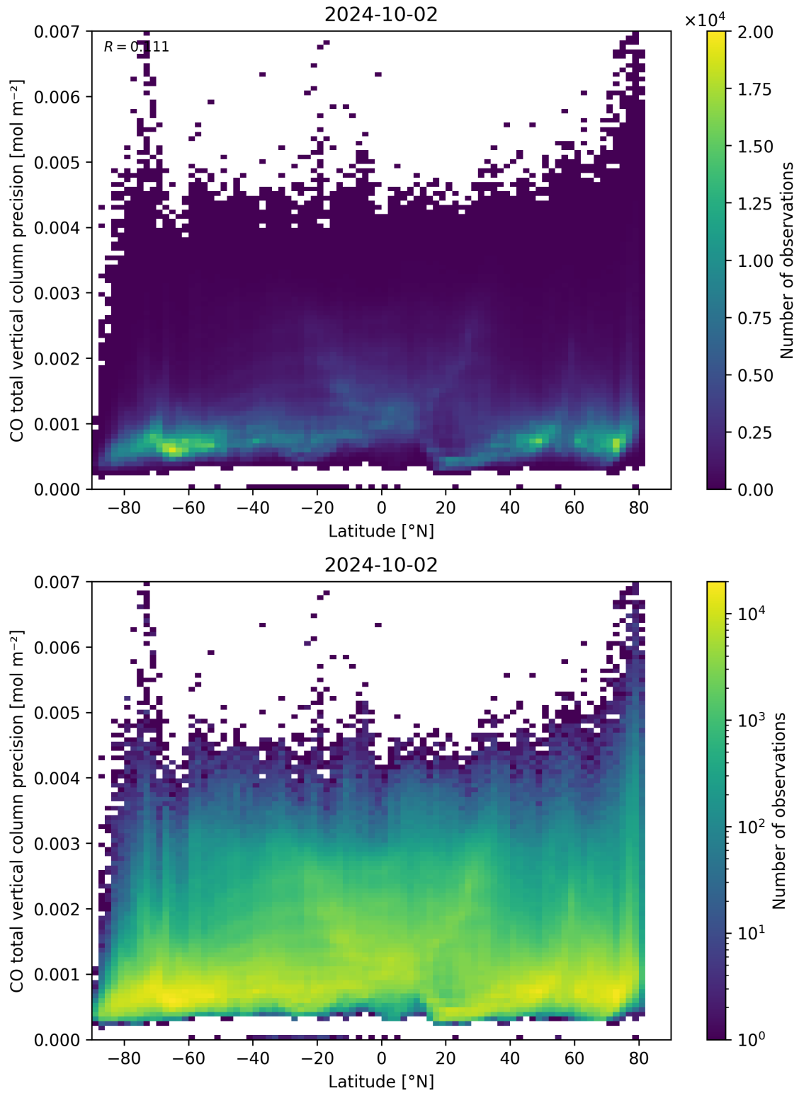
Figure 53: Scatter density plot of “Latitude” against “CO total vertical column precision” for 2024-10-01 to 2024-10-03.
