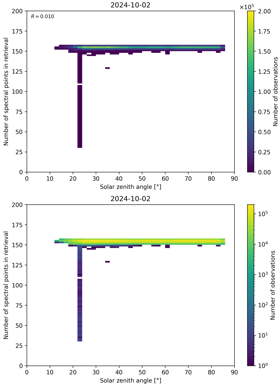
Figure 68: Scatter density plot of “Solar zenith angle” against “Number of spectral points in retrieval” for 2024-10-01 to 2024-10-03.
