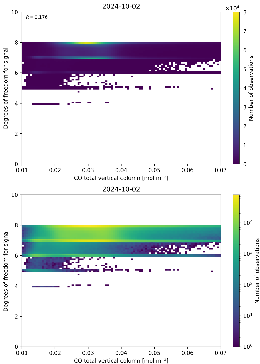
Figure 41: Scatter density plot of “CO total vertical column” against “Degrees of freedom for signal” for 2024-10-01 to 2024-10-03.
