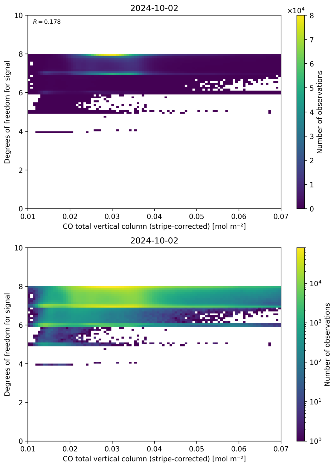
Figure 38: Scatter density plot of “CO total vertical column (stripe-corrected)” against “Degrees of freedom for signal” for 2024-10-01 to 2024-10-03.
