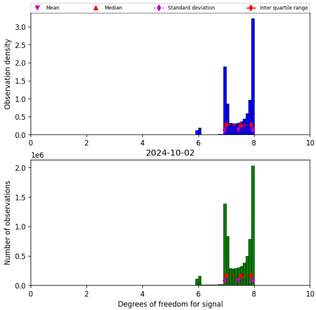
Figure 23: Histogram of “Degrees of freedom for signal” for 2024-10-01 to 2024-10-03
