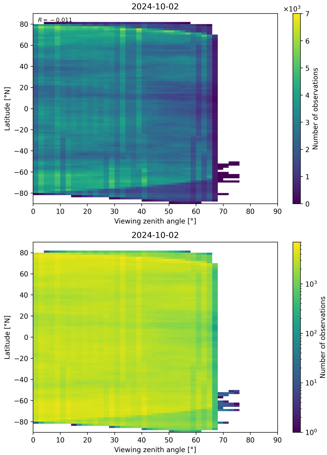
Figure 74: Scatter density plot of “Viewing zenith angle” against “Latitude” for 2024-10-01 to 2024-10-03.
