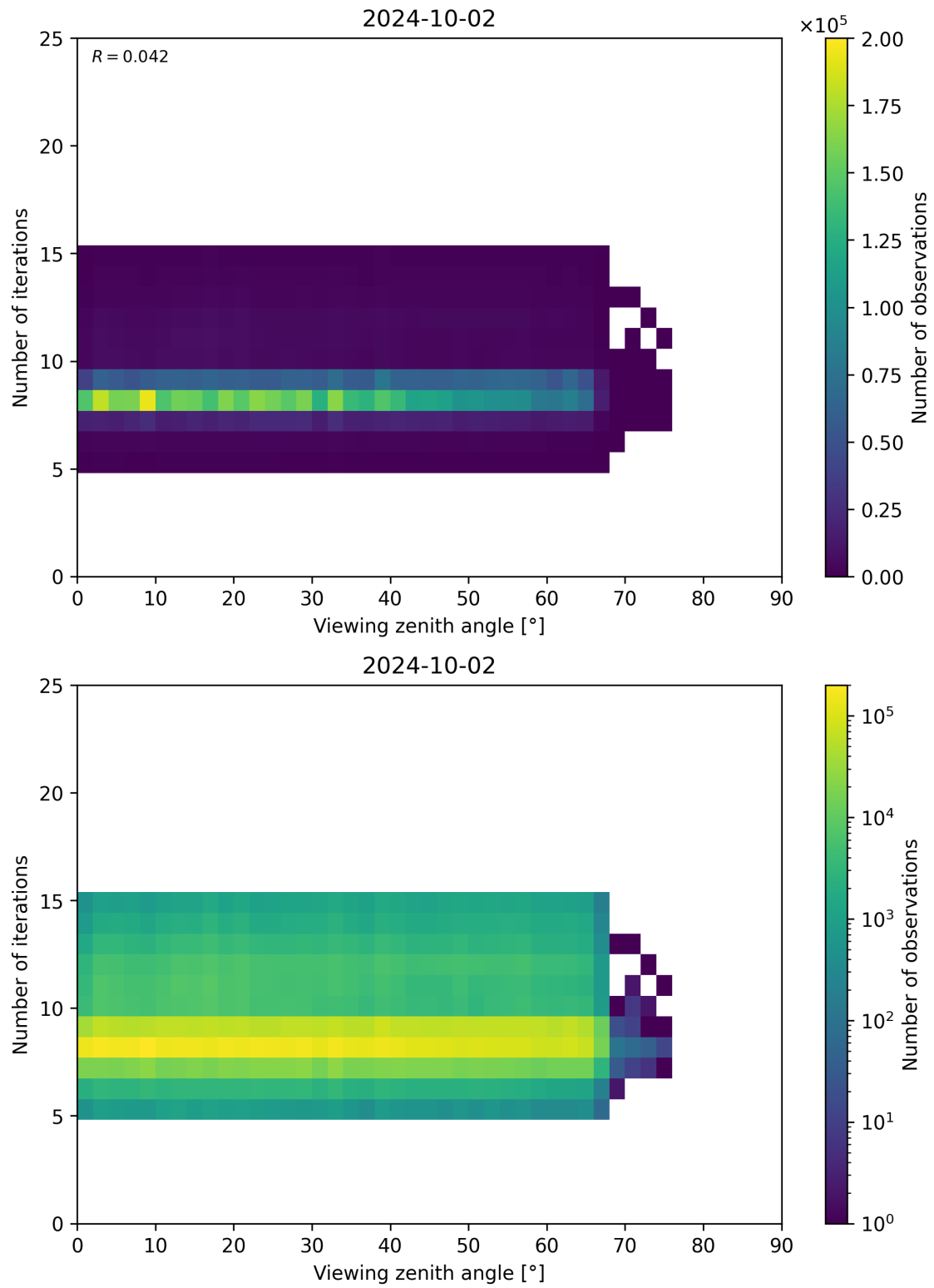
Figure 75: Scatter density plot of “Viewing zenith angle” against “Number of iterations” for 2024-10-01 to 2024-10-03.
