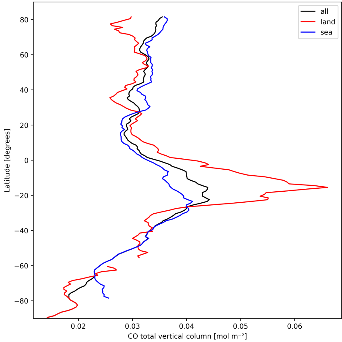
Figure 10: Zonal average of “CO total vertical column” for 2024-10-01 to 2024-10-03.
