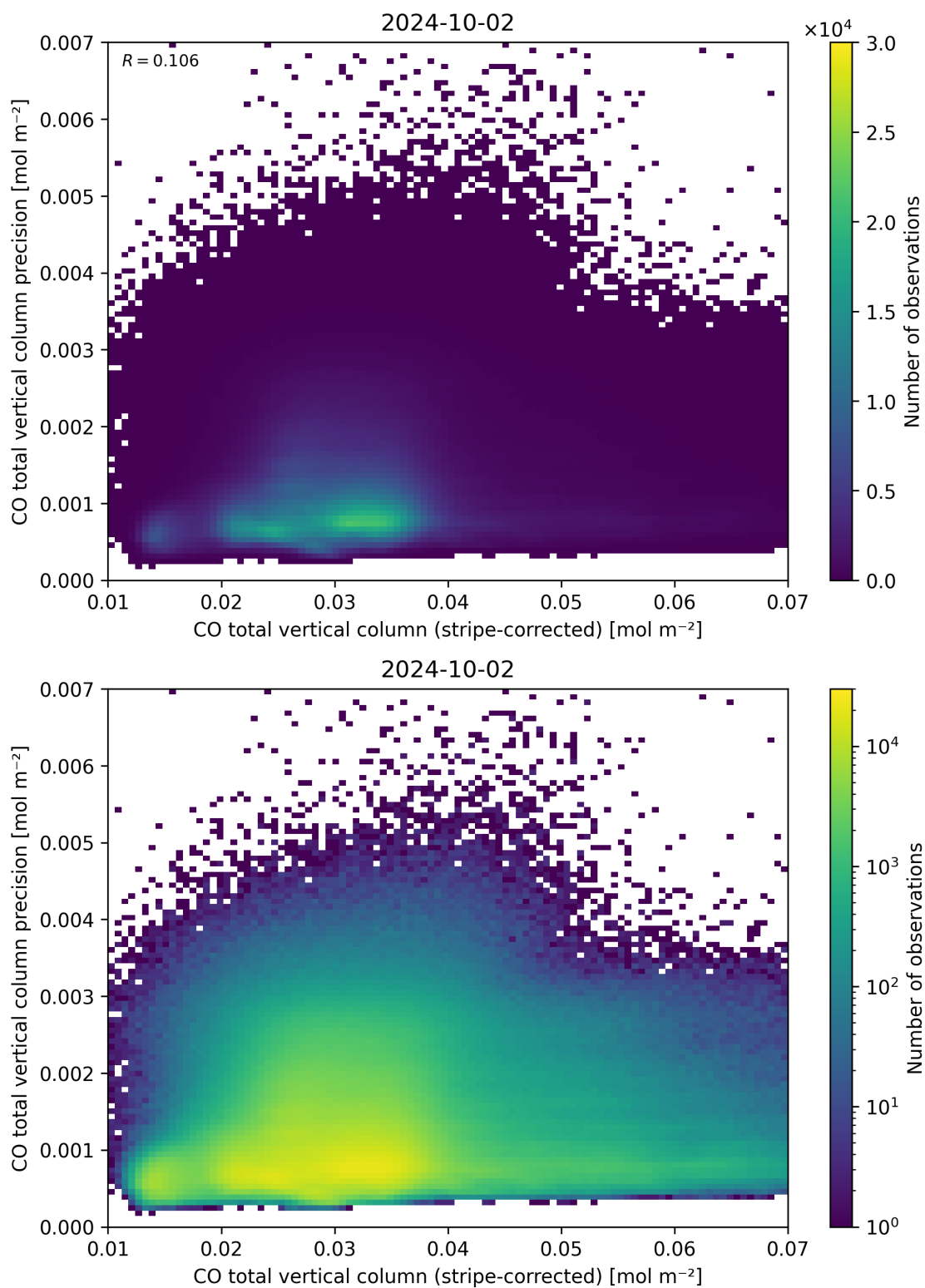
Figure 36: Scatter density plot of “CO total vertical column (stripe-corrected)” against “CO total vertical column precision” for 2024-10-01 to 2024-10-03.
