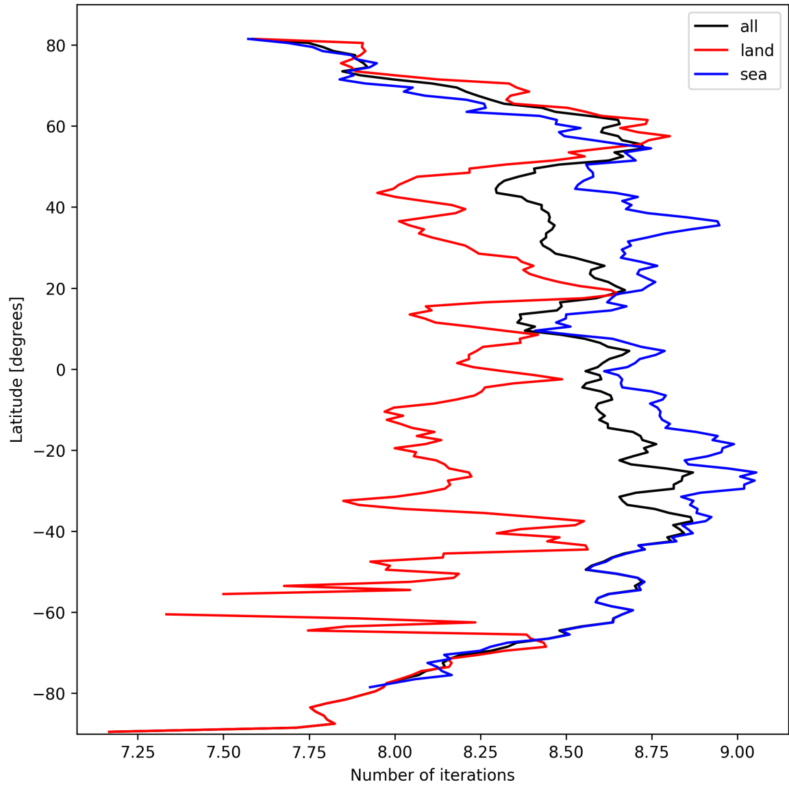
Figure 16: Zonal average of “Number of iterations” for 2024-10-01 to 2024-10-03.
