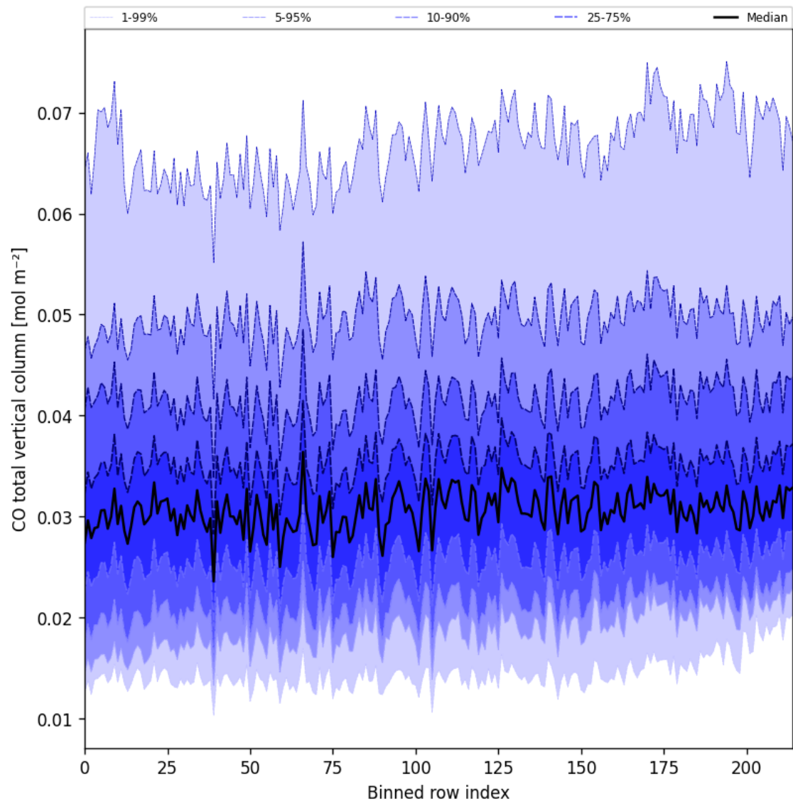
Figure 26: Along track statistics of “CO total vertical column” for 2024-10-01 to 2024-10-03
