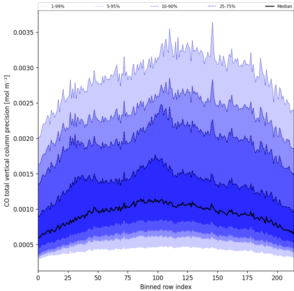
Figure 28: Along track statistics of “CO total vertical column precision” for 2024-10-01 to 2024-10-03
