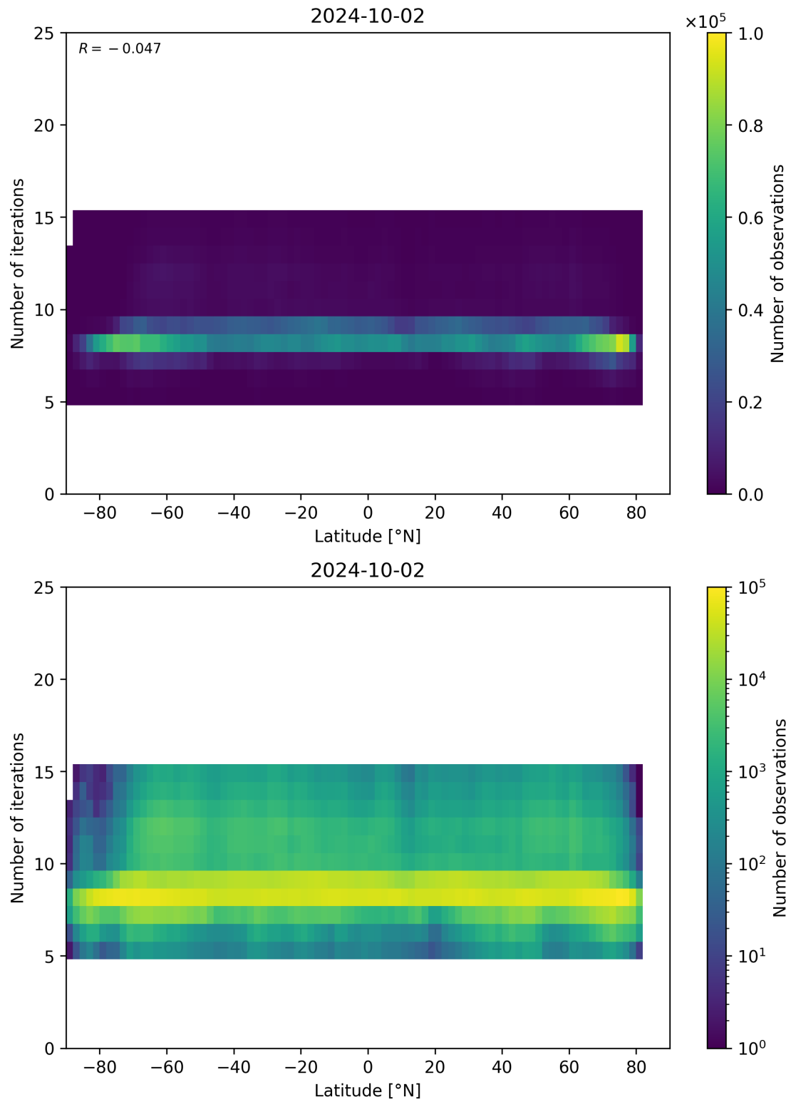
Figure 56: Scatter density plot of “Latitude” against “Number of iterations” for 2024-10-01 to 2024-10-03.
