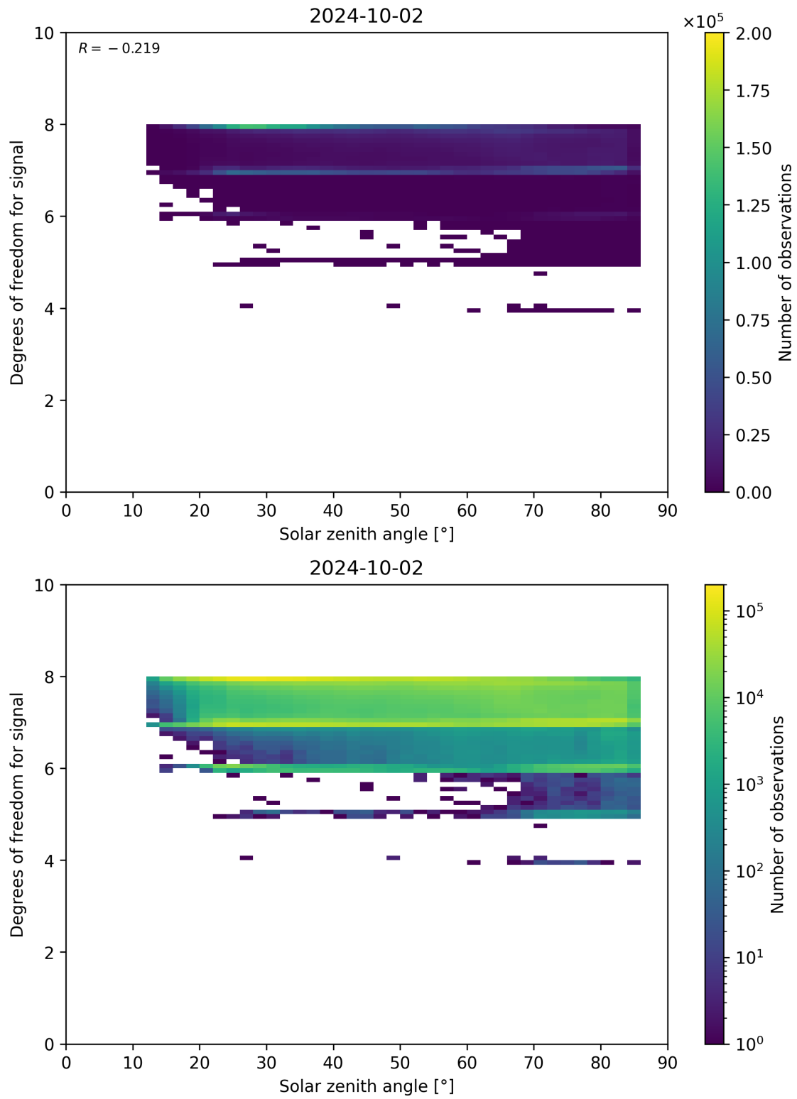
Figure 65: Scatter density plot of “Solar zenith angle” against “Degrees of freedom for signal” for 2024-10-01 to 2024-10-03.
