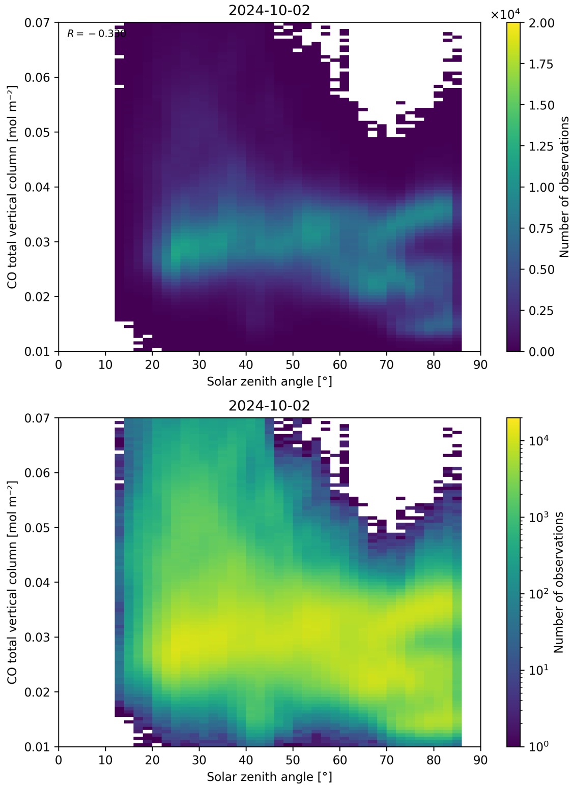
Figure 61: Scatter density plot of “Solar zenith angle” against “CO total vertical column” for 2024-10-01 to 2024-10-03.
