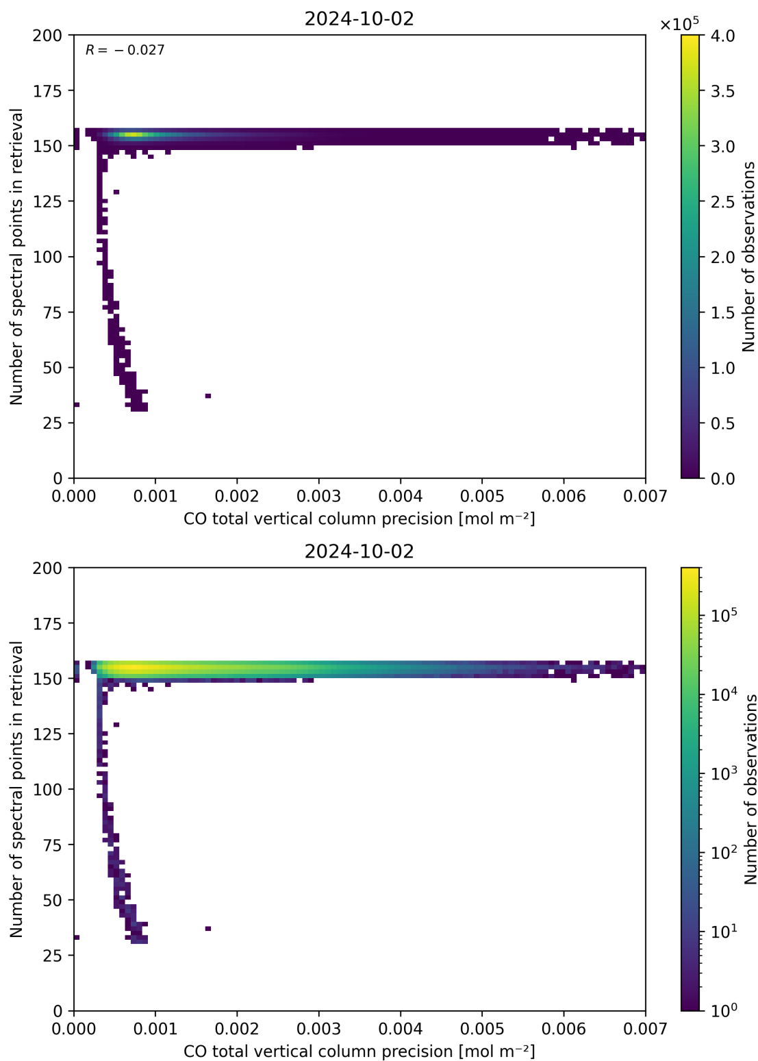
Figure 47: Scatter density plot of “CO total vertical column precision” against “Number of spectral points in retrieval” for 2024-10-01 to 2024-10-03.
