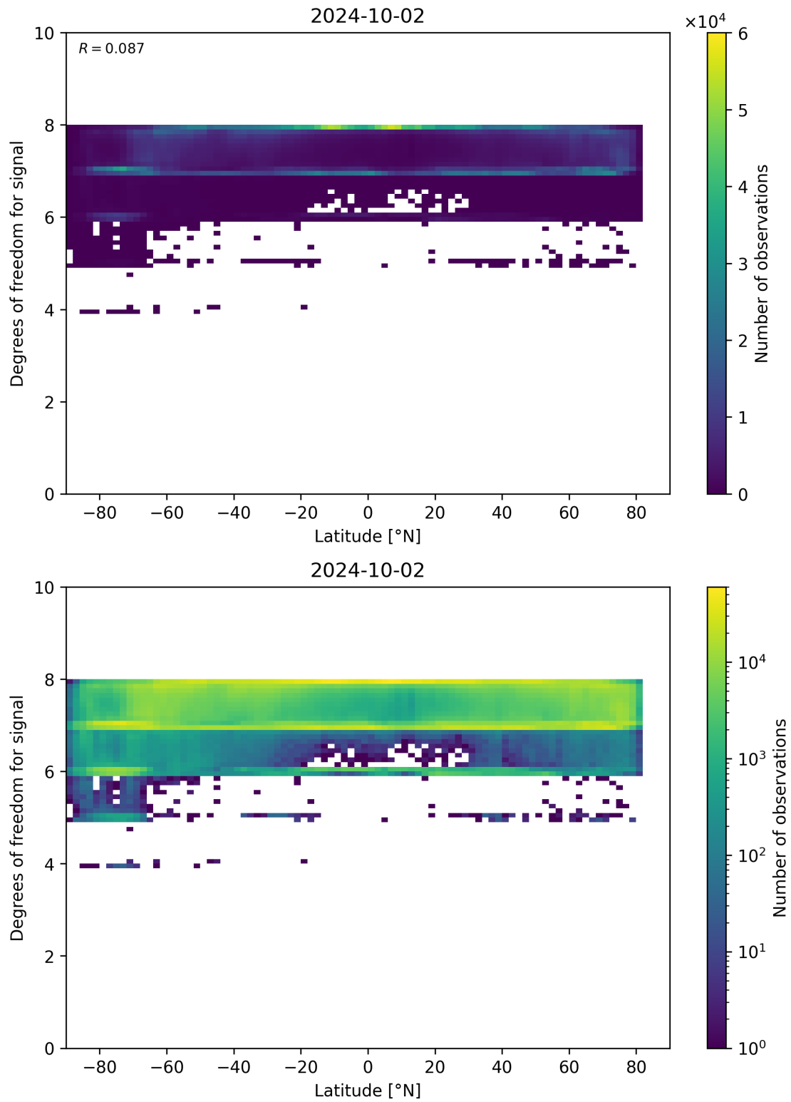
Figure 55: Scatter density plot of “Latitude” against “Degrees of freedom for signal” for 2024-10-01 to 2024-10-03.
