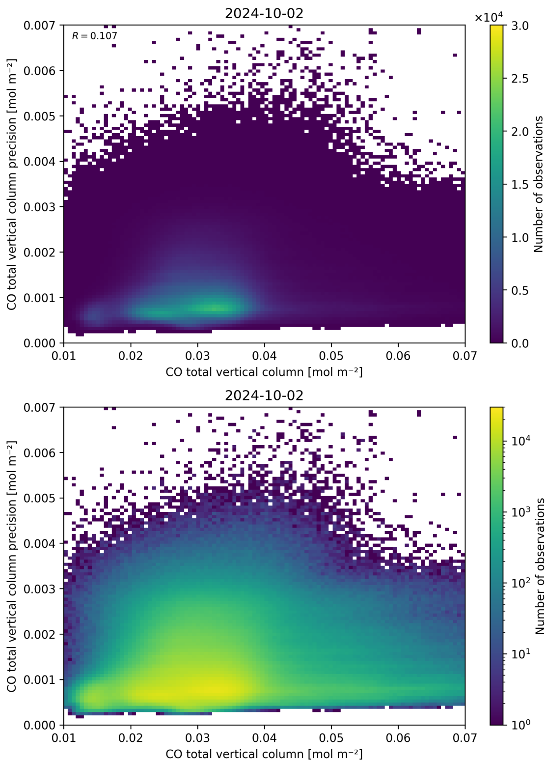
Figure 34: Scatter density plot of “CO total vertical column” against “CO total vertical column precision” for 2024-10-01 to 2024-10-03.
