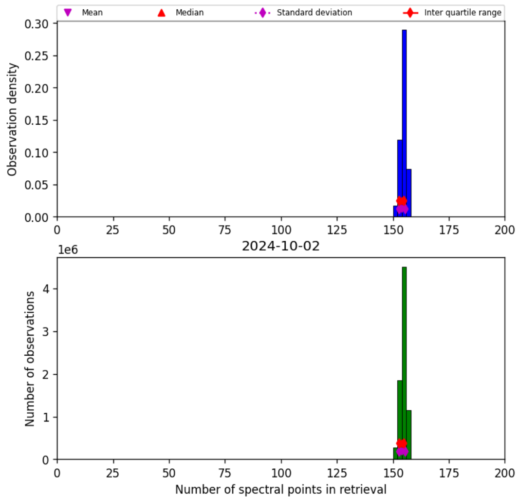
Figure 21: Histogram of “Number of spectral points in retrieval” for 2024-10-01 to 2024-10-03
