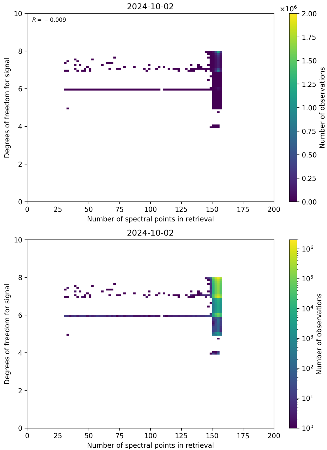
Figure 59: Scatter density plot of “Number of spectral points in retrieval” against “Degrees of freedom for signal” for 2024-10-01 to 2024-10-03.
