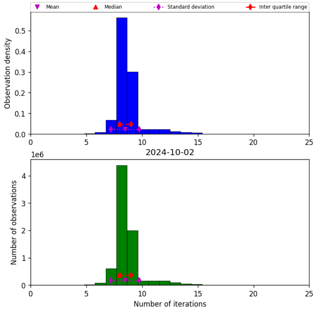
Figure 24: Histogram of “Number of iterations” for 2024-10-01 to 2024-10-03
