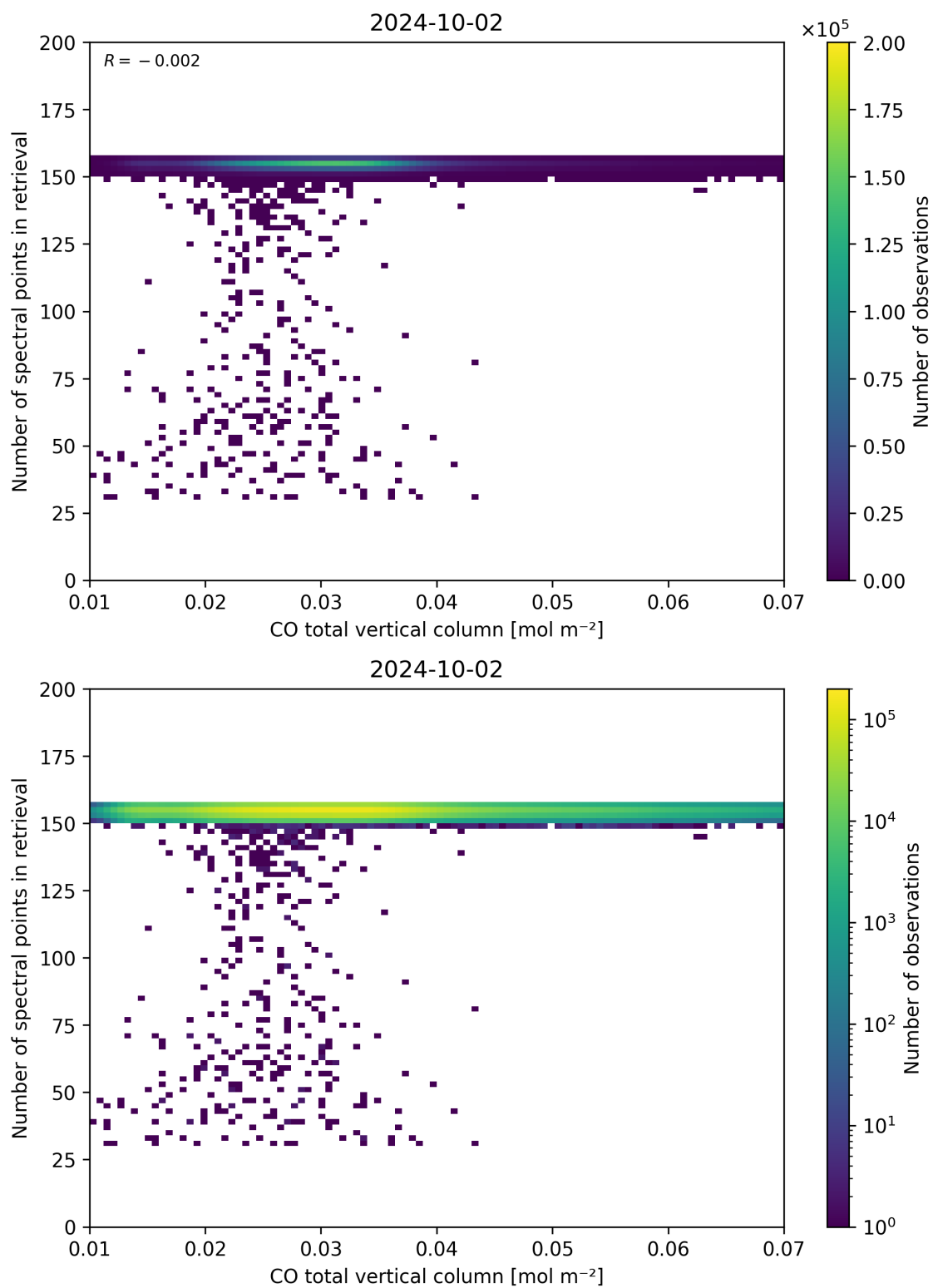
Figure 43: Scatter density plot of “CO total vertical column” against “Number of spectral points in retrieval” for 2024-10-01 to 2024-10-03.
