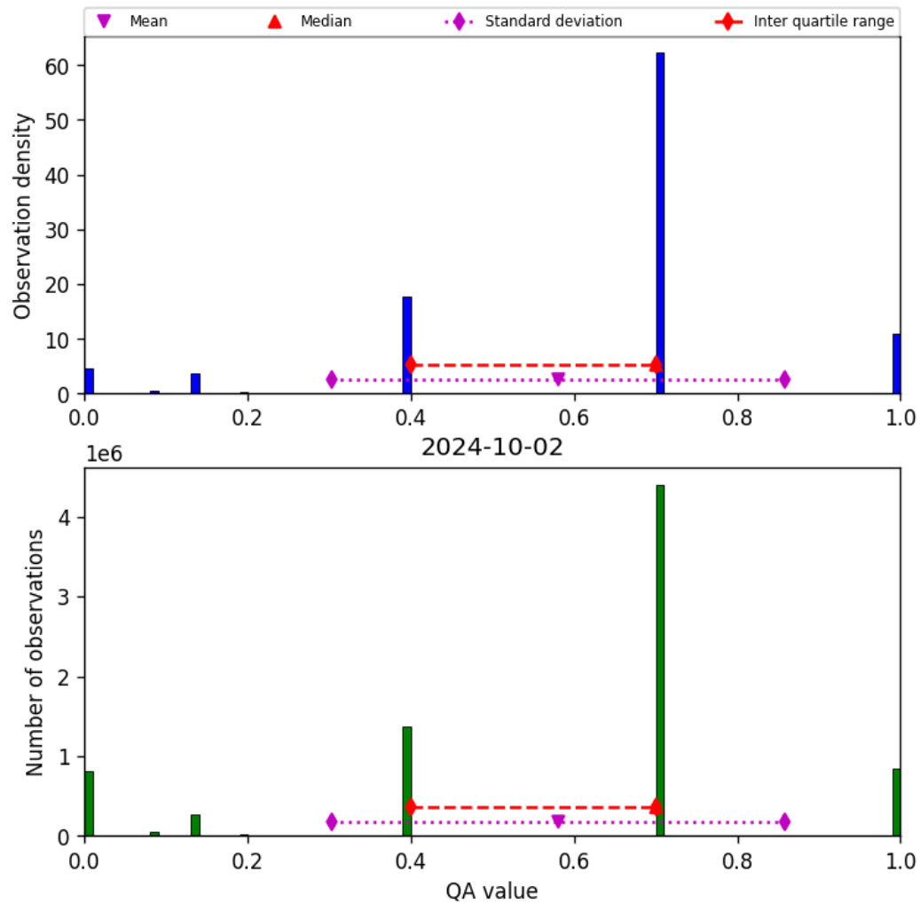
Figure 17: Histogram of “QA value” for 2024-10-01 to 2024-10-03
