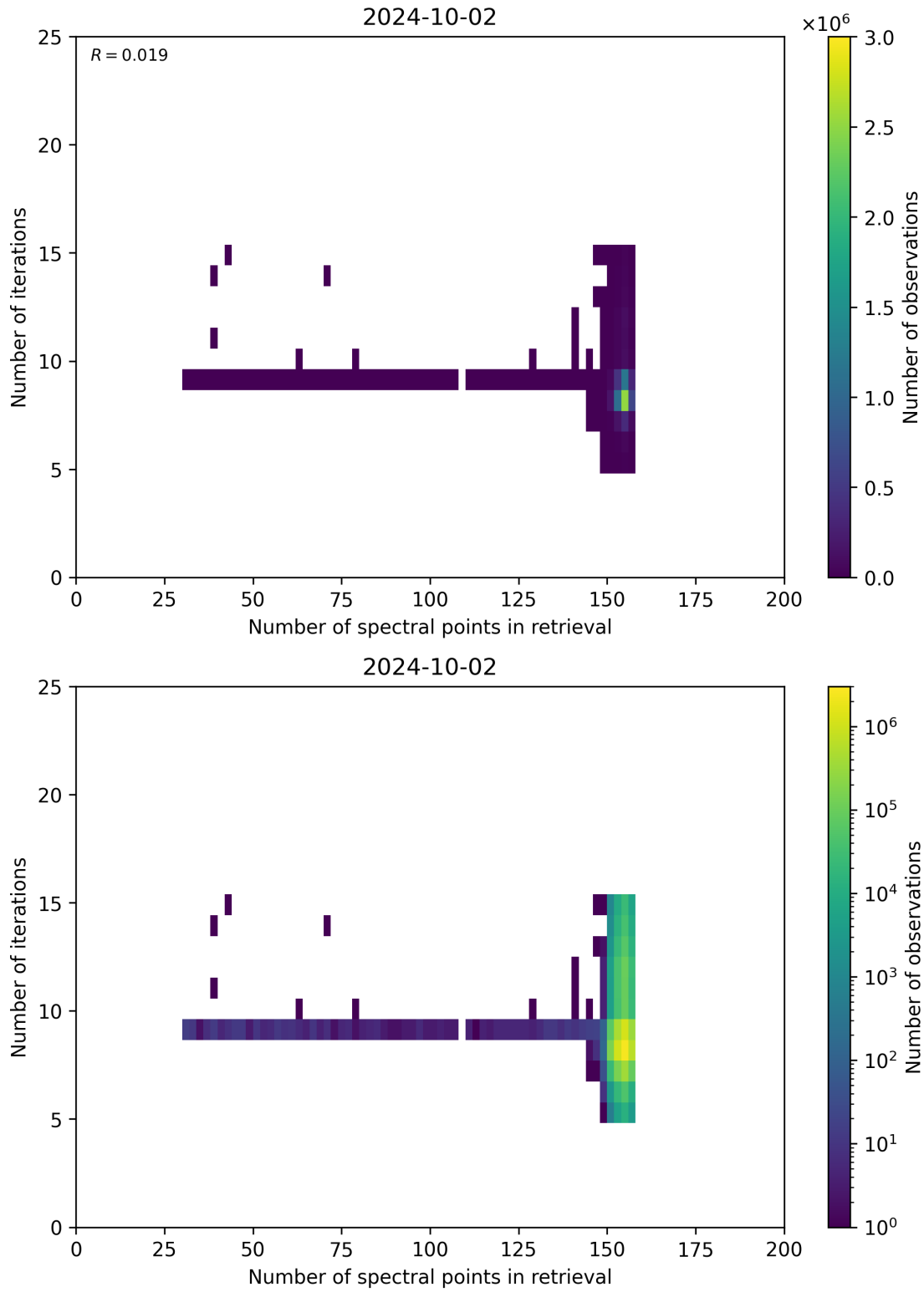
Figure 60: Scatter density plot of “Number of spectral points in retrieval” against “Number of iterations” for 2024-10-01 to 2024-10-03.
