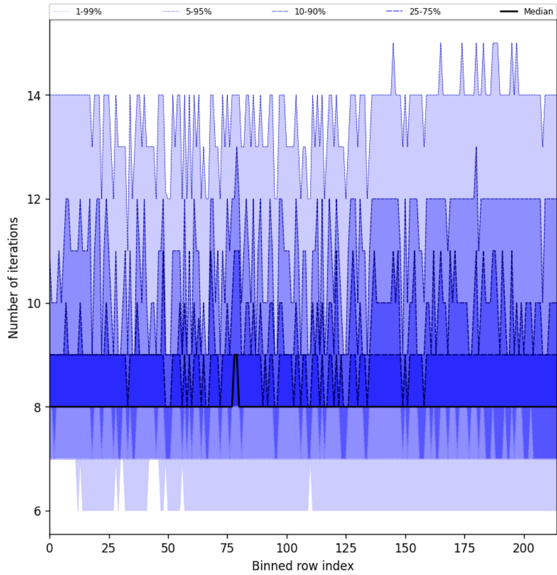
Figure 32: Along track statistics of “Number of iterations” for 2024-10-01 to 2024-10-03
