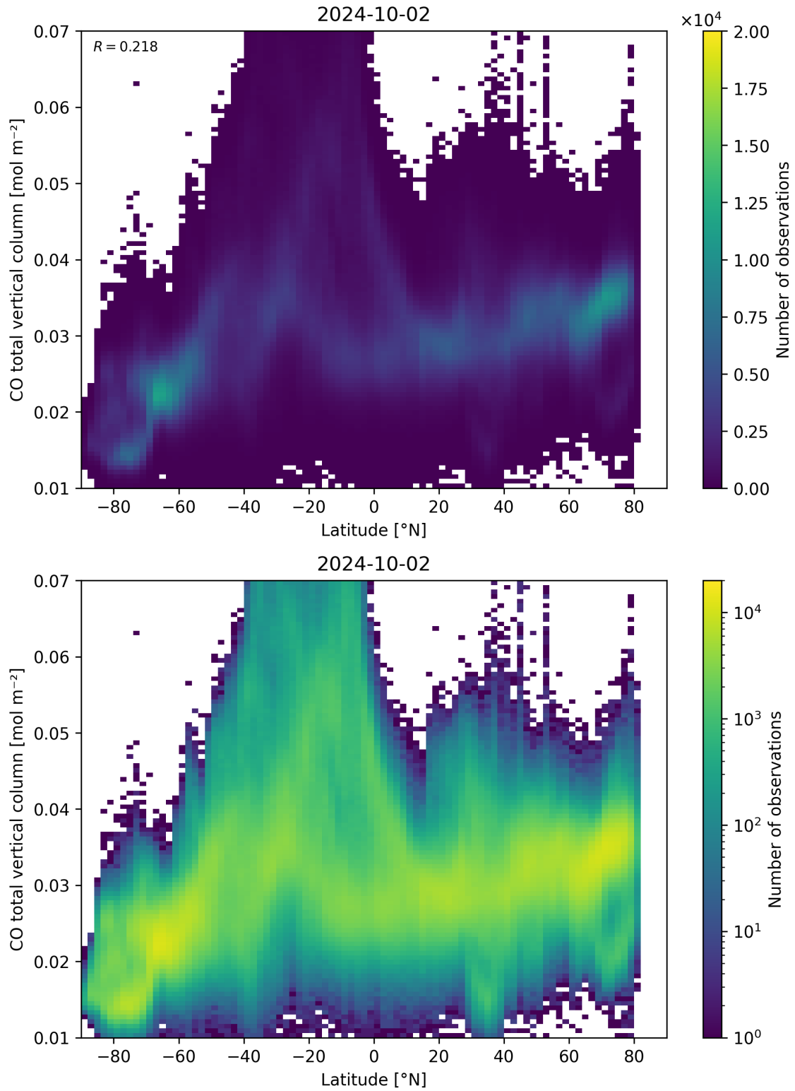
Figure 51: Scatter density plot of “Latitude” against “CO total vertical column” for 2024-10-01 to 2024-10-03.
