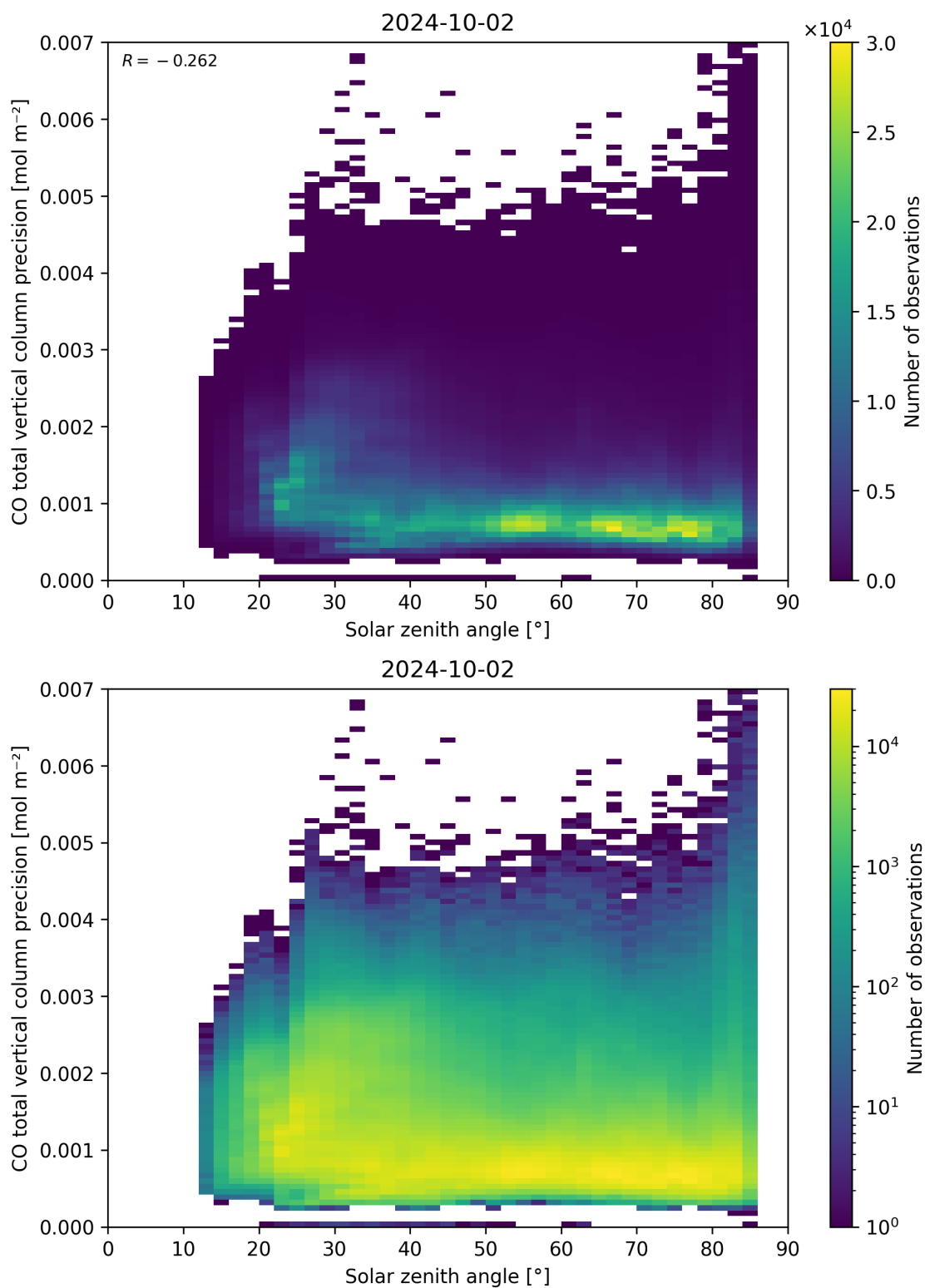
Figure 63: Scatter density plot of “Solar zenith angle” against “CO total vertical column precision” for 2024-10-01 to 2024-10-03.
