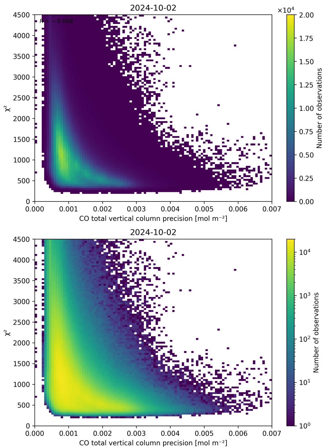
Figure 44: Scatter density plot of “CO total vertical column precision” against “ \chi^2 ” for 2024-10-01 to 2024-10-03.
