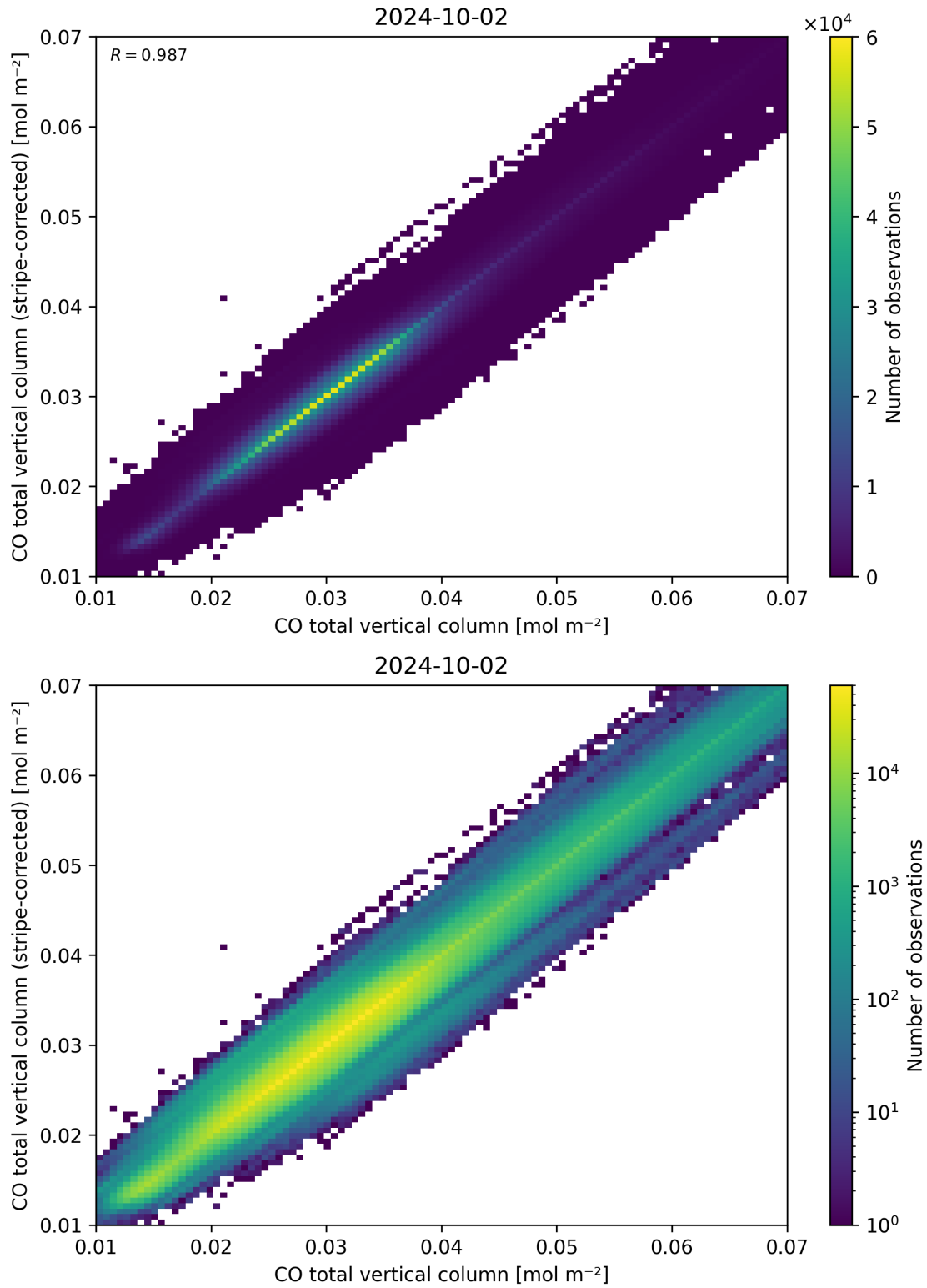
Figure 33: Scatter density plot of “CO total vertical column” against “CO total vertical column (stripe-corrected)” for 2024-10-01 to 2024-10-03.
