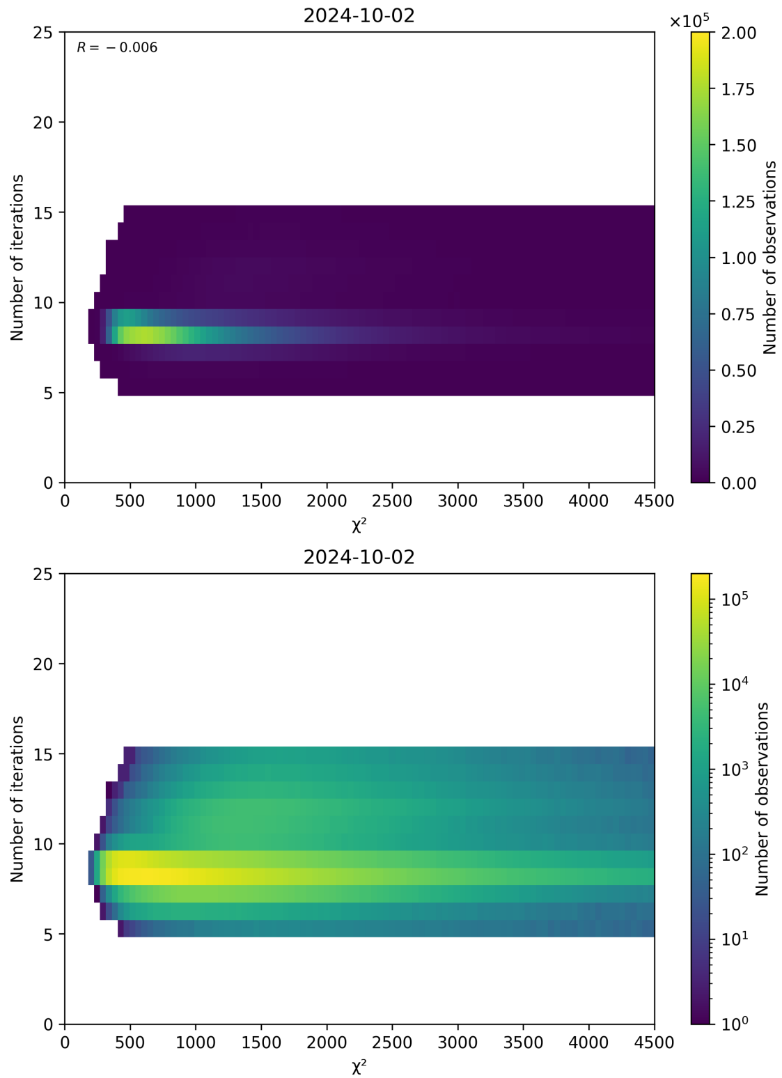
Figure 49: Scatter density plot of “ \chi^2 ” against “Number of iterations” for 2024-10-01 to 2024-10-03.
