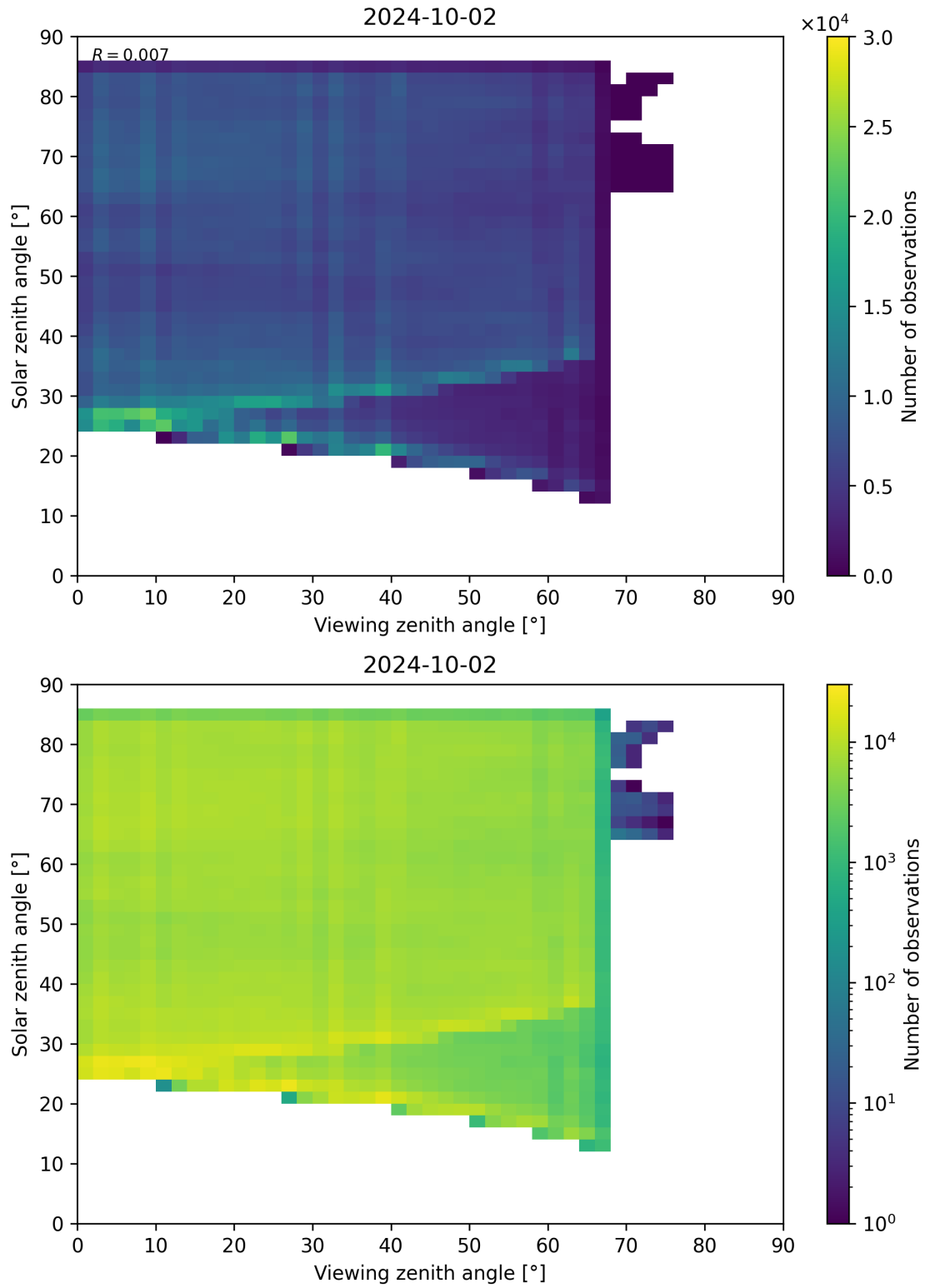
Figure 77: Scatter density plot of “Viewing zenith angle” against “Solar zenith angle” for 2024-10-01 to 2024-10-03.
