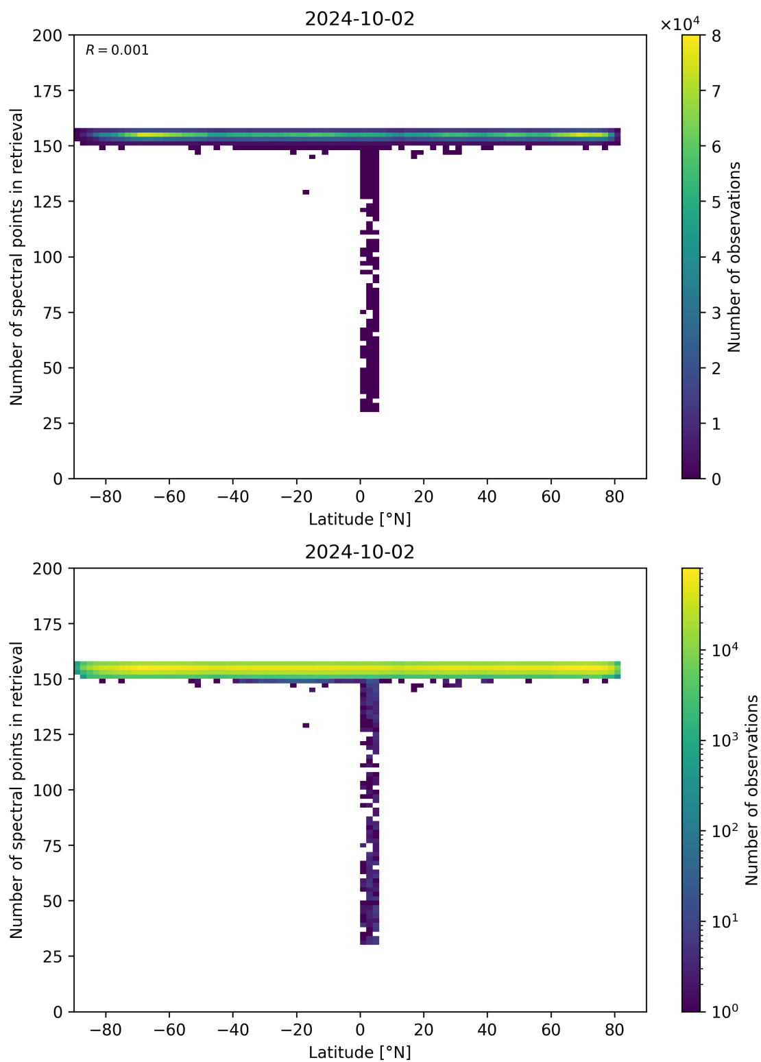
Figure 57: Scatter density plot of “Latitude” against “Number of spectral points in retrieval” for 2024-10-01 to 2024-10-03.
