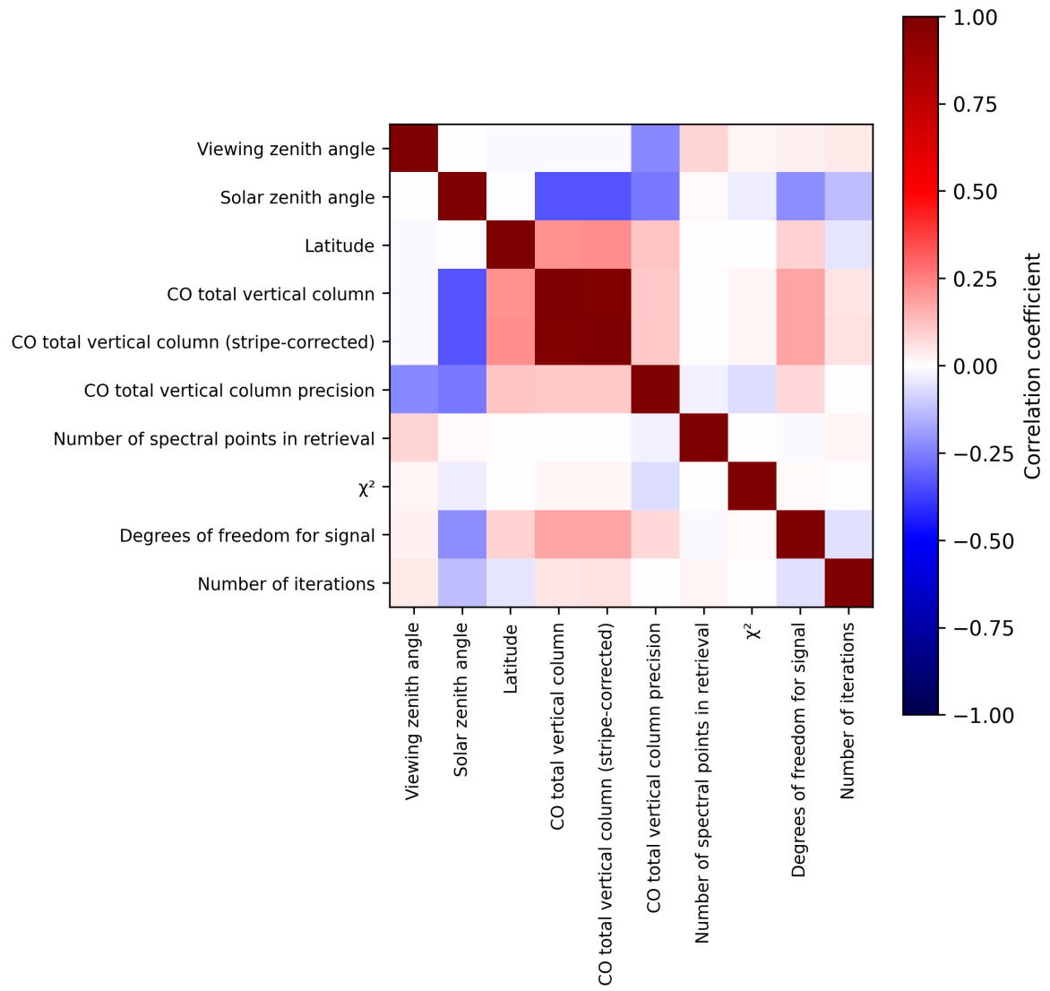
Figure 2: Map of correlation matrix for 2024-10-01 to 2024-10-03.
