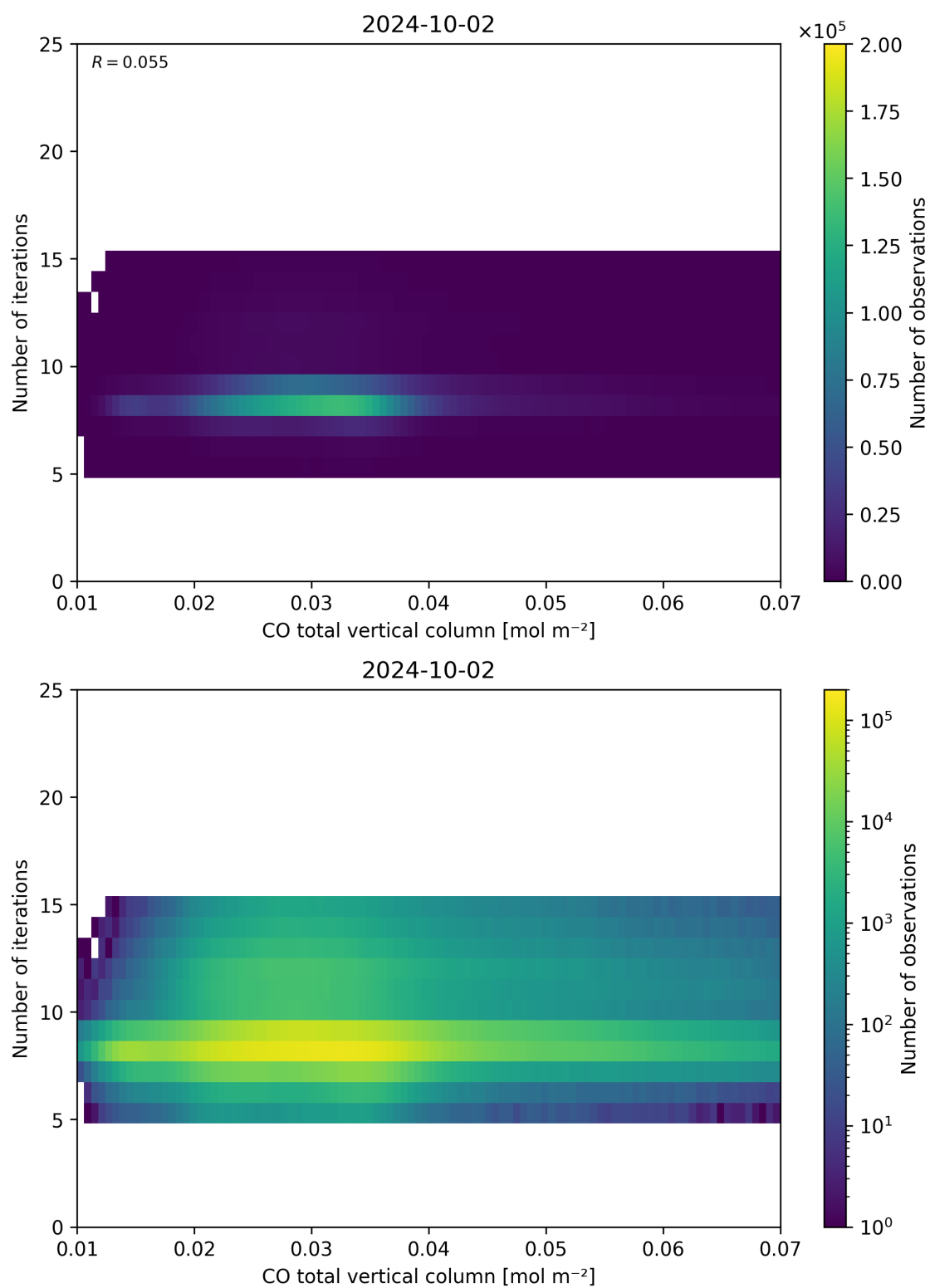
Figure 42: Scatter density plot of “CO total vertical column” against “Number of iterations” for 2024-10-01 to 2024-10-03.
