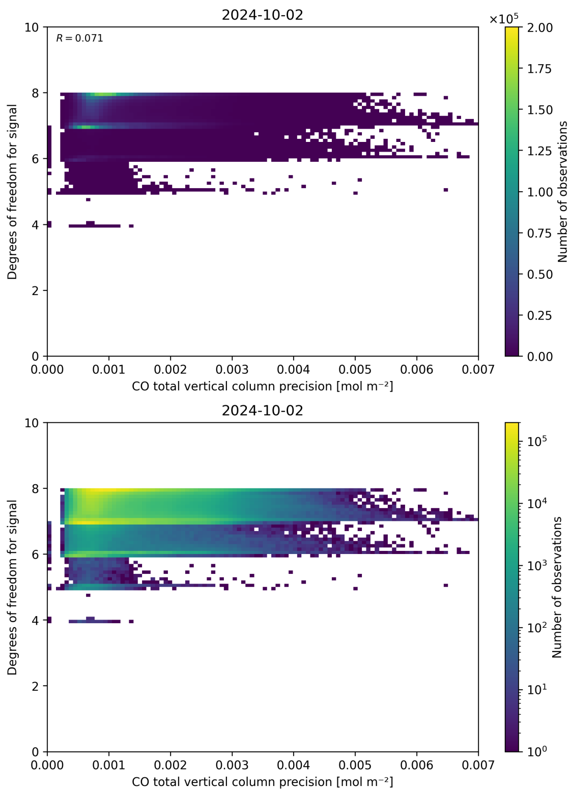
Figure 45: Scatter density plot of “CO total vertical column precision” against “Degrees of freedom for signal” for 2024-10-01 to 2024-10-03.
