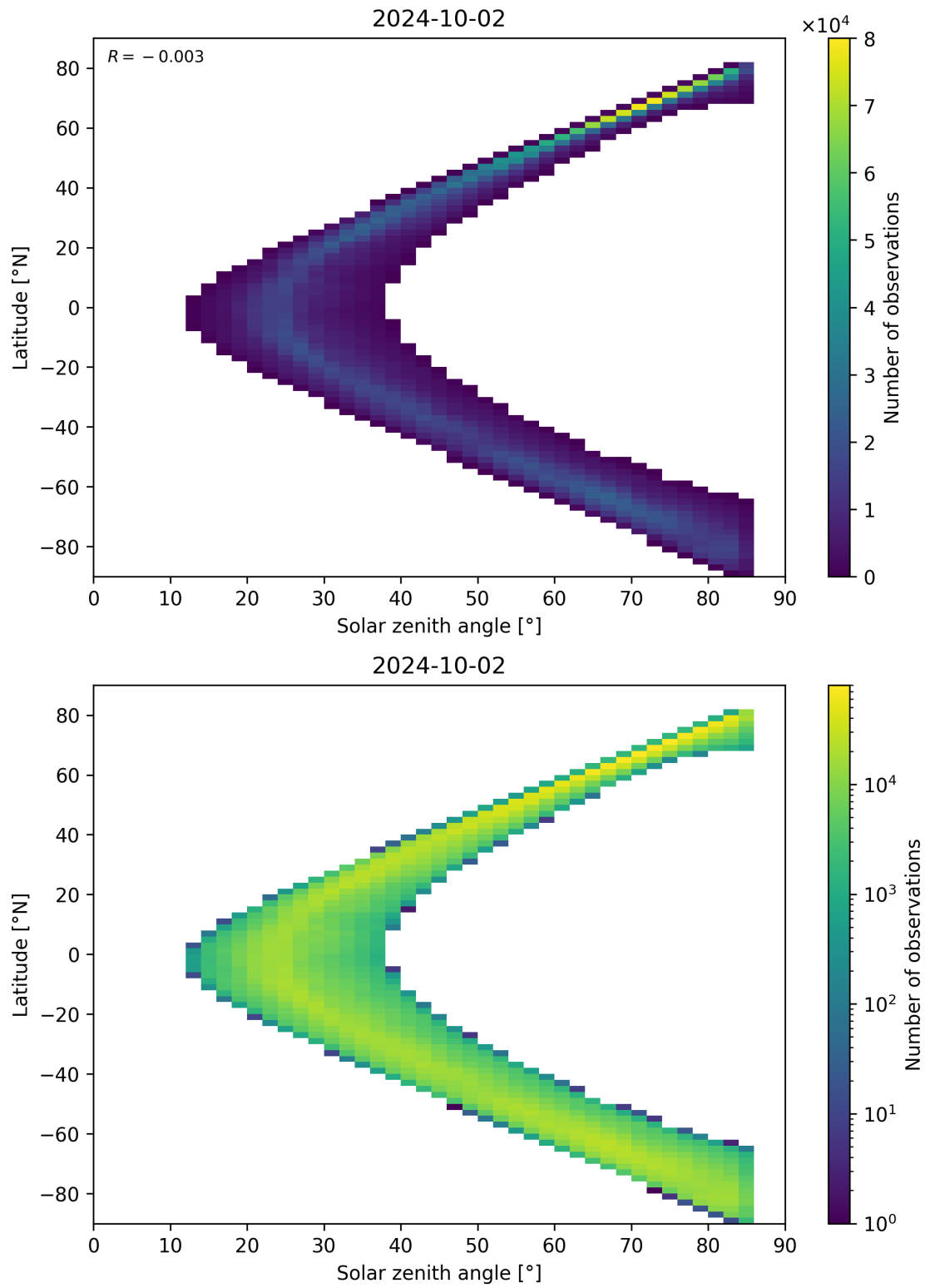
Figure 66: Scatter density plot of “Solar zenith angle” against “Latitude” for 2024-10-01 to 2024-10-03.
