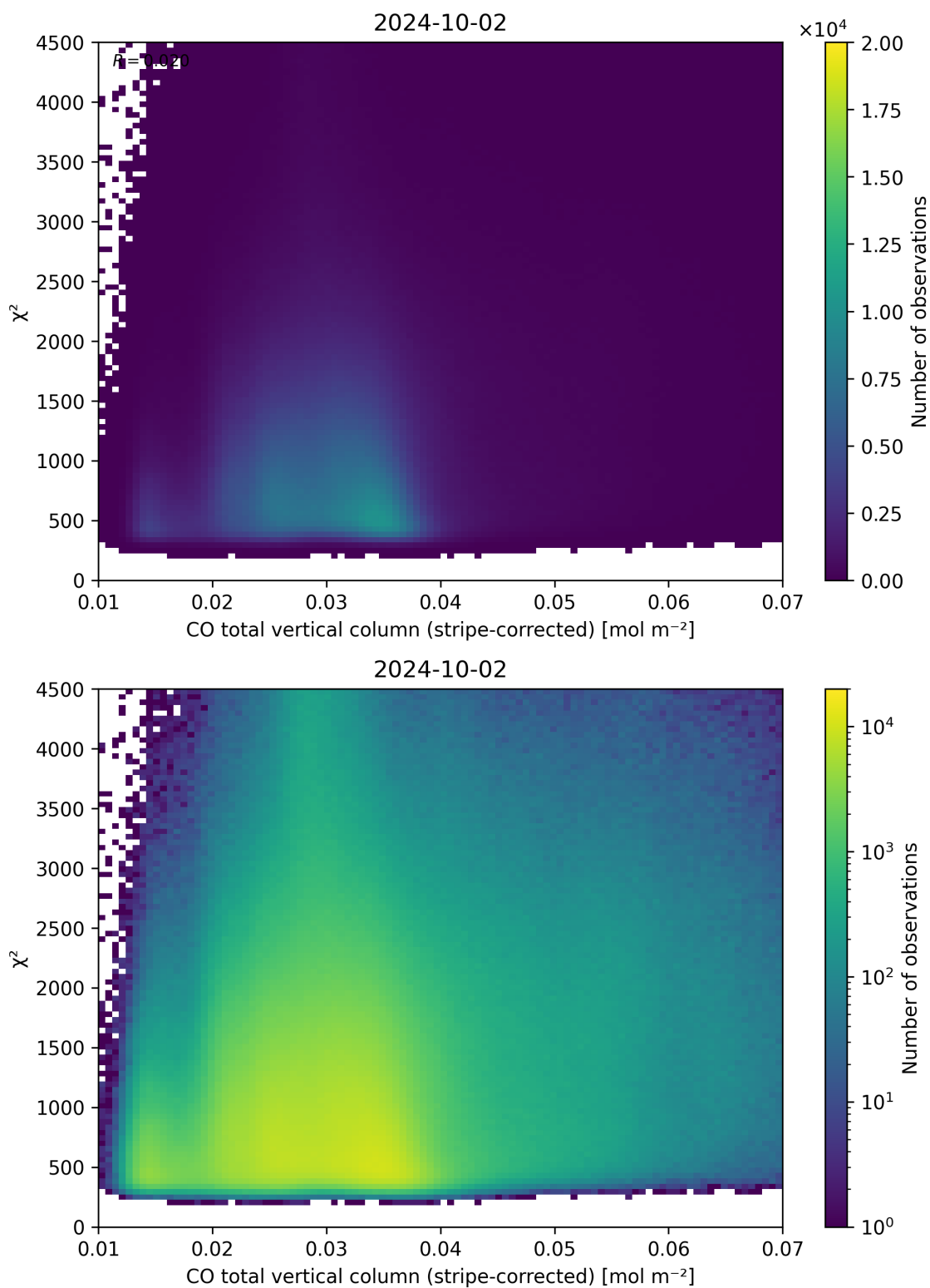
Figure 37: Scatter density plot of “CO total vertical column (stripe-corrected)” against “ \chi^2 ” for 2024-10-01 to 2024-10-03.
