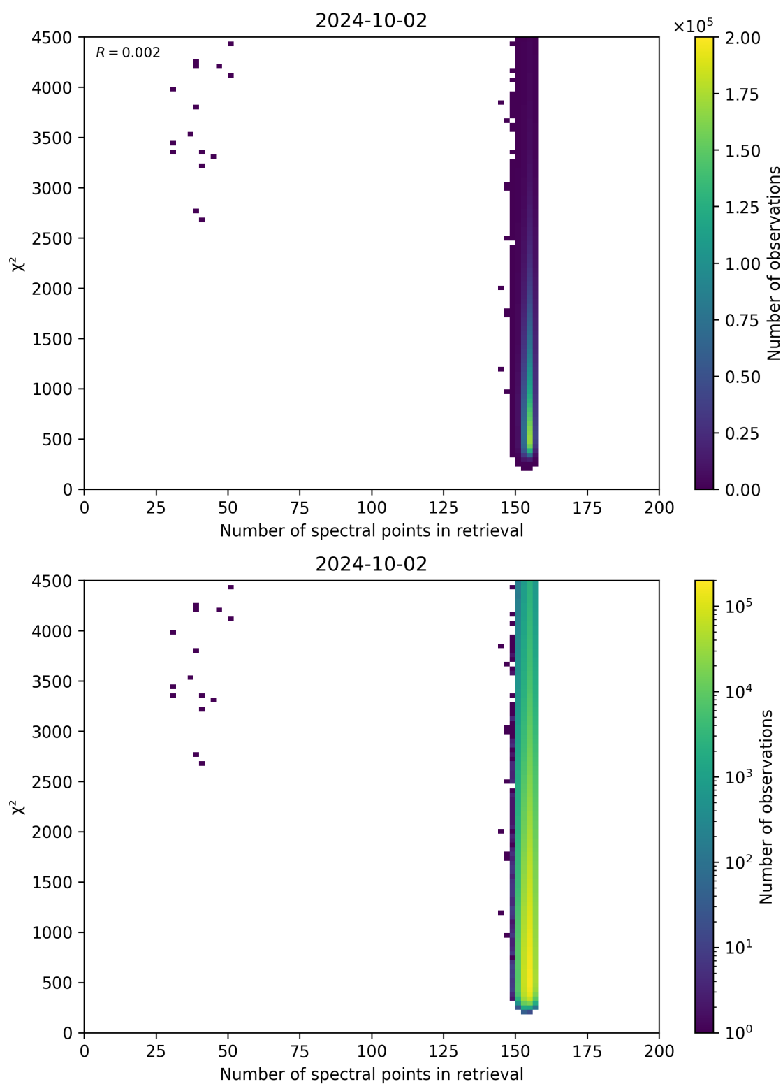
Figure 58: Scatter density plot of “Number of spectral points in retrieval” against “ \chi^2 ” for 2024-10-01 to 2024-10-03.
