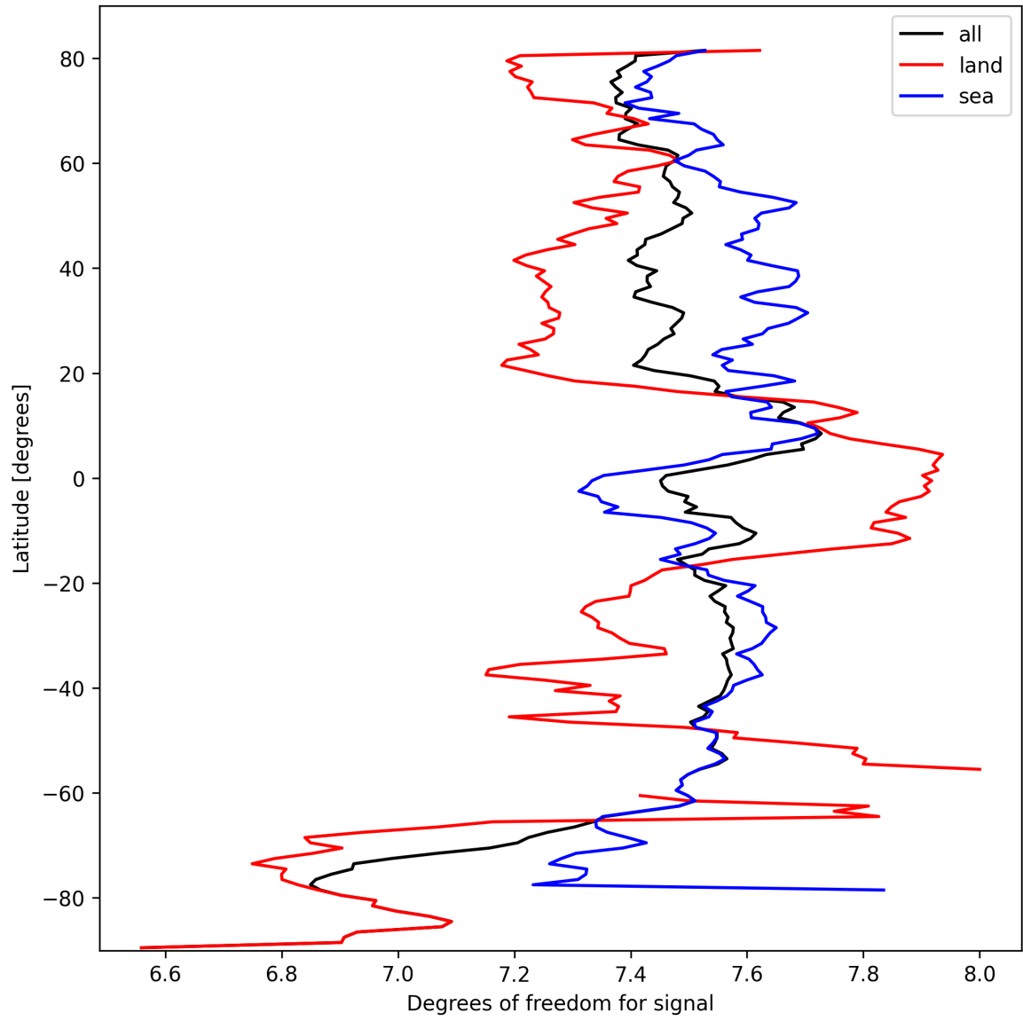
Figure 15: Zonal average of “Degrees of freedom for signal” for 2024-10-01 to 2024-10-03.
