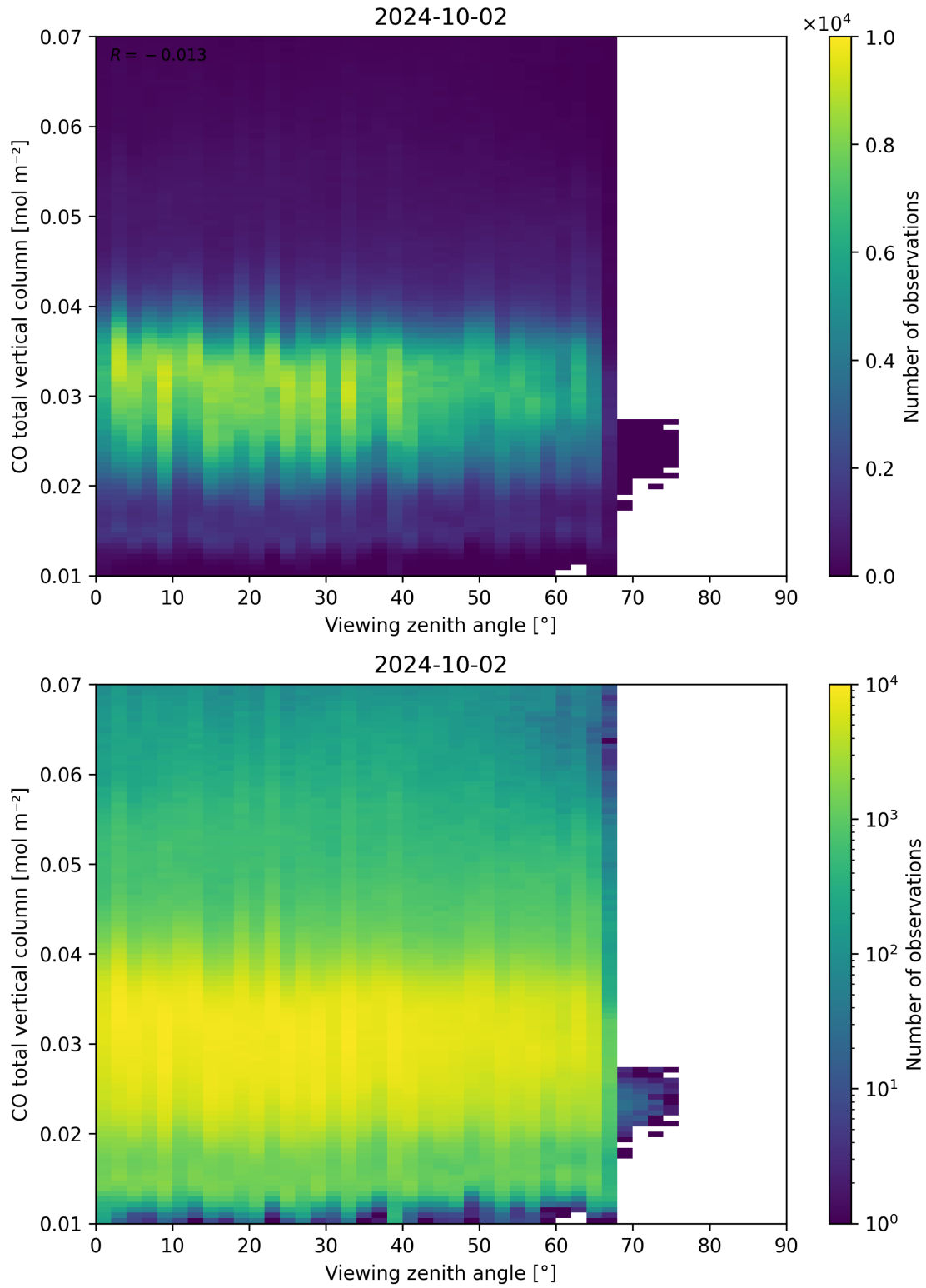
Figure 69: Scatter density plot of “Viewing zenith angle” against “CO total vertical column” for 2024-10-01 to 2024-10-03.
