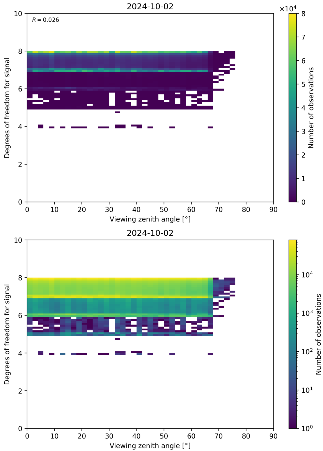
Figure 73: Scatter density plot of “Viewing zenith angle” against “Degrees of freedom for signal” for 2024-10-01 to 2024-10-03.
