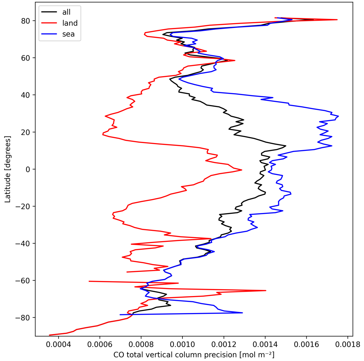
Figure 12: Zonal average of “CO total vertical column precision” for 2024-10-01 to 2024-10-03.
