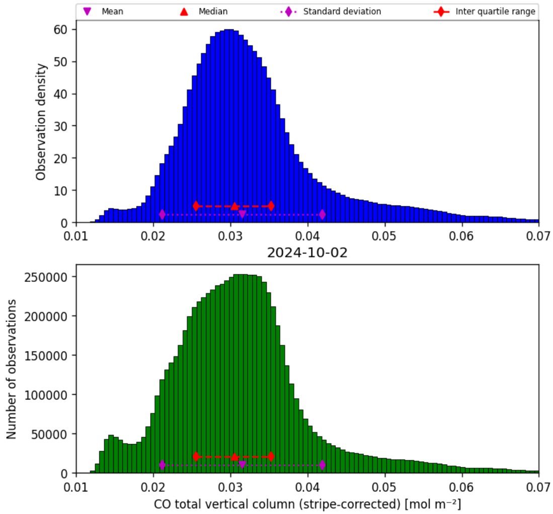
Figure 19: Histogram of “CO total vertical column (stripe-corrected)” for 2024-10-01 to 2024-10-03
