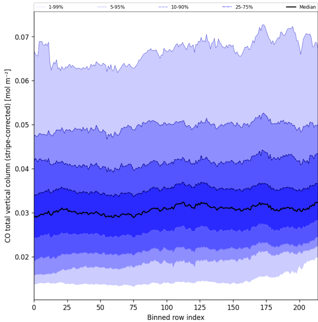
Figure 27: Along track statistics of “CO total vertical column (stripe-corrected)” for 2024-10-01 to 2024-10-03
