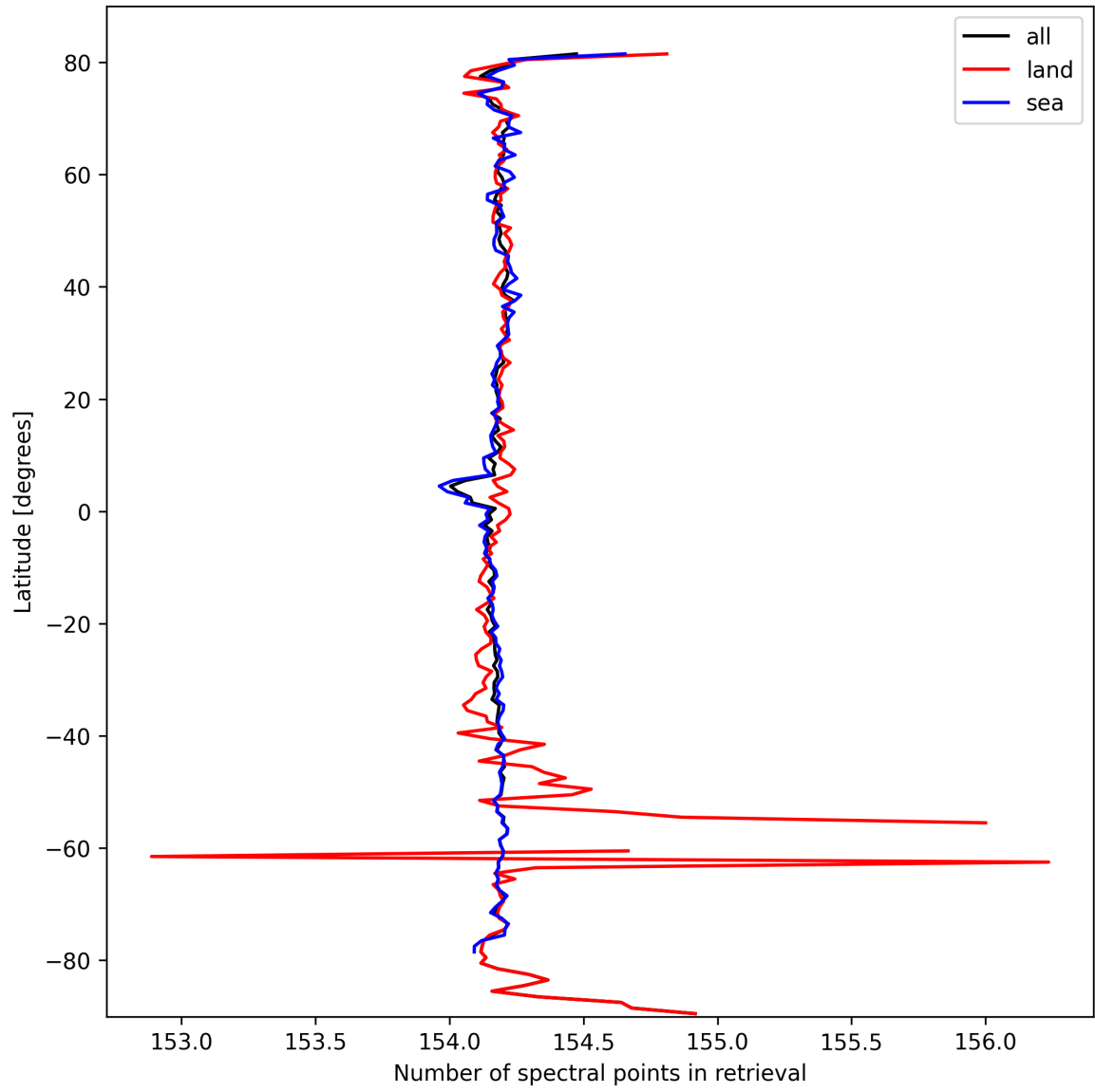
Figure 13: Zonal average of “Number of spectral points in retrieval” for 2024-10-01 to 2024-10-03.
