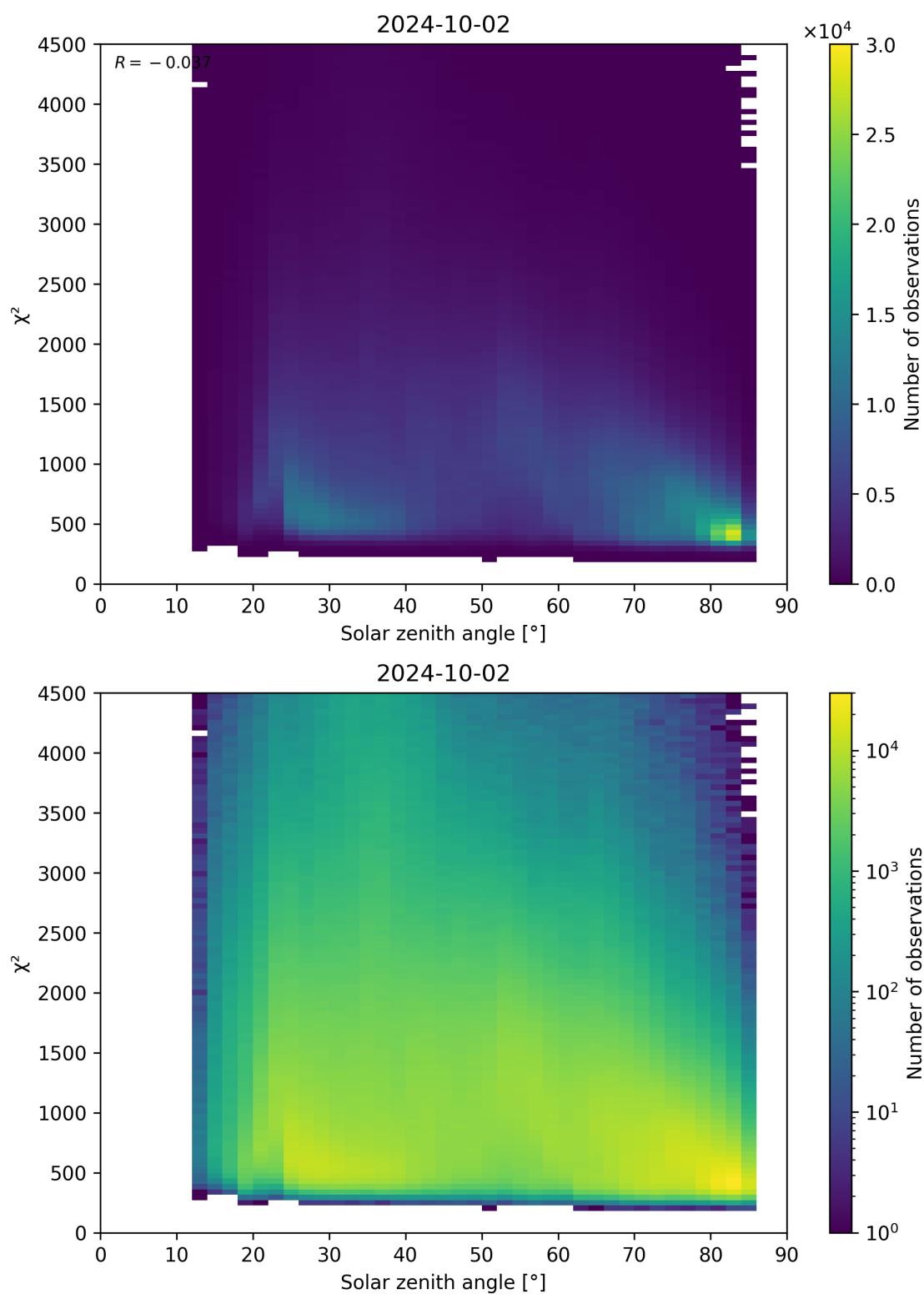
Figure 64: Scatter density plot of “Solar zenith angle” against “ \chi^2 ” for 2024-10-01 to 2024-10-03.
