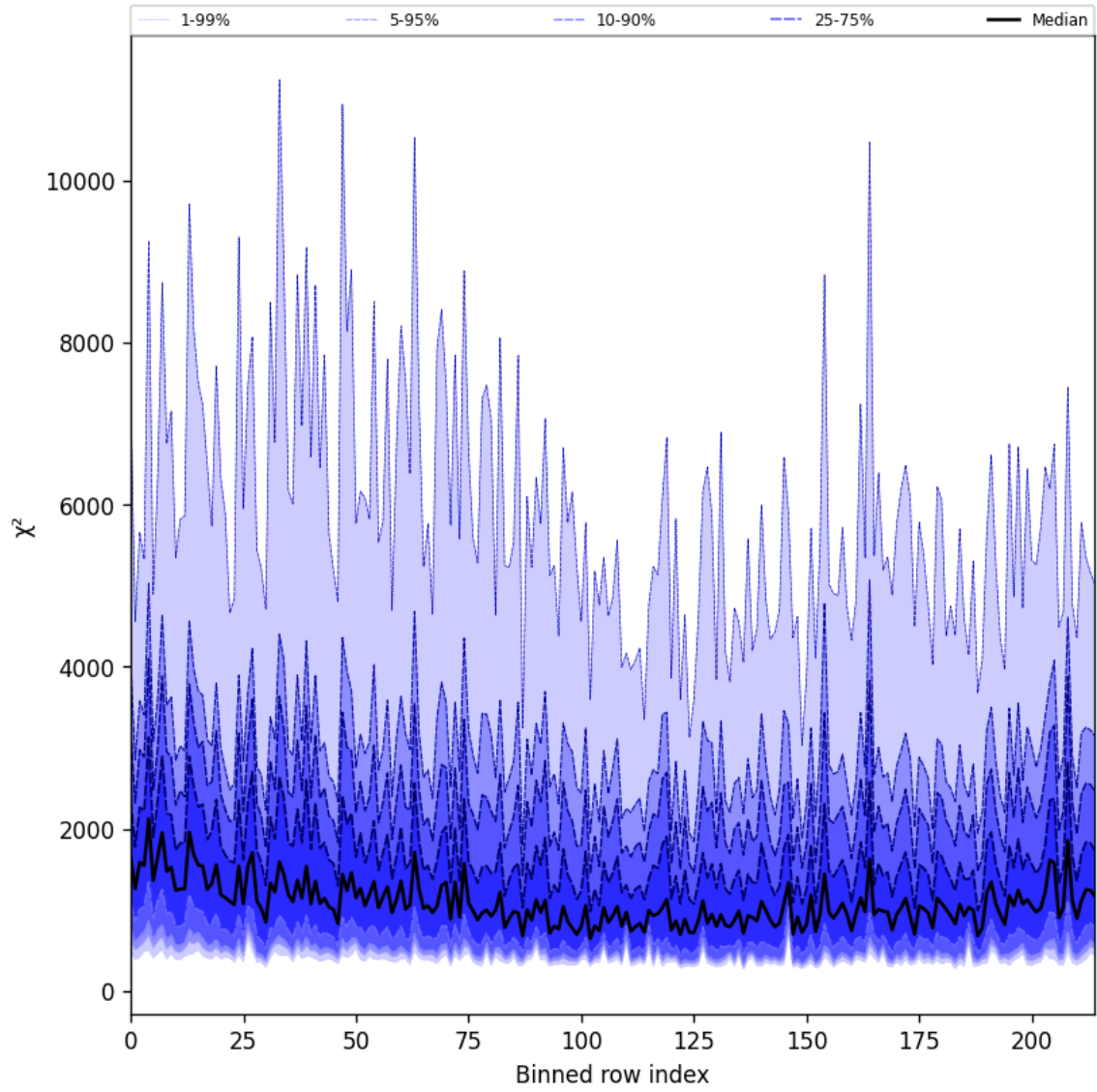
Figure 30: Along track statistics of “ \chi^2 ” for 2024-10-01 to 2024-10-03
