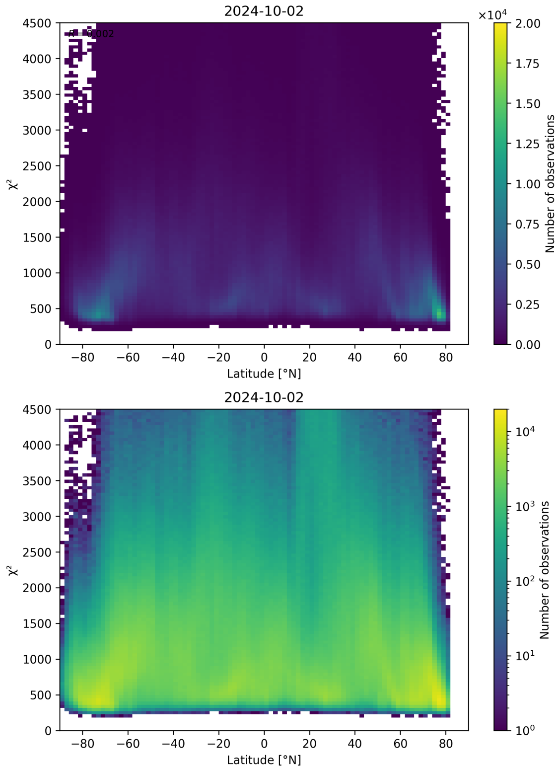
Figure 54: Scatter density plot of “Latitude” against “ \chi^2 ” for 2024-10-01 to 2024-10-03.
