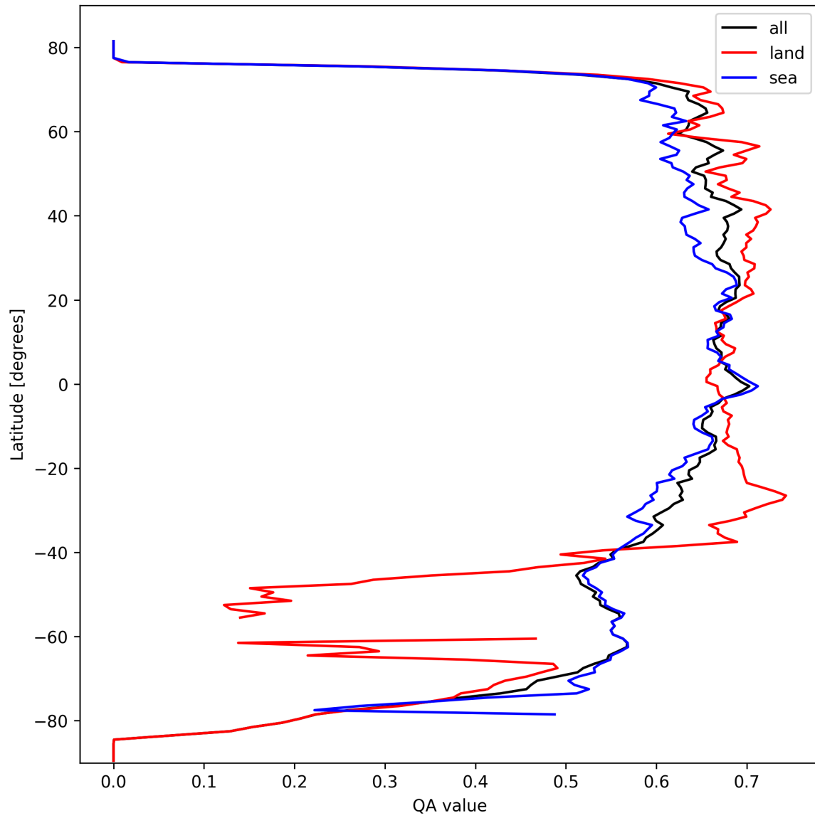
Figure 9: Zonal average of “QA value” for 2024-10-01 to 2024-10-03.
