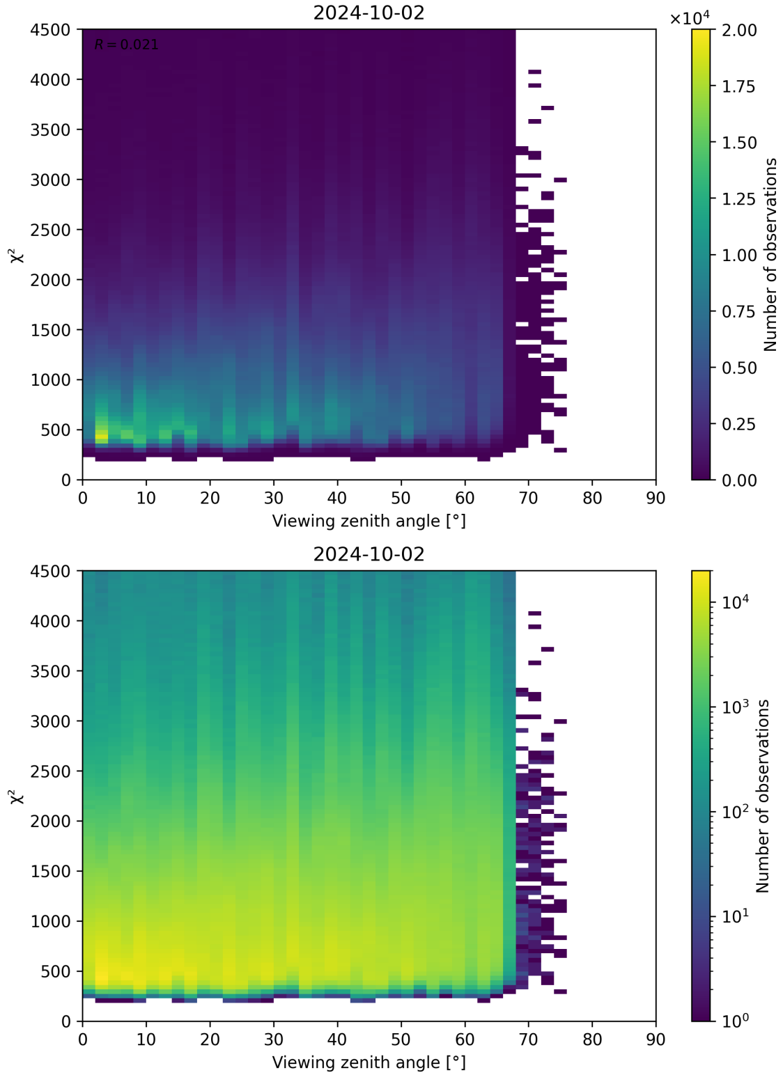
Figure 72: Scatter density plot of “Viewing zenith angle” against “ \chi^2 ” for 2024-10-01 to 2024-10-03.
