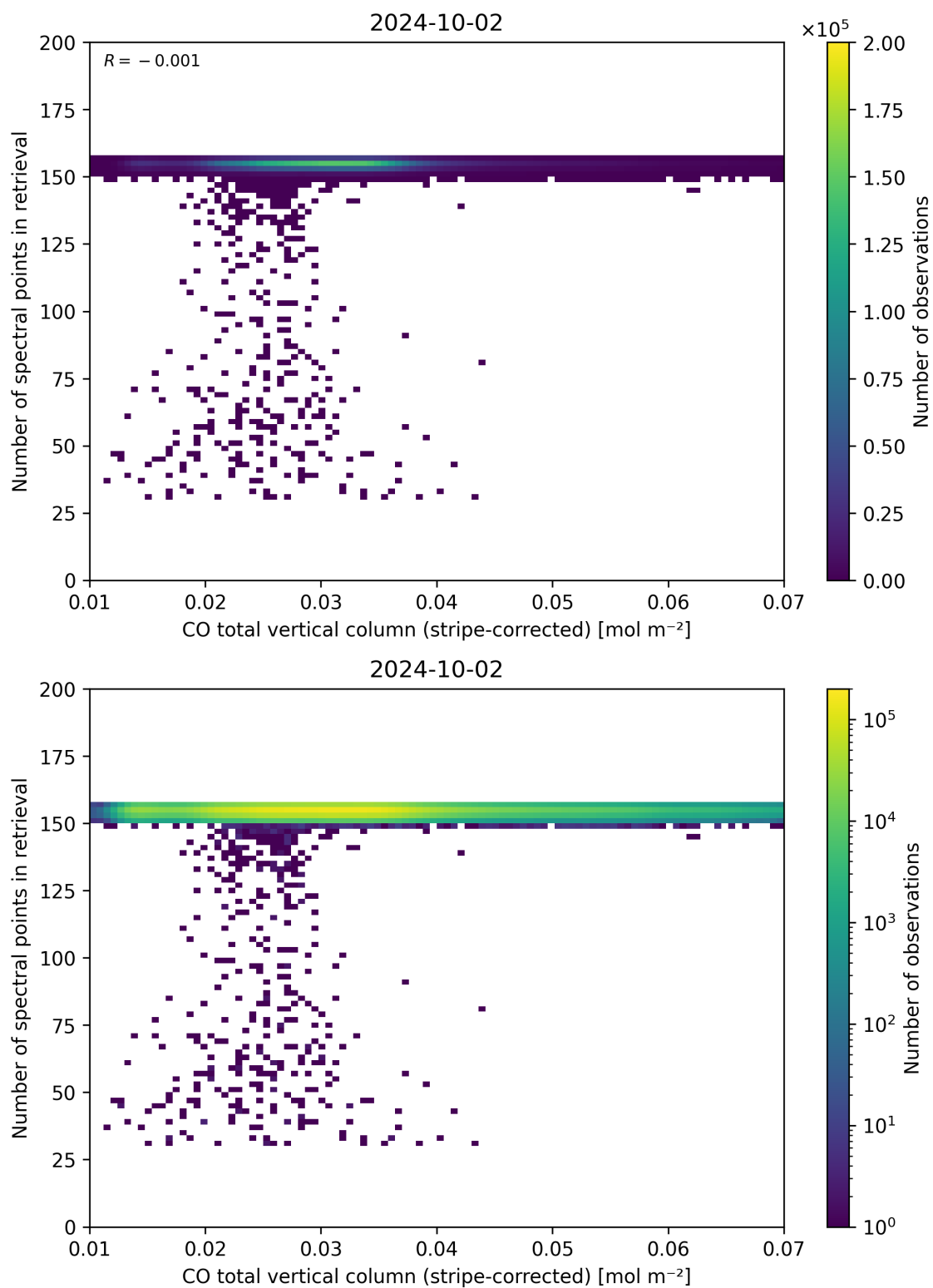
Figure 40: Scatter density plot of “CO total vertical column (stripe-corrected)” against “Number of spectral points in retrieval” for 2024-10-01 to 2024-10-03.
