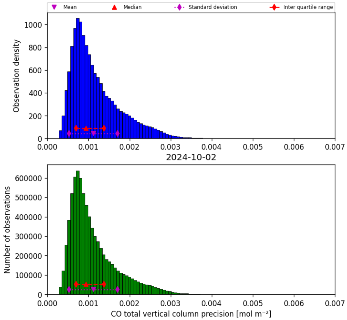
Figure 20: Histogram of “CO total vertical column precision” for 2024-10-01 to 2024-10-03
