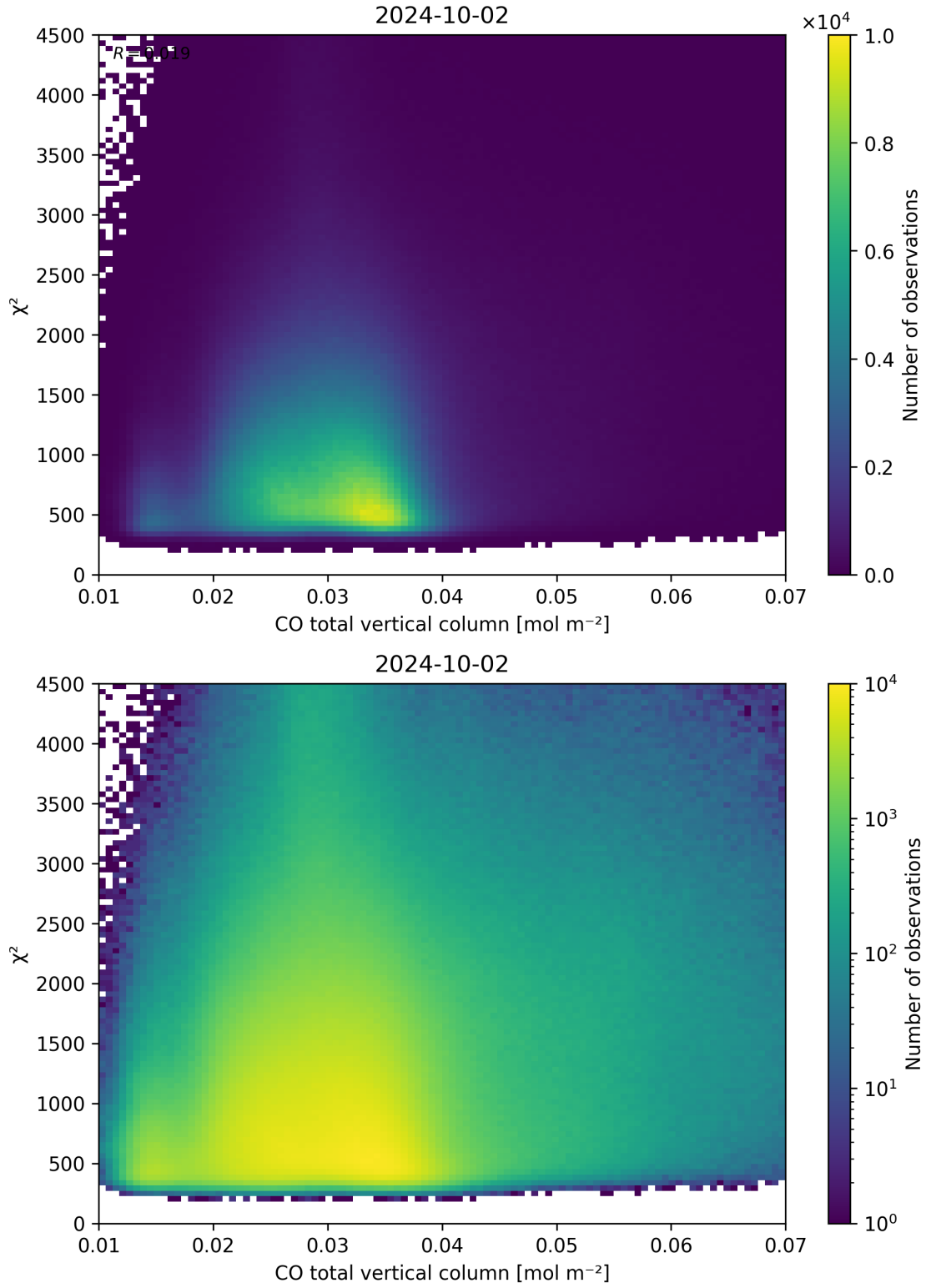
Figure 35: Scatter density plot of “CO total vertical column” against “ \chi^2 ” for 2024-10-01 to 2024-10-03.
