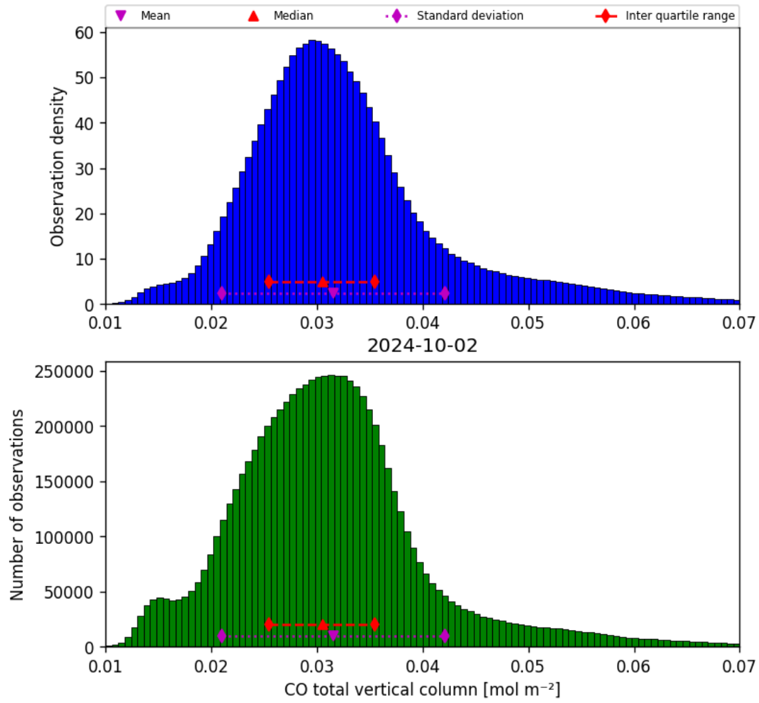
Figure 18: Histogram of “CO total vertical column” for 2024-10-01 to 2024-10-03
