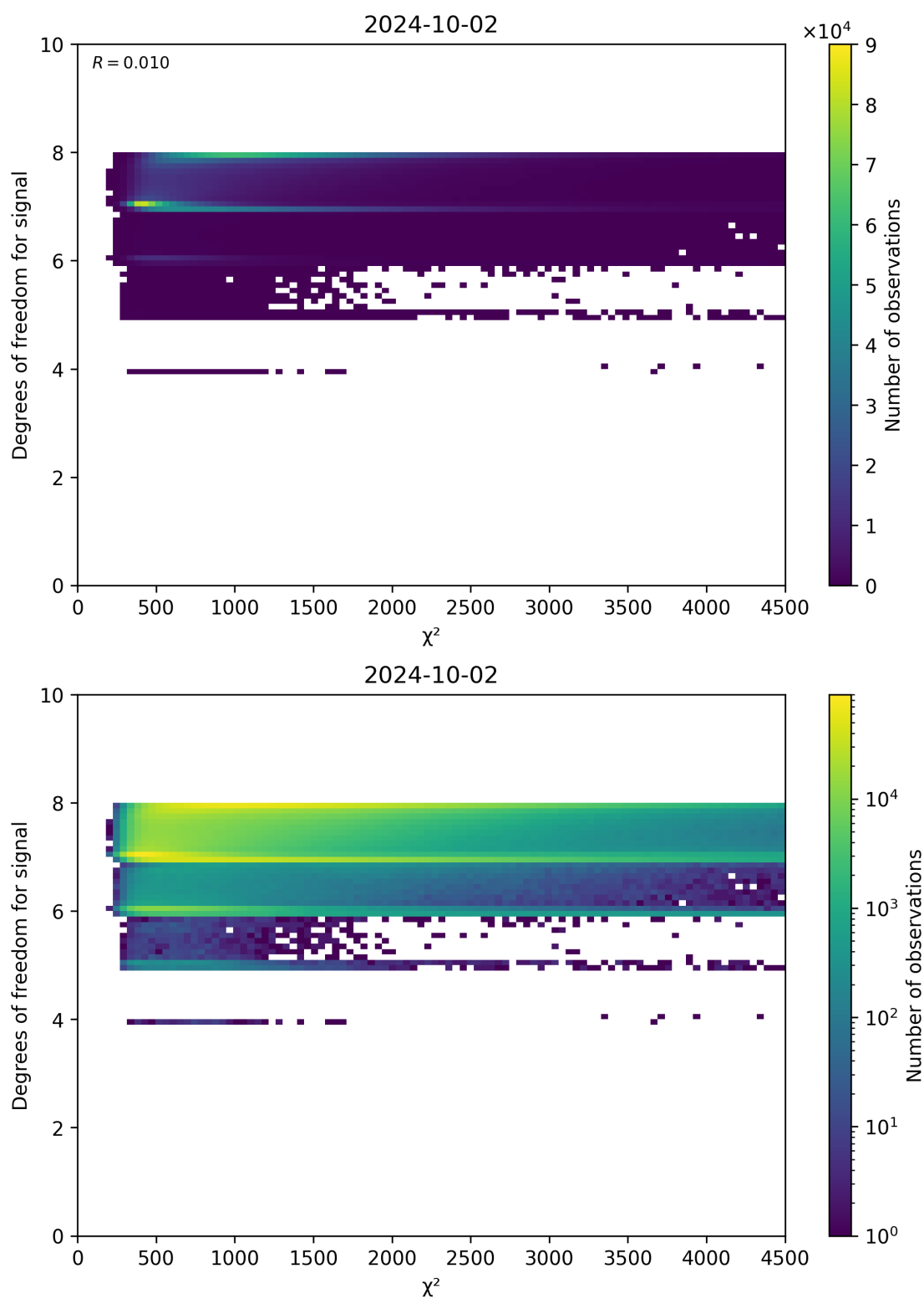
Figure 48: Scatter density plot of " \chi^2 " against "Degrees of freedom for signal" for 2024-10-01 to 2024-10-03.
