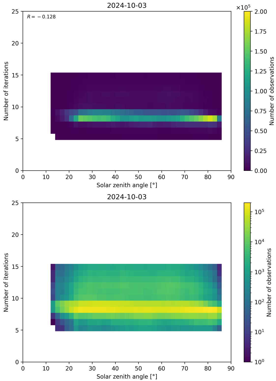
Figure 67: Scatter density plot of “Solar zenith angle” against “Number of iterations” for 2024-10-03 to 2024-10-04.
