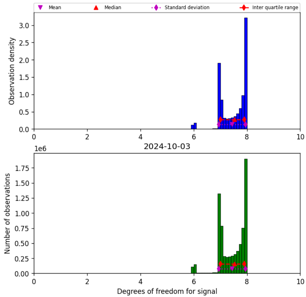
Figure 23: Histogram of “Degrees of freedom for signal” for 2024-10-03 to 2024-10-04
