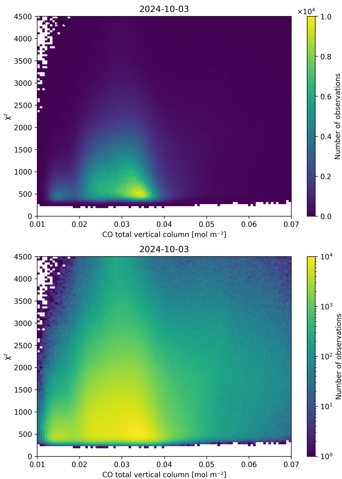
Figure 35: Scatter density plot of “CO total vertical column” against “ \chi^2 ” for 2024-10-03 to 2024-10-04.
