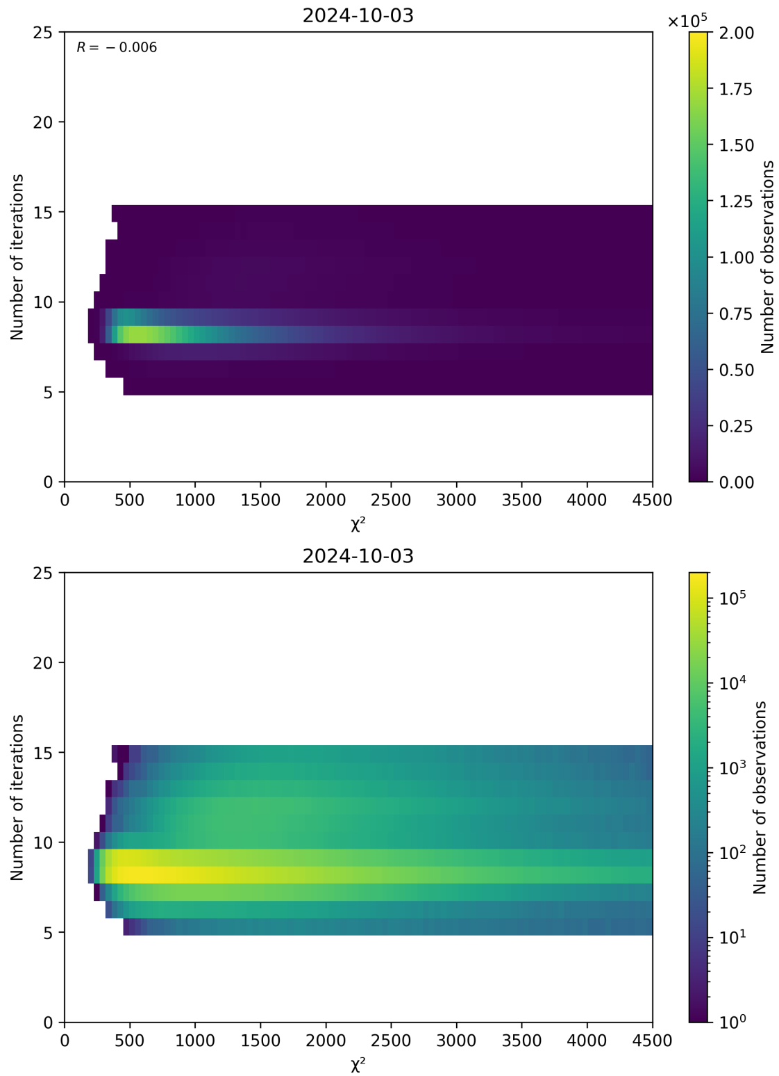
Figure 49: Scatter density plot of “ \chi^2 ” against “Number of iterations” for 2024-10-03 to 2024-10-04.
