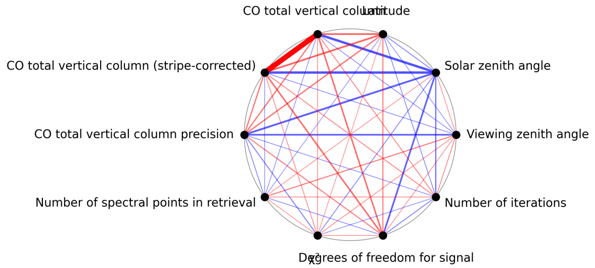
Figure 1: Map of correlation graph for 2024-10-03 to 2024-10-04.
