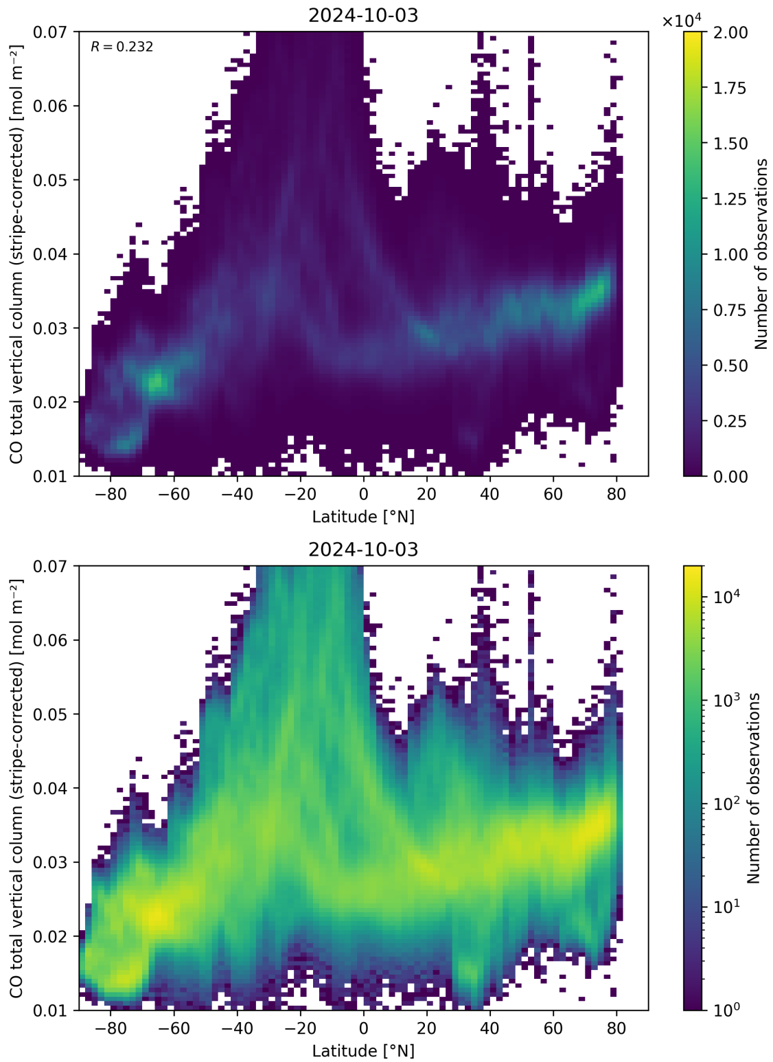
Figure 52: Scatter density plot of “Latitude” against “CO total vertical column (stripe-corrected)” for 2024-10-03 to 2024-10-04.
