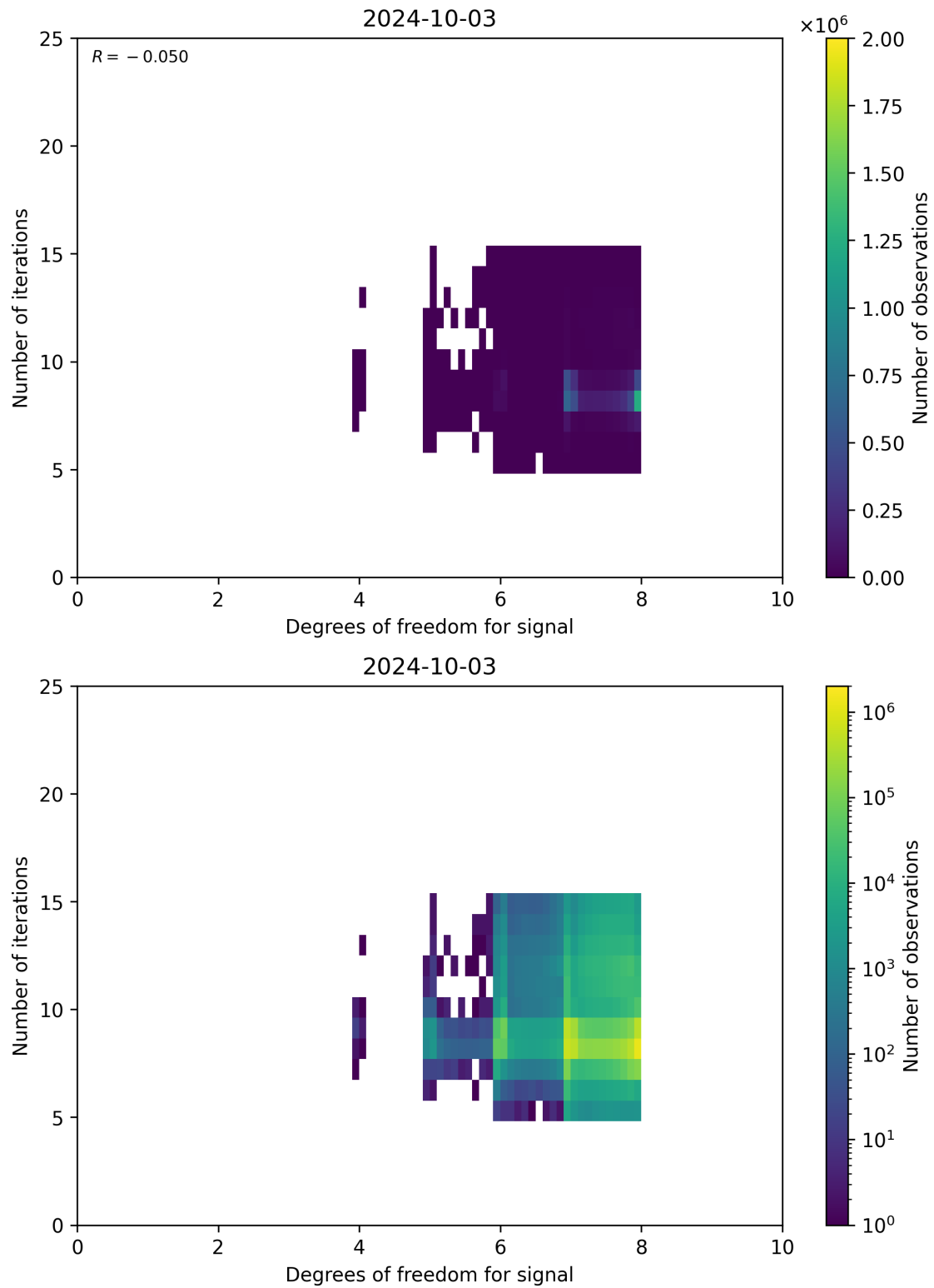
Figure 50: Scatter density plot of “Degrees of freedom for signal” against “Number of iterations” for 2024-10-03 to 2024-10-04.
