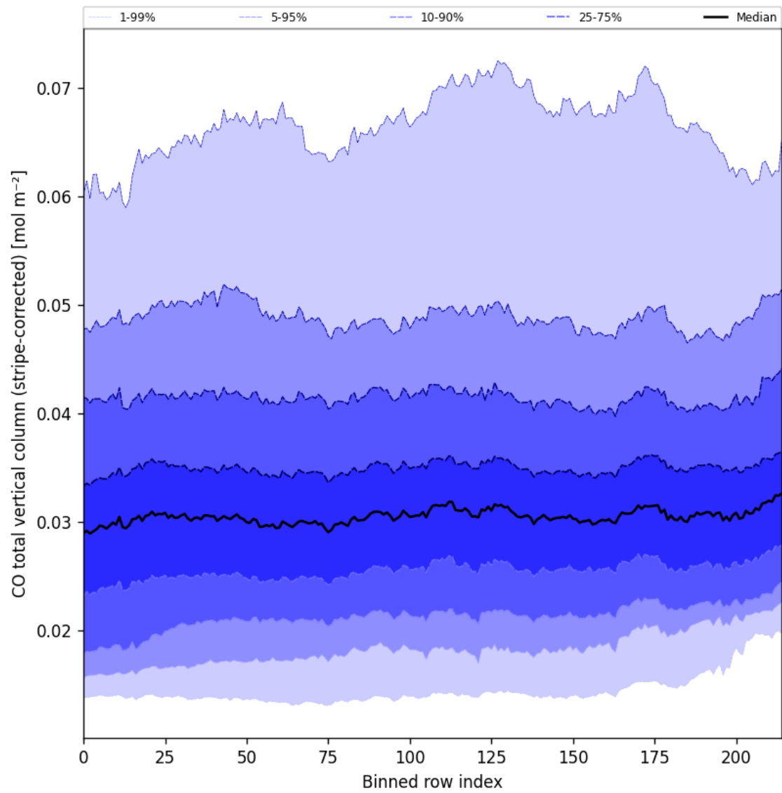
Figure 27: Along track statistics of “CO total vertical column (stripe-corrected)” for 2024-10-03 to 2024-10-04
