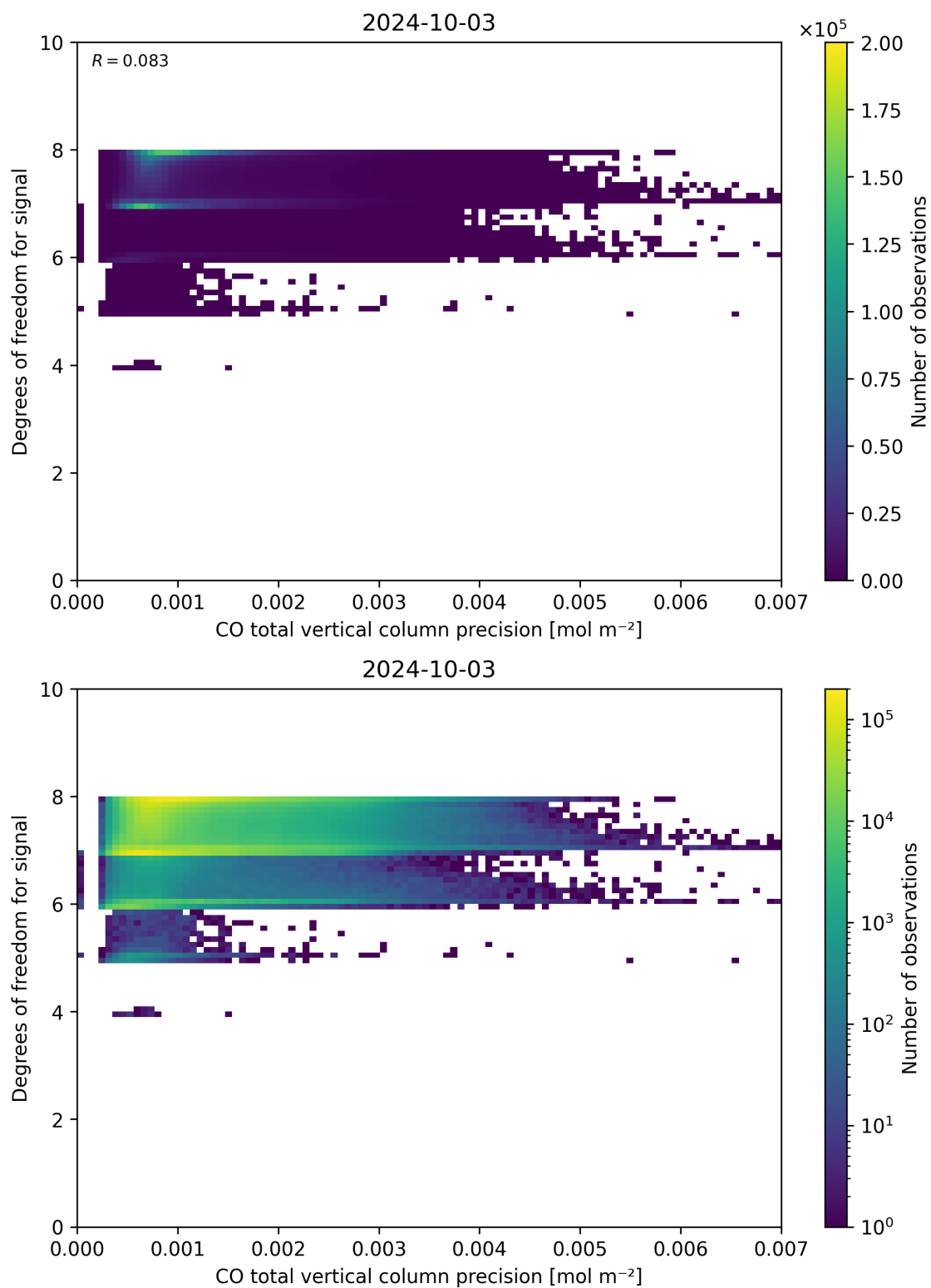
Figure 45: Scatter density plot of “CO total vertical column precision” against “Degrees of freedom for signal” for 2024-10-03 to 2024-10-04.
