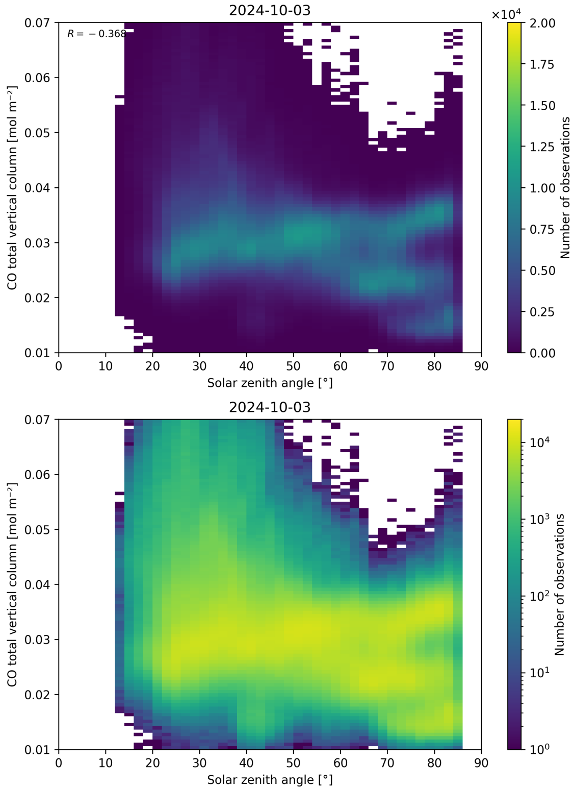
Figure 61: Scatter density plot of “Solar zenith angle” against “CO total vertical column” for 2024-10-03 to 2024-10-04.
