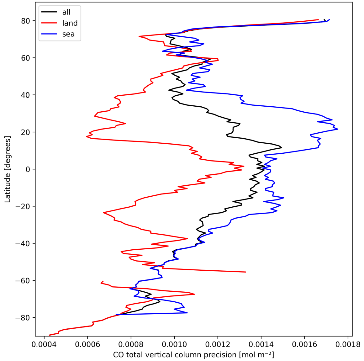
Figure 12: Zonal average of “CO total vertical column precision” for 2024-10-03 to 2024-10-04.
