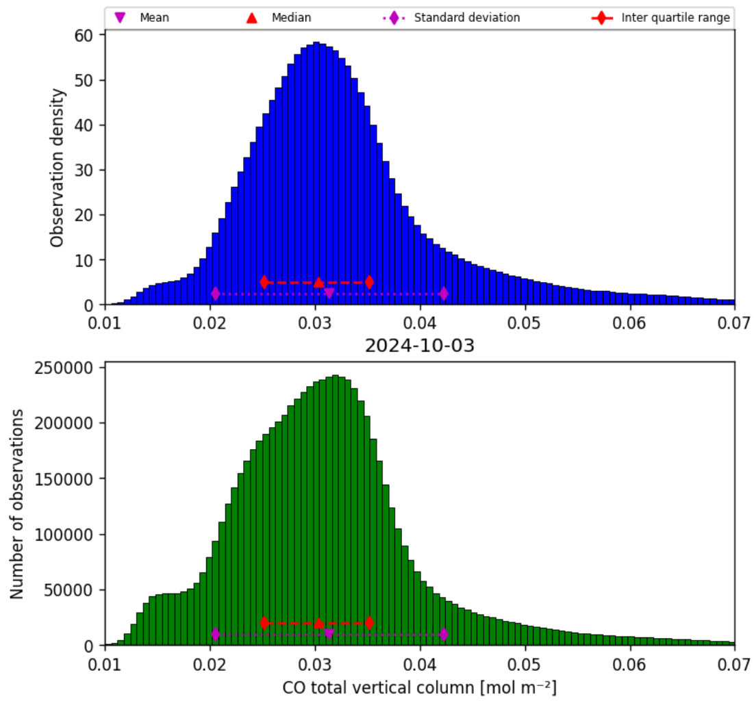
Figure 18: Histogram of “CO total vertical column” for 2024-10-03 to 2024-10-04
