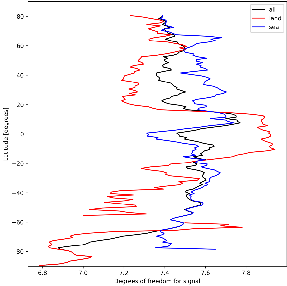
Figure 15: Zonal average of “Degrees of freedom for signal” for 2024-10-03 to 2024-10-04.
