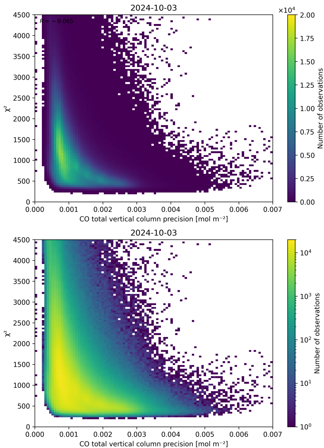
Figure 44: Scatter density plot of “CO total vertical column precision” against “ \chi^2 ” for 2024-10-03 to 2024-10-04.
