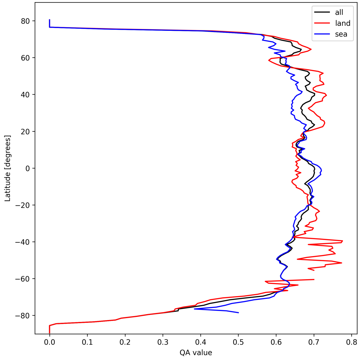
Figure 9: Zonal average of “QA value” for 2024-10-03 to 2024-10-04.
