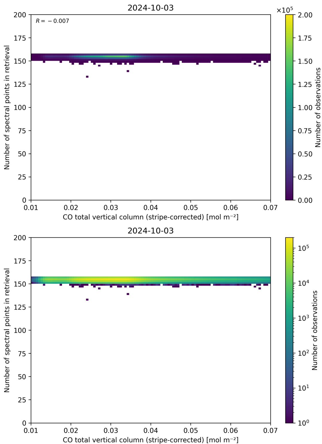
Figure 40: Scatter density plot of “CO total vertical column (stripe-corrected)” against “Number of spectral points in retrieval” for 2024-10-03 to 2024-10-04.
