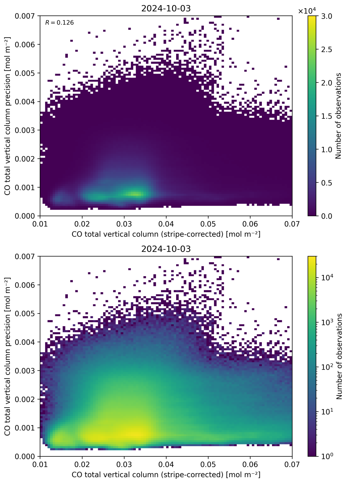
Figure 36: Scatter density plot of “CO total vertical column (stripe-corrected)” against “CO total vertical column precision” for 2024-10-03 to 2024-10-04.
