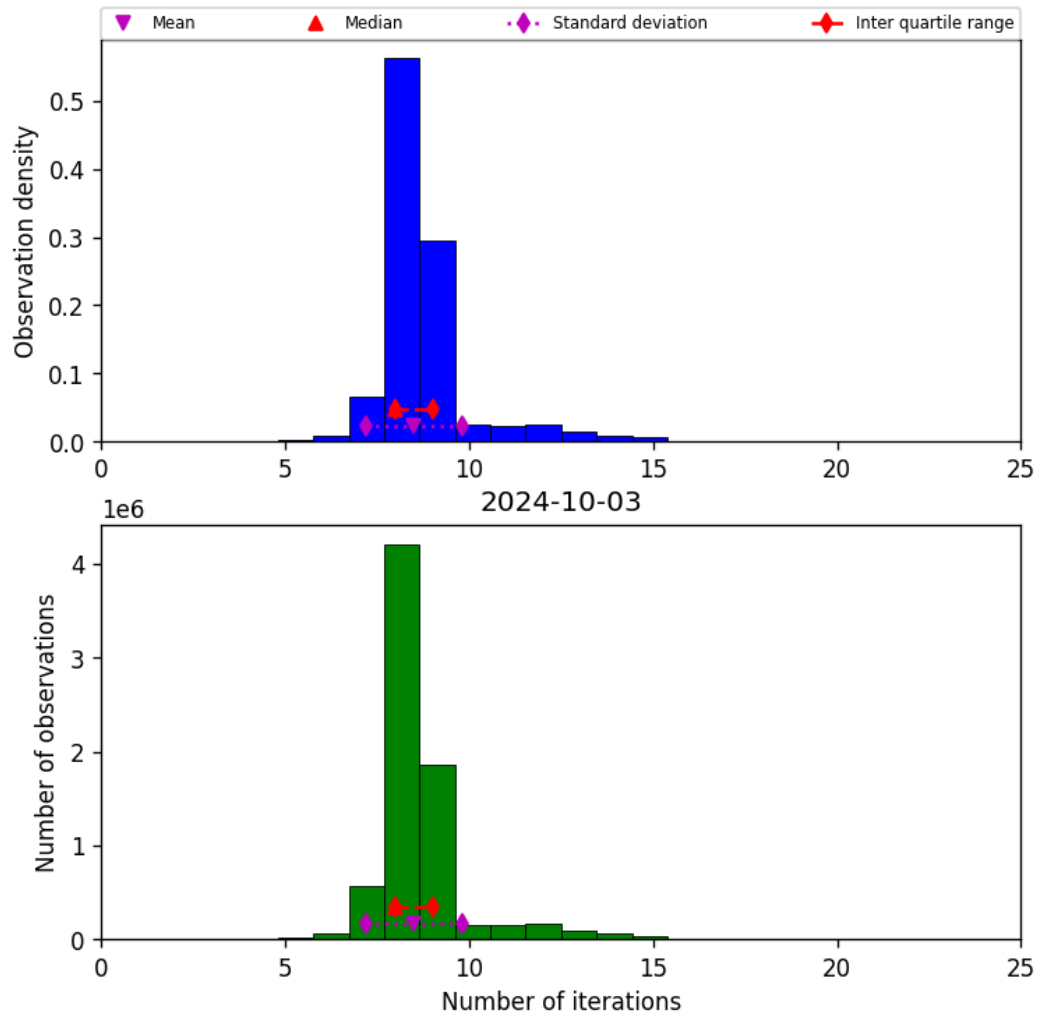
Figure 24: Histogram of “Number of iterations” for 2024-10-03 to 2024-10-04
