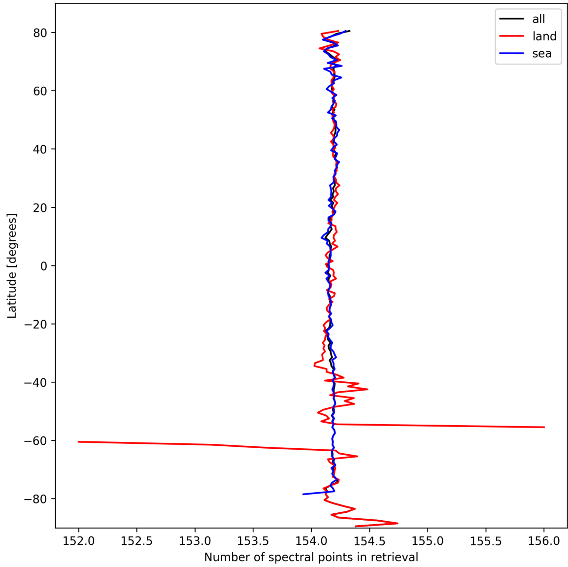
Figure 13: Zonal average of “Number of spectral points in retrieval” for 2024-10-03 to 2024-10-04.
