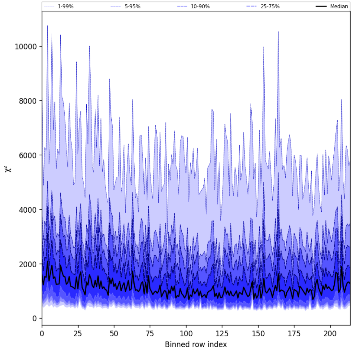
Figure 30: Along track statistics of “ \chi^2 ” for 2024-10-03 to 2024-10-04
