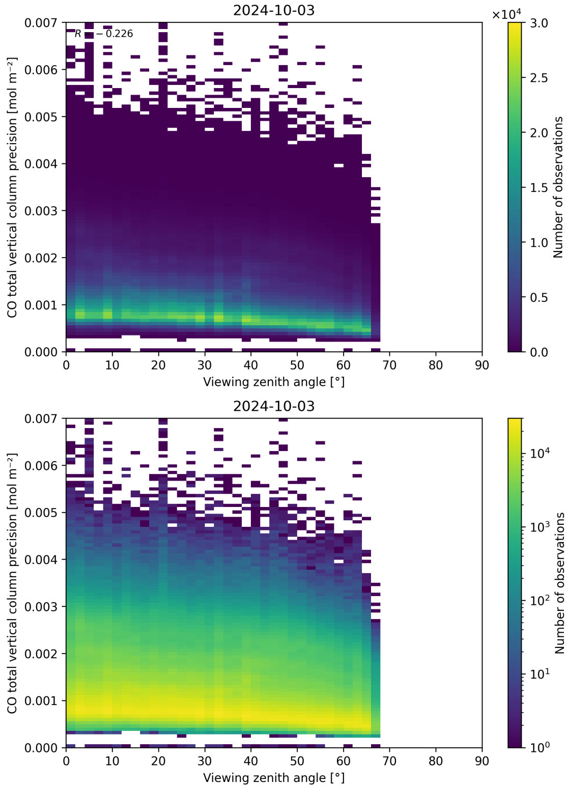
Figure 71: Scatter density plot of “Viewing zenith angle” against “CO total vertical column precision” for 2024-10-03 to 2024-10-04.
