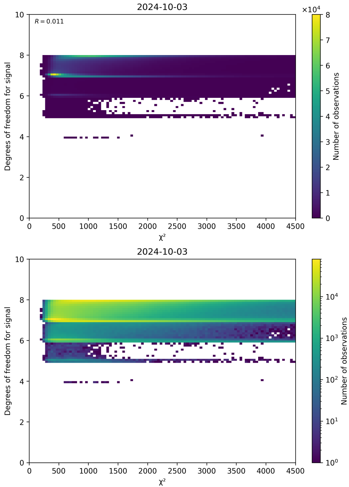
Figure 48: Scatter density plot of “ \chi^2 ” against “Degrees of freedom for signal” for 2024-10-03 to 2024-10-04.
