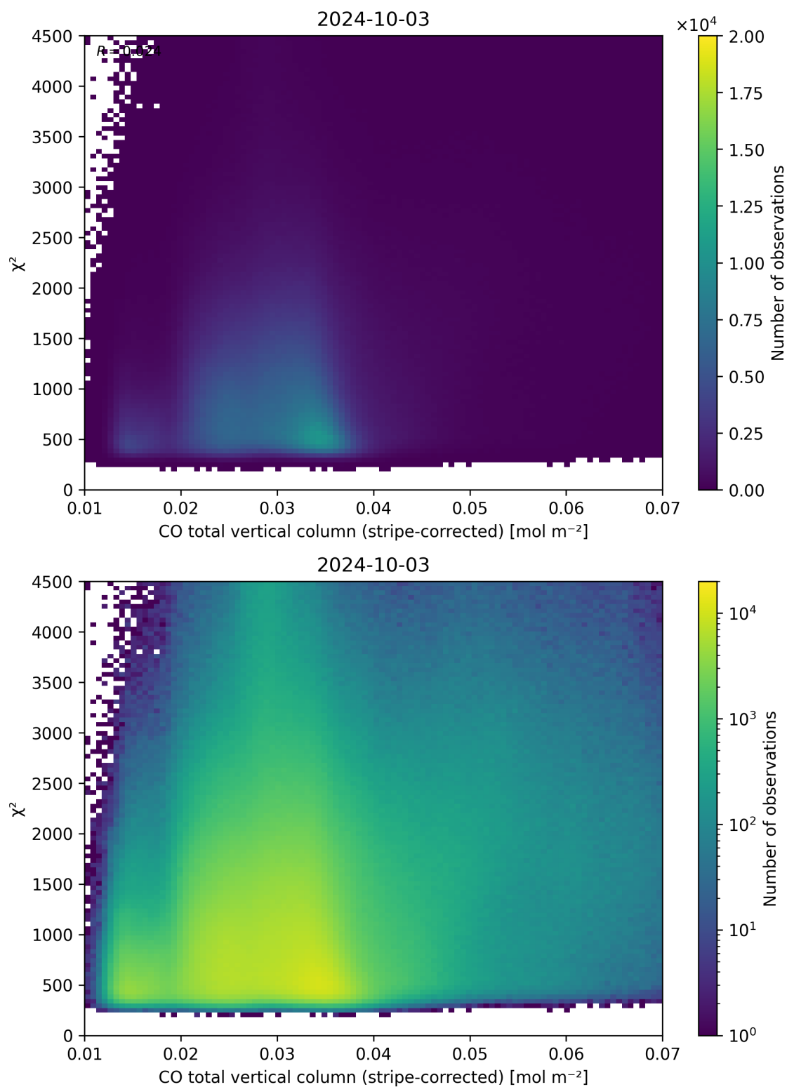
Figure 37: Scatter density plot of “CO total vertical column (stripe-corrected)” against “ \chi^2 ” for 2024-10-03 to 2024-10-04.
