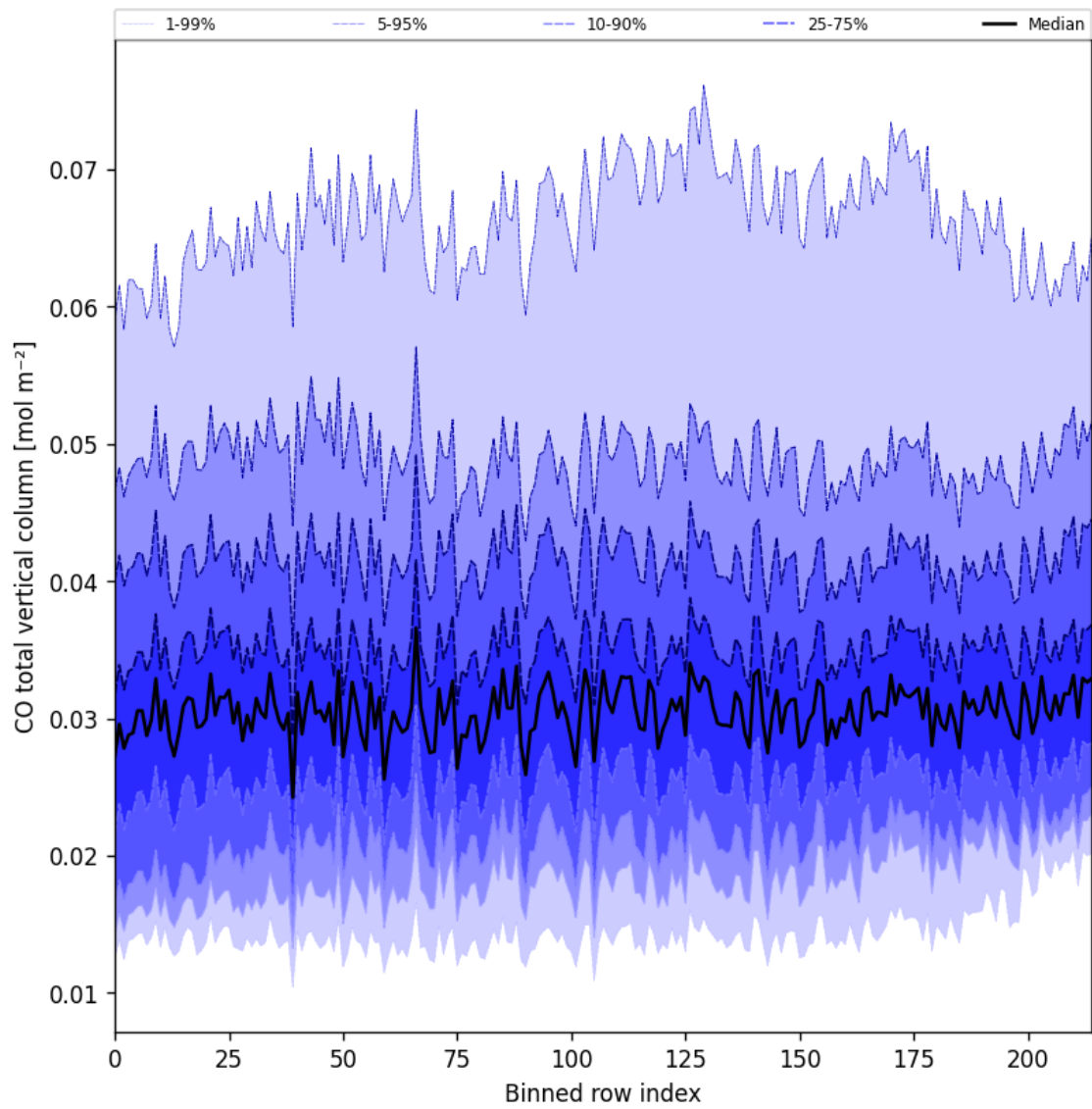
Figure 26: Along track statistics of “CO total vertical column” for 2024-10-03 to 2024-10-04
