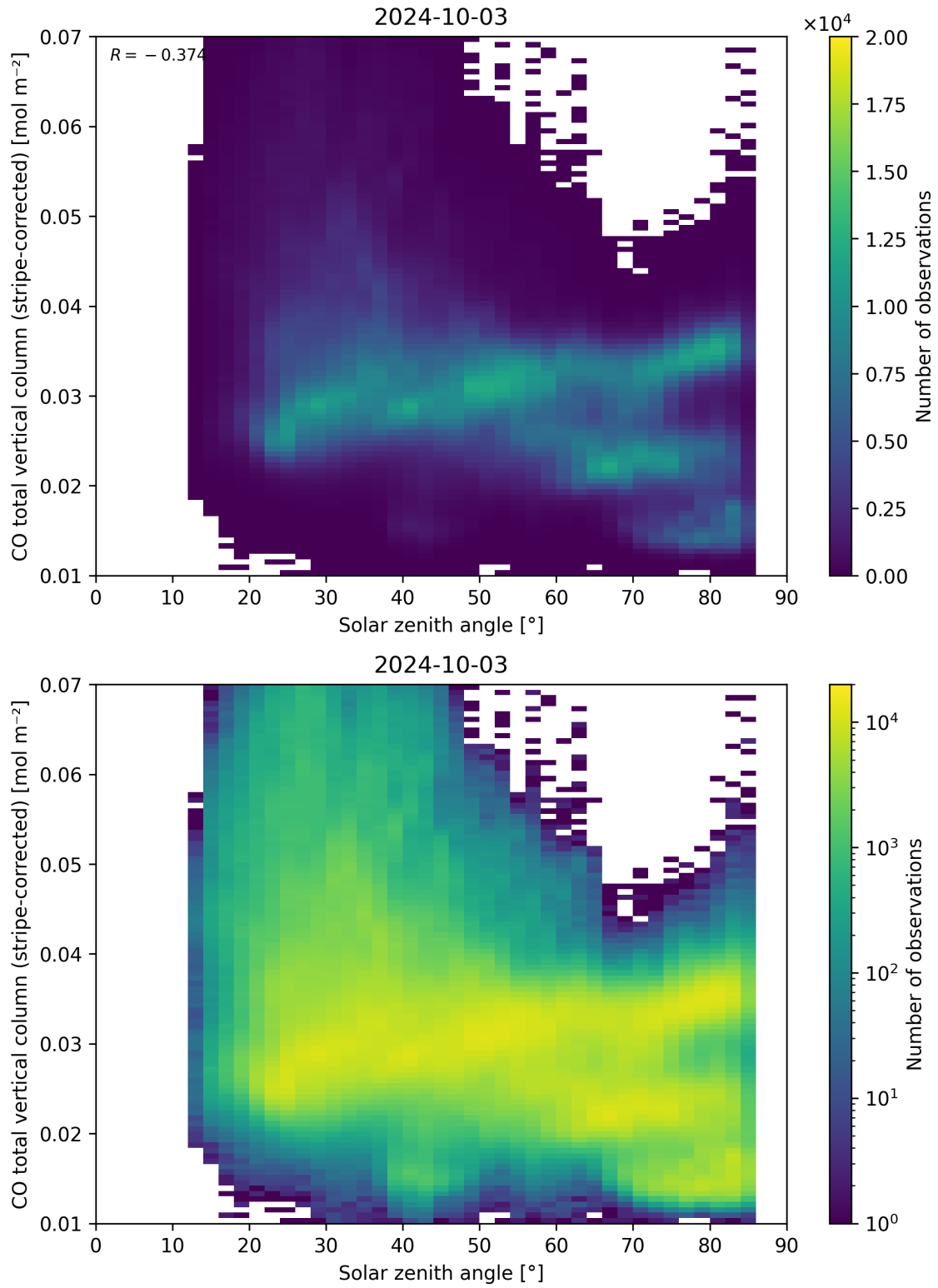
Figure 62: Scatter density plot of “Solar zenith angle” against “CO total vertical column (stripe-corrected)” for 2024-10-03 to 2024-10-04.
