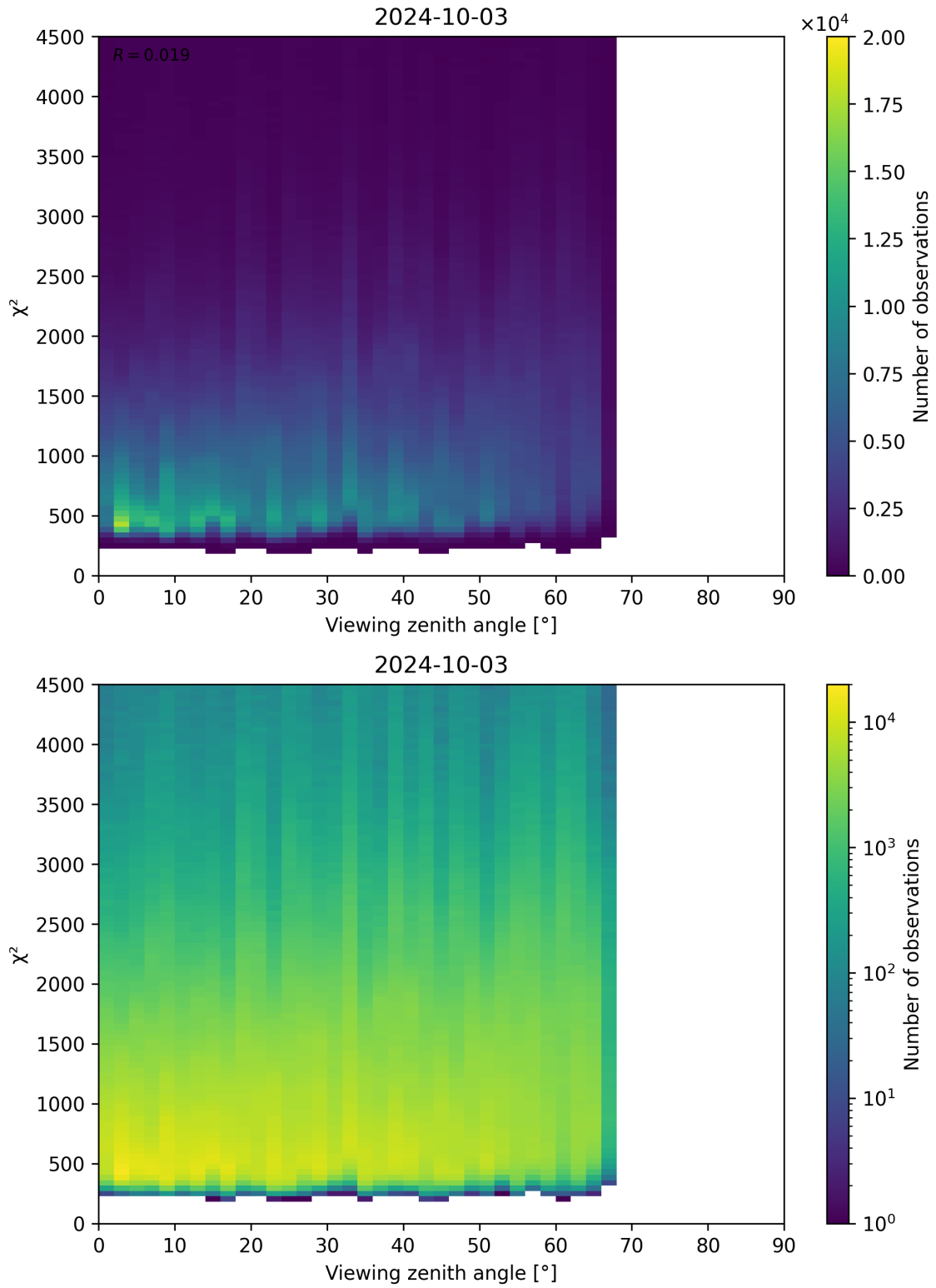
Figure 72: Scatter density plot of “Viewing zenith angle” against “ \chi^2 ” for 2024-10-03 to 2024-10-04.
