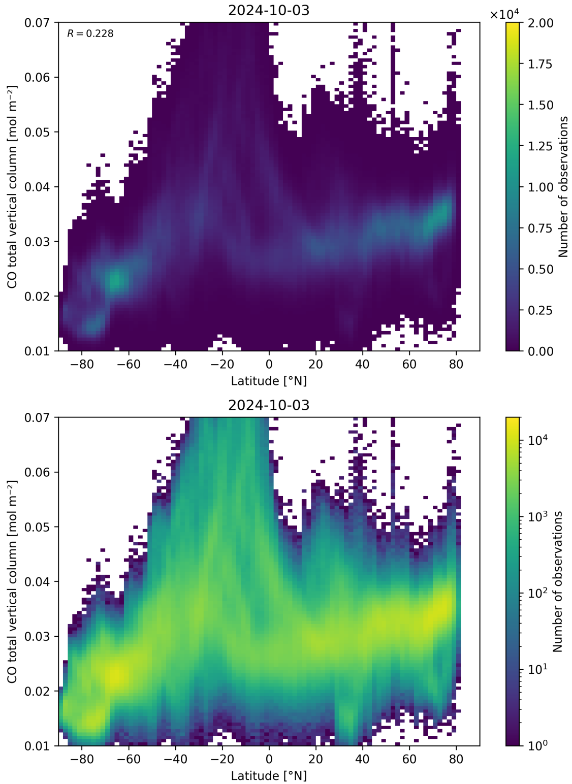
Figure 51: Scatter density plot of “Latitude” against “CO total vertical column” for 2024-10-03 to 2024-10-04.
