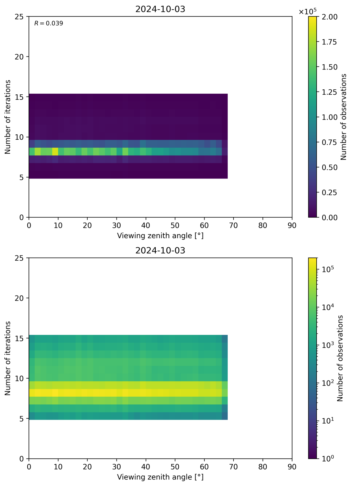
Figure 75: Scatter density plot of “Viewing zenith angle” against “Number of iterations” for 2024-10-03 to 2024-10-04.
