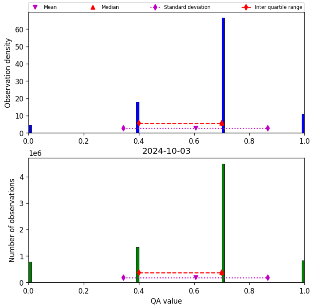
Figure 17: Histogram of “QA value” for 2024-10-03 to 2024-10-04
