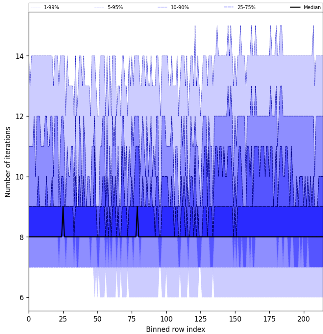
Figure 32: Along track statistics of “Number of iterations” for 2024-10-03 to 2024-10-04
