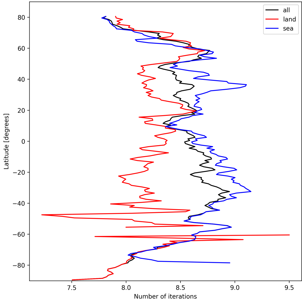
Figure 16: Zonal average of “Number of iterations” for 2024-10-03 to 2024-10-04.
