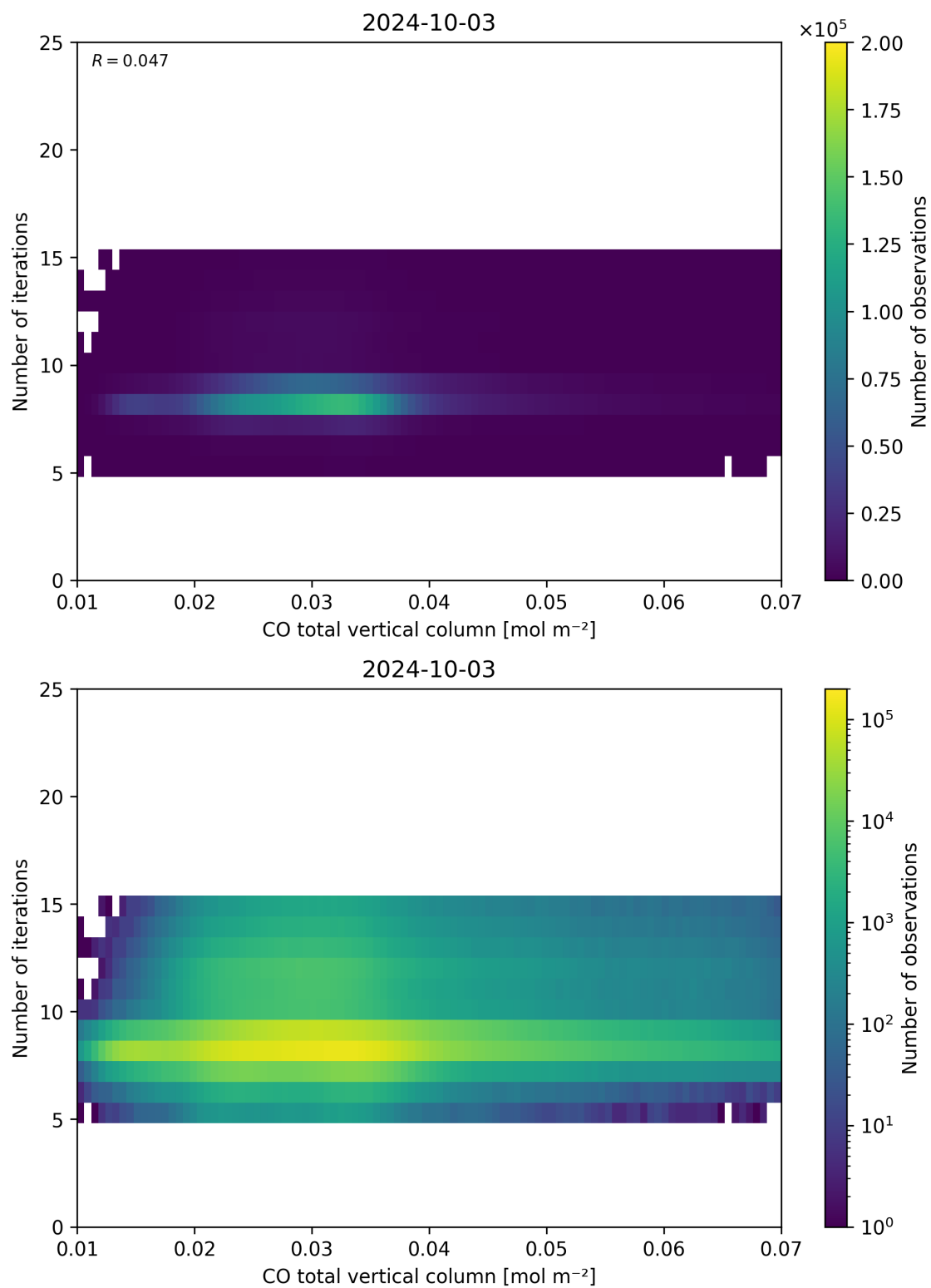
Figure 42: Scatter density plot of “CO total vertical column” against “Number of iterations” for 2024-10-03 to 2024-10-04.
