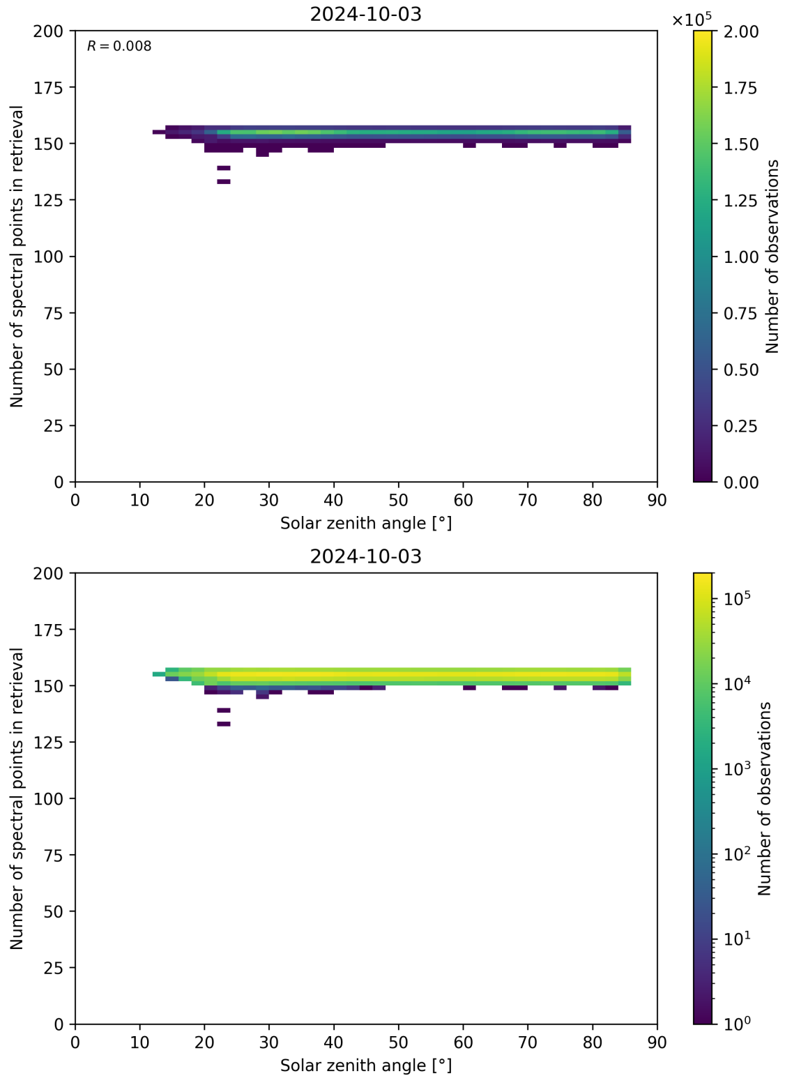
Figure 68: Scatter density plot of “Solar zenith angle” against “Number of spectral points in retrieval” for 2024-10-03 to 2024-10-04.
