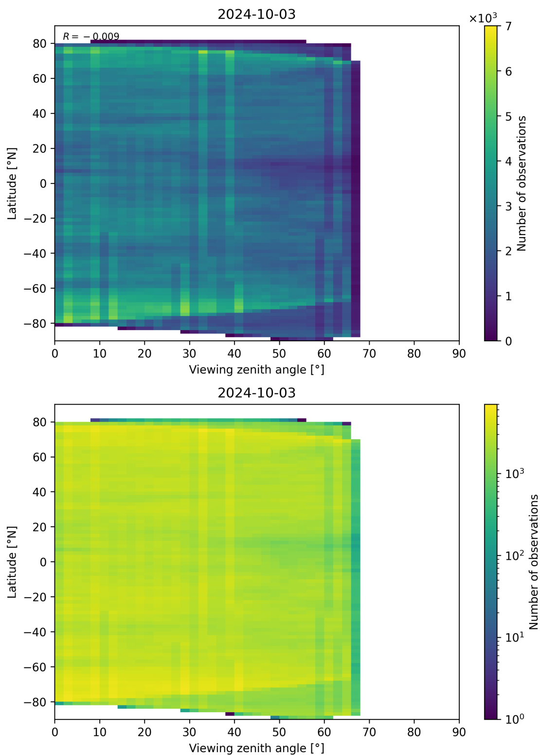
Figure 74: Scatter density plot of “Viewing zenith angle” against “Latitude” for 2024-10-03 to 2024-10-04.
