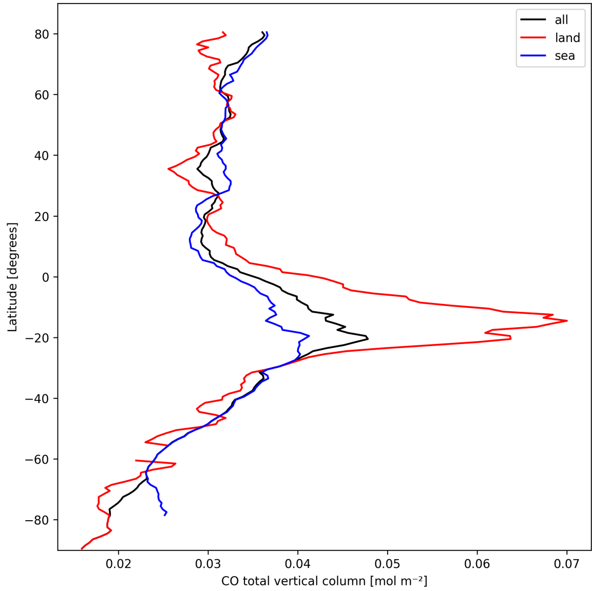
Figure 10: Zonal average of “CO total vertical column” for 2024-10-03 to 2024-10-04.
