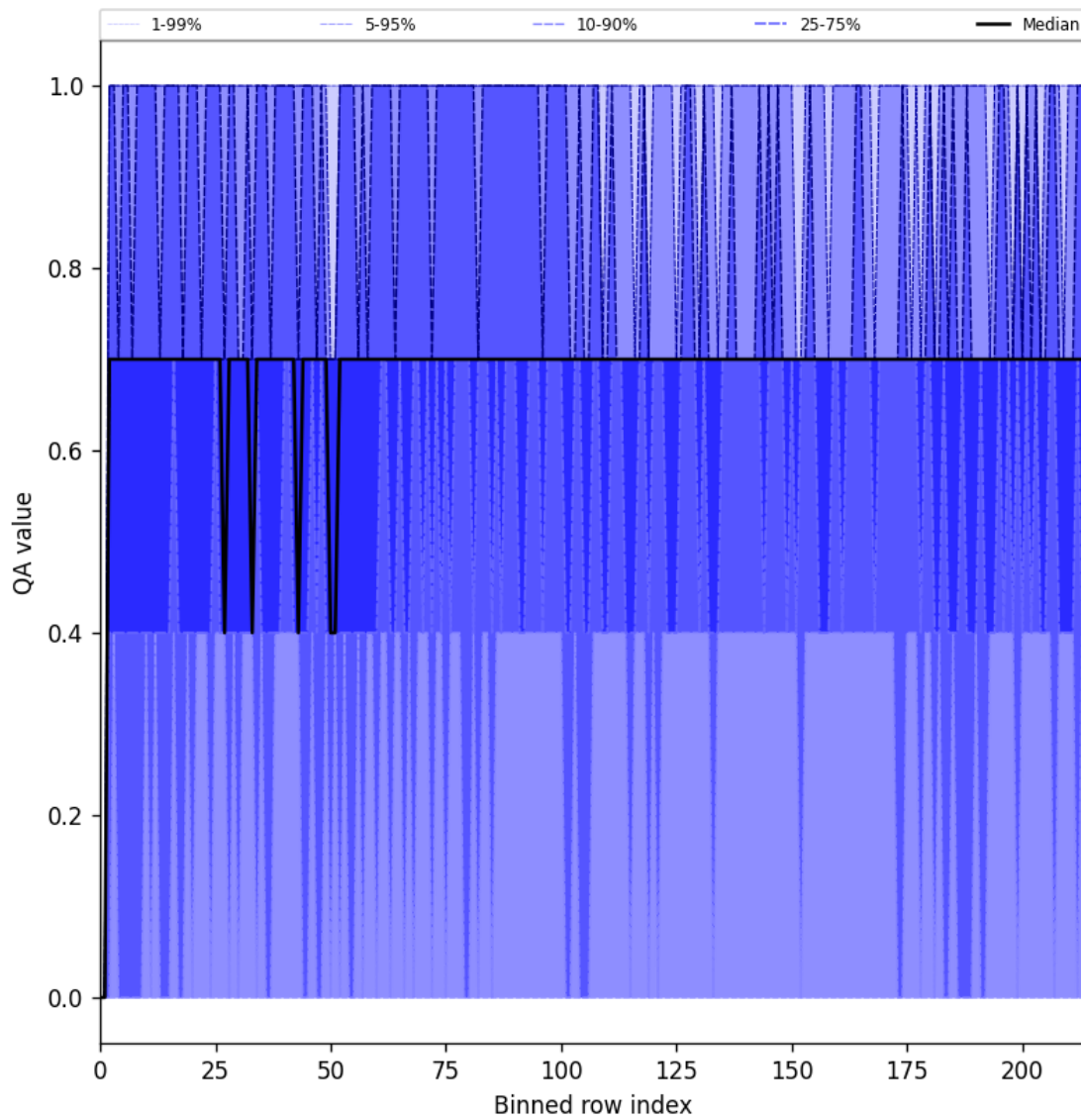
Figure 25: Along track statistics of “QA value” for 2024-10-03 to 2024-10-04
