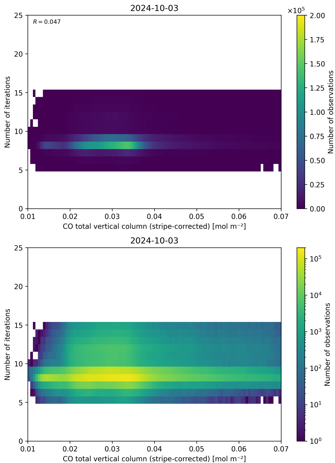
Figure 39: Scatter density plot of “CO total vertical column (stripe-corrected)” against “Number of iterations” for 2024-10-03 to 2024-10-04.
