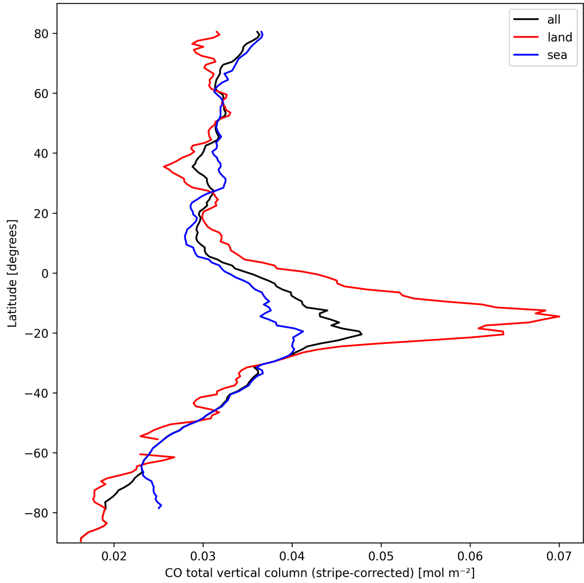
Figure 11: Zonal average of “CO total vertical column (stripe-corrected)” for 2024-10-03 to 2024-10-04.
