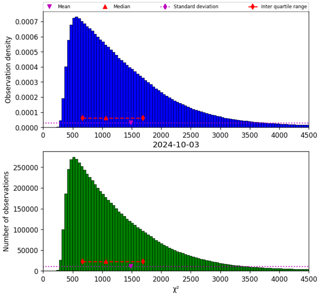
Figure 22: Histogram of “ \chi^2 ” for 2024-10-03 to 2024-10-04
