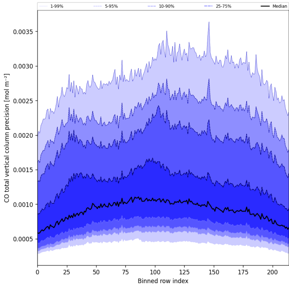
Figure 28: Along track statistics of “CO total vertical column precision” for 2024-10-03 to 2024-10-04
