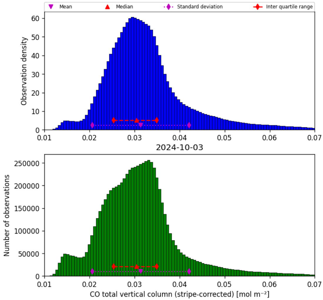
Figure 19: Histogram of “CO total vertical column (stripe-corrected)” for 2024-10-03 to 2024-10-04
