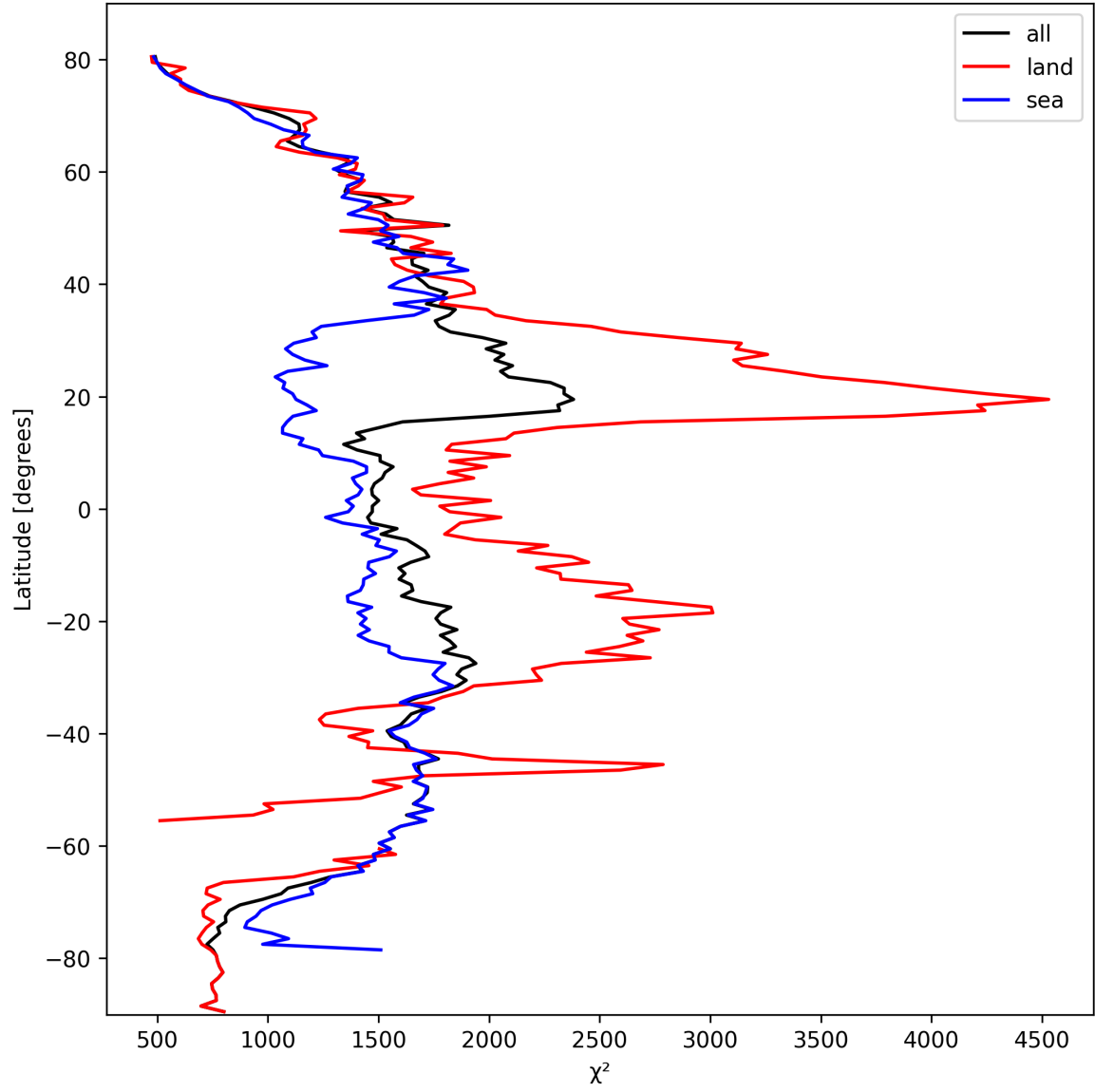
Figure 14: Zonal average of “ \chi^2 ” for 2024-10-03 to 2024-10-04.
