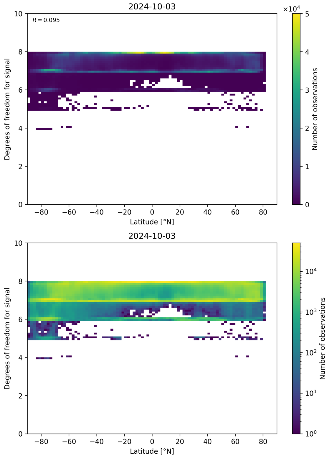
Figure 55: Scatter density plot of “Latitude” against “Degrees of freedom for signal” for 2024-10-03 to 2024-10-04.
