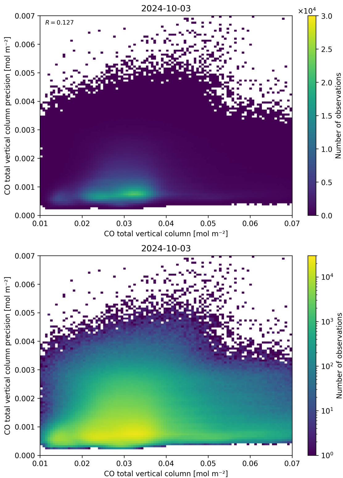
Figure 34: Scatter density plot of “CO total vertical column” against “CO total vertical column precision” for 2024-10-03 to 2024-10-04.
