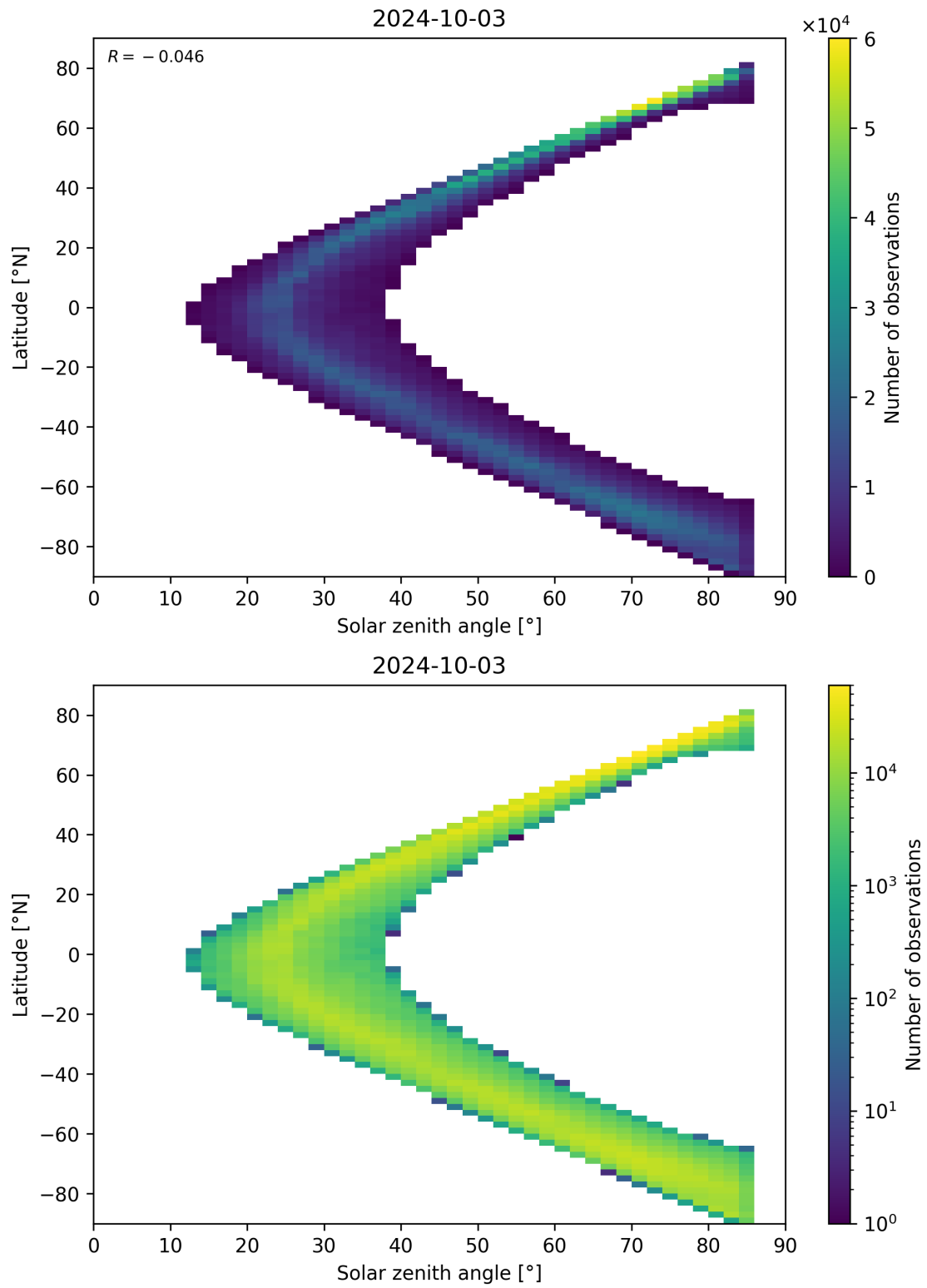
Figure 66: Scatter density plot of “Solar zenith angle” against “Latitude” for 2024-10-03 to 2024-10-04.
