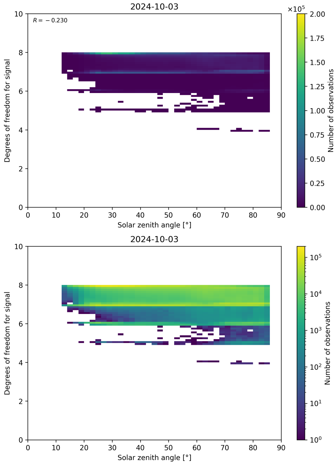
Figure 65: Scatter density plot of “Solar zenith angle” against “Degrees of freedom for signal” for 2024-10-03 to 2024-10-04.
