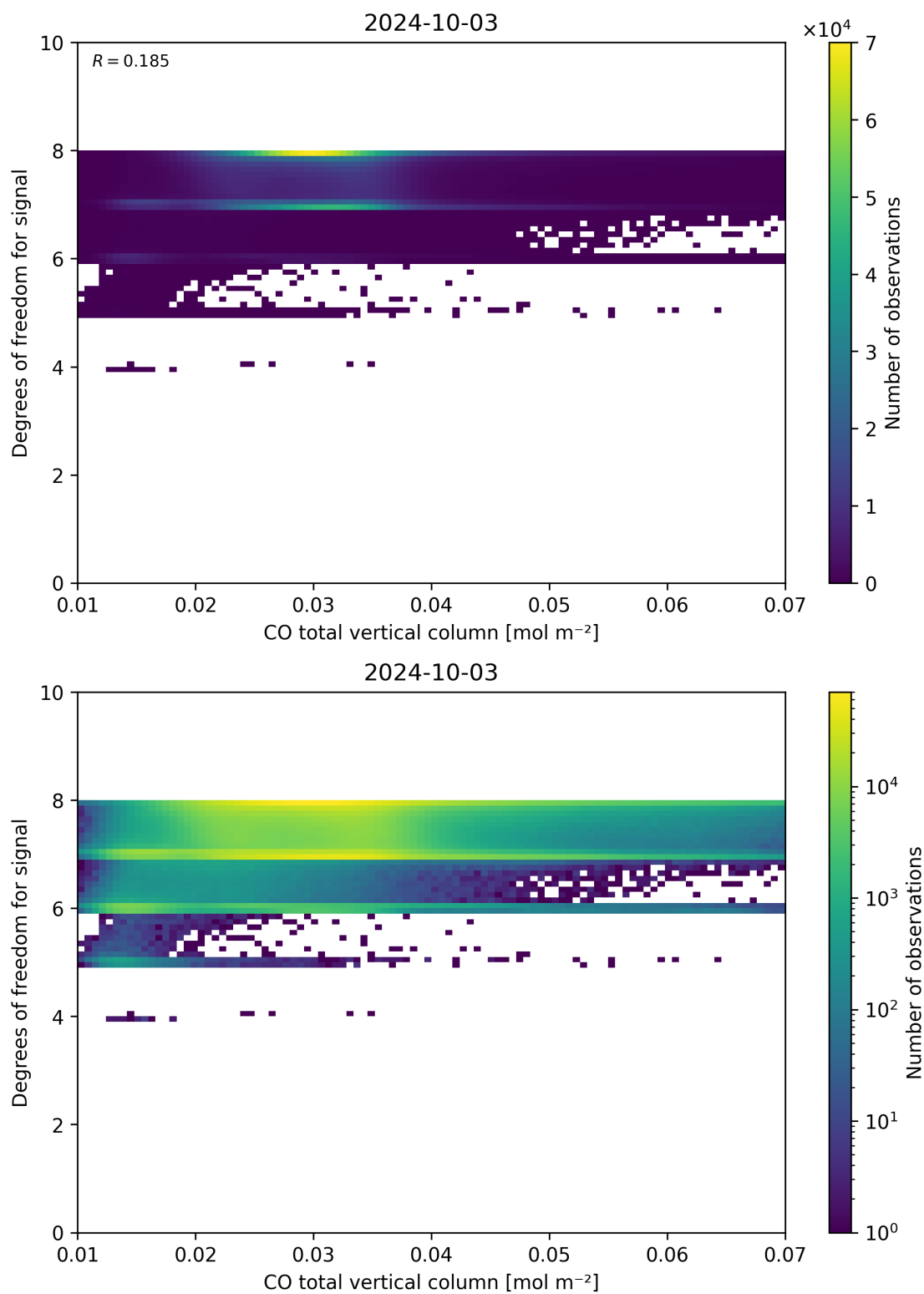
Figure 41: Scatter density plot of “CO total vertical column” against “Degrees of freedom for signal” for 2024-10-03 to 2024-10-04.
