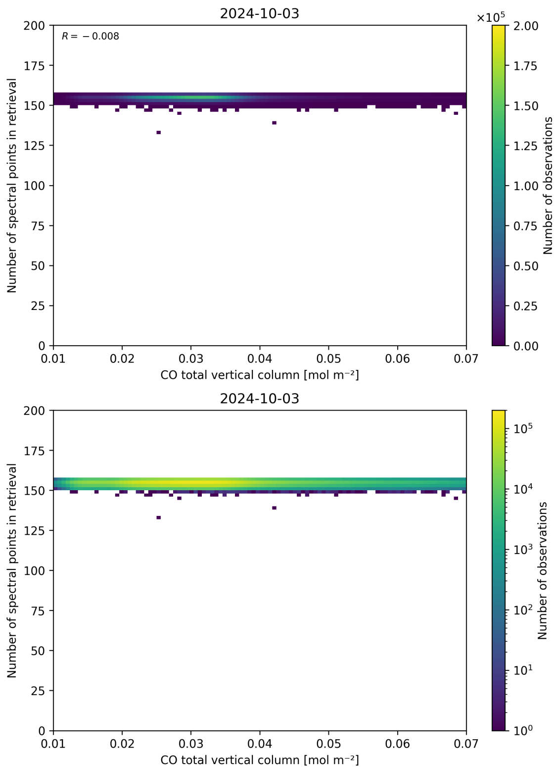
Figure 43: Scatter density plot of “CO total vertical column” against “Number of spectral points in retrieval” for 2024-10-03 to 2024-10-04.
