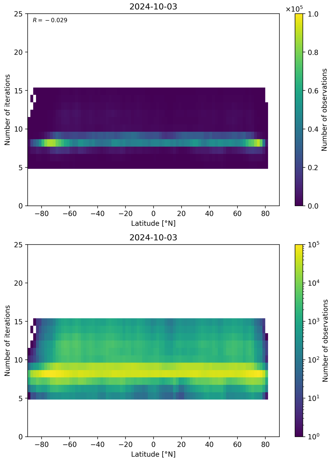
Figure 56: Scatter density plot of “Latitude” against “Number of iterations” for 2024-10-03 to 2024-10-04.
