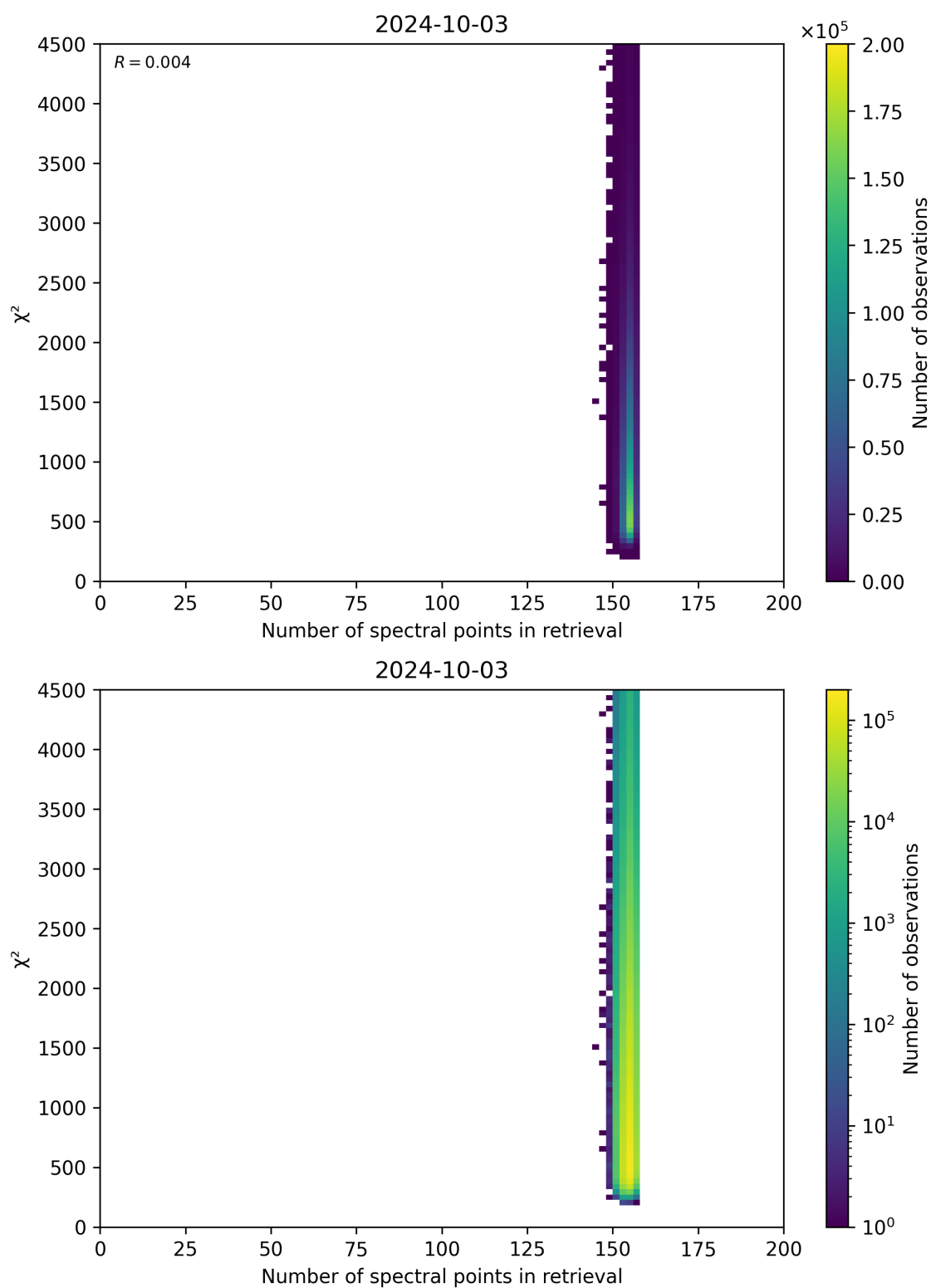
Figure 58: Scatter density plot of “Number of spectral points in retrieval” against “ \chi^2 ” for 2024-10-03 to 2024-10-04.
