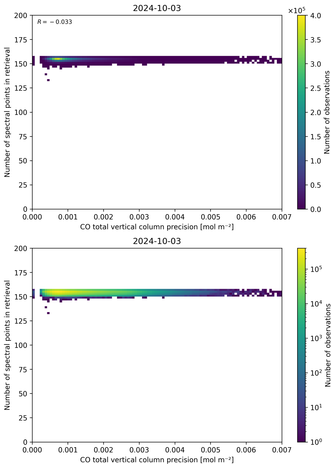
Figure 47: Scatter density plot of “CO total vertical column precision” against “Number of spectral points in retrieval” for 2024-10-03 to 2024-10-04.
