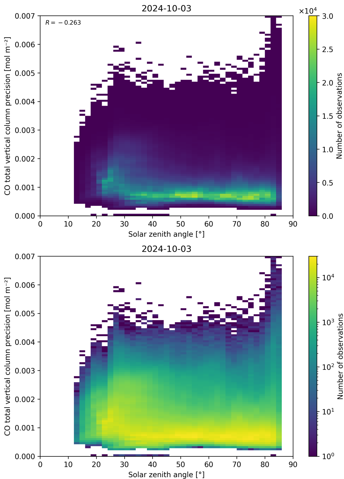
Figure 63: Scatter density plot of “Solar zenith angle” against “CO total vertical column precision” for 2024-10-03 to 2024-10-04.
