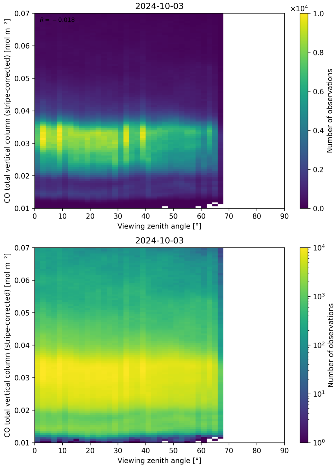
Figure 70: Scatter density plot of “Viewing zenith angle” against “CO total vertical column (stripe-corrected)” for 2024-10-03 to 2024-10-04.
