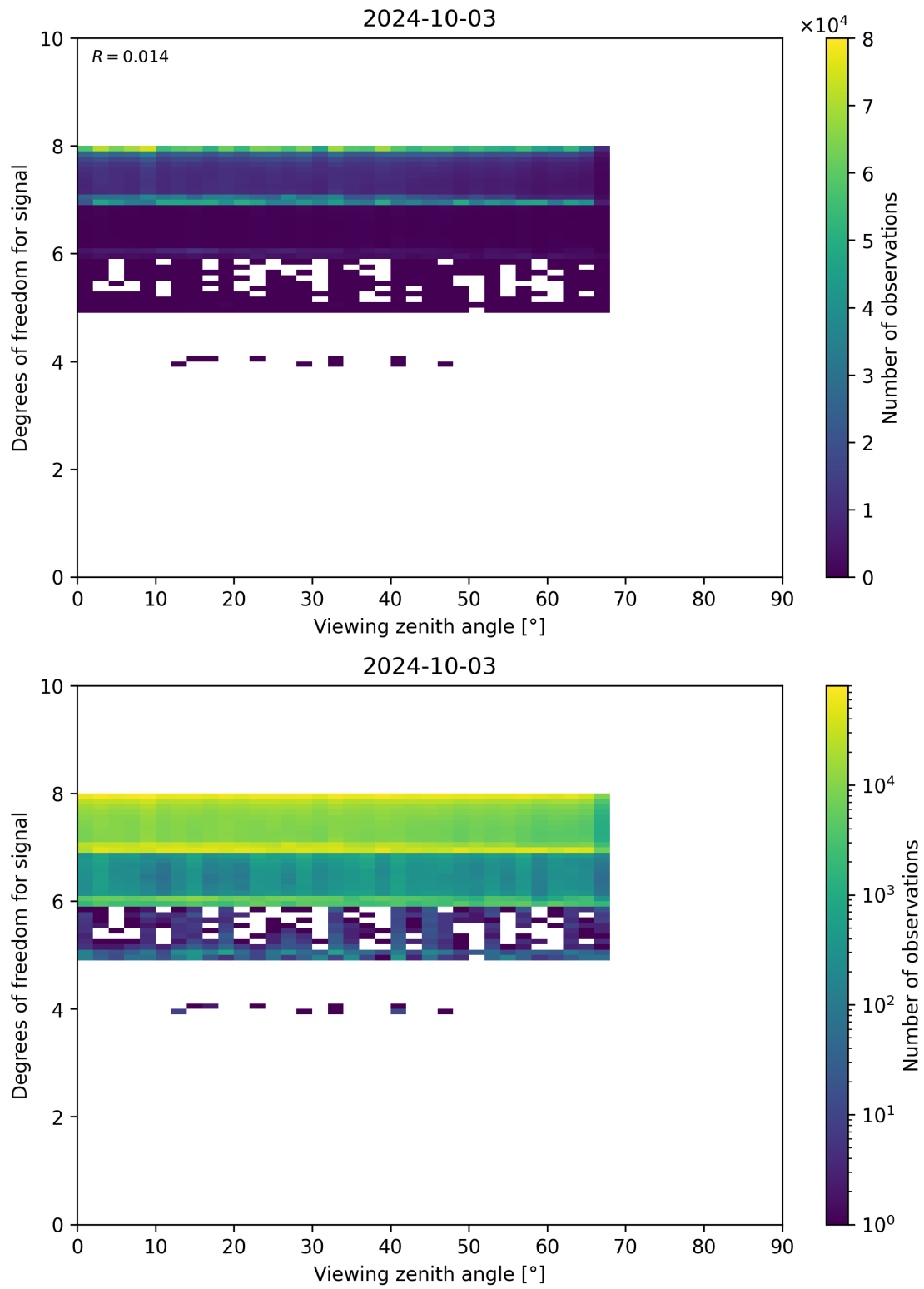
Figure 73: Scatter density plot of “Viewing zenith angle” against “Degrees of freedom for signal” for 2024-10-03 to 2024-10-04.
