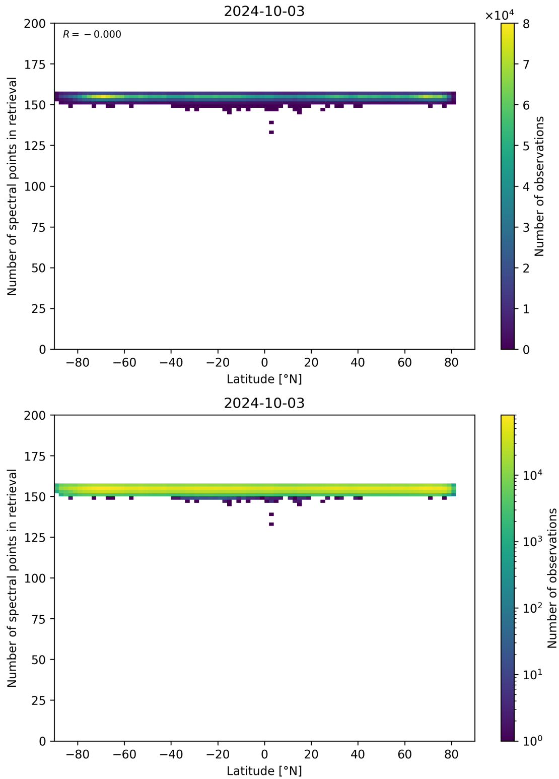
Figure 57: Scatter density plot of “Latitude” against “Number of spectral points in retrieval” for 2024-10-03 to 2024-10-04.
