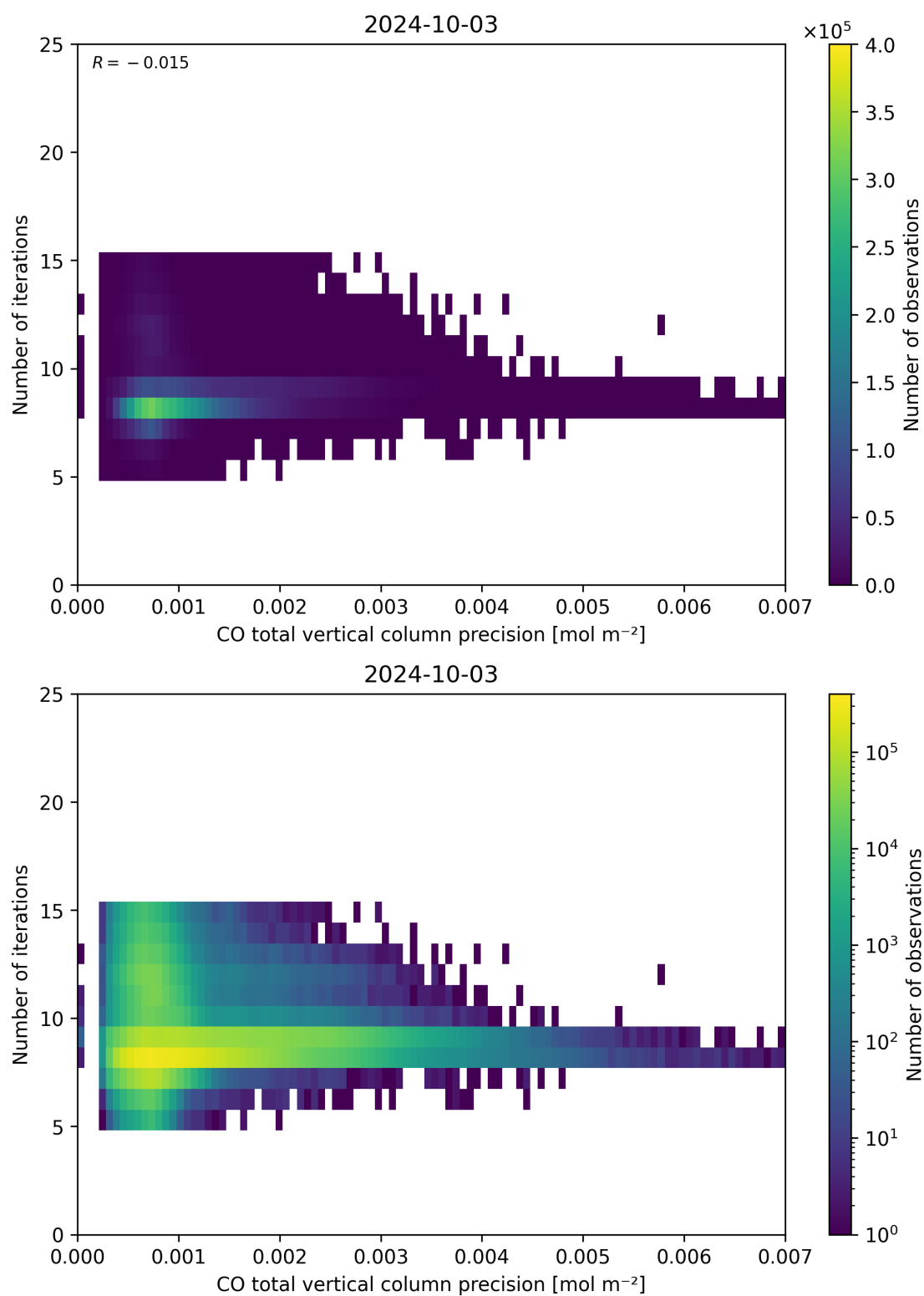
Figure 46: Scatter density plot of “CO total vertical column precision” against “Number of iterations” for 2024-10-03 to 2024-10-04.
