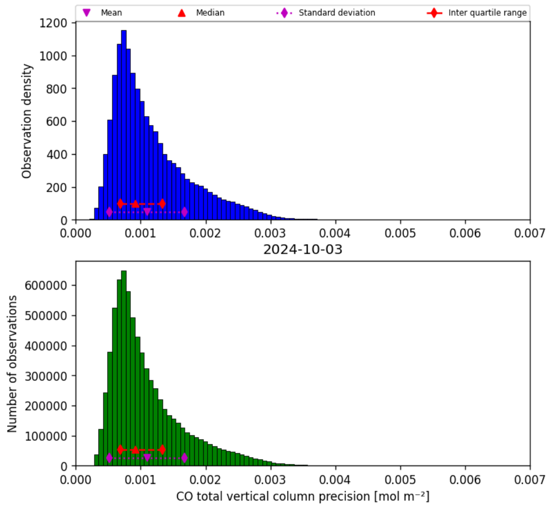
Figure 20: Histogram of “CO total vertical column precision” for 2024-10-03 to 2024-10-04
