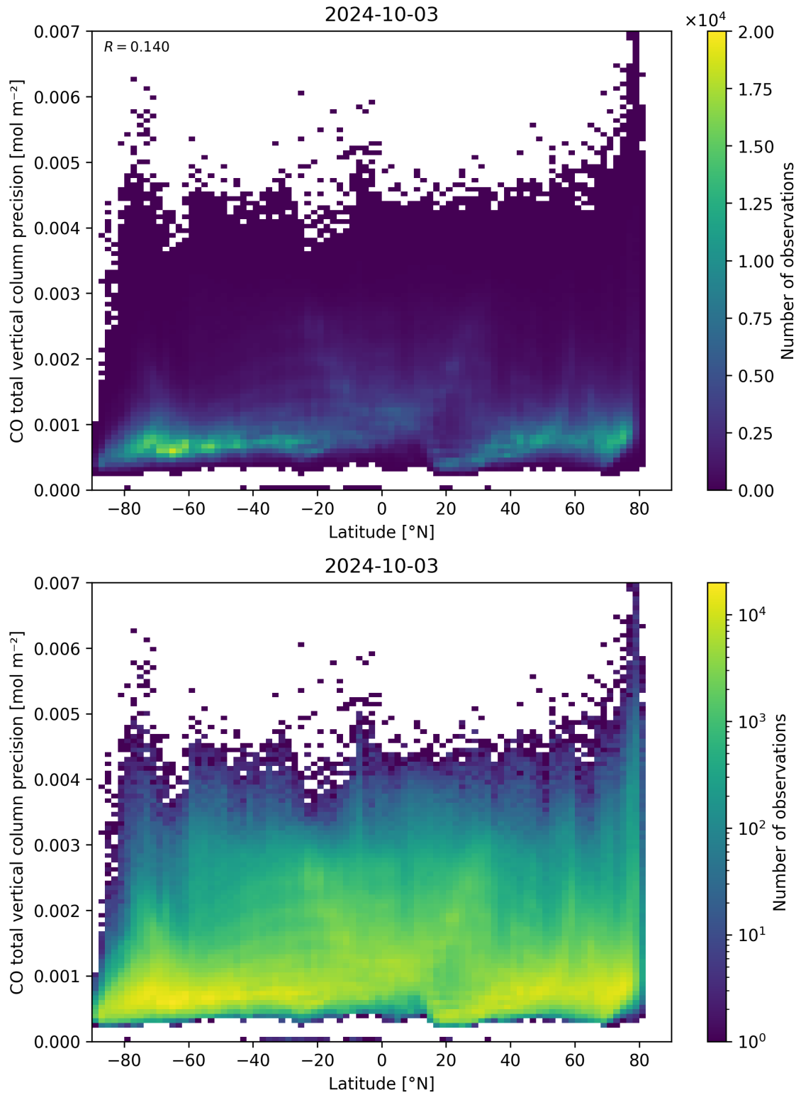
Figure 53: Scatter density plot of “Latitude” against “CO total vertical column precision” for 2024-10-03 to 2024-10-04.
