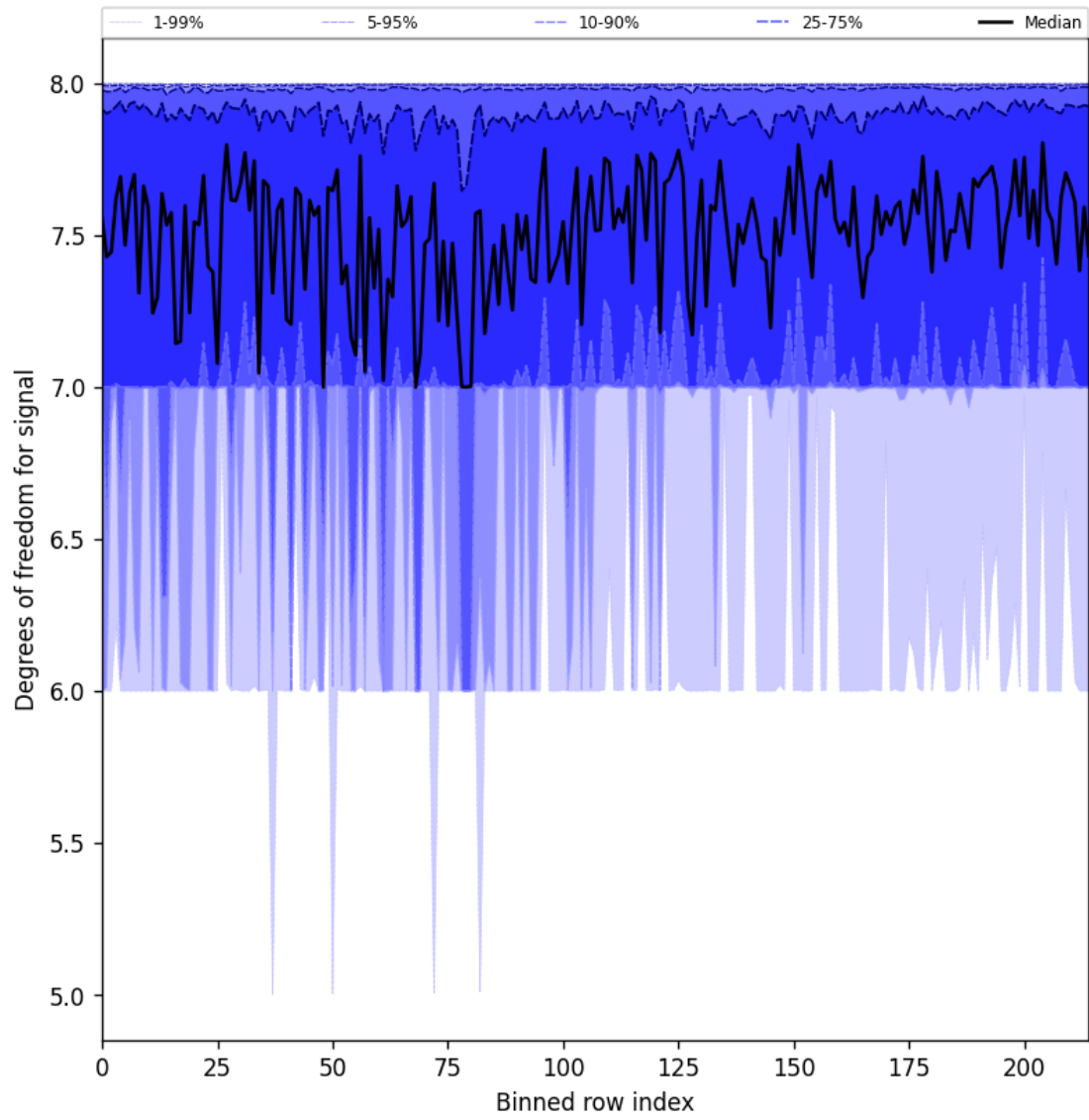
Figure 31: Along track statistics of “Degrees of freedom for signal” for 2024-10-03 to 2024-10-04
