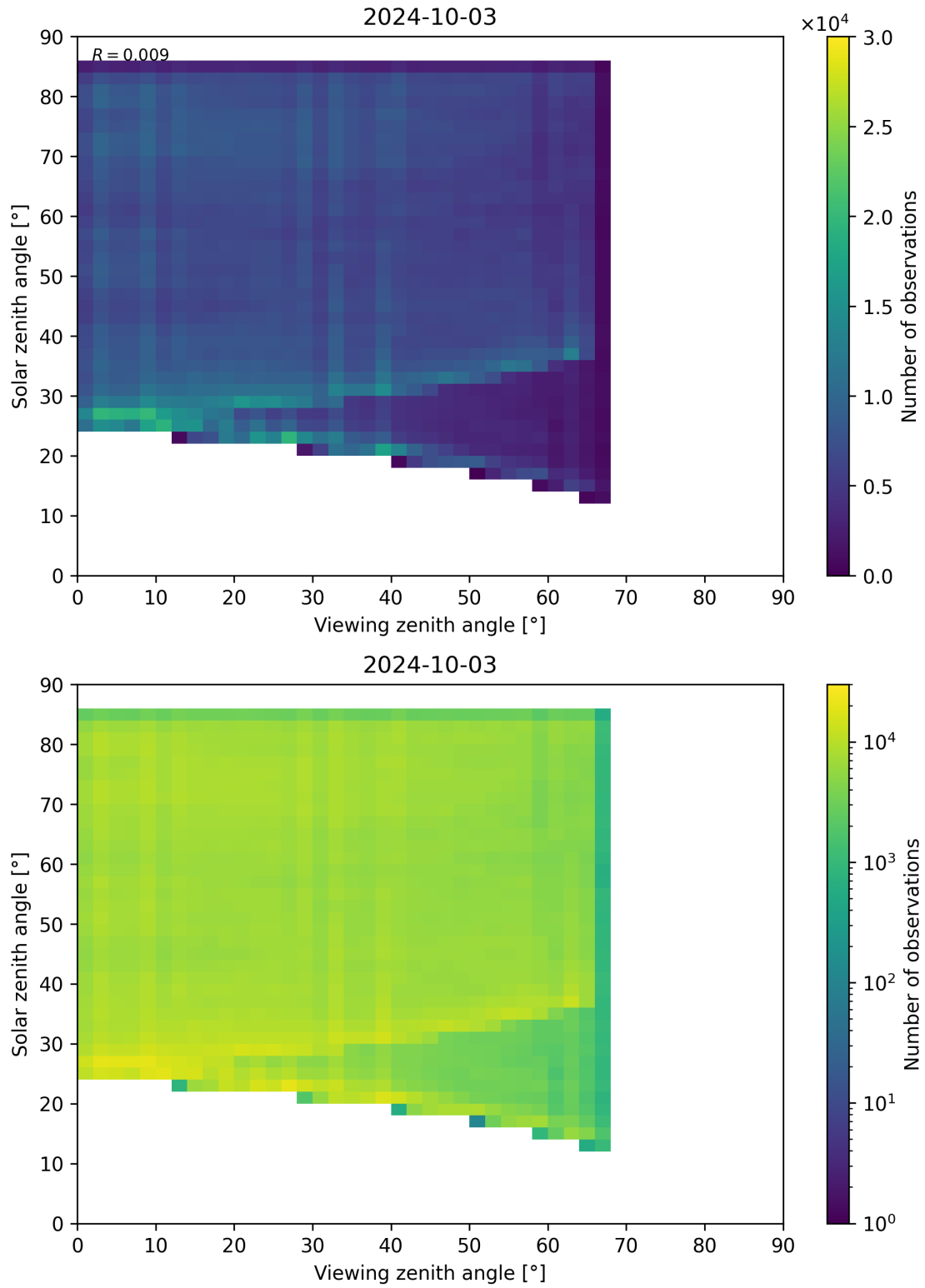
Figure 77: Scatter density plot of “Viewing zenith angle” against “Solar zenith angle” for 2024-10-03 to 2024-10-04.
