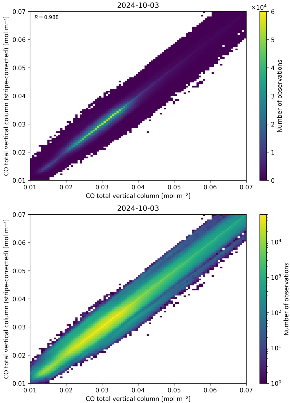
Figure 33: Scatter density plot of “CO total vertical column” against “CO total vertical column (stripe-corrected)” for 2024-10-03 to 2024-10-04.
