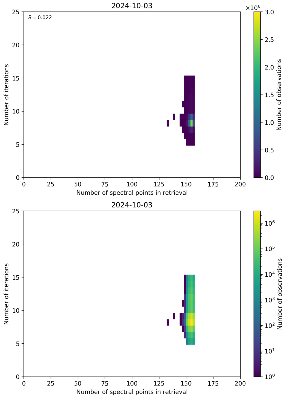
Figure 60: Scatter density plot of “Number of spectral points in retrieval” against “Number of iterations” for 2024-10-03 to 2024-10-04.
