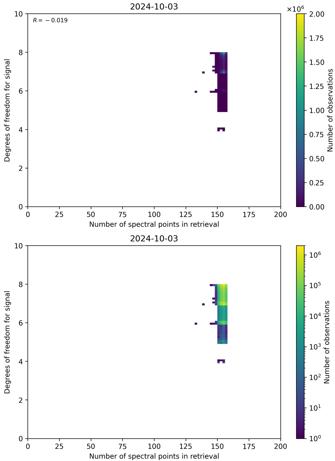
Figure 59: Scatter density plot of “Number of spectral points in retrieval” against “Degrees of freedom for signal” for 2024-10-03 to 2024-10-04.
