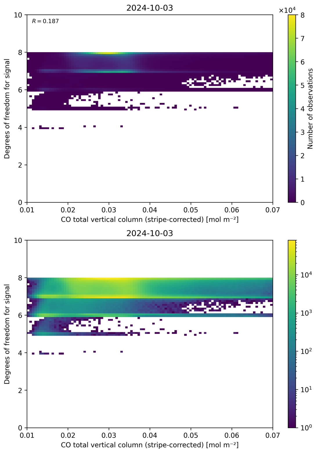
Figure 38: Scatter density plot of “CO total vertical column (stripe-corrected)” against “Degrees of freedom for signal” for 2024-10-03 to 2024-10-04.
