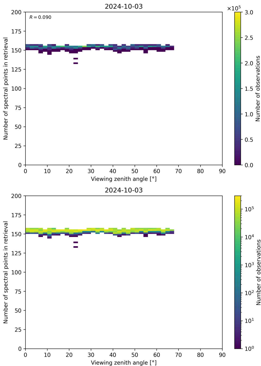
Figure 76: Scatter density plot of “Viewing zenith angle” against “Number of spectral points in retrieval” for 2024-10-03 to 2024-10-04.
