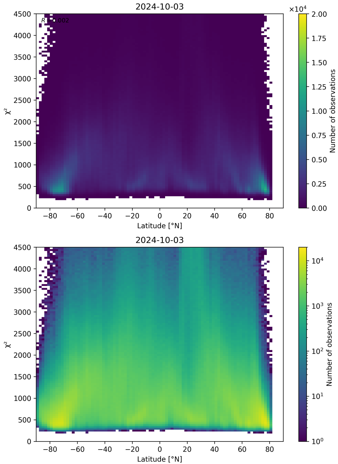
Figure 54: Scatter density plot of “Latitude” against “ \chi^2 ” for 2024-10-03 to 2024-10-04.
