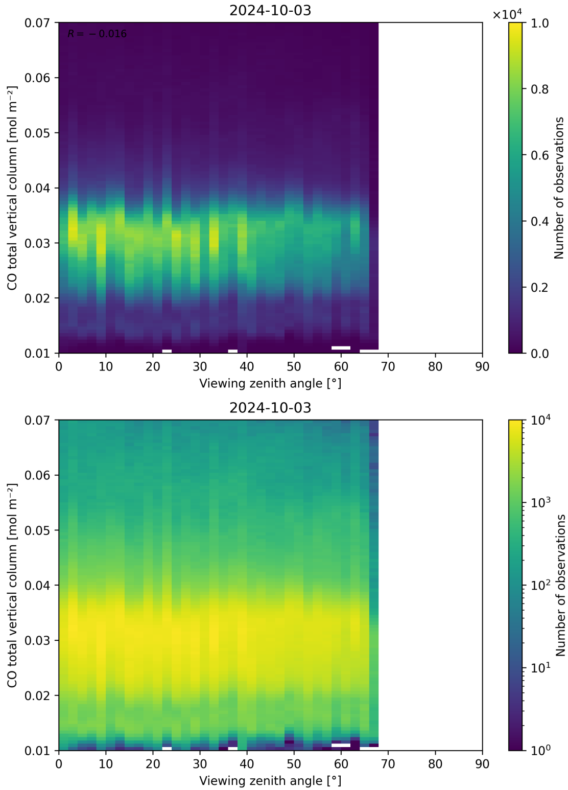
Figure 69: Scatter density plot of “Viewing zenith angle” against “CO total vertical column” for 2024-10-03 to 2024-10-04.
