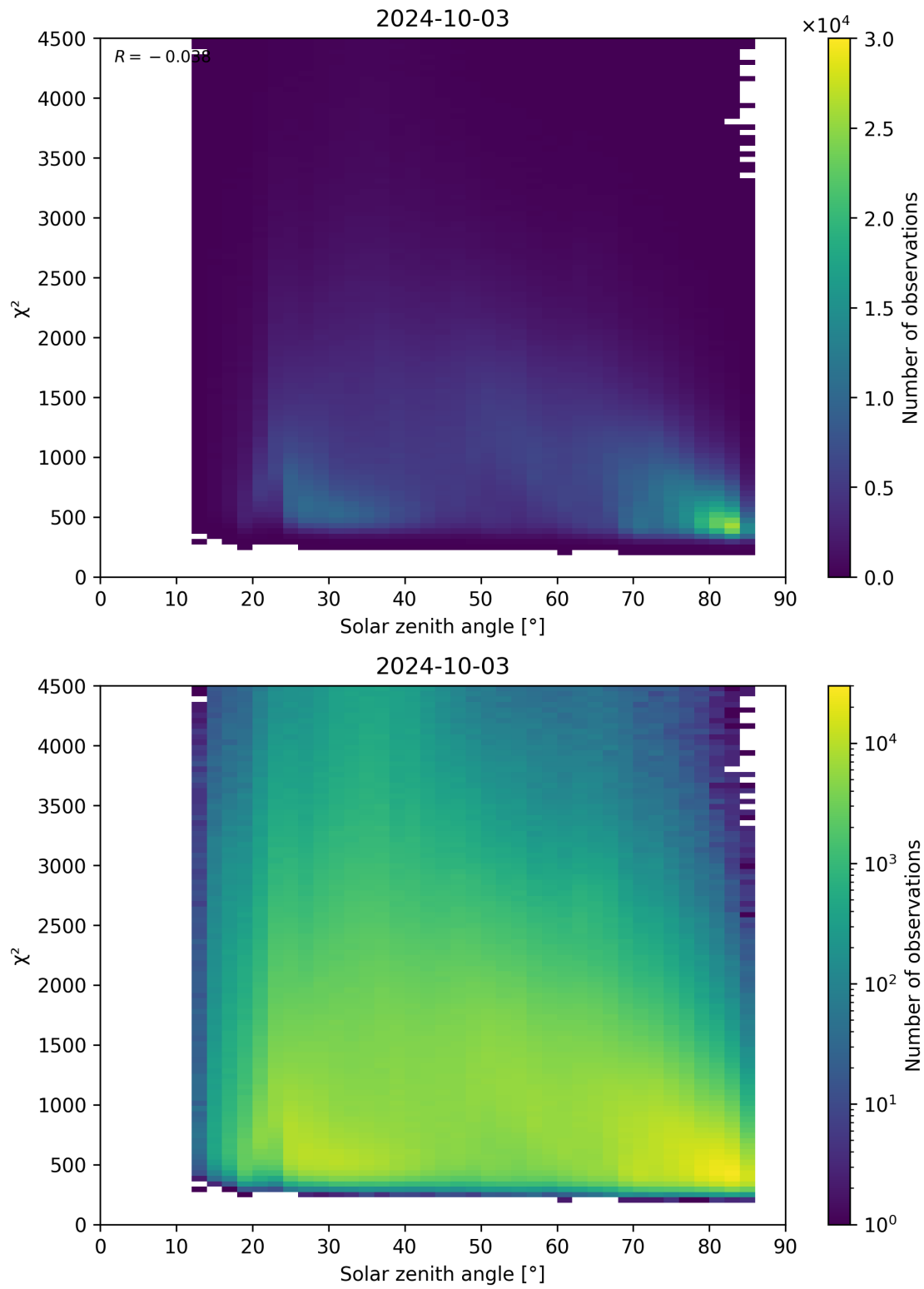
Figure 64: Scatter density plot of “Solar zenith angle” against “ \chi^2 ” for 2024-10-03 to 2024-10-04.
