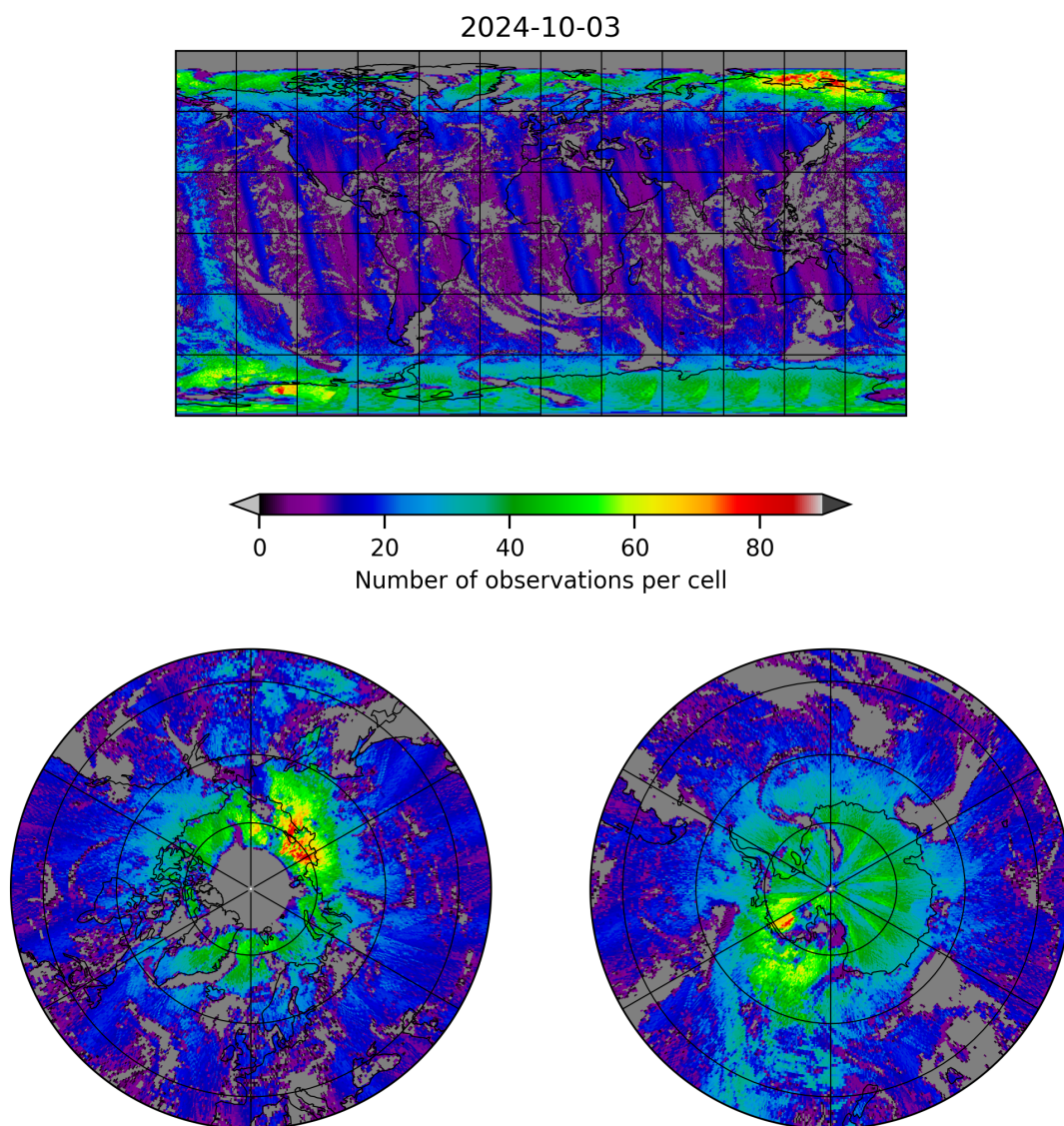
Figure 8: Map of the number of observations for 2024-10-03 to 2024-10-04
