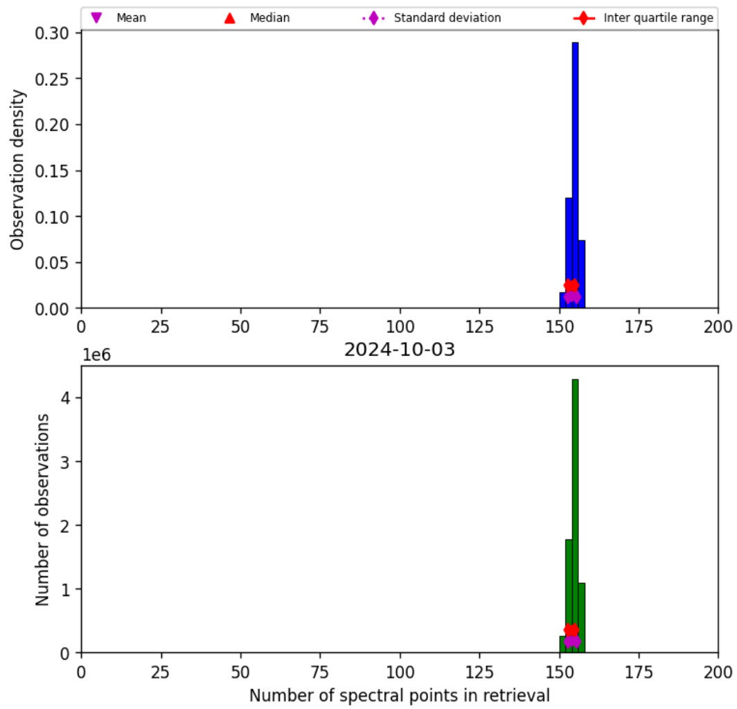
Figure 21: Histogram of “Number of spectral points in retrieval” for 2024-10-03 to 2024-10-04
