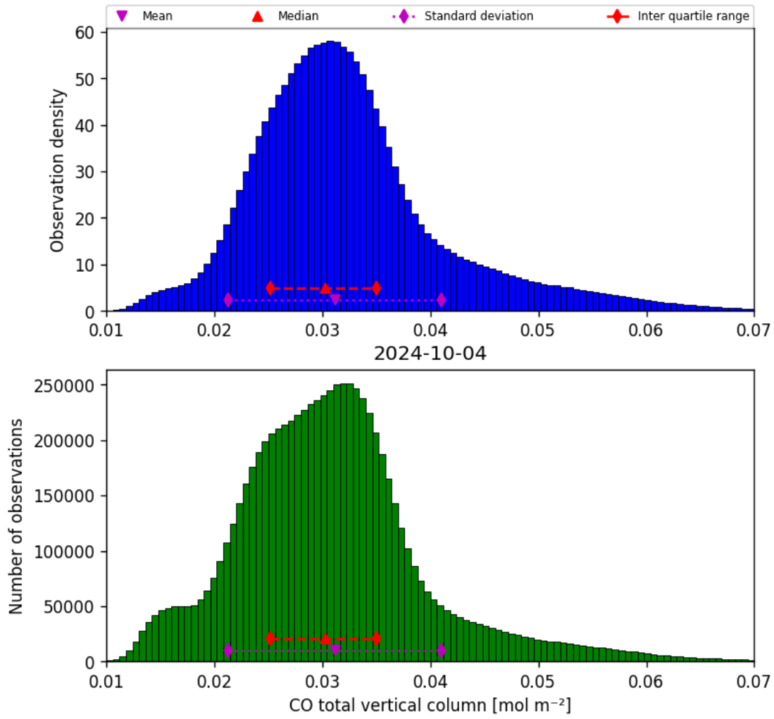
Figure 18: Histogram of “CO total vertical column” for 2024-10-03 to 2024-10-05
