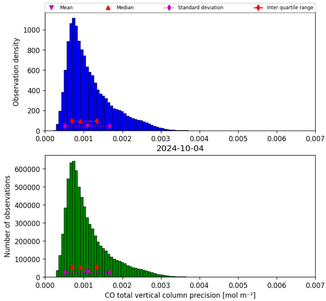
Figure 20: Histogram of “CO total vertical column precision” for 2024-10-03 to 2024-10-05
