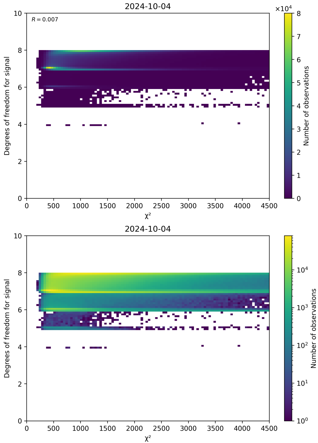
Figure 48: Scatter density plot of “ \chi^2 ” against “Degrees of freedom for signal” for 2024-10-03 to 2024-10-05.
