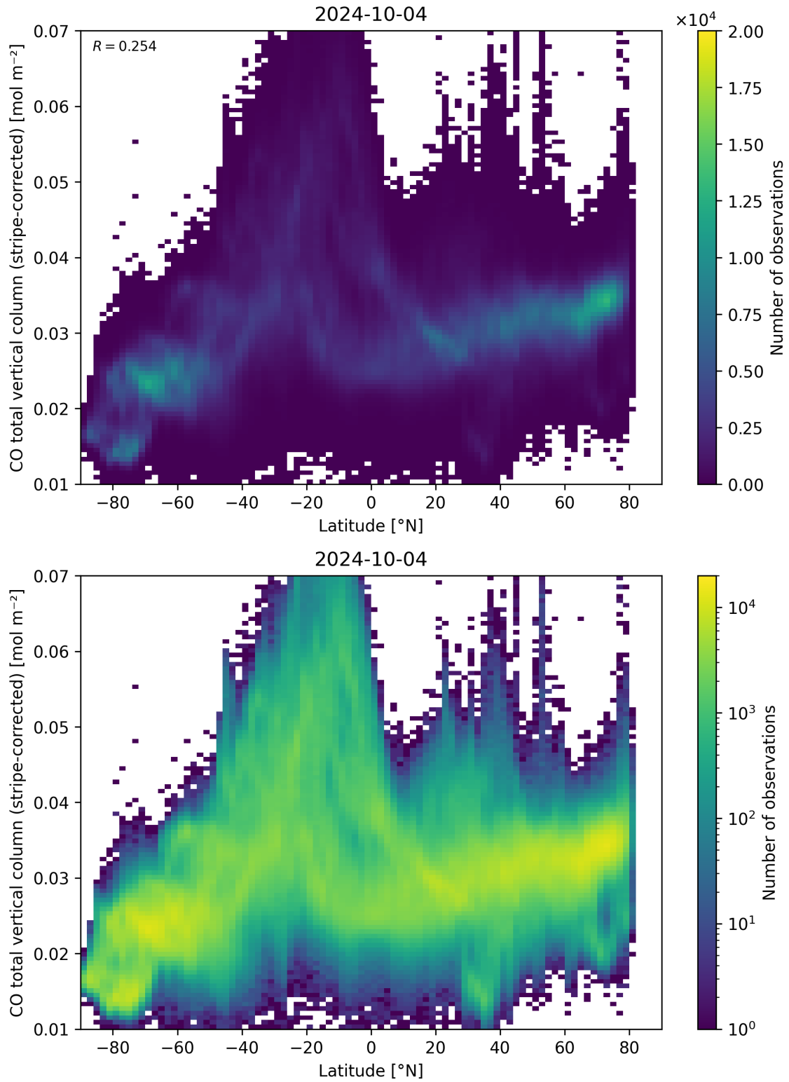
Figure 52: Scatter density plot of “Latitude” against “CO total vertical column (stripe-corrected)” for 2024-10-03 to 2024-10-05.
