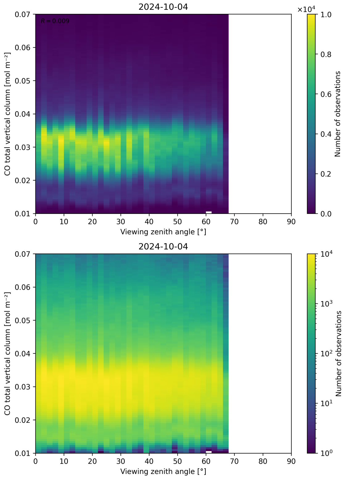
Figure 69: Scatter density plot of “Viewing zenith angle” against “CO total vertical column” for 2024-10-03 to 2024-10-05.
