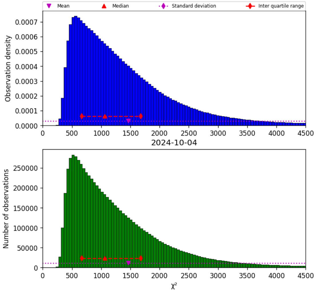
Figure 22: Histogram of “ \chi^2 ” for 2024-10-03 to 2024-10-05
