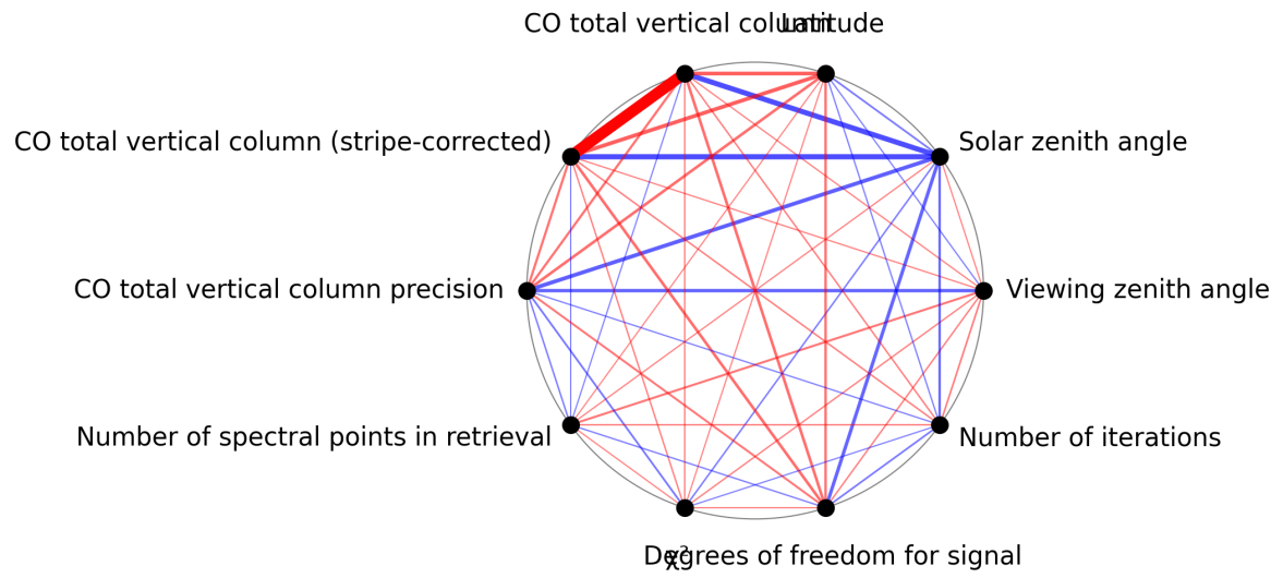
Figure 1: Map of correlation graph for 2024-10-03 to 2024-10-05.
