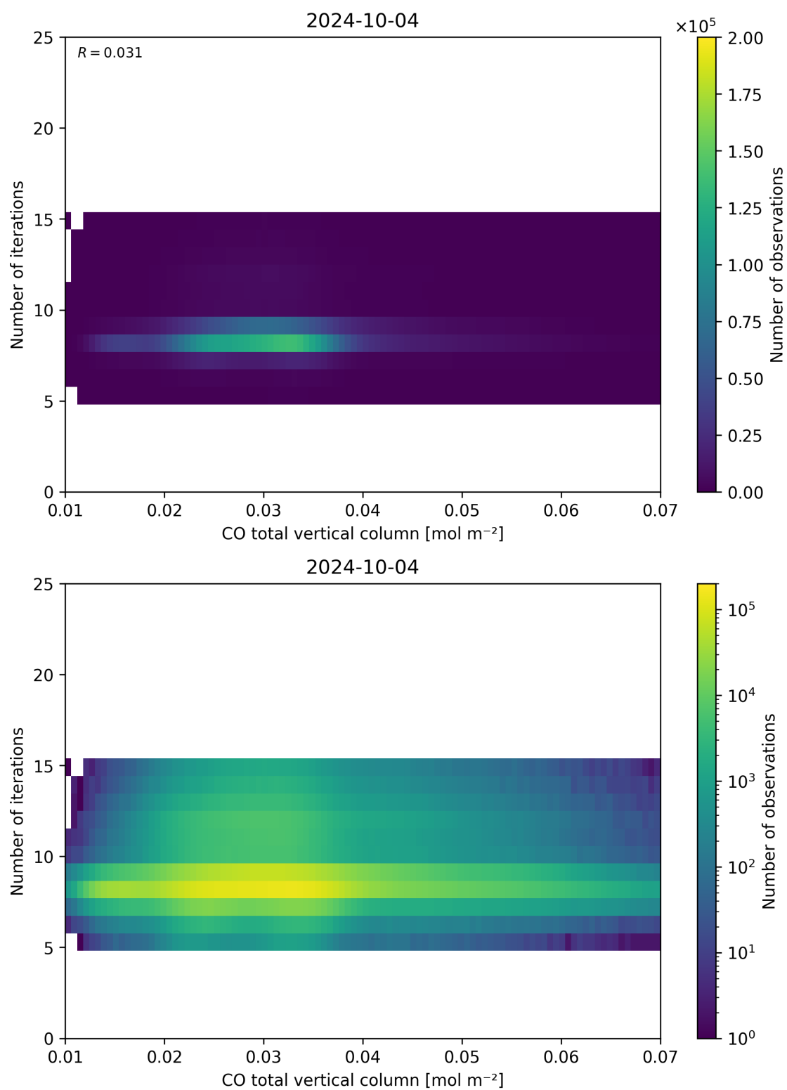
Figure 42: Scatter density plot of “CO total vertical column” against “Number of iterations” for 2024-10-03 to 2024-10-05.
