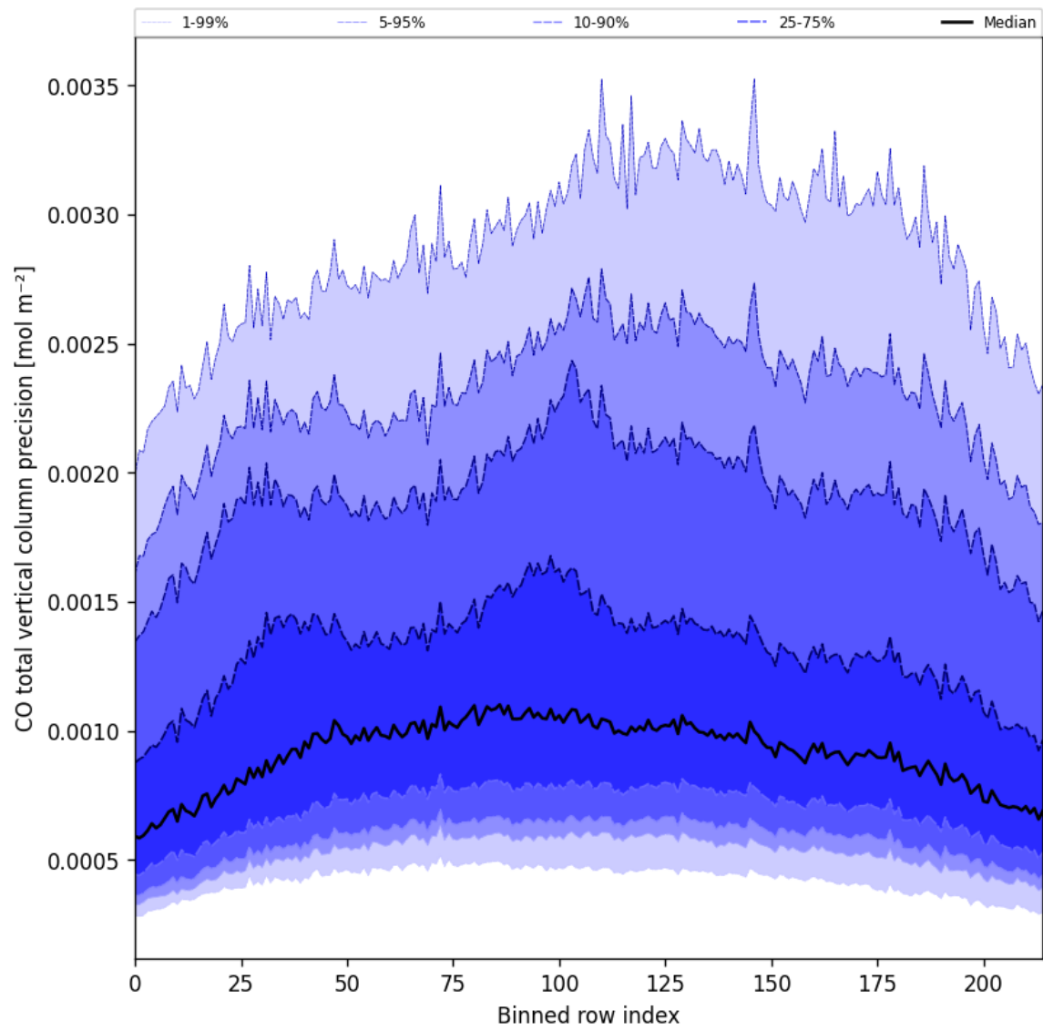
Figure 28: Along track statistics of “CO total vertical column precision” for 2024-10-03 to 2024-10-05
