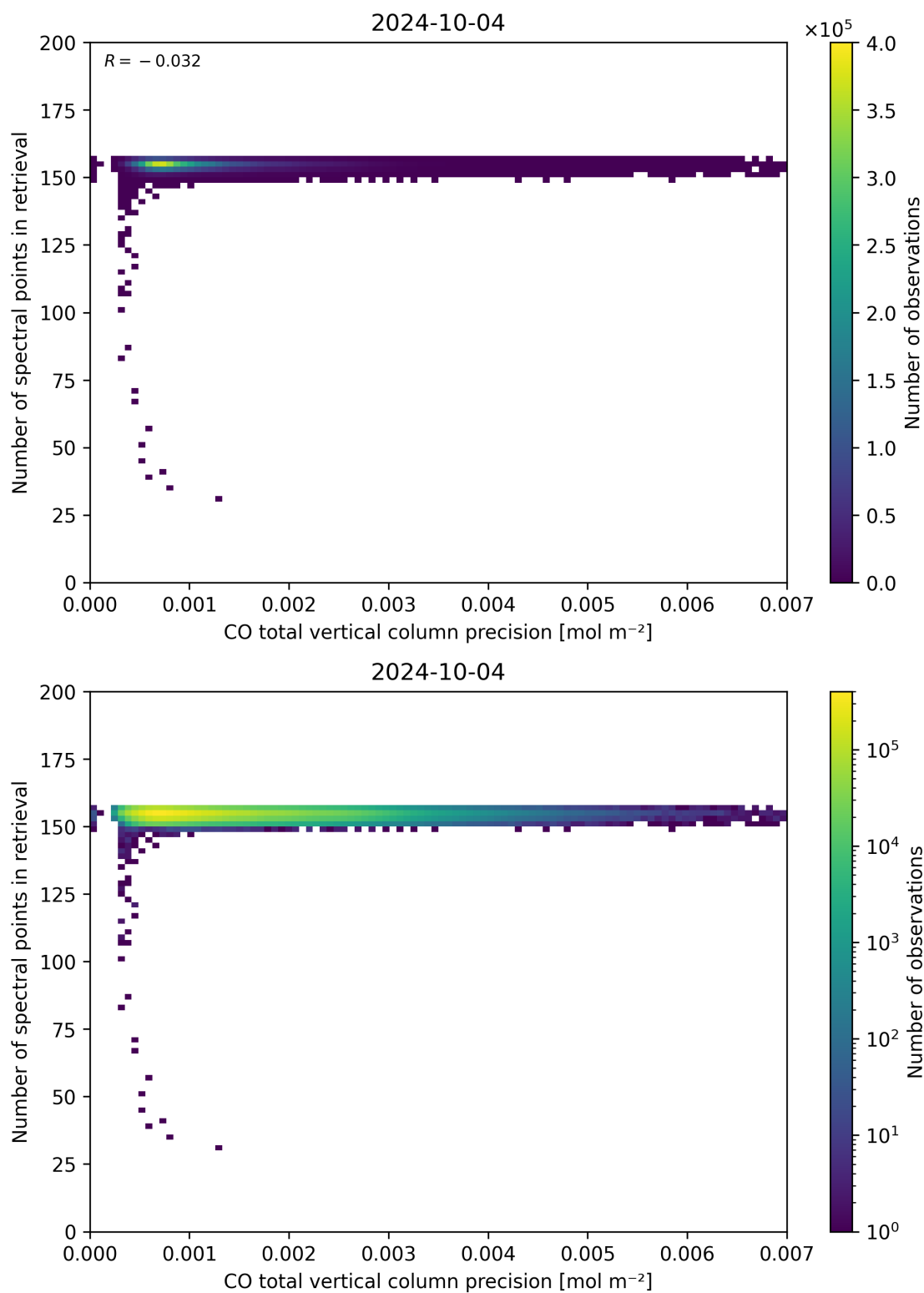
Figure 47: Scatter density plot of “CO total vertical column precision” against “Number of spectral points in retrieval” for 2024-10-03 to 2024-10-05.
