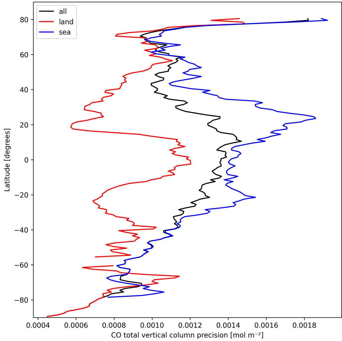
Figure 12: Zonal average of “CO total vertical column precision” for 2024-10-03 to 2024-10-05.
