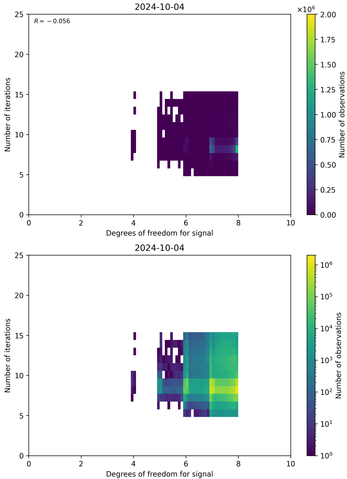
Figure 50: Scatter density plot of “Degrees of freedom for signal” against “Number of iterations” for 2024-10-03 to 2024-10-05.
