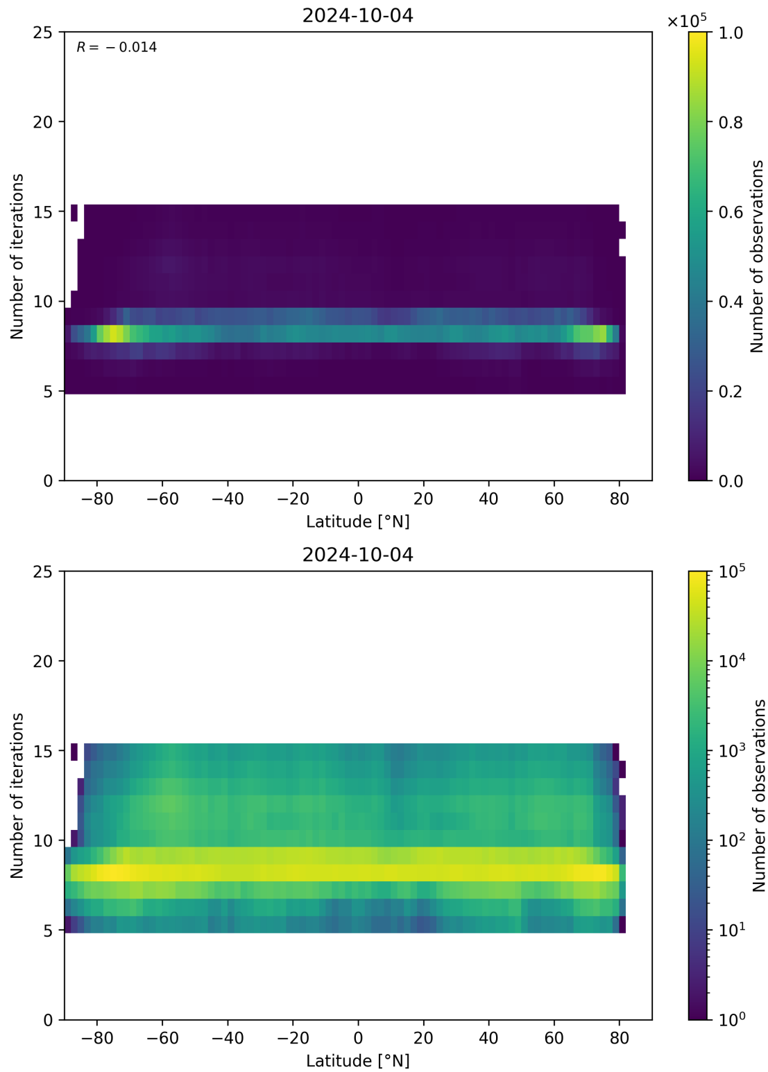
Figure 56: Scatter density plot of “Latitude” against “Number of iterations” for 2024-10-03 to 2024-10-05.
