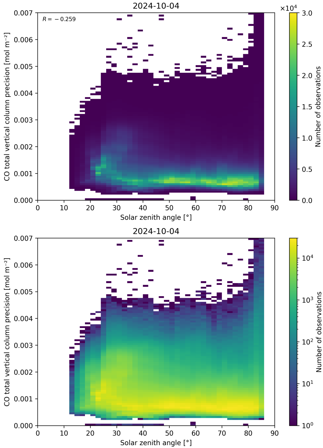
Figure 63: Scatter density plot of “Solar zenith angle” against “CO total vertical column precision” for 2024-10-03 to 2024-10-05.
