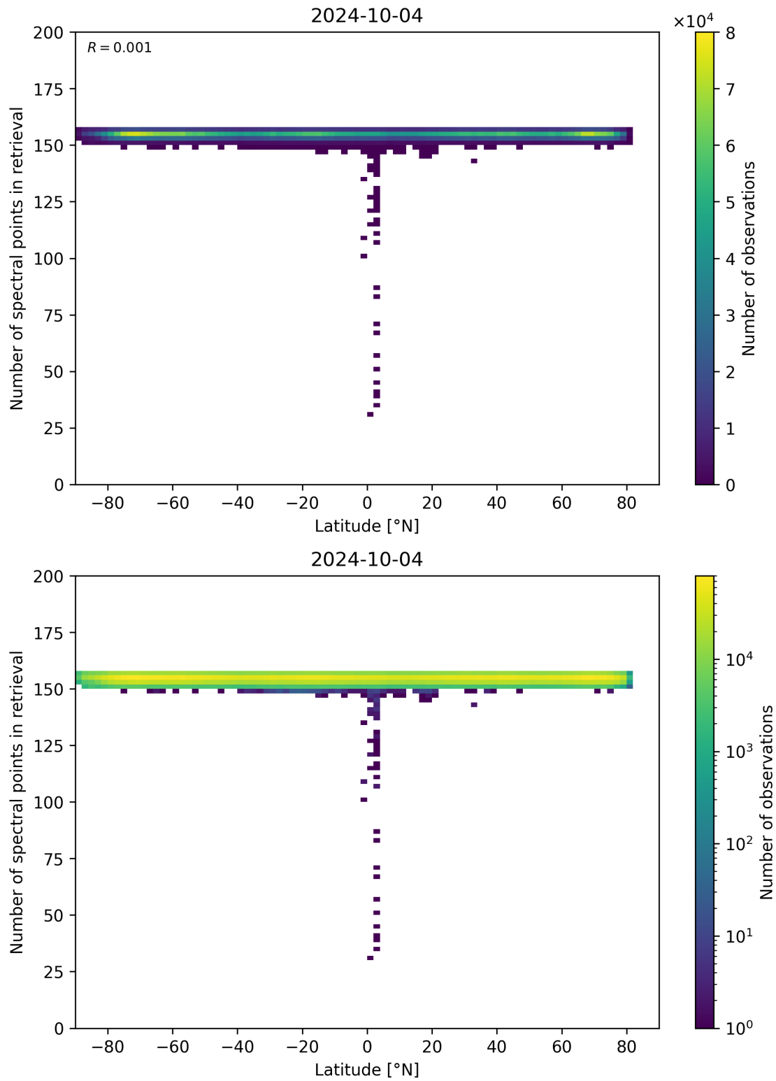
Figure 57: Scatter density plot of “Latitude” against “Number of spectral points in retrieval” for 2024-10-03 to 2024-10-05.
