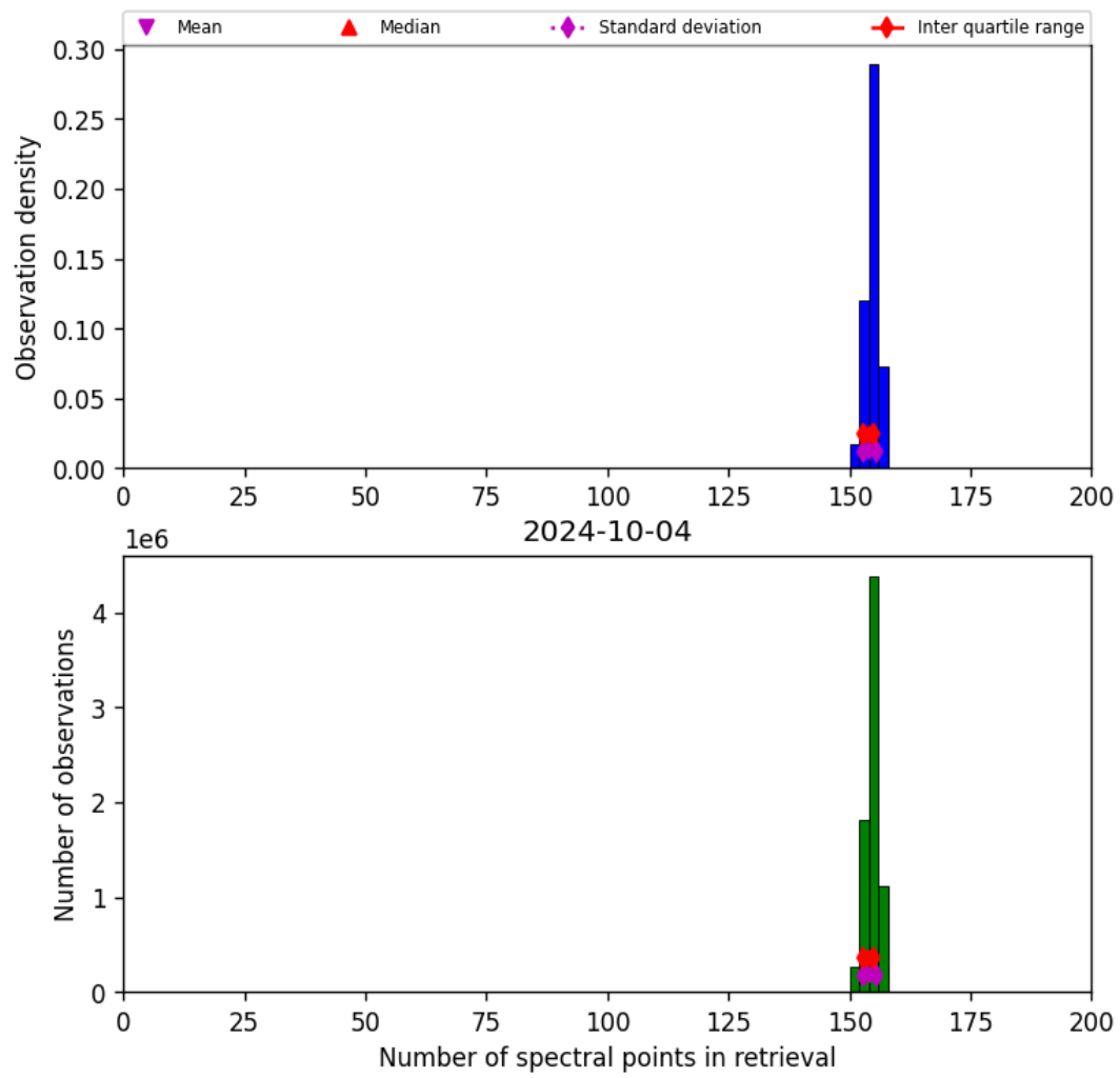
Figure 21: Histogram of “Number of spectral points in retrieval” for 2024-10-03 to 2024-10-05
