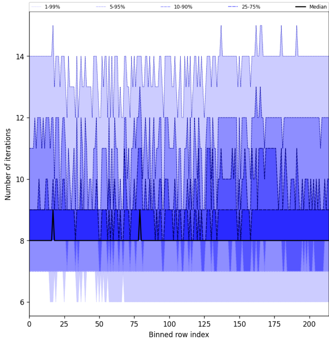
Figure 32: Along track statistics of “Number of iterations” for 2024-10-03 to 2024-10-05
