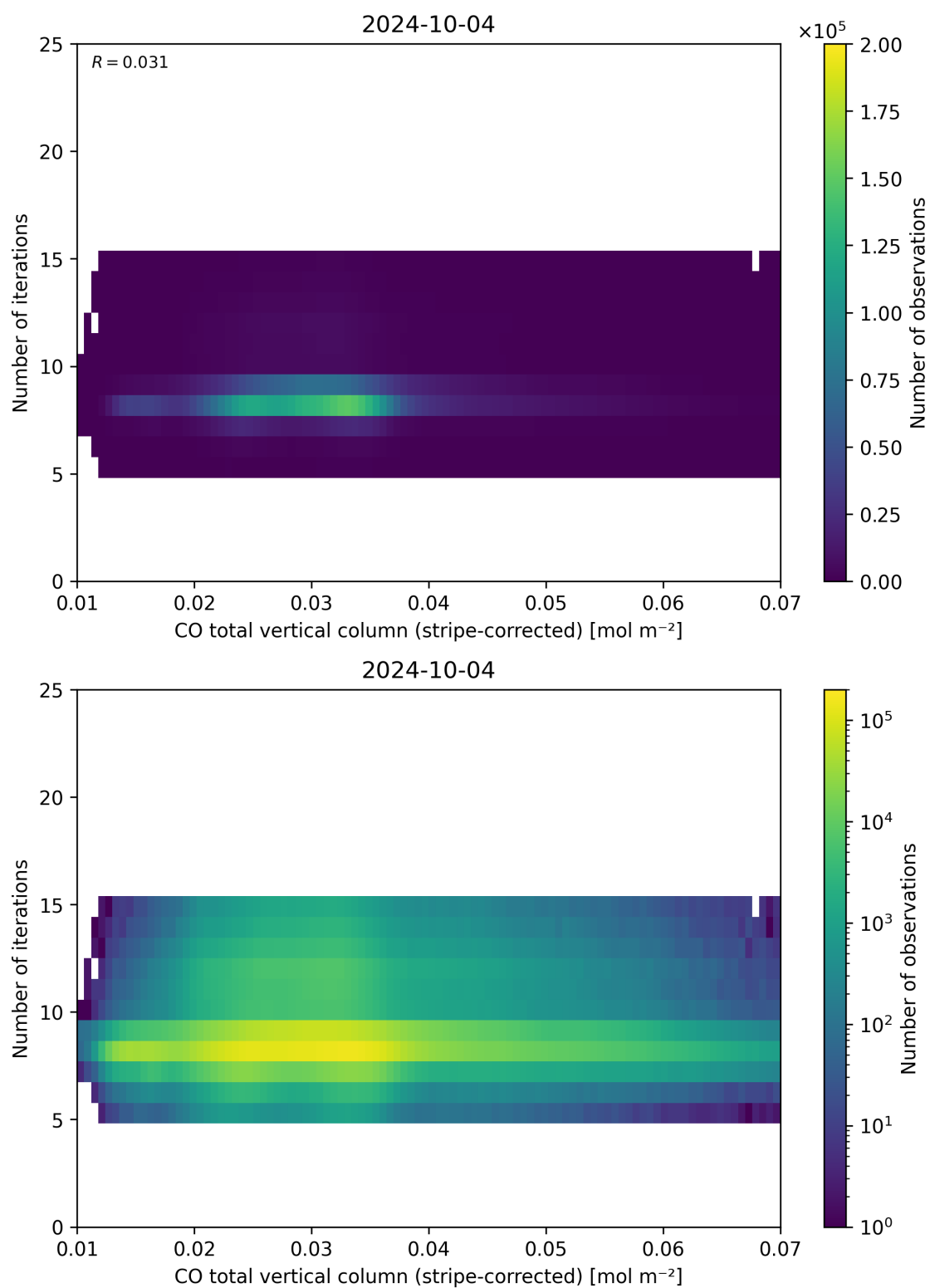
Figure 39: Scatter density plot of “CO total vertical column (stripe-corrected)” against “Number of iterations” for 2024-10-03 to 2024-10-05.
