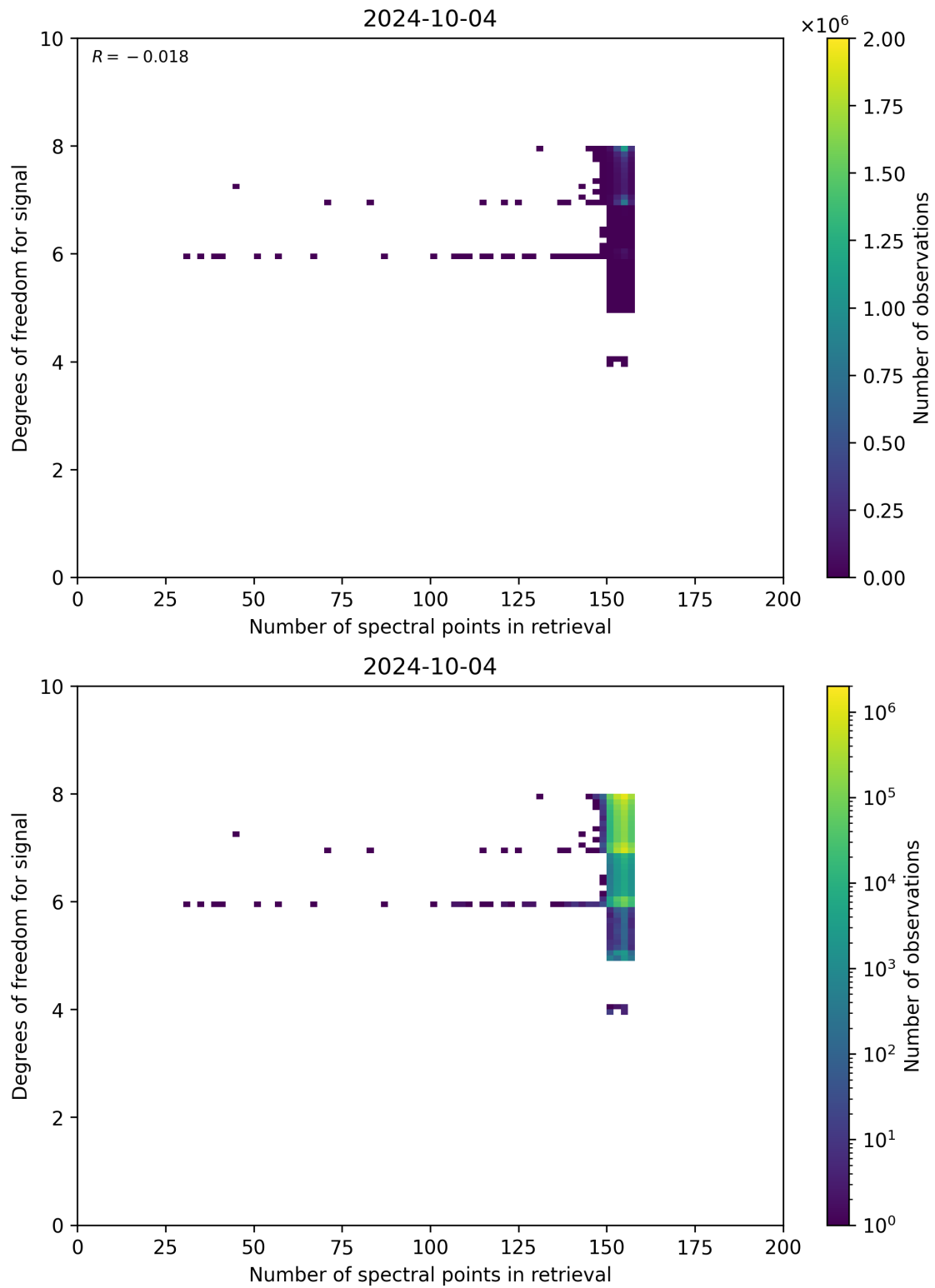
Figure 59: Scatter density plot of “Number of spectral points in retrieval” against “Degrees of freedom for signal” for 2024-10-03 to 2024-10-05.
