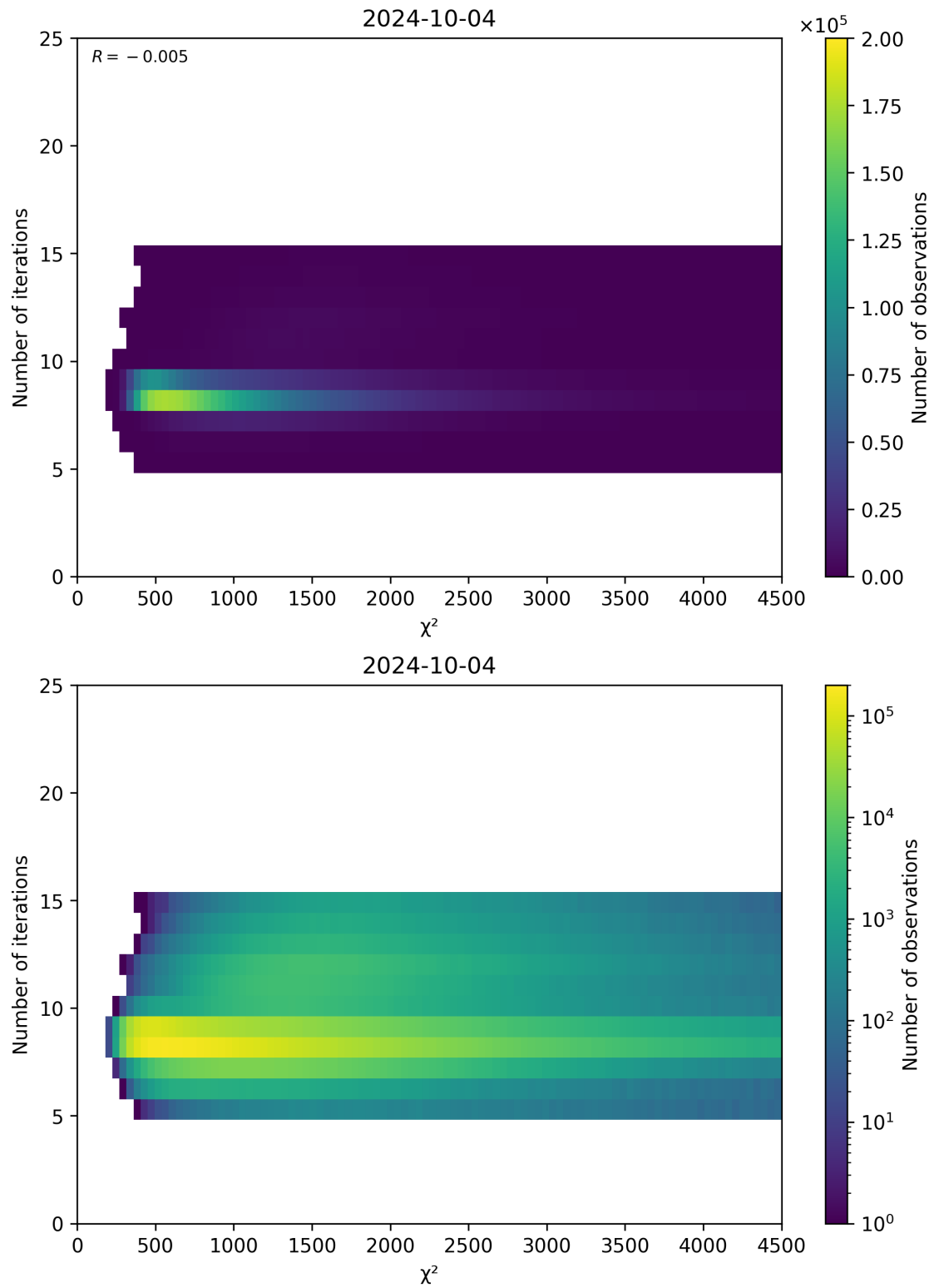
Figure 49: Scatter density plot of “ \chi^2 ” against “Number of iterations” for 2024-10-03 to 2024-10-05.
