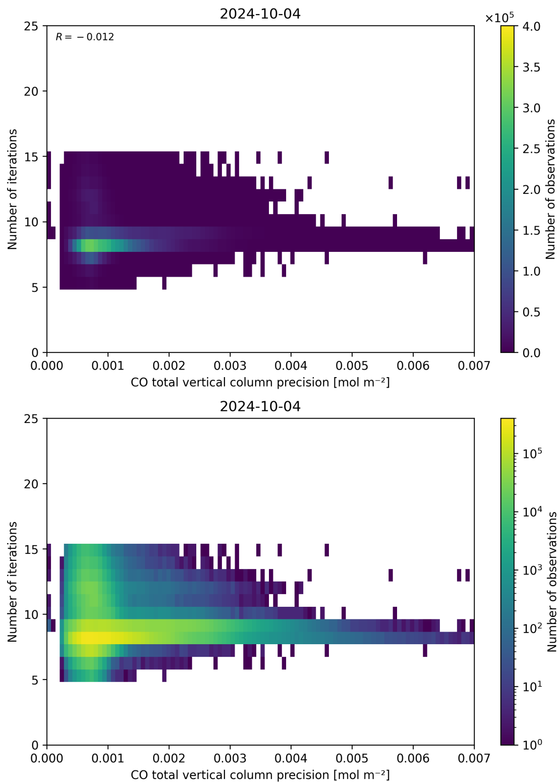
Figure 46: Scatter density plot of “CO total vertical column precision” against “Number of iterations” for 2024-10-03 to 2024-10-05.
