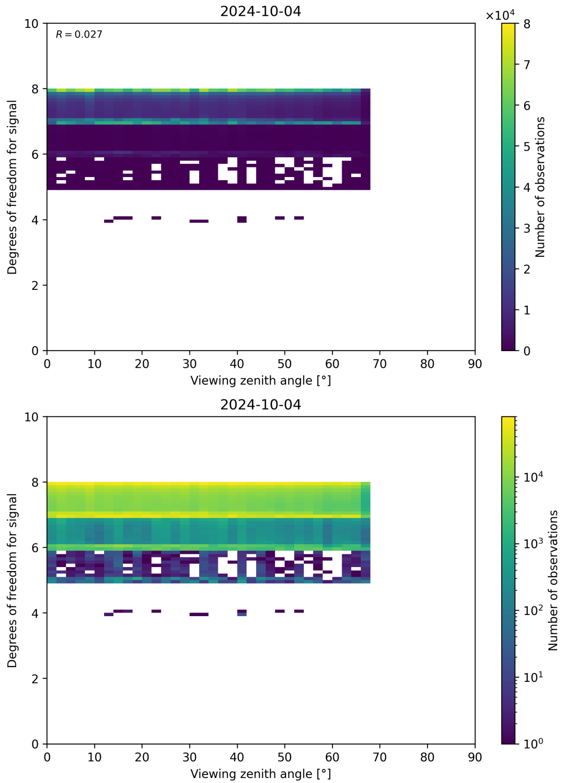
Figure 73: Scatter density plot of “Viewing zenith angle” against “Degrees of freedom for signal” for 2024-10-03 to 2024-10-05.
