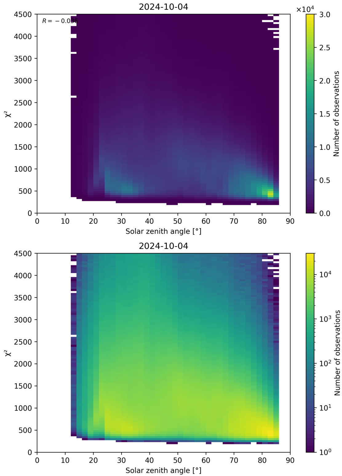
Figure 64: Scatter density plot of “Solar zenith angle” against “ \chi^2 ” for 2024-10-03 to 2024-10-05.
