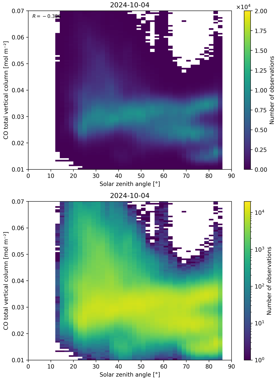
Figure 61: Scatter density plot of “Solar zenith angle” against “CO total vertical column” for 2024-10-03 to 2024-10-05.
