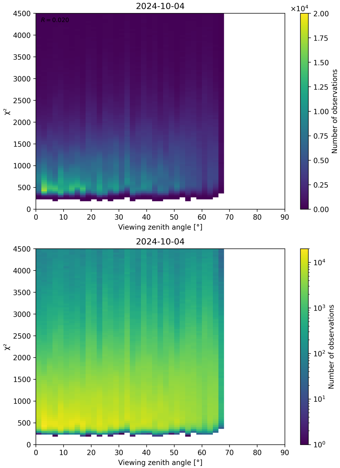
Figure 72: Scatter density plot of “Viewing zenith angle” against “ \chi^2 ” for 2024-10-03 to 2024-10-05.
