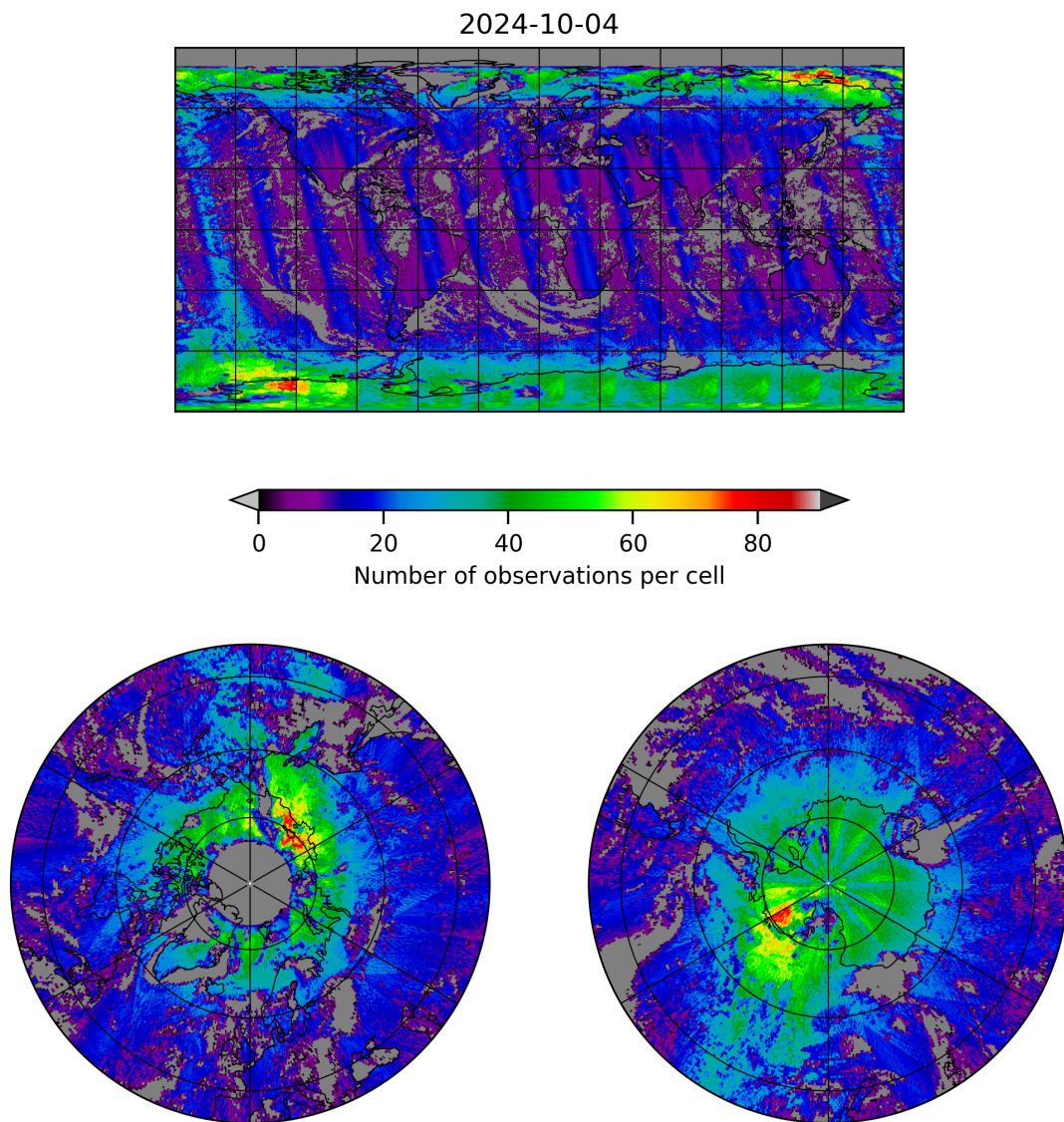
Figure 8: Map of the number of observations for 2024-10-03 to 2024-10-05
