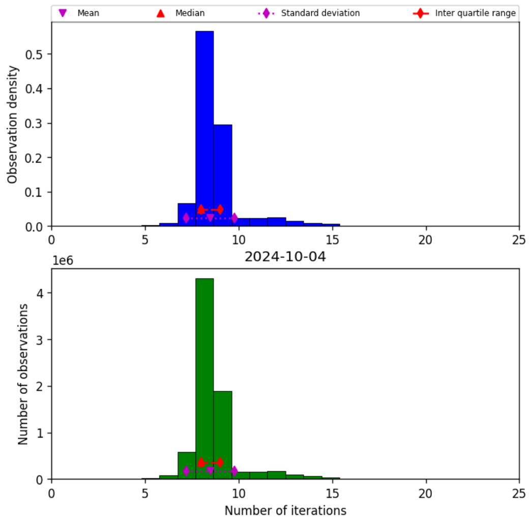
Figure 24: Histogram of “Number of iterations” for 2024-10-03 to 2024-10-05
