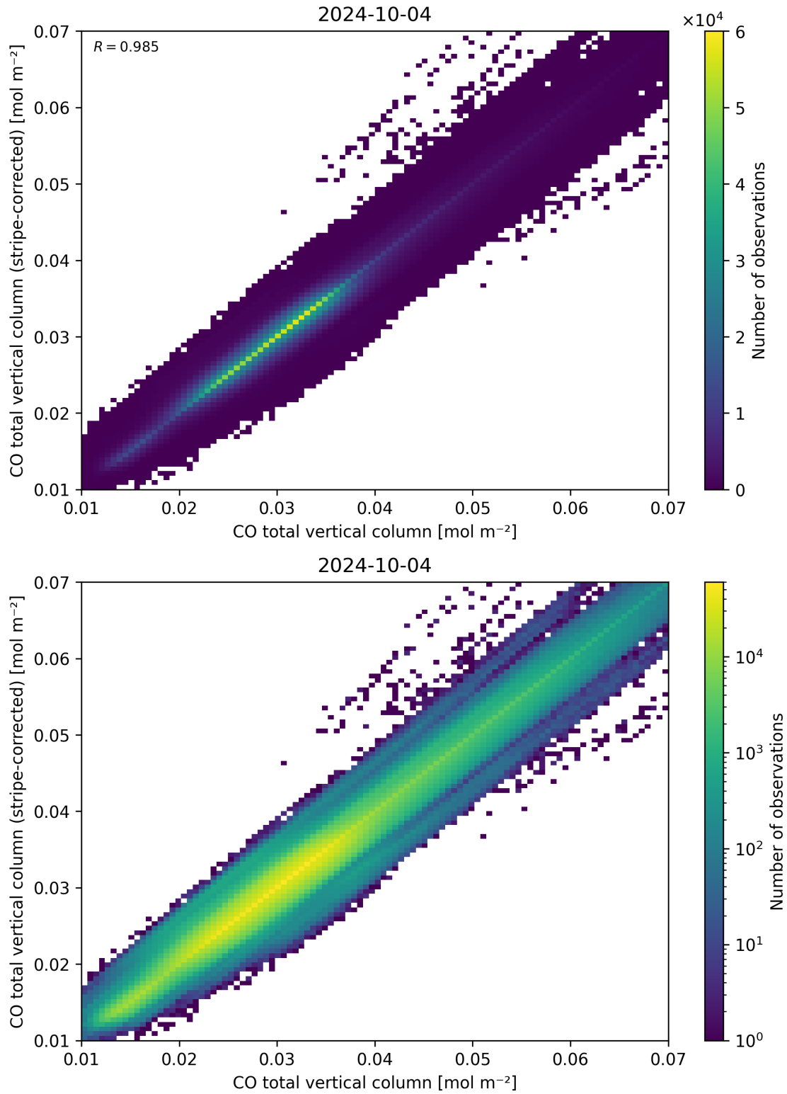
Figure 33: Scatter density plot of “CO total vertical column” against “CO total vertical column (stripe-corrected)” for 2024-10-03 to 2024-10-05.
