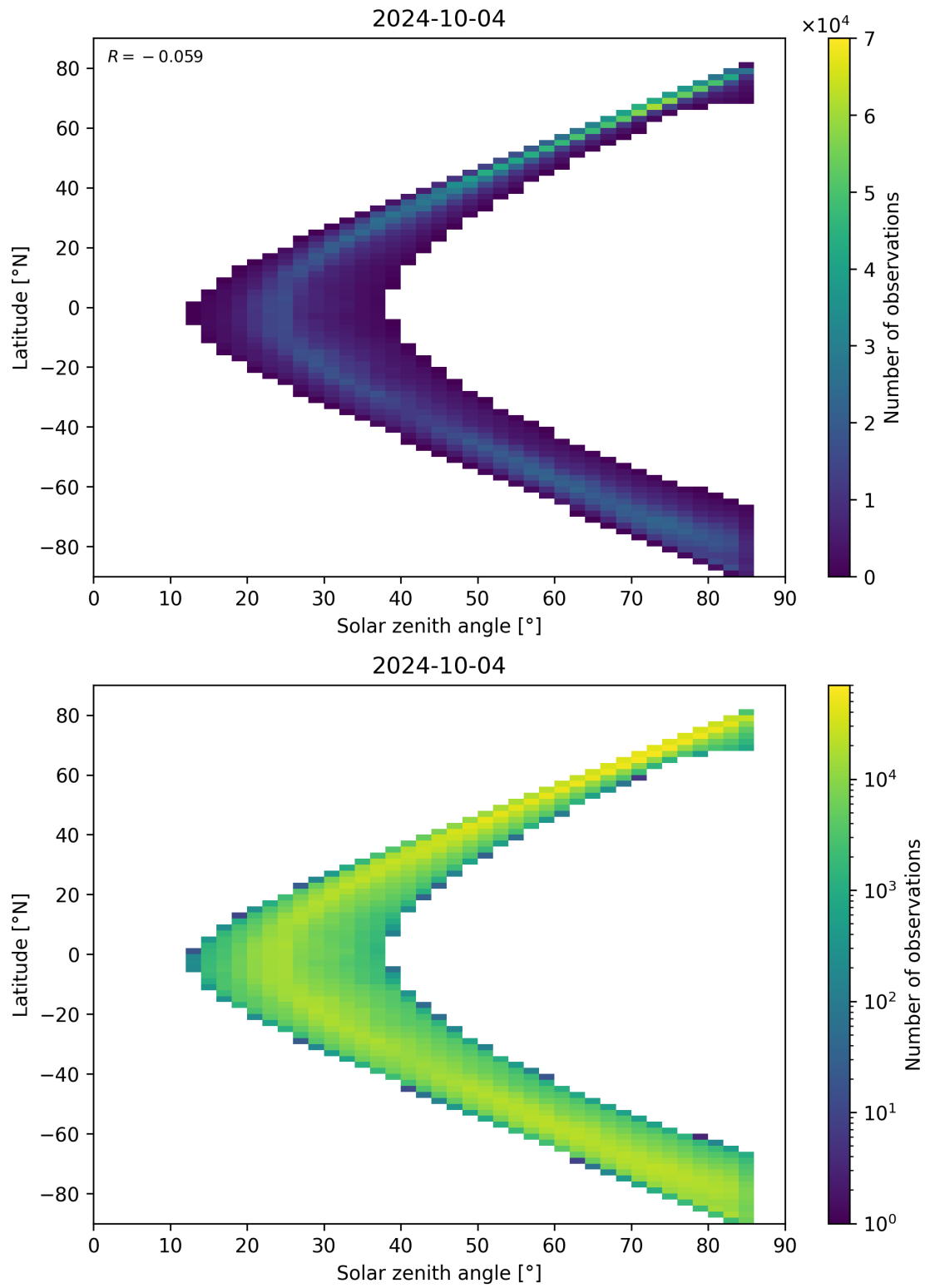
Figure 66: Scatter density plot of “Solar zenith angle” against “Latitude” for 2024-10-03 to 2024-10-05.
