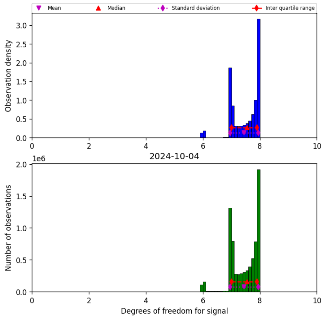
Figure 23: Histogram of “Degrees of freedom for signal” for 2024-10-03 to 2024-10-05
