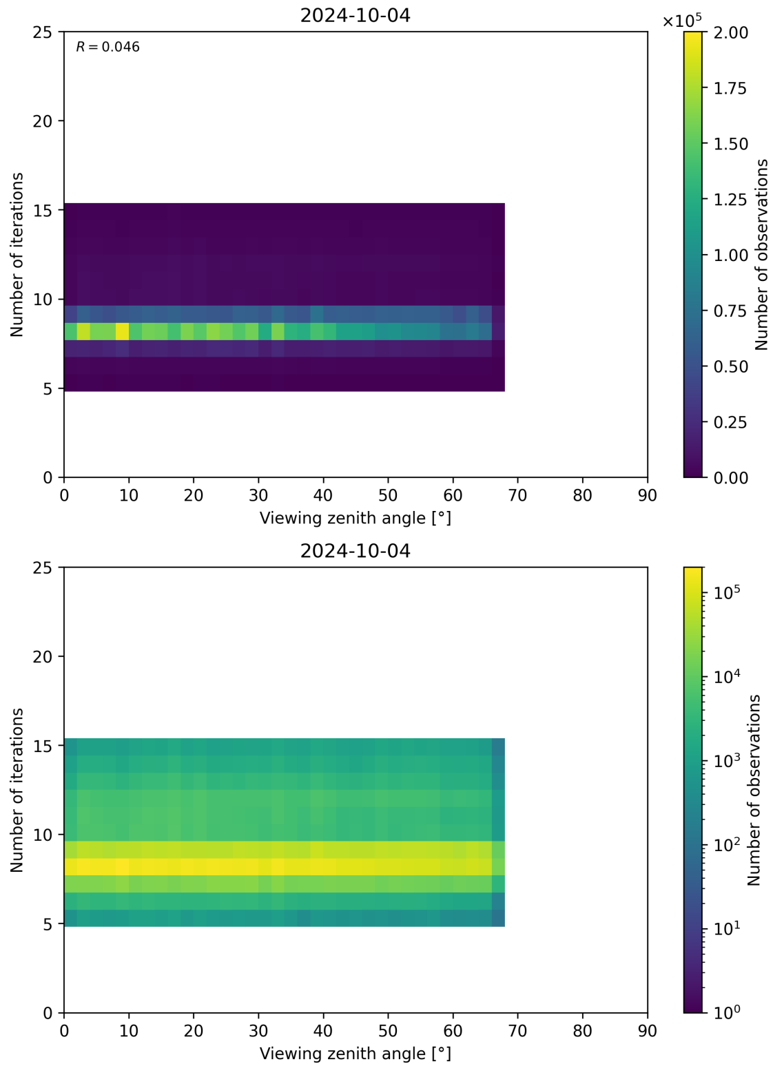
Figure 75: Scatter density plot of “Viewing zenith angle” against “Number of iterations” for 2024-10-03 to 2024-10-05.
