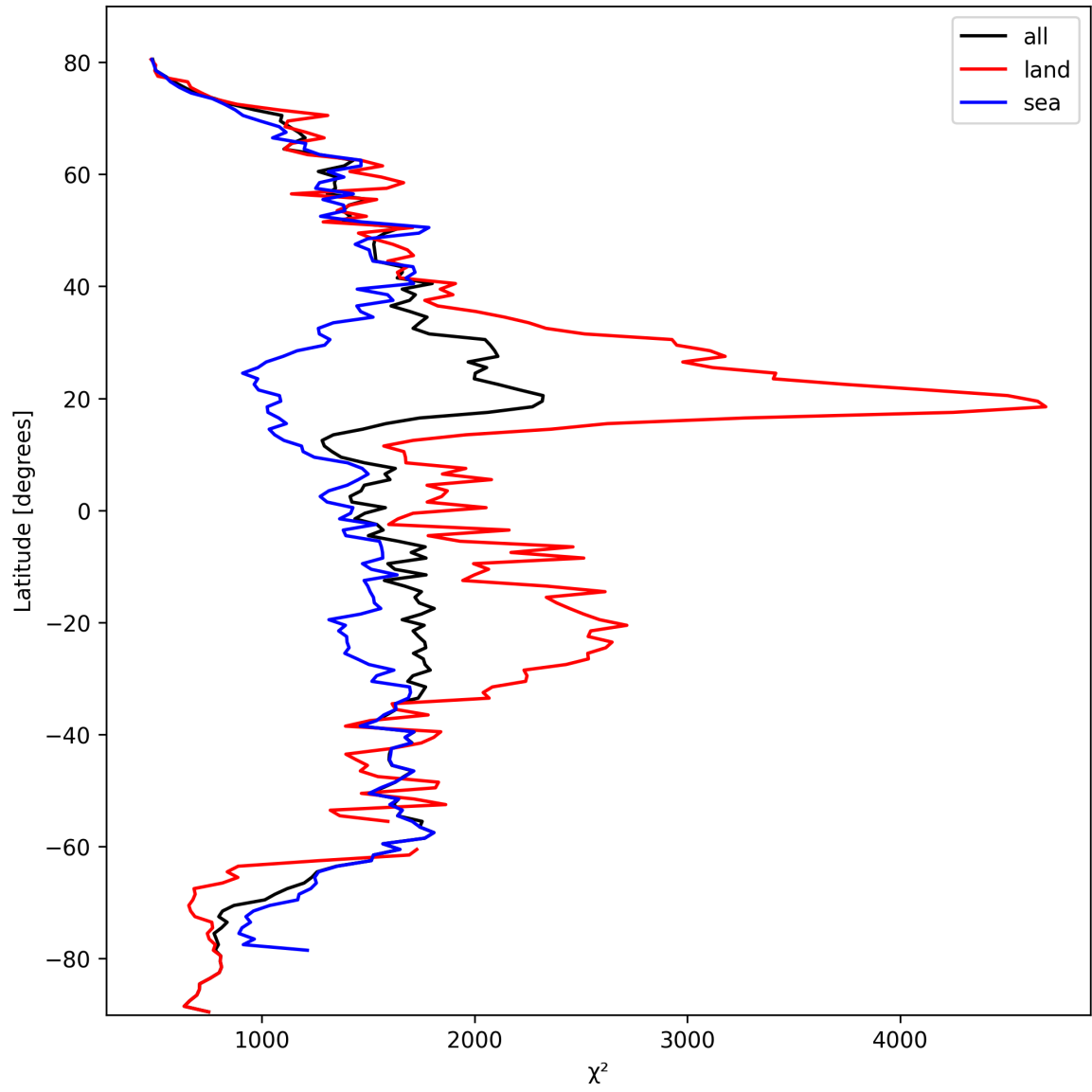
Figure 14: Zonal average of “ \chi^2 ” for 2024-10-03 to 2024-10-05.
