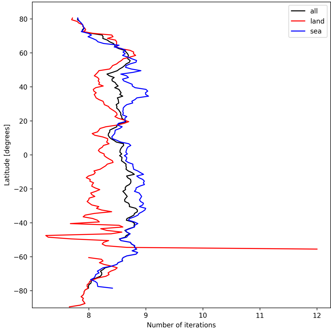
Figure 16: Zonal average of “Number of iterations” for 2024-10-03 to 2024-10-05.
