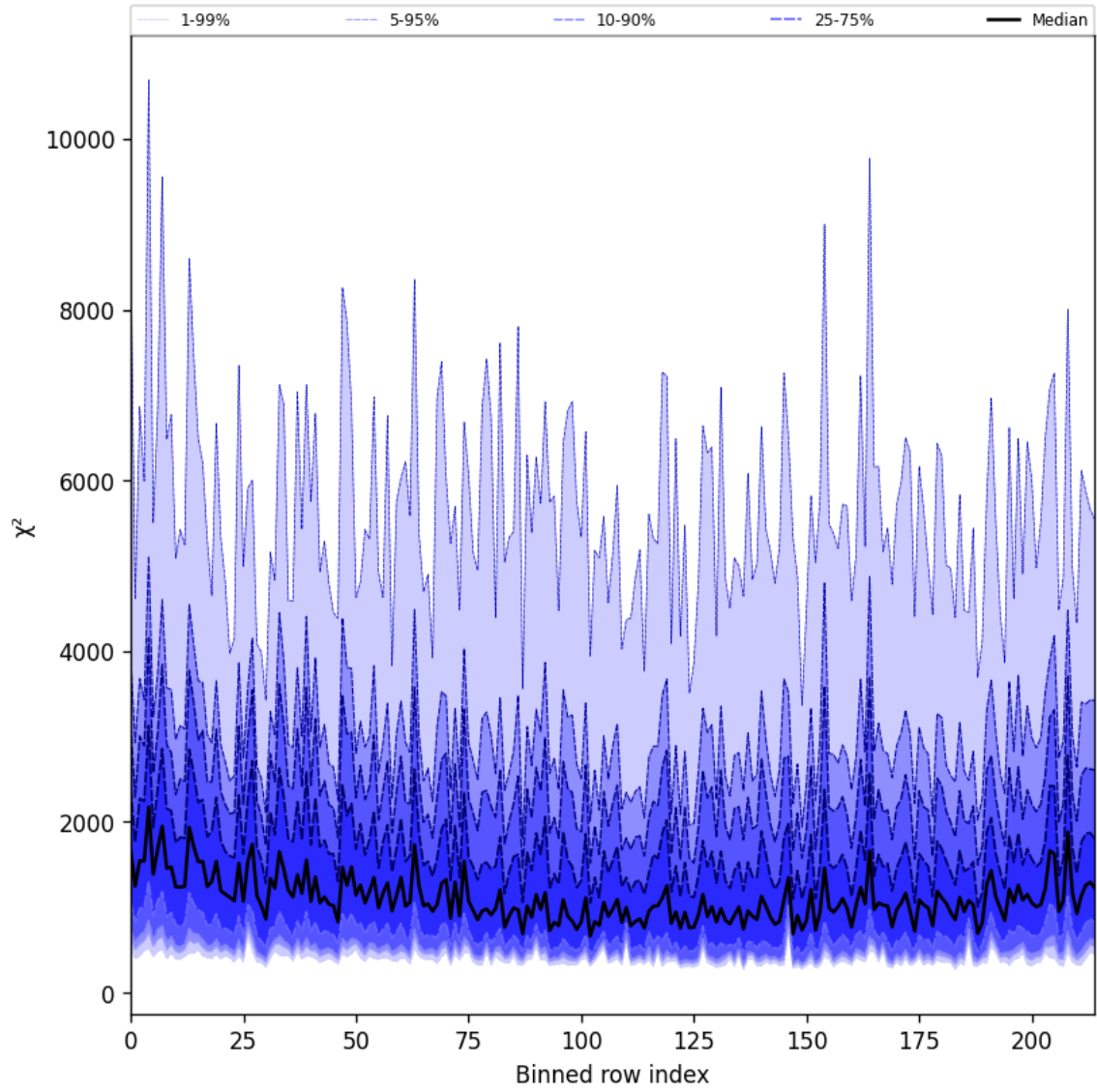
Figure 30: Along track statistics of “ \chi^2 ” for 2024-10-03 to 2024-10-05
