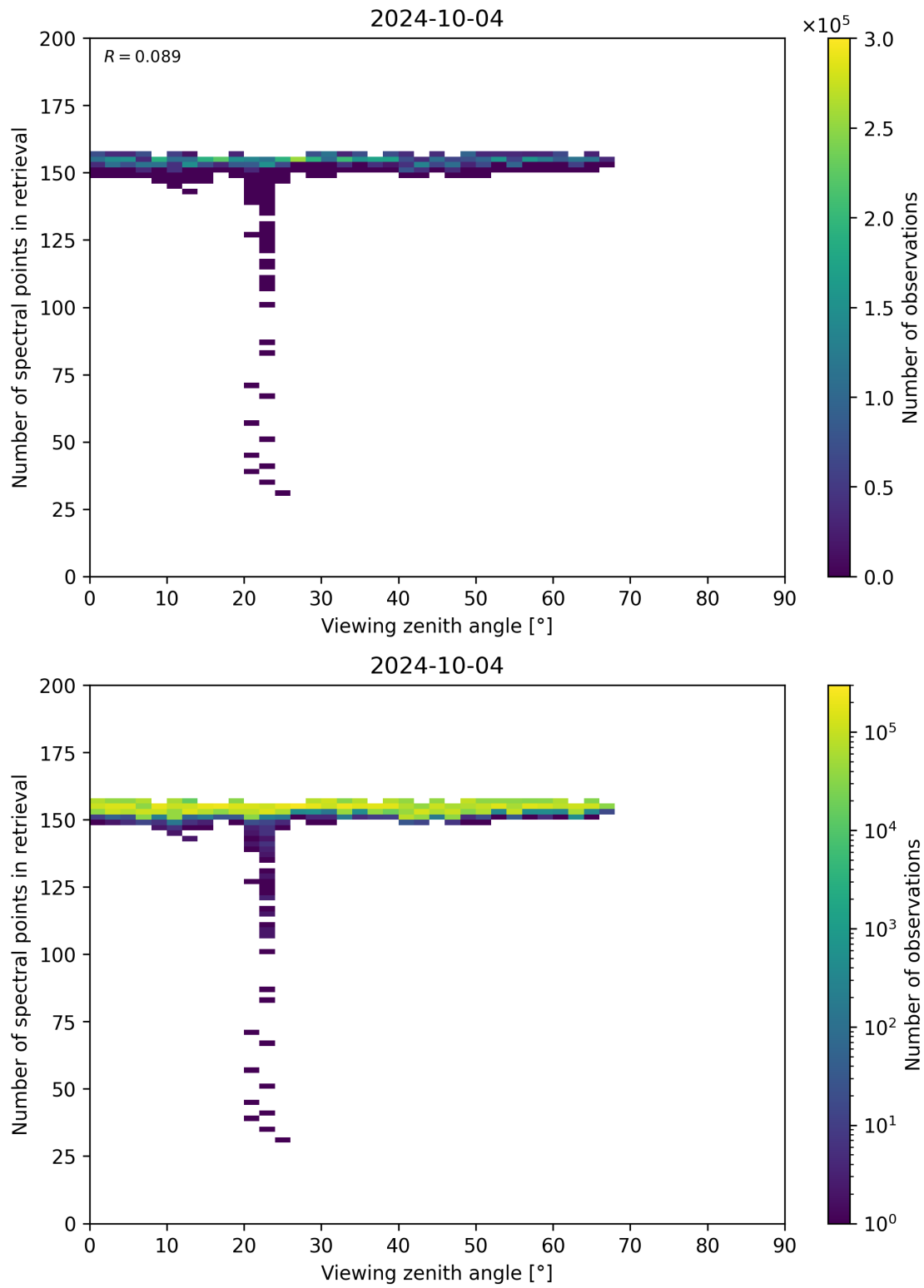
Figure 76: Scatter density plot of “Viewing zenith angle” against “Number of spectral points in retrieval” for 2024-10-03 to 2024-10-05.
