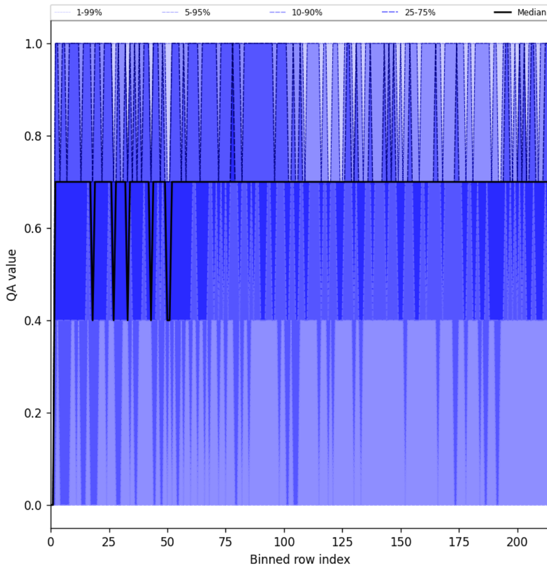
Figure 25: Along track statistics of “QA value” for 2024-10-03 to 2024-10-05
