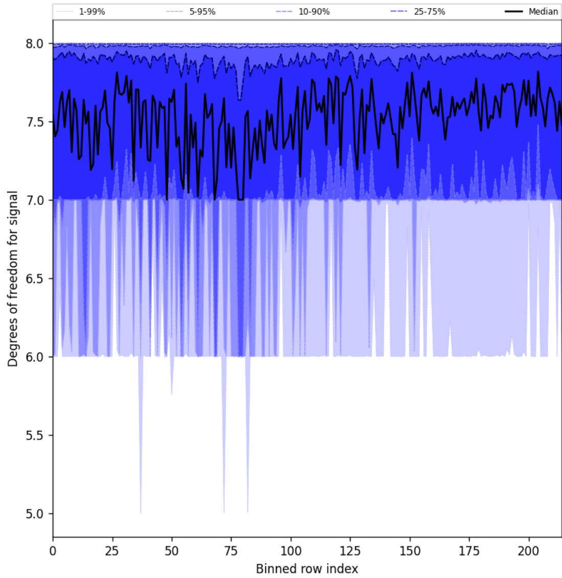
Figure 31: Along track statistics of “Degrees of freedom for signal” for 2024-10-03 to 2024-10-05
