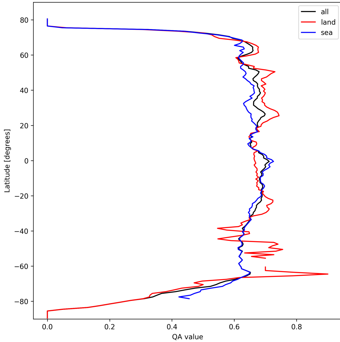
Figure 9: Zonal average of “QA value” for 2024-10-03 to 2024-10-05.
