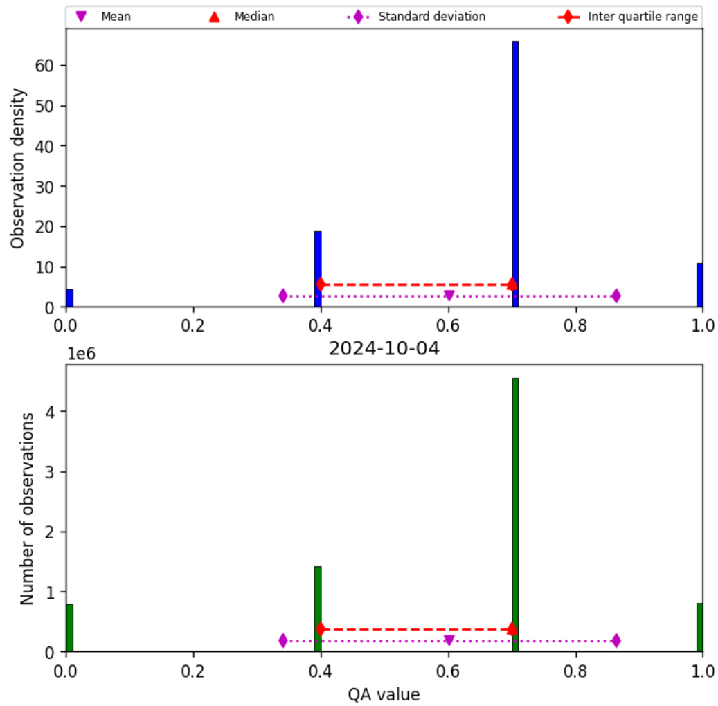
Figure 17: Histogram of “QA value” for 2024-10-03 to 2024-10-05
