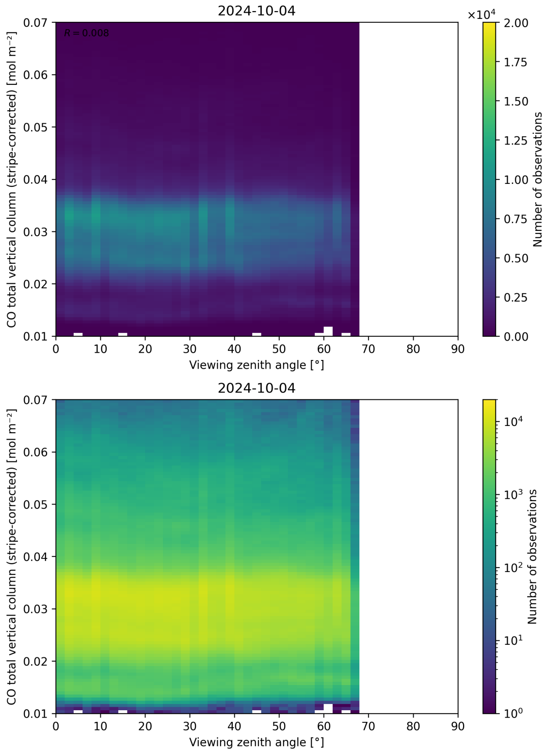
Figure 70: Scatter density plot of “Viewing zenith angle” against “CO total vertical column (stripe-corrected)” for 2024-10-03 to 2024-10-05.
