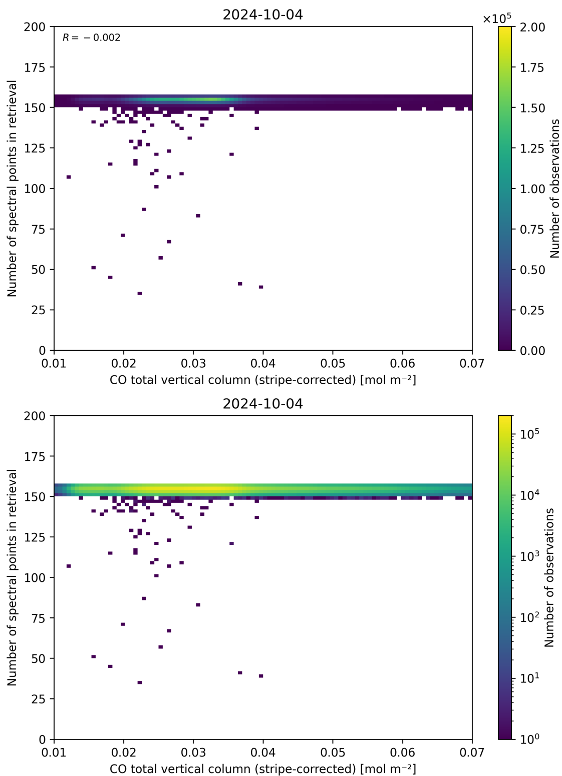
Figure 40: Scatter density plot of “CO total vertical column (stripe-corrected)” against “Number of spectral points in retrieval” for 2024-10-03 to 2024-10-05.
