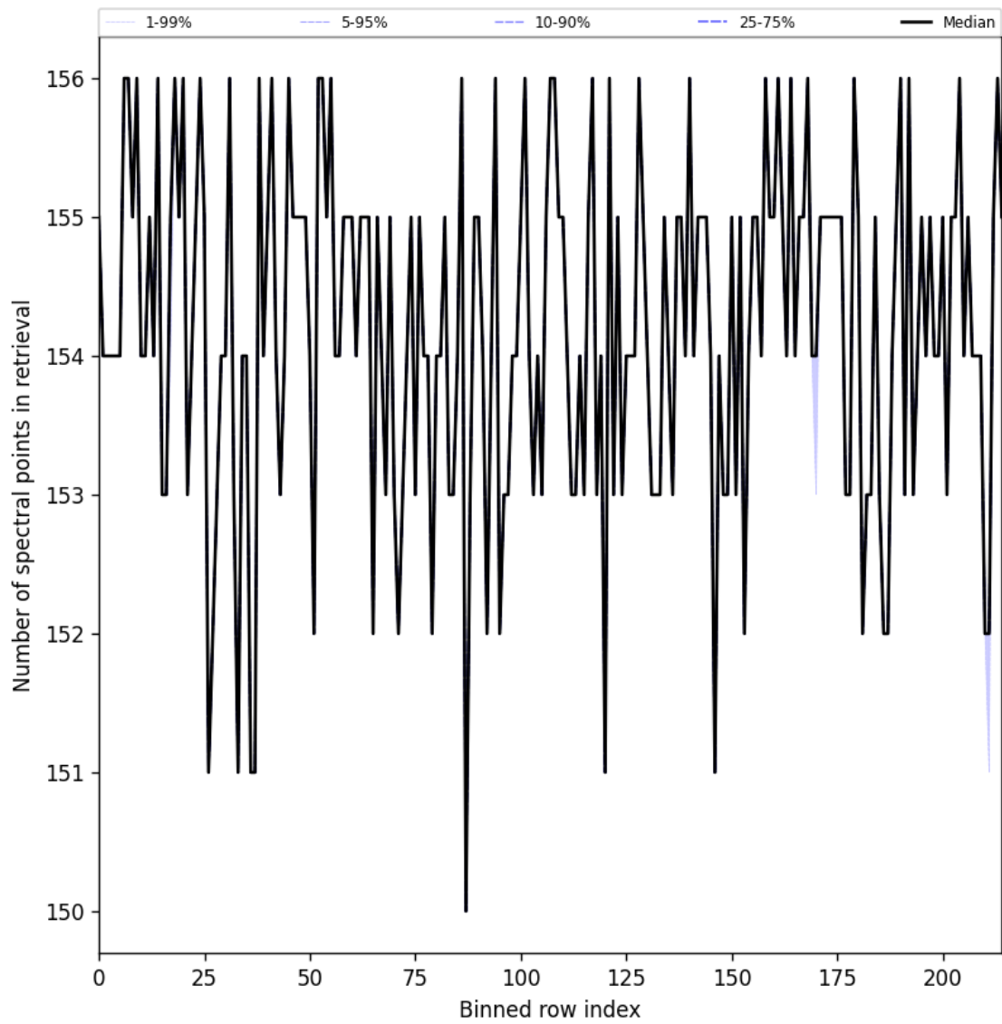
Figure 29: Along track statistics of “Number of spectral points in retrieval” for 2024-10-03 to 2024-10-05
