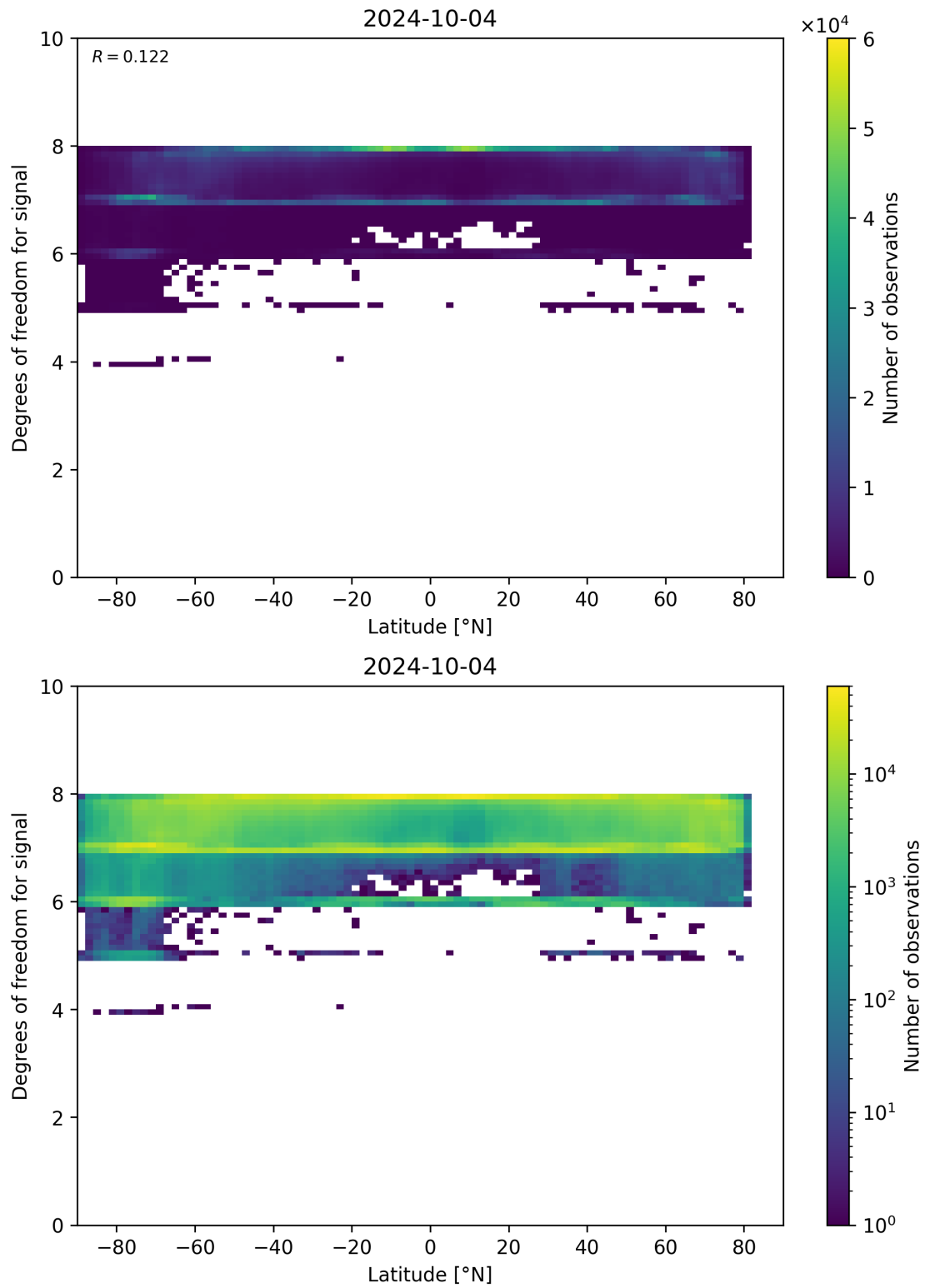
Figure 55: Scatter density plot of “Latitude” against “Degrees of freedom for signal” for 2024-10-03 to 2024-10-05.
