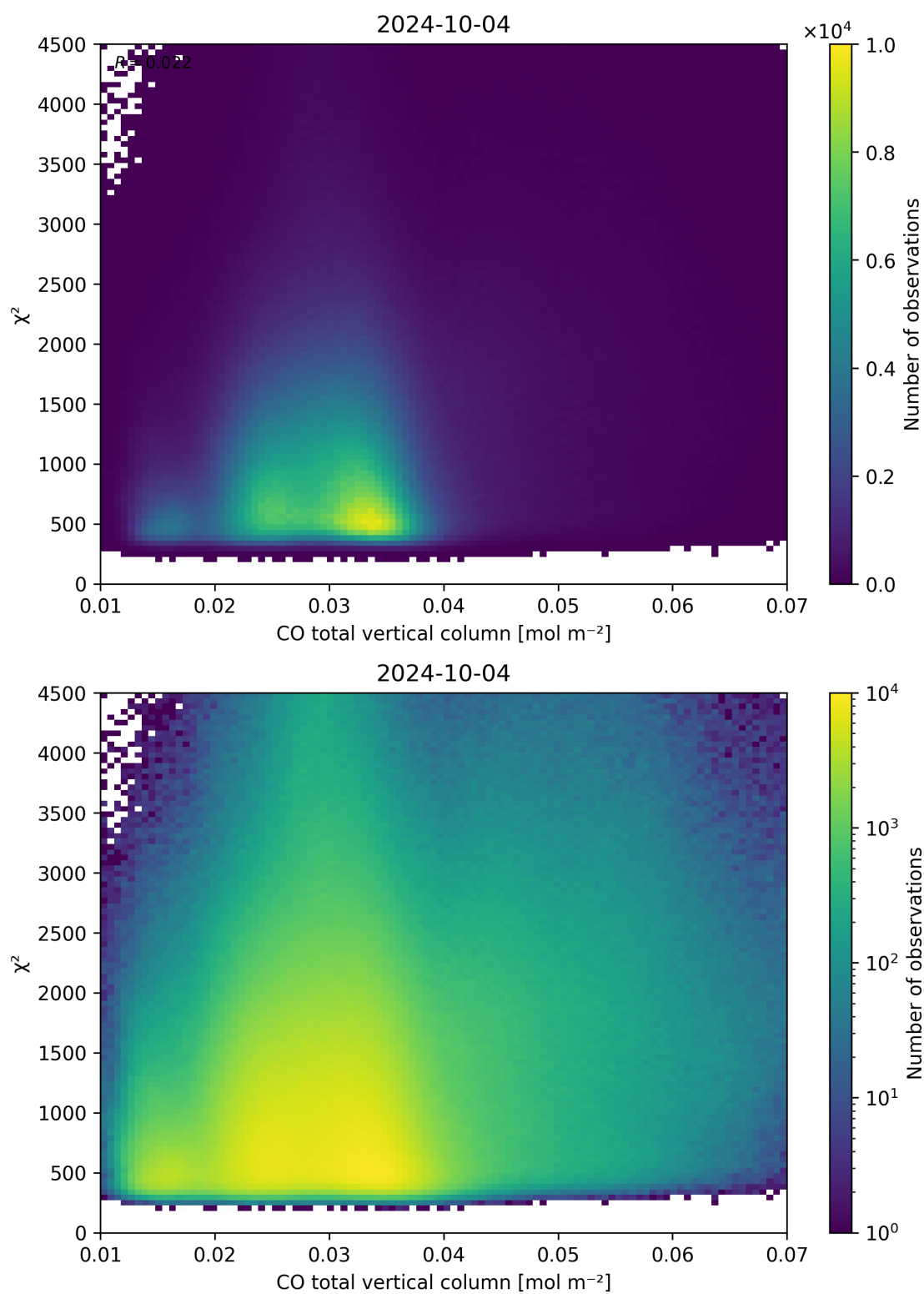
Figure 35: Scatter density plot of “CO total vertical column” against “ \chi^2 ” for 2024-10-03 to 2024-10-05.
