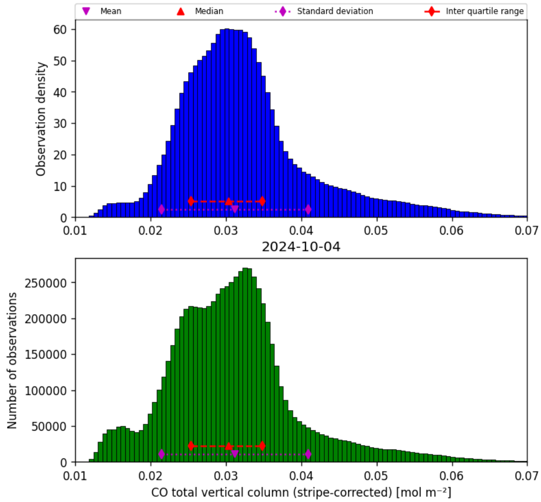
Figure 19: Histogram of “CO total vertical column (stripe-corrected)” for 2024-10-03 to 2024-10-05
