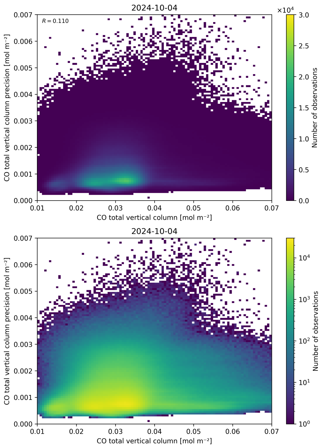
Figure 34: Scatter density plot of “CO total vertical column” against “CO total vertical column precision” for 2024-10-03 to 2024-10-05.
