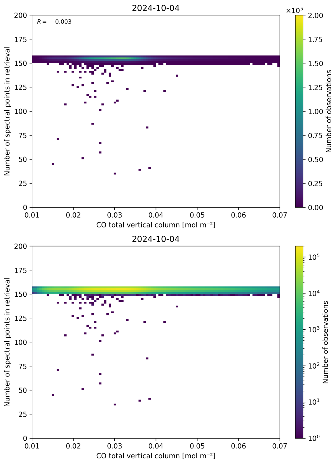
Figure 43: Scatter density plot of “CO total vertical column” against “Number of spectral points in retrieval” for 2024-10-03 to 2024-10-05.
