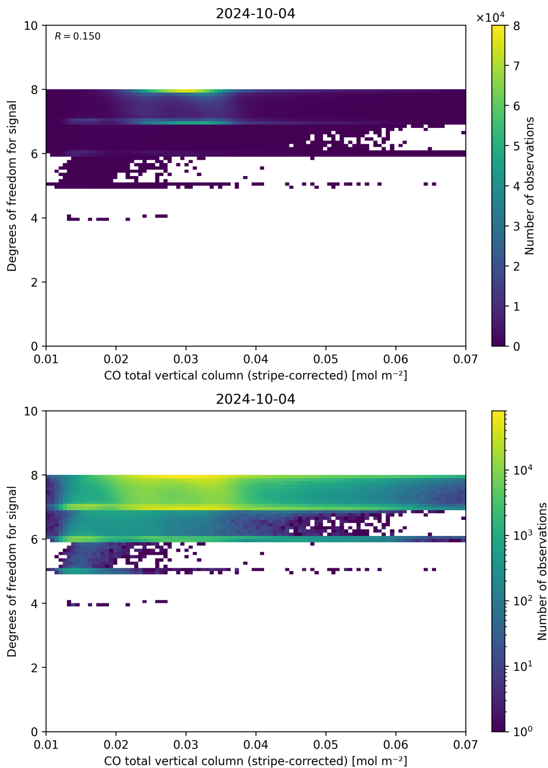
Figure 38: Scatter density plot of “CO total vertical column (stripe-corrected)” against “Degrees of freedom for signal” for 2024-10-03 to 2024-10-05.
