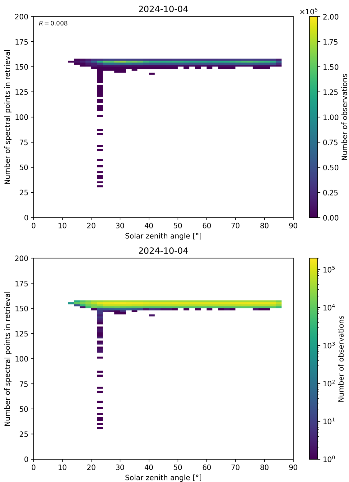
Figure 68: Scatter density plot of “Solar zenith angle” against “Number of spectral points in retrieval” for 2024-10-03 to 2024-10-05.
