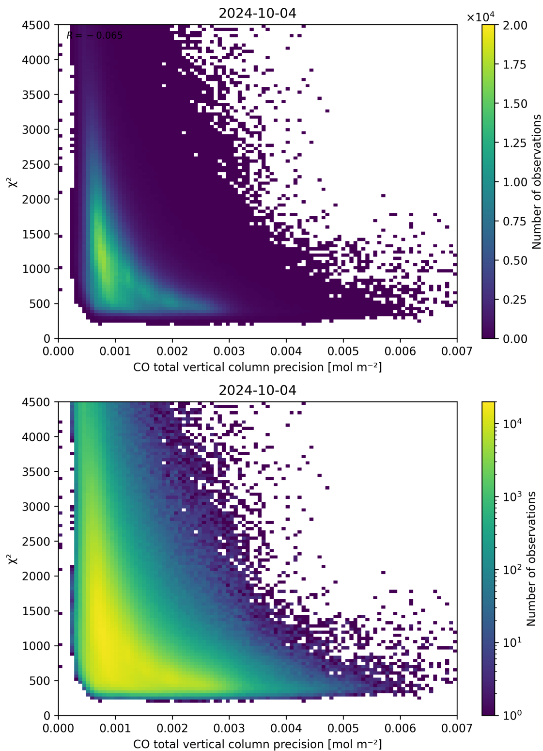
Figure 44: Scatter density plot of “CO total vertical column precision” against “ \chi^2 ” for 2024-10-03 to 2024-10-05.
