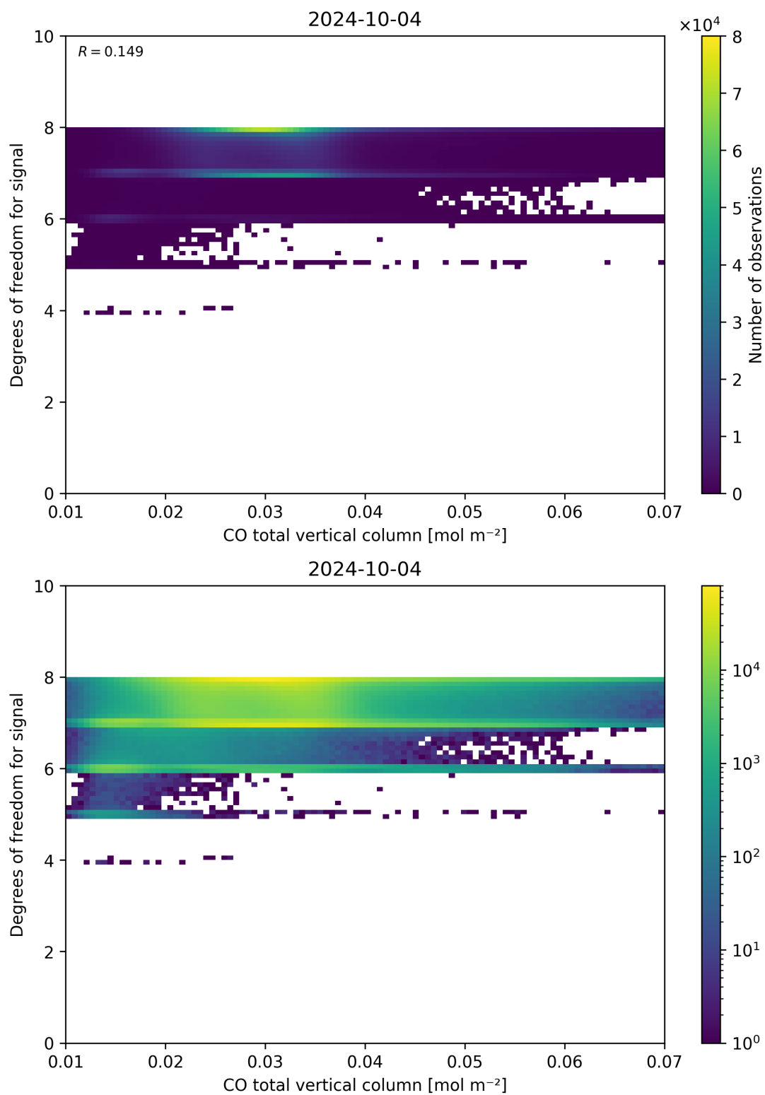
Figure 41: Scatter density plot of “CO total vertical column” against “Degrees of freedom for signal” for 2024-10-03 to 2024-10-05.
