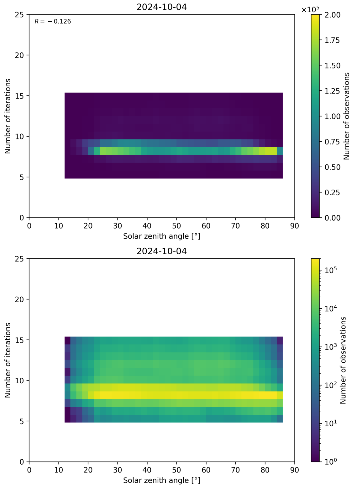
Figure 67: Scatter density plot of “Solar zenith angle” against “Number of iterations” for 2024-10-03 to 2024-10-05.
