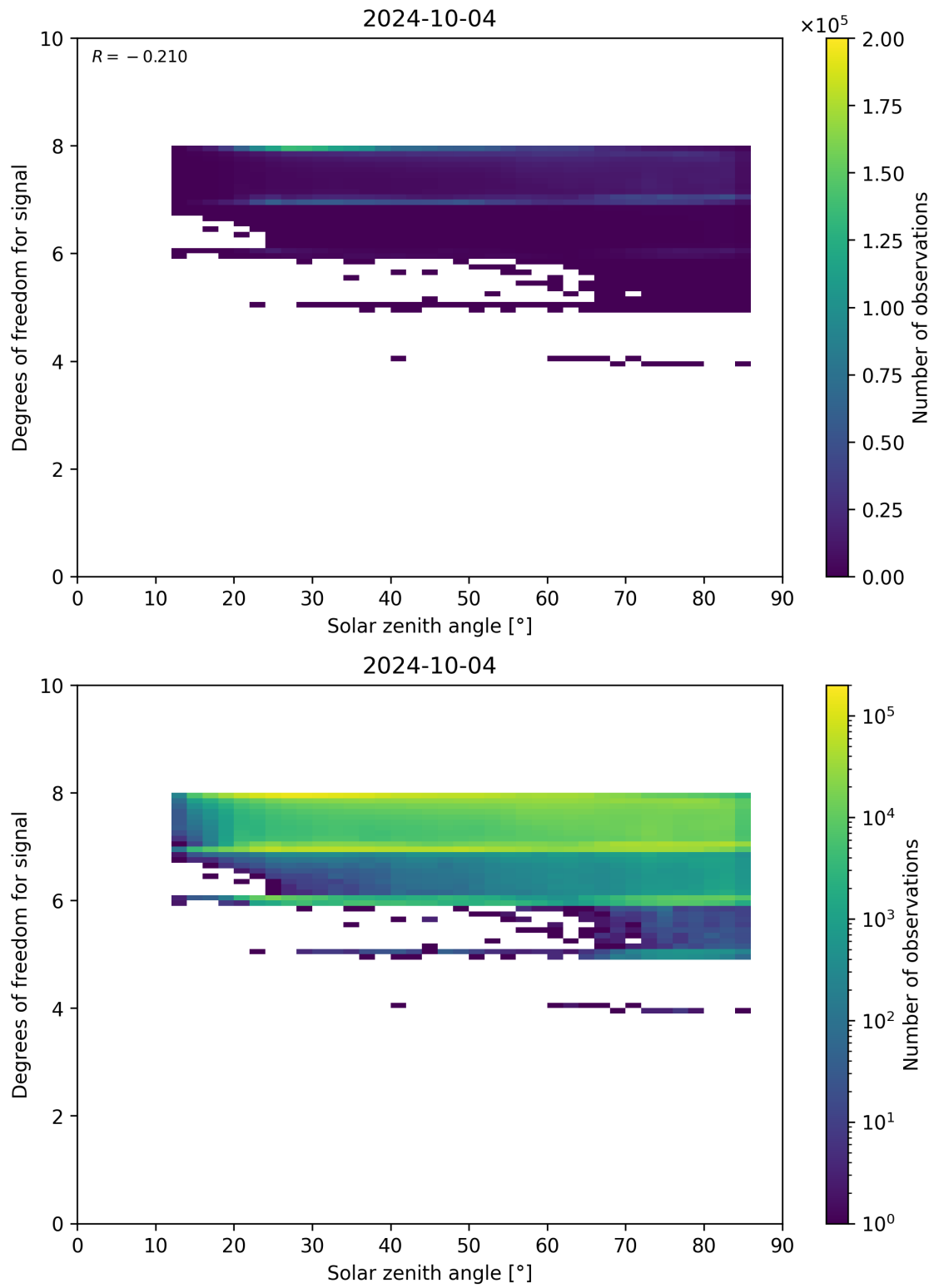
Figure 65: Scatter density plot of “Solar zenith angle” against “Degrees of freedom for signal” for 2024-10-03 to 2024-10-05.
