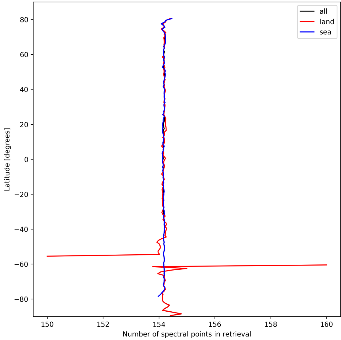
Figure 13: Zonal average of “Number of spectral points in retrieval” for 2024-10-03 to 2024-10-05.
