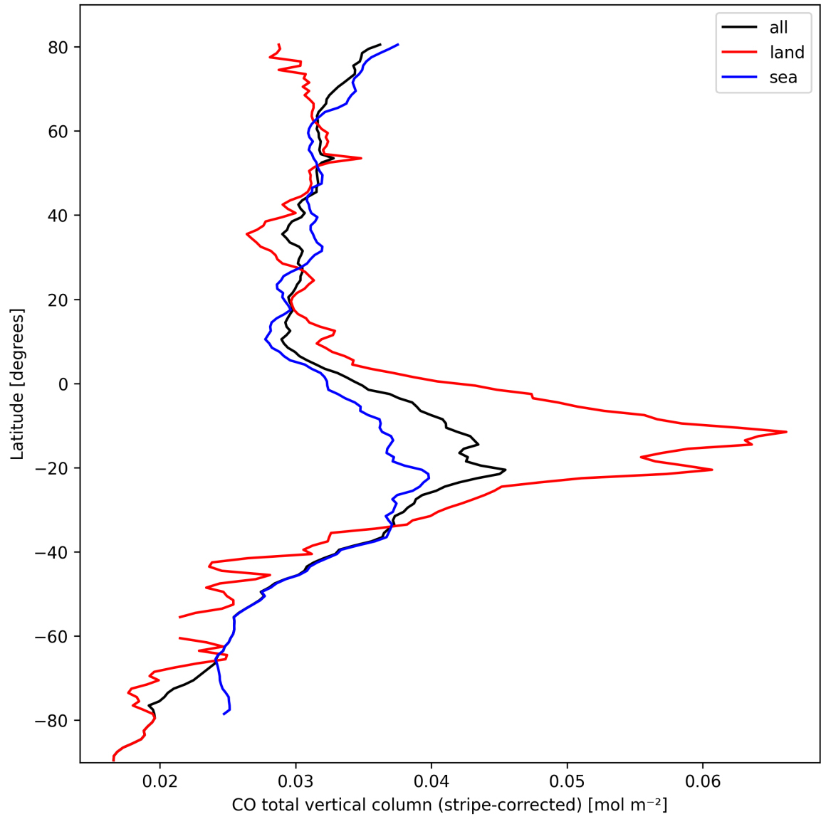
Figure 11: Zonal average of “CO total vertical column (stripe-corrected)” for 2024-10-03 to 2024-10-05.
