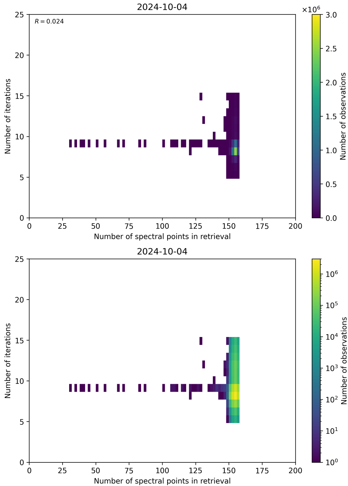
Figure 60: Scatter density plot of “Number of spectral points in retrieval” against “Number of iterations” for 2024-10-03 to 2024-10-05.
