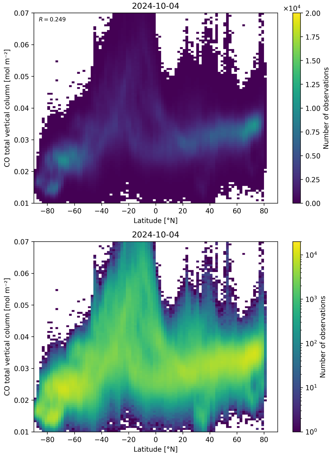
Figure 51: Scatter density plot of “Latitude” against “CO total vertical column” for 2024-10-03 to 2024-10-05.
