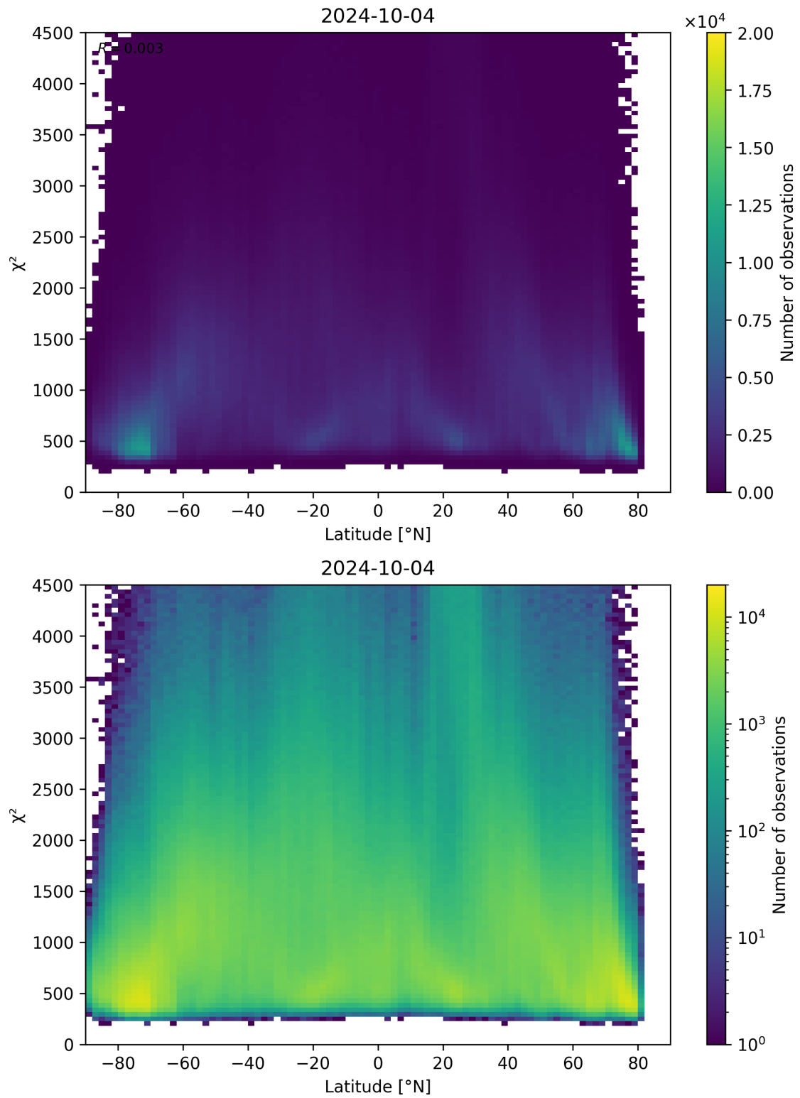
Figure 54: Scatter density plot of “Latitude” against “ \chi^2 ” for 2024-10-03 to 2024-10-05.
