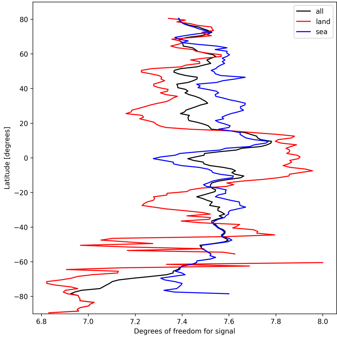
Figure 15: Zonal average of “Degrees of freedom for signal” for 2024-10-03 to 2024-10-05.
