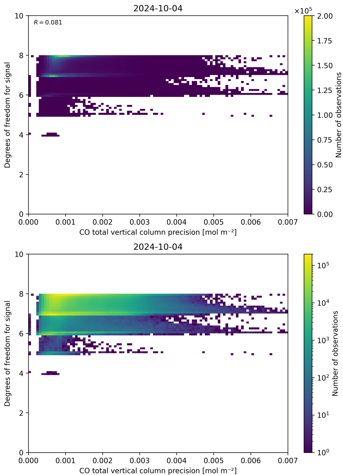
Figure 45: Scatter density plot of “CO total vertical column precision” against “Degrees of freedom for signal” for 2024-10-03 to 2024-10-05.
