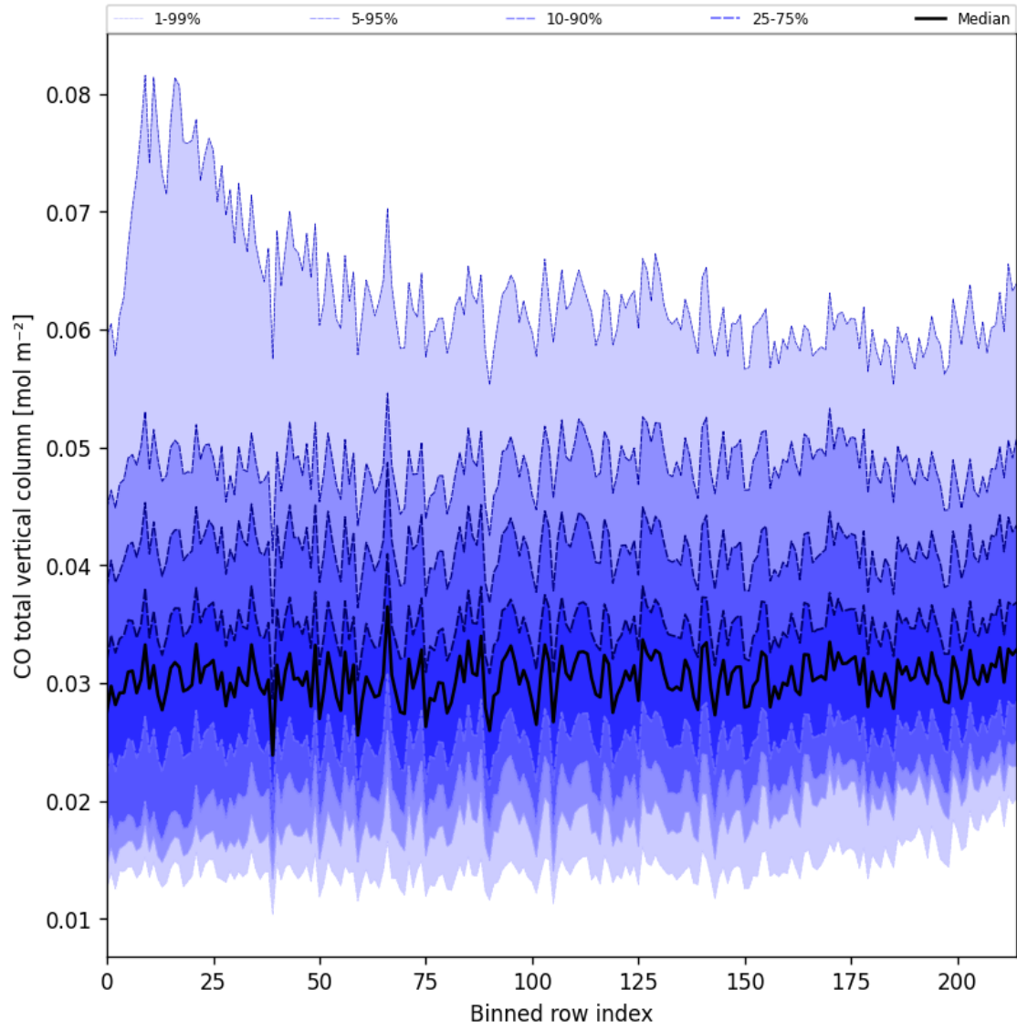
Figure 26: Along track statistics of “CO total vertical column” for 2024-10-03 to 2024-10-05
