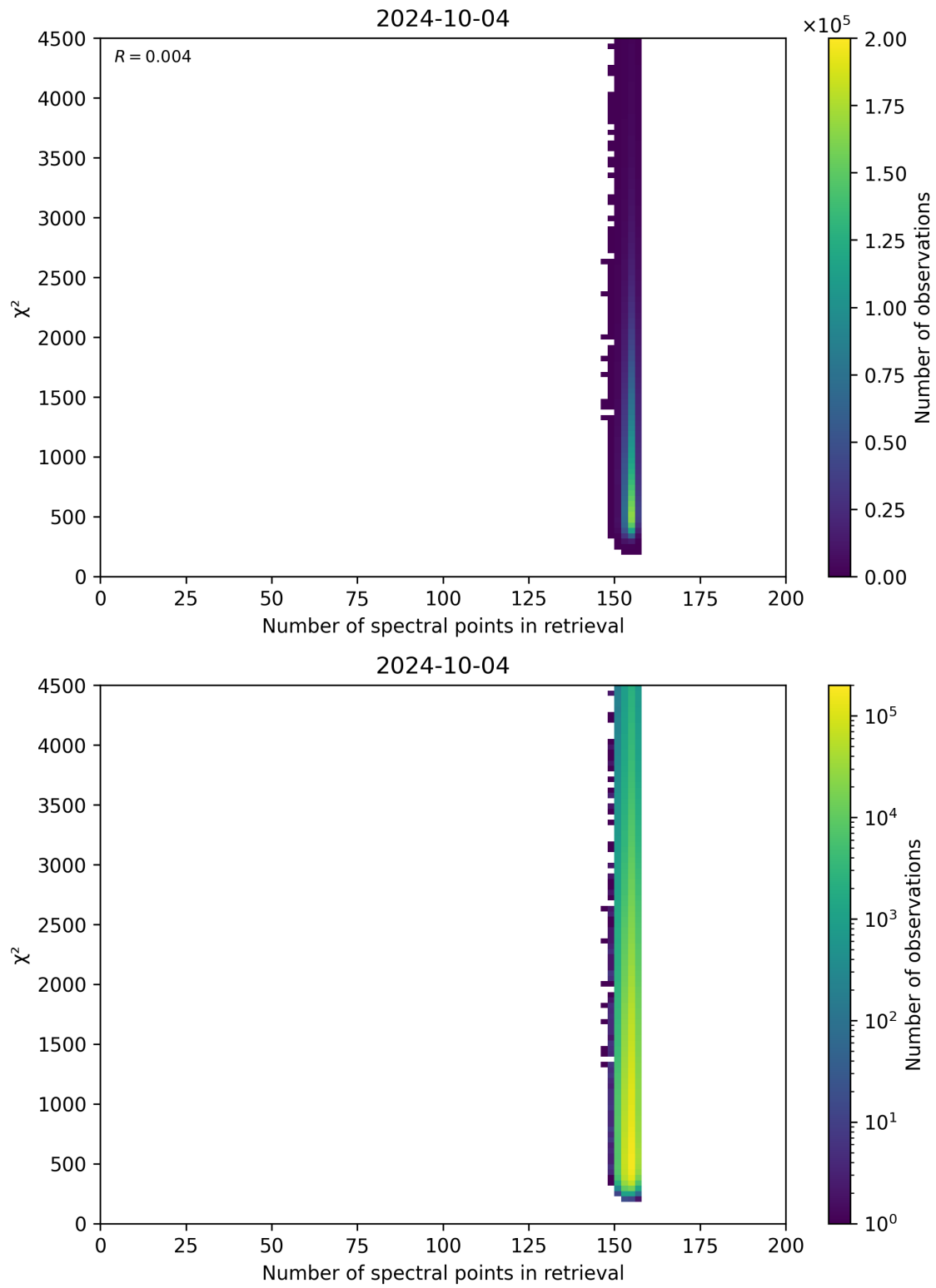
Figure 58: Scatter density plot of “Number of spectral points in retrieval” against “ \chi^2 ” for 2024-10-03 to 2024-10-05.
