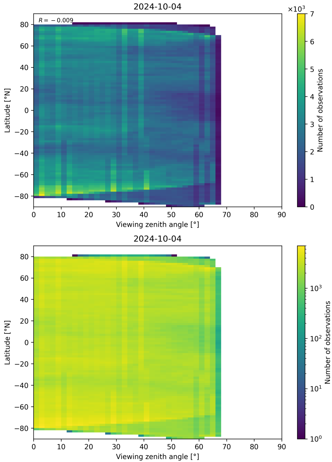
Figure 74: Scatter density plot of “Viewing zenith angle” against “Latitude” for 2024-10-03 to 2024-10-05.
