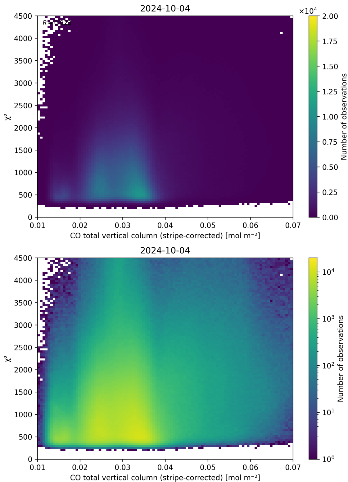
Figure 37: Scatter density plot of “CO total vertical column (stripe-corrected)” against “ \chi^2 ” for 2024-10-03 to 2024-10-05.
