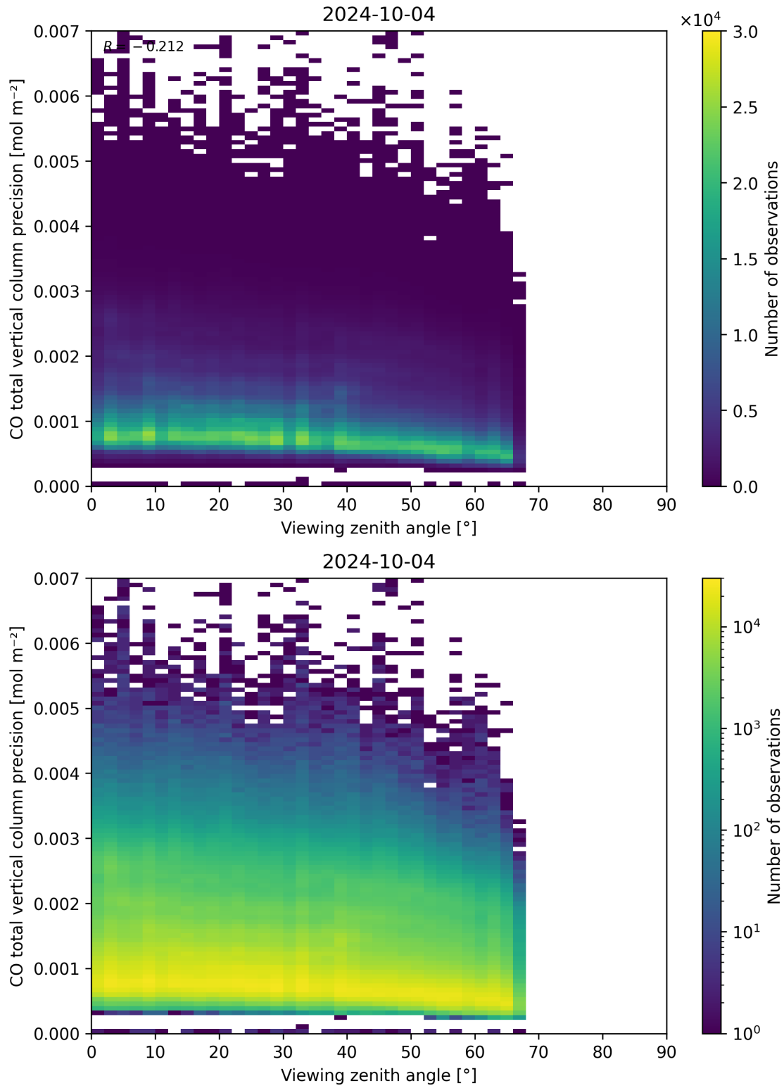
Figure 71: Scatter density plot of “Viewing zenith angle” against “CO total vertical column precision” for 2024-10-03 to 2024-10-05.
