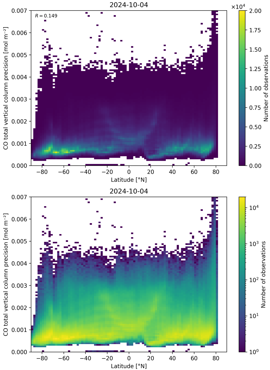
Figure 53: Scatter density plot of “Latitude” against “CO total vertical column precision” for 2024-10-03 to 2024-10-05.
