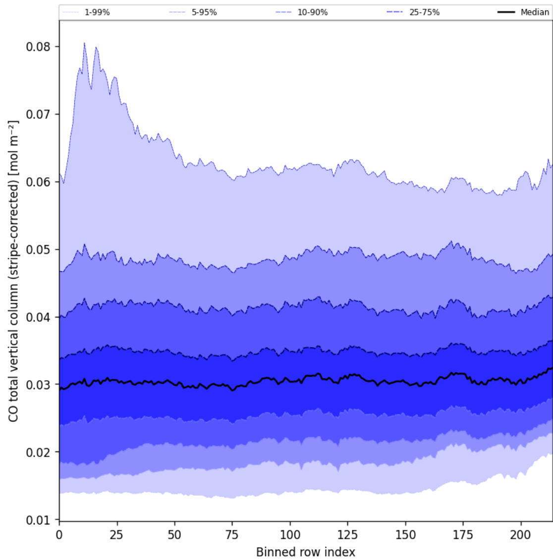
Figure 27: Along track statistics of “CO total vertical column (stripe-corrected)” for 2024-10-03 to 2024-10-05
