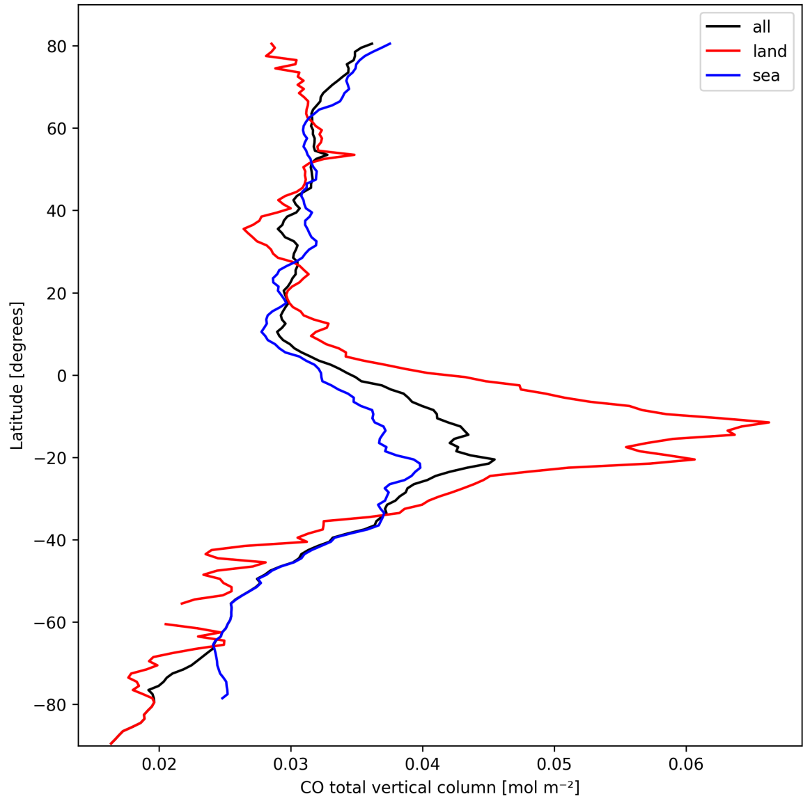
Figure 10: Zonal average of “CO total vertical column” for 2024-10-03 to 2024-10-05.
