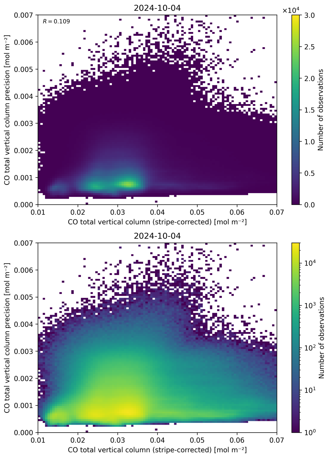
Figure 36: Scatter density plot of “CO total vertical column (stripe-corrected)” against “CO total vertical column precision” for 2024-10-03 to 2024-10-05.
