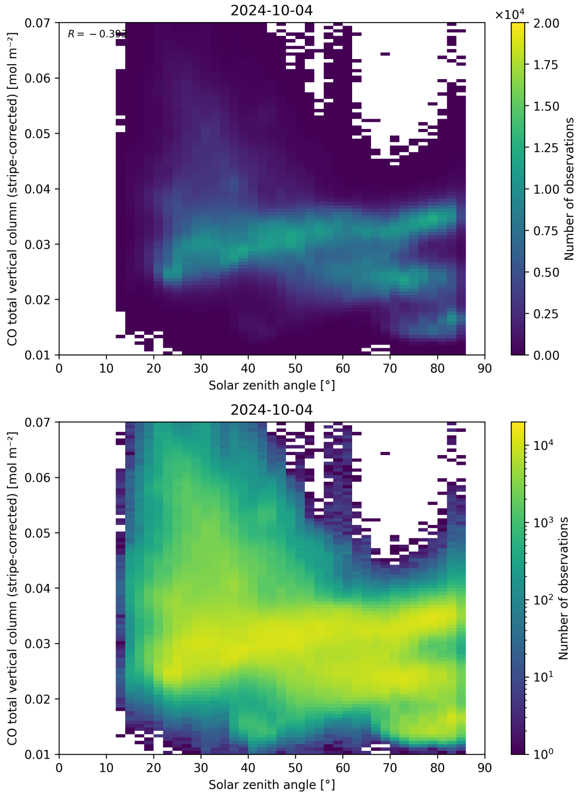
Figure 62: Scatter density plot of “Solar zenith angle” against “CO total vertical column (stripe-corrected)” for 2024-10-03 to 2024-10-05.
