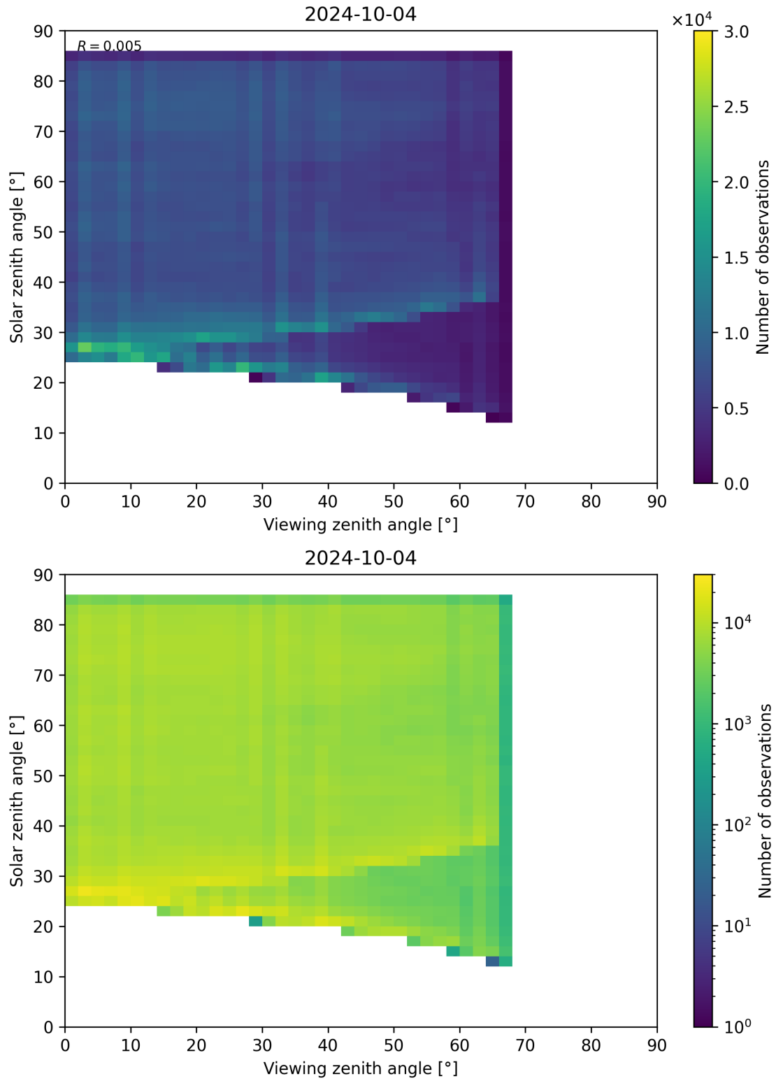
Figure 77: Scatter density plot of “Viewing zenith angle” against “Solar zenith angle” for 2024-10-03 to 2024-10-05.
