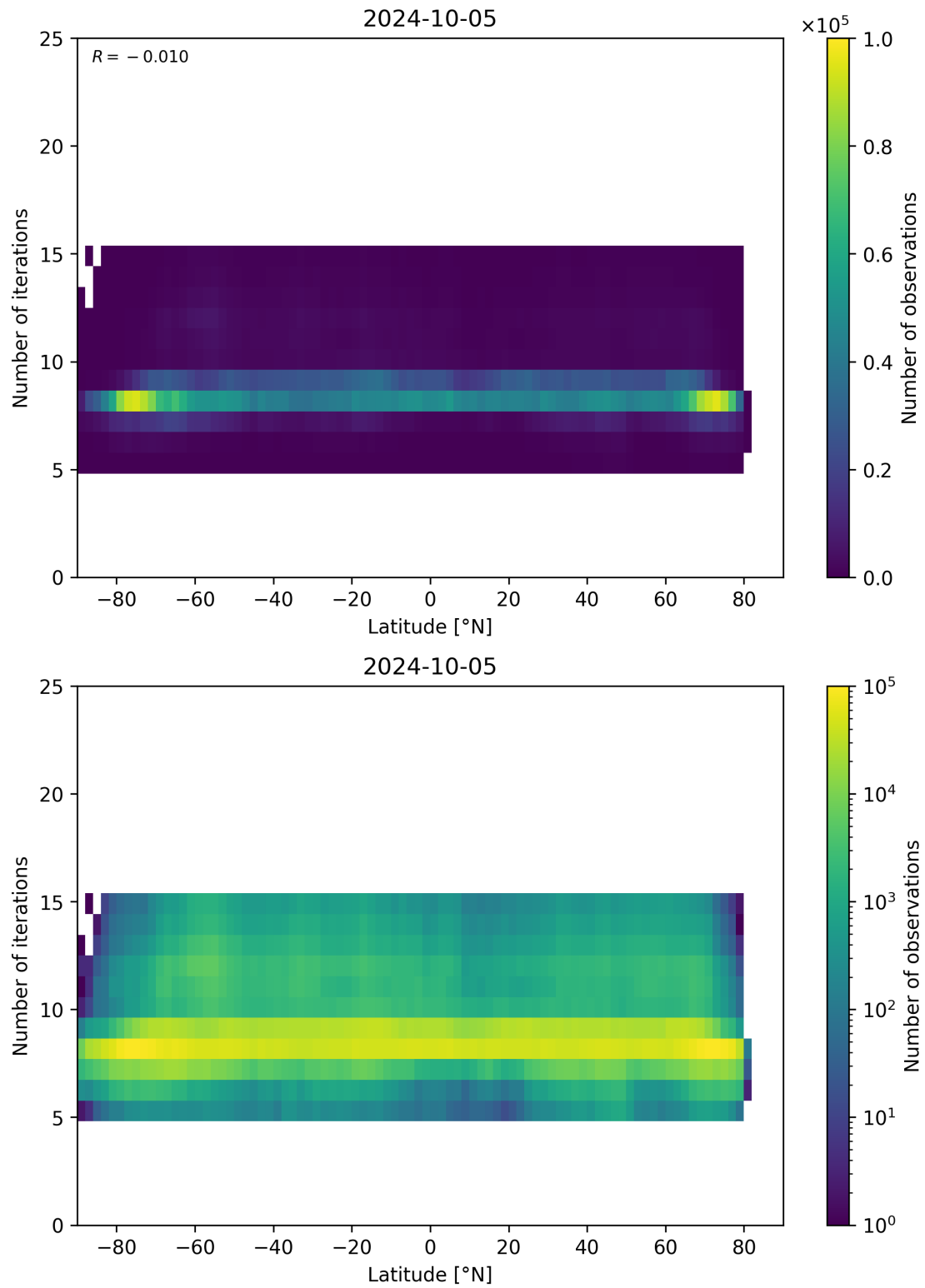
Figure 56: Scatter density plot of “Latitude” against “Number of iterations” for 2024-10-04 to 2024-10-06.
