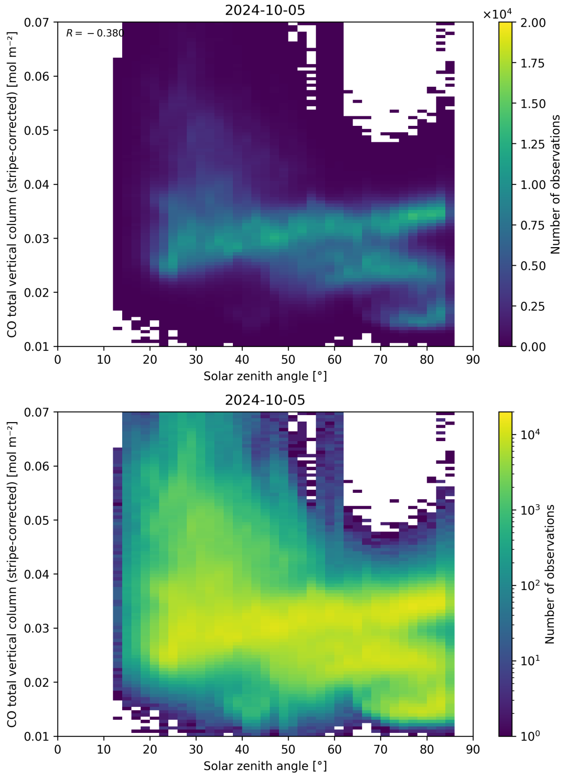
Figure 62: Scatter density plot of “Solar zenith angle” against “CO total vertical column (stripe-corrected)” for 2024-10-04 to 2024-10-06.
