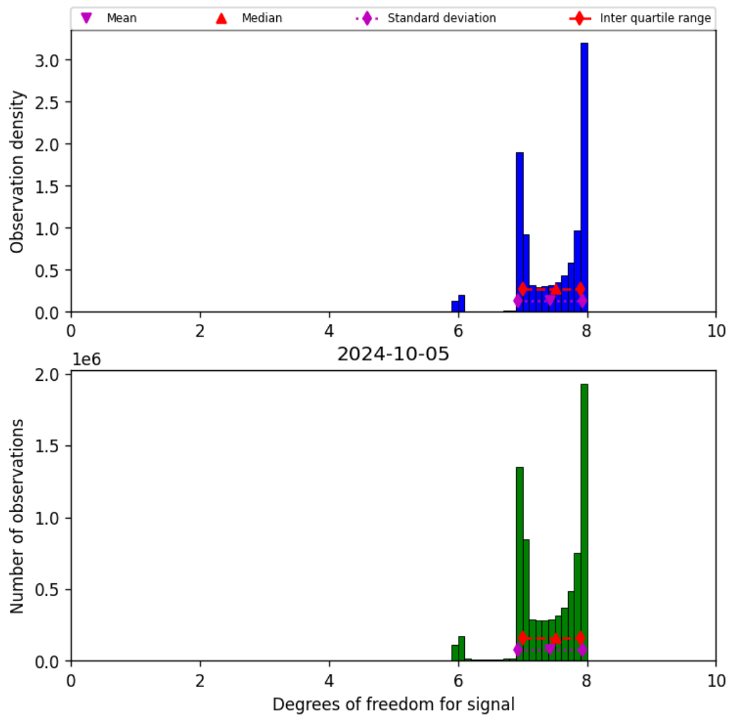
Figure 23: Histogram of “Degrees of freedom for signal” for 2024-10-04 to 2024-10-06
