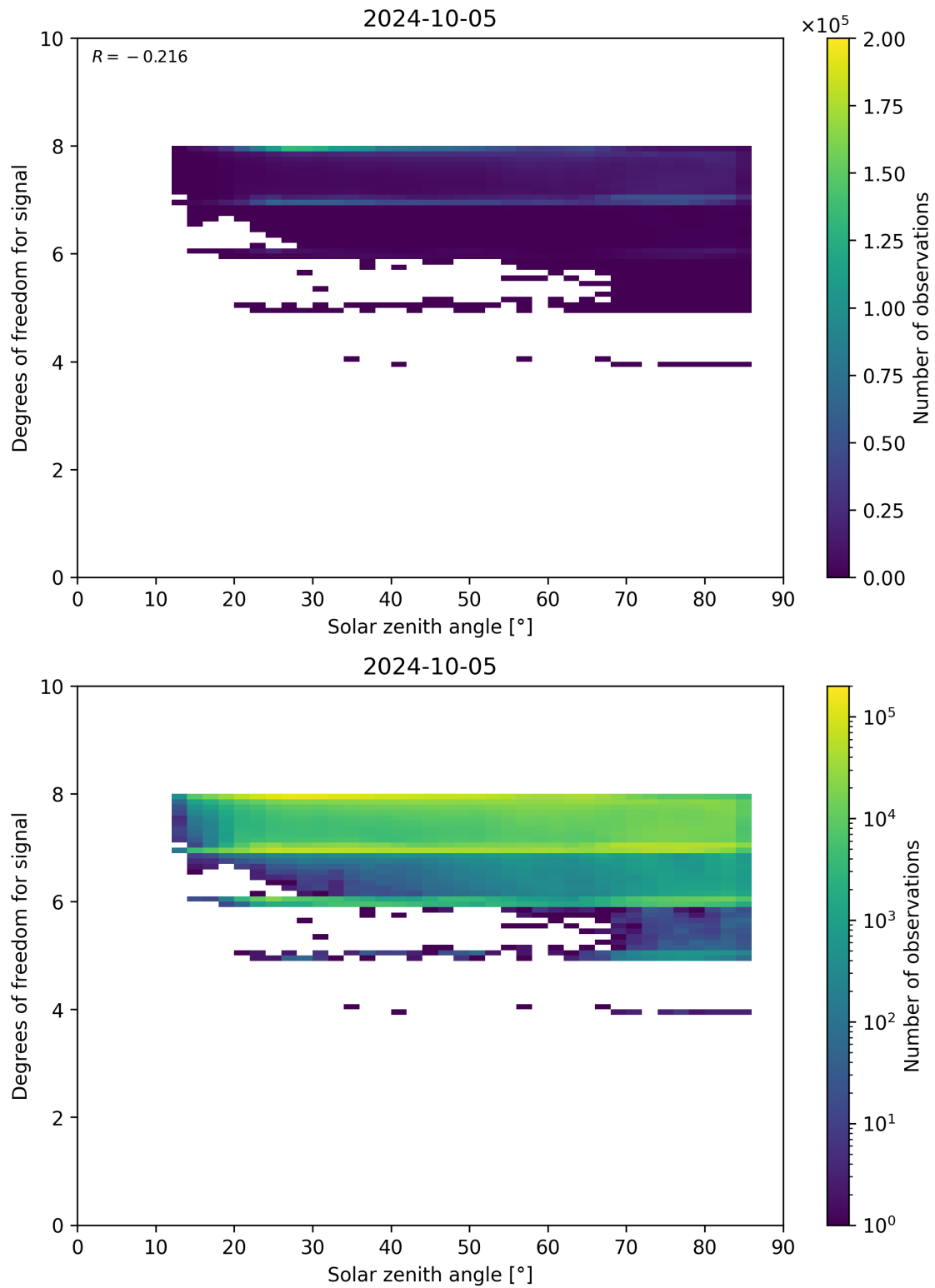
Figure 65: Scatter density plot of “Solar zenith angle” against “Degrees of freedom for signal” for 2024-10-04 to 2024-10-06.
