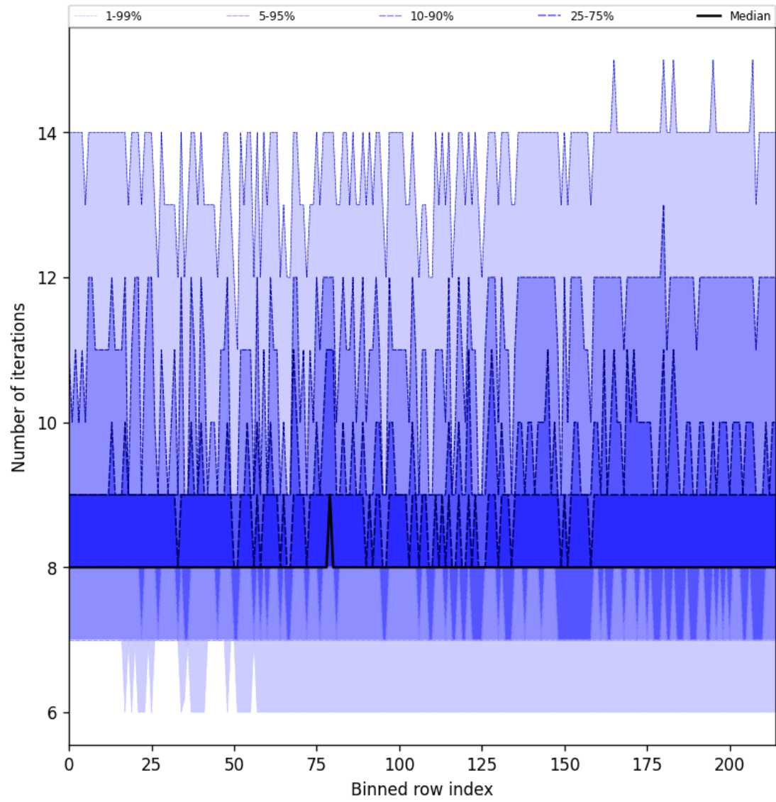
Figure 32: Along track statistics of “Number of iterations” for 2024-10-04 to 2024-10-06
