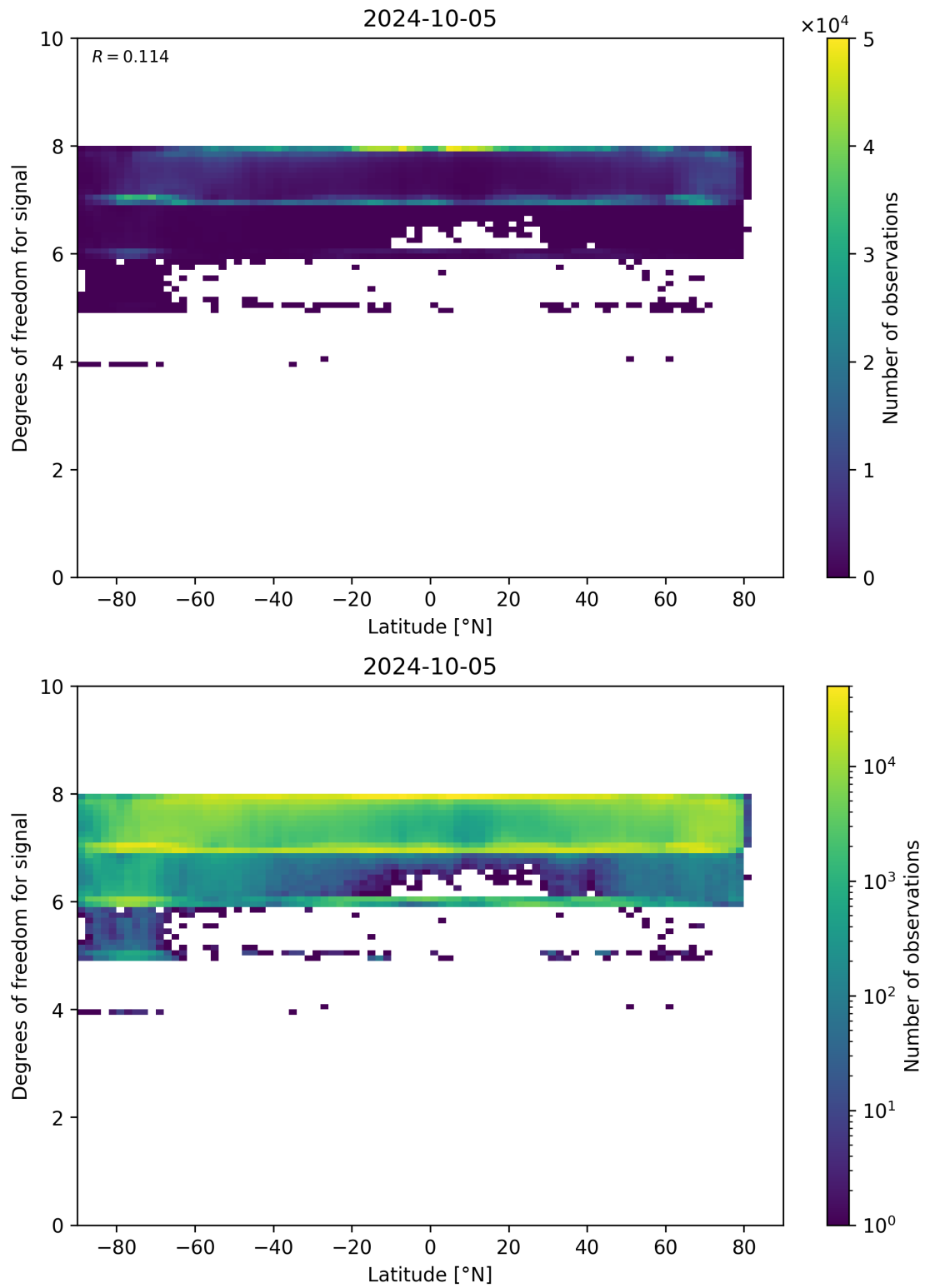
Figure 55: Scatter density plot of “Latitude” against “Degrees of freedom for signal” for 2024-10-04 to 2024-10-06.
