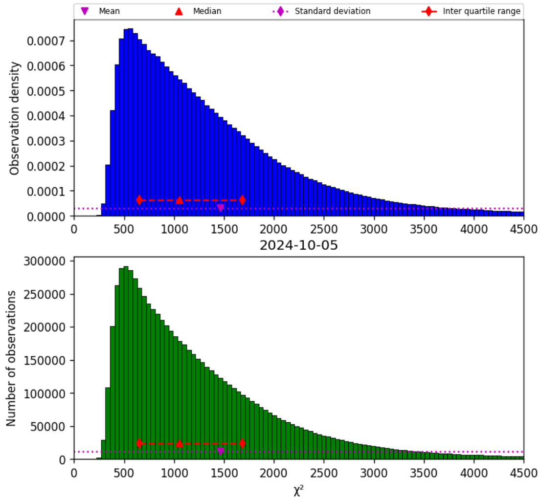
Figure 22: Histogram of “ \chi^2 ” for 2024-10-04 to 2024-10-06
