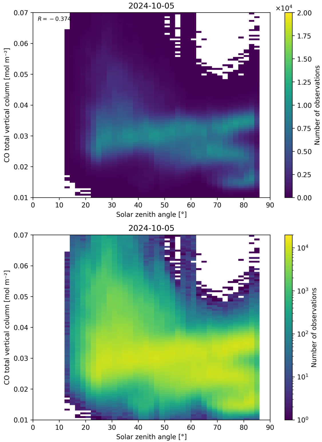
Figure 61: Scatter density plot of “Solar zenith angle” against “CO total vertical column” for 2024-10-04 to 2024-10-06.
