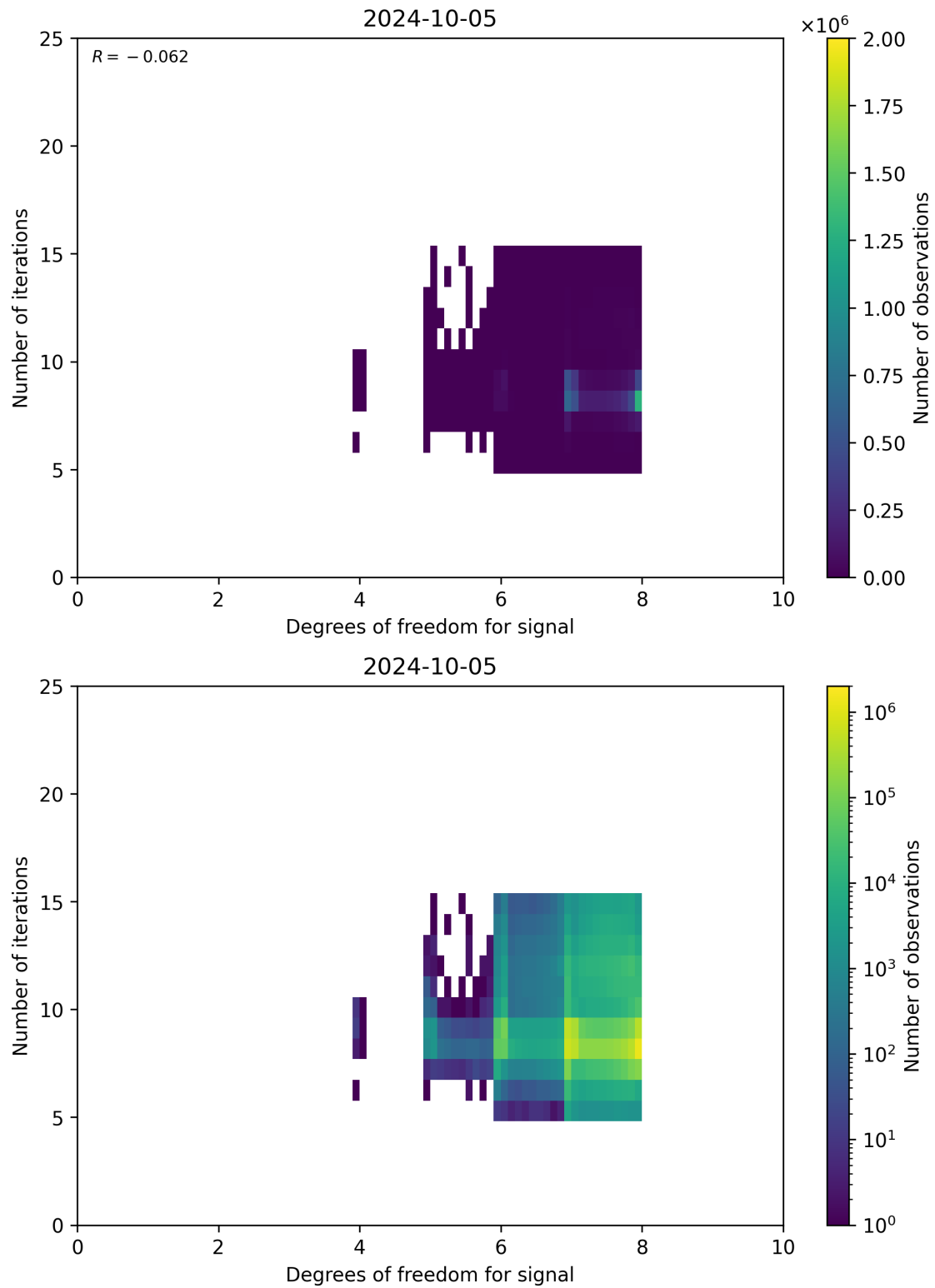
Figure 50: Scatter density plot of “Degrees of freedom for signal” against “Number of iterations” for 2024-10-04 to 2024-10-06.
