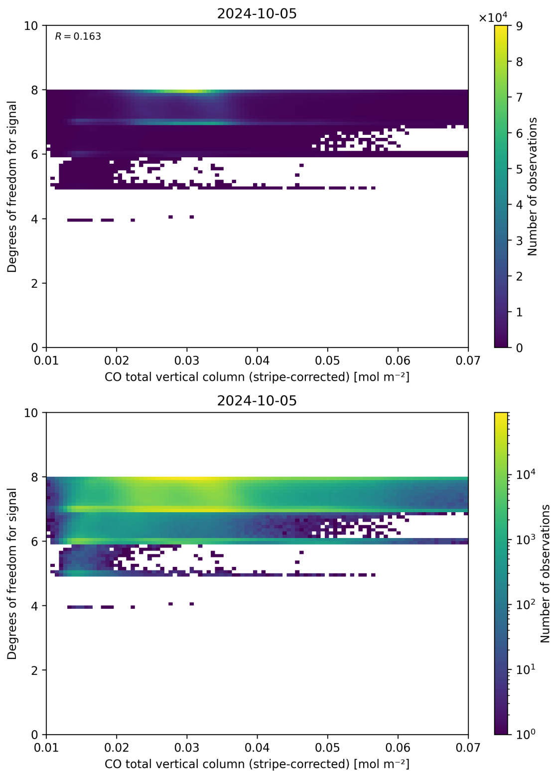
Figure 38: Scatter density plot of “CO total vertical column (stripe-corrected)” against “Degrees of freedom for signal” for 2024-10-04 to 2024-10-06.
