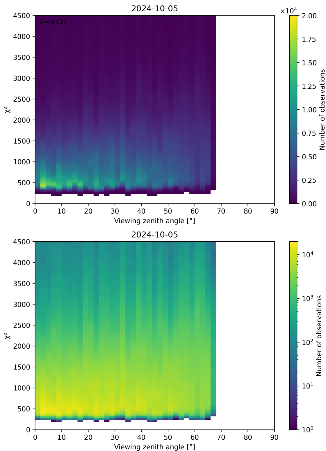
Figure 72: Scatter density plot of “Viewing zenith angle” against “ \chi^2 ” for 2024-10-04 to 2024-10-06.
