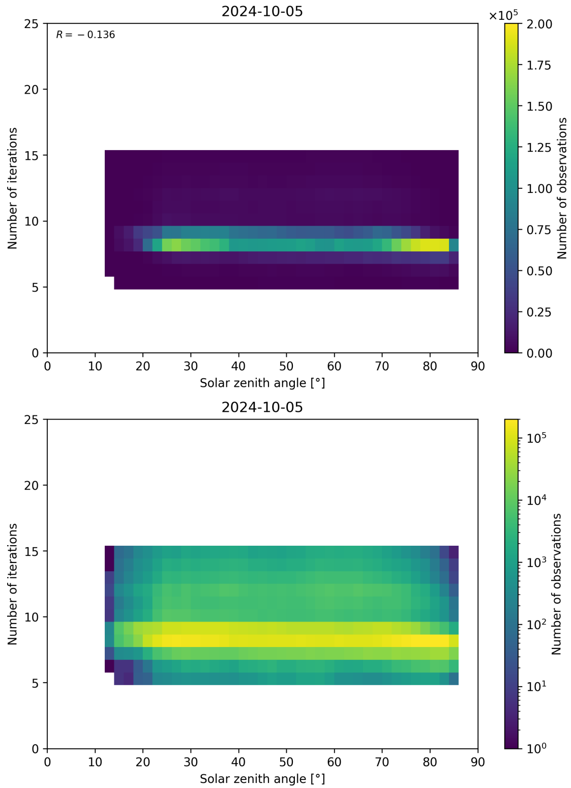
Figure 67: Scatter density plot of “Solar zenith angle” against “Number of iterations” for 2024-10-04 to 2024-10-06.
