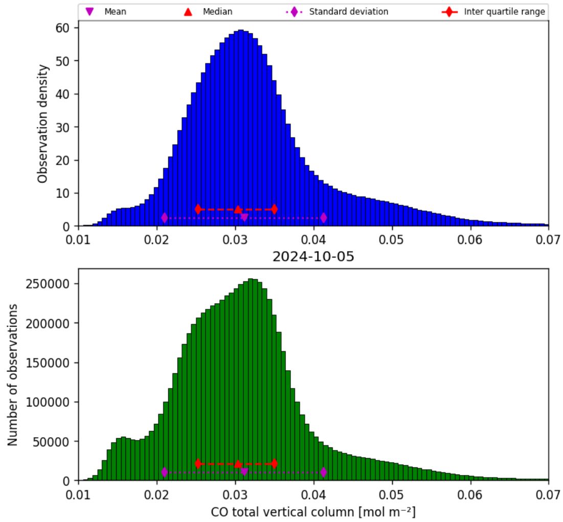
Figure 18: Histogram of “CO total vertical column” for 2024-10-04 to 2024-10-06
