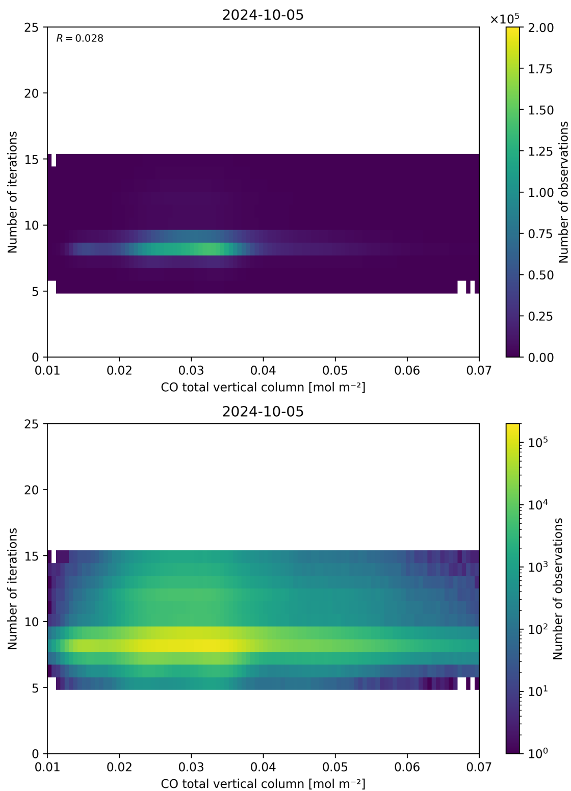
Figure 42: Scatter density plot of “CO total vertical column” against “Number of iterations” for 2024-10-04 to 2024-10-06.
