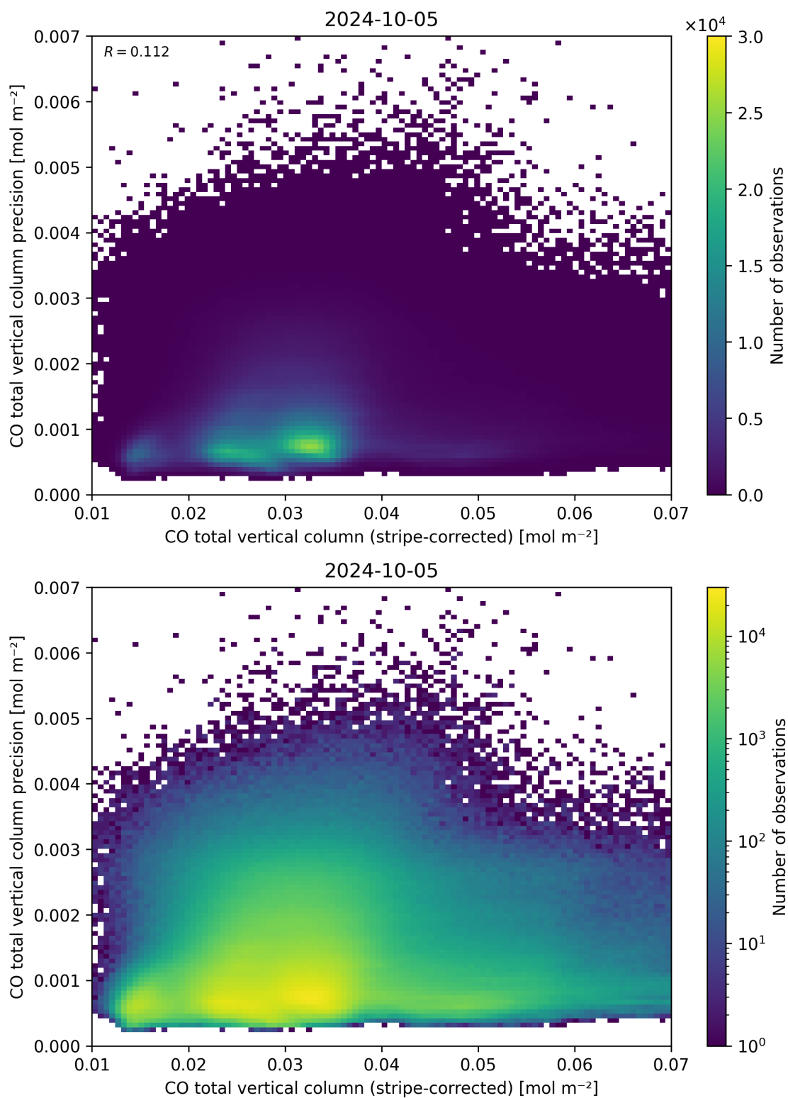
Figure 36: Scatter density plot of “CO total vertical column (stripe-corrected)” against “CO total vertical column precision” for 2024-10-04 to 2024-10-06.
