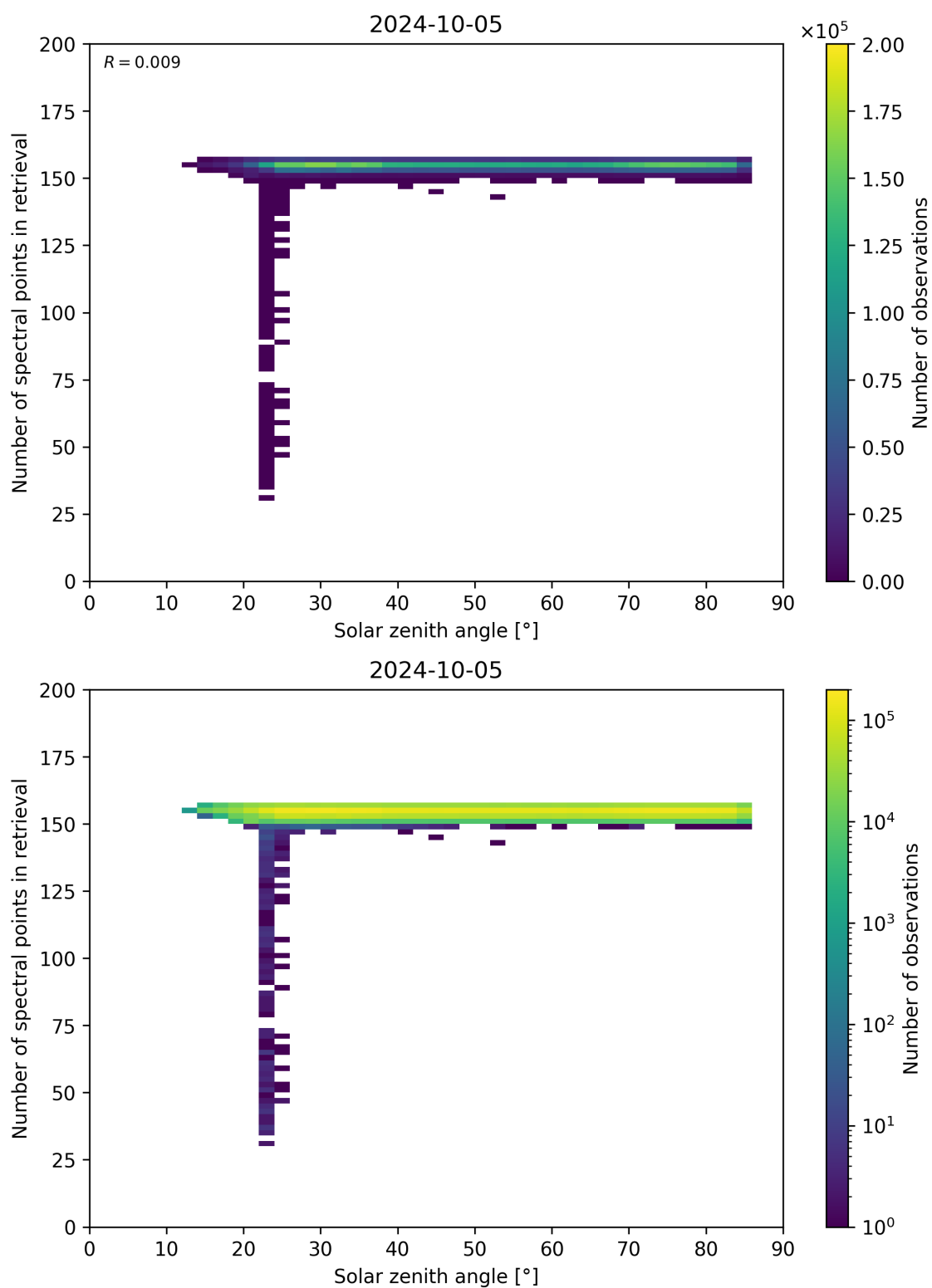
Figure 68: Scatter density plot of “Solar zenith angle” against “Number of spectral points in retrieval” for 2024-10-04 to 2024-10-06.
