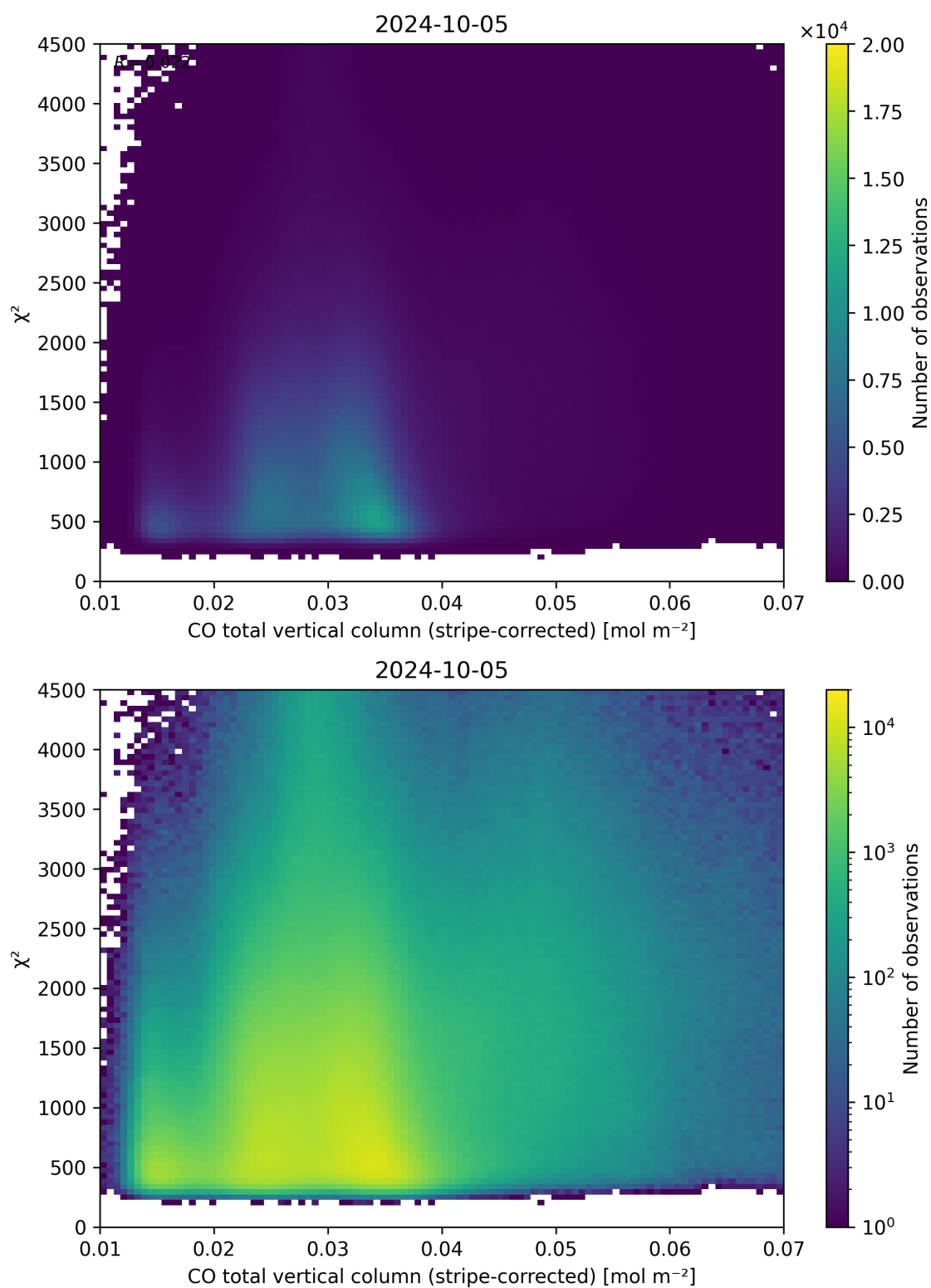
Figure 37: Scatter density plot of “CO total vertical column (stripe-corrected)” against “ \chi^2 ” for 2024-10-04 to 2024-10-06.
