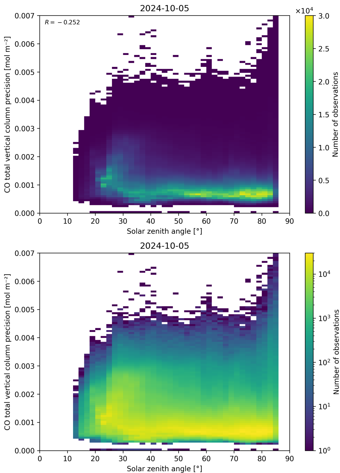
Figure 63: Scatter density plot of “Solar zenith angle” against “CO total vertical column precision” for 2024-10-04 to 2024-10-06.
