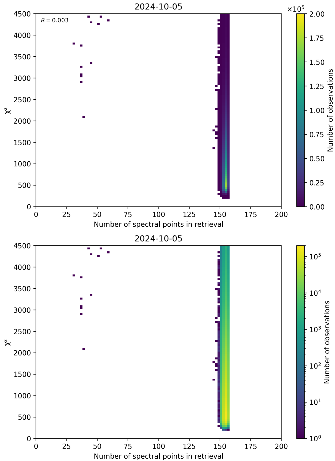
Figure 58: Scatter density plot of “Number of spectral points in retrieval” against “ \chi^2 ” for 2024-10-04 to 2024-10-06.
