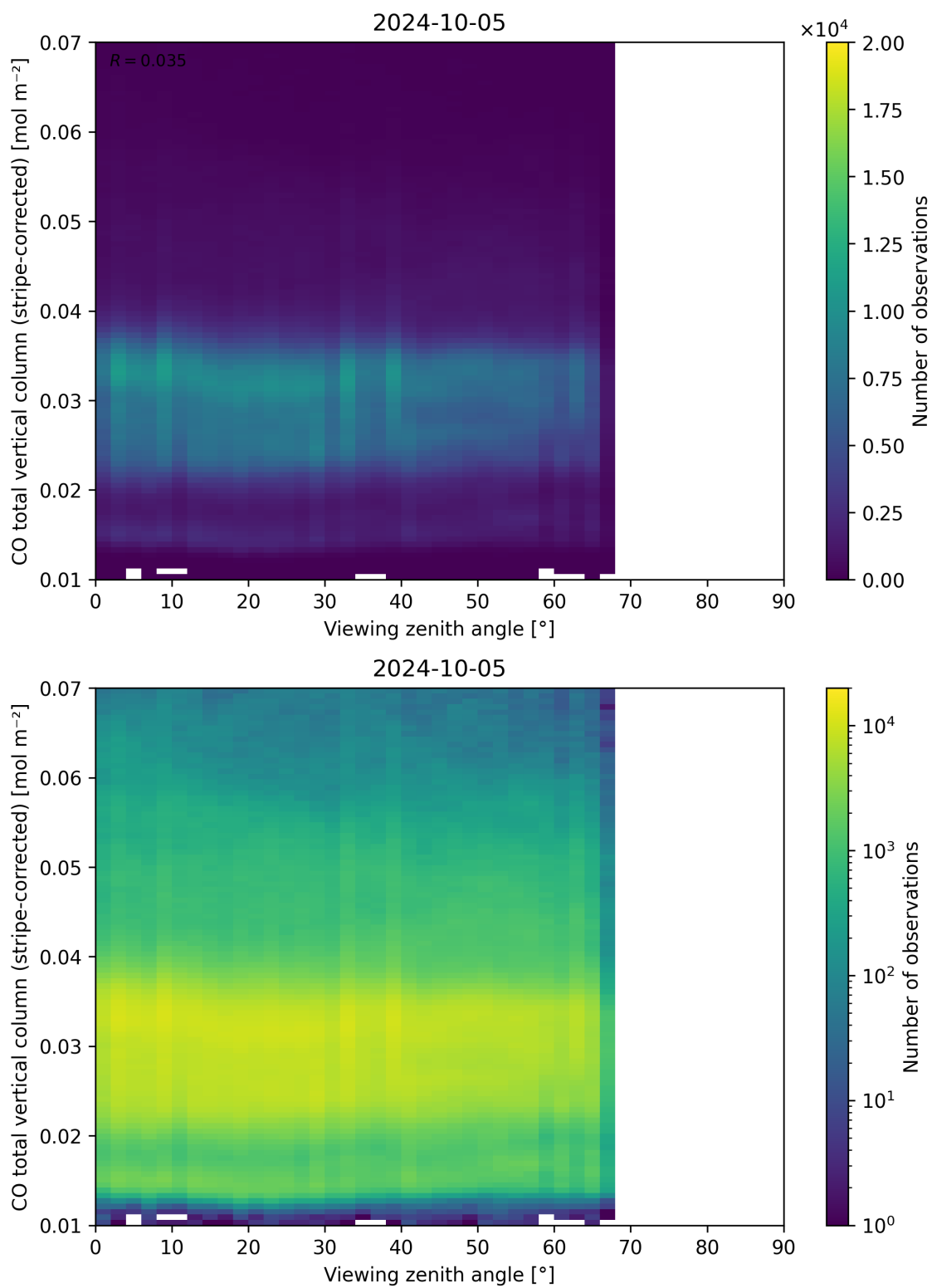
Figure 70: Scatter density plot of “Viewing zenith angle” against “CO total vertical column (stripe-corrected)” for 2024-10-04 to 2024-10-06.
