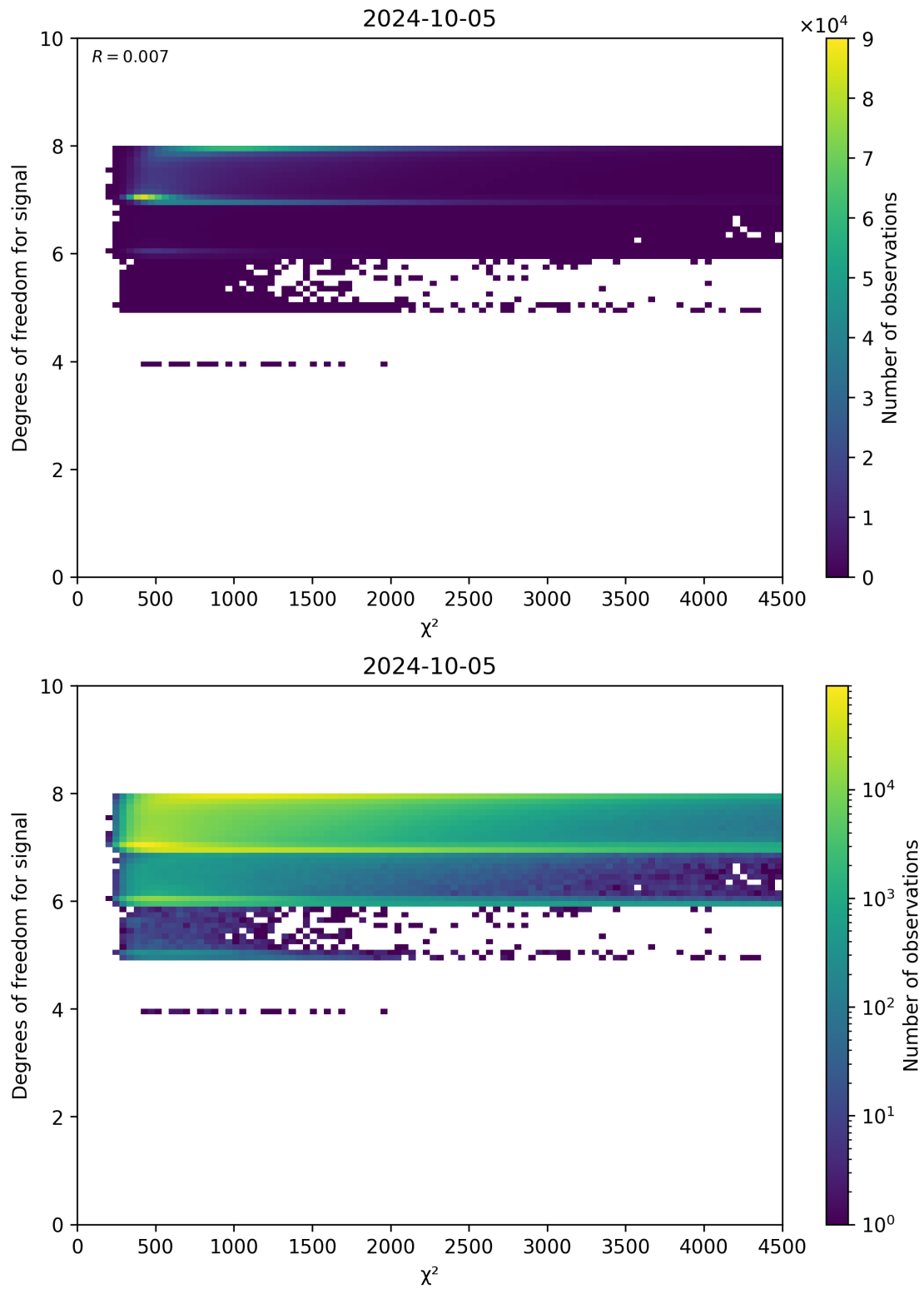
Figure 48: Scatter density plot of “ \chi^2 ” against “Degrees of freedom for signal” for 2024-10-04 to 2024-10-06.
