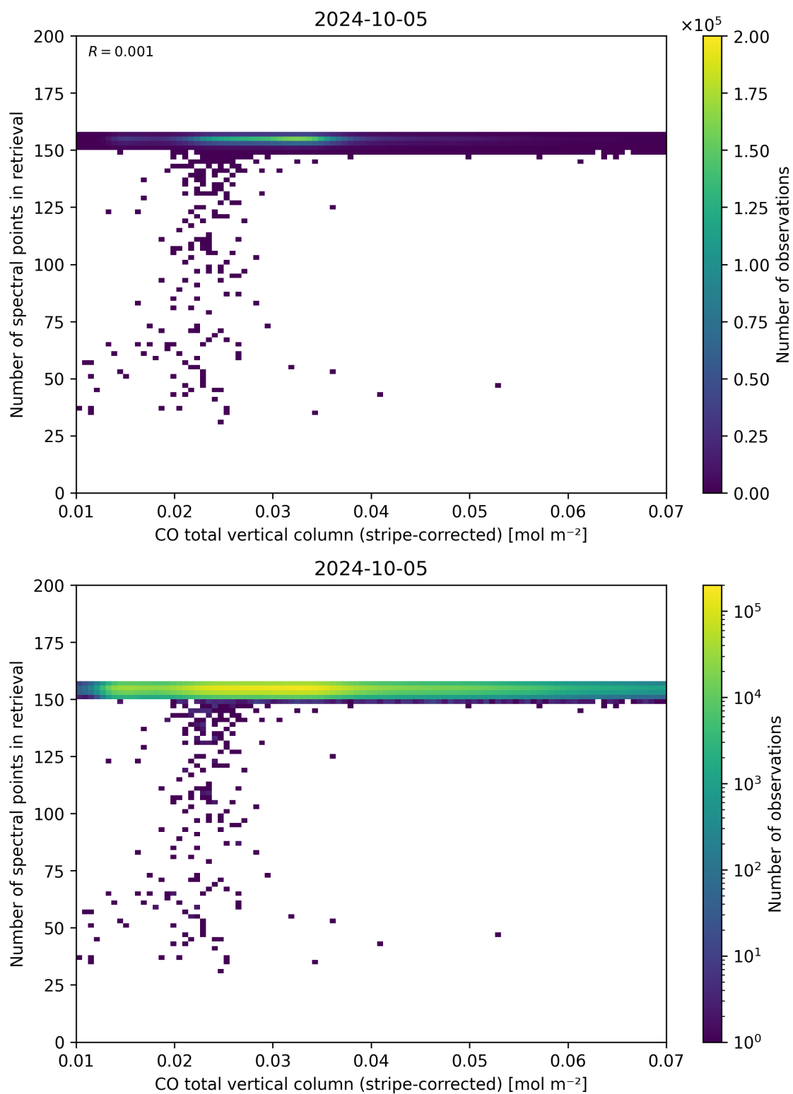
Figure 40: Scatter density plot of “CO total vertical column (stripe-corrected)” against “Number of spectral points in retrieval” for 2024-10-04 to 2024-10-06.
