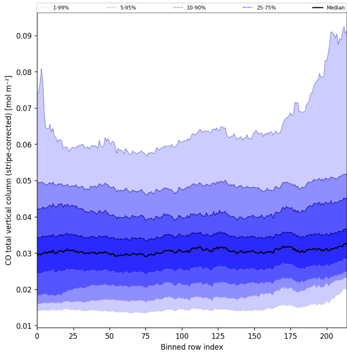
Figure 27: Along track statistics of “CO total vertical column (stripe-corrected)” for 2024-10-04 to 2024-10-06
