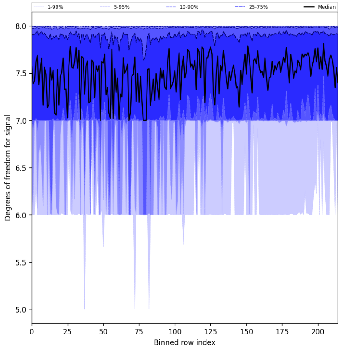
Figure 31: Along track statistics of “Degrees of freedom for signal” for 2024-10-04 to 2024-10-06
