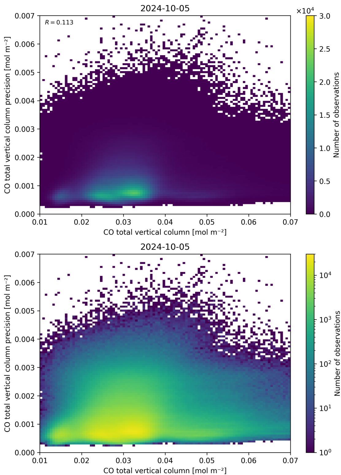
Figure 34: Scatter density plot of “CO total vertical column” against “CO total vertical column precision” for 2024-10-04 to 2024-10-06.
