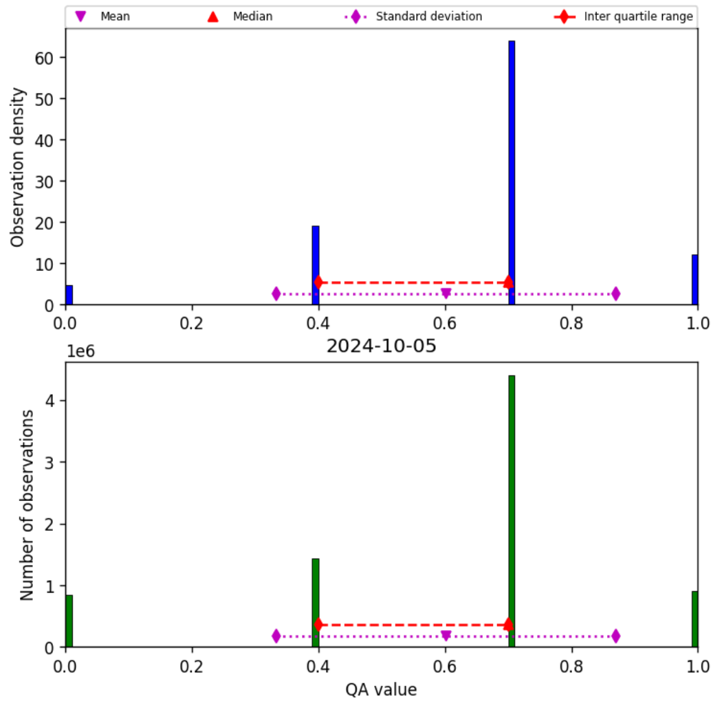
Figure 17: Histogram of “QA value” for 2024-10-04 to 2024-10-06
