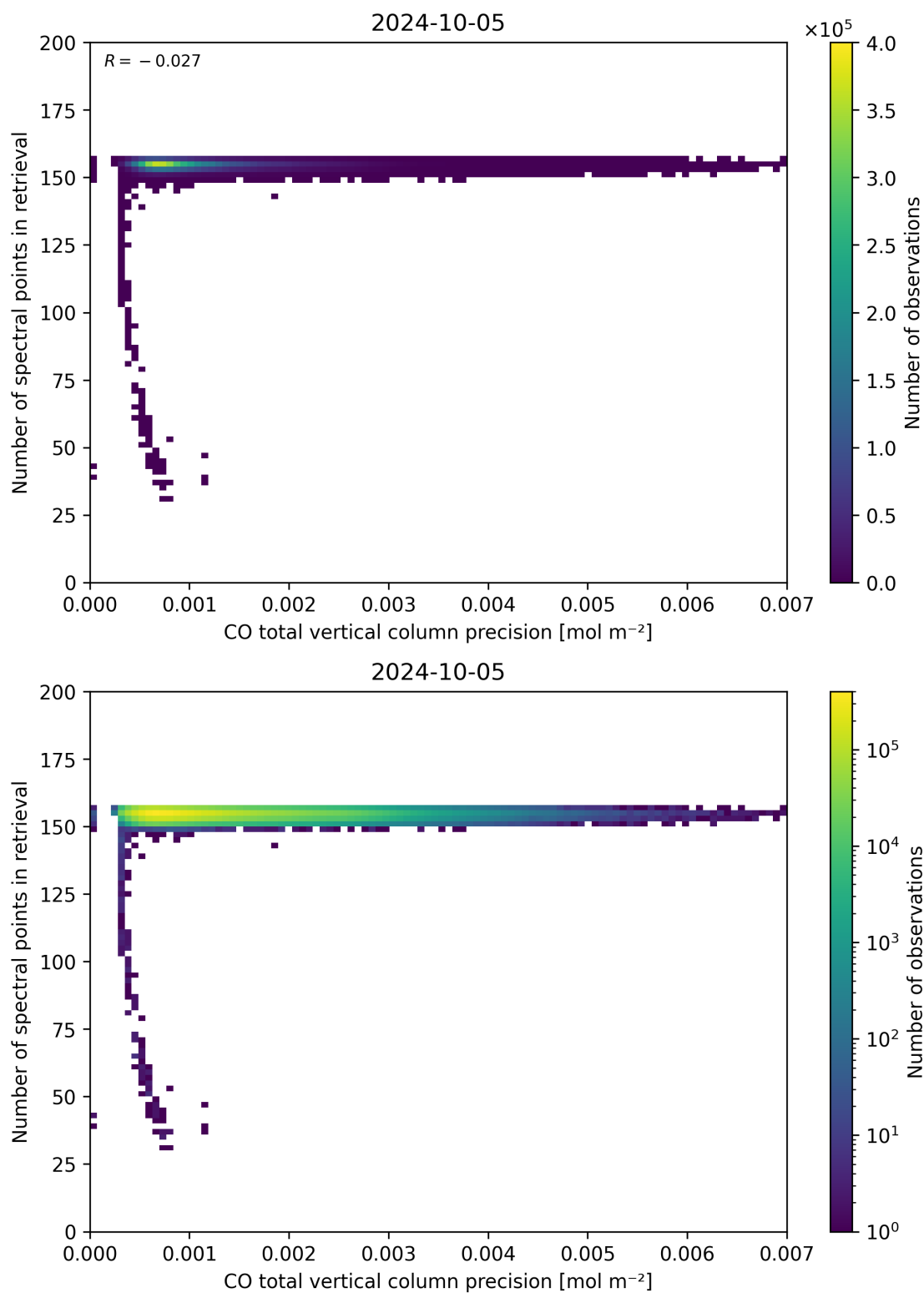
Figure 47: Scatter density plot of “CO total vertical column precision” against “Number of spectral points in retrieval” for 2024-10-04 to 2024-10-06.
