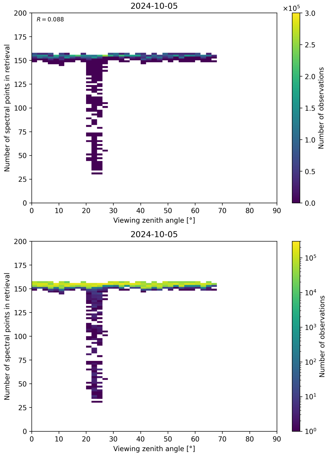
Figure 76: Scatter density plot of “Viewing zenith angle” against “Number of spectral points in retrieval” for 2024-10-04 to 2024-10-06.
