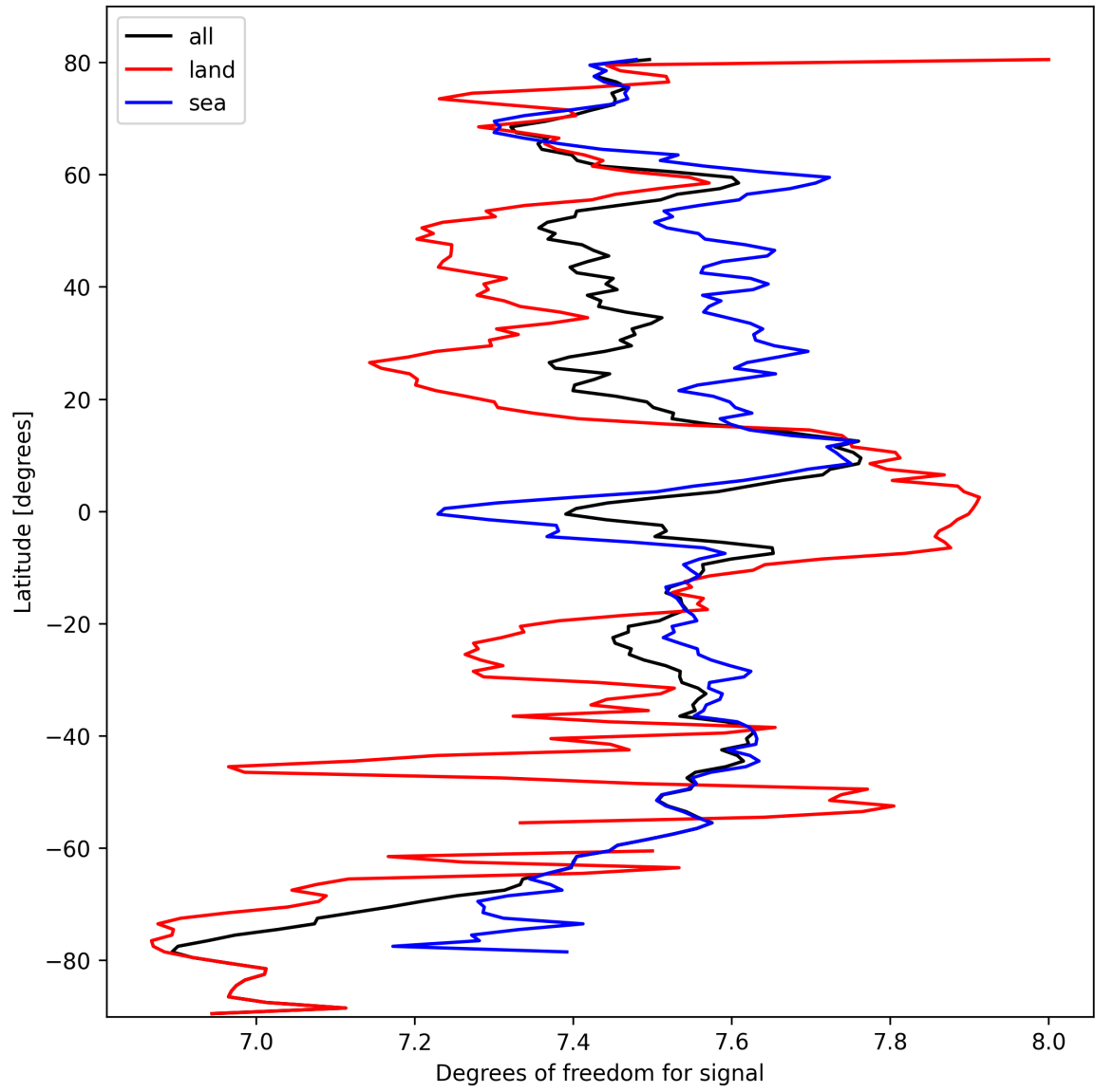
Figure 15: Zonal average of “Degrees of freedom for signal” for 2024-10-04 to 2024-10-06.
