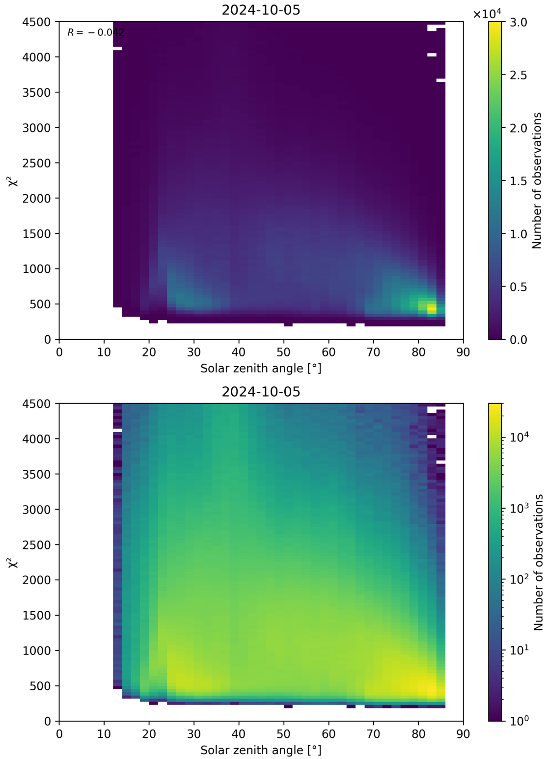
Figure 64: Scatter density plot of “Solar zenith angle” against “ \chi^2 ” for 2024-10-04 to 2024-10-06.
