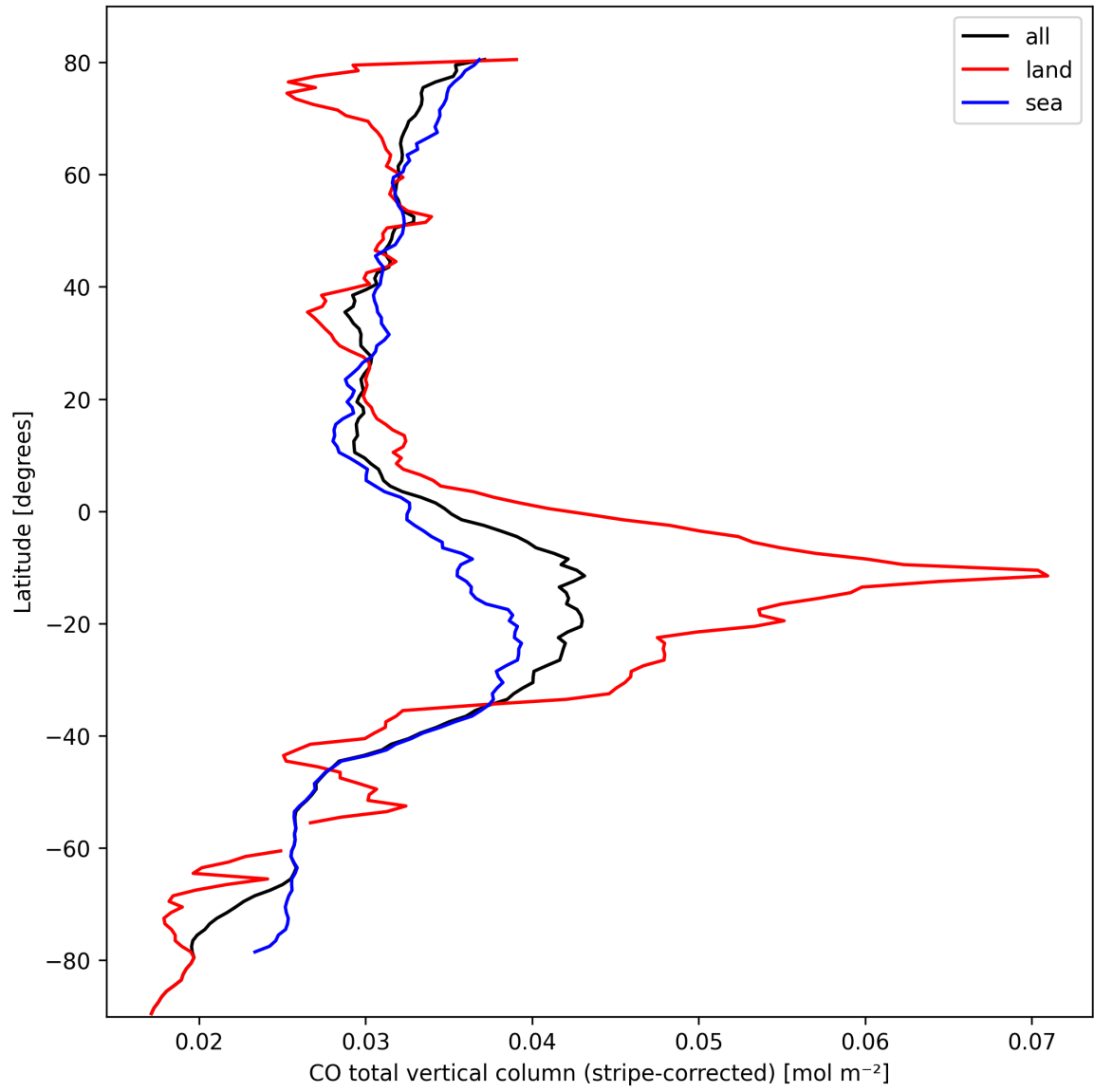
Figure 11: Zonal average of “CO total vertical column (stripe-corrected)” for 2024-10-04 to 2024-10-06.
