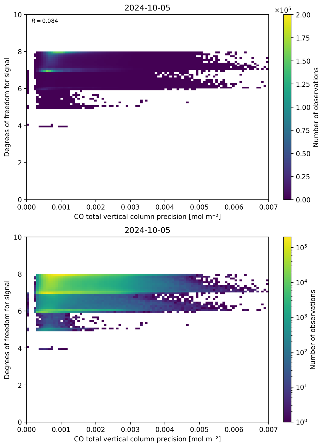
Figure 45: Scatter density plot of “CO total vertical column precision” against “Degrees of freedom for signal” for 2024-10-04 to 2024-10-06.
