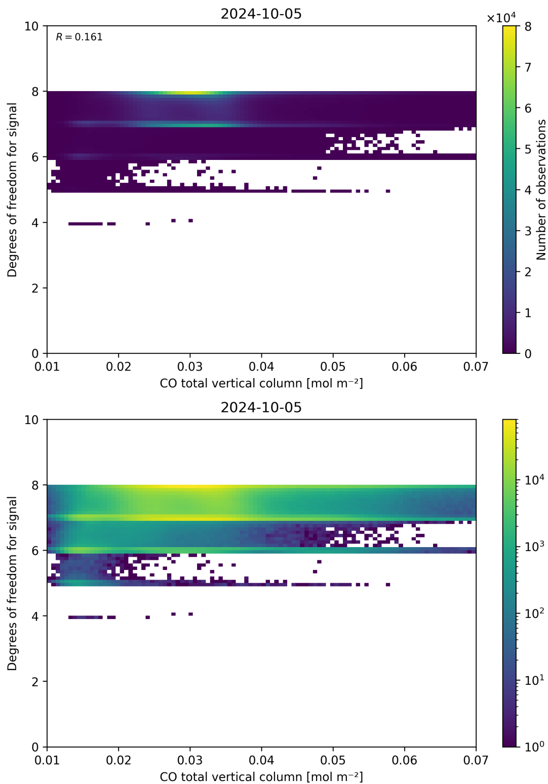
Figure 41: Scatter density plot of “CO total vertical column” against “Degrees of freedom for signal” for 2024-10-04 to 2024-10-06.
