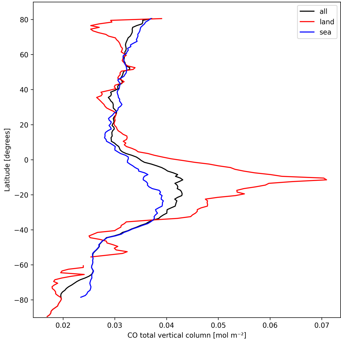
Figure 10: Zonal average of “CO total vertical column” for 2024-10-04 to 2024-10-06.
