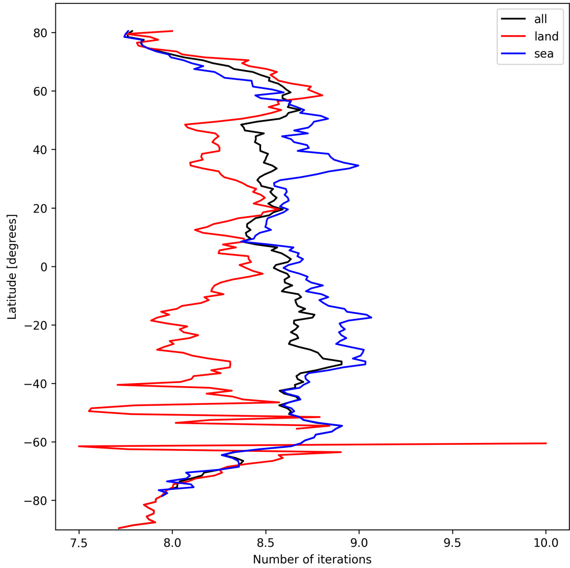
Figure 16: Zonal average of “Number of iterations” for 2024-10-04 to 2024-10-06.
