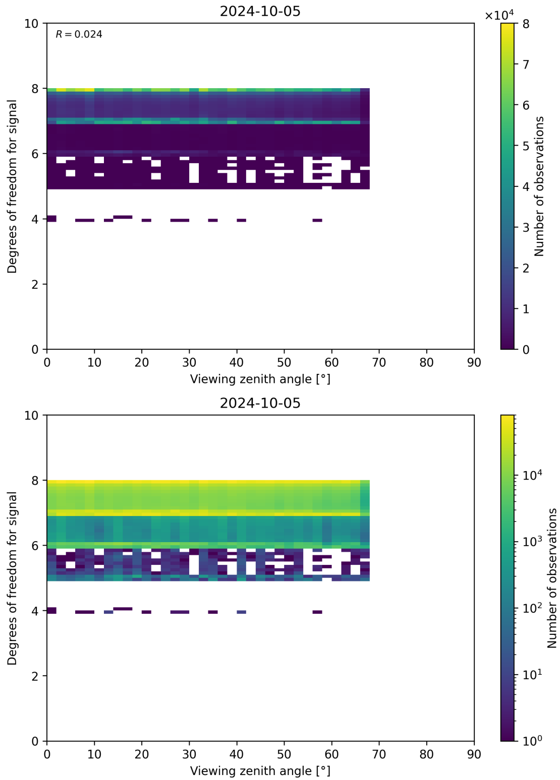
Figure 73: Scatter density plot of “Viewing zenith angle” against “Degrees of freedom for signal” for 2024-10-04 to 2024-10-06.
