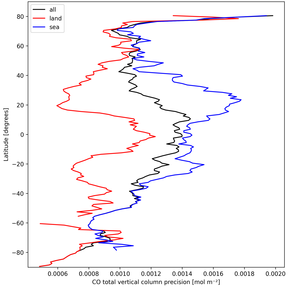
Figure 12: Zonal average of “CO total vertical column precision” for 2024-10-04 to 2024-10-06.
