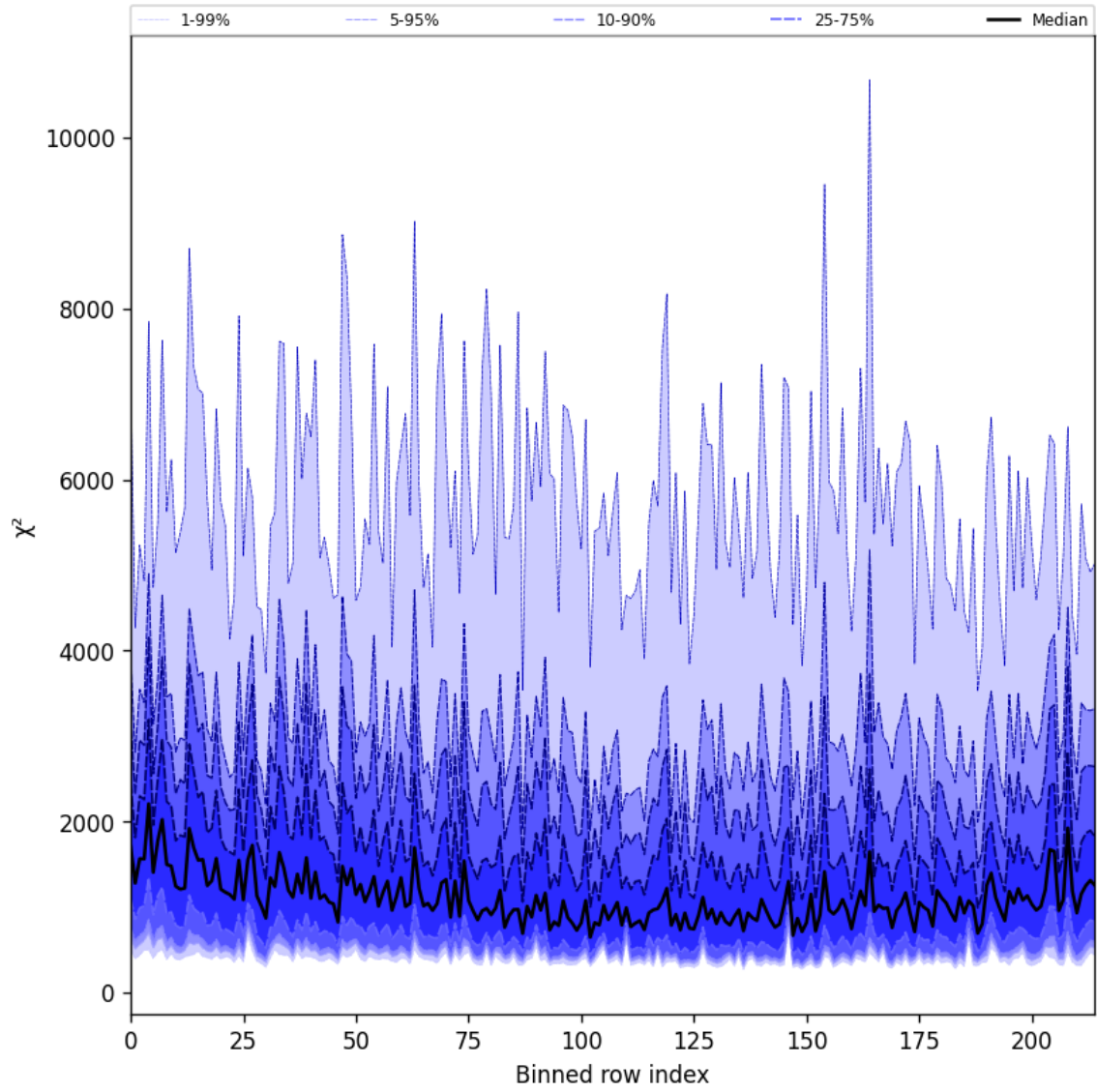
Figure 30: Along track statistics of “ \chi^2 ” for 2024-10-04 to 2024-10-06
