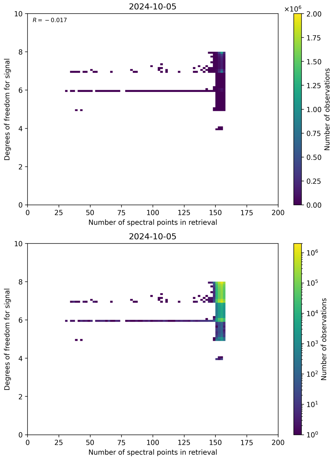
Figure 59: Scatter density plot of “Number of spectral points in retrieval” against “Degrees of freedom for signal” for 2024-10-04 to 2024-10-06.
