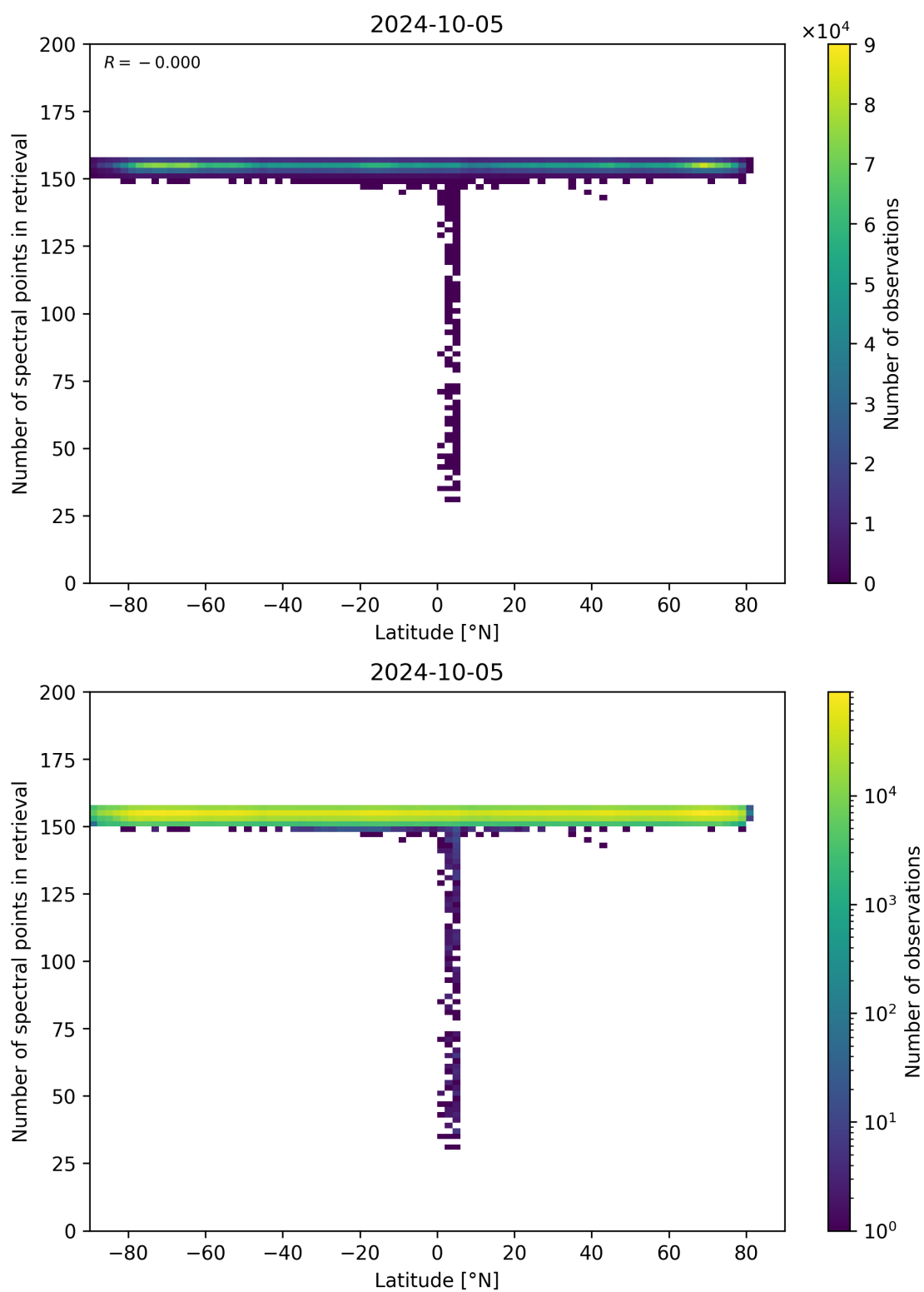
Figure 57: Scatter density plot of “Latitude” against “Number of spectral points in retrieval” for 2024-10-04 to 2024-10-06.
