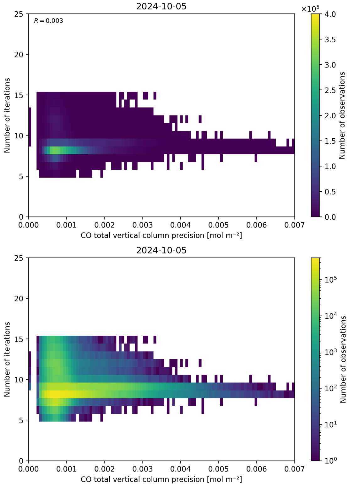
Figure 46: Scatter density plot of “CO total vertical column precision” against “Number of iterations” for 2024-10-04 to 2024-10-06.
