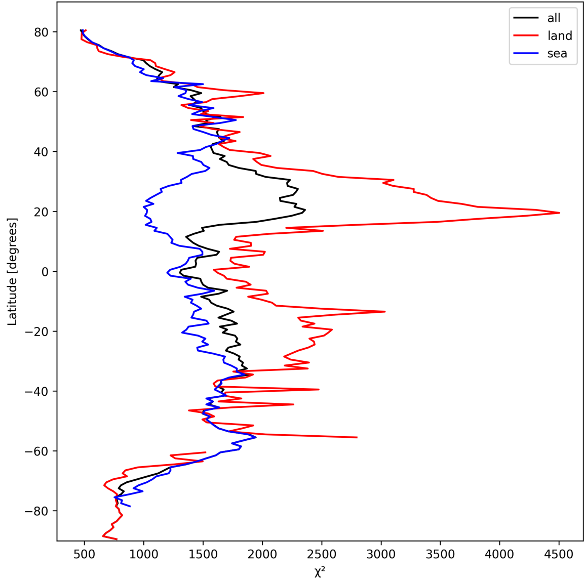
Figure 14: Zonal average of “ \chi^2 ” for 2024-10-04 to 2024-10-06.
