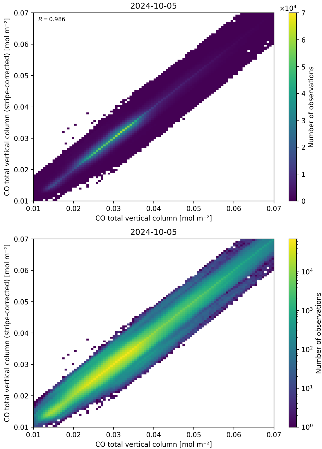
Figure 33: Scatter density plot of “CO total vertical column” against “CO total vertical column (stripe-corrected)” for 2024-10-04 to 2024-10-06.
