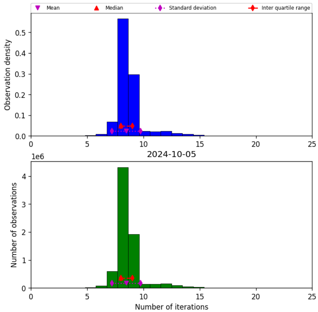
Figure 24: Histogram of “Number of iterations” for 2024-10-04 to 2024-10-06
