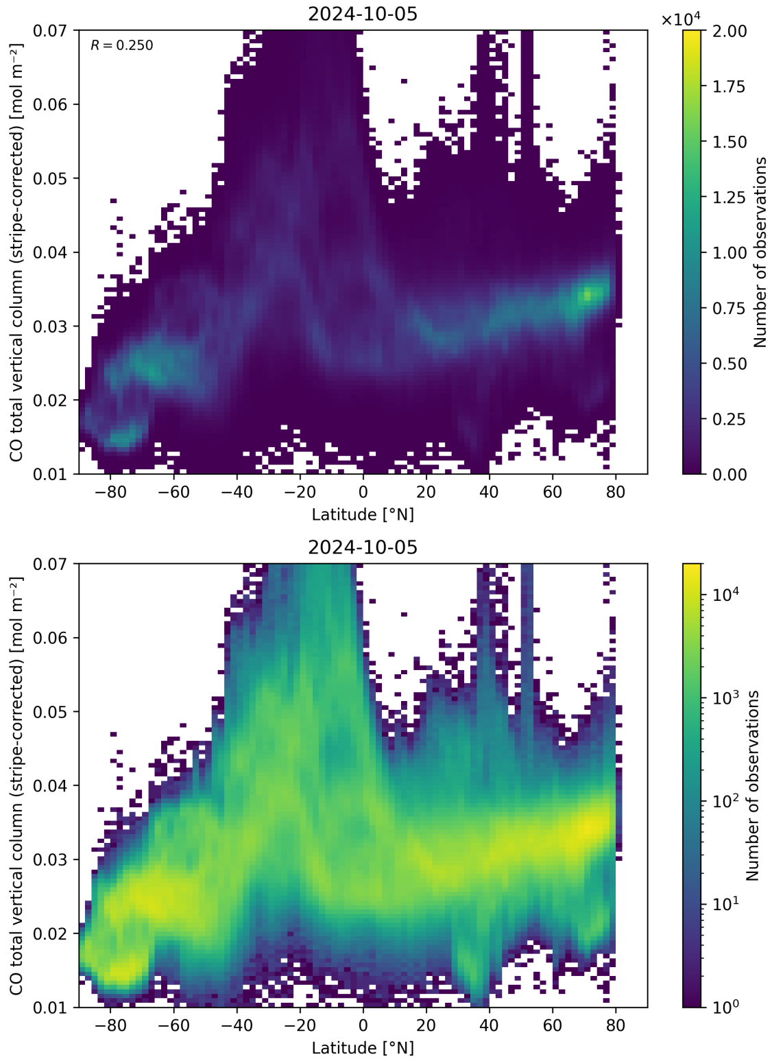
Figure 52: Scatter density plot of “Latitude” against “CO total vertical column (stripe-corrected)” for 2024-10-04 to 2024-10-06.
