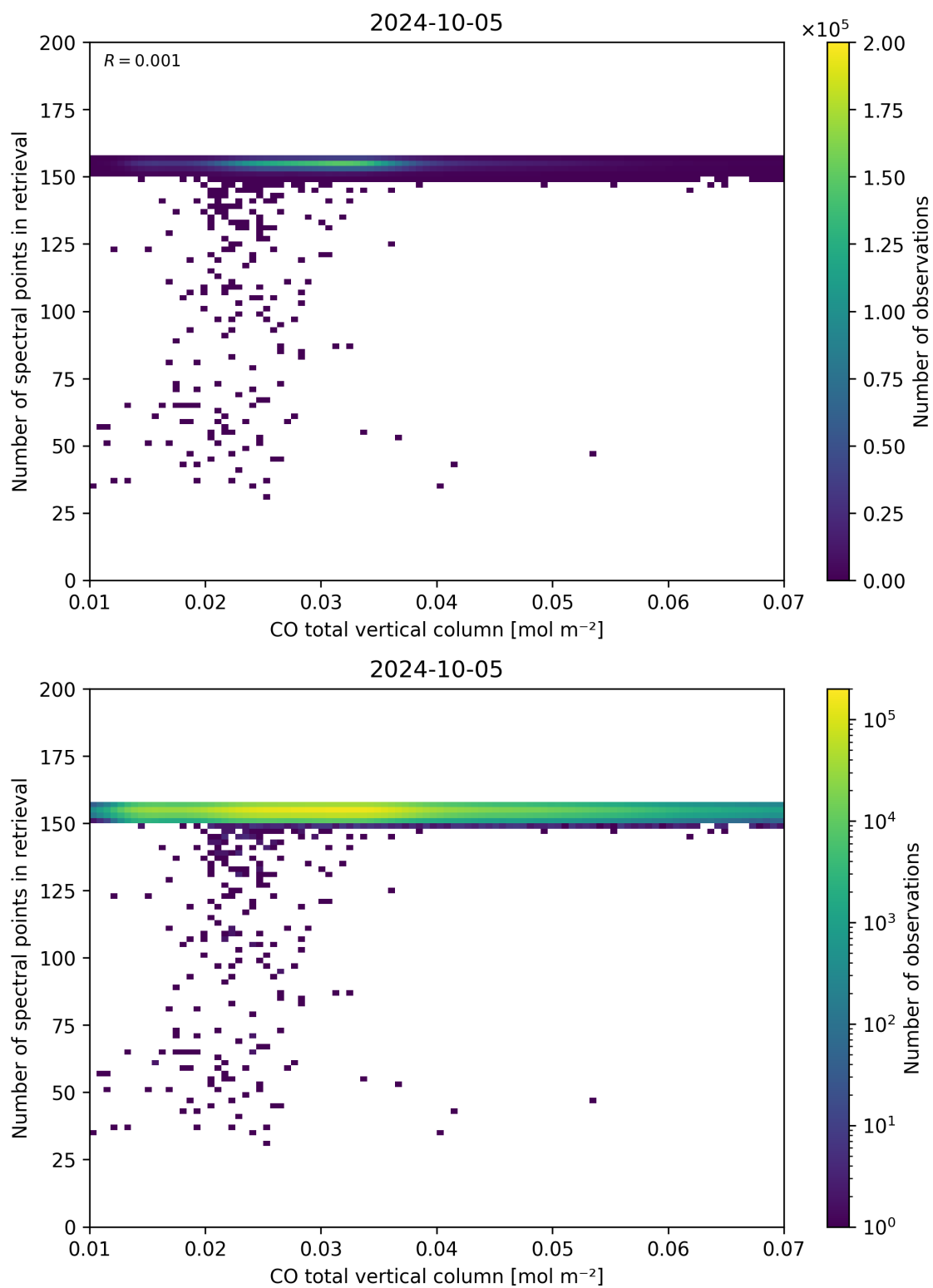
Figure 43: Scatter density plot of “CO total vertical column” against “Number of spectral points in retrieval” for 2024-10-04 to 2024-10-06.
