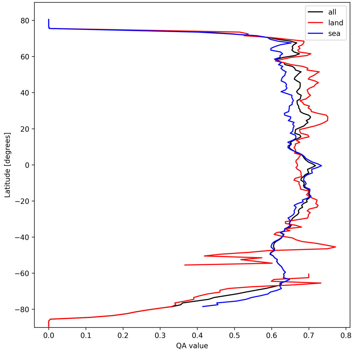
Figure 9: Zonal average of “QA value” for 2024-10-04 to 2024-10-06.
