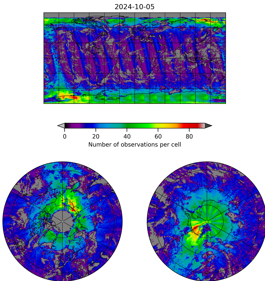
Figure 8: Map of the number of observations for 2024-10-04 to 2024-10-06
