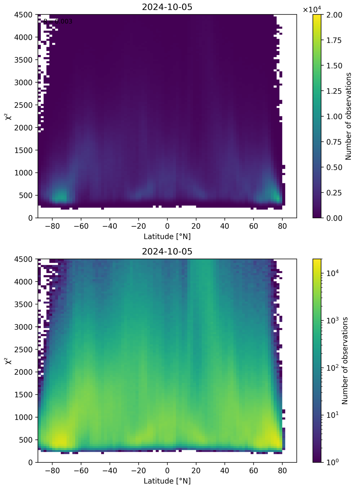
Figure 54: Scatter density plot of “Latitude” against “ \chi^2 ” for 2024-10-04 to 2024-10-06.
