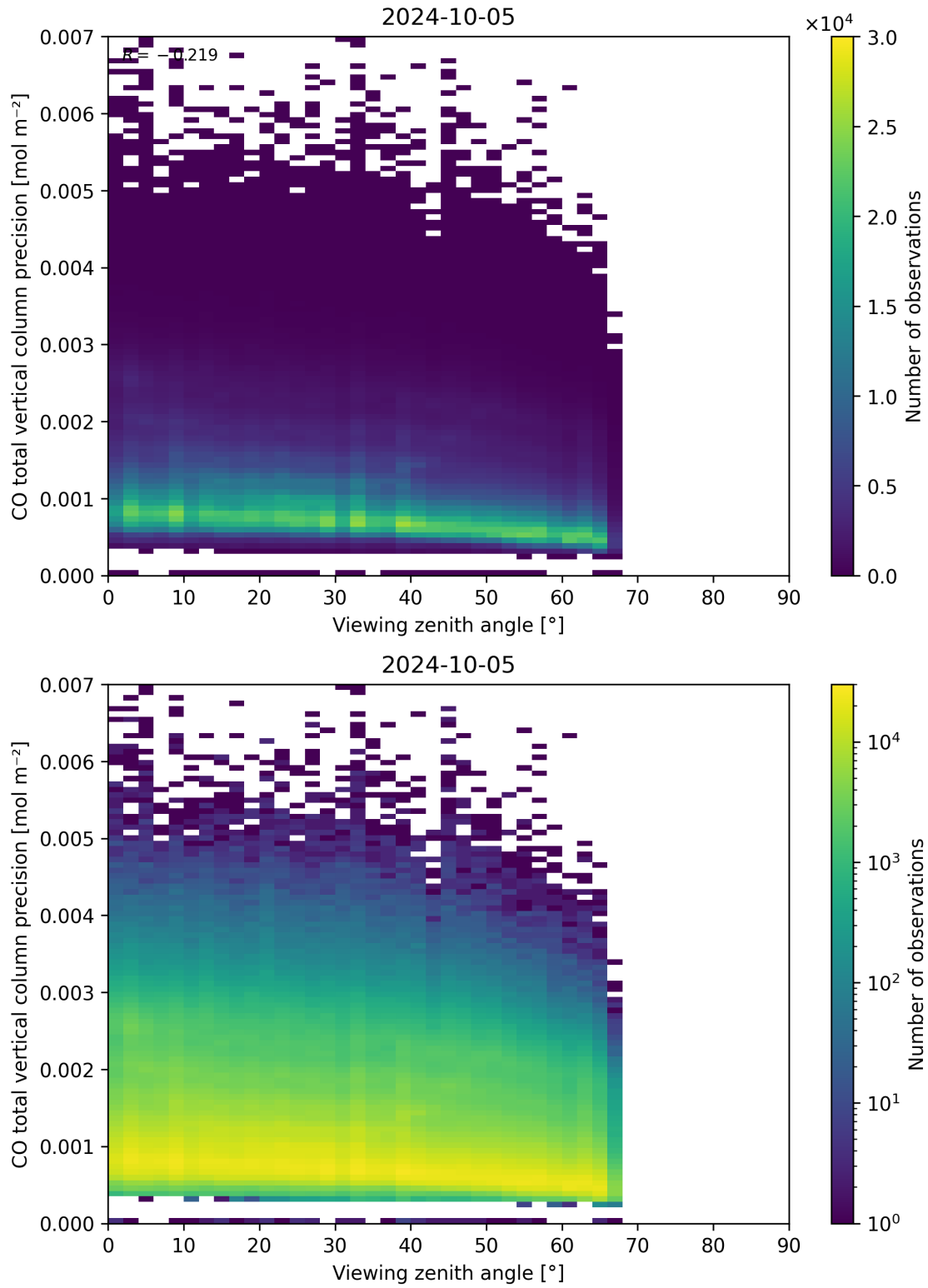
Figure 71: Scatter density plot of “Viewing zenith angle” against “CO total vertical column precision” for 2024-10-04 to 2024-10-06.
