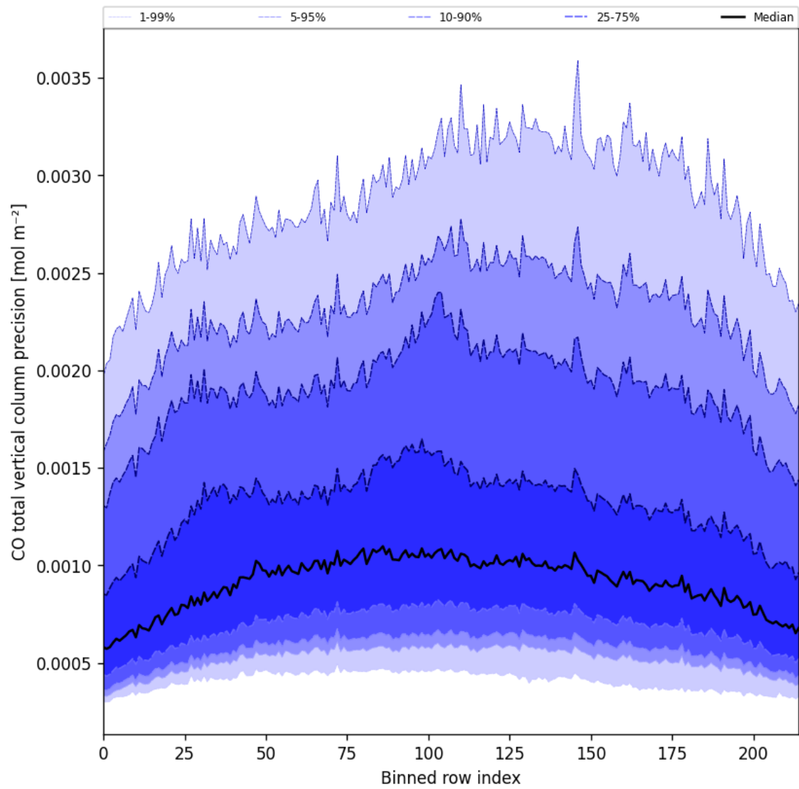
Figure 28: Along track statistics of “CO total vertical column precision” for 2024-10-04 to 2024-10-06
