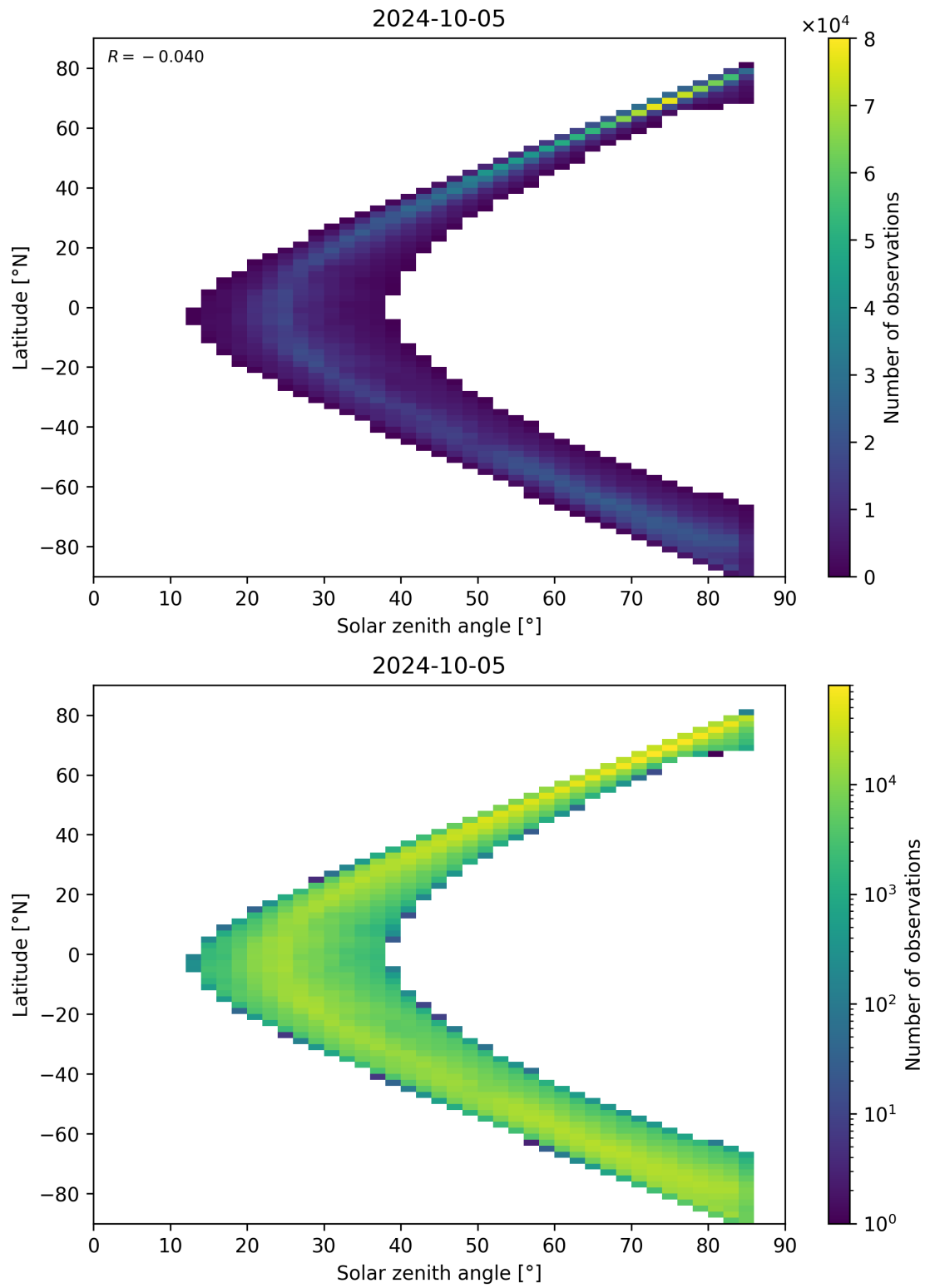
Figure 66: Scatter density plot of “Solar zenith angle” against “Latitude” for 2024-10-04 to 2024-10-06.
