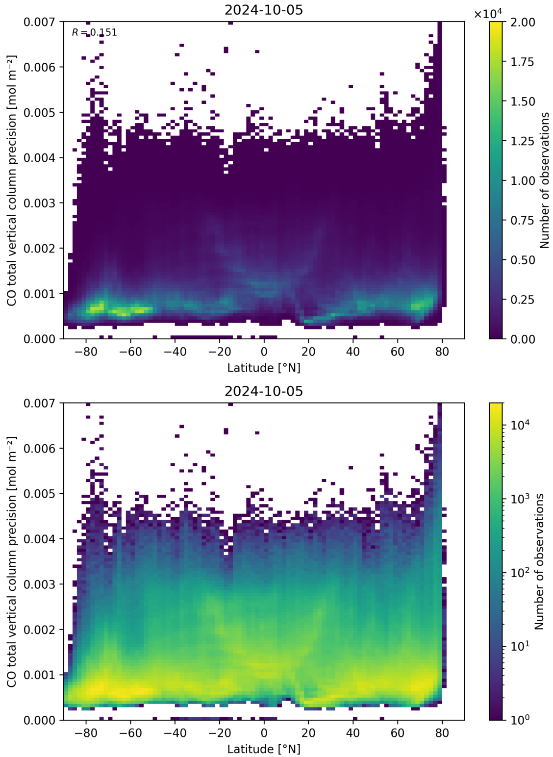
Figure 53: Scatter density plot of “Latitude” against “CO total vertical column precision” for 2024-10-04 to 2024-10-06.
