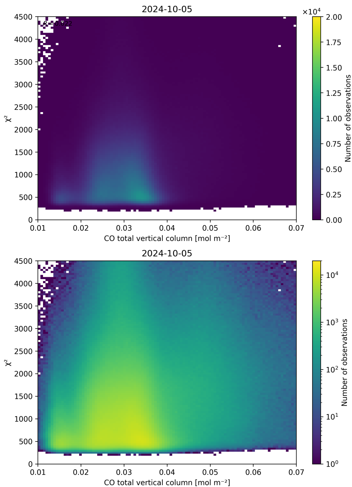
Figure 35: Scatter density plot of “CO total vertical column” against “ \chi^2 ” for 2024-10-04 to 2024-10-06.
