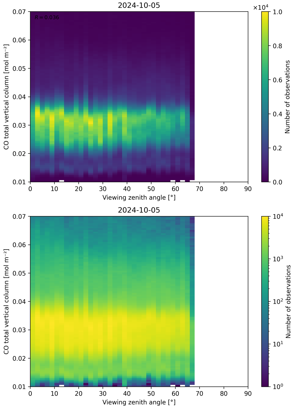
Figure 69: Scatter density plot of “Viewing zenith angle” against “CO total vertical column” for 2024-10-04 to 2024-10-06.
