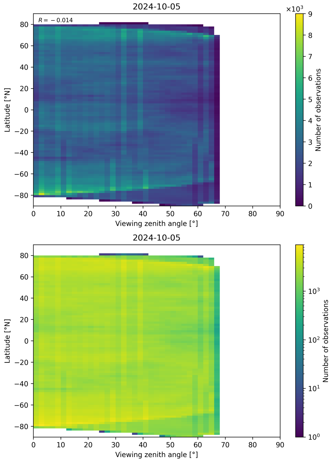
Figure 74: Scatter density plot of “Viewing zenith angle” against “Latitude” for 2024-10-04 to 2024-10-06.
