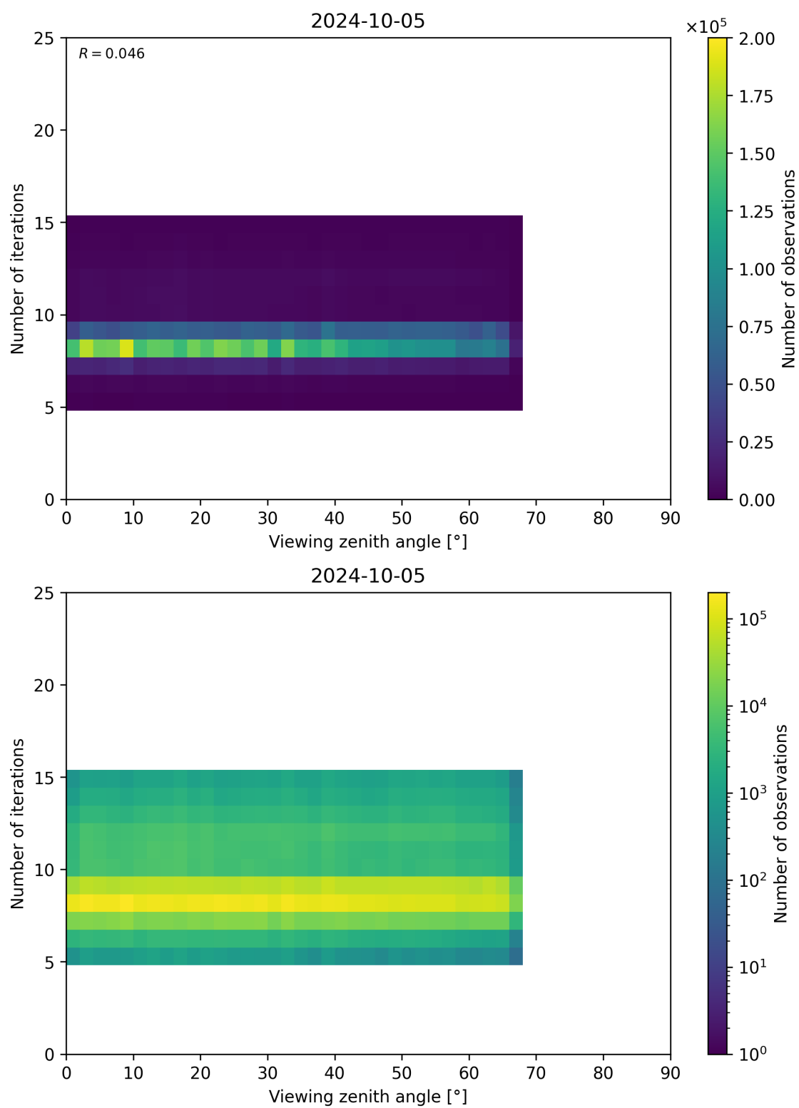
Figure 75: Scatter density plot of “Viewing zenith angle” against “Number of iterations” for 2024-10-04 to 2024-10-06.
