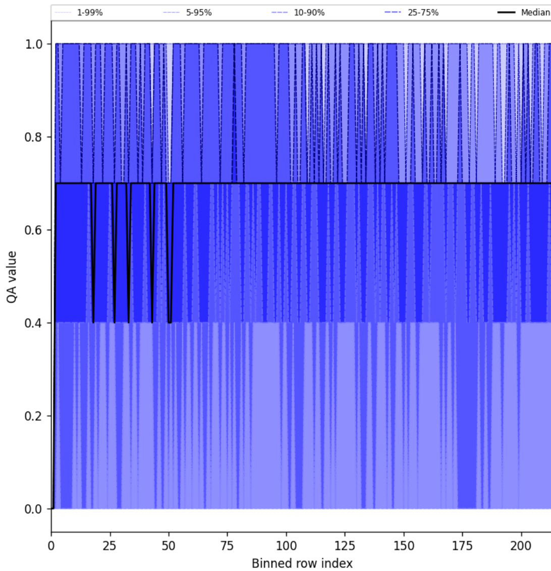
Figure 25: Along track statistics of “QA value” for 2024-10-04 to 2024-10-06
