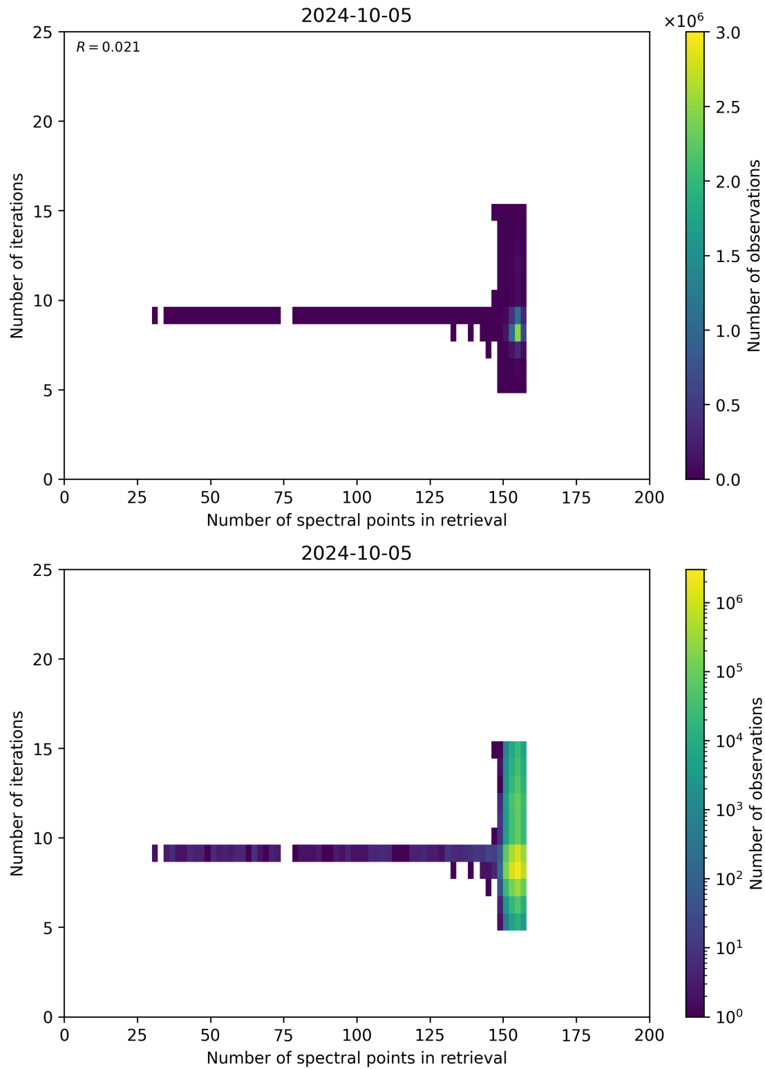
Figure 60: Scatter density plot of “Number of spectral points in retrieval” against “Number of iterations” for 2024-10-04 to 2024-10-06.
