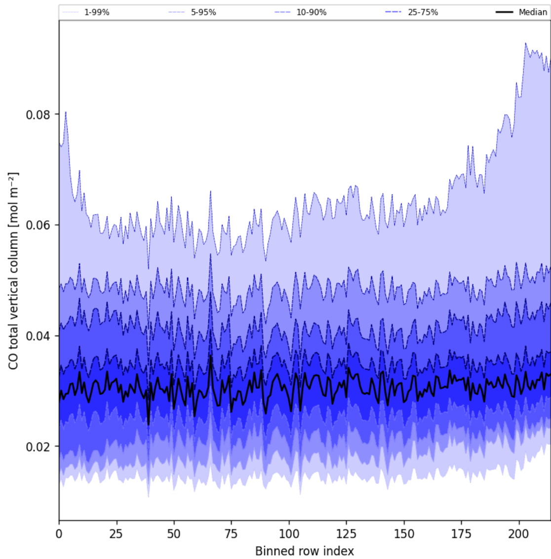
Figure 26: Along track statistics of “CO total vertical column” for 2024-10-04 to 2024-10-06
