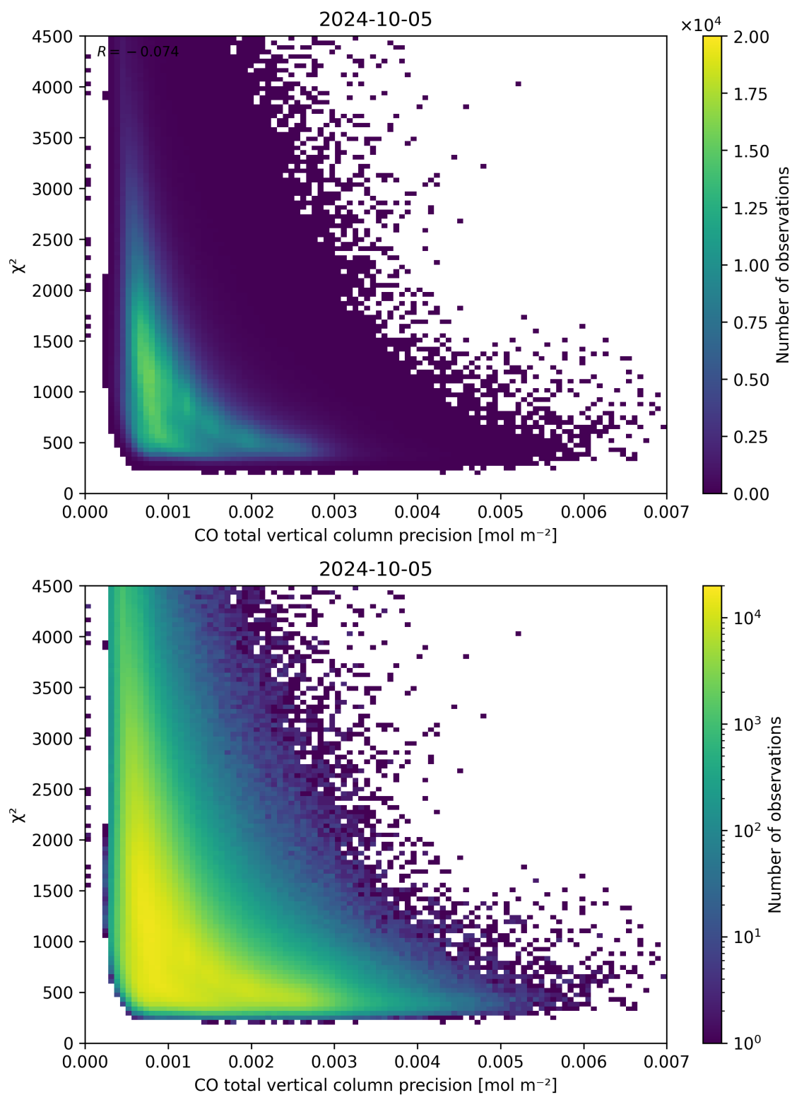
Figure 44: Scatter density plot of “CO total vertical column precision” against “ \chi^2 ” for 2024-10-04 to 2024-10-06.
