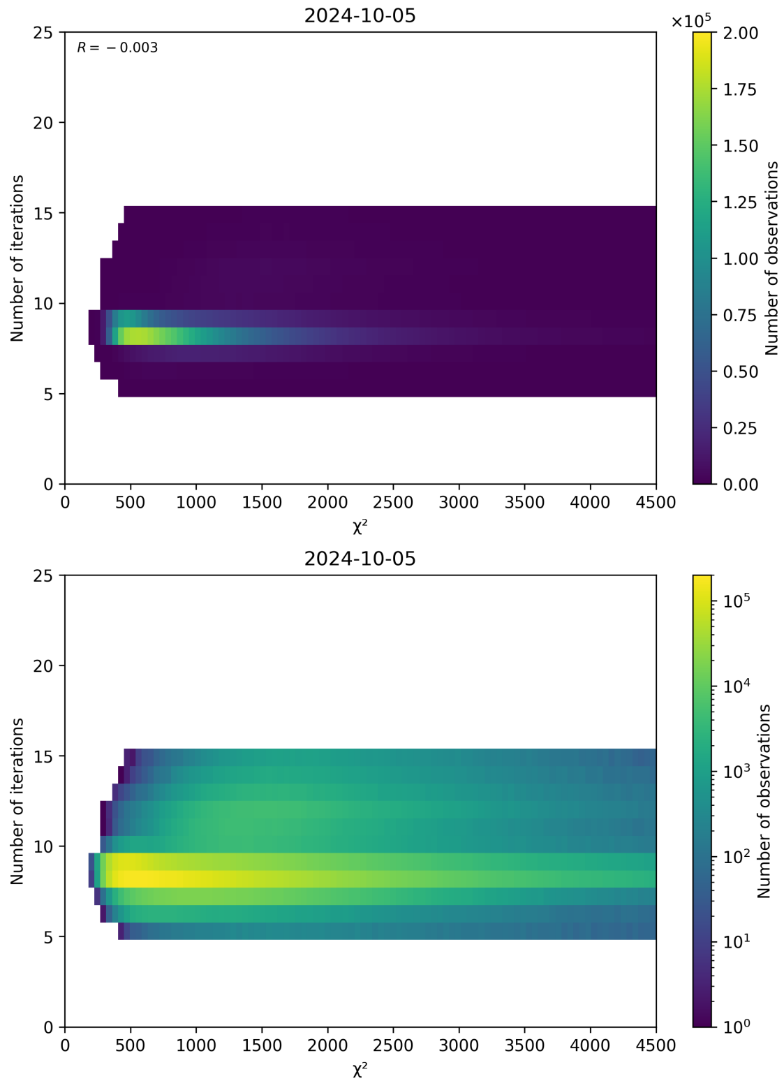
Figure 49: Scatter density plot of “ \chi^2 ” against “Number of iterations” for 2024-10-04 to 2024-10-06.
