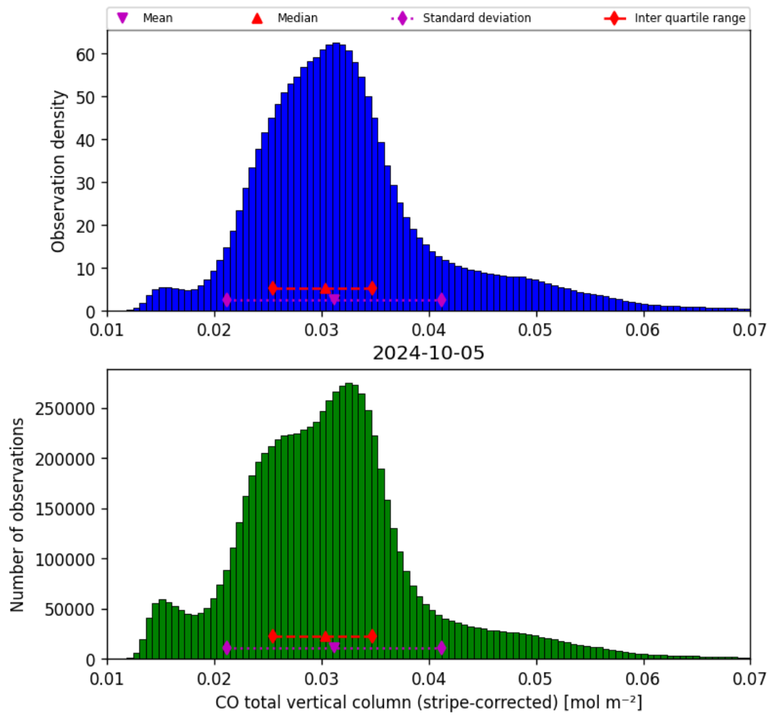
Figure 19: Histogram of “CO total vertical column (stripe-corrected)” for 2024-10-04 to 2024-10-06
