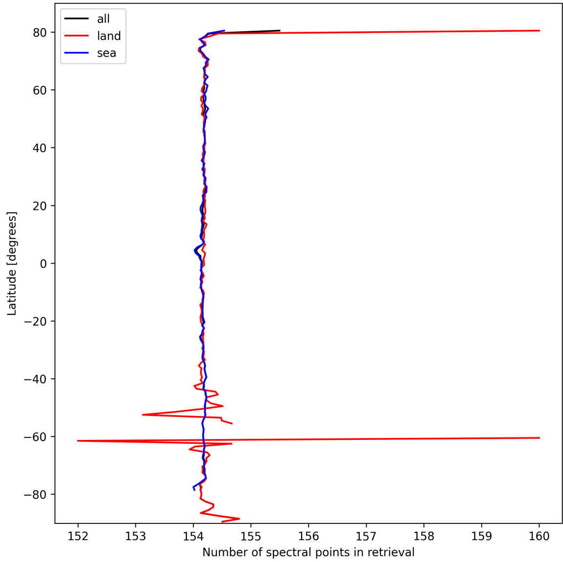
Figure 13: Zonal average of “Number of spectral points in retrieval” for 2024-10-04 to 2024-10-06.
