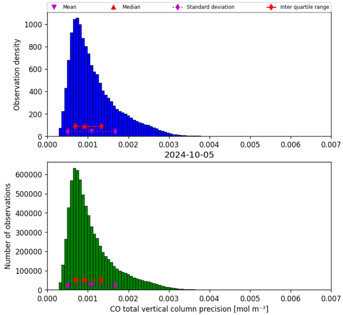
Figure 20: Histogram of “CO total vertical column precision” for 2024-10-04 to 2024-10-06
