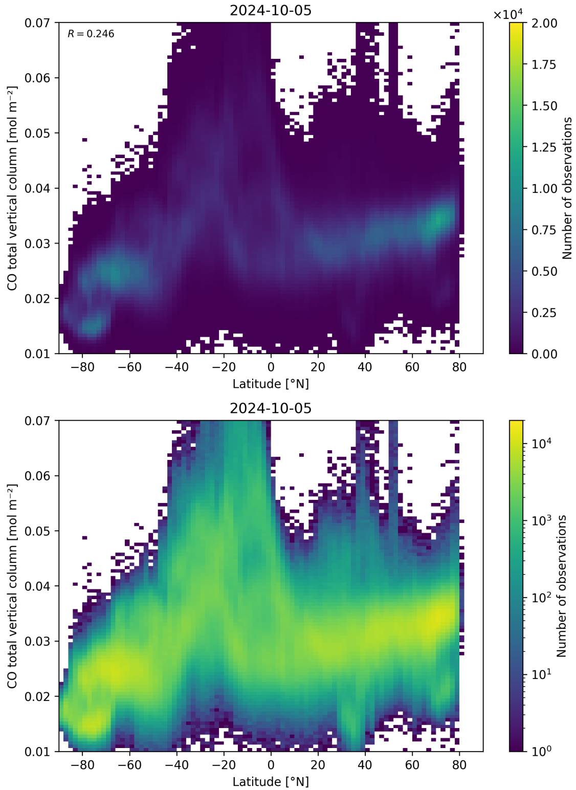
Figure 51: Scatter density plot of “Latitude” against “CO total vertical column” for 2024-10-04 to 2024-10-06.
