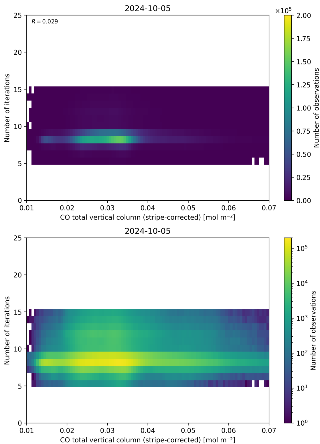
Figure 39: Scatter density plot of “CO total vertical column (stripe-corrected)” against “Number of iterations” for 2024-10-04 to 2024-10-06.
