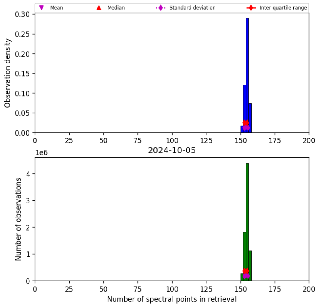
Figure 21: Histogram of “Number of spectral points in retrieval” for 2024-10-04 to 2024-10-06
