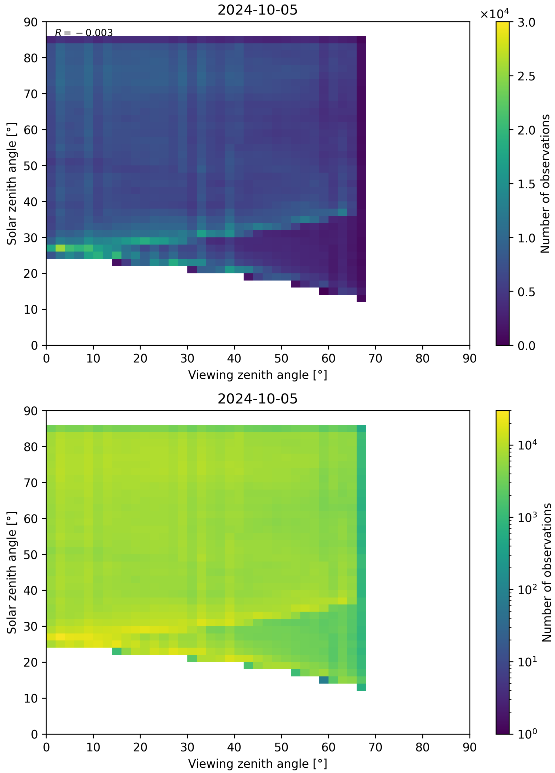
Figure 77: Scatter density plot of “Viewing zenith angle” against “Solar zenith angle” for 2024-10-04 to 2024-10-06.
