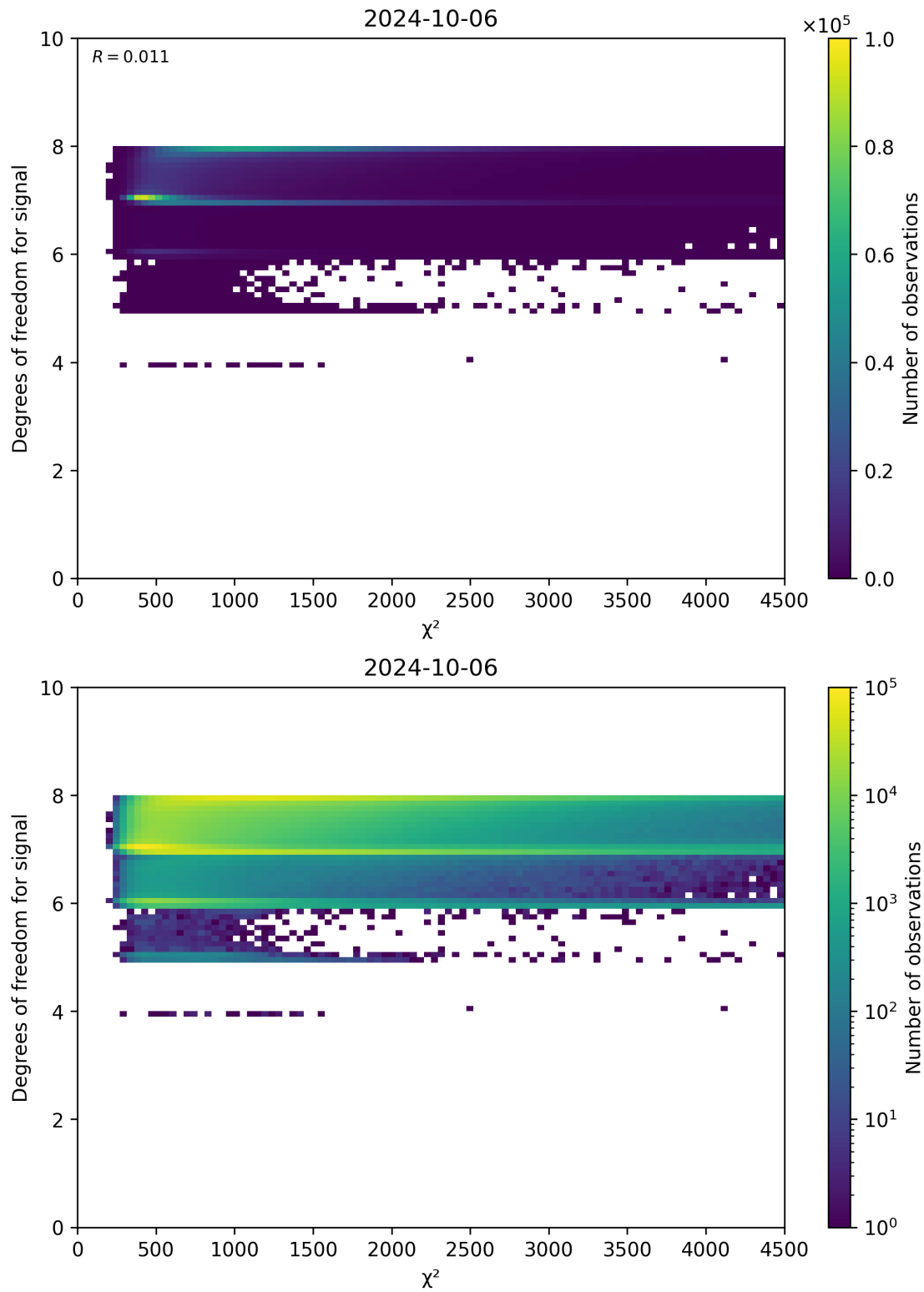
Figure 48: Scatter density plot of “ \chi^2 ” against “Degrees of freedom for signal” for 2024-10-05 to 2024-10-07.
