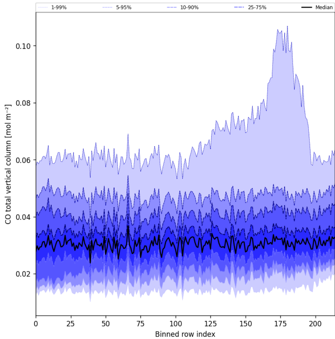
Figure 26: Along track statistics of “CO total vertical column” for 2024-10-05 to 2024-10-07
