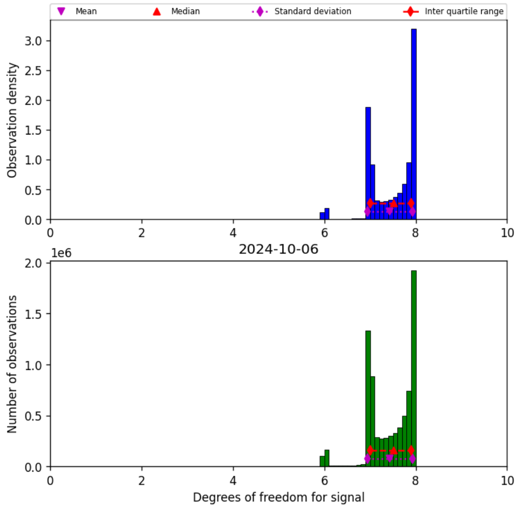
Figure 23: Histogram of “Degrees of freedom for signal” for 2024-10-05 to 2024-10-07
