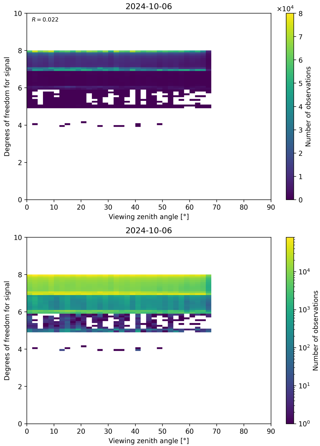
Figure 73: Scatter density plot of “Viewing zenith angle” against “Degrees of freedom for signal” for 2024-10-05 to 2024-10-07.
