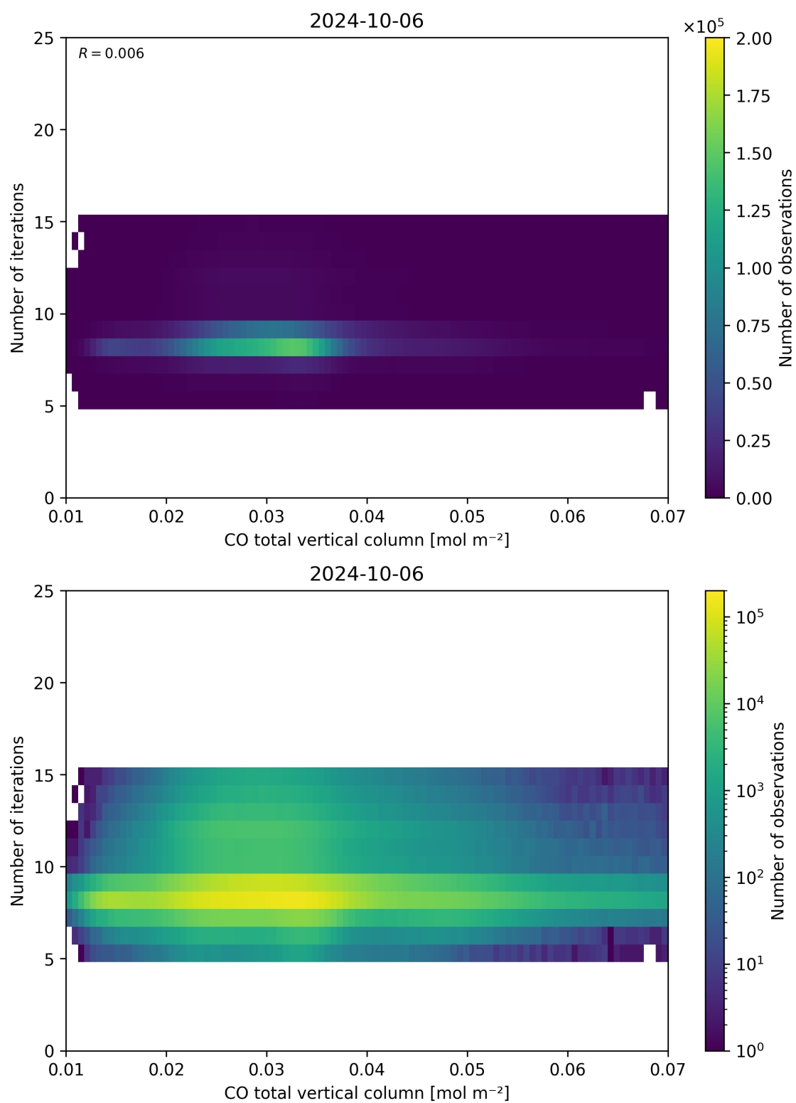
Figure 42: Scatter density plot of “CO total vertical column” against “Number of iterations” for 2024-10-05 to 2024-10-07.
