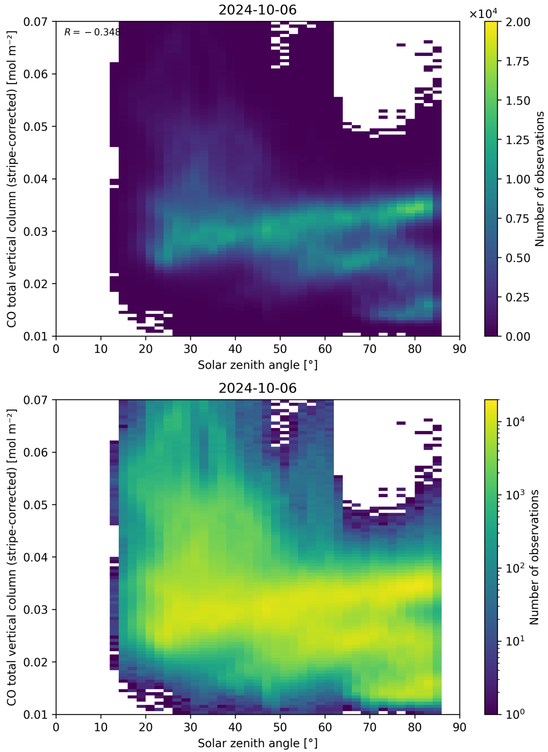
Figure 62: Scatter density plot of “Solar zenith angle” against “CO total vertical column (stripe-corrected)” for 2024-10-05 to 2024-10-07.
