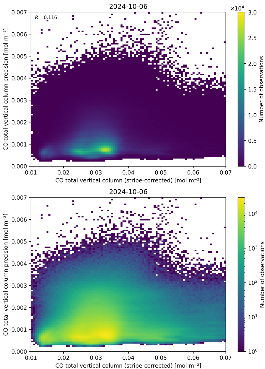
Figure 36: Scatter density plot of “CO total vertical column (stripe-corrected)” against “CO total vertical column precision” for 2024-10-05 to 2024-10-07.
