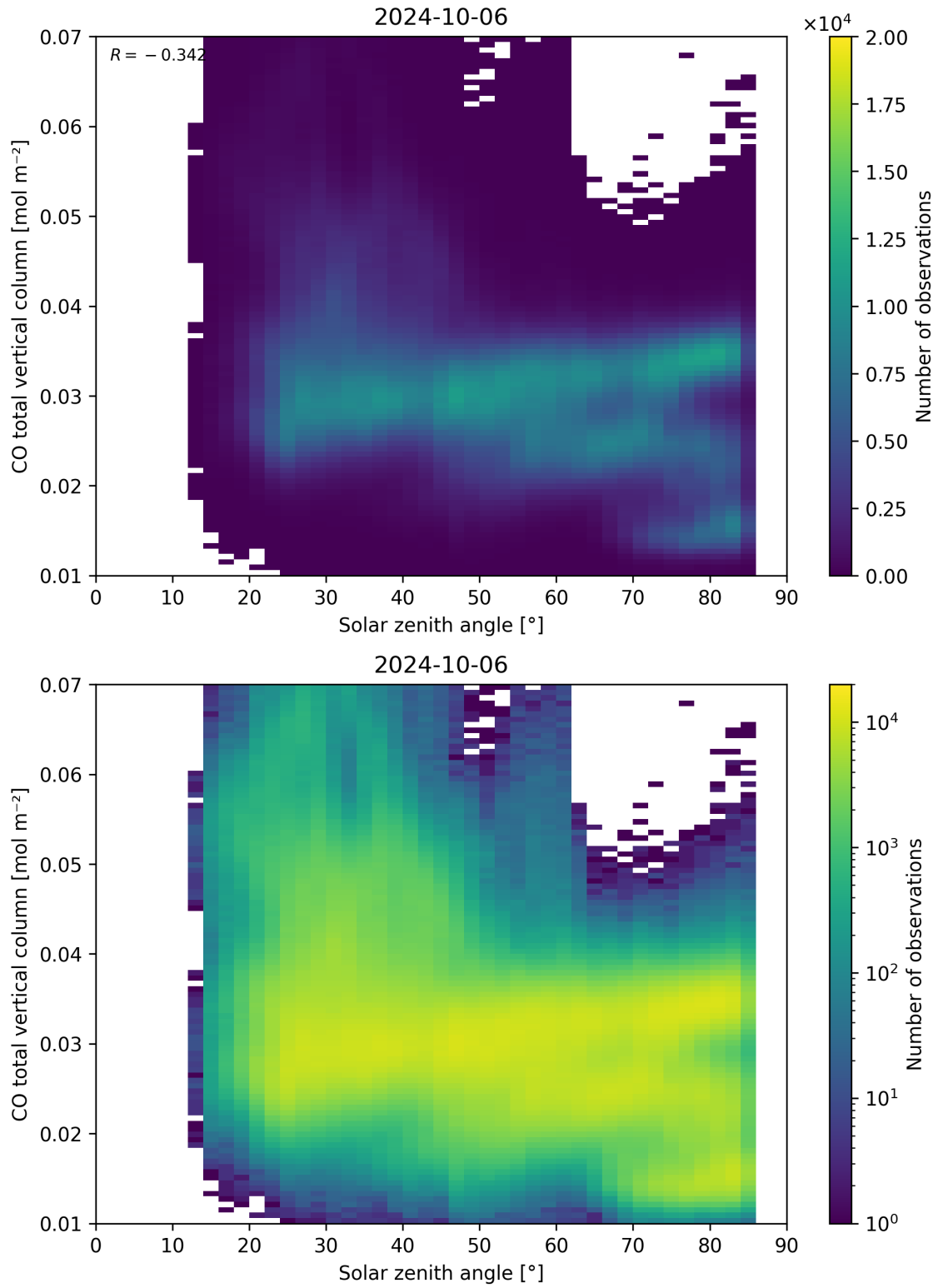
Figure 61: Scatter density plot of “Solar zenith angle” against “CO total vertical column” for 2024-10-05 to 2024-10-07.
