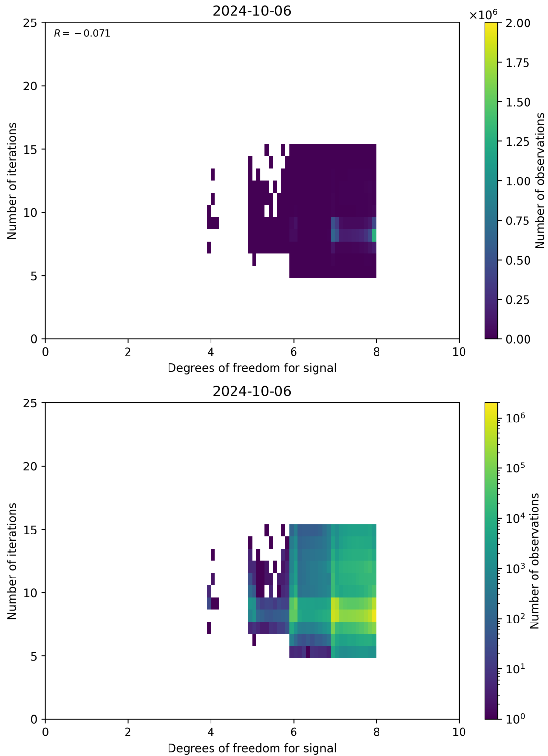
Figure 50: Scatter density plot of “Degrees of freedom for signal” against “Number of iterations” for 2024-10-05 to 2024-10-07.
