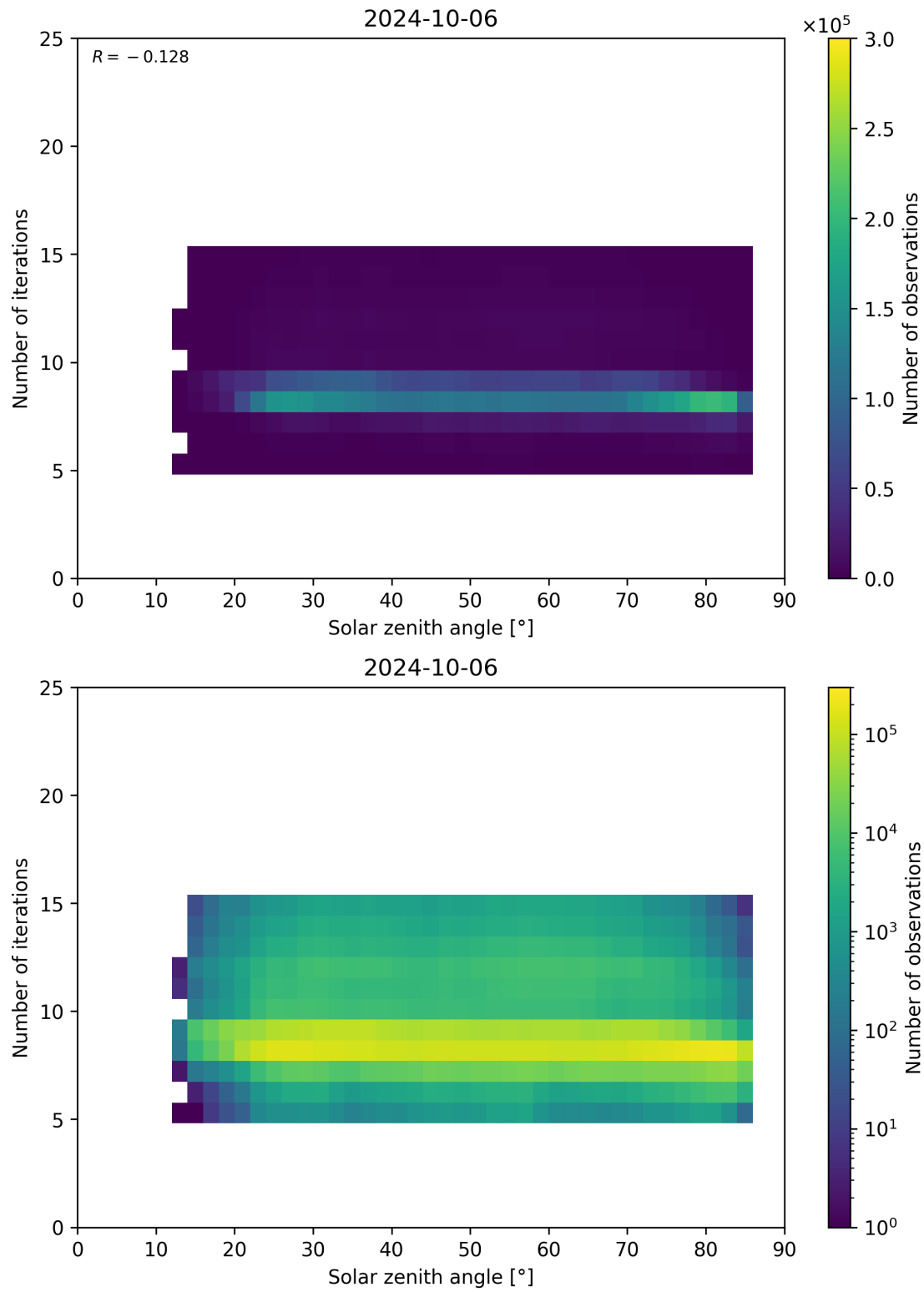
Figure 67: Scatter density plot of “Solar zenith angle” against “Number of iterations” for 2024-10-05 to 2024-10-07.
