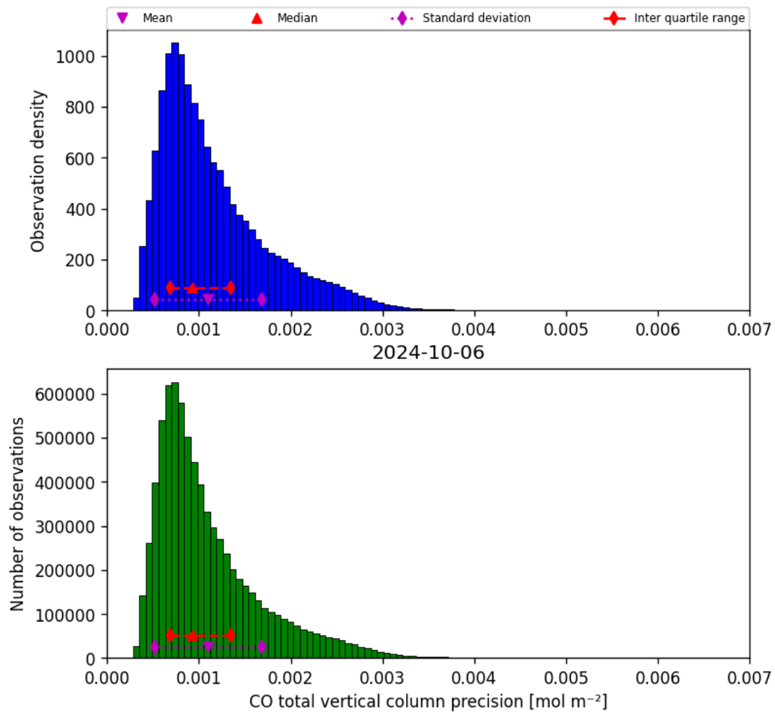
Figure 20: Histogram of “CO total vertical column precision” for 2024-10-05 to 2024-10-07
