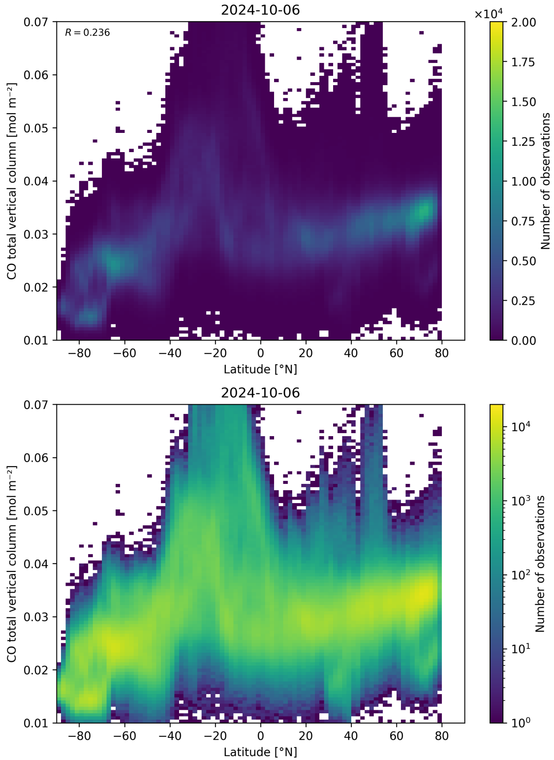
Figure 51: Scatter density plot of “Latitude” against “CO total vertical column” for 2024-10-05 to 2024-10-07.
