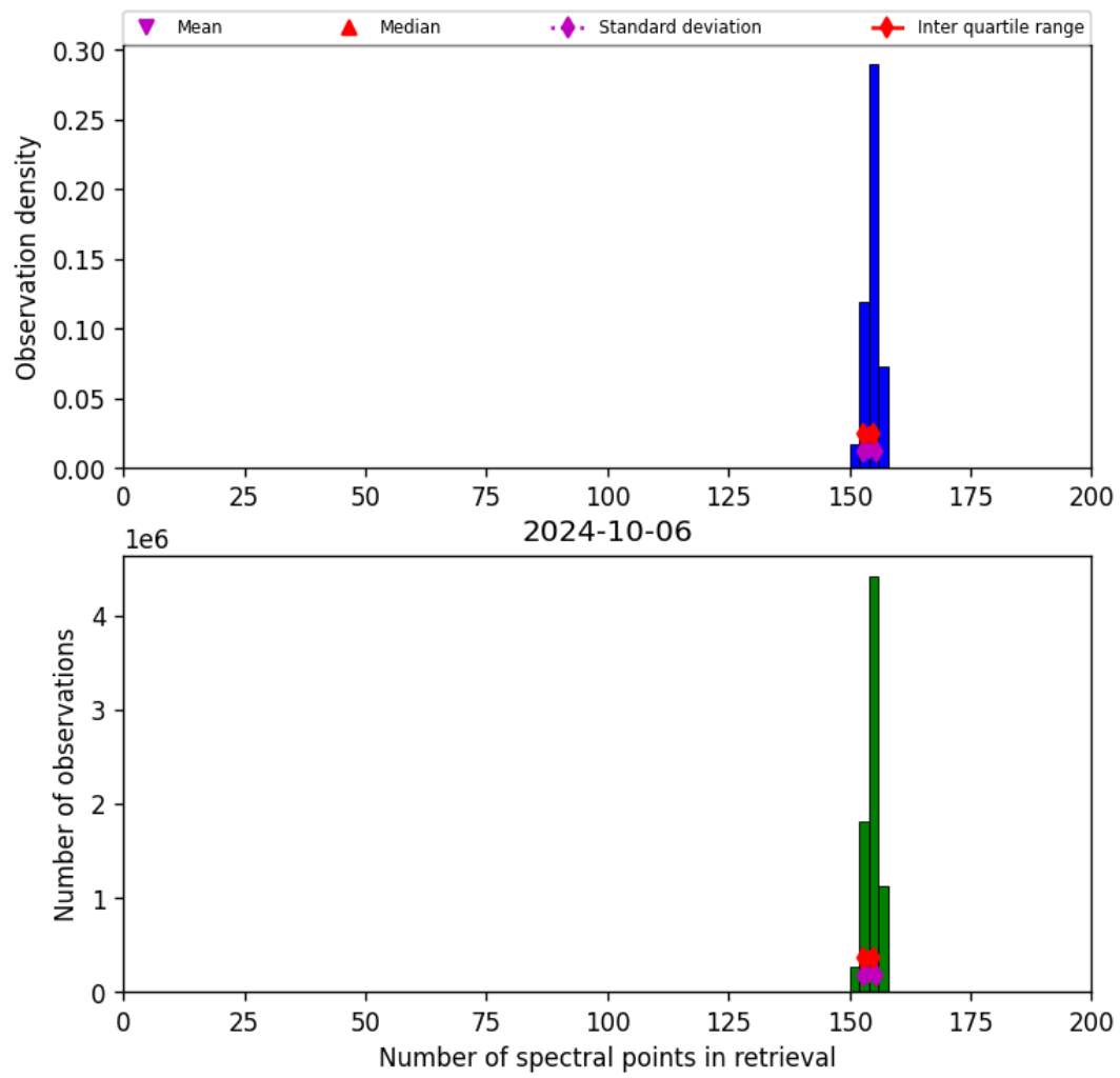
Figure 21: Histogram of “Number of spectral points in retrieval” for 2024-10-05 to 2024-10-07
