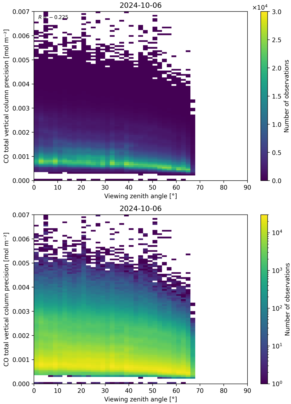
Figure 71: Scatter density plot of “Viewing zenith angle” against “CO total vertical column precision” for 2024-10-05 to 2024-10-07.
