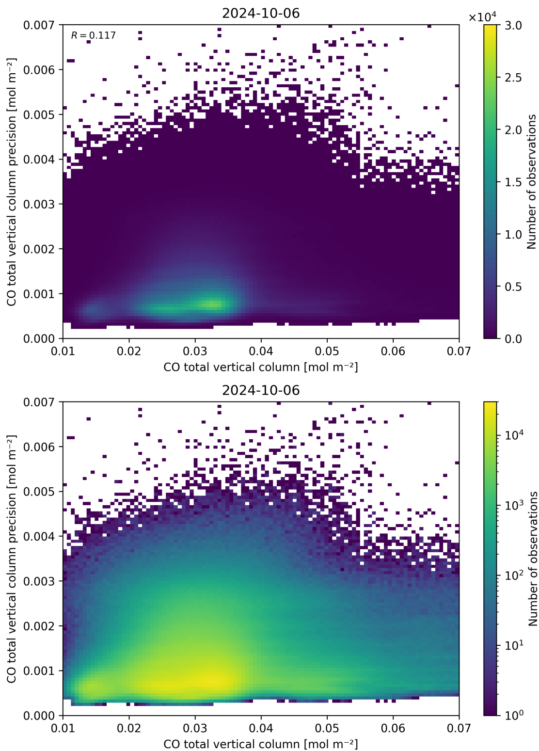
Figure 34: Scatter density plot of “CO total vertical column” against “CO total vertical column precision” for 2024-10-05 to 2024-10-07.
