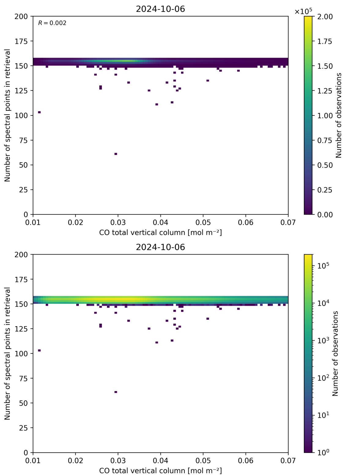
Figure 43: Scatter density plot of “CO total vertical column” against “Number of spectral points in retrieval” for 2024-10-05 to 2024-10-07.
