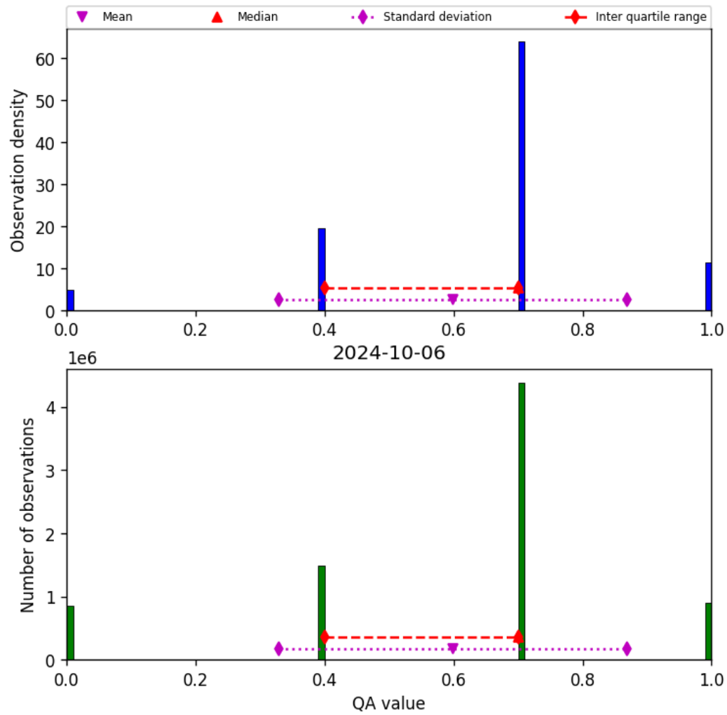
Figure 17: Histogram of “QA value” for 2024-10-05 to 2024-10-07
