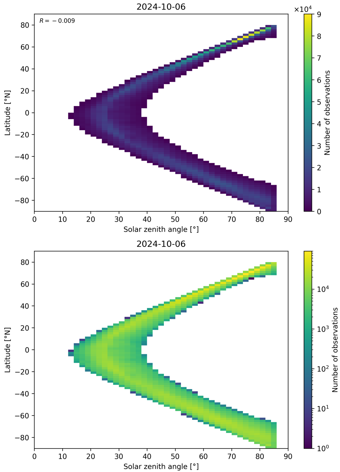
Figure 66: Scatter density plot of “Solar zenith angle” against “Latitude” for 2024-10-05 to 2024-10-07.
