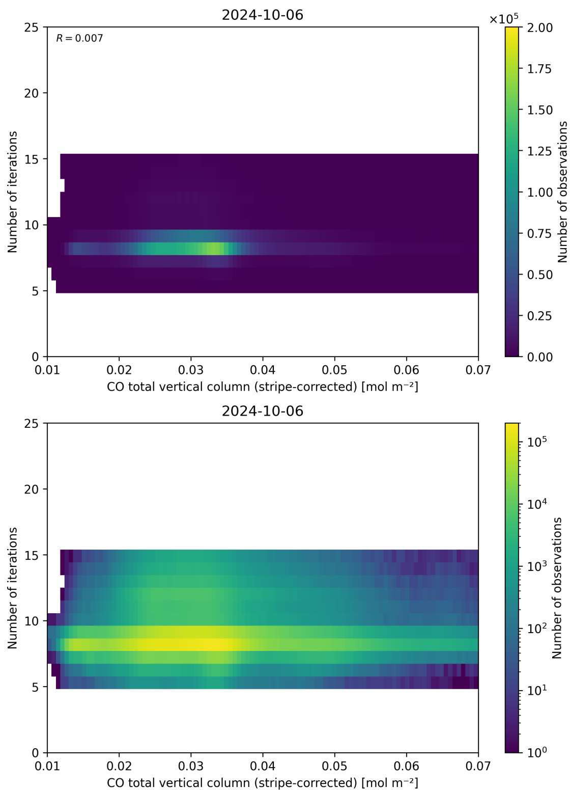
Figure 39: Scatter density plot of “CO total vertical column (stripe-corrected)” against “Number of iterations” for 2024-10-05 to 2024-10-07.
