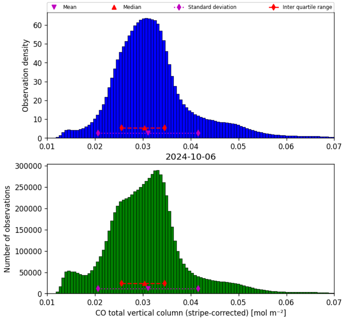
Figure 19: Histogram of “CO total vertical column (stripe-corrected)” for 2024-10-05 to 2024-10-07
