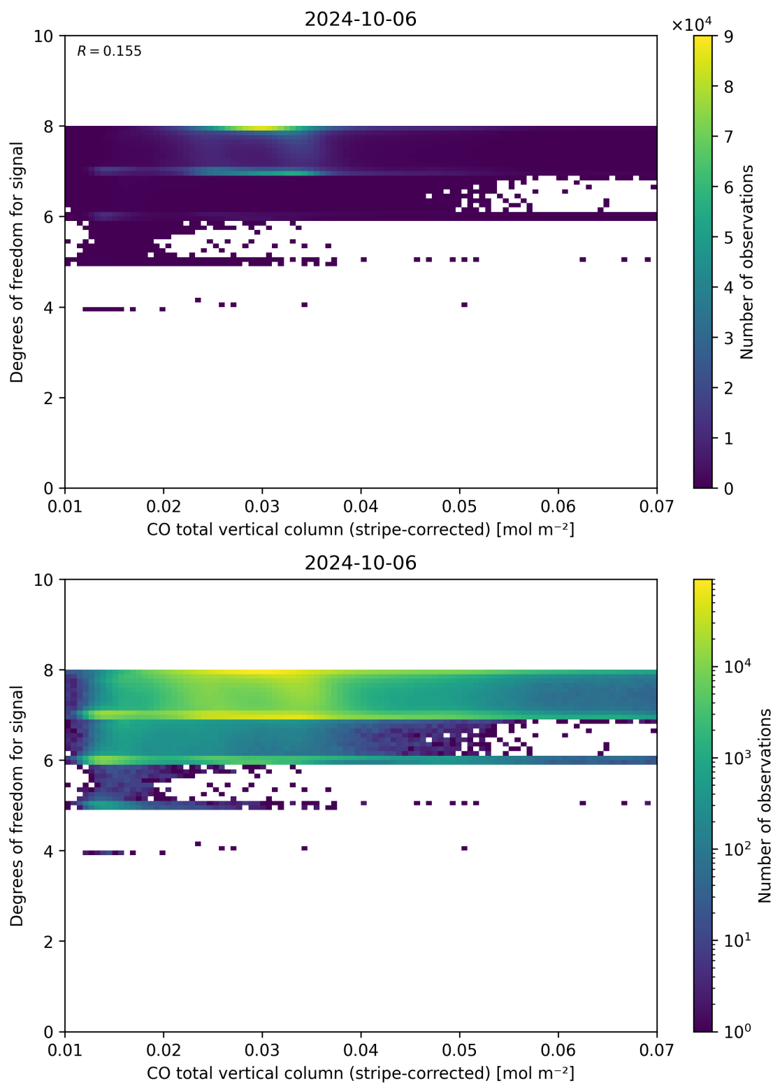
Figure 38: Scatter density plot of “CO total vertical column (stripe-corrected)” against “Degrees of freedom for signal” for 2024-10-05 to 2024-10-07.
