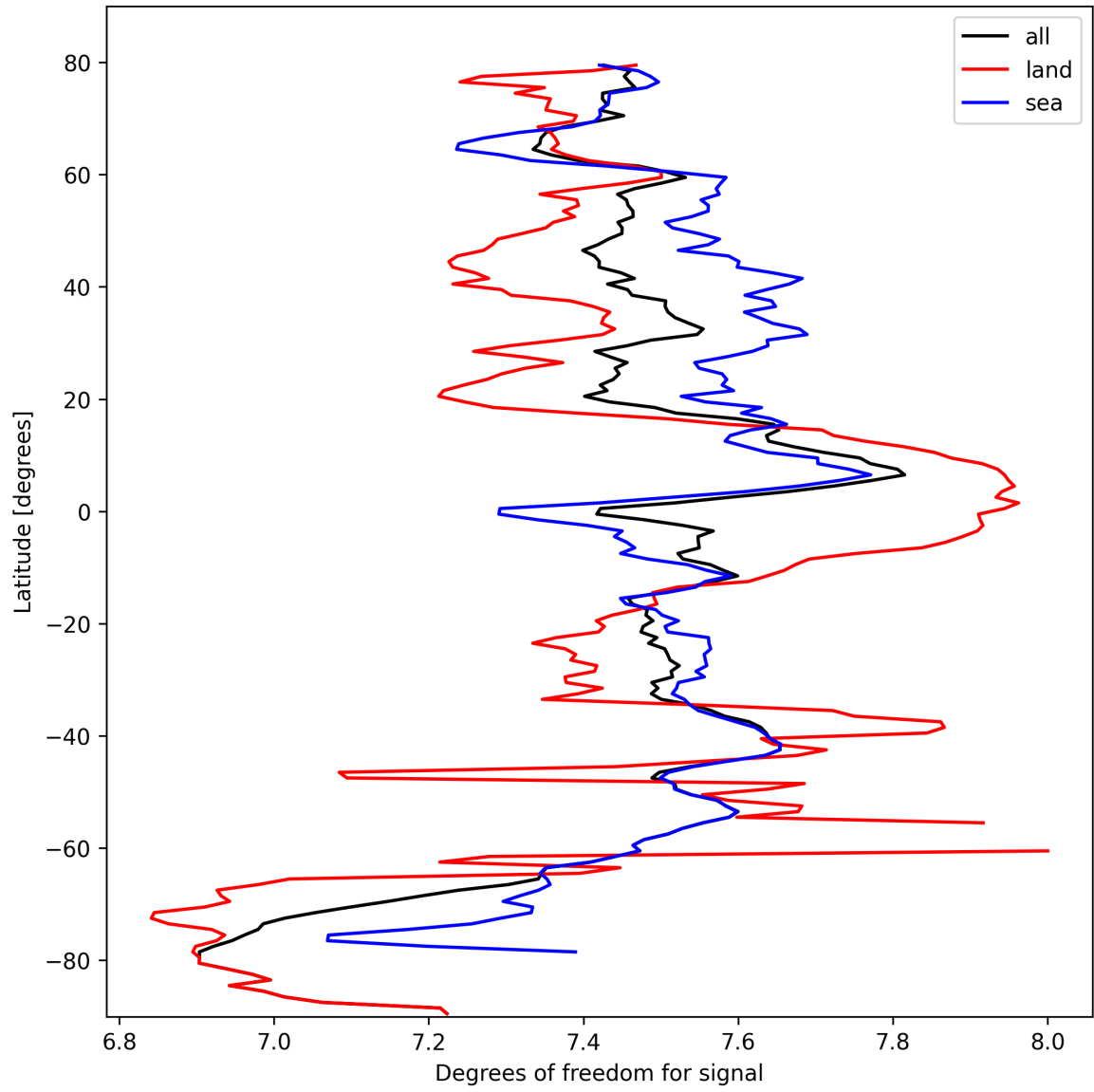
Figure 15: Zonal average of “Degrees of freedom for signal” for 2024-10-05 to 2024-10-07.
