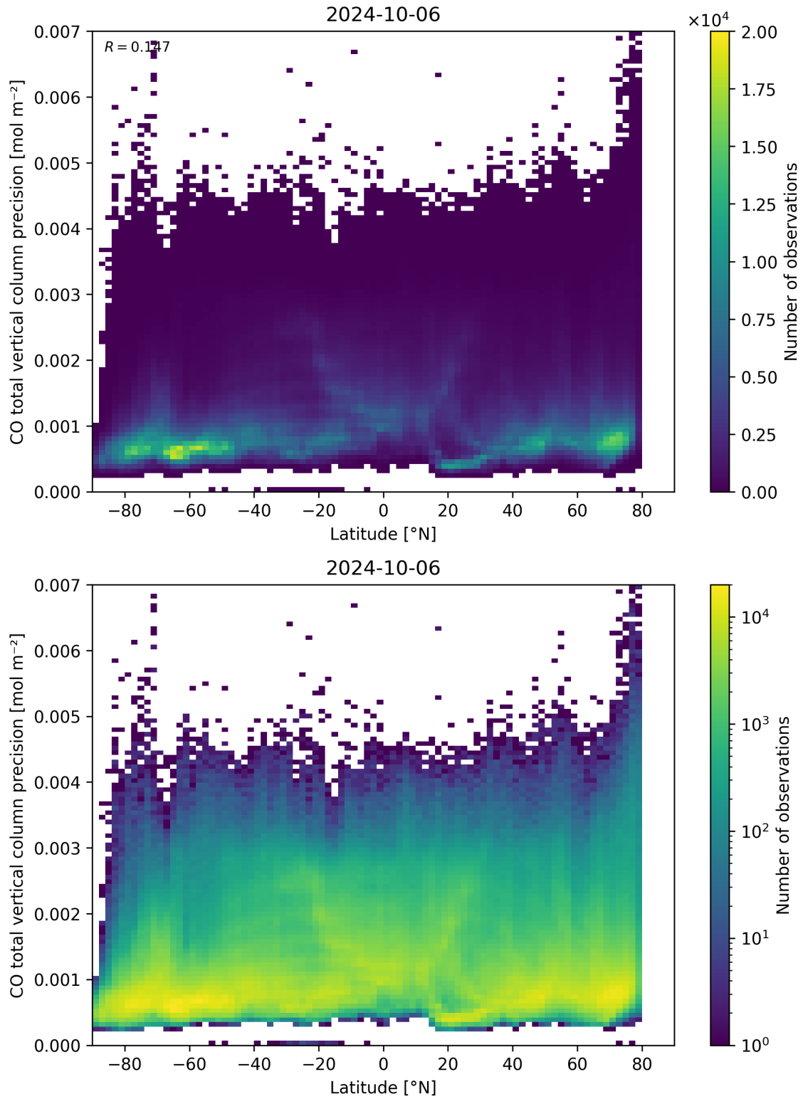
Figure 53: Scatter density plot of “Latitude” against “CO total vertical column precision” for 2024-10-05 to 2024-10-07.
