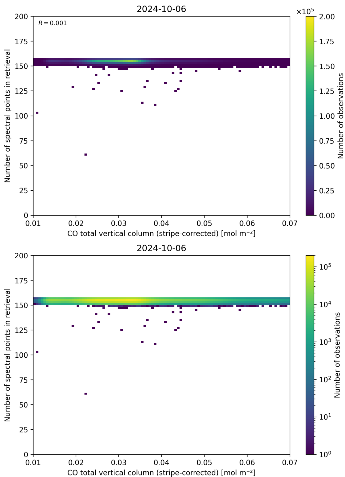
Figure 40: Scatter density plot of “CO total vertical column (stripe-corrected)” against “Number of spectral points in retrieval” for 2024-10-05 to 2024-10-07.
