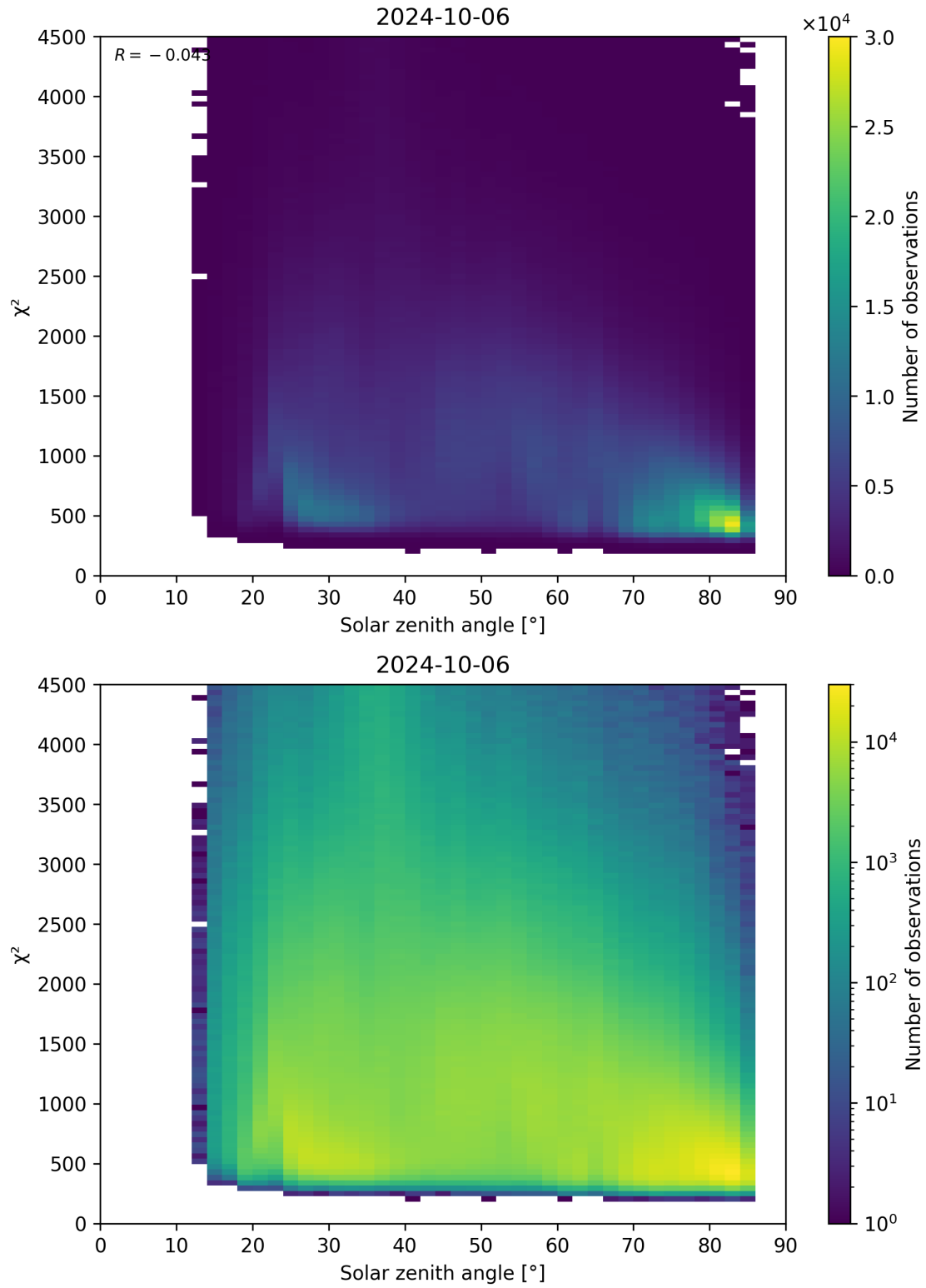
Figure 64: Scatter density plot of “Solar zenith angle” against “ \chi^2 ” for 2024-10-05 to 2024-10-07.
