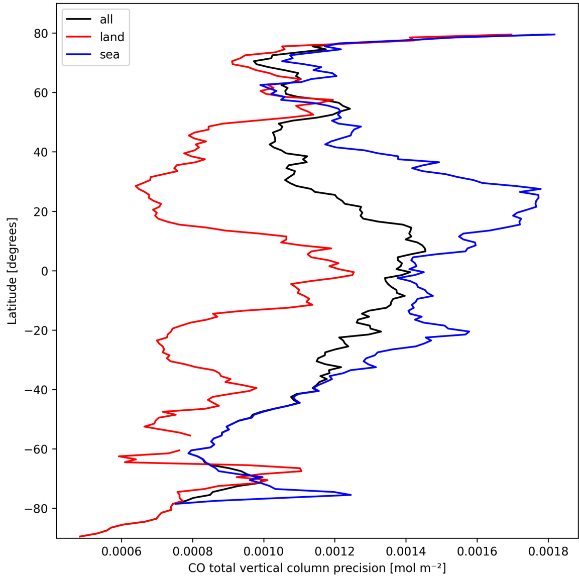
Figure 12: Zonal average of “CO total vertical column precision” for 2024-10-05 to 2024-10-07.
