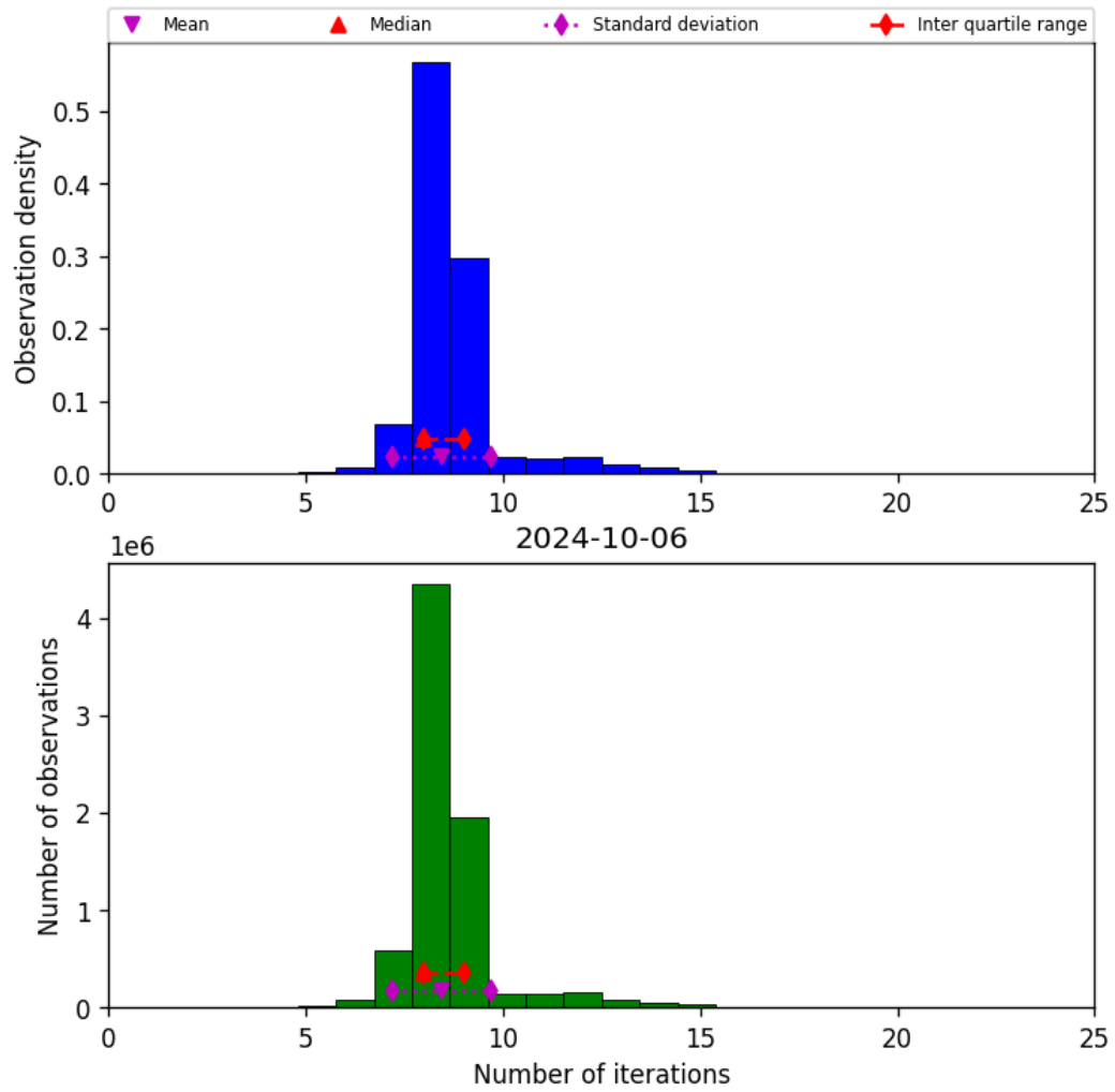
Figure 24: Histogram of “Number of iterations” for 2024-10-05 to 2024-10-07
