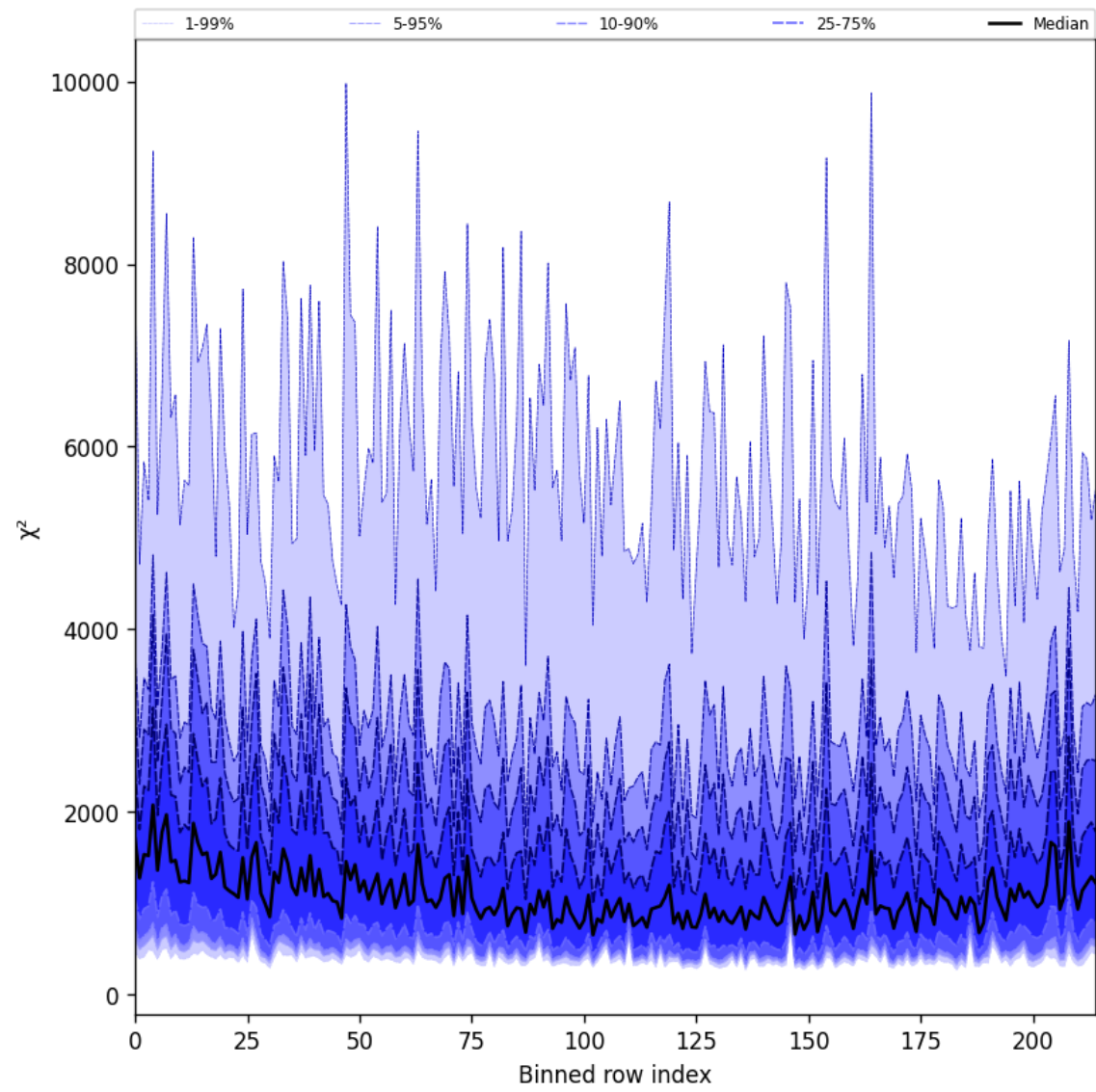
Figure 30: Along track statistics of “ \chi^2 ” for 2024-10-05 to 2024-10-07
