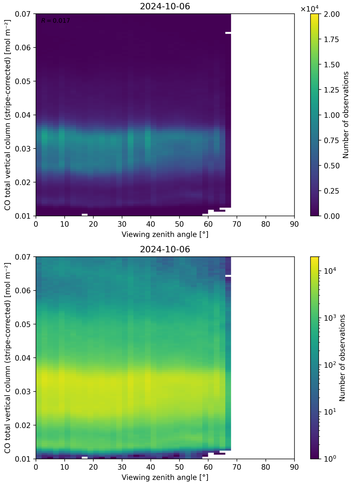
Figure 70: Scatter density plot of “Viewing zenith angle” against “CO total vertical column (stripe-corrected)” for 2024-10-05 to 2024-10-07.
