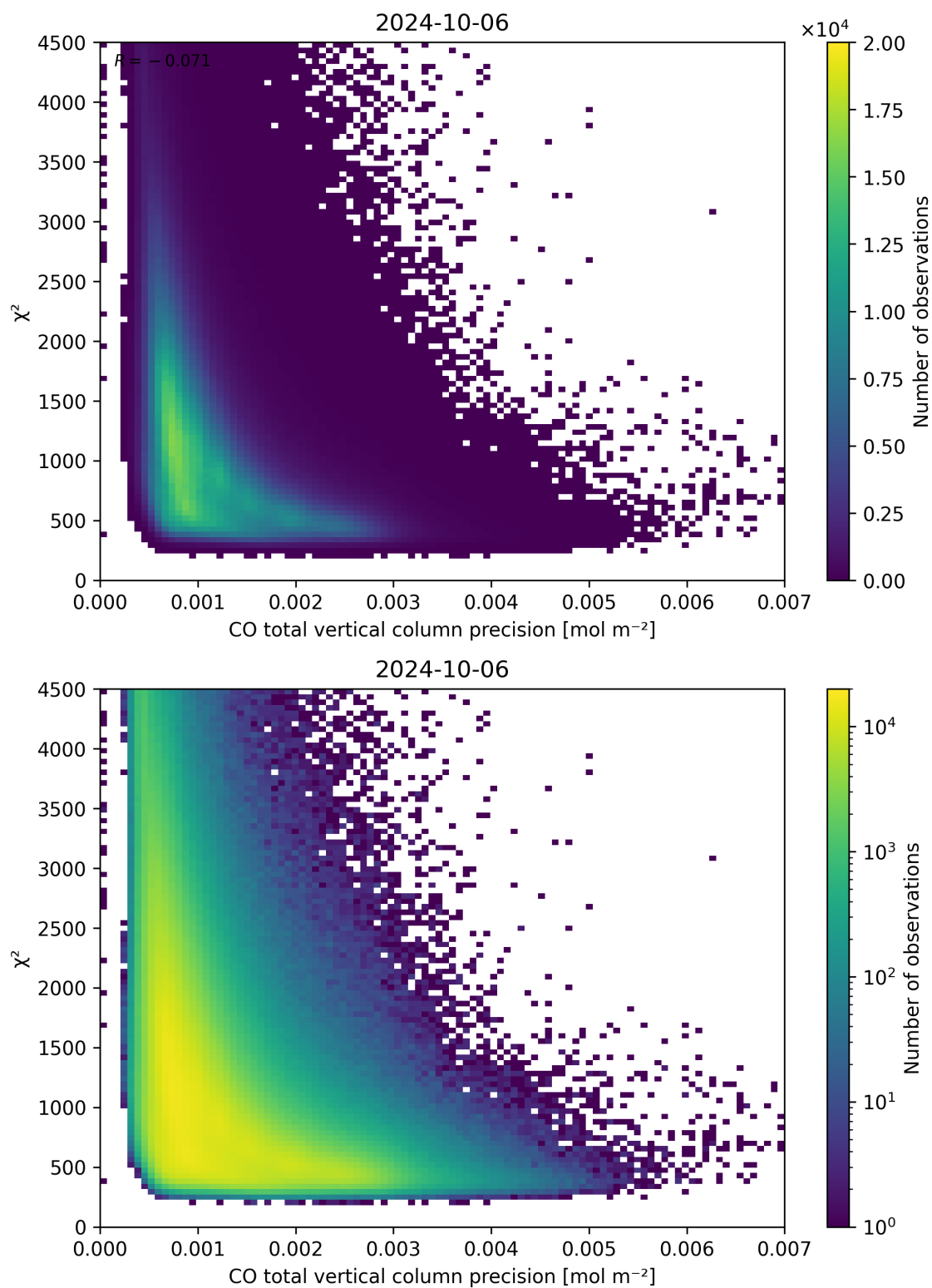
Figure 44: Scatter density plot of “CO total vertical column precision” against “ \chi^2 ” for 2024-10-05 to 2024-10-07.
