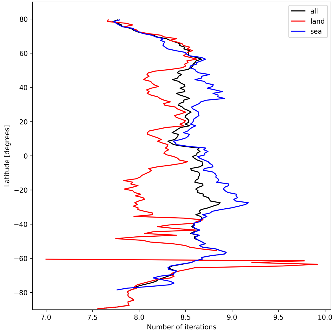
Figure 16: Zonal average of “Number of iterations” for 2024-10-05 to 2024-10-07.
