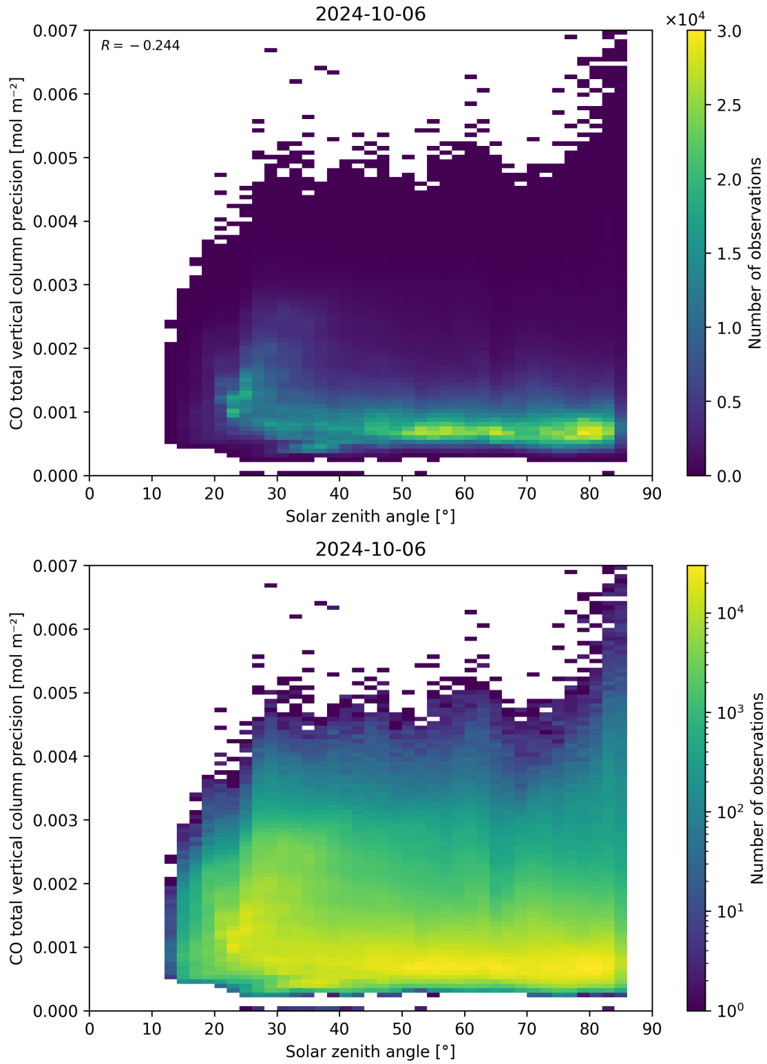
Figure 63: Scatter density plot of “Solar zenith angle” against “CO total vertical column precision” for 2024-10-05 to 2024-10-07.
