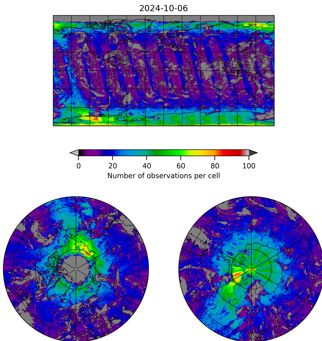
Figure 8: Map of the number of observations for 2024-10-05 to 2024-10-07
