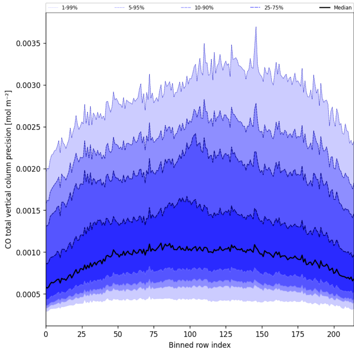
Figure 28: Along track statistics of “CO total vertical column precision” for 2024-10-05 to 2024-10-07
