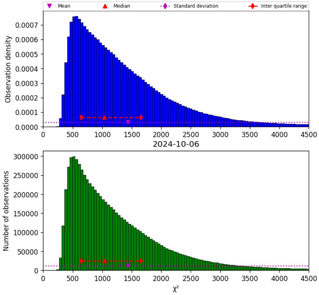
Figure 22: Histogram of " \chi^2 " for 2024-10-05 to 2024-10-07
