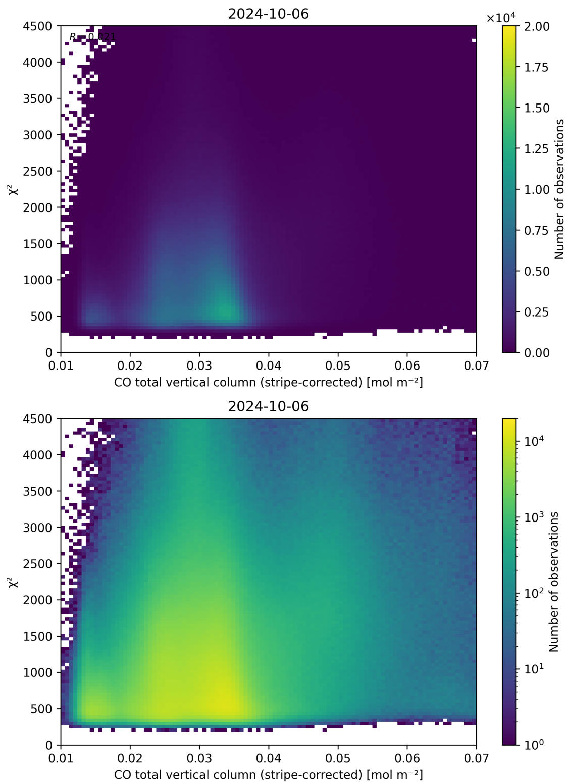
Figure 37: Scatter density plot of “CO total vertical column (stripe-corrected)” against “ \chi^2 ” for 2024-10-05 to 2024-10-07.
