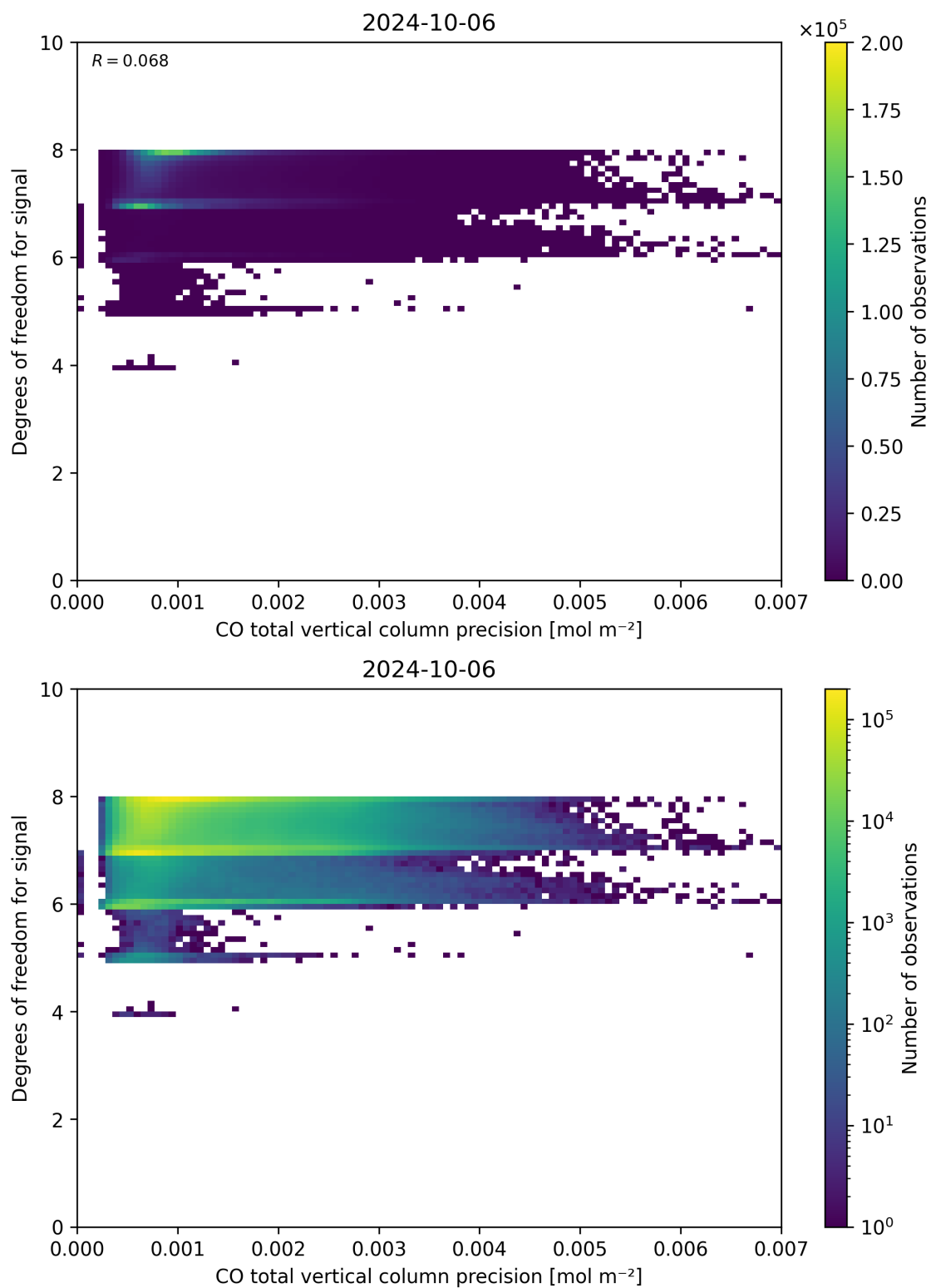
Figure 45: Scatter density plot of “CO total vertical column precision” against “Degrees of freedom for signal” for 2024-10-05 to 2024-10-07.
