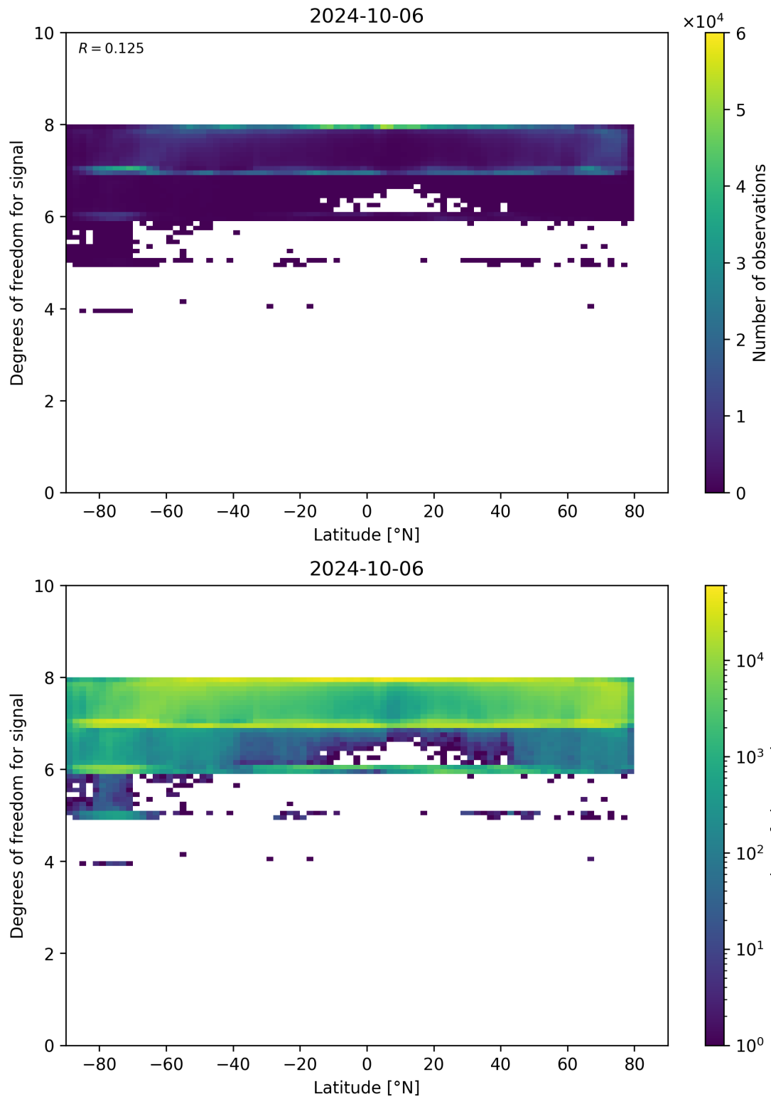
Figure 55: Scatter density plot of “Latitude” against “Degrees of freedom for signal” for 2024-10-05 to 2024-10-07.
