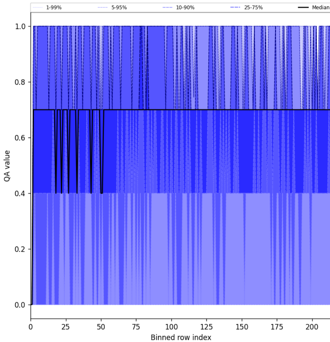
Figure 25: Along track statistics of “QA value” for 2024-10-05 to 2024-10-07
