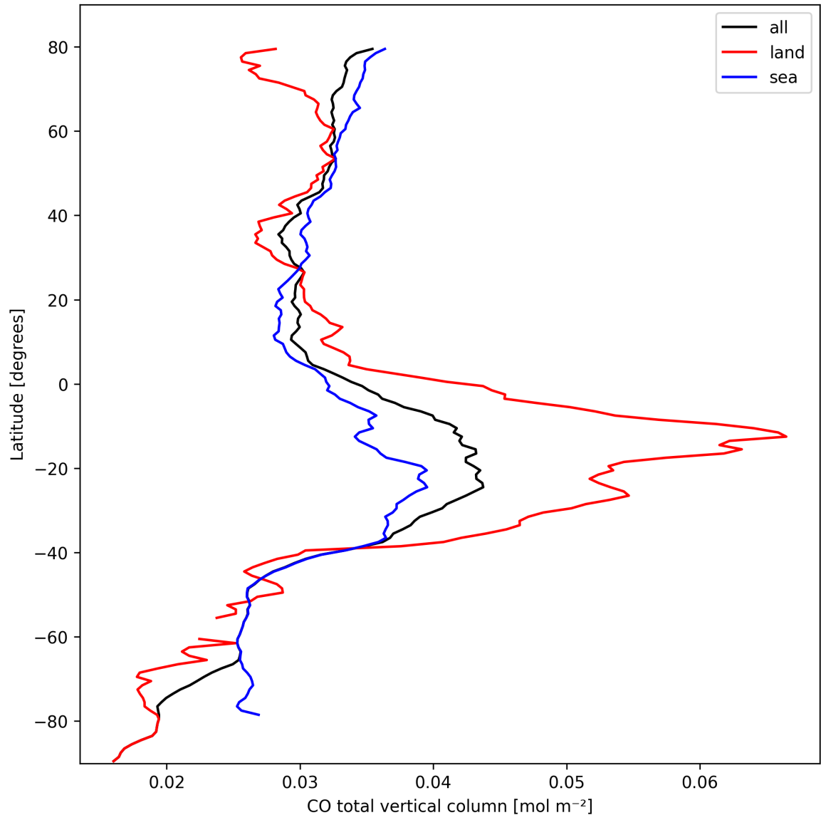
Figure 10: Zonal average of “CO total vertical column” for 2024-10-05 to 2024-10-07.
