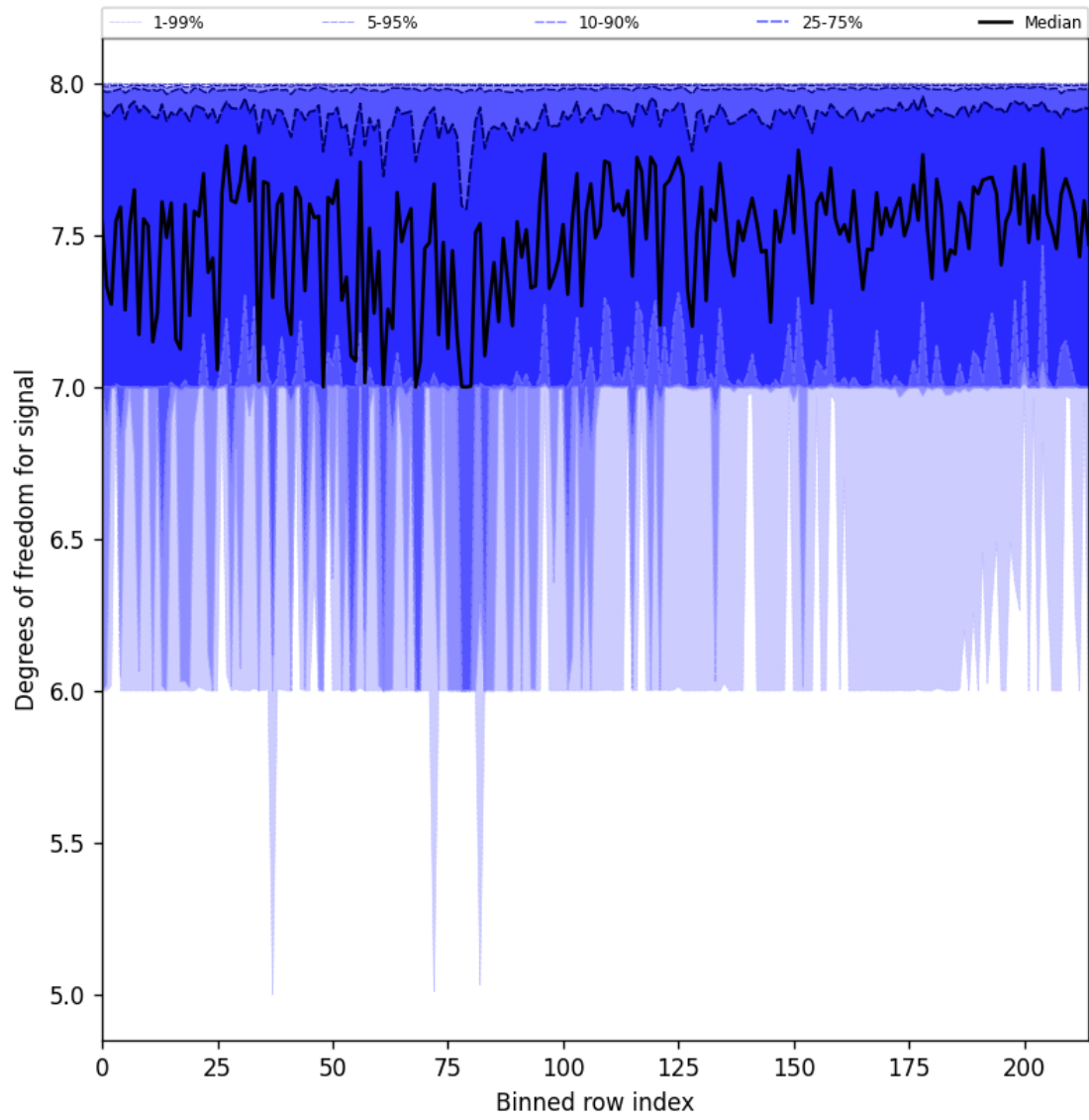
Figure 31: Along track statistics of “Degrees of freedom for signal” for 2024-10-05 to 2024-10-07
