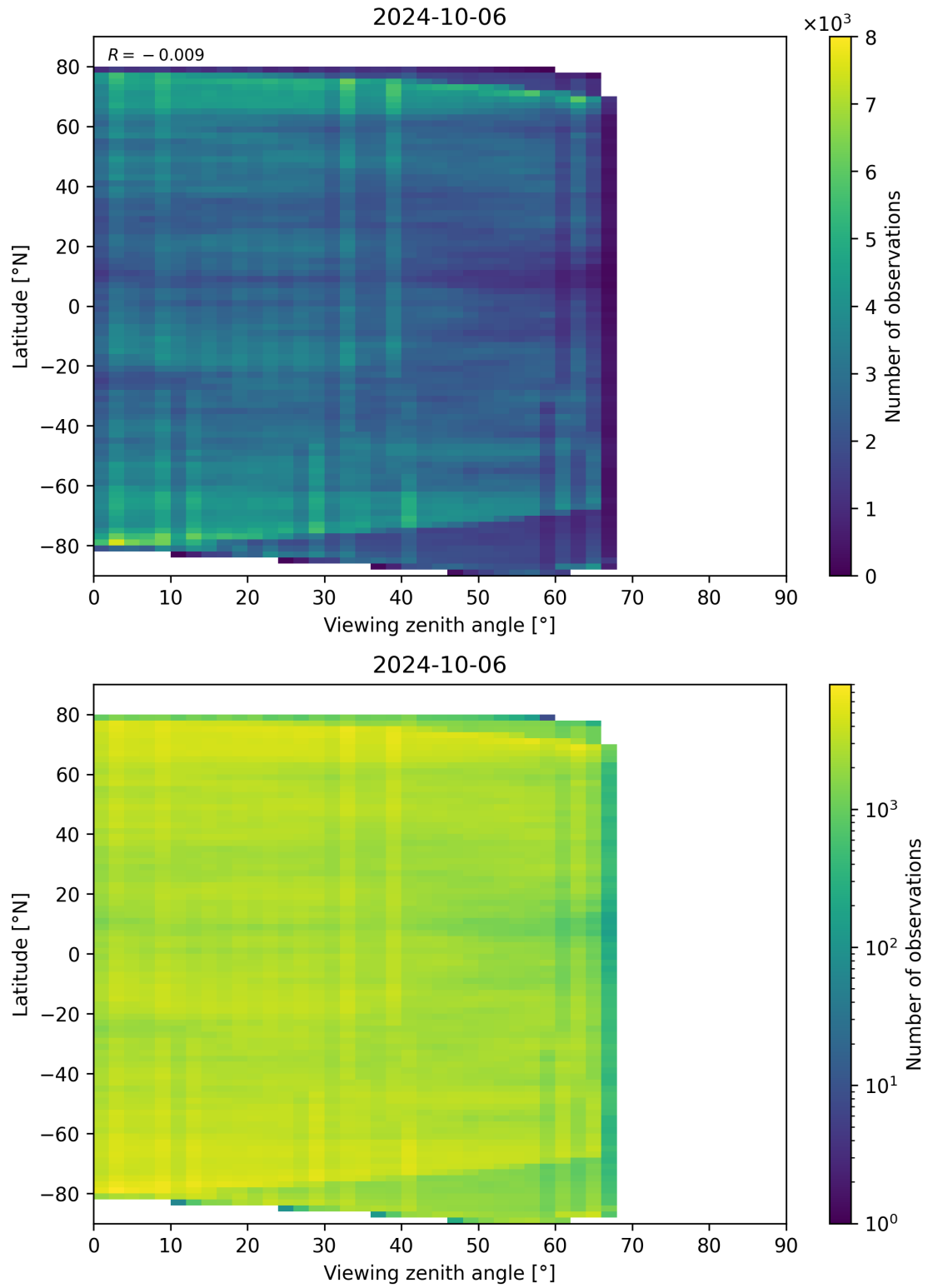
Figure 74: Scatter density plot of “Viewing zenith angle” against “Latitude” for 2024-10-05 to 2024-10-07.
