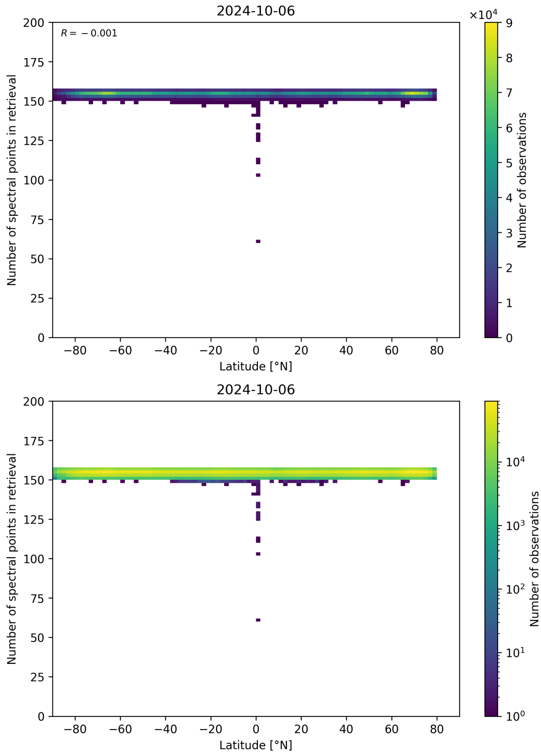
Figure 57: Scatter density plot of “Latitude” against “Number of spectral points in retrieval” for 2024-10-05 to 2024-10-07.
