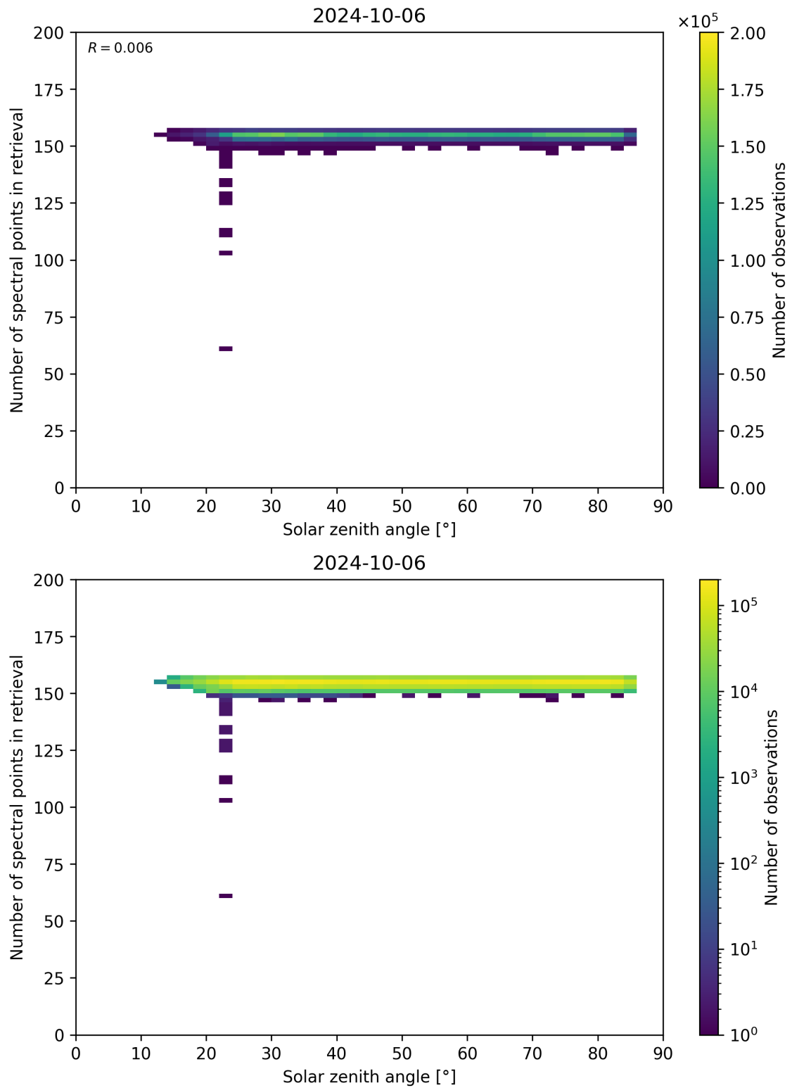
Figure 68: Scatter density plot of “Solar zenith angle” against “Number of spectral points in retrieval” for 2024-10-05 to 2024-10-07.
