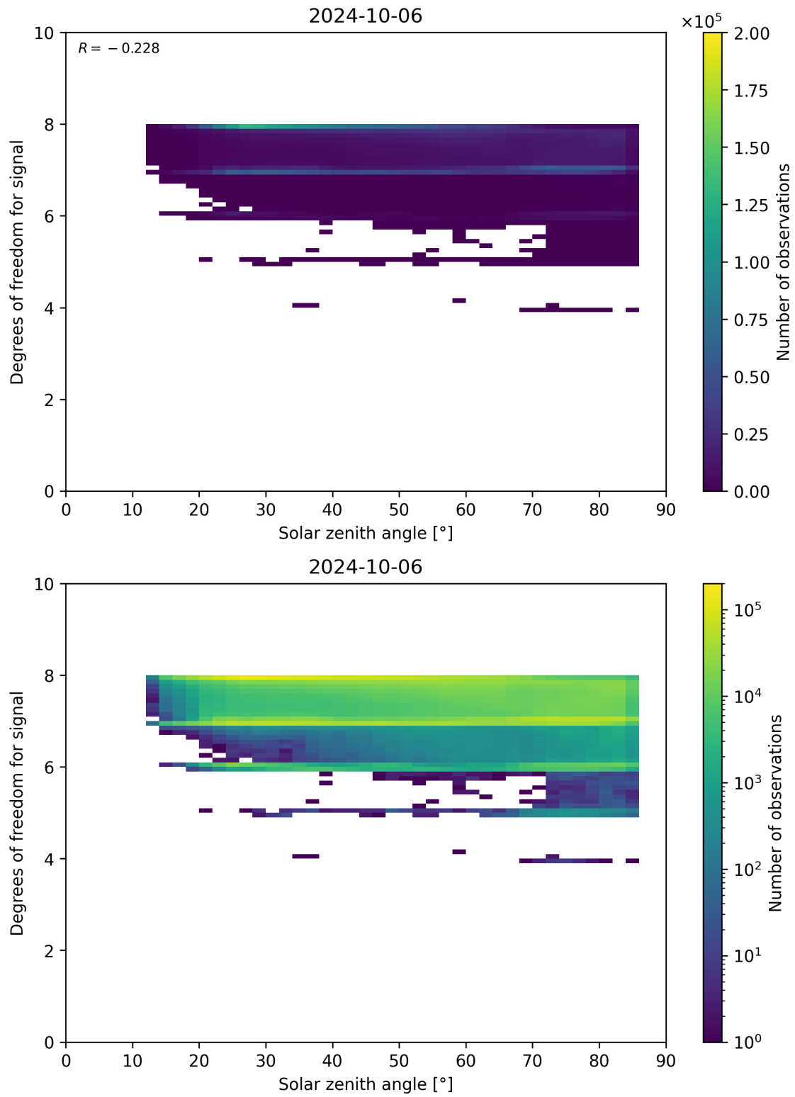
Figure 65: Scatter density plot of “Solar zenith angle” against “Degrees of freedom for signal” for 2024-10-05 to 2024-10-07.
