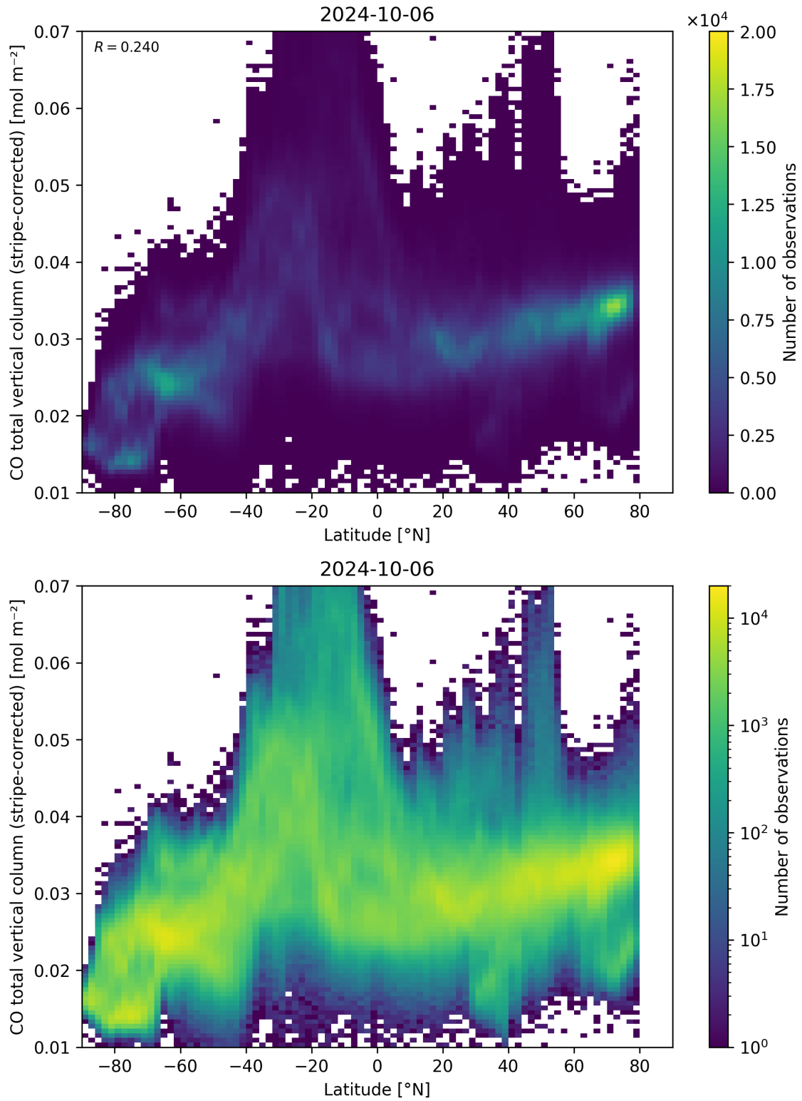
Figure 52: Scatter density plot of “Latitude” against “CO total vertical column (stripe-corrected)” for 2024-10-05 to 2024-10-07.
