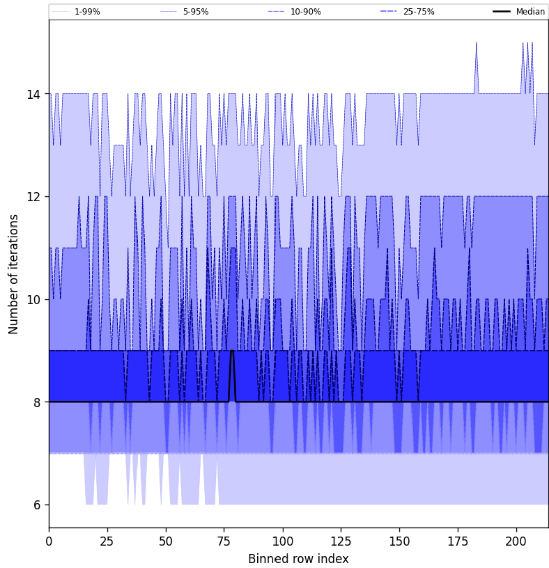
Figure 32: Along track statistics of “Number of iterations” for 2024-10-05 to 2024-10-07
