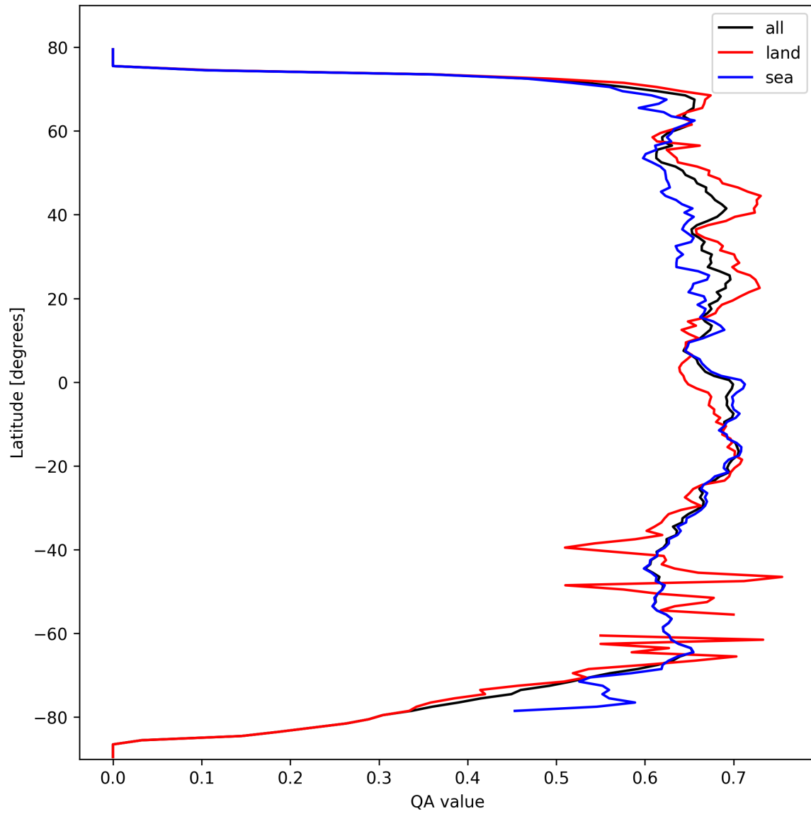
Figure 9: Zonal average of “QA value” for 2024-10-05 to 2024-10-07.
