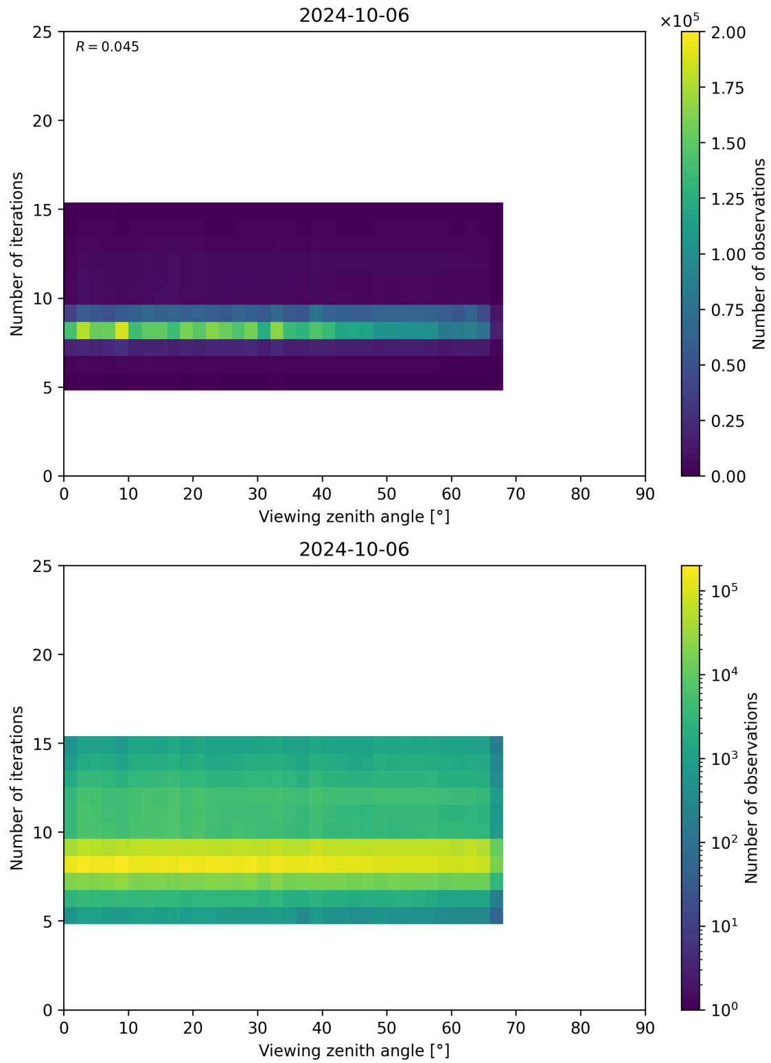
Figure 75: Scatter density plot of “Viewing zenith angle” against “Number of iterations” for 2024-10-05 to 2024-10-07.
