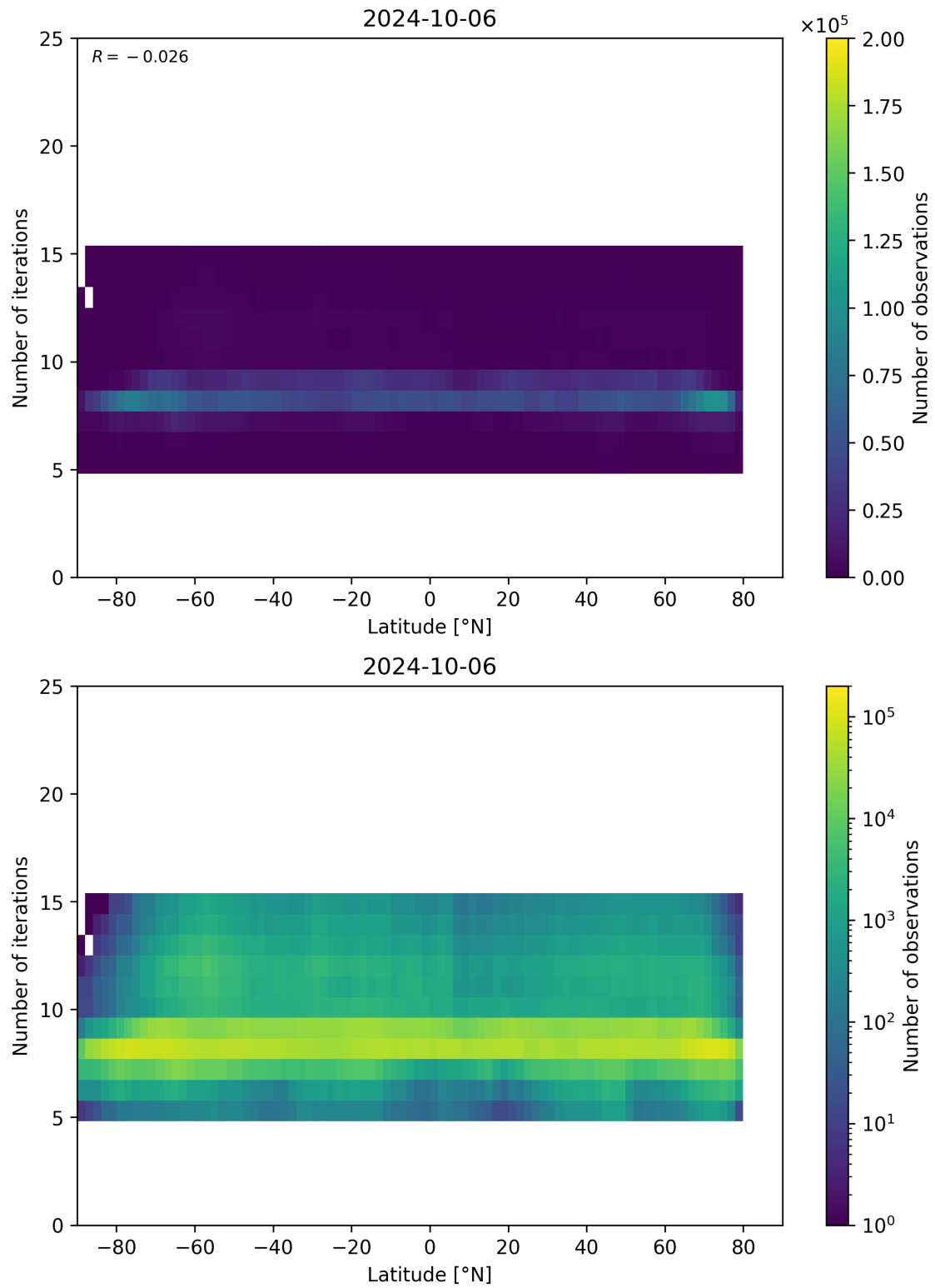
Figure 56: Scatter density plot of “Latitude” against “Number of iterations” for 2024-10-05 to 2024-10-07.
