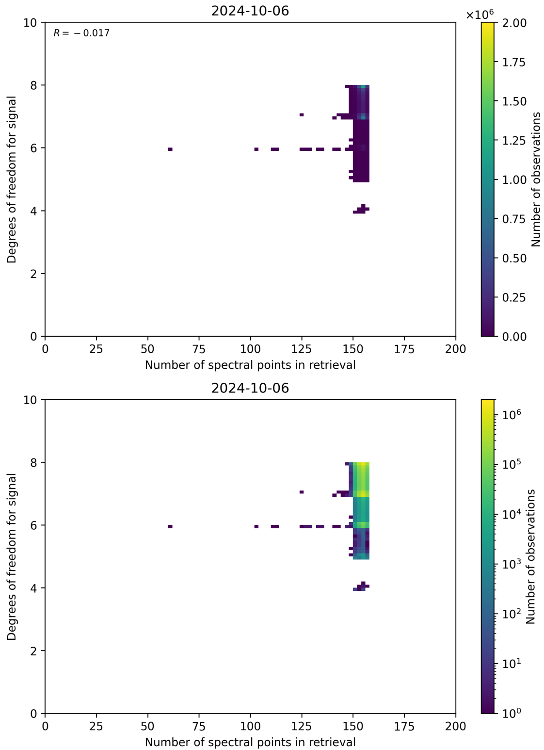
Figure 59: Scatter density plot of “Number of spectral points in retrieval” against “Degrees of freedom for signal” for 2024-10-05 to 2024-10-07.
