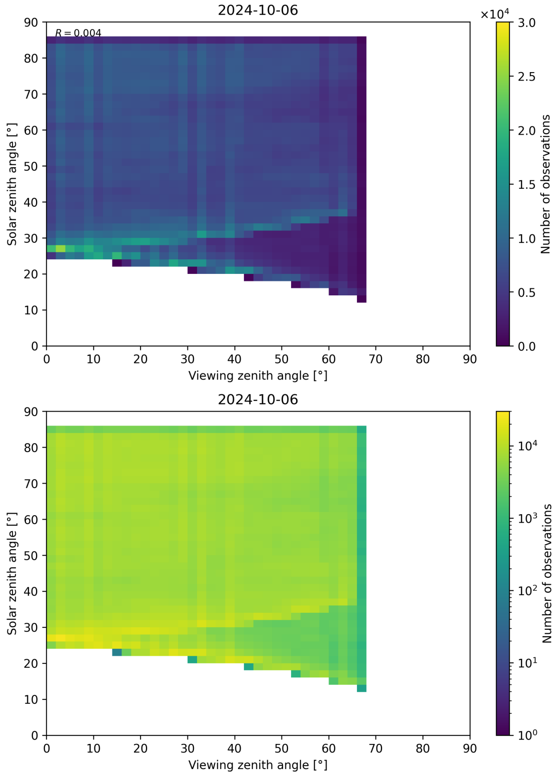
Figure 77: Scatter density plot of “Viewing zenith angle” against “Solar zenith angle” for 2024-10-05 to 2024-10-07.
