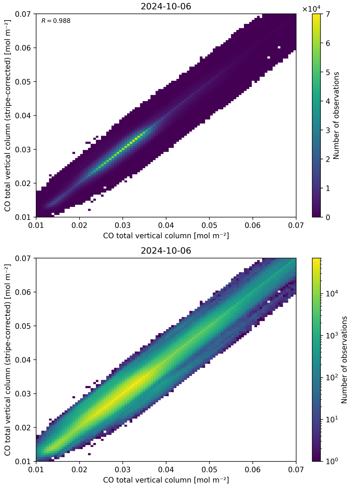
Figure 33: Scatter density plot of “CO total vertical column” against “CO total vertical column (stripe-corrected)” for 2024-10-05 to 2024-10-07.
