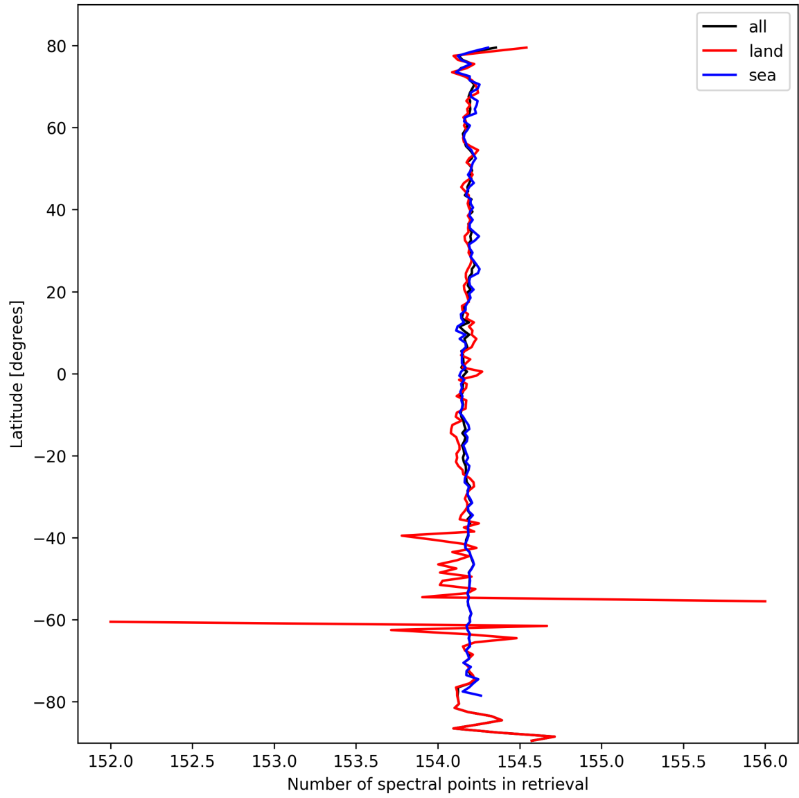
Figure 13: Zonal average of “Number of spectral points in retrieval” for 2024-10-05 to 2024-10-07.
