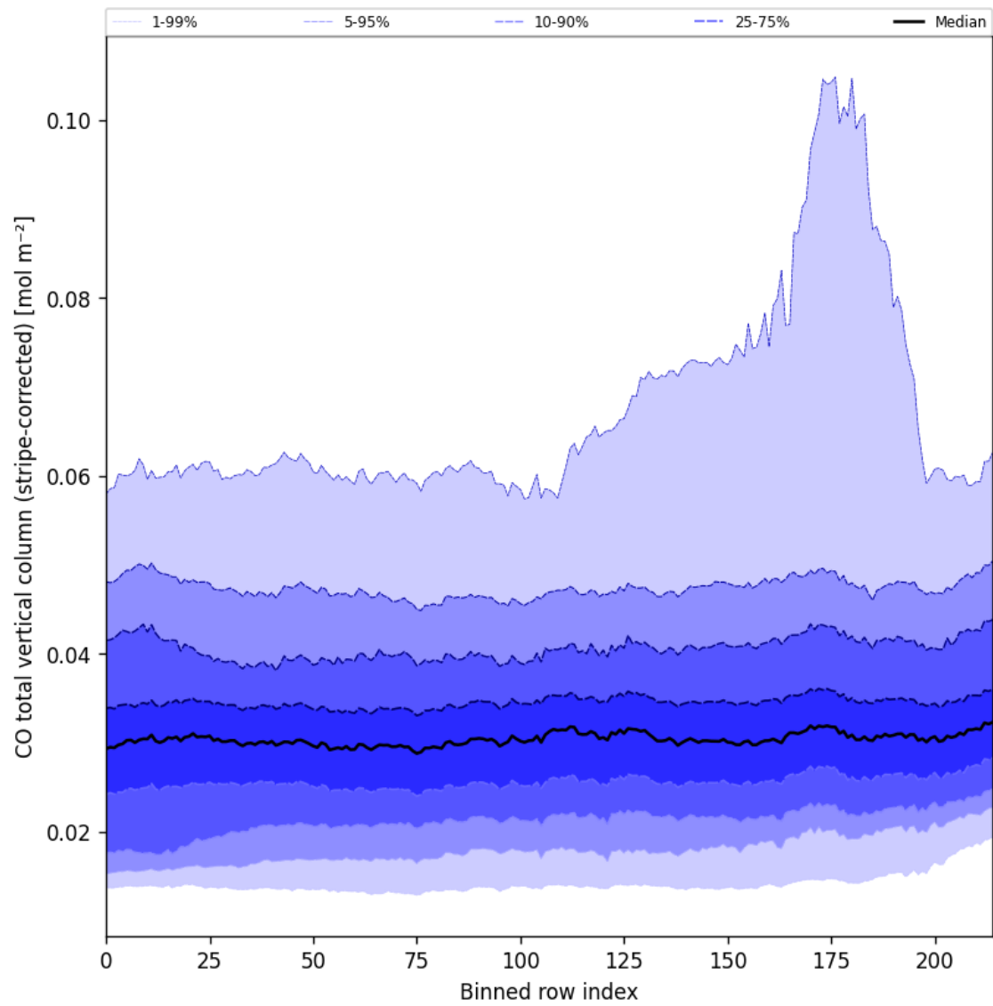
Figure 27: Along track statistics of “CO total vertical column (stripe-corrected)” for 2024-10-05 to 2024-10-07
