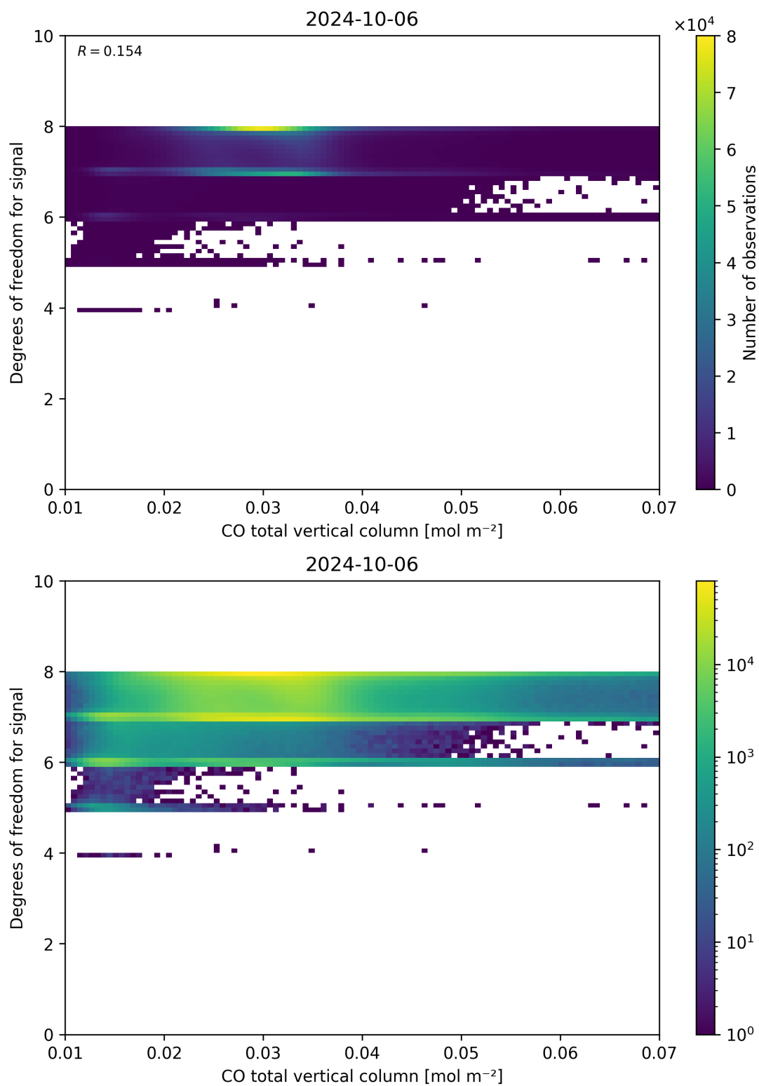
Figure 41: Scatter density plot of “CO total vertical column” against “Degrees of freedom for signal” for 2024-10-05 to 2024-10-07.
