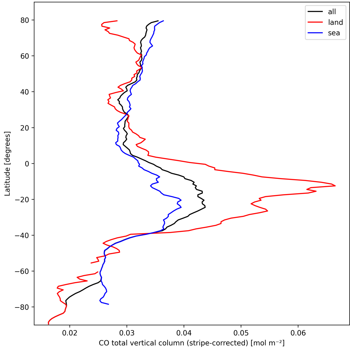
Figure 11: Zonal average of “CO total vertical column (stripe-corrected)” for 2024-10-05 to 2024-10-07.
