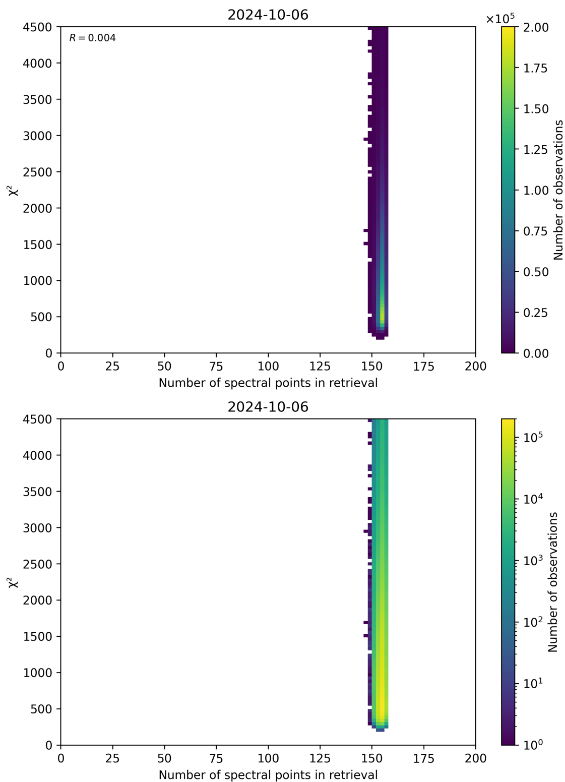
Figure 58: Scatter density plot of “Number of spectral points in retrieval” against “ \chi^2 ” for 2024-10-05 to 2024-10-07.
