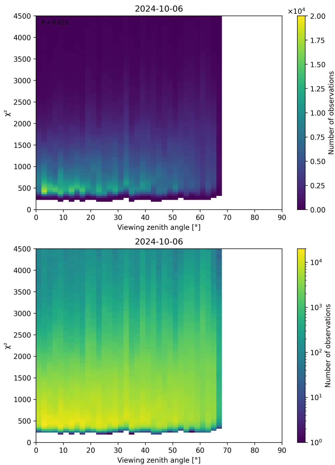
Figure 72: Scatter density plot of “Viewing zenith angle” against “ \chi^2 ” for 2024-10-05 to 2024-10-07.
