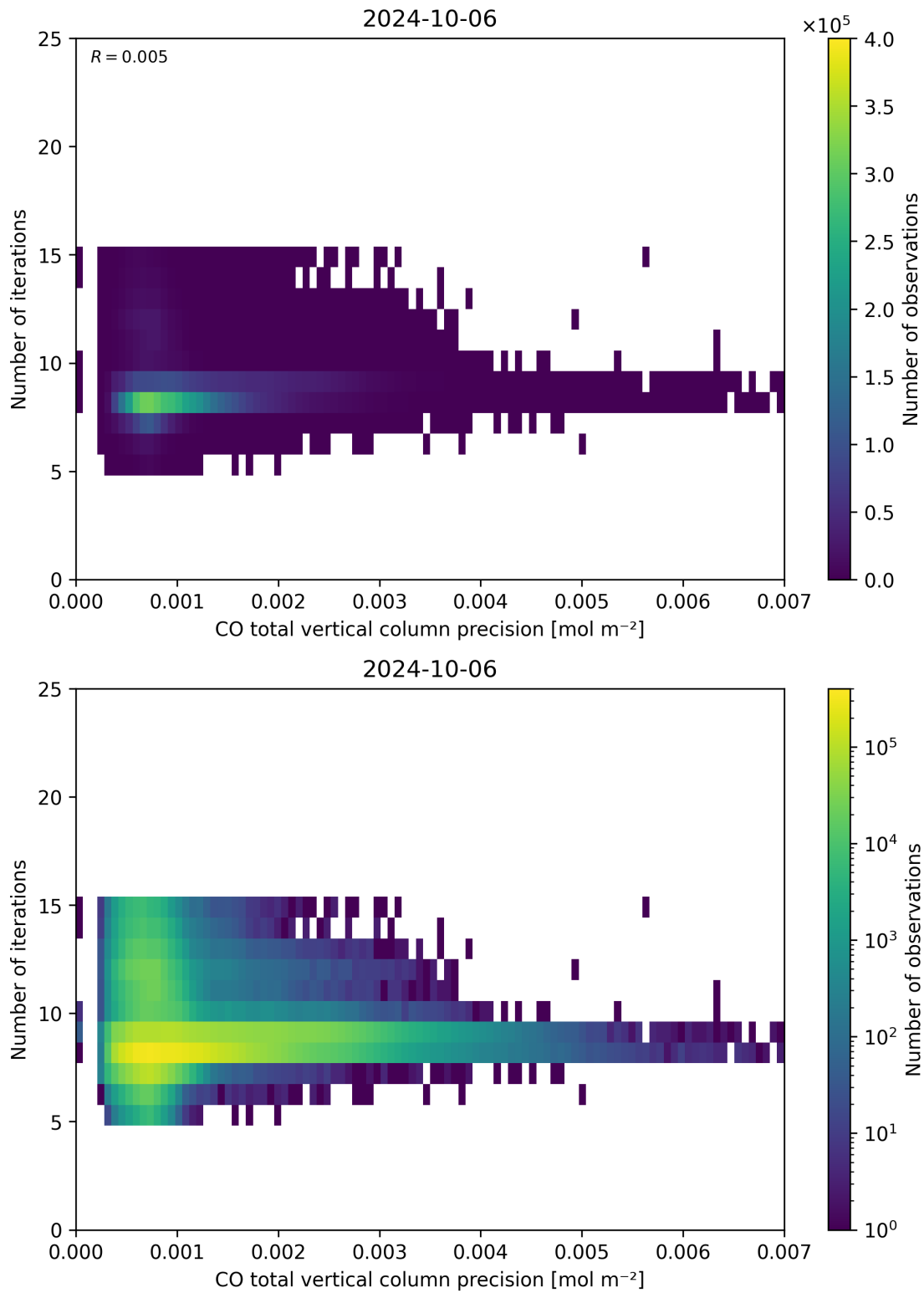
Figure 46: Scatter density plot of “CO total vertical column precision” against “Number of iterations” for 2024-10-05 to 2024-10-07.
