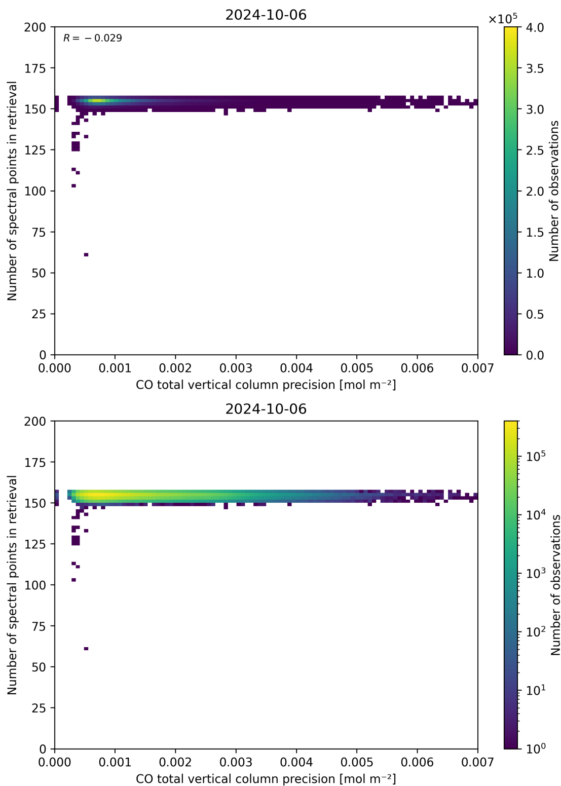
Figure 47: Scatter density plot of “CO total vertical column precision” against “Number of spectral points in retrieval” for 2024-10-05 to 2024-10-07.
