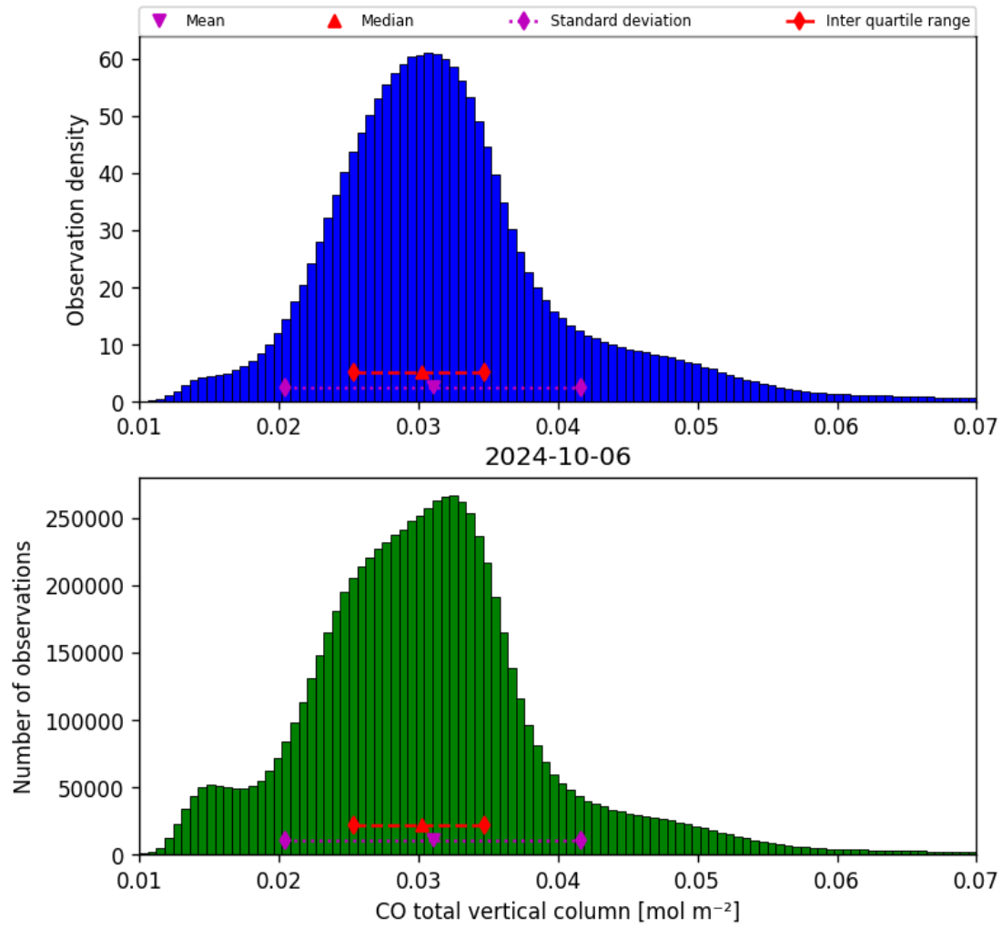
Figure 18: Histogram of “CO total vertical column” for 2024-10-05 to 2024-10-07
