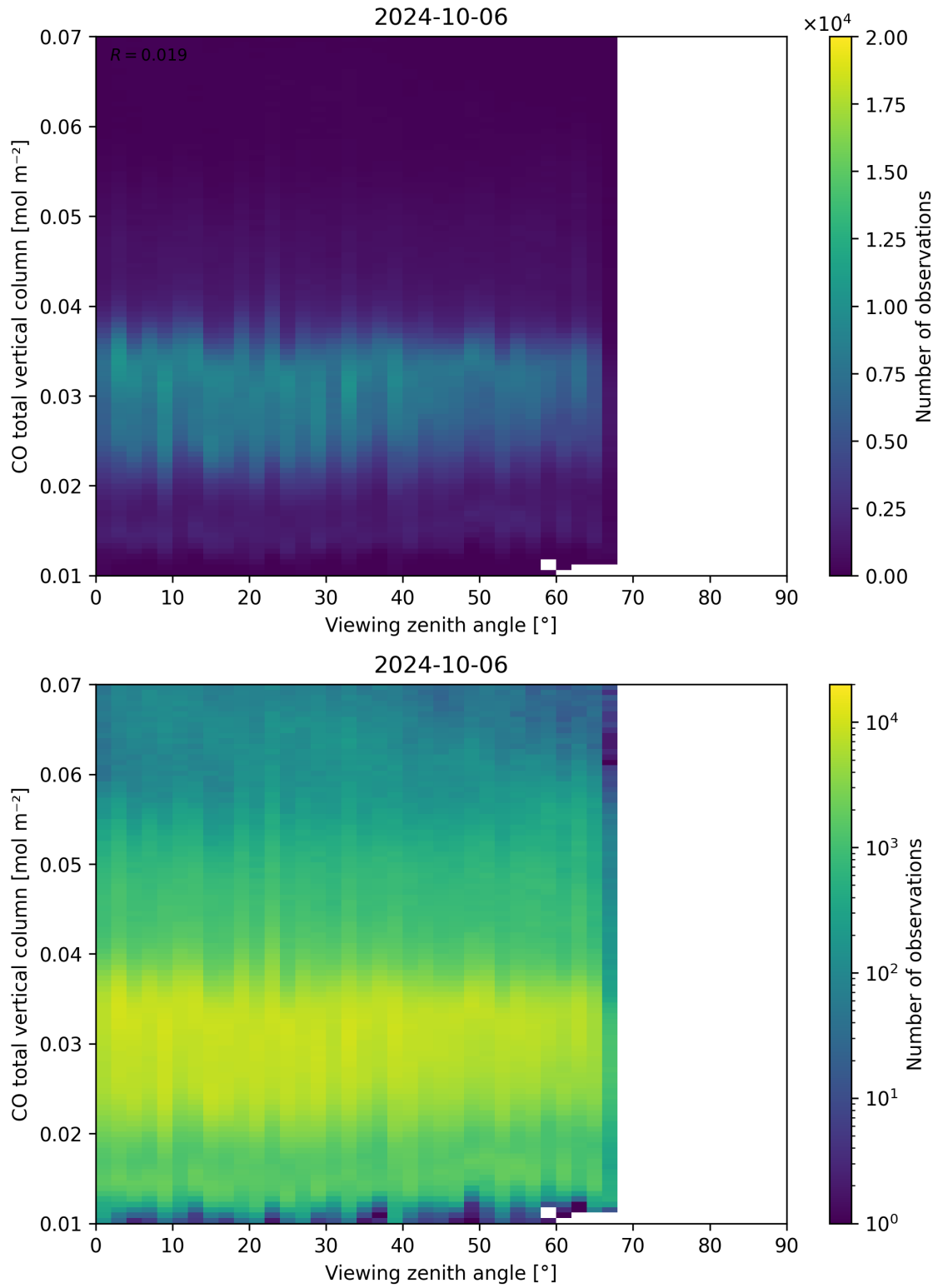
Figure 69: Scatter density plot of “Viewing zenith angle” against “CO total vertical column” for 2024-10-05 to 2024-10-07.
