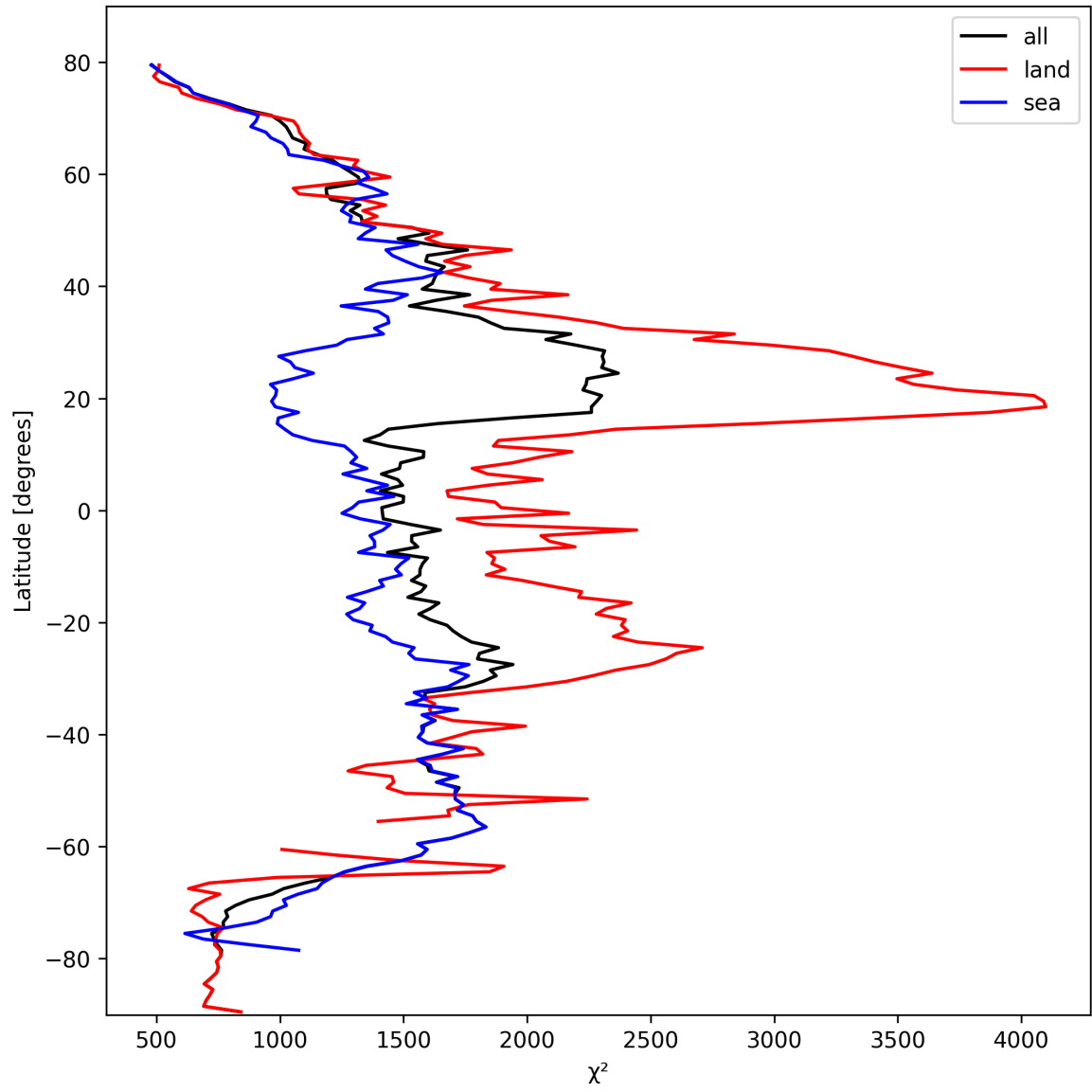
Figure 14: Zonal average of “ \chi^2 ” for 2024-10-05 to 2024-10-07.
