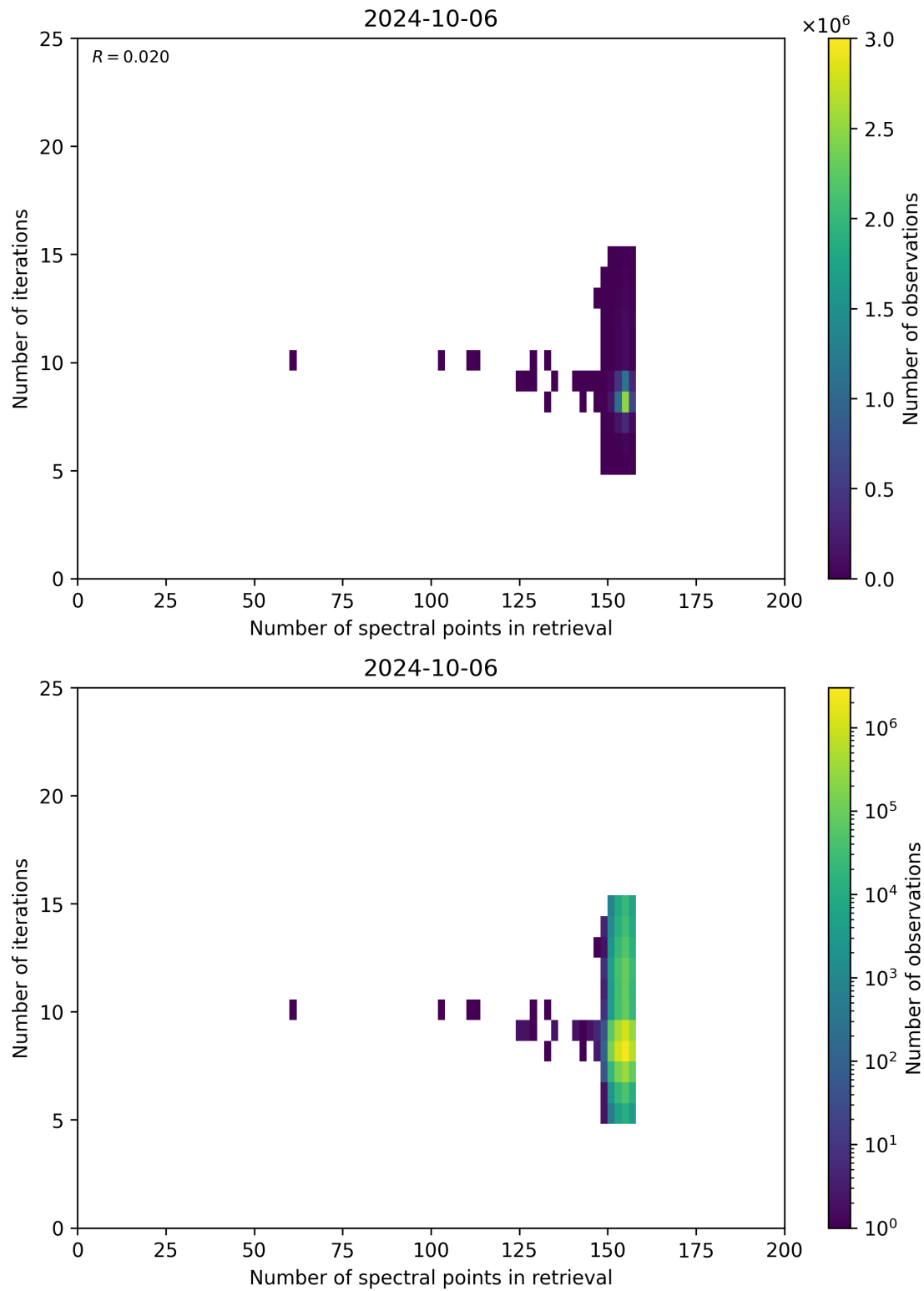
Figure 60: Scatter density plot of “Number of spectral points in retrieval” against “Number of iterations” for 2024-10-05 to 2024-10-07.
