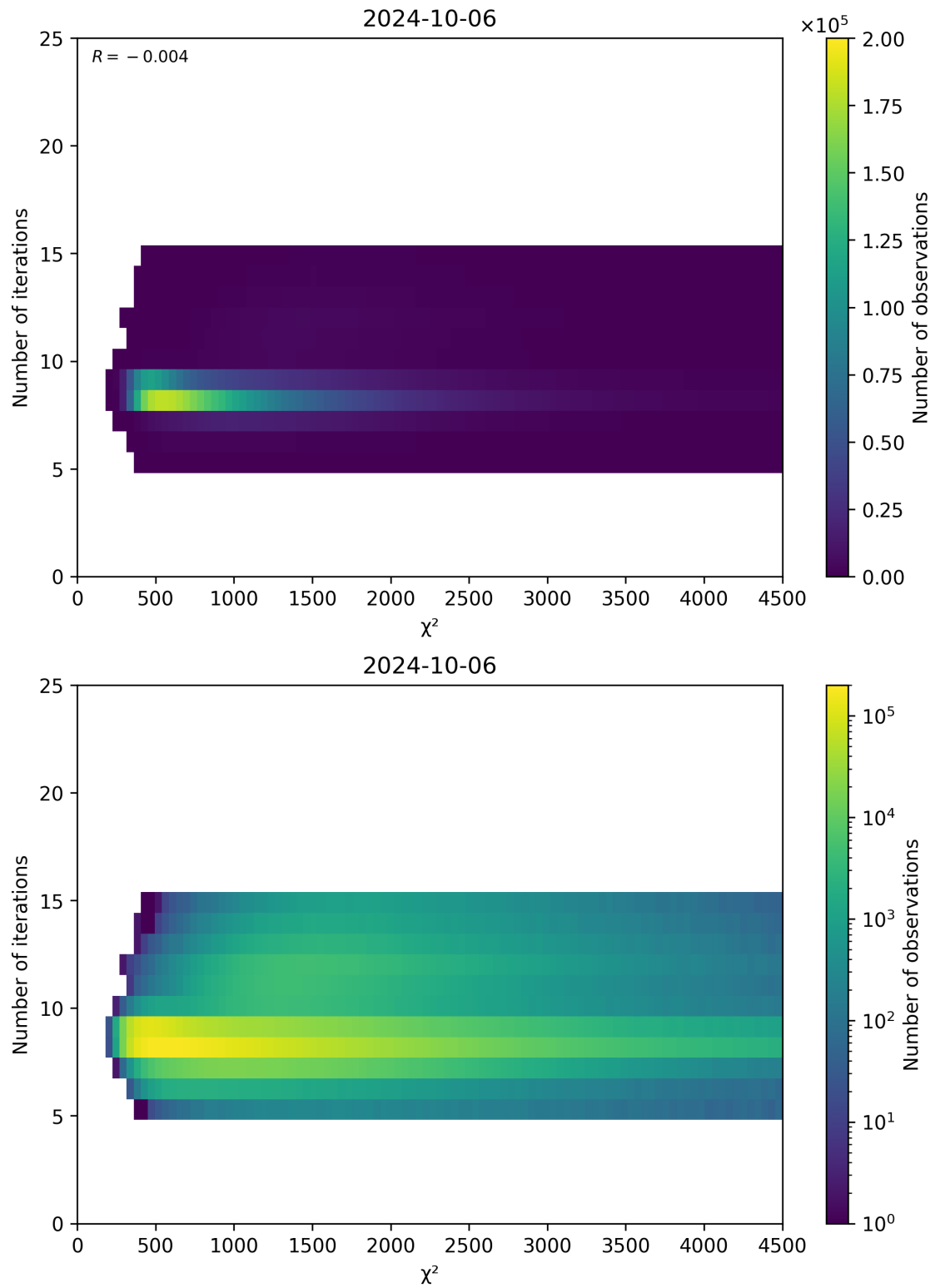
Figure 49: Scatter density plot of “ \chi^2 ” against “Number of iterations” for 2024-10-05 to 2024-10-07.
