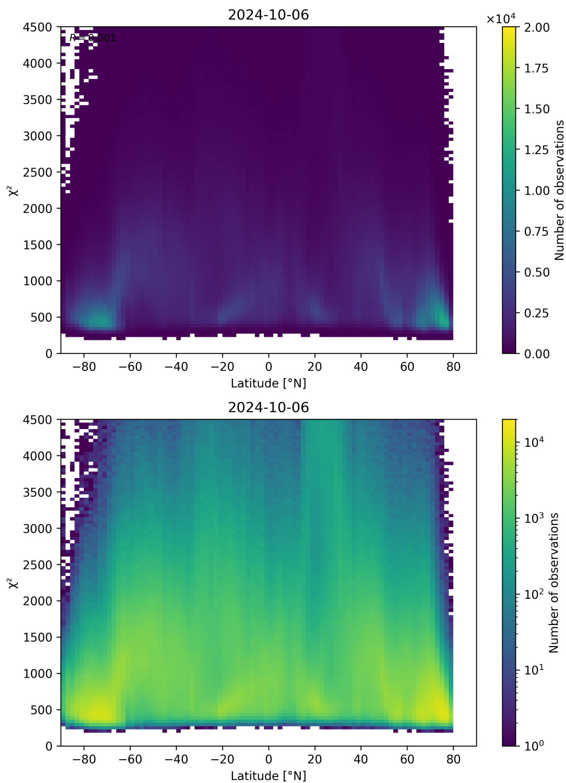
Figure 54: Scatter density plot of “Latitude” against “ \chi^2 ” for 2024-10-05 to 2024-10-07.
