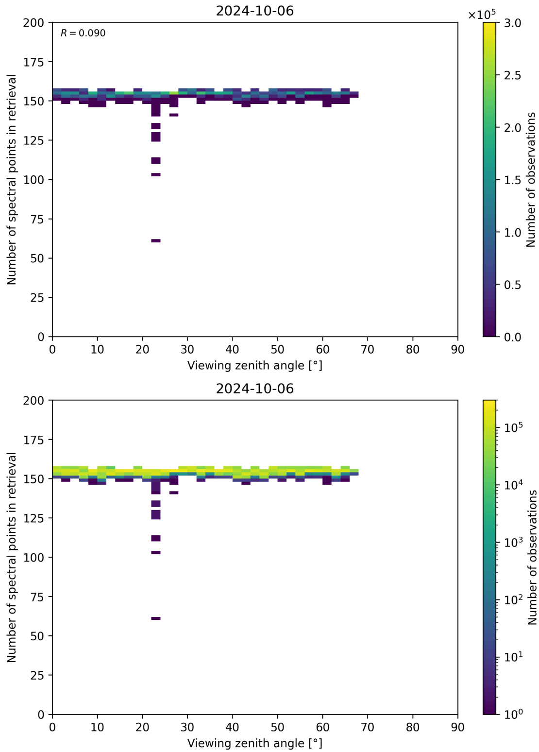
Figure 76: Scatter density plot of “Viewing zenith angle” against “Number of spectral points in retrieval” for 2024-10-05 to 2024-10-07.
