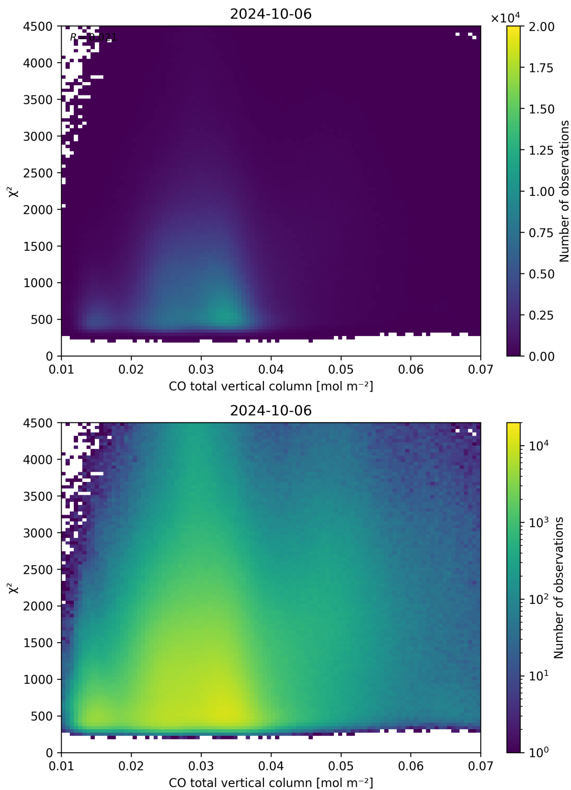
Figure 35: Scatter density plot of “CO total vertical column” against “ \chi^2 ” for 2024-10-05 to 2024-10-07.
