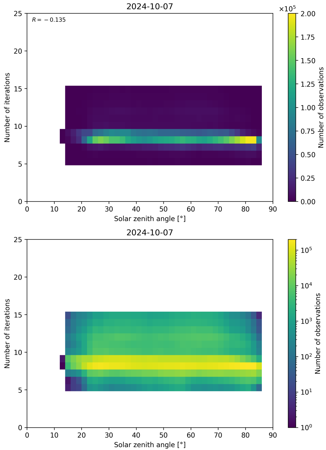
Figure 67: Scatter density plot of “Solar zenith angle” against “Number of iterations” for 2024-10-06 to 2024-10-08.
