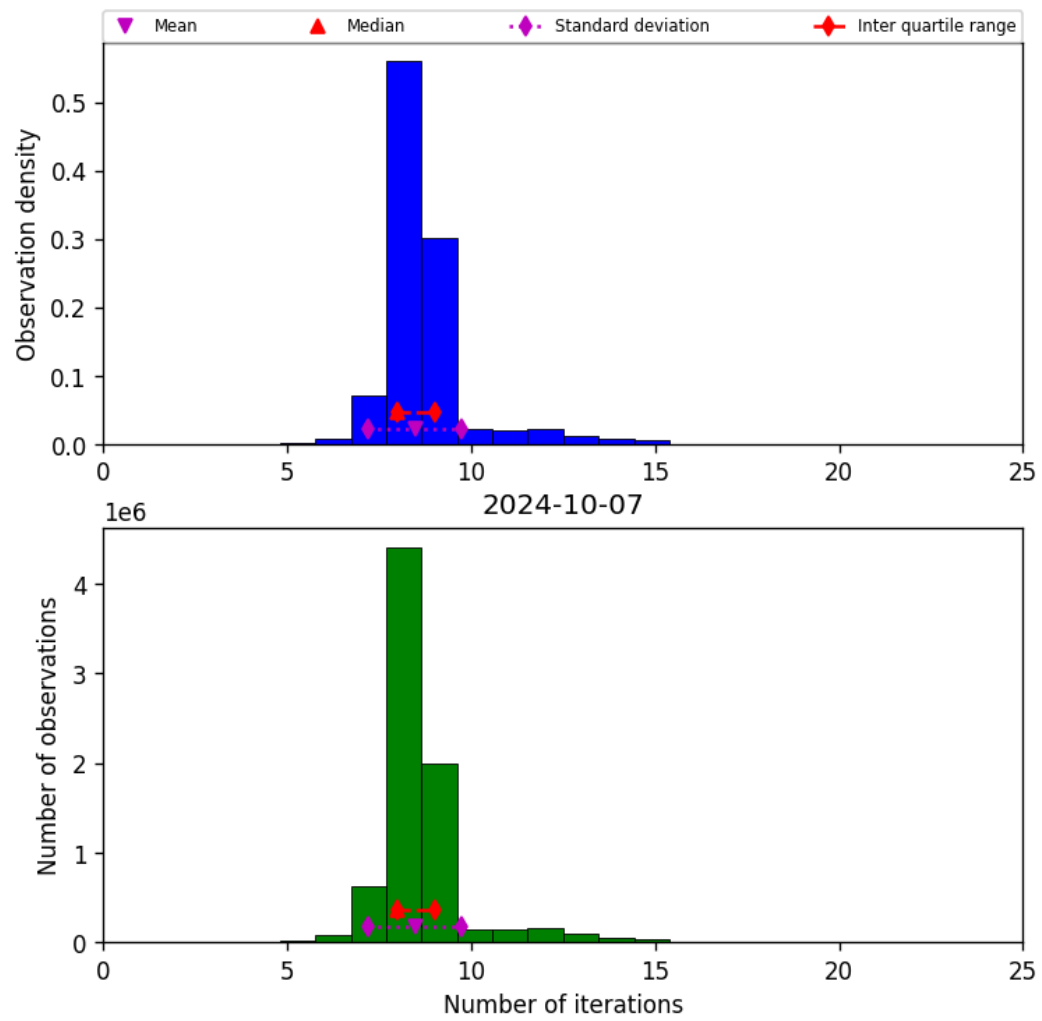
Figure 24: Histogram of “Number of iterations” for 2024-10-06 to 2024-10-08
