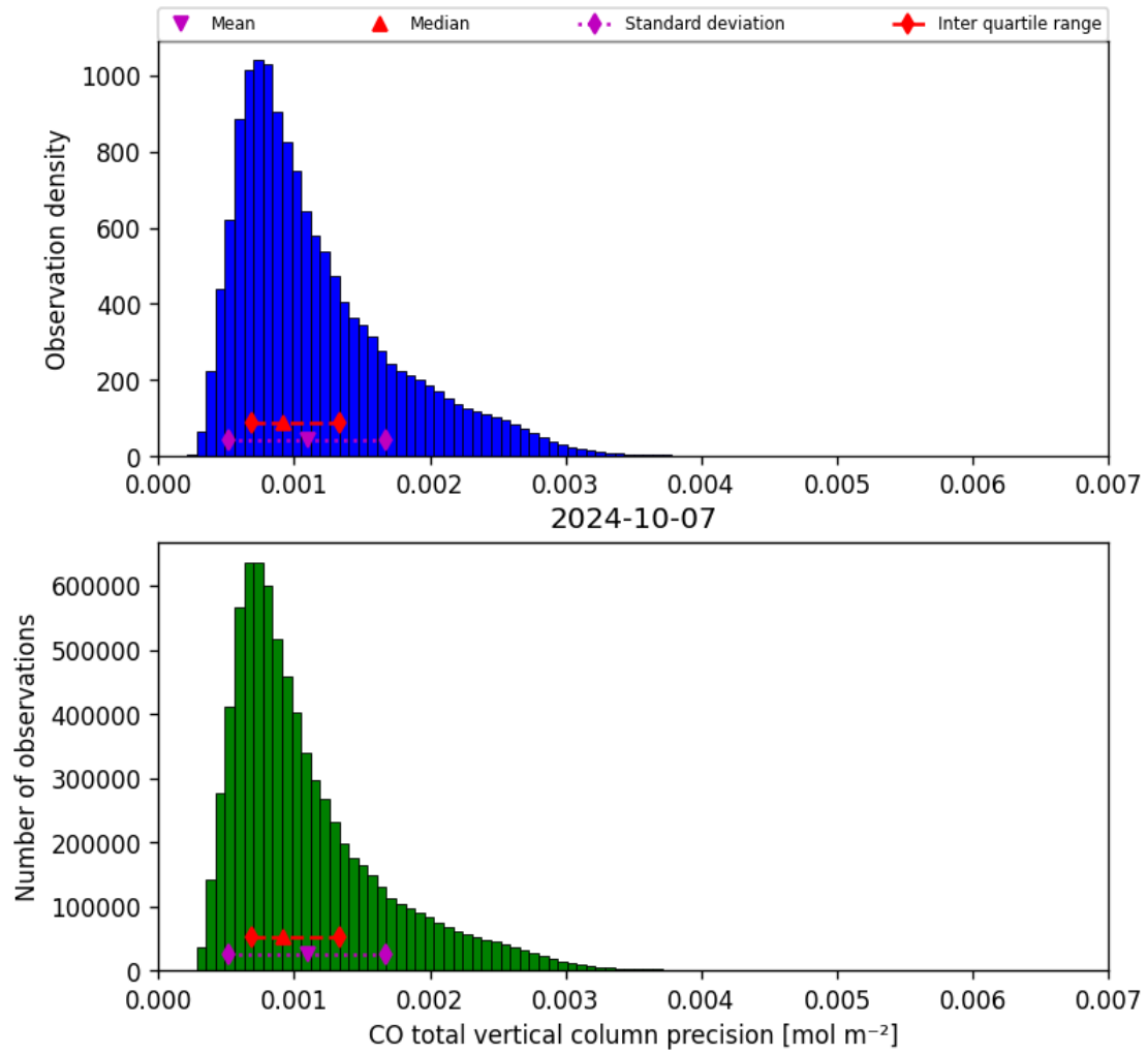
Figure 20: Histogram of “CO total vertical column precision” for 2024-10-06 to 2024-10-08
