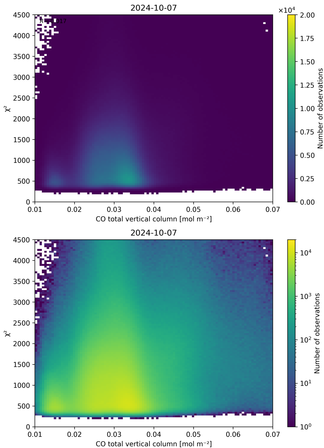
Figure 35: Scatter density plot of “CO total vertical column” against “ \chi^2 ” for 2024-10-06 to 2024-10-08.
