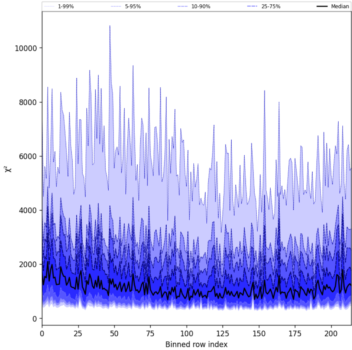
Figure 30: Along track statistics of “ \chi^2 ” for 2024-10-06 to 2024-10-08
