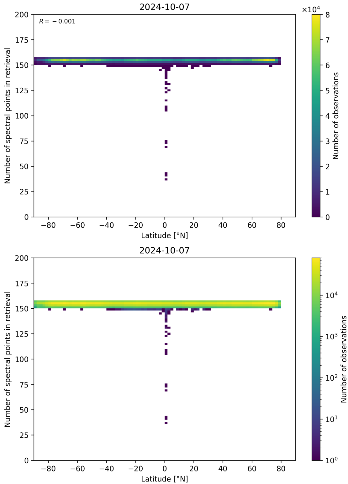
Figure 57: Scatter density plot of “Latitude” against “Number of spectral points in retrieval” for 2024-10-06 to 2024-10-08.
