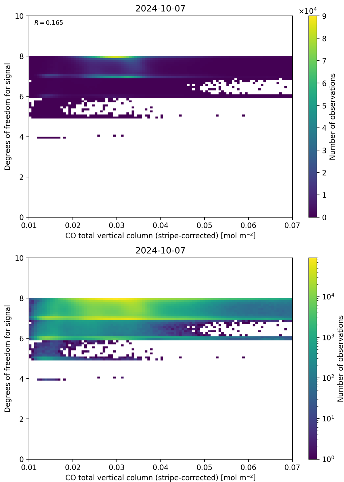
Figure 38: Scatter density plot of “CO total vertical column (stripe-corrected)” against “Degrees of freedom for signal” for 2024-10-06 to 2024-10-08.
