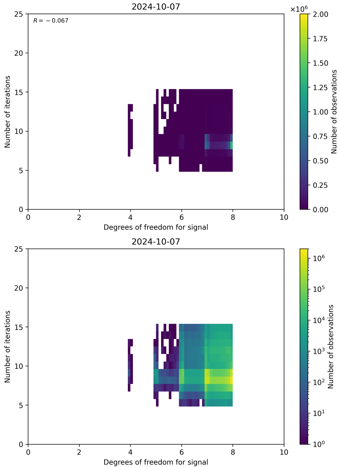
Figure 50: Scatter density plot of “Degrees of freedom for signal” against “Number of iterations” for 2024-10-06 to 2024-10-08.
