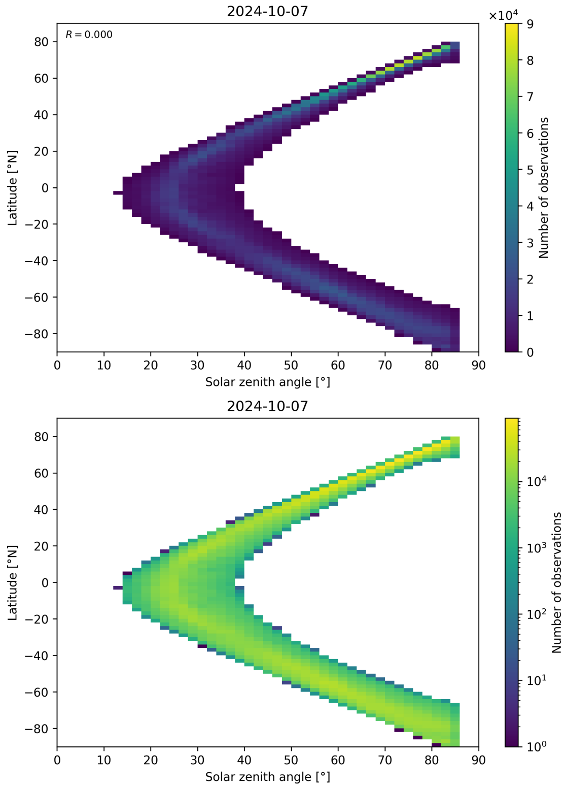
Figure 66: Scatter density plot of “Solar zenith angle” against “Latitude” for 2024-10-06 to 2024-10-08.
