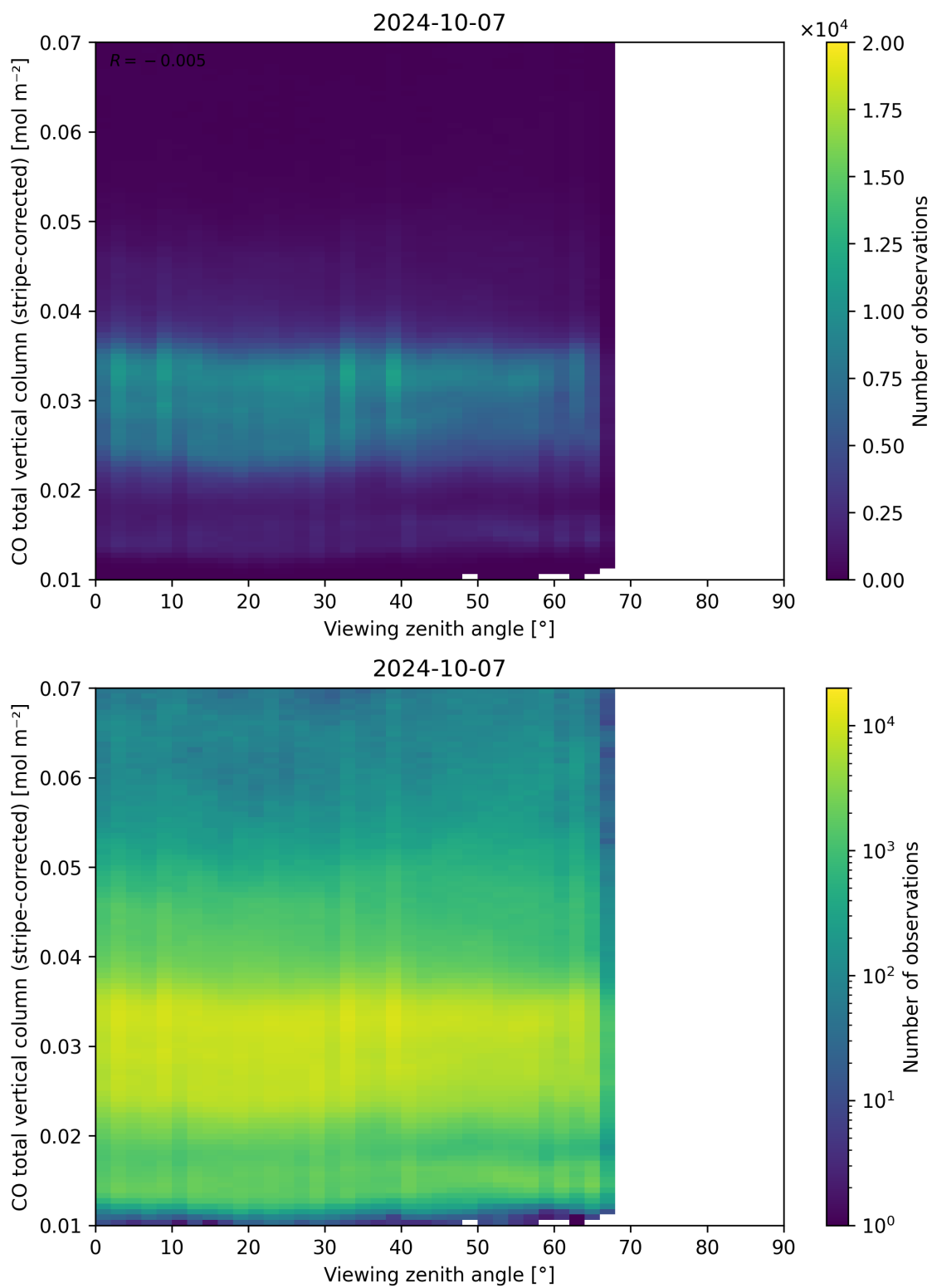
Figure 70: Scatter density plot of “Viewing zenith angle” against “CO total vertical column (stripe-corrected)” for 2024-10-06 to 2024-10-08.
