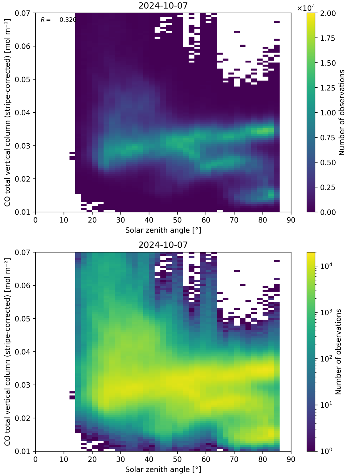
Figure 62: Scatter density plot of “Solar zenith angle” against “CO total vertical column (stripe-corrected)” for 2024-10-06 to 2024-10-08.
