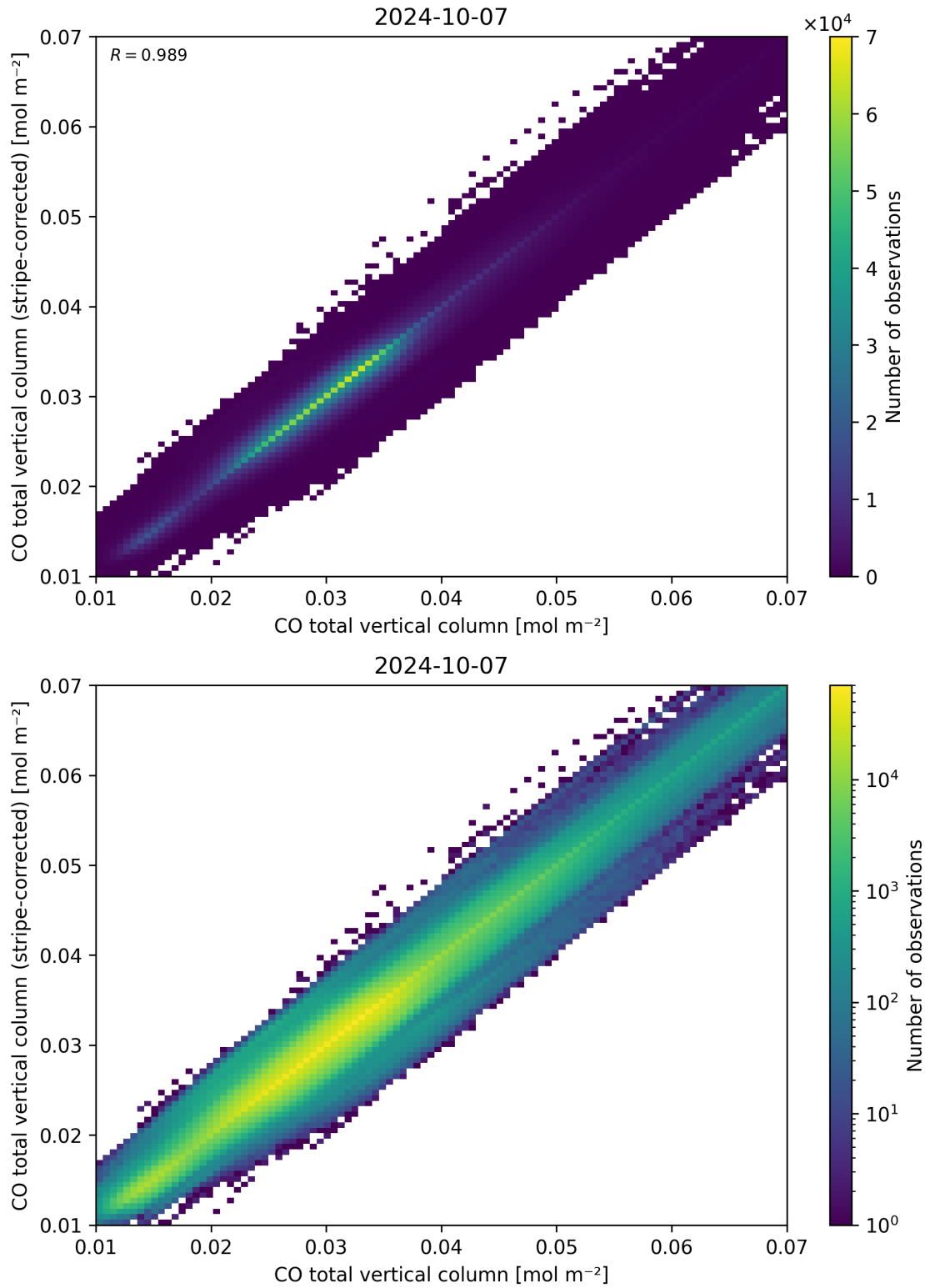
Figure 33: Scatter density plot of “CO total vertical column” against “CO total vertical column (stripe-corrected)” for 2024-10-06 to 2024-10-08.
