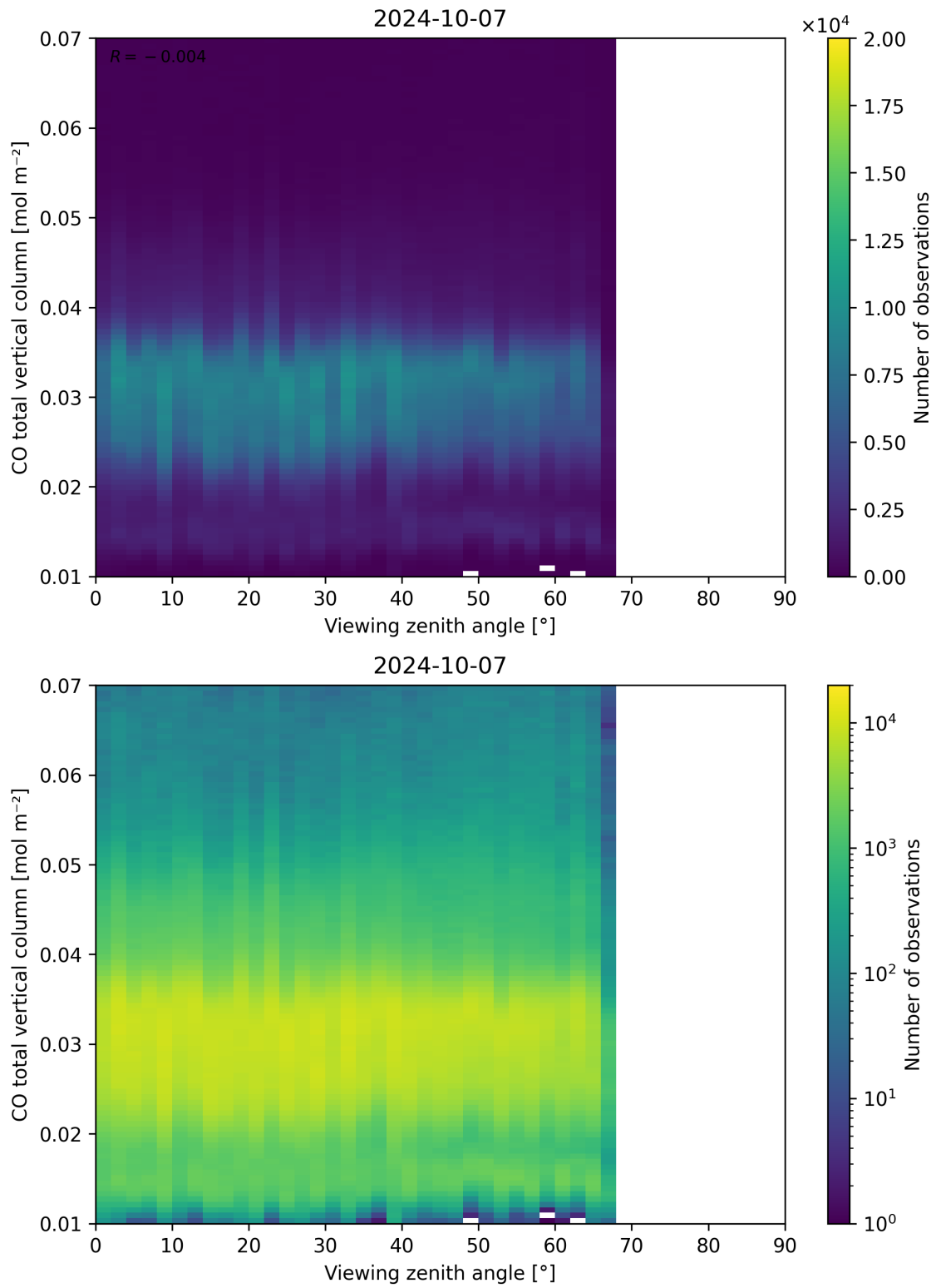
Figure 69: Scatter density plot of “Viewing zenith angle” against “CO total vertical column” for 2024-10-06 to 2024-10-08.
