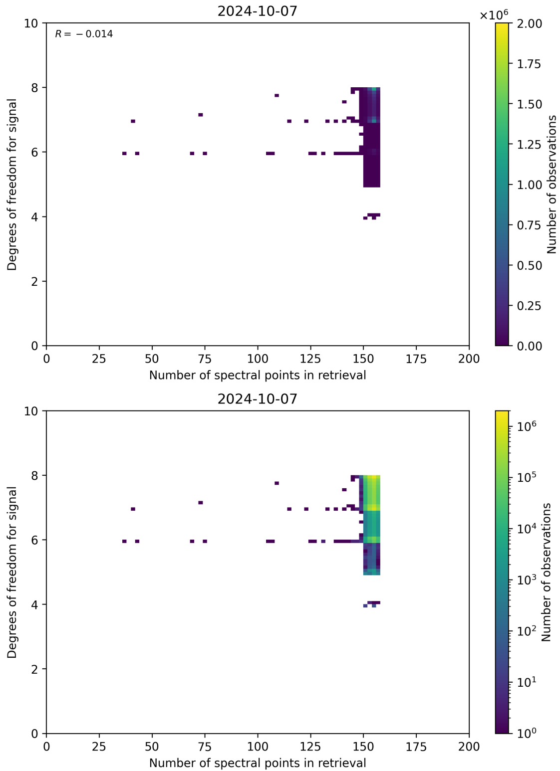
Figure 59: Scatter density plot of “Number of spectral points in retrieval” against “Degrees of freedom for signal” for 2024-10-06 to 2024-10-08.
