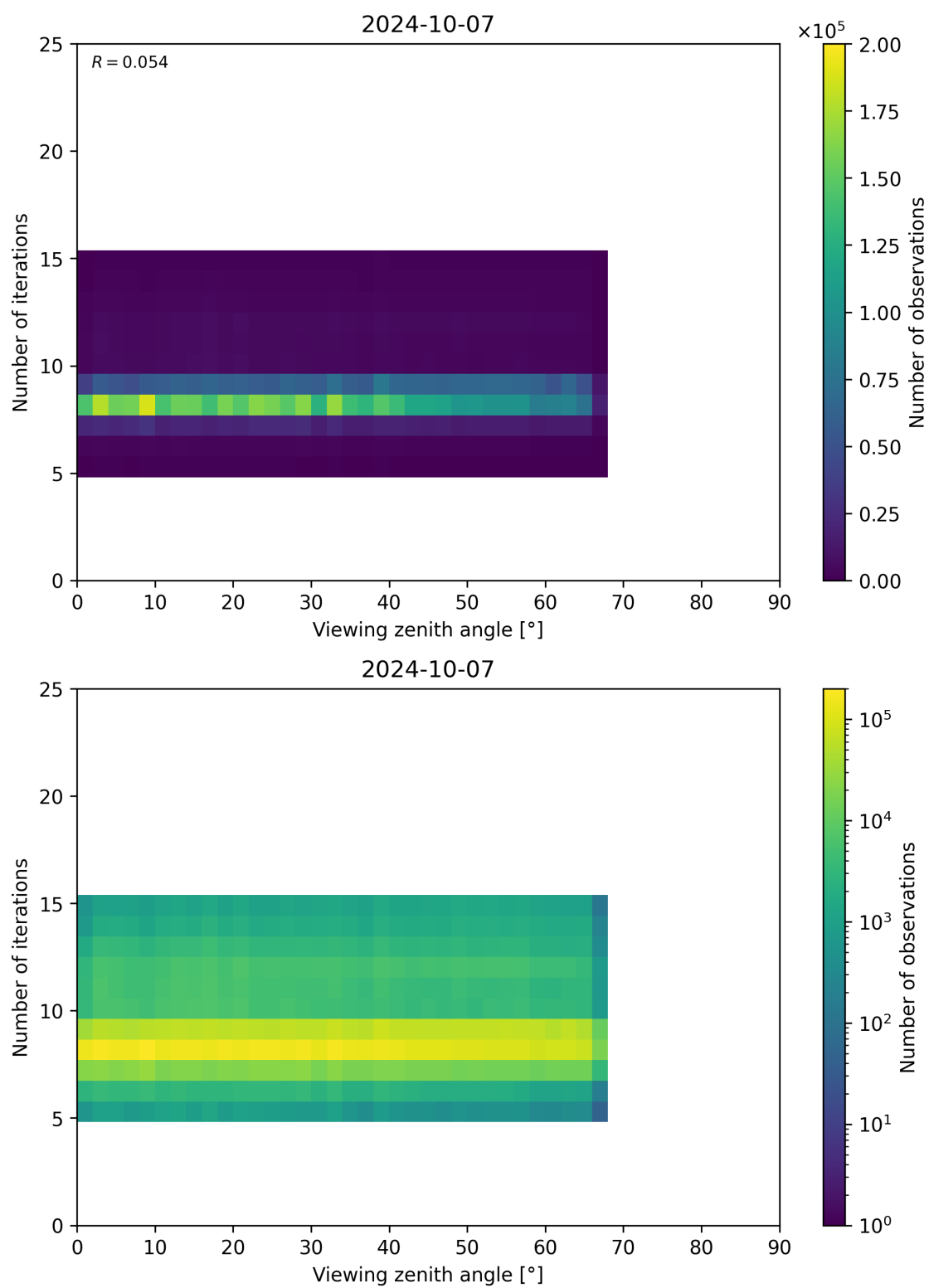
Figure 75: Scatter density plot of “Viewing zenith angle” against “Number of iterations” for 2024-10-06 to 2024-10-08.
