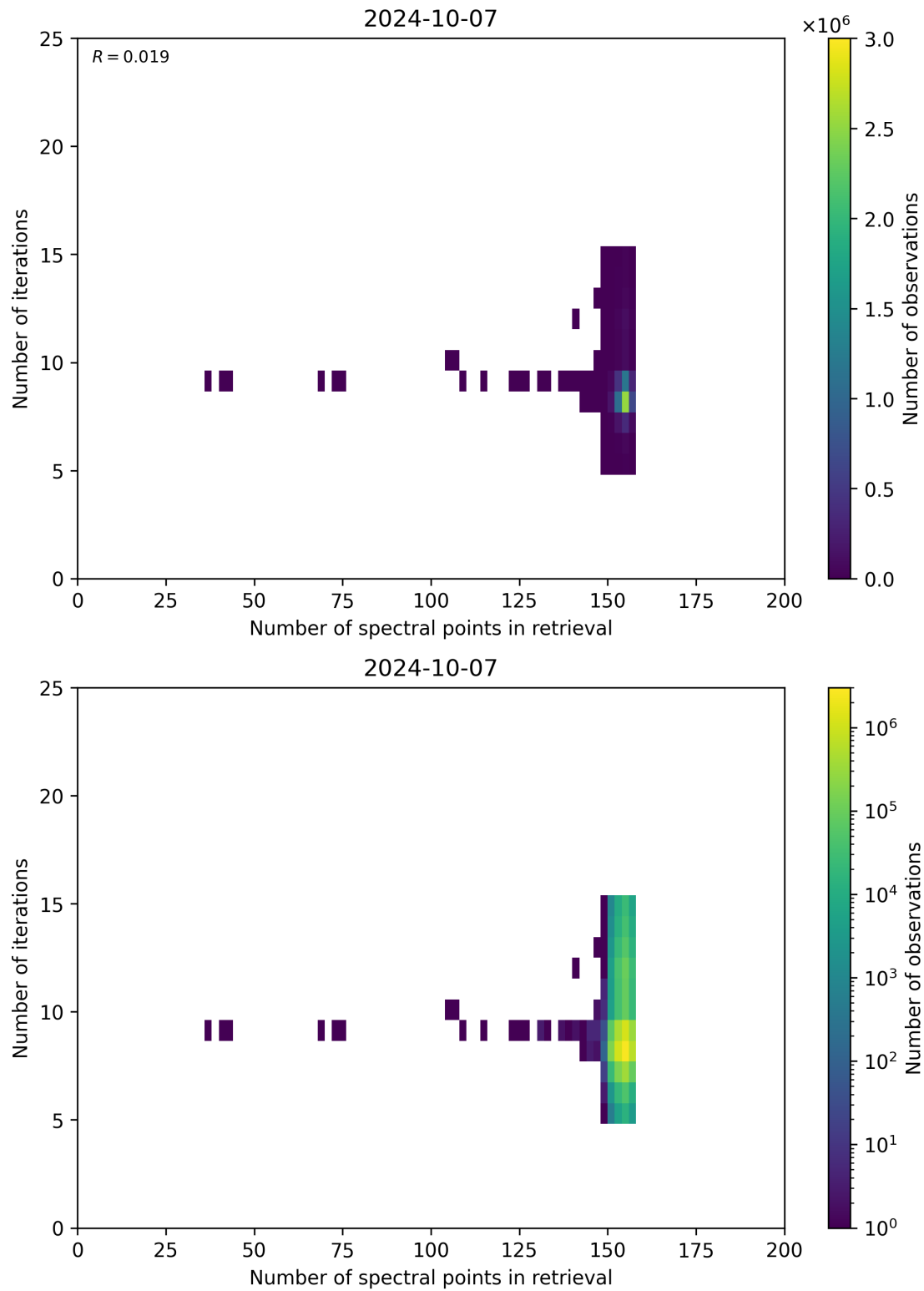
Figure 60: Scatter density plot of “Number of spectral points in retrieval” against “Number of iterations” for 2024-10-06 to 2024-10-08.
