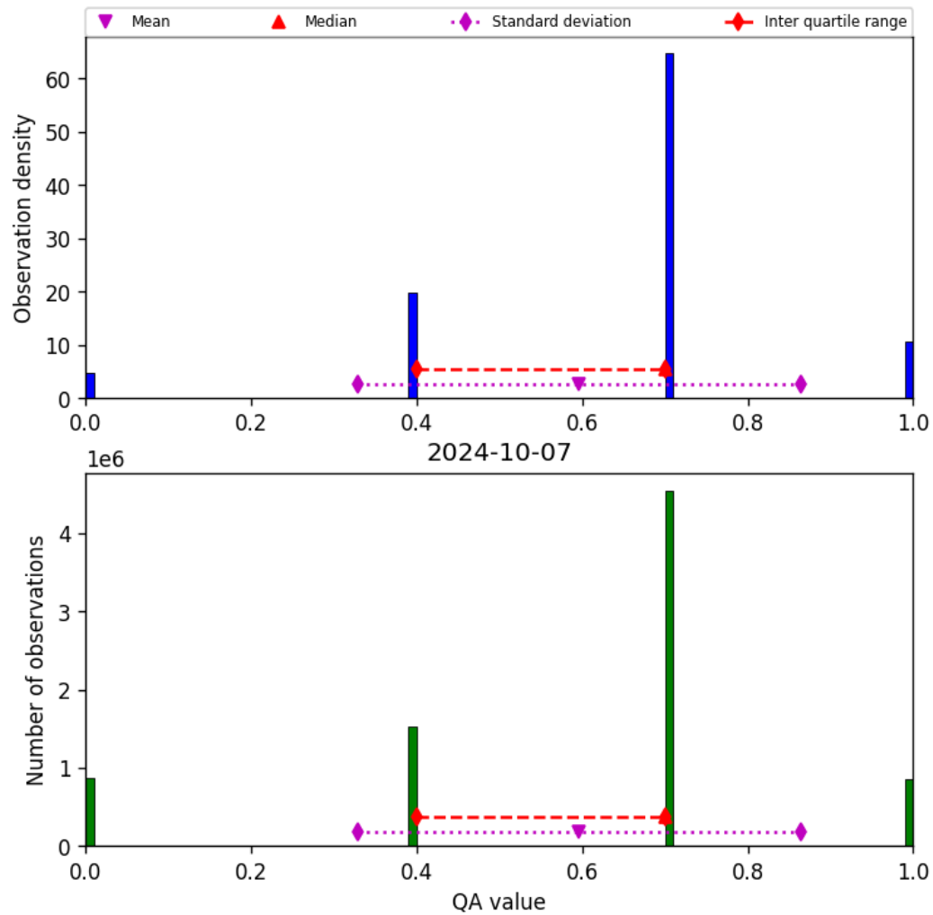
Figure 17: Histogram of “QA value” for 2024-10-06 to 2024-10-08
