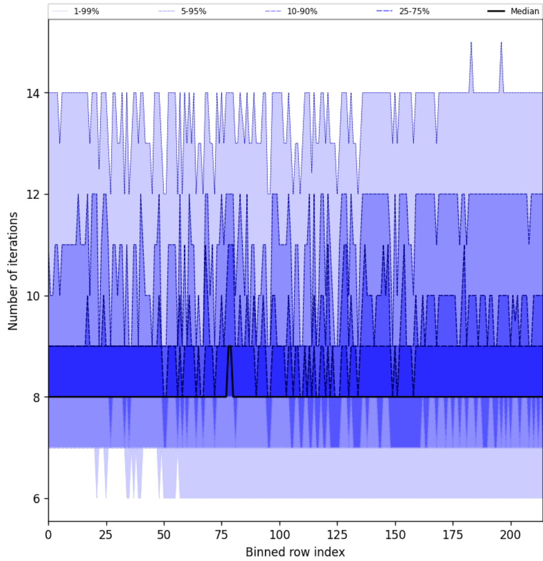
Figure 32: Along track statistics of “Number of iterations” for 2024-10-06 to 2024-10-08
