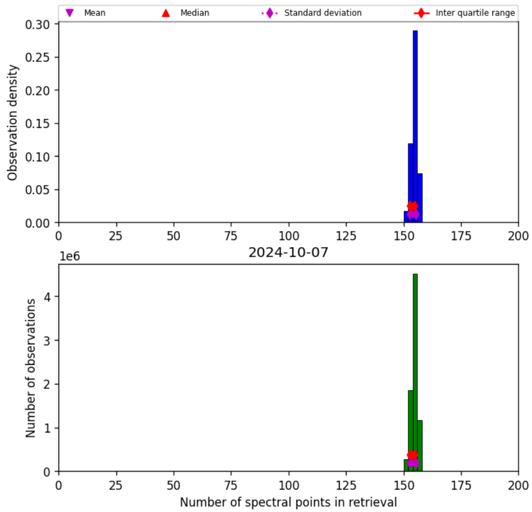
Figure 21: Histogram of “Number of spectral points in retrieval” for 2024-10-06 to 2024-10-08
