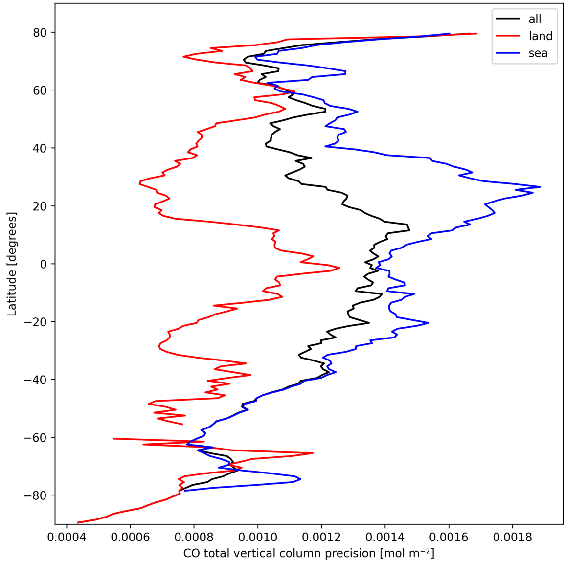
Figure 12: Zonal average of “CO total vertical column precision” for 2024-10-06 to 2024-10-08.
