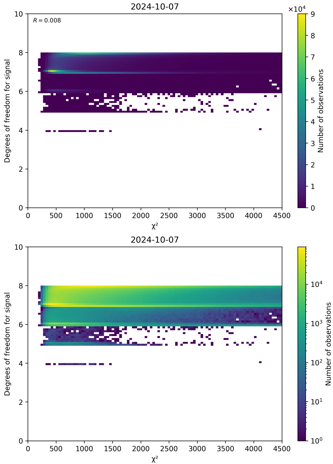
Figure 48: Scatter density plot of “ \chi^2 ” against “Degrees of freedom for signal” for 2024-10-06 to 2024-10-08.
