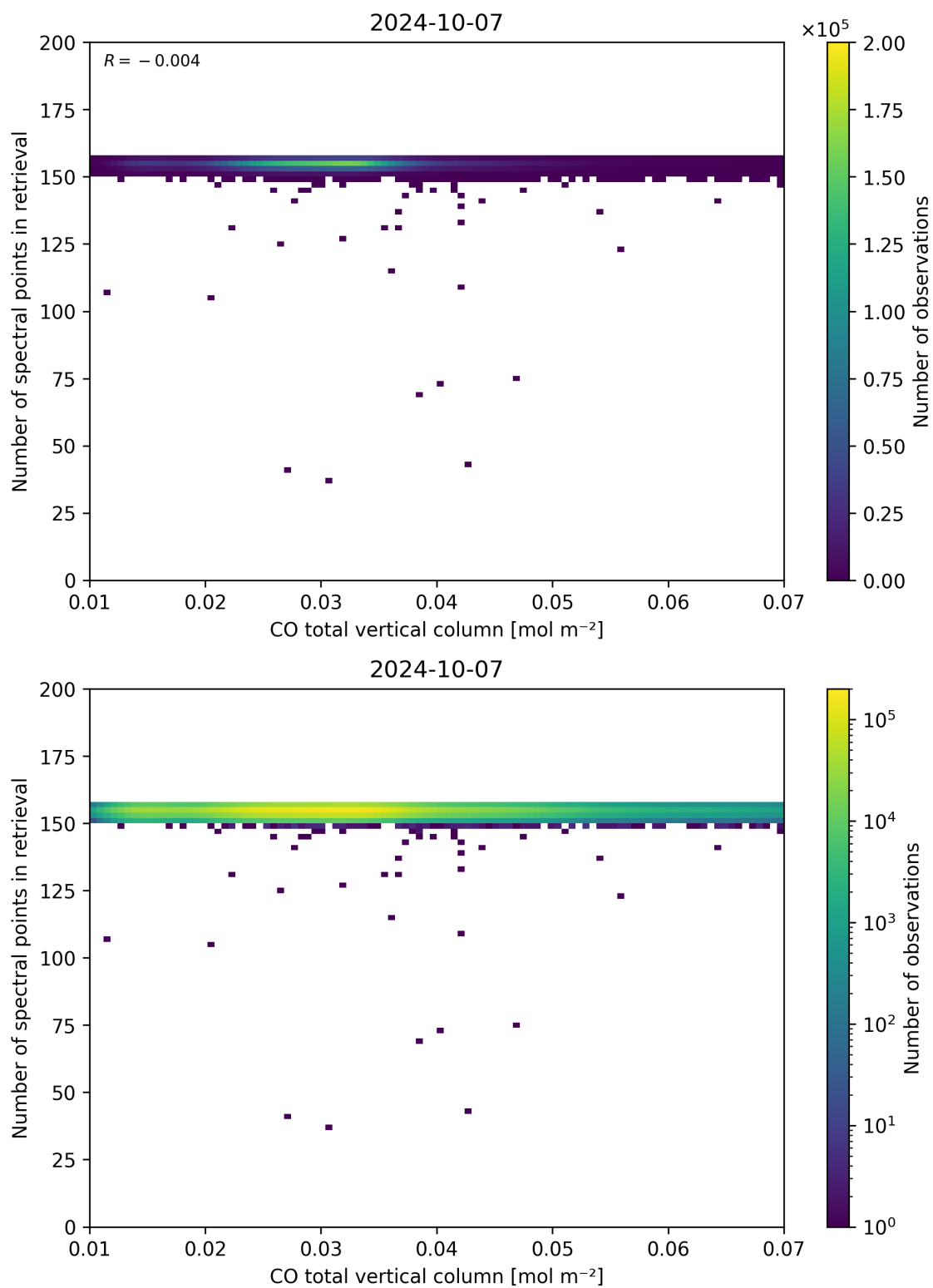
Figure 43: Scatter density plot of “CO total vertical column” against “Number of spectral points in retrieval” for 2024-10-06 to 2024-10-08.
