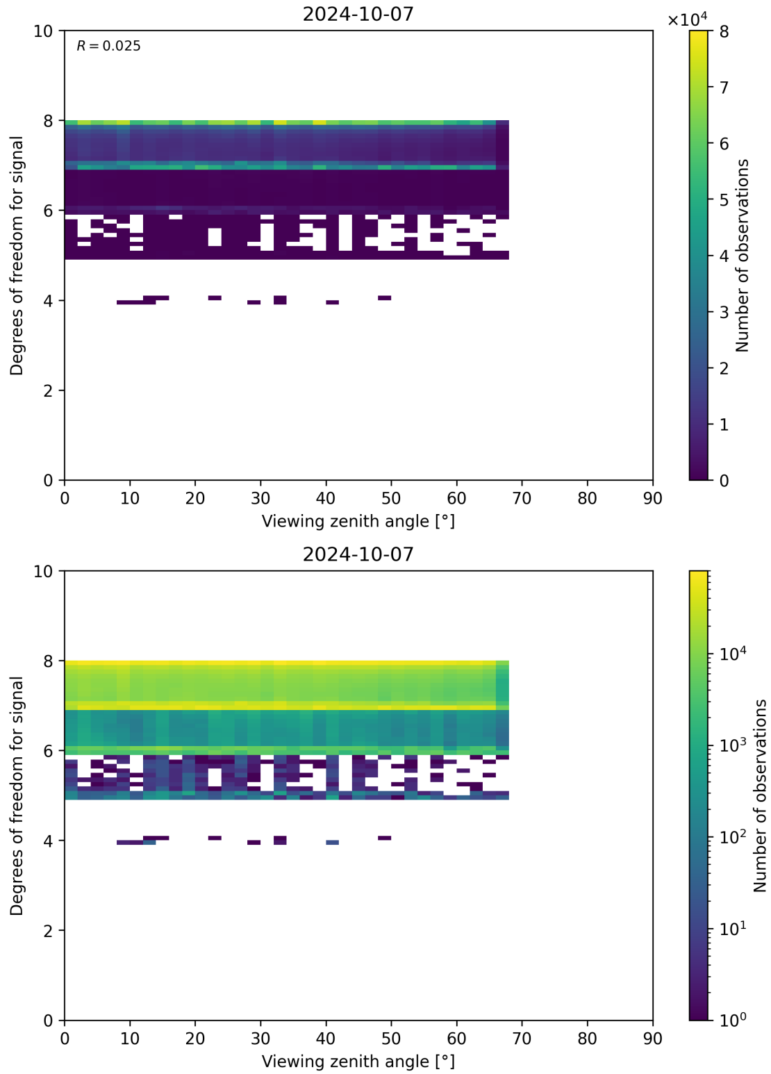
Figure 73: Scatter density plot of “Viewing zenith angle” against “Degrees of freedom for signal” for 2024-10-06 to 2024-10-08.
