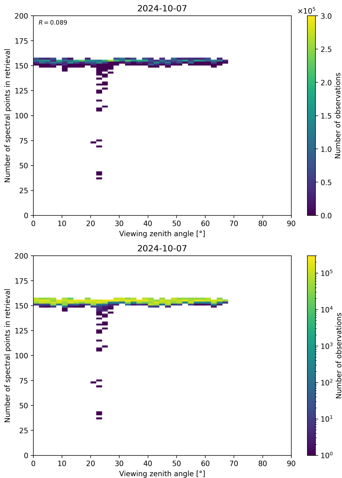
Figure 76: Scatter density plot of “Viewing zenith angle” against “Number of spectral points in retrieval” for 2024-10-06 to 2024-10-08.
