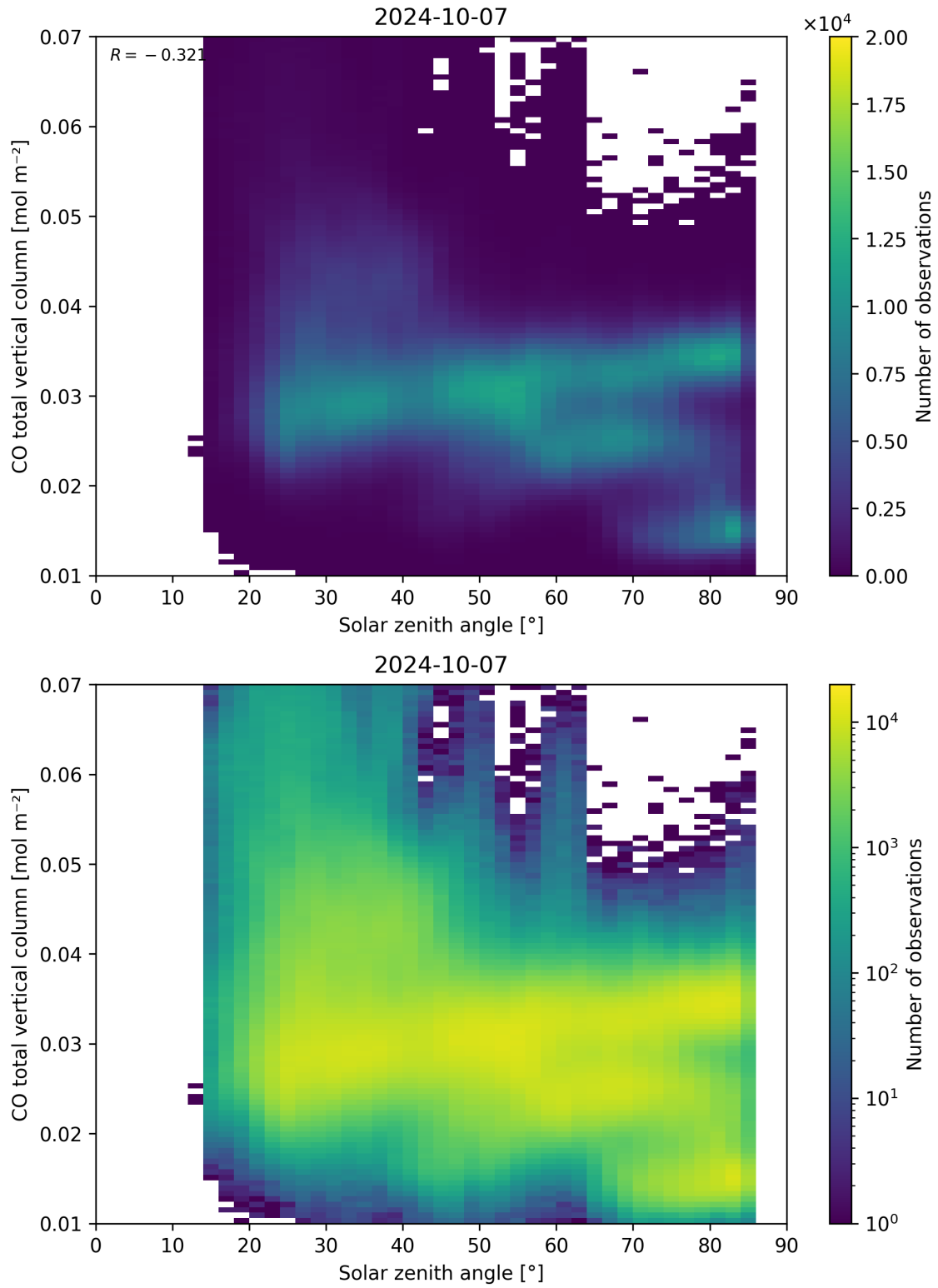
Figure 61: Scatter density plot of “Solar zenith angle” against “CO total vertical column” for 2024-10-06 to 2024-10-08.
