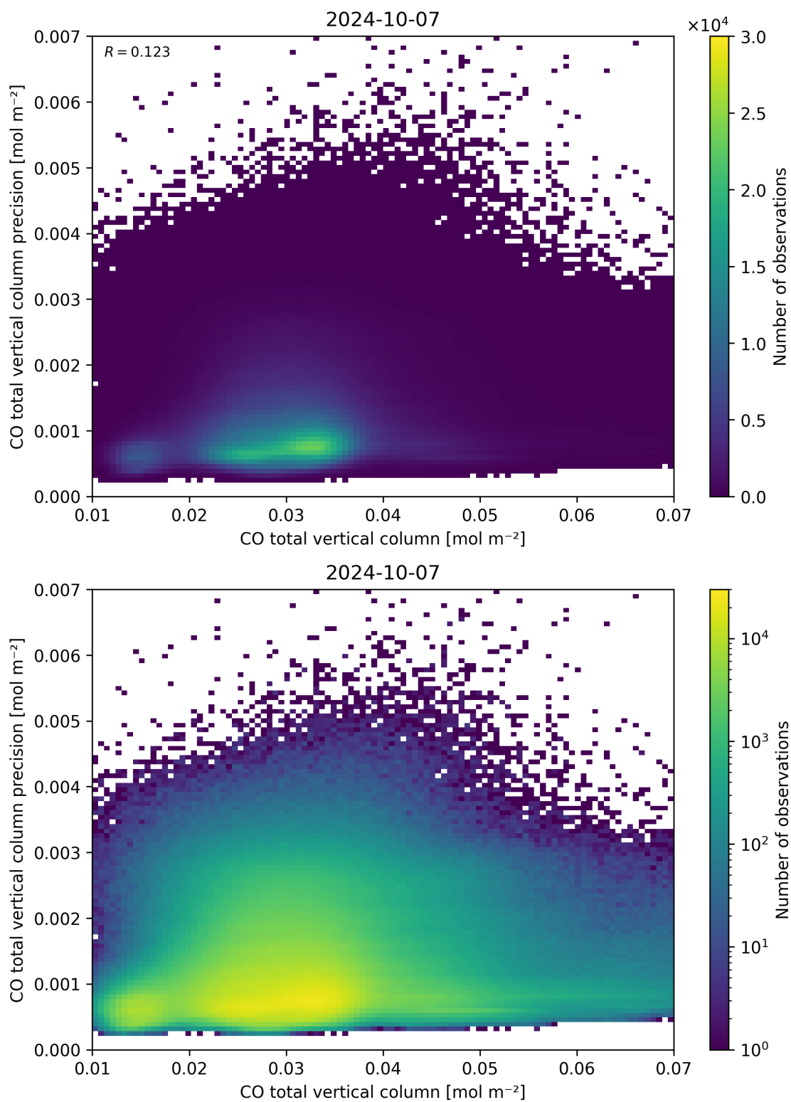
Figure 34: Scatter density plot of “CO total vertical column” against “CO total vertical column precision” for 2024-10-06 to 2024-10-08.
