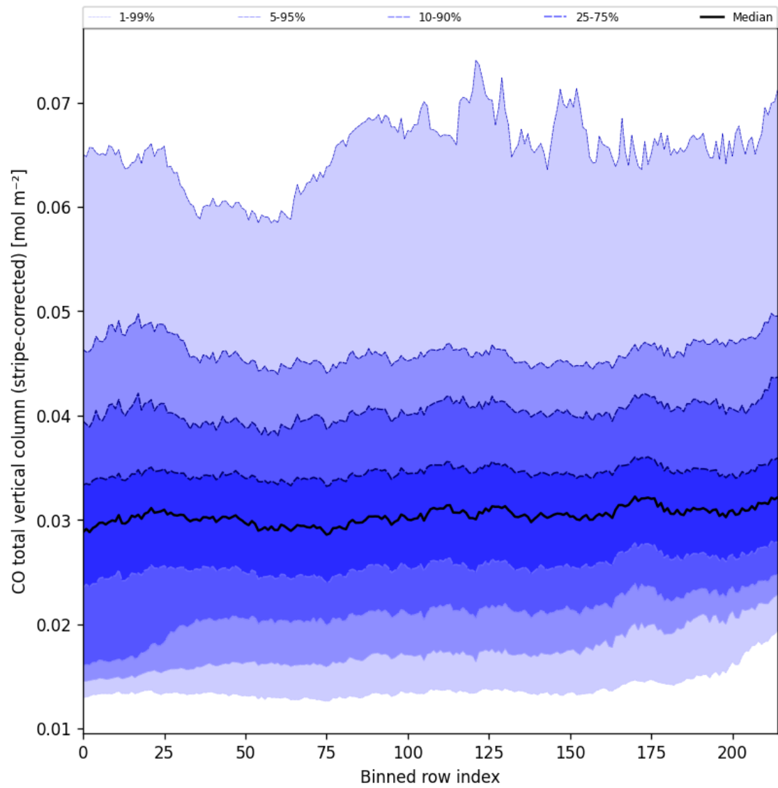
Figure 27: Along track statistics of “CO total vertical column (stripe-corrected)” for 2024-10-06 to 2024-10-08
