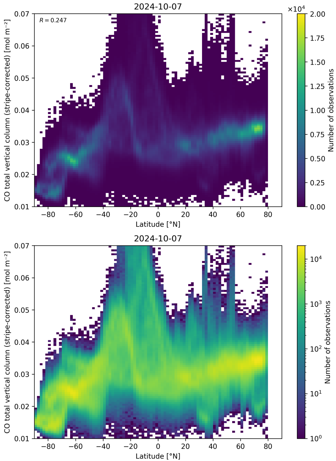
Figure 52: Scatter density plot of “Latitude” against “CO total vertical column (stripe-corrected)” for 2024-10-06 to 2024-10-08.
