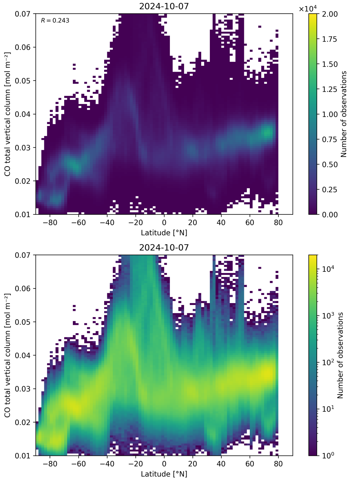
Figure 51: Scatter density plot of “Latitude” against “CO total vertical column” for 2024-10-06 to 2024-10-08.
