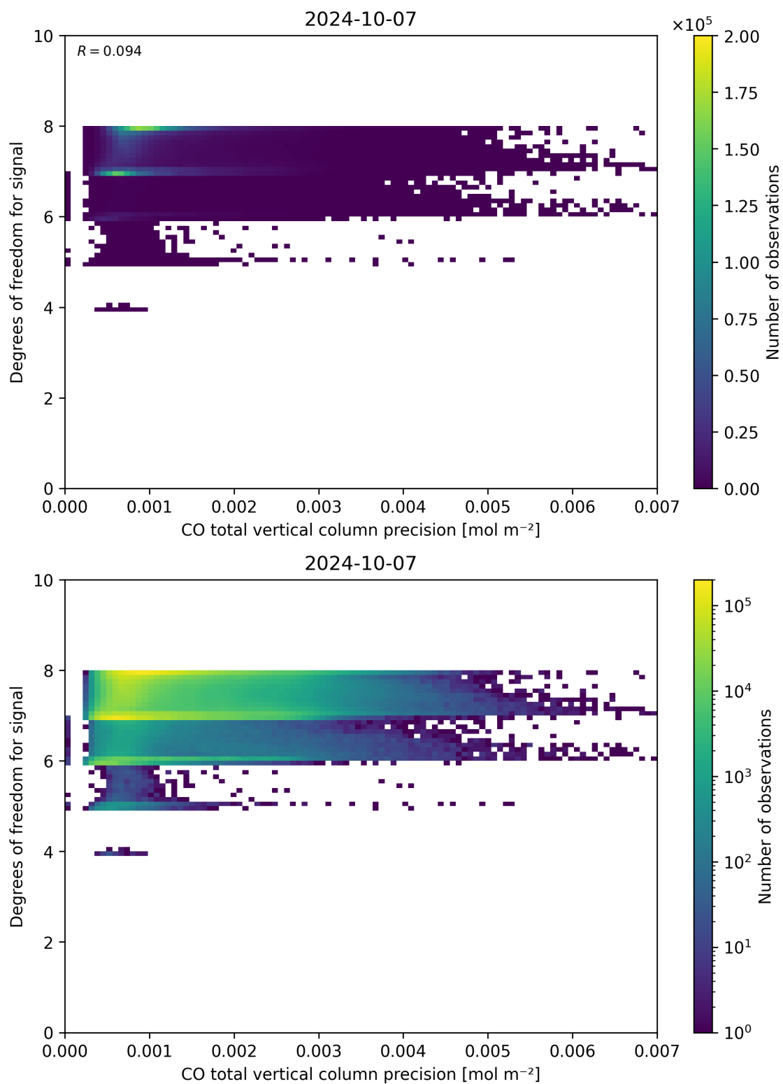
Figure 45: Scatter density plot of “CO total vertical column precision” against “Degrees of freedom for signal” for 2024-10-06 to 2024-10-08.
