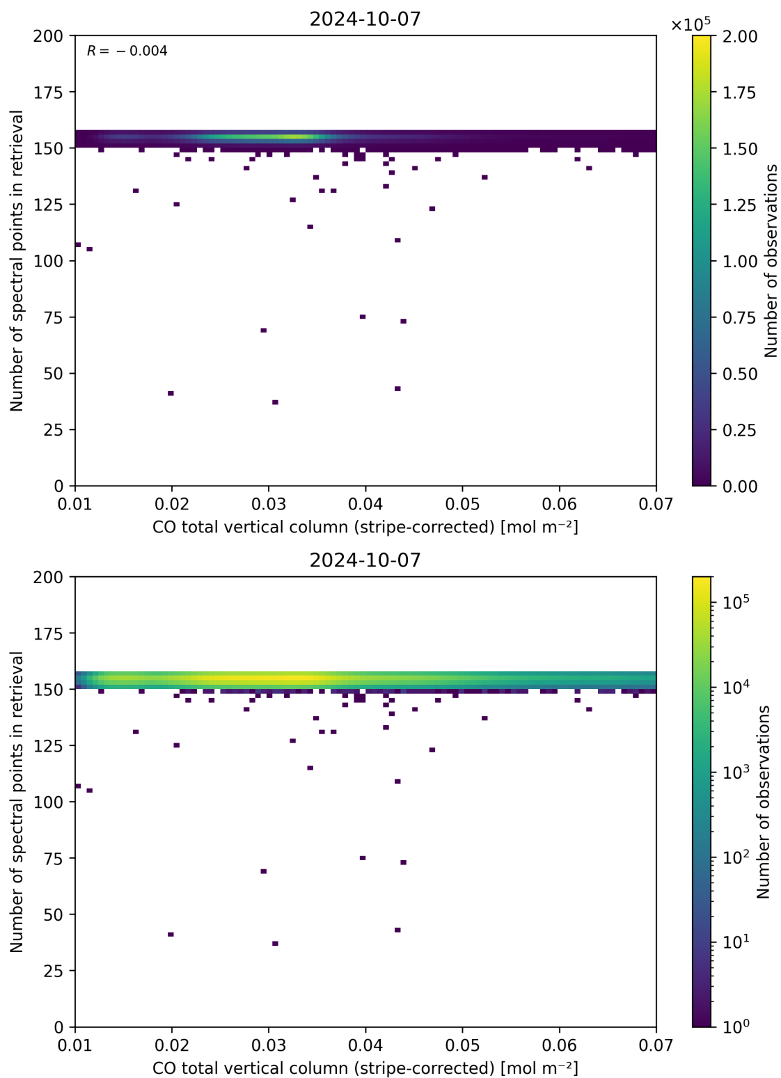
Figure 40: Scatter density plot of “CO total vertical column (stripe-corrected)” against “Number of spectral points in retrieval” for 2024-10-06 to 2024-10-08.
