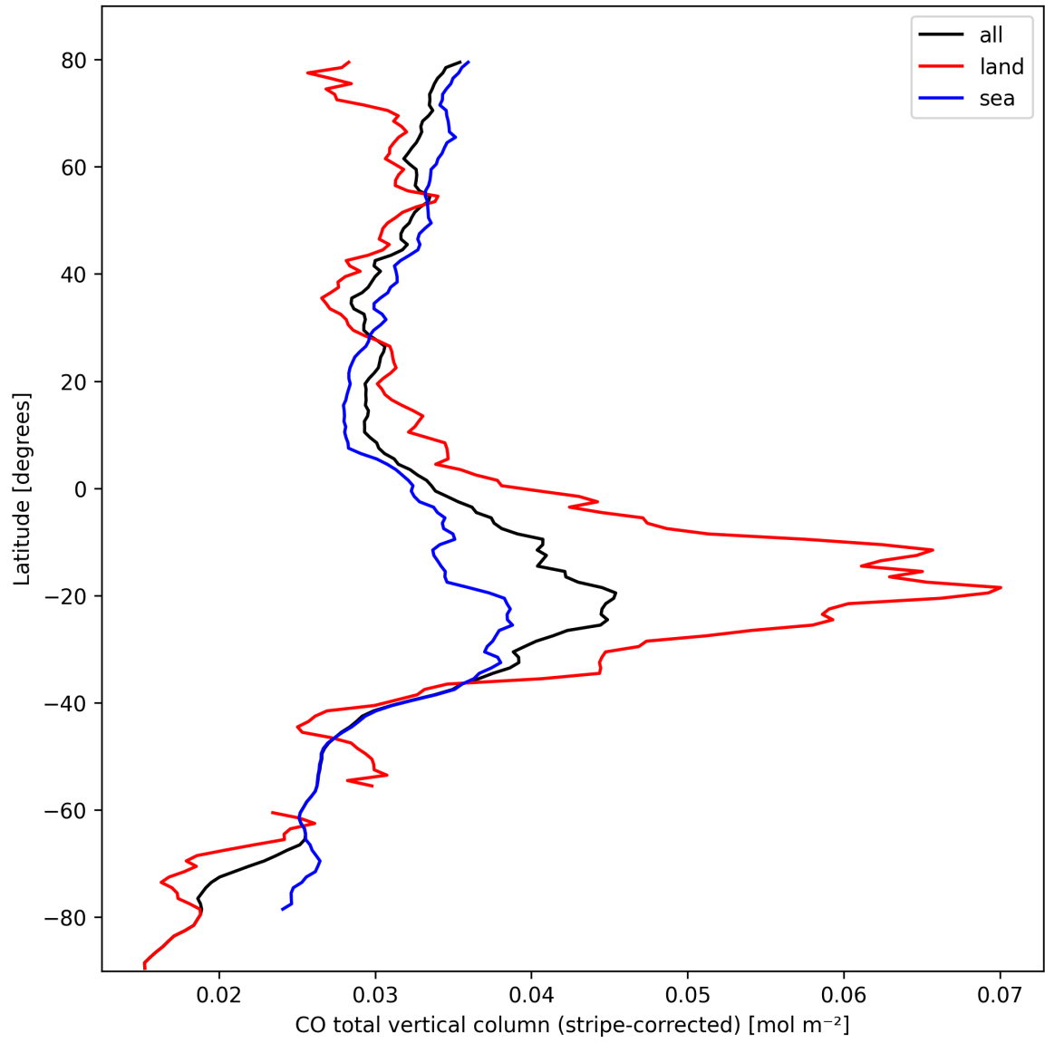
Figure 11: Zonal average of “CO total vertical column (stripe-corrected)” for 2024-10-06 to 2024-10-08.
