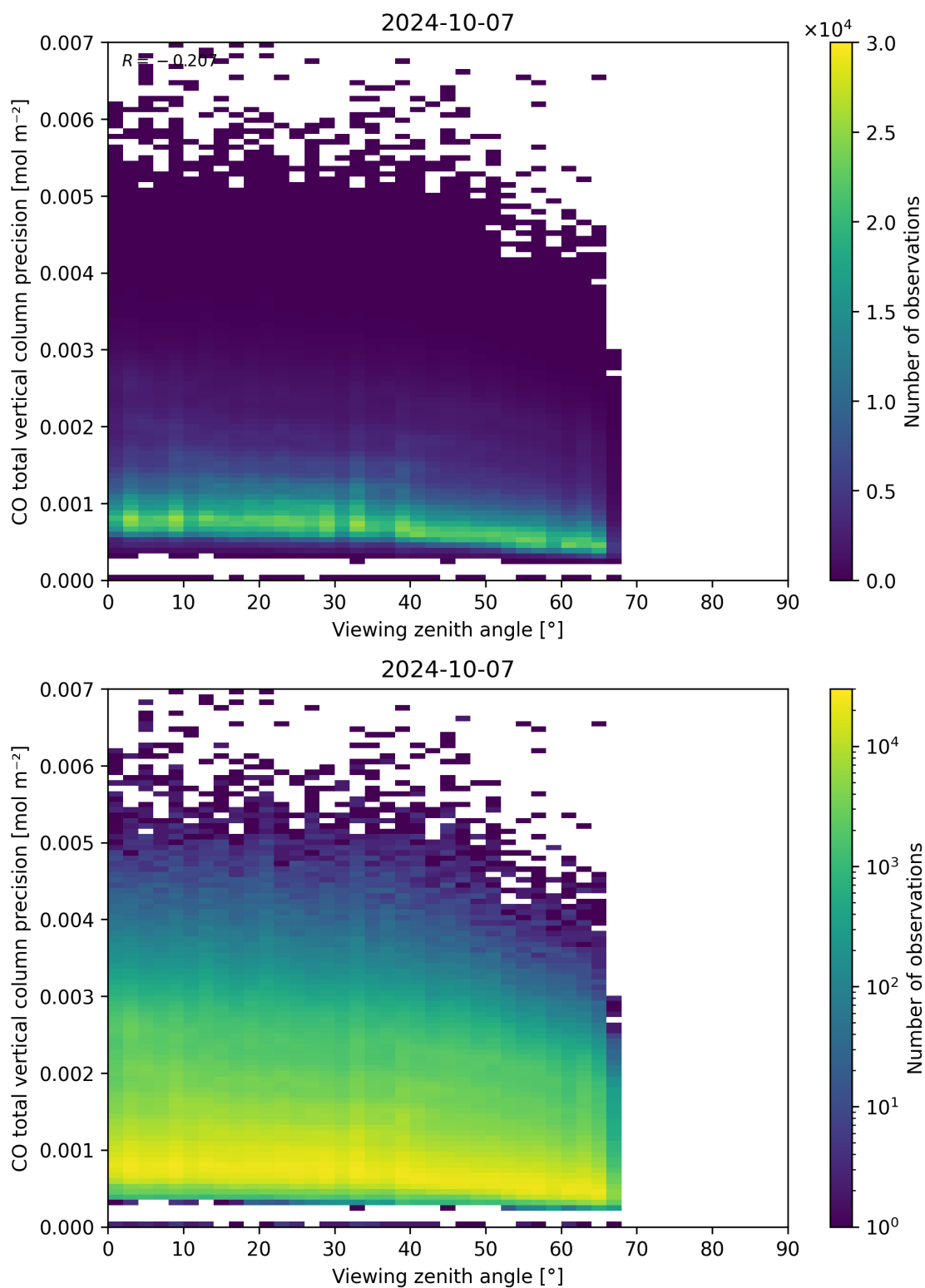
Figure 71: Scatter density plot of “Viewing zenith angle” against “CO total vertical column precision” for 2024-10-06 to 2024-10-08.
