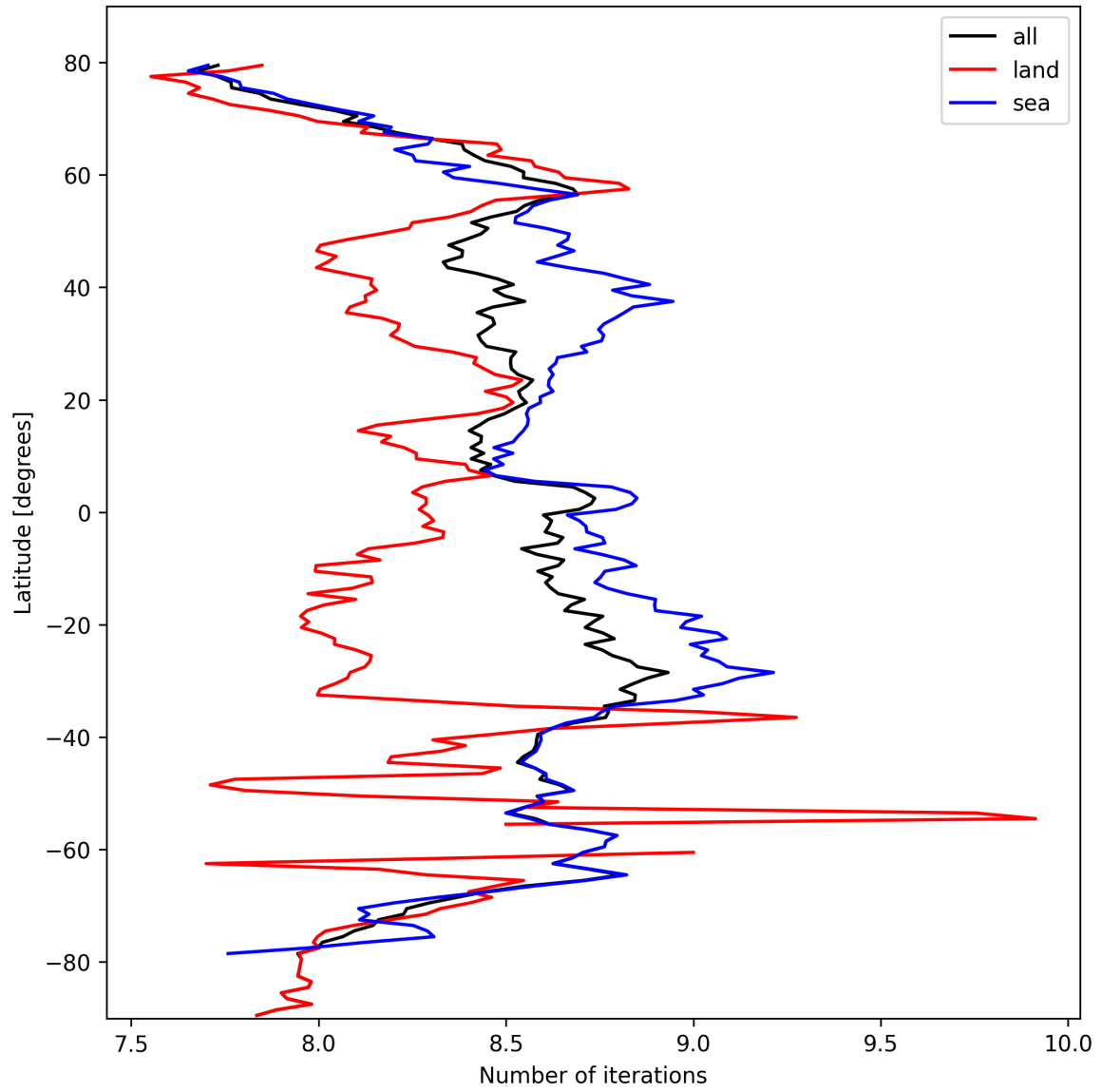
Figure 16: Zonal average of “Number of iterations” for 2024-10-06 to 2024-10-08.
