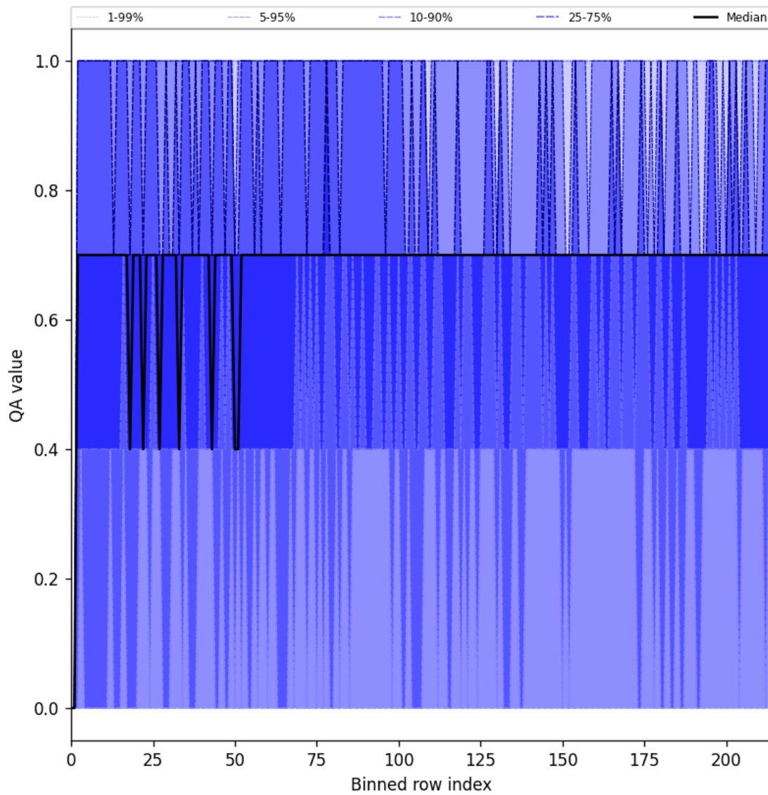
Figure 25: Along track statistics of “QA value” for 2024-10-06 to 2024-10-08
