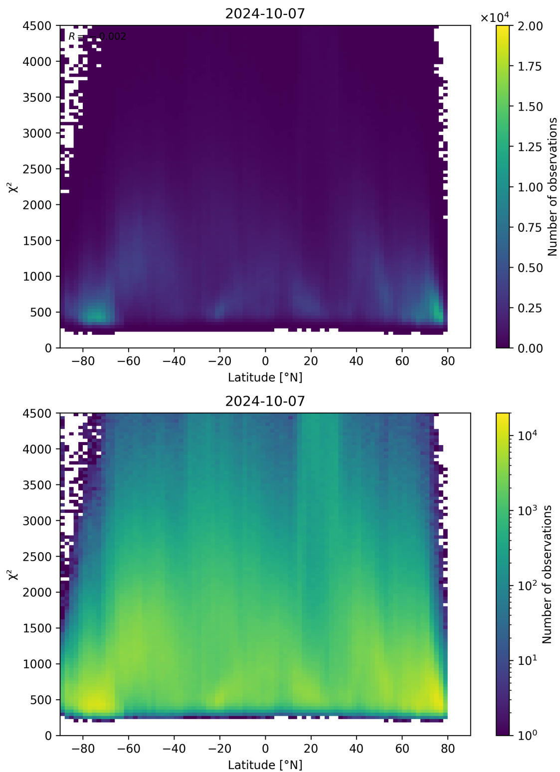
Figure 54: Scatter density plot of “Latitude” against “ \chi^2 ” for 2024-10-06 to 2024-10-08.
