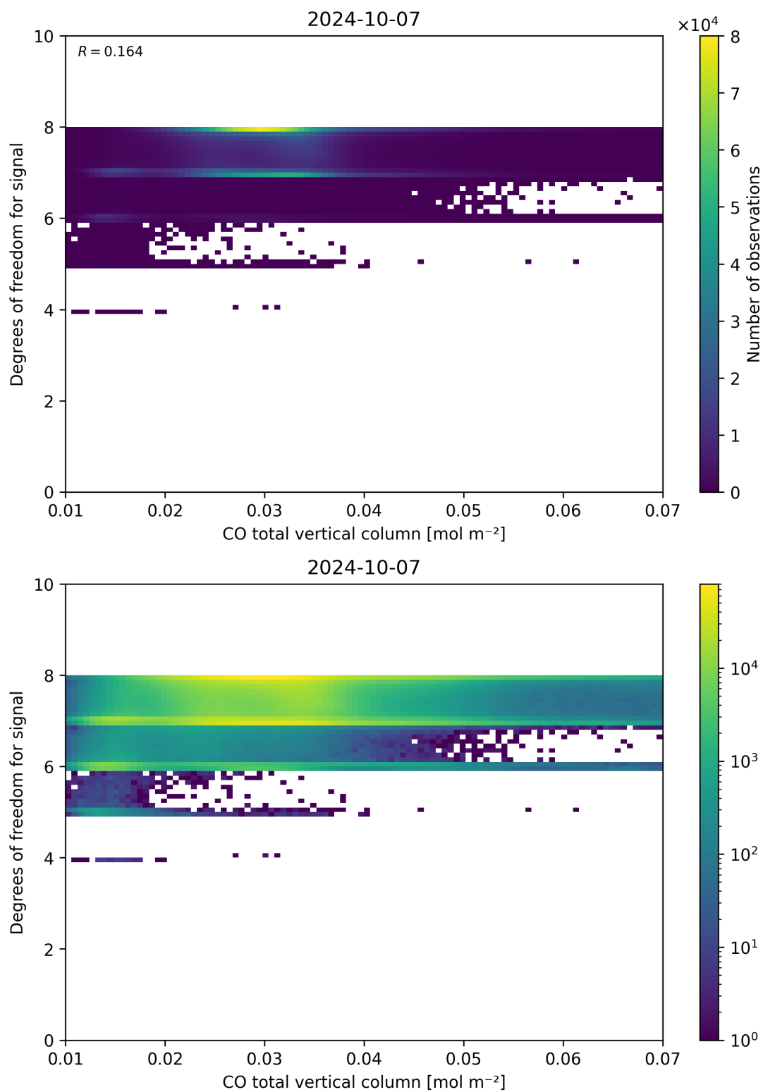
Figure 41: Scatter density plot of “CO total vertical column” against “Degrees of freedom for signal” for 2024-10-06 to 2024-10-08.
