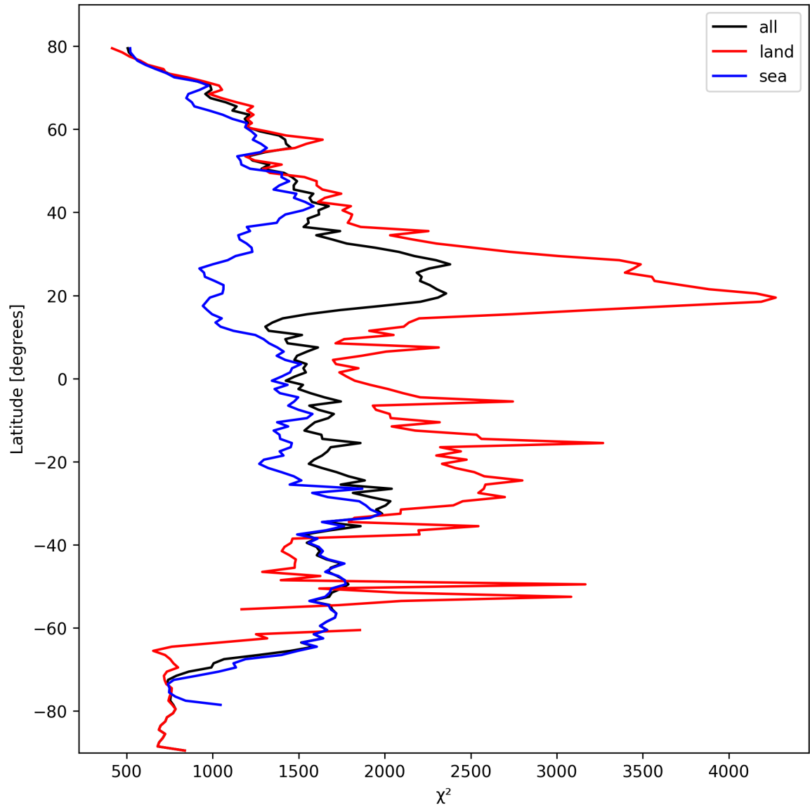
Figure 14: Zonal average of “ \chi^2 ” for 2024-10-06 to 2024-10-08.
