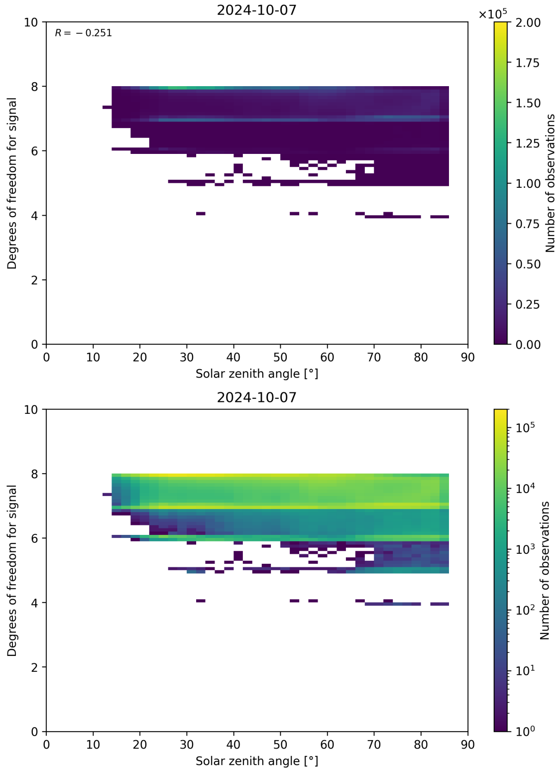
Figure 65: Scatter density plot of “Solar zenith angle” against “Degrees of freedom for signal” for 2024-10-06 to 2024-10-08.
