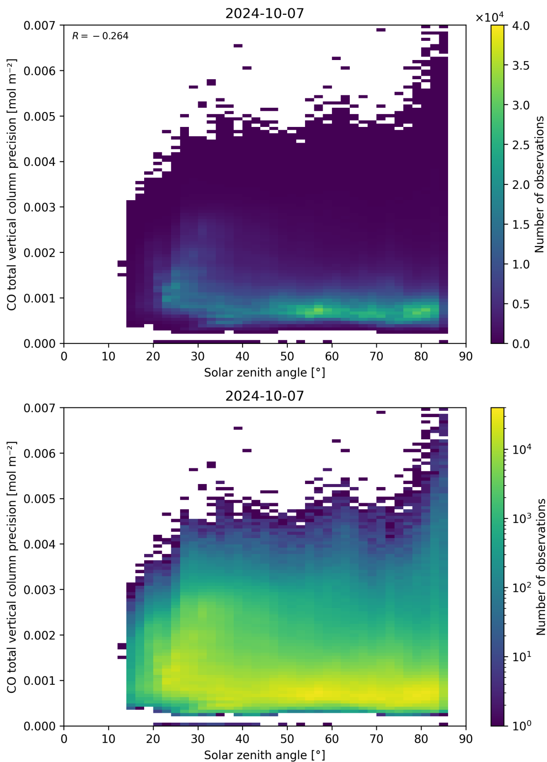
Figure 63: Scatter density plot of “Solar zenith angle” against “CO total vertical column precision” for 2024-10-06 to 2024-10-08.
