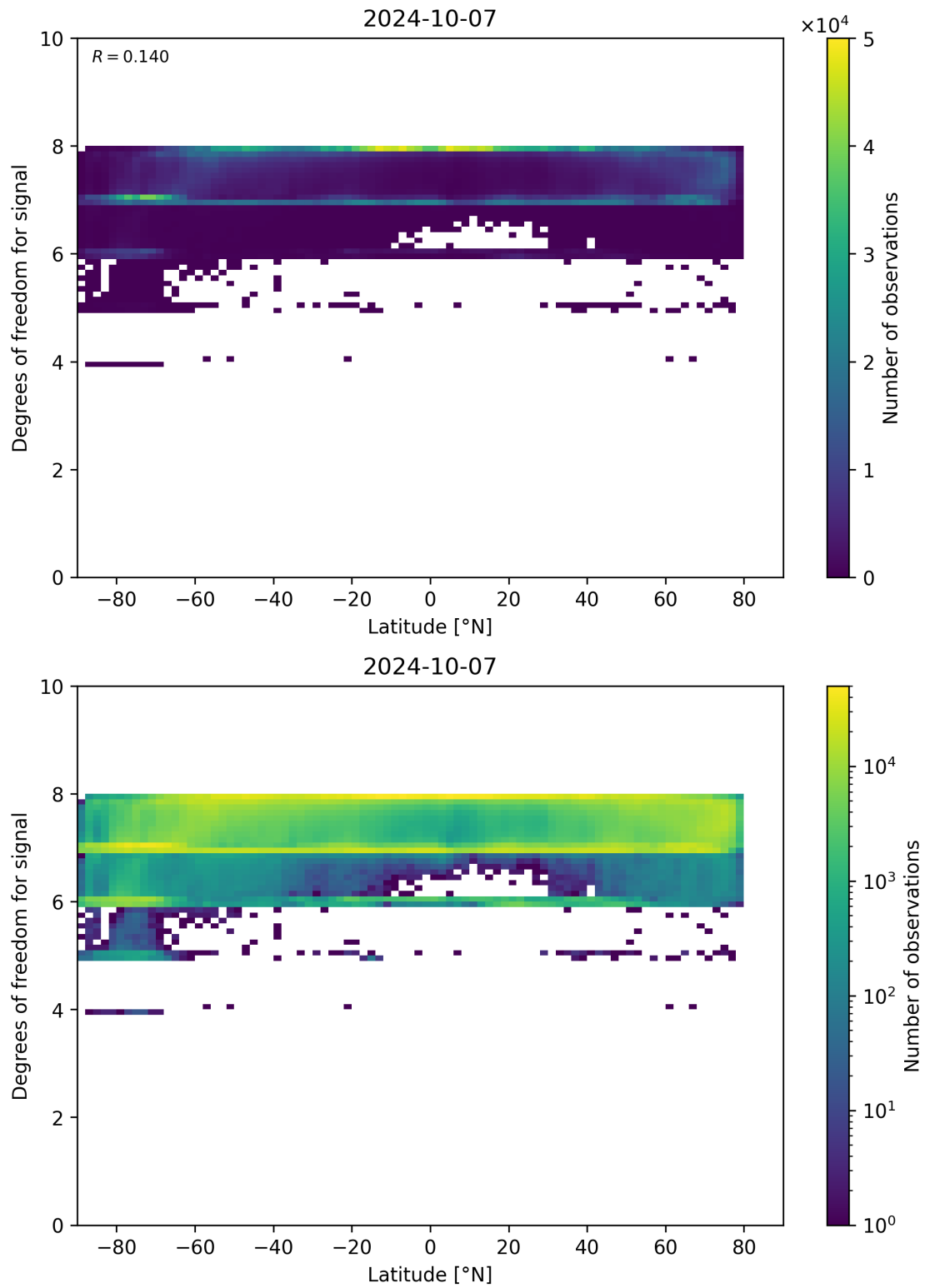
Figure 55: Scatter density plot of “Latitude” against “Degrees of freedom for signal” for 2024-10-06 to 2024-10-08.
