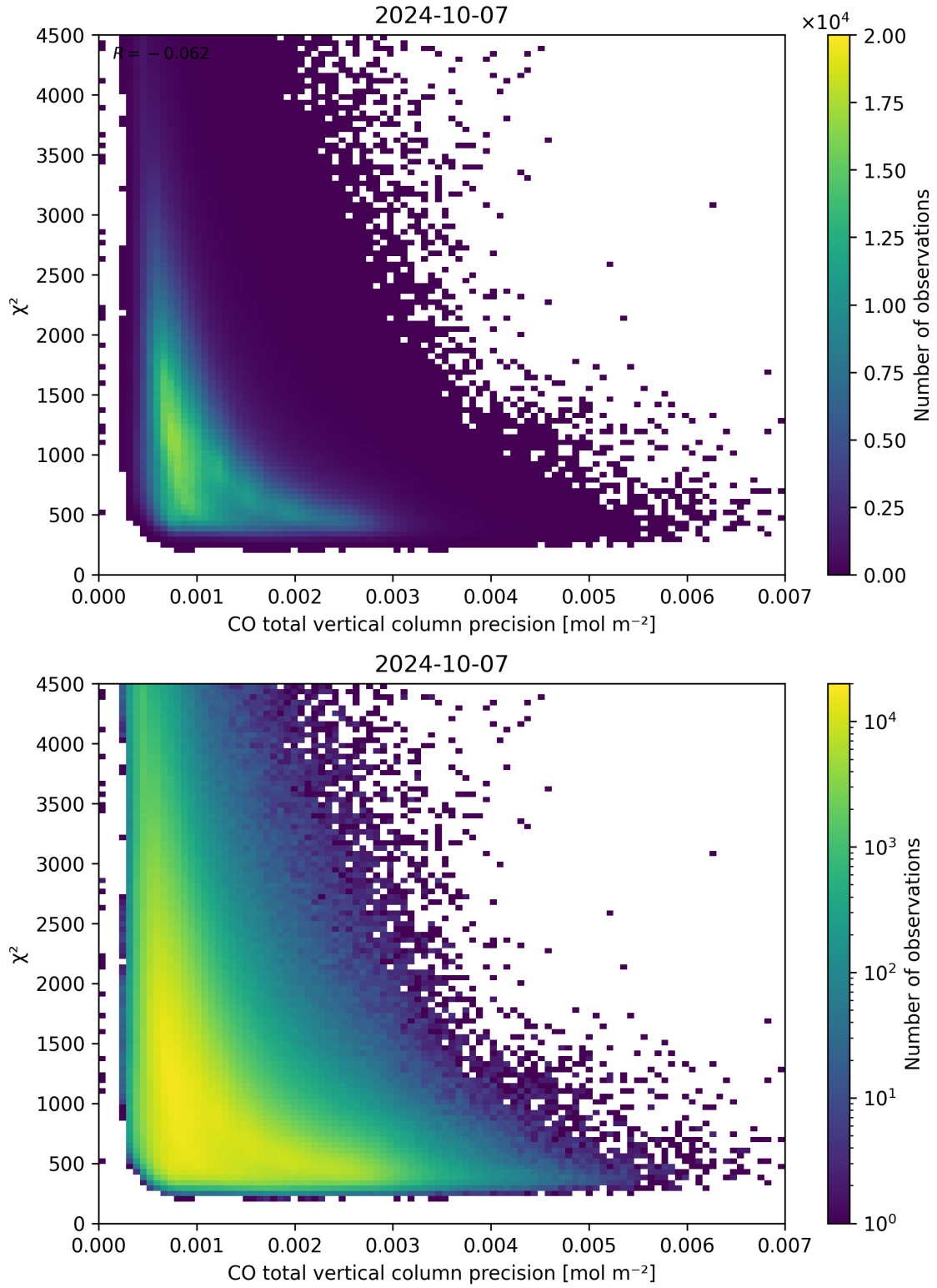
Figure 44: Scatter density plot of “CO total vertical column precision” against “ \chi^2 ” for 2024-10-06 to 2024-10-08.
