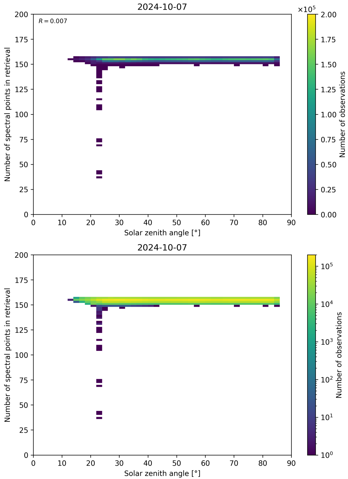
Figure 68: Scatter density plot of “Solar zenith angle” against “Number of spectral points in retrieval” for 2024-10-06 to 2024-10-08.
