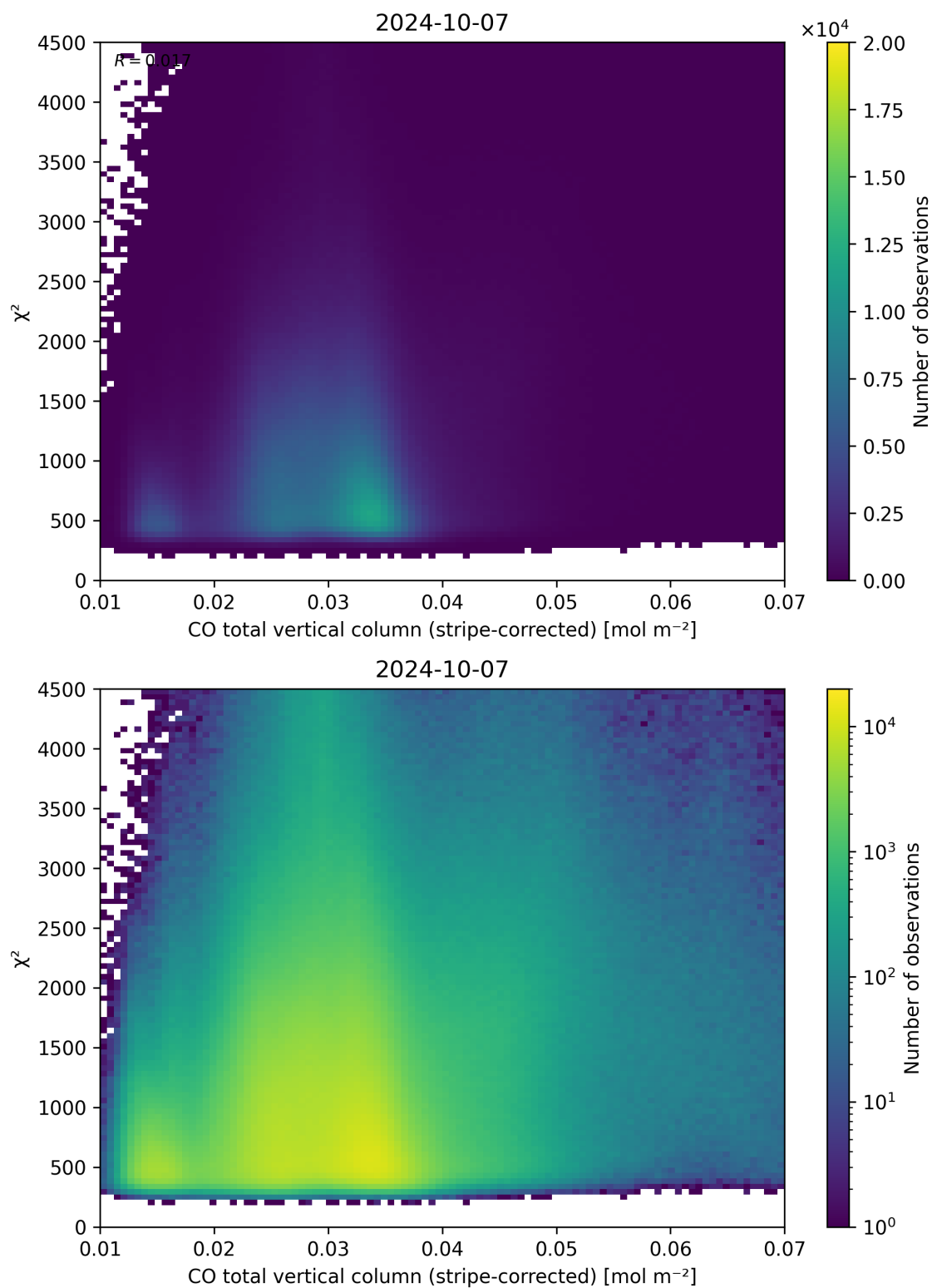
Figure 37: Scatter density plot of “CO total vertical column (stripe-corrected)” against “ \chi^2 ” for 2024-10-06 to 2024-10-08.
