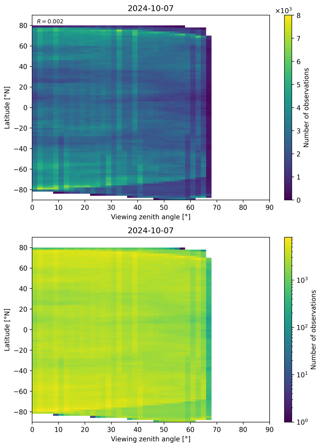
Figure 74: Scatter density plot of “Viewing zenith angle” against “Latitude” for 2024-10-06 to 2024-10-08.
