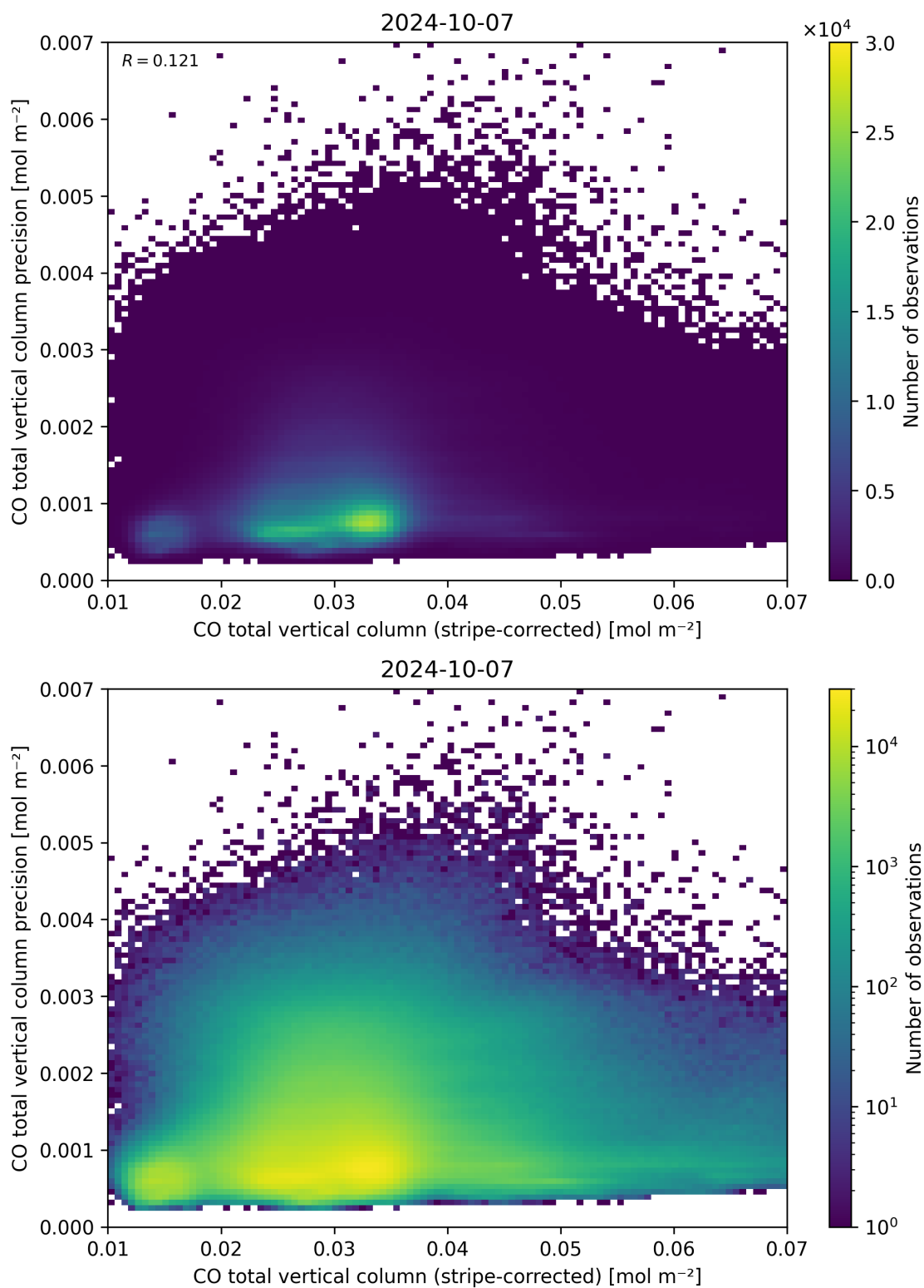
Figure 36: Scatter density plot of “CO total vertical column (stripe-corrected)” against “CO total vertical column precision” for 2024-10-06 to 2024-10-08.
