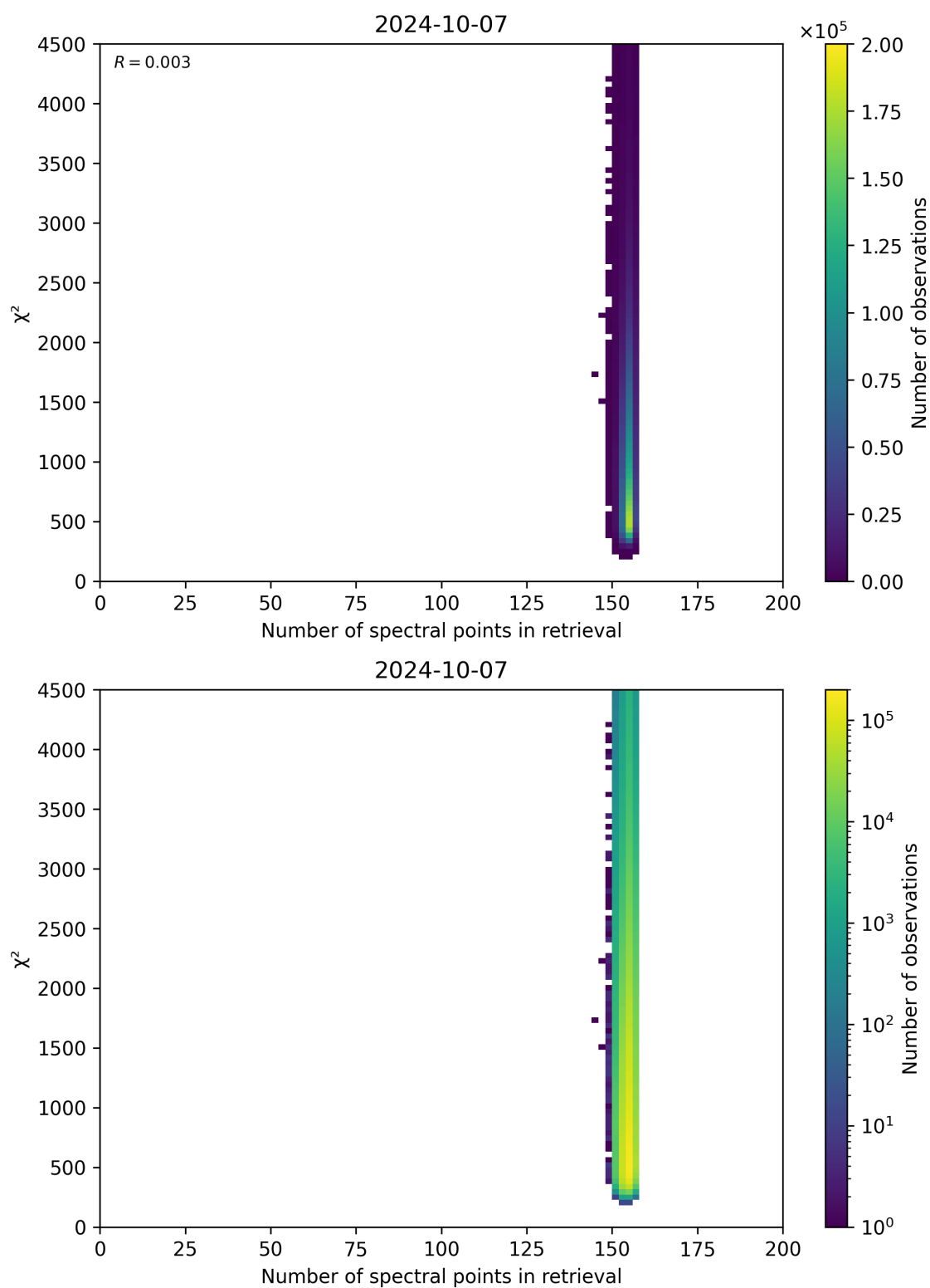
Figure 58: Scatter density plot of “Number of spectral points in retrieval” against “ \chi^2 ” for 2024-10-06 to 2024-10-08.
