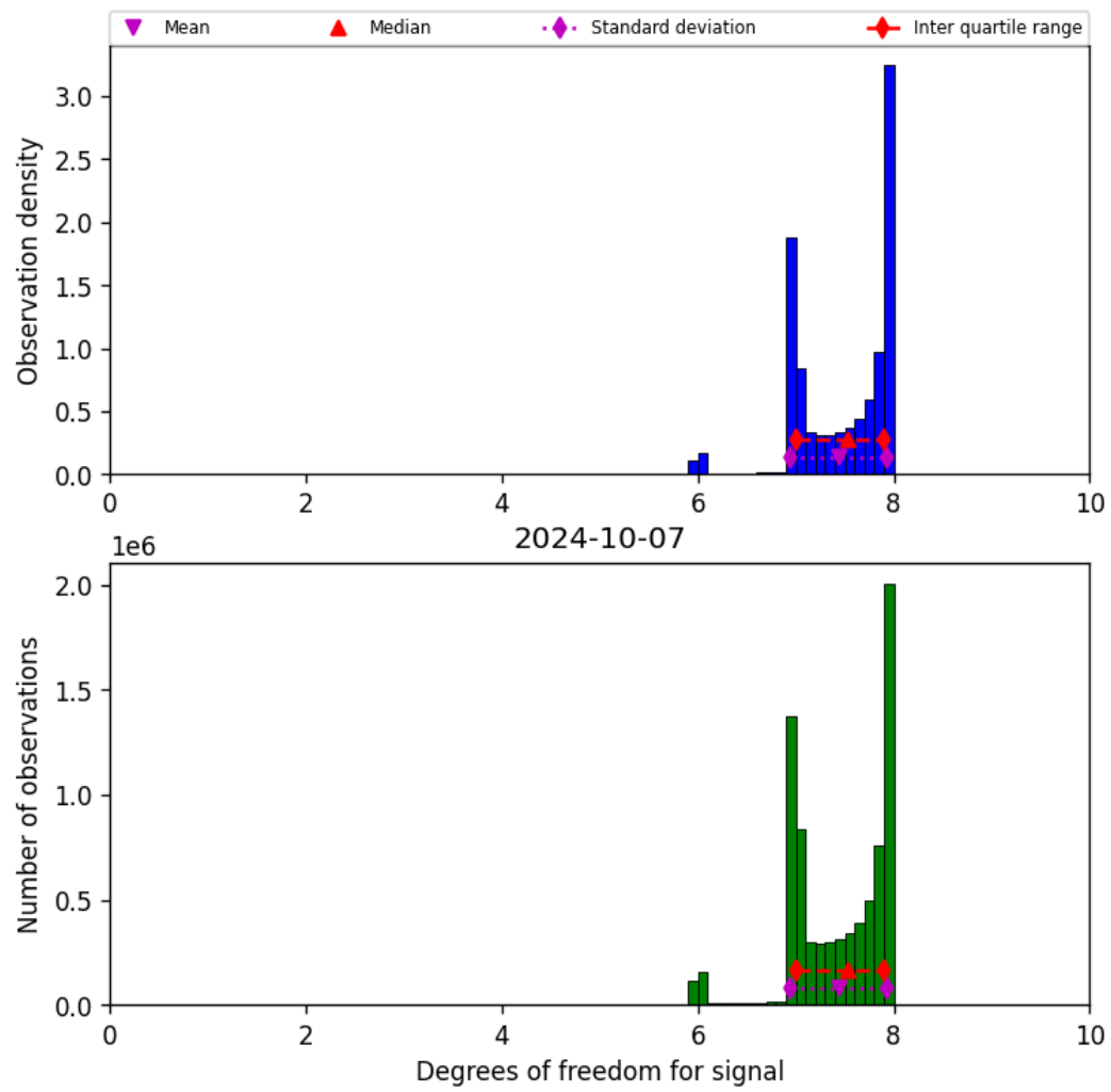
Figure 23: Histogram of “Degrees of freedom for signal” for 2024-10-06 to 2024-10-08
