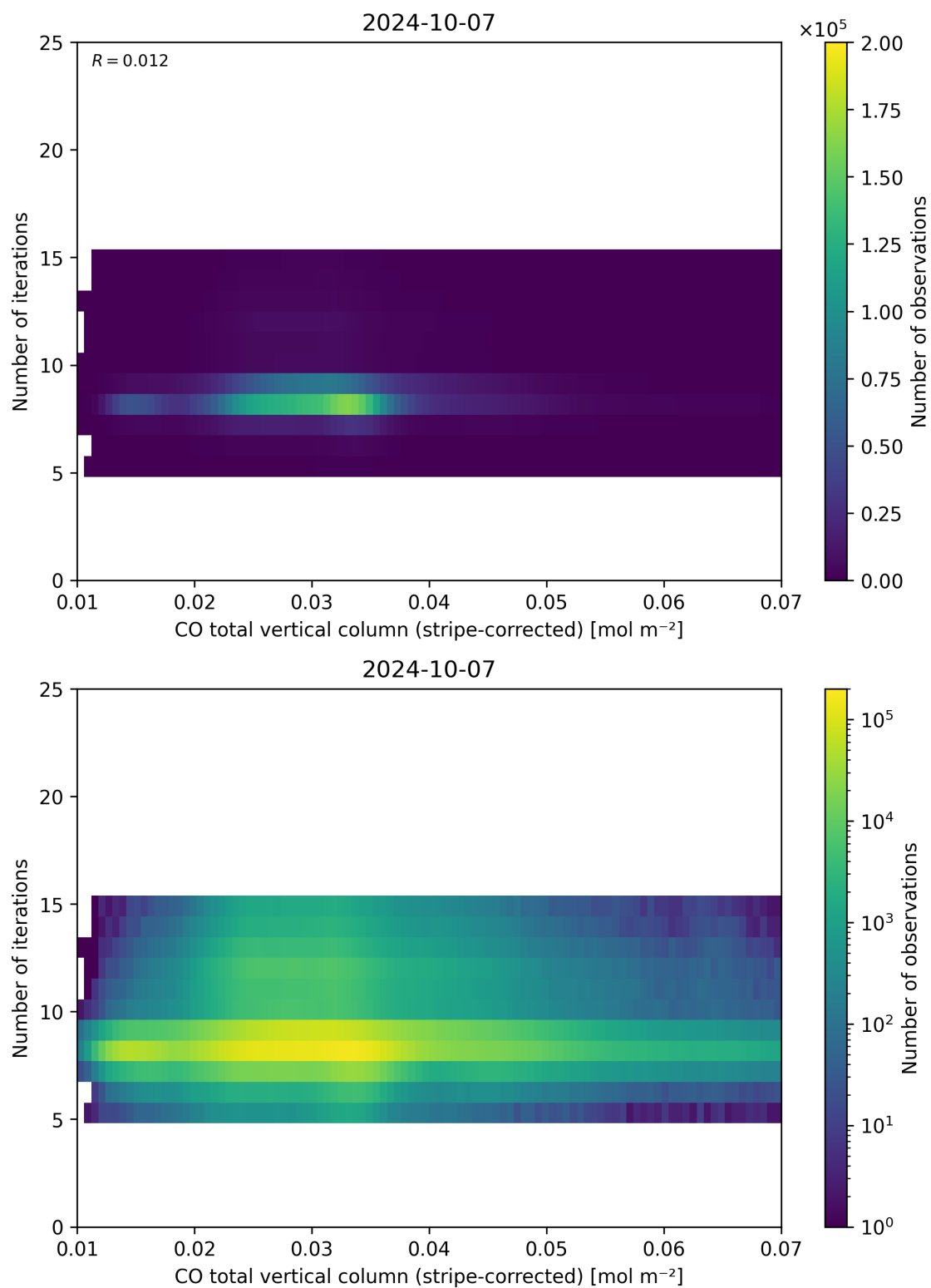
Figure 39: Scatter density plot of “CO total vertical column (stripe-corrected)” against “Number of iterations” for 2024-10-06 to 2024-10-08.
