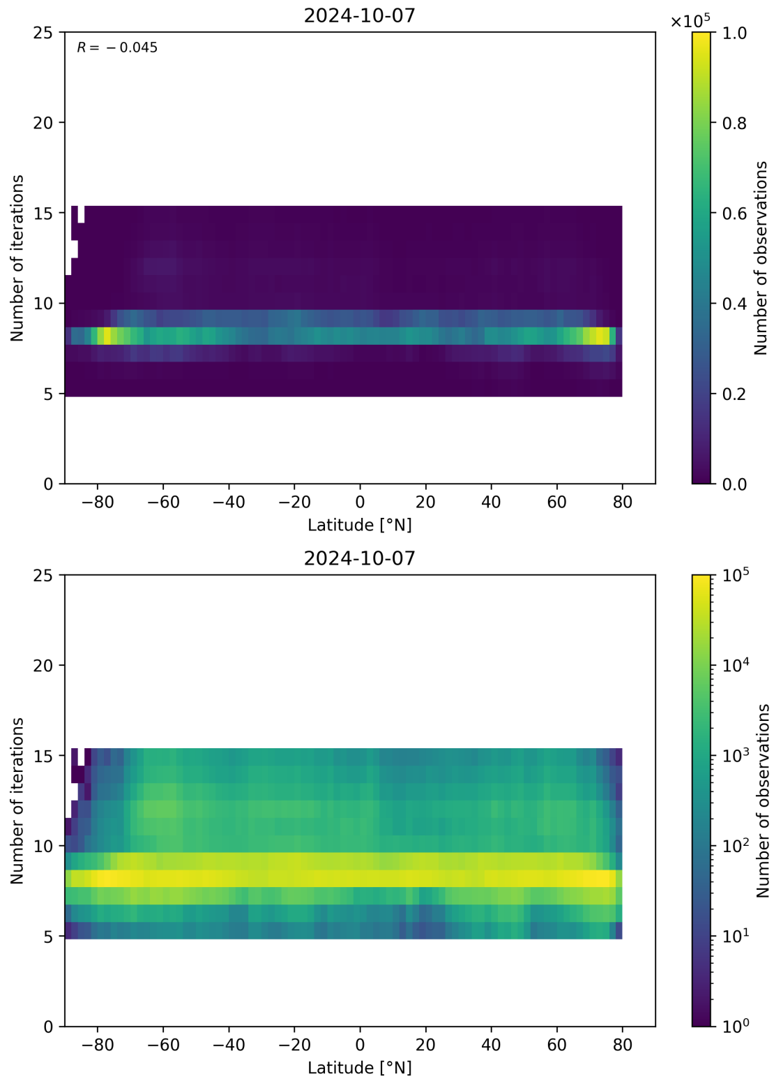
Figure 56: Scatter density plot of “Latitude” against “Number of iterations” for 2024-10-06 to 2024-10-08.
