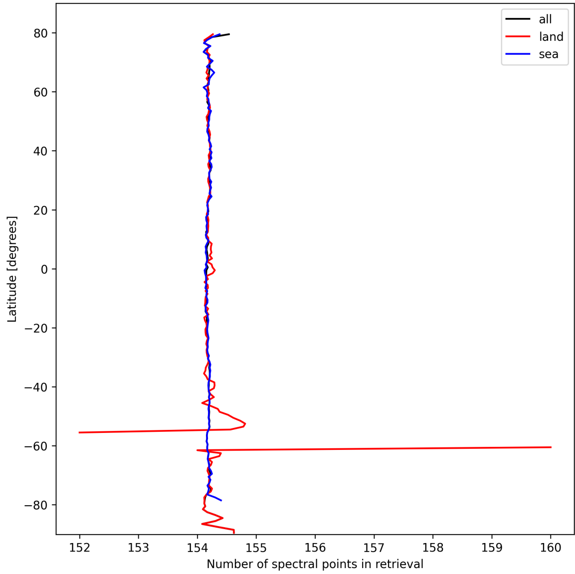
Figure 13: Zonal average of “Number of spectral points in retrieval” for 2024-10-06 to 2024-10-08.
