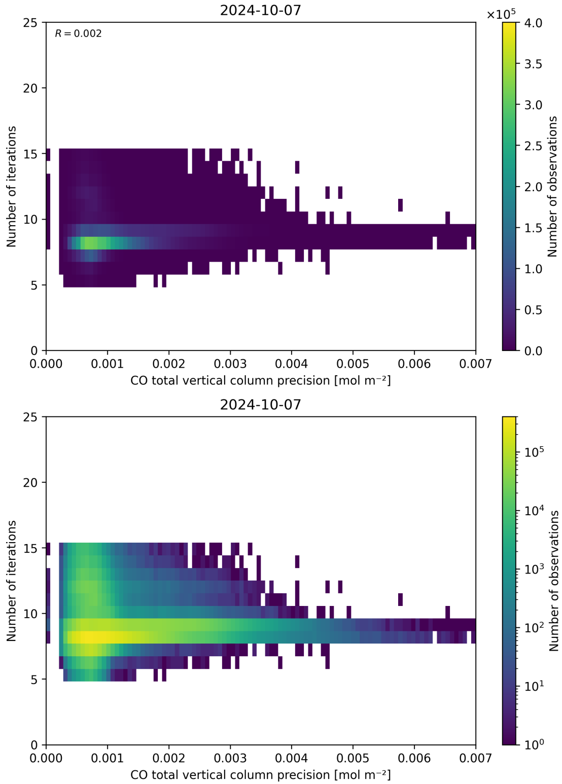
Figure 46: Scatter density plot of “CO total vertical column precision” against “Number of iterations” for 2024-10-06 to 2024-10-08.
