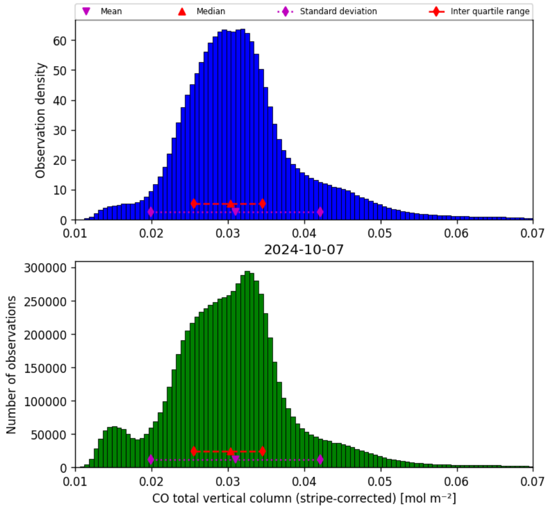
Figure 19: Histogram of “CO total vertical column (stripe-corrected)” for 2024-10-06 to 2024-10-08
