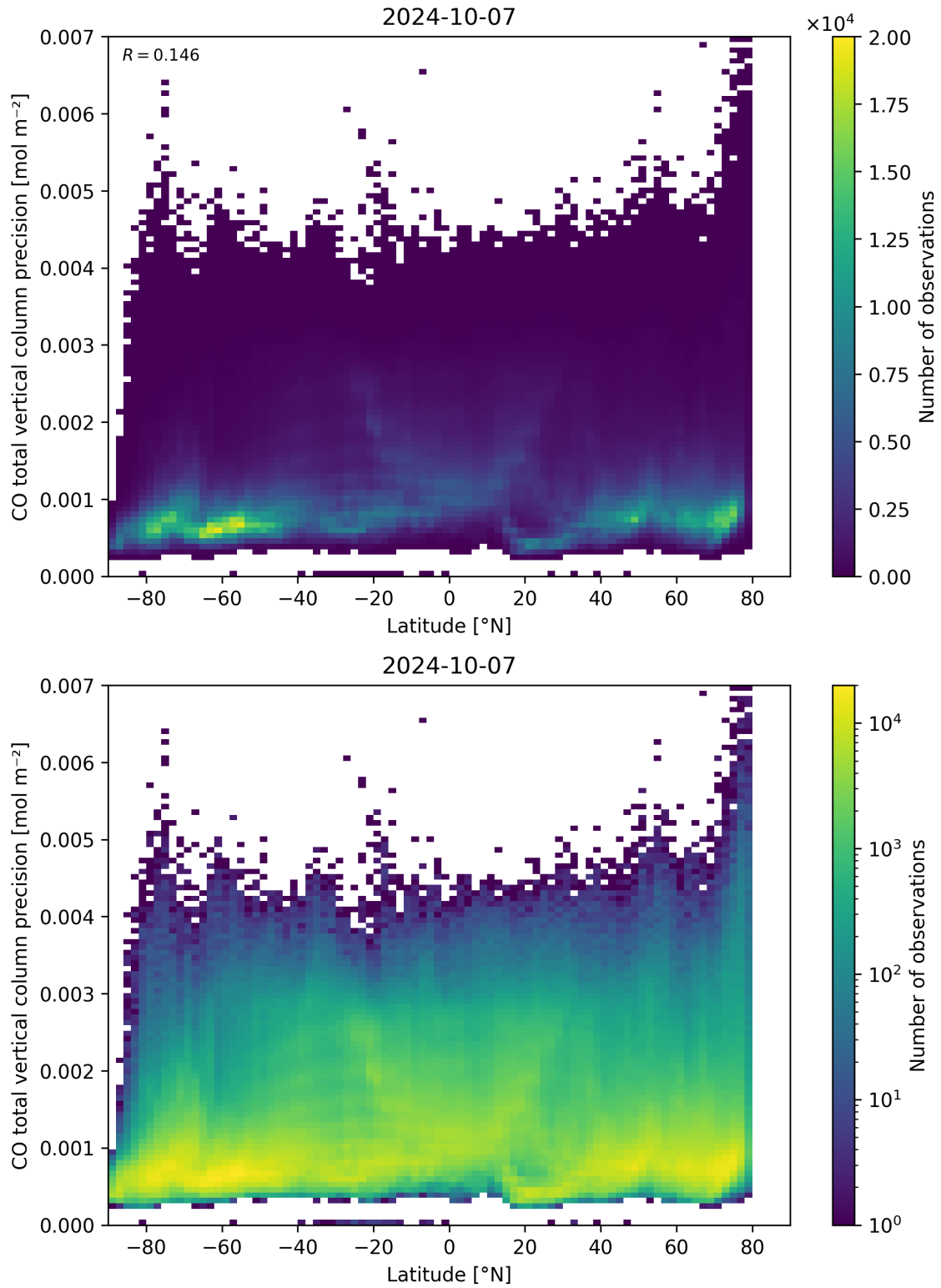
Figure 53: Scatter density plot of “Latitude” against “CO total vertical column precision” for 2024-10-06 to 2024-10-08.
