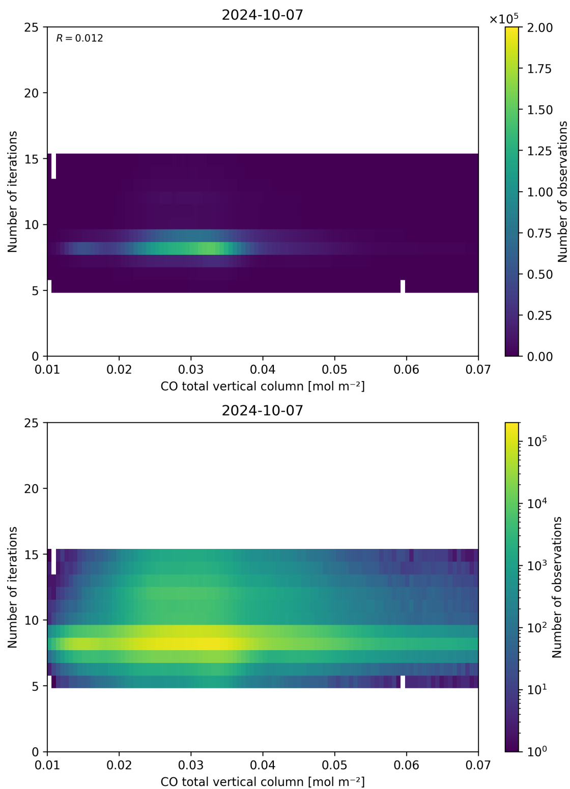
Figure 42: Scatter density plot of “CO total vertical column” against “Number of iterations” for 2024-10-06 to 2024-10-08.
