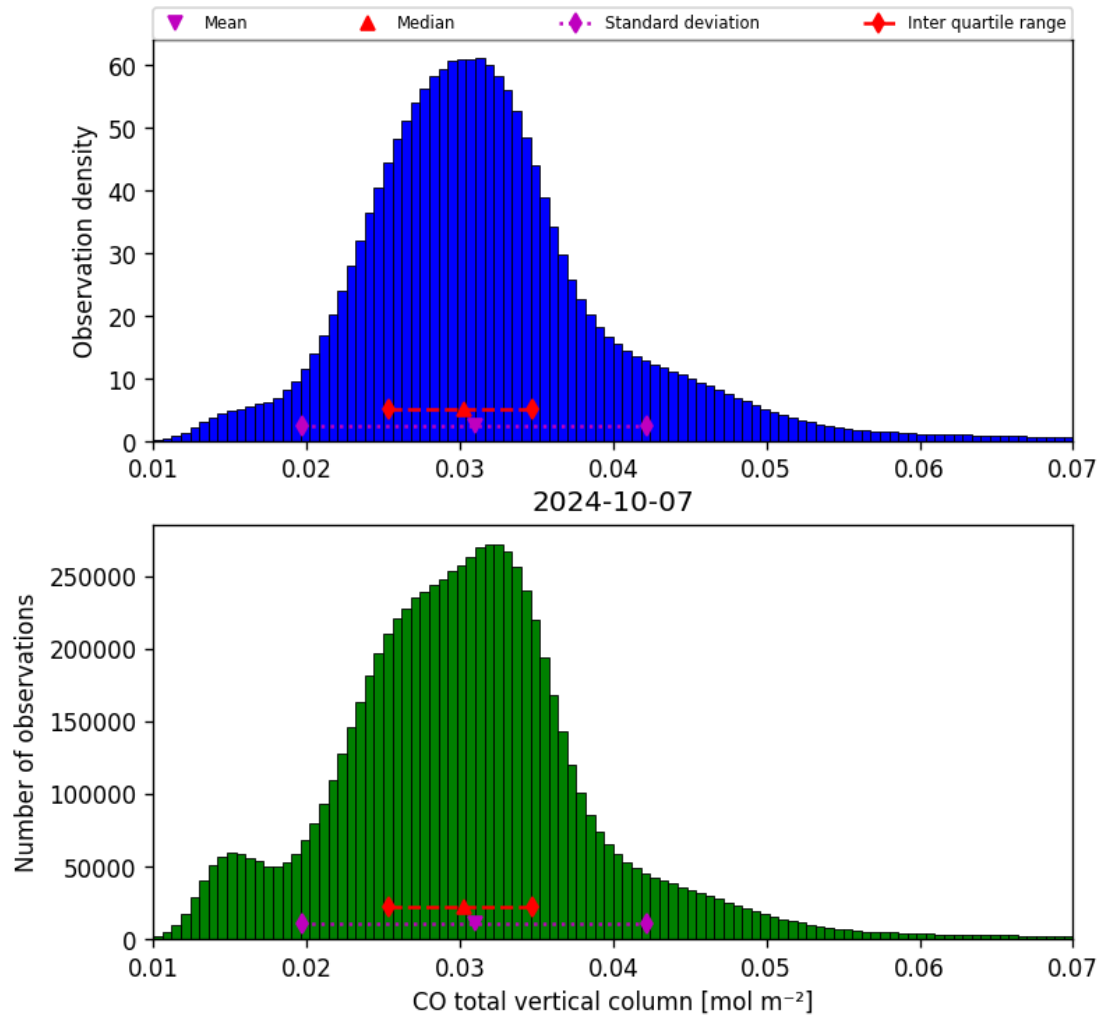
Figure 18: Histogram of “CO total vertical column” for 2024-10-06 to 2024-10-08
