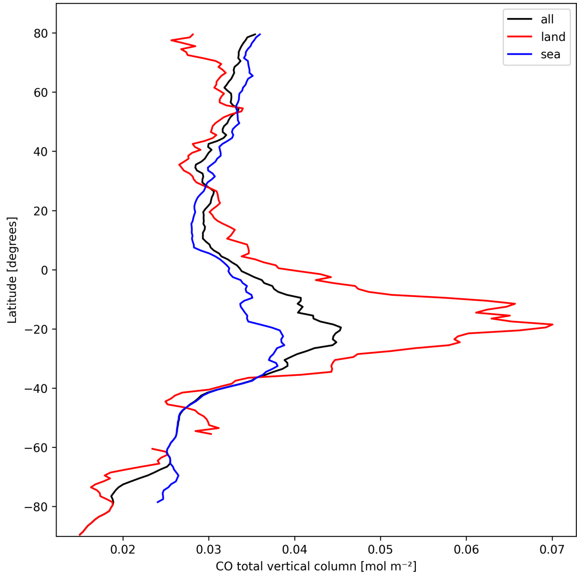
Figure 10: Zonal average of “CO total vertical column” for 2024-10-06 to 2024-10-08.
