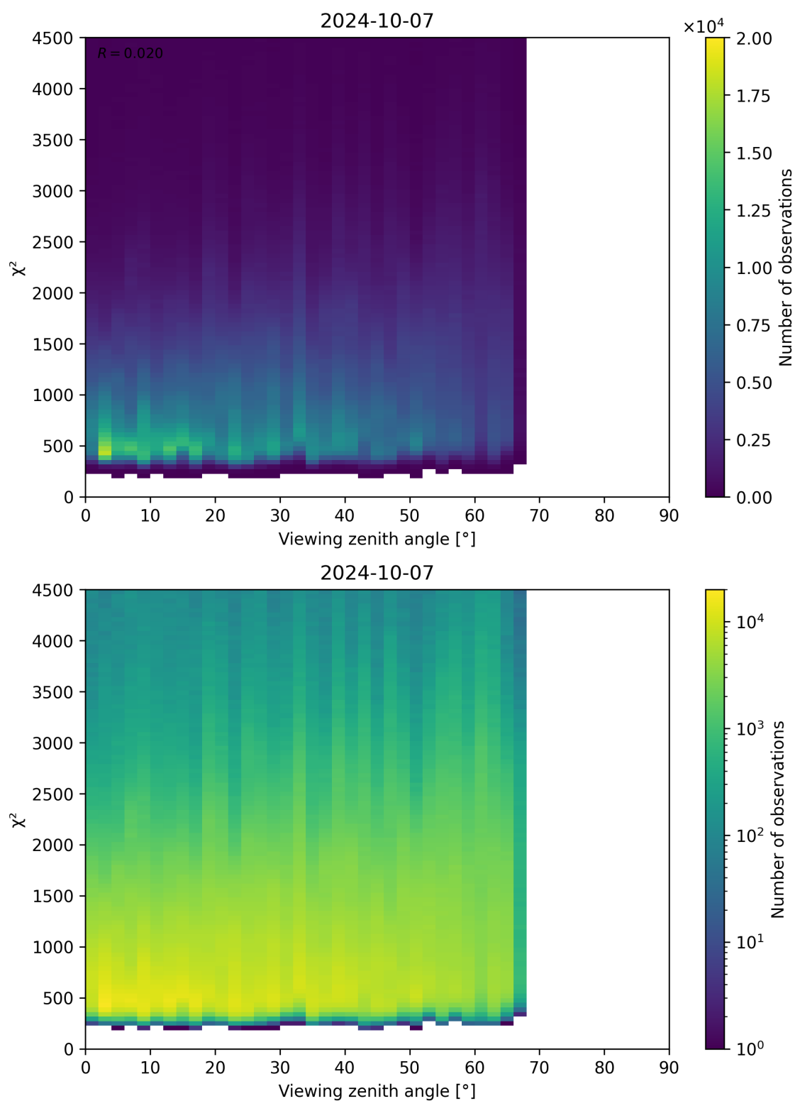
Figure 72: Scatter density plot of “Viewing zenith angle” against “ \chi^2 ” for 2024-10-06 to 2024-10-08.
