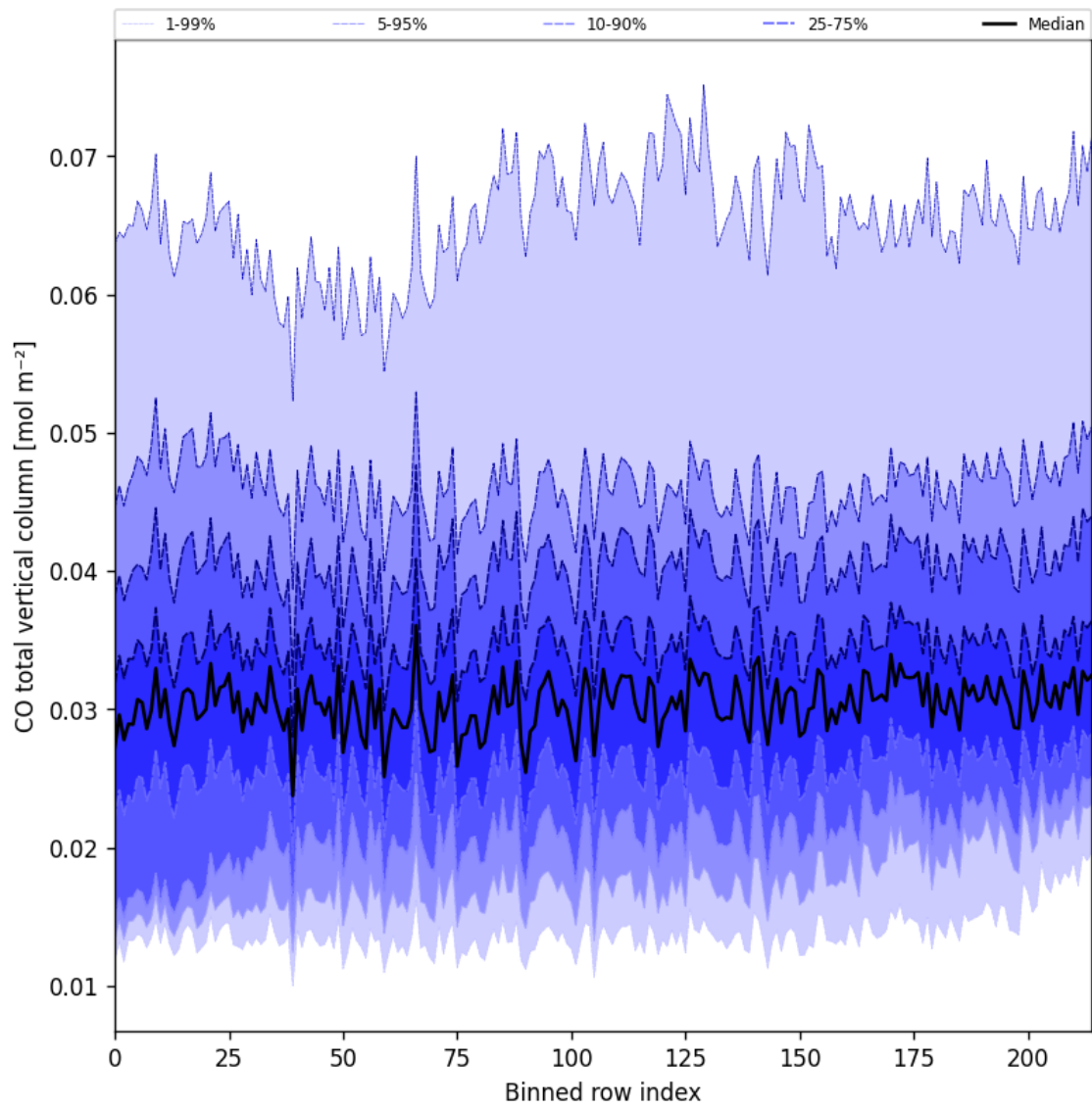
Figure 26: Along track statistics of “CO total vertical column” for 2024-10-06 to 2024-10-08
