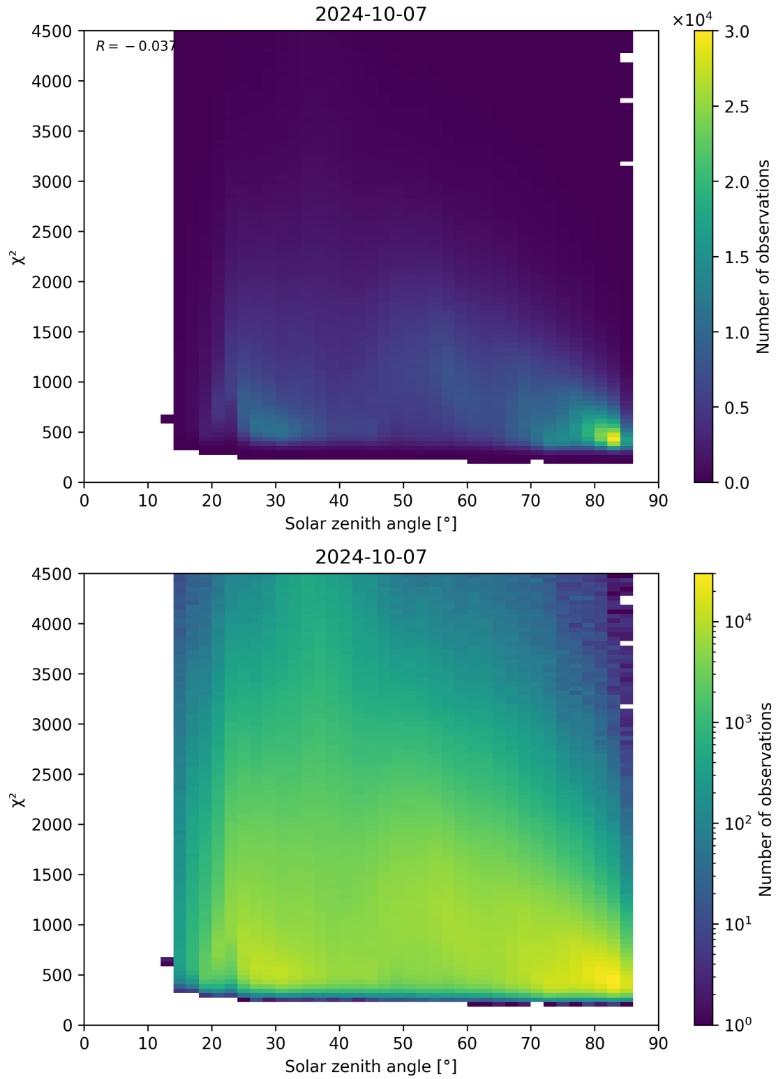
Figure 64: Scatter density plot of “Solar zenith angle” against “ \chi^2 ” for 2024-10-06 to 2024-10-08.
