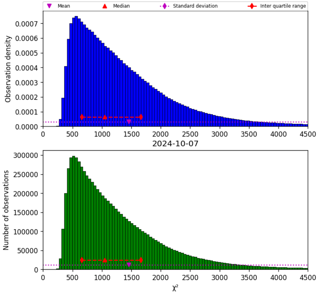
Figure 22: Histogram of “ \chi^2 ” for 2024-10-06 to 2024-10-08
