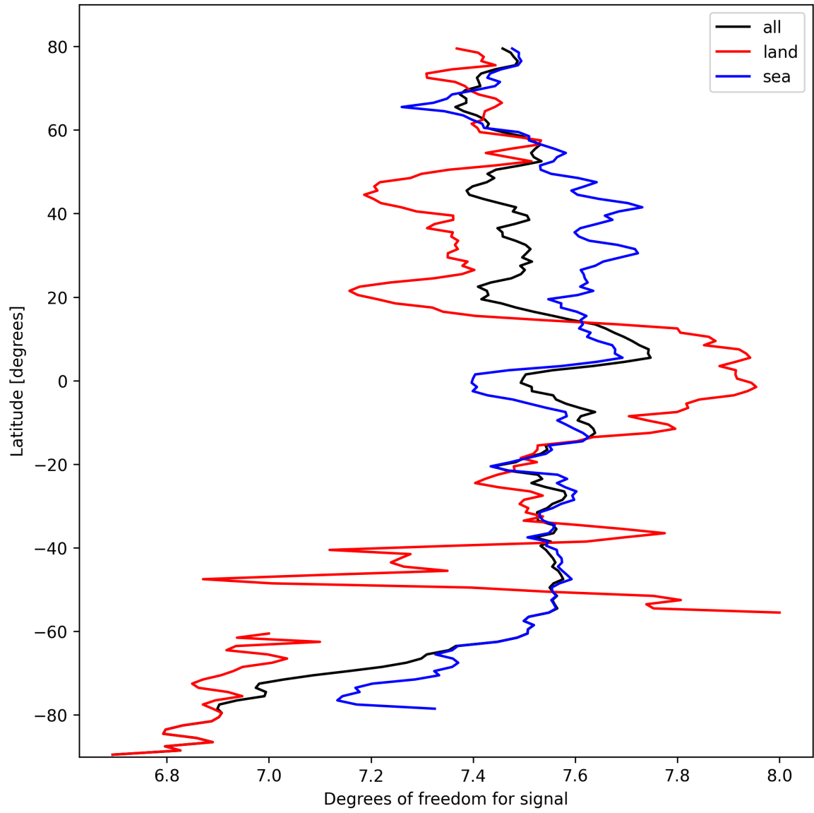
Figure 15: Zonal average of “Degrees of freedom for signal” for 2024-10-06 to 2024-10-08.
