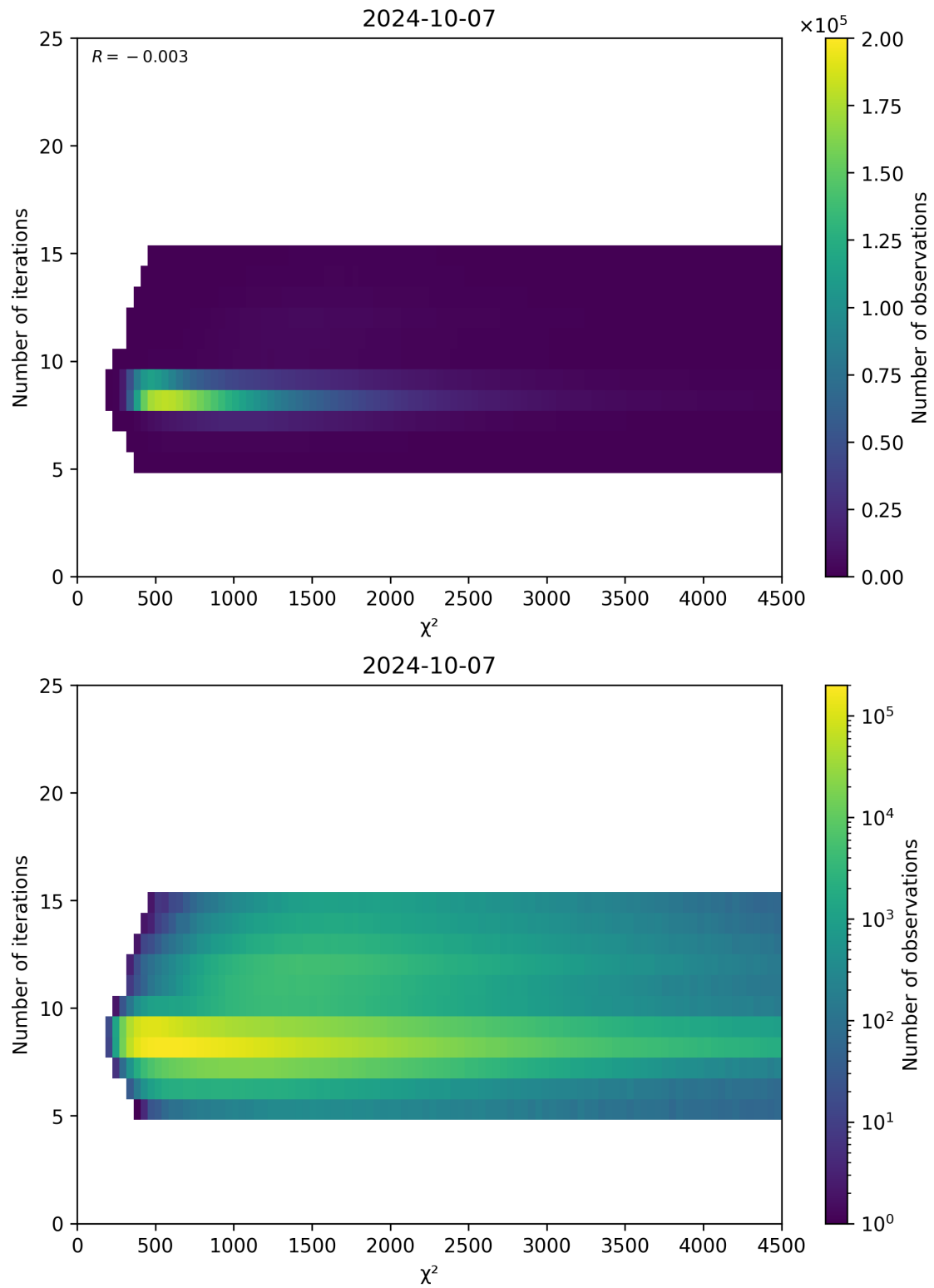
Figure 49: Scatter density plot of “ \chi^2 ” against “Number of iterations” for 2024-10-06 to 2024-10-08.
