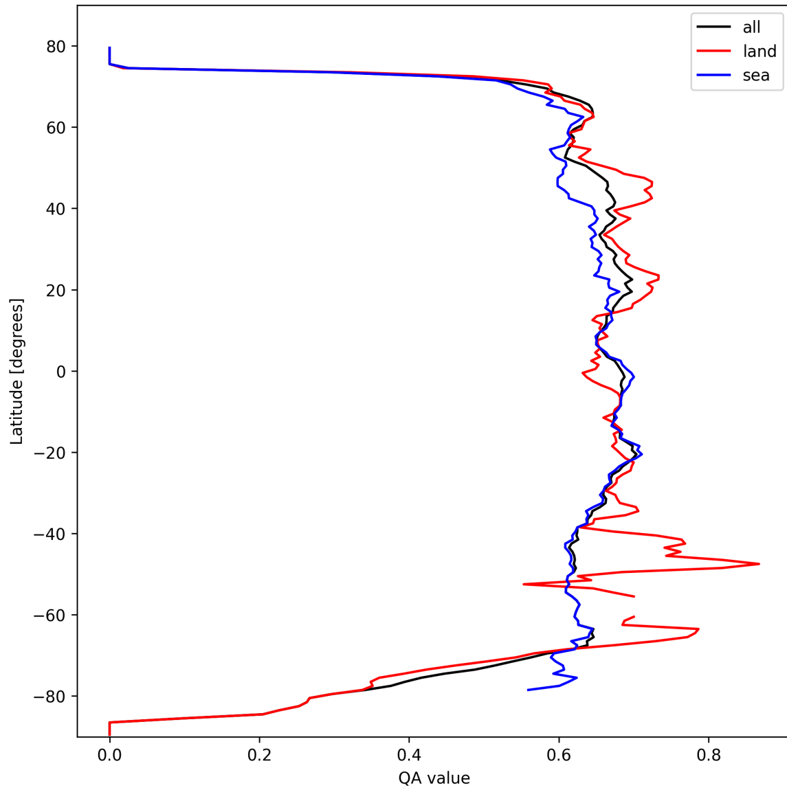
Figure 9: Zonal average of “QA value” for 2024-10-06 to 2024-10-08.
