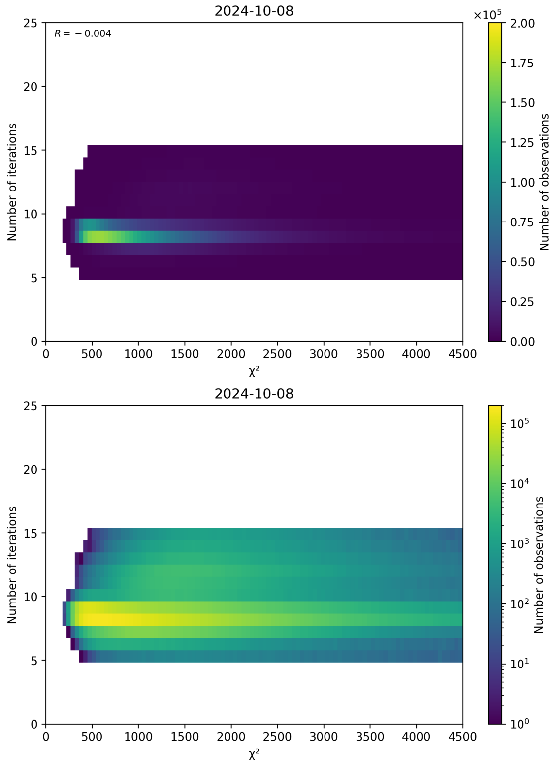
Figure 49: Scatter density plot of “ \chi^2 ” against “Number of iterations” for 2024-10-08 to 2024-10-09.
