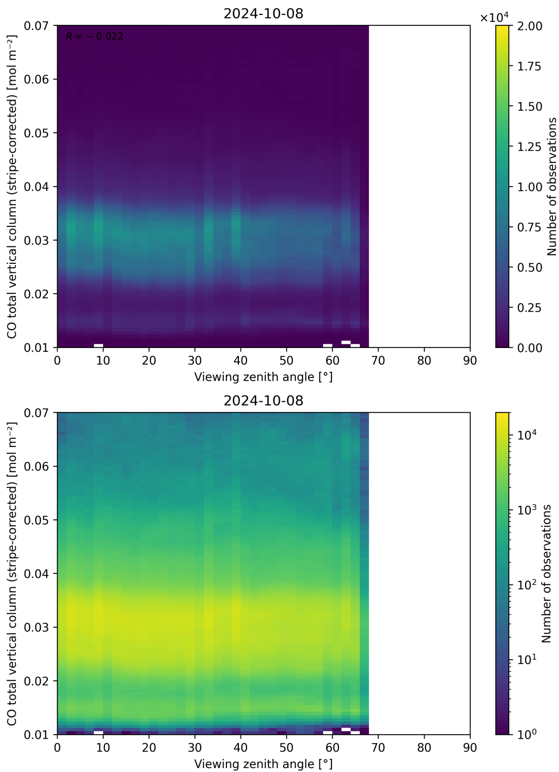
Figure 70: Scatter density plot of “Viewing zenith angle” against “CO total vertical column (stripe-corrected)” for 2024-10-08 to 2024-10-09.
