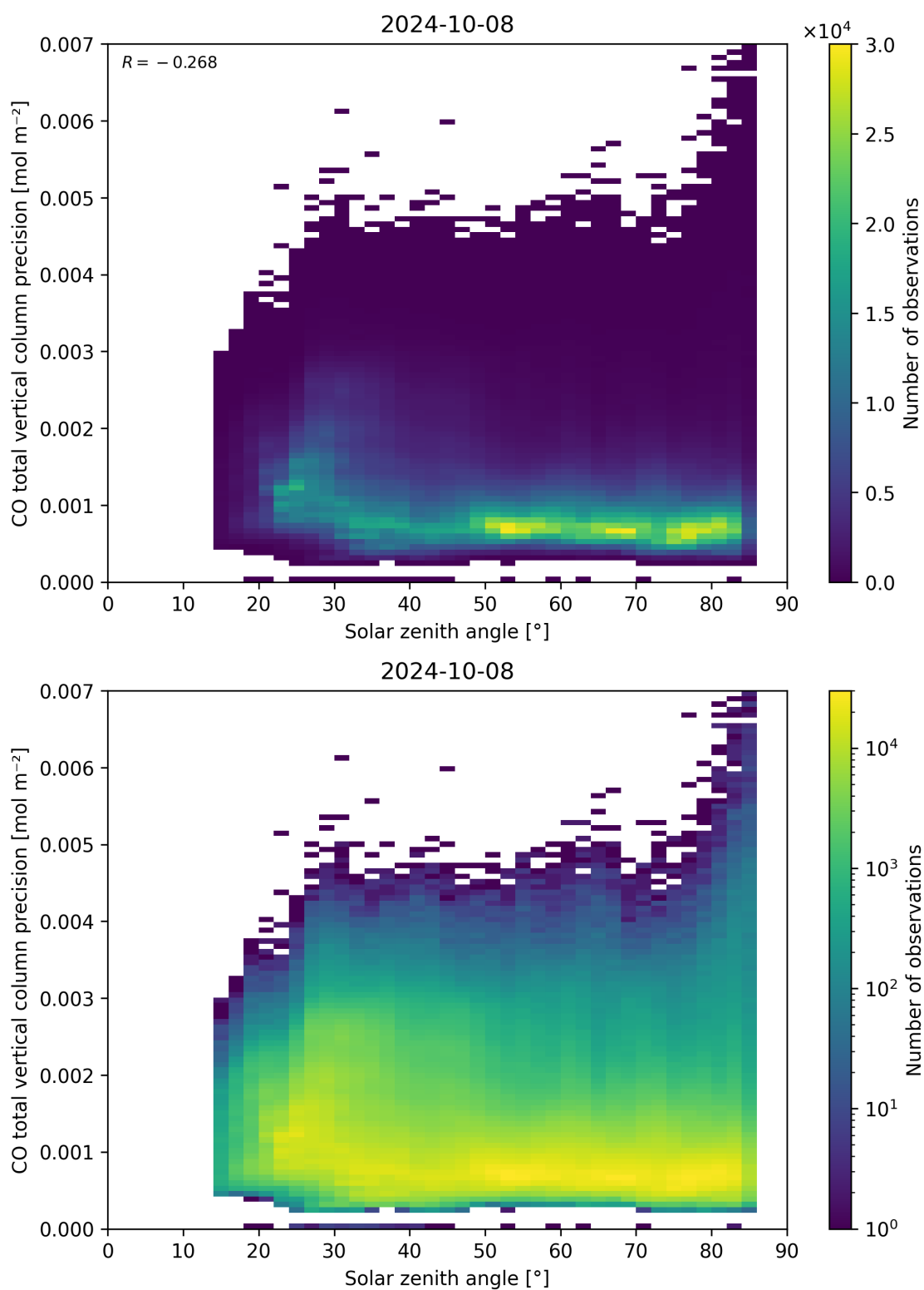
Figure 63: Scatter density plot of “Solar zenith angle” against “CO total vertical column precision” for 2024-10-08 to 2024-10-09.
