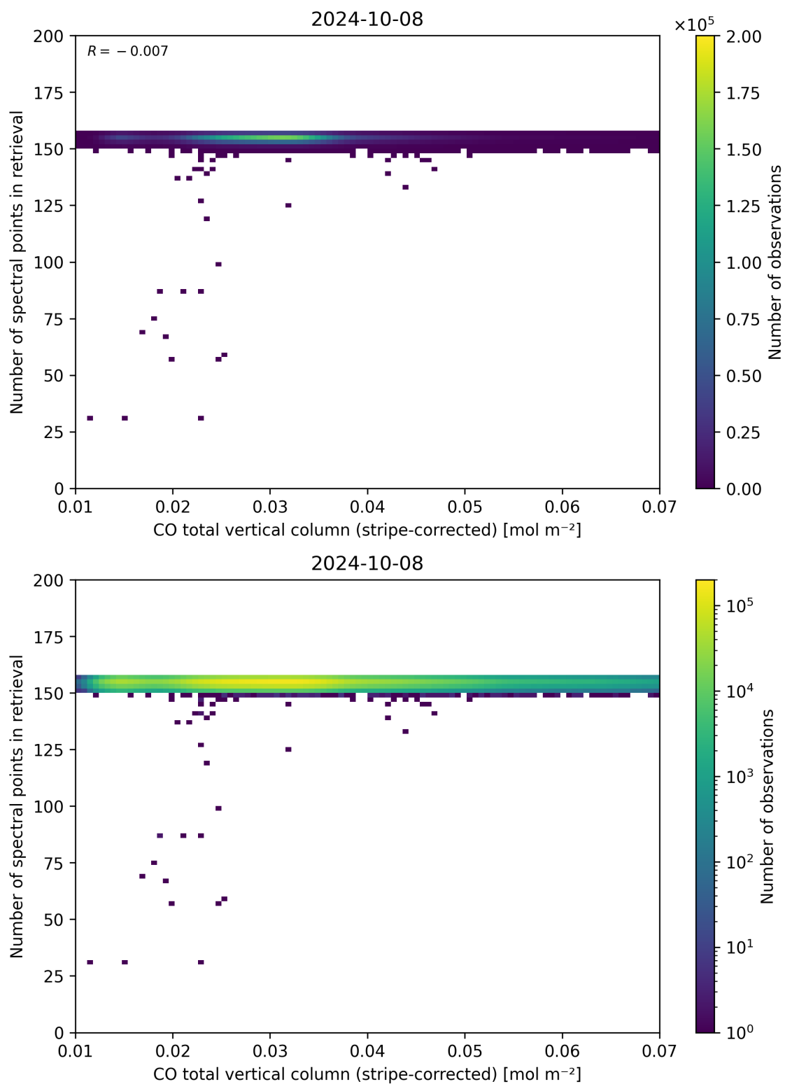
Figure 40: Scatter density plot of “CO total vertical column (stripe-corrected)” against “Number of spectral points in retrieval” for 2024-10-08 to 2024-10-09.
