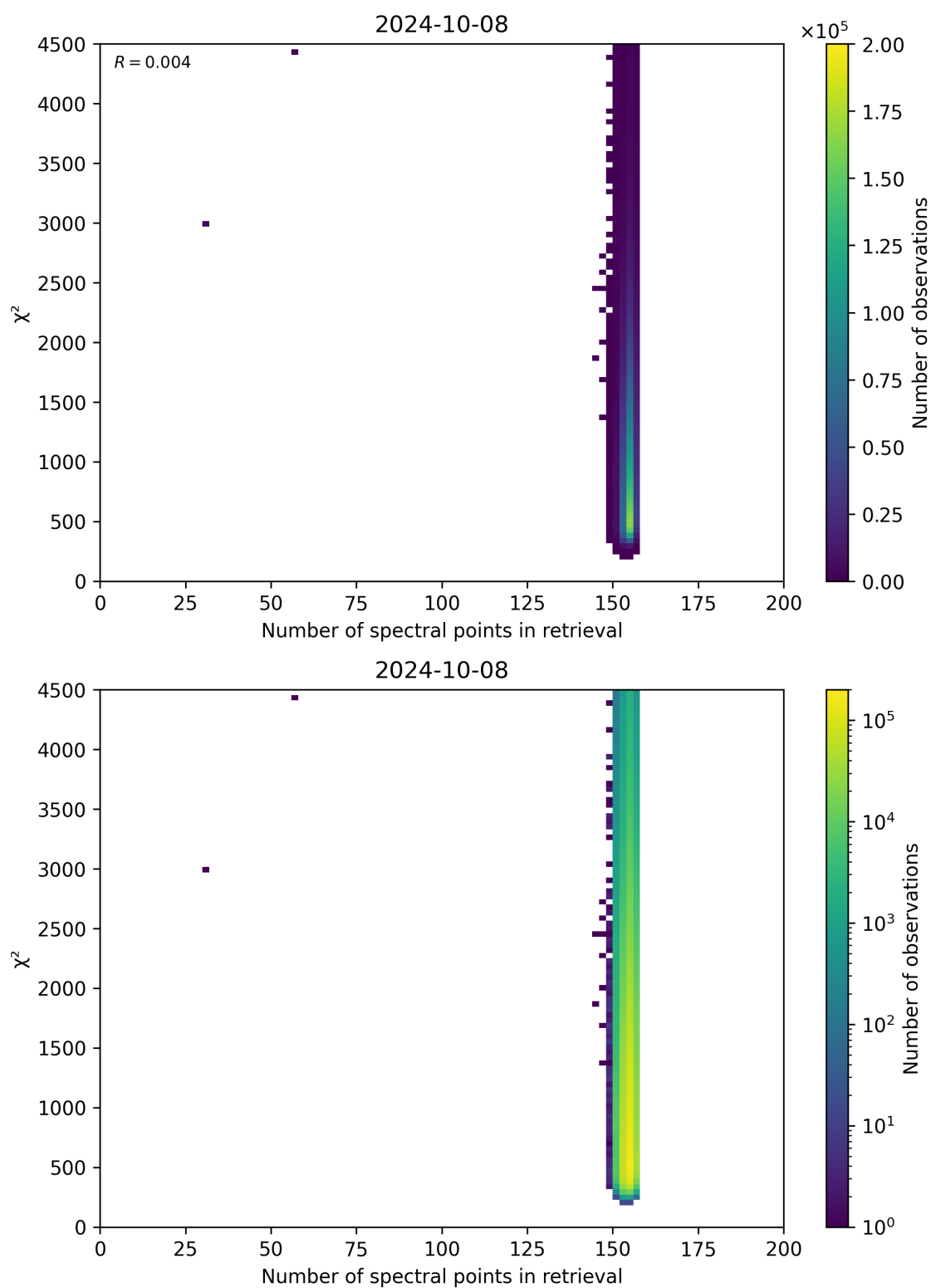
Figure 58: Scatter density plot of “Number of spectral points in retrieval” against “ \chi^2 ” for 2024-10-08 to 2024-10-09.
