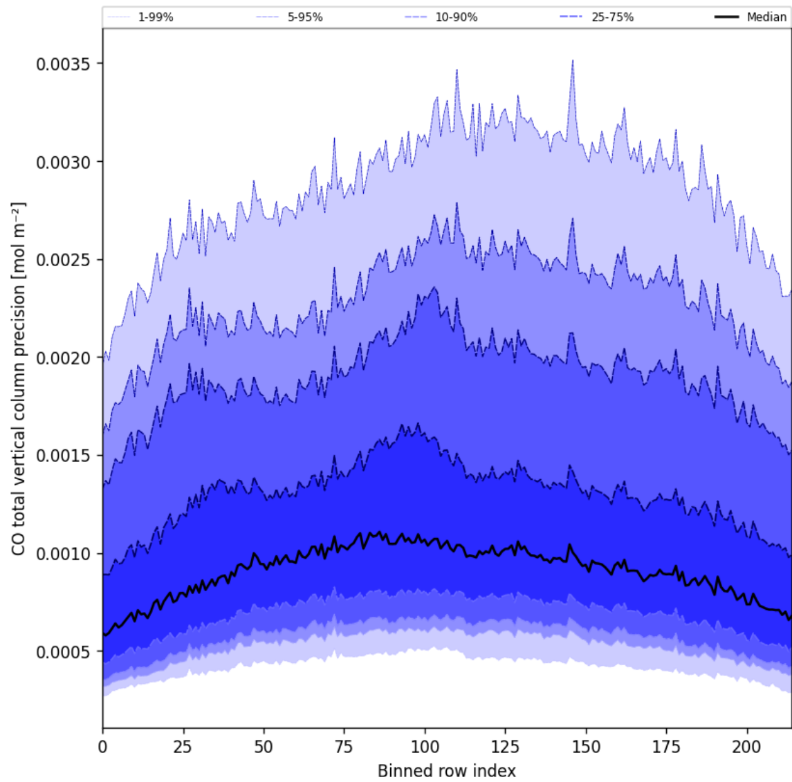
Figure 28: Along track statistics of “CO total vertical column precision” for 2024-10-08 to 2024-10-09
