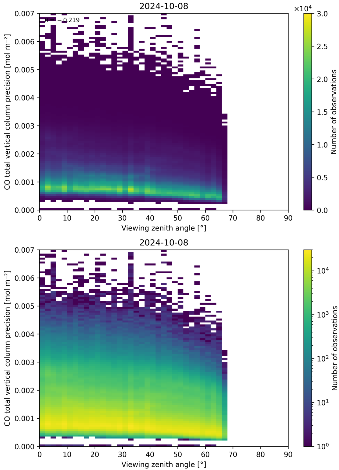
Figure 71: Scatter density plot of “Viewing zenith angle” against “CO total vertical column precision” for 2024-10-08 to 2024-10-09.
