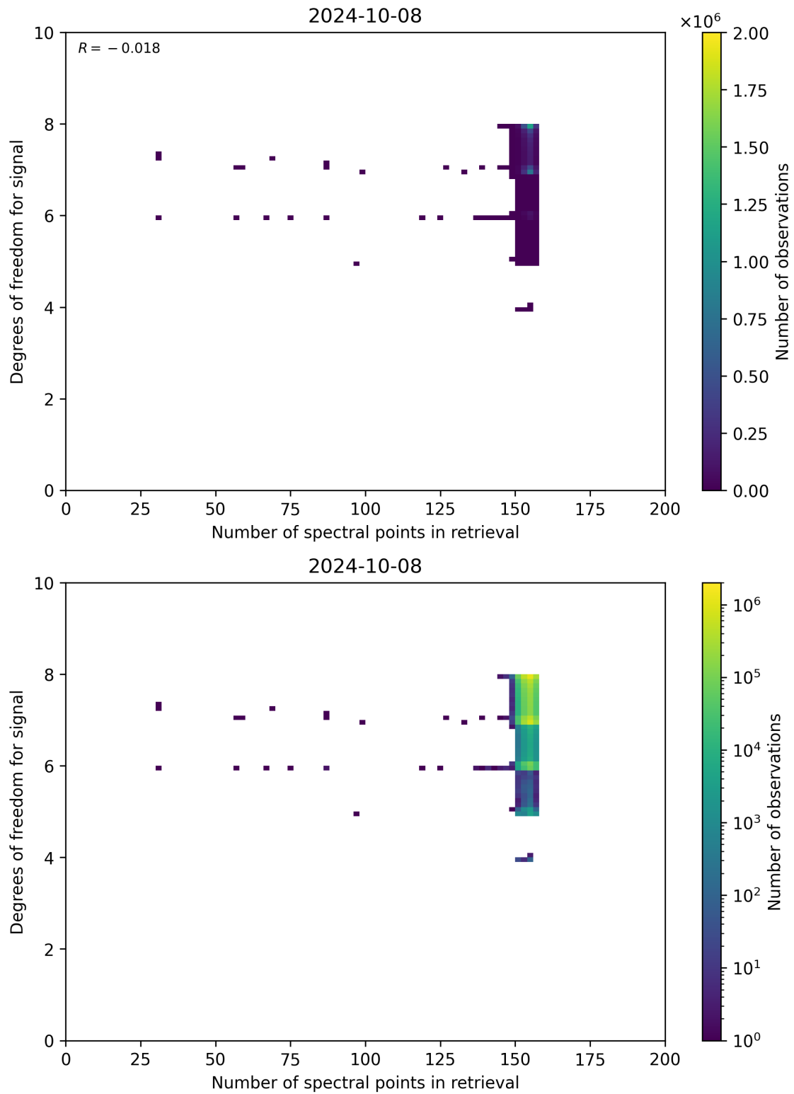
Figure 59: Scatter density plot of “Number of spectral points in retrieval” against “Degrees of freedom for signal” for 2024-10-08 to 2024-10-09.
