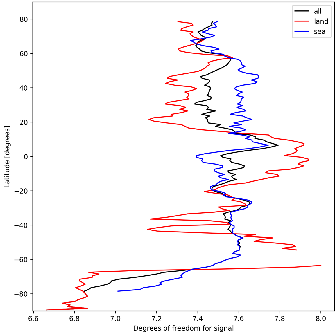
Figure 15: Zonal average of “Degrees of freedom for signal” for 2024-10-08 to 2024-10-09.
