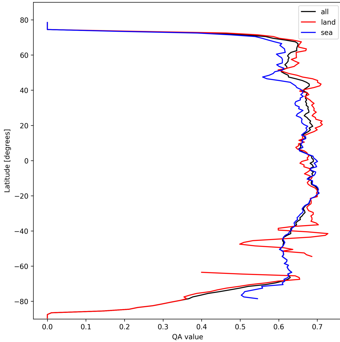
Figure 9: Zonal average of “QA value” for 2024-10-08 to 2024-10-09.
