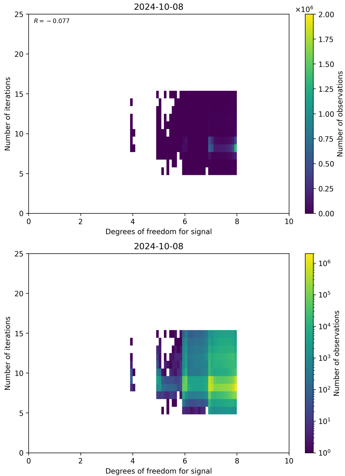
Figure 50: Scatter density plot of “Degrees of freedom for signal” against “Number of iterations” for 2024-10-08 to 2024-10-09.
