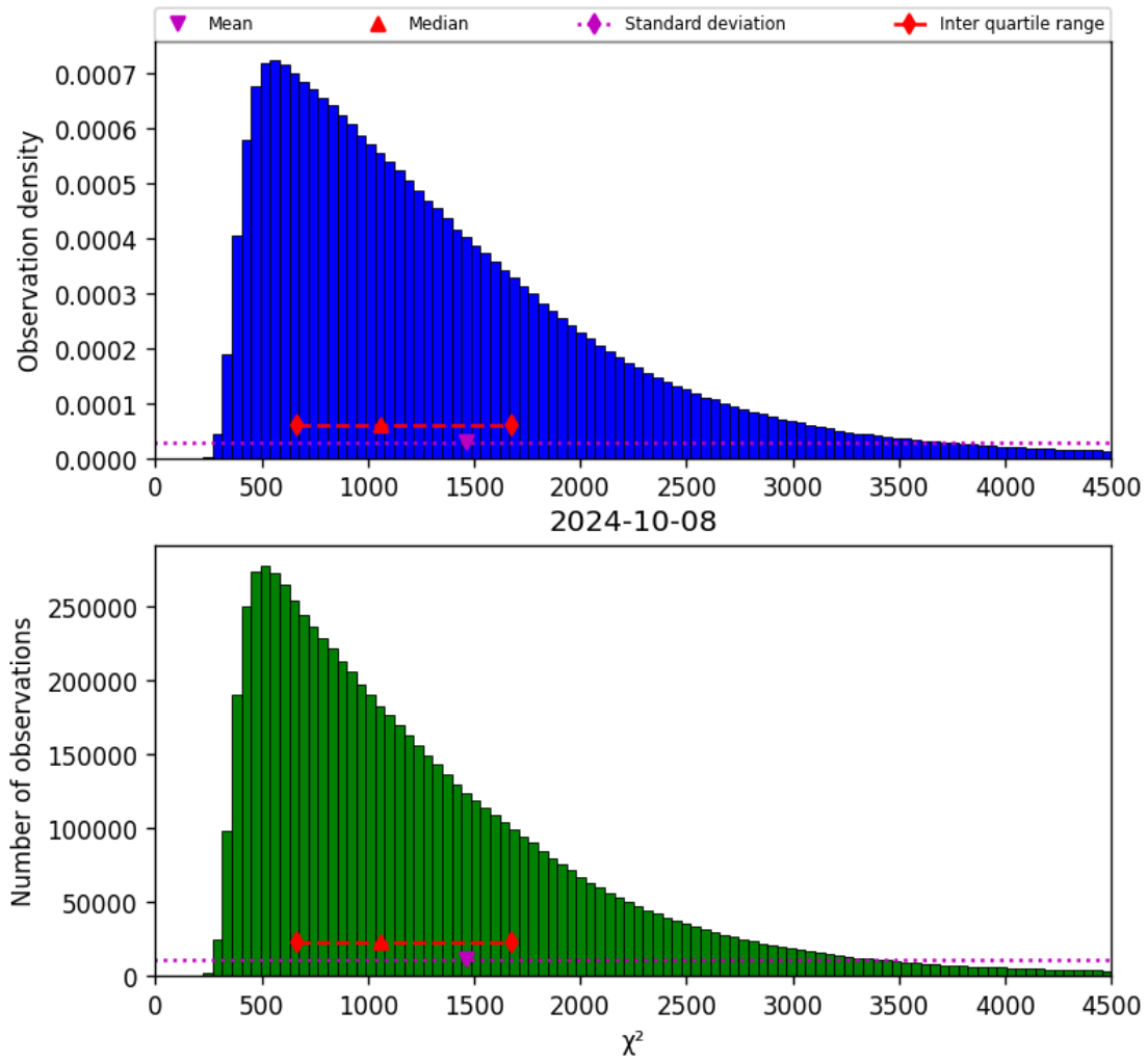
Figure 22: Histogram of “ \chi^2 ” for 2024-10-08 to 2024-10-09
