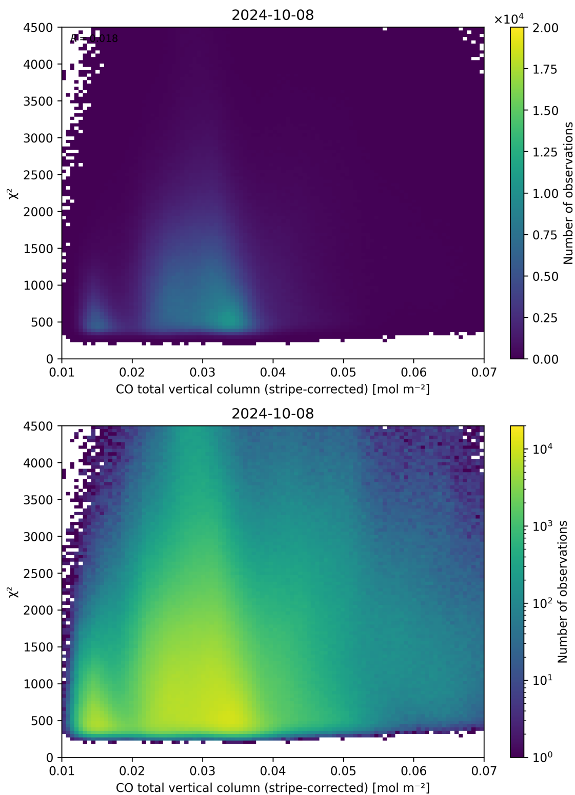
Figure 37: Scatter density plot of “CO total vertical column (stripe-corrected)” against “ \chi^2 ” for 2024-10-08 to 2024-10-09.
