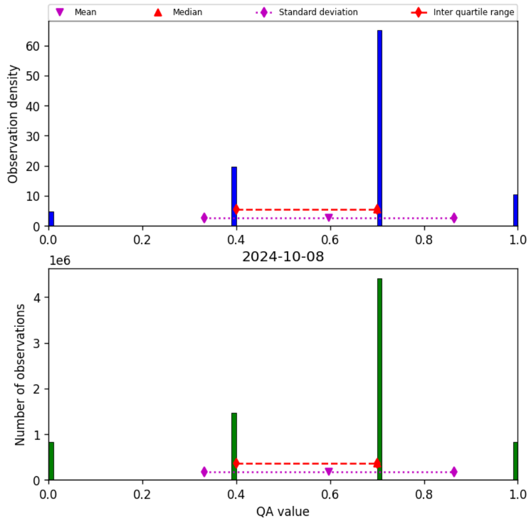
Figure 17: Histogram of “QA value” for 2024-10-08 to 2024-10-09
