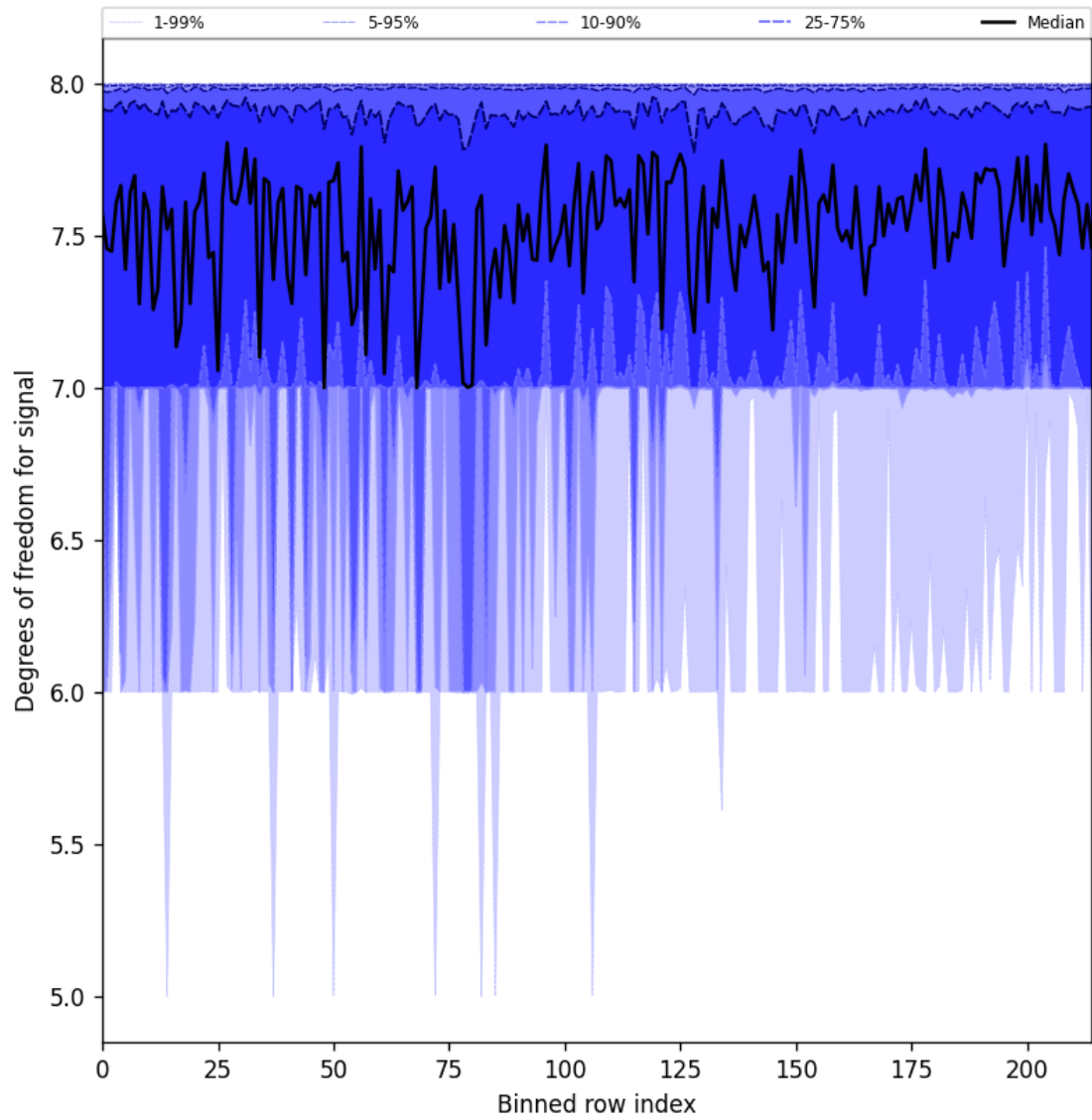
Figure 31: Along track statistics of “Degrees of freedom for signal” for 2024-10-08 to 2024-10-09
