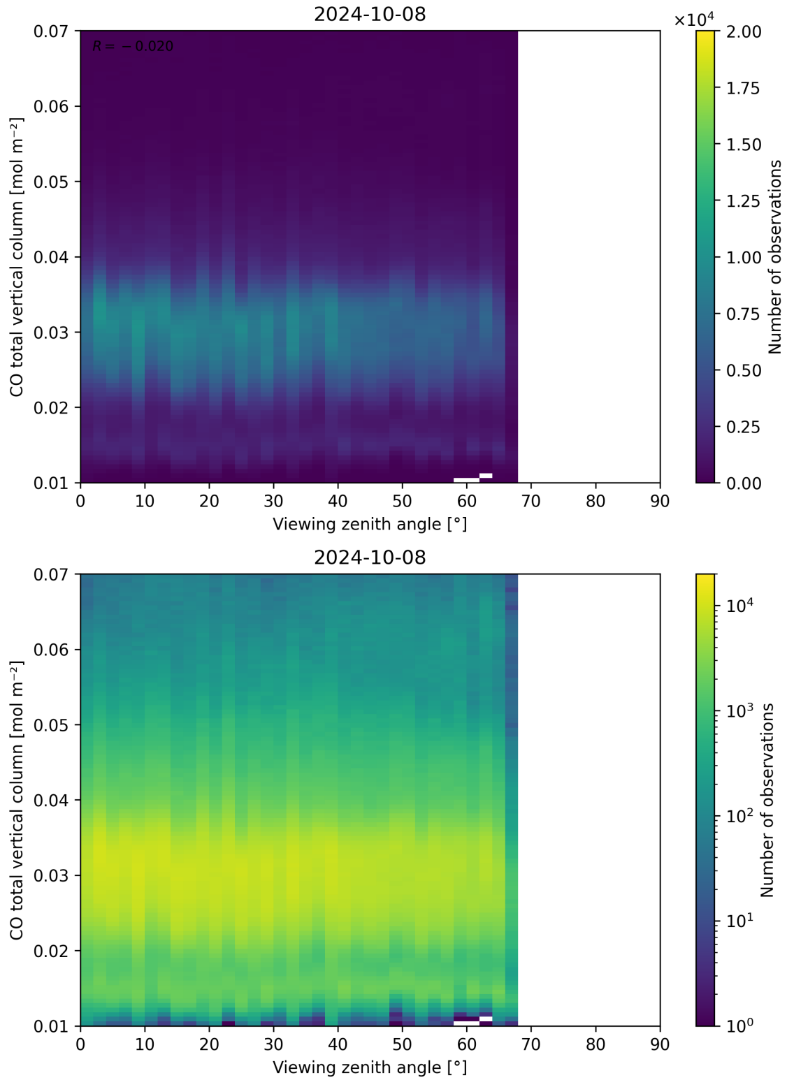
Figure 69: Scatter density plot of “Viewing zenith angle” against “CO total vertical column” for 2024-10-08 to 2024-10-09.
