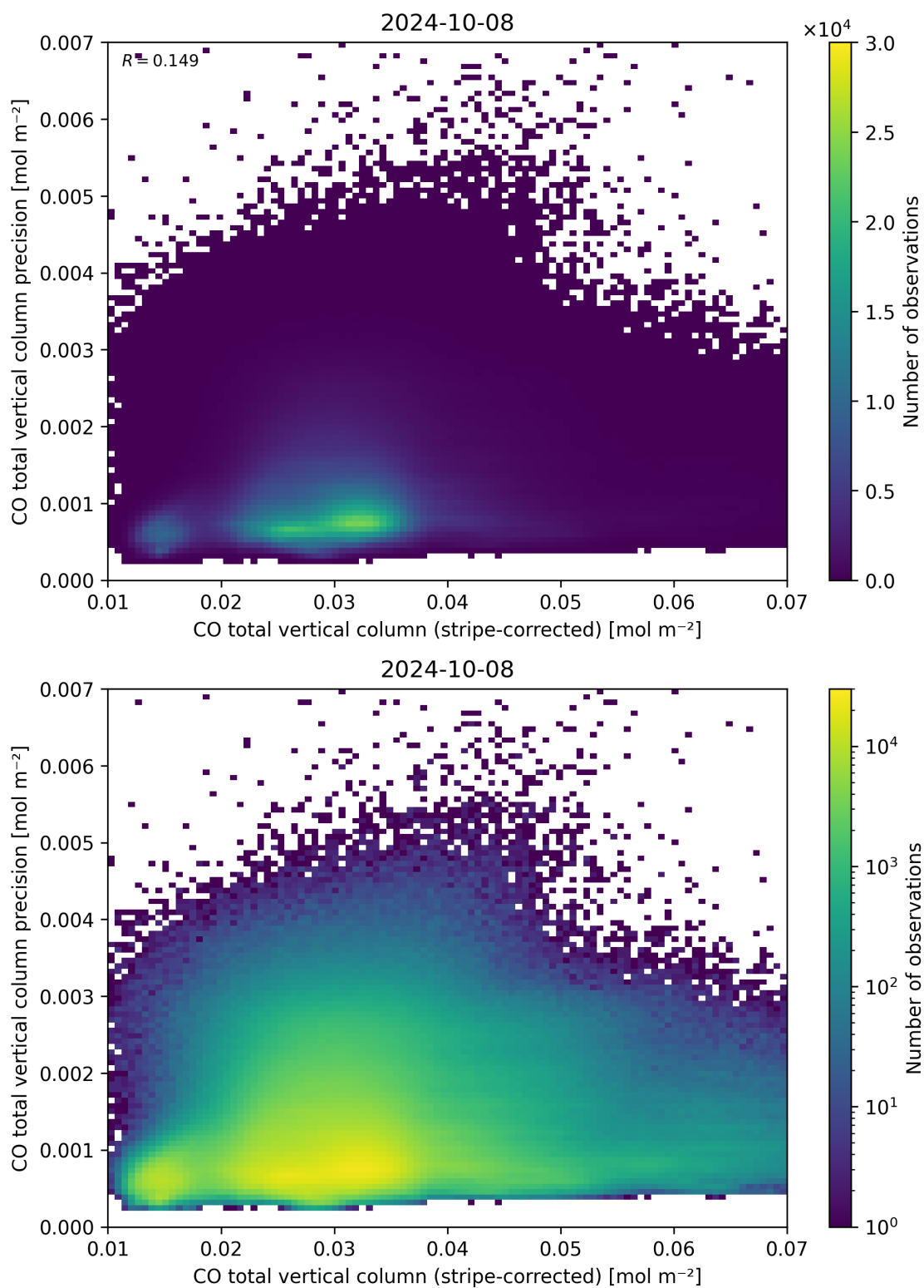
Figure 36: Scatter density plot of “CO total vertical column (stripe-corrected)” against “CO total vertical column precision” for 2024-10-08 to 2024-10-09.
