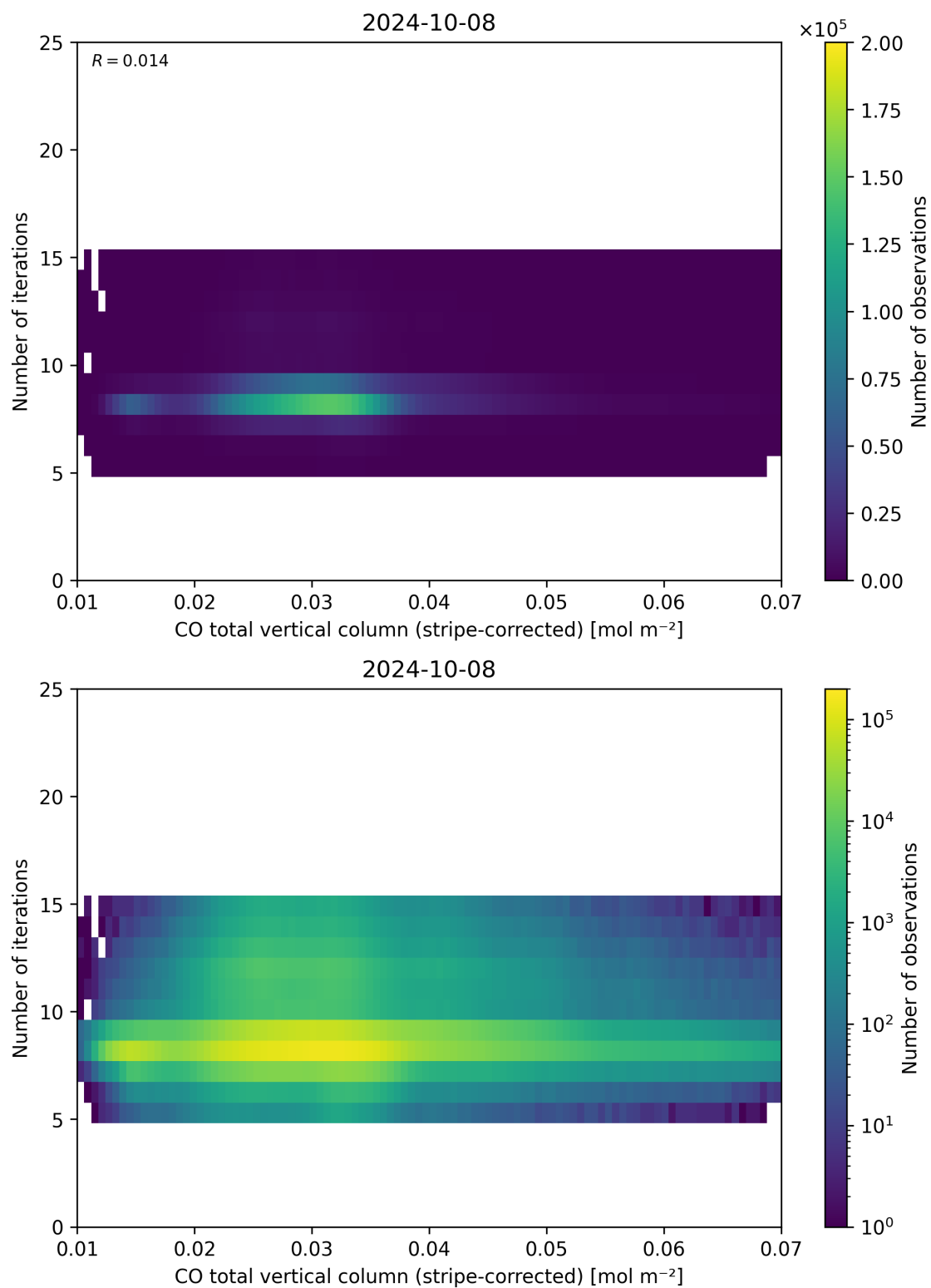
Figure 39: Scatter density plot of “CO total vertical column (stripe-corrected)” against “Number of iterations” for 2024-10-08 to 2024-10-09.
