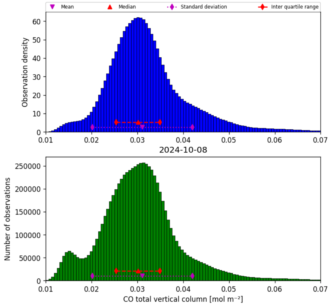
Figure 18: Histogram of “CO total vertical column” for 2024-10-08 to 2024-10-09
