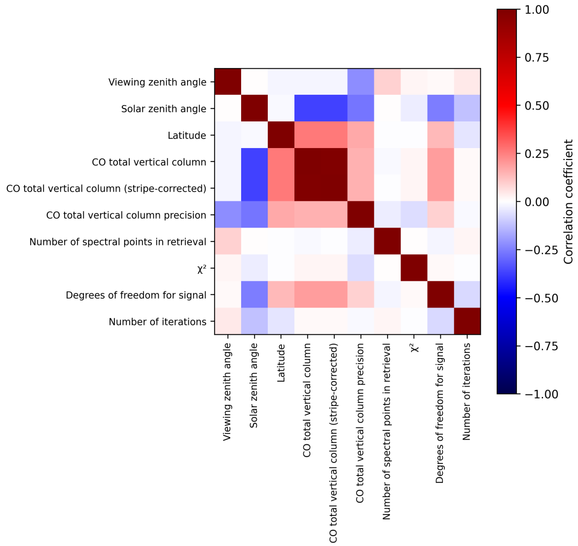
Figure 2: Map of correlation matrix for 2024-10-08 to 2024-10-09.
