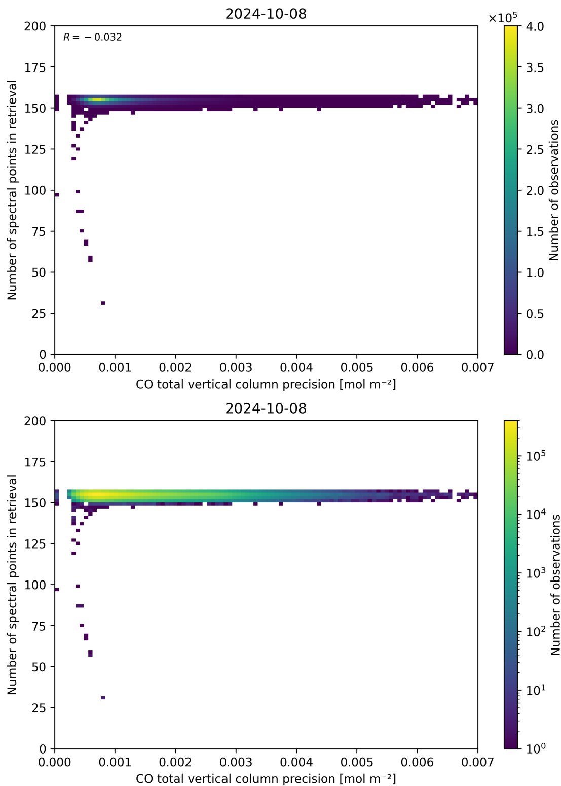
Figure 47: Scatter density plot of “CO total vertical column precision” against “Number of spectral points in retrieval” for 2024-10-08 to 2024-10-09.
