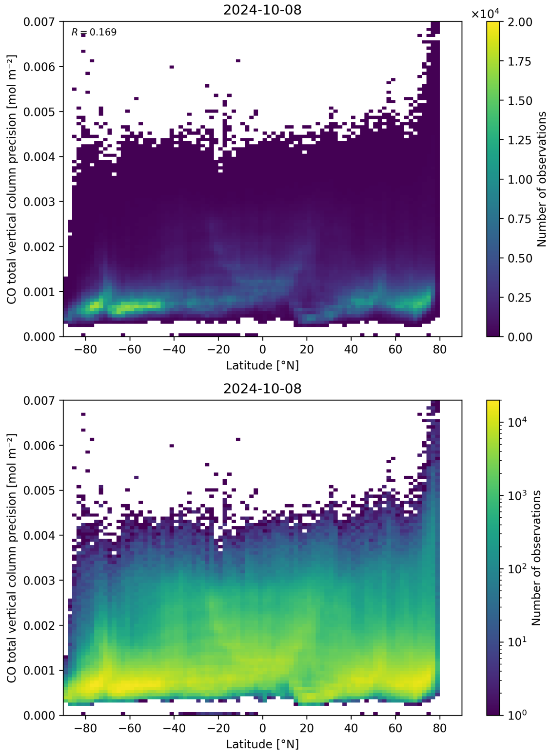
Figure 53: Scatter density plot of “Latitude” against “CO total vertical column precision” for 2024-10-08 to 2024-10-09.
