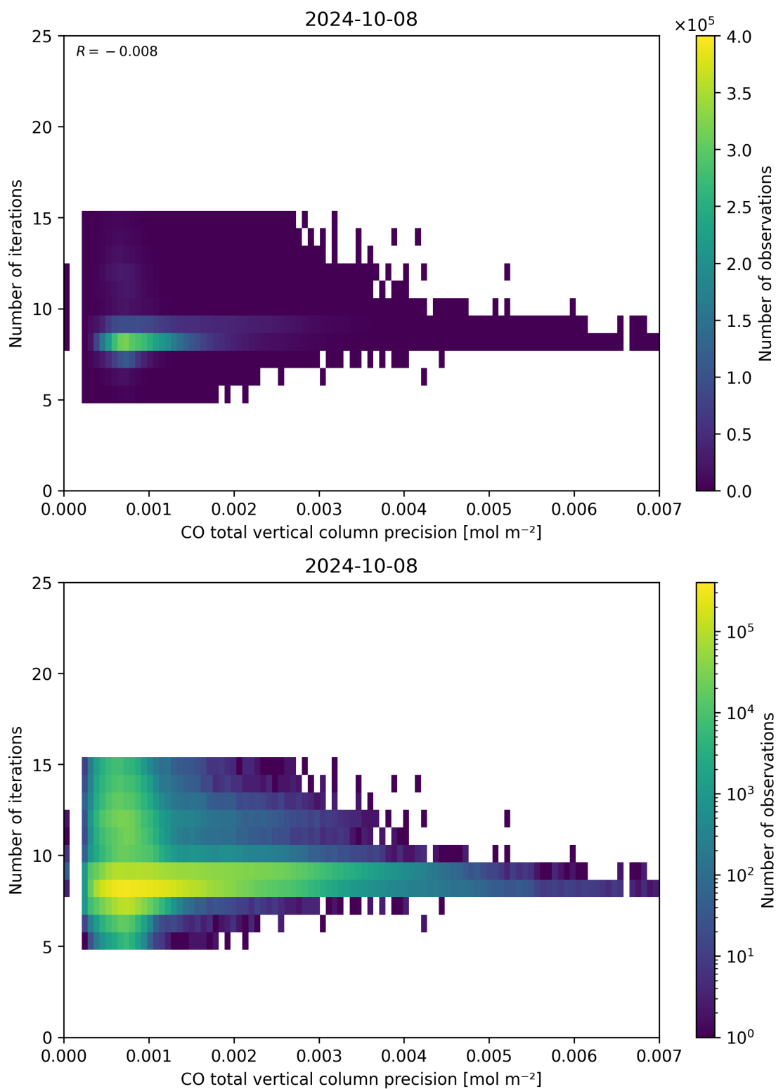
Figure 46: Scatter density plot of “CO total vertical column precision” against “Number of iterations” for 2024-10-08 to 2024-10-09.
