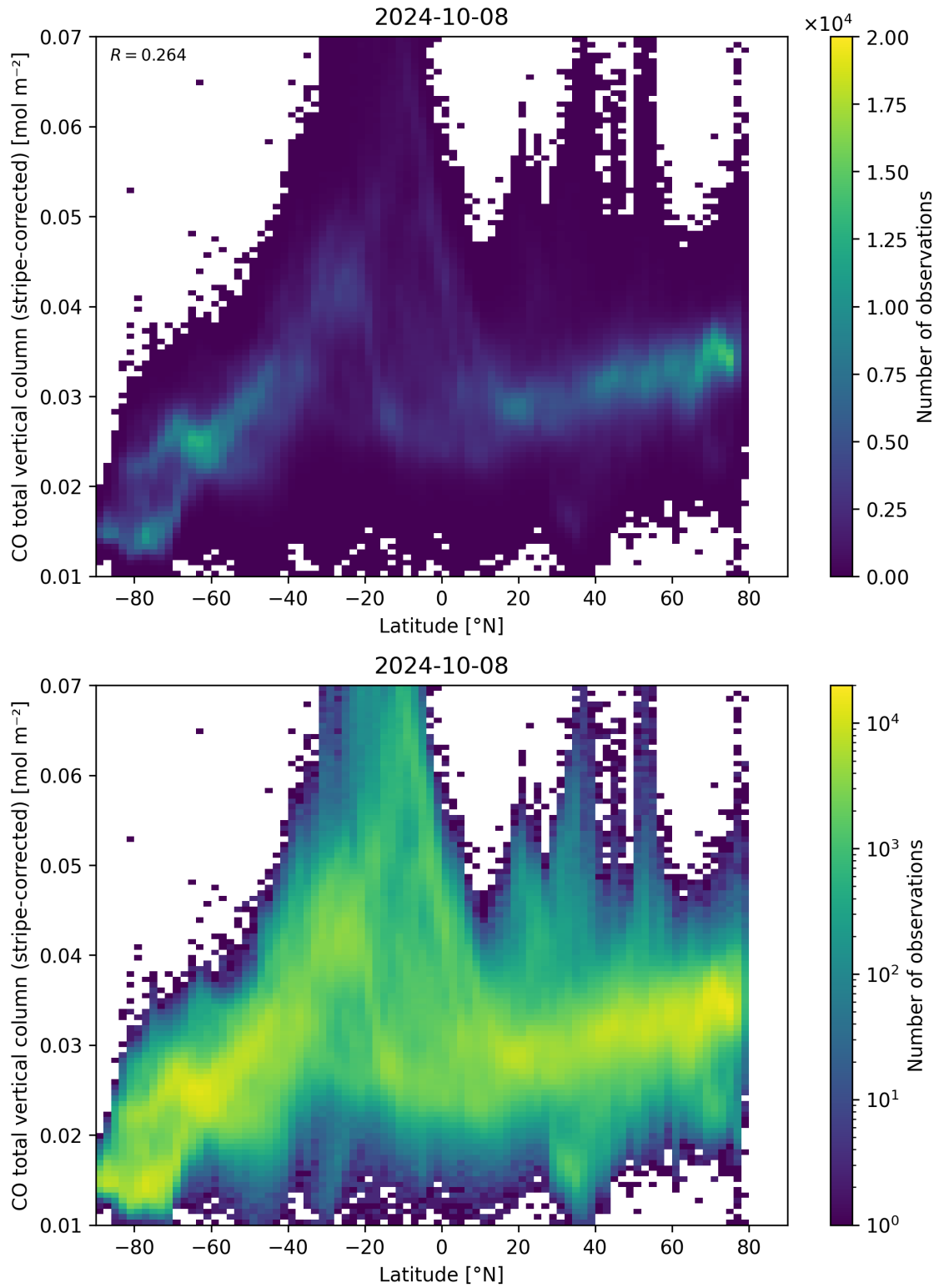
Figure 52: Scatter density plot of “Latitude” against “CO total vertical column (stripe-corrected)” for 2024-10-08 to 2024-10-09.
