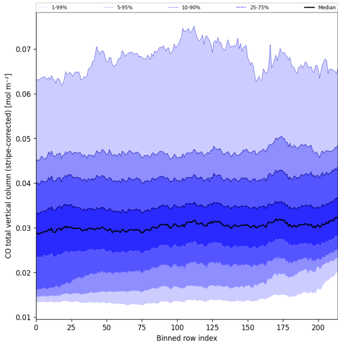
Figure 27: Along track statistics of “CO total vertical column (stripe-corrected)” for 2024-10-08 to 2024-10-09
