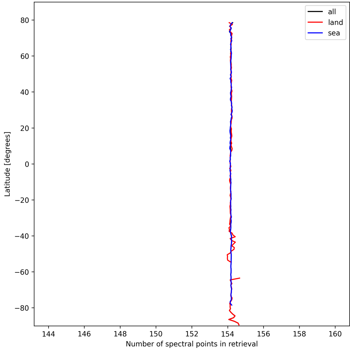
Figure 13: Zonal average of “Number of spectral points in retrieval” for 2024-10-08 to 2024-10-09.
