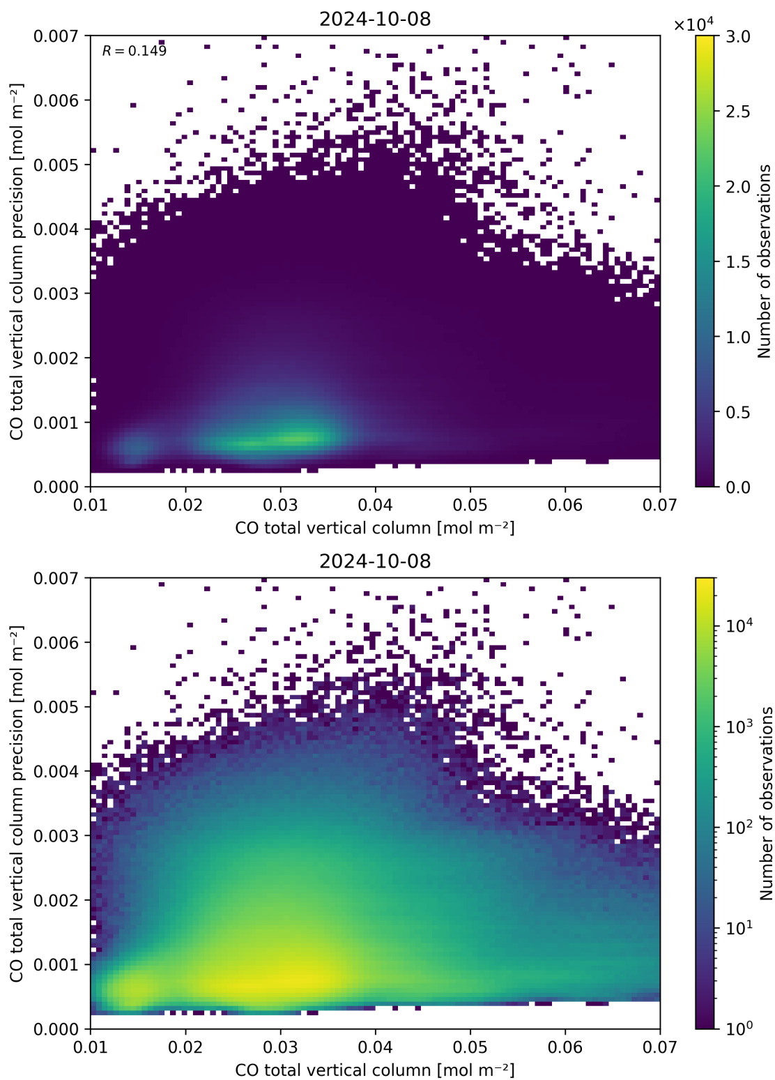
Figure 34: Scatter density plot of “CO total vertical column” against “CO total vertical column precision” for 2024-10-08 to 2024-10-09.
