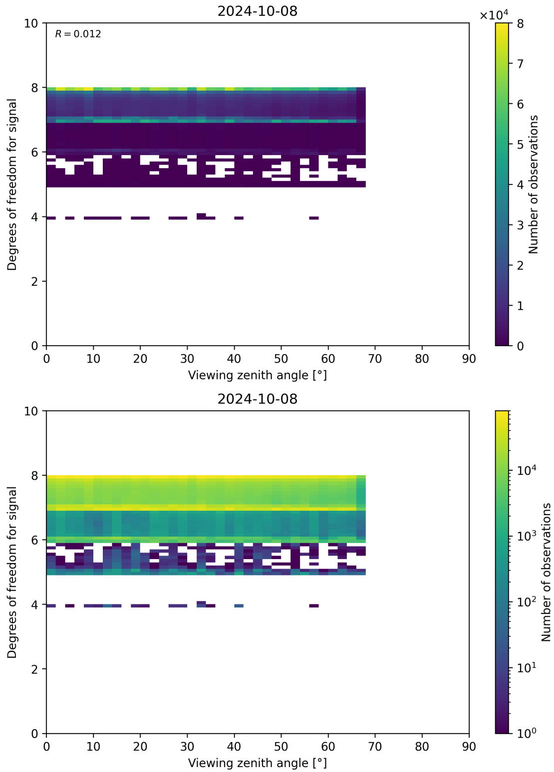
Figure 73: Scatter density plot of “Viewing zenith angle” against “Degrees of freedom for signal” for 2024-10-08 to 2024-10-09.
