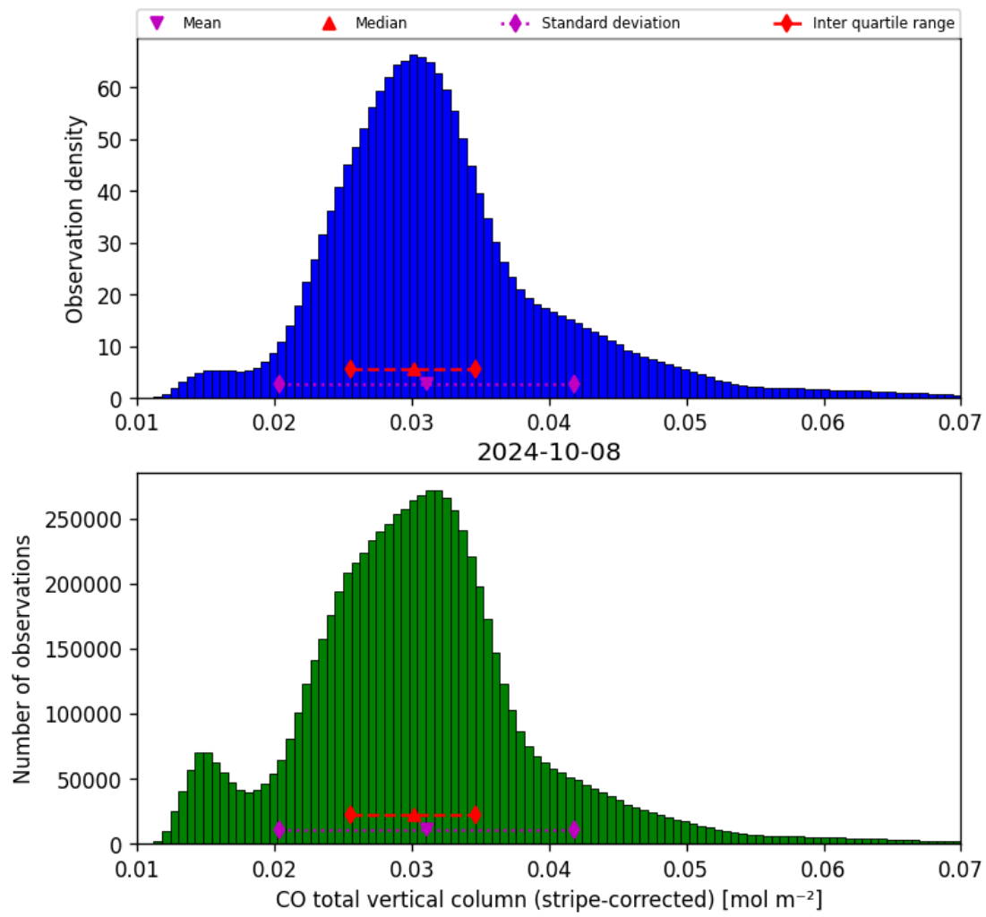
Figure 19: Histogram of “CO total vertical column (stripe-corrected)” for 2024-10-08 to 2024-10-09
