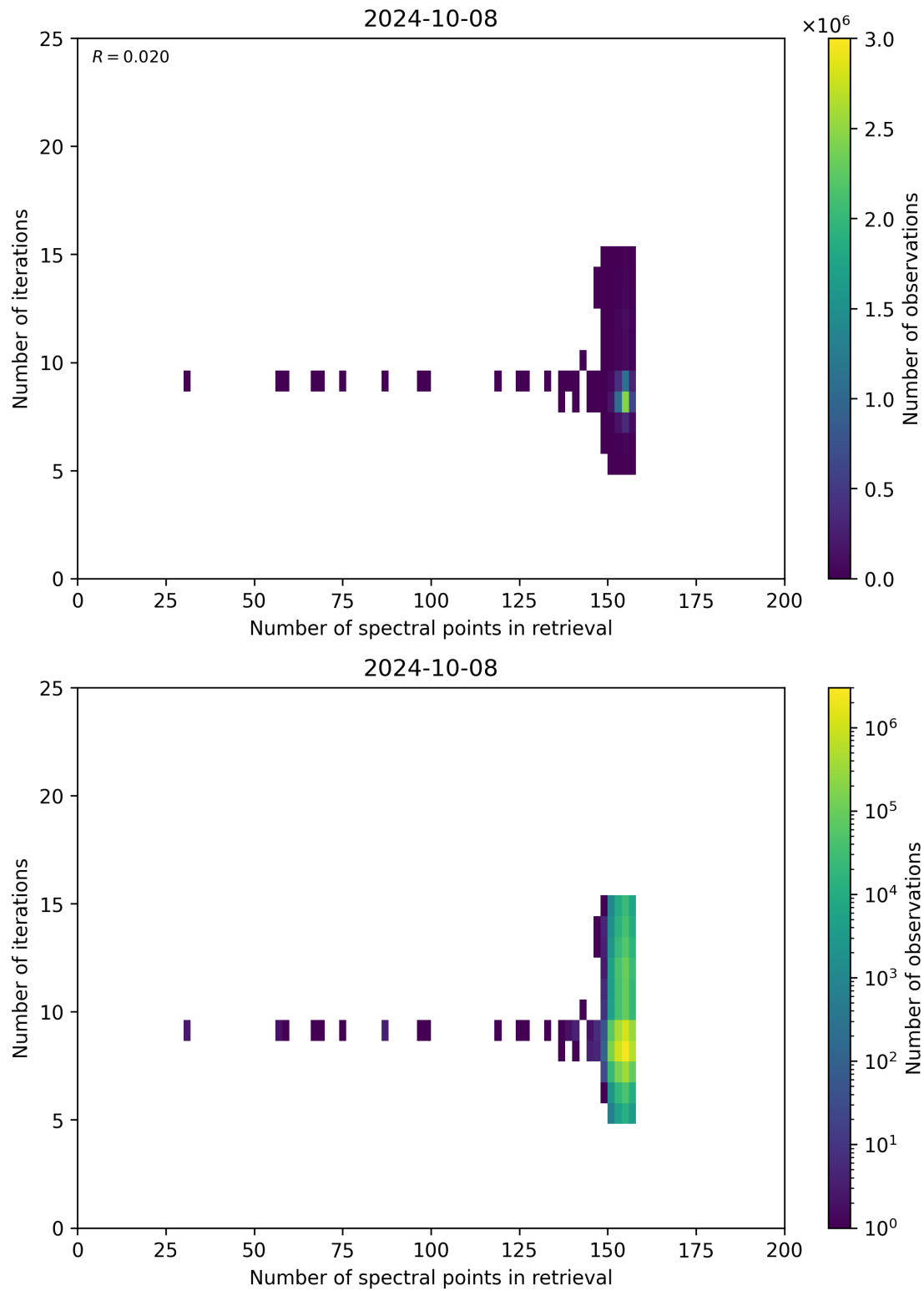
Figure 60: Scatter density plot of “Number of spectral points in retrieval” against “Number of iterations” for 2024-10-08 to 2024-10-09.
