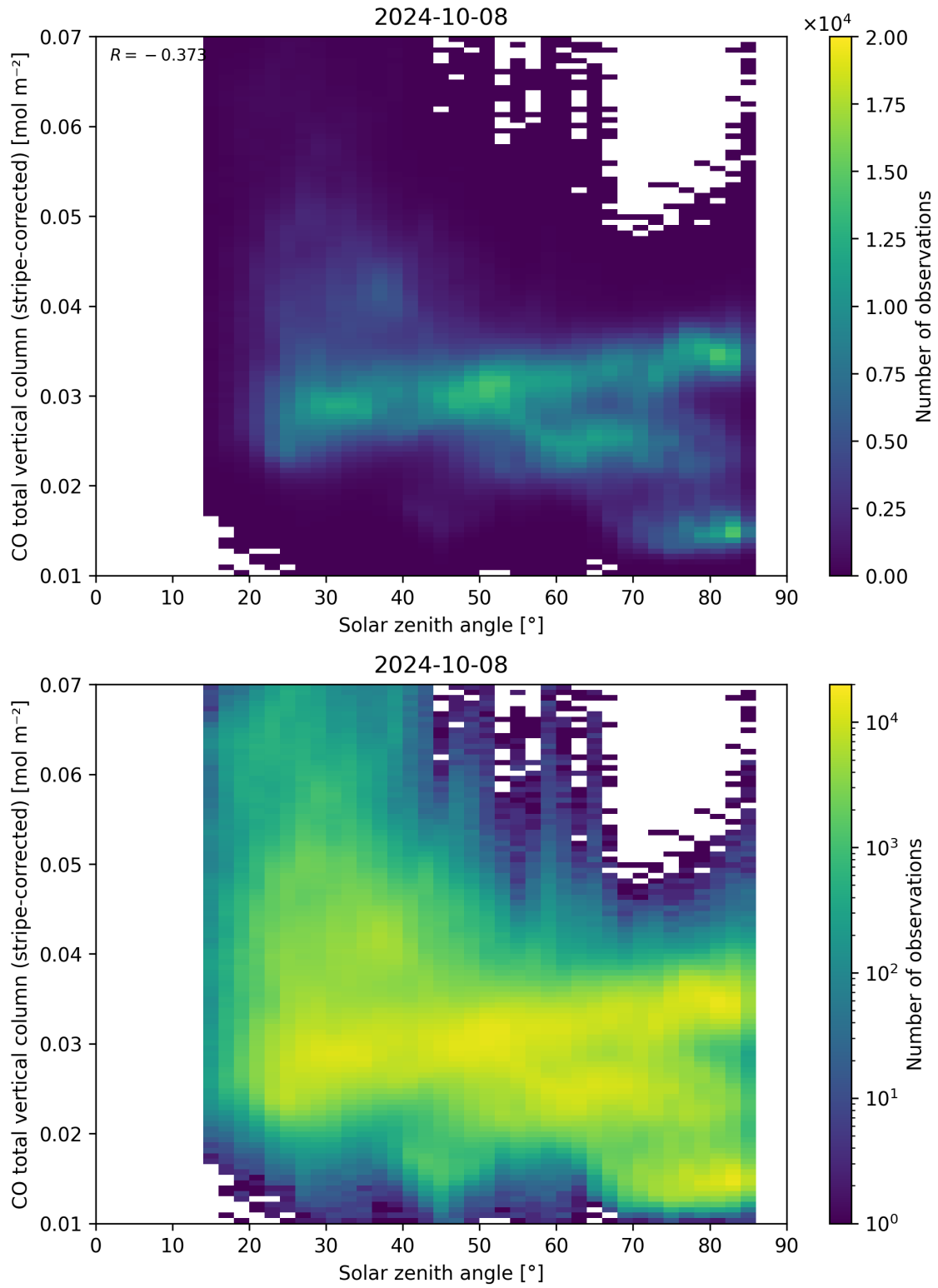
Figure 62: Scatter density plot of “Solar zenith angle” against “CO total vertical column (stripe-corrected)” for 2024-10-08 to 2024-10-09.
