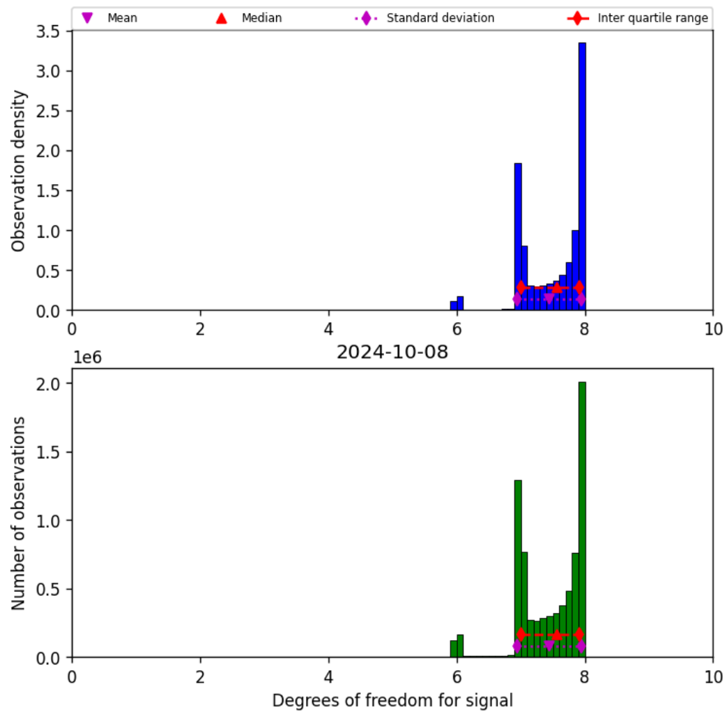
Figure 23: Histogram of “Degrees of freedom for signal” for 2024-10-08 to 2024-10-09
