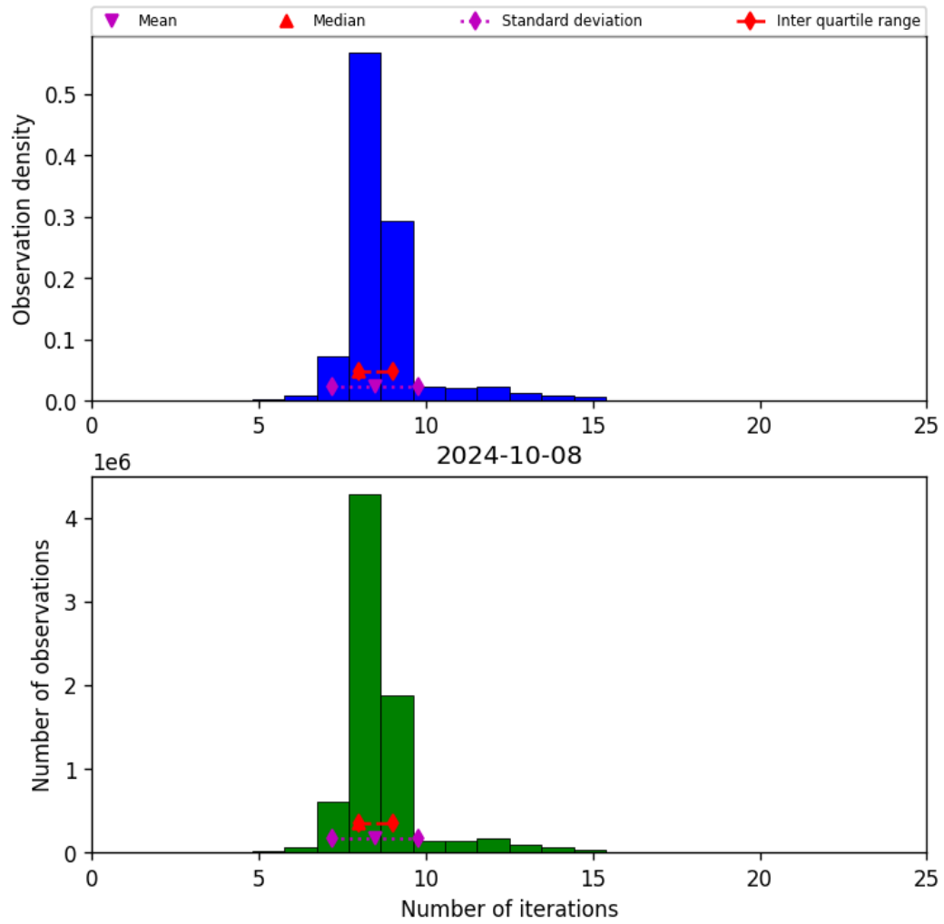
Figure 24: Histogram of “Number of iterations” for 2024-10-08 to 2024-10-09
