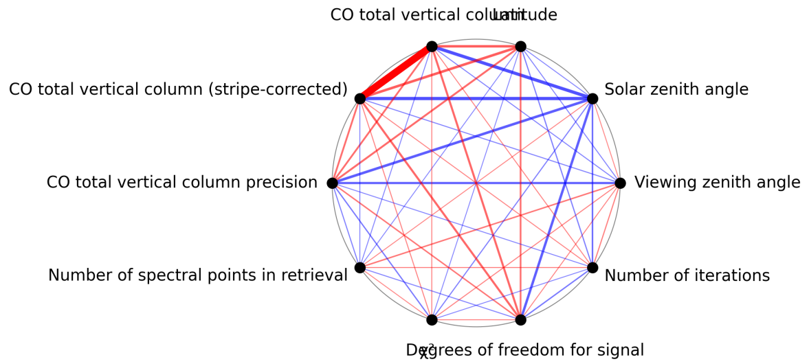
Figure 1: Map of correlation graph for 2024-10-08 to 2024-10-09.
