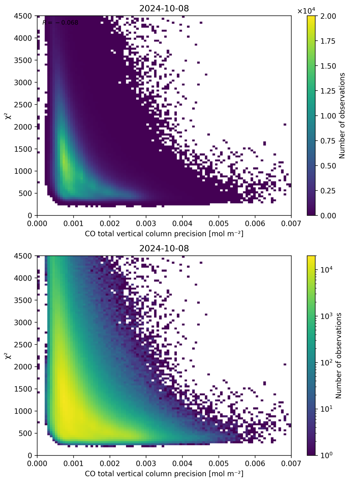
Figure 44: Scatter density plot of “CO total vertical column precision” against “ \chi^2 ” for 2024-10-08 to 2024-10-09.
