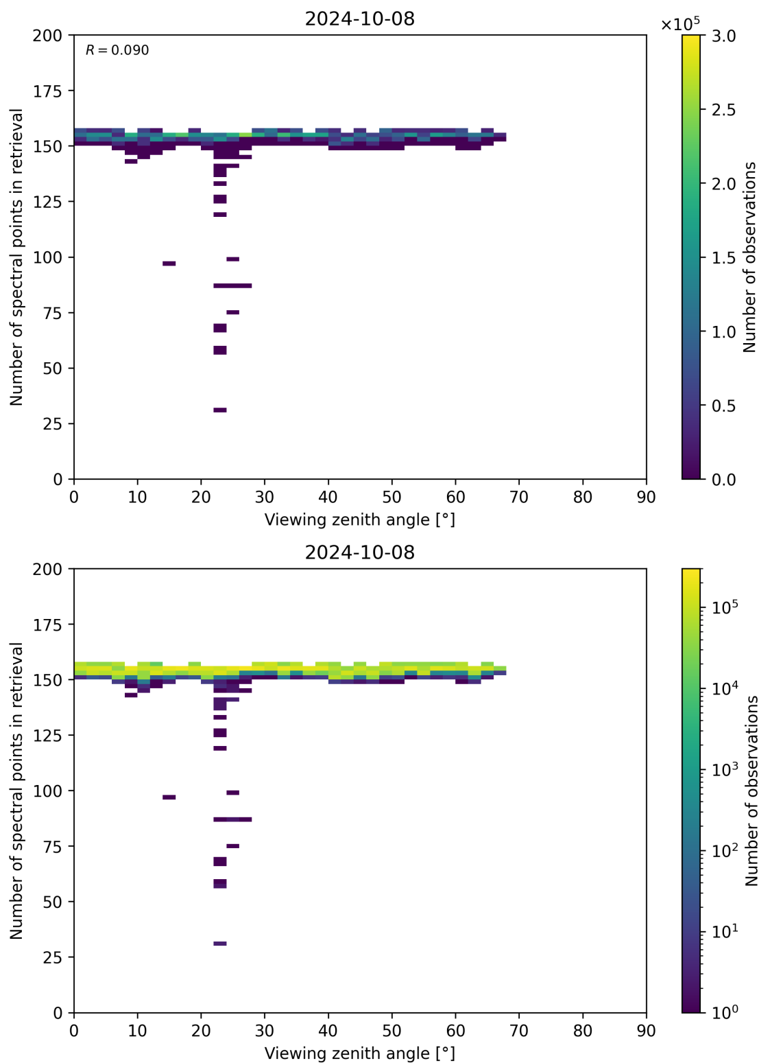
Figure 76: Scatter density plot of “Viewing zenith angle” against “Number of spectral points in retrieval” for 2024-10-08 to 2024-10-09.
