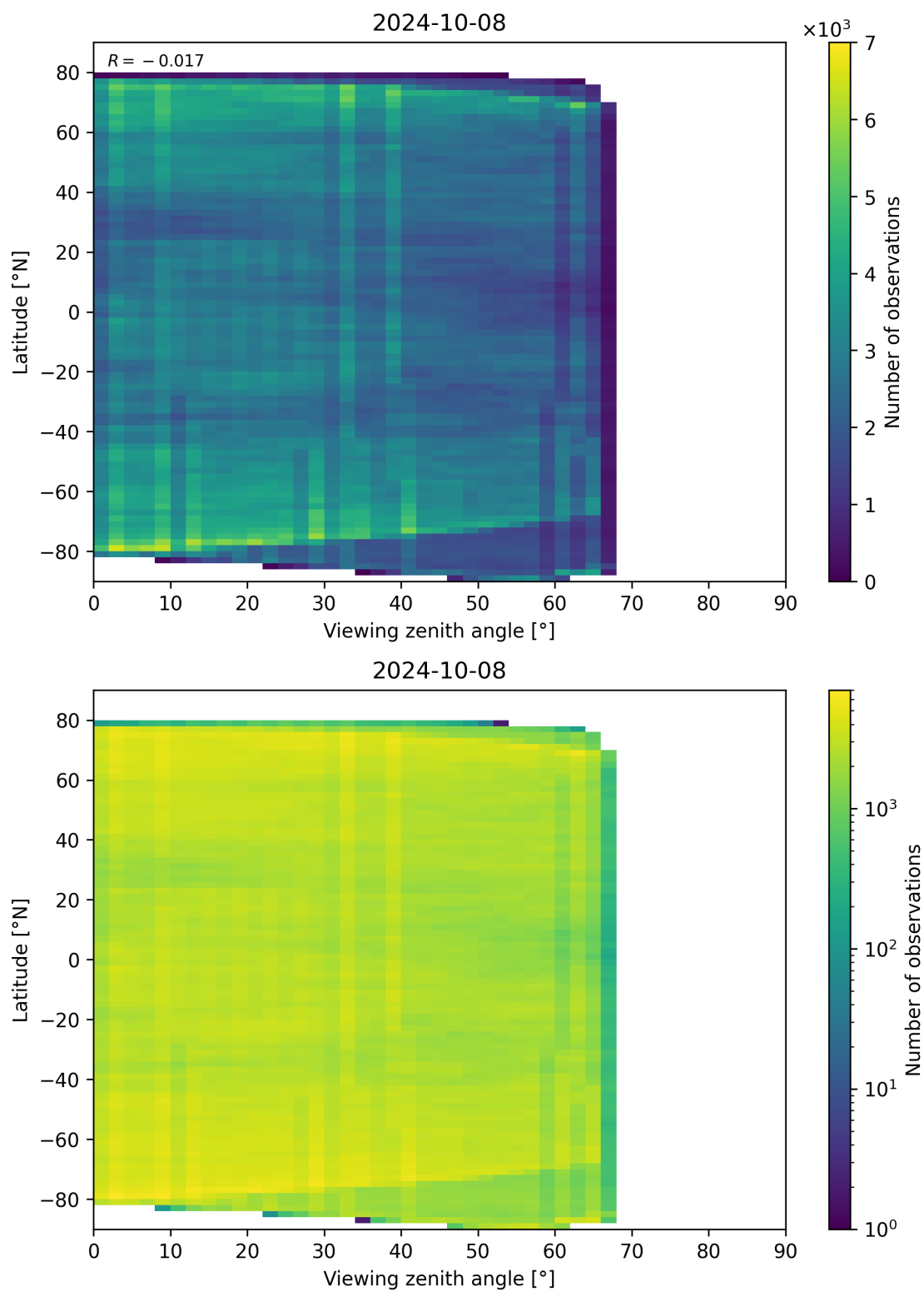
Figure 74: Scatter density plot of “Viewing zenith angle” against “Latitude” for 2024-10-08 to 2024-10-09.
