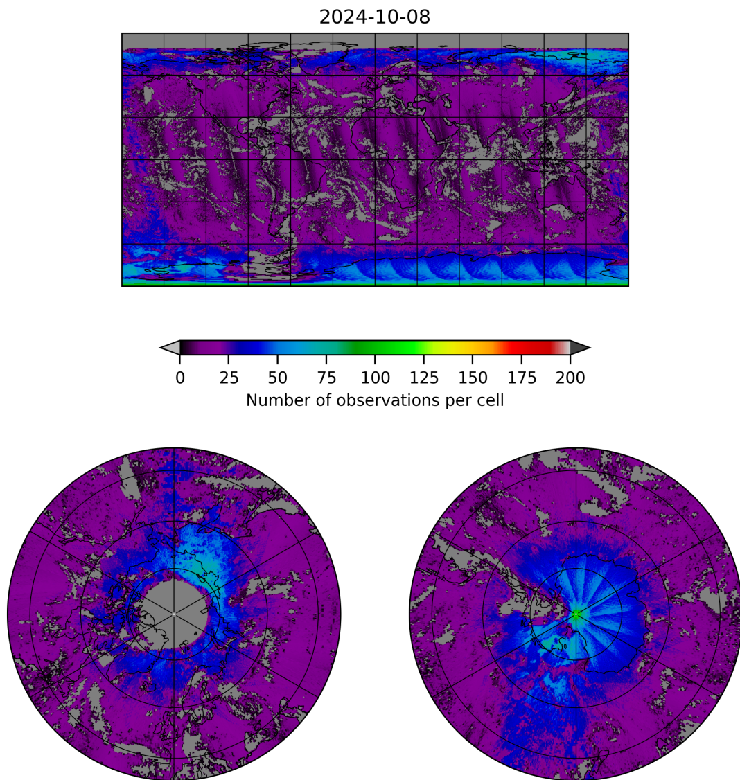
Figure 8: Map of the number of observations for 2024-10-08 to 2024-10-09
