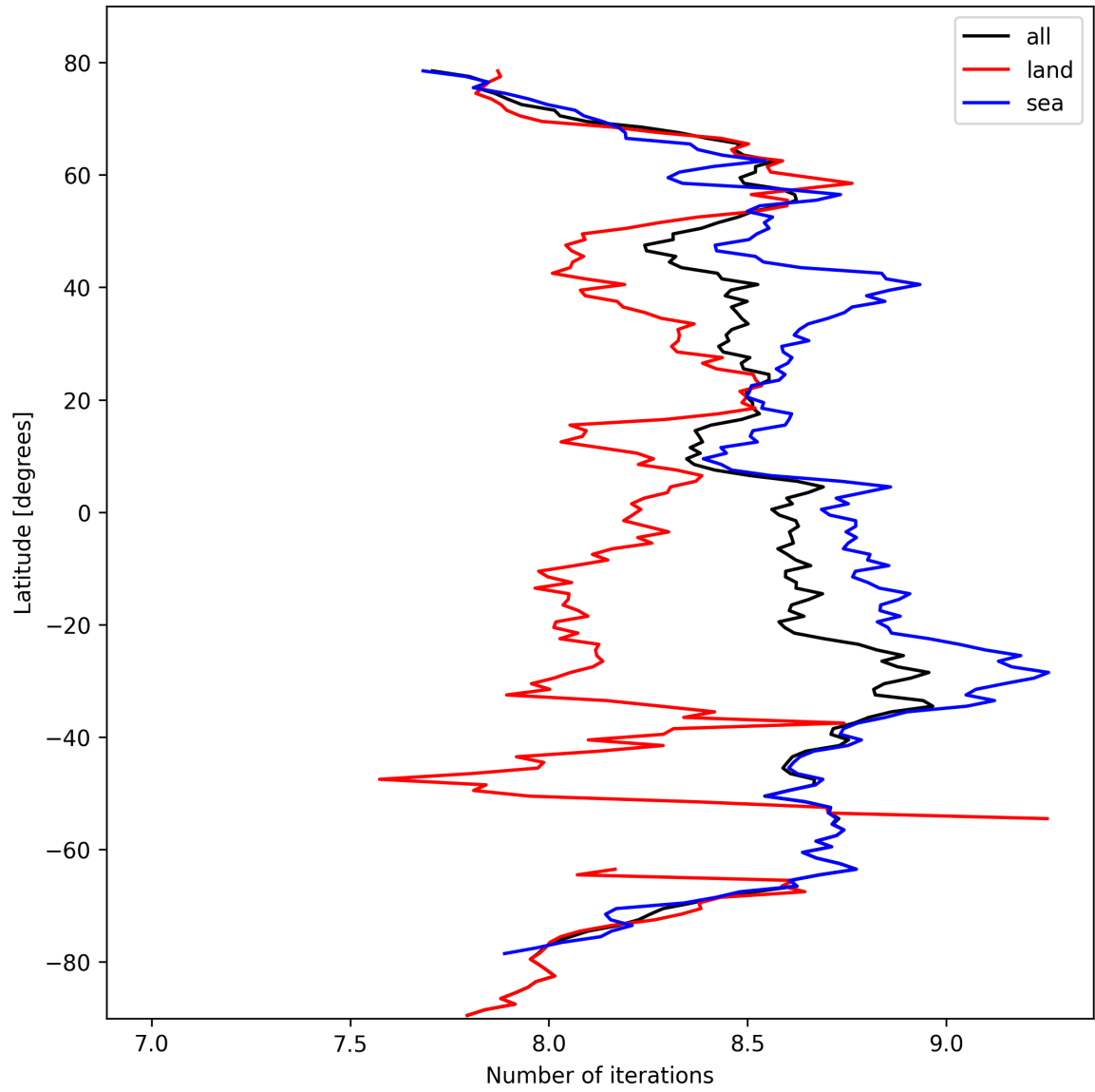
Figure 16: Zonal average of “Number of iterations” for 2024-10-08 to 2024-10-09.
