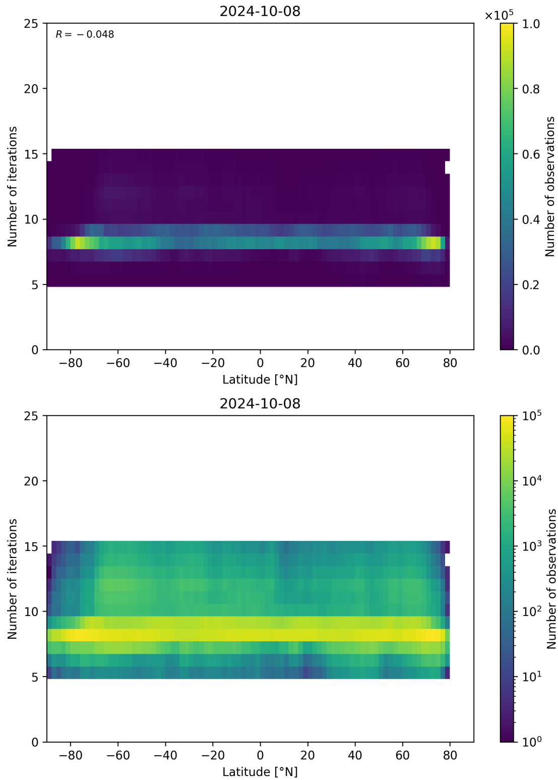
Figure 56: Scatter density plot of “Latitude” against “Number of iterations” for 2024-10-08 to 2024-10-09.
