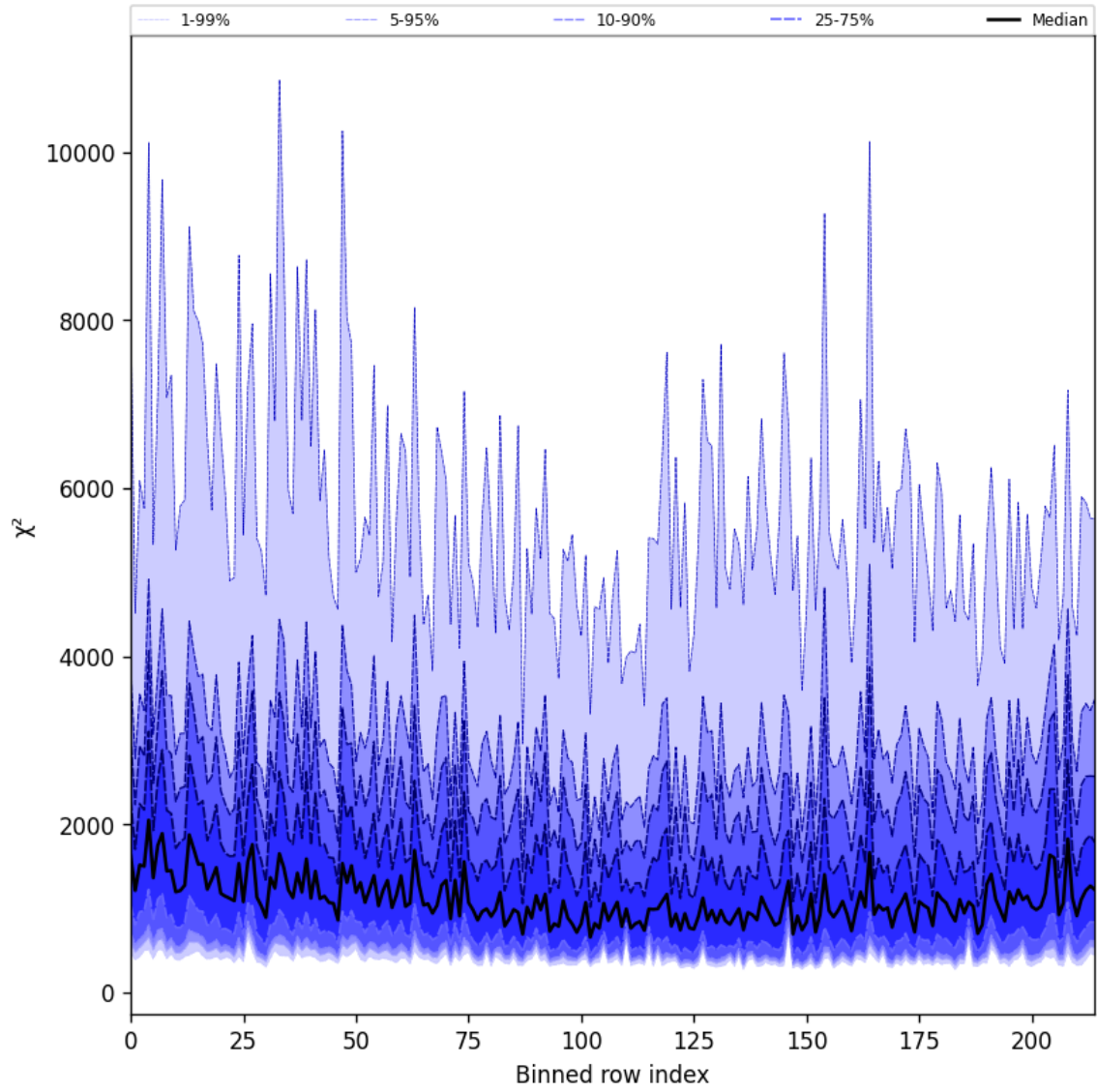
Figure 30: Along track statistics of “ \chi^2 ” for 2024-10-08 to 2024-10-09
