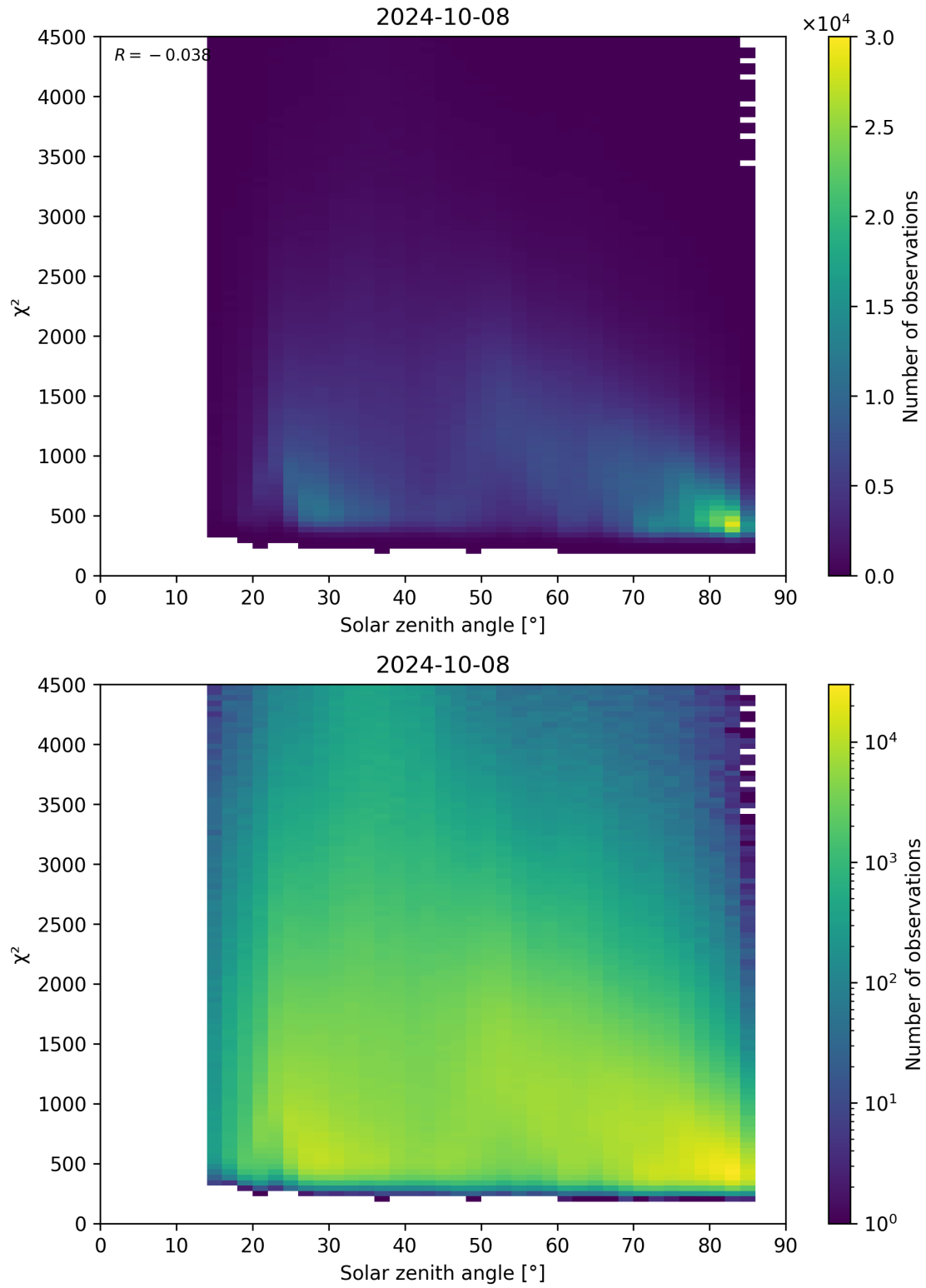
Figure 64: Scatter density plot of “Solar zenith angle” against “ \chi^2 ” for 2024-10-08 to 2024-10-09.
