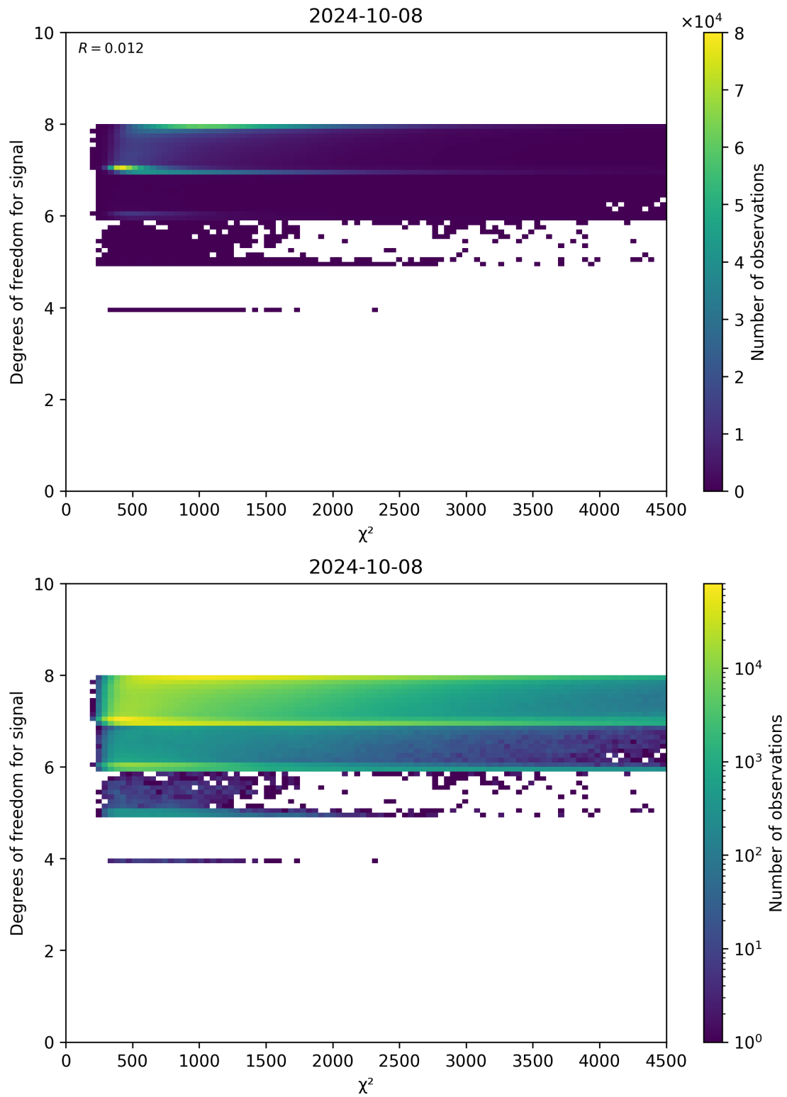
Figure 48: Scatter density plot of “ \chi^2 ” against “Degrees of freedom for signal” for 2024-10-08 to 2024-10-09.
