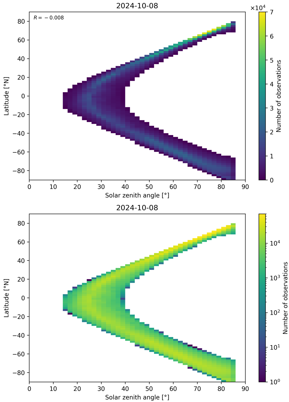
Figure 66: Scatter density plot of “Solar zenith angle” against “Latitude” for 2024-10-08 to 2024-10-09.
