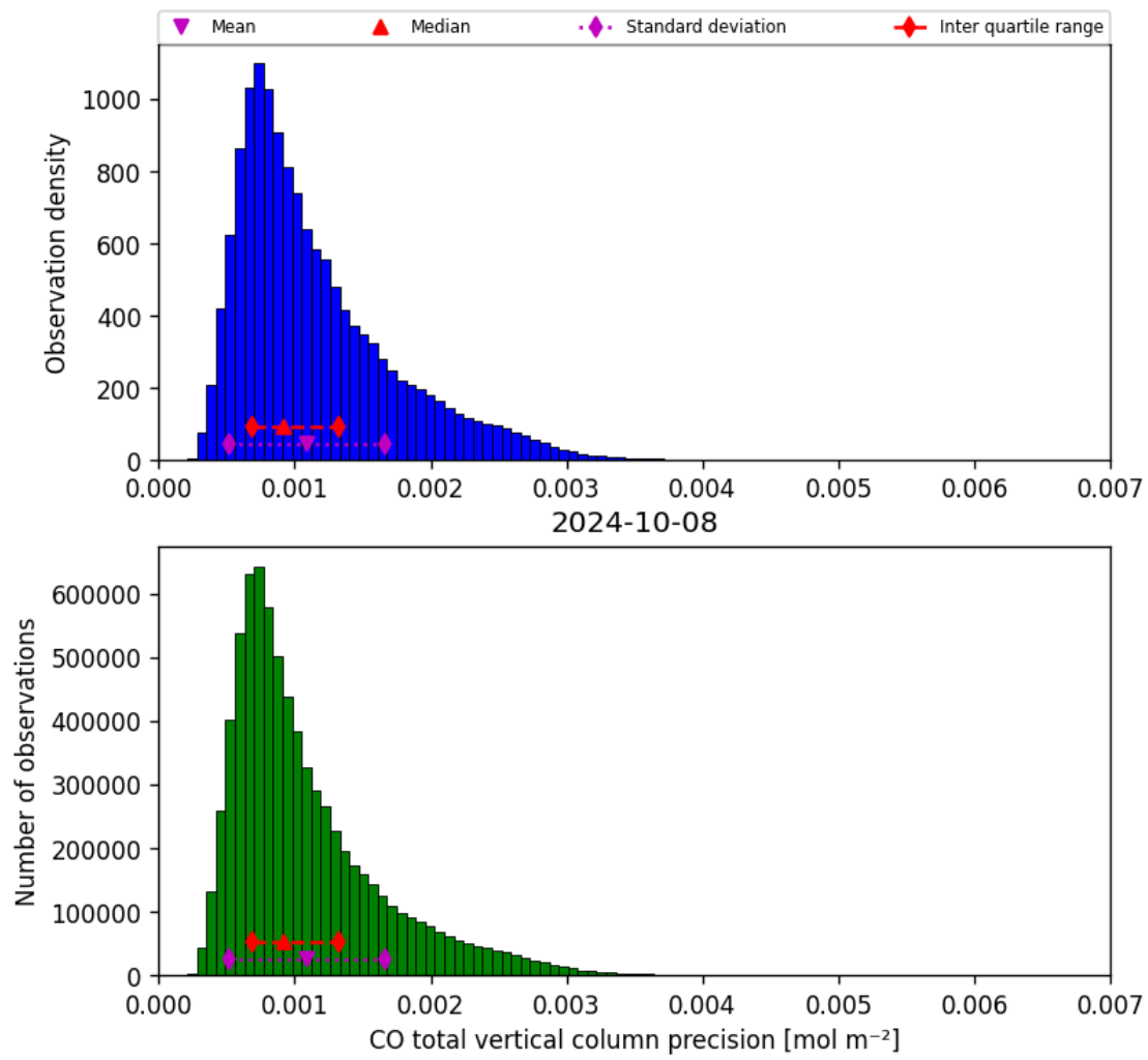
Figure 20: Histogram of “CO total vertical column precision” for 2024-10-08 to 2024-10-09
