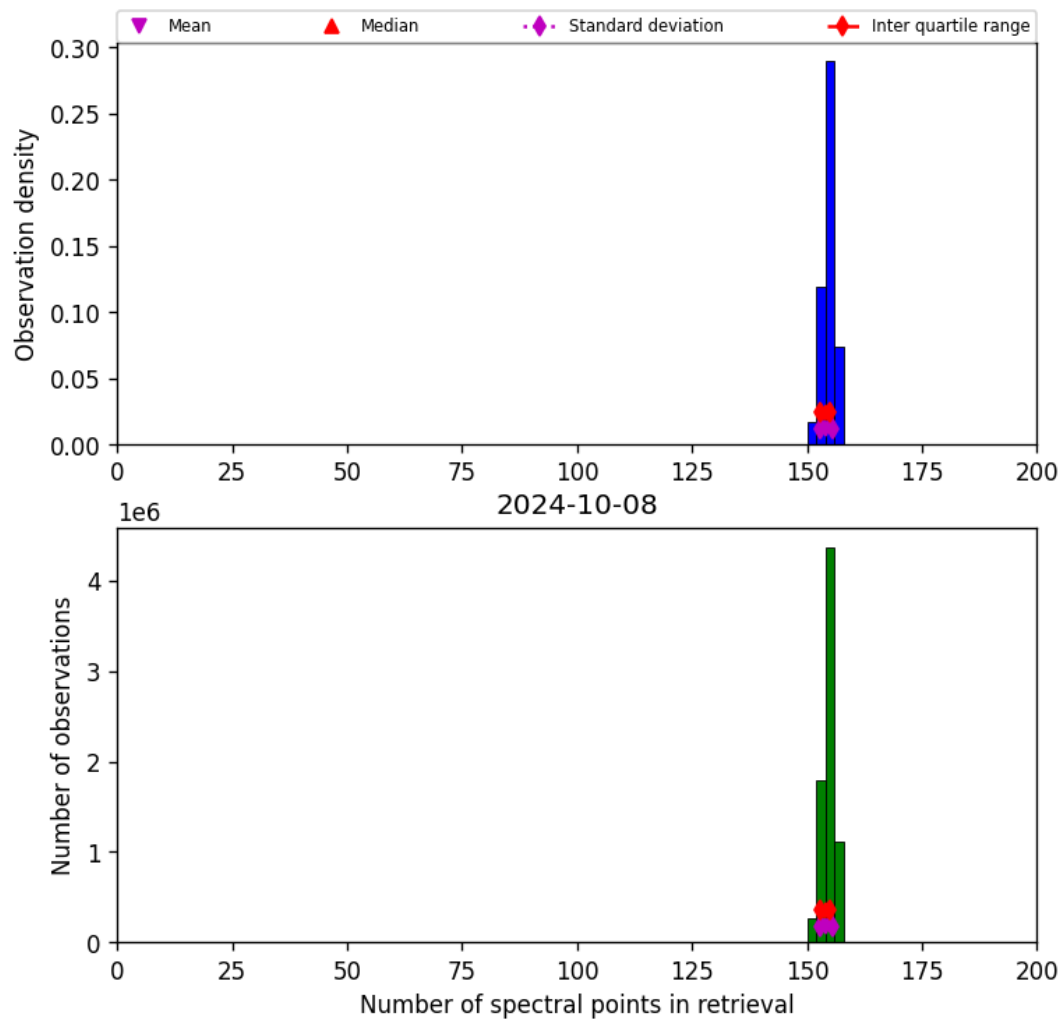
Figure 21: Histogram of “Number of spectral points in retrieval” for 2024-10-08 to 2024-10-09
