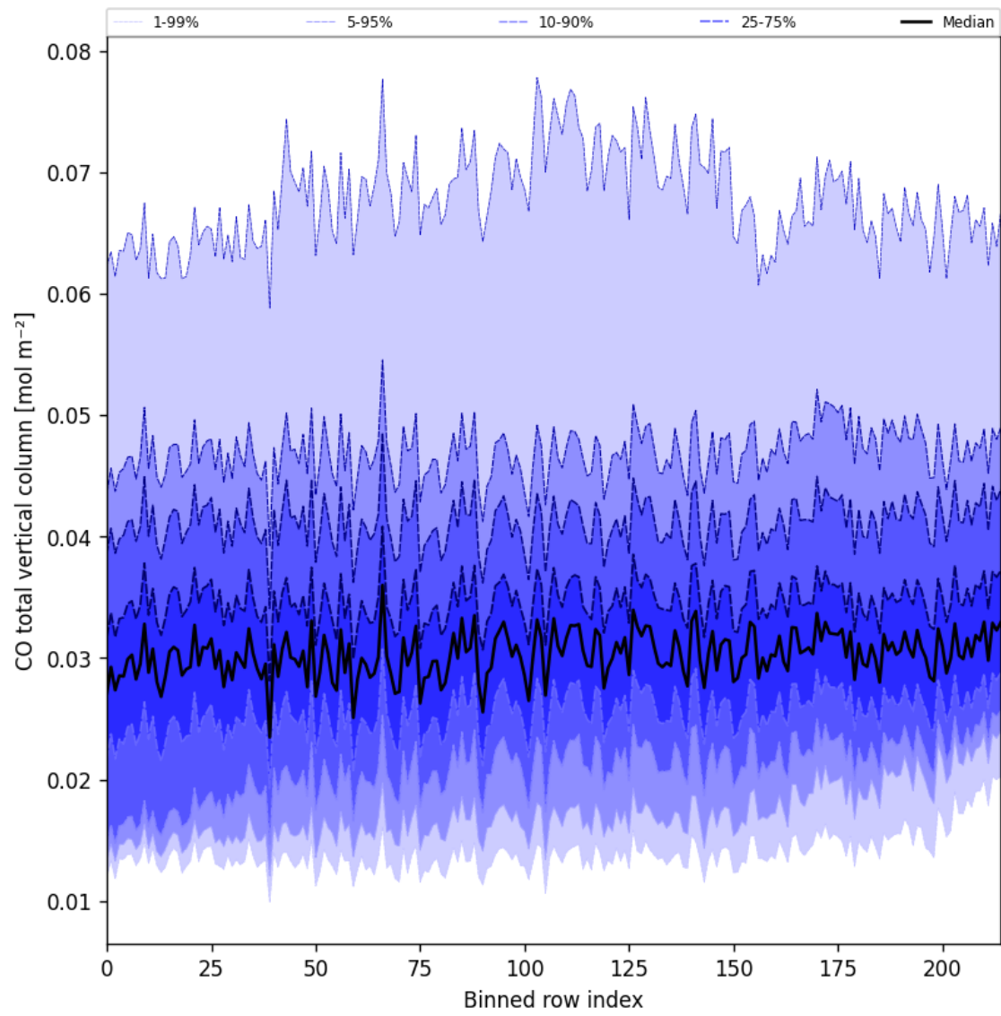
Figure 26: Along track statistics of “CO total vertical column” for 2024-10-08 to 2024-10-09
