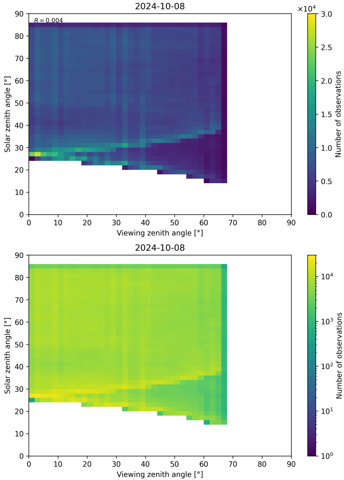
Figure 77: Scatter density plot of “Viewing zenith angle” against “Solar zenith angle” for 2024-10-08 to 2024-10-09.
