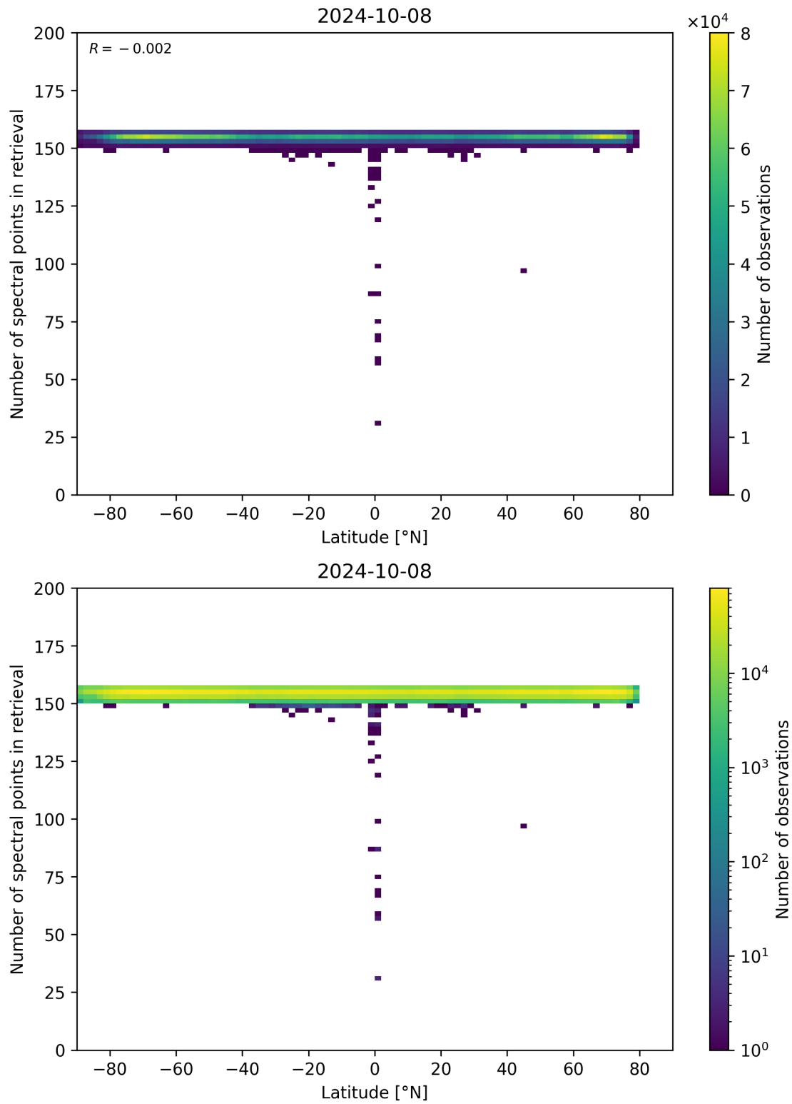
Figure 57: Scatter density plot of “Latitude” against “Number of spectral points in retrieval” for 2024-10-08 to 2024-10-09.
