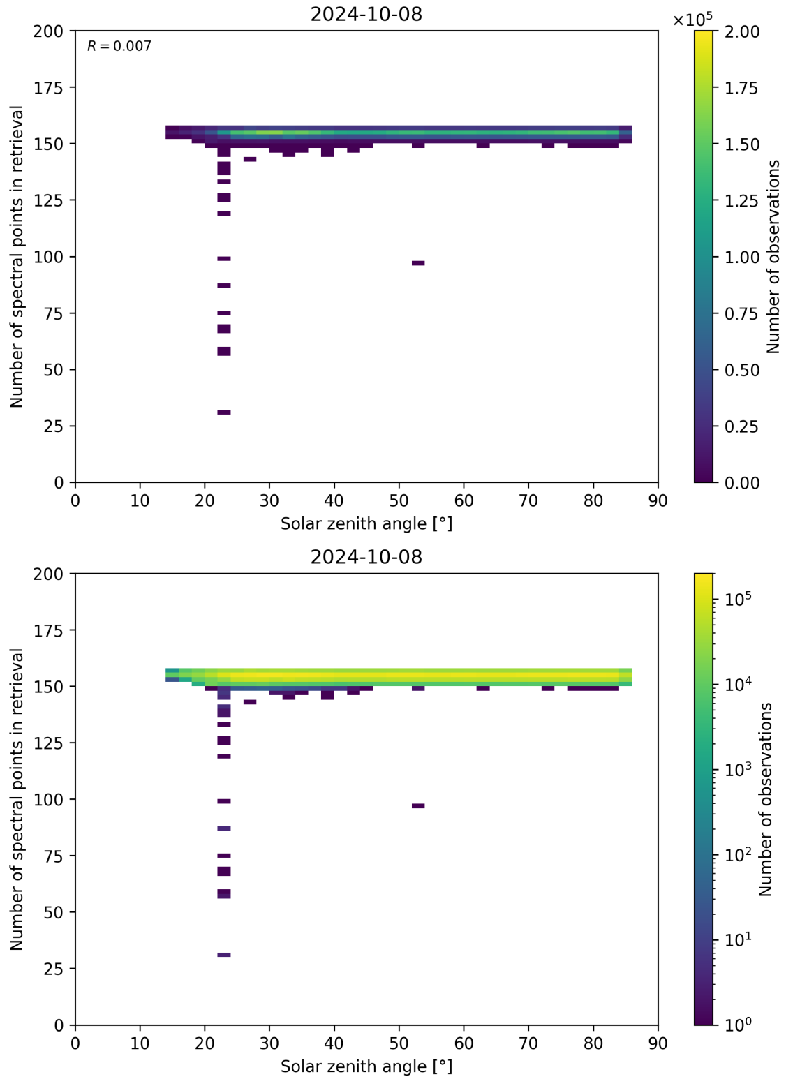
Figure 68: Scatter density plot of “Solar zenith angle” against “Number of spectral points in retrieval” for 2024-10-08 to 2024-10-09.
