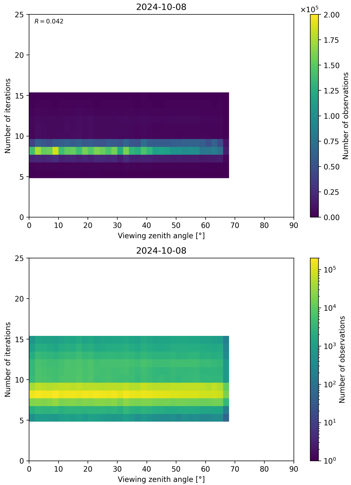
Figure 75: Scatter density plot of “Viewing zenith angle” against “Number of iterations” for 2024-10-08 to 2024-10-09.
