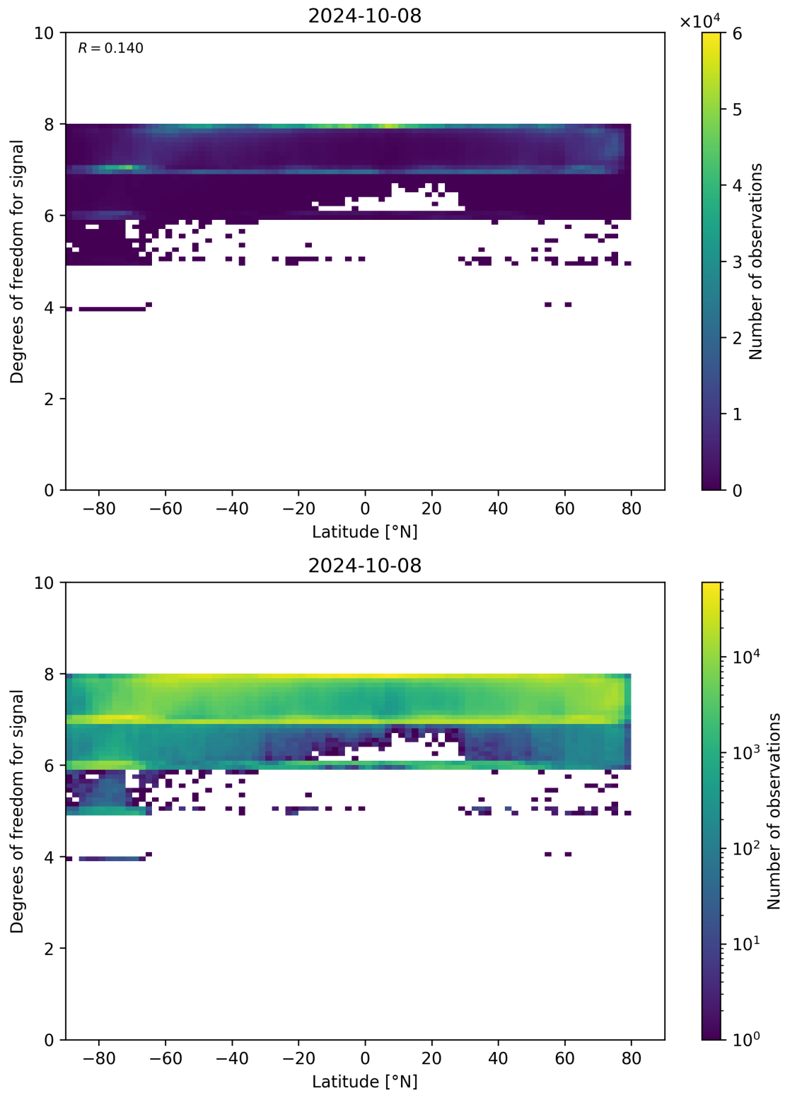
Figure 55: Scatter density plot of “Latitude” against “Degrees of freedom for signal” for 2024-10-08 to 2024-10-09.
