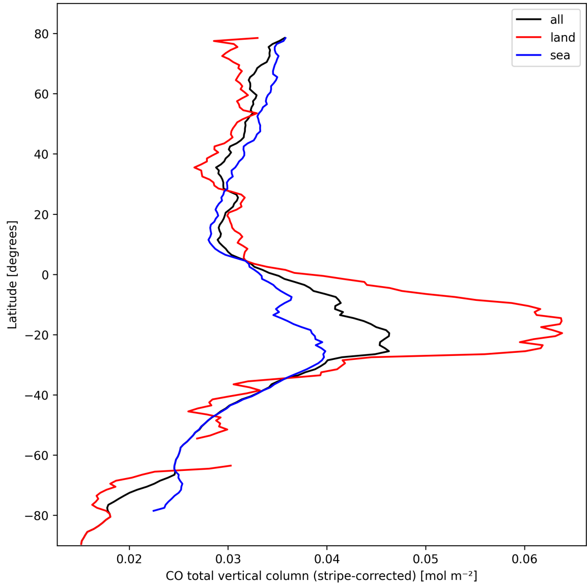
Figure 11: Zonal average of “CO total vertical column (stripe-corrected)” for 2024-10-08 to 2024-10-09.
