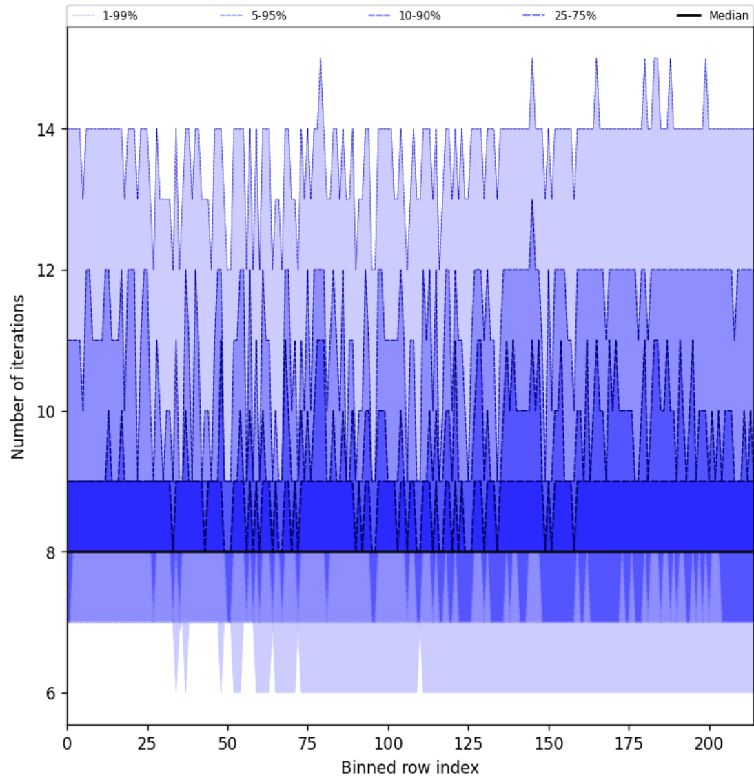
Figure 32: Along track statistics of “Number of iterations” for 2024-10-08 to 2024-10-09
