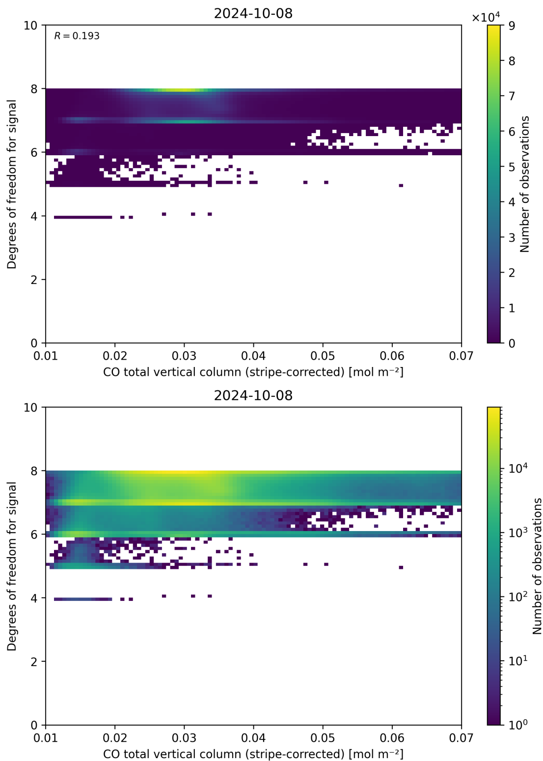
Figure 38: Scatter density plot of “CO total vertical column (stripe-corrected)” against “Degrees of freedom for signal” for 2024-10-08 to 2024-10-09.
