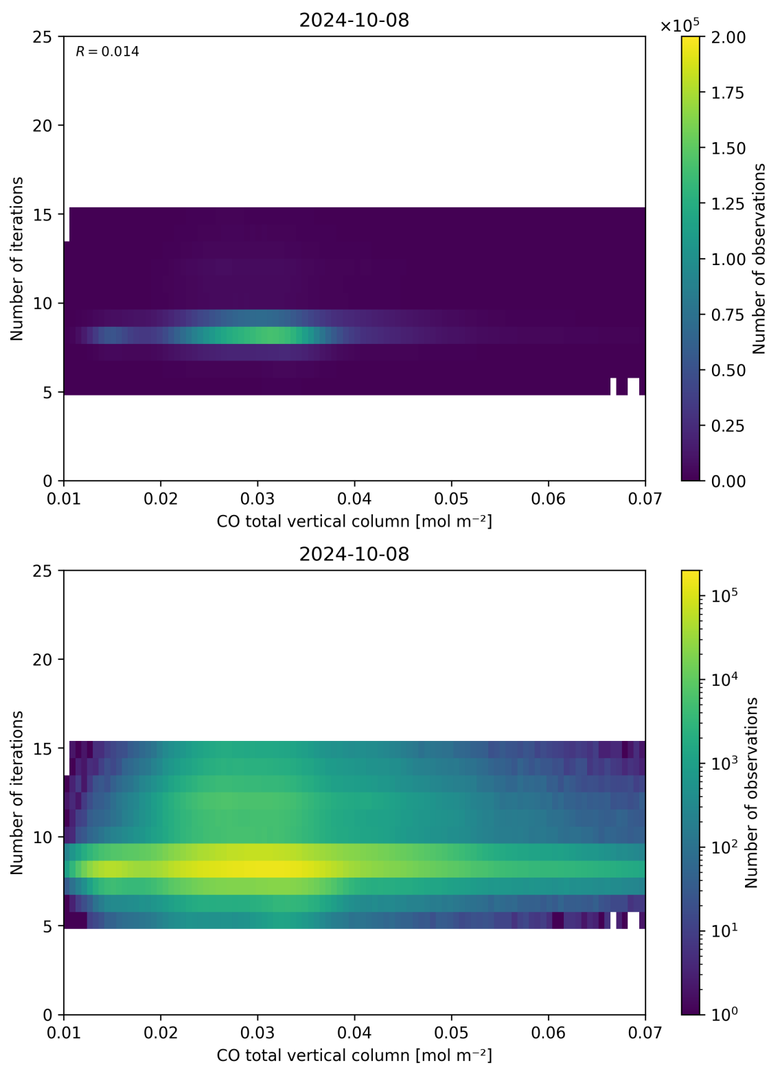
Figure 42: Scatter density plot of “CO total vertical column” against “Number of iterations” for 2024-10-08 to 2024-10-09.
