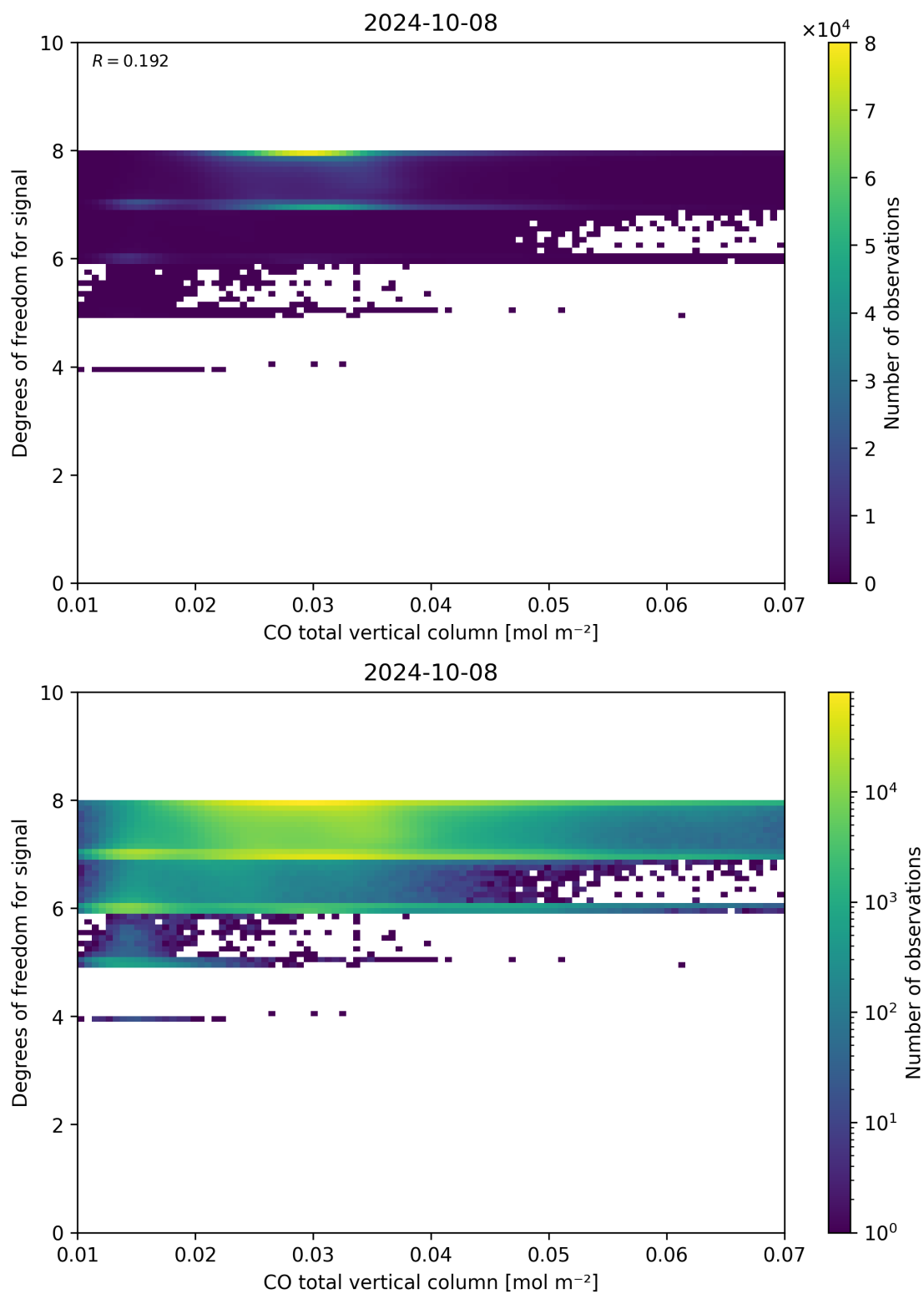
Figure 41: Scatter density plot of “CO total vertical column” against “Degrees of freedom for signal” for 2024-10-08 to 2024-10-09.
