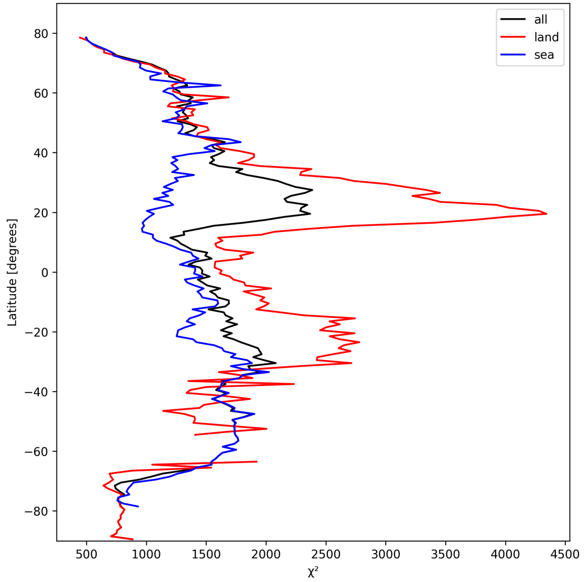
Figure 14: Zonal average of “ \chi^2 ” for 2024-10-08 to 2024-10-09.
