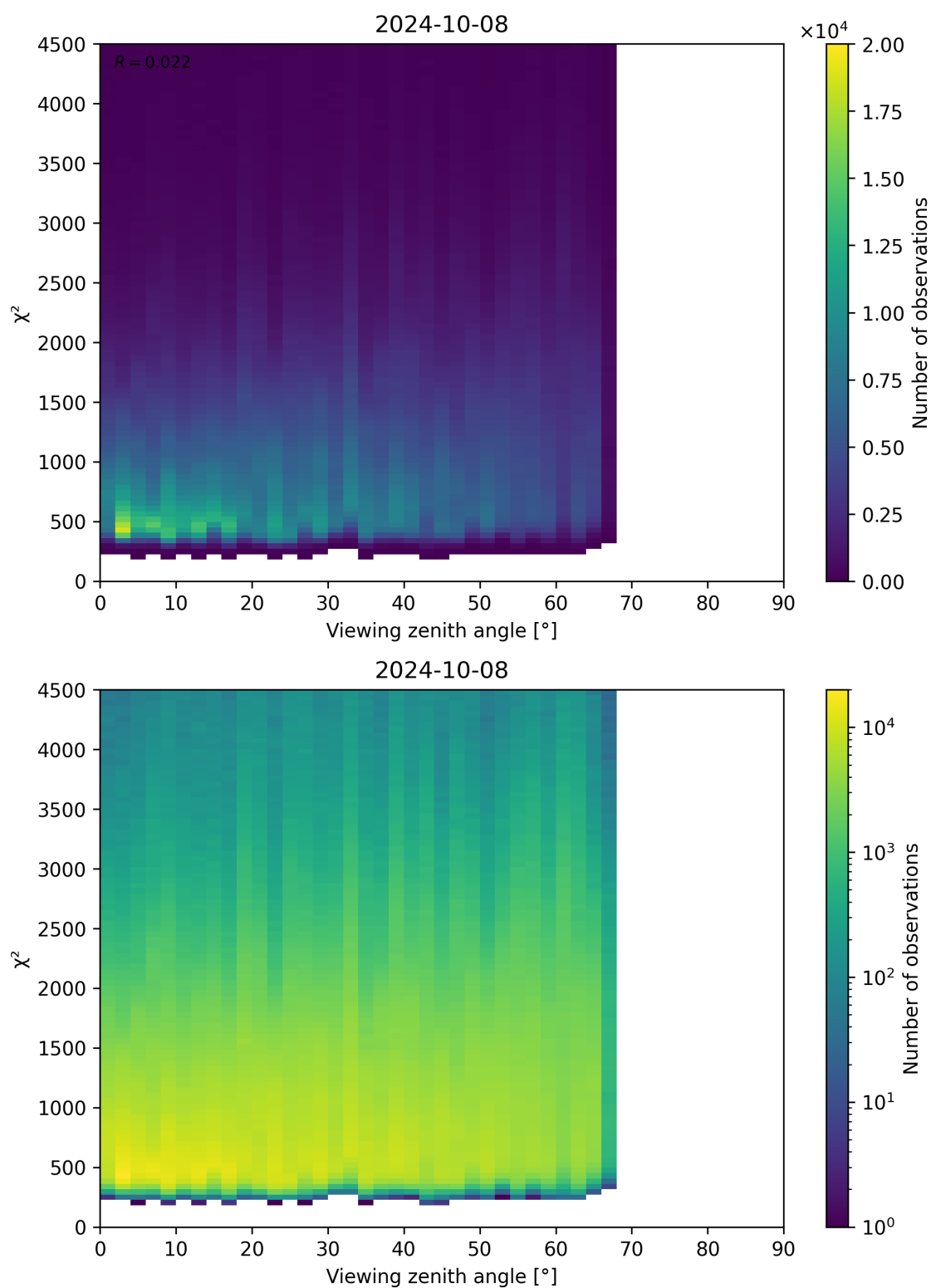
Figure 72: Scatter density plot of “Viewing zenith angle” against “ \chi^2 ” for 2024-10-08 to 2024-10-09.
