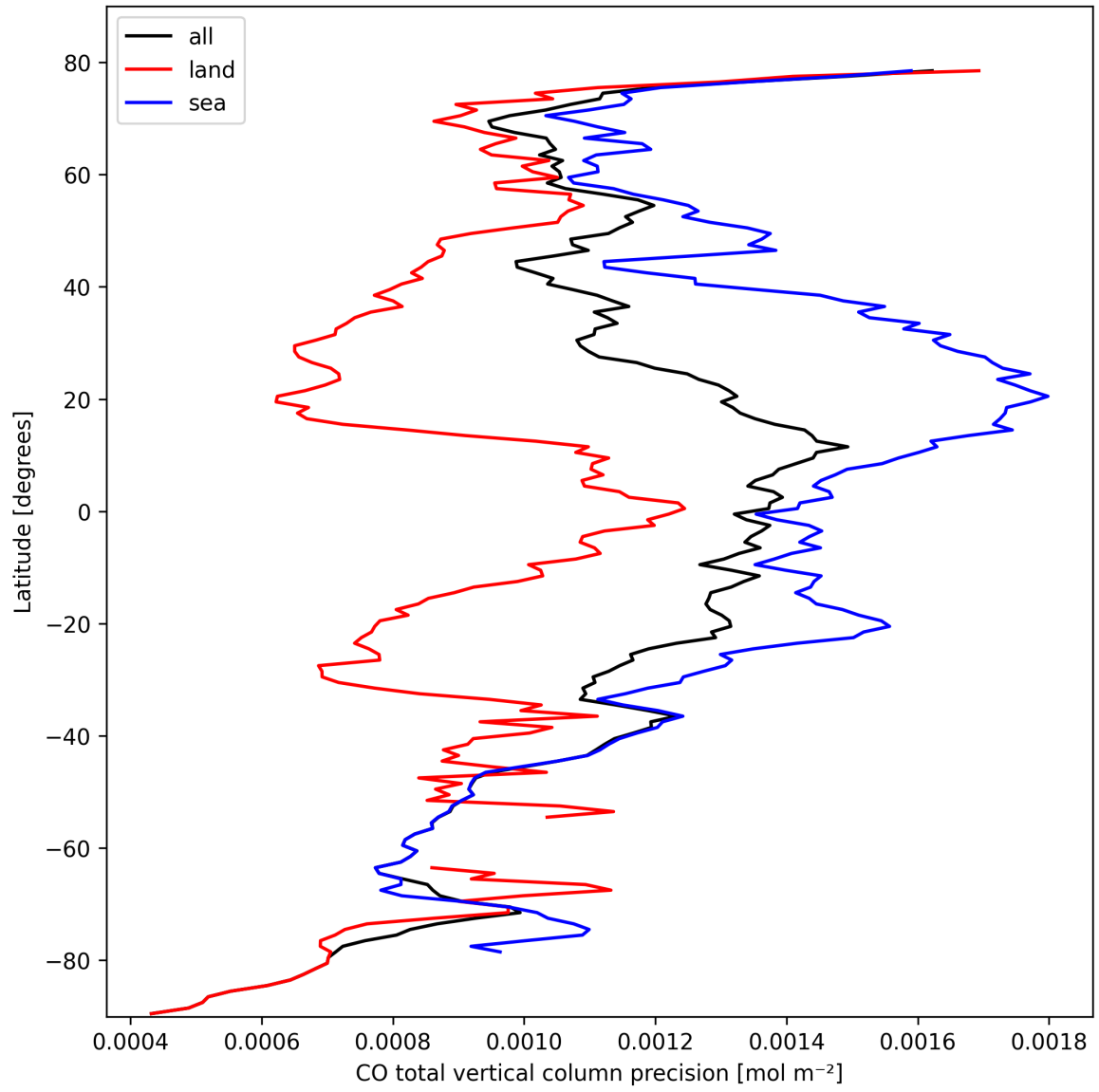
Figure 12: Zonal average of "CO total vertical column precision" for 2024-10-08 to 2024-10-09.
