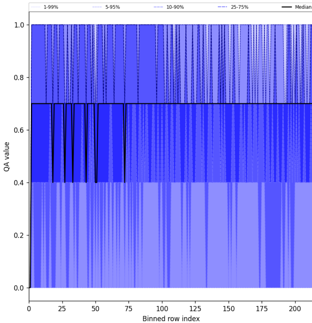
Figure 25: Along track statistics of “QA value” for 2024-10-08 to 2024-10-09
