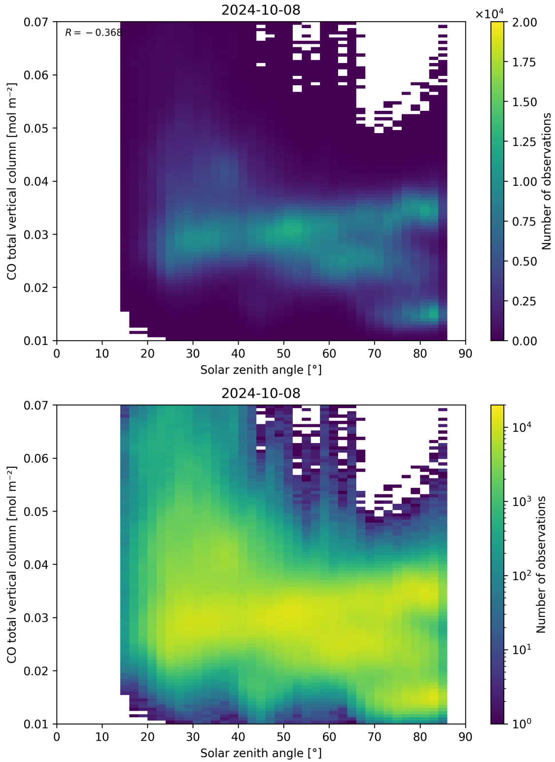
Figure 61: Scatter density plot of “Solar zenith angle” against “CO total vertical column” for 2024-10-08 to 2024-10-09.
