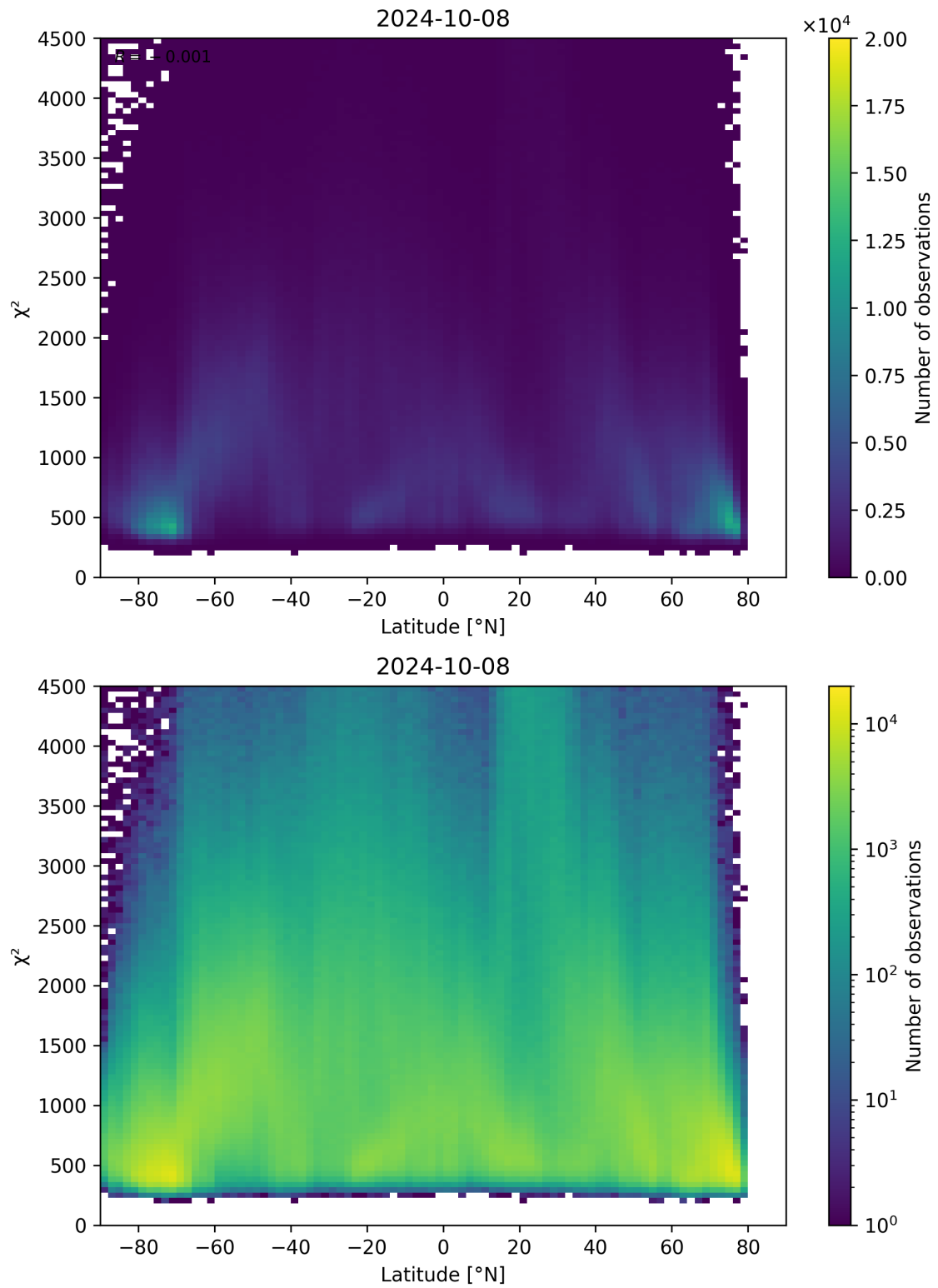
Figure 54: Scatter density plot of “Latitude” against “ \chi^2 ” for 2024-10-08 to 2024-10-09.
