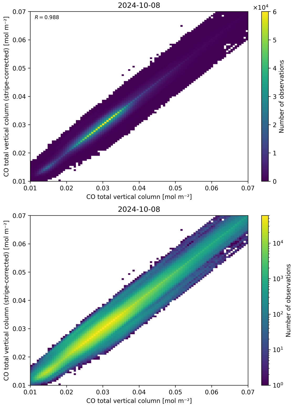
Figure 33: Scatter density plot of “CO total vertical column” against “CO total vertical column (stripe-corrected)” for 2024-10-08 to 2024-10-09.
