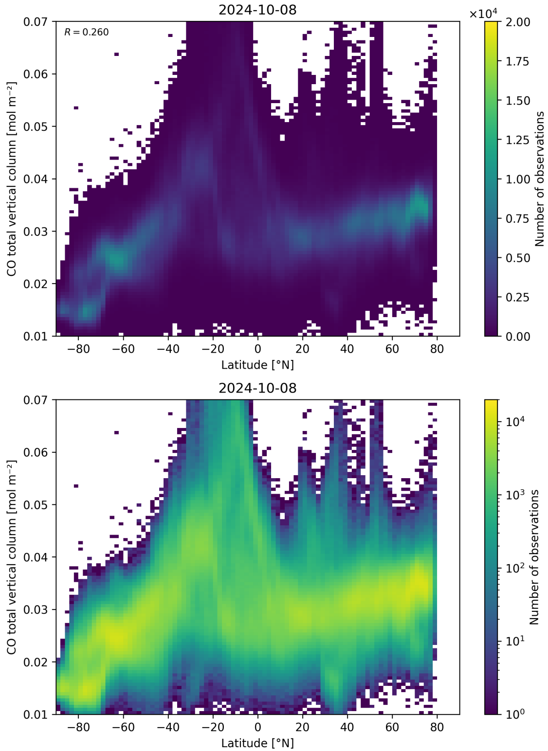
Figure 51: Scatter density plot of “Latitude” against “CO total vertical column” for 2024-10-08 to 2024-10-09.
