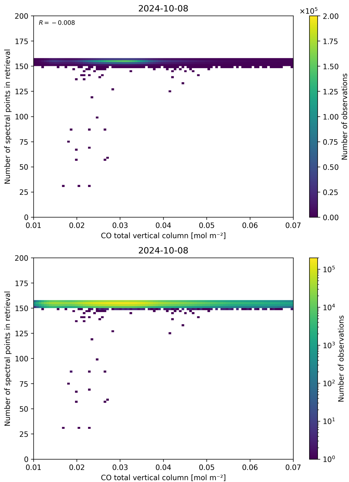
Figure 43: Scatter density plot of “CO total vertical column” against “Number of spectral points in retrieval” for 2024-10-08 to 2024-10-09.
