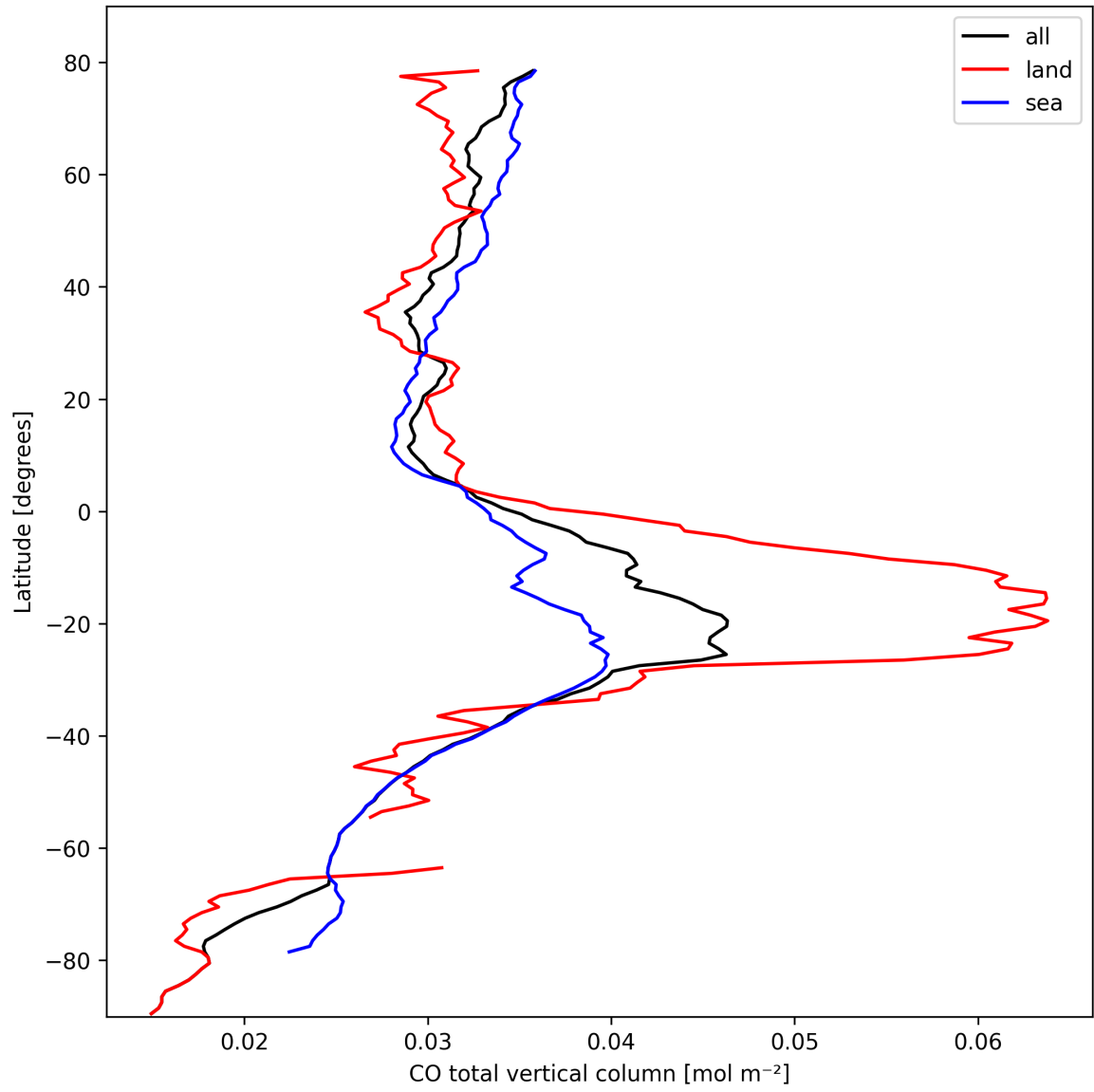
Figure 10: Zonal average of “CO total vertical column” for 2024-10-08 to 2024-10-09.
