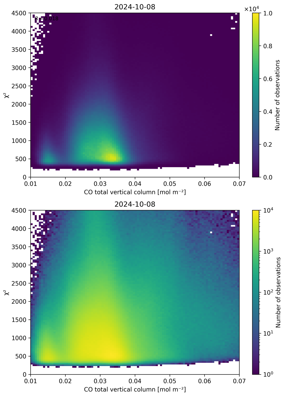
Figure 35: Scatter density plot of “CO total vertical column” against “ \chi^2 ” for 2024-10-08 to 2024-10-09.
