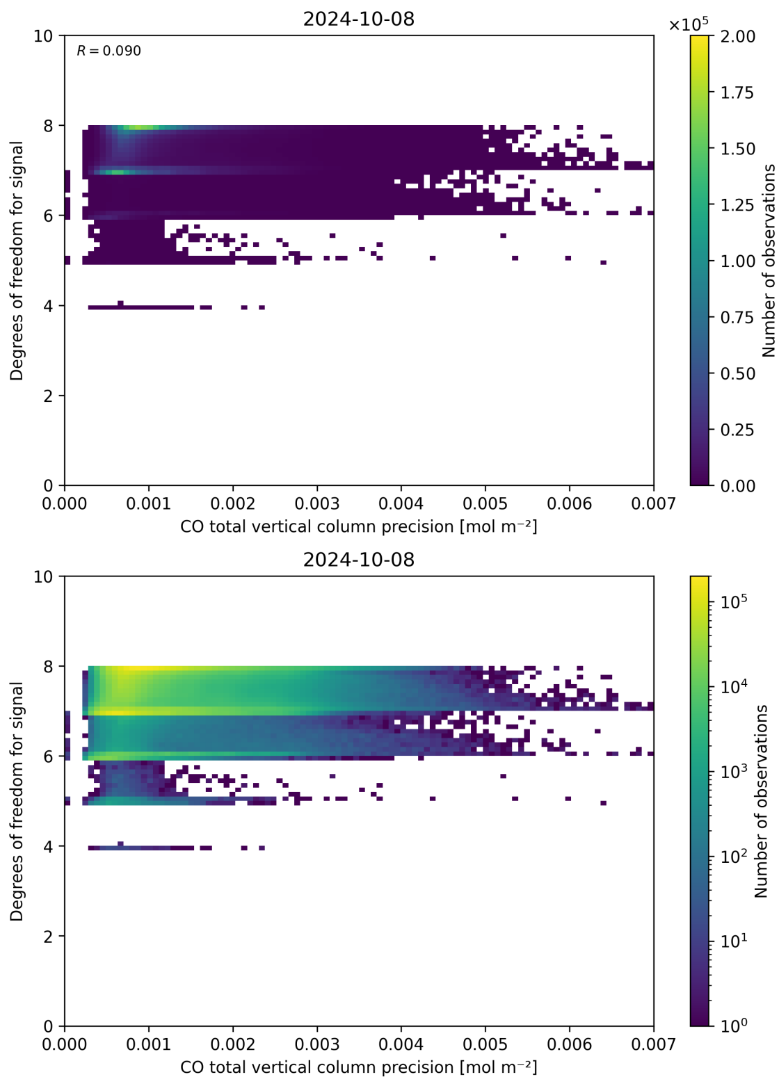
Figure 45: Scatter density plot of “CO total vertical column precision” against “Degrees of freedom for signal” for 2024-10-08 to 2024-10-09.
