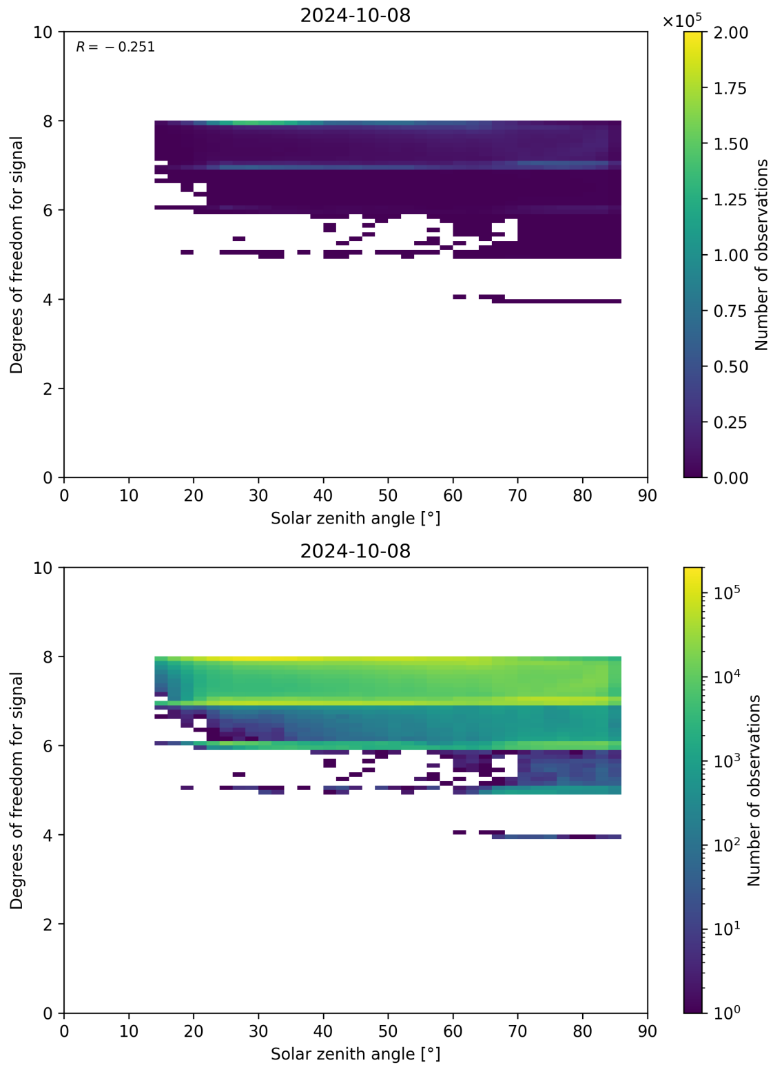
Figure 65: Scatter density plot of “Solar zenith angle” against “Degrees of freedom for signal” for 2024-10-08 to 2024-10-09.
