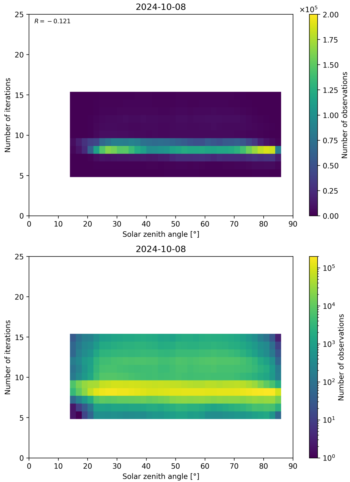
Figure 67: Scatter density plot of “Solar zenith angle” against “Number of iterations” for 2024-10-08 to 2024-10-09.
