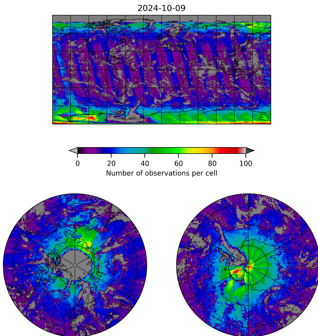
Figure 8: Map of the number of observations for 2024-10-08 to 2024-10-10
