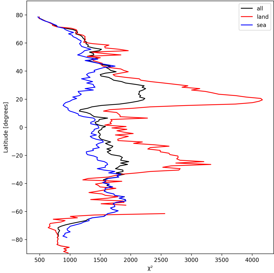
Figure 14: Zonal average of “ \chi^2 ” for 2024-10-08 to 2024-10-10.
