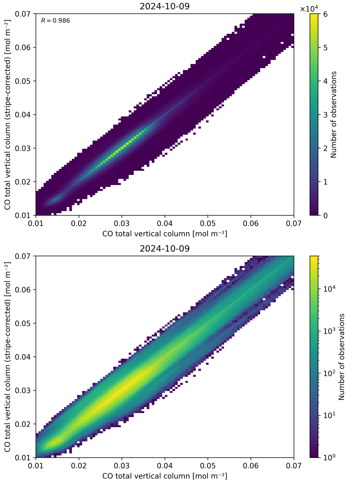
Figure 33: Scatter density plot of “CO total vertical column” against “CO total vertical column (stripe-corrected)” for 2024-10-08 to 2024-10-10.
