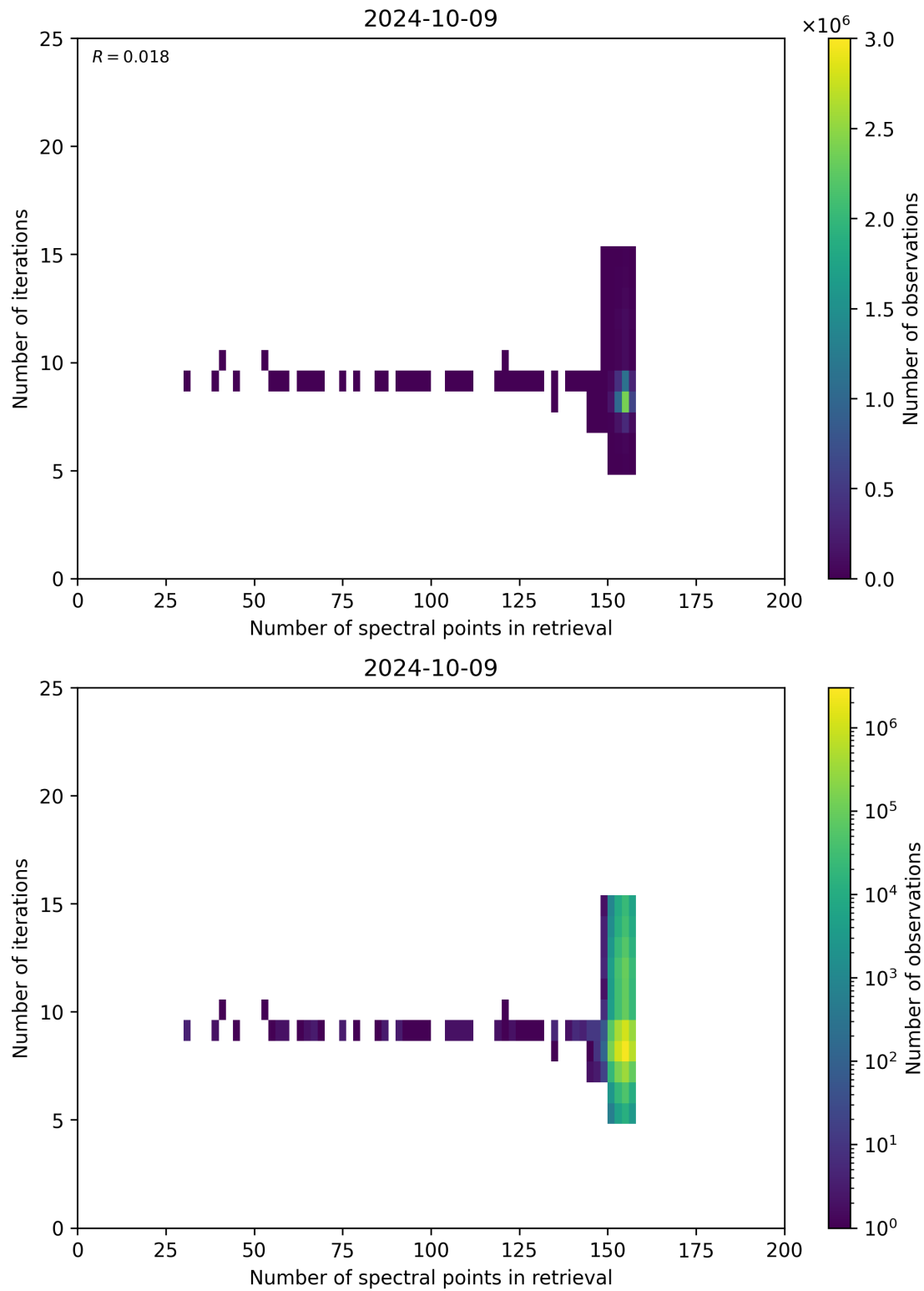
Figure 60: Scatter density plot of “Number of spectral points in retrieval” against “Number of iterations” for 2024-10-08 to 2024-10-10.
