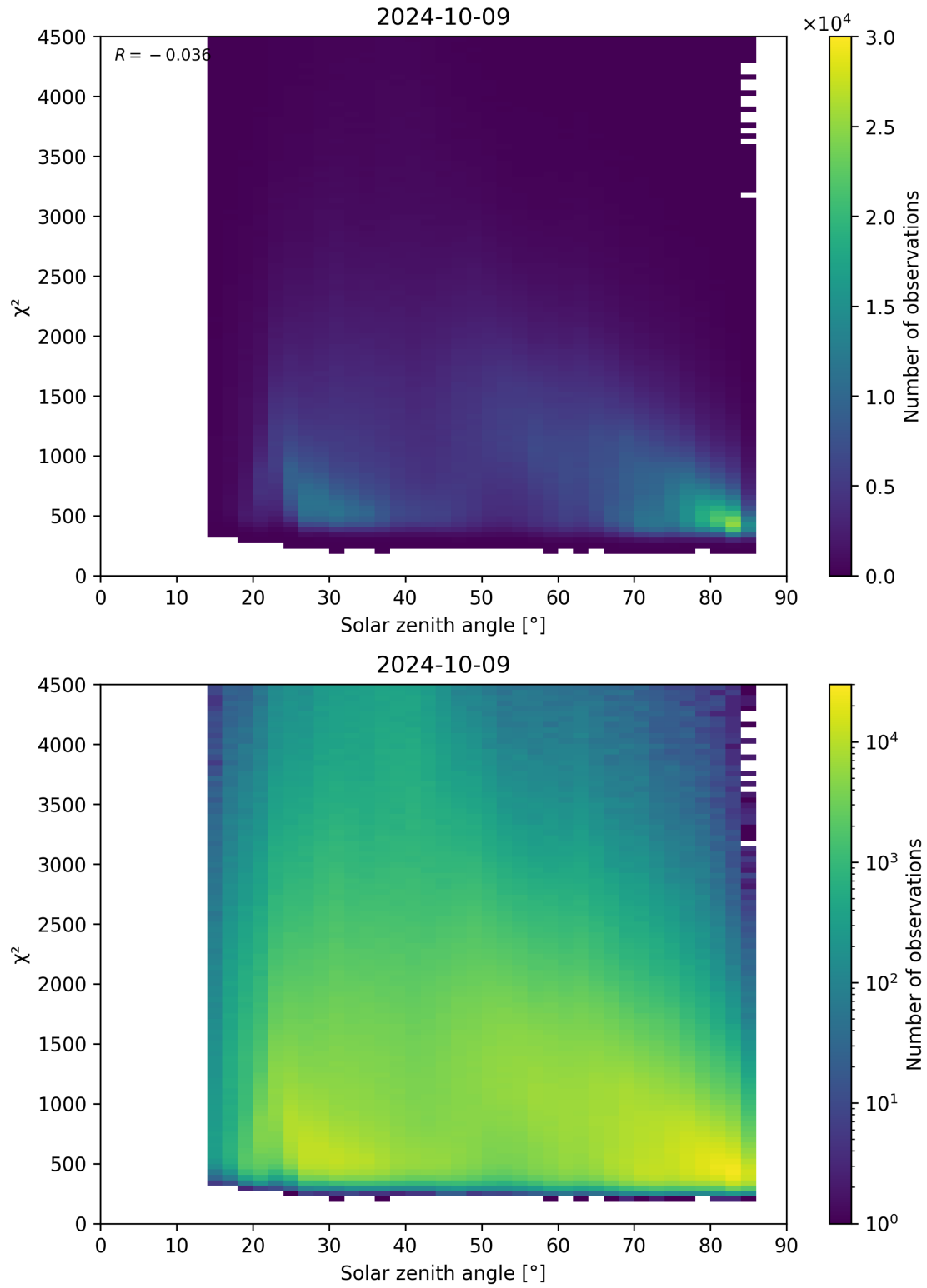
Figure 64: Scatter density plot of “Solar zenith angle” against “ \chi^2 ” for 2024-10-08 to 2024-10-10.
