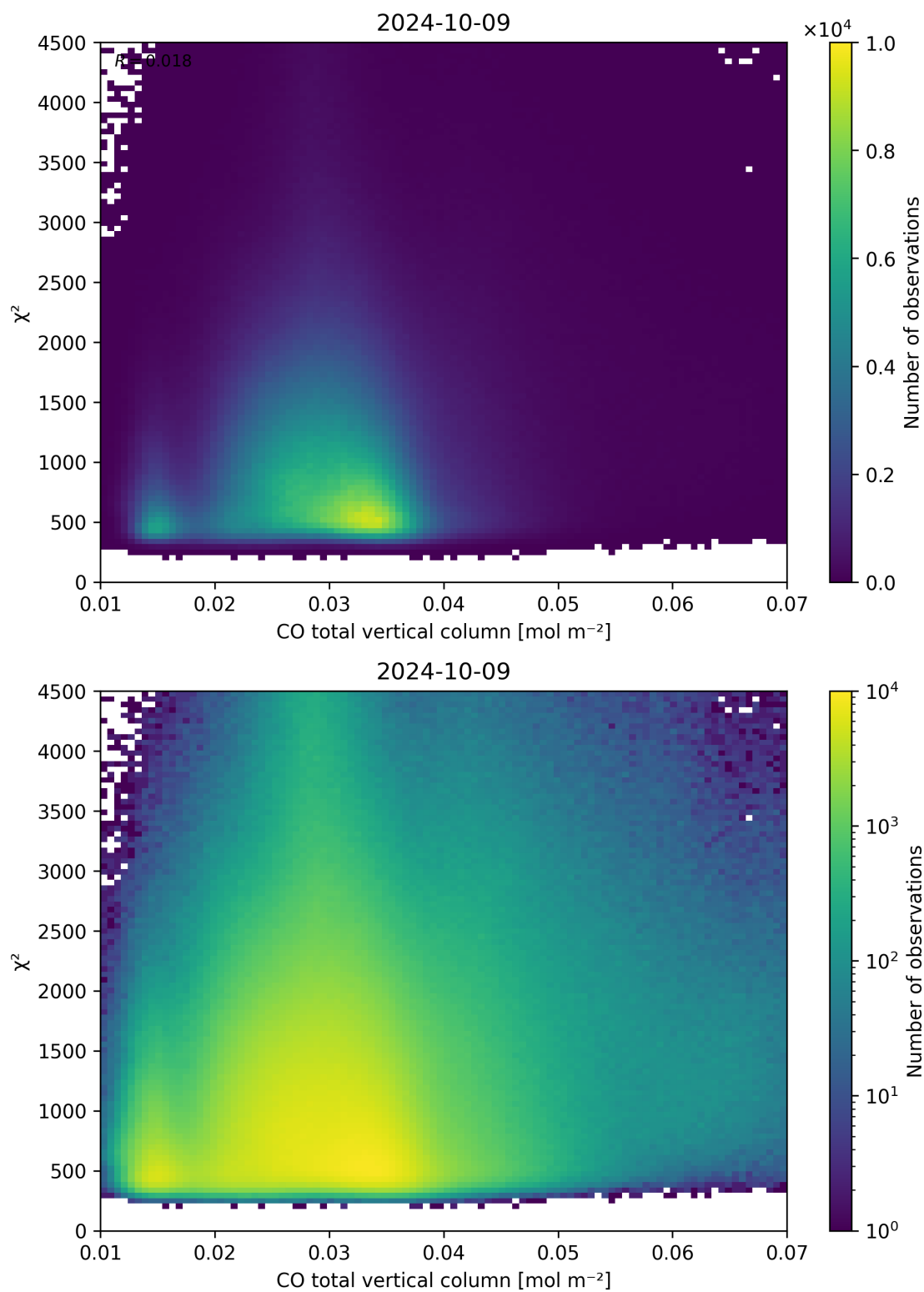
Figure 35: Scatter density plot of “CO total vertical column” against “ \chi^2 ” for 2024-10-08 to 2024-10-10.
