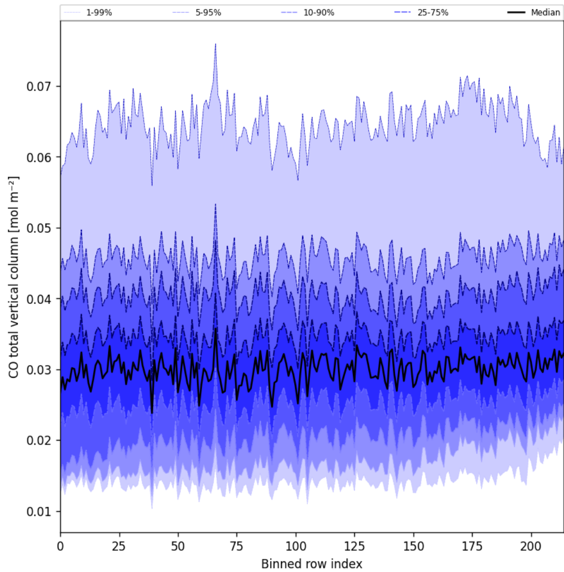
Figure 26: Along track statistics of “CO total vertical column” for 2024-10-08 to 2024-10-10
