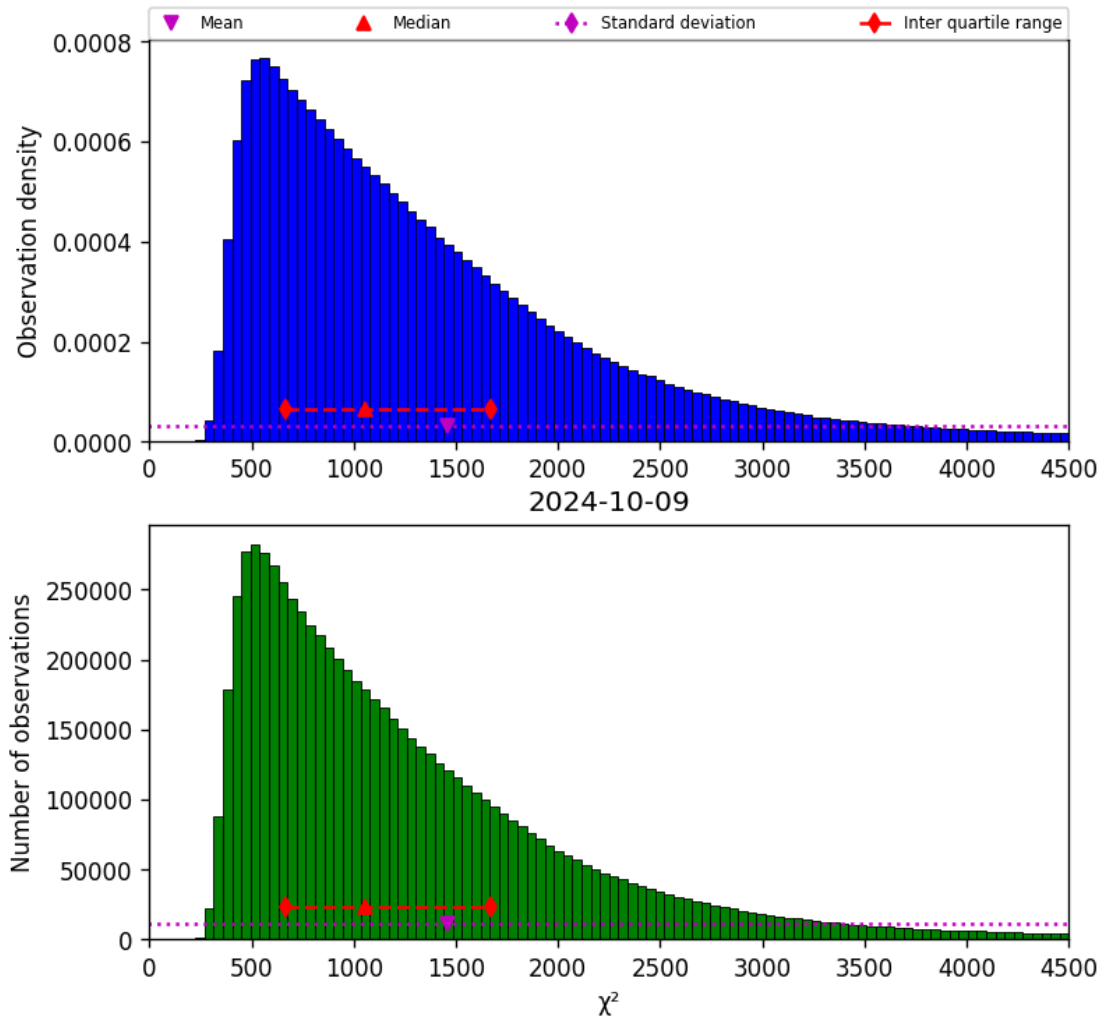
Figure 22: Histogram of “ \chi^2 ” for 2024-10-08 to 2024-10-10
