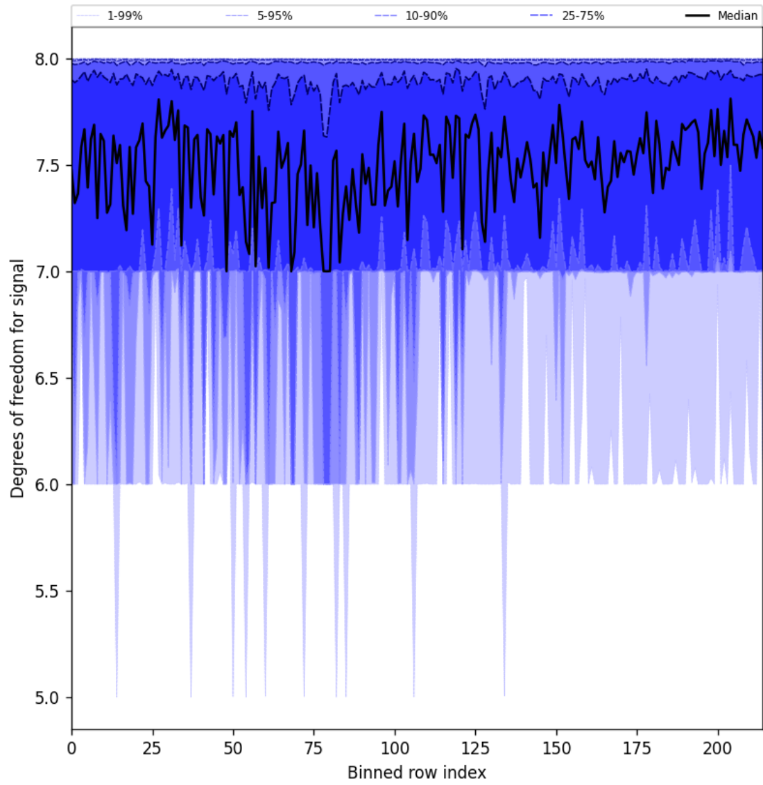
Figure 31: Along track statistics of “Degrees of freedom for signal” for 2024-10-08 to 2024-10-10
