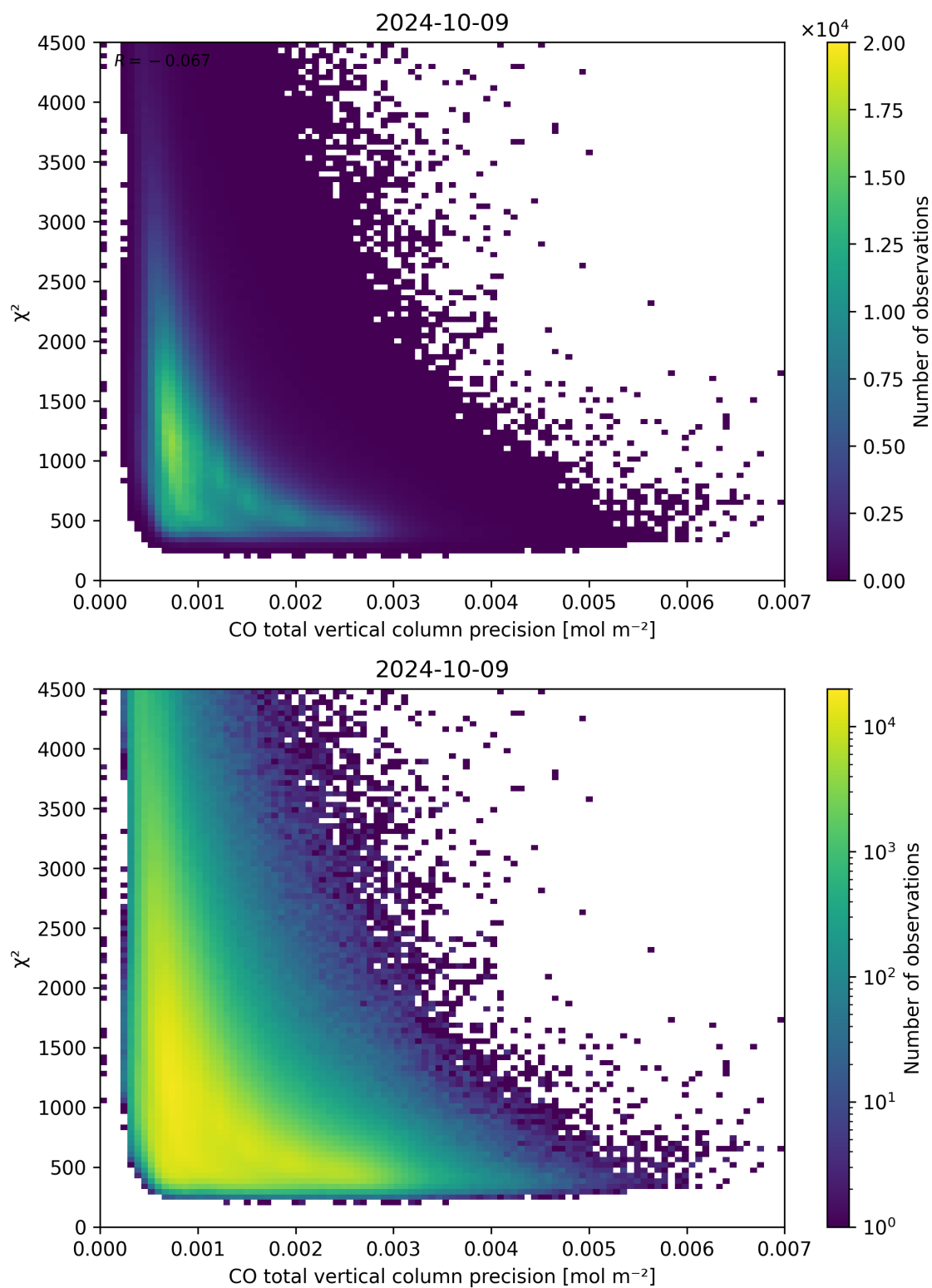
Figure 44: Scatter density plot of “CO total vertical column precision” against “ \chi^2 ” for 2024-10-08 to 2024-10-10.
