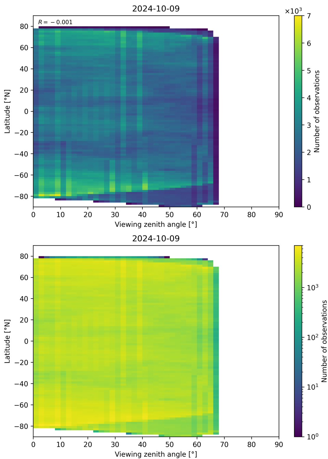
Figure 74: Scatter density plot of “Viewing zenith angle” against “Latitude” for 2024-10-08 to 2024-10-10.
