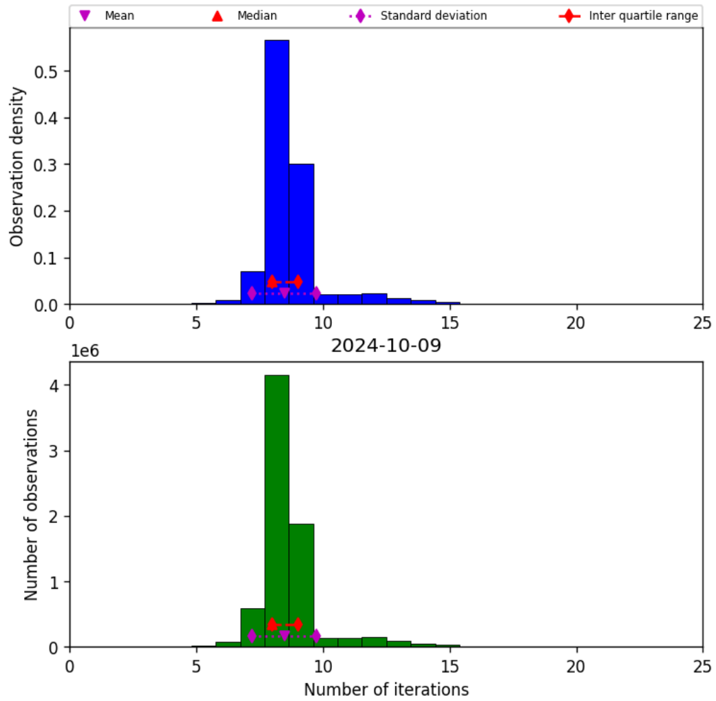
Figure 24: Histogram of “Number of iterations” for 2024-10-08 to 2024-10-10
