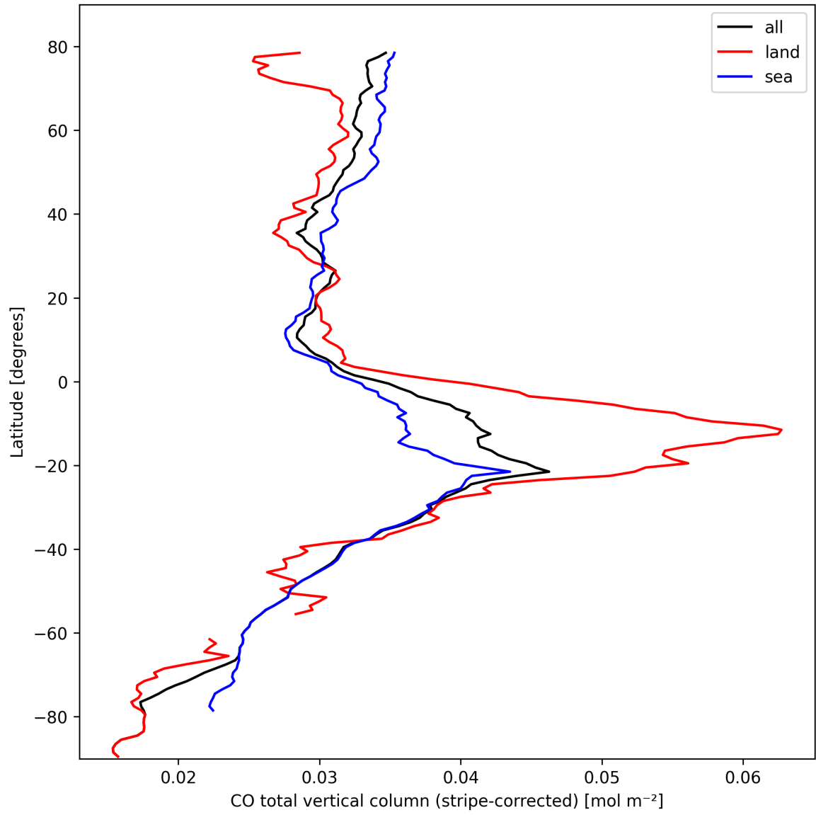
Figure 11: Zonal average of “CO total vertical column (stripe-corrected)” for 2024-10-08 to 2024-10-10.
