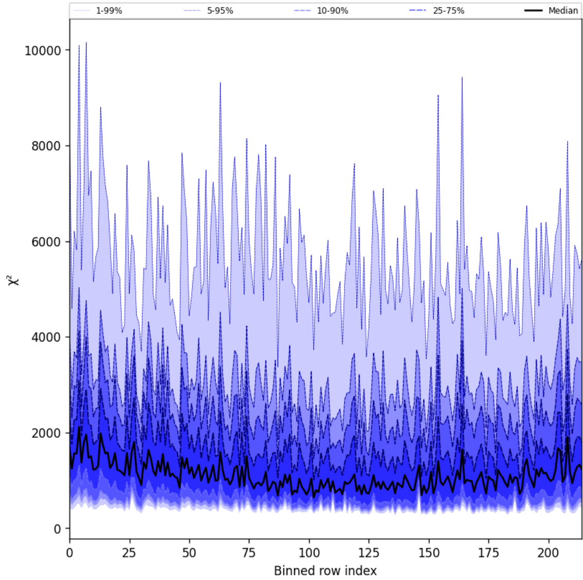
Figure 30: Along track statistics of “ \chi^2 ” for 2024-10-08 to 2024-10-10
