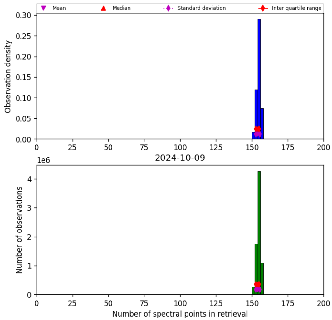
Figure 21: Histogram of “Number of spectral points in retrieval” for 2024-10-08 to 2024-10-10
