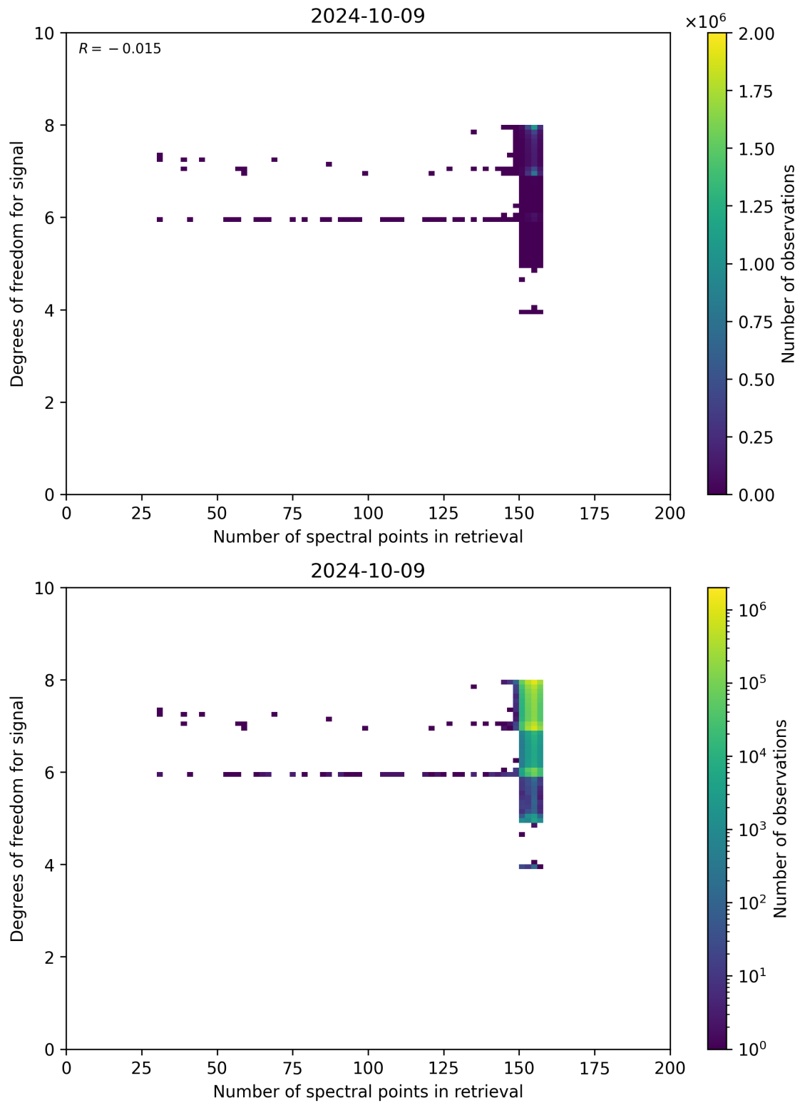
Figure 59: Scatter density plot of “Number of spectral points in retrieval” against “Degrees of freedom for signal” for 2024-10-08 to 2024-10-10.
