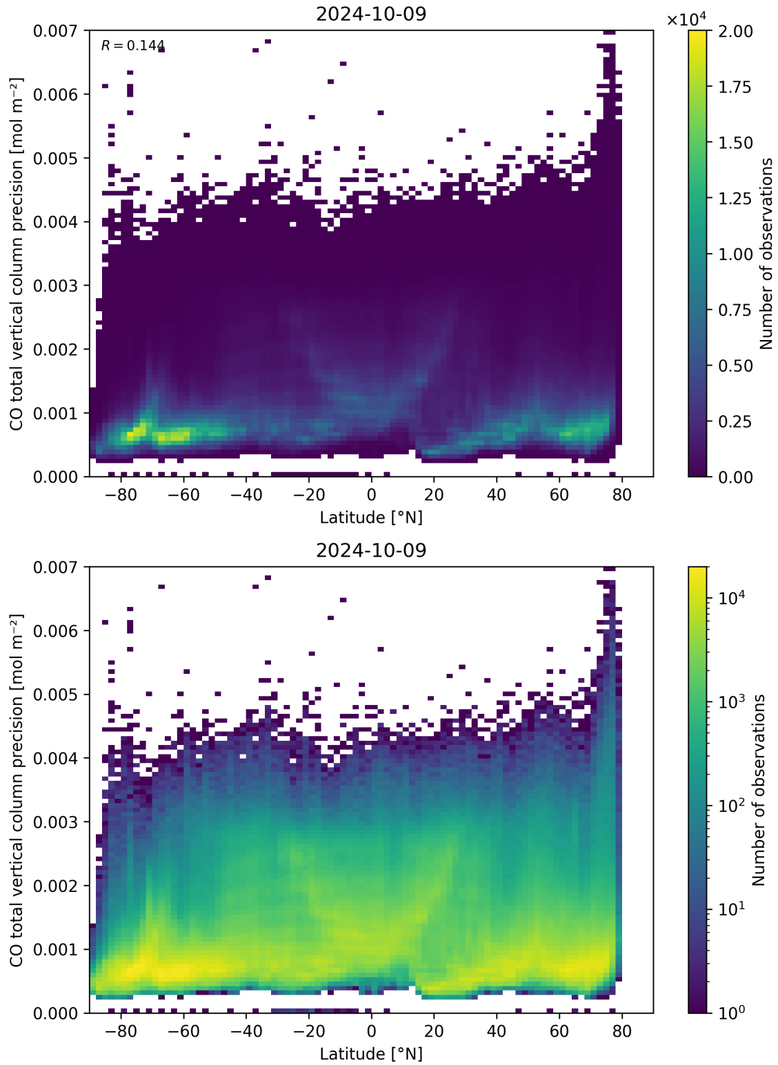
Figure 53: Scatter density plot of “Latitude” against “CO total vertical column precision” for 2024-10-08 to 2024-10-10.
