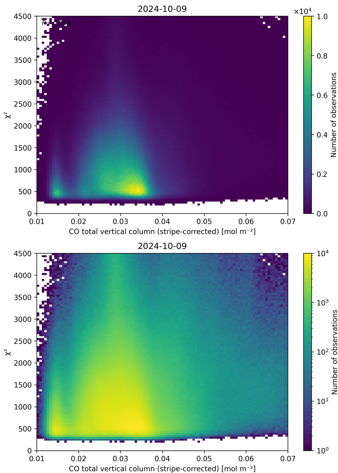
Figure 37: Scatter density plot of “CO total vertical column (stripe-corrected)” against “ \chi^2 ” for 2024-10-08 to 2024-10-10.
