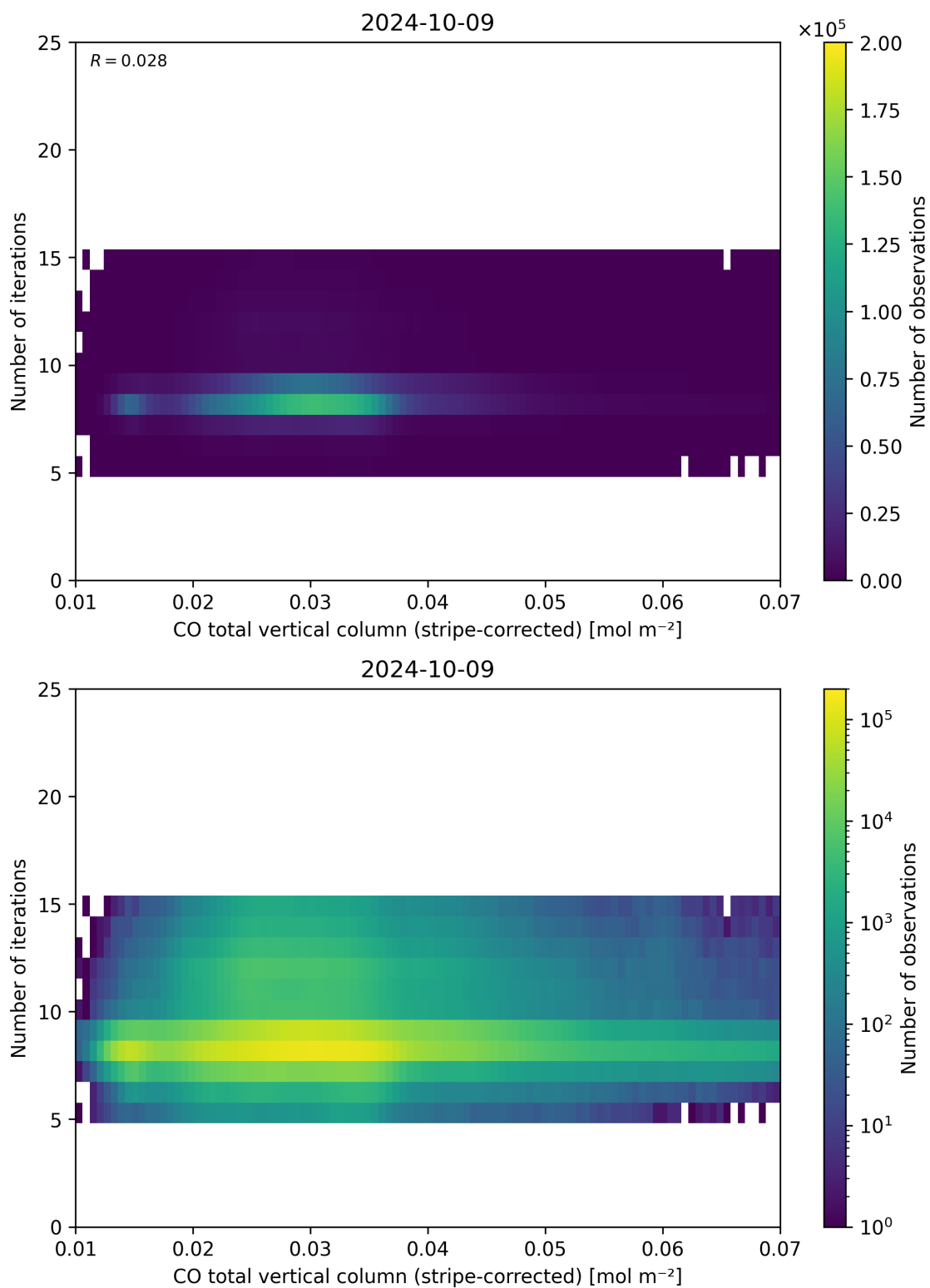
Figure 39: Scatter density plot of “CO total vertical column (stripe-corrected)” against “Number of iterations” for 2024-10-08 to 2024-10-10.
