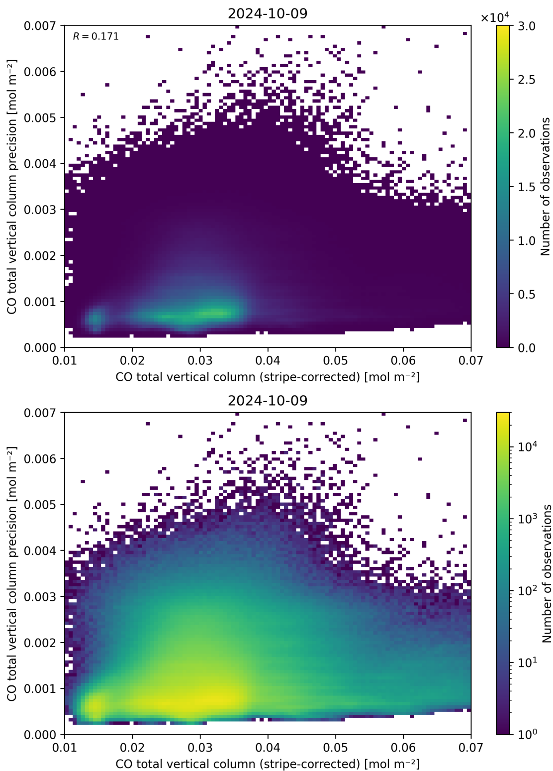
Figure 36: Scatter density plot of “CO total vertical column (stripe-corrected)” against “CO total vertical column precision” for 2024-10-08 to 2024-10-10.
