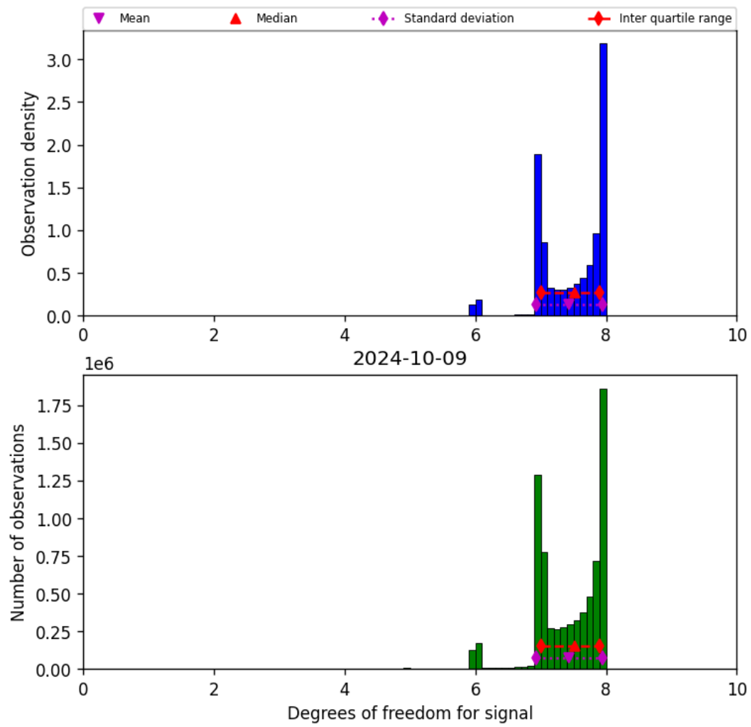
Figure 23: Histogram of “Degrees of freedom for signal” for 2024-10-08 to 2024-10-10
