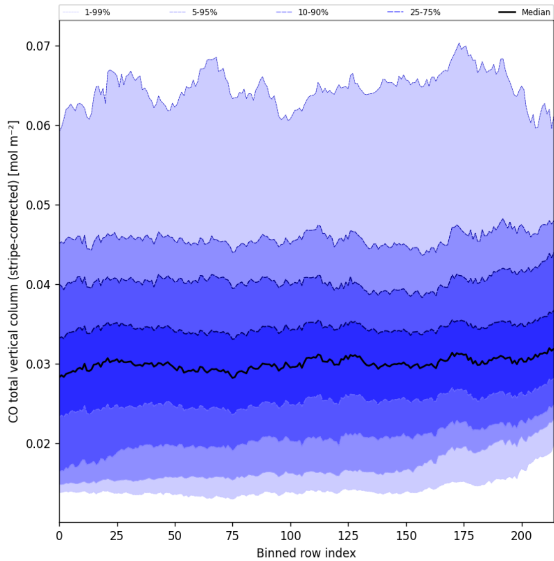
Figure 27: Along track statistics of “CO total vertical column (stripe-corrected)” for 2024-10-08 to 2024-10-10
