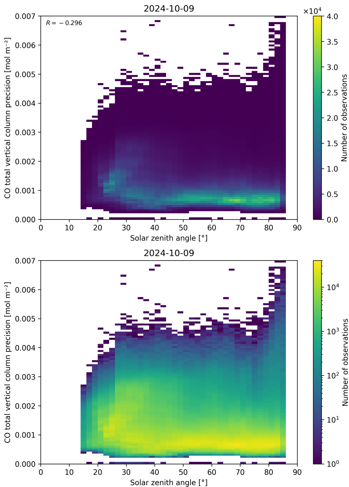
Figure 63: Scatter density plot of “Solar zenith angle” against “CO total vertical column precision” for 2024-10-08 to 2024-10-10.
