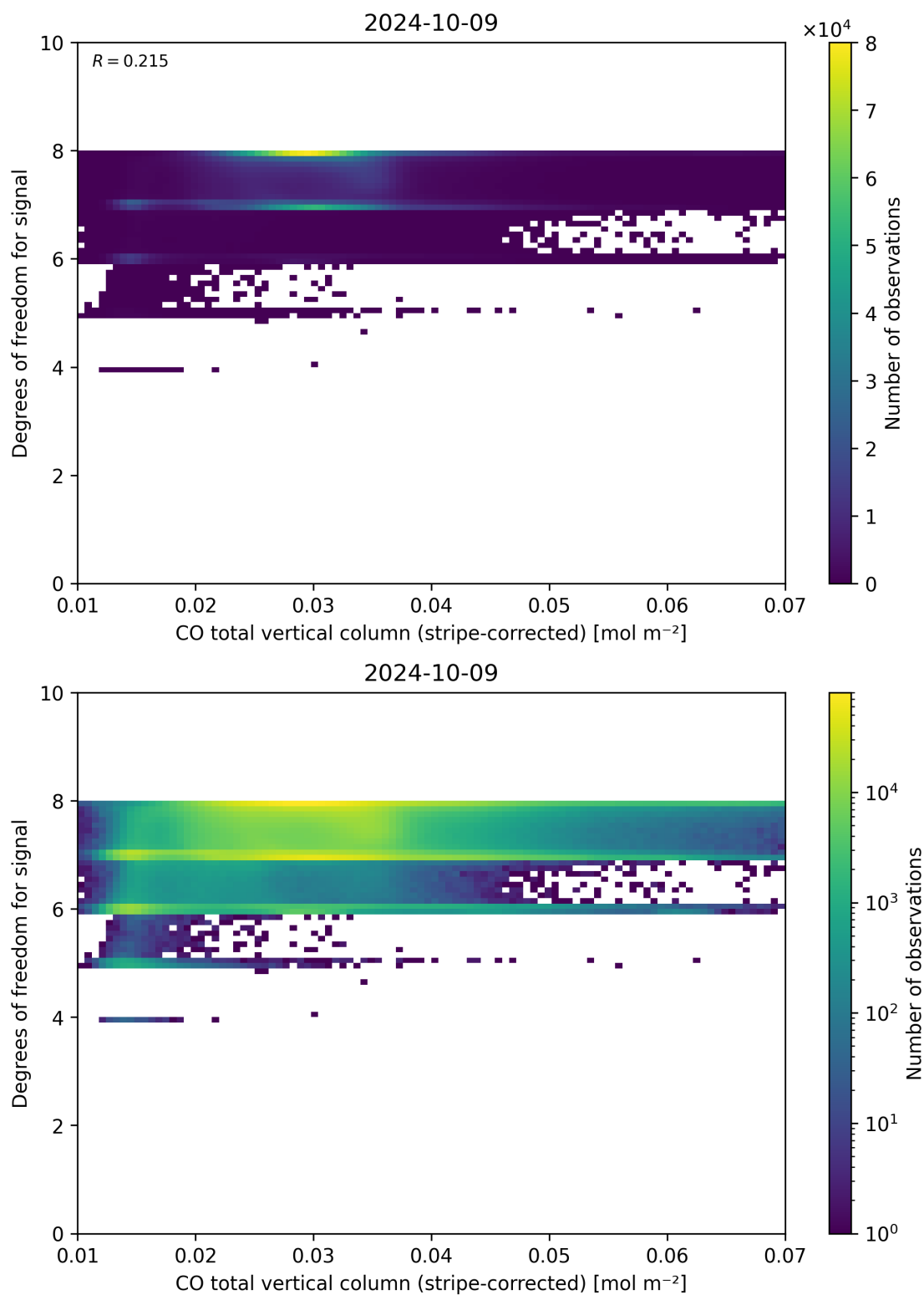
Figure 38: Scatter density plot of “CO total vertical column (stripe-corrected)” against “Degrees of freedom for signal” for 2024-10-08 to 2024-10-10.
