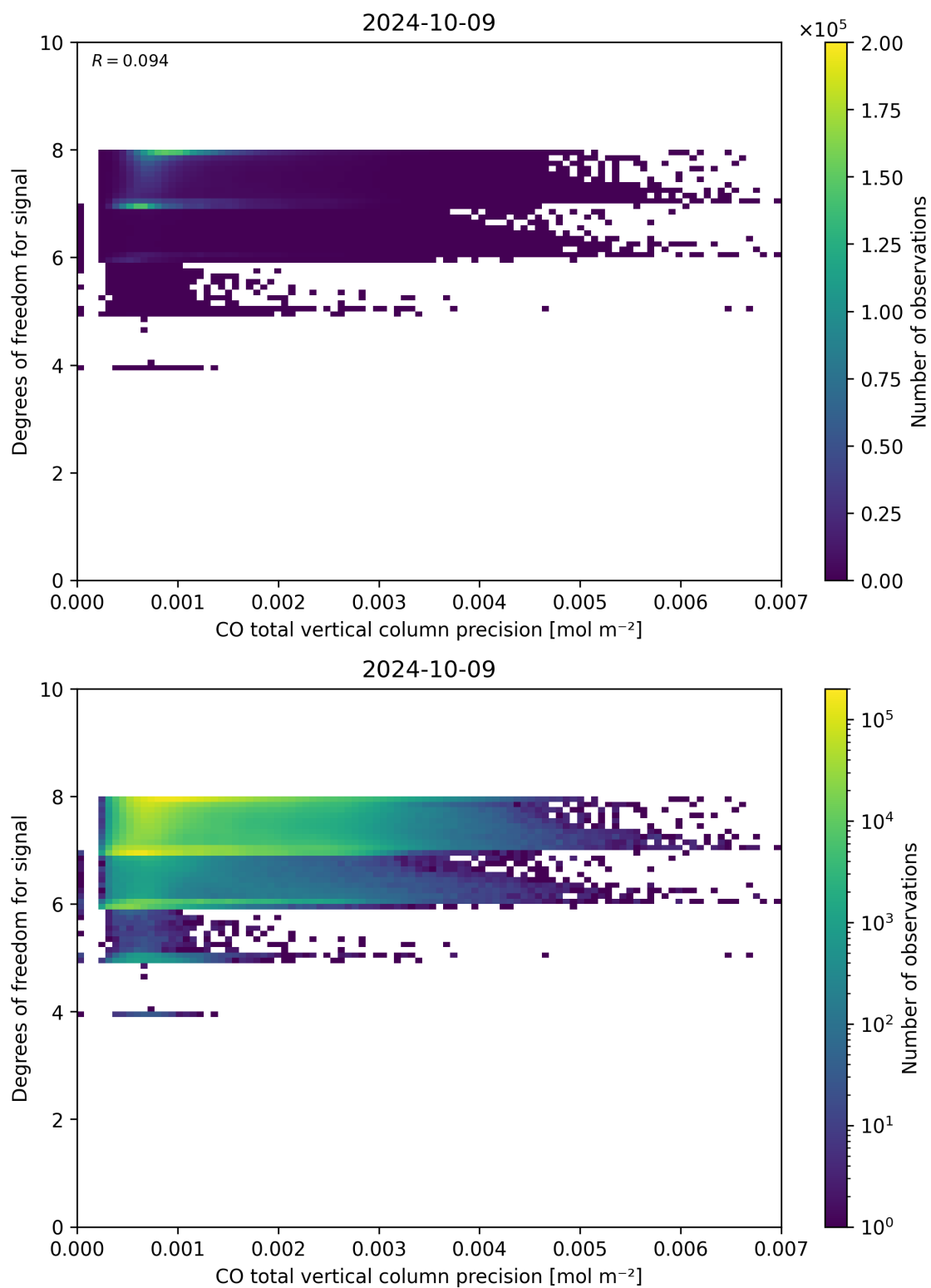
Figure 45: Scatter density plot of “CO total vertical column precision” against “Degrees of freedom for signal” for 2024-10-08 to 2024-10-10.
