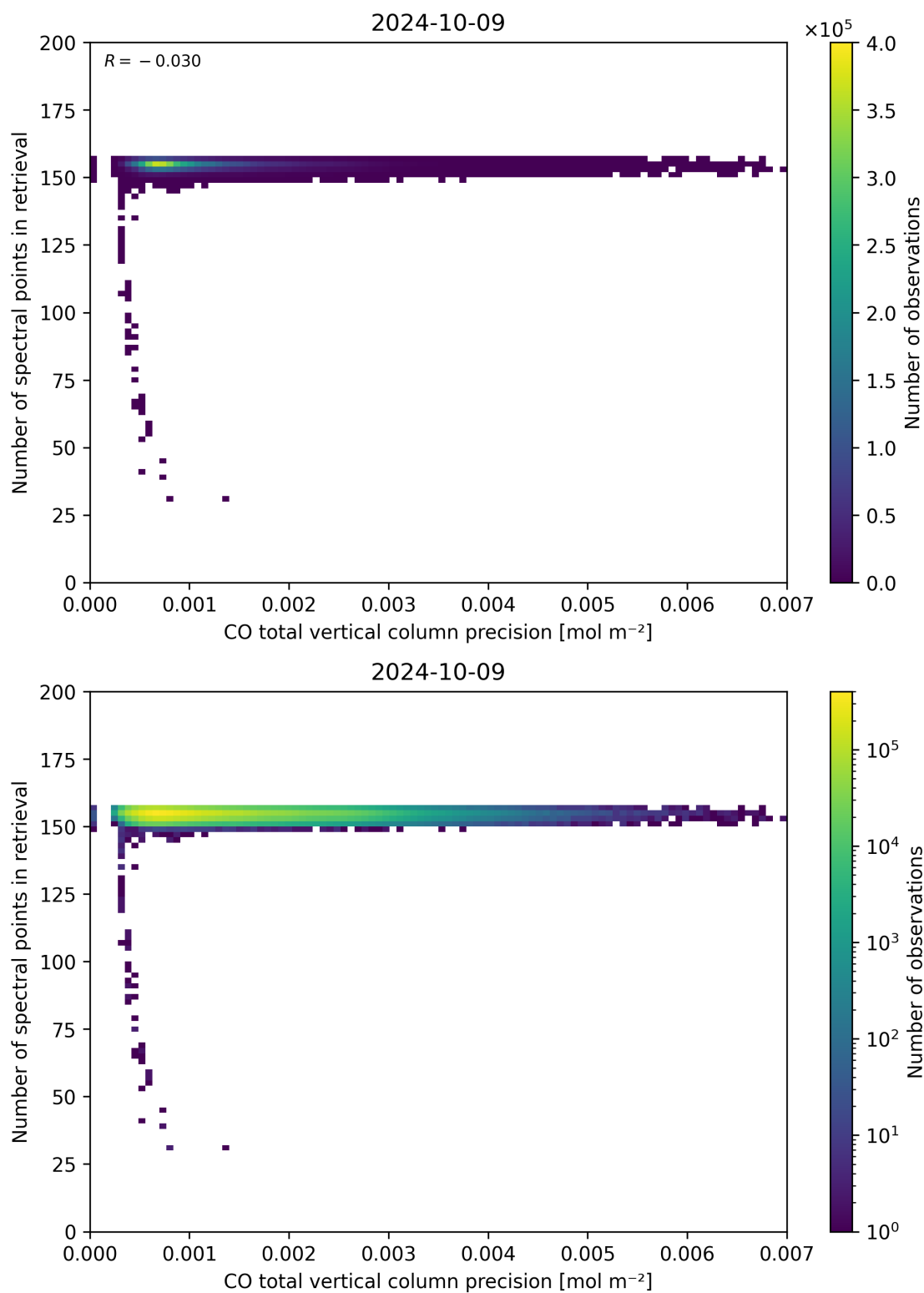
Figure 47: Scatter density plot of “CO total vertical column precision” against “Number of spectral points in retrieval” for 2024-10-08 to 2024-10-10.
