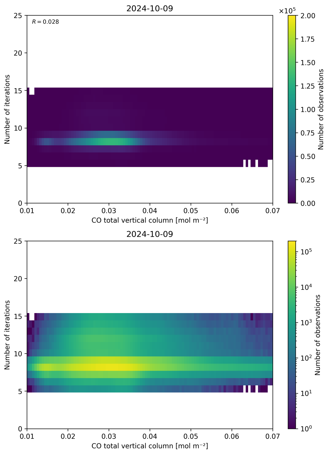
Figure 42: Scatter density plot of “CO total vertical column” against “Number of iterations” for 2024-10-08 to 2024-10-10.
