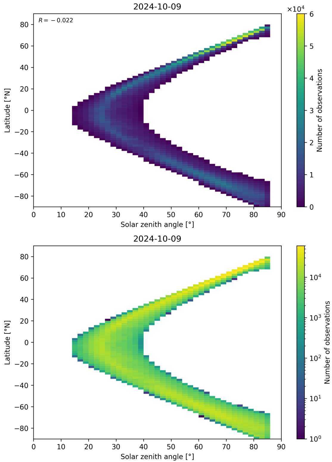
Figure 66: Scatter density plot of “Solar zenith angle” against “Latitude” for 2024-10-08 to 2024-10-10.
