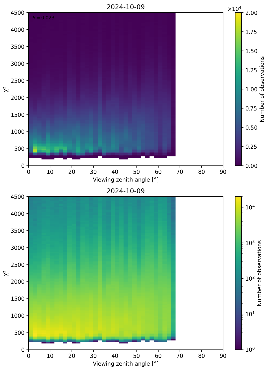
Figure 72: Scatter density plot of “Viewing zenith angle” against “ \chi^2 ” for 2024-10-08 to 2024-10-10.
