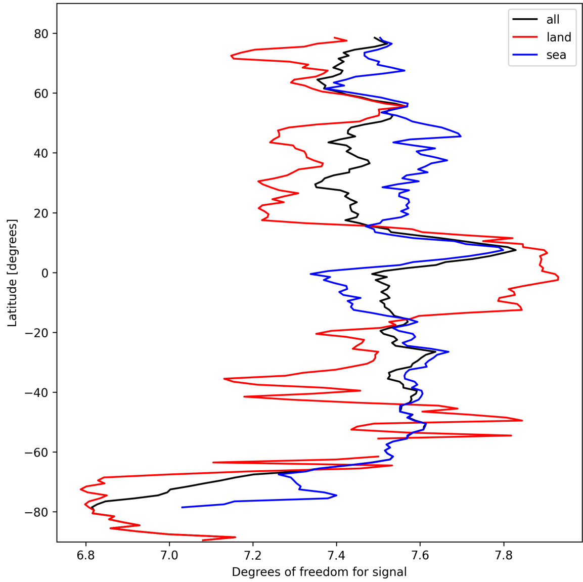
Figure 15: Zonal average of “Degrees of freedom for signal” for 2024-10-08 to 2024-10-10.
