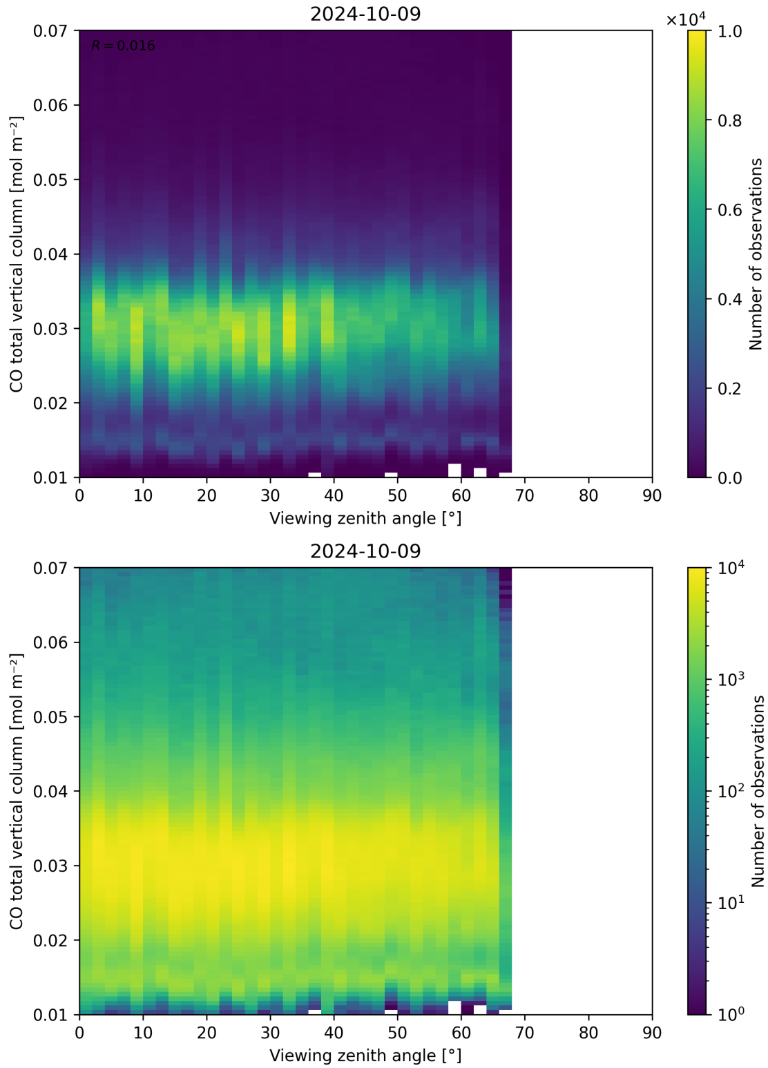
Figure 69: Scatter density plot of “Viewing zenith angle” against “CO total vertical column” for 2024-10-08 to 2024-10-10.
