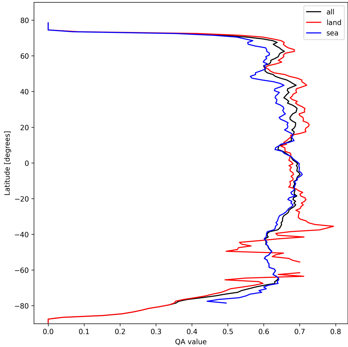
Figure 9: Zonal average of “QA value” for 2024-10-08 to 2024-10-10.
