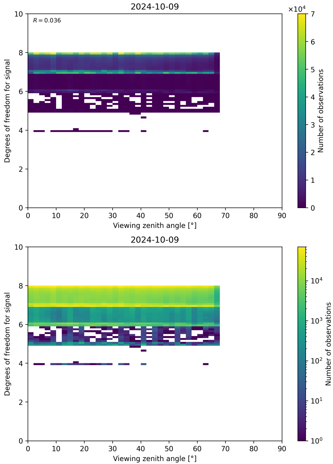
Figure 73: Scatter density plot of “Viewing zenith angle” against “Degrees of freedom for signal” for 2024-10-08 to 2024-10-10.
