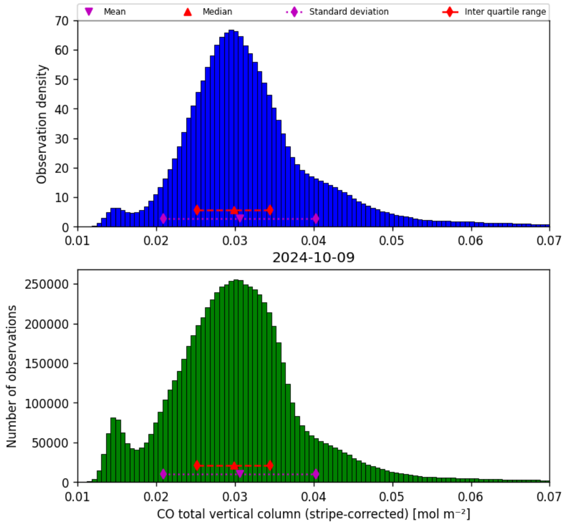
Figure 19: Histogram of “CO total vertical column (stripe-corrected)” for 2024-10-08 to 2024-10-10
