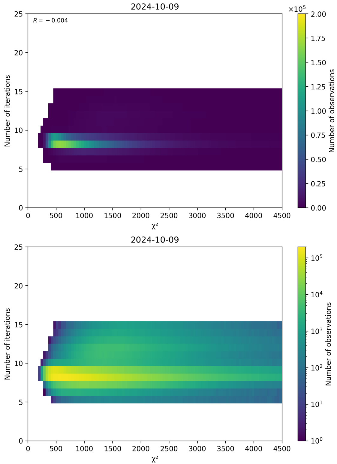
Figure 49: Scatter density plot of “ \chi^2 ” against “Number of iterations” for 2024-10-08 to 2024-10-10.
