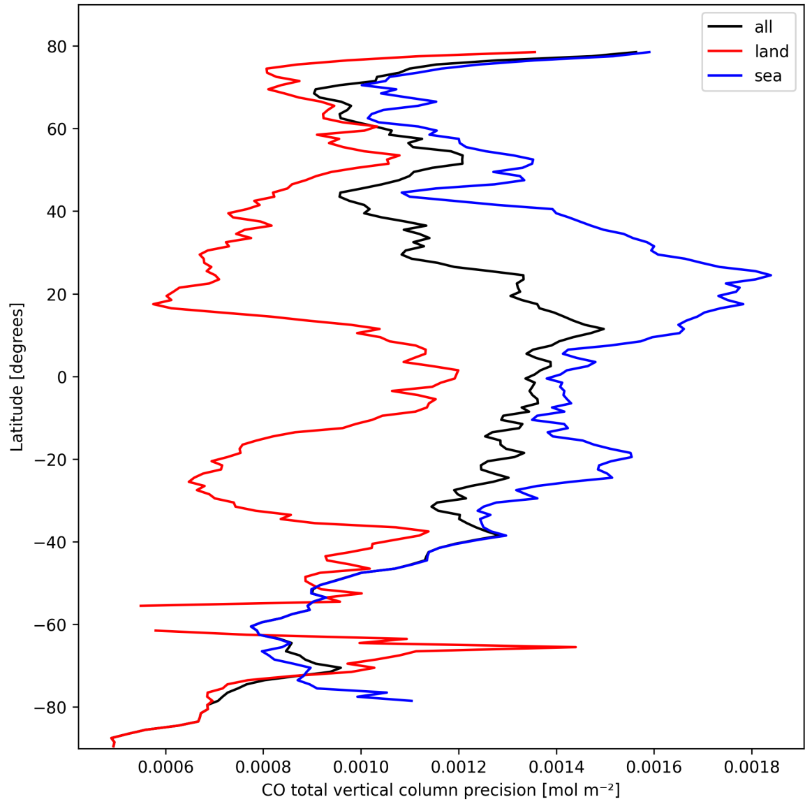
Figure 12: Zonal average of “CO total vertical column precision” for 2024-10-08 to 2024-10-10.
