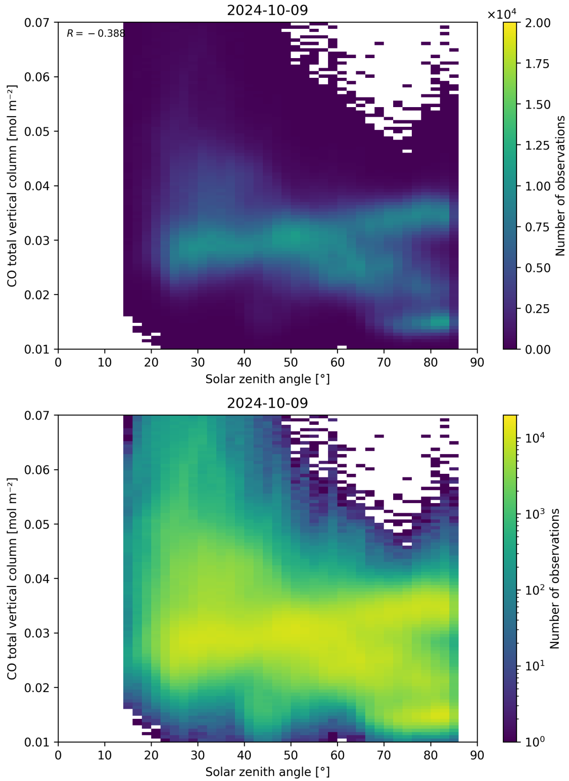
Figure 61: Scatter density plot of “Solar zenith angle” against “CO total vertical column” for 2024-10-08 to 2024-10-10.
