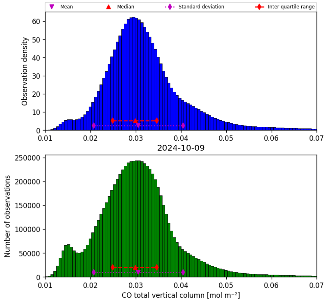
Figure 18: Histogram of “CO total vertical column” for 2024-10-08 to 2024-10-10
