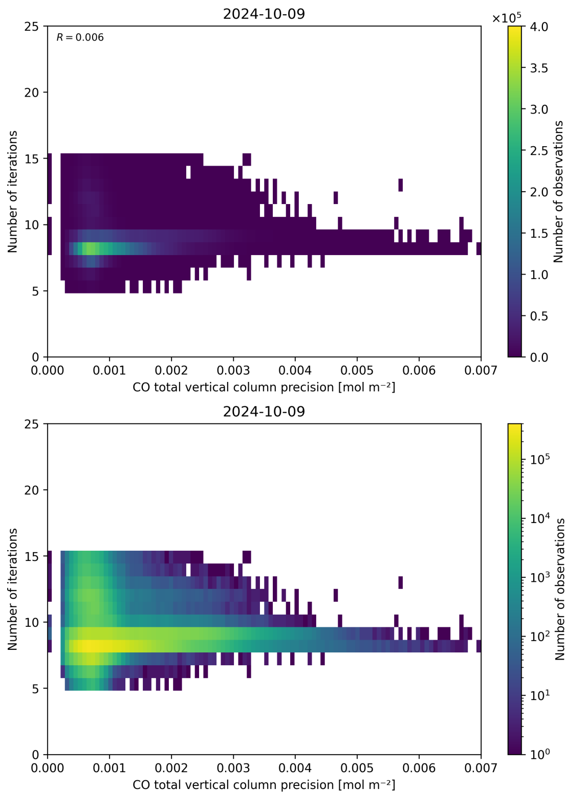
Figure 46: Scatter density plot of “CO total vertical column precision” against “Number of iterations” for 2024-10-08 to 2024-10-10.
