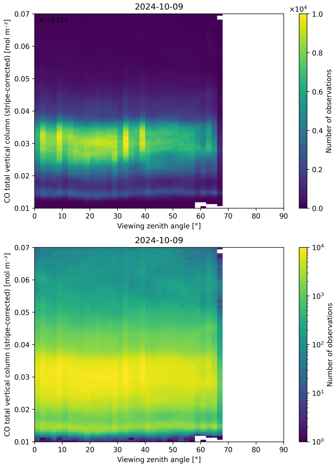
Figure 70: Scatter density plot of “Viewing zenith angle” against “CO total vertical column (stripe-corrected)” for 2024-10-08 to 2024-10-10.
