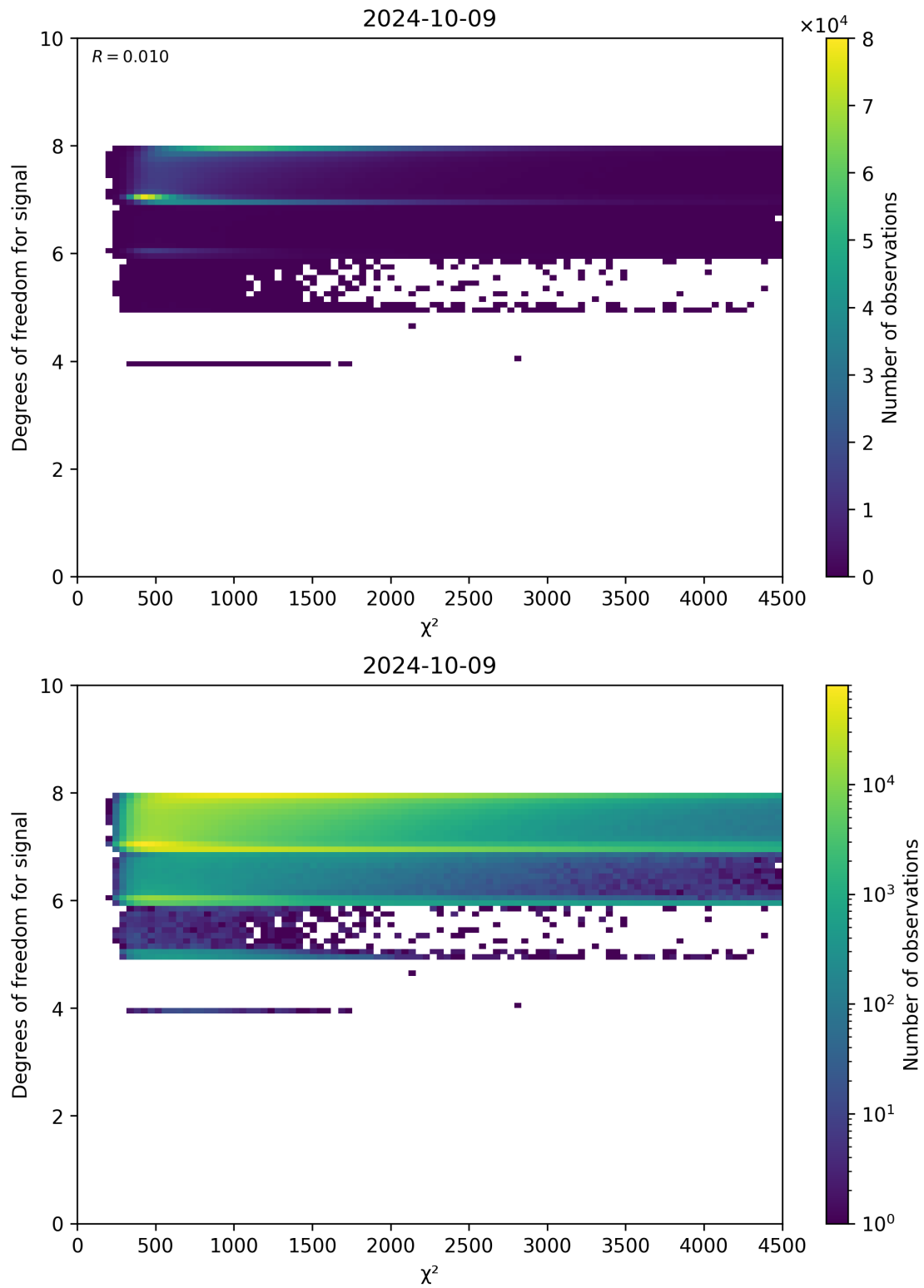
Figure 48: Scatter density plot of “ \chi^2 ” against “Degrees of freedom for signal” for 2024-10-08 to 2024-10-10.
