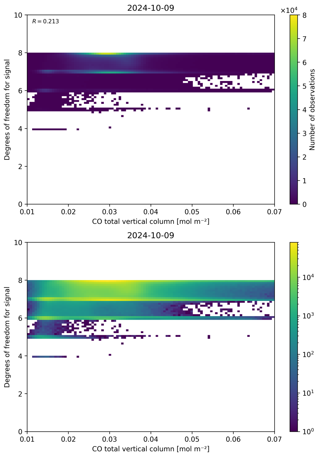
Figure 41: Scatter density plot of “CO total vertical column” against “Degrees of freedom for signal” for 2024-10-08 to 2024-10-10.
