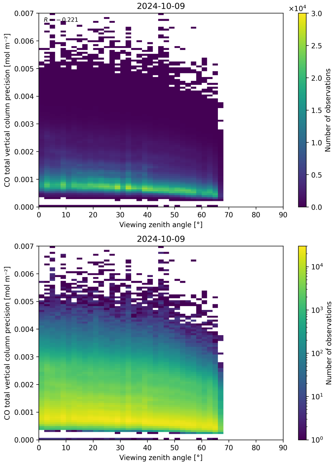
Figure 71: Scatter density plot of “Viewing zenith angle” against “CO total vertical column precision” for 2024-10-08 to 2024-10-10.
