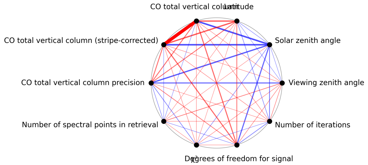
Figure 1: Map of correlation graph for 2024-10-08 to 2024-10-10.
