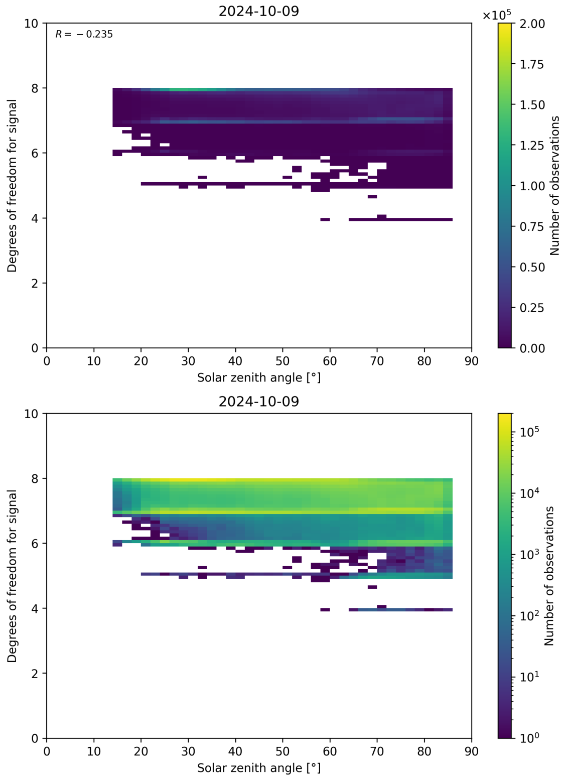
Figure 65: Scatter density plot of “Solar zenith angle” against “Degrees of freedom for signal” for 2024-10-08 to 2024-10-10.
