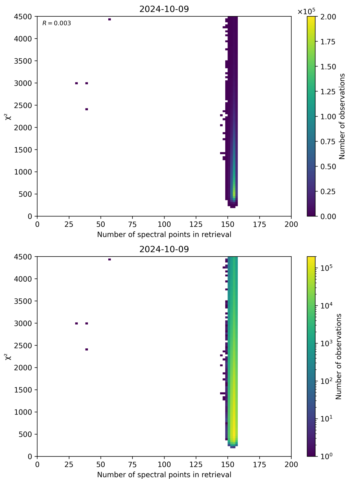
Figure 58: Scatter density plot of “Number of spectral points in retrieval” against “ \chi^2 ” for 2024-10-08 to 2024-10-10.
