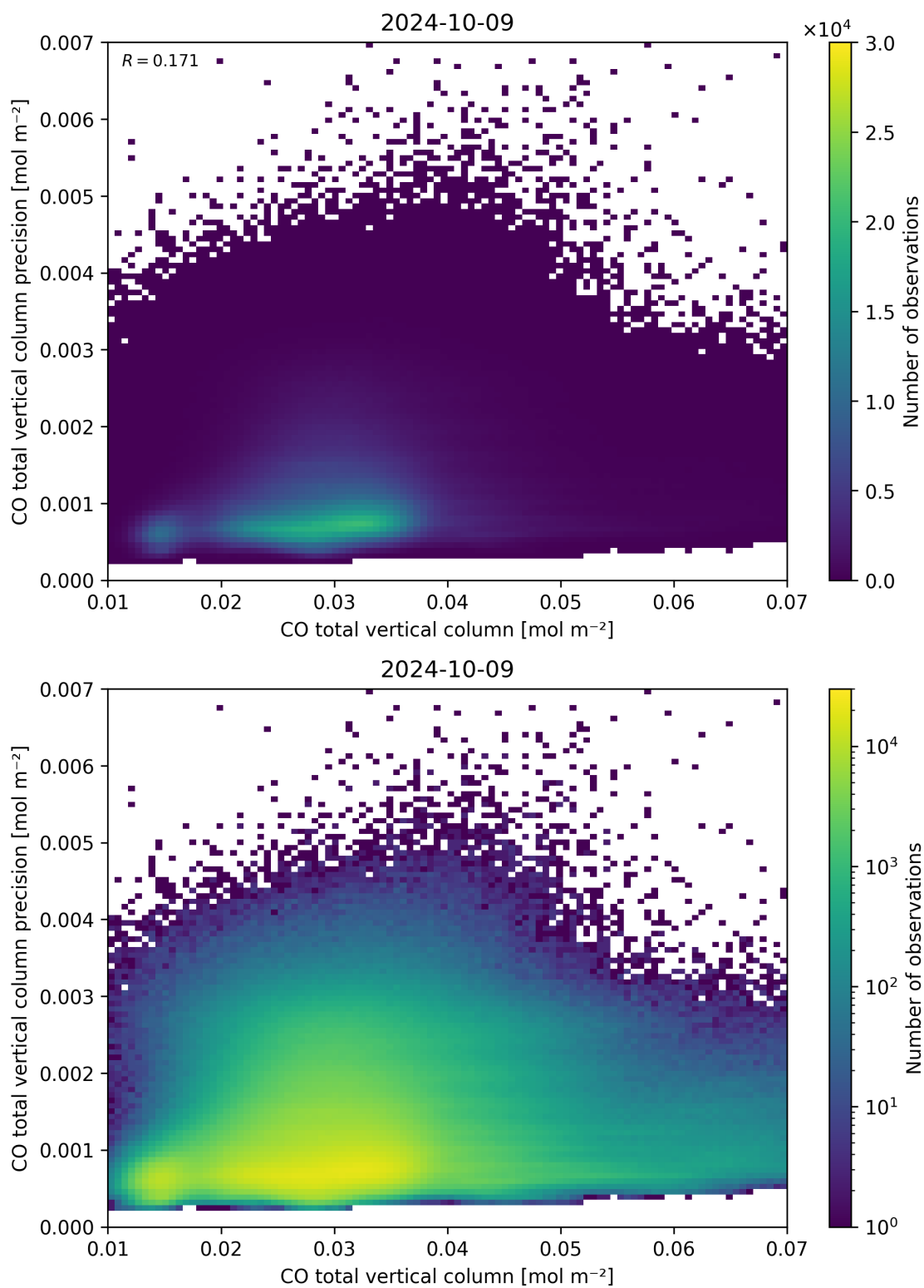
Figure 34: Scatter density plot of “CO total vertical column” against “CO total vertical column precision” for 2024-10-08 to 2024-10-10.
