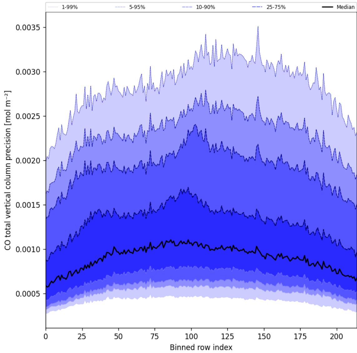
Figure 28: Along track statistics of “CO total vertical column precision” for 2024-10-08 to 2024-10-10
