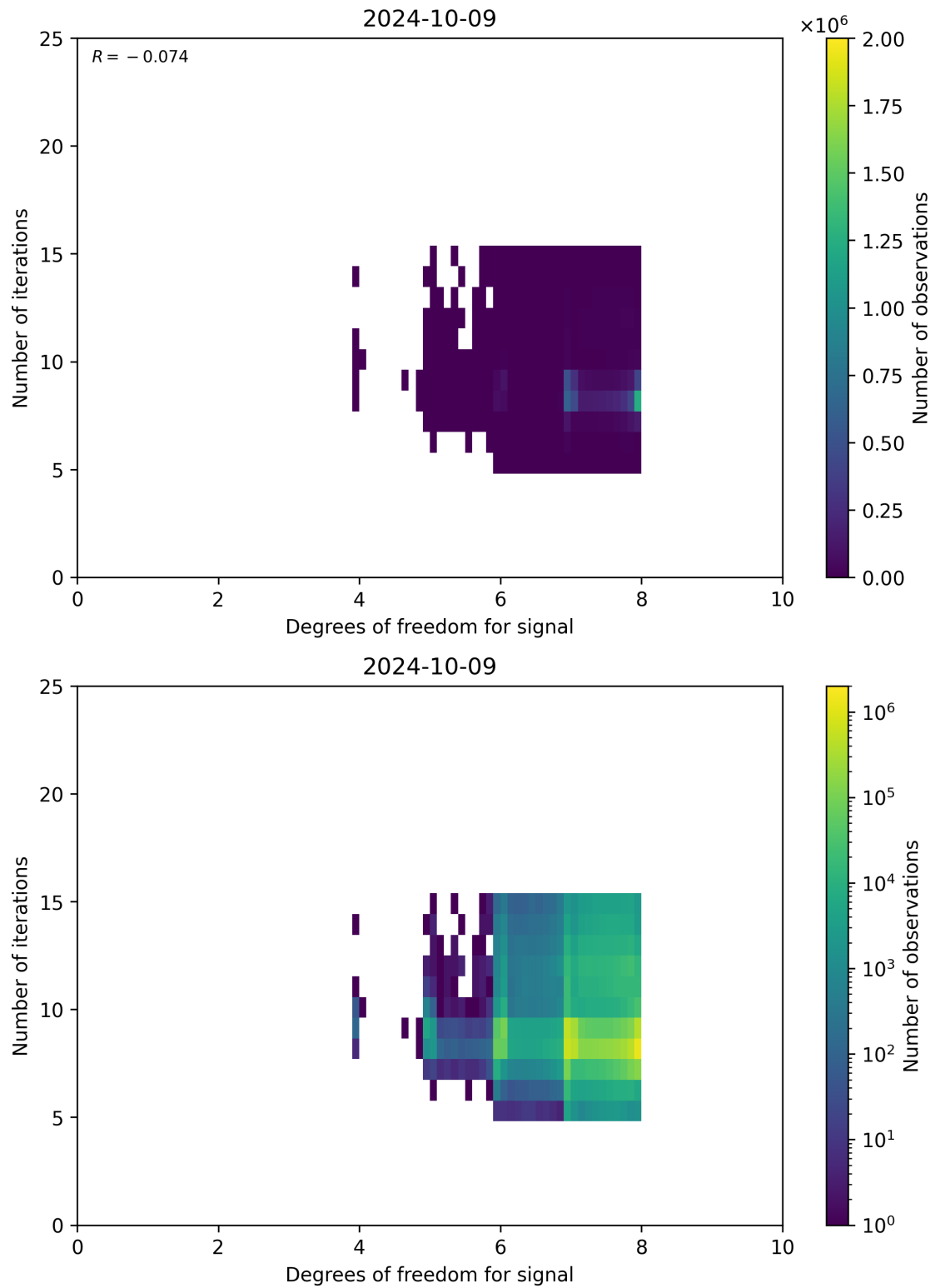
Figure 50: Scatter density plot of “Degrees of freedom for signal” against “Number of iterations” for 2024-10-08 to 2024-10-10.
