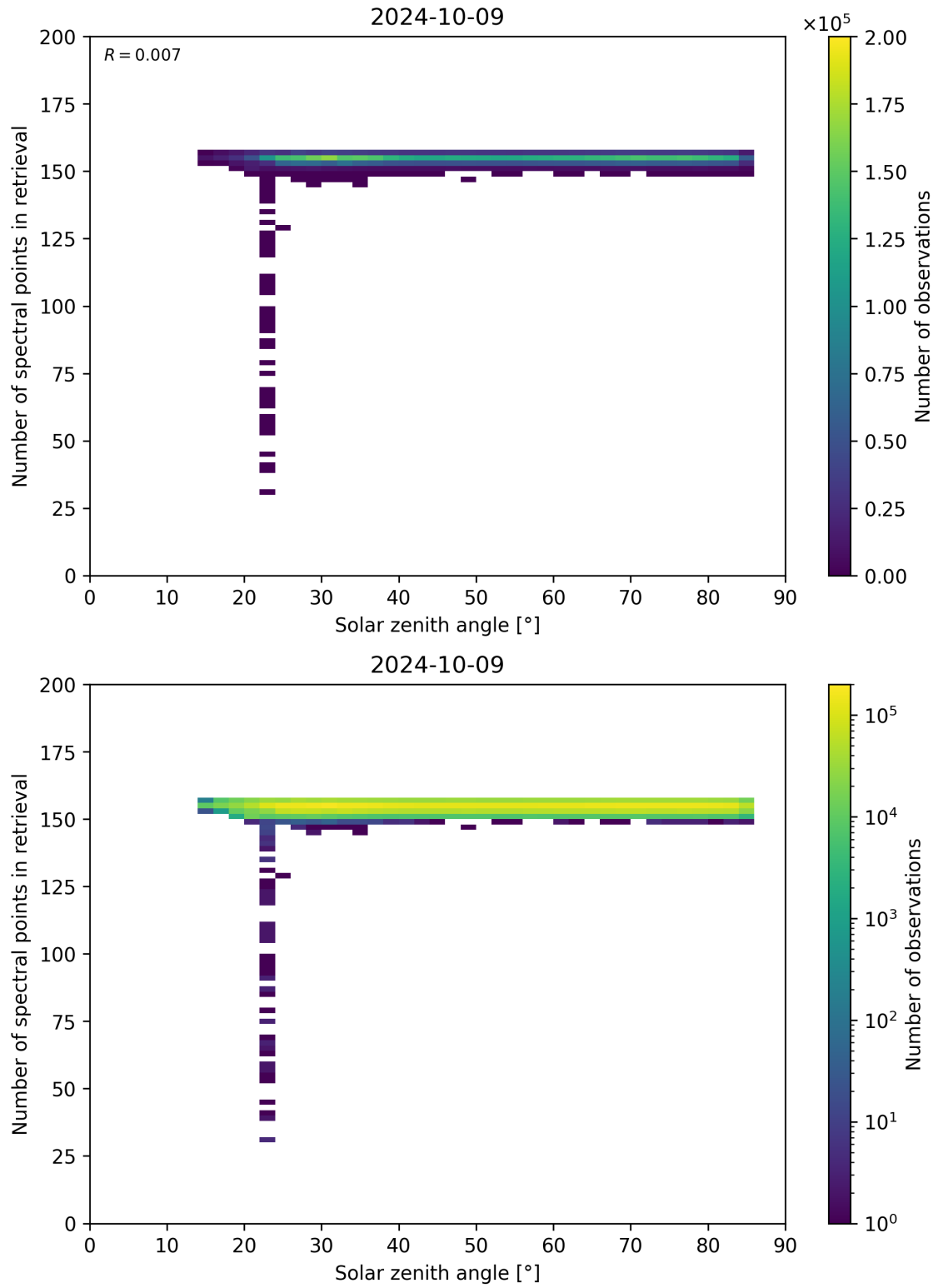
Figure 68: Scatter density plot of “Solar zenith angle” against “Number of spectral points in retrieval” for 2024-10-08 to 2024-10-10.
