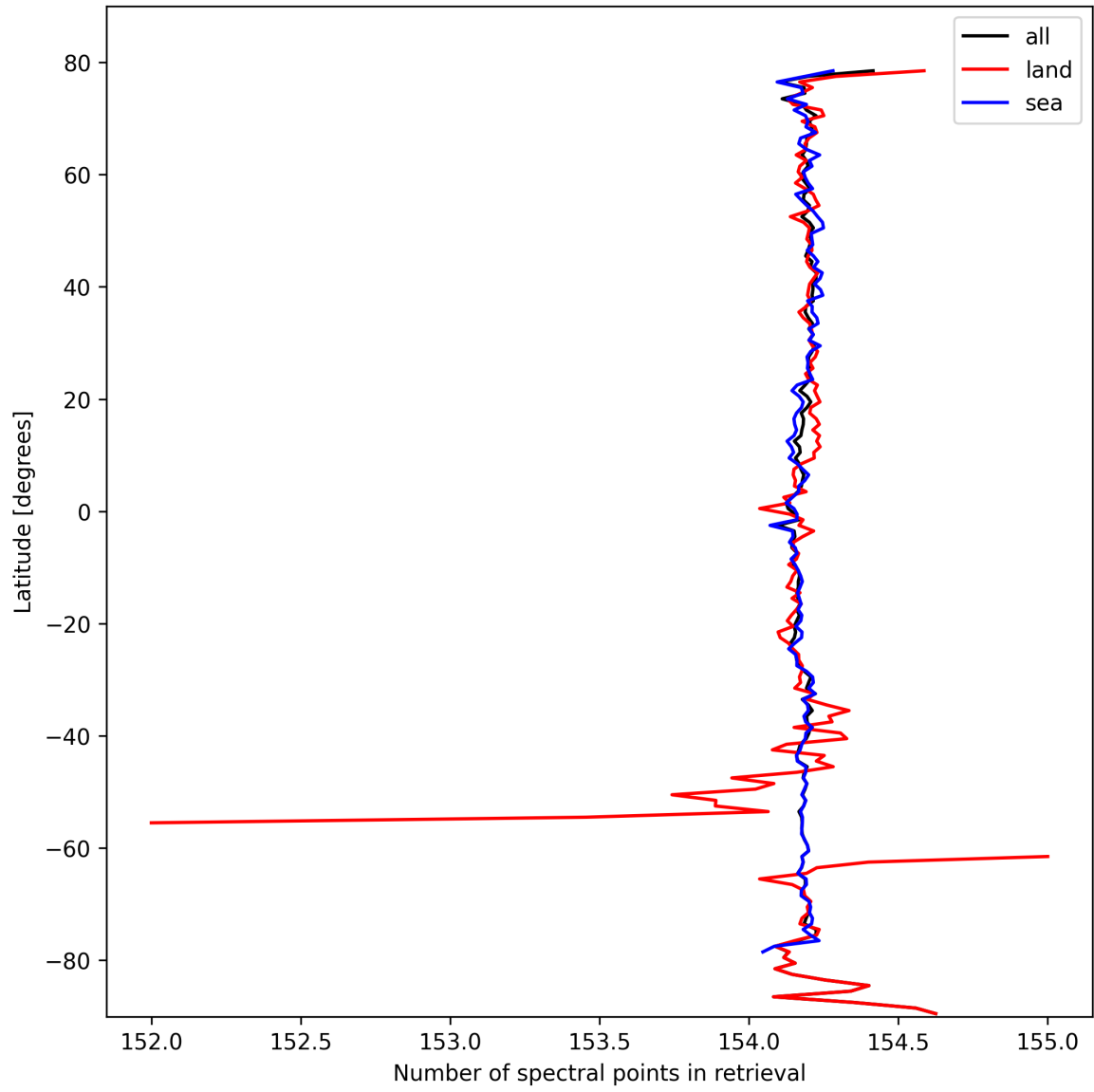
Figure 13: Zonal average of “Number of spectral points in retrieval” for 2024-10-08 to 2024-10-10.
