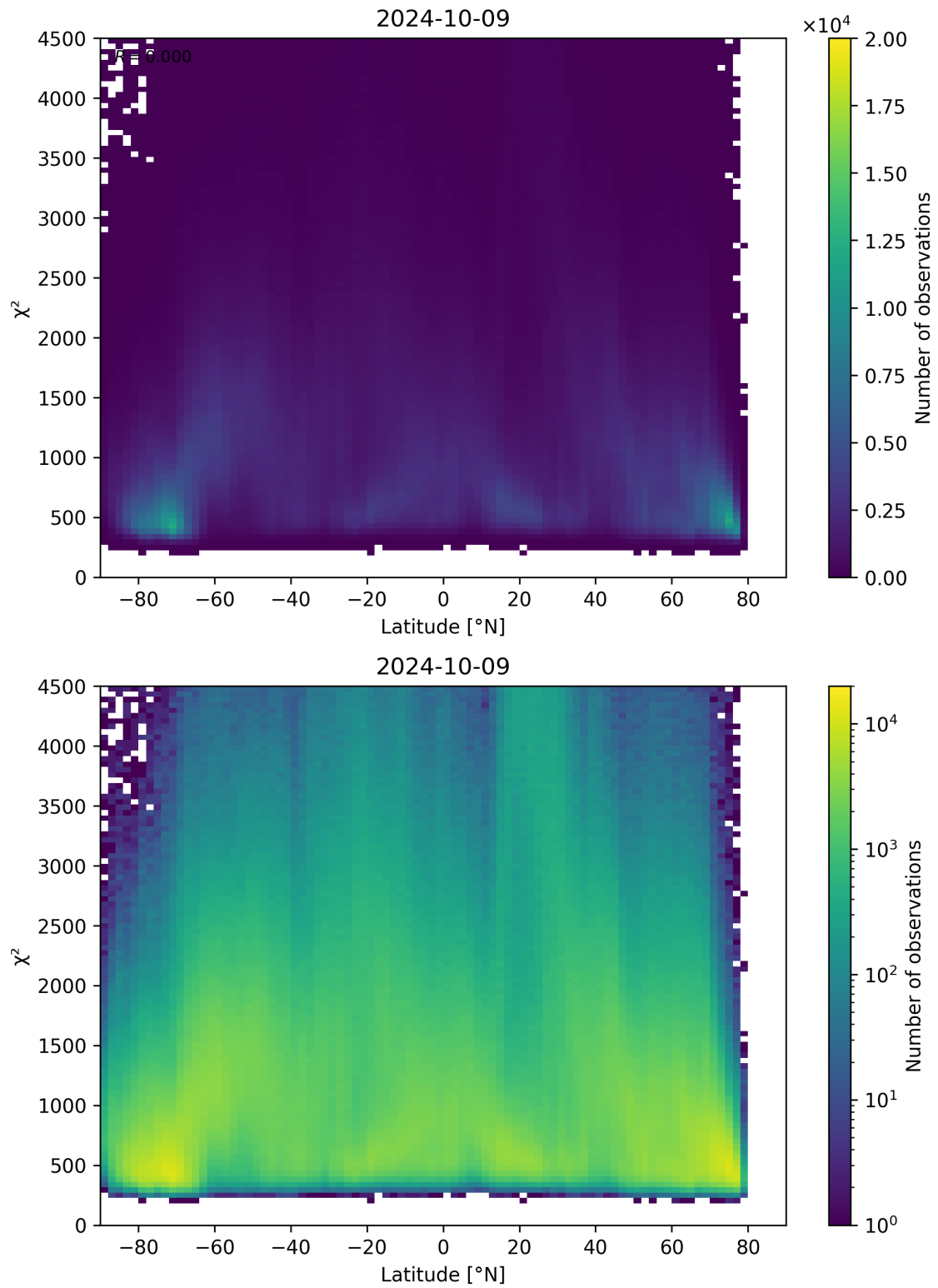
Figure 54: Scatter density plot of “Latitude” against “ \chi^2 ” for 2024-10-08 to 2024-10-10.
