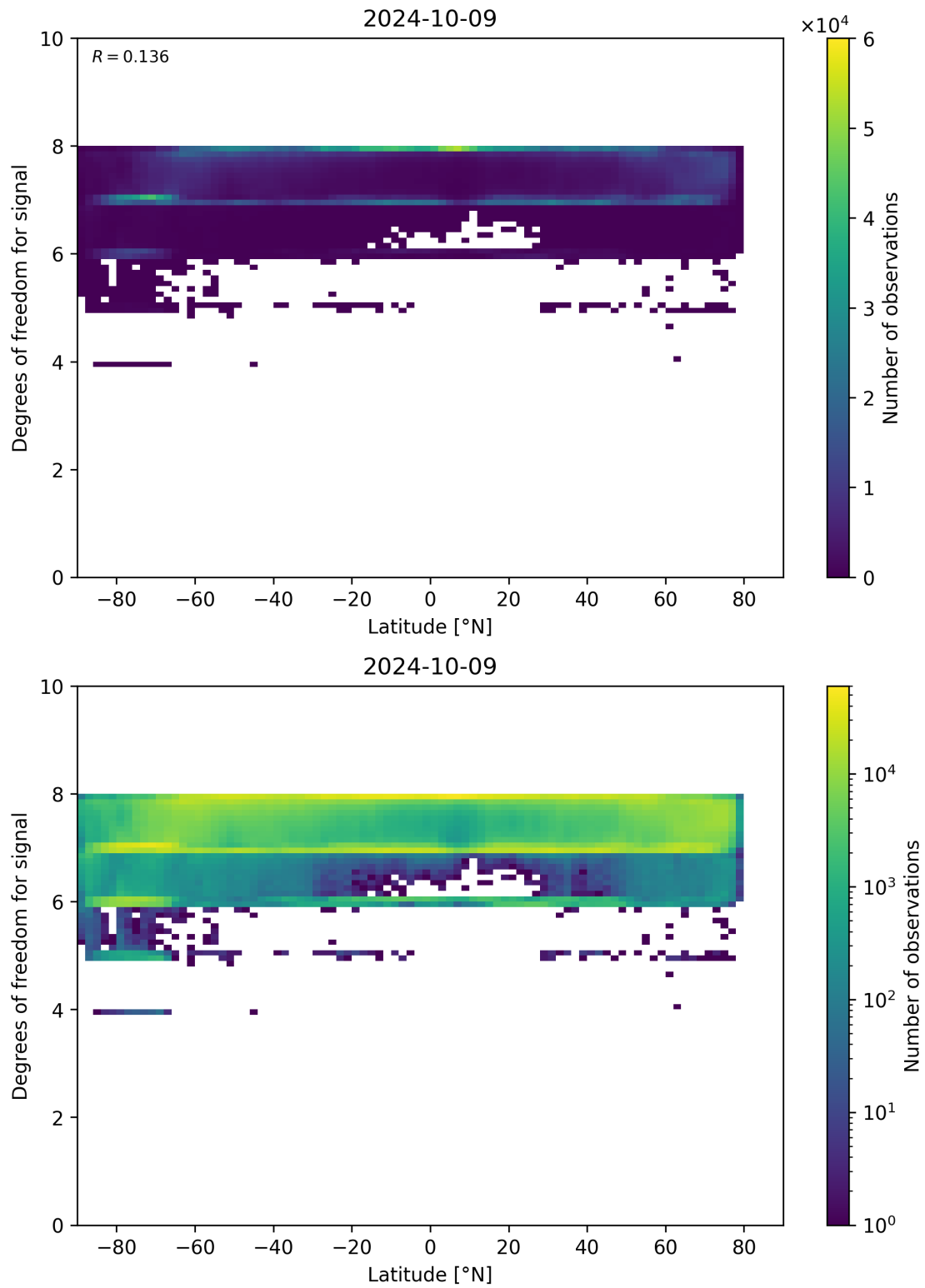
Figure 55: Scatter density plot of “Latitude” against “Degrees of freedom for signal” for 2024-10-08 to 2024-10-10.
