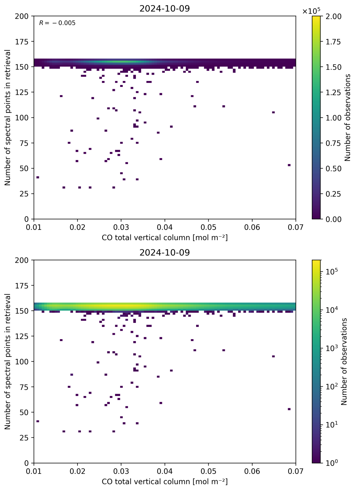
Figure 43: Scatter density plot of “CO total vertical column” against “Number of spectral points in retrieval” for 2024-10-08 to 2024-10-10.
