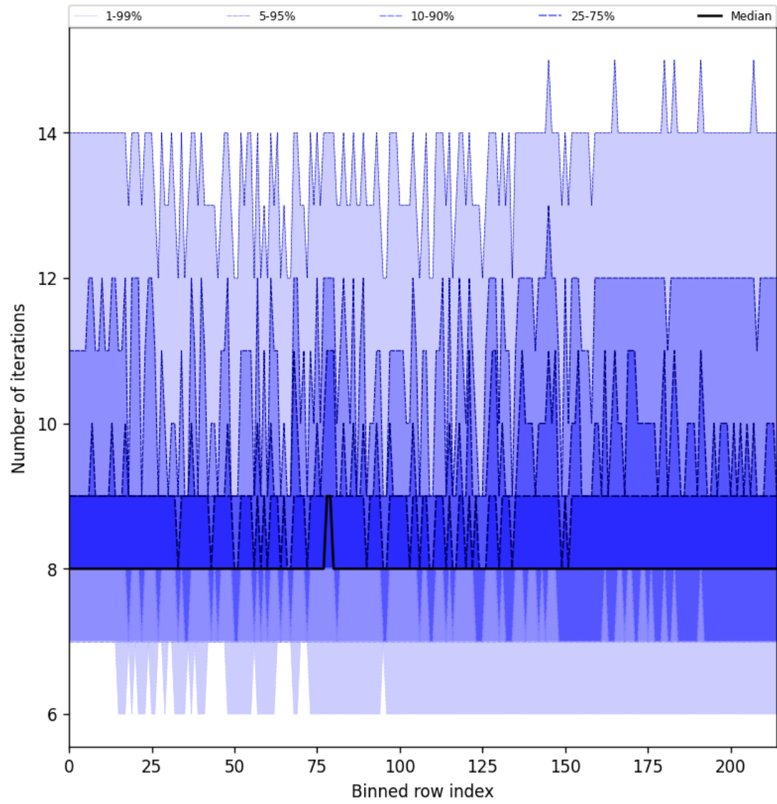
Figure 32: Along track statistics of “Number of iterations” for 2024-10-08 to 2024-10-10
