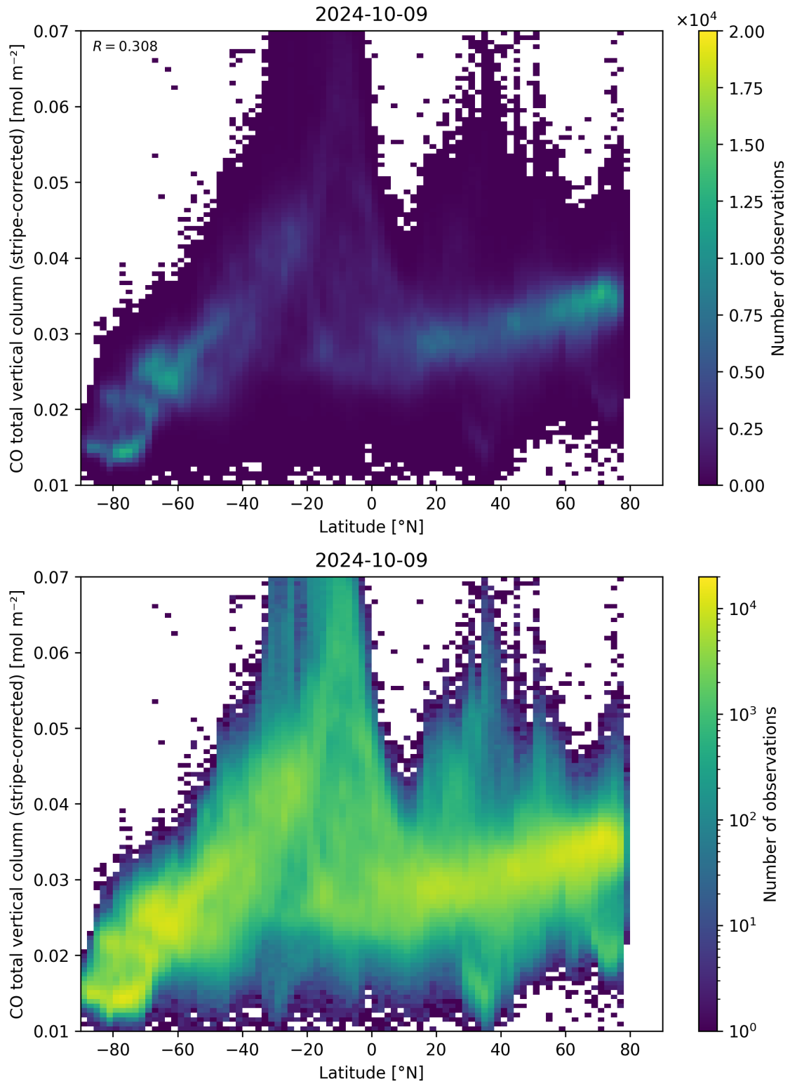
Figure 52: Scatter density plot of “Latitude” against “CO total vertical column (stripe-corrected)” for 2024-10-08 to 2024-10-10.
