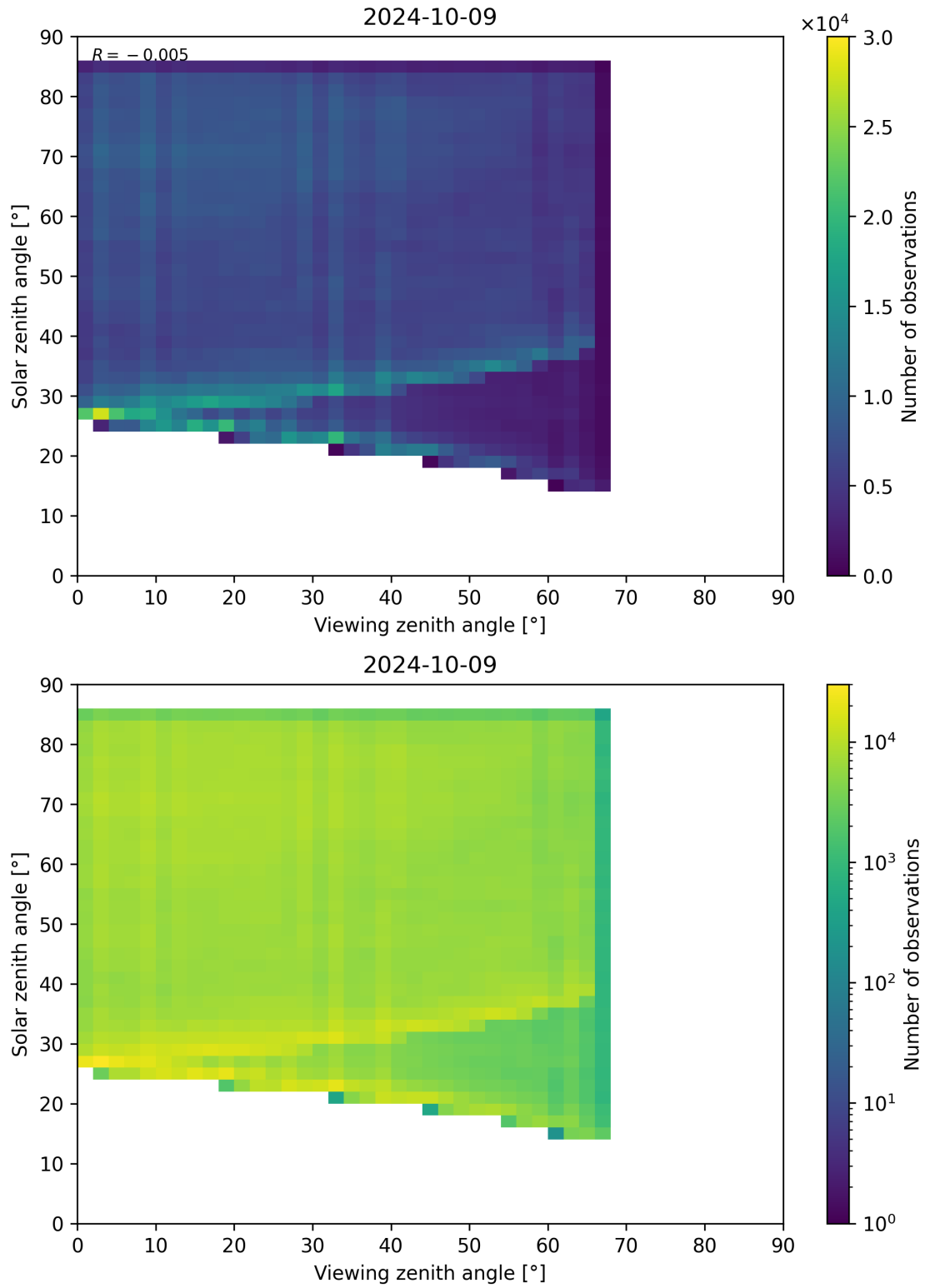
Figure 77: Scatter density plot of “Viewing zenith angle” against “Solar zenith angle” for 2024-10-08 to 2024-10-10.
