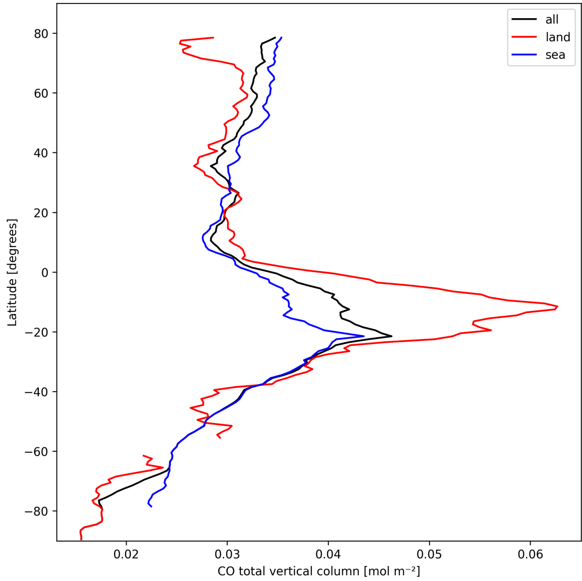
Figure 10: Zonal average of “CO total vertical column” for 2024-10-08 to 2024-10-10.
