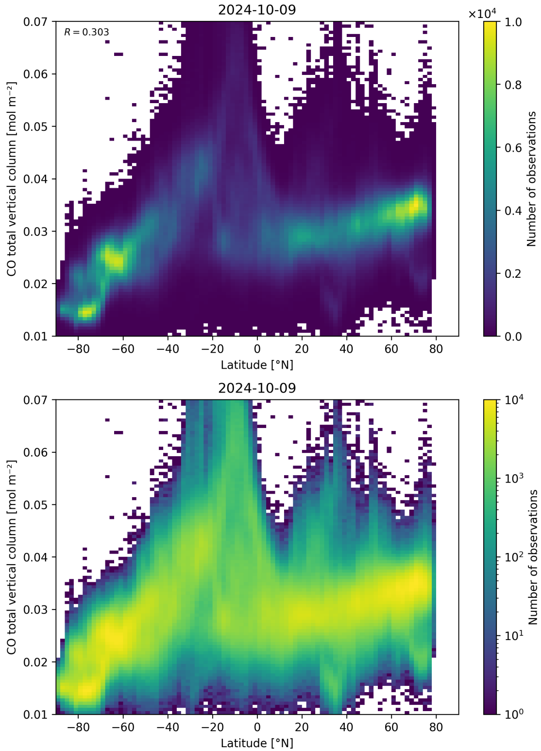
Figure 51: Scatter density plot of “Latitude” against “CO total vertical column” for 2024-10-08 to 2024-10-10.
