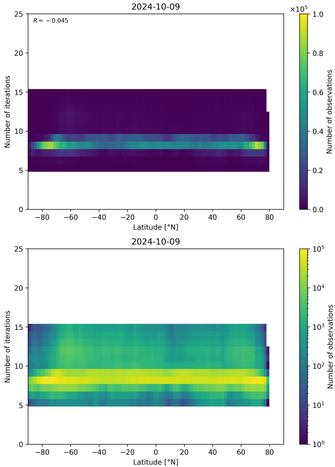
Figure 56: Scatter density plot of “Latitude” against “Number of iterations” for 2024-10-08 to 2024-10-10.
