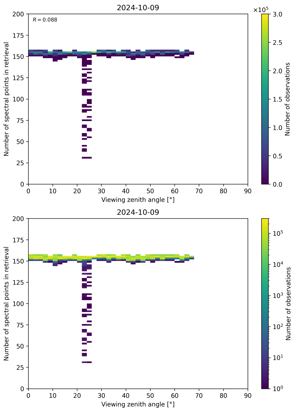
Figure 76: Scatter density plot of “Viewing zenith angle” against “Number of spectral points in retrieval” for 2024-10-08 to 2024-10-10.
