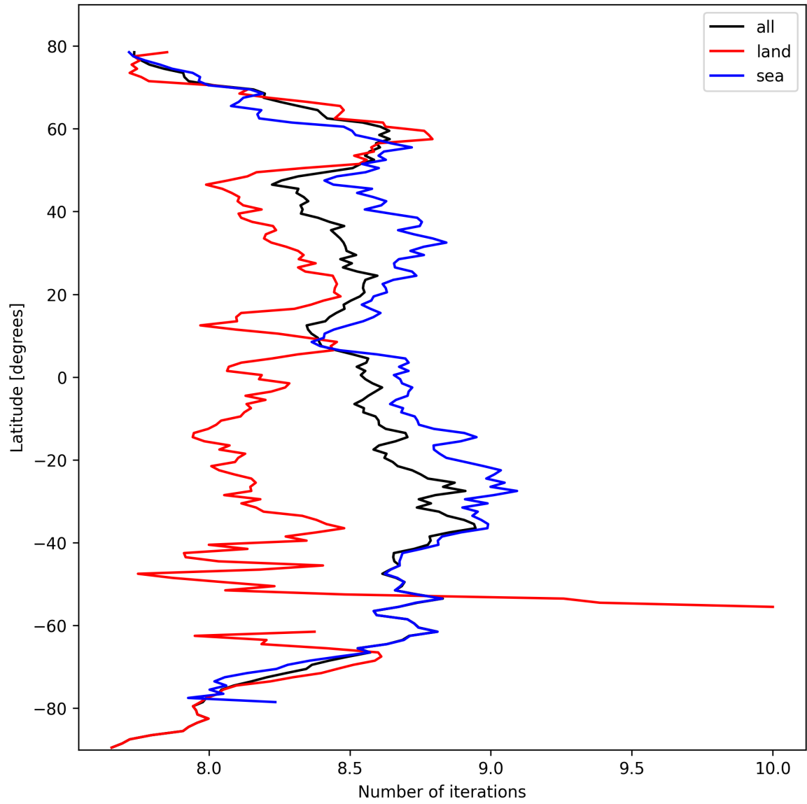
Figure 16: Zonal average of “Number of iterations” for 2024-10-08 to 2024-10-10.
