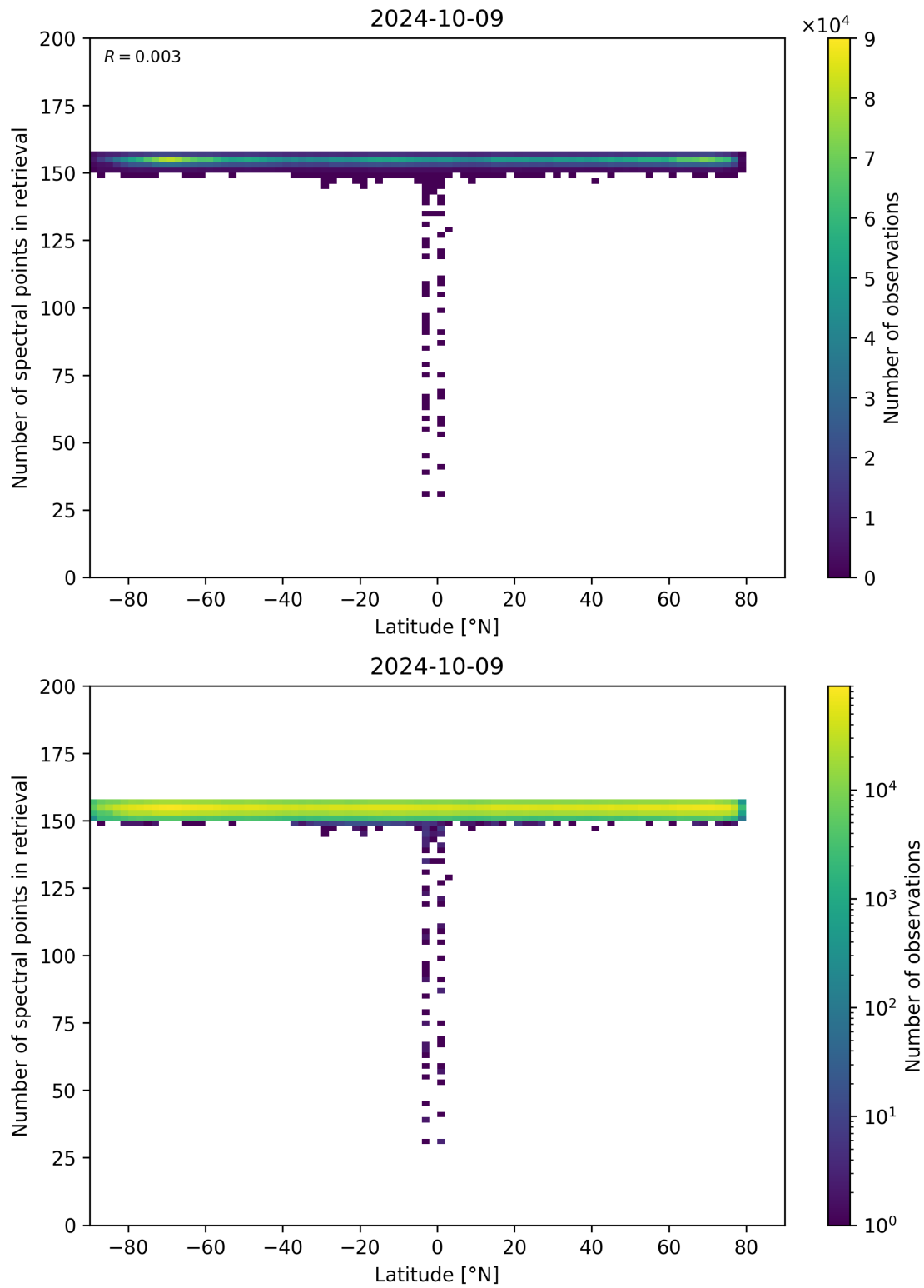
Figure 57: Scatter density plot of “Latitude” against “Number of spectral points in retrieval” for 2024-10-08 to 2024-10-10.
