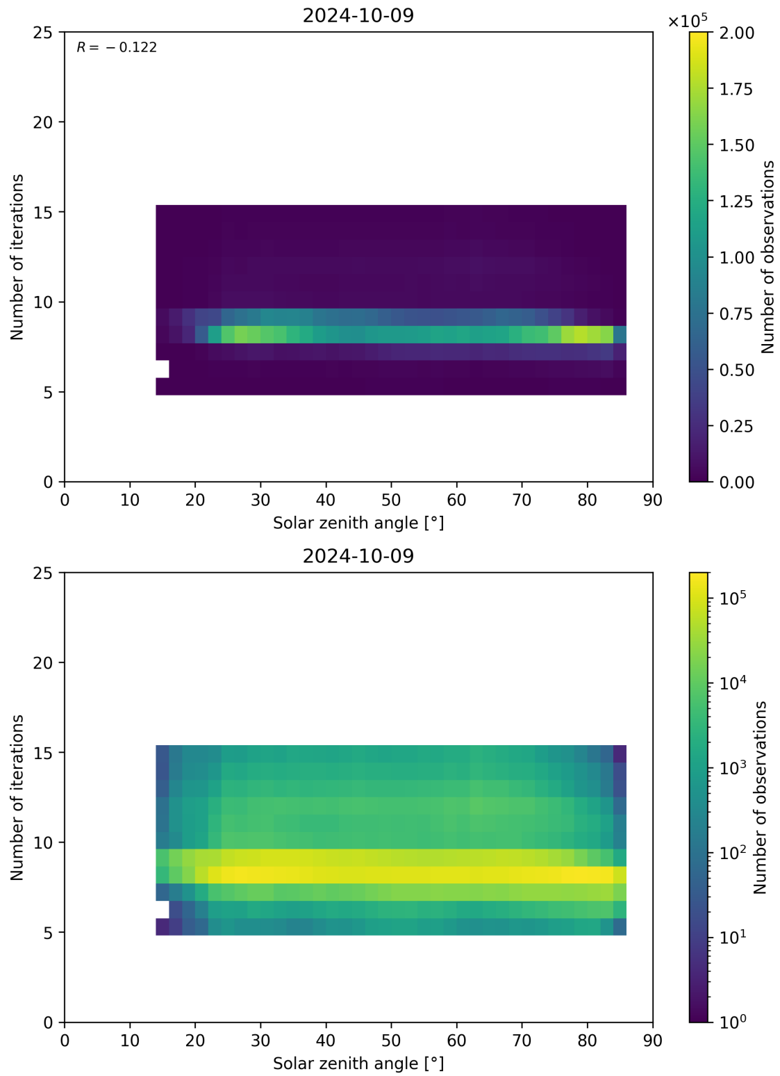
Figure 67: Scatter density plot of “Solar zenith angle” against “Number of iterations” for 2024-10-08 to 2024-10-10.
