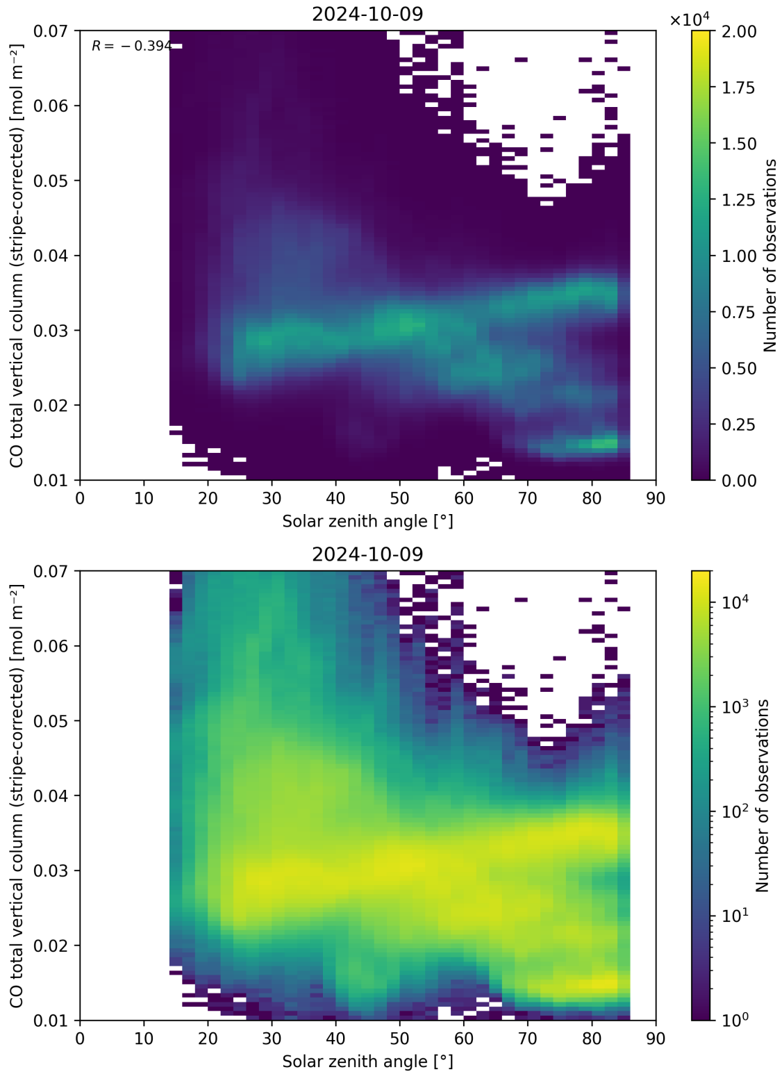
Figure 62: Scatter density plot of “Solar zenith angle” against “CO total vertical column (stripe-corrected)” for 2024-10-08 to 2024-10-10.
