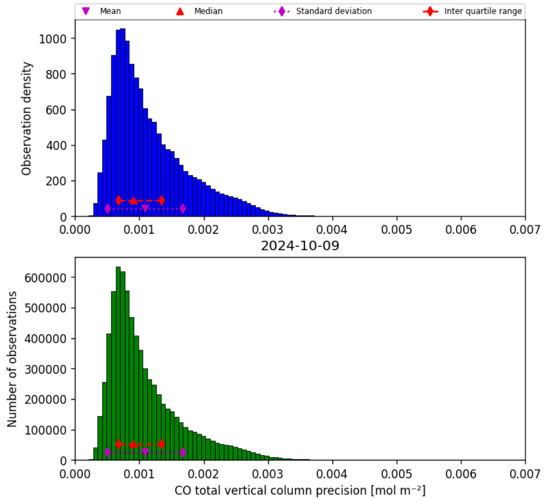
Figure 20: Histogram of “CO total vertical column precision” for 2024-10-08 to 2024-10-10
