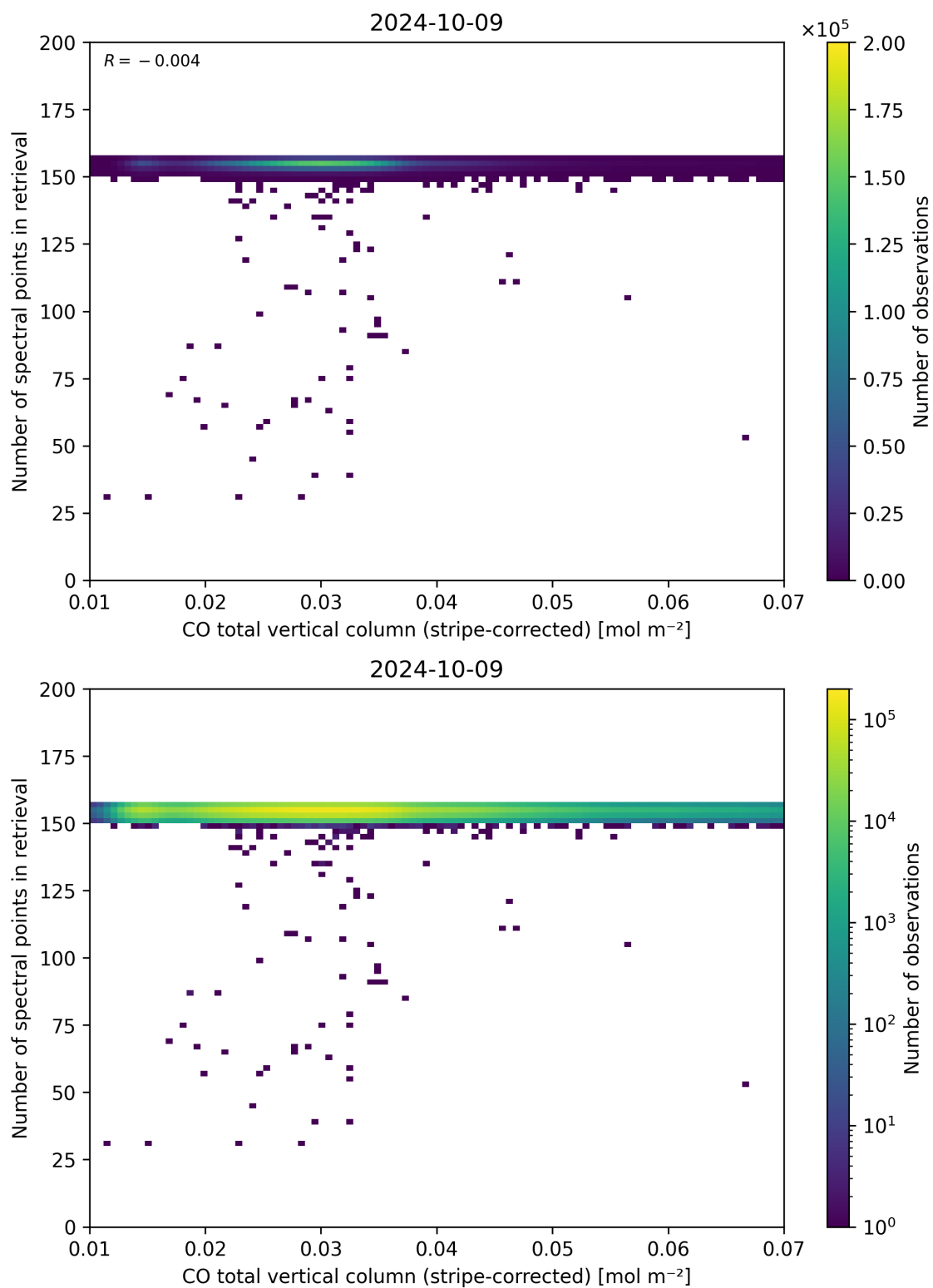
Figure 40: Scatter density plot of “CO total vertical column (stripe-corrected)” against “Number of spectral points in retrieval” for 2024-10-08 to 2024-10-10.
