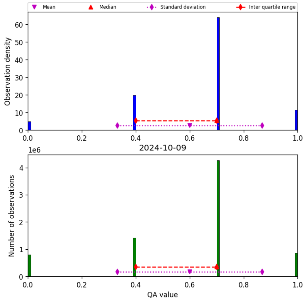
Figure 17: Histogram of “QA value” for 2024-10-08 to 2024-10-10
