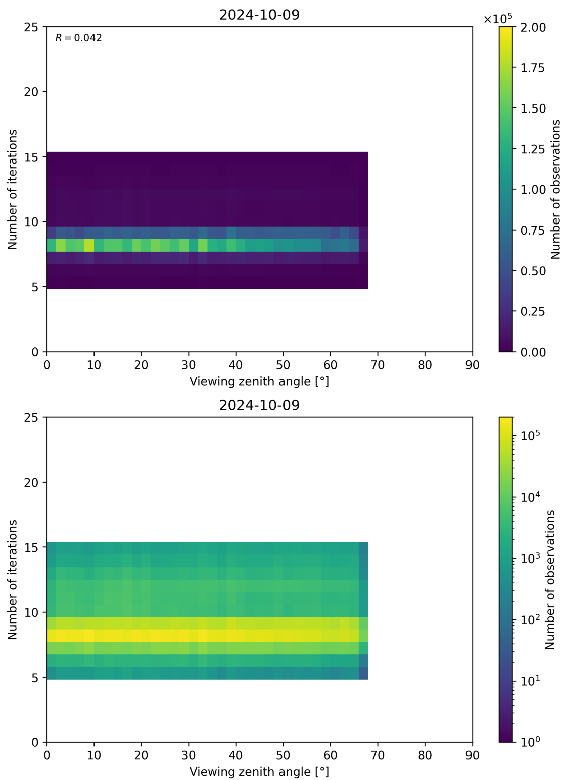
Figure 75: Scatter density plot of “Viewing zenith angle” against “Number of iterations” for 2024-10-08 to 2024-10-10.
