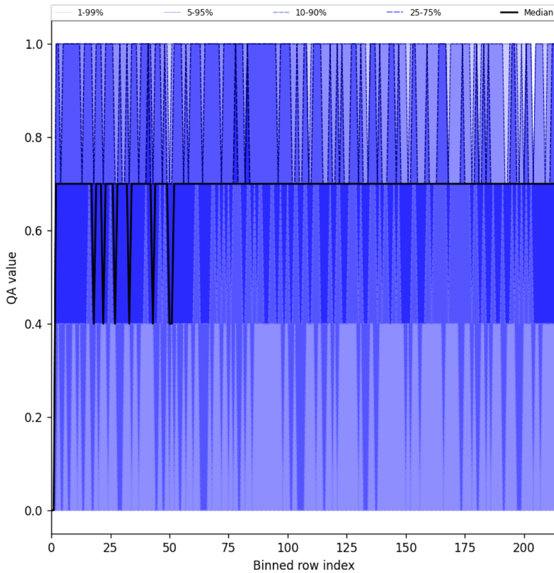
Figure 25: Along track statistics of “QA value” for 2024-10-08 to 2024-10-10
