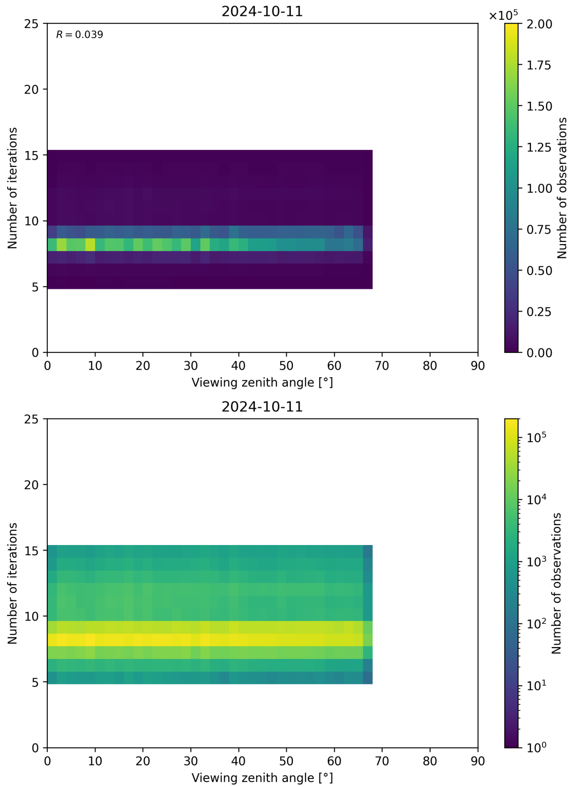
Figure 75: Scatter density plot of “Viewing zenith angle” against “Number of iterations” for 2024-10-10 to 2024-10-12.
