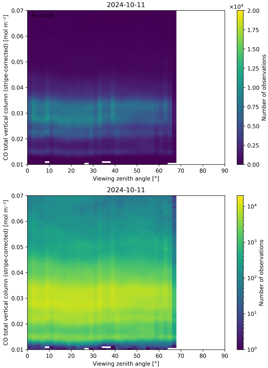
Figure 70: Scatter density plot of “Viewing zenith angle” against “CO total vertical column (stripe-corrected)” for 2024-10-10 to 2024-10-12.
