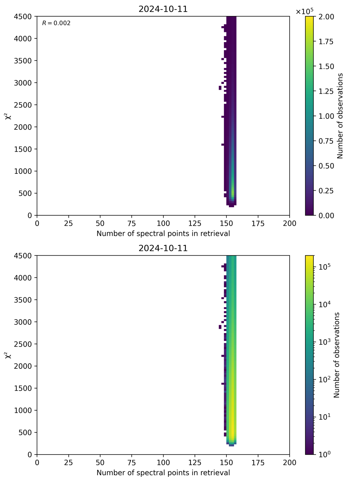
Figure 58: Scatter density plot of “Number of spectral points in retrieval” against “ \chi^2 ” for 2024-10-10 to 2024-10-12.
