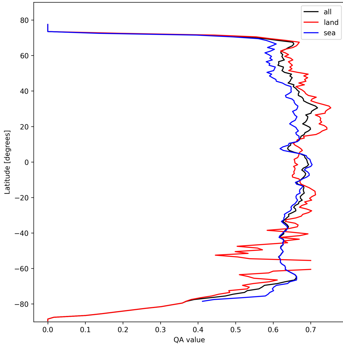
Figure 9: Zonal average of “QA value” for 2024-10-10 to 2024-10-12.
