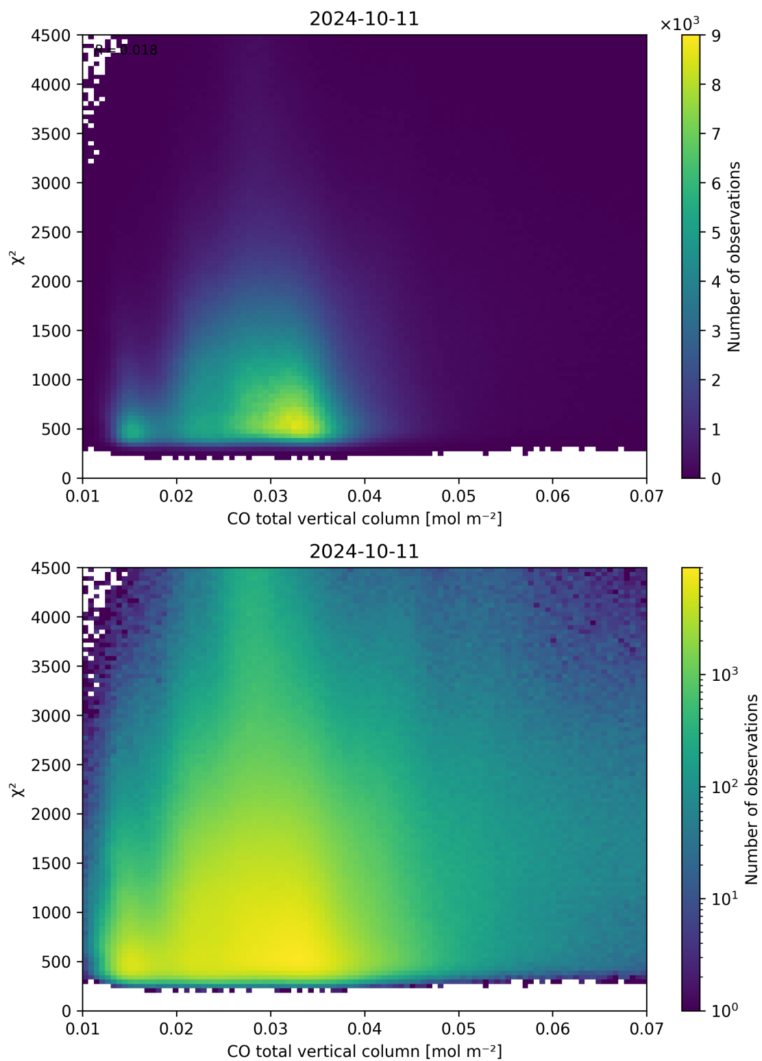
Figure 35: Scatter density plot of “CO total vertical column” against “ \chi^2 ” for 2024-10-10 to 2024-10-12.
