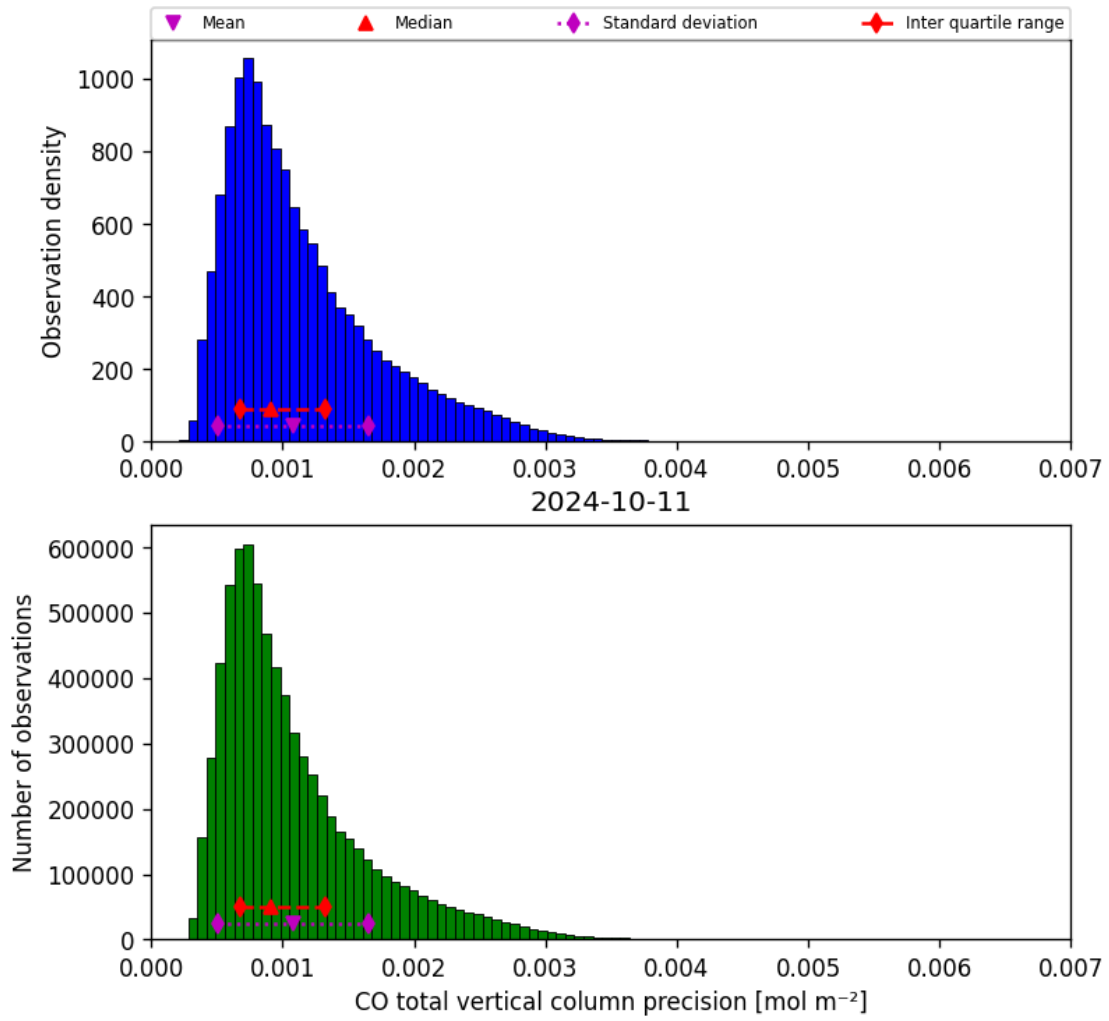
Figure 20: Histogram of “CO total vertical column precision” for 2024-10-10 to 2024-10-12
