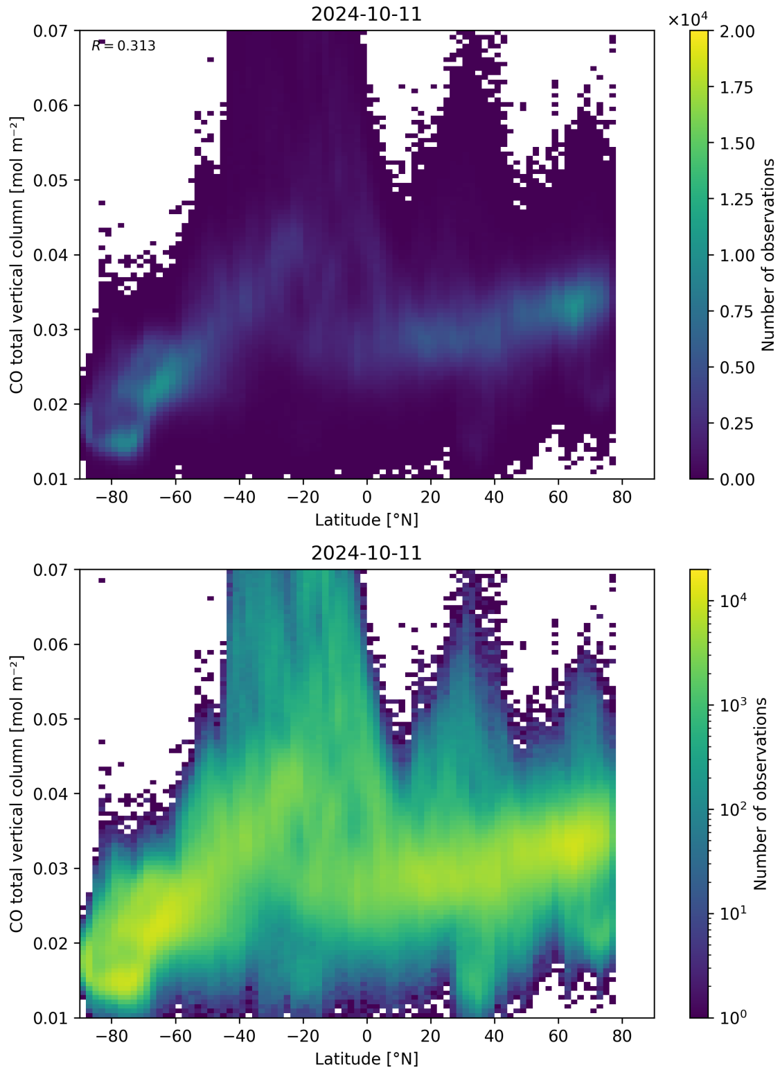
Figure 51: Scatter density plot of “Latitude” against “CO total vertical column” for 2024-10-10 to 2024-10-12.
