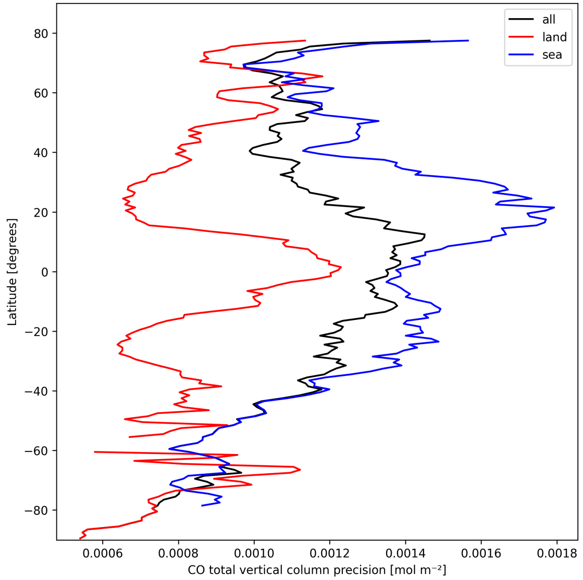
Figure 12: Zonal average of “CO total vertical column precision” for 2024-10-10 to 2024-10-12.
