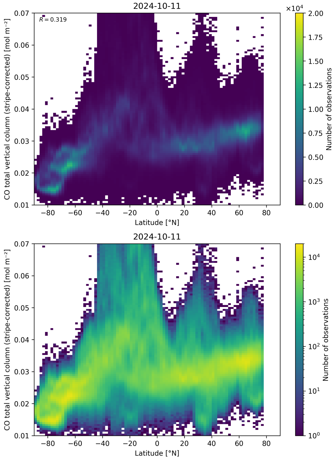
Figure 52: Scatter density plot of “Latitude” against “CO total vertical column (stripe-corrected)” for 2024-10-10 to 2024-10-12.
