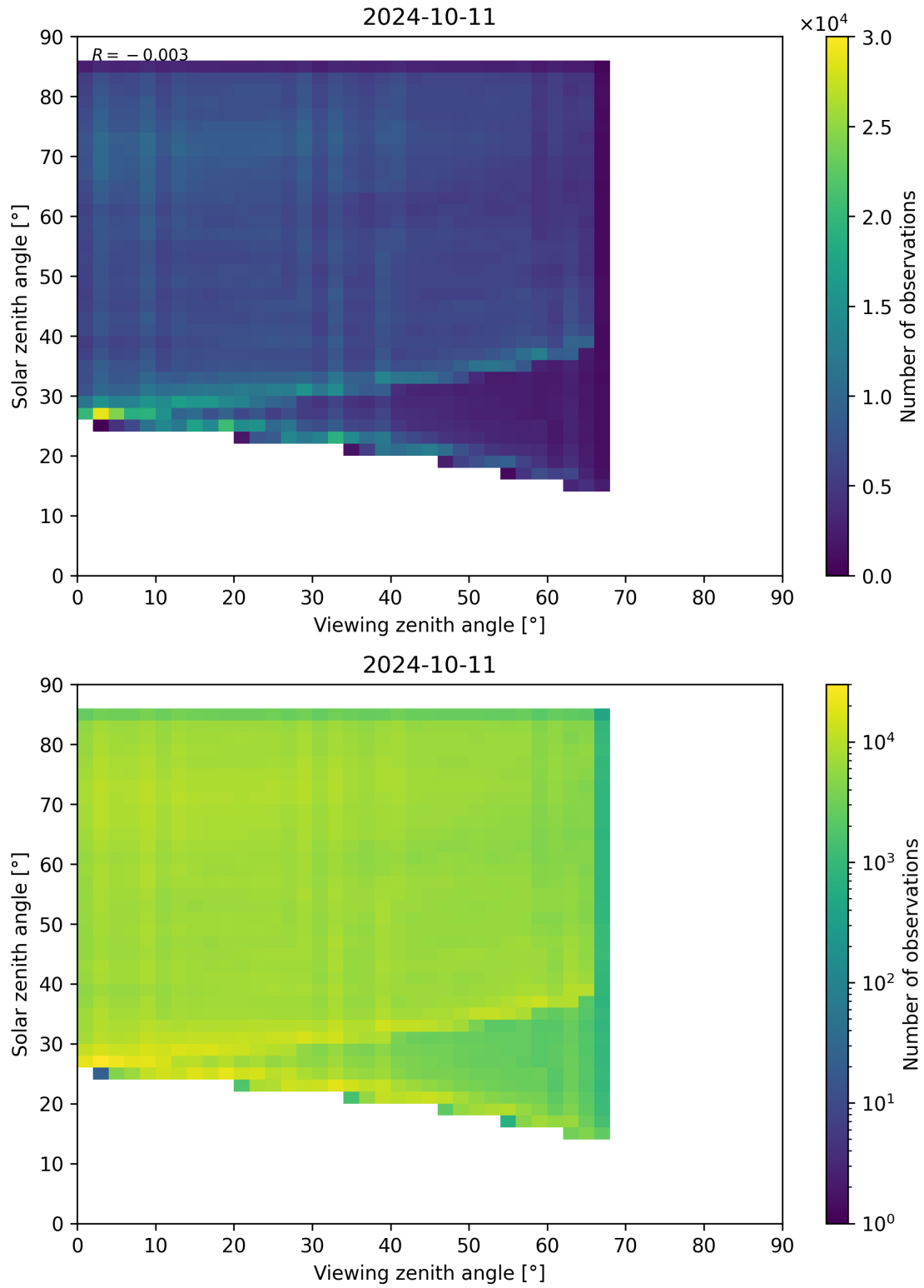
Figure 77: Scatter density plot of “Viewing zenith angle” against “Solar zenith angle” for 2024-10-10 to 2024-10-12.
