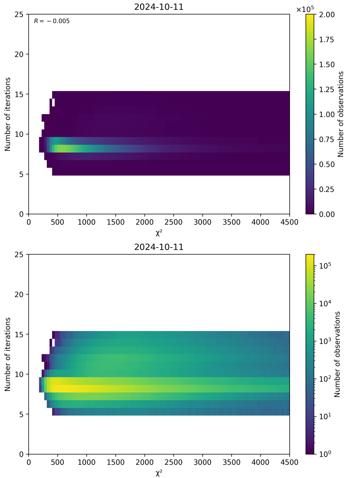
Figure 49: Scatter density plot of “ \chi^2 ” against “Number of iterations” for 2024-10-10 to 2024-10-12.
