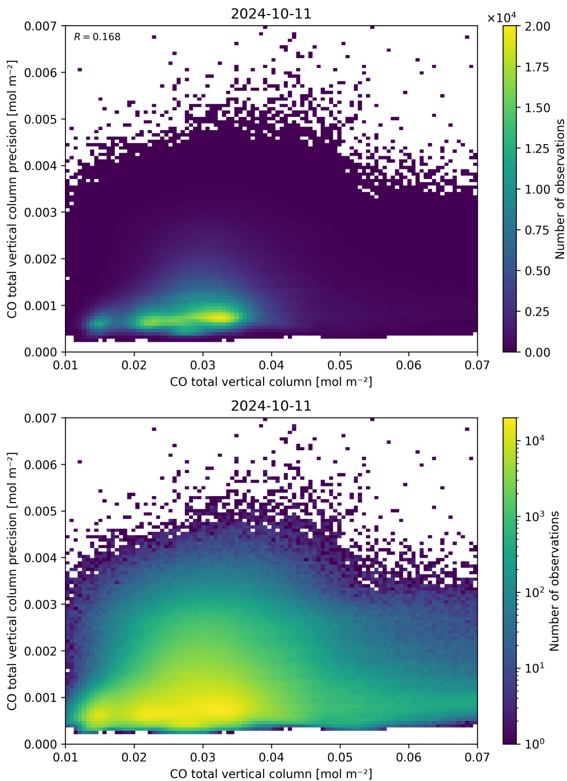
Figure 34: Scatter density plot of “CO total vertical column” against “CO total vertical column precision” for 2024-10-10 to 2024-10-12.
