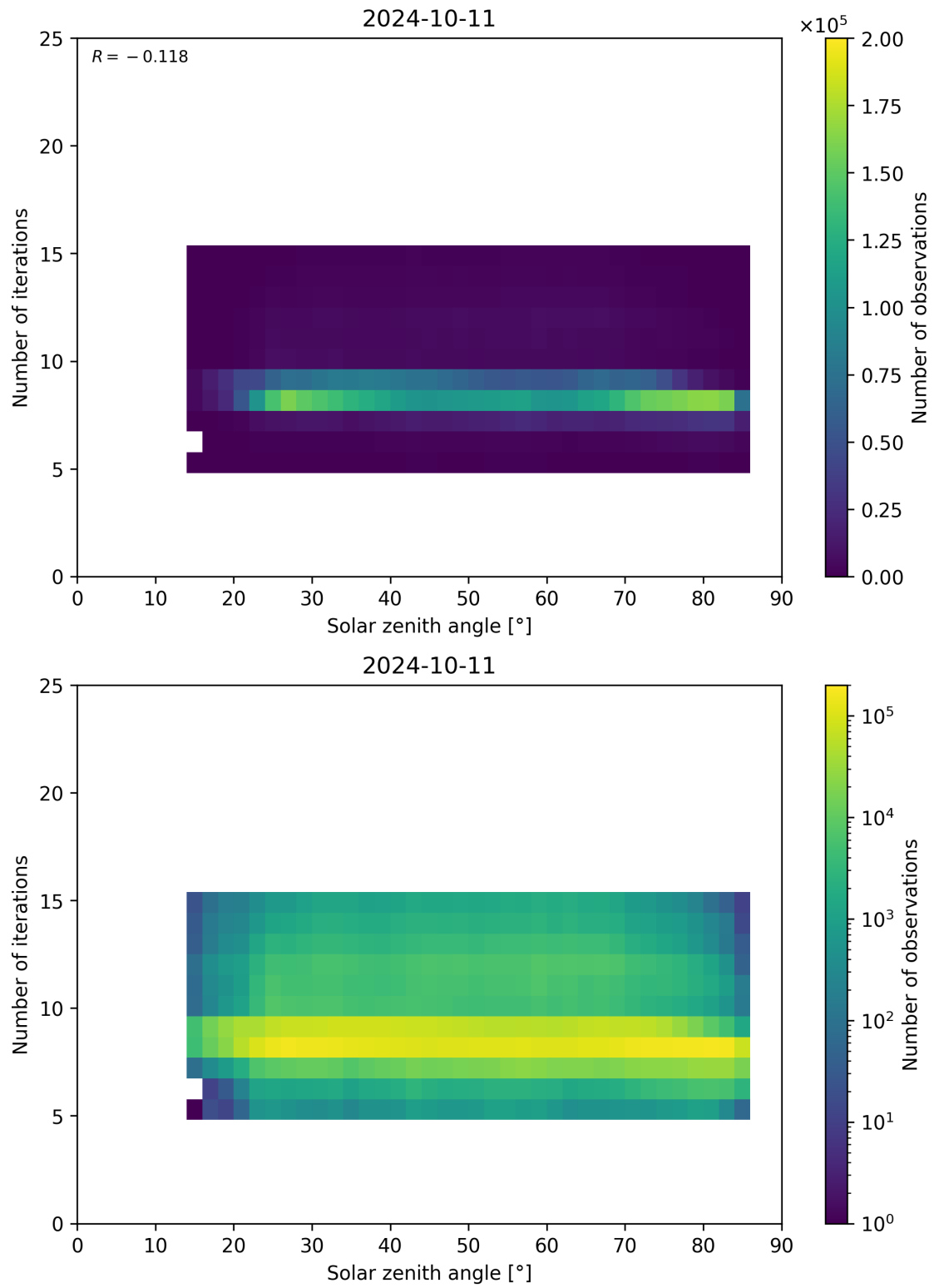
Figure 67: Scatter density plot of “Solar zenith angle” against “Number of iterations” for 2024-10-10 to 2024-10-12.
