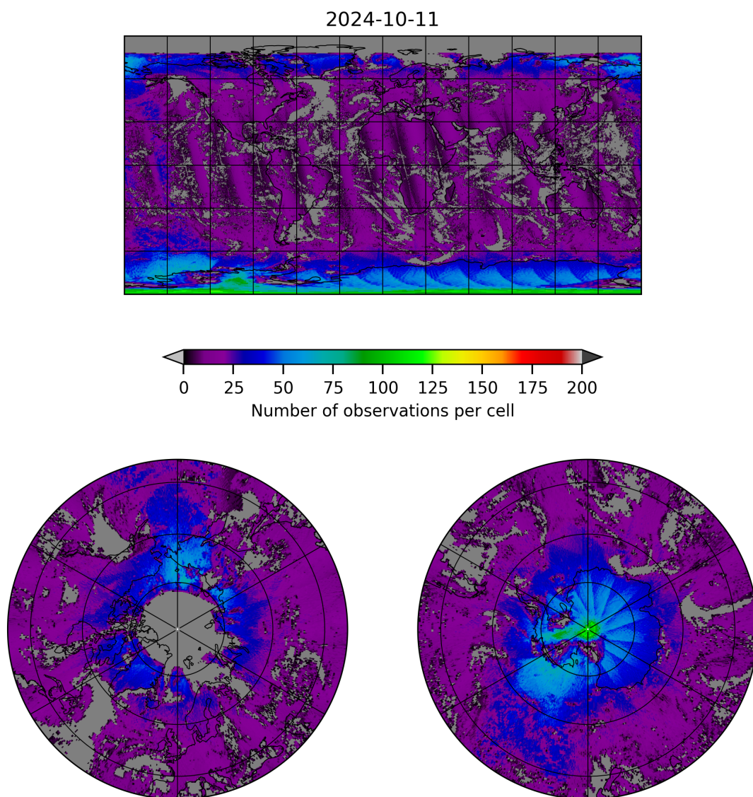
Figure 8: Map of the number of observations for 2024-10-10 to 2024-10-12
