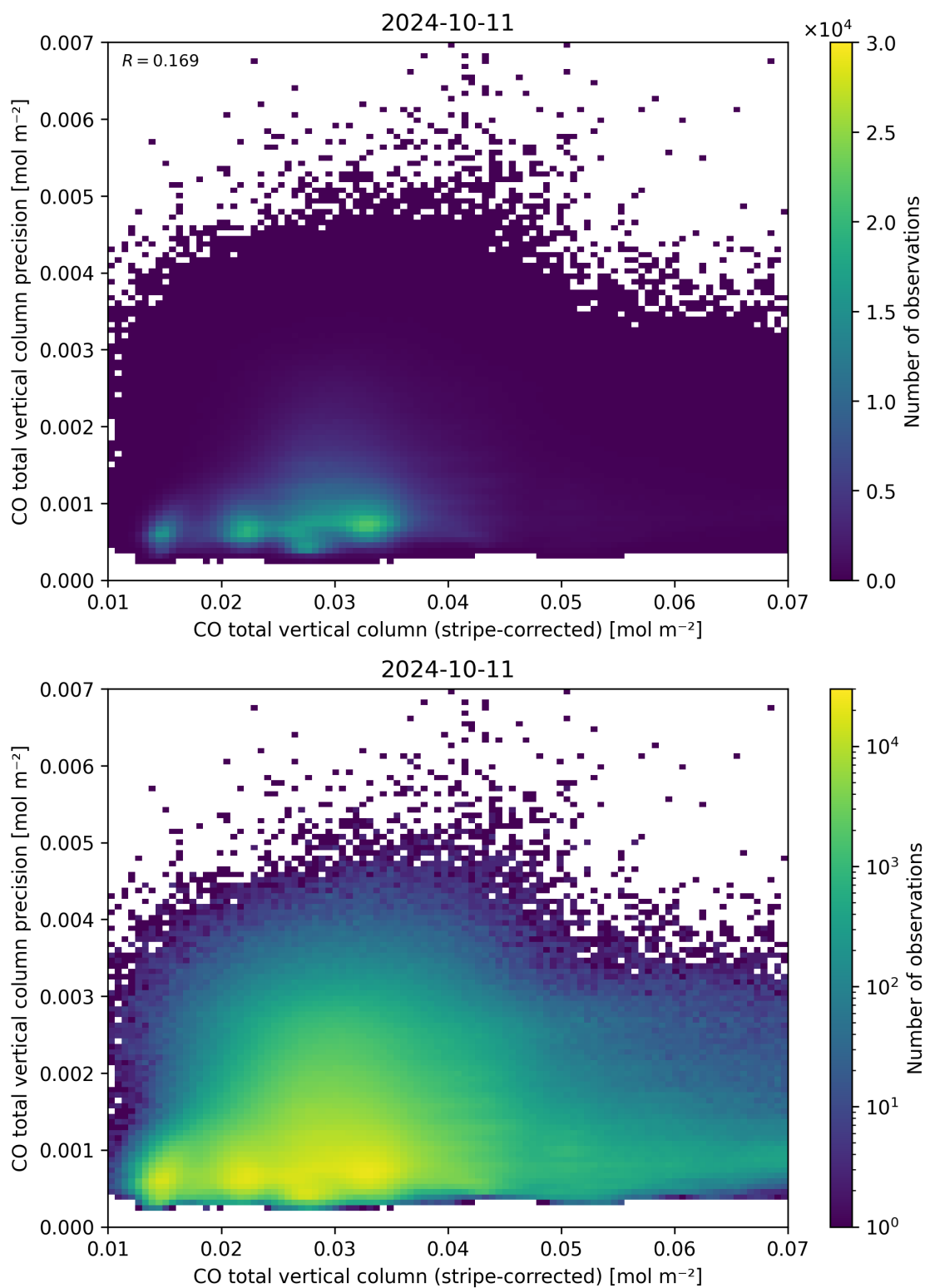
Figure 36: Scatter density plot of “CO total vertical column (stripe-corrected)” against “CO total vertical column precision” for 2024-10-10 to 2024-10-12.
