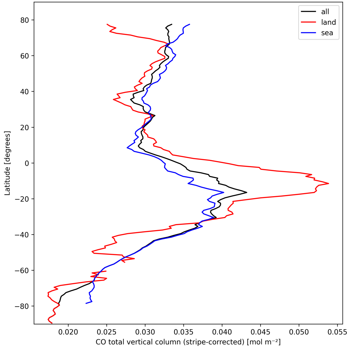
Figure 11: Zonal average of “CO total vertical column (stripe-corrected)” for 2024-10-10 to 2024-10-12.
