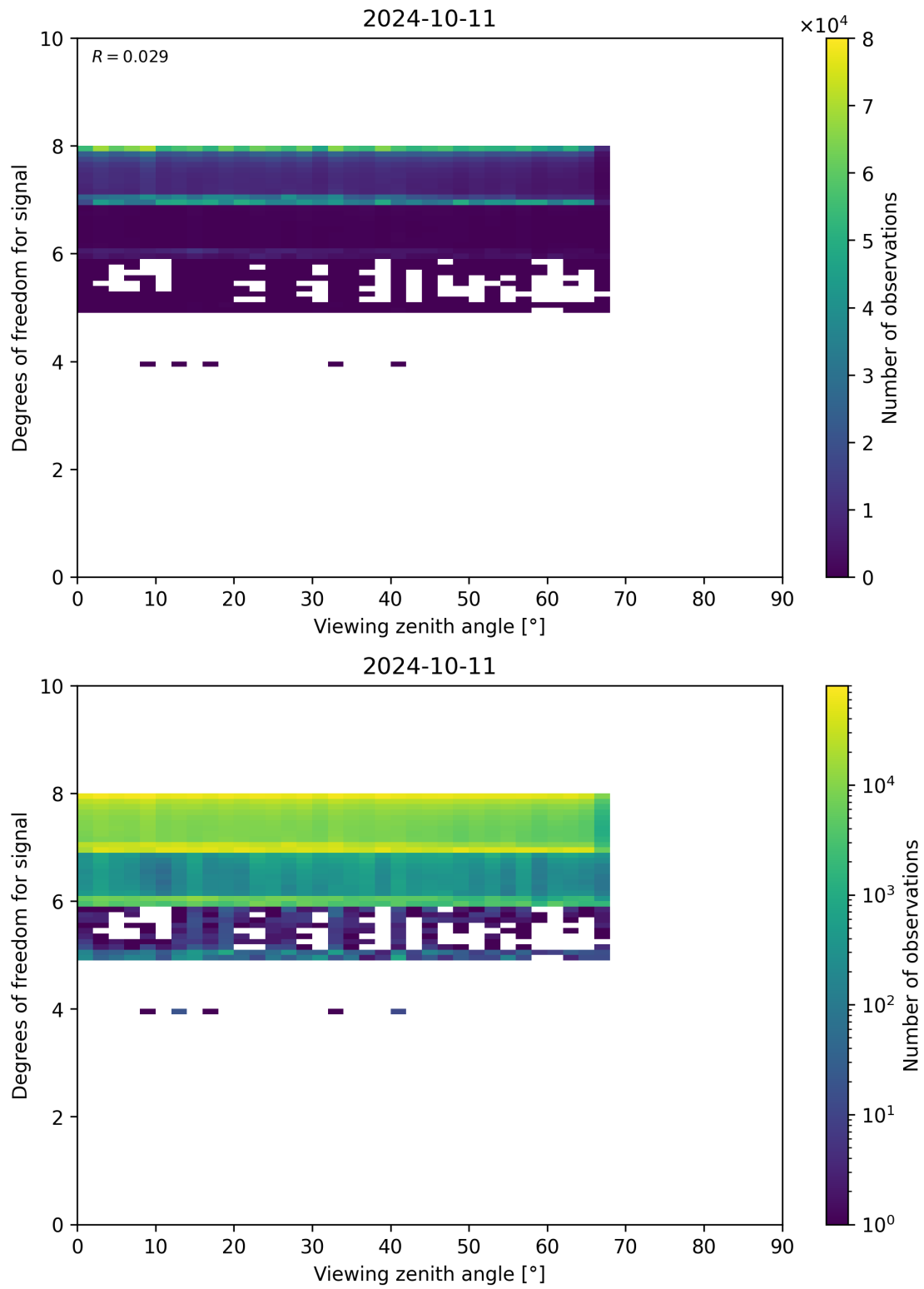
Figure 73: Scatter density plot of “Viewing zenith angle” against “Degrees of freedom for signal” for 2024-10-10 to 2024-10-12.
