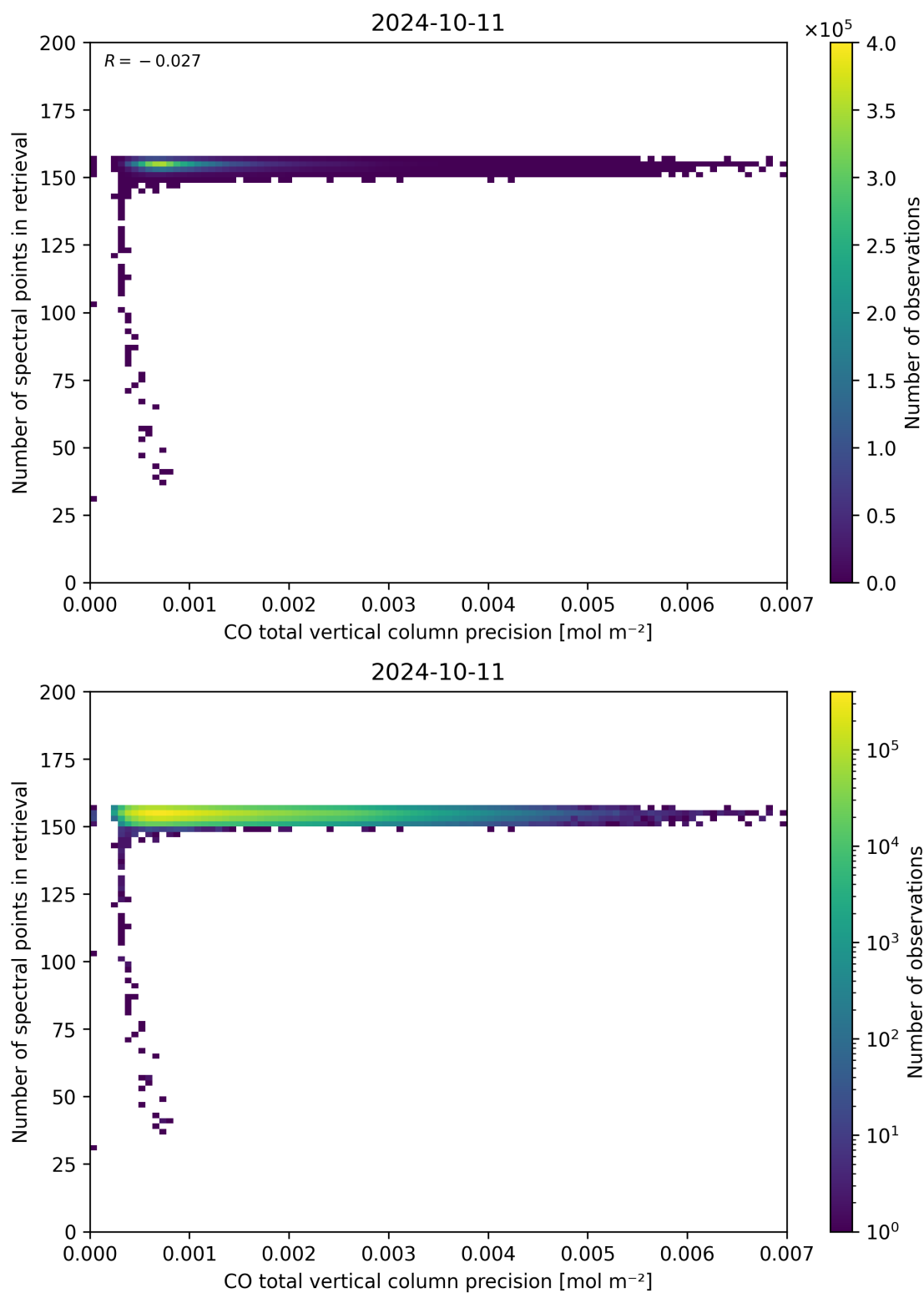
Figure 47: Scatter density plot of “CO total vertical column precision” against “Number of spectral points in retrieval” for 2024-10-10 to 2024-10-12.
