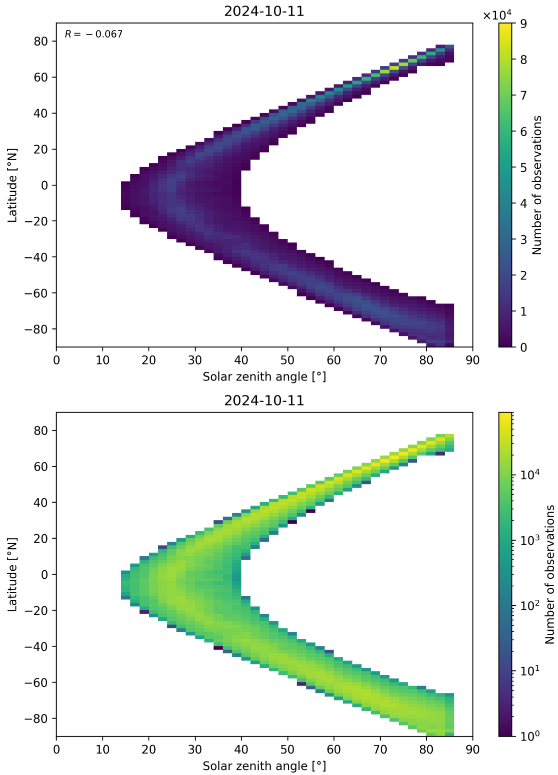
Figure 66: Scatter density plot of “Solar zenith angle” against “Latitude” for 2024-10-10 to 2024-10-12.
