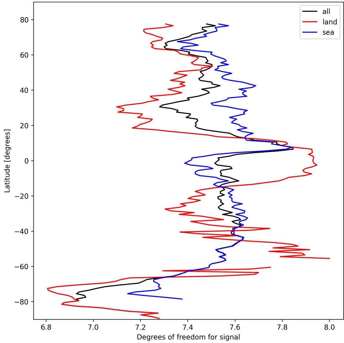
Figure 15: Zonal average of “Degrees of freedom for signal” for 2024-10-10 to 2024-10-12.
