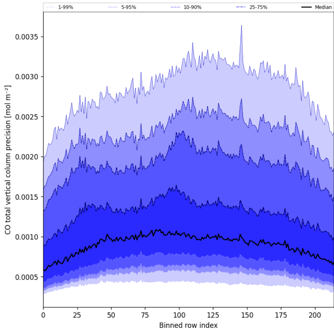
Figure 28: Along track statistics of “CO total vertical column precision” for 2024-10-10 to 2024-10-12
