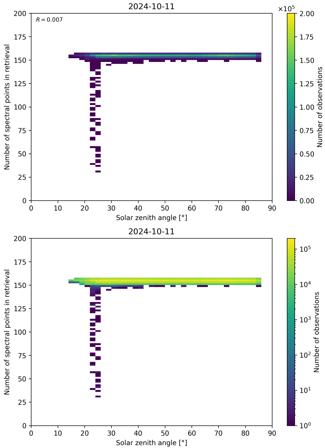
Figure 68: Scatter density plot of “Solar zenith angle” against “Number of spectral points in retrieval” for 2024-10-10 to 2024-10-12.
