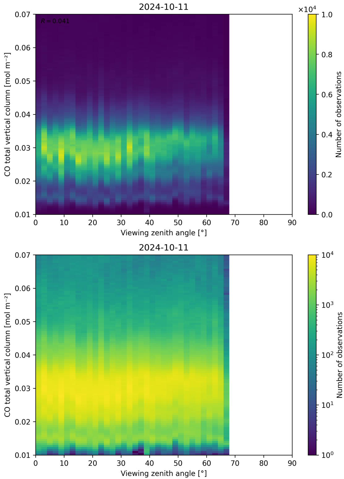
Figure 69: Scatter density plot of “Viewing zenith angle” against “CO total vertical column” for 2024-10-10 to 2024-10-12.
