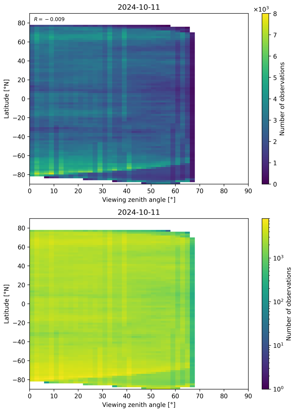
Figure 74: Scatter density plot of “Viewing zenith angle” against “Latitude” for 2024-10-10 to 2024-10-12.
