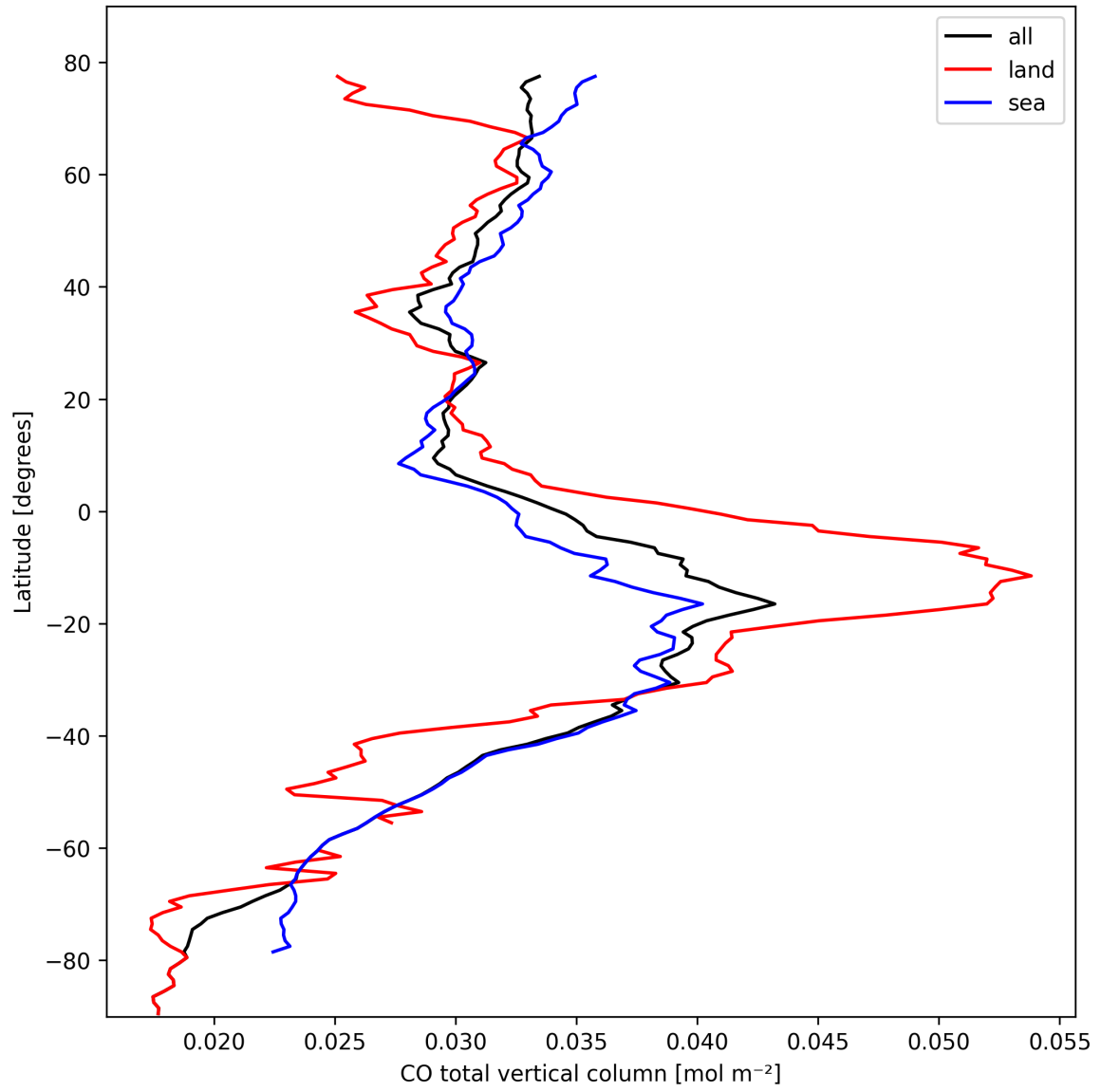
Figure 10: Zonal average of “CO total vertical column” for 2024-10-10 to 2024-10-12.
