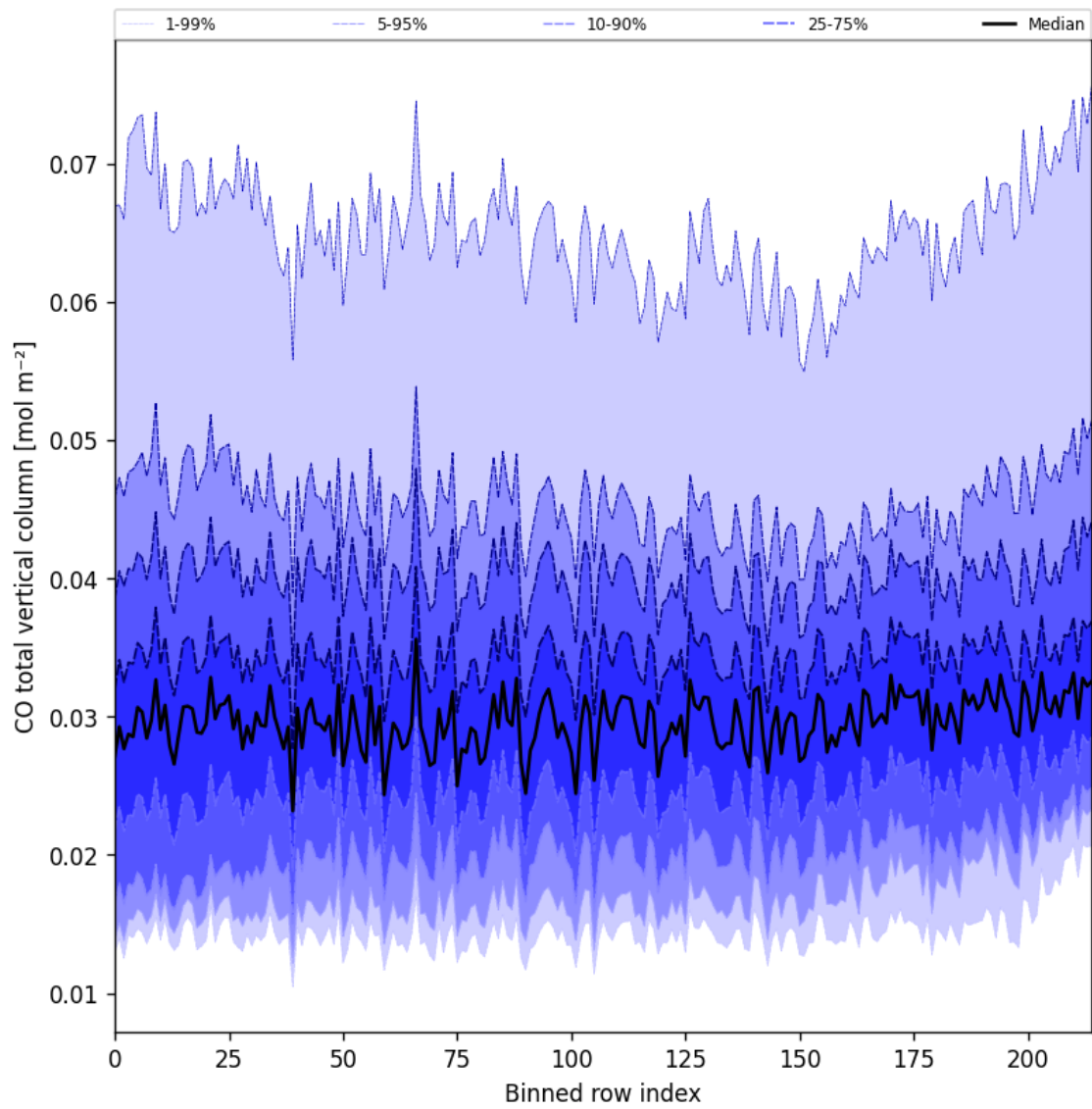
Figure 26: Along track statistics of “CO total vertical column” for 2024-10-10 to 2024-10-12
