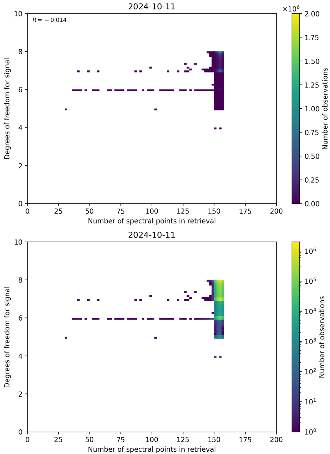
Figure 59: Scatter density plot of “Number of spectral points in retrieval” against “Degrees of freedom for signal” for 2024-10-10 to 2024-10-12.
