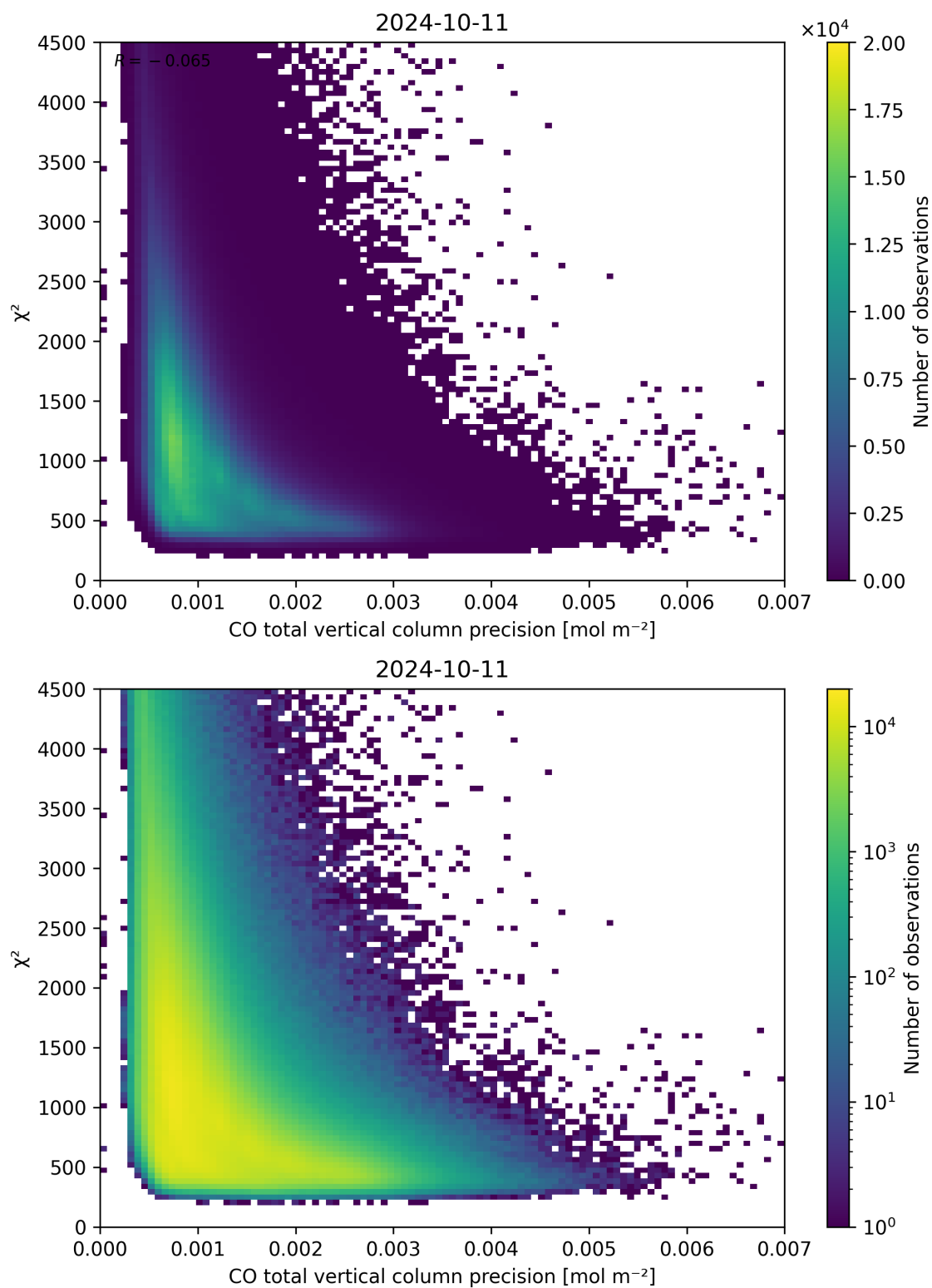
Figure 44: Scatter density plot of “CO total vertical column precision” against “ \chi^2 ” for 2024-10-10 to 2024-10-12.
