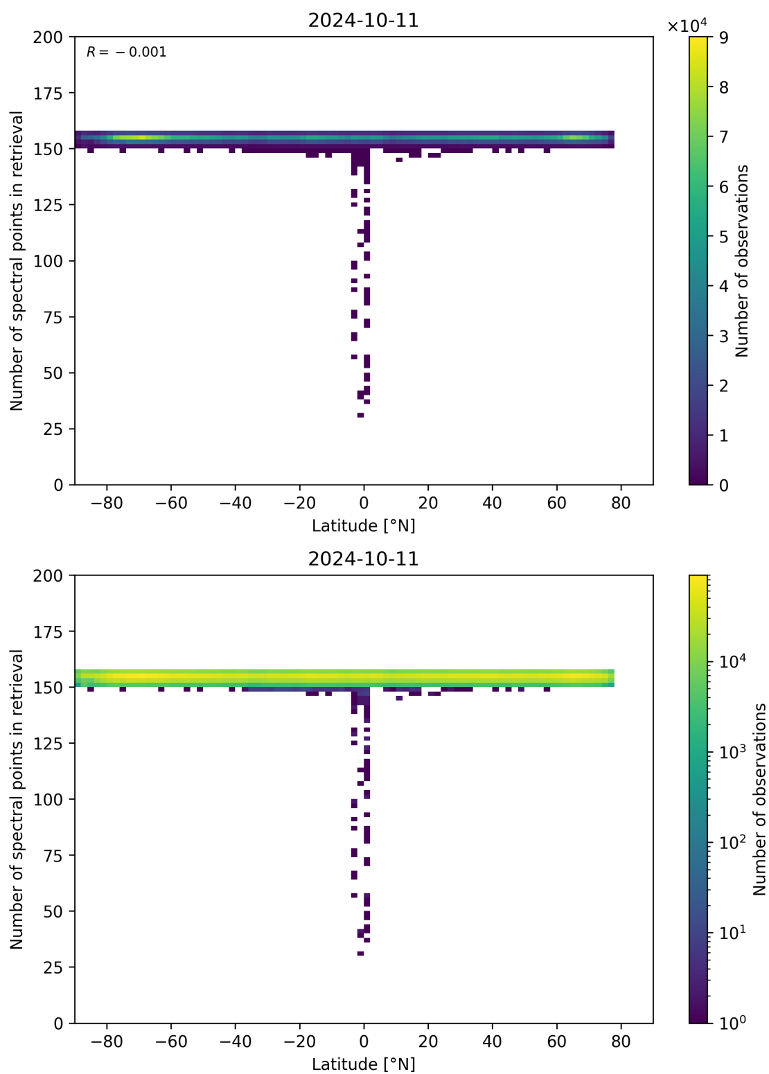
Figure 57: Scatter density plot of “Latitude” against “Number of spectral points in retrieval” for 2024-10-10 to 2024-10-12.
