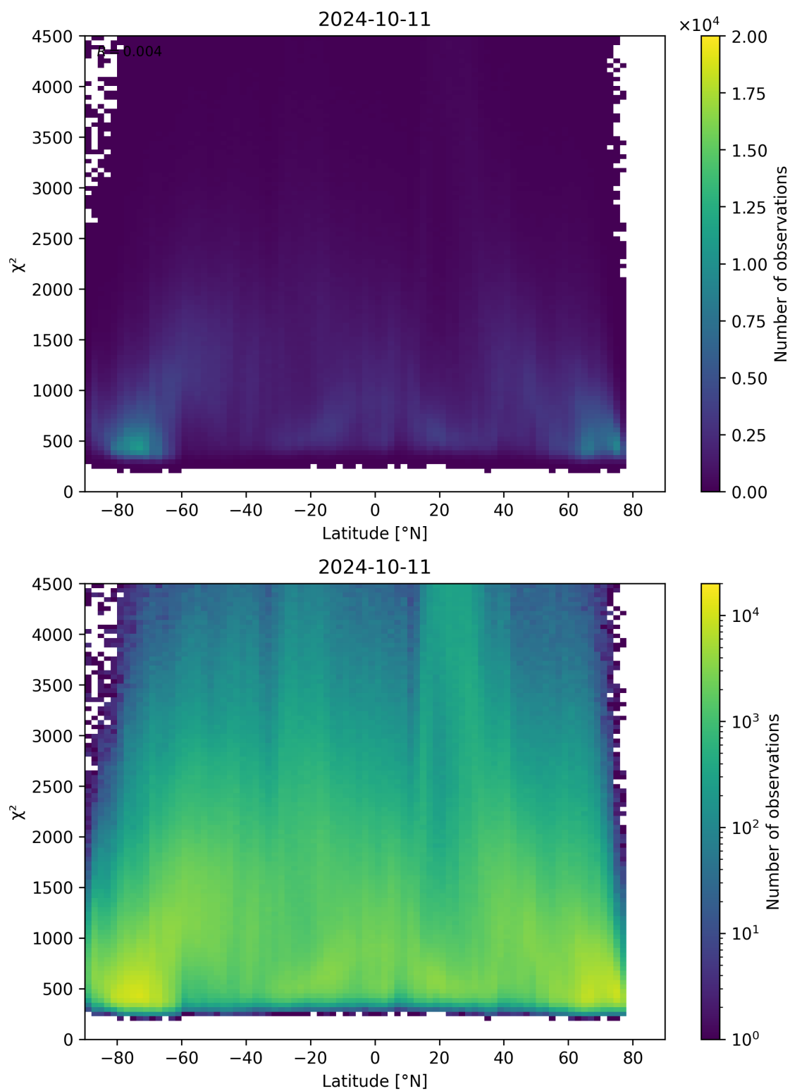
Figure 54: Scatter density plot of “Latitude” against “ \chi^2 ” for 2024-10-10 to 2024-10-12.
