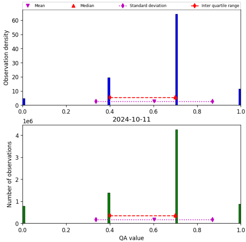
Figure 17: Histogram of “QA value” for 2024-10-10 to 2024-10-12
