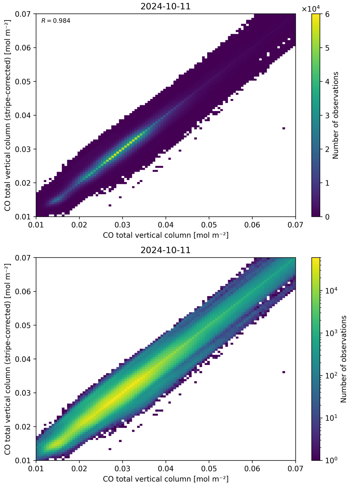
Figure 33: Scatter density plot of “CO total vertical column” against “CO total vertical column (stripe-corrected)” for 2024-10-10 to 2024-10-12.
