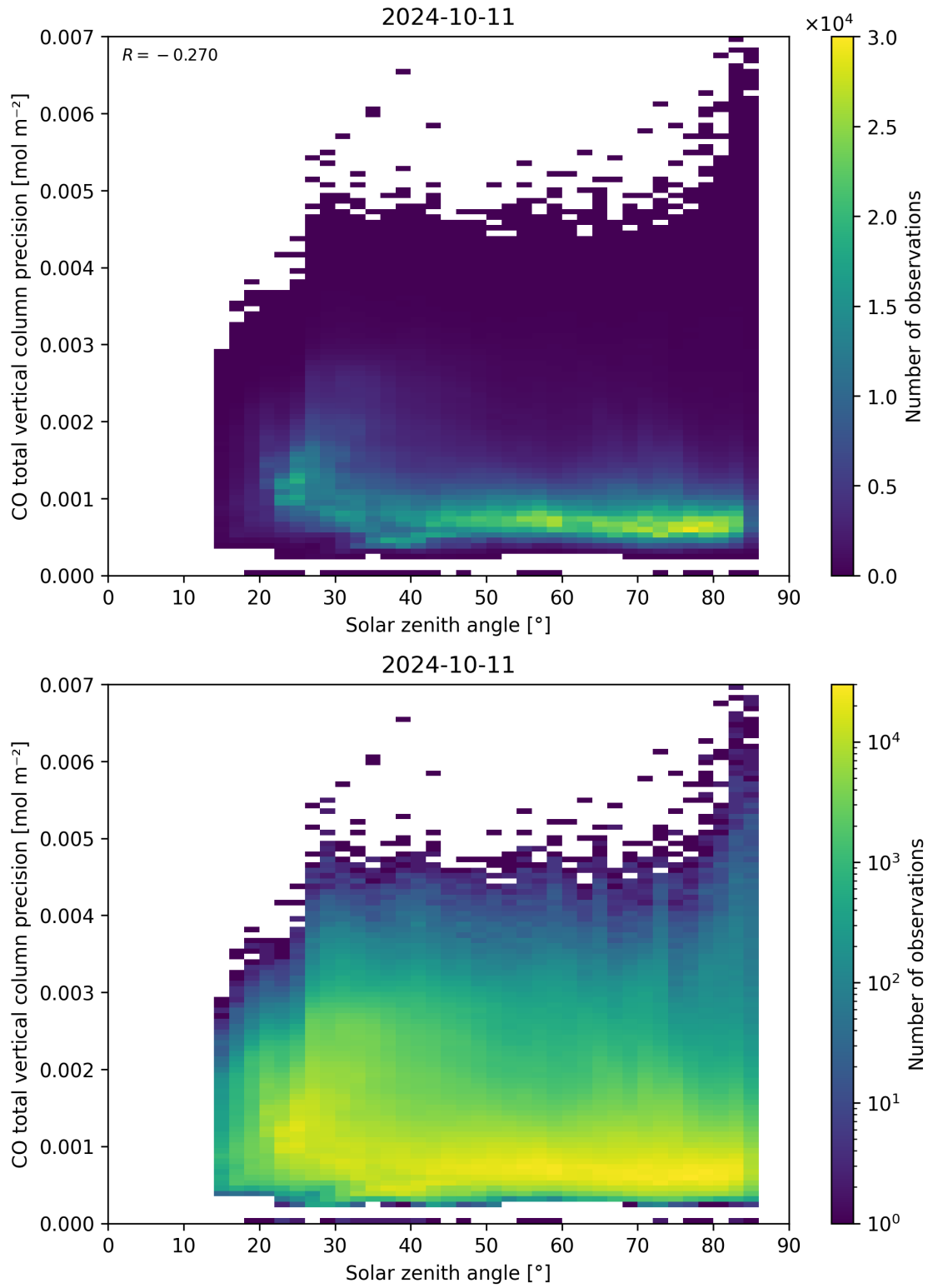
Figure 63: Scatter density plot of “Solar zenith angle” against “CO total vertical column precision” for 2024-10-10 to 2024-10-12.
