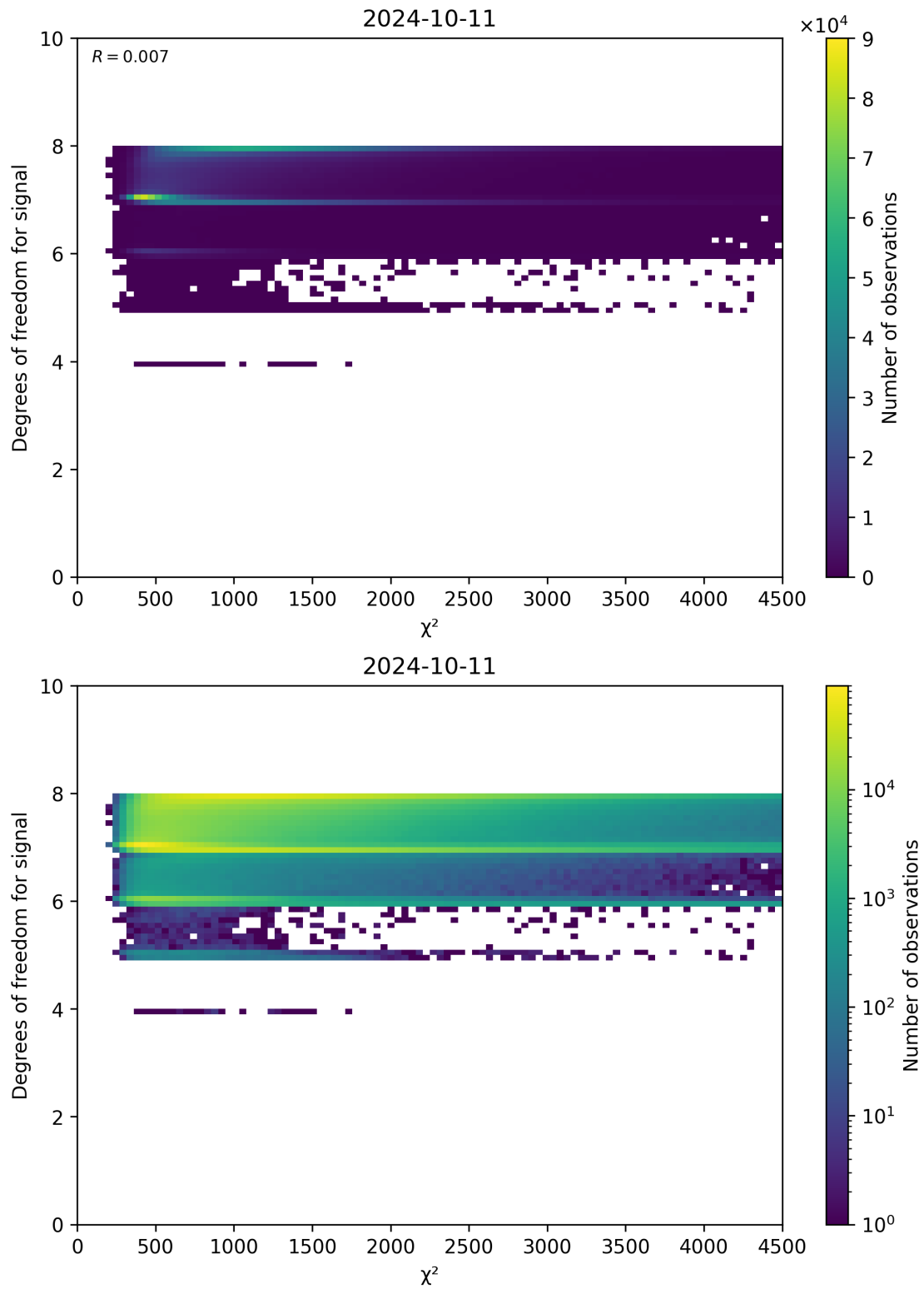
Figure 48: Scatter density plot of “ \chi^2 ” against “Degrees of freedom for signal” for 2024-10-10 to 2024-10-12.
