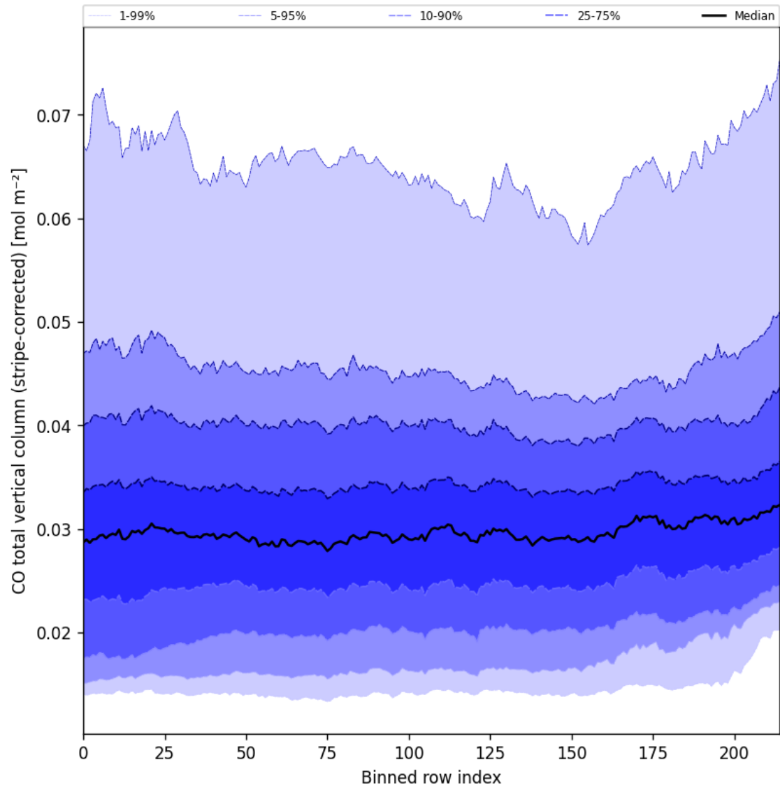
Figure 27: Along track statistics of “CO total vertical column (stripe-corrected)” for 2024-10-10 to 2024-10-12
