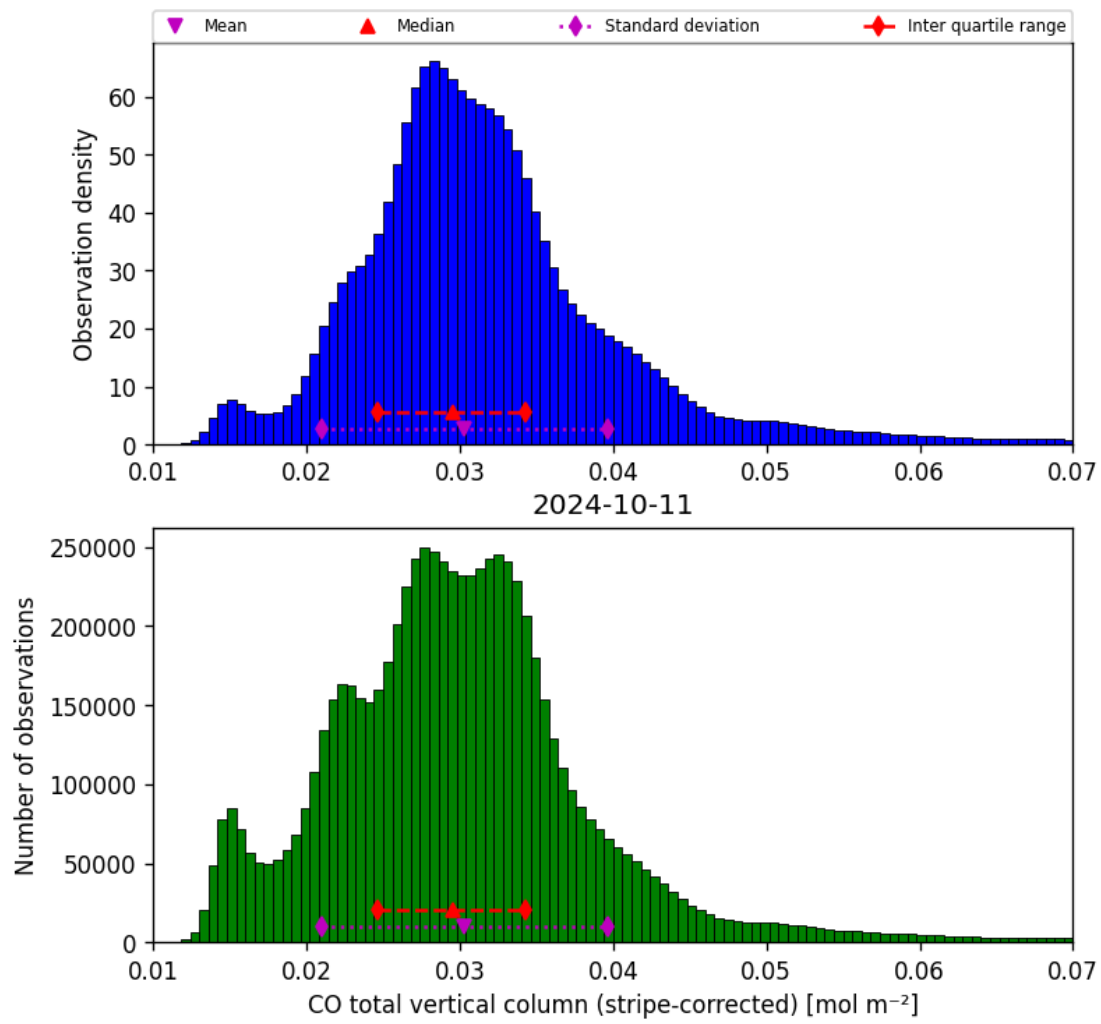
Figure 19: Histogram of “CO total vertical column (stripe-corrected)” for 2024-10-10 to 2024-10-12
