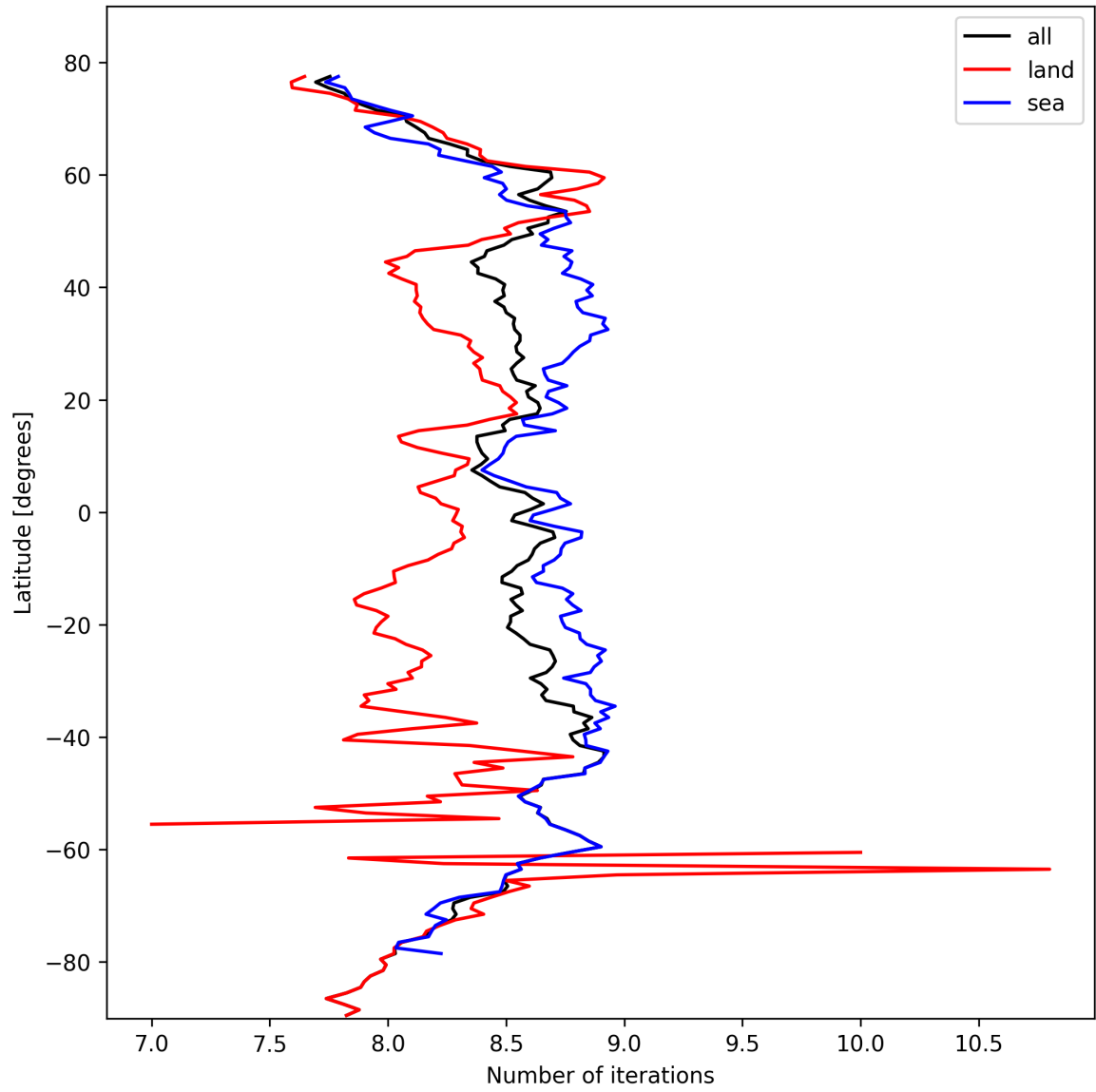
Figure 16: Zonal average of “Number of iterations” for 2024-10-10 to 2024-10-12.
