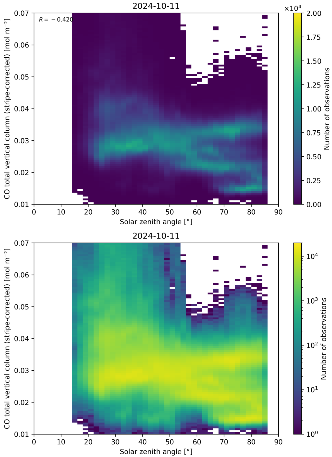
Figure 62: Scatter density plot of “Solar zenith angle” against “CO total vertical column (stripe-corrected)” for 2024-10-10 to 2024-10-12.
