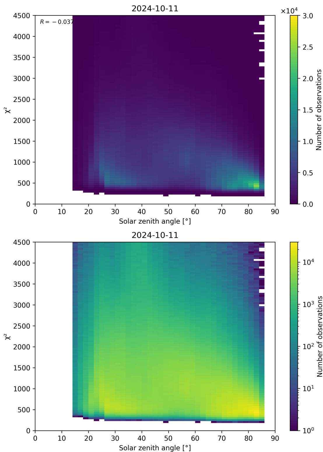
Figure 64: Scatter density plot of “Solar zenith angle” against “ \chi^2 ” for 2024-10-10 to 2024-10-12.
