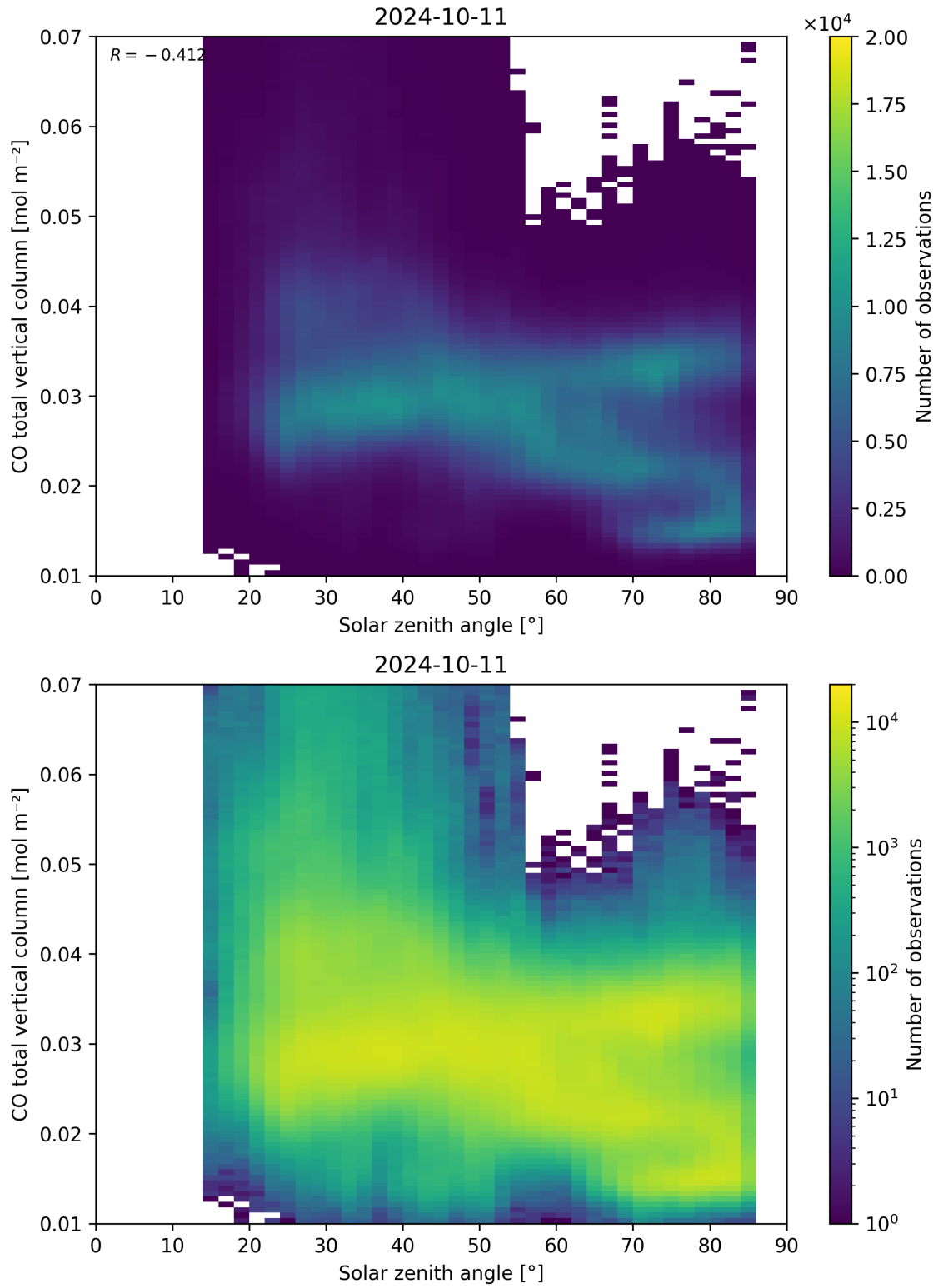
Figure 61: Scatter density plot of “Solar zenith angle” against “CO total vertical column” for 2024-10-10 to 2024-10-12.
