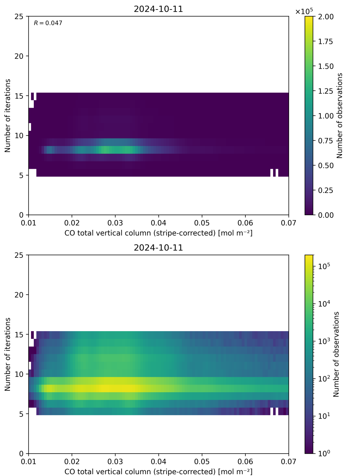
Figure 39: Scatter density plot of “CO total vertical column (stripe-corrected)” against “Number of iterations” for 2024-10-10 to 2024-10-12.
