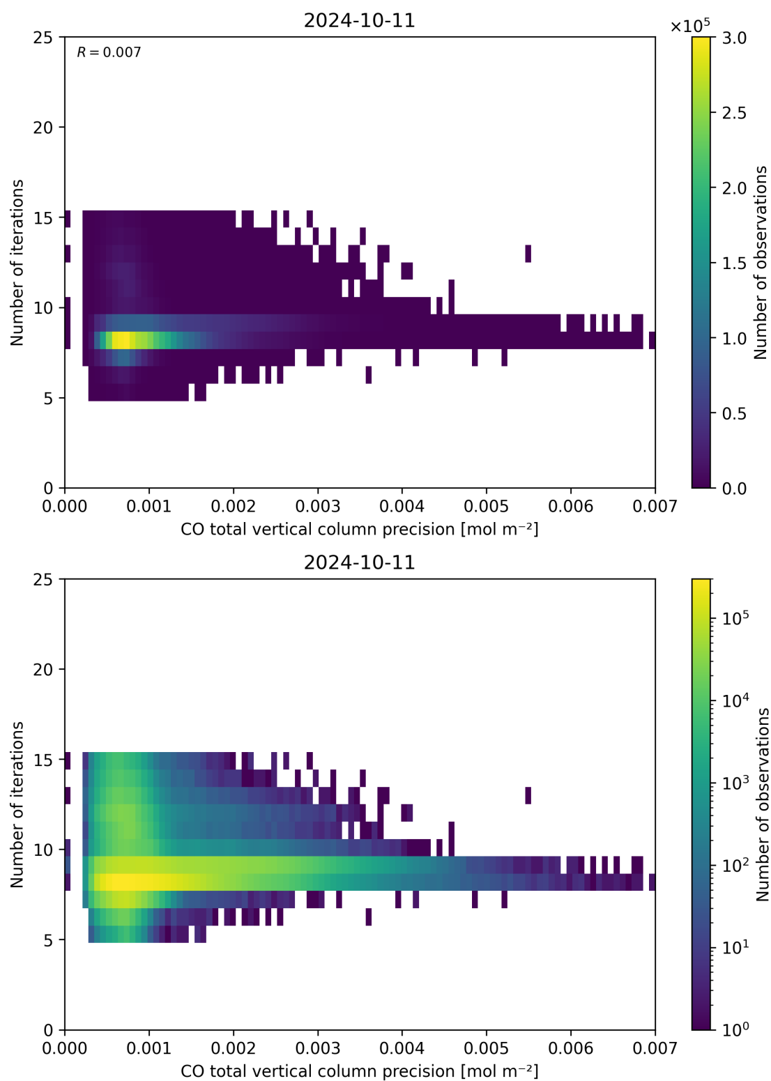
Figure 46: Scatter density plot of “CO total vertical column precision” against “Number of iterations” for 2024-10-10 to 2024-10-12.
