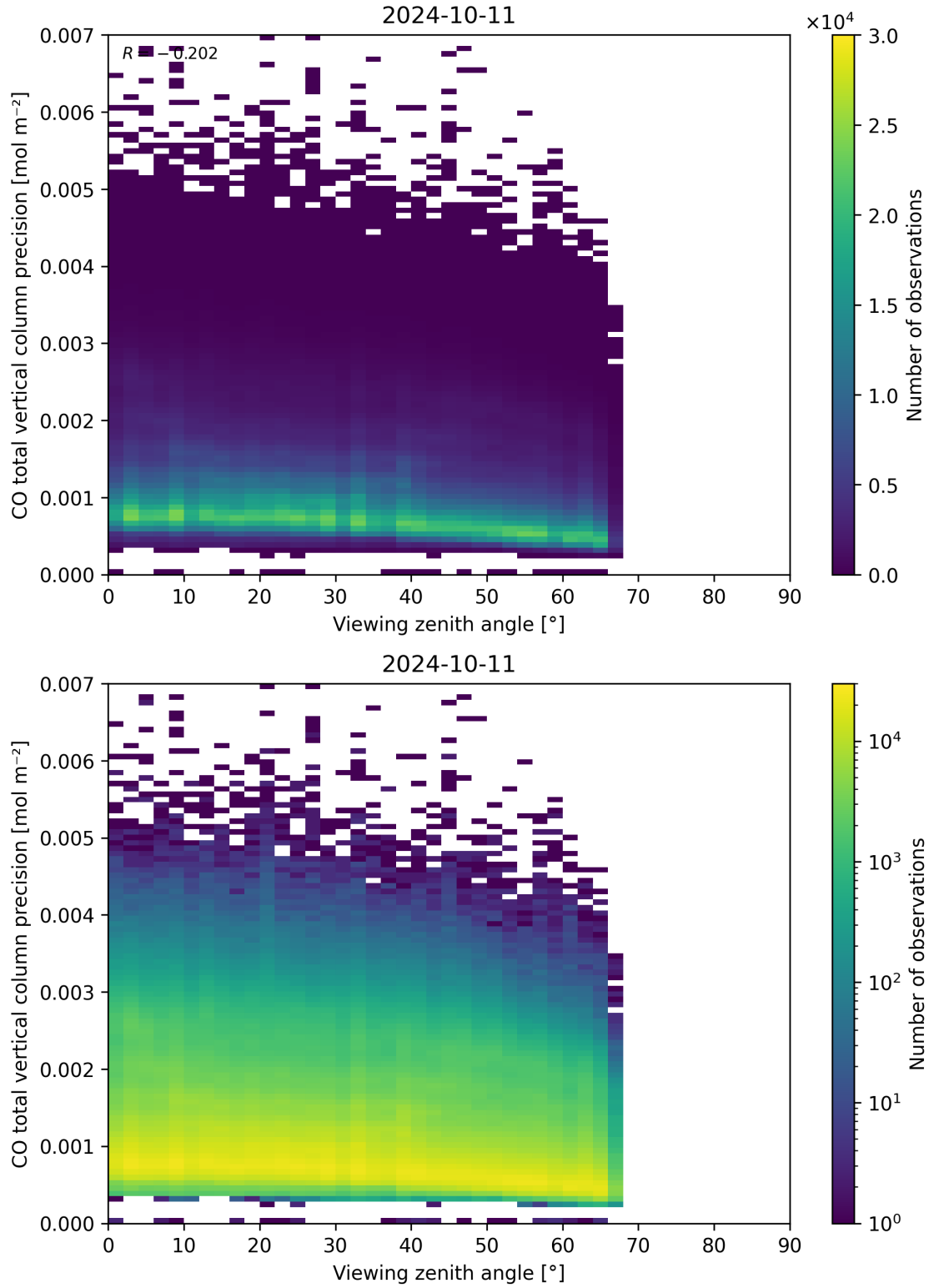
Figure 71: Scatter density plot of “Viewing zenith angle” against “CO total vertical column precision” for 2024-10-10 to 2024-10-12.
