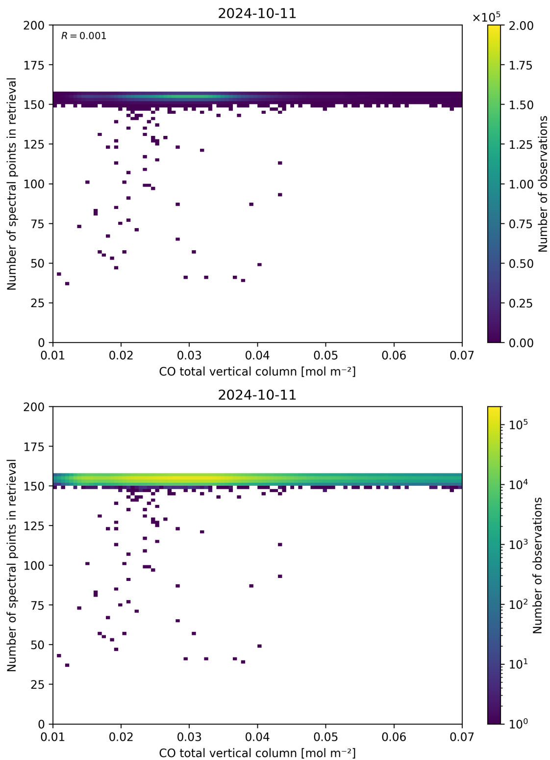
Figure 43: Scatter density plot of “CO total vertical column” against “Number of spectral points in retrieval” for 2024-10-10 to 2024-10-12.
