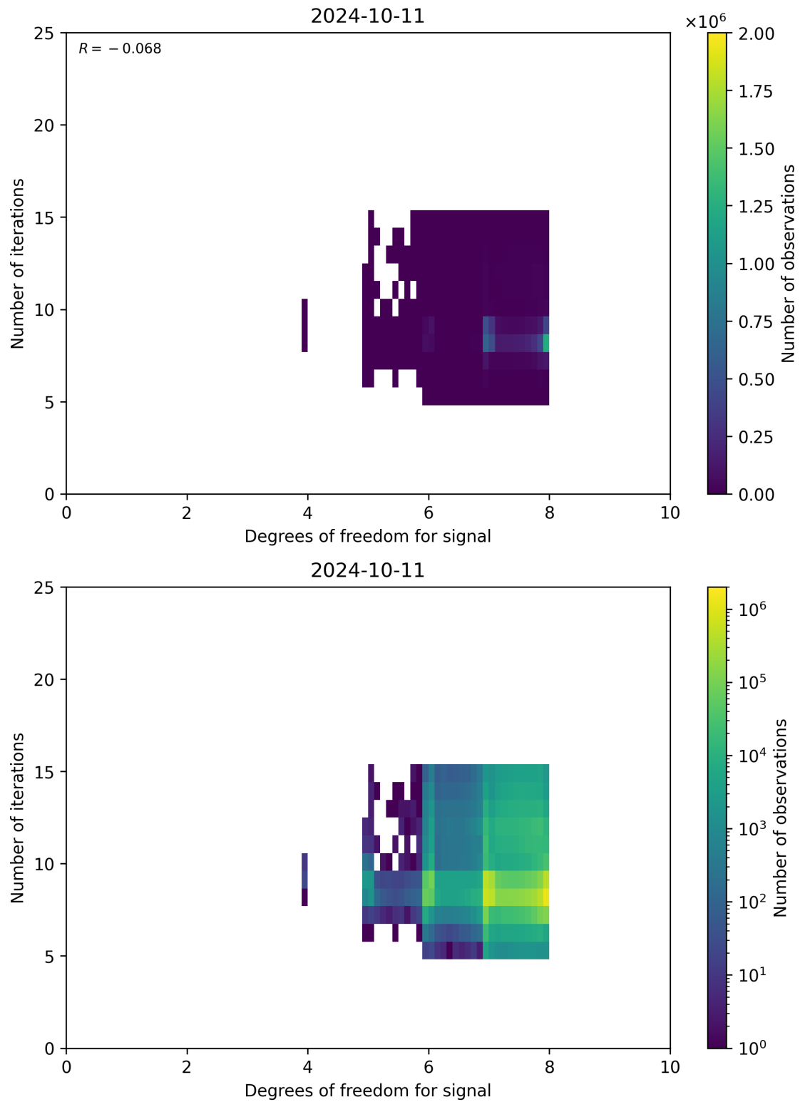
Figure 50: Scatter density plot of “Degrees of freedom for signal” against “Number of iterations” for 2024-10-10 to 2024-10-12.
