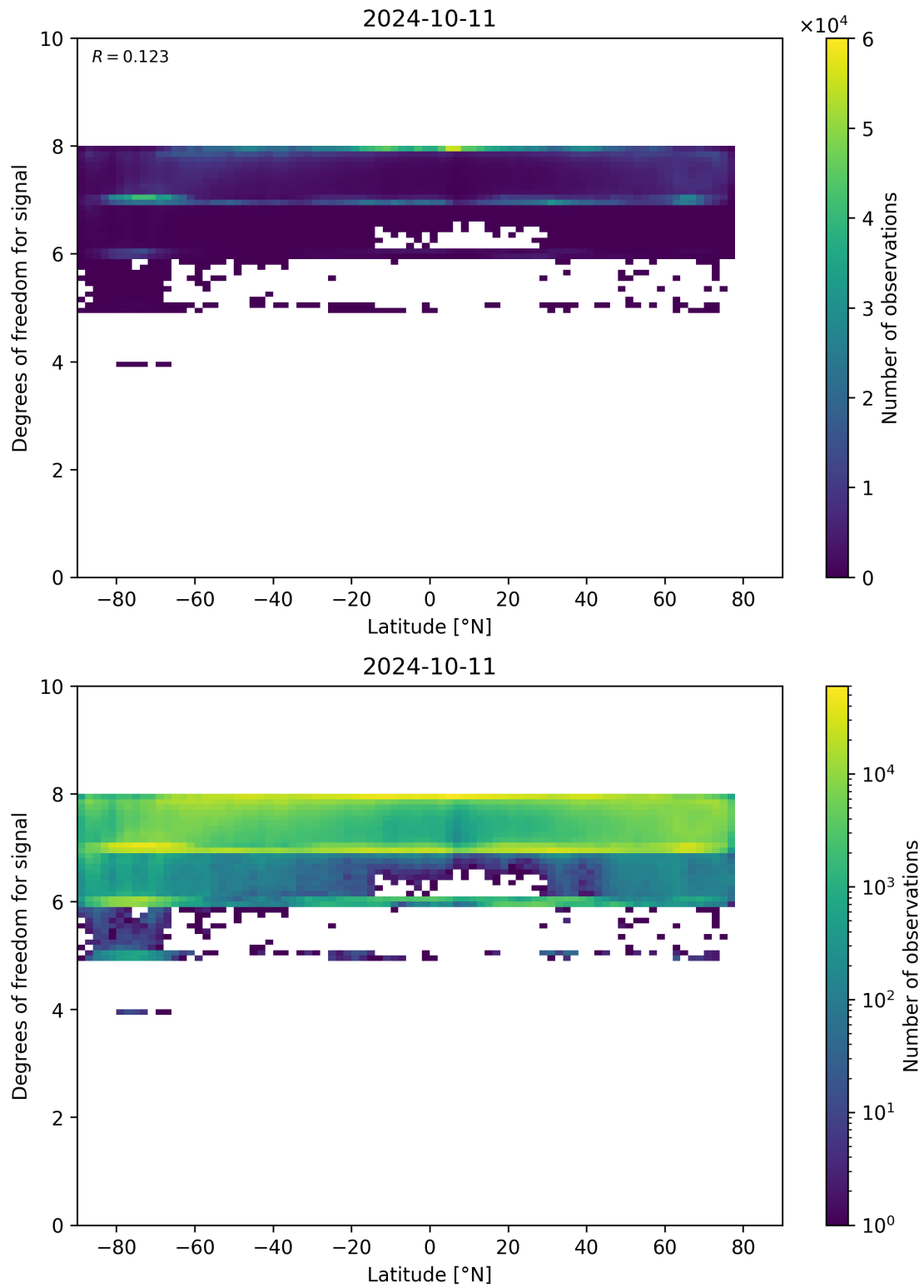
Figure 55: Scatter density plot of “Latitude” against “Degrees of freedom for signal” for 2024-10-10 to 2024-10-12.
