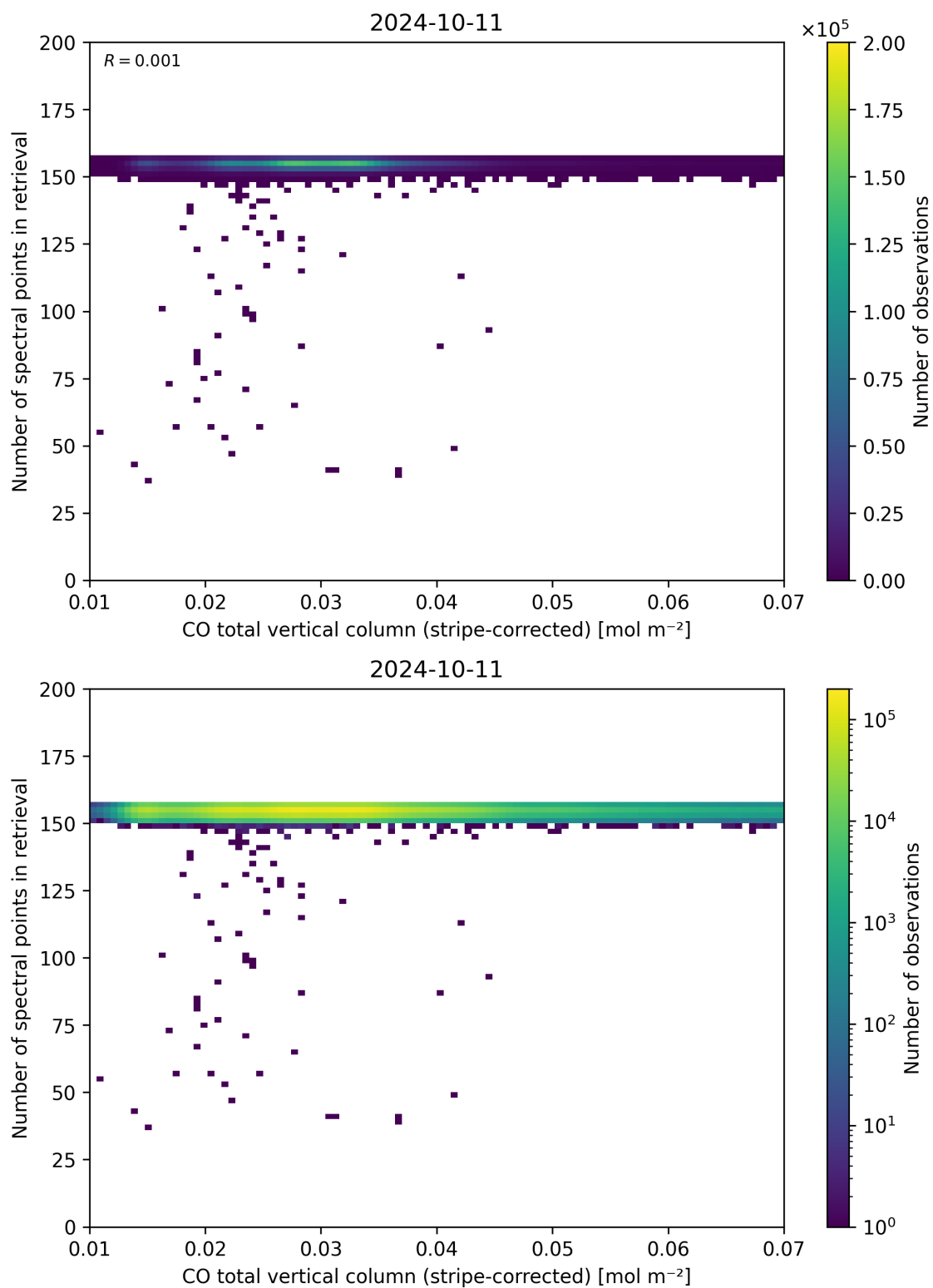
Figure 40: Scatter density plot of “CO total vertical column (stripe-corrected)” against “Number of spectral points in retrieval” for 2024-10-10 to 2024-10-12.
