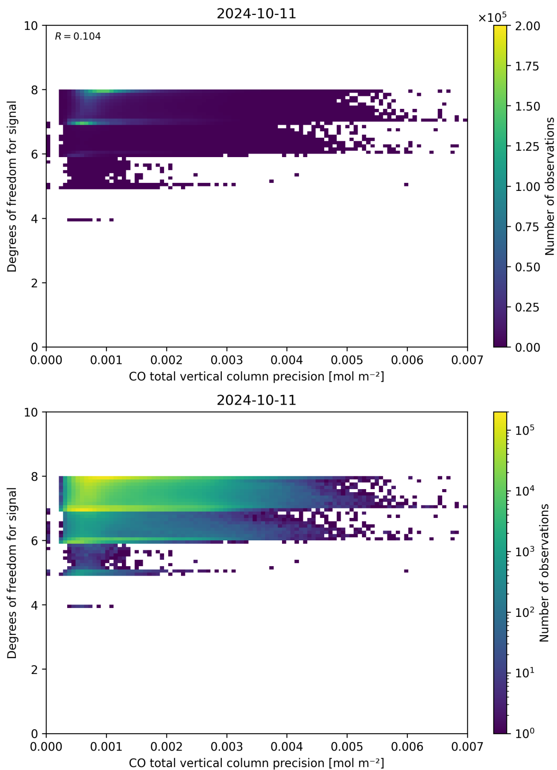
Figure 45: Scatter density plot of “CO total vertical column precision” against “Degrees of freedom for signal” for 2024-10-10 to 2024-10-12.
