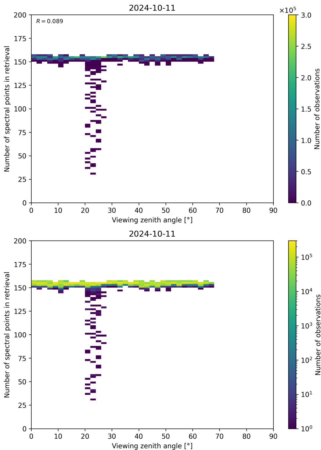
Figure 76: Scatter density plot of “Viewing zenith angle” against “Number of spectral points in retrieval” for 2024-10-10 to 2024-10-12.
