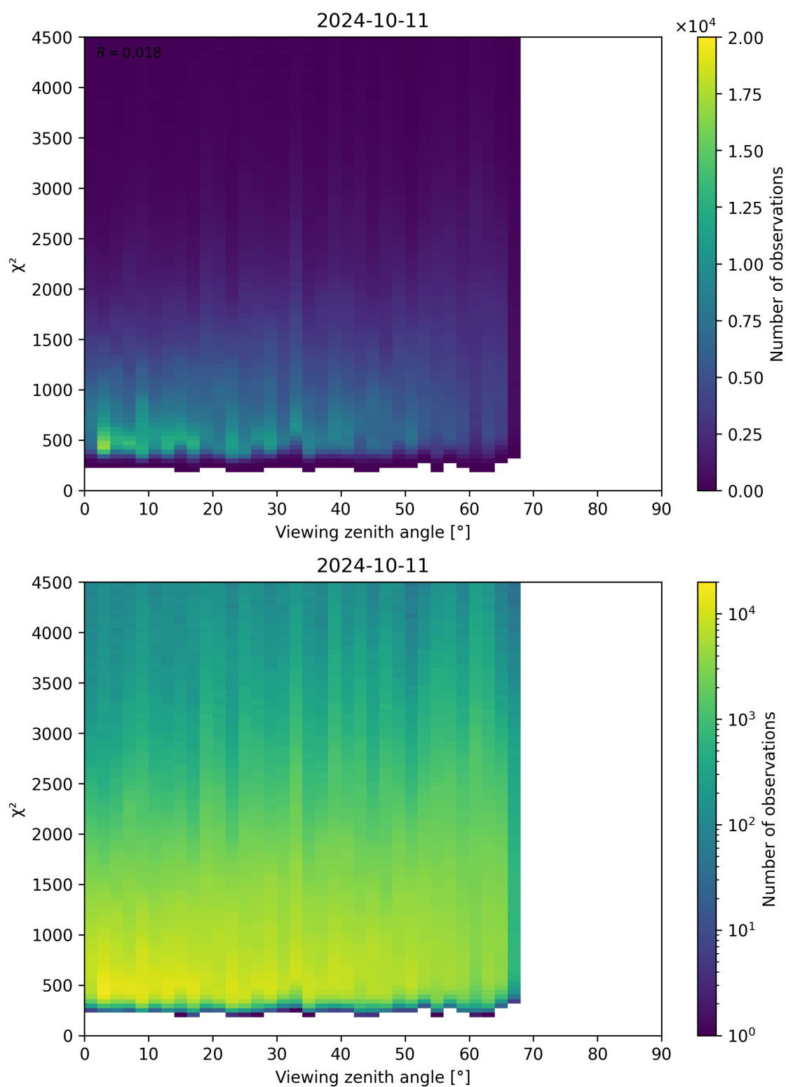
Figure 72: Scatter density plot of “Viewing zenith angle” against “ \chi^2 ” for 2024-10-10 to 2024-10-12.
