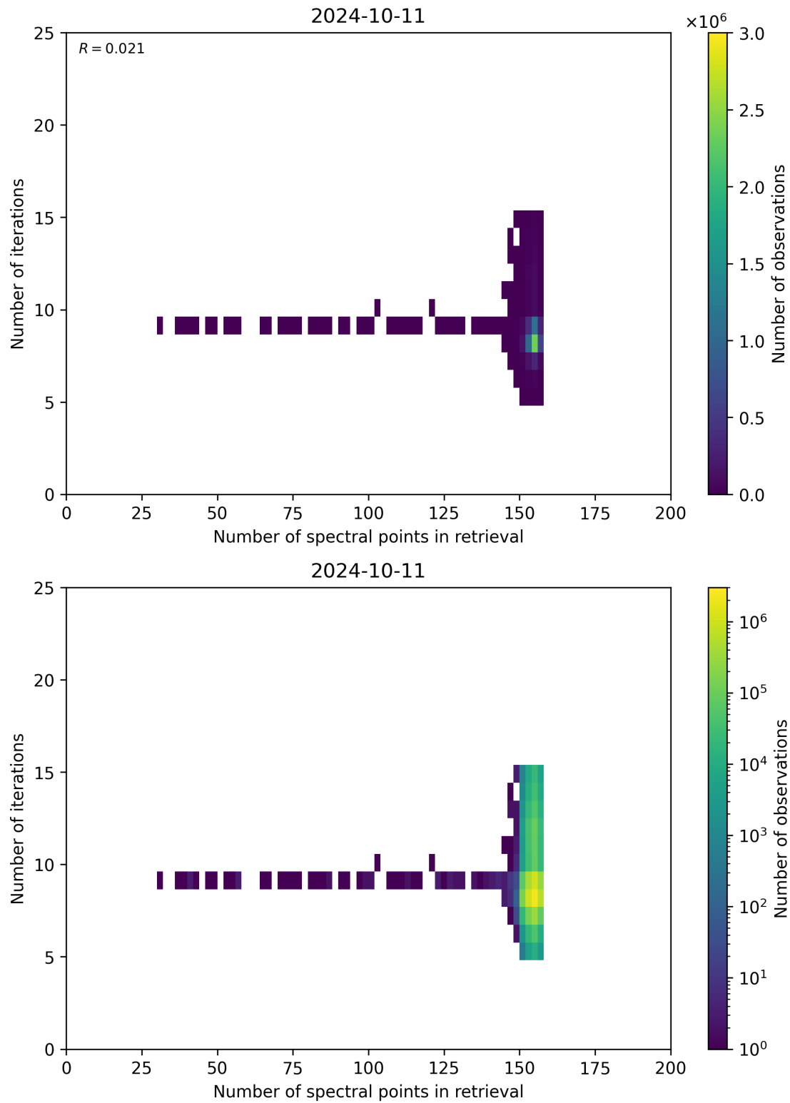
Figure 60: Scatter density plot of “Number of spectral points in retrieval” against “Number of iterations” for 2024-10-10 to 2024-10-12.
