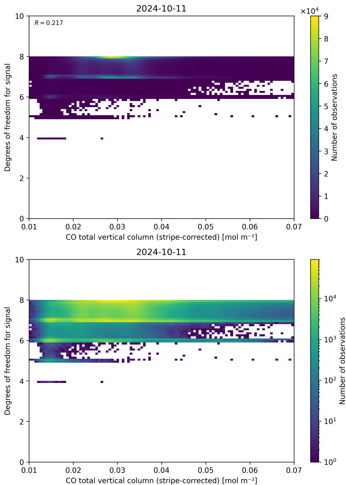
Figure 38: Scatter density plot of “CO total vertical column (stripe-corrected)” against “Degrees of freedom for signal” for 2024-10-10 to 2024-10-12.
