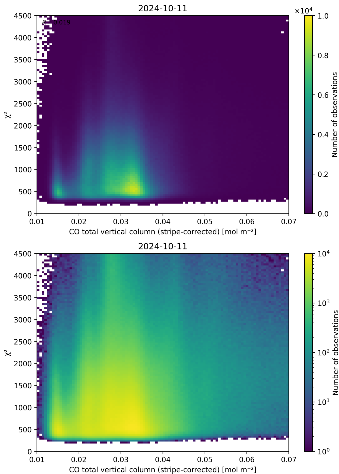
Figure 37: Scatter density plot of “CO total vertical column (stripe-corrected)” against “ \chi^2 ” for 2024-10-10 to 2024-10-12.
