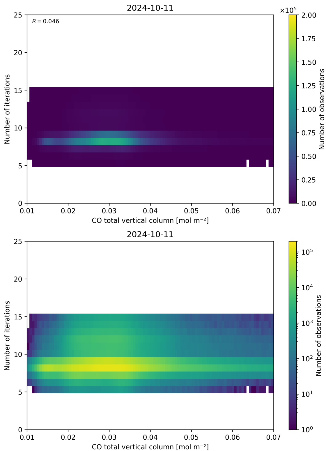
Figure 42: Scatter density plot of “CO total vertical column” against “Number of iterations” for 2024-10-10 to 2024-10-12.
