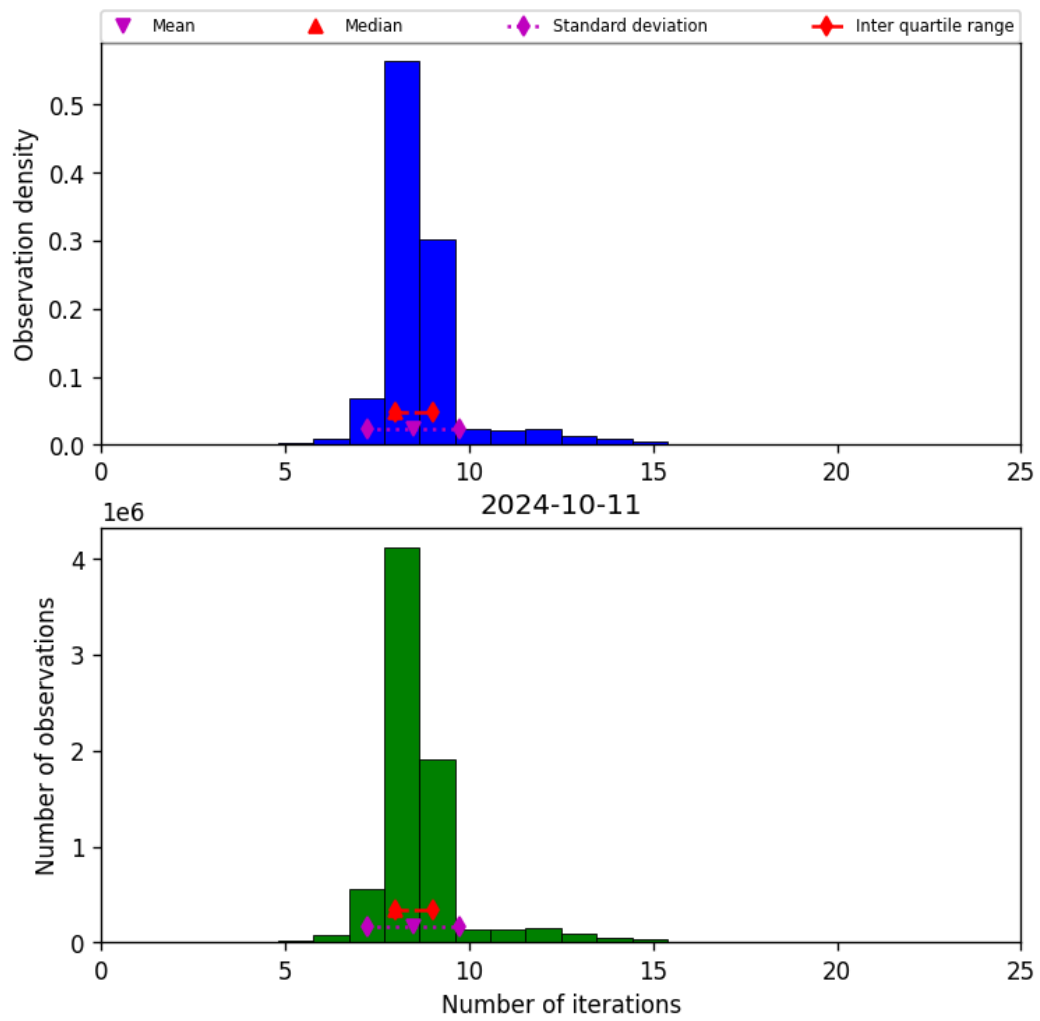
Figure 24: Histogram of “Number of iterations” for 2024-10-10 to 2024-10-12
