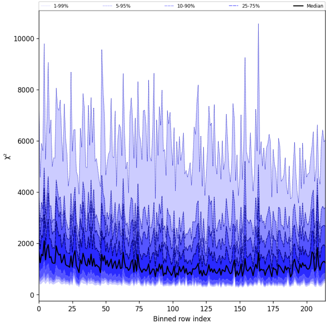
Figure 30: Along track statistics of “ \chi^2 ” for 2024-10-10 to 2024-10-12
