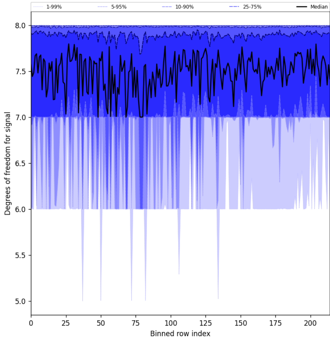
Figure 31: Along track statistics of “Degrees of freedom for signal” for 2024-10-10 to 2024-10-12
