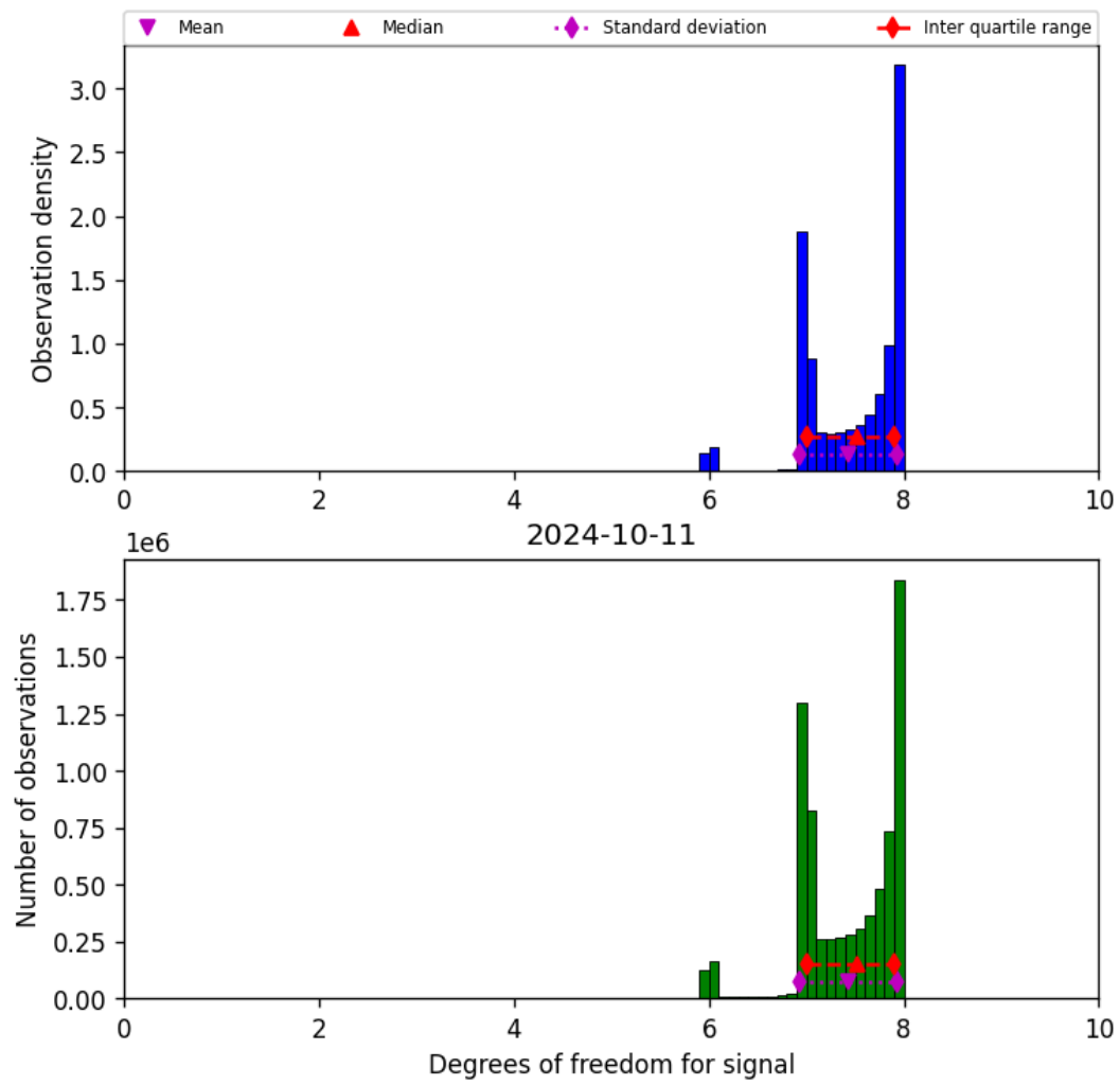
Figure 23: Histogram of “Degrees of freedom for signal” for 2024-10-10 to 2024-10-12
