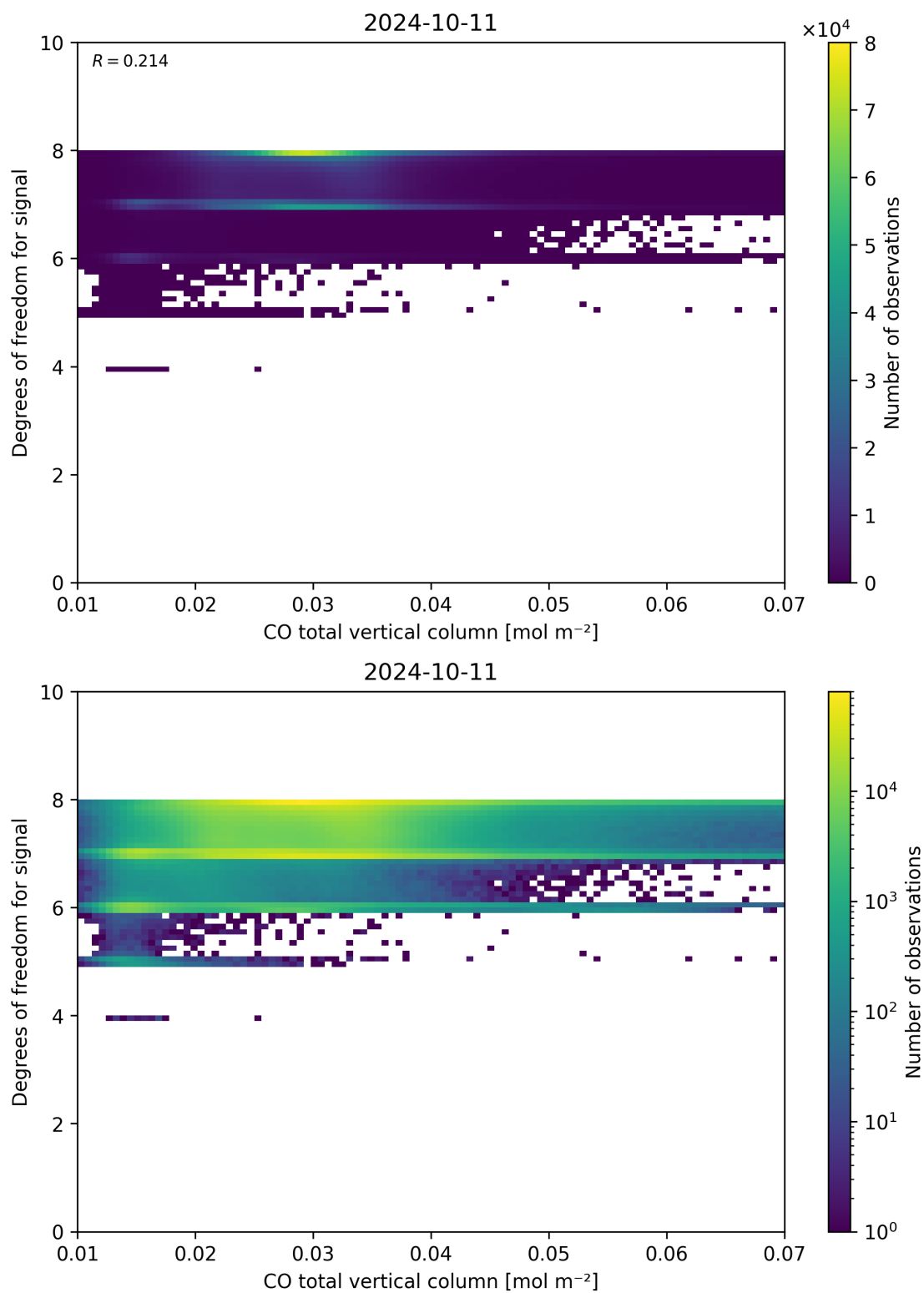
Figure 41: Scatter density plot of “CO total vertical column” against “Degrees of freedom for signal” for 2024-10-10 to 2024-10-12.
