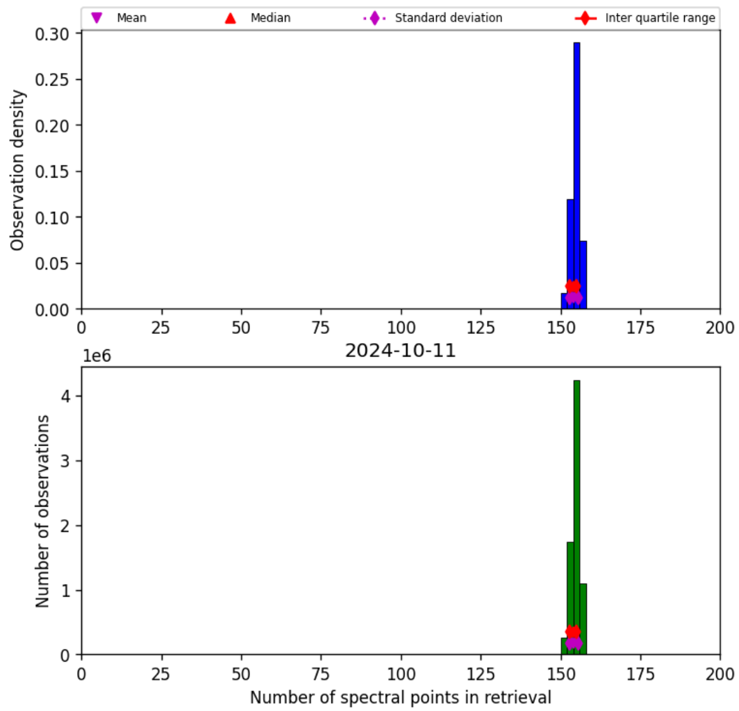
Figure 21: Histogram of “Number of spectral points in retrieval” for 2024-10-10 to 2024-10-12
