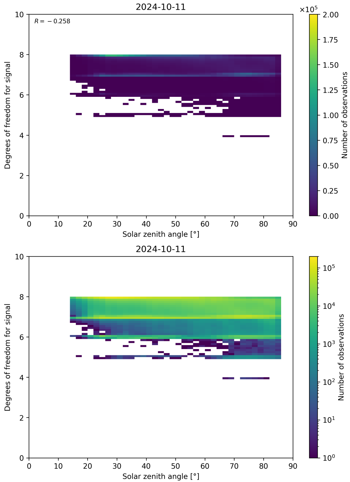
Figure 65: Scatter density plot of “Solar zenith angle” against “Degrees of freedom for signal” for 2024-10-10 to 2024-10-12.
