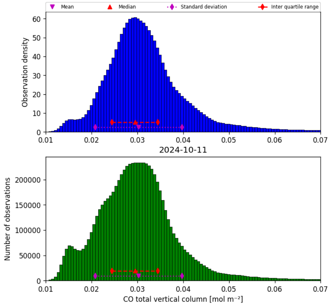
Figure 18: Histogram of “CO total vertical column” for 2024-10-10 to 2024-10-12
