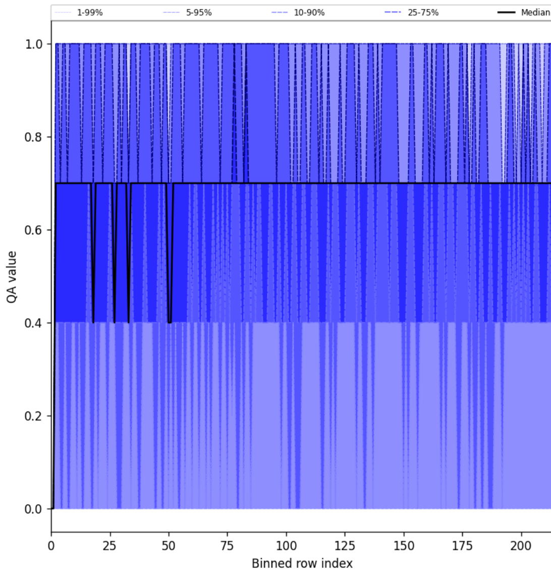
Figure 25: Along track statistics of “QA value” for 2024-10-10 to 2024-10-12
