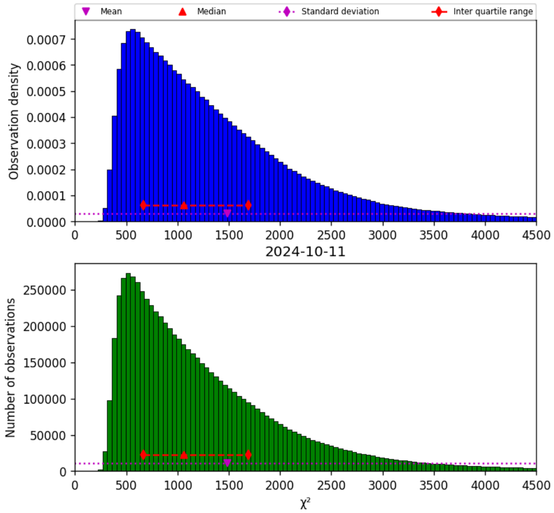
Figure 22: Histogram of “ \chi^2 ” for 2024-10-10 to 2024-10-12
