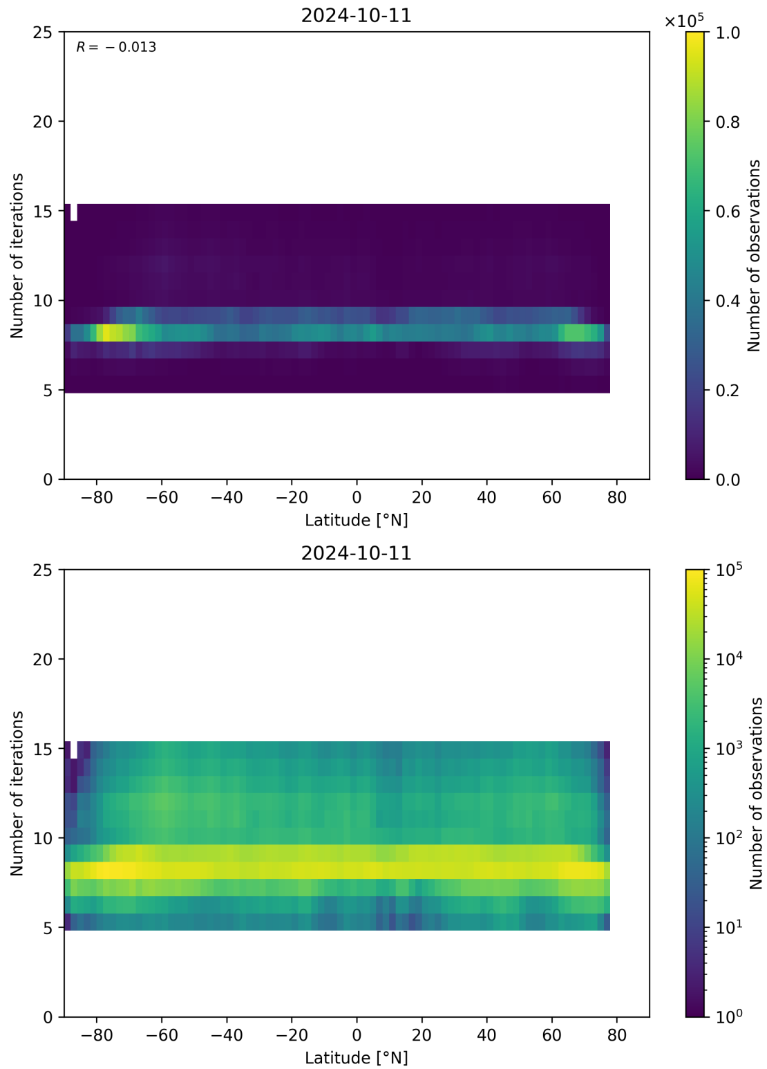
Figure 56: Scatter density plot of “Latitude” against “Number of iterations” for 2024-10-10 to 2024-10-12.
