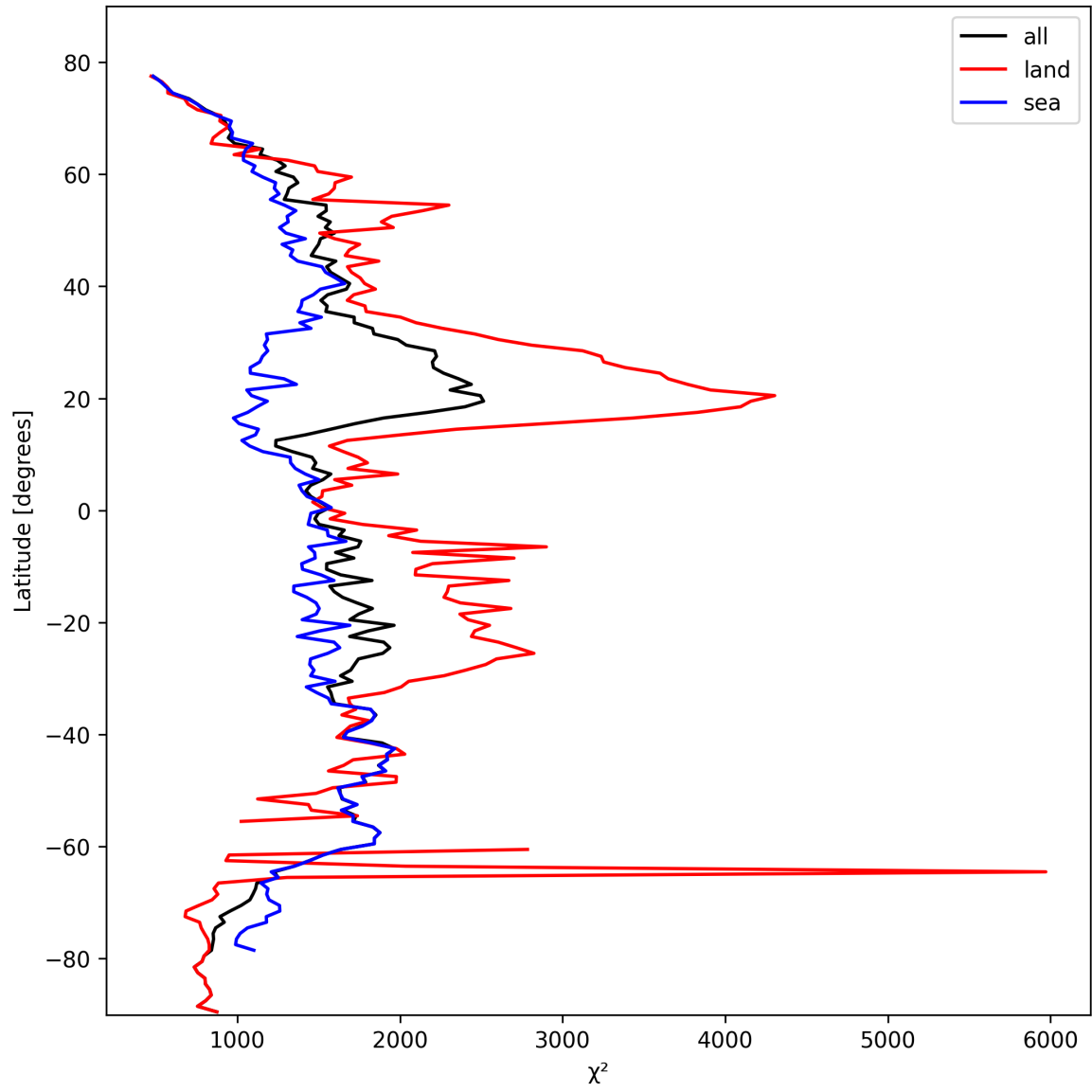
Figure 14: Zonal average of “ \chi^2 ” for 2024-10-10 to 2024-10-12.
