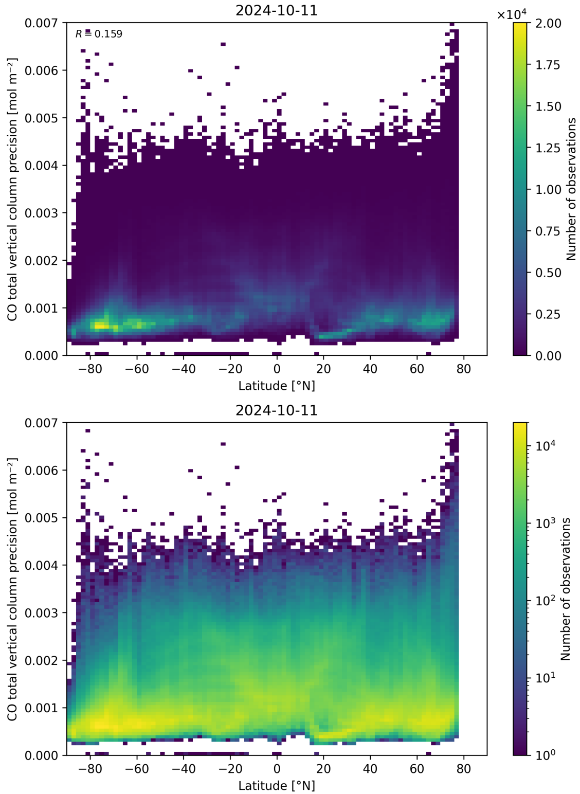
Figure 53: Scatter density plot of “Latitude” against “CO total vertical column precision” for 2024-10-10 to 2024-10-12.
