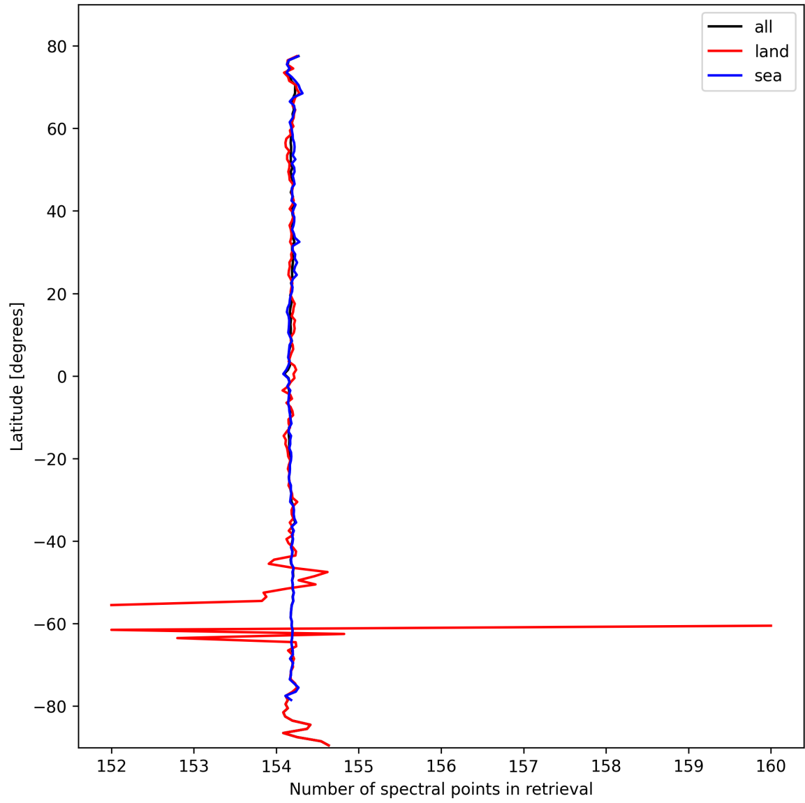
Figure 13: Zonal average of “Number of spectral points in retrieval” for 2024-10-10 to 2024-10-12.
