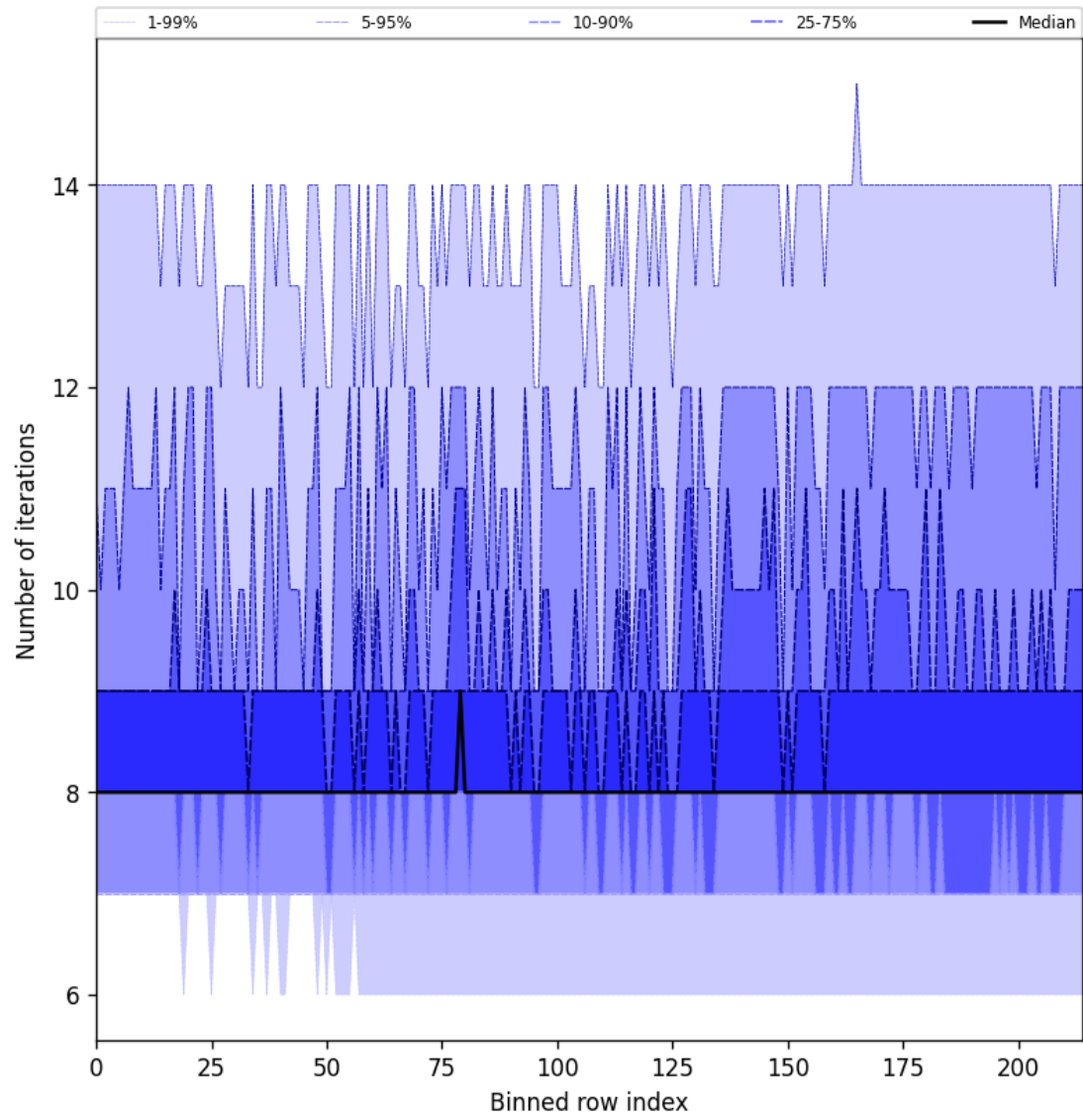
Figure 32: Along track statistics of “Number of iterations” for 2024-10-10 to 2024-10-12
