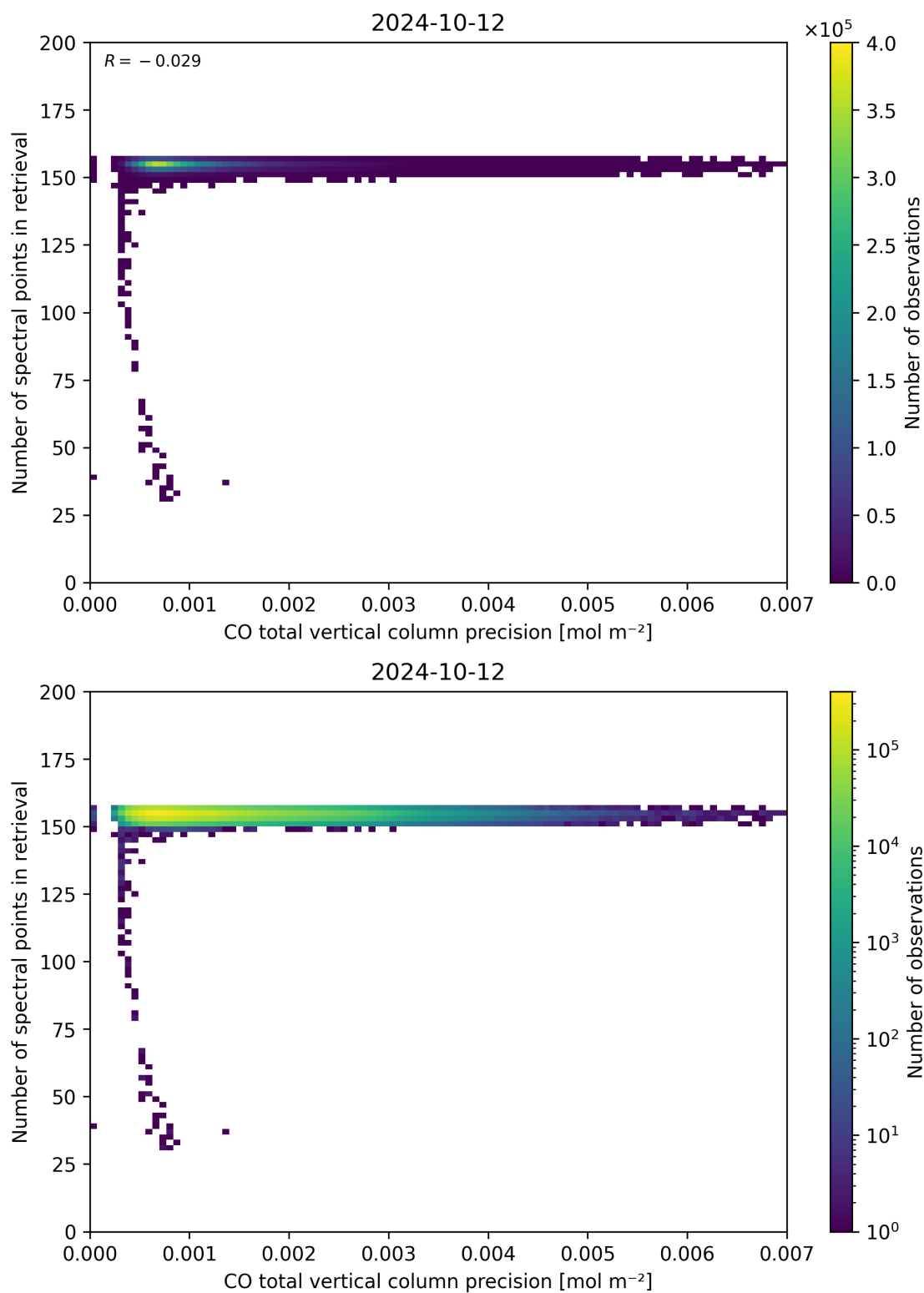
Figure 47: Scatter density plot of “CO total vertical column precision” against “Number of spectral points in retrieval” for 2024-10-11 to 2024-10-13.
