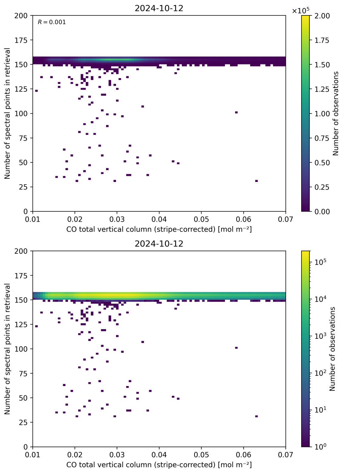
Figure 40: Scatter density plot of “CO total vertical column (stripe-corrected)” against “Number of spectral points in retrieval” for 2024-10-11 to 2024-10-13.
