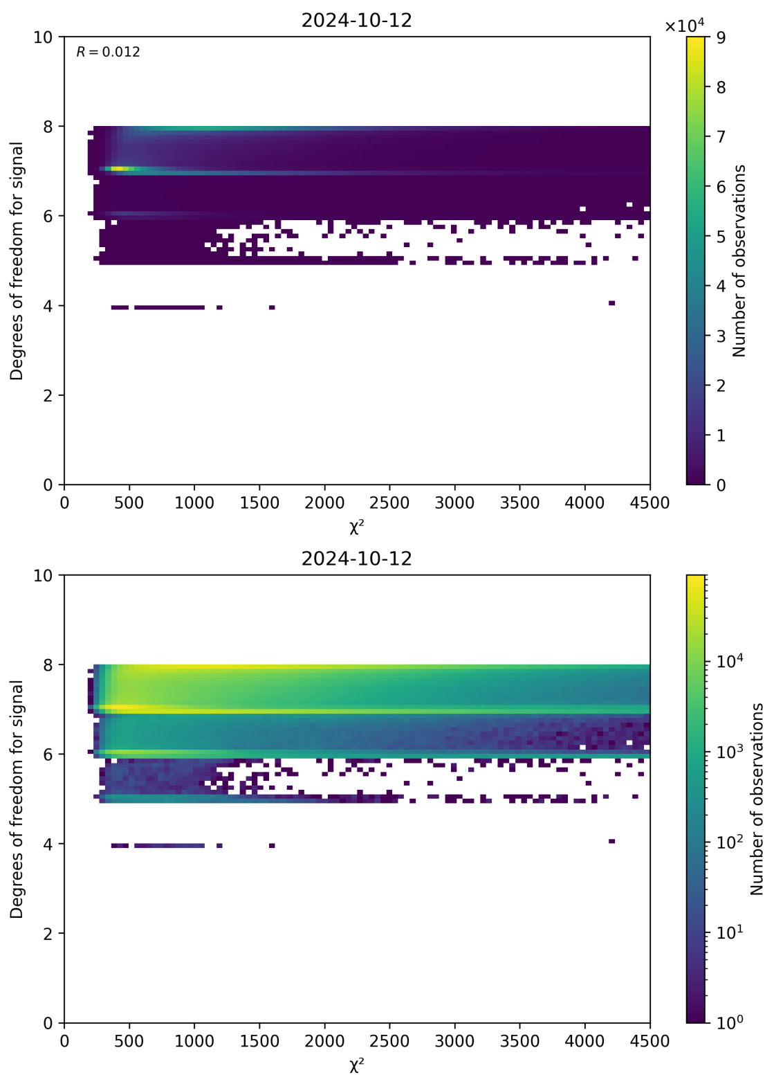
Figure 48: Scatter density plot of “ \chi^2 ” against “Degrees of freedom for signal” for 2024-10-11 to 2024-10-13.
