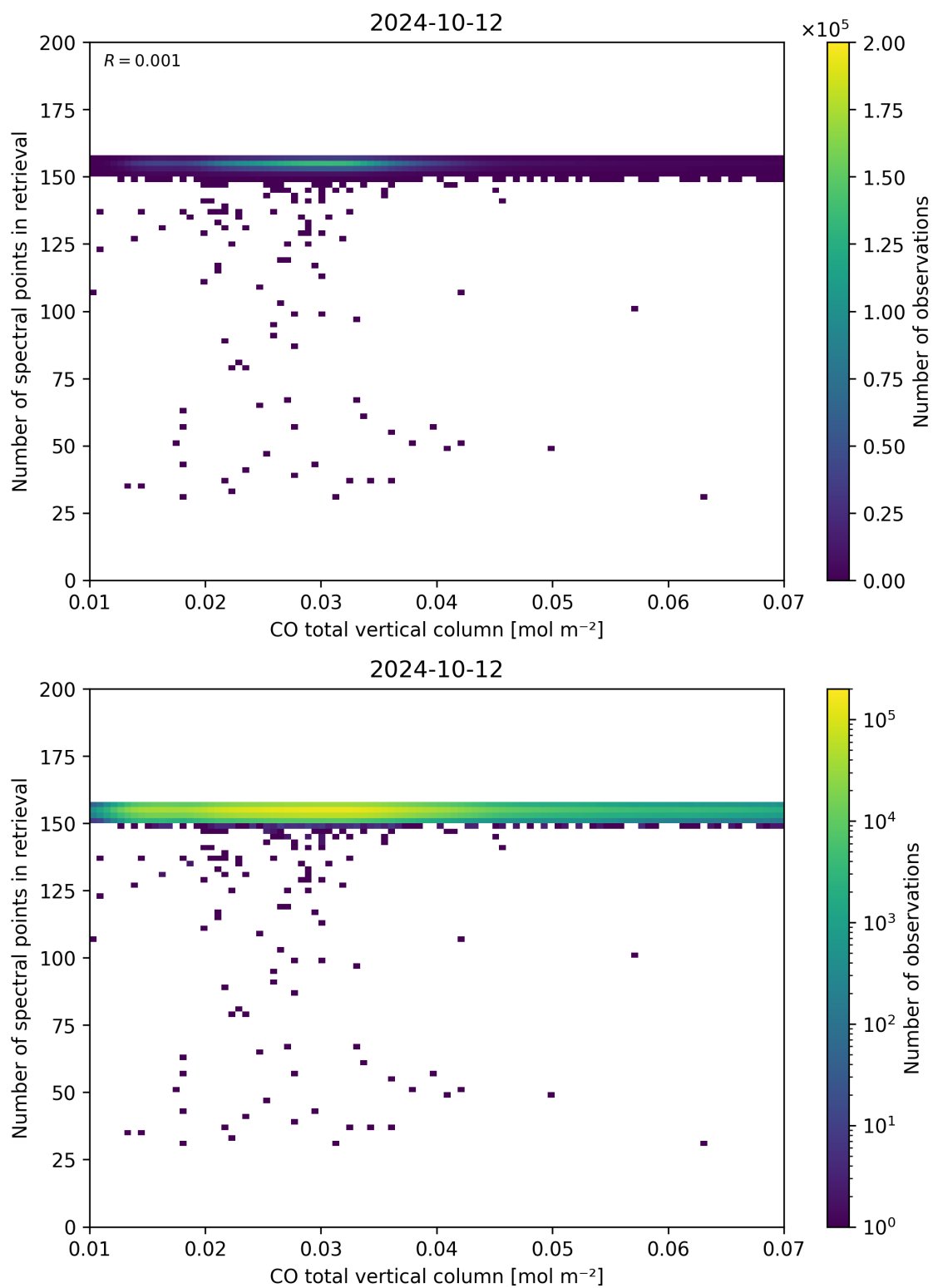
Figure 43: Scatter density plot of “CO total vertical column” against “Number of spectral points in retrieval” for 2024-10-11 to 2024-10-13.
