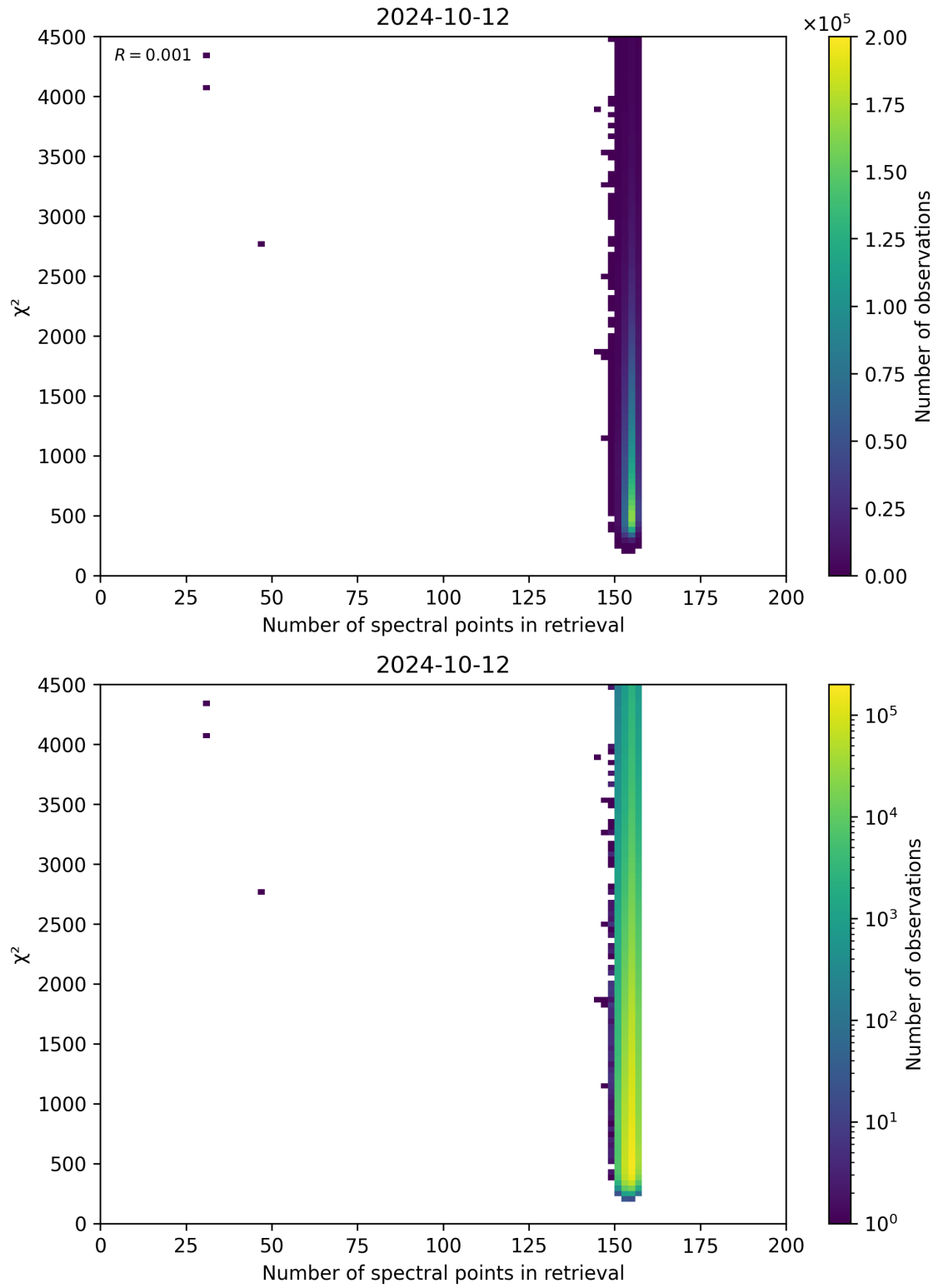
Figure 58: Scatter density plot of “Number of spectral points in retrieval” against “ \chi^2 ” for 2024-10-11 to 2024-10-13.
