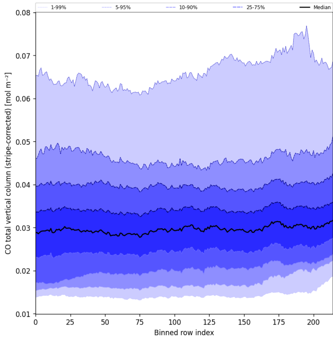
Figure 27: Along track statistics of “CO total vertical column (stripe-corrected)” for 2024-10-11 to 2024-10-13
