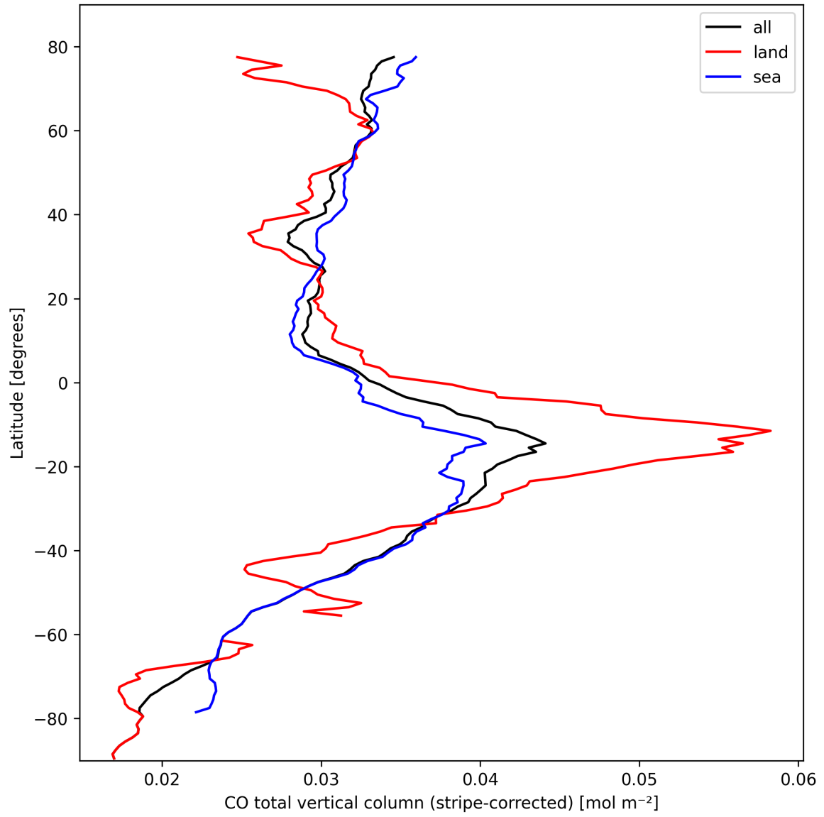
Figure 11: Zonal average of “CO total vertical column (stripe-corrected)” for 2024-10-11 to 2024-10-13.
