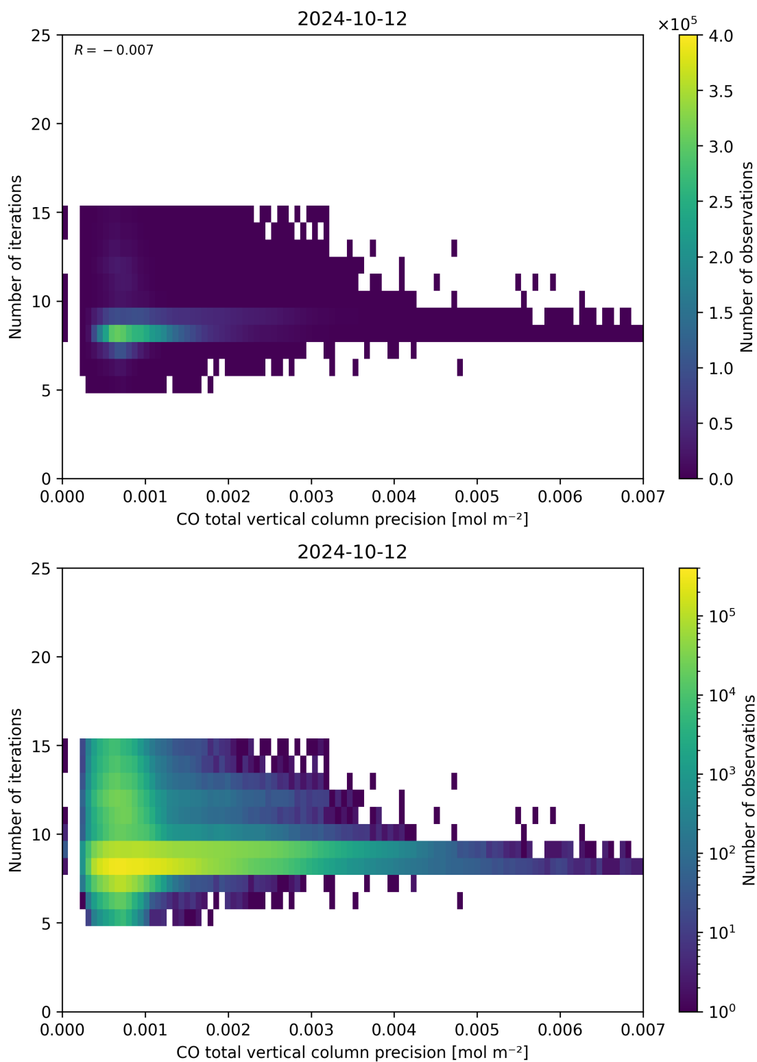
Figure 46: Scatter density plot of “CO total vertical column precision” against “Number of iterations” for 2024-10-11 to 2024-10-13.
