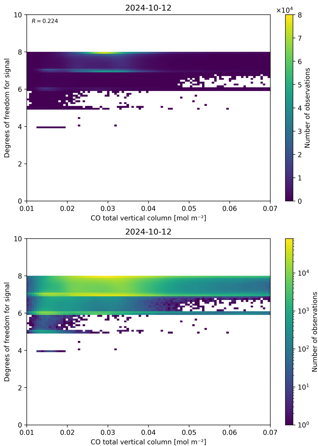
Figure 41: Scatter density plot of “CO total vertical column” against “Degrees of freedom for signal” for 2024-10-11 to 2024-10-13.
