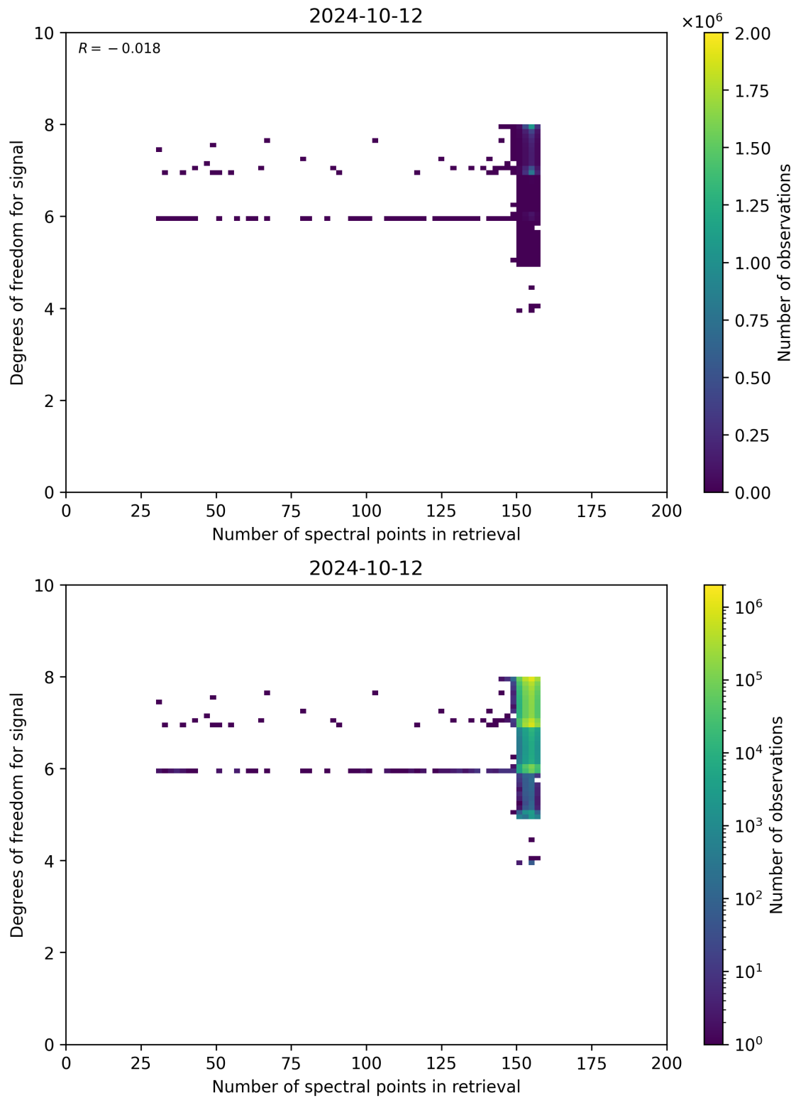
Figure 59: Scatter density plot of “Number of spectral points in retrieval” against “Degrees of freedom for signal” for 2024-10-11 to 2024-10-13.
