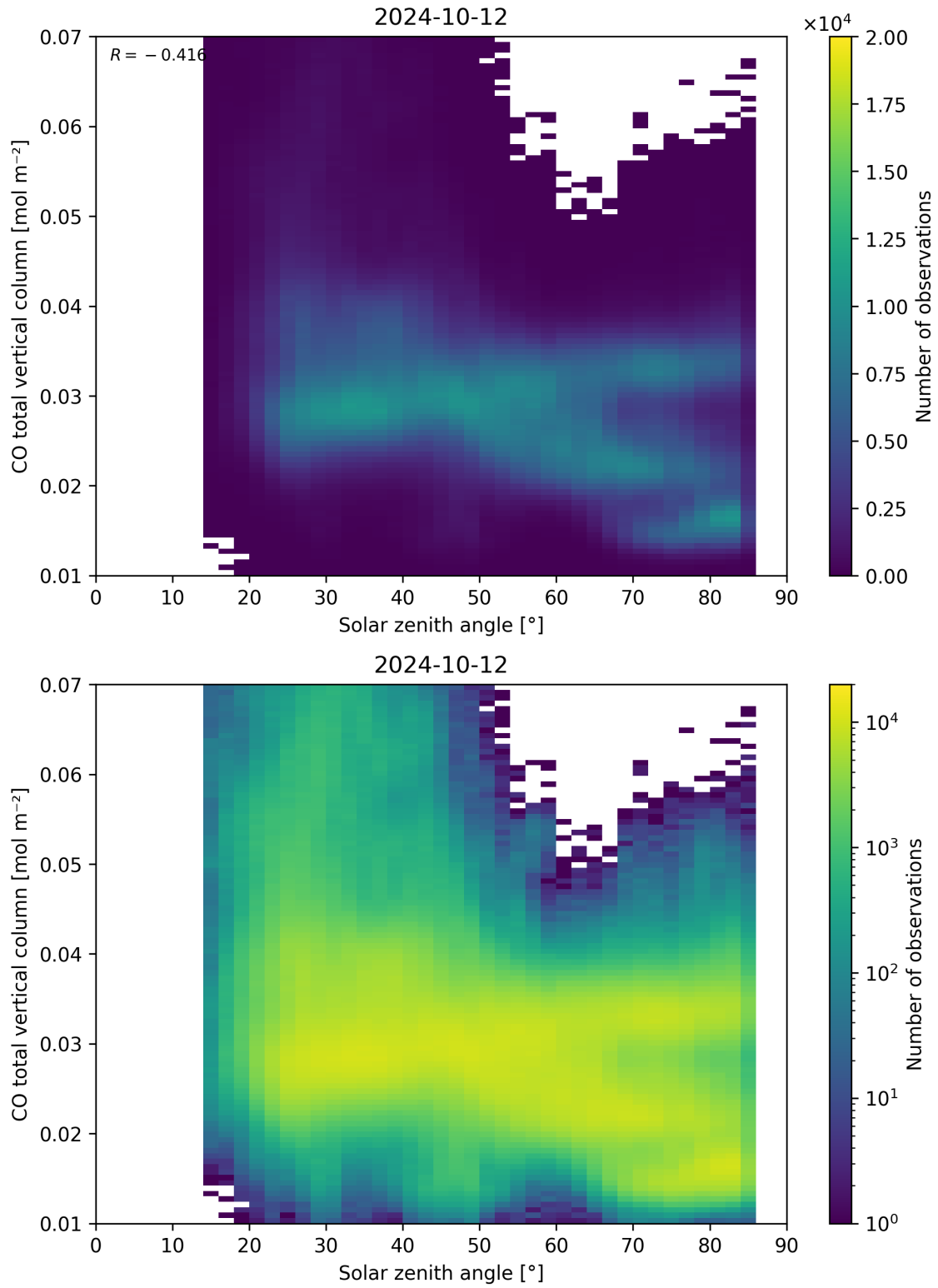
Figure 61: Scatter density plot of “Solar zenith angle” against “CO total vertical column” for 2024-10-11 to 2024-10-13.
