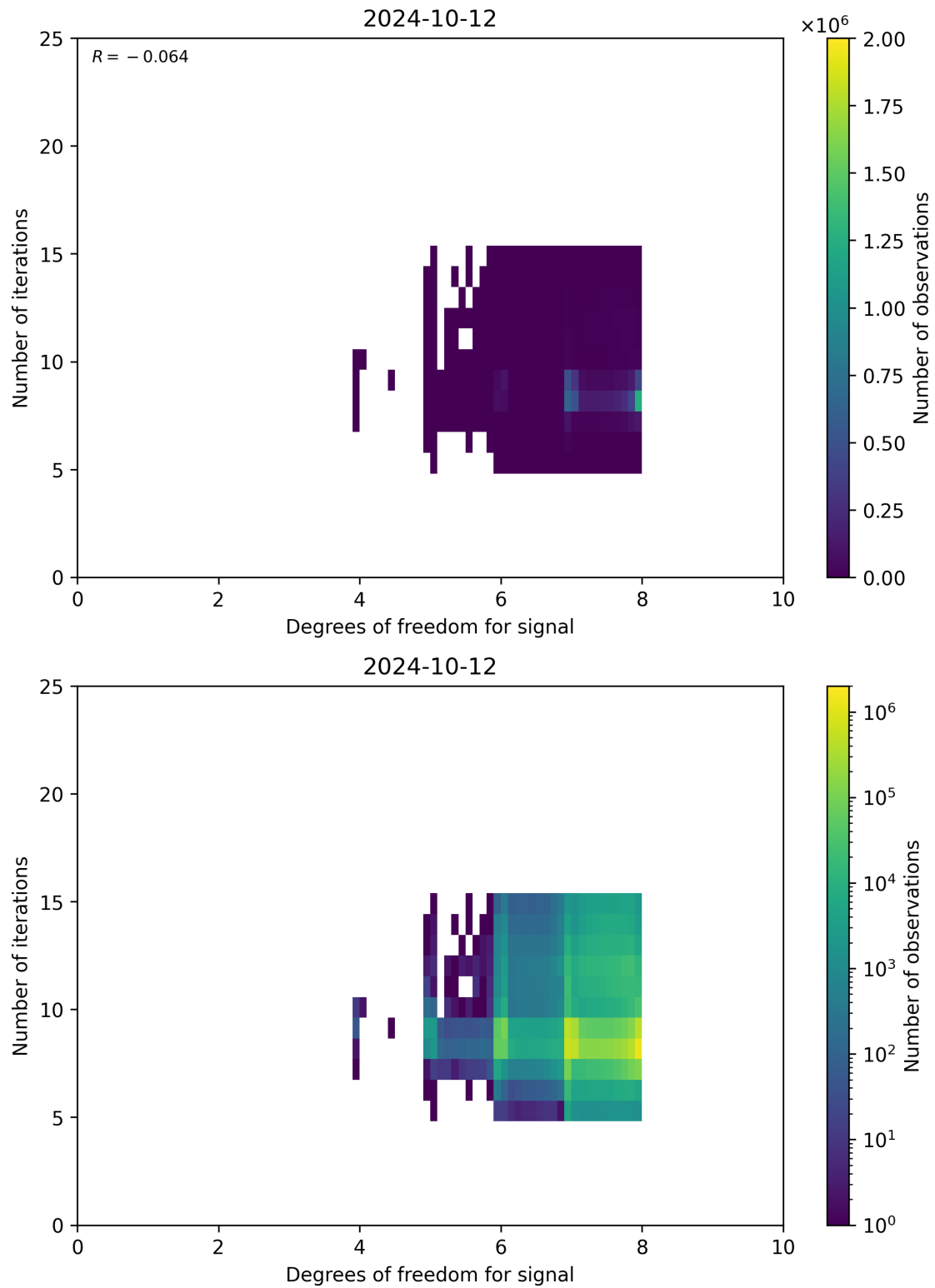
Figure 50: Scatter density plot of “Degrees of freedom for signal” against “Number of iterations” for 2024-10-11 to 2024-10-13.
