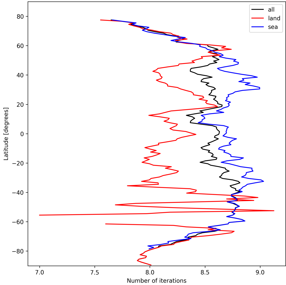
Figure 16: Zonal average of “Number of iterations” for 2024-10-11 to 2024-10-13.
