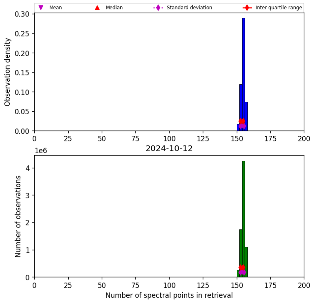
Figure 21: Histogram of “Number of spectral points in retrieval” for 2024-10-11 to 2024-10-13
