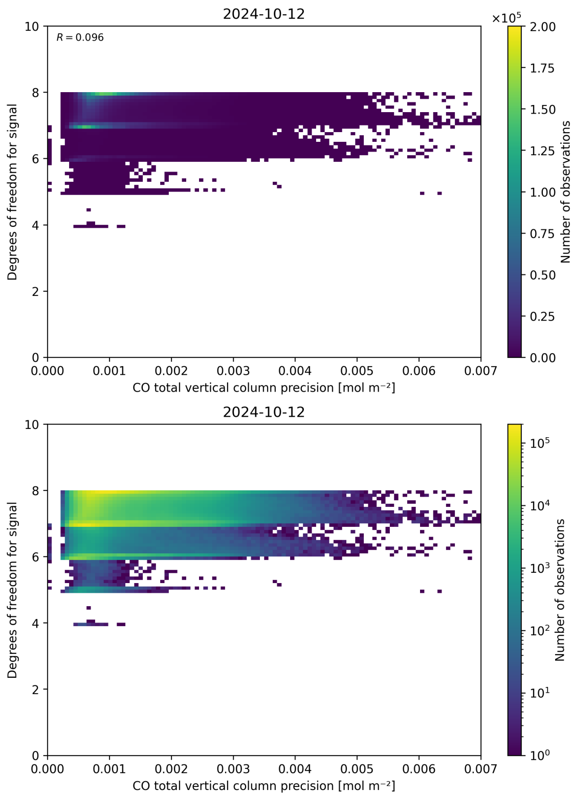
Figure 45: Scatter density plot of “CO total vertical column precision” against “Degrees of freedom for signal” for 2024-10-11 to 2024-10-13.
