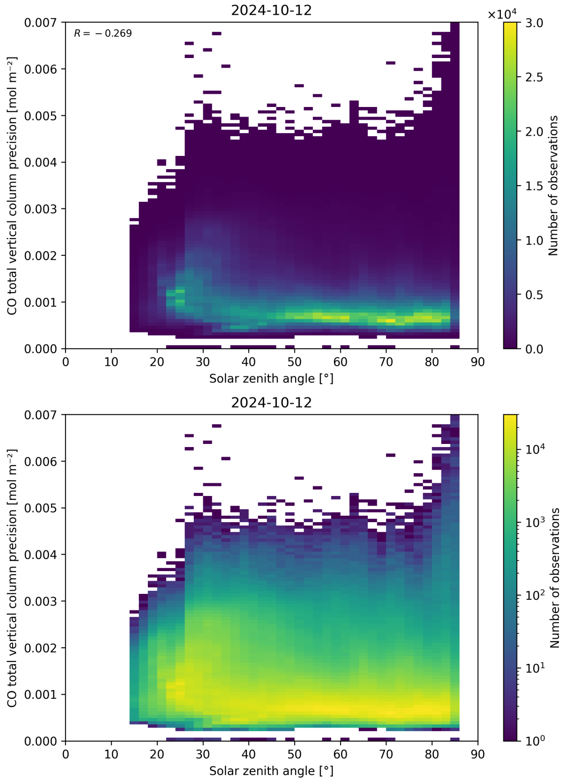
Figure 63: Scatter density plot of “Solar zenith angle” against “CO total vertical column precision” for 2024-10-11 to 2024-10-13.
