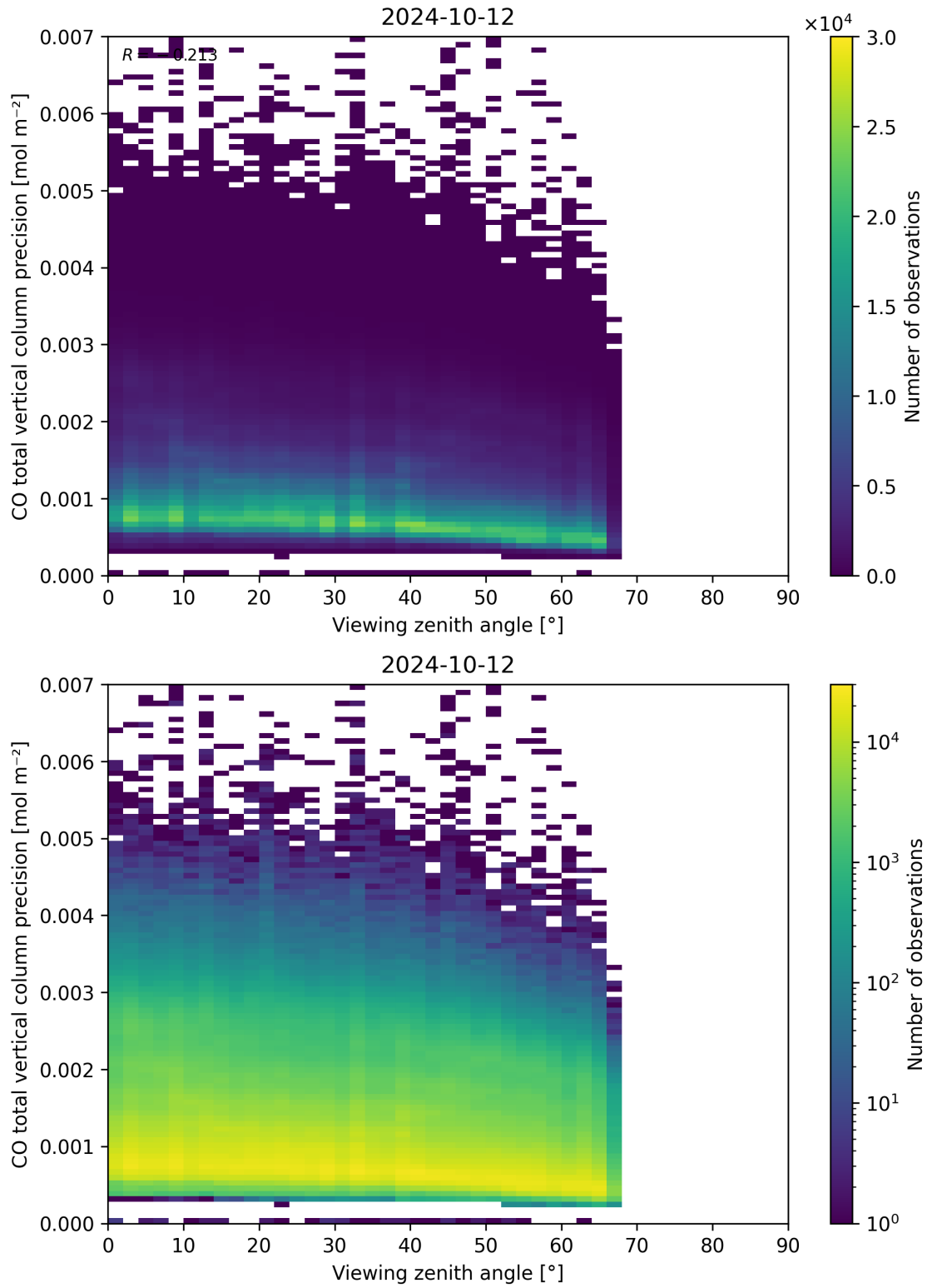
Figure 71: Scatter density plot of “Viewing zenith angle” against “CO total vertical column precision” for 2024-10-11 to 2024-10-13.
