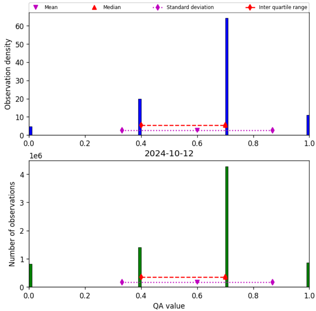
Figure 17: Histogram of “QA value” for 2024-10-11 to 2024-10-13
