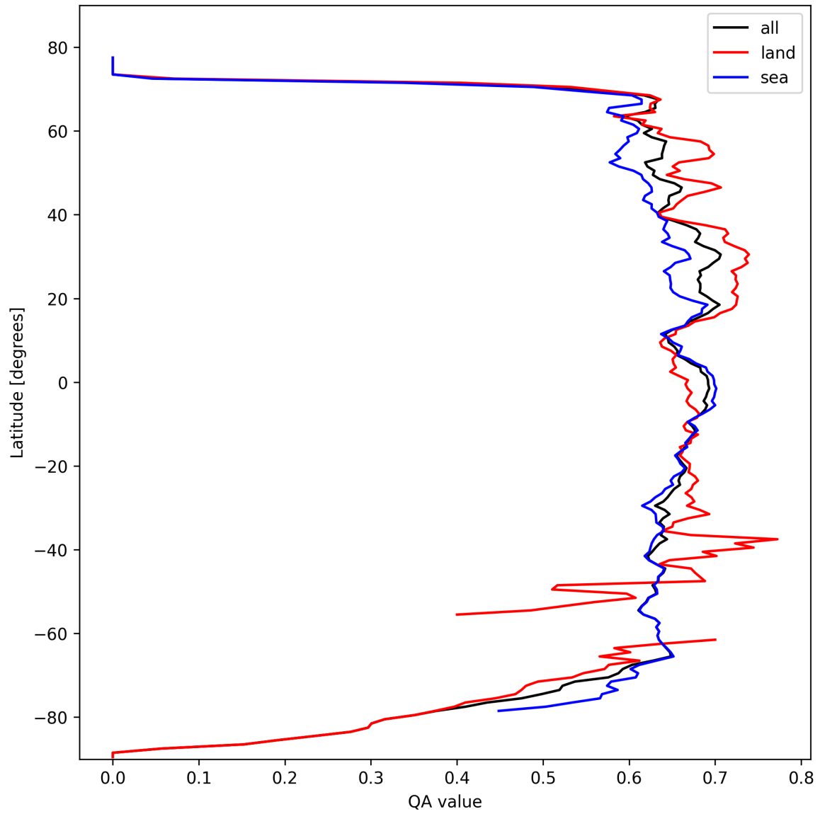
Figure 9: Zonal average of “QA value” for 2024-10-11 to 2024-10-13.
