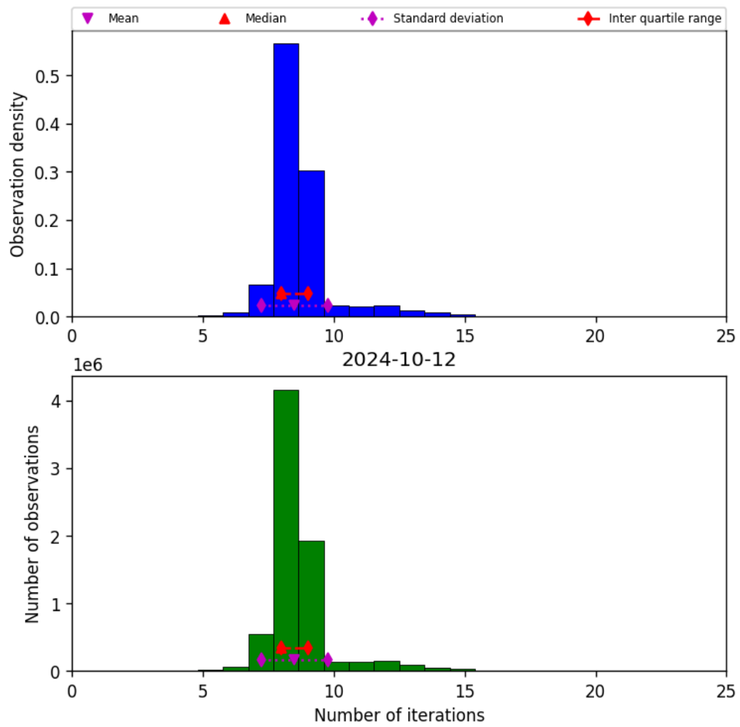
Figure 24: Histogram of “Number of iterations” for 2024-10-11 to 2024-10-13
