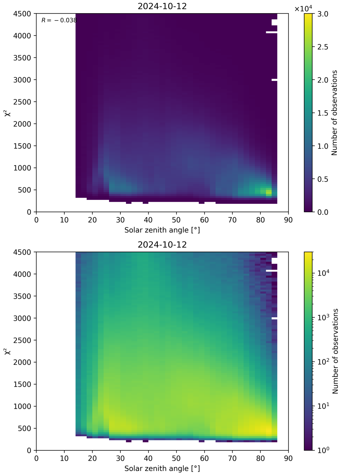
Figure 64: Scatter density plot of “Solar zenith angle” against “ \chi^2 ” for 2024-10-11 to 2024-10-13.
