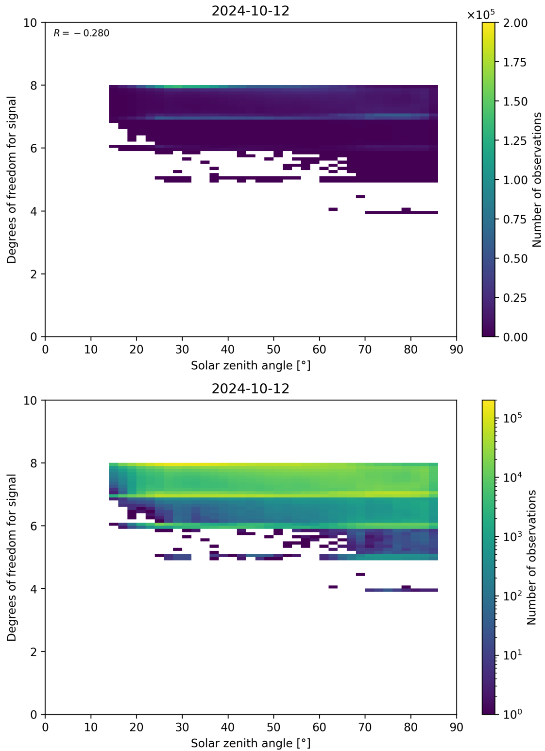
Figure 65: Scatter density plot of “Solar zenith angle” against “Degrees of freedom for signal” for 2024-10-11 to 2024-10-13.
