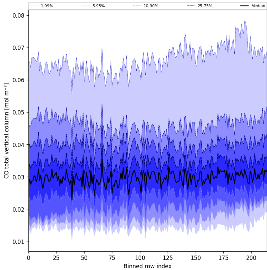
Figure 26: Along track statistics of “CO total vertical column” for 2024-10-11 to 2024-10-13
