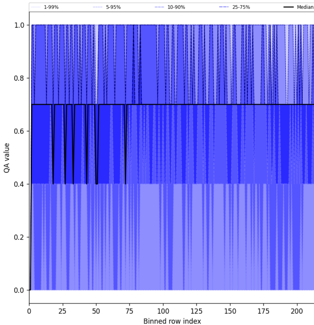
Figure 25: Along track statistics of “QA value” for 2024-10-11 to 2024-10-13
