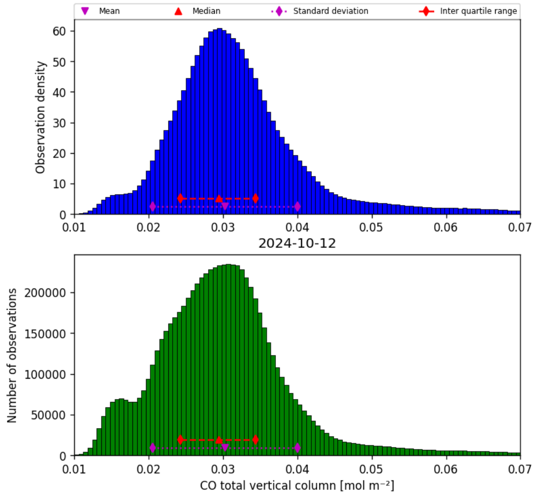
Figure 18: Histogram of “CO total vertical column” for 2024-10-11 to 2024-10-13
