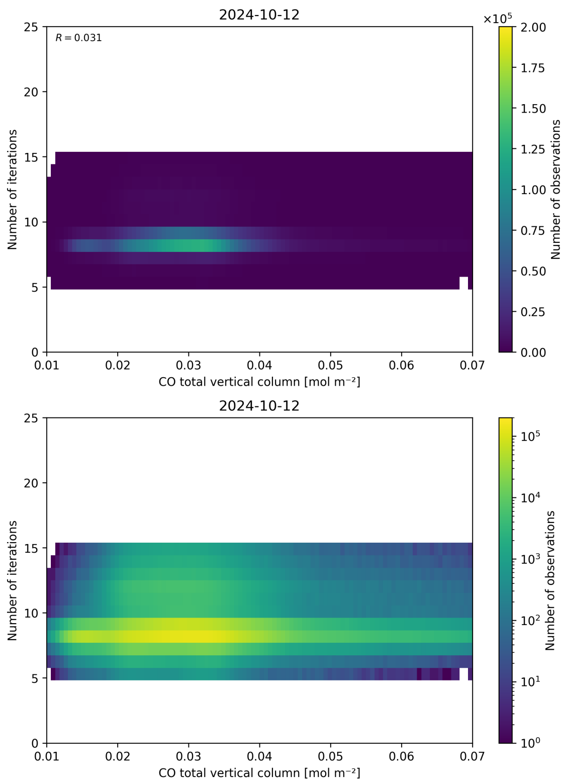
Figure 42: Scatter density plot of “CO total vertical column” against “Number of iterations” for 2024-10-11 to 2024-10-13.
