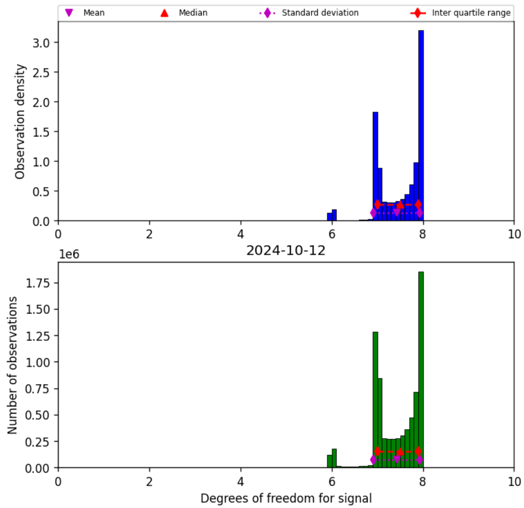
Figure 23: Histogram of “Degrees of freedom for signal” for 2024-10-11 to 2024-10-13
