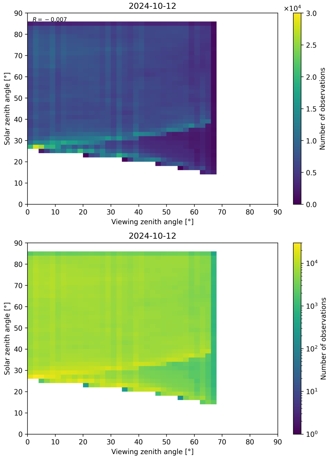
Figure 77: Scatter density plot of “Viewing zenith angle” against “Solar zenith angle” for 2024-10-11 to 2024-10-13.
