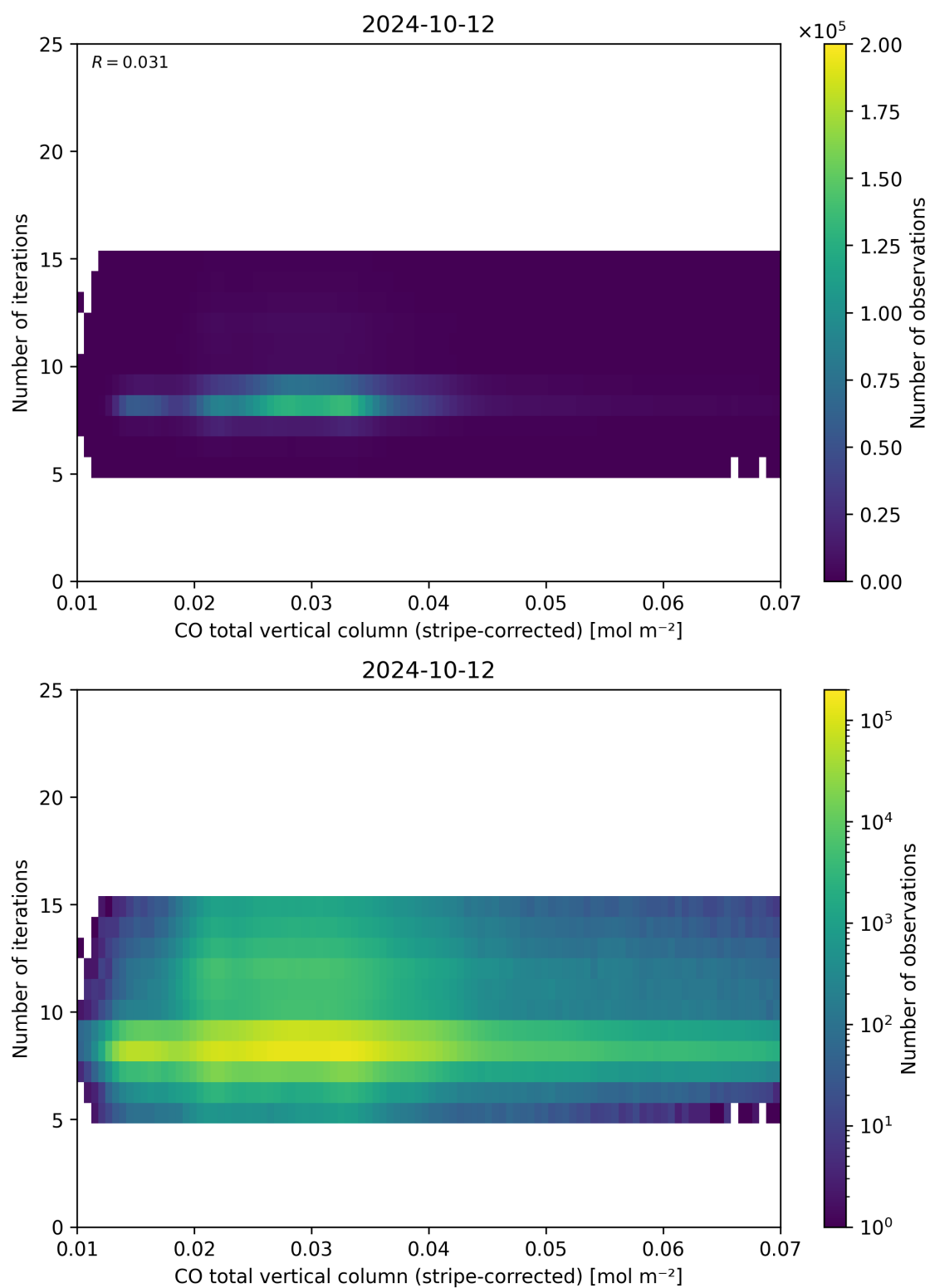
Figure 39: Scatter density plot of “CO total vertical column (stripe-corrected)” against “Number of iterations” for 2024-10-11 to 2024-10-13.
