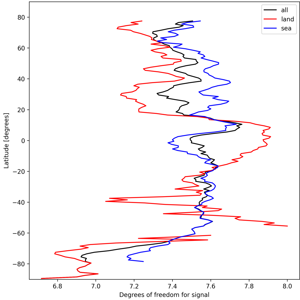
Figure 15: Zonal average of “Degrees of freedom for signal” for 2024-10-11 to 2024-10-13.
