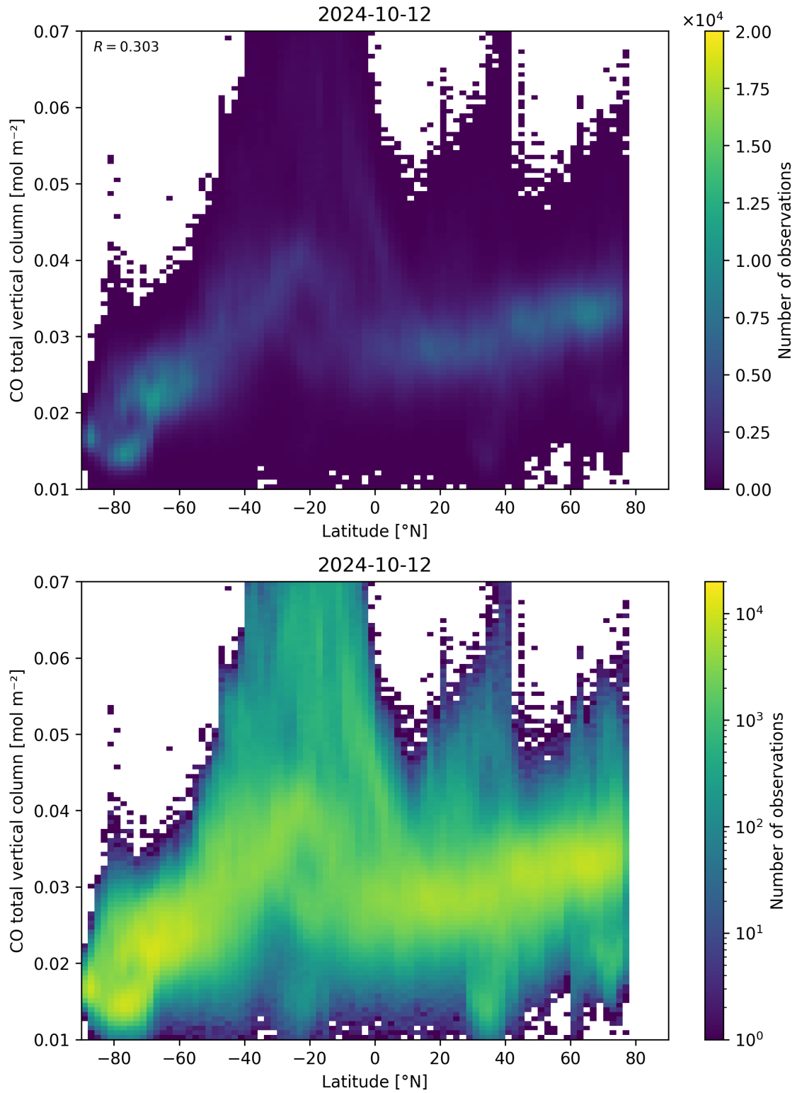
Figure 51: Scatter density plot of “Latitude” against “CO total vertical column” for 2024-10-11 to 2024-10-13.
