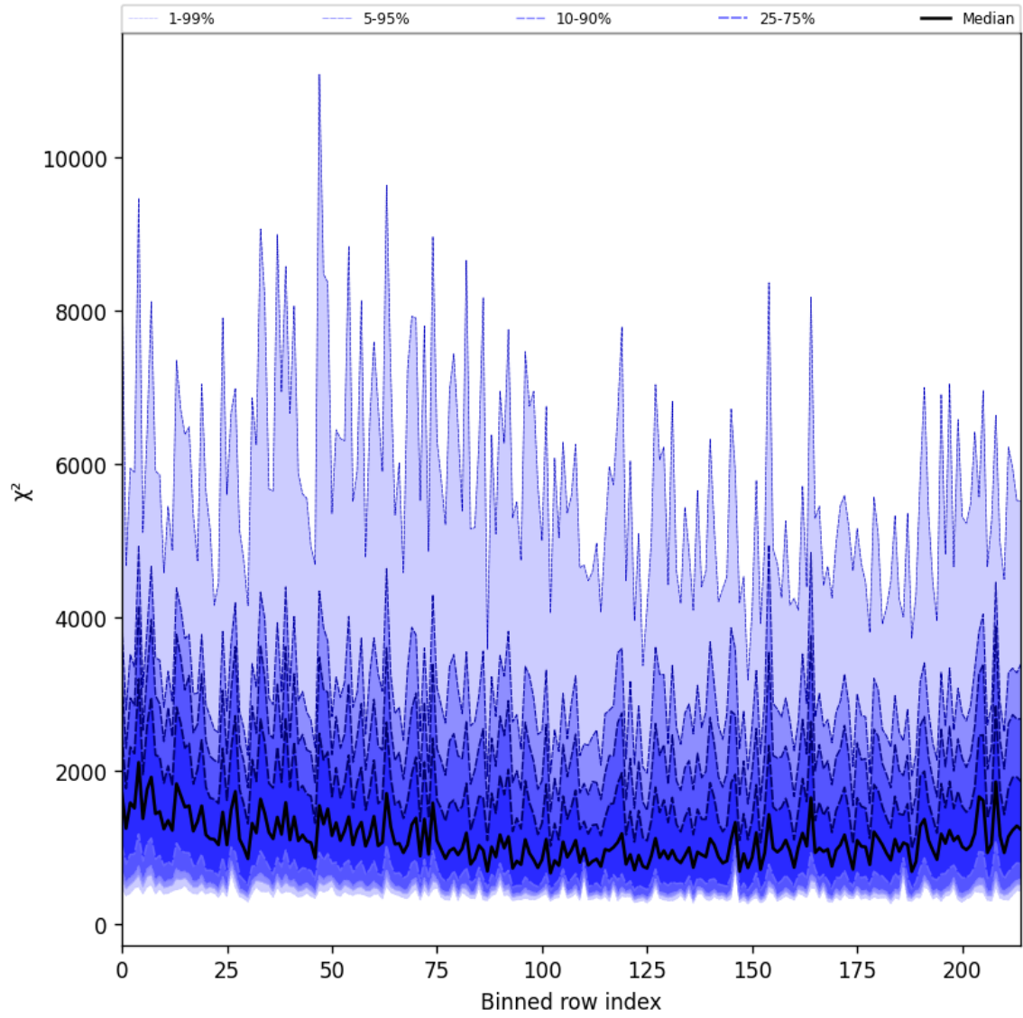
Figure 30: Along track statistics of “ \chi^2 ” for 2024-10-11 to 2024-10-13
