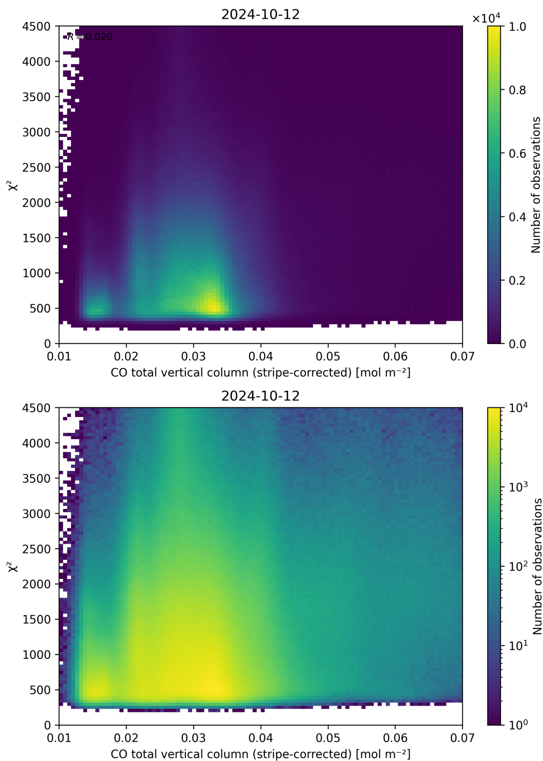
Figure 37: Scatter density plot of “CO total vertical column (stripe-corrected)” against “ \chi^2 ” for 2024-10-11 to 2024-10-13.
