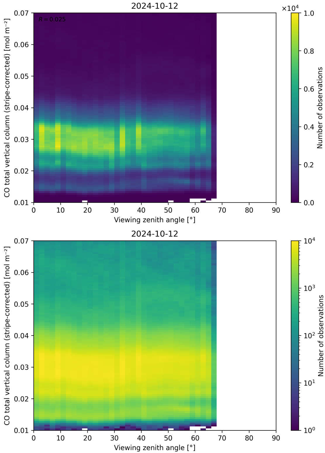
Figure 70: Scatter density plot of “Viewing zenith angle” against “CO total vertical column (stripe-corrected)” for 2024-10-11 to 2024-10-13.
