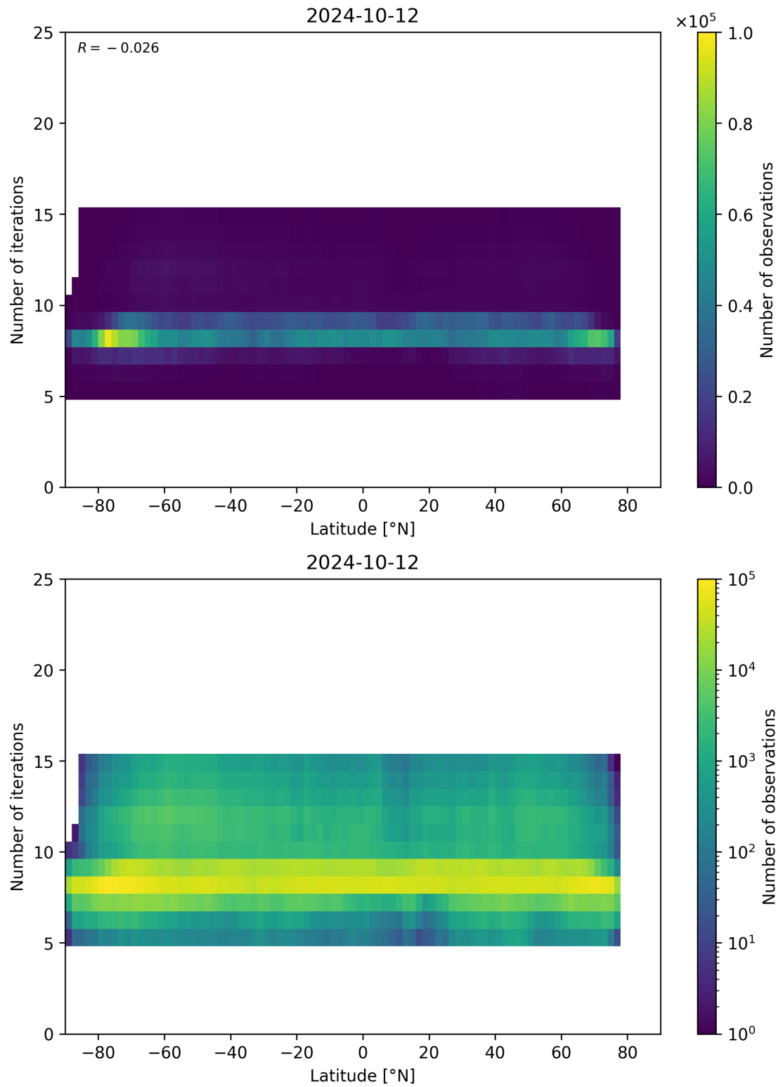
Figure 56: Scatter density plot of “Latitude” against “Number of iterations” for 2024-10-11 to 2024-10-13.
