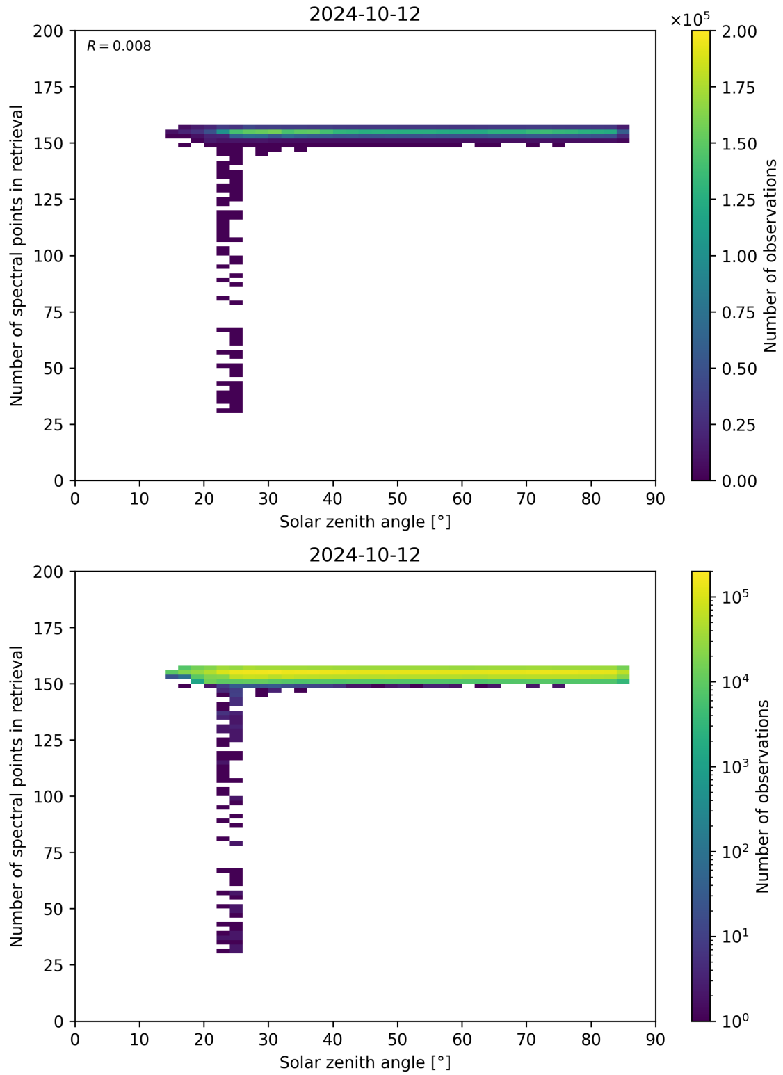
Figure 68: Scatter density plot of “Solar zenith angle” against “Number of spectral points in retrieval” for 2024-10-11 to 2024-10-13.
