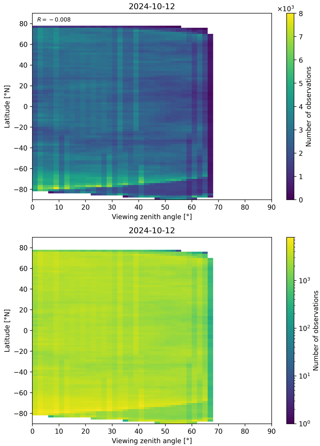
Figure 74: Scatter density plot of “Viewing zenith angle” against “Latitude” for 2024-10-11 to 2024-10-13.
