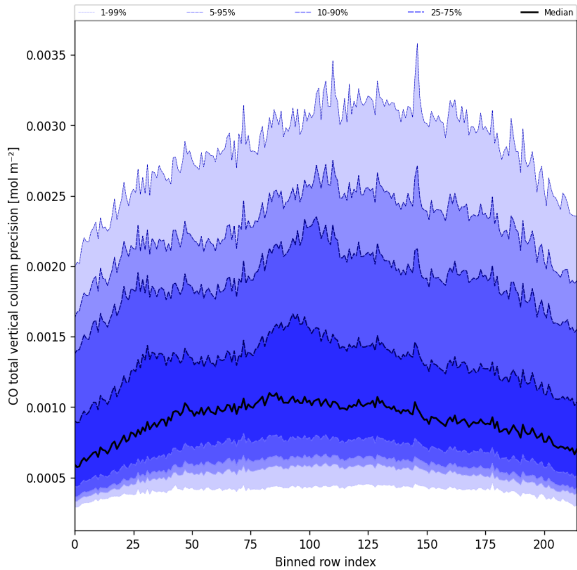
Figure 28: Along track statistics of “CO total vertical column precision” for 2024-10-11 to 2024-10-13
