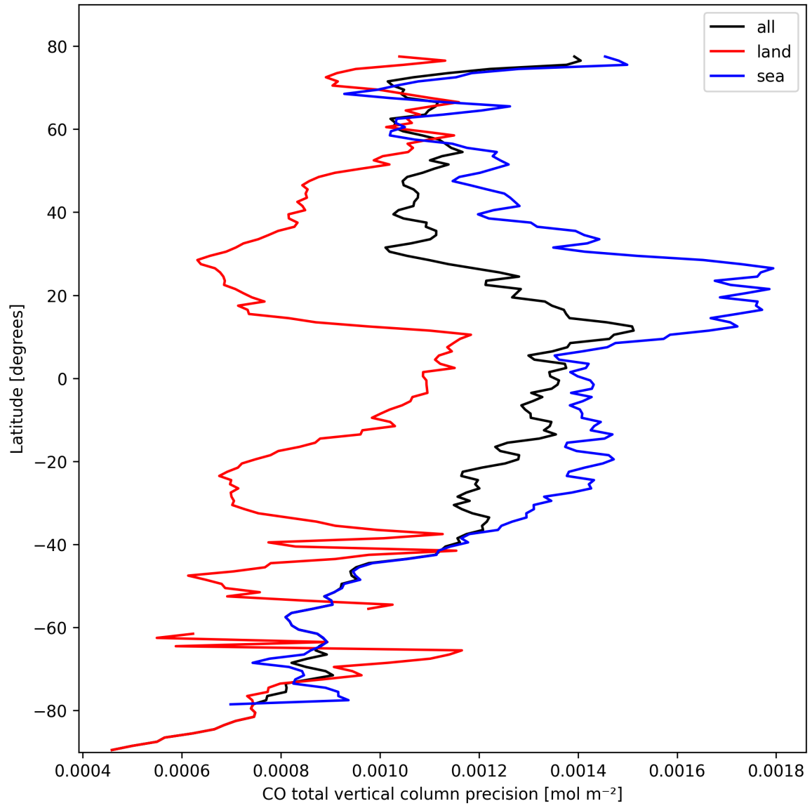
Figure 12: Zonal average of “CO total vertical column precision” for 2024-10-11 to 2024-10-13.
