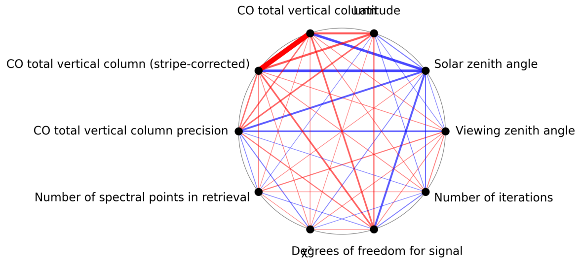
Figure 1: Map of correlation graph for 2024-10-11 to 2024-10-13.
