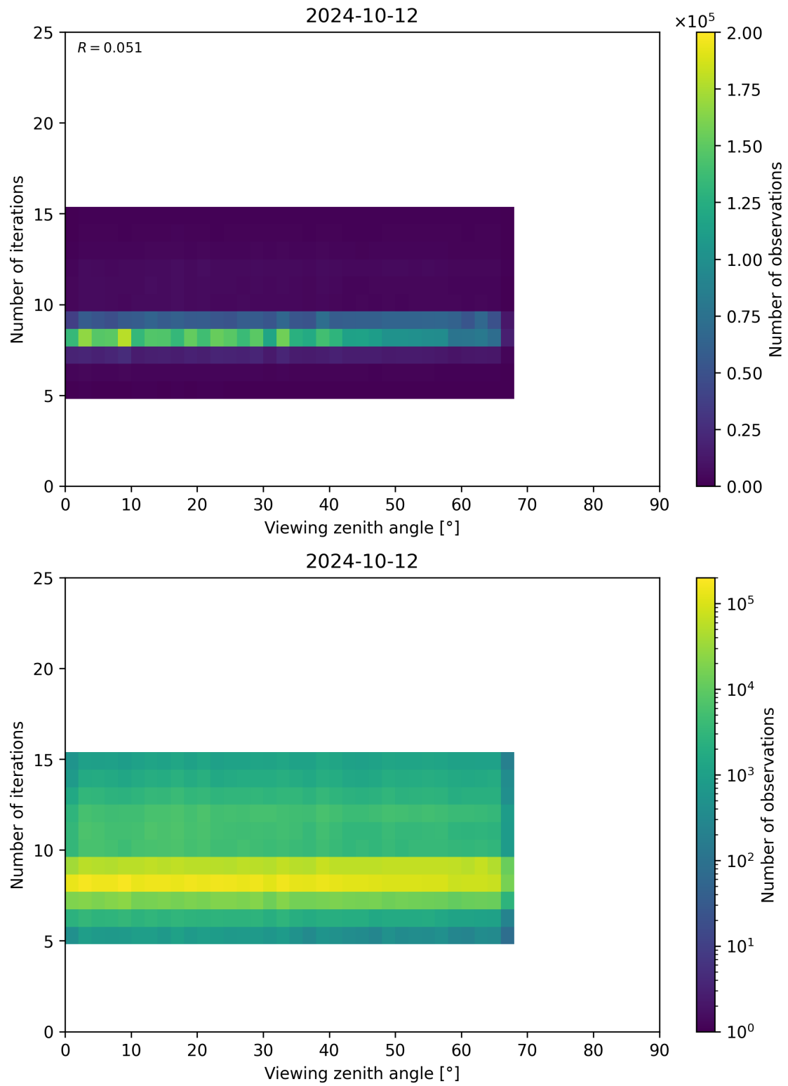
Figure 75: Scatter density plot of “Viewing zenith angle” against “Number of iterations” for 2024-10-11 to 2024-10-13.
