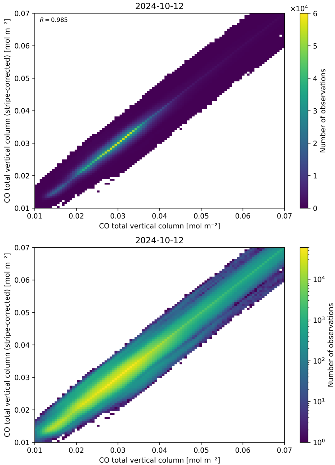
Figure 33: Scatter density plot of “CO total vertical column” against “CO total vertical column (stripe-corrected)” for 2024-10-11 to 2024-10-13.
