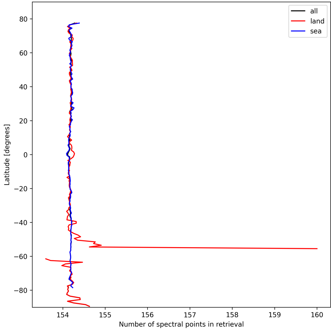
Figure 13: Zonal average of “Number of spectral points in retrieval” for 2024-10-11 to 2024-10-13.
