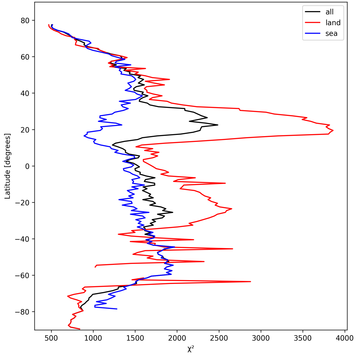
Figure 14: Zonal average of “ \chi^2 ” for 2024-10-11 to 2024-10-13.
