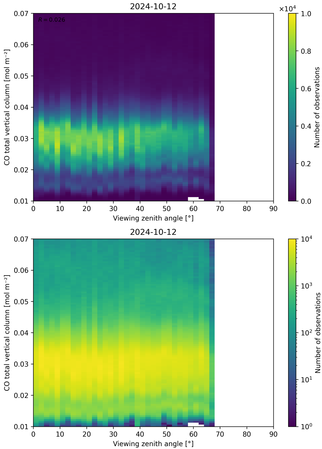
Figure 69: Scatter density plot of “Viewing zenith angle” against “CO total vertical column” for 2024-10-11 to 2024-10-13.
