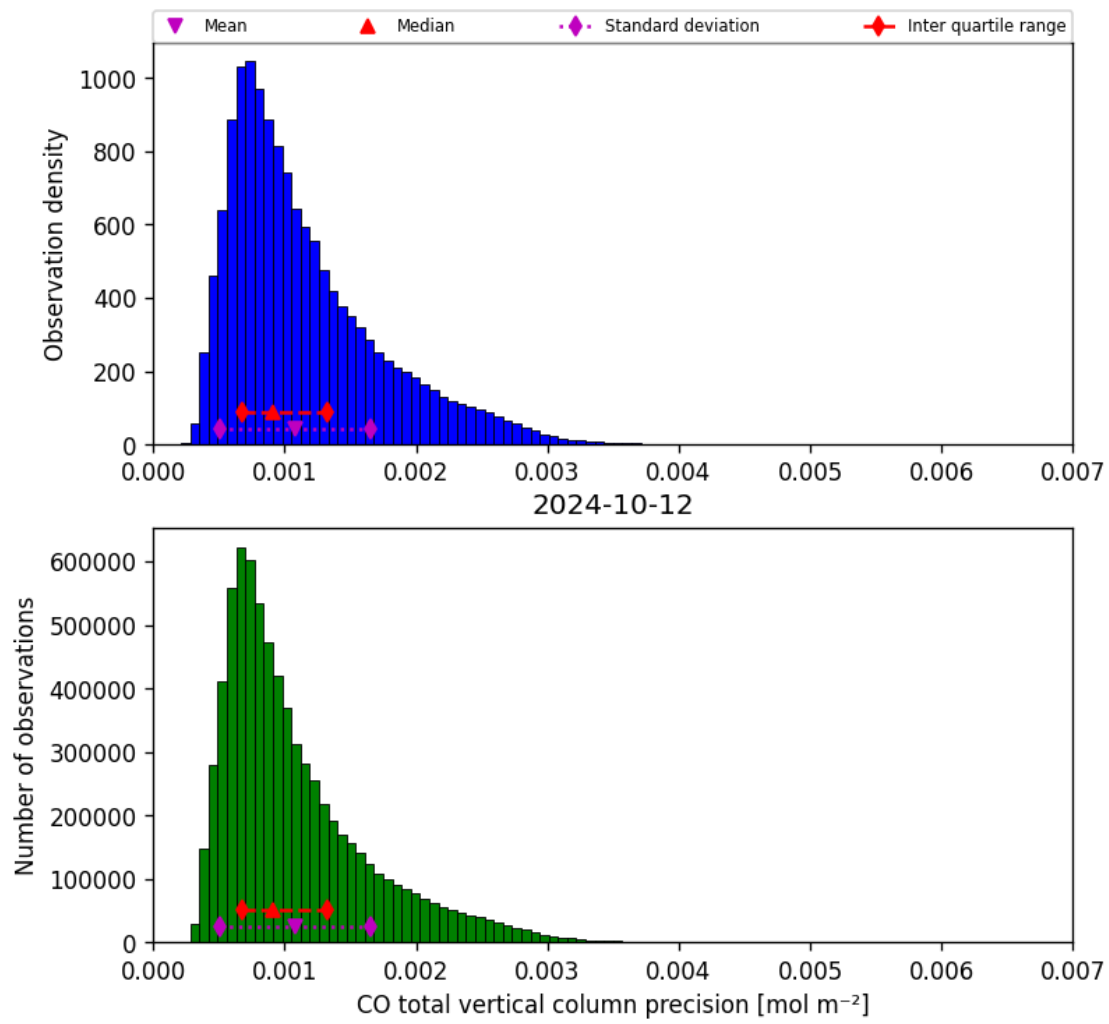
Figure 20: Histogram of “CO total vertical column precision” for 2024-10-11 to 2024-10-13
