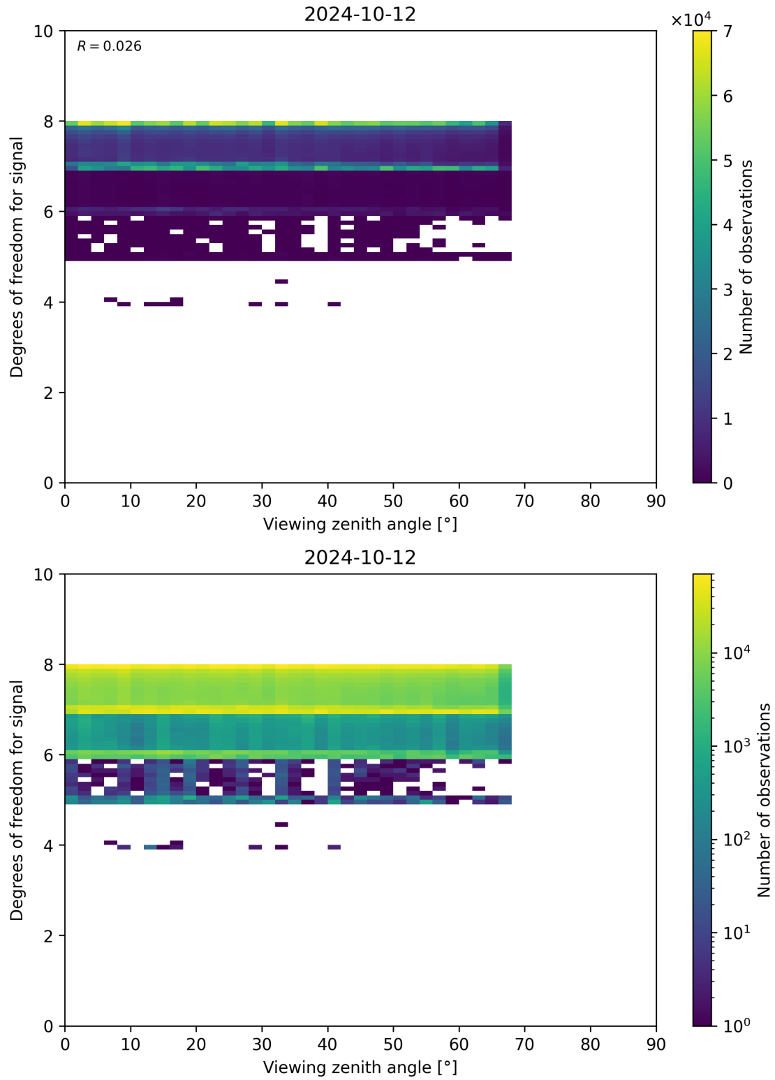
Figure 73: Scatter density plot of “Viewing zenith angle” against “Degrees of freedom for signal” for 2024-10-11 to 2024-10-13.
