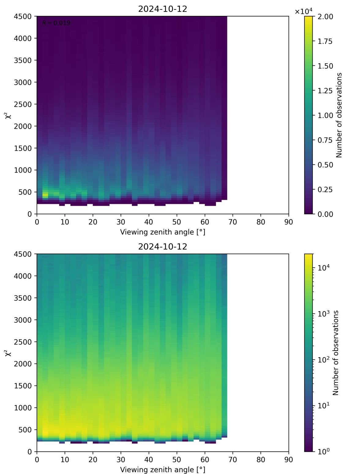
Figure 72: Scatter density plot of “Viewing zenith angle” against “ \chi^2 ” for 2024-10-11 to 2024-10-13.
