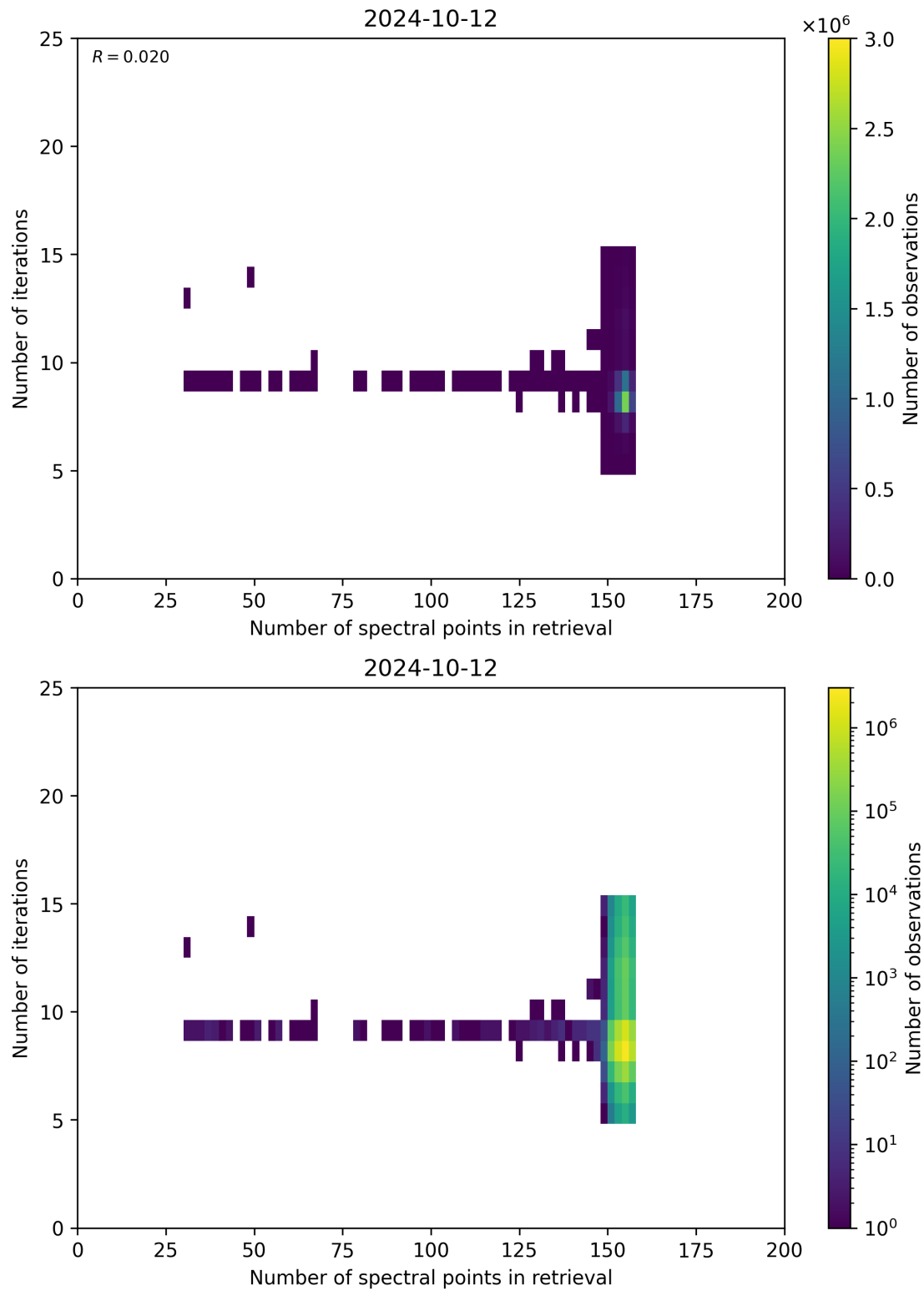
Figure 60: Scatter density plot of “Number of spectral points in retrieval” against “Number of iterations” for 2024-10-11 to 2024-10-13.
