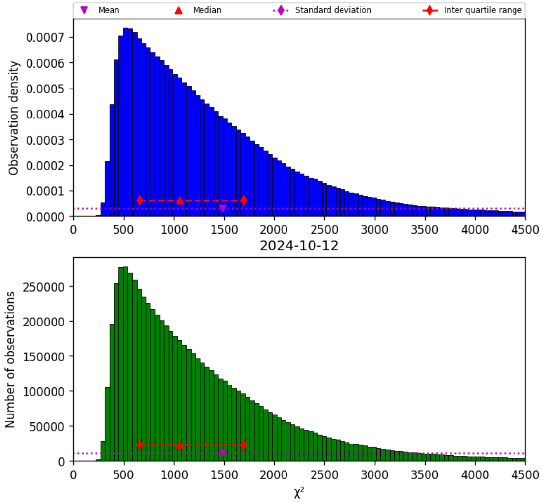
Figure 22: Histogram of “ \chi^2 ” for 2024-10-11 to 2024-10-13
