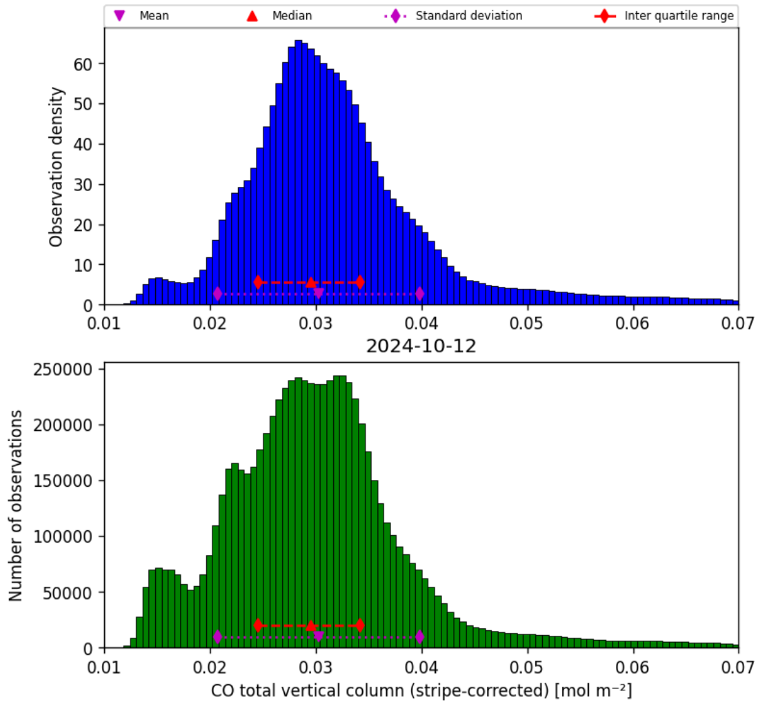
Figure 19: Histogram of “CO total vertical column (stripe-corrected)” for 2024-10-11 to 2024-10-13
