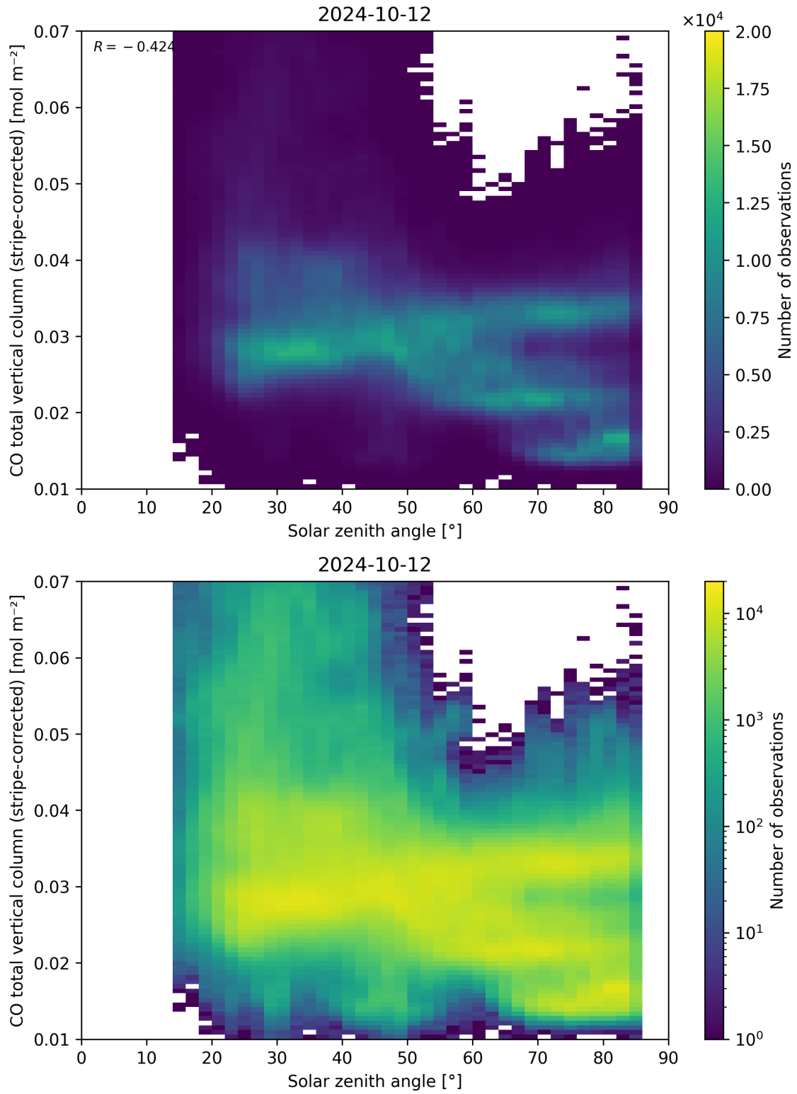
Figure 62: Scatter density plot of “Solar zenith angle” against “CO total vertical column (stripe-corrected)” for 2024-10-11 to 2024-10-13.
