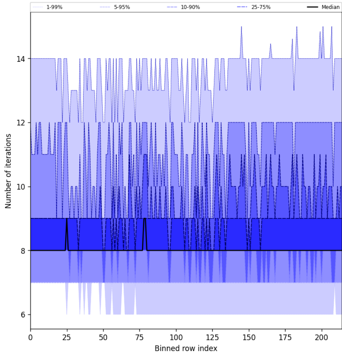
Figure 32: Along track statistics of “Number of iterations” for 2024-10-11 to 2024-10-13
