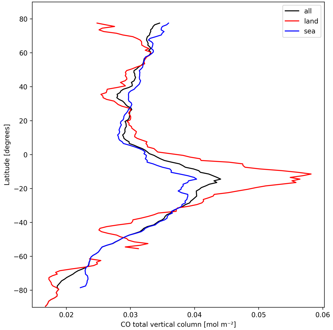
Figure 10: Zonal average of “CO total vertical column” for 2024-10-11 to 2024-10-13.
