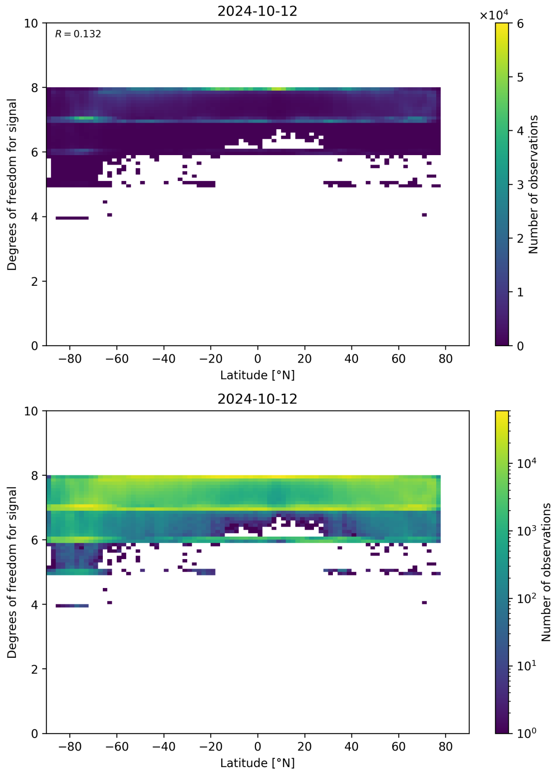
Figure 55: Scatter density plot of “Latitude” against “Degrees of freedom for signal” for 2024-10-11 to 2024-10-13.
