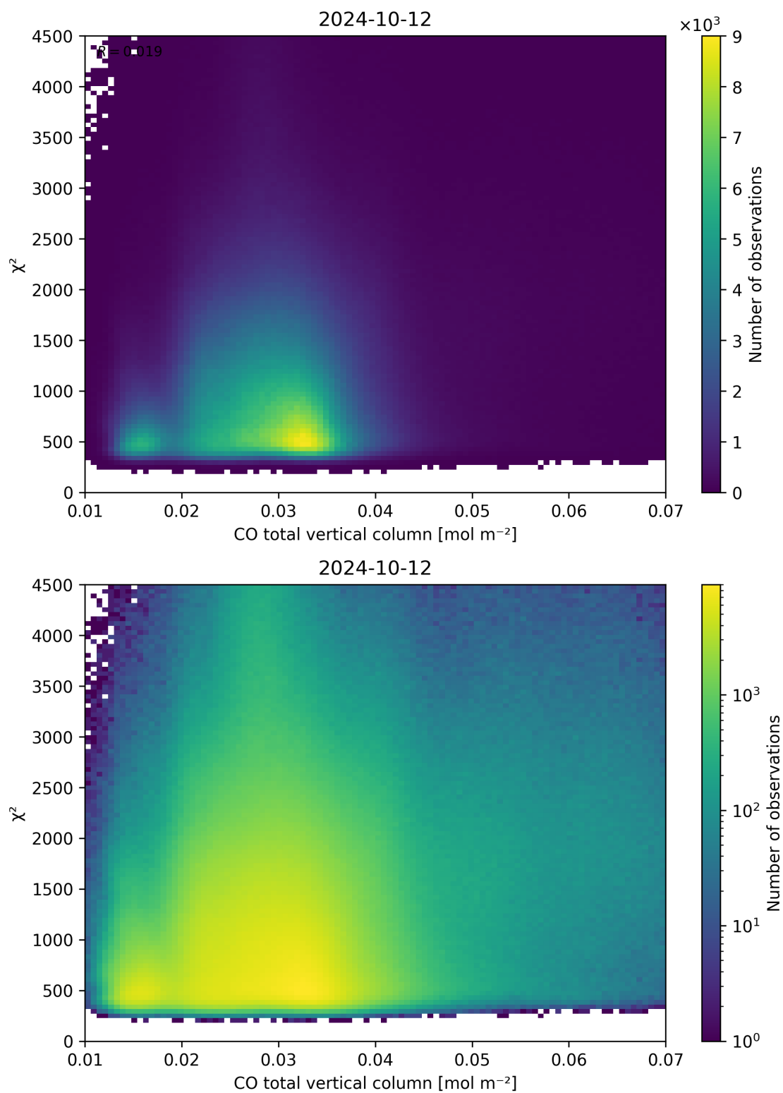
Figure 35: Scatter density plot of “CO total vertical column” against “ \chi^2 ” for 2024-10-11 to 2024-10-13.
