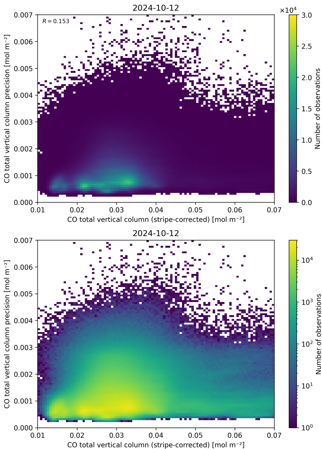
Figure 36: Scatter density plot of “CO total vertical column (stripe-corrected)” against “CO total vertical column precision” for 2024-10-11 to 2024-10-13.
