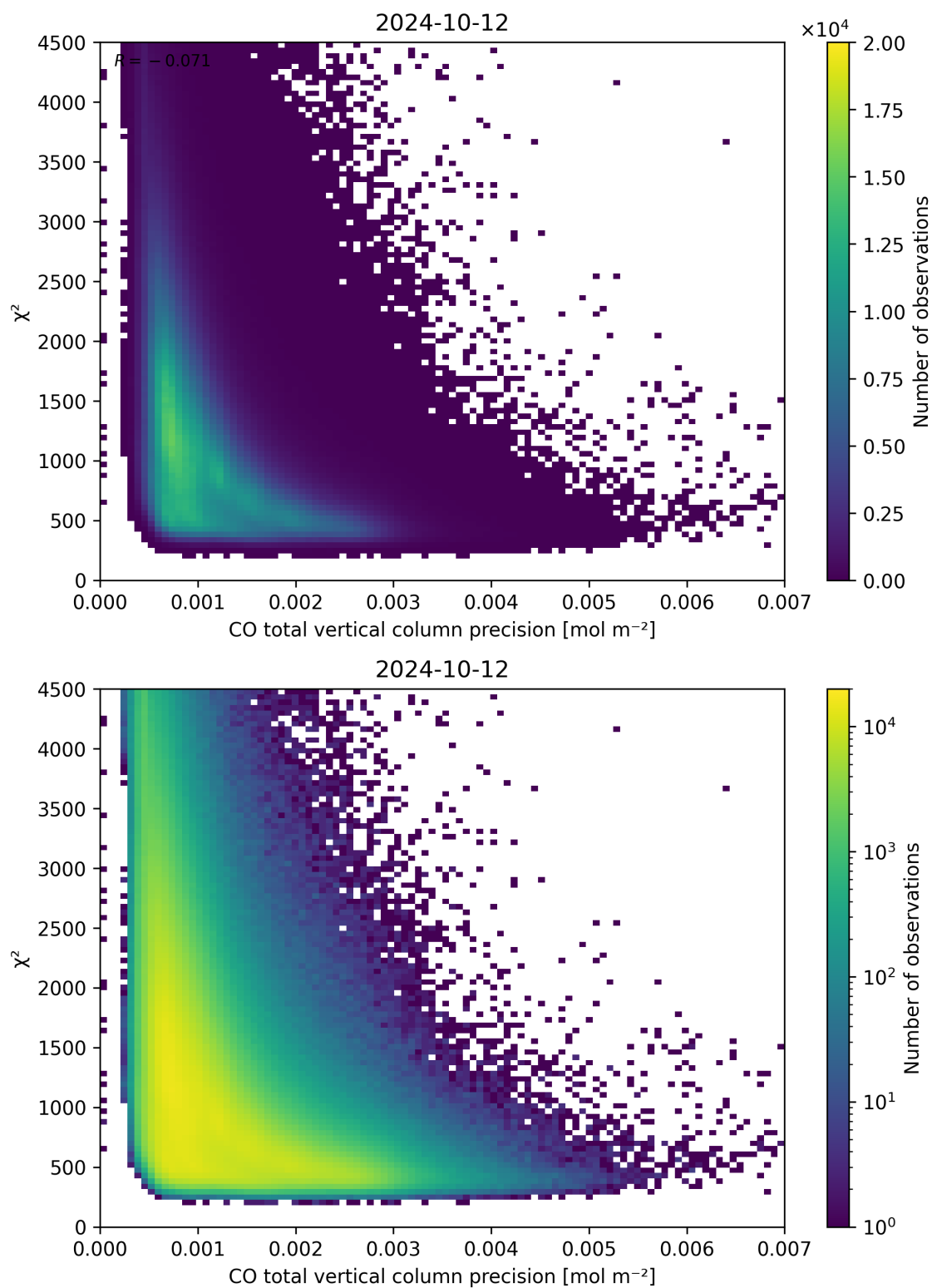
Figure 44: Scatter density plot of “CO total vertical column precision” against “ \chi^2 ” for 2024-10-11 to 2024-10-13.
