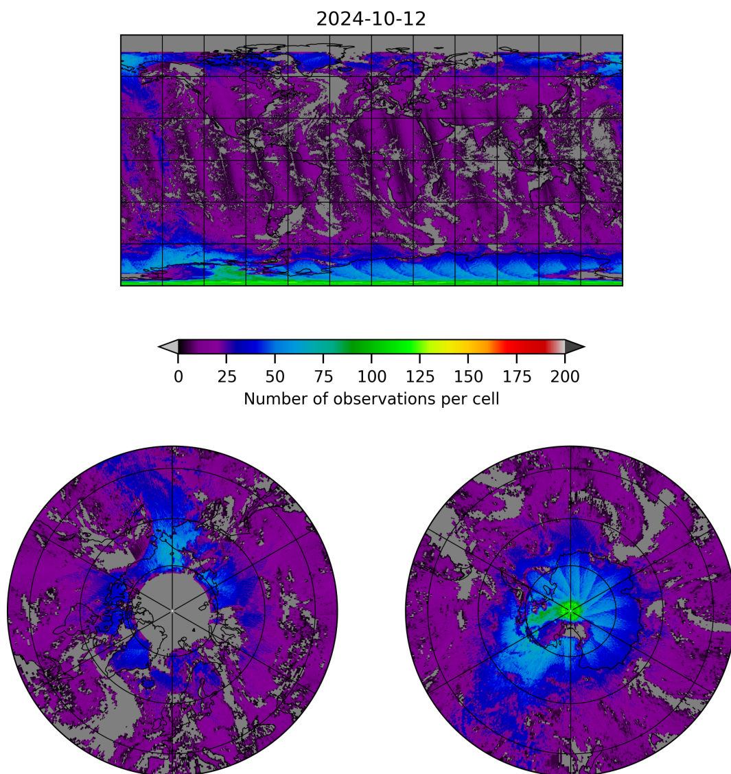
Figure 8: Map of the number of observations for 2024-10-11 to 2024-10-13
