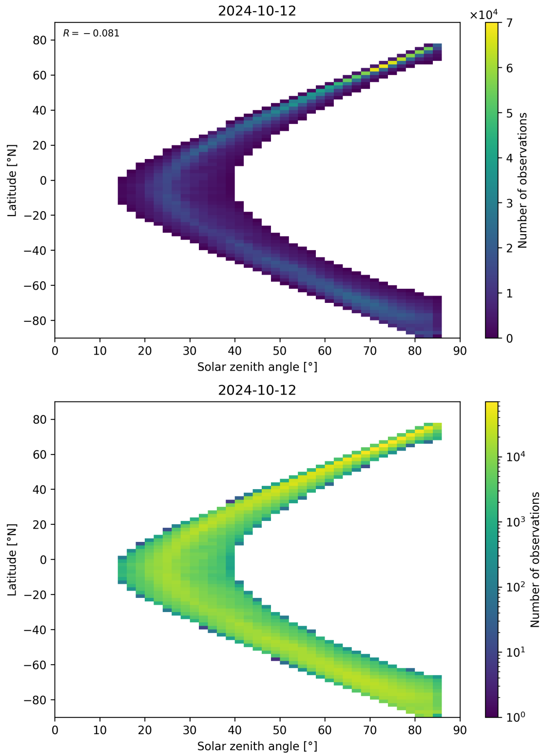
Figure 66: Scatter density plot of “Solar zenith angle” against “Latitude” for 2024-10-11 to 2024-10-13.
