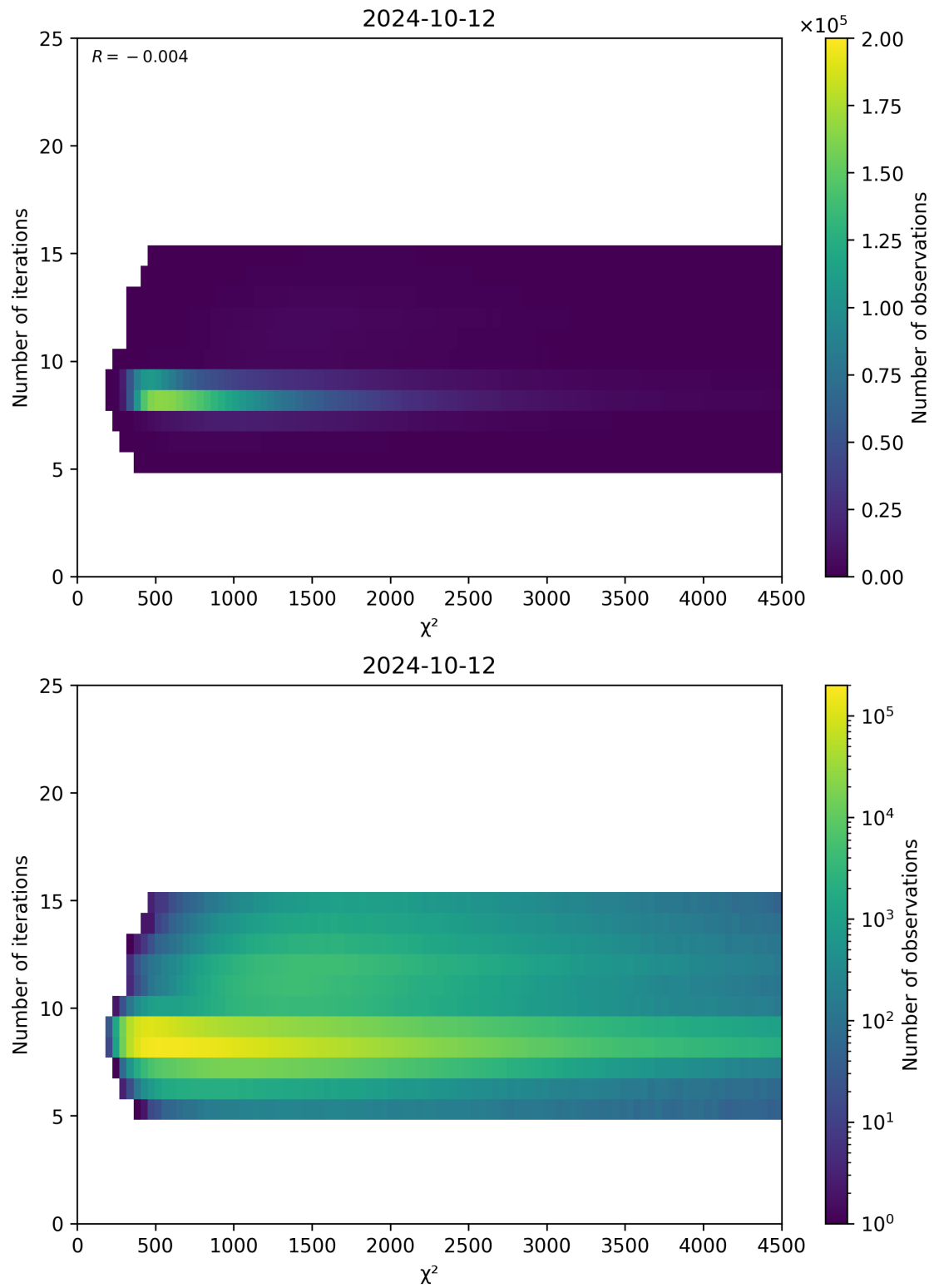
Figure 49: Scatter density plot of “ \chi^2 ” against “Number of iterations” for 2024-10-11 to 2024-10-13.
