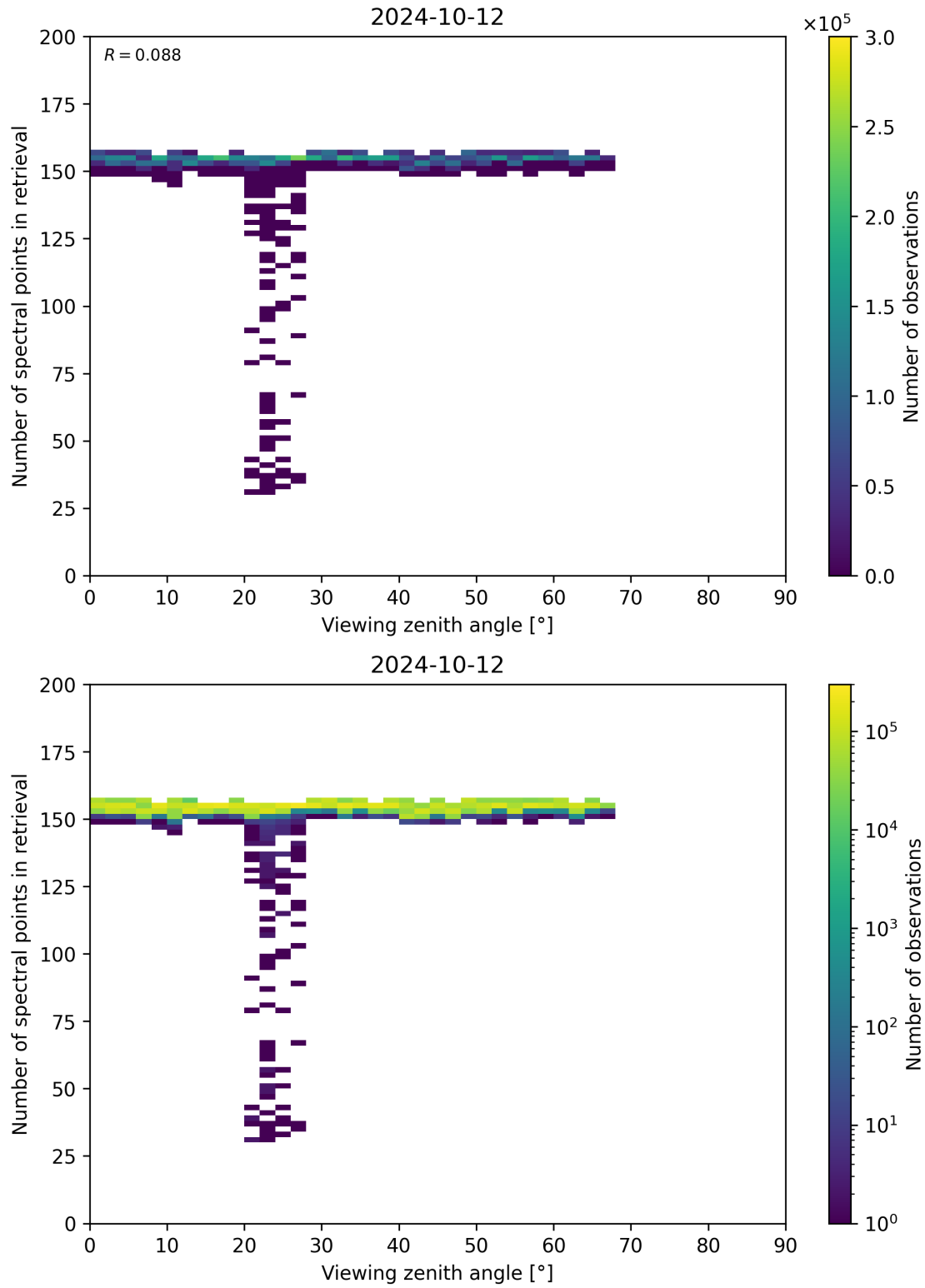
Figure 76: Scatter density plot of “Viewing zenith angle” against “Number of spectral points in retrieval” for 2024-10-11 to 2024-10-13.
