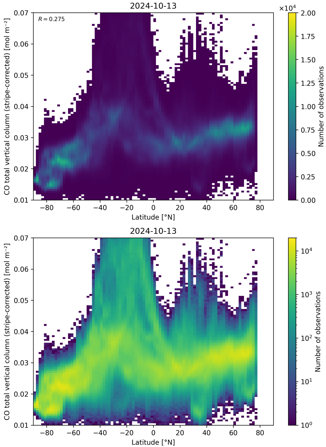
Figure 52: Scatter density plot of “Latitude” against “CO total vertical column (stripe-corrected)” for 2024-10-12 to 2024-10-14.
