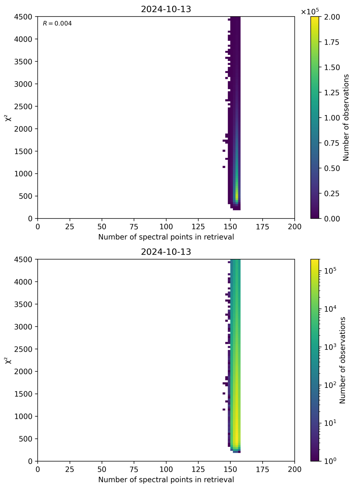
Figure 58: Scatter density plot of “Number of spectral points in retrieval” against “ \chi^2 ” for 2024-10-12 to 2024-10-14.
