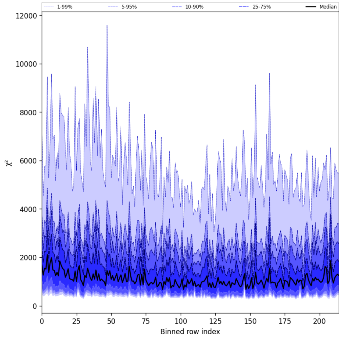
Figure 30: Along track statistics of “ \chi^2 ” for 2024-10-12 to 2024-10-14
