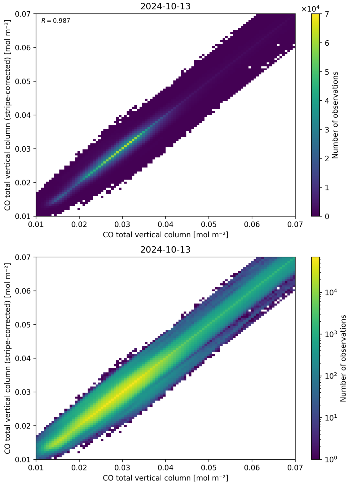
Figure 33: Scatter density plot of “CO total vertical column” against “CO total vertical column (stripe-corrected)” for 2024-10-12 to 2024-10-14.
