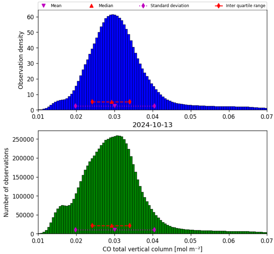
Figure 18: Histogram of “CO total vertical column” for 2024-10-12 to 2024-10-14
