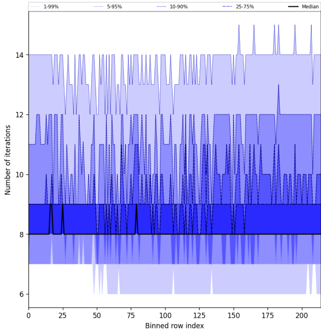
Figure 32: Along track statistics of “Number of iterations” for 2024-10-12 to 2024-10-14
