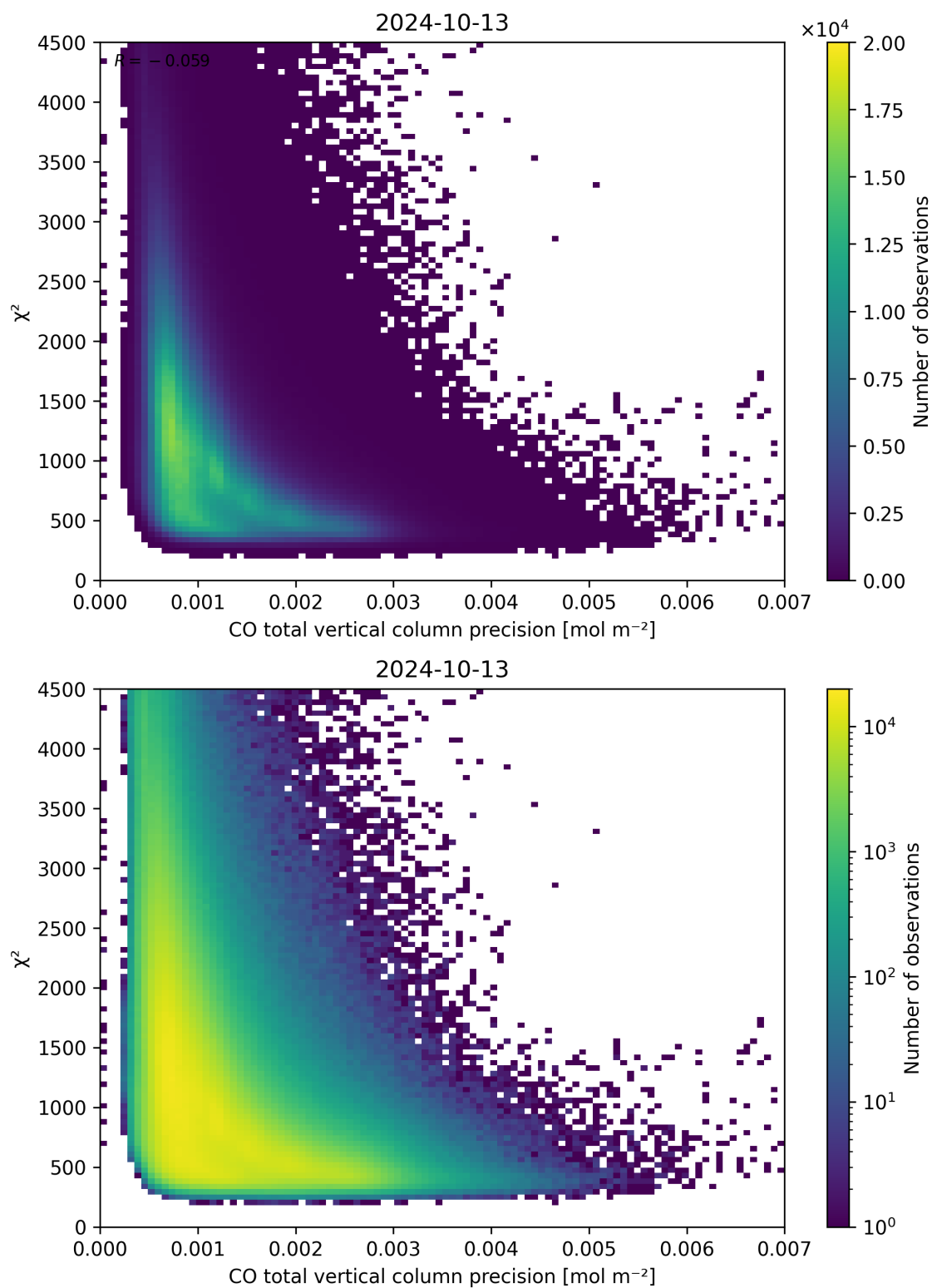
Figure 44: Scatter density plot of “CO total vertical column precision” against “ \chi^2 ” for 2024-10-12 to 2024-10-14.
