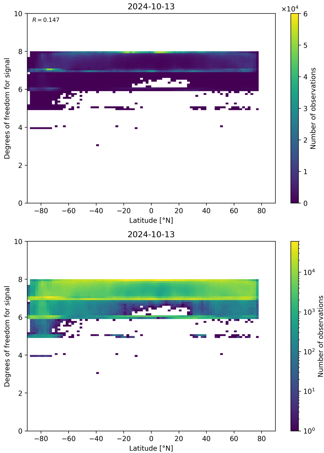
Figure 55: Scatter density plot of “Latitude” against “Degrees of freedom for signal” for 2024-10-12 to 2024-10-14.
