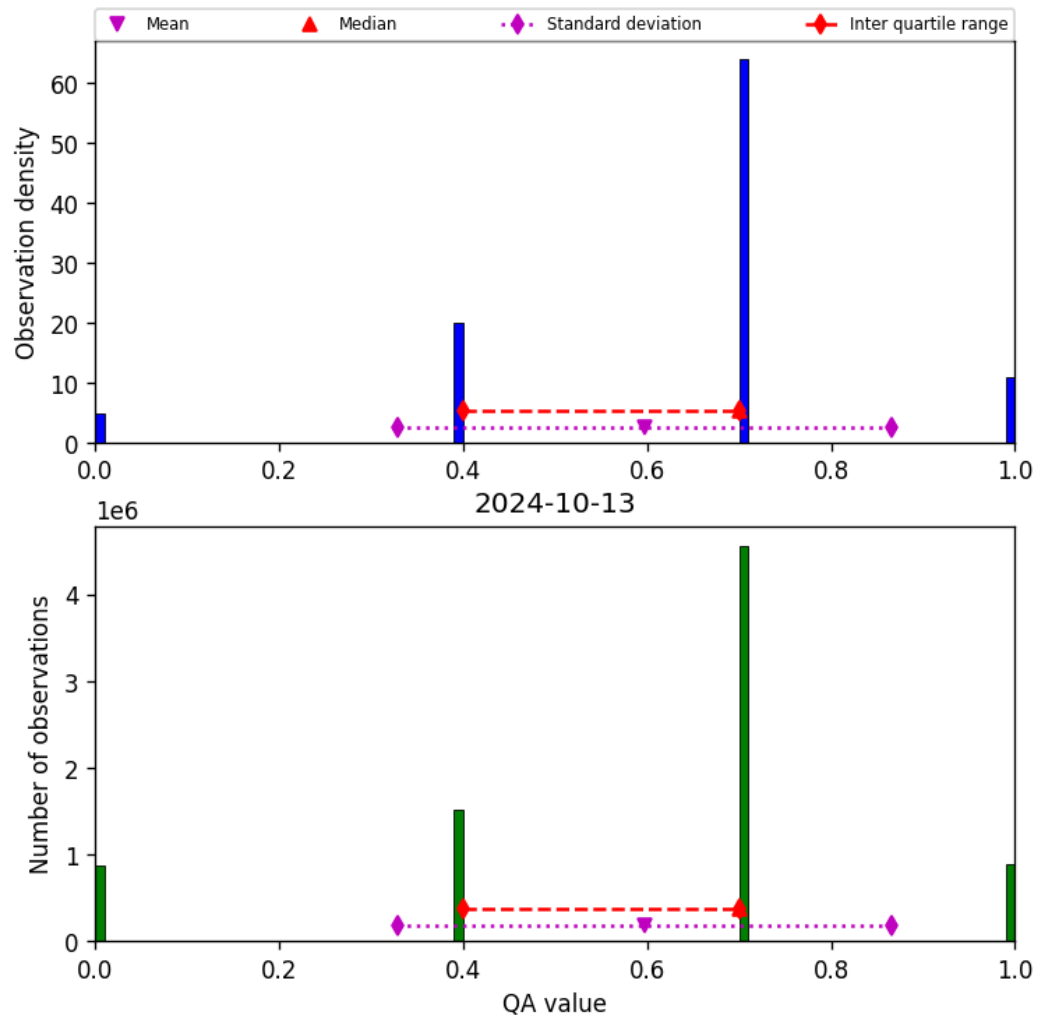
Figure 17: Histogram of “QA value” for 2024-10-12 to 2024-10-14
