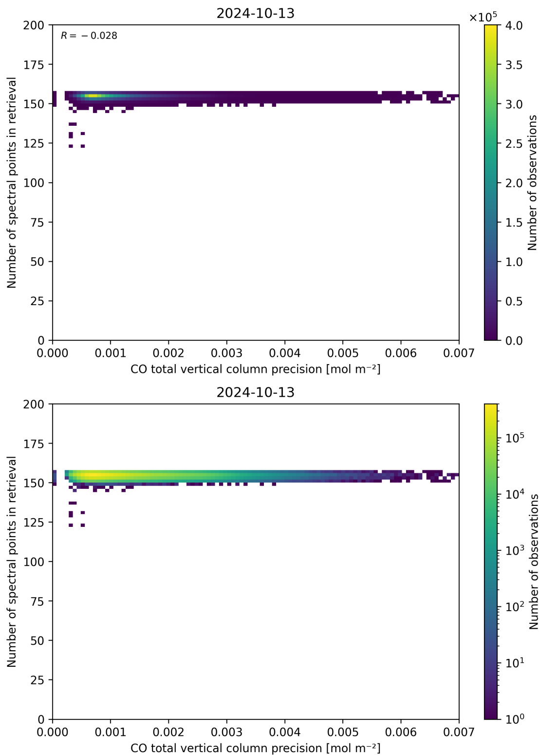
Figure 47: Scatter density plot of “CO total vertical column precision” against “Number of spectral points in retrieval” for 2024-10-12 to 2024-10-14.
