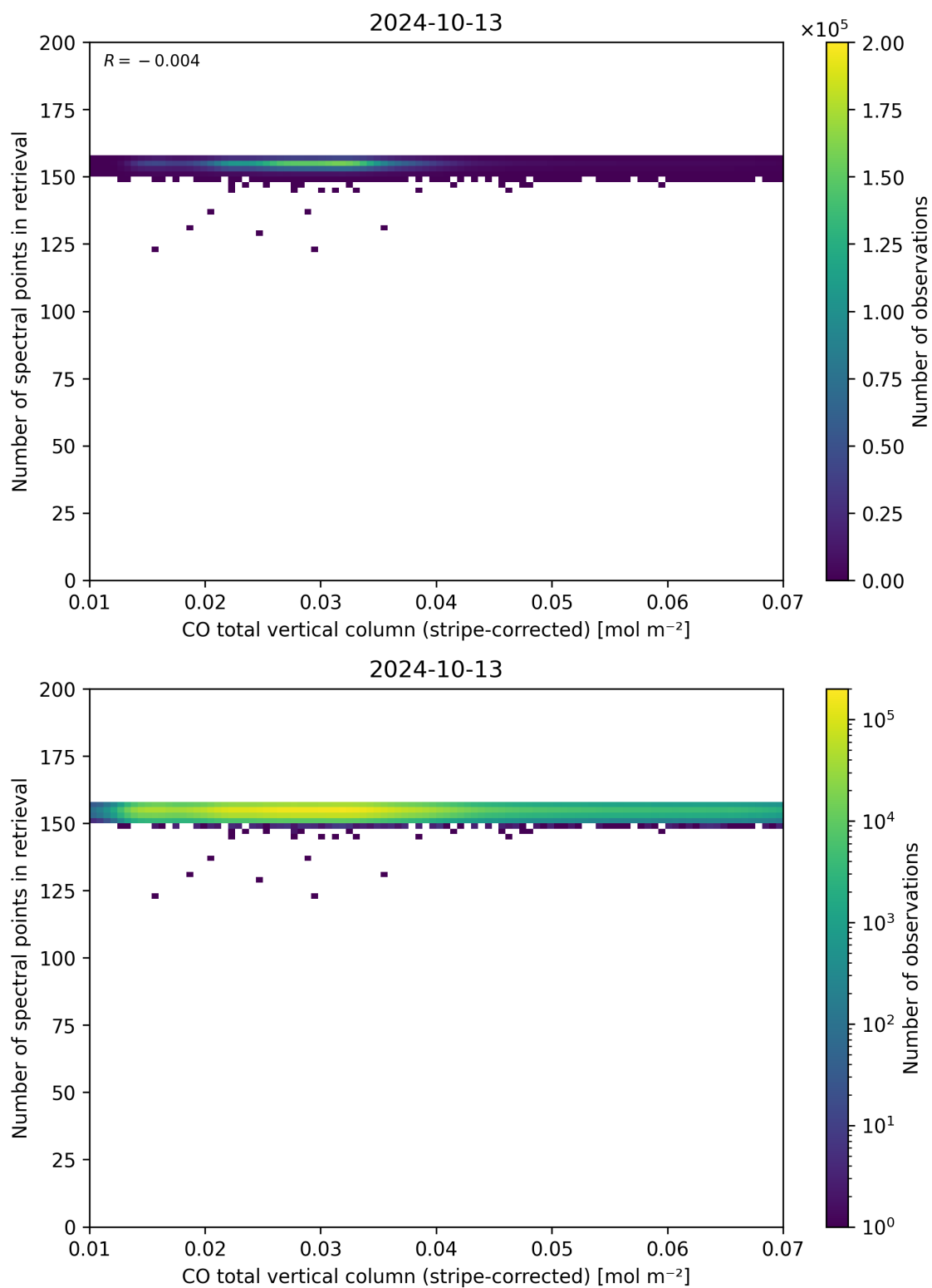
Figure 40: Scatter density plot of “CO total vertical column (stripe-corrected)” against “Number of spectral points in retrieval” for 2024-10-12 to 2024-10-14.
