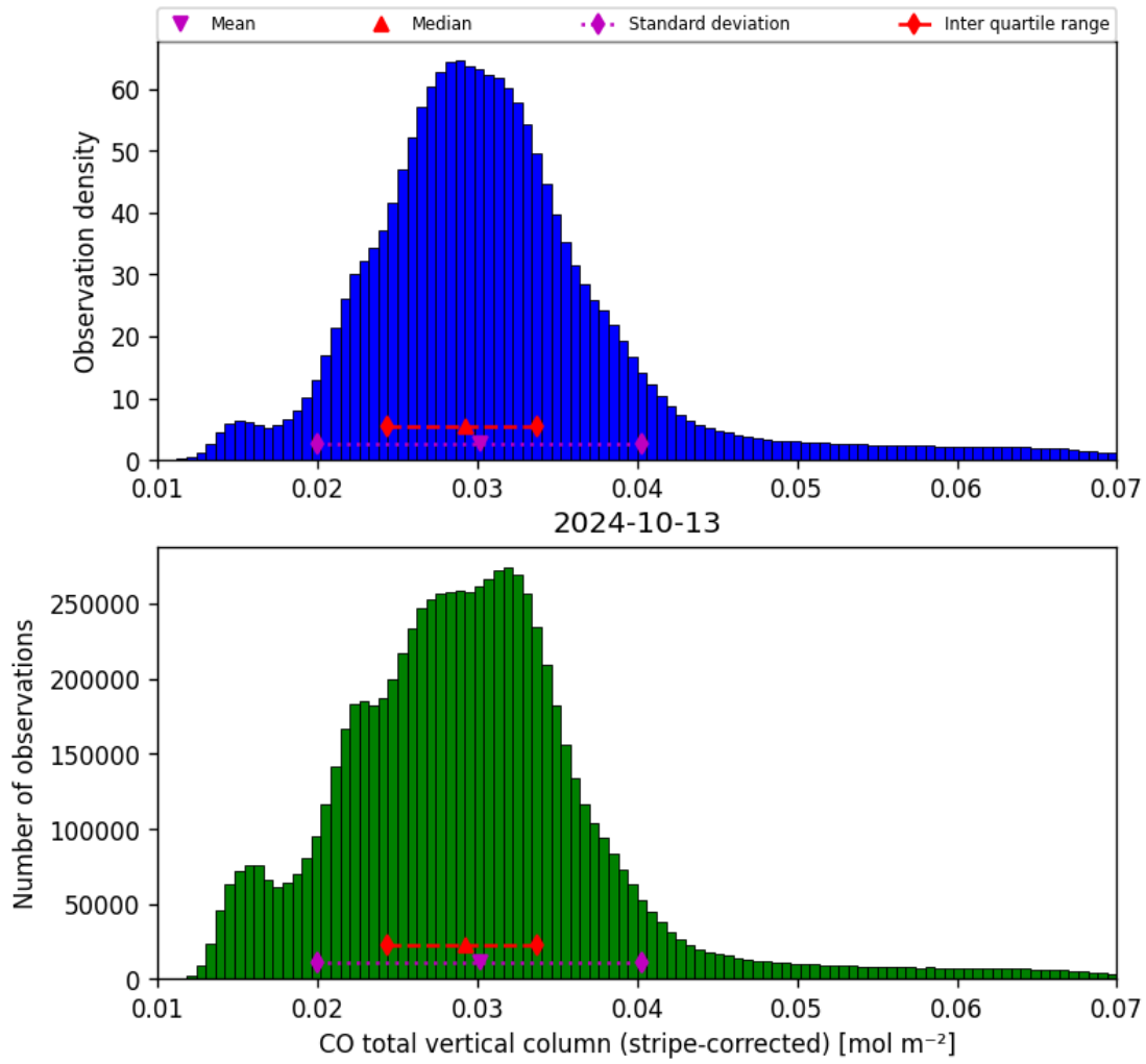
Figure 19: Histogram of “CO total vertical column (stripe-corrected)” for 2024-10-12 to 2024-10-14
