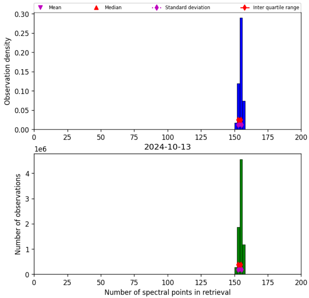
Figure 21: Histogram of “Number of spectral points in retrieval” for 2024-10-12 to 2024-10-14
