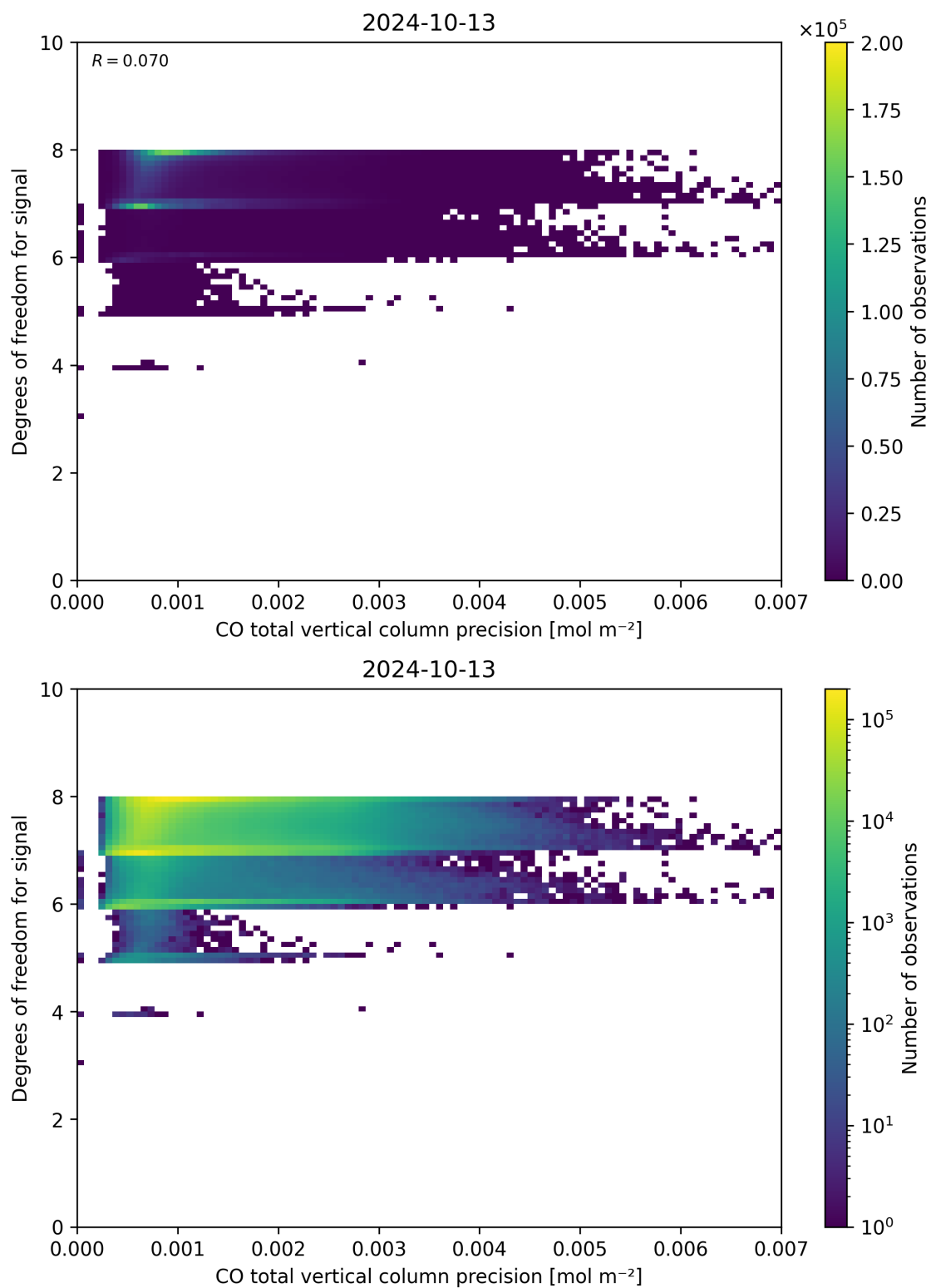
Figure 45: Scatter density plot of “CO total vertical column precision” against “Degrees of freedom for signal” for 2024-10-12 to 2024-10-14.
