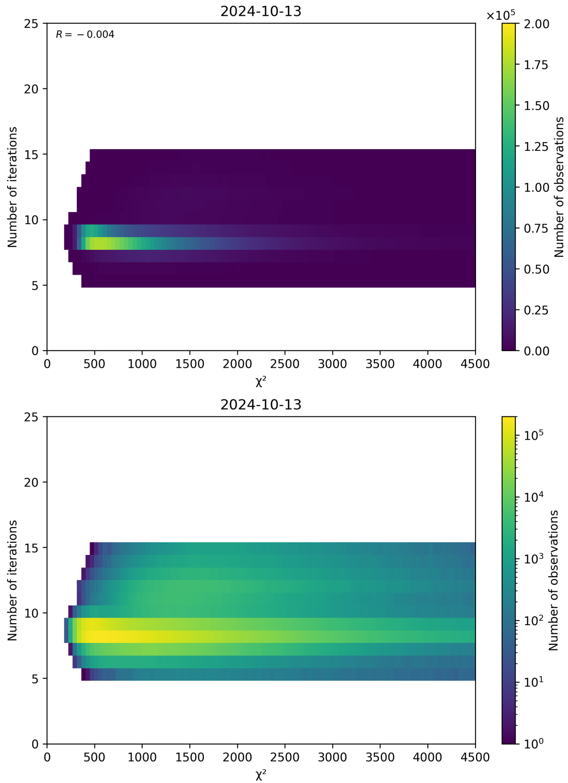
Figure 49: Scatter density plot of “ \chi^2 ” against “Number of iterations” for 2024-10-12 to 2024-10-14.
