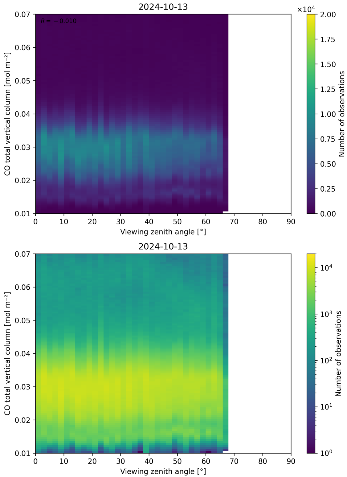
Figure 69: Scatter density plot of “Viewing zenith angle” against “CO total vertical column” for 2024-10-12 to 2024-10-14.
