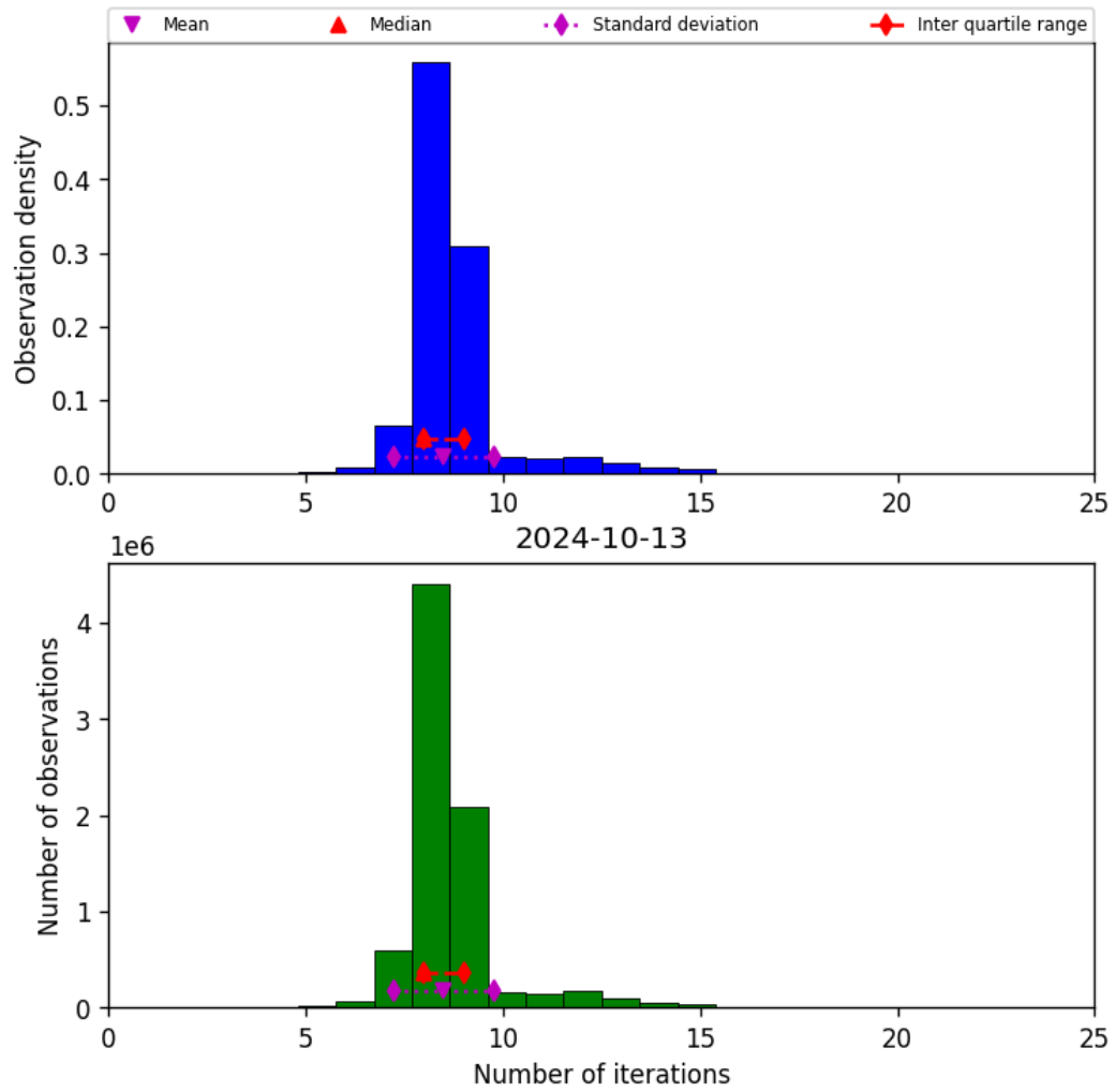
Figure 24: Histogram of “Number of iterations” for 2024-10-12 to 2024-10-14
