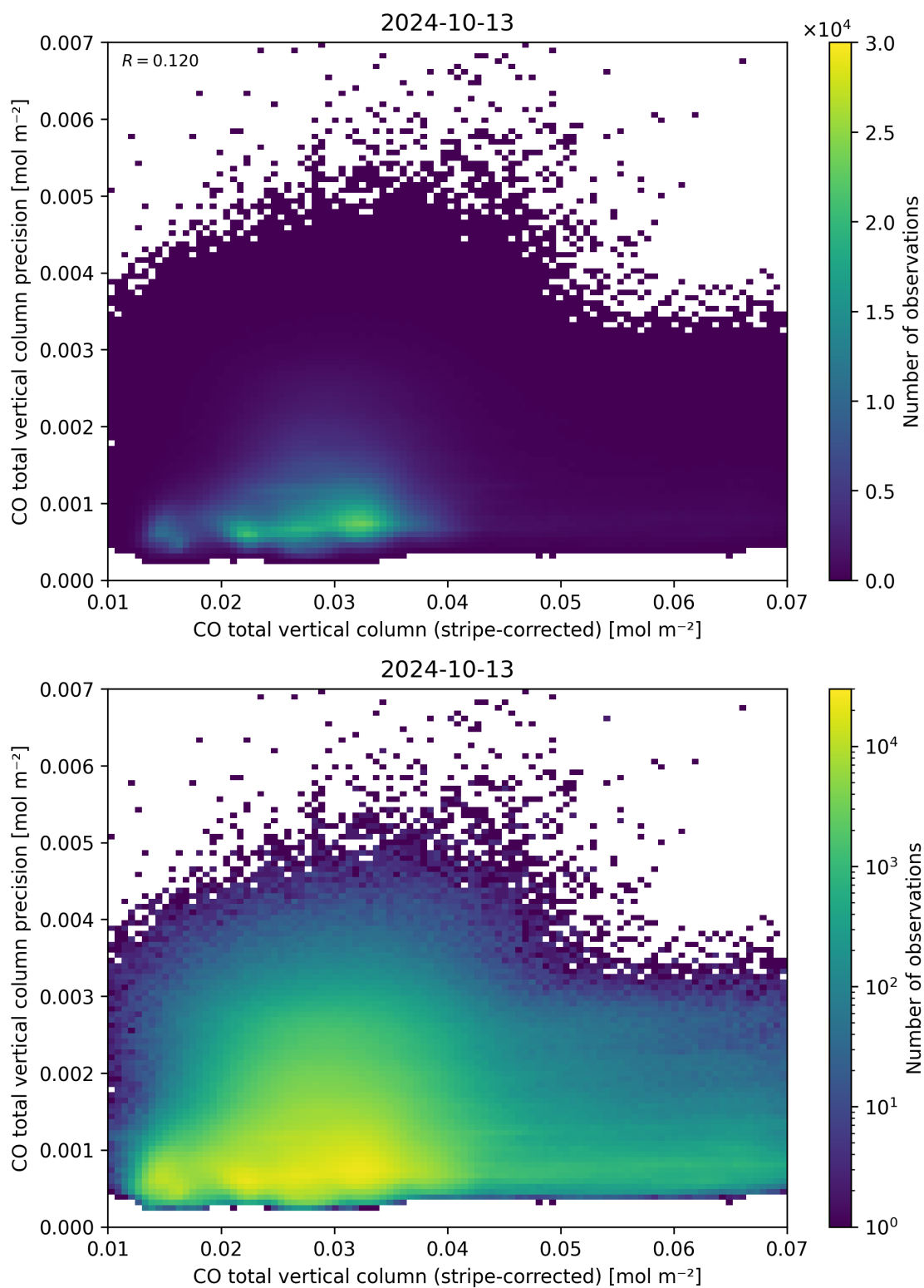
Figure 36: Scatter density plot of “CO total vertical column (stripe-corrected)” against “CO total vertical column precision” for 2024-10-12 to 2024-10-14.
