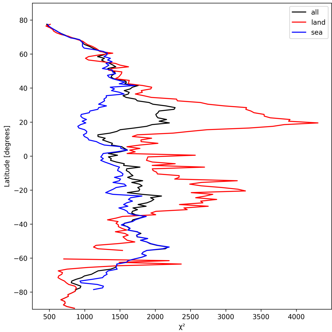
Figure 14: Zonal average of “ \chi^2 ” for 2024-10-12 to 2024-10-14.
