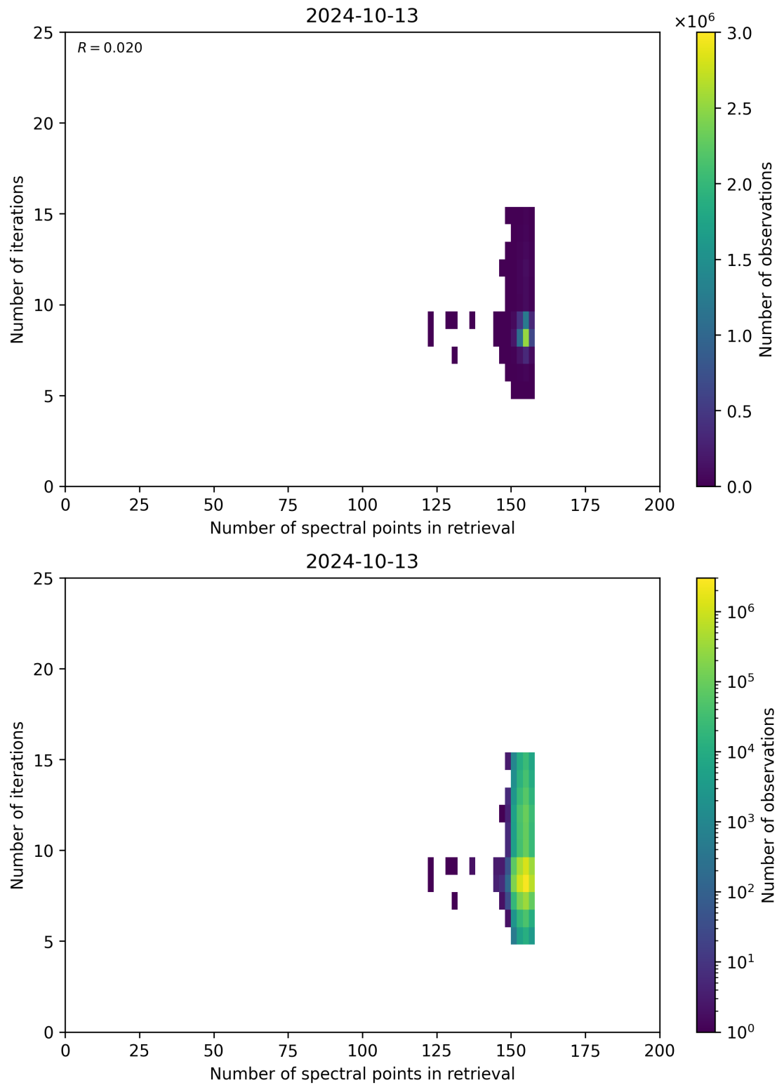
Figure 60: Scatter density plot of “Number of spectral points in retrieval” against “Number of iterations” for 2024-10-12 to 2024-10-14.
