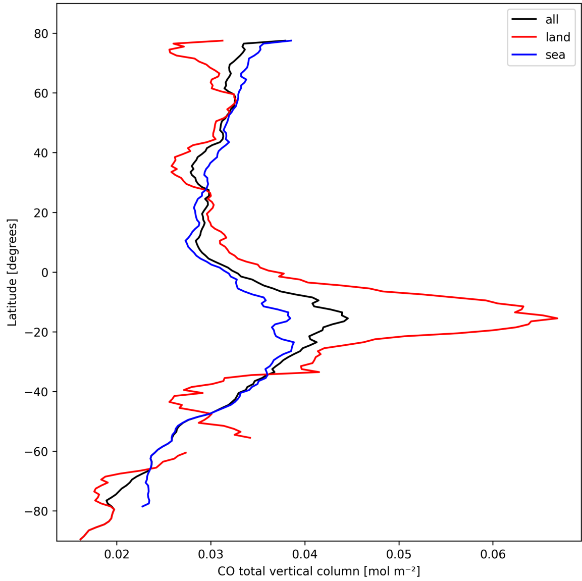
Figure 10: Zonal average of “CO total vertical column” for 2024-10-12 to 2024-10-14.
