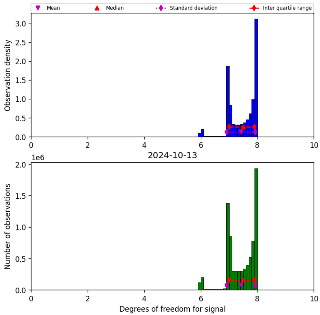
Figure 23: Histogram of “Degrees of freedom for signal” for 2024-10-12 to 2024-10-14
