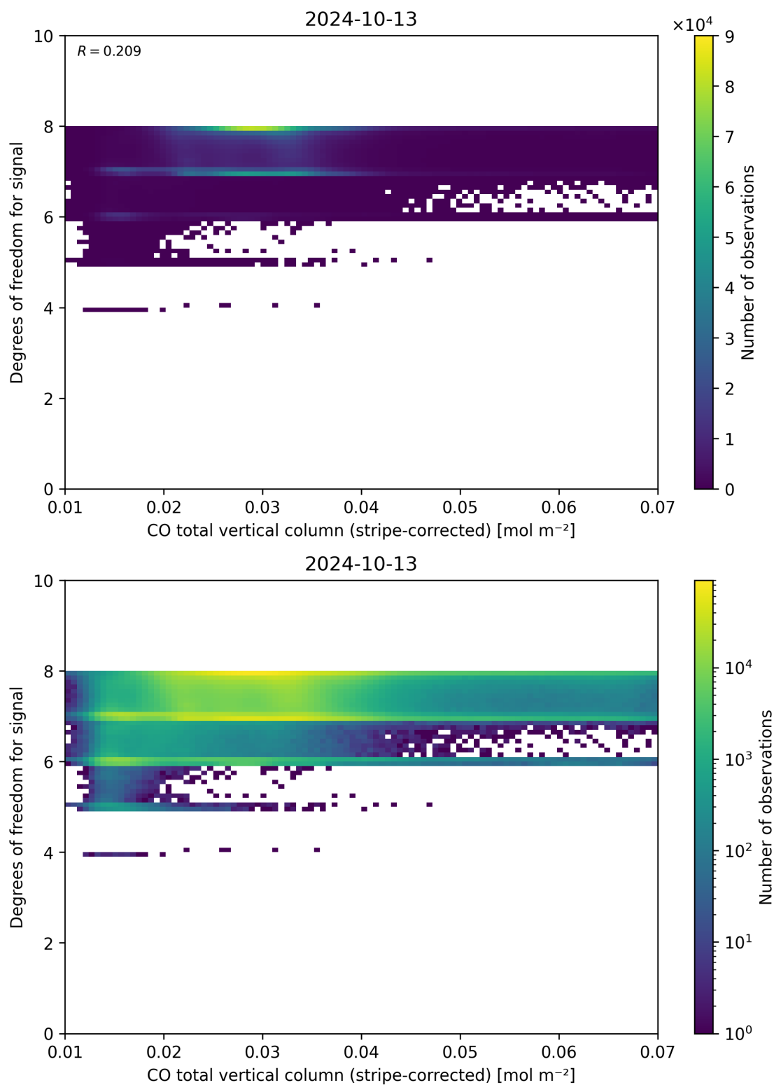
Figure 38: Scatter density plot of “CO total vertical column (stripe-corrected)” against “Degrees of freedom for signal” for 2024-10-12 to 2024-10-14.
