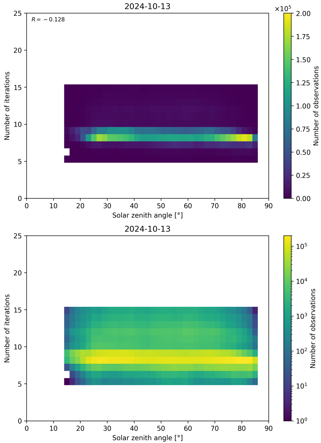
Figure 67: Scatter density plot of “Solar zenith angle” against “Number of iterations” for 2024-10-12 to 2024-10-14.
