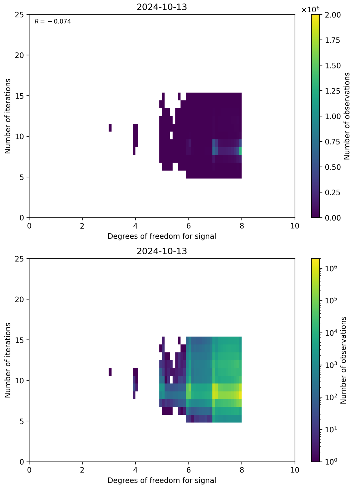
Figure 50: Scatter density plot of “Degrees of freedom for signal” against “Number of iterations” for 2024-10-12 to 2024-10-14.
