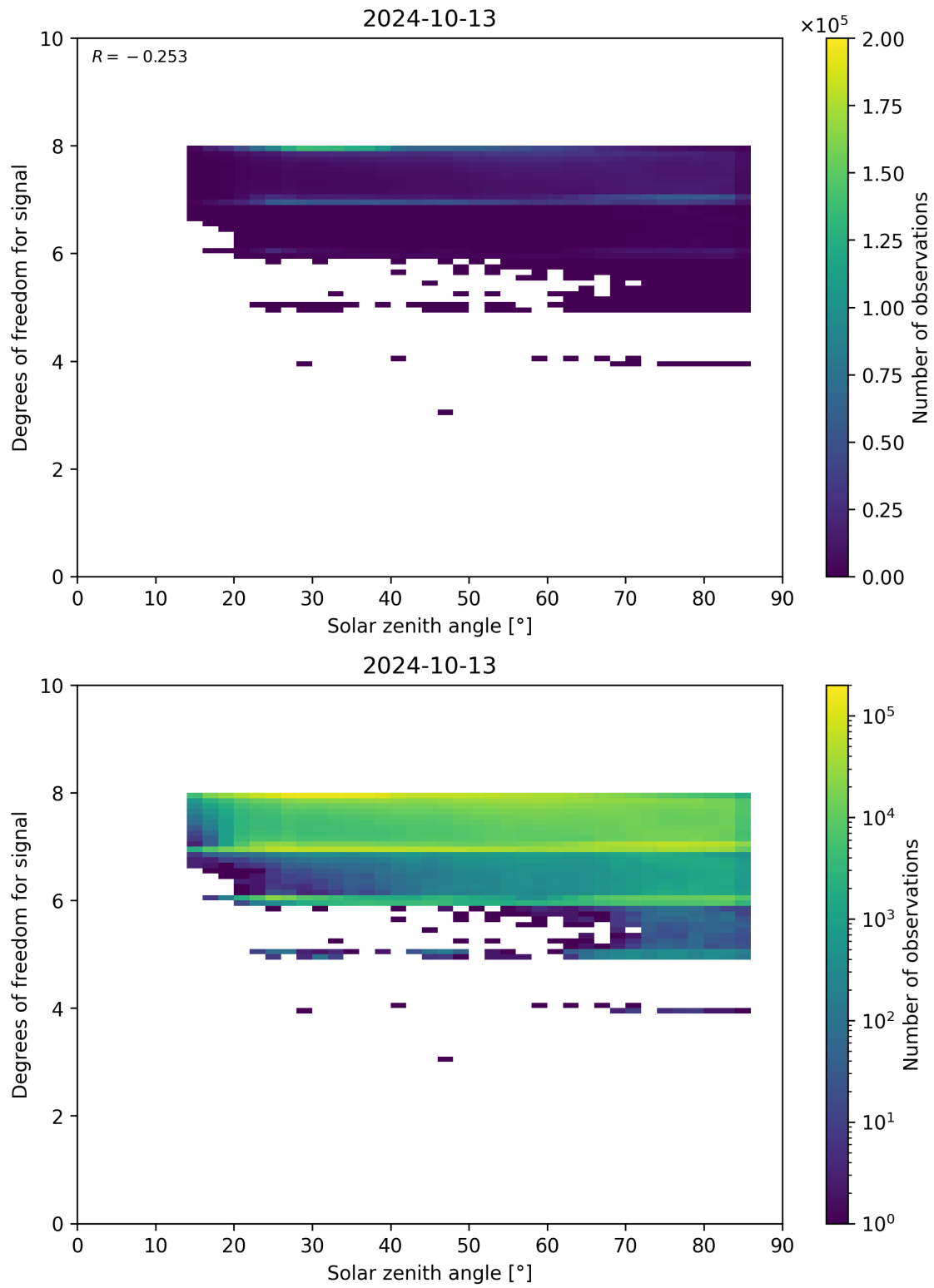
Figure 65: Scatter density plot of “Solar zenith angle” against “Degrees of freedom for signal” for 2024-10-12 to 2024-10-14.
