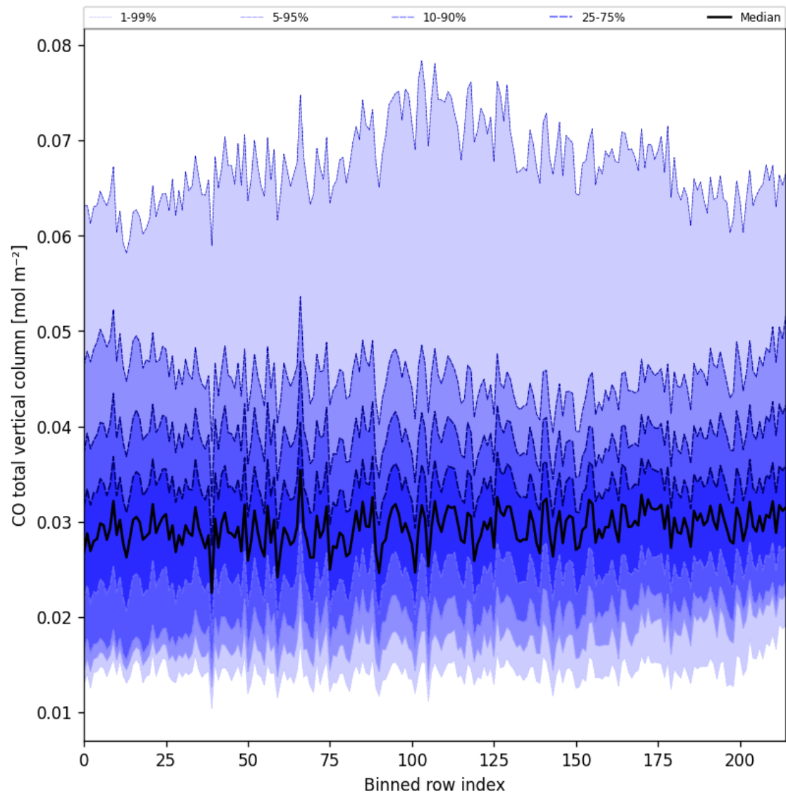
Figure 26: Along track statistics of “CO total vertical column” for 2024-10-12 to 2024-10-14
