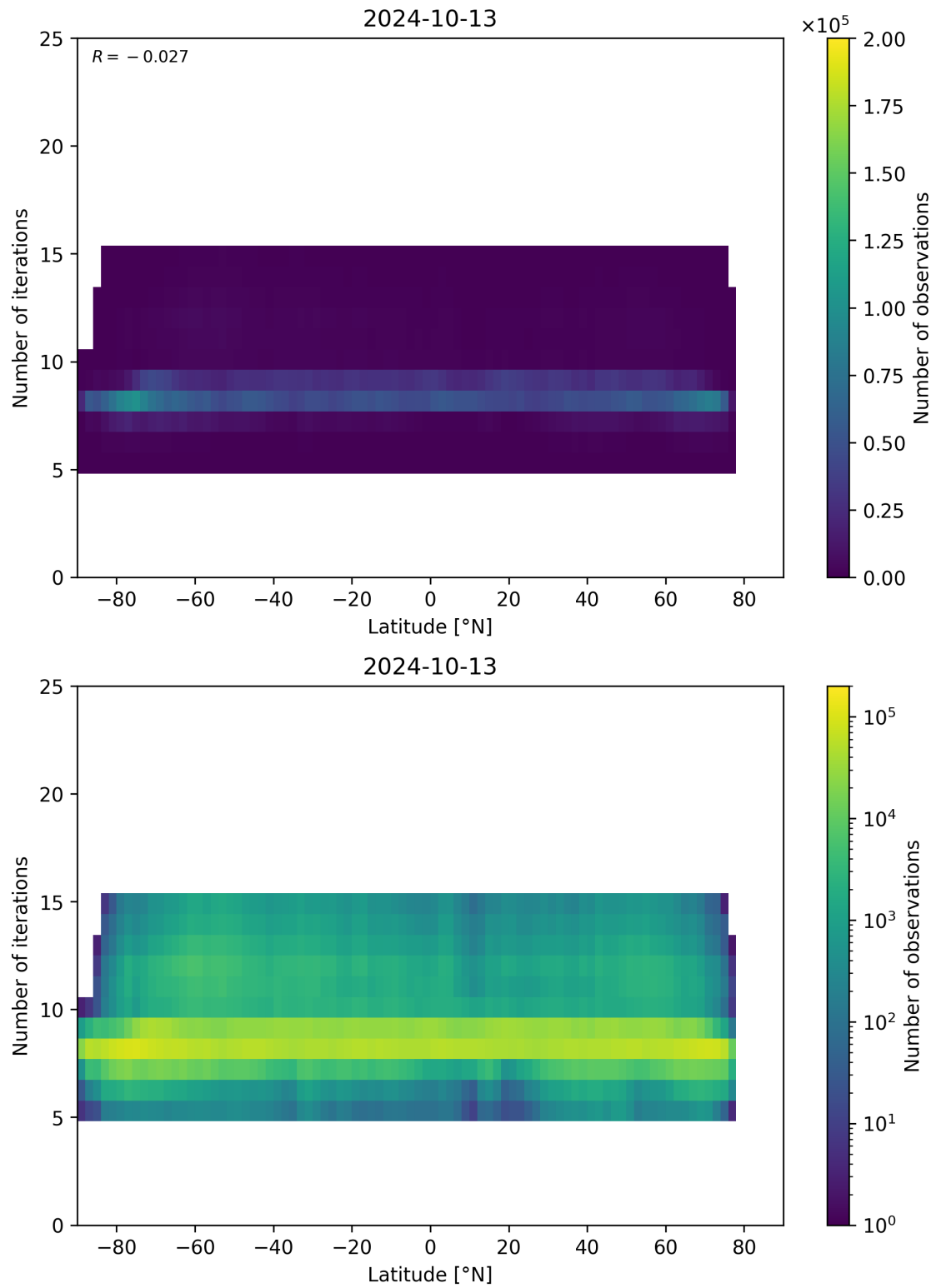
Figure 56: Scatter density plot of “Latitude” against “Number of iterations” for 2024-10-12 to 2024-10-14.
