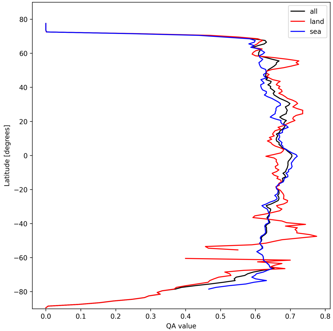
Figure 9: Zonal average of “QA value” for 2024-10-12 to 2024-10-14.
