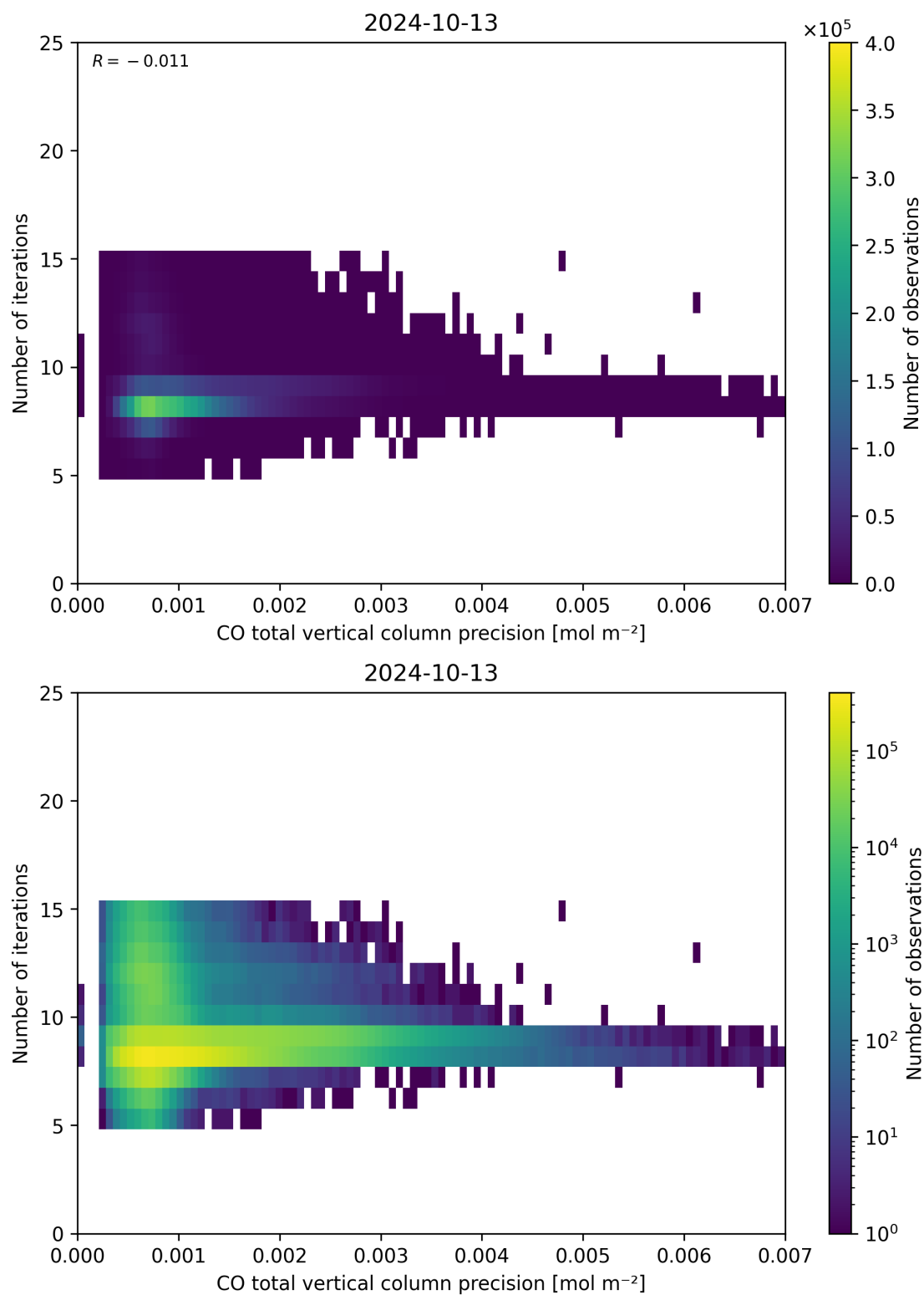
Figure 46: Scatter density plot of “CO total vertical column precision” against “Number of iterations” for 2024-10-12 to 2024-10-14.
