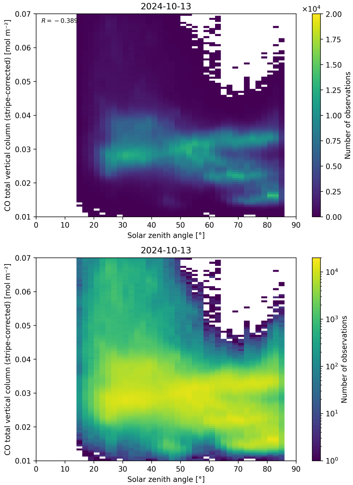
Figure 62: Scatter density plot of “Solar zenith angle” against “CO total vertical column (stripe-corrected)” for 2024-10-12 to 2024-10-14.
