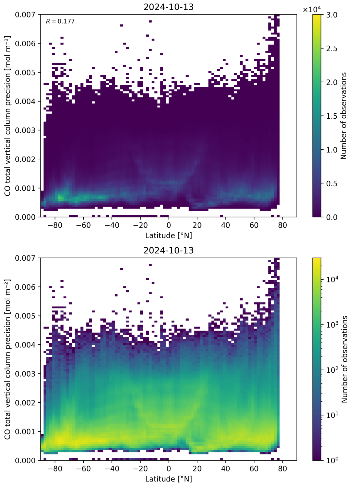
Figure 53: Scatter density plot of “Latitude” against “CO total vertical column precision” for 2024-10-12 to 2024-10-14.
