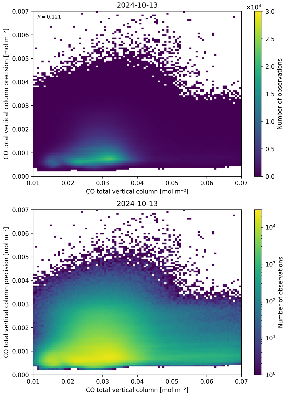
Figure 34: Scatter density plot of “CO total vertical column” against “CO total vertical column precision” for 2024-10-12 to 2024-10-14.
