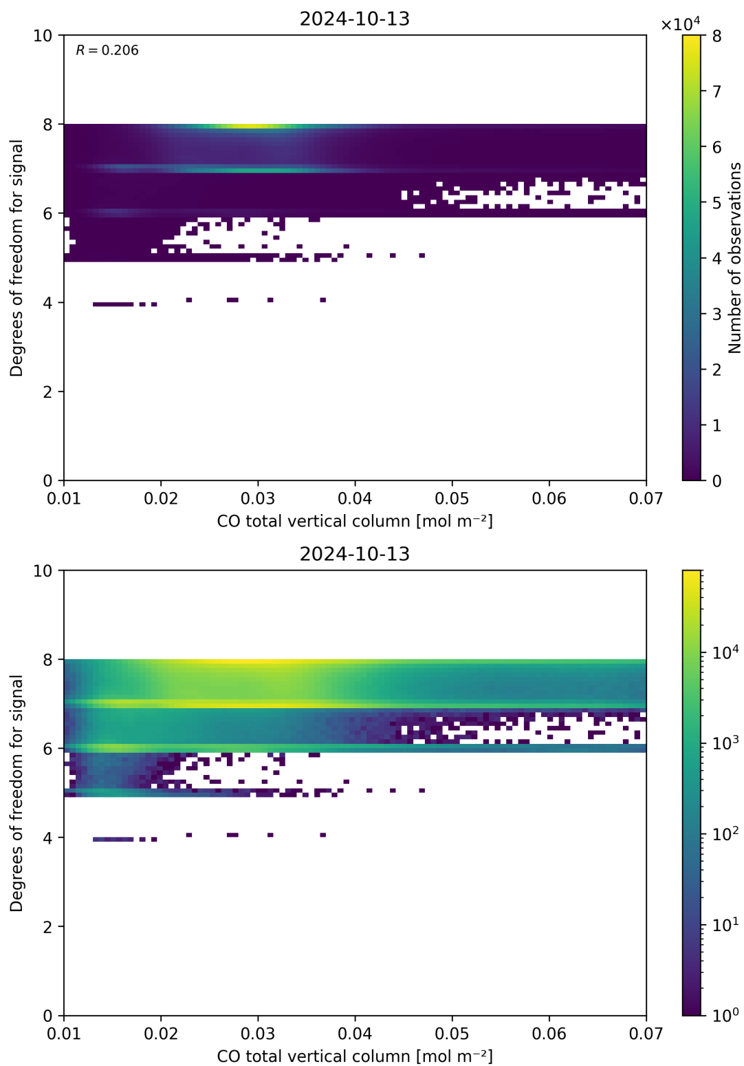
Figure 41: Scatter density plot of “CO total vertical column” against “Degrees of freedom for signal” for 2024-10-12 to 2024-10-14.
