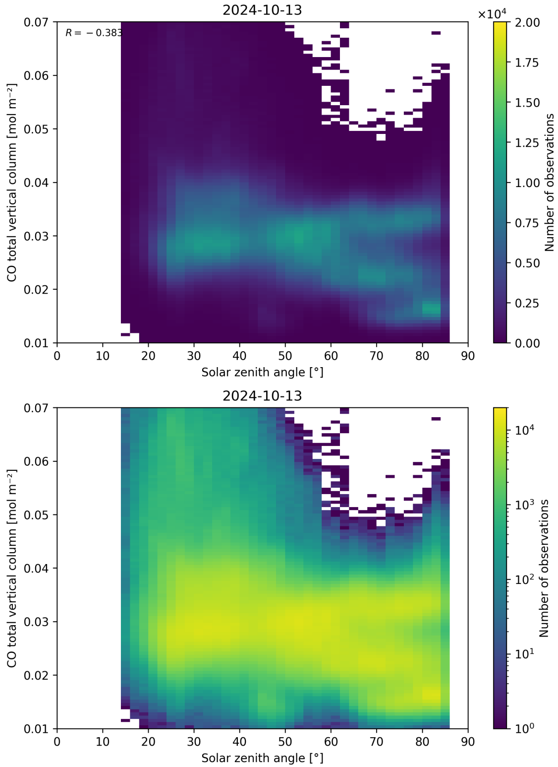
Figure 61: Scatter density plot of “Solar zenith angle” against “CO total vertical column” for 2024-10-12 to 2024-10-14.
