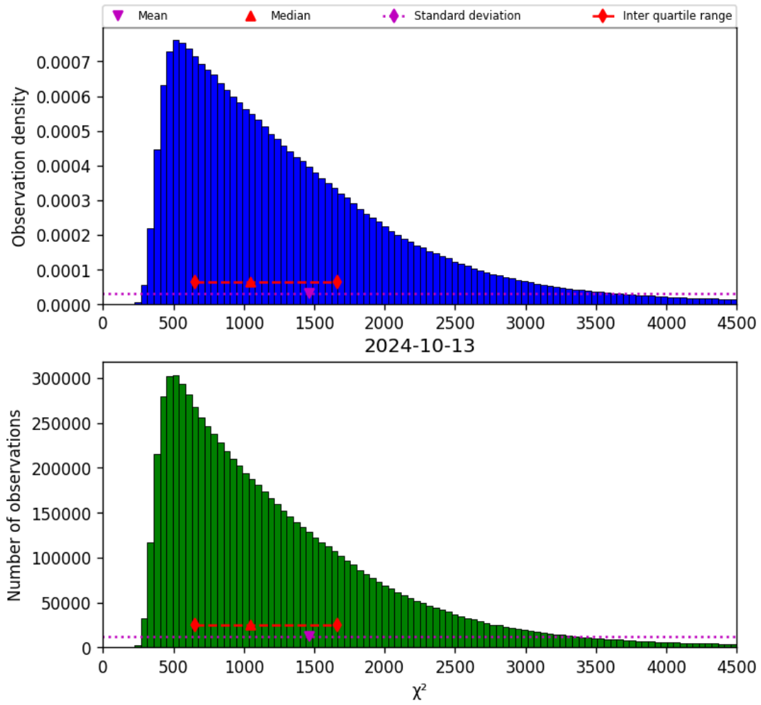
Figure 22: Histogram of “ \chi^2 ” for 2024-10-12 to 2024-10-14
