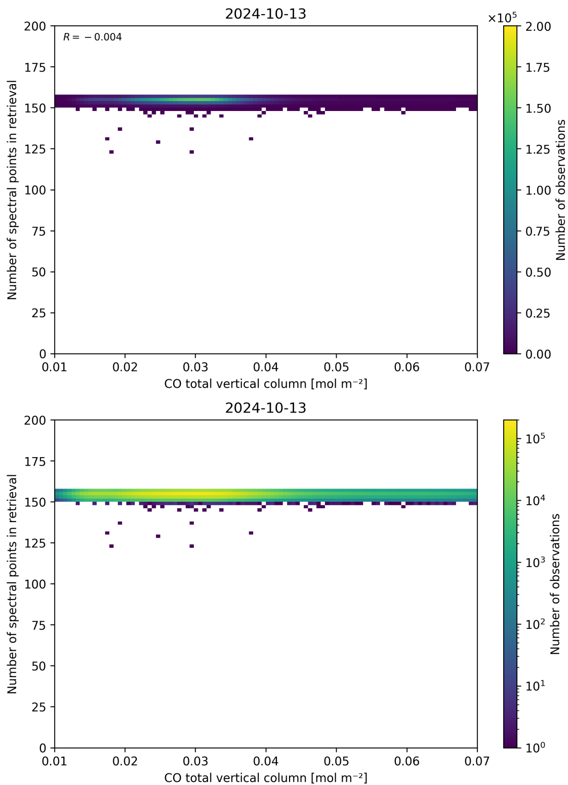
Figure 43: Scatter density plot of “CO total vertical column” against “Number of spectral points in retrieval” for 2024-10-12 to 2024-10-14.
