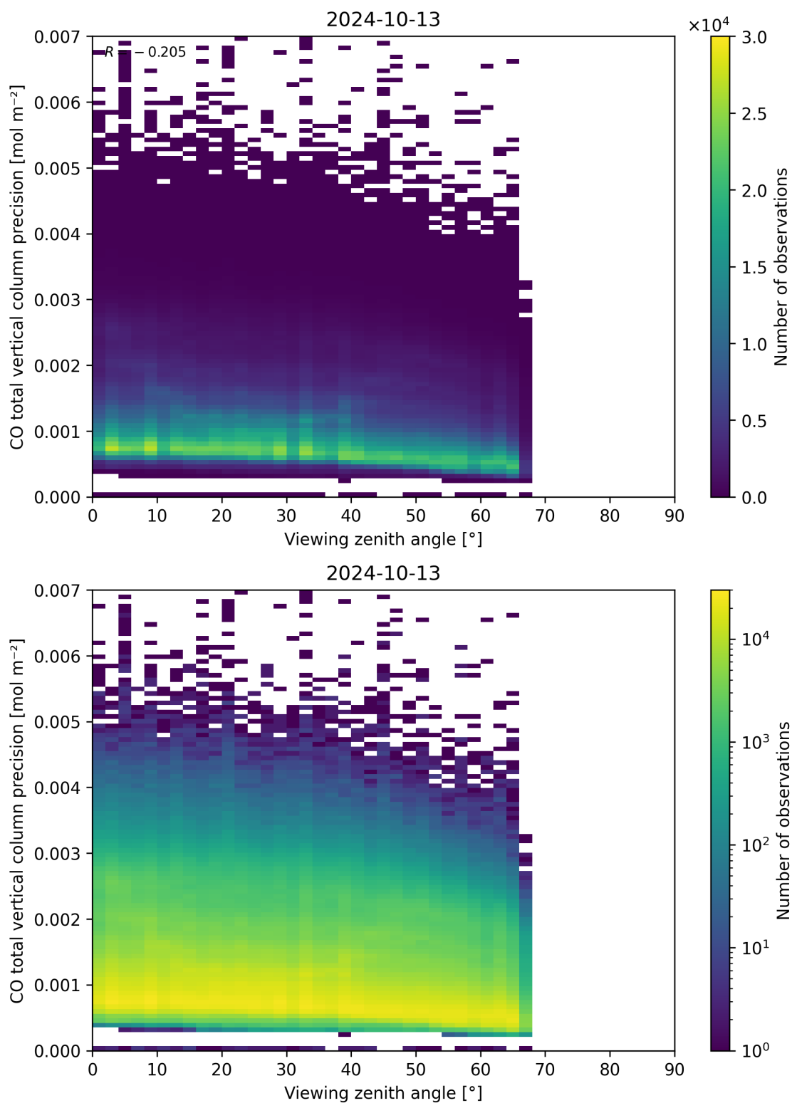
Figure 71: Scatter density plot of “Viewing zenith angle” against “CO total vertical column precision” for 2024-10-12 to 2024-10-14.
