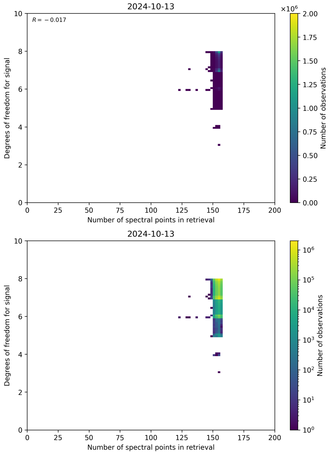
Figure 59: Scatter density plot of “Number of spectral points in retrieval” against “Degrees of freedom for signal” for 2024-10-12 to 2024-10-14.
