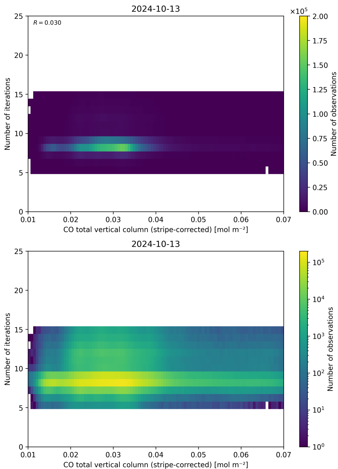
Figure 39: Scatter density plot of “CO total vertical column (stripe-corrected)” against “Number of iterations” for 2024-10-12 to 2024-10-14.
