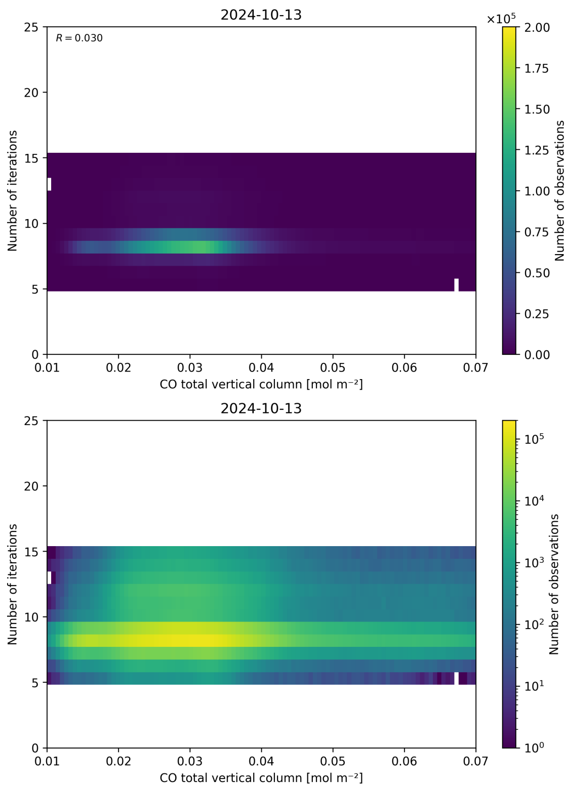
Figure 42: Scatter density plot of “CO total vertical column” against “Number of iterations” for 2024-10-12 to 2024-10-14.
