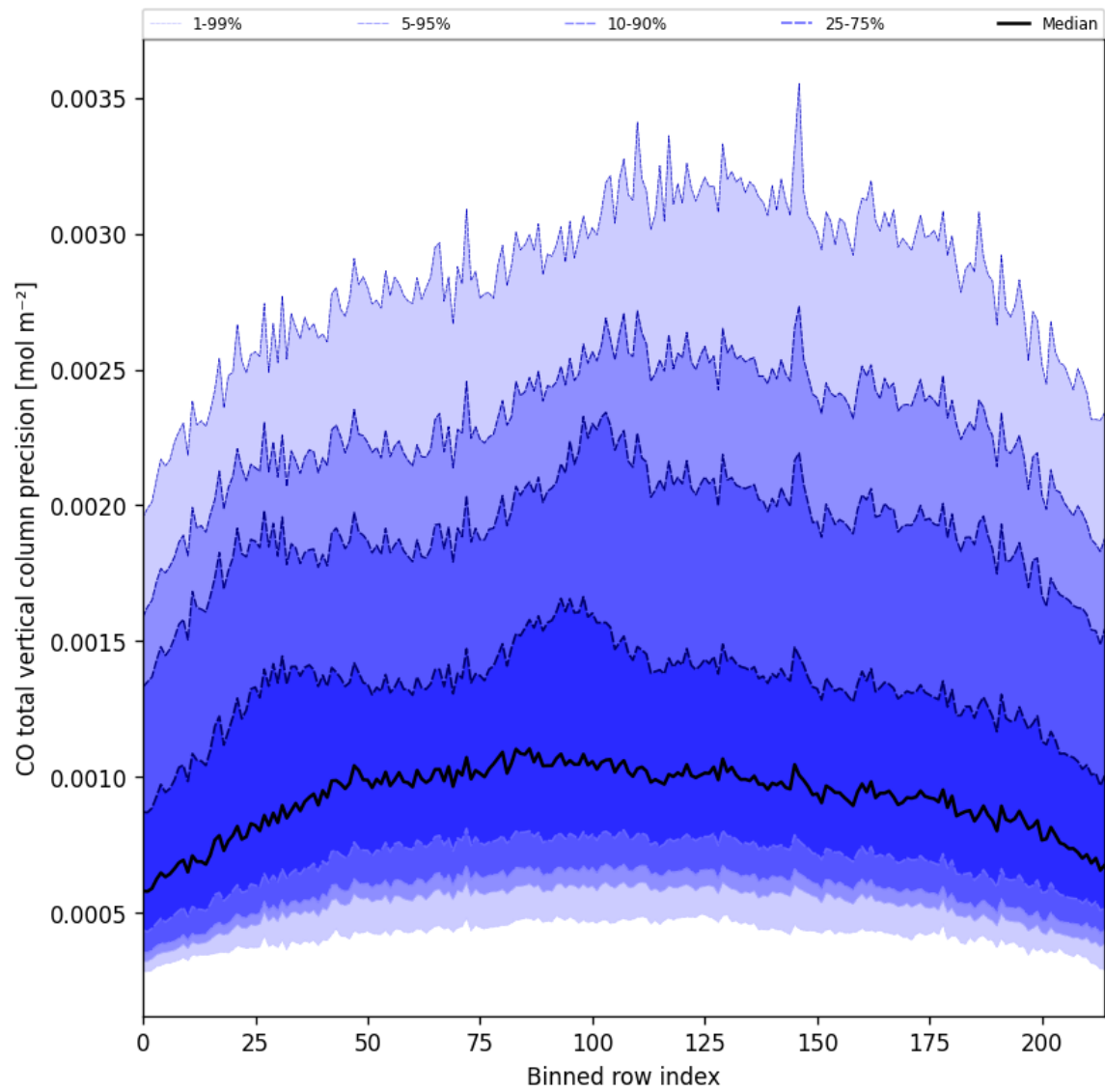
Figure 28: Along track statistics of “CO total vertical column precision” for 2024-10-12 to 2024-10-14
