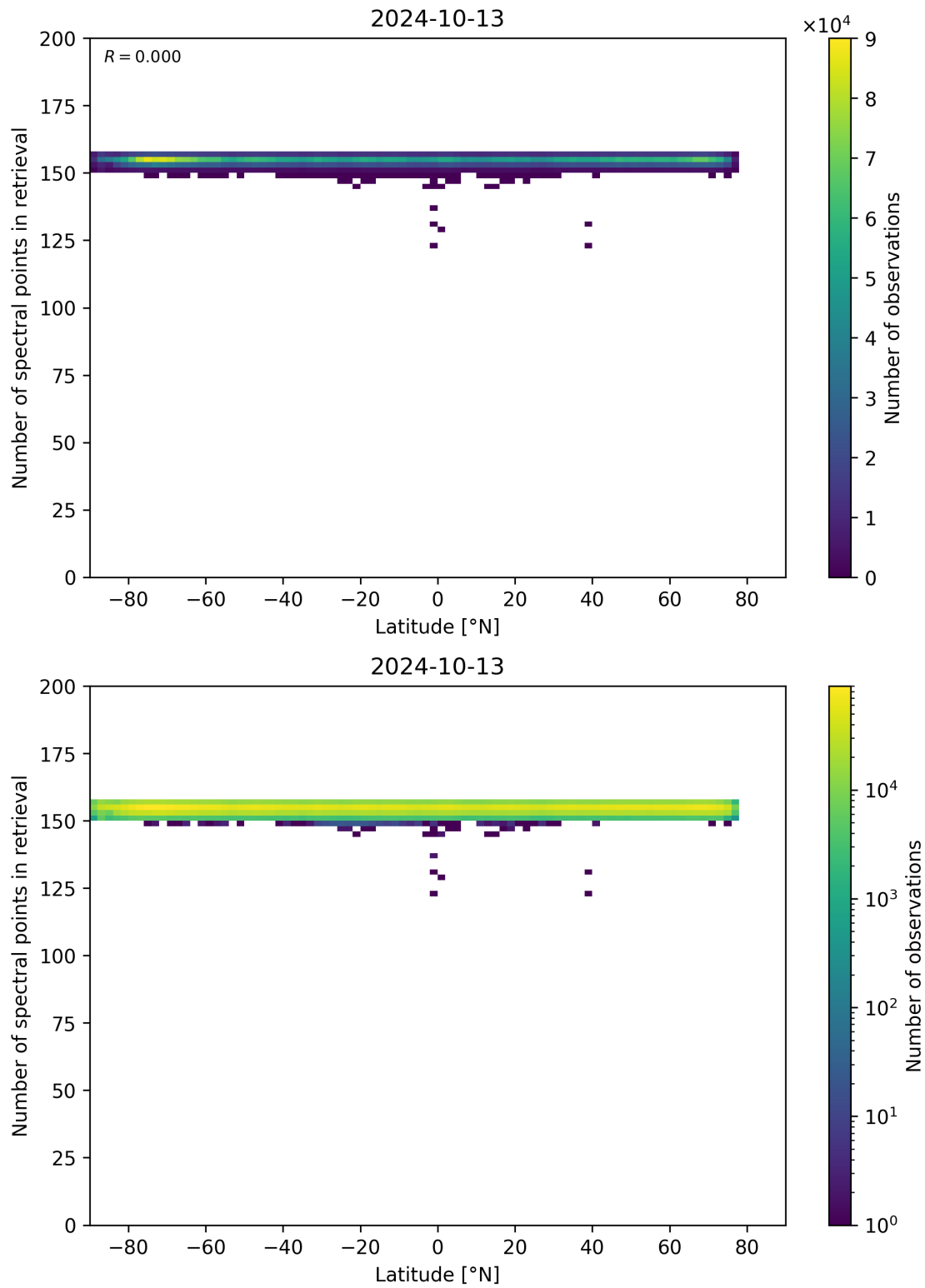
Figure 57: Scatter density plot of “Latitude” against “Number of spectral points in retrieval” for 2024-10-12 to 2024-10-14.
