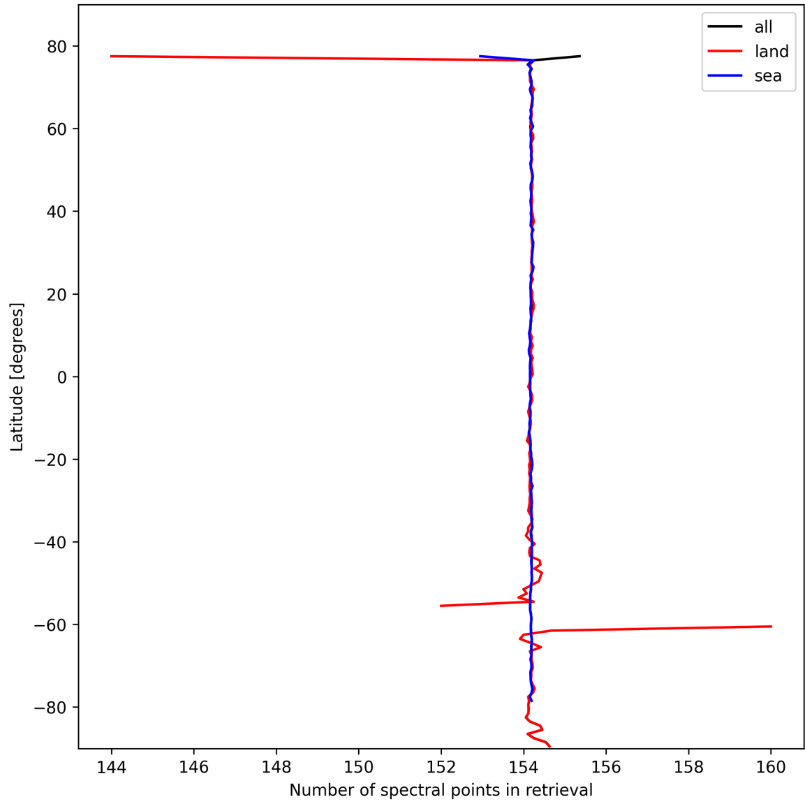
Figure 13: Zonal average of “Number of spectral points in retrieval” for 2024-10-12 to 2024-10-14.
