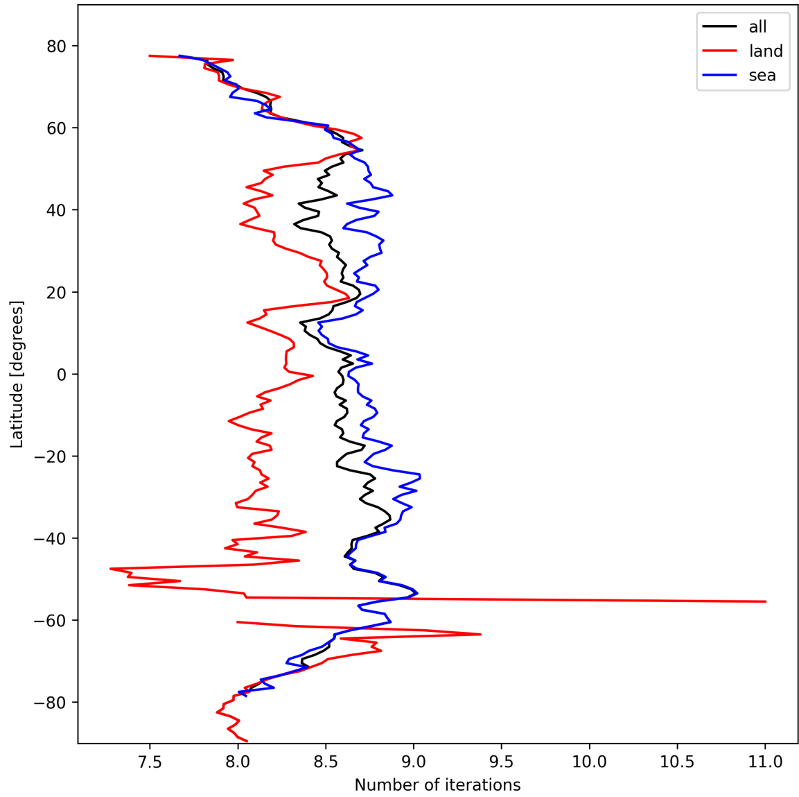
Figure 16: Zonal average of “Number of iterations” for 2024-10-12 to 2024-10-14.
