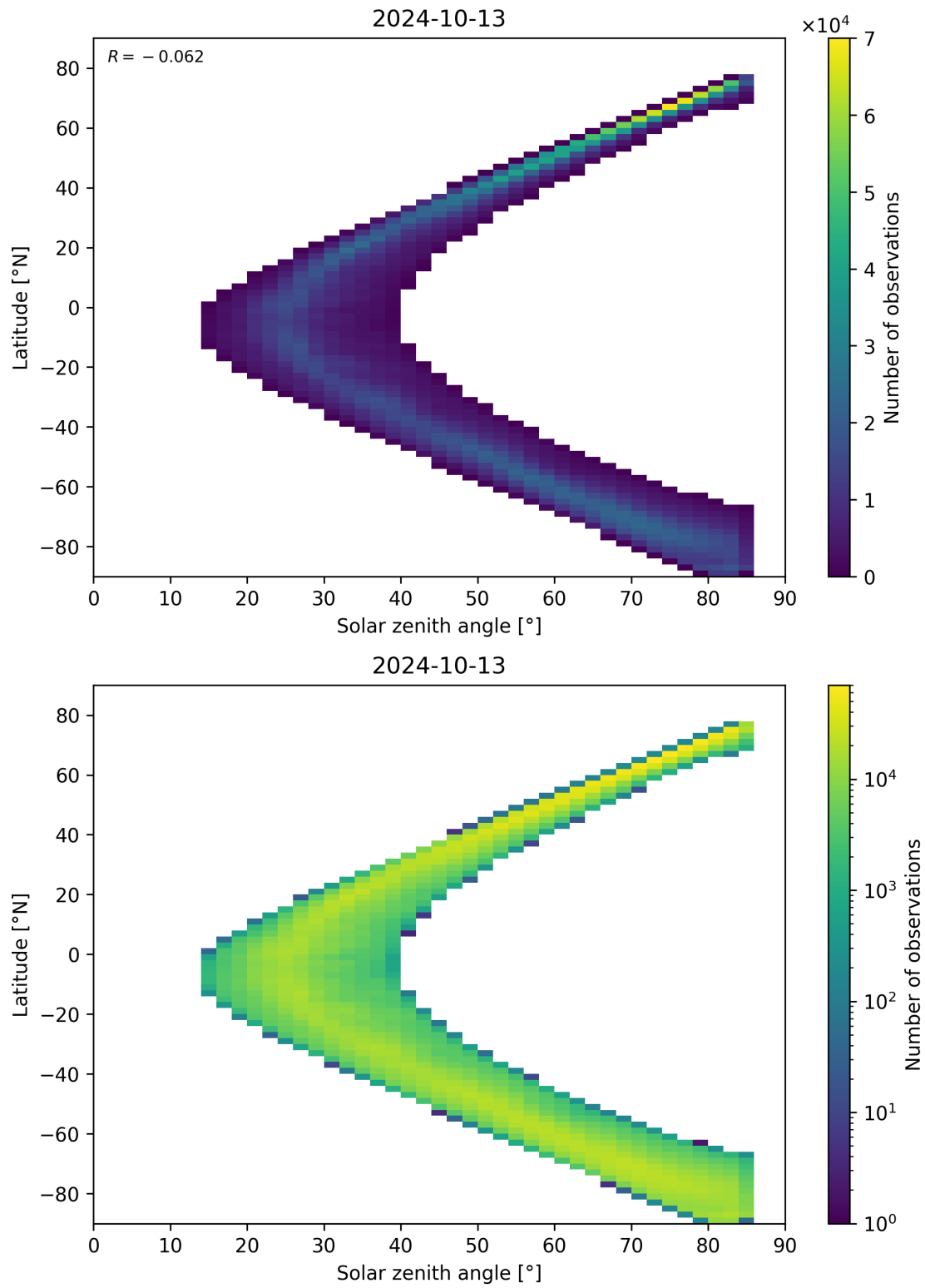
Figure 66: Scatter density plot of “Solar zenith angle” against “Latitude” for 2024-10-12 to 2024-10-14.
