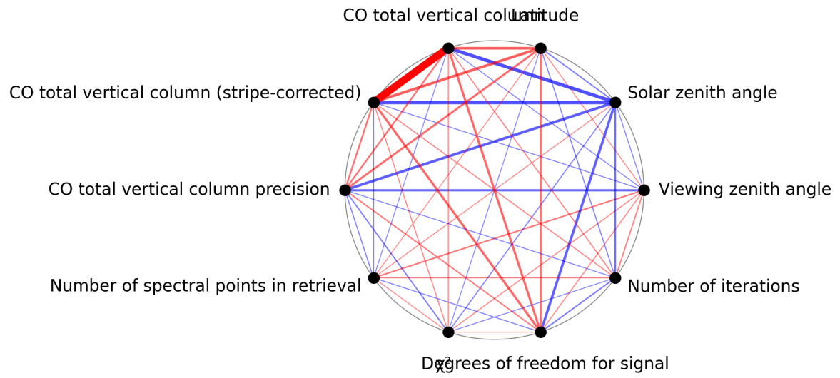
Figure 1: Map of correlation graph for 2024-10-12 to 2024-10-14.
