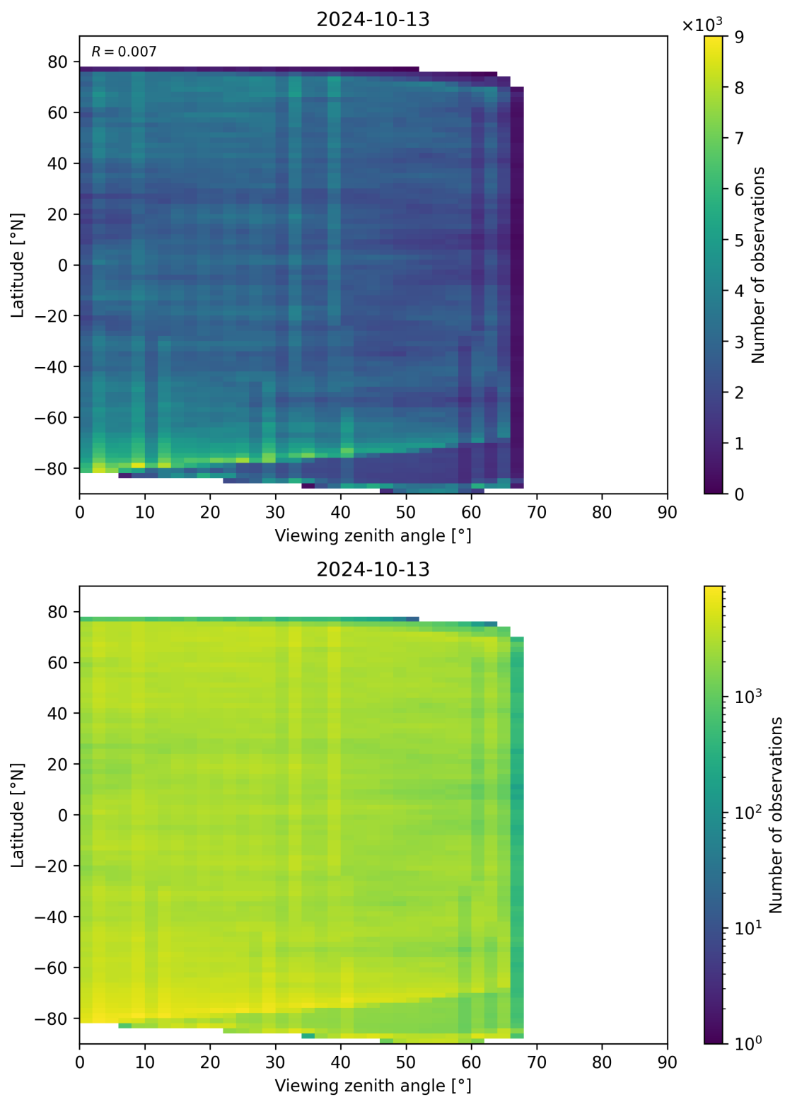
Figure 74: Scatter density plot of “Viewing zenith angle” against “Latitude” for 2024-10-12 to 2024-10-14.
