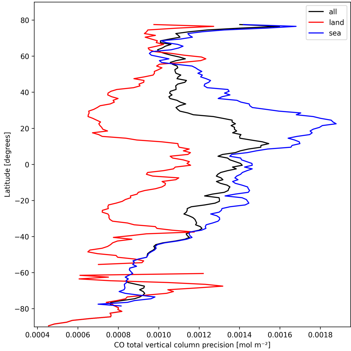
Figure 12: Zonal average of “CO total vertical column precision” for 2024-10-12 to 2024-10-14.
