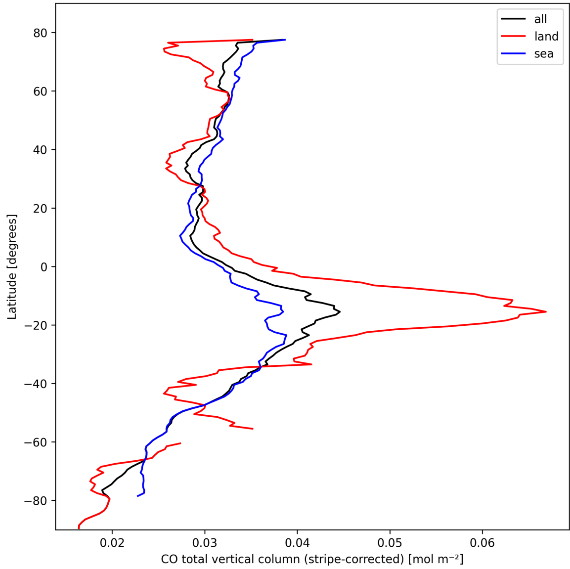
Figure 11: Zonal average of “CO total vertical column (stripe-corrected)” for 2024-10-12 to 2024-10-14.
