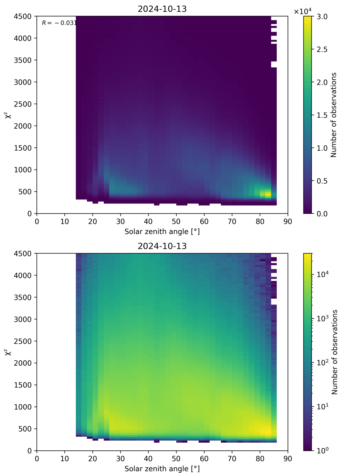
Figure 64: Scatter density plot of “Solar zenith angle” against “ \chi^2 ” for 2024-10-12 to 2024-10-14.
