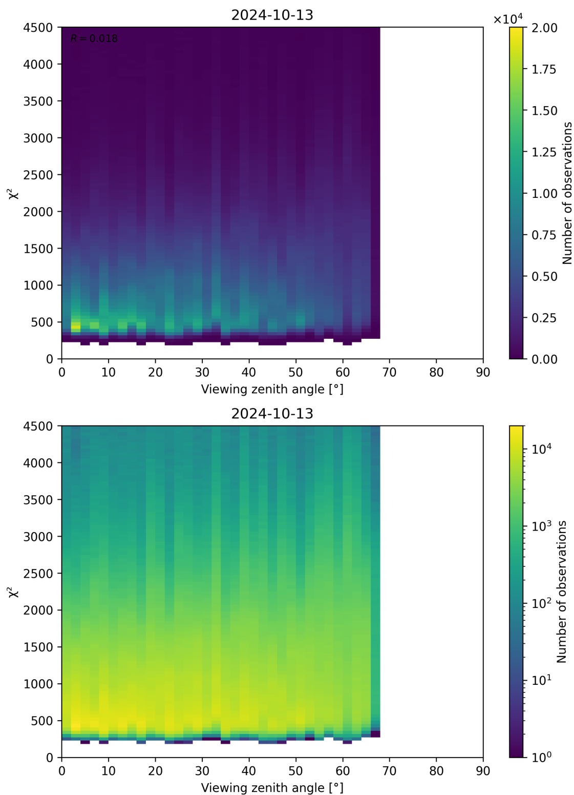
Figure 72: Scatter density plot of “Viewing zenith angle” against “ \chi^2 ” for 2024-10-12 to 2024-10-14.
