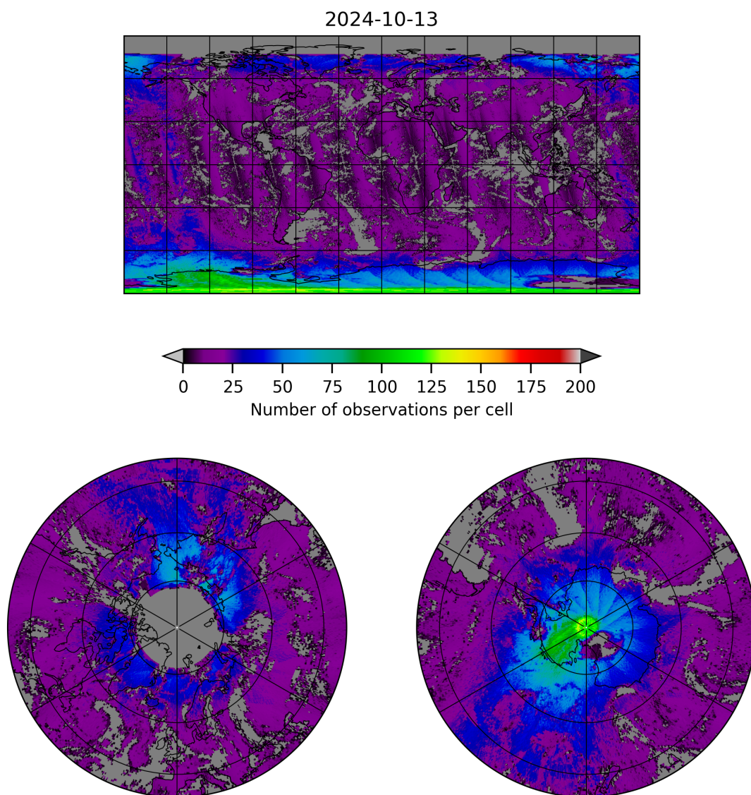
Figure 8: Map of the number of observations for 2024-10-12 to 2024-10-14
