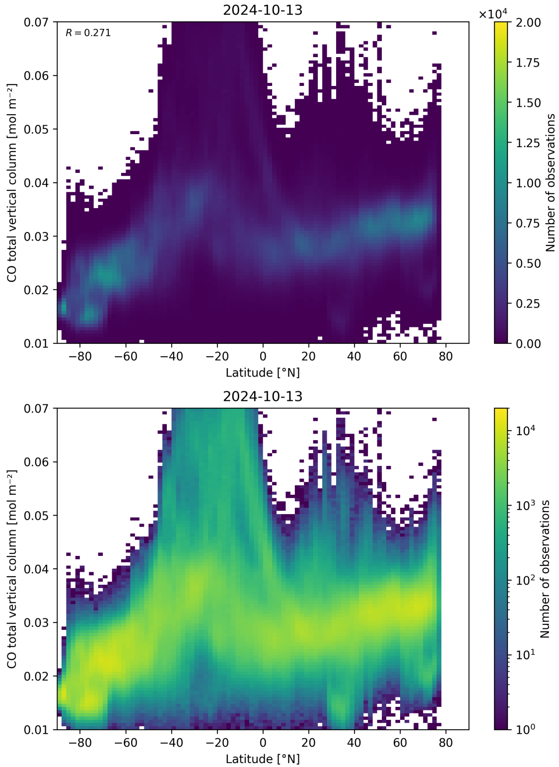
Figure 51: Scatter density plot of “Latitude” against “CO total vertical column” for 2024-10-12 to 2024-10-14.
