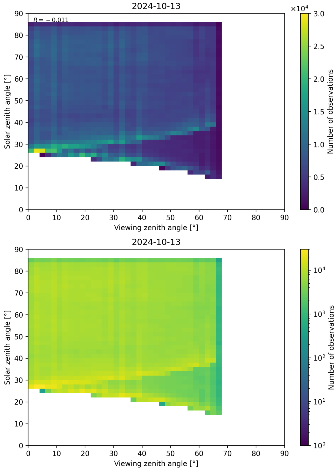
Figure 77: Scatter density plot of “Viewing zenith angle” against “Solar zenith angle” for 2024-10-12 to 2024-10-14.
