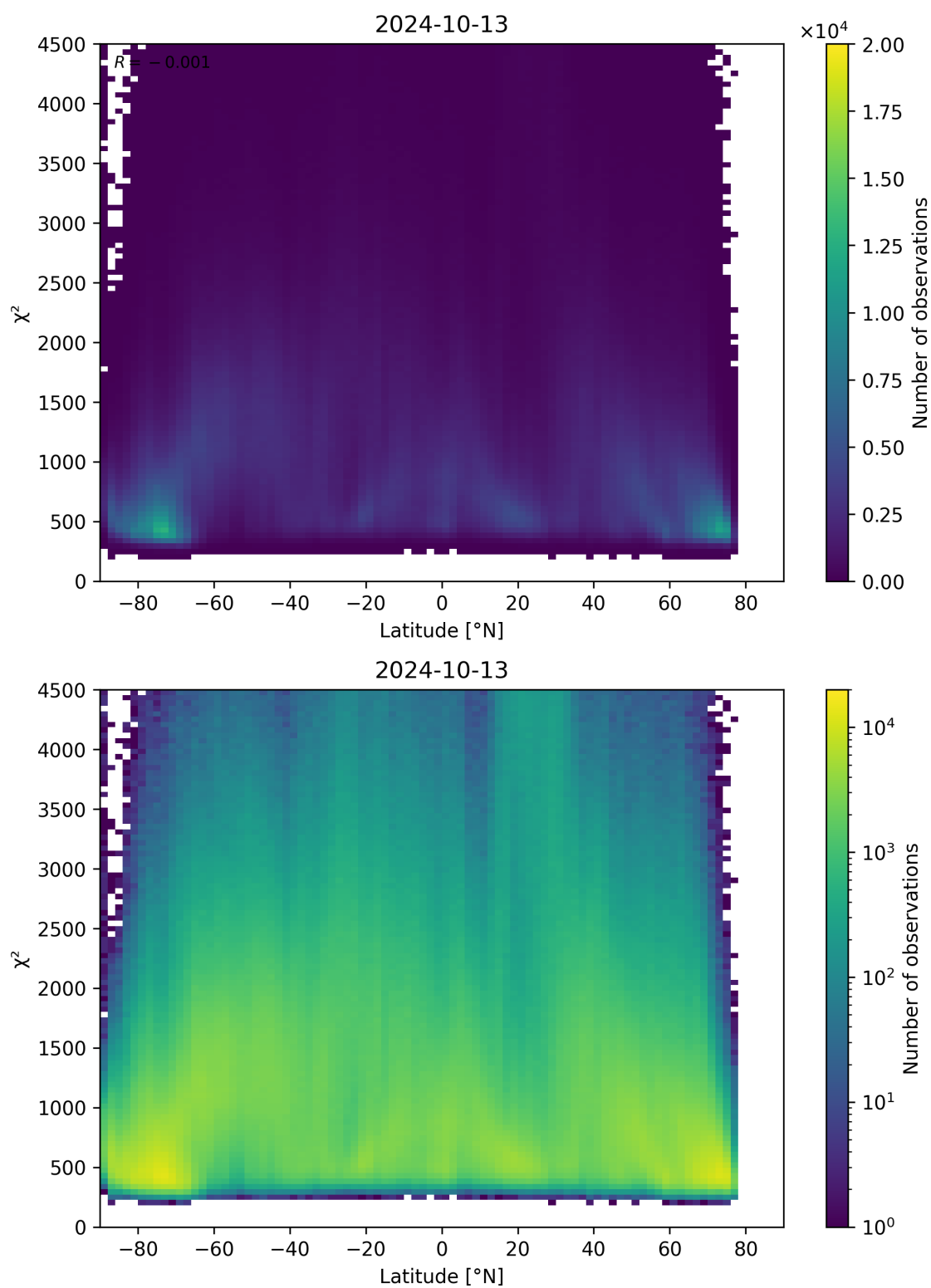
Figure 54: Scatter density plot of “Latitude” against “ \chi^2 ” for 2024-10-12 to 2024-10-14.
