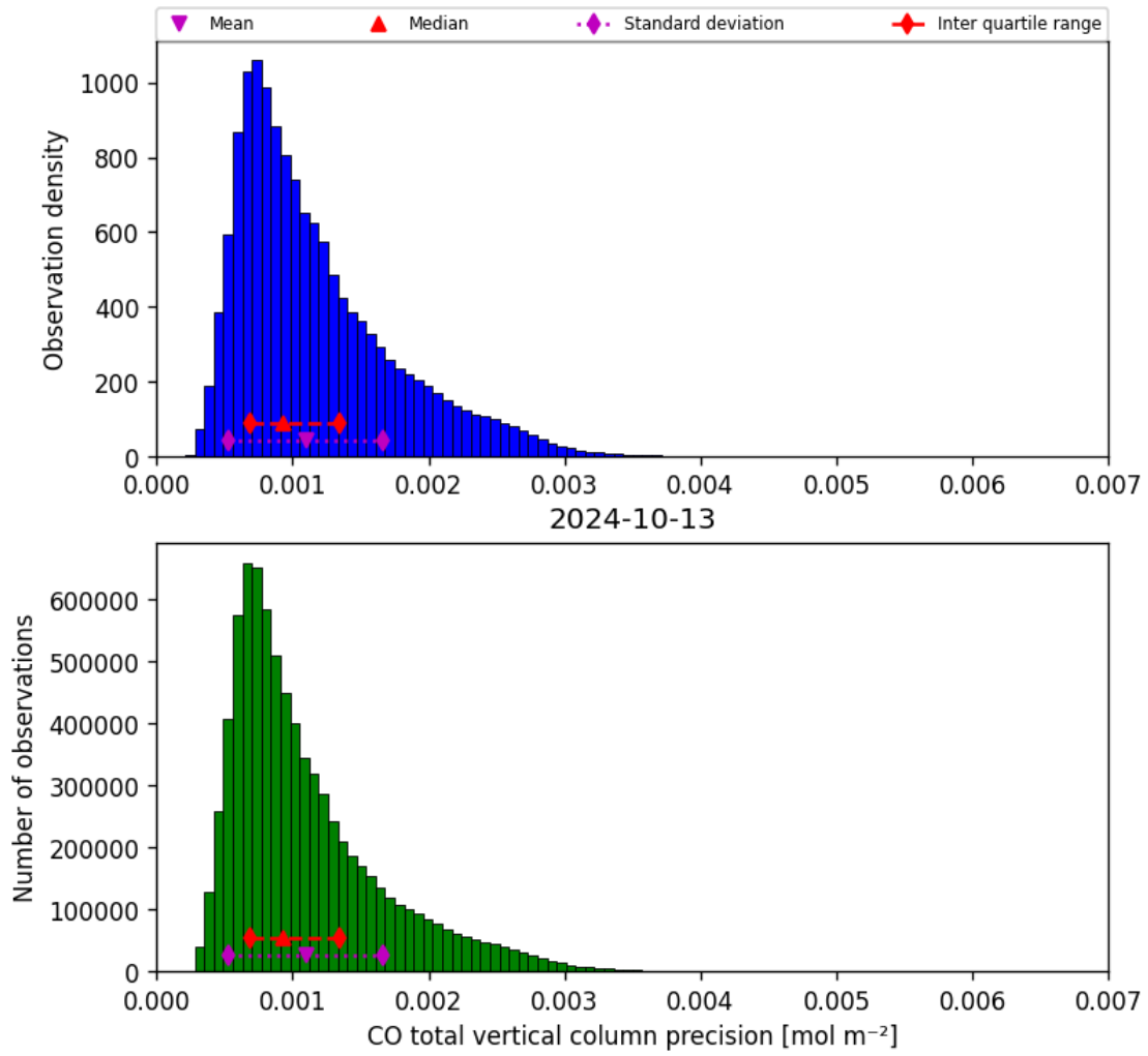
Figure 20: Histogram of “CO total vertical column precision” for 2024-10-12 to 2024-10-14
