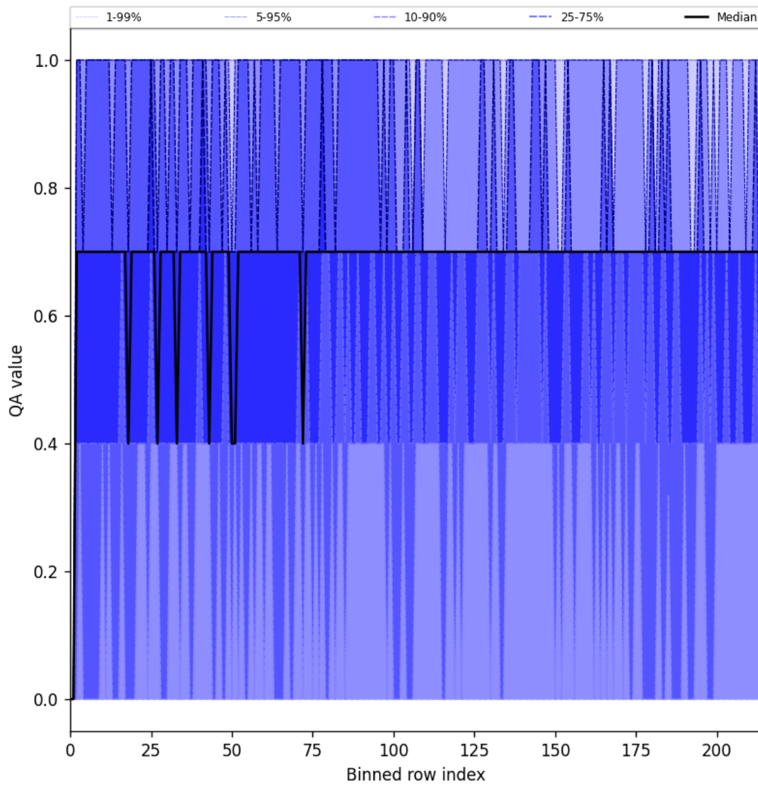
Figure 25: Along track statistics of “QA value” for 2024-10-12 to 2024-10-14
