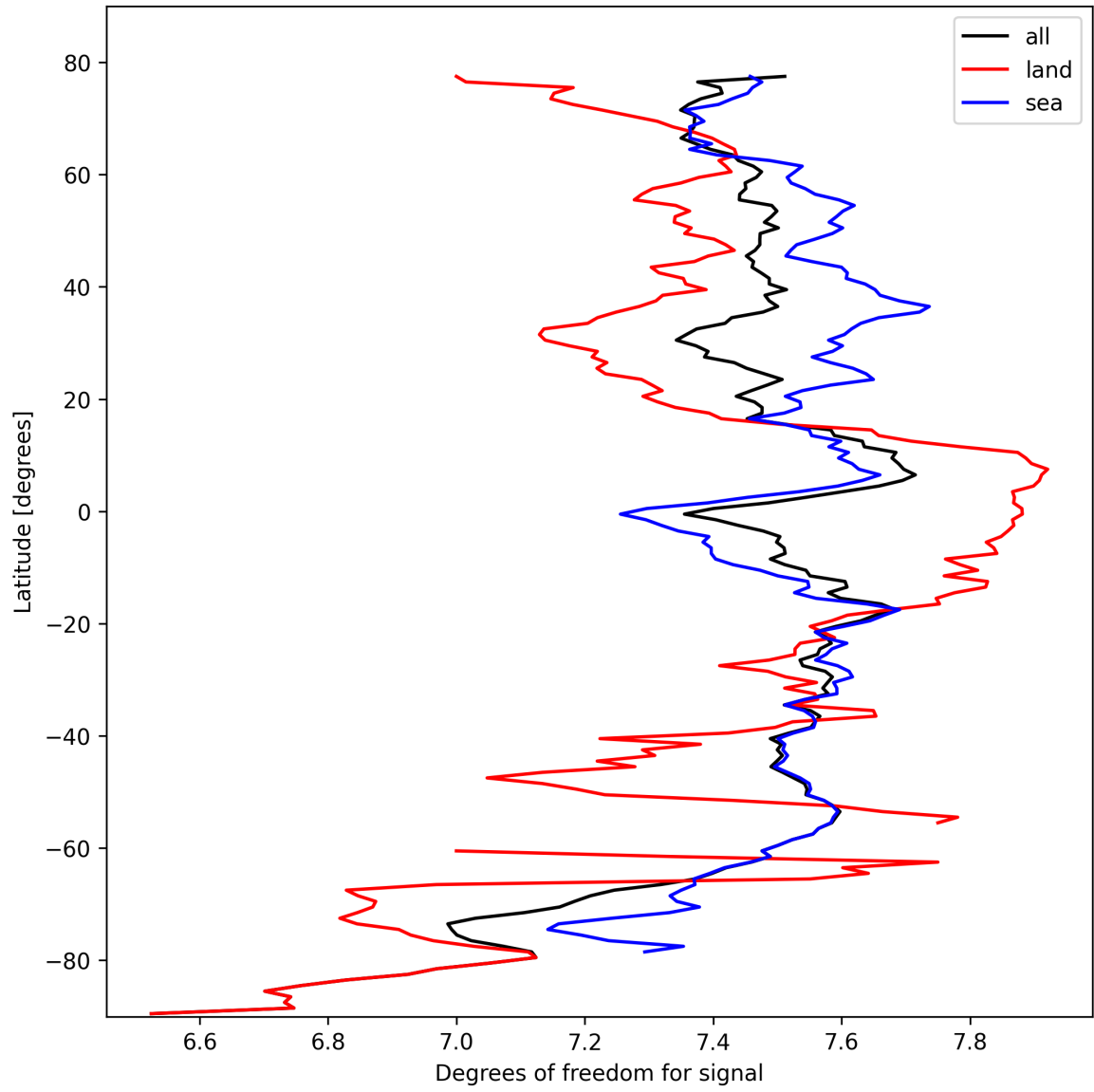
Figure 15: Zonal average of “Degrees of freedom for signal” for 2024-10-12 to 2024-10-14.
