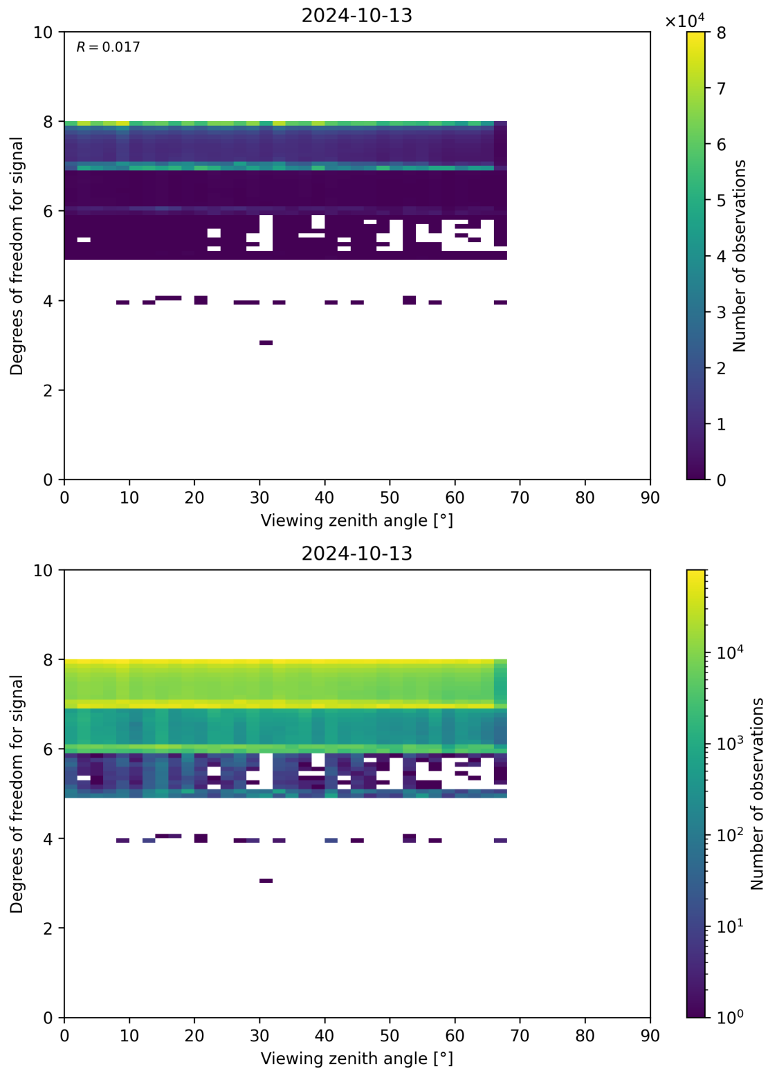
Figure 73: Scatter density plot of “Viewing zenith angle” against “Degrees of freedom for signal” for 2024-10-12 to 2024-10-14.
