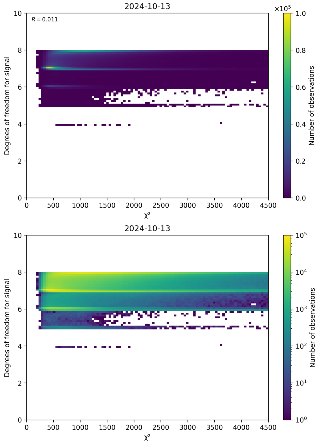
Figure 48: Scatter density plot of “ \chi^2 ” against “Degrees of freedom for signal” for 2024-10-12 to 2024-10-14.
