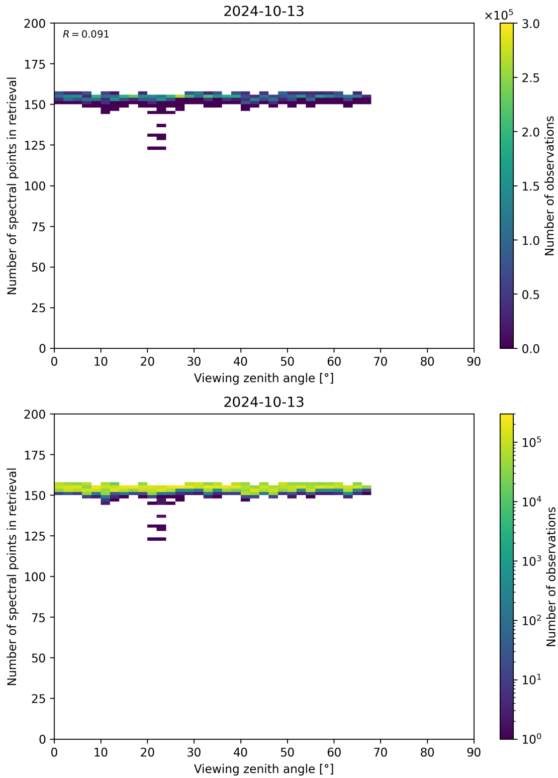
Figure 76: Scatter density plot of “Viewing zenith angle” against “Number of spectral points in retrieval” for 2024-10-12 to 2024-10-14.
