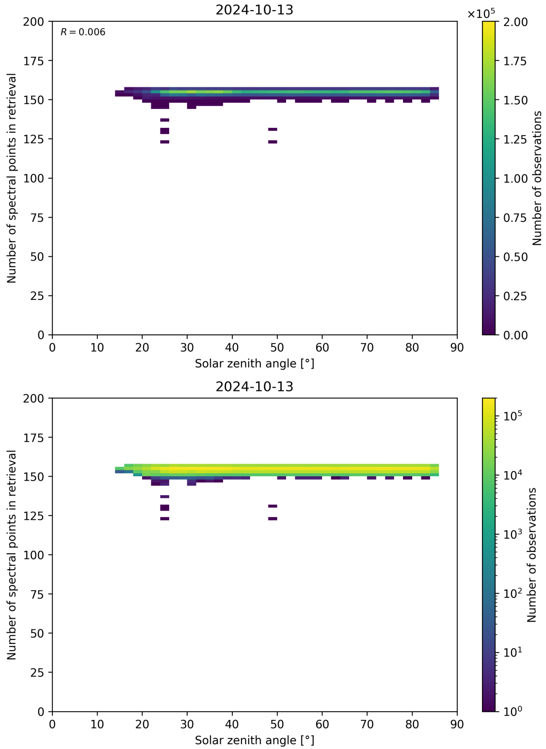
Figure 68: Scatter density plot of “Solar zenith angle” against “Number of spectral points in retrieval” for 2024-10-12 to 2024-10-14.
