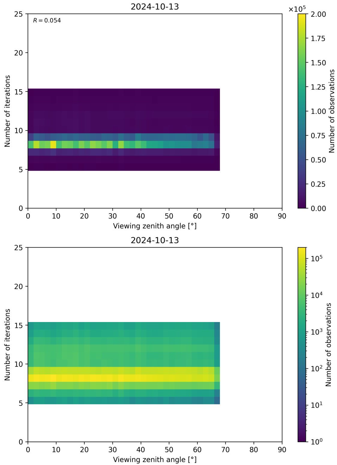
Figure 75: Scatter density plot of “Viewing zenith angle” against “Number of iterations” for 2024-10-12 to 2024-10-14.
