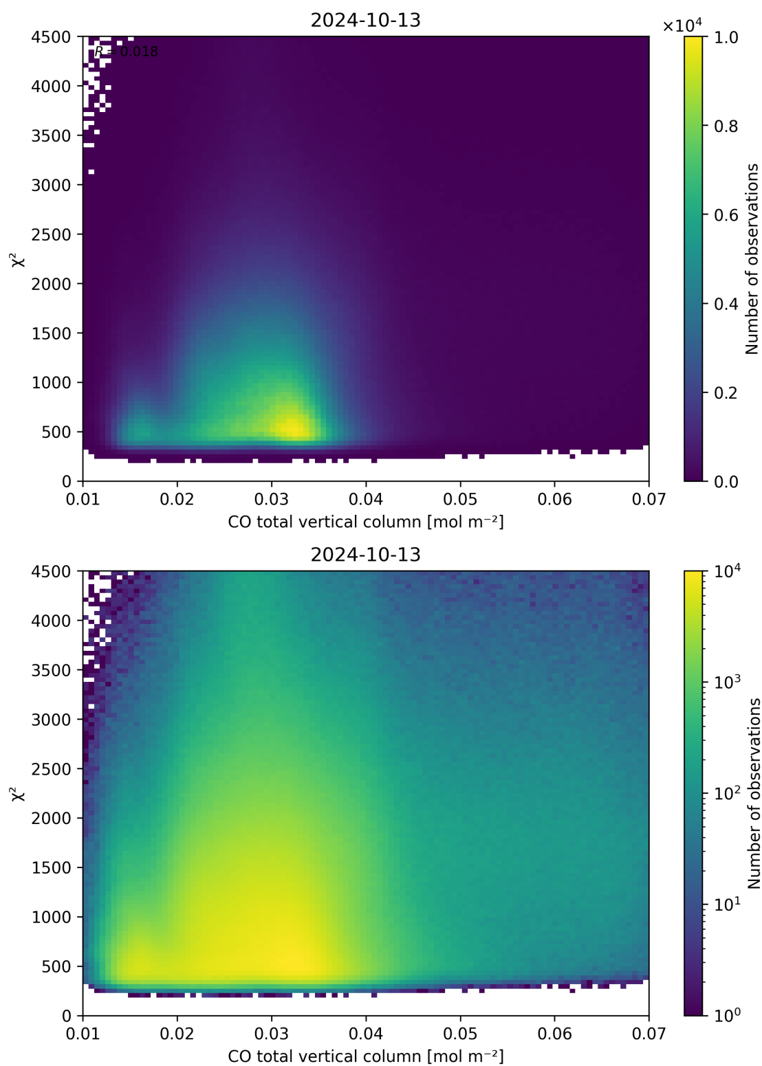
Figure 35: Scatter density plot of “CO total vertical column” against “ \chi^2 ” for 2024-10-12 to 2024-10-14.
