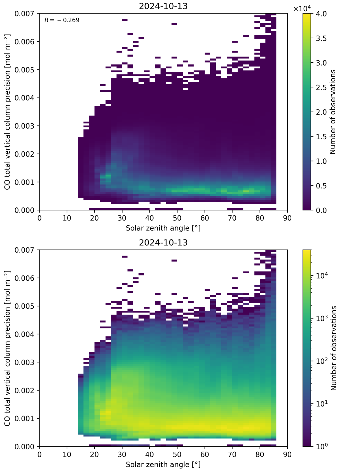
Figure 63: Scatter density plot of “Solar zenith angle” against “CO total vertical column precision” for 2024-10-12 to 2024-10-14.
