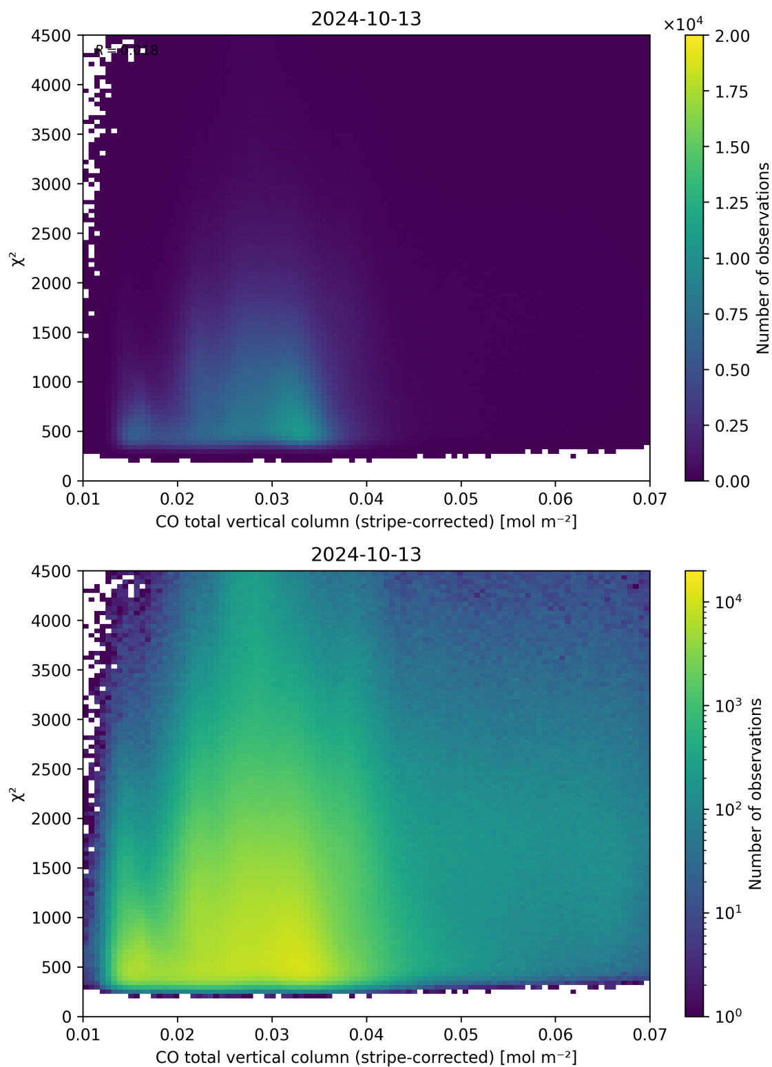
Figure 37: Scatter density plot of “CO total vertical column (stripe-corrected)” against “ \chi^2 ” for 2024-10-12 to 2024-10-14.
