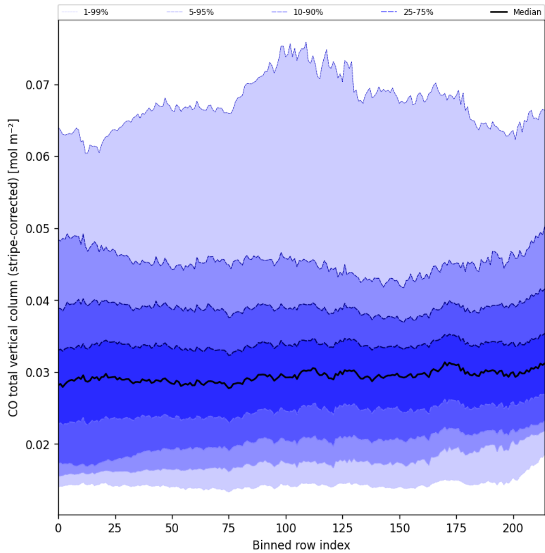
Figure 27: Along track statistics of “CO total vertical column (stripe-corrected)” for 2024-10-12 to 2024-10-14
