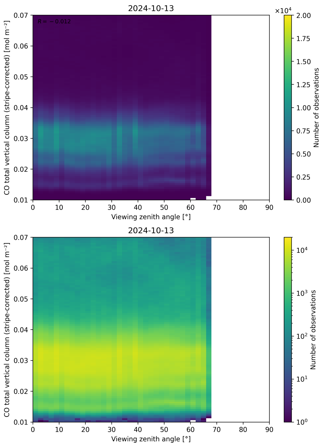
Figure 70: Scatter density plot of “Viewing zenith angle” against “CO total vertical column (stripe-corrected)” for 2024-10-12 to 2024-10-14.
