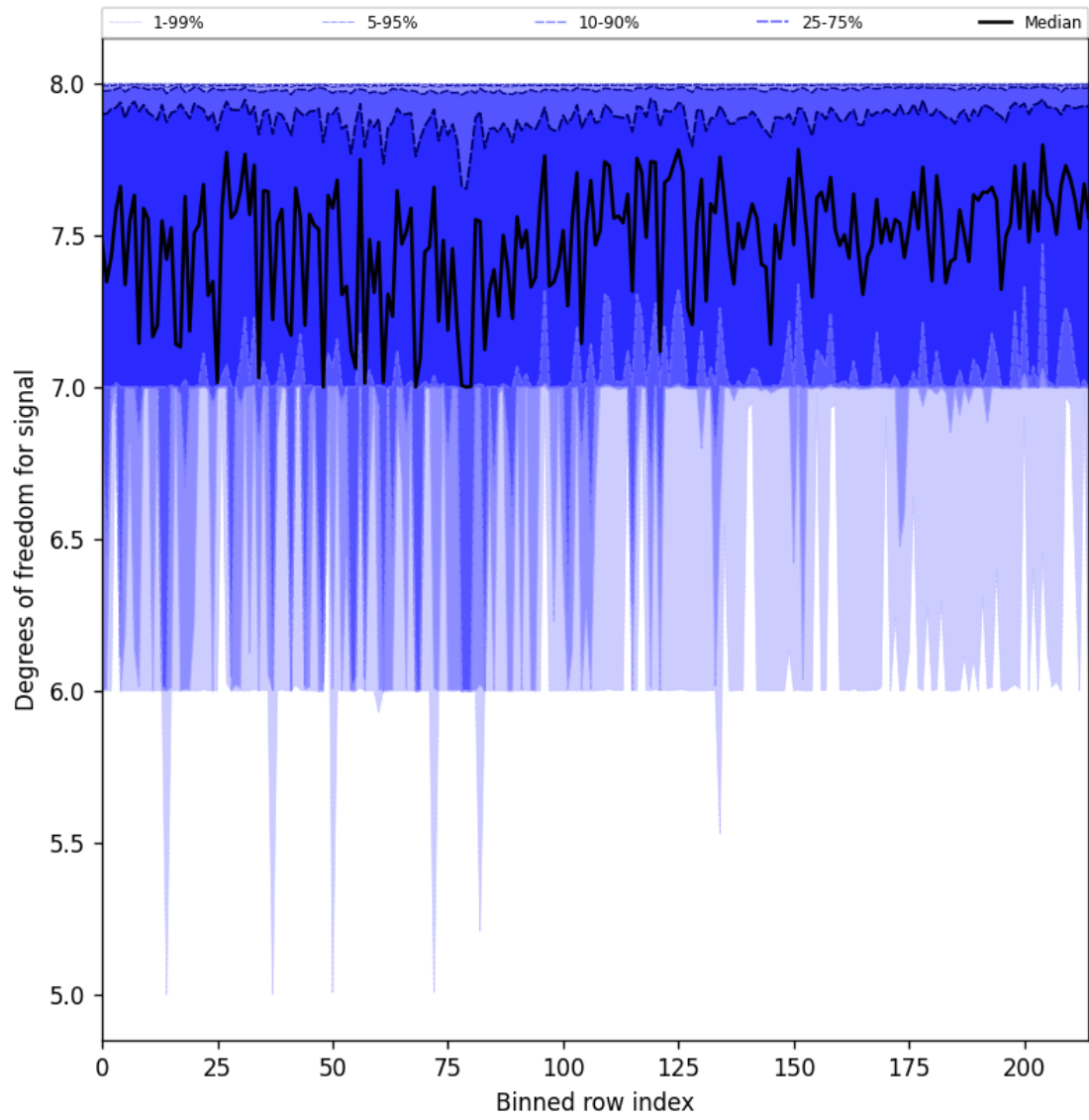
Figure 31: Along track statistics of “Degrees of freedom for signal” for 2024-10-12 to 2024-10-14
