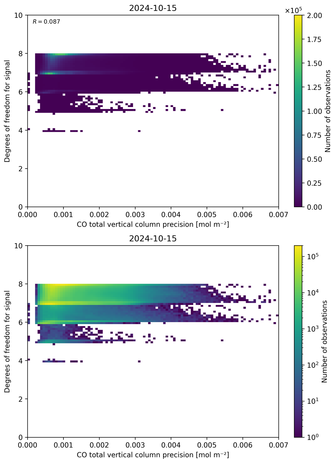
Figure 45: Scatter density plot of “CO total vertical column precision” against “Degrees of freedom for signal” for 2024-10-14 to 2024-10-16.
