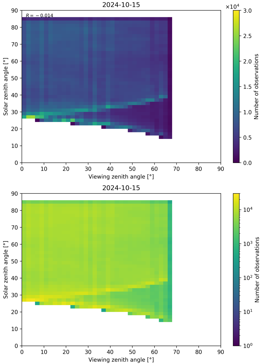
Figure 77: Scatter density plot of “Viewing zenith angle” against “Solar zenith angle” for 2024-10-14 to 2024-10-16.
