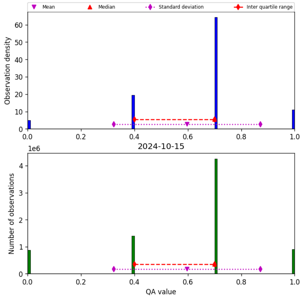
Figure 17: Histogram of “QA value” for 2024-10-14 to 2024-10-16
