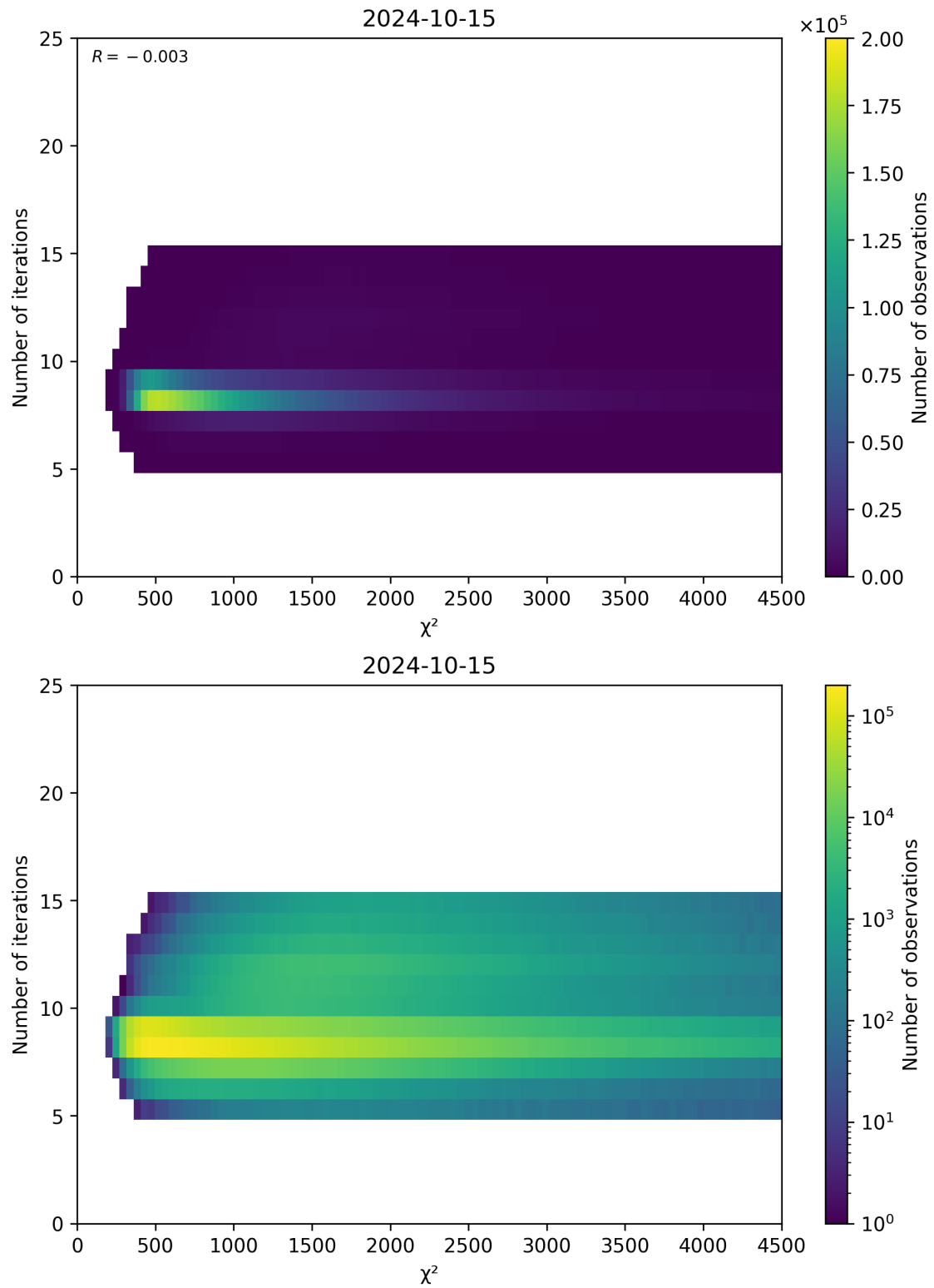
Figure 49: Scatter density plot of “ \chi^2 ” against “Number of iterations” for 2024-10-14 to 2024-10-16.
