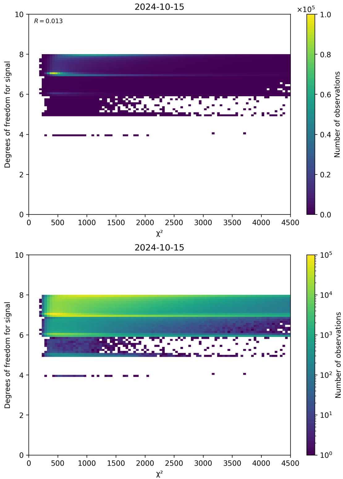
Figure 48: Scatter density plot of “ \chi^2 ” against “Degrees of freedom for signal” for 2024-10-14 to 2024-10-16.
