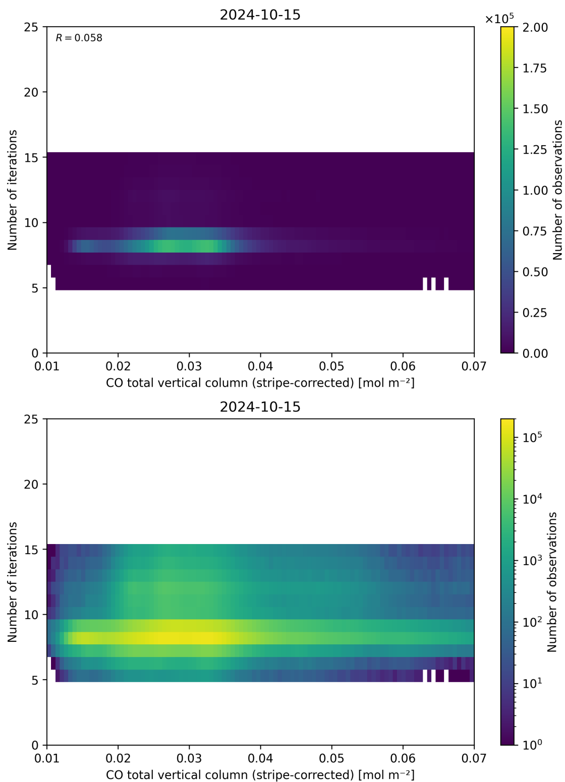
Figure 39: Scatter density plot of “CO total vertical column (stripe-corrected)” against “Number of iterations” for 2024-10-14 to 2024-10-16.
