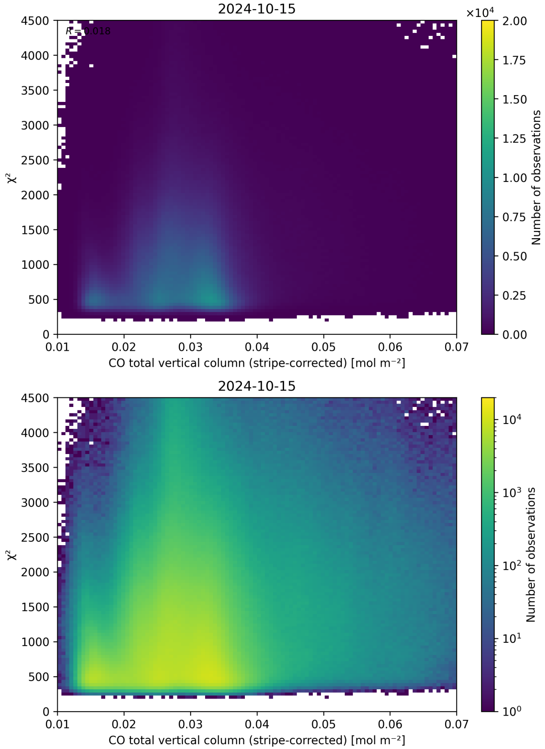
Figure 37: Scatter density plot of “CO total vertical column (stripe-corrected)” against “ \chi^2 ” for 2024-10-14 to 2024-10-16.
