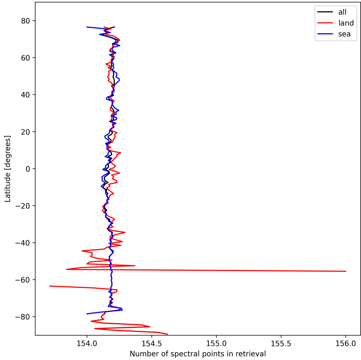
Figure 13: Zonal average of “Number of spectral points in retrieval” for 2024-10-14 to 2024-10-16.
