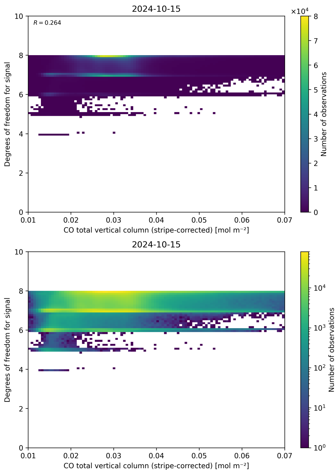
Figure 38: Scatter density plot of “CO total vertical column (stripe-corrected)” against “Degrees of freedom for signal” for 2024-10-14 to 2024-10-16.
