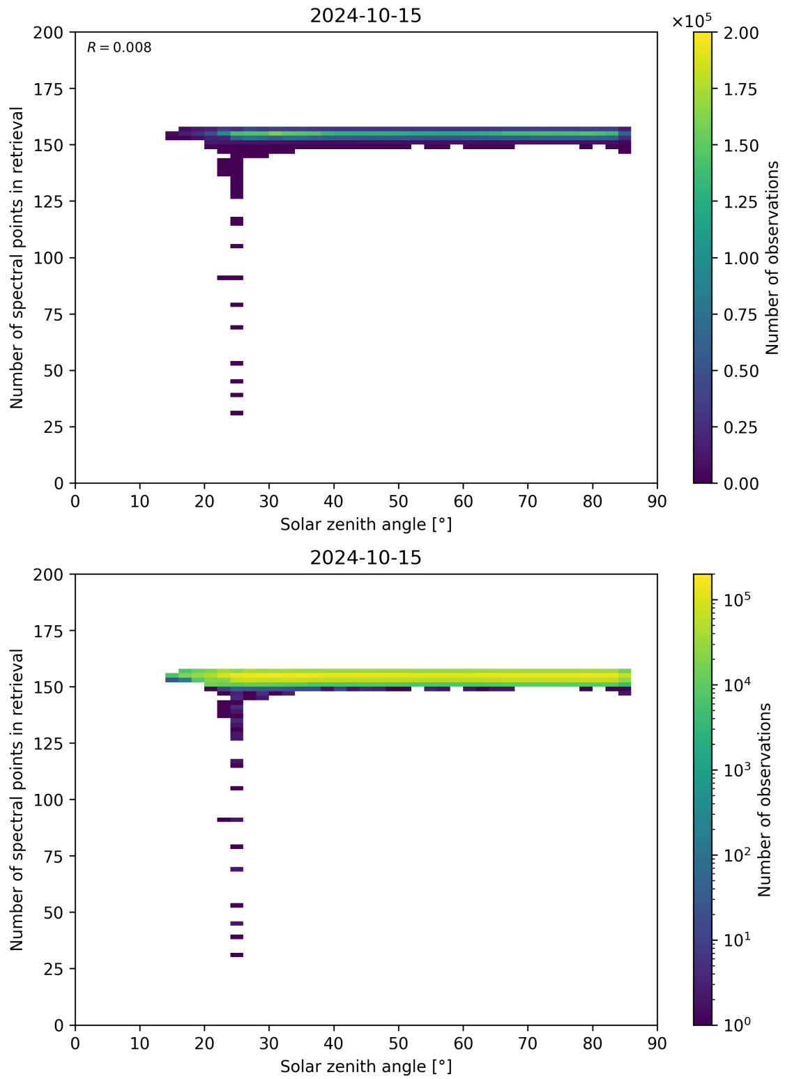
Figure 68: Scatter density plot of “Solar zenith angle” against “Number of spectral points in retrieval” for 2024-10-14 to 2024-10-16.
