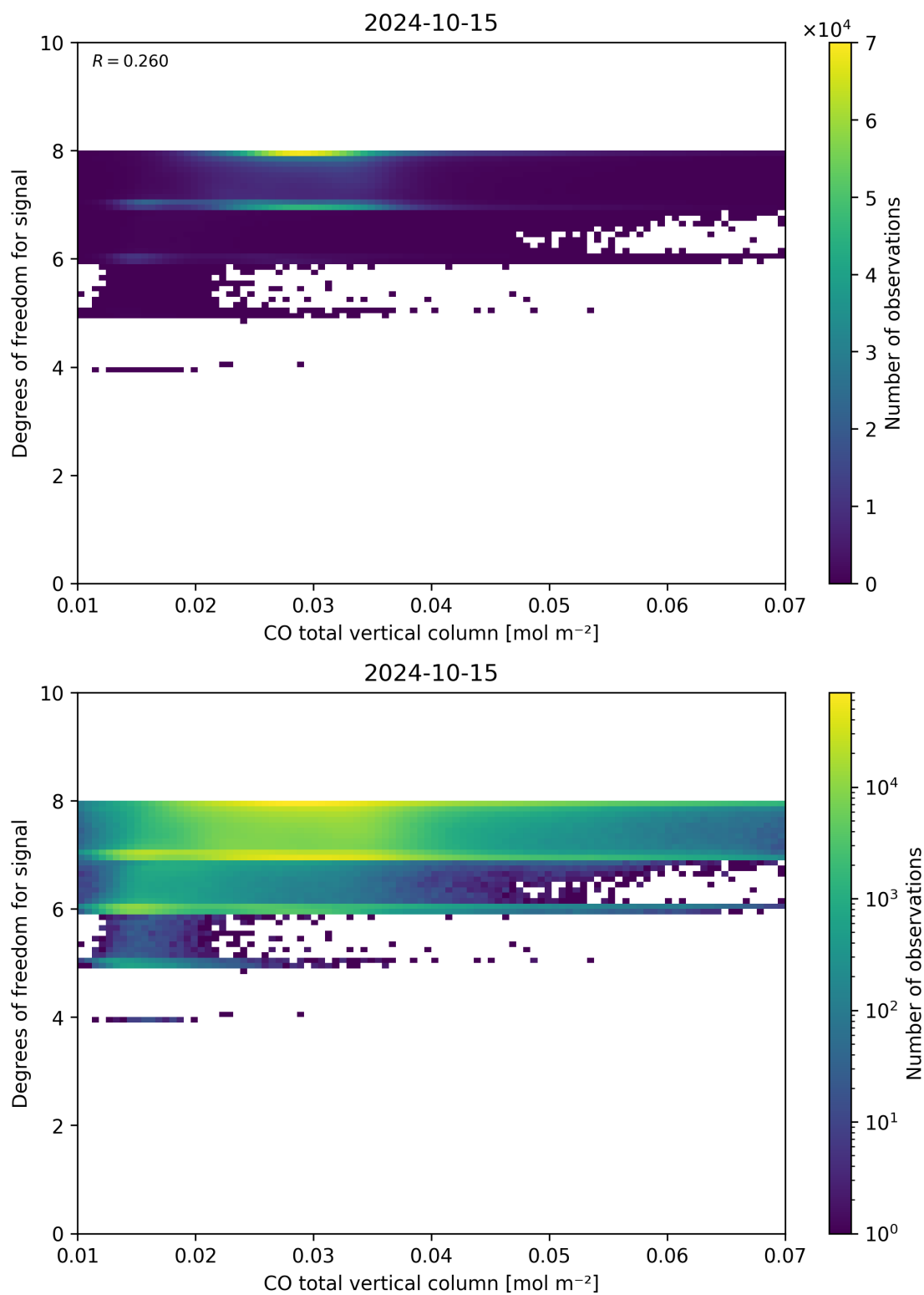
Figure 41: Scatter density plot of “CO total vertical column” against “Degrees of freedom for signal” for 2024-10-14 to 2024-10-16.
