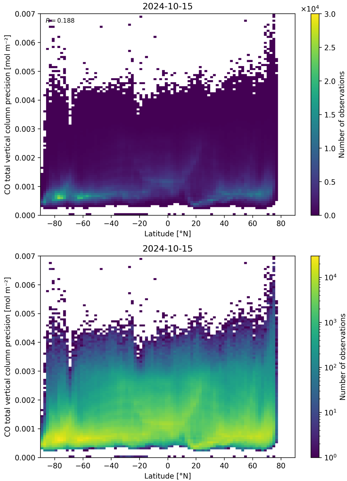
Figure 53: Scatter density plot of “Latitude” against “CO total vertical column precision” for 2024-10-14 to 2024-10-16.
