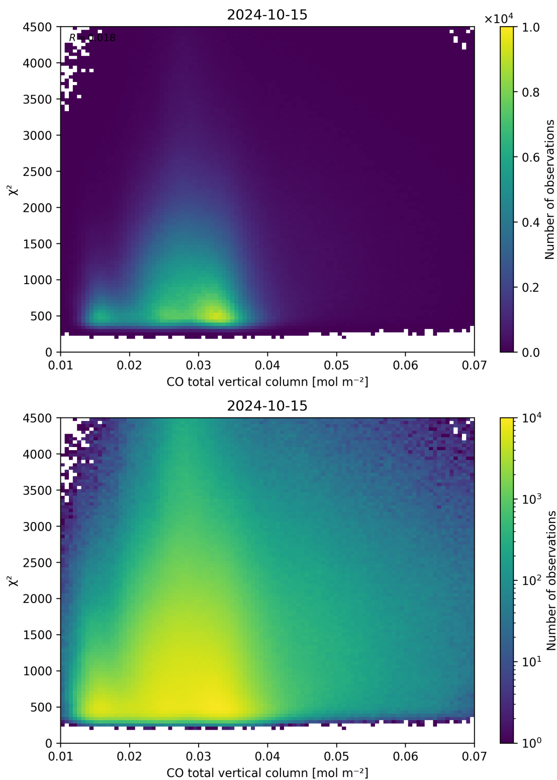
Figure 35: Scatter density plot of “CO total vertical column” against “ \chi^2 ” for 2024-10-14 to 2024-10-16.
