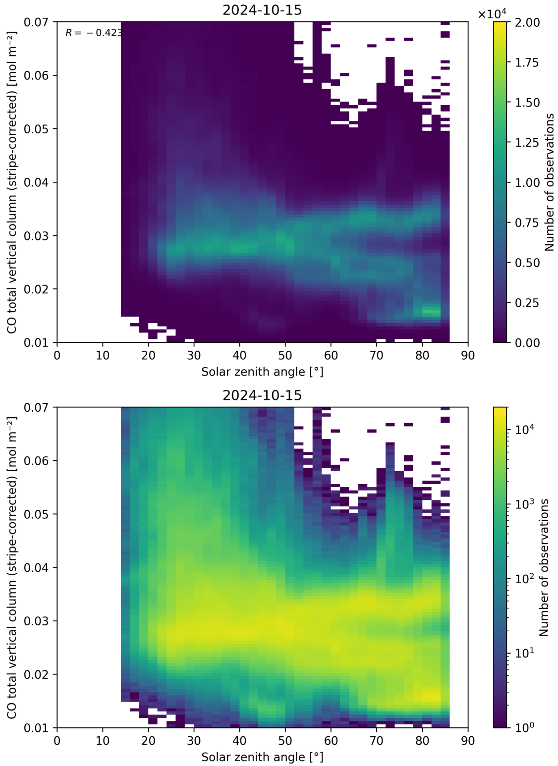
Figure 62: Scatter density plot of “Solar zenith angle” against “CO total vertical column (stripe-corrected)” for 2024-10-14 to 2024-10-16.
