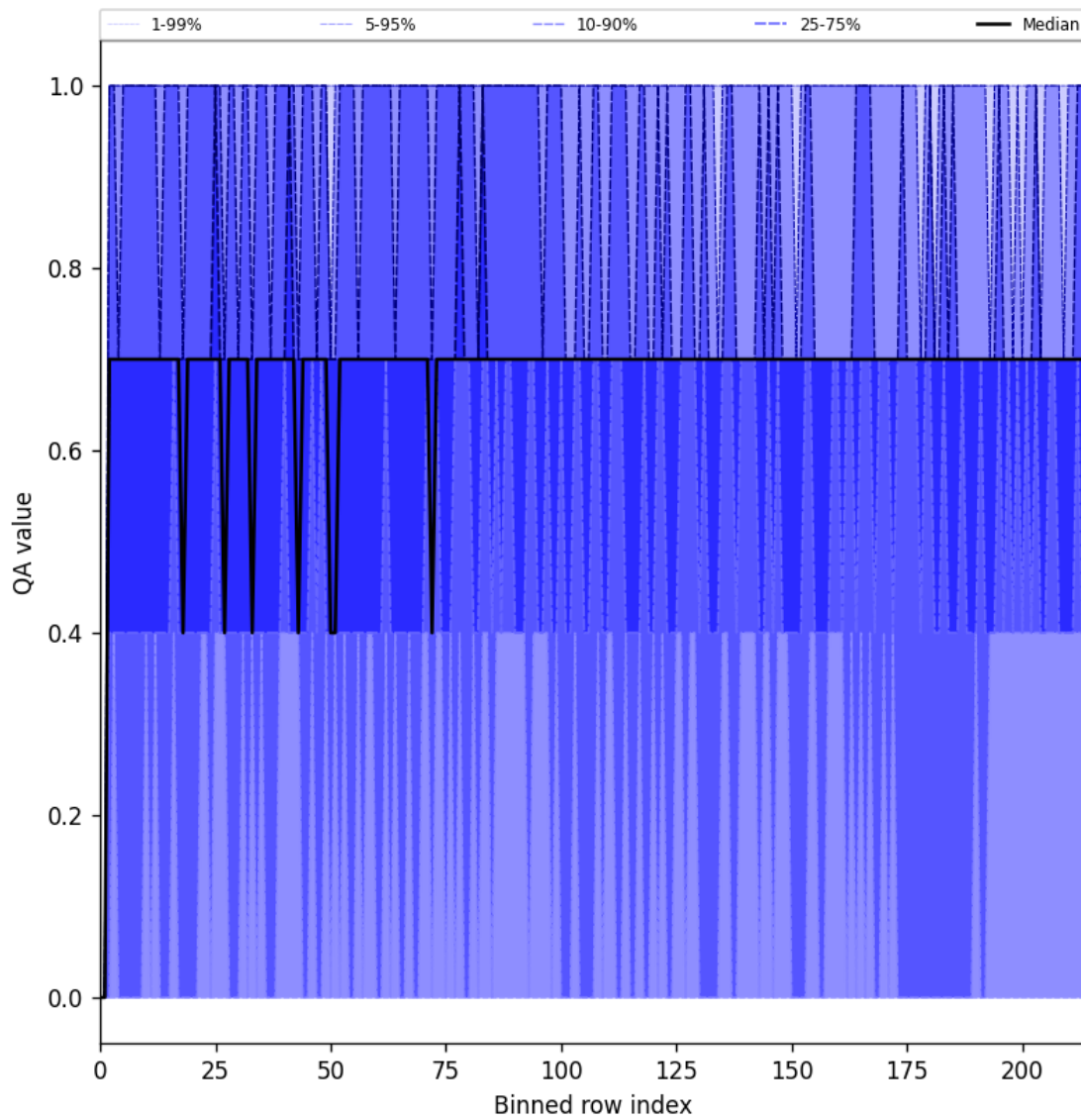
Figure 25: Along track statistics of “QA value” for 2024-10-14 to 2024-10-16
