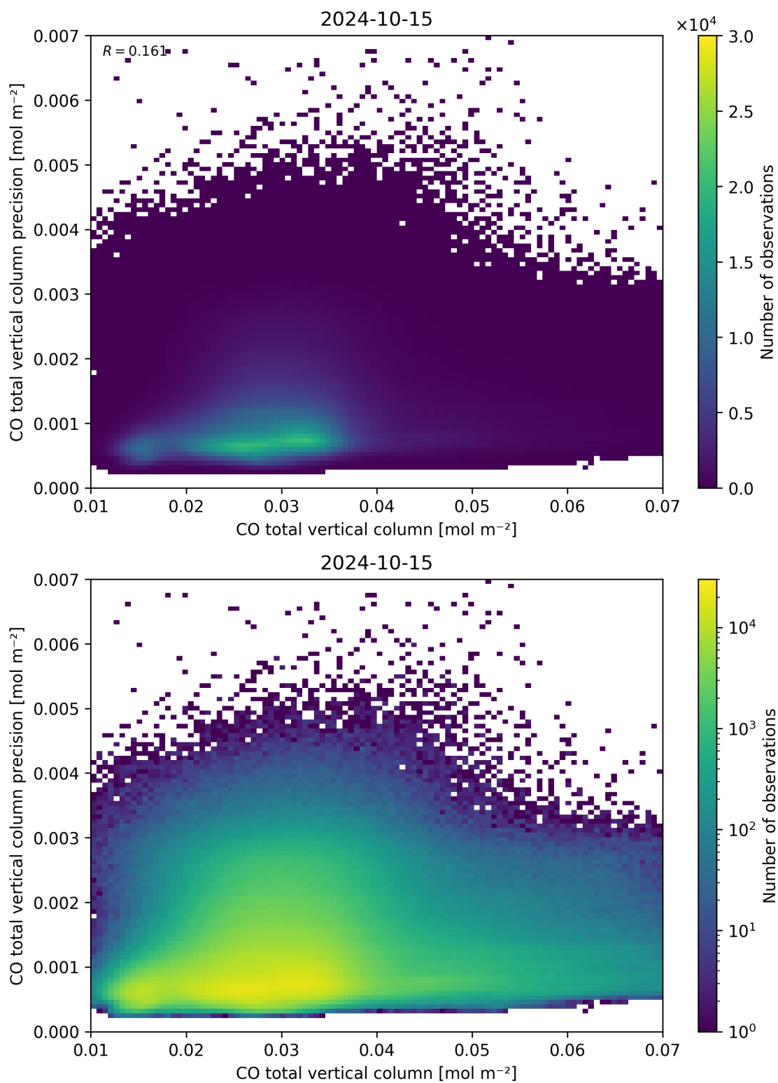
Figure 34: Scatter density plot of “CO total vertical column” against “CO total vertical column precision” for 2024-10-14 to 2024-10-16.
