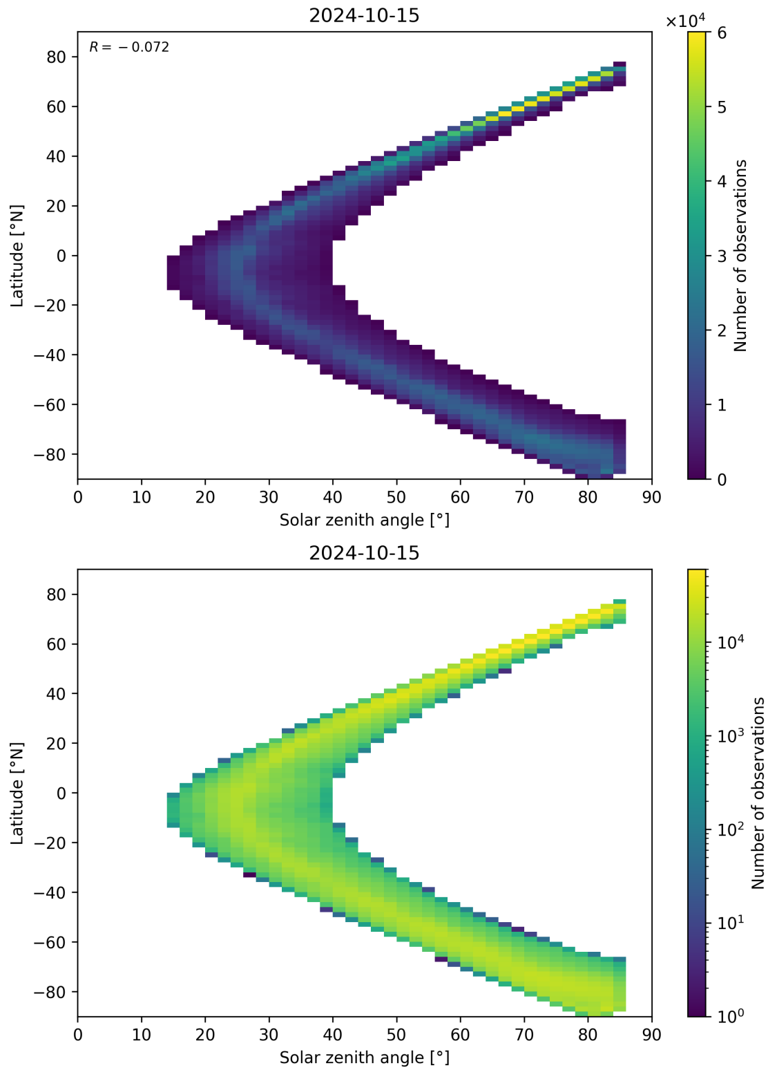
Figure 66: Scatter density plot of “Solar zenith angle” against “Latitude” for 2024-10-14 to 2024-10-16.
