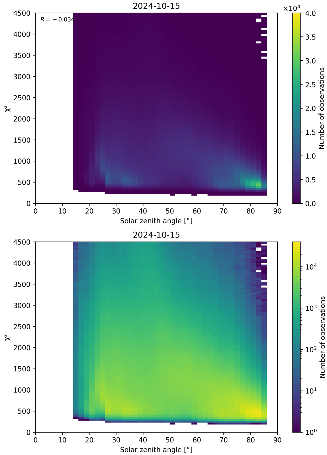
Figure 64: Scatter density plot of “Solar zenith angle” against “ \chi^2 ” for 2024-10-14 to 2024-10-16.
