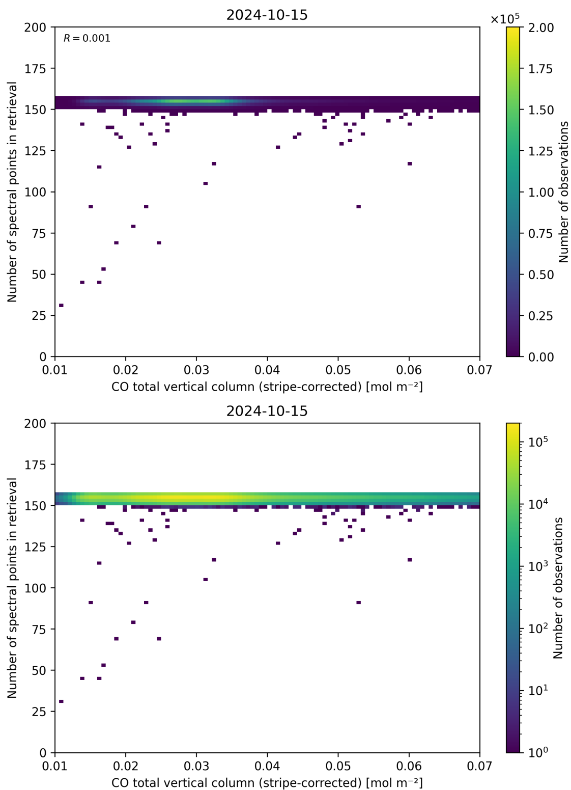
Figure 40: Scatter density plot of “CO total vertical column (stripe-corrected)” against “Number of spectral points in retrieval” for 2024-10-14 to 2024-10-16.
