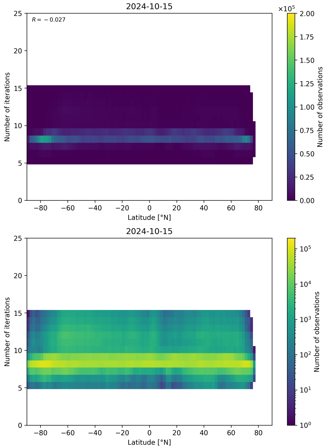
Figure 56: Scatter density plot of “Latitude” against “Number of iterations” for 2024-10-14 to 2024-10-16.
