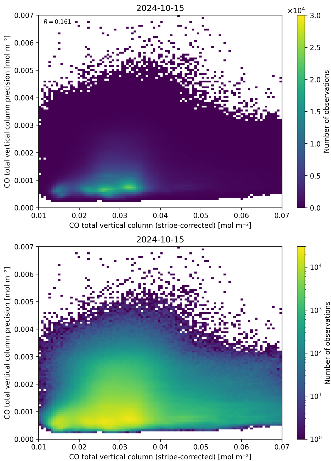
Figure 36: Scatter density plot of “CO total vertical column (stripe-corrected)” against “CO total vertical column precision” for 2024-10-14 to 2024-10-16.
