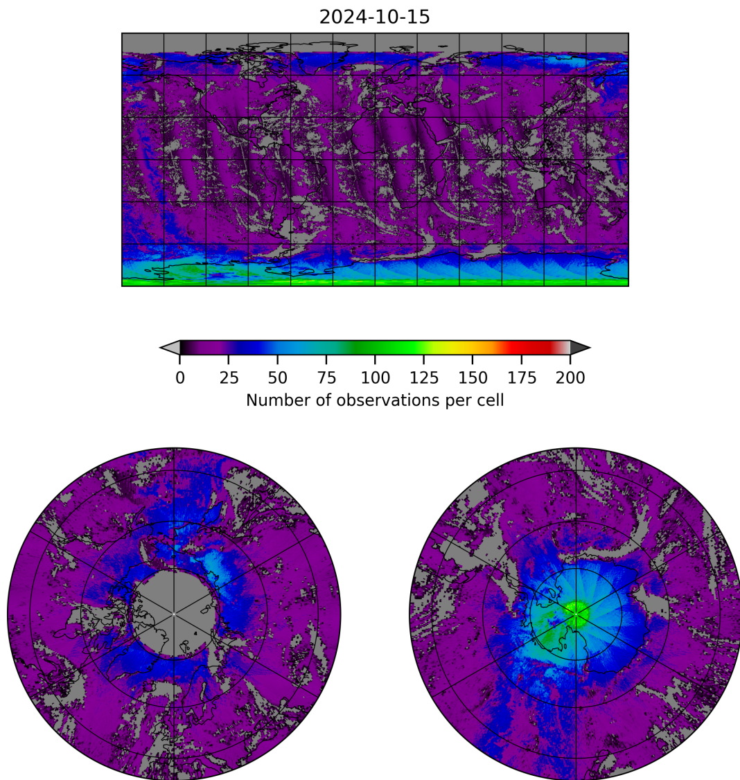
Figure 8: Map of the number of observations for 2024-10-14 to 2024-10-16
