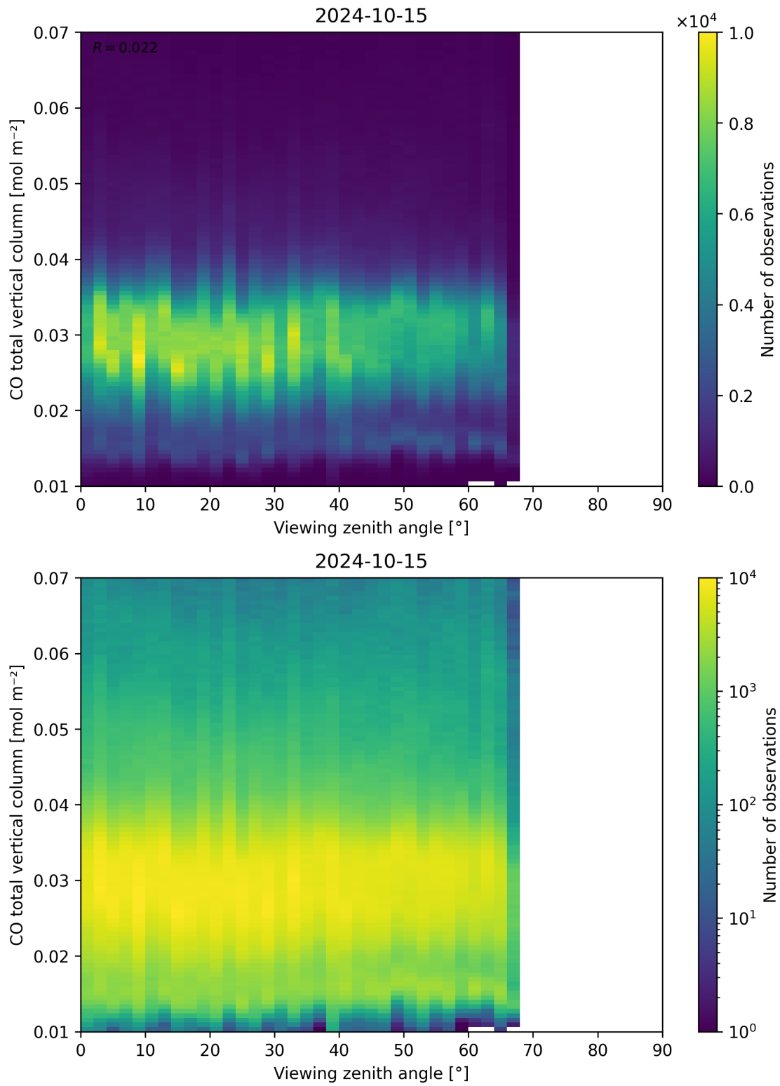
Figure 69: Scatter density plot of “Viewing zenith angle” against “CO total vertical column” for 2024-10-14 to 2024-10-16.
