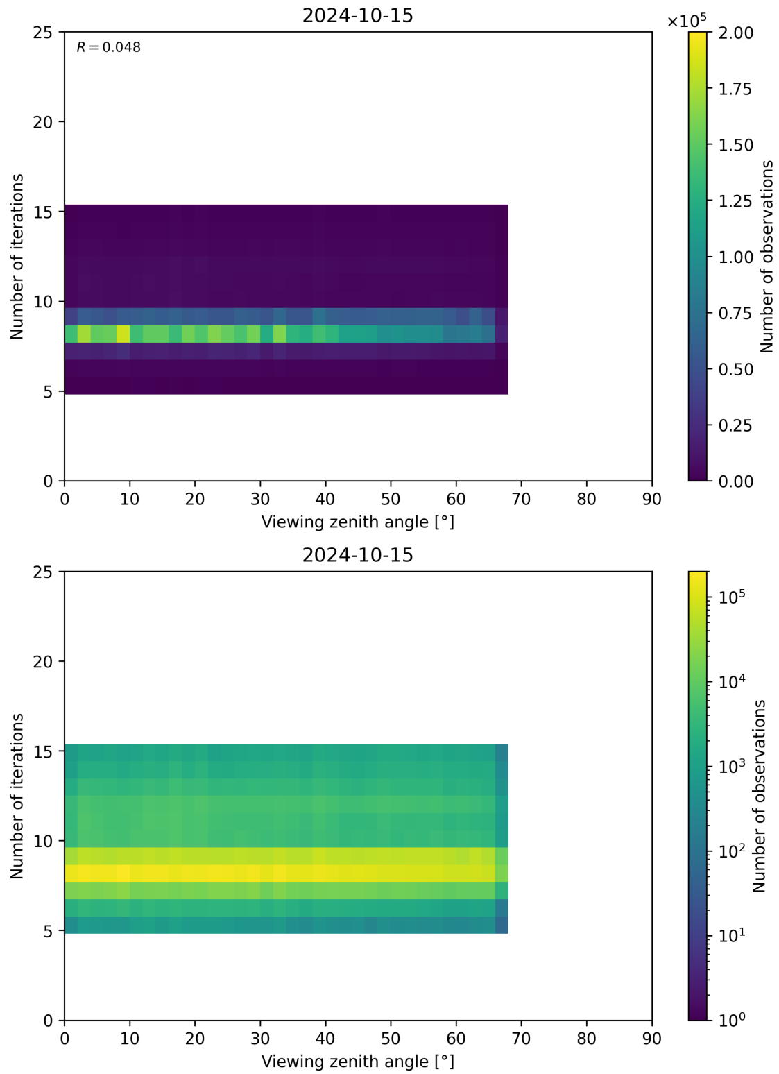
Figure 75: Scatter density plot of “Viewing zenith angle” against “Number of iterations” for 2024-10-14 to 2024-10-16.
