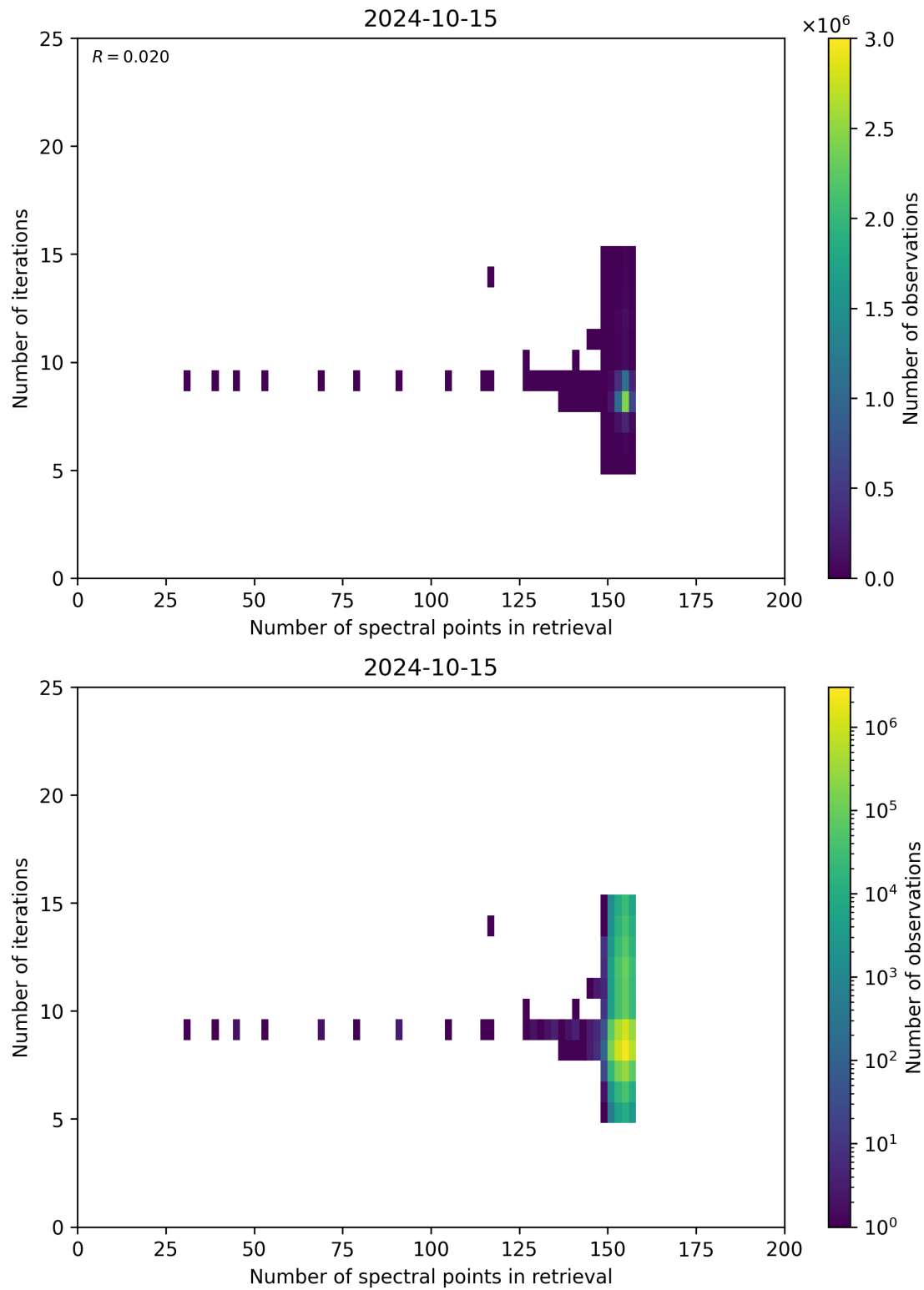
Figure 60: Scatter density plot of “Number of spectral points in retrieval” against “Number of iterations” for 2024-10-14 to 2024-10-16.
