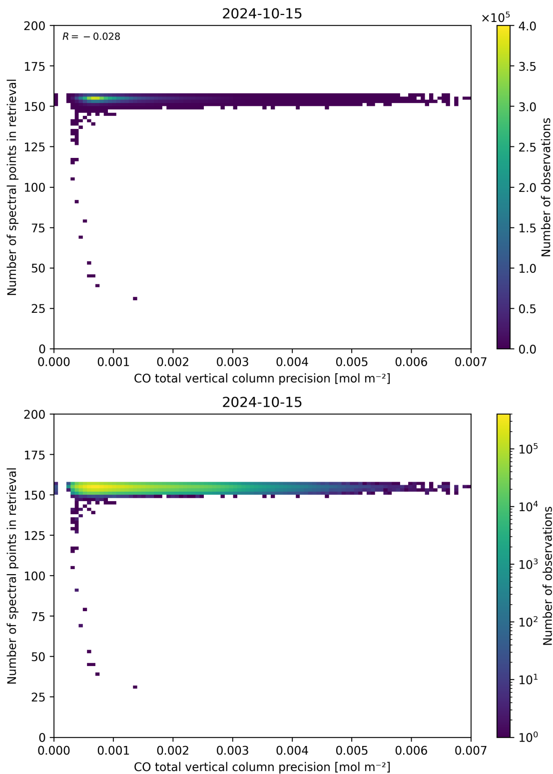
Figure 47: Scatter density plot of “CO total vertical column precision” against “Number of spectral points in retrieval” for 2024-10-14 to 2024-10-16.
