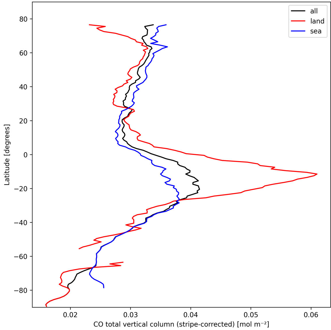
Figure 11: Zonal average of “CO total vertical column (stripe-corrected)” for 2024-10-14 to 2024-10-16.
