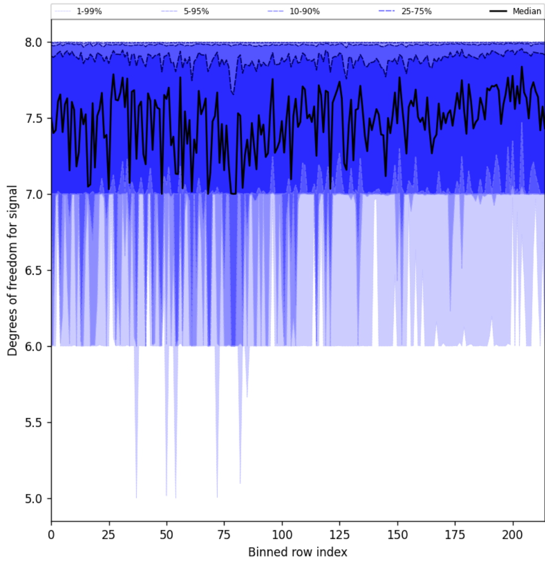
Figure 31: Along track statistics of “Degrees of freedom for signal” for 2024-10-14 to 2024-10-16
