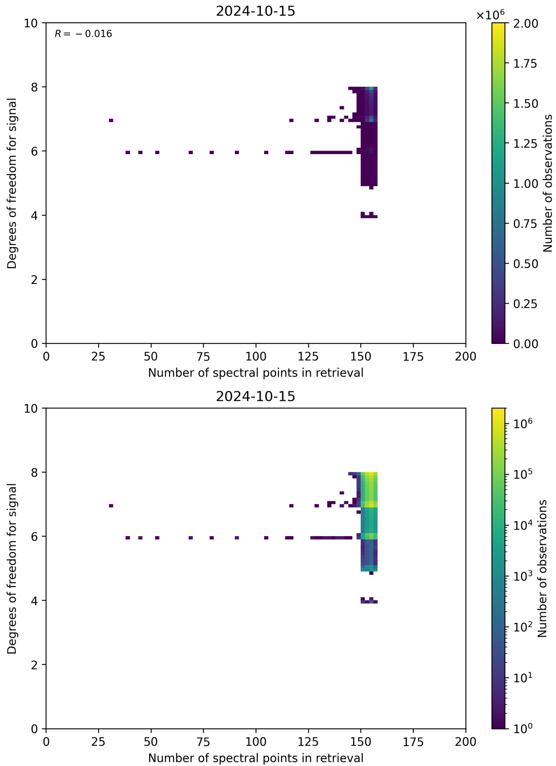
Figure 59: Scatter density plot of “Number of spectral points in retrieval” against “Degrees of freedom for signal” for 2024-10-14 to 2024-10-16.
