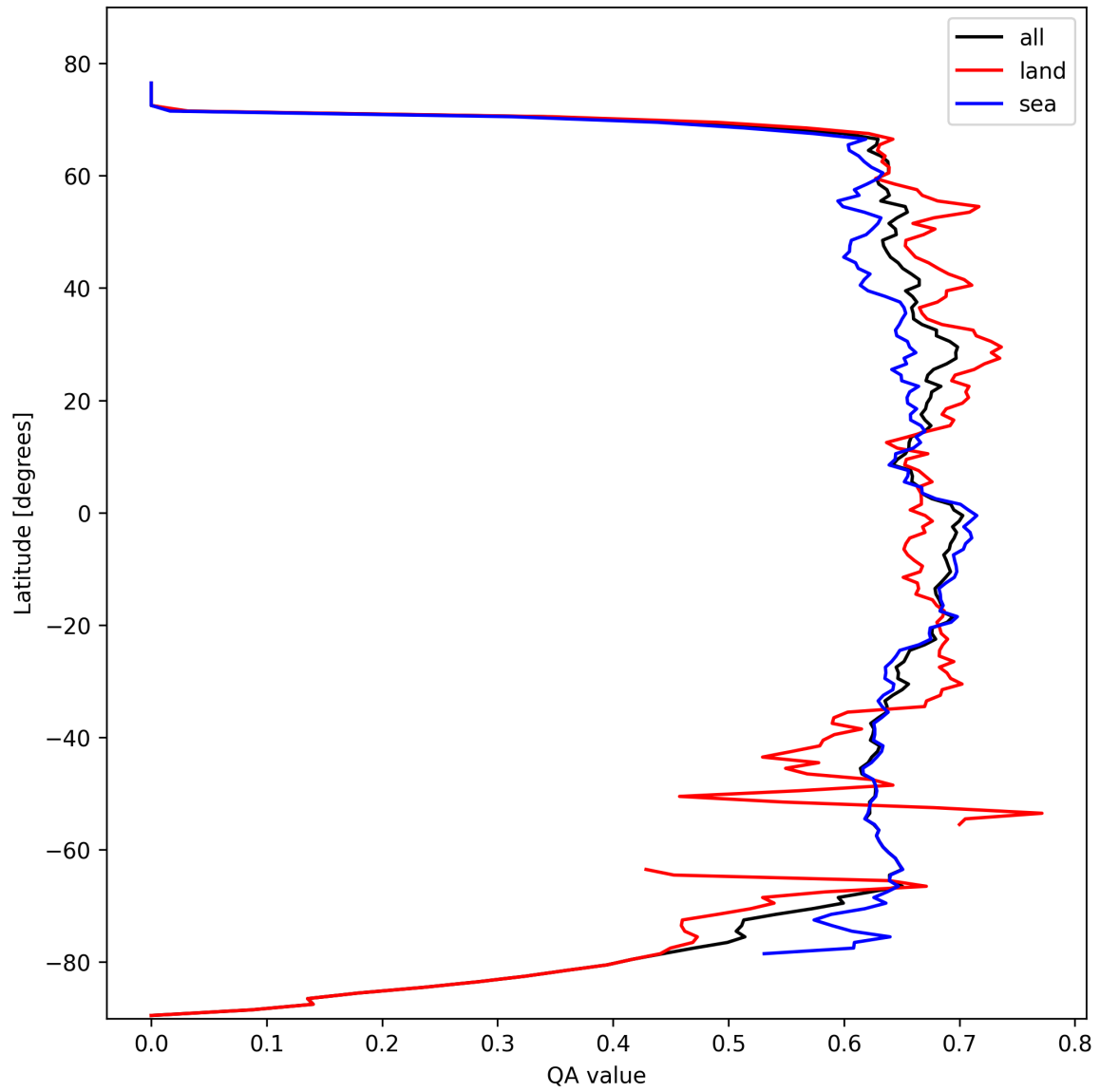
Figure 9: Zonal average of “QA value” for 2024-10-14 to 2024-10-16.
