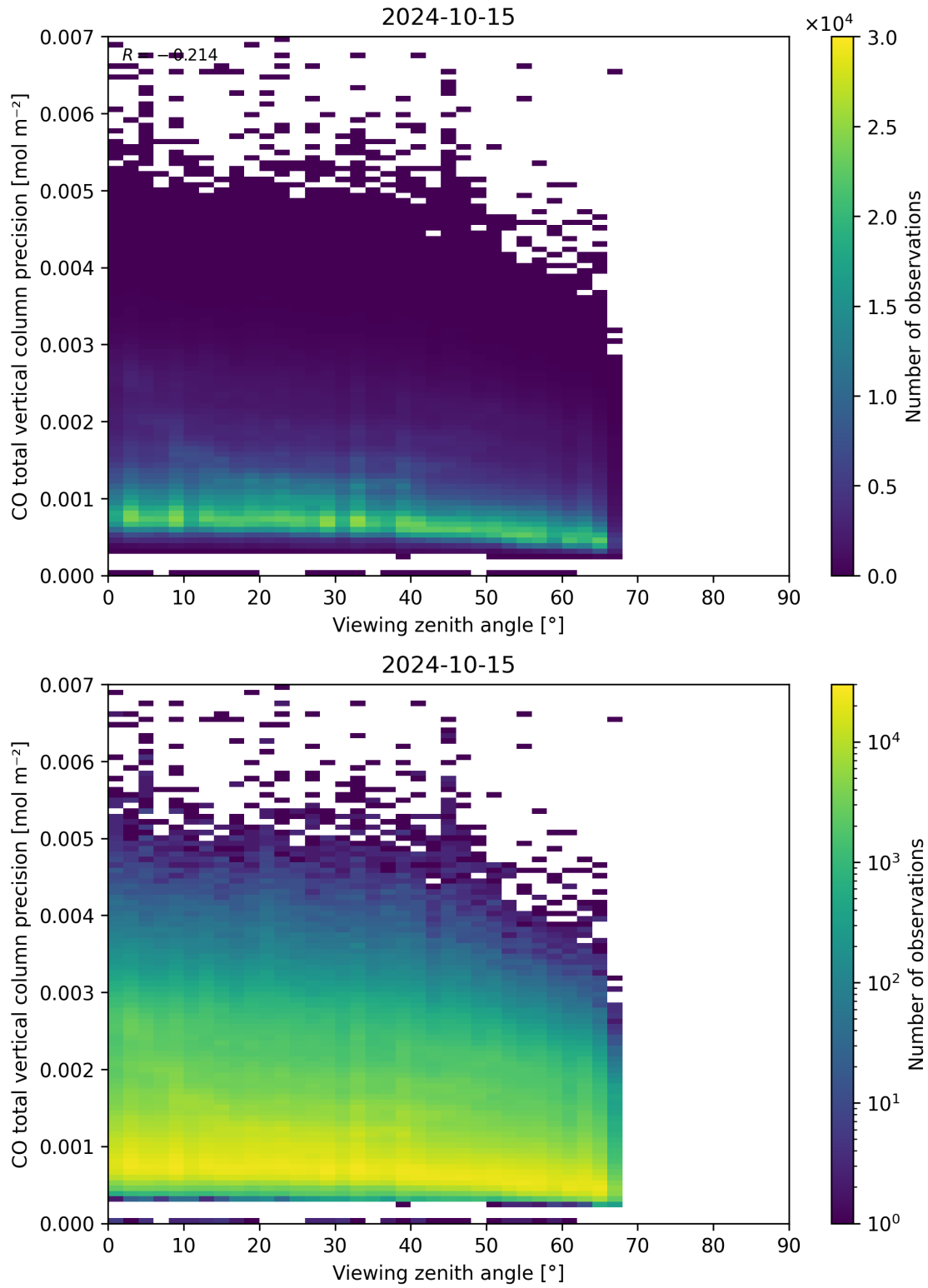
Figure 71: Scatter density plot of “Viewing zenith angle” against “CO total vertical column precision” for 2024-10-14 to 2024-10-16.
