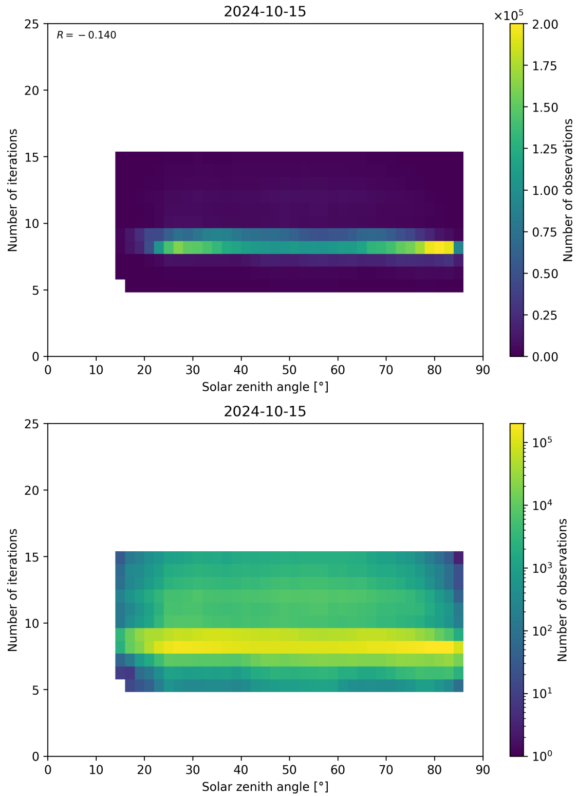
Figure 67: Scatter density plot of “Solar zenith angle” against “Number of iterations” for 2024-10-14 to 2024-10-16.
