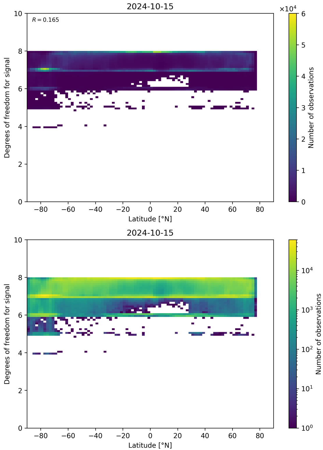
Figure 55: Scatter density plot of “Latitude” against “Degrees of freedom for signal” for 2024-10-14 to 2024-10-16.
