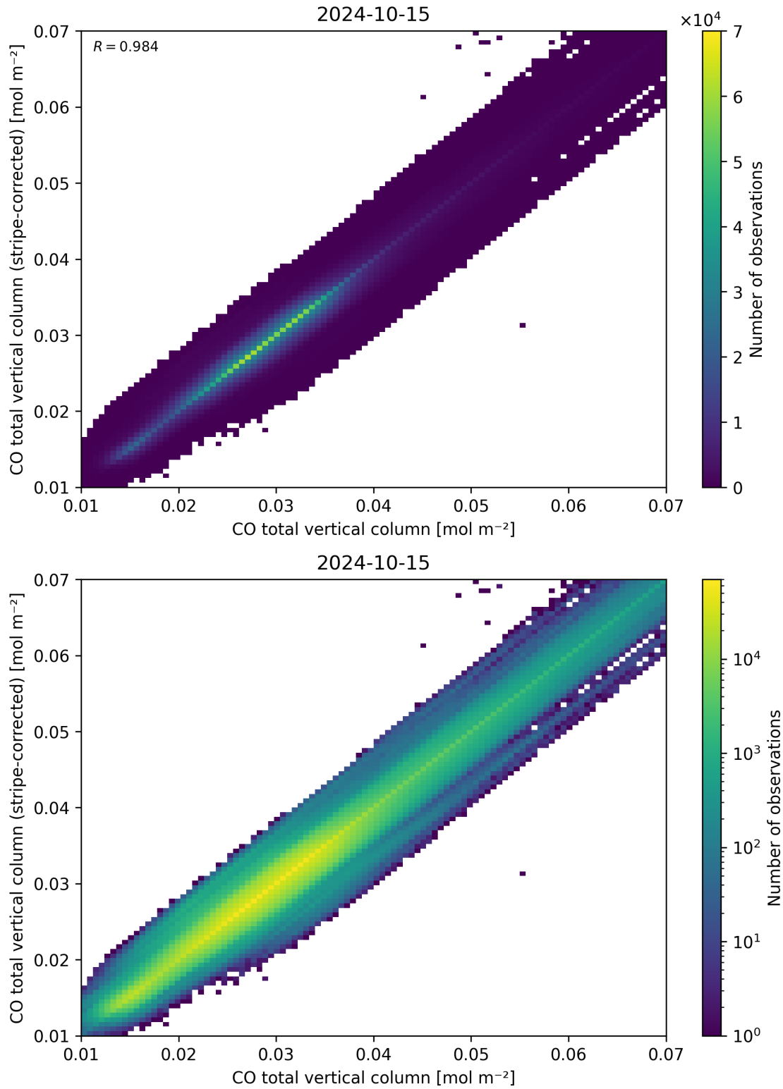
Figure 33: Scatter density plot of “CO total vertical column” against “CO total vertical column (stripe-corrected)” for 2024-10-14 to 2024-10-16.
