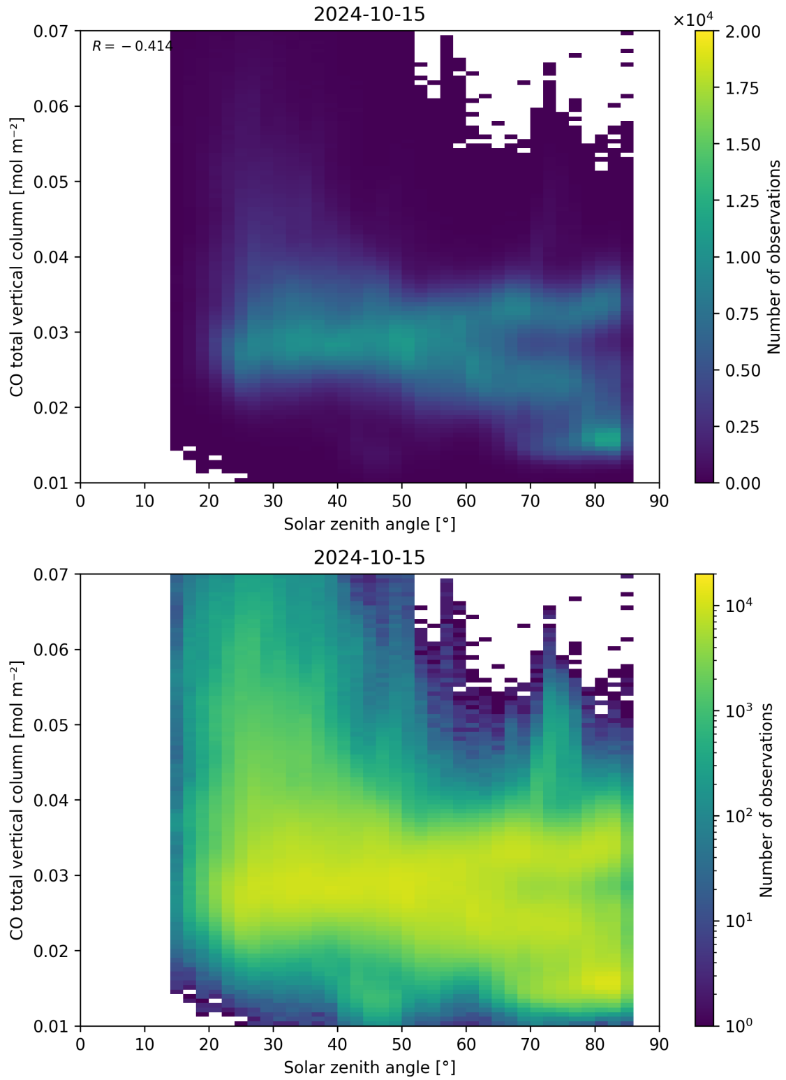
Figure 61: Scatter density plot of “Solar zenith angle” against “CO total vertical column” for 2024-10-14 to 2024-10-16.
