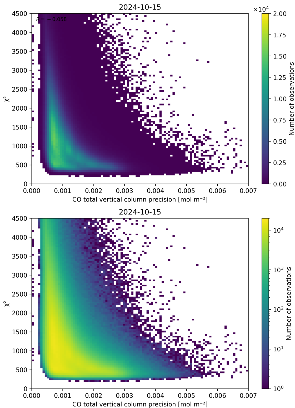
Figure 44: Scatter density plot of “CO total vertical column precision” against “ \chi^2 ” for 2024-10-14 to 2024-10-16.
