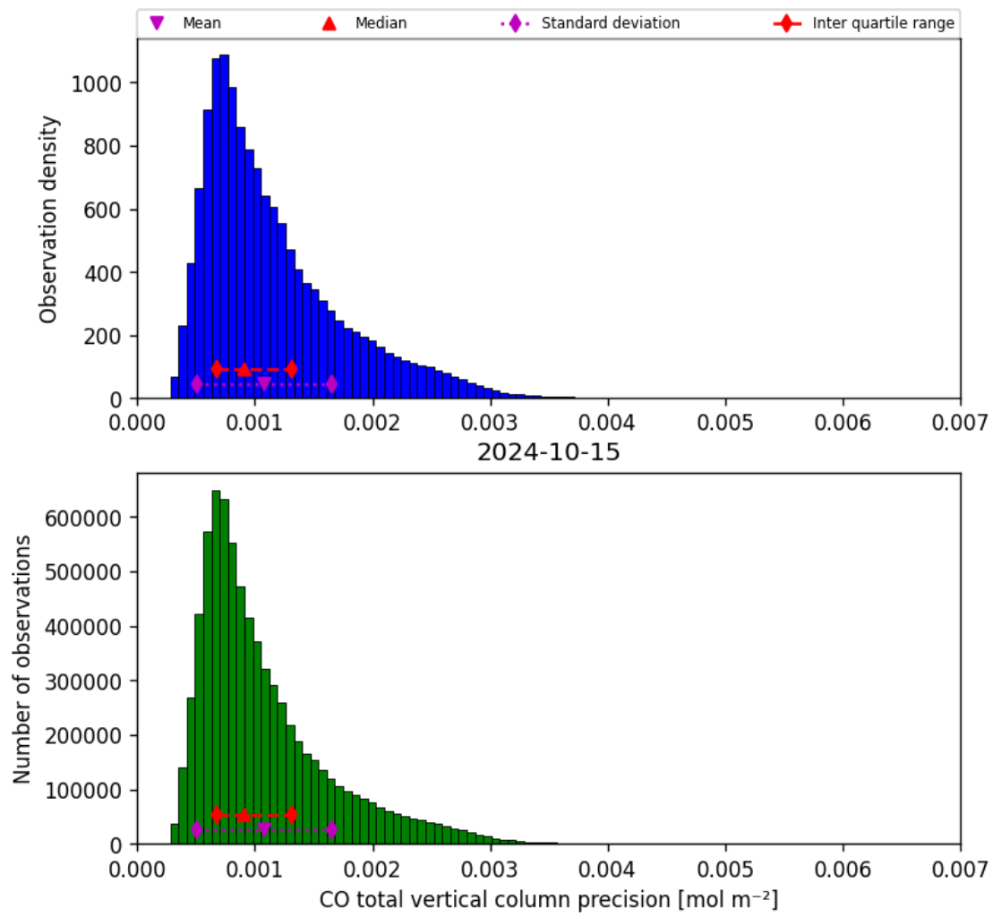
Figure 20: Histogram of “CO total vertical column precision” for 2024-10-14 to 2024-10-16
