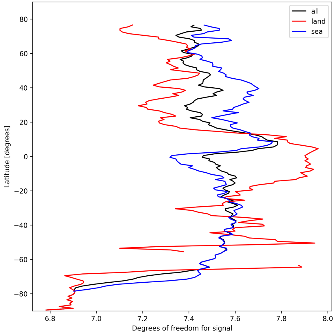
Figure 15: Zonal average of “Degrees of freedom for signal” for 2024-10-14 to 2024-10-16.
