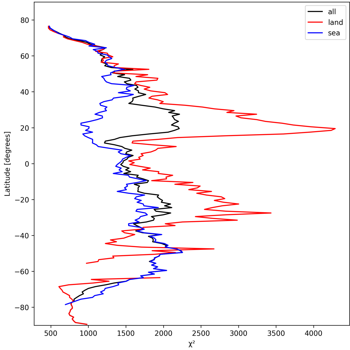
Figure 14: Zonal average of “ \chi^2 ” for 2024-10-14 to 2024-10-16.
