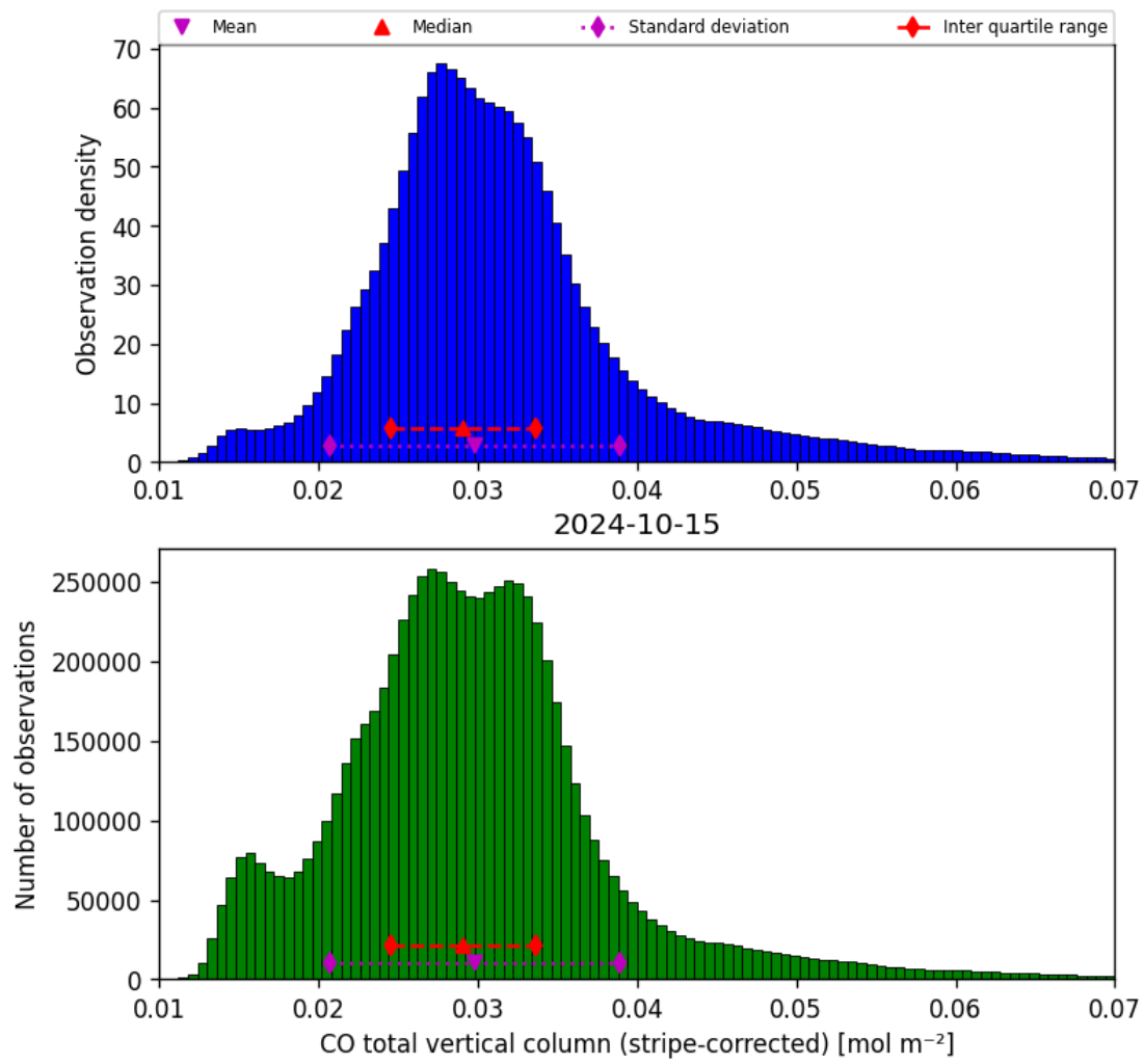
Figure 19: Histogram of “CO total vertical column (stripe-corrected)” for 2024-10-14 to 2024-10-16
