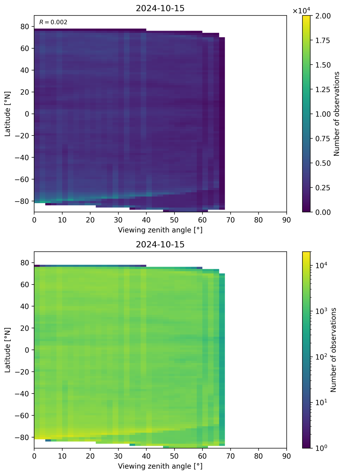
Figure 74: Scatter density plot of “Viewing zenith angle” against “Latitude” for 2024-10-14 to 2024-10-16.
