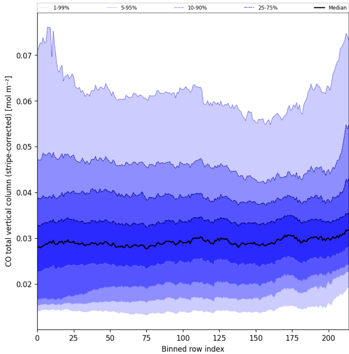
Figure 27: Along track statistics of “CO total vertical column (stripe-corrected)” for 2024-10-14 to 2024-10-16
