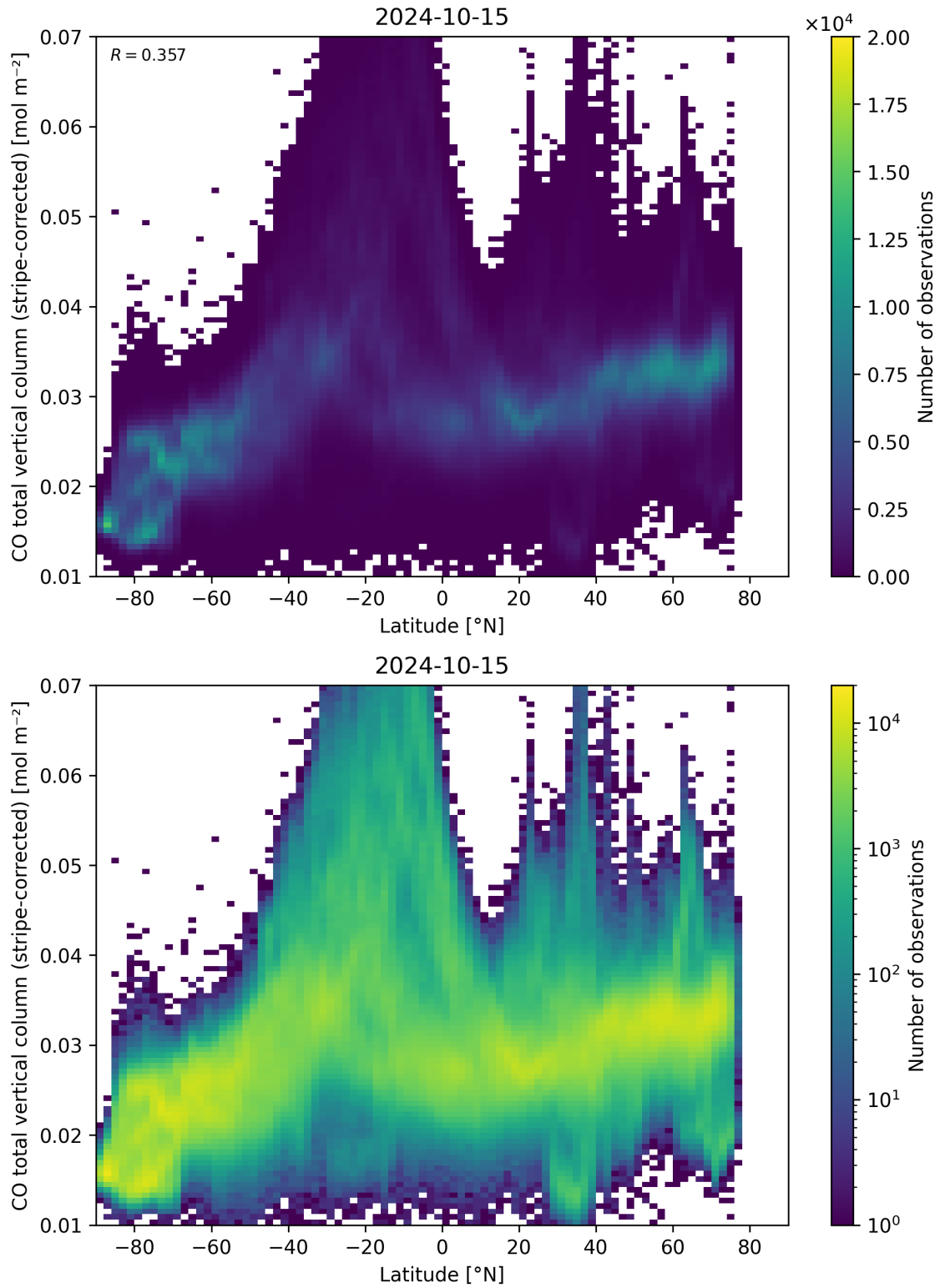
Figure 52: Scatter density plot of “Latitude” against “CO total vertical column (stripe-corrected)” for 2024-10-14 to 2024-10-16.
