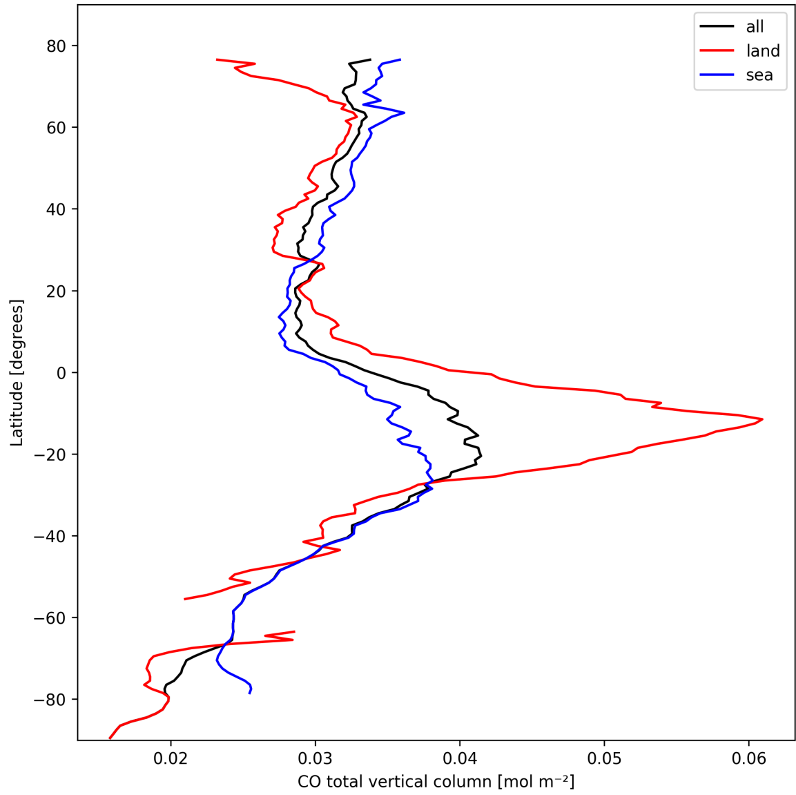
Figure 10: Zonal average of “CO total vertical column” for 2024-10-14 to 2024-10-16.
