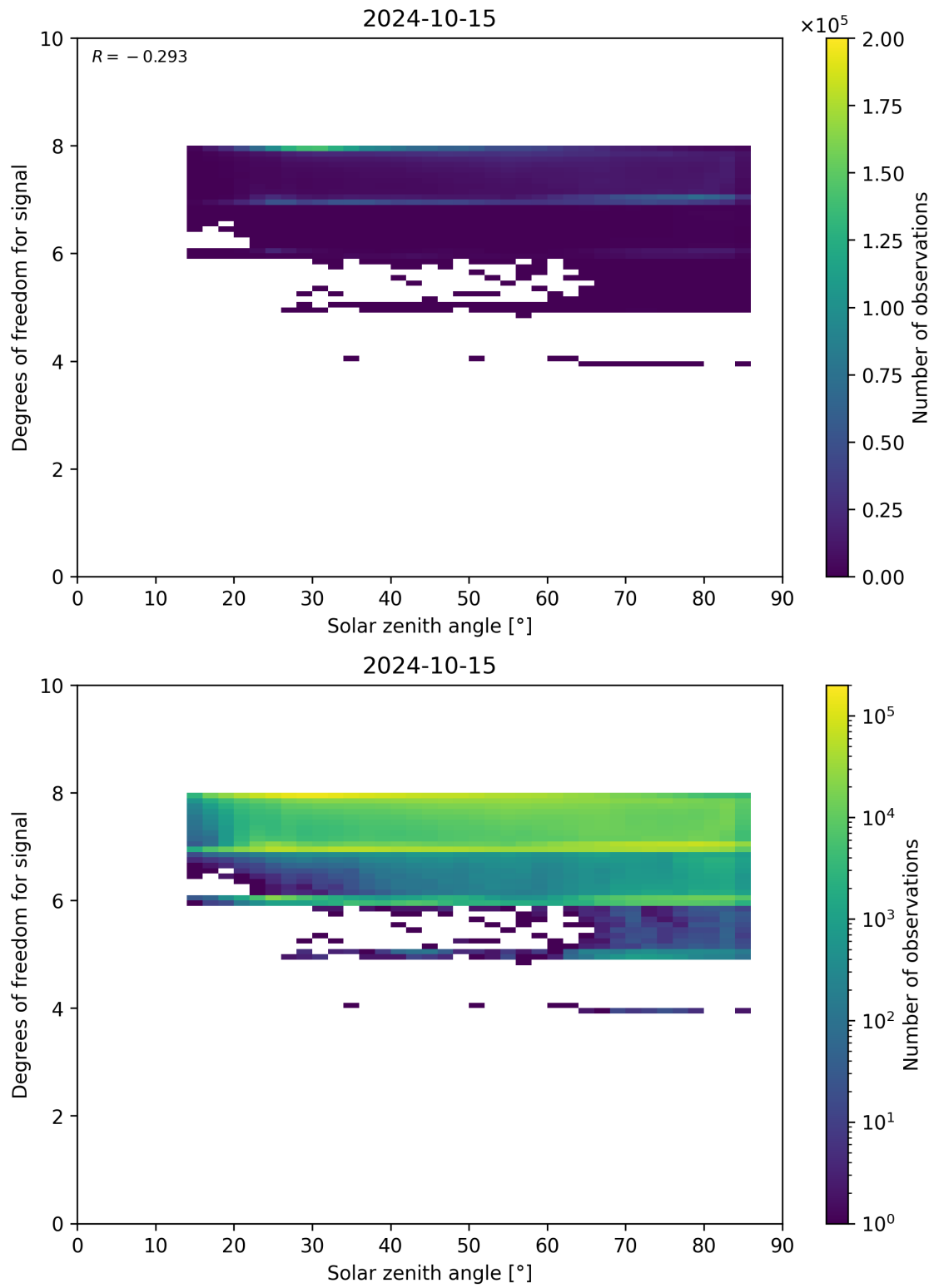
Figure 65: Scatter density plot of “Solar zenith angle” against “Degrees of freedom for signal” for 2024-10-14 to 2024-10-16.
