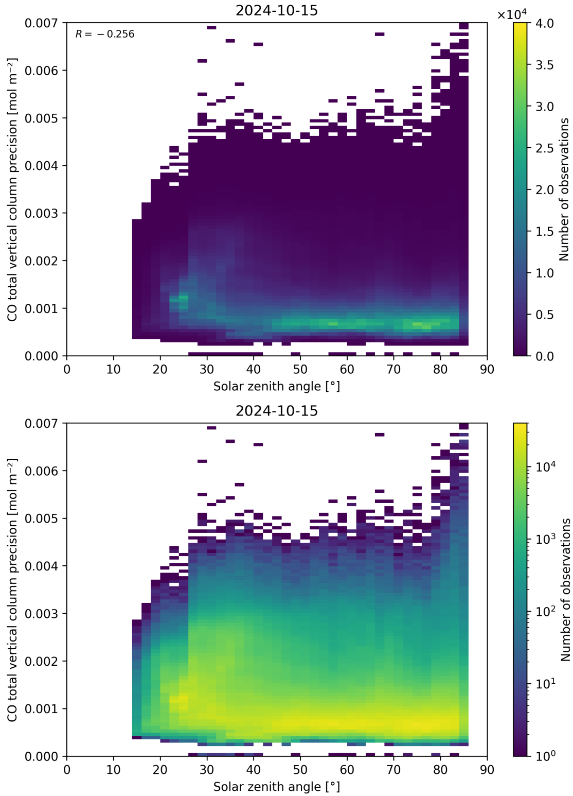
Figure 63: Scatter density plot of “Solar zenith angle” against “CO total vertical column precision” for 2024-10-14 to 2024-10-16.
