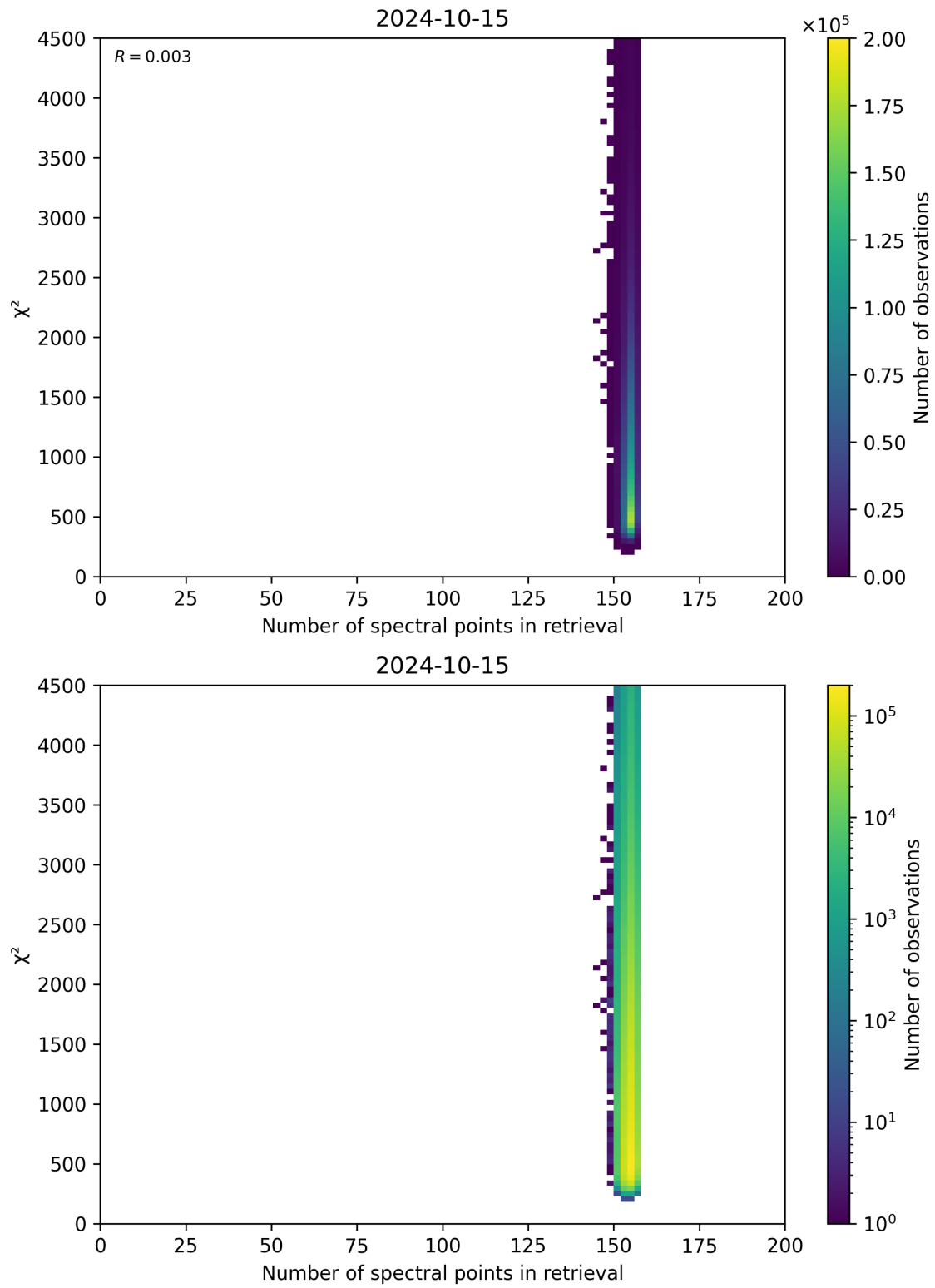
Figure 58: Scatter density plot of “Number of spectral points in retrieval” against “ \chi^2 ” for 2024-10-14 to 2024-10-16.
