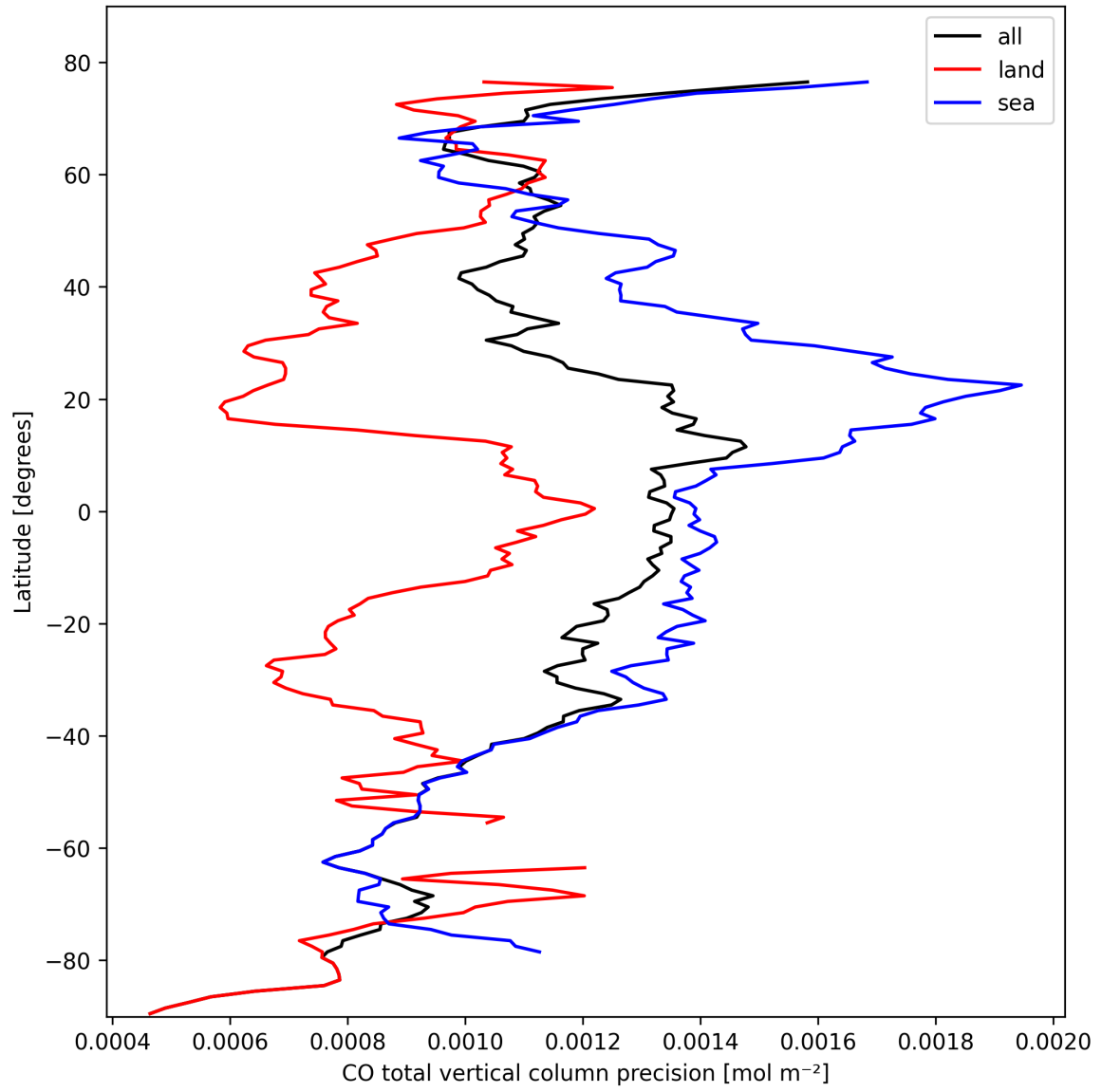
Figure 12: Zonal average of “CO total vertical column precision” for 2024-10-14 to 2024-10-16.
