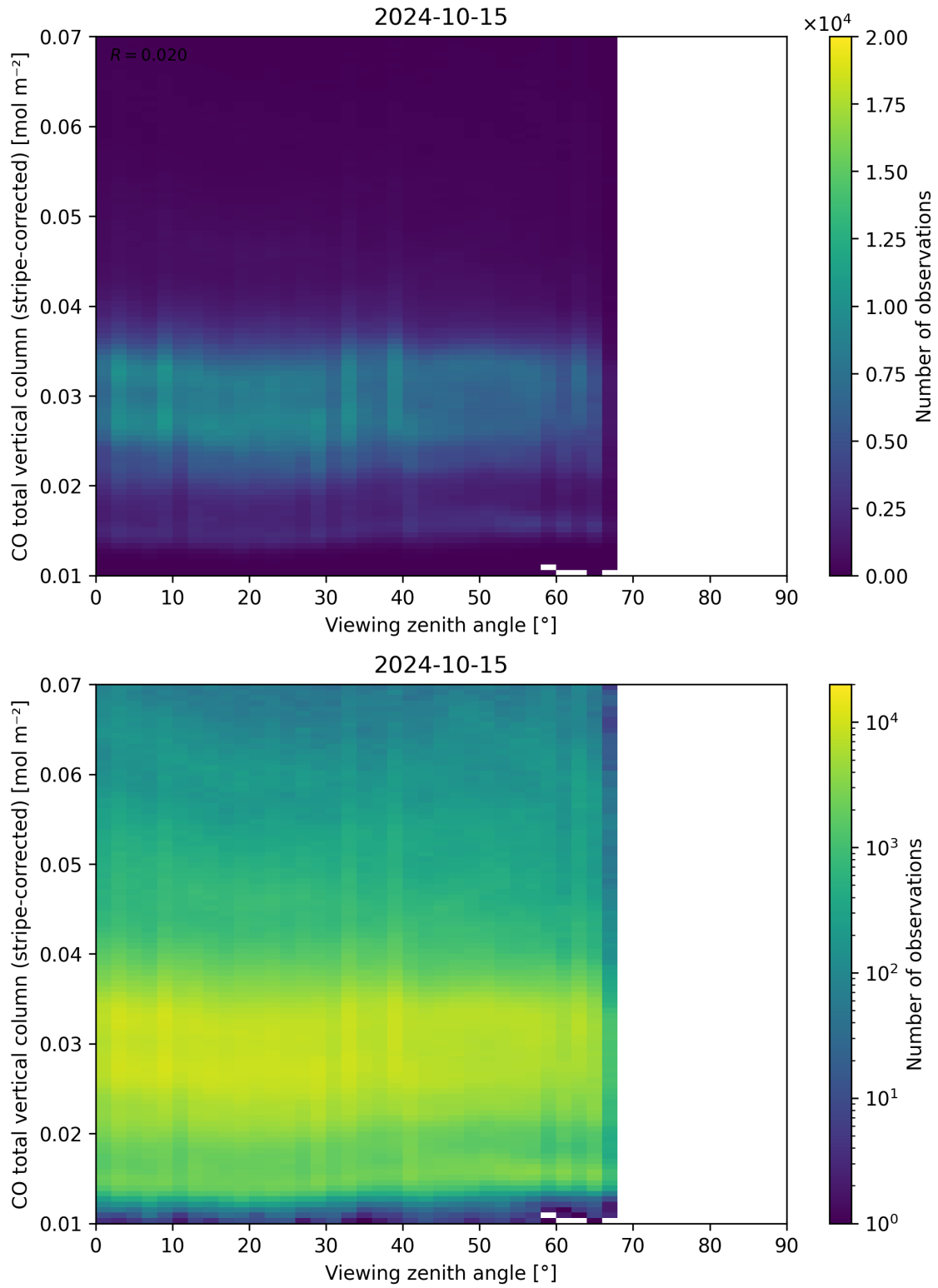
Figure 70: Scatter density plot of “Viewing zenith angle” against “CO total vertical column (stripe-corrected)” for 2024-10-14 to 2024-10-16.
