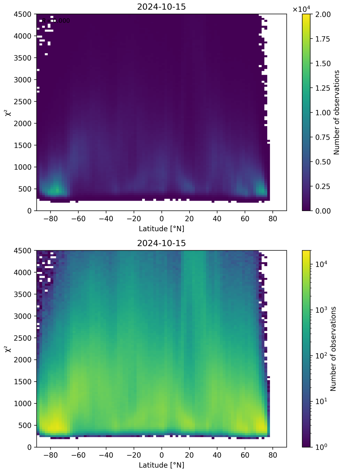
Figure 54: Scatter density plot of “Latitude” against “ \chi^2 ” for 2024-10-14 to 2024-10-16.
