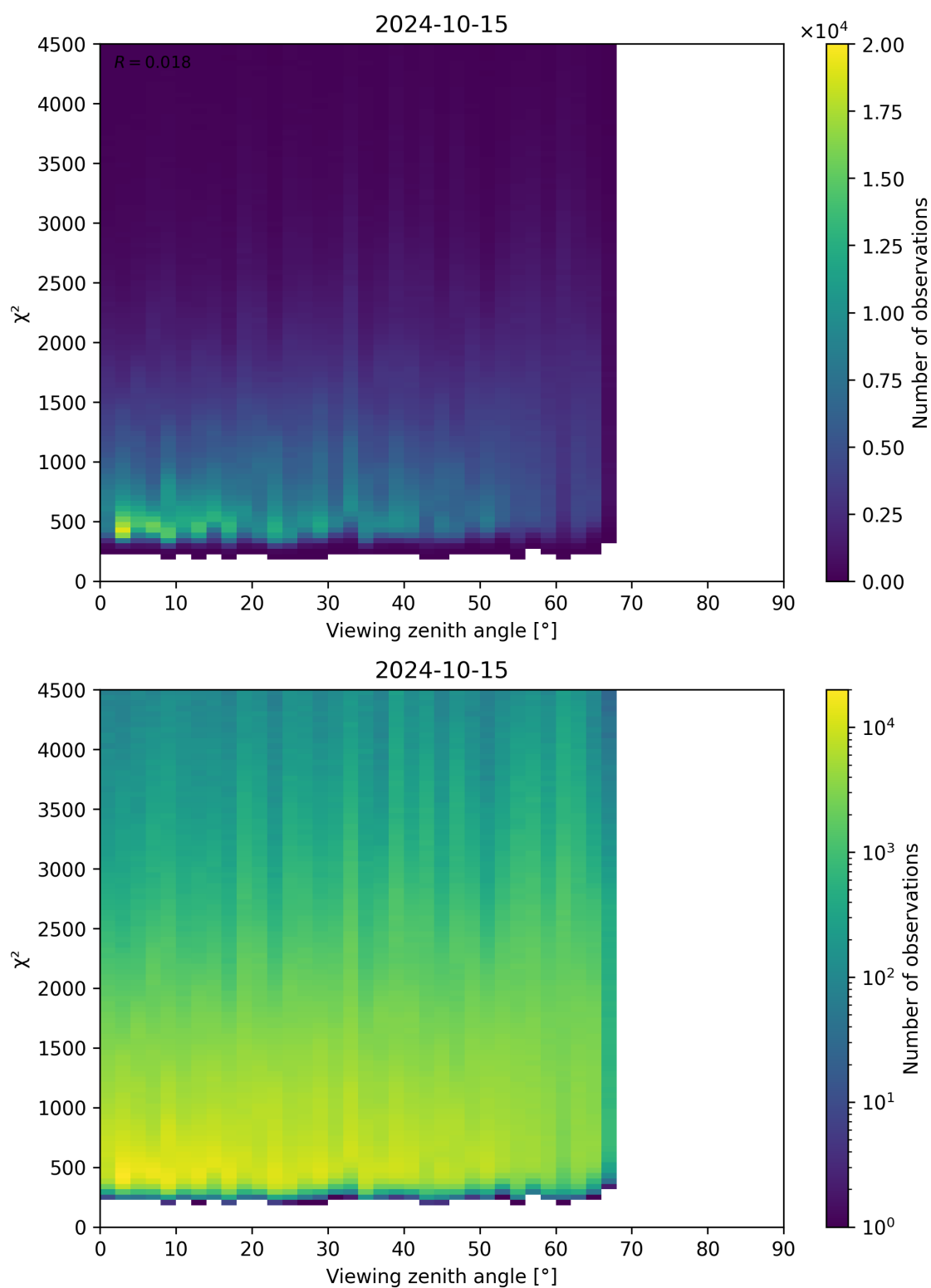
Figure 72: Scatter density plot of “Viewing zenith angle” against “ \chi^2 ” for 2024-10-14 to 2024-10-16.
