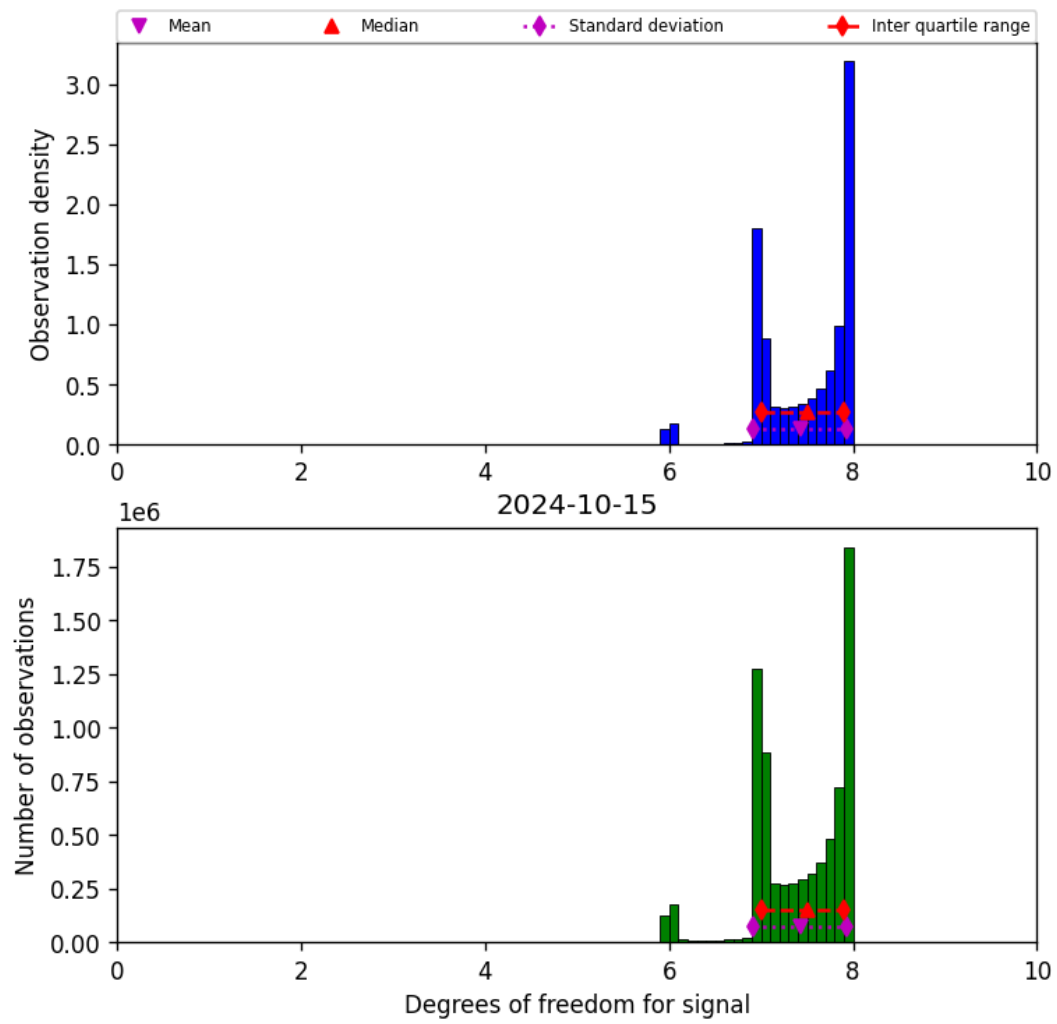
Figure 23: Histogram of “Degrees of freedom for signal” for 2024-10-14 to 2024-10-16
