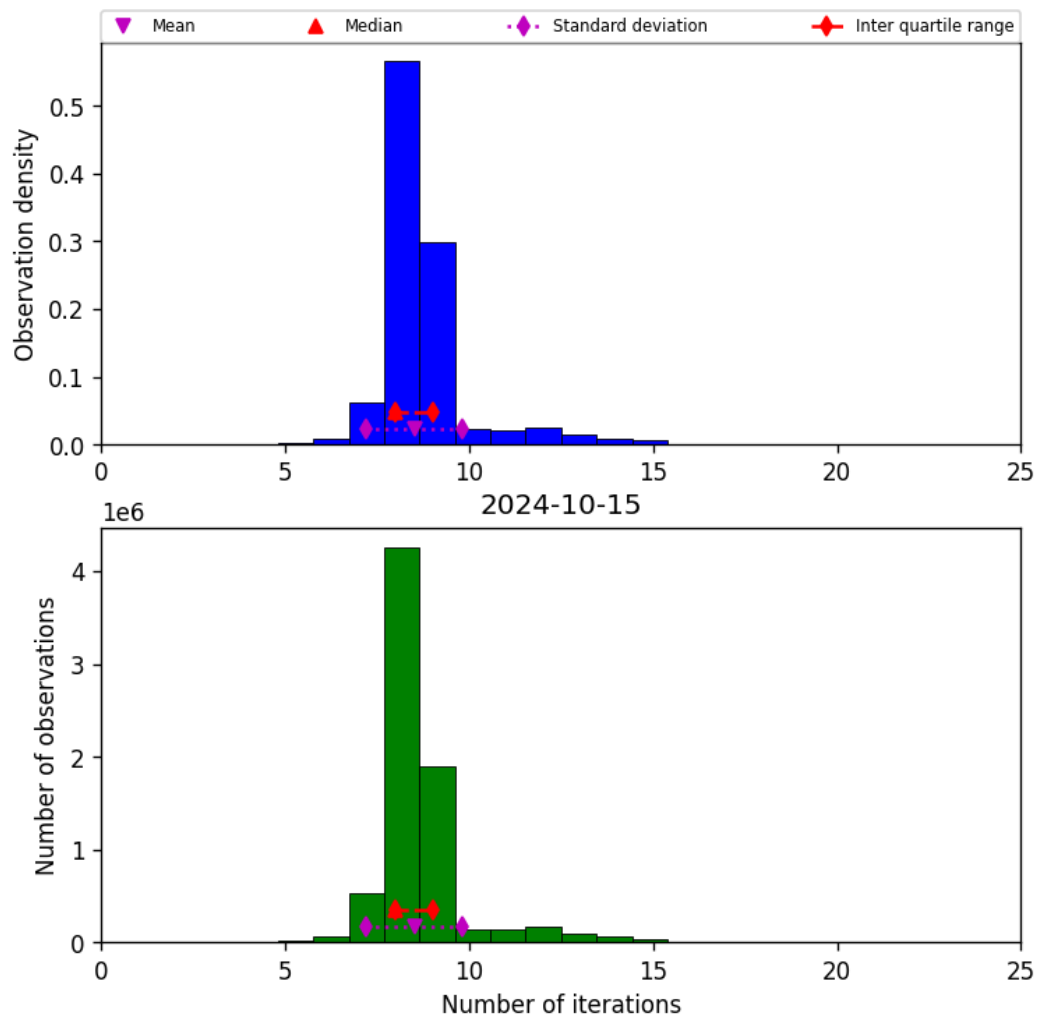
Figure 24: Histogram of “Number of iterations” for 2024-10-14 to 2024-10-16
