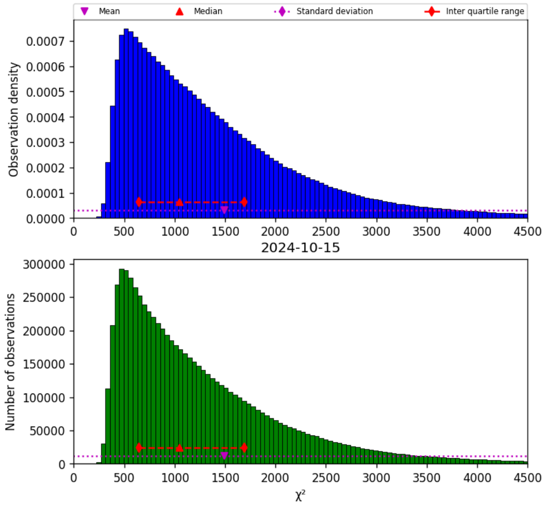
Figure 22: Histogram of “ \chi^2 ” for 2024-10-14 to 2024-10-16
