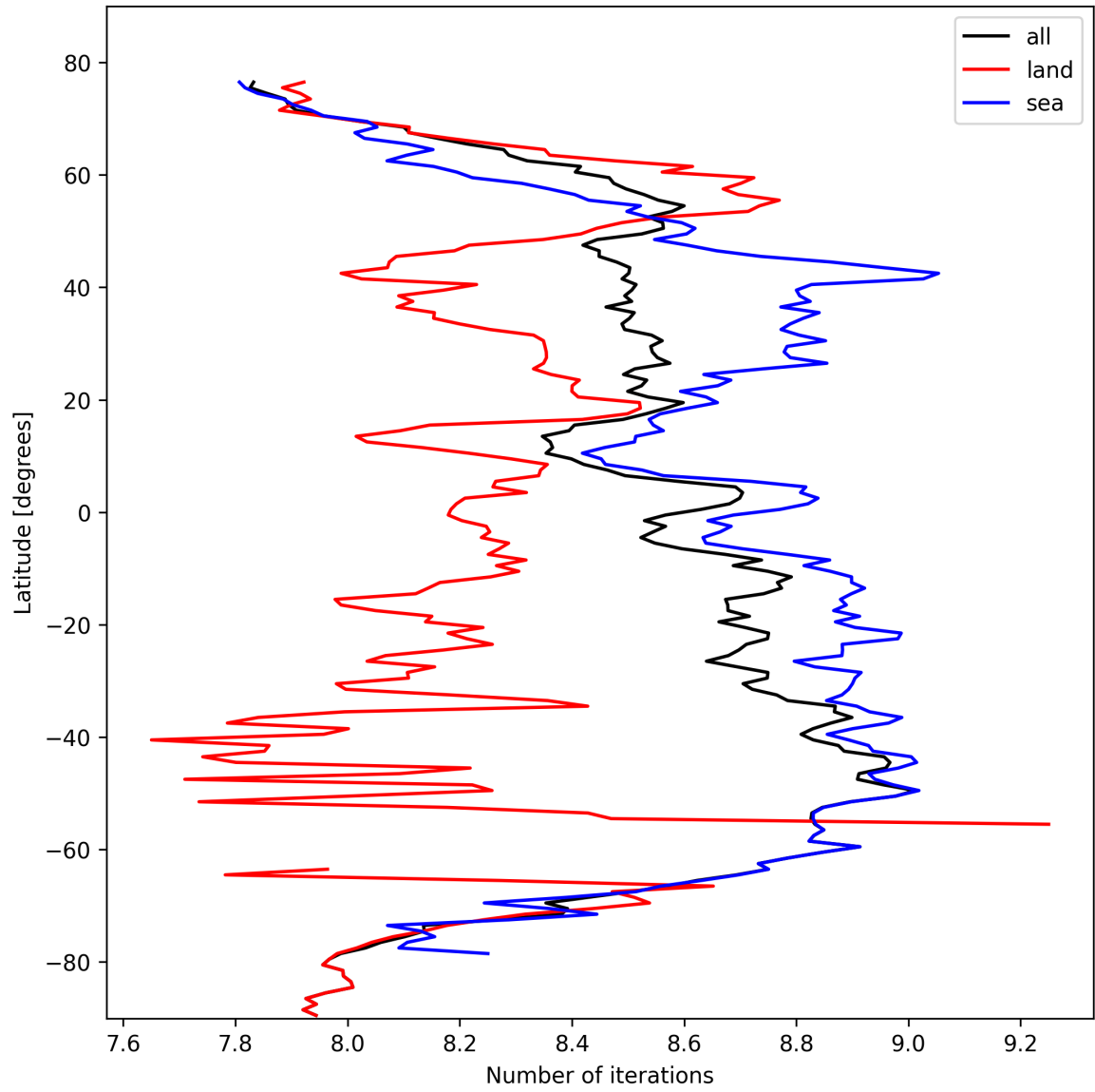
Figure 16: Zonal average of “Number of iterations” for 2024-10-14 to 2024-10-16.
