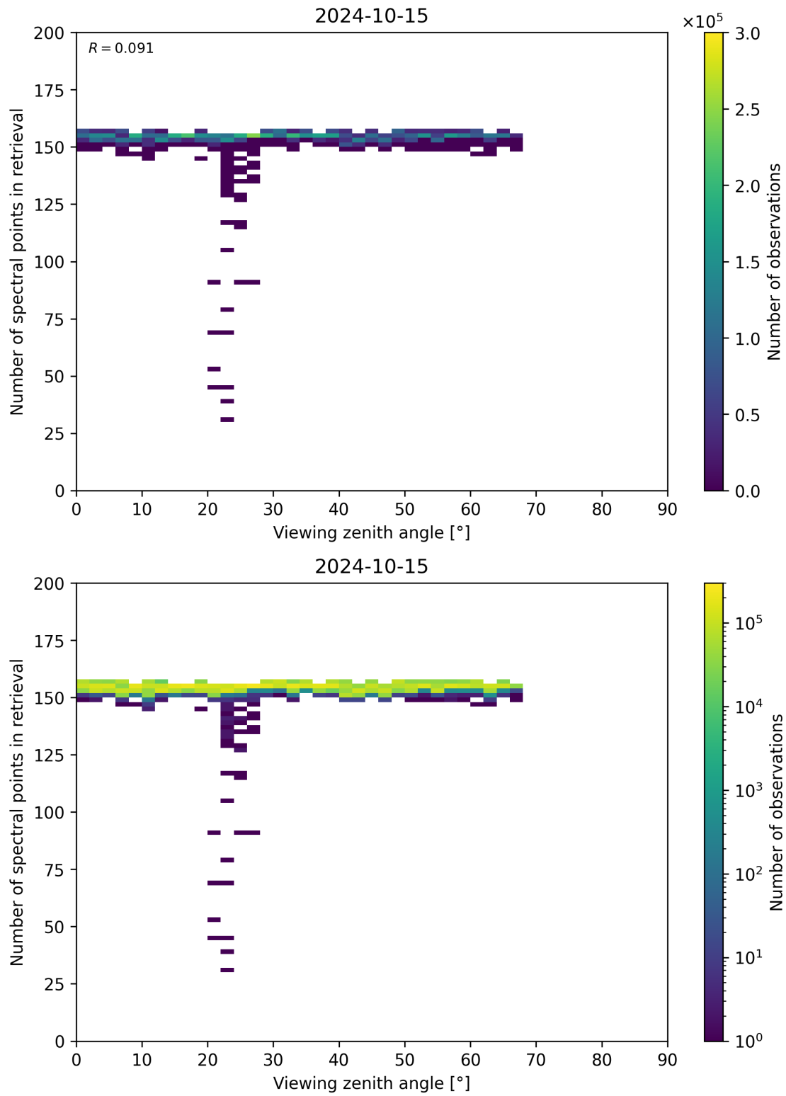
Figure 76: Scatter density plot of “Viewing zenith angle” against “Number of spectral points in retrieval” for 2024-10-14 to 2024-10-16.
