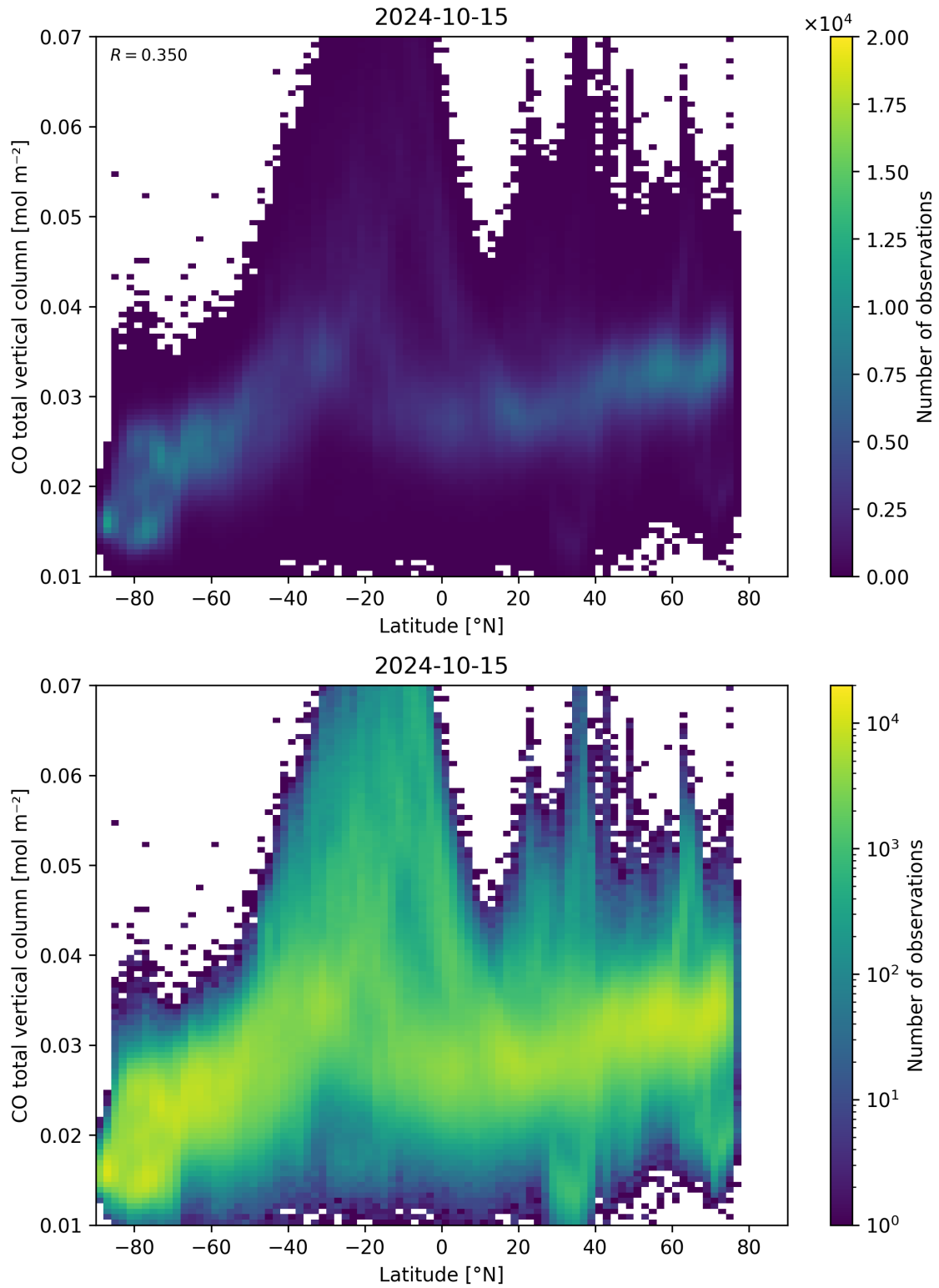
Figure 51: Scatter density plot of “Latitude” against “CO total vertical column” for 2024-10-14 to 2024-10-16.
