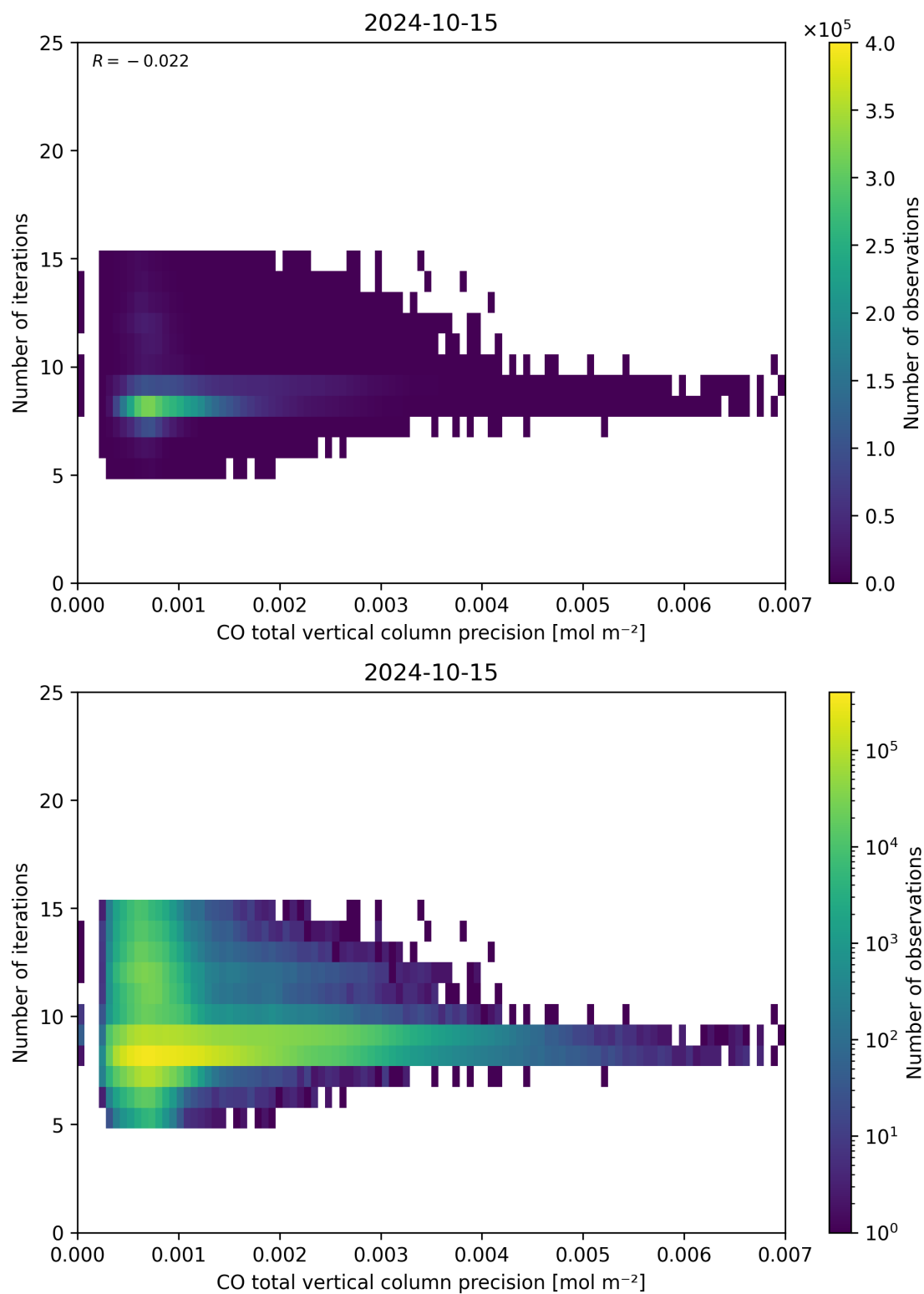
Figure 46: Scatter density plot of “CO total vertical column precision” against “Number of iterations” for 2024-10-14 to 2024-10-16.
