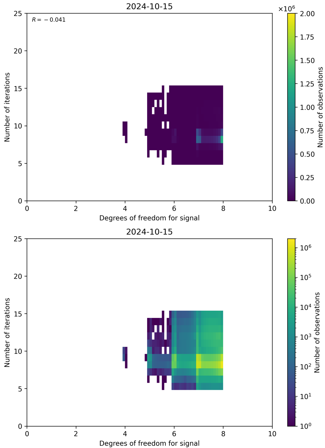
Figure 50: Scatter density plot of “Degrees of freedom for signal” against “Number of iterations” for 2024-10-14 to 2024-10-16.
