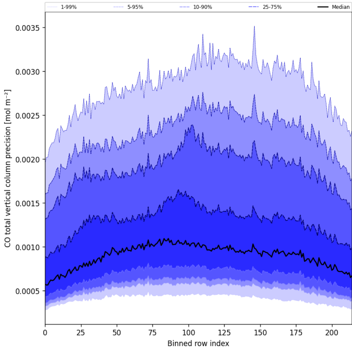
Figure 28: Along track statistics of “CO total vertical column precision” for 2024-10-14 to 2024-10-16
