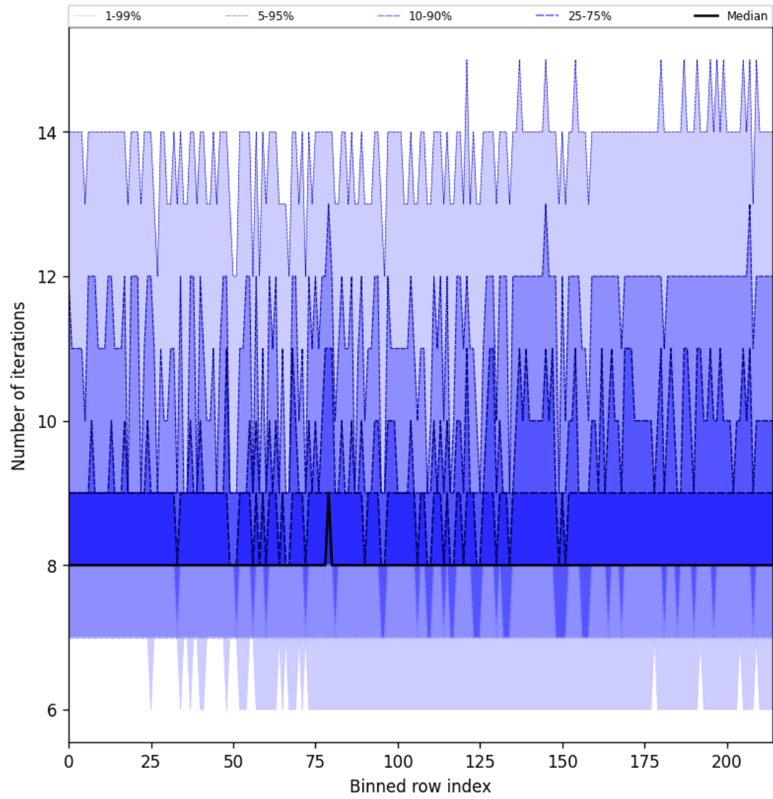
Figure 32: Along track statistics of “Number of iterations” for 2024-10-14 to 2024-10-16
