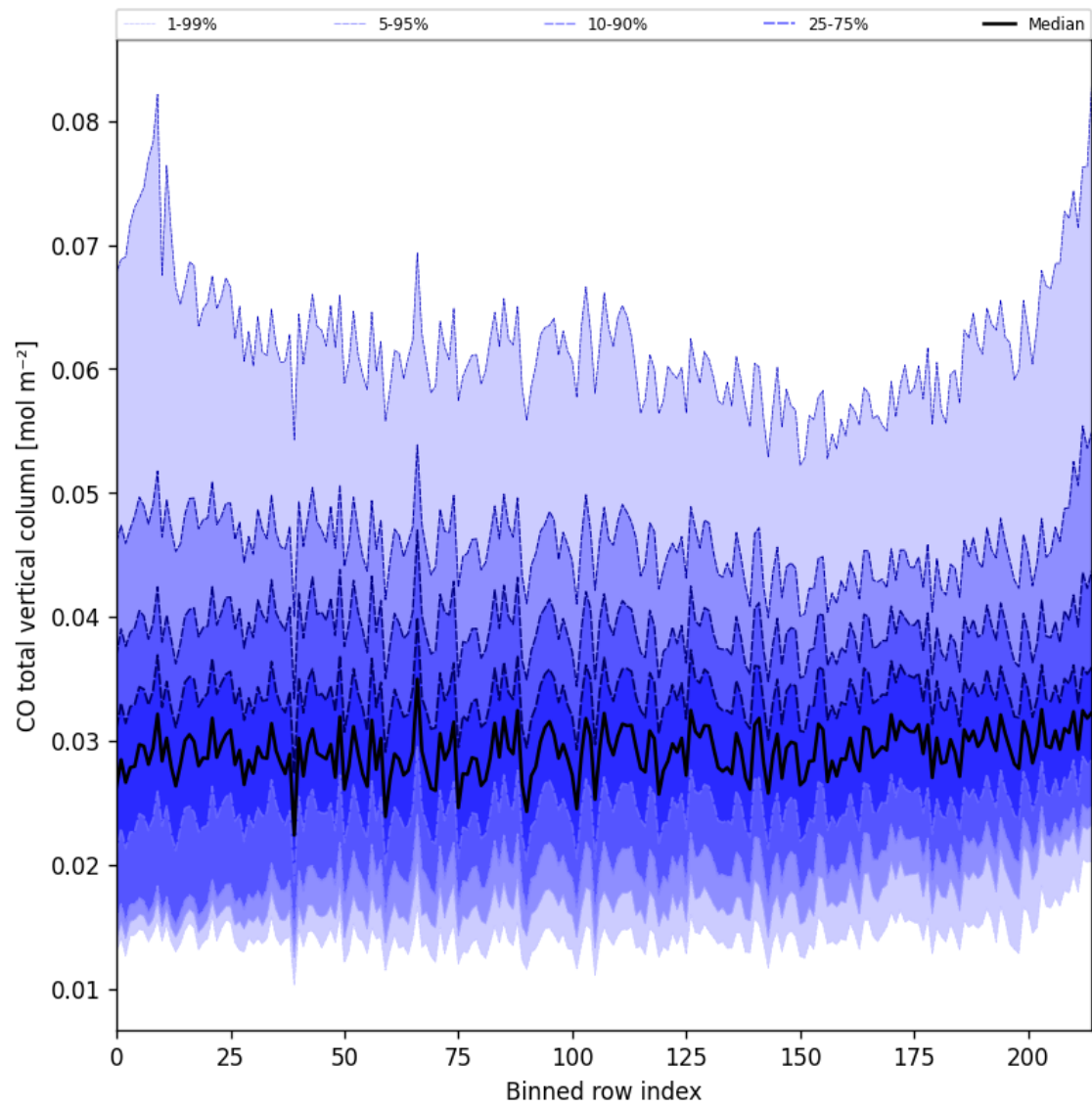
Figure 26: Along track statistics of “CO total vertical column” for 2024-10-14 to 2024-10-16
