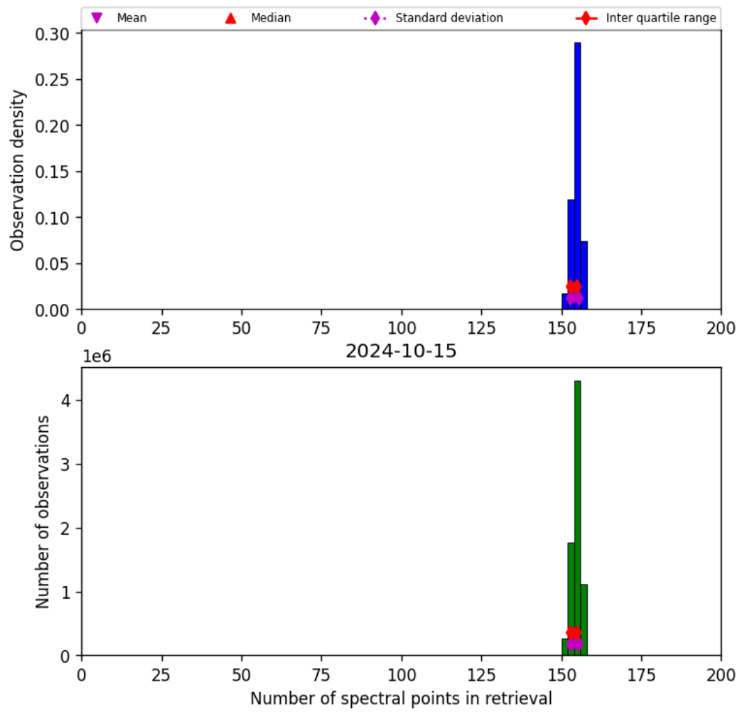
Figure 21: Histogram of “Number of spectral points in retrieval” for 2024-10-14 to 2024-10-16
