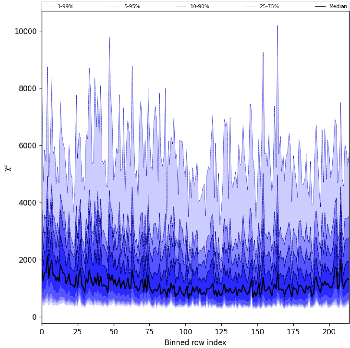
Figure 30: Along track statistics of “ \chi^2 ” for 2024-10-14 to 2024-10-16
