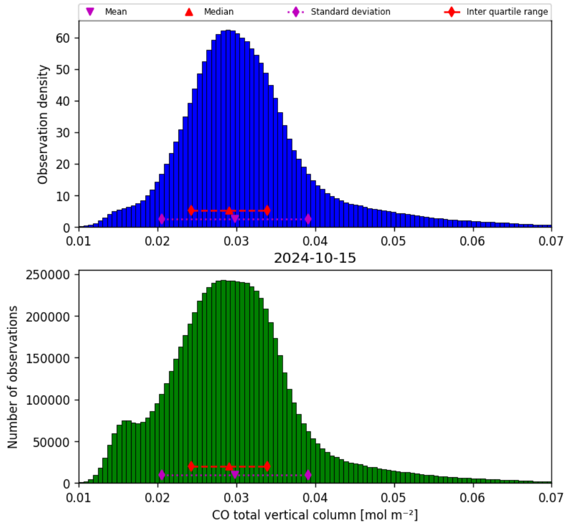
Figure 18: Histogram of “CO total vertical column” for 2024-10-14 to 2024-10-16
