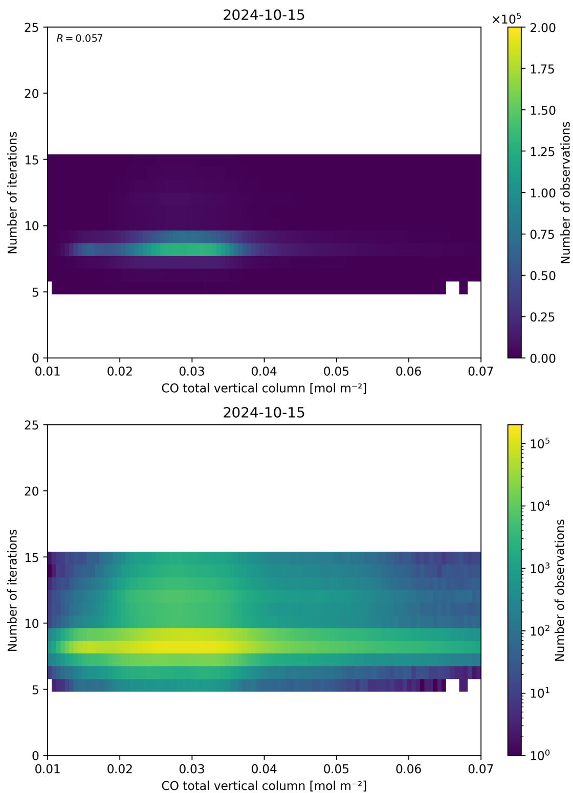
Figure 42: Scatter density plot of “CO total vertical column” against “Number of iterations” for 2024-10-14 to 2024-10-16.
