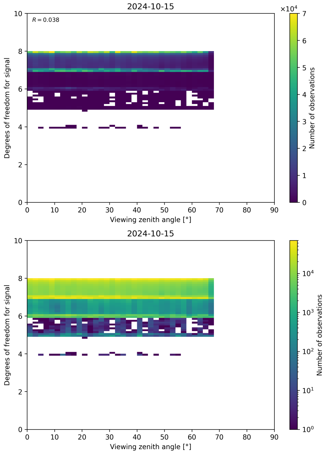
Figure 73: Scatter density plot of “Viewing zenith angle” against “Degrees of freedom for signal” for 2024-10-14 to 2024-10-16.
