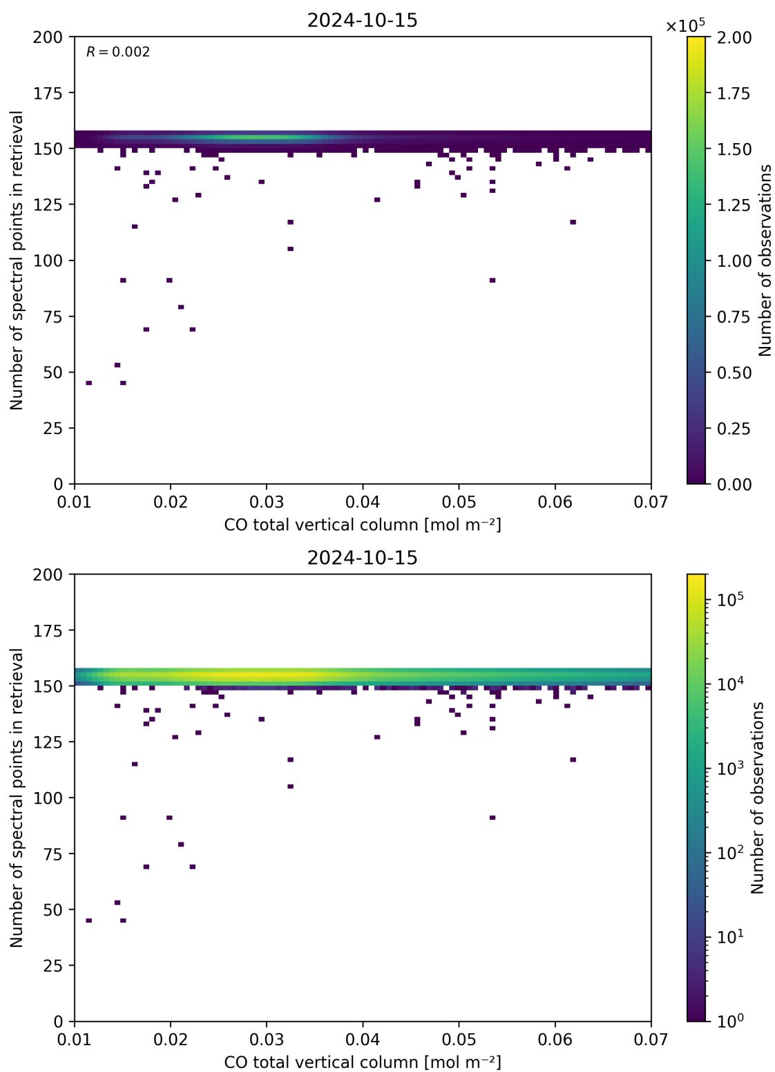
Figure 43: Scatter density plot of “CO total vertical column” against “Number of spectral points in retrieval” for 2024-10-14 to 2024-10-16.
