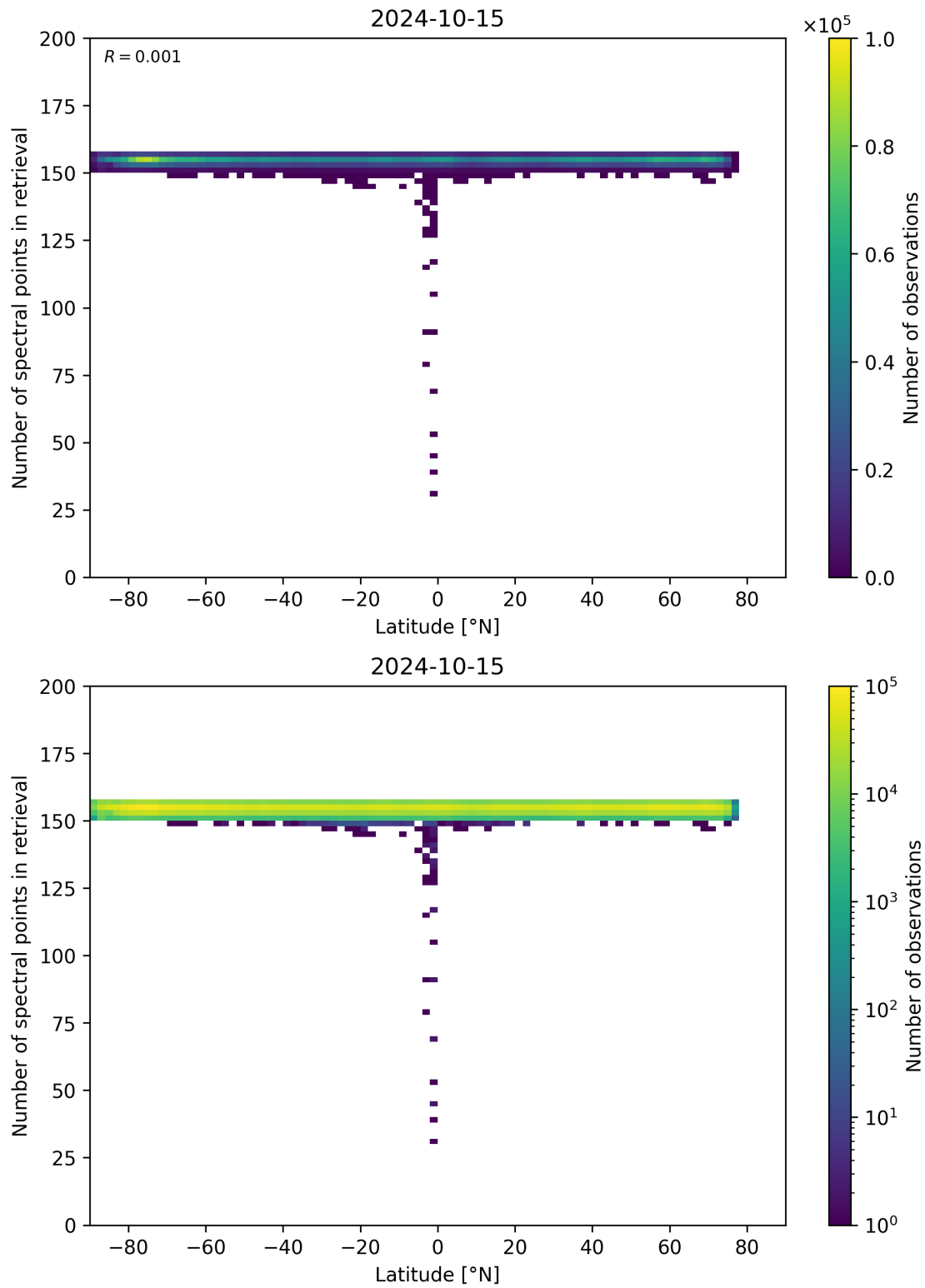
Figure 57: Scatter density plot of “Latitude” against “Number of spectral points in retrieval” for 2024-10-14 to 2024-10-16.
