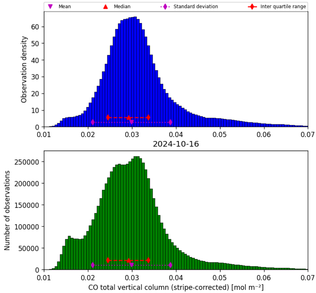
Figure 19: Histogram of “CO total vertical column (stripe-corrected)” for 2024-10-15 to 2024-10-17
