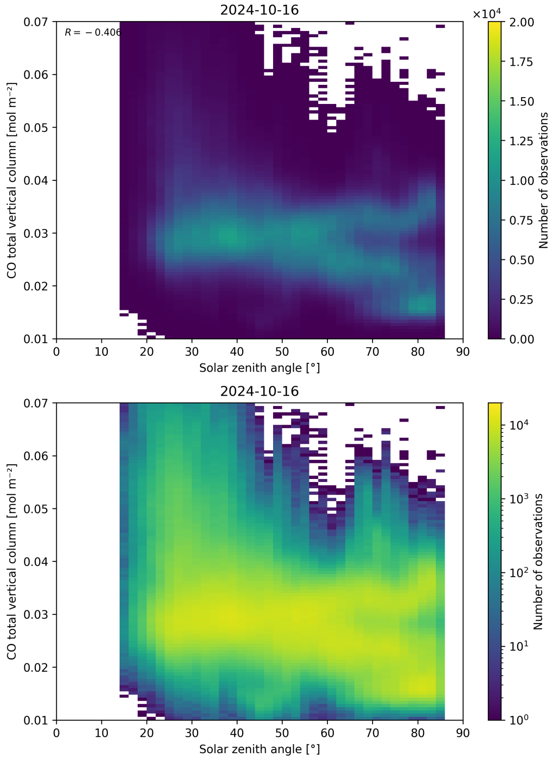
Figure 61: Scatter density plot of “Solar zenith angle” against “CO total vertical column” for 2024-10-15 to 2024-10-17.
