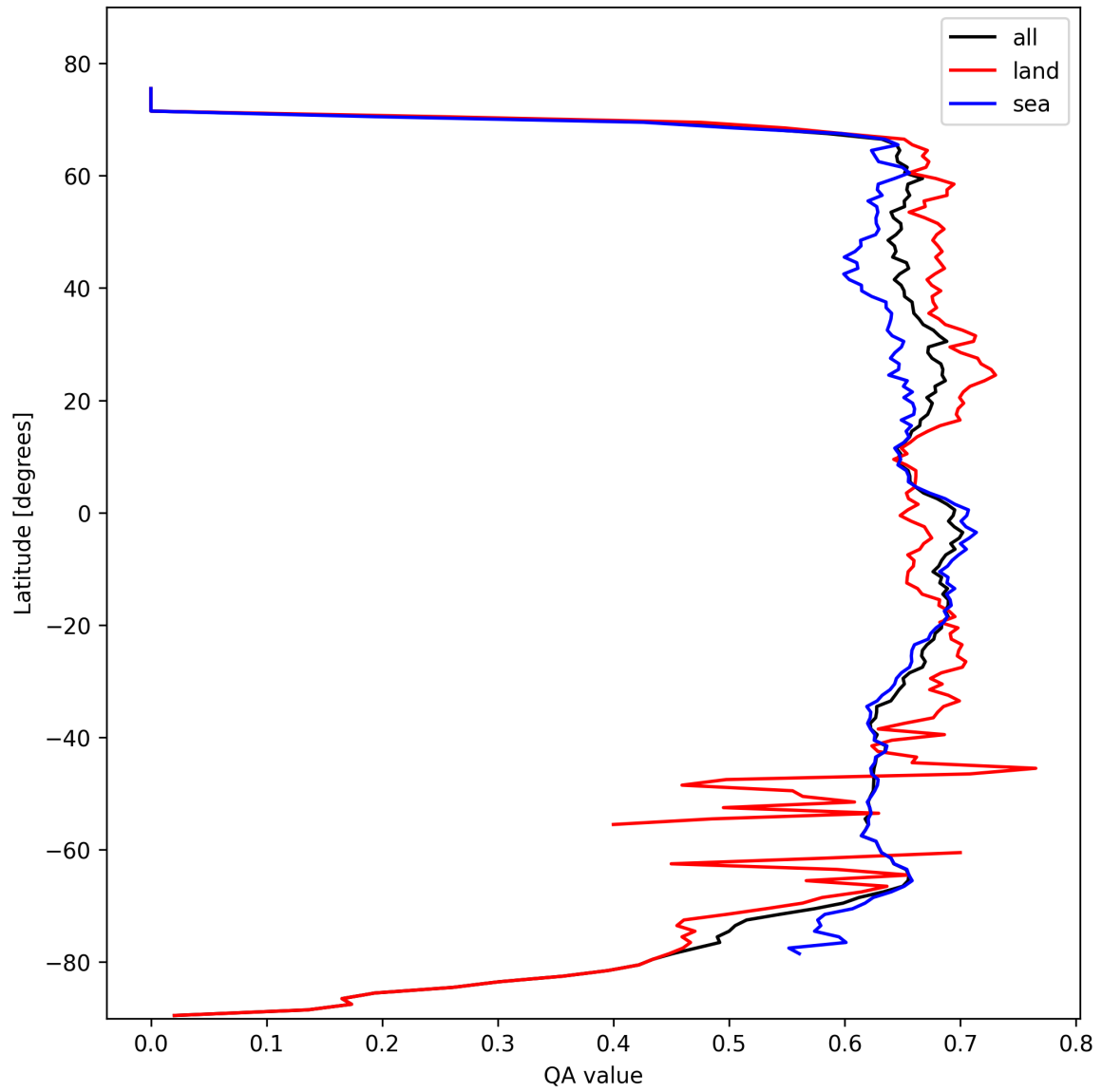
Figure 9: Zonal average of “QA value” for 2024-10-15 to 2024-10-17.
