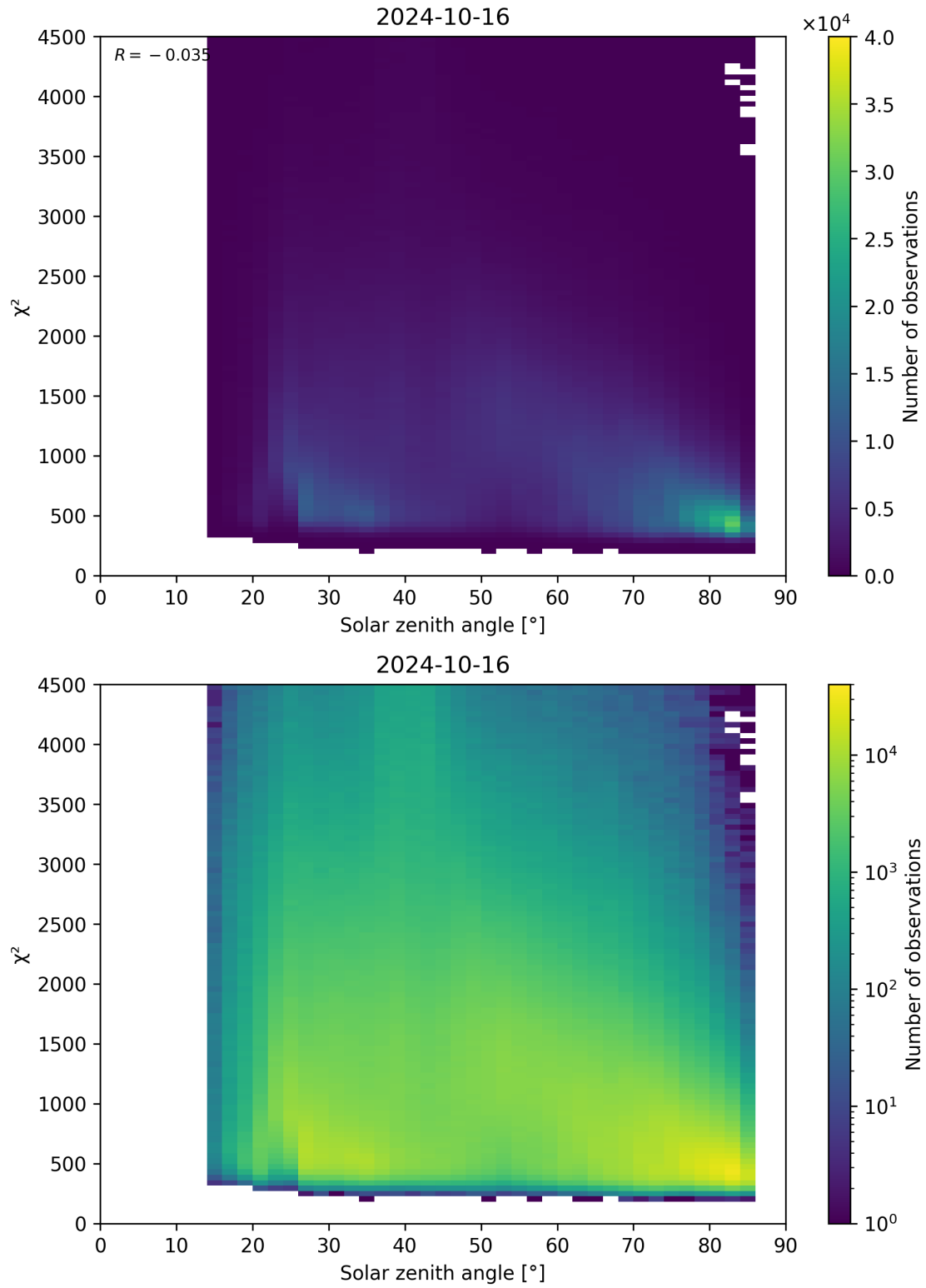
Figure 64: Scatter density plot of “Solar zenith angle” against “ \chi^2 ” for 2024-10-15 to 2024-10-17.
