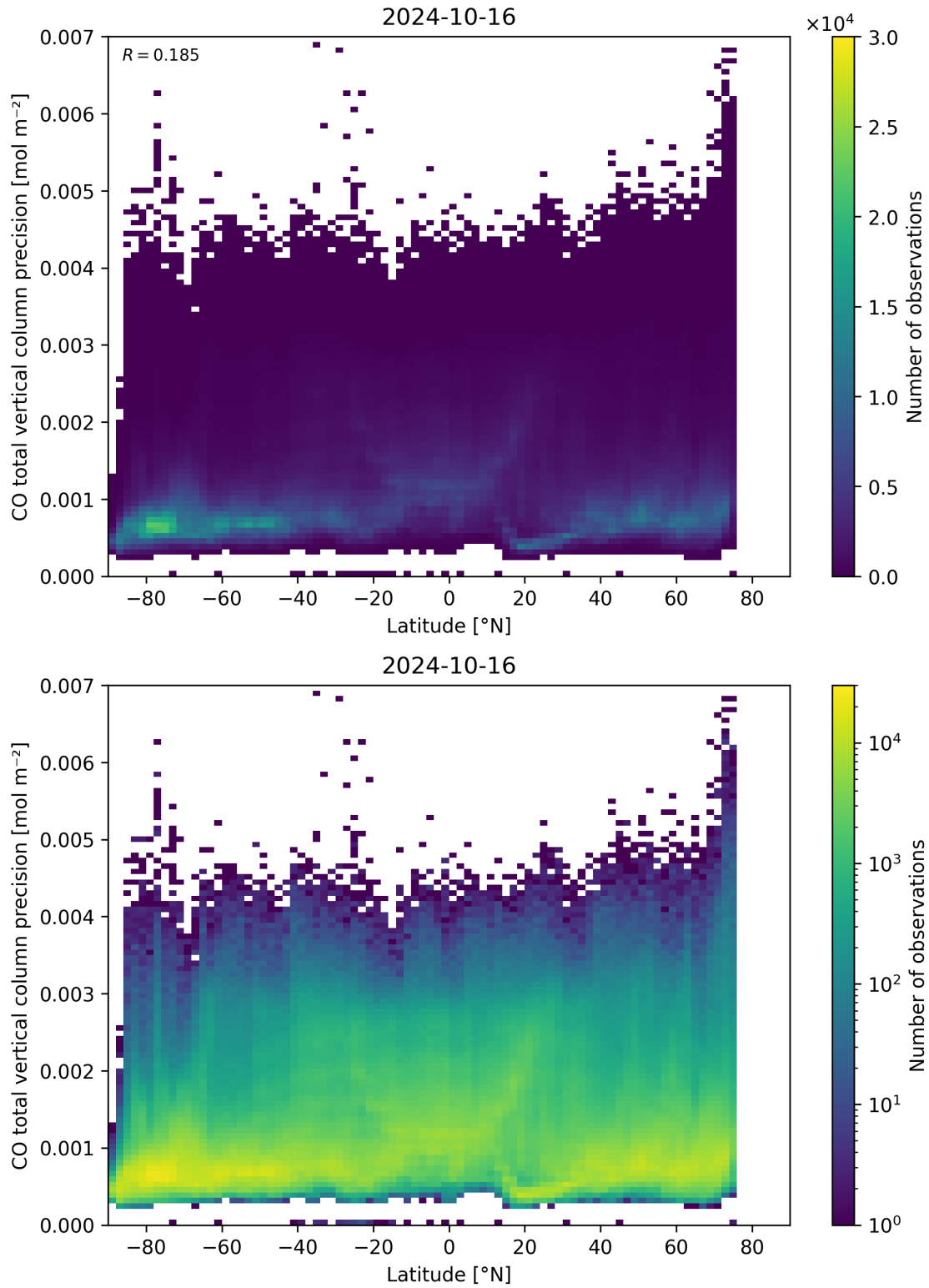
Figure 53: Scatter density plot of “Latitude” against “CO total vertical column precision” for 2024-10-15 to 2024-10-17.
