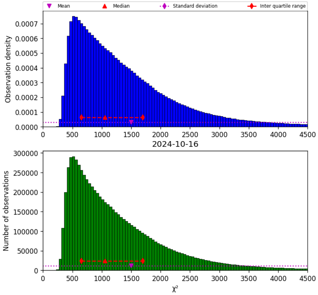
Figure 22: Histogram of “ \chi^2 ” for 2024-10-15 to 2024-10-17
