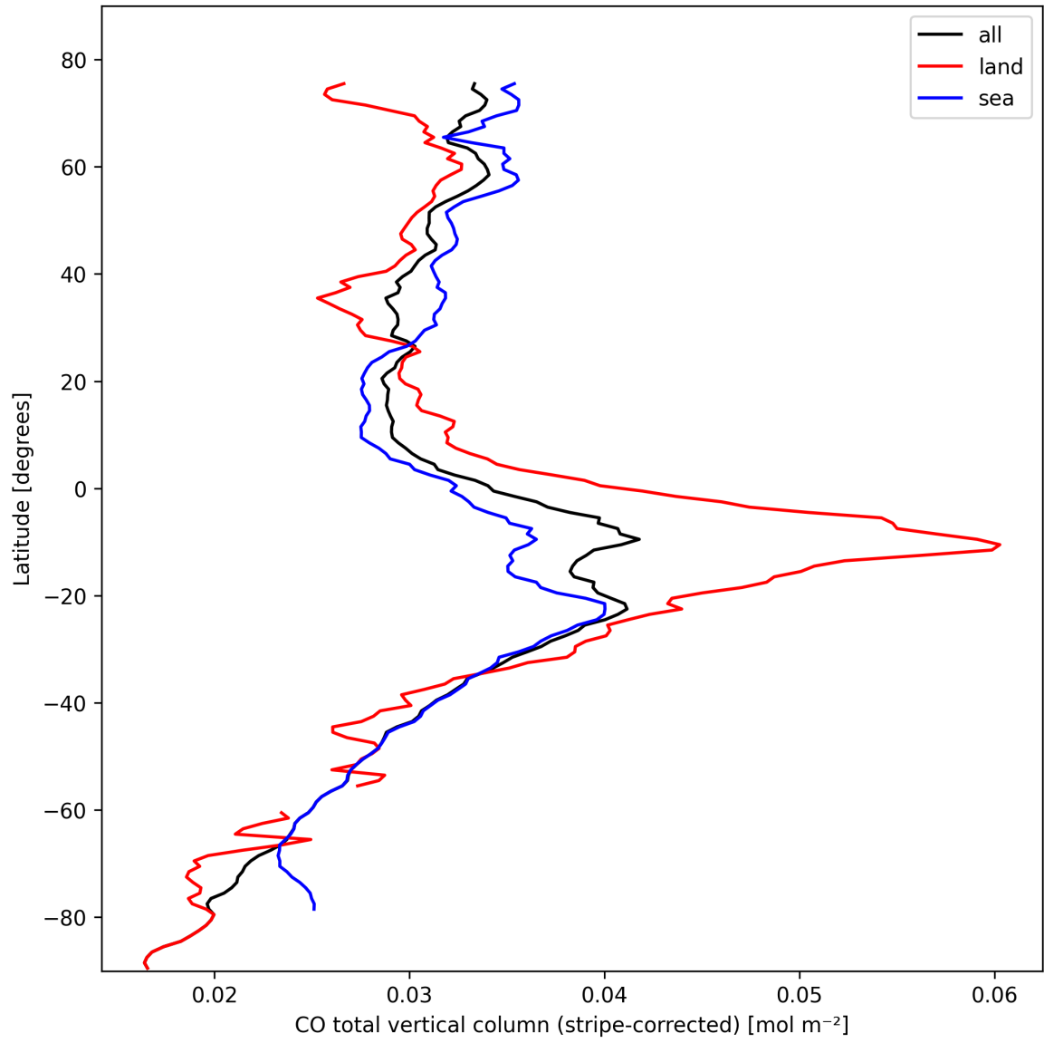
Figure 11: Zonal average of “CO total vertical column (stripe-corrected)” for 2024-10-15 to 2024-10-17.
