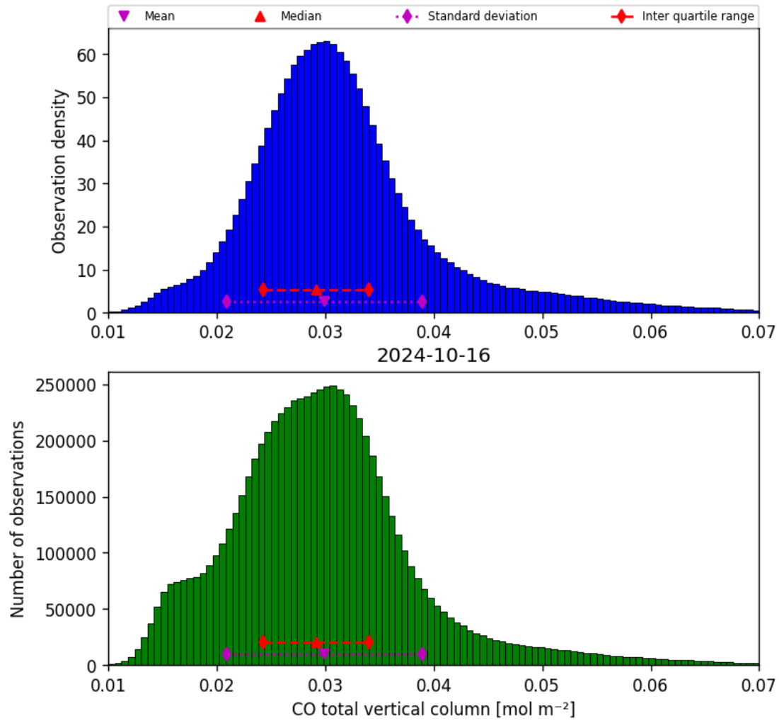
Figure 18: Histogram of “CO total vertical column” for 2024-10-15 to 2024-10-17
