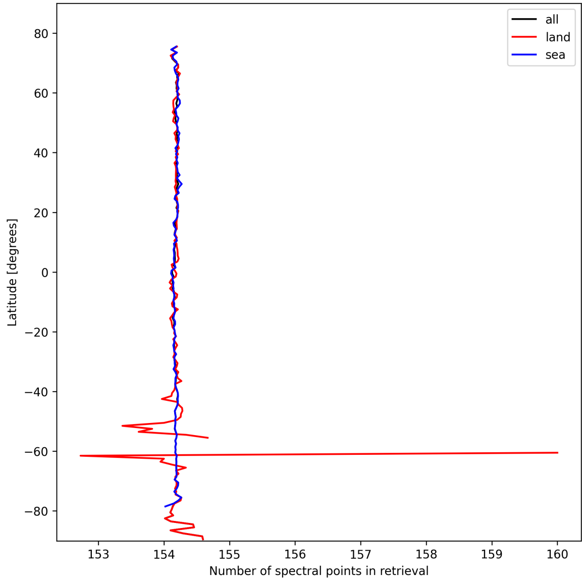
Figure 13: Zonal average of “Number of spectral points in retrieval” for 2024-10-15 to 2024-10-17.
