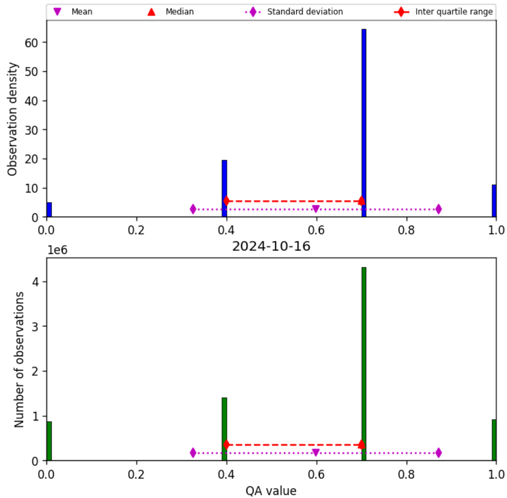
Figure 17: Histogram of “QA value” for 2024-10-15 to 2024-10-17
