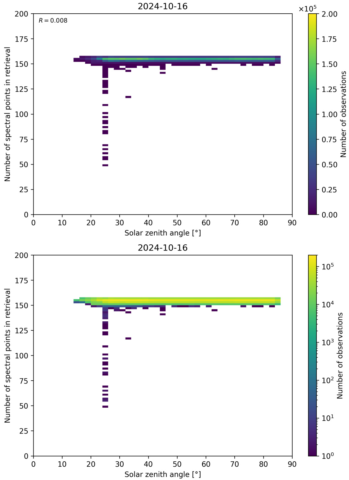
Figure 68: Scatter density plot of “Solar zenith angle” against “Number of spectral points in retrieval” for 2024-10-15 to 2024-10-17.
