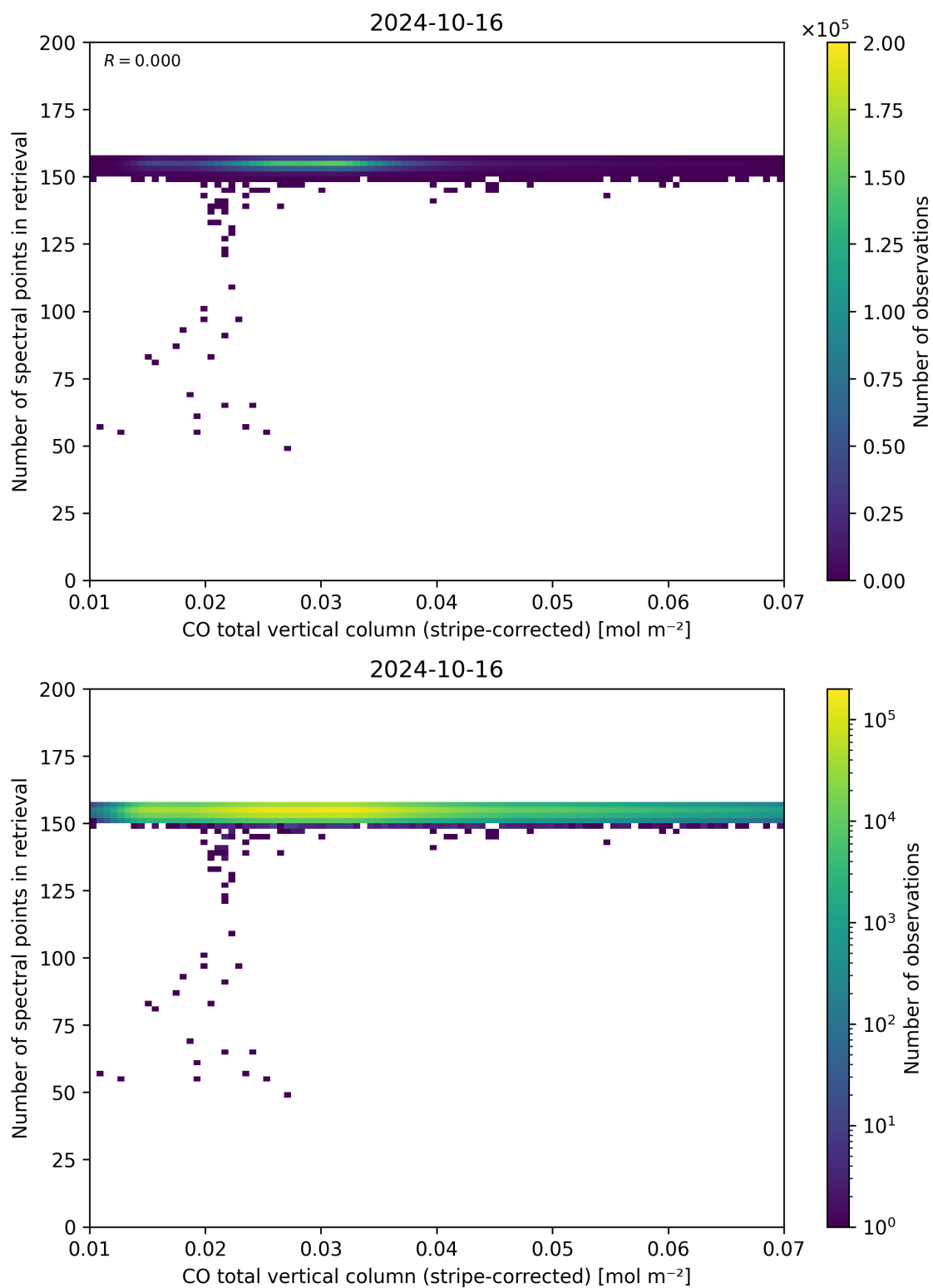
Figure 40: Scatter density plot of “CO total vertical column (stripe-corrected)” against “Number of spectral points in retrieval” for 2024-10-15 to 2024-10-17.
