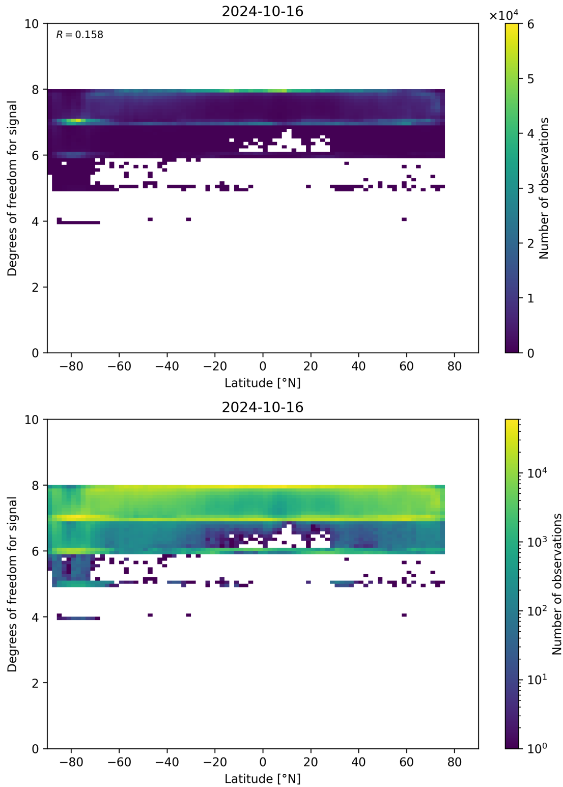
Figure 55: Scatter density plot of “Latitude” against “Degrees of freedom for signal” for 2024-10-15 to 2024-10-17.
