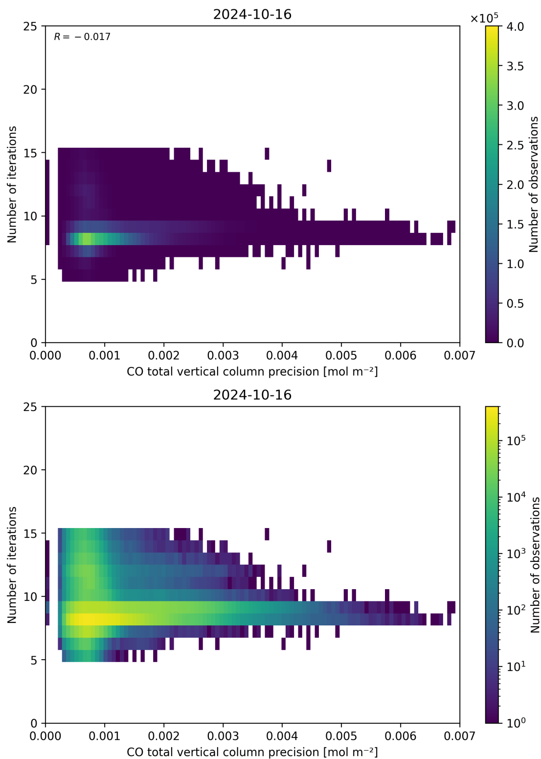
Figure 46: Scatter density plot of “CO total vertical column precision” against “Number of iterations” for 2024-10-15 to 2024-10-17.
