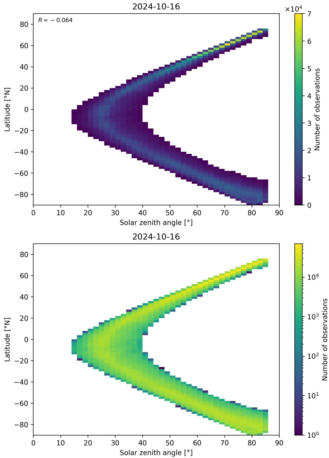
Figure 66: Scatter density plot of “Solar zenith angle” against “Latitude” for 2024-10-15 to 2024-10-17.
