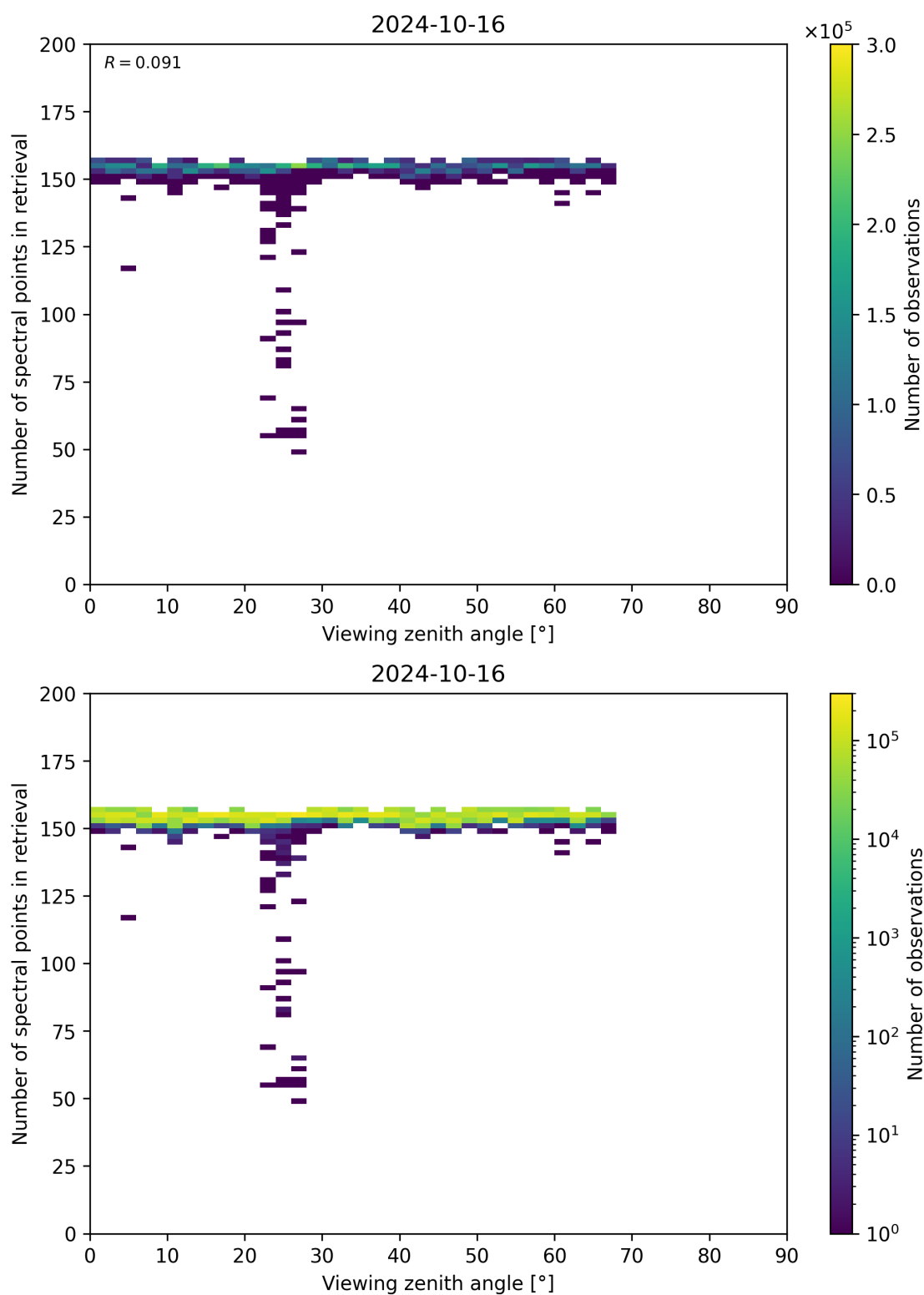
Figure 76: Scatter density plot of “Viewing zenith angle” against “Number of spectral points in retrieval” for 2024-10-15 to 2024-10-17.
