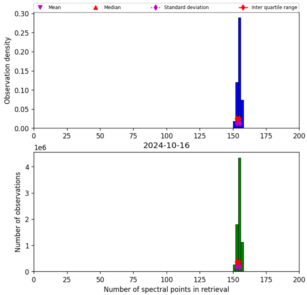
Figure 21: Histogram of “Number of spectral points in retrieval” for 2024-10-15 to 2024-10-17
