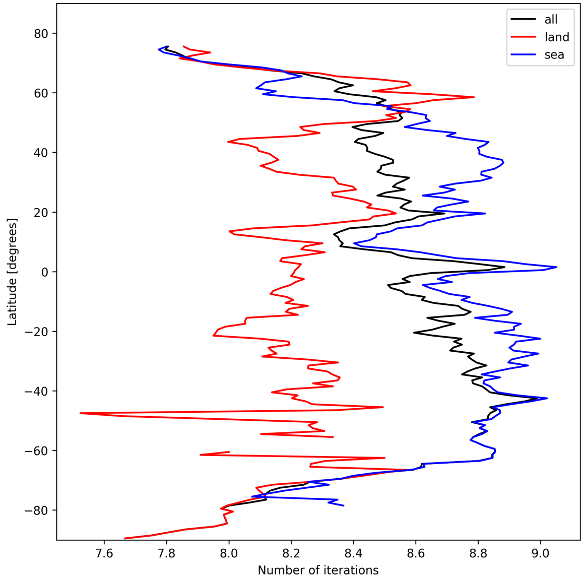
Figure 16: Zonal average of “Number of iterations” for 2024-10-15 to 2024-10-17.
