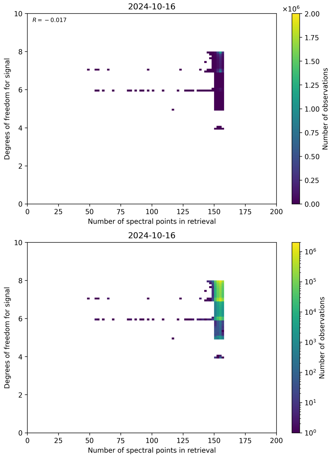
Figure 59: Scatter density plot of “Number of spectral points in retrieval” against “Degrees of freedom for signal” for 2024-10-15 to 2024-10-17.
