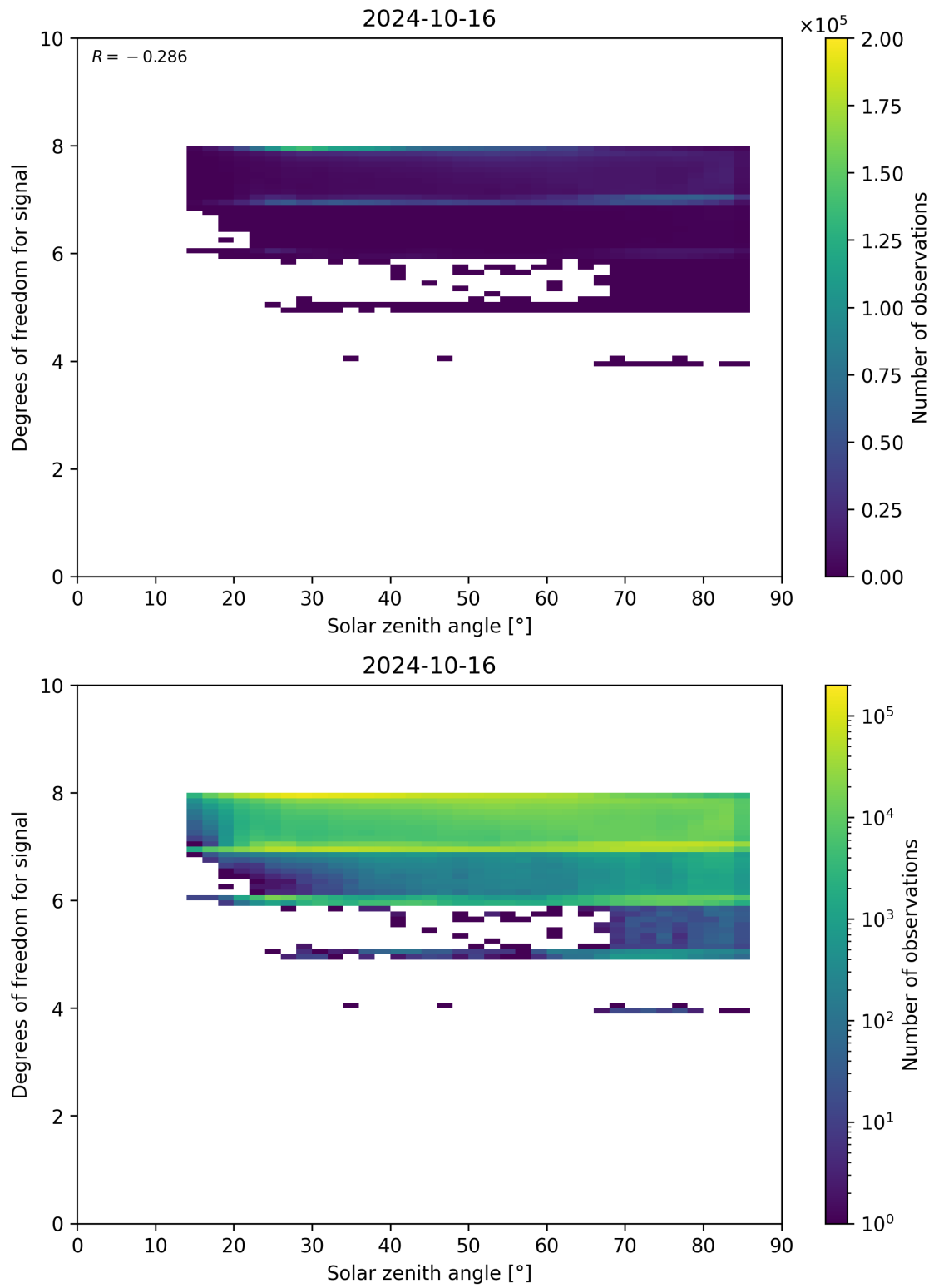
Figure 65: Scatter density plot of “Solar zenith angle” against “Degrees of freedom for signal” for 2024-10-15 to 2024-10-17.
