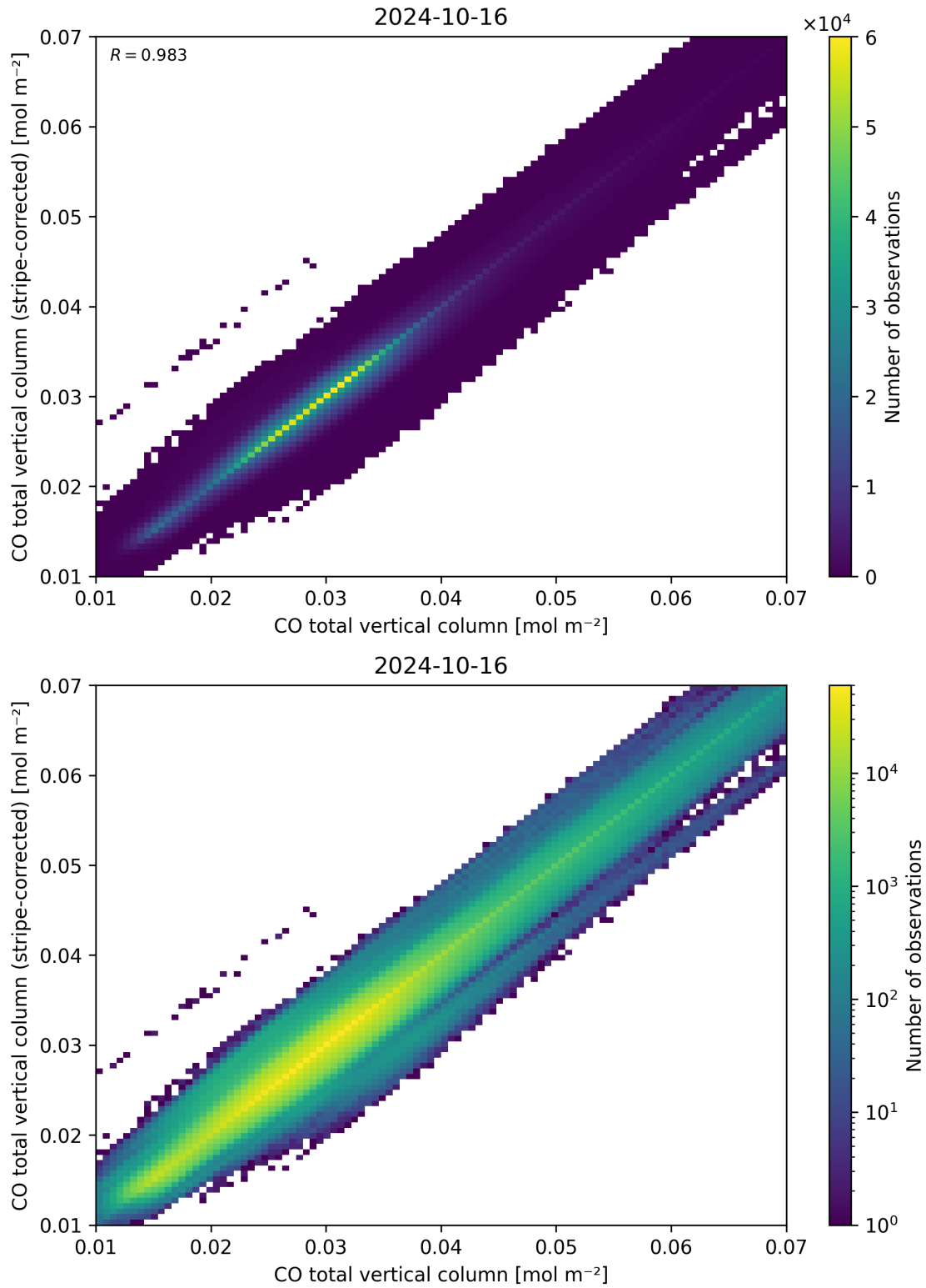
Figure 33: Scatter density plot of “CO total vertical column” against “CO total vertical column (stripe-corrected)” for 2024-10-15 to 2024-10-17.
