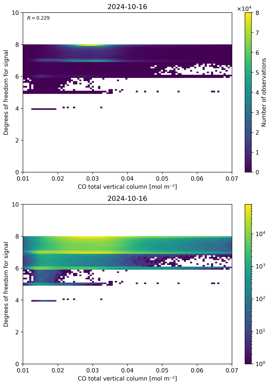
Figure 41: Scatter density plot of “CO total vertical column” against “Degrees of freedom for signal” for 2024-10-15 to 2024-10-17.
