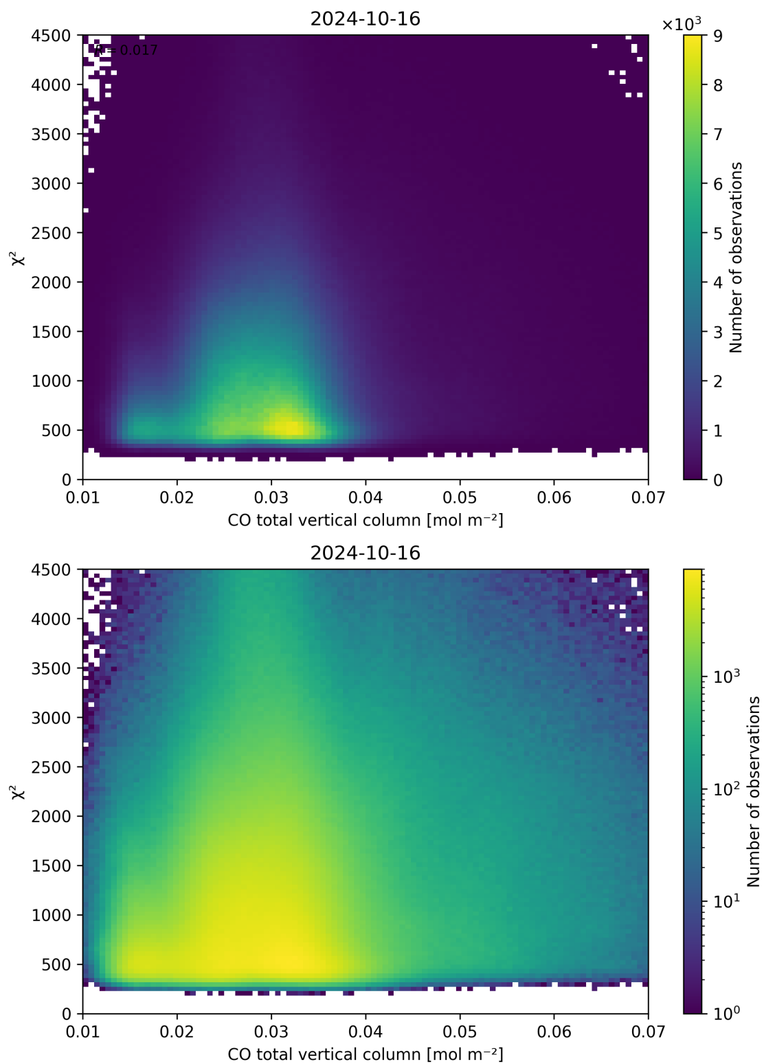
Figure 35: Scatter density plot of “CO total vertical column” against “ \chi^2 ” for 2024-10-15 to 2024-10-17.
