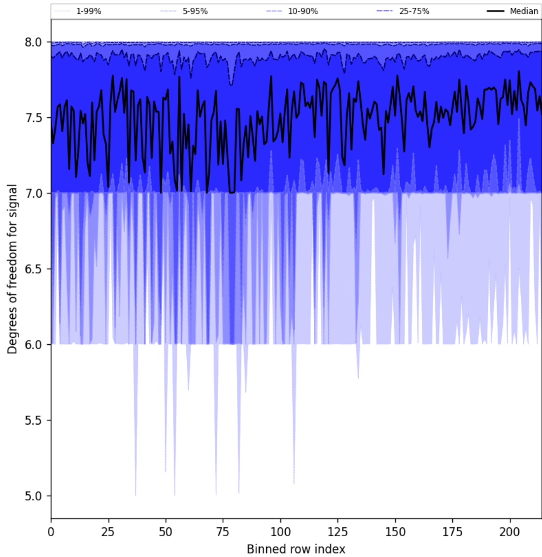
Figure 31: Along track statistics of “Degrees of freedom for signal” for 2024-10-15 to 2024-10-17
