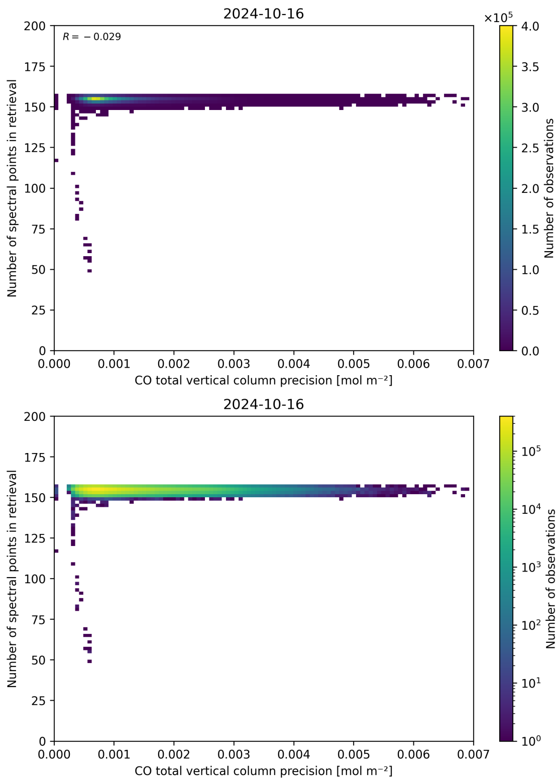
Figure 47: Scatter density plot of “CO total vertical column precision” against “Number of spectral points in retrieval” for 2024-10-15 to 2024-10-17.
