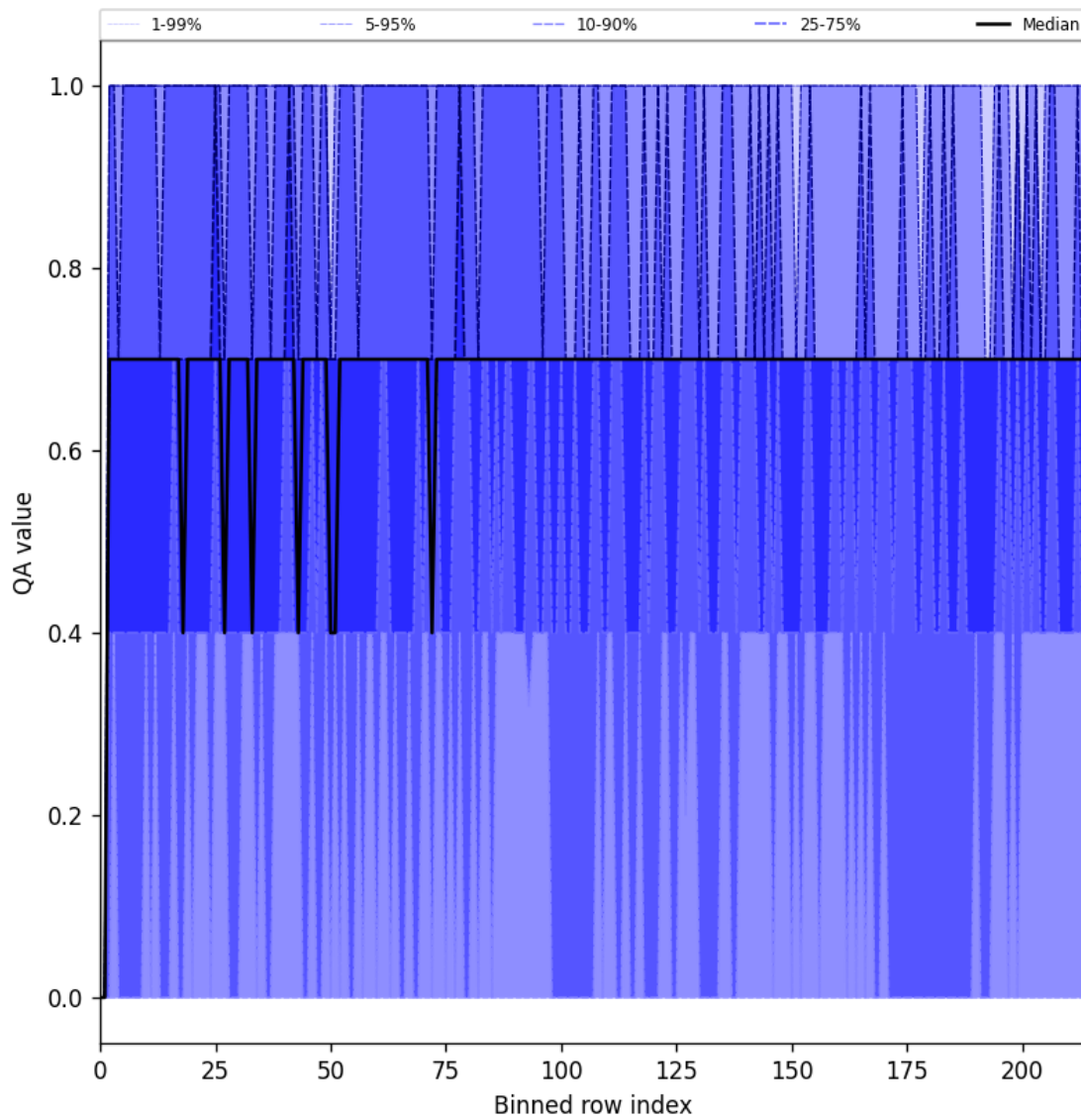
Figure 25: Along track statistics of “QA value” for 2024-10-15 to 2024-10-17
