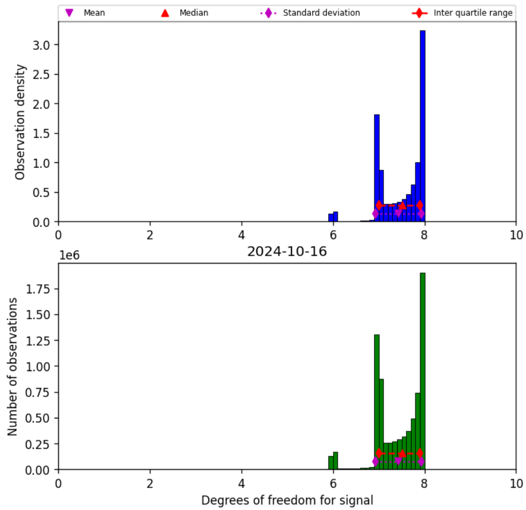
Figure 23: Histogram of “Degrees of freedom for signal” for 2024-10-15 to 2024-10-17
