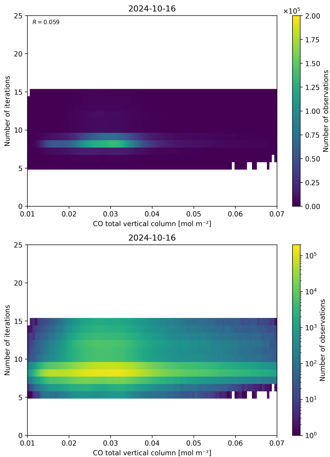
Figure 42: Scatter density plot of “CO total vertical column” against “Number of iterations” for 2024-10-15 to 2024-10-17.
