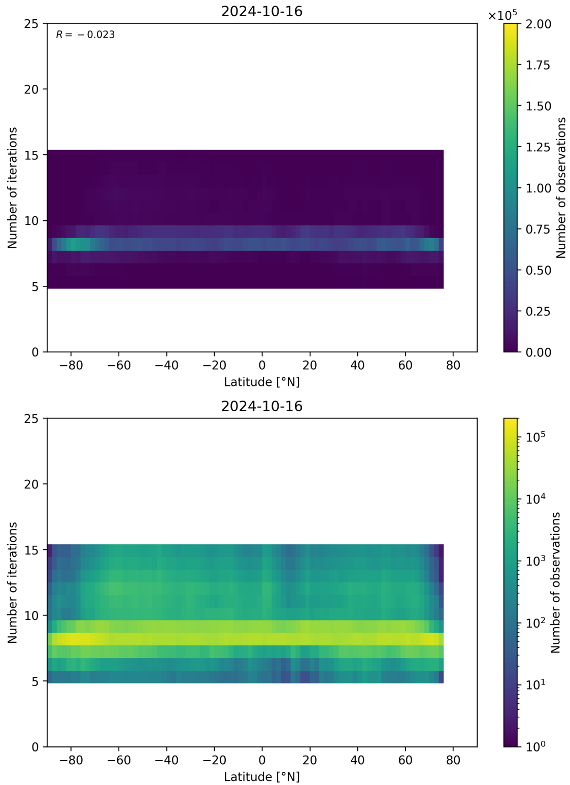
Figure 56: Scatter density plot of “Latitude” against “Number of iterations” for 2024-10-15 to 2024-10-17.
