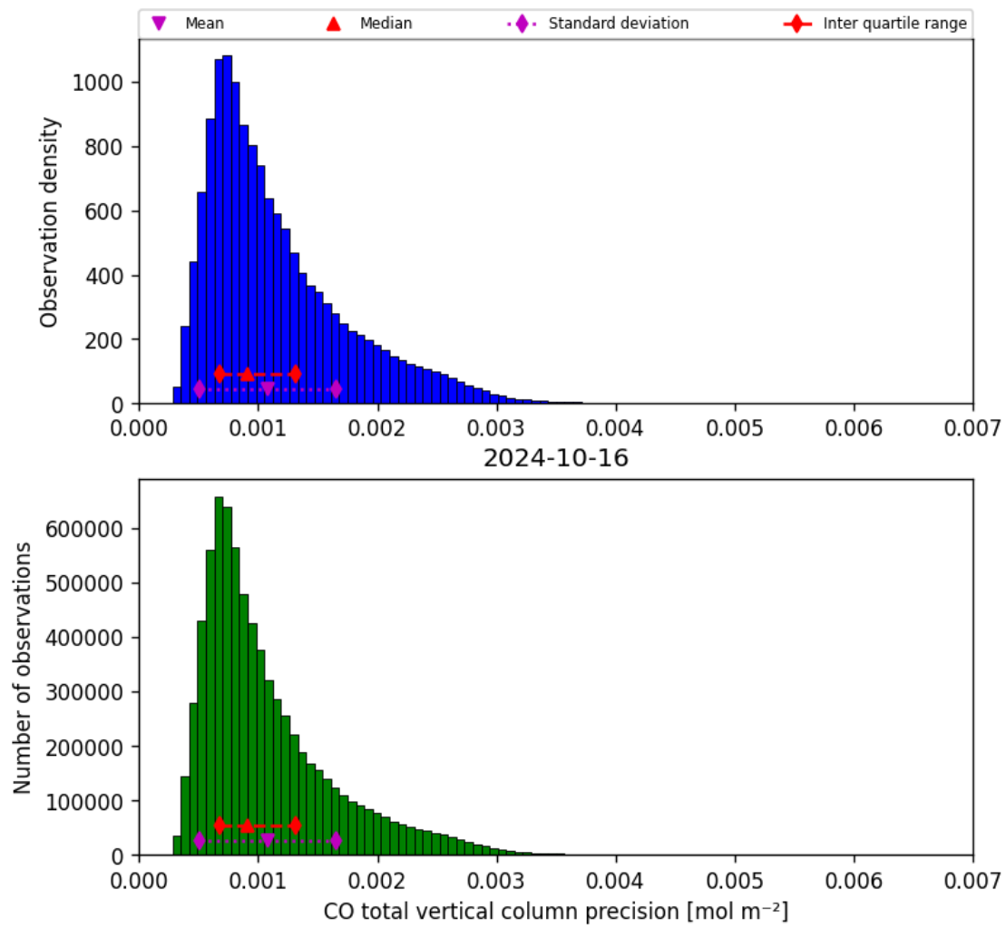
Figure 20: Histogram of “CO total vertical column precision” for 2024-10-15 to 2024-10-17
