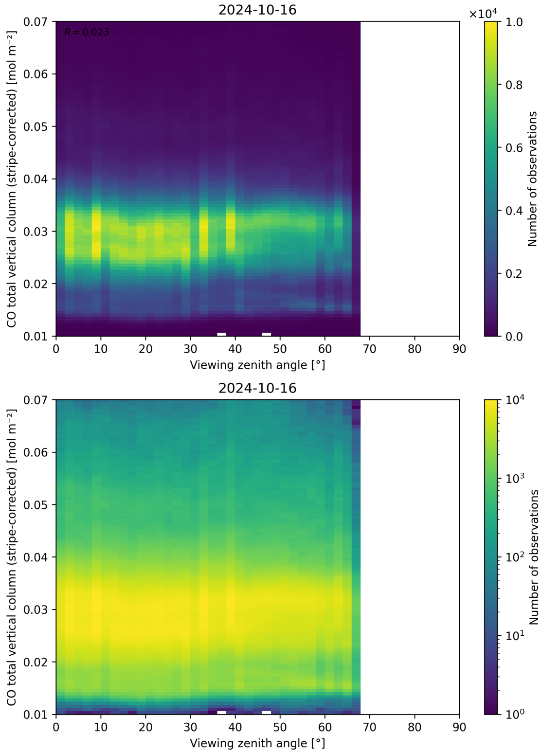
Figure 70: Scatter density plot of “Viewing zenith angle” against “CO total vertical column (stripe-corrected)” for 2024-10-15 to 2024-10-17.
