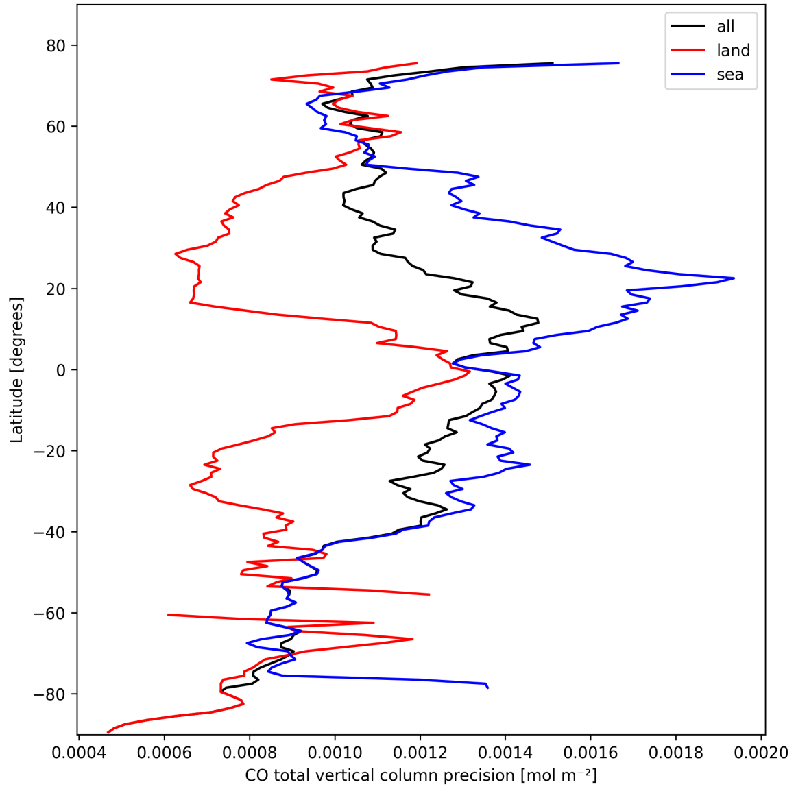
Figure 12: Zonal average of “CO total vertical column precision” for 2024-10-15 to 2024-10-17.
