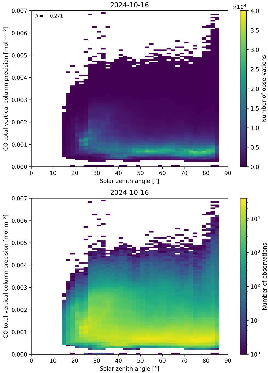
Figure 63: Scatter density plot of “Solar zenith angle” against “CO total vertical column precision” for 2024-10-15 to 2024-10-17.
