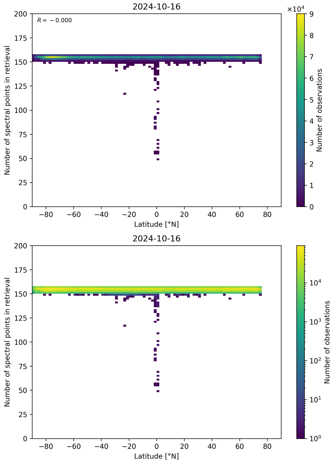
Figure 57: Scatter density plot of “Latitude” against “Number of spectral points in retrieval” for 2024-10-15 to 2024-10-17.
