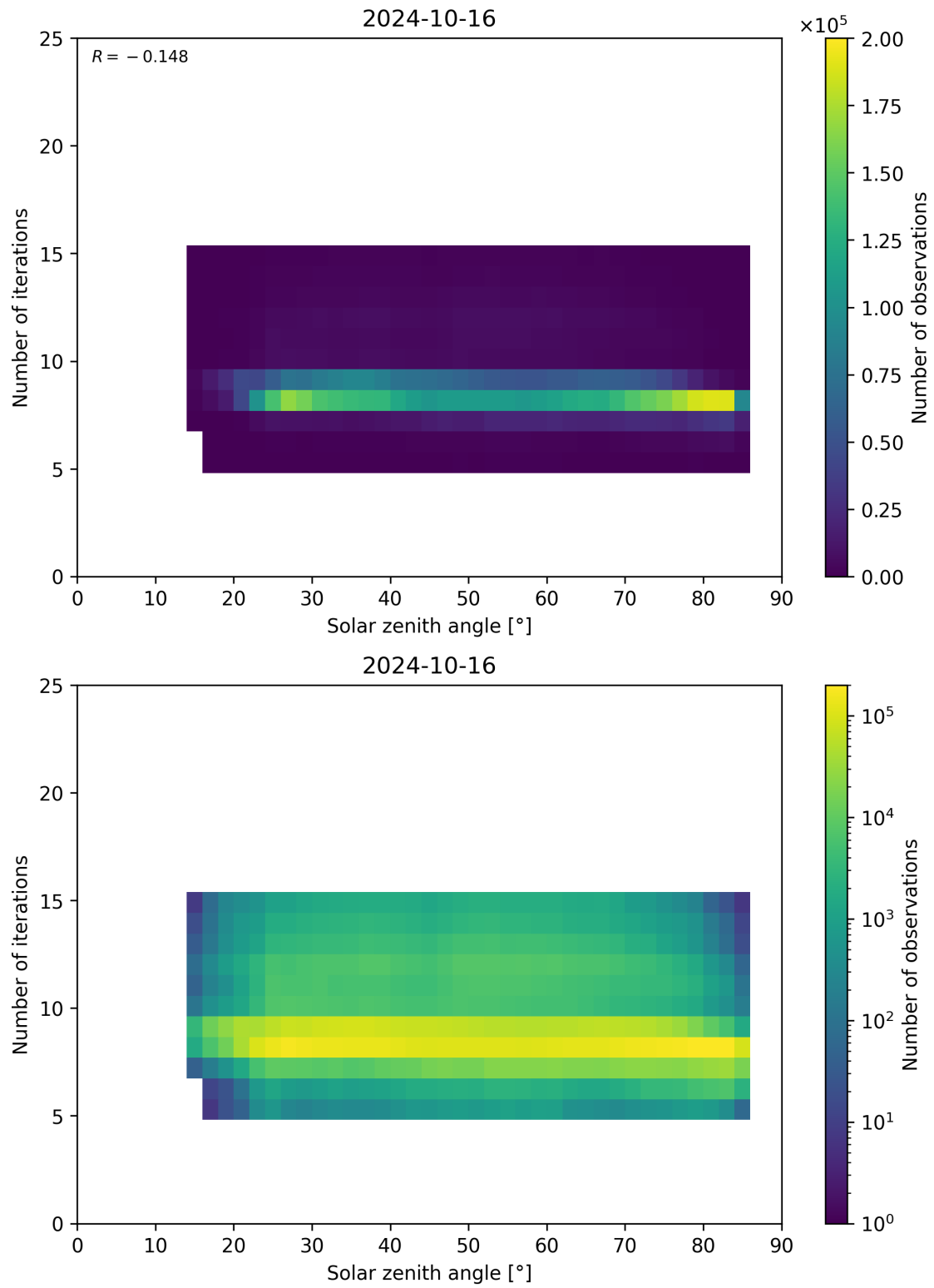
Figure 67: Scatter density plot of “Solar zenith angle” against “Number of iterations” for 2024-10-15 to 2024-10-17.
