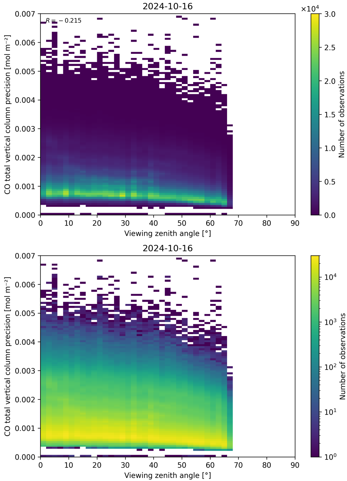
Figure 71: Scatter density plot of “Viewing zenith angle” against “CO total vertical column precision” for 2024-10-15 to 2024-10-17.
