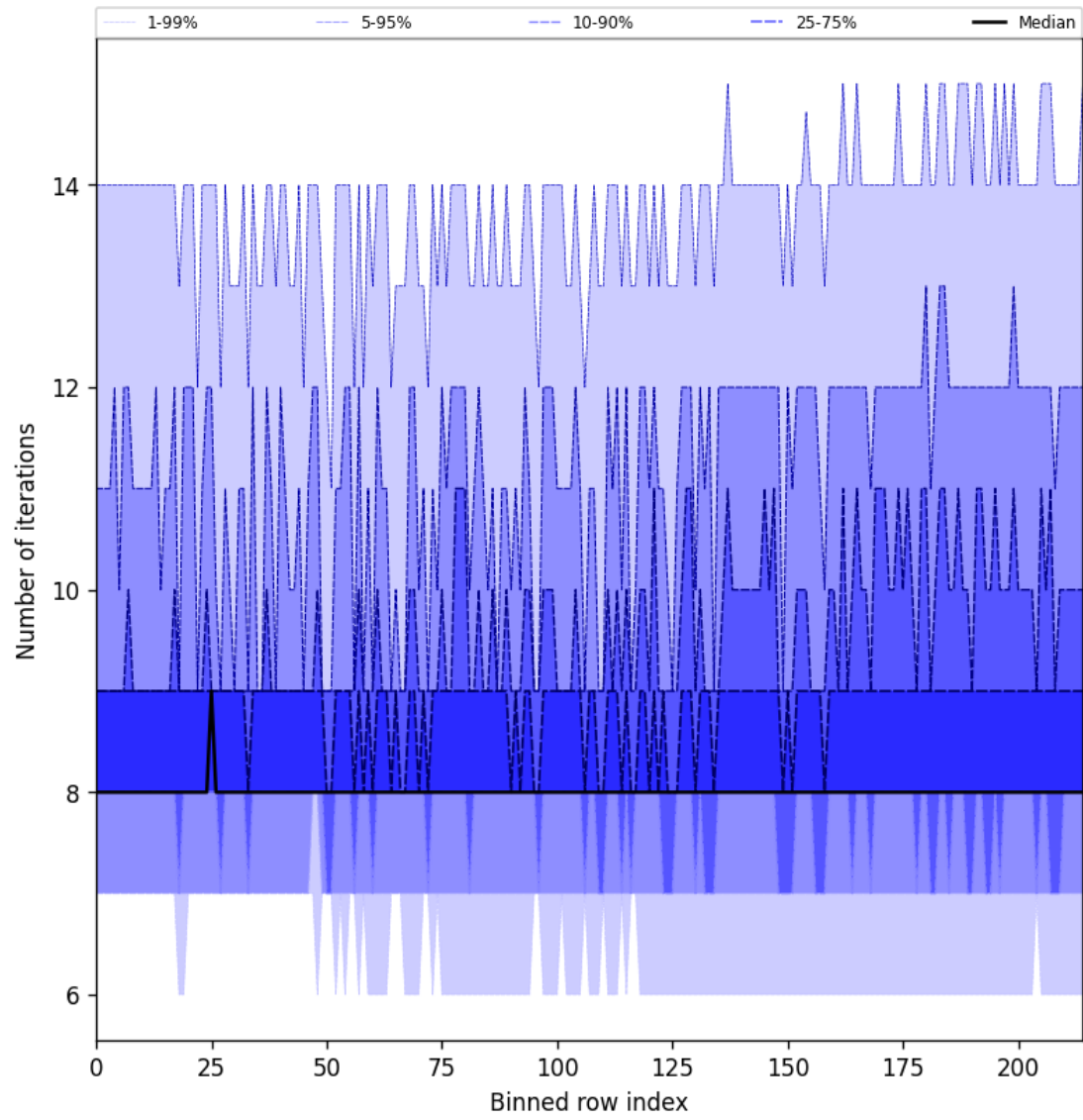
Figure 32: Along track statistics of “Number of iterations” for 2024-10-15 to 2024-10-17
