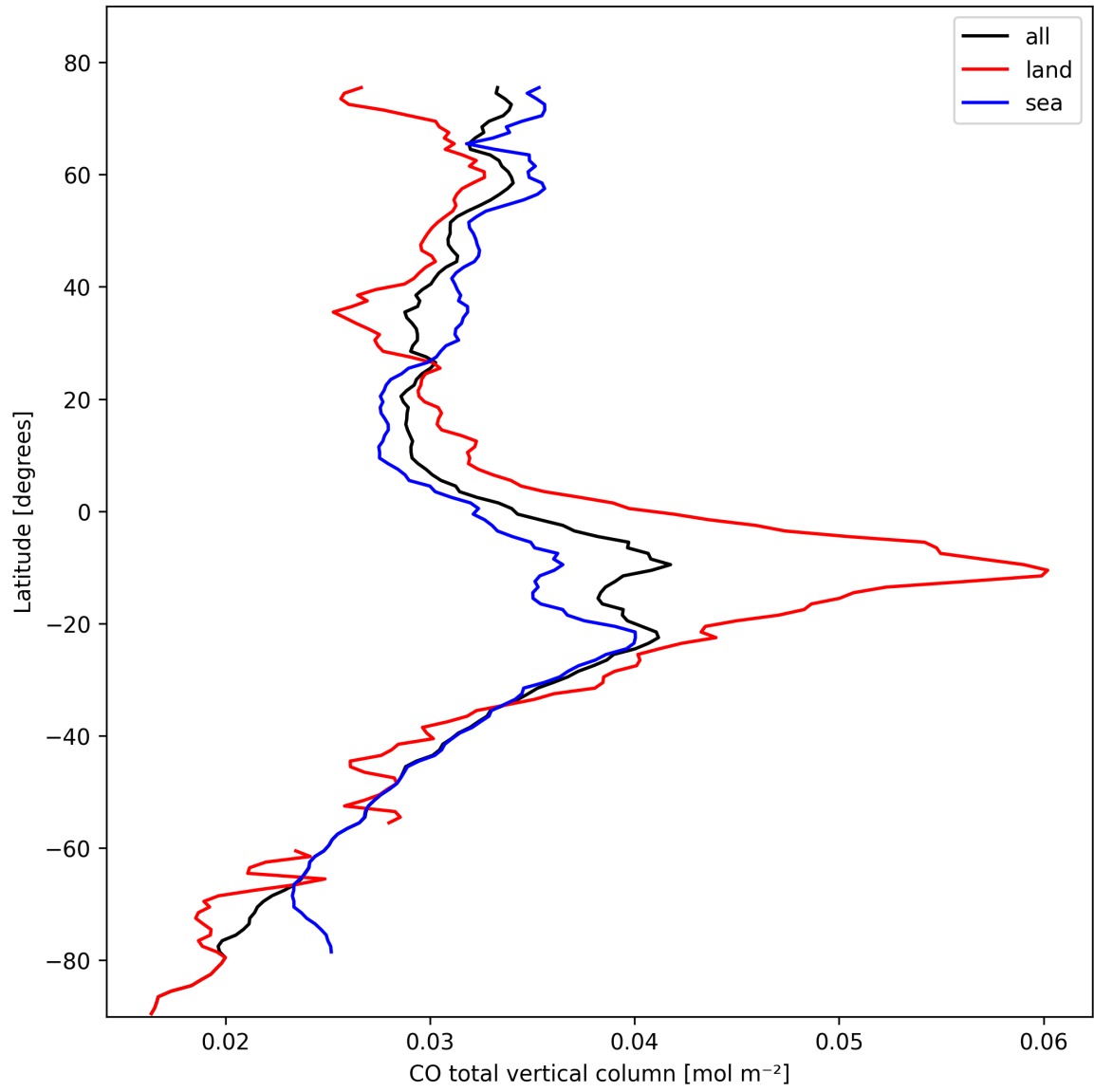
Figure 10: Zonal average of “CO total vertical column” for 2024-10-15 to 2024-10-17.
