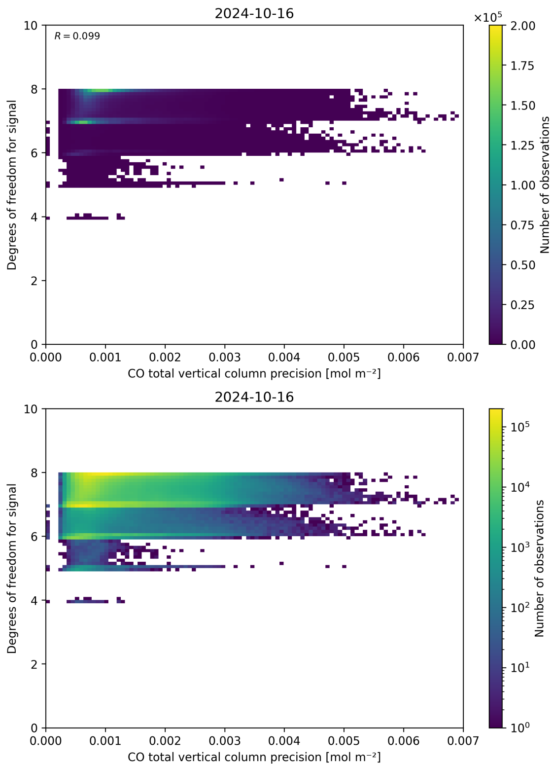
Figure 45: Scatter density plot of “CO total vertical column precision” against “Degrees of freedom for signal” for 2024-10-15 to 2024-10-17.
