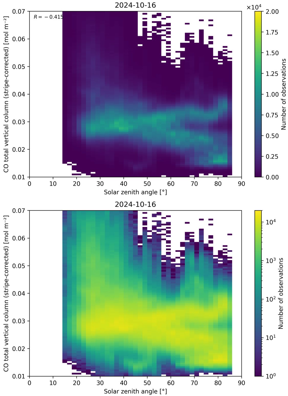
Figure 62: Scatter density plot of “Solar zenith angle” against “CO total vertical column (stripe-corrected)” for 2024-10-15 to 2024-10-17.
