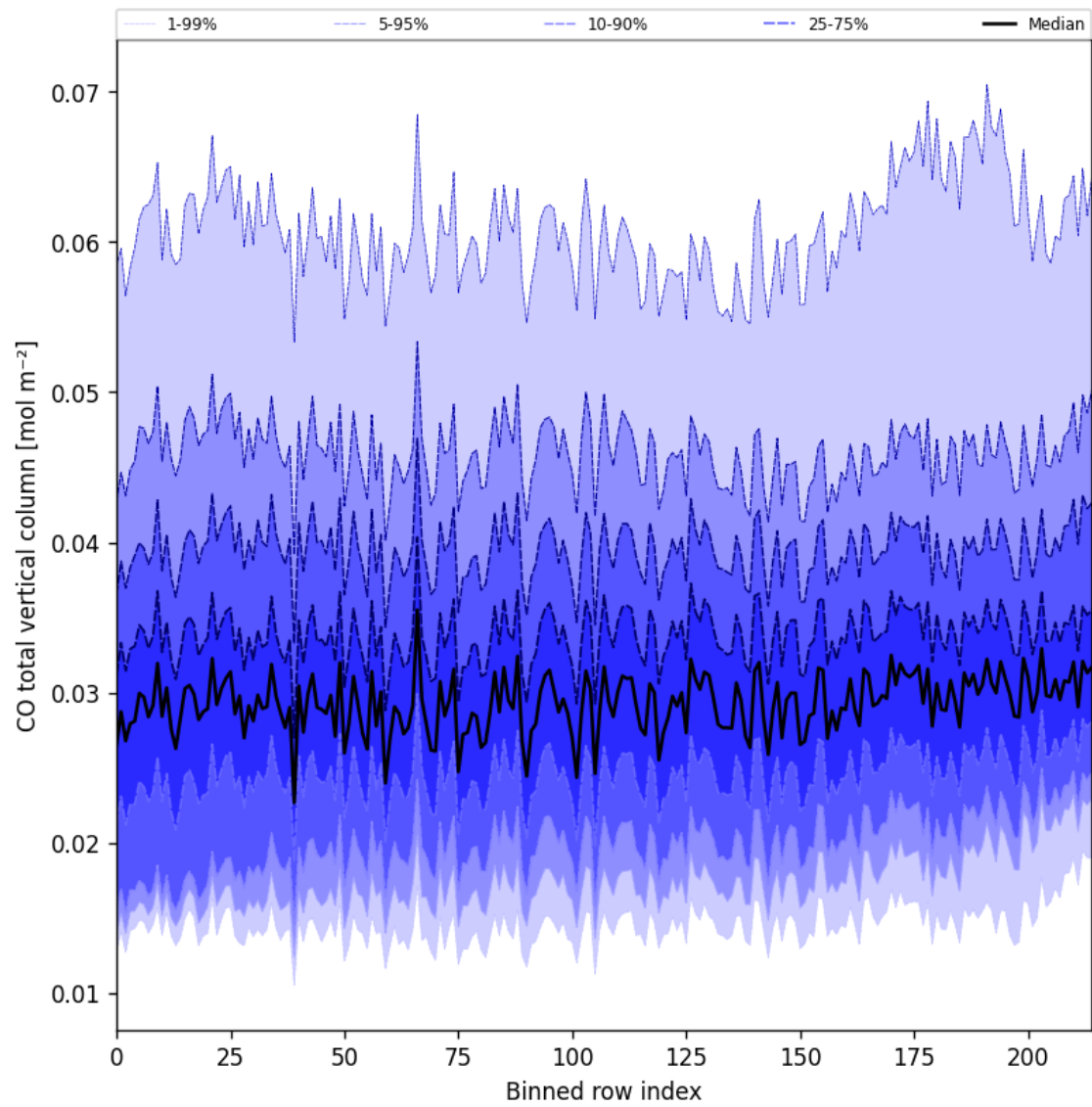
Figure 26: Along track statistics of “CO total vertical column” for 2024-10-15 to 2024-10-17
