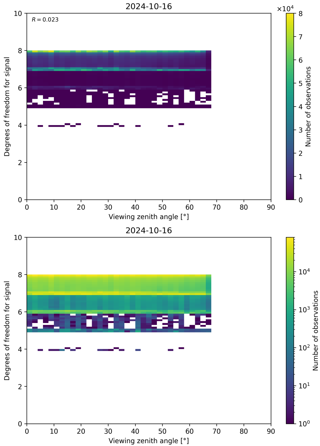
Figure 73: Scatter density plot of “Viewing zenith angle” against “Degrees of freedom for signal” for 2024-10-15 to 2024-10-17.
