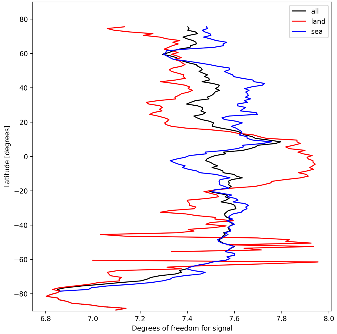
Figure 15: Zonal average of “Degrees of freedom for signal” for 2024-10-15 to 2024-10-17.
