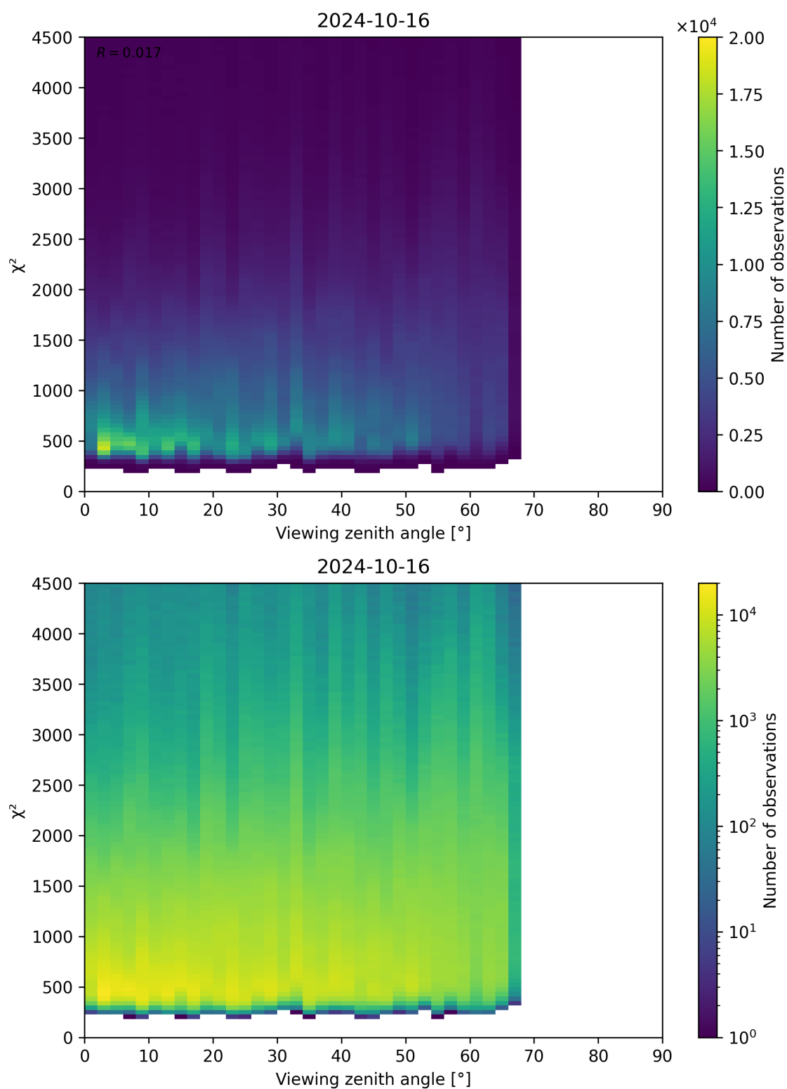
Figure 72: Scatter density plot of “Viewing zenith angle” against “ \chi^2 ” for 2024-10-15 to 2024-10-17.
