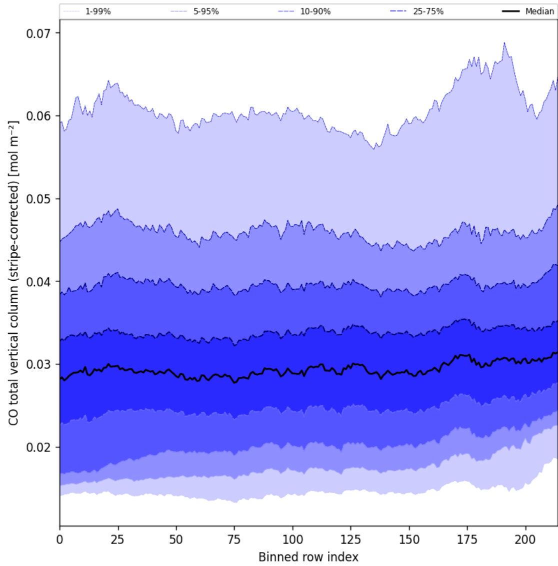
Figure 27: Along track statistics of “CO total vertical column (stripe-corrected)” for 2024-10-15 to 2024-10-17
