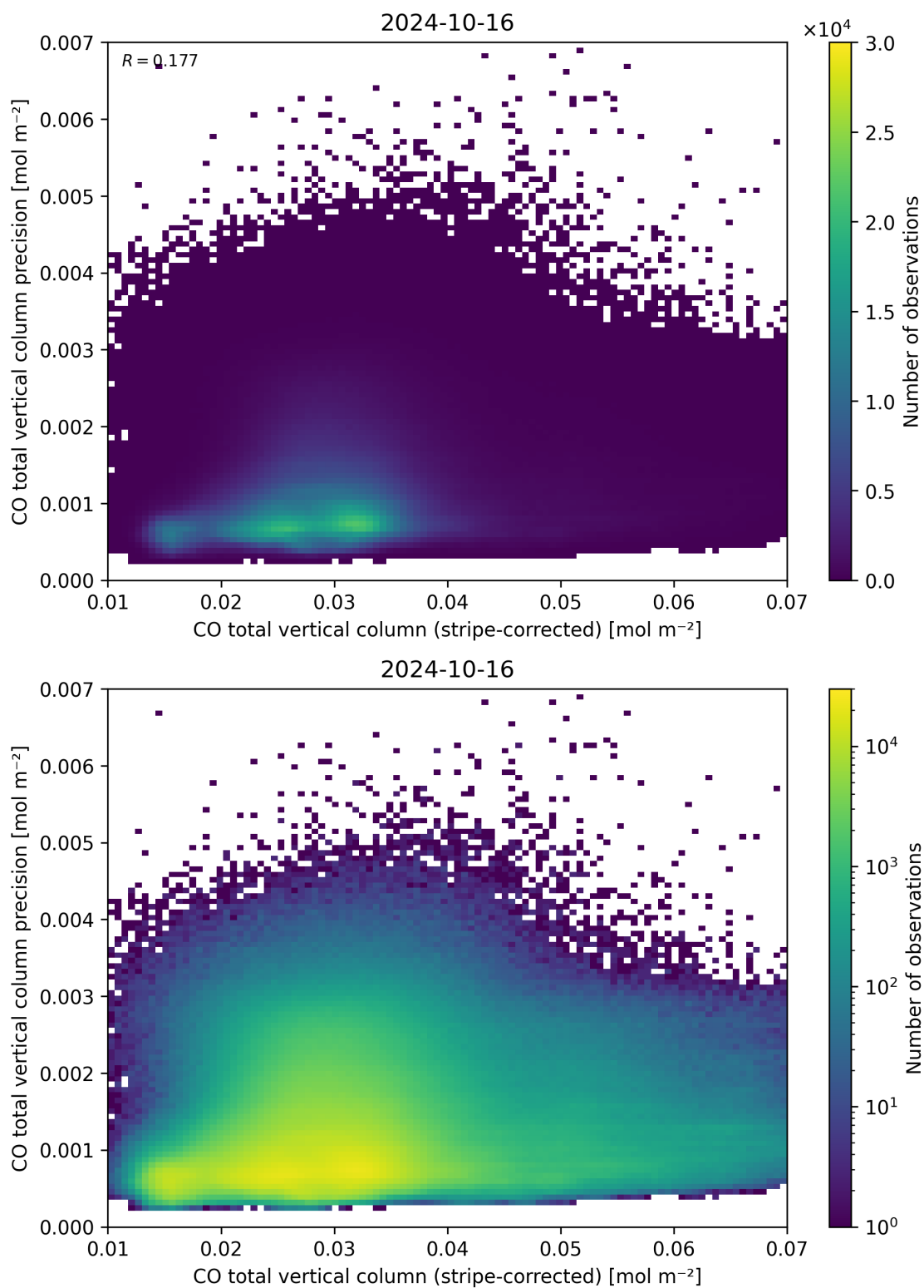
Figure 36: Scatter density plot of “CO total vertical column (stripe-corrected)” against “CO total vertical column precision” for 2024-10-15 to 2024-10-17.
