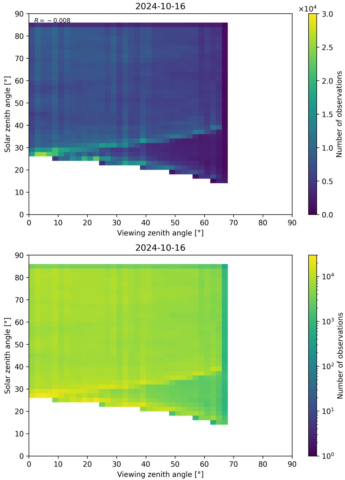
Figure 77: Scatter density plot of “Viewing zenith angle” against “Solar zenith angle” for 2024-10-15 to 2024-10-17.
