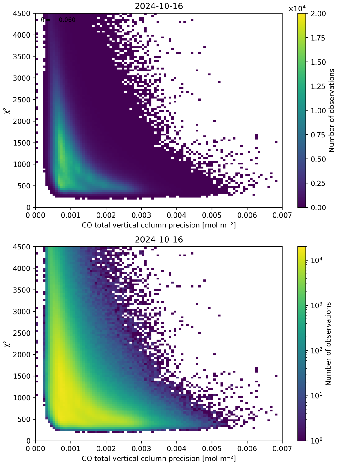
Figure 44: Scatter density plot of “CO total vertical column precision” against “ \chi^2 ” for 2024-10-15 to 2024-10-17.
