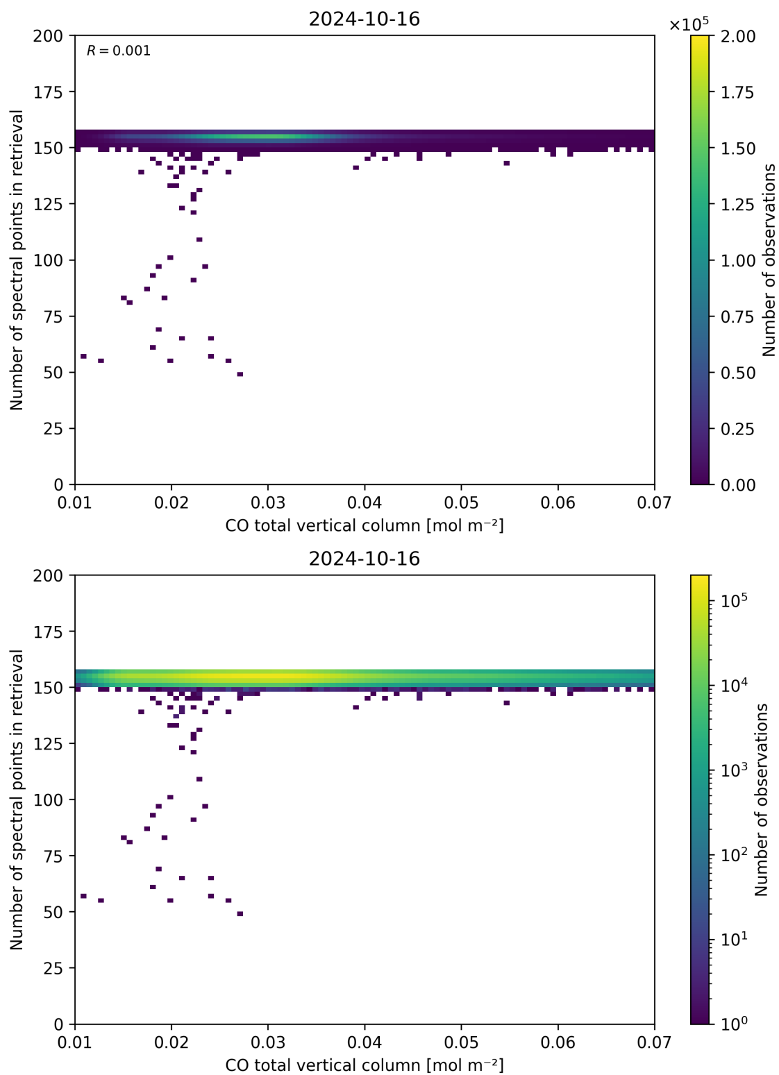
Figure 43: Scatter density plot of “CO total vertical column” against “Number of spectral points in retrieval” for 2024-10-15 to 2024-10-17.
