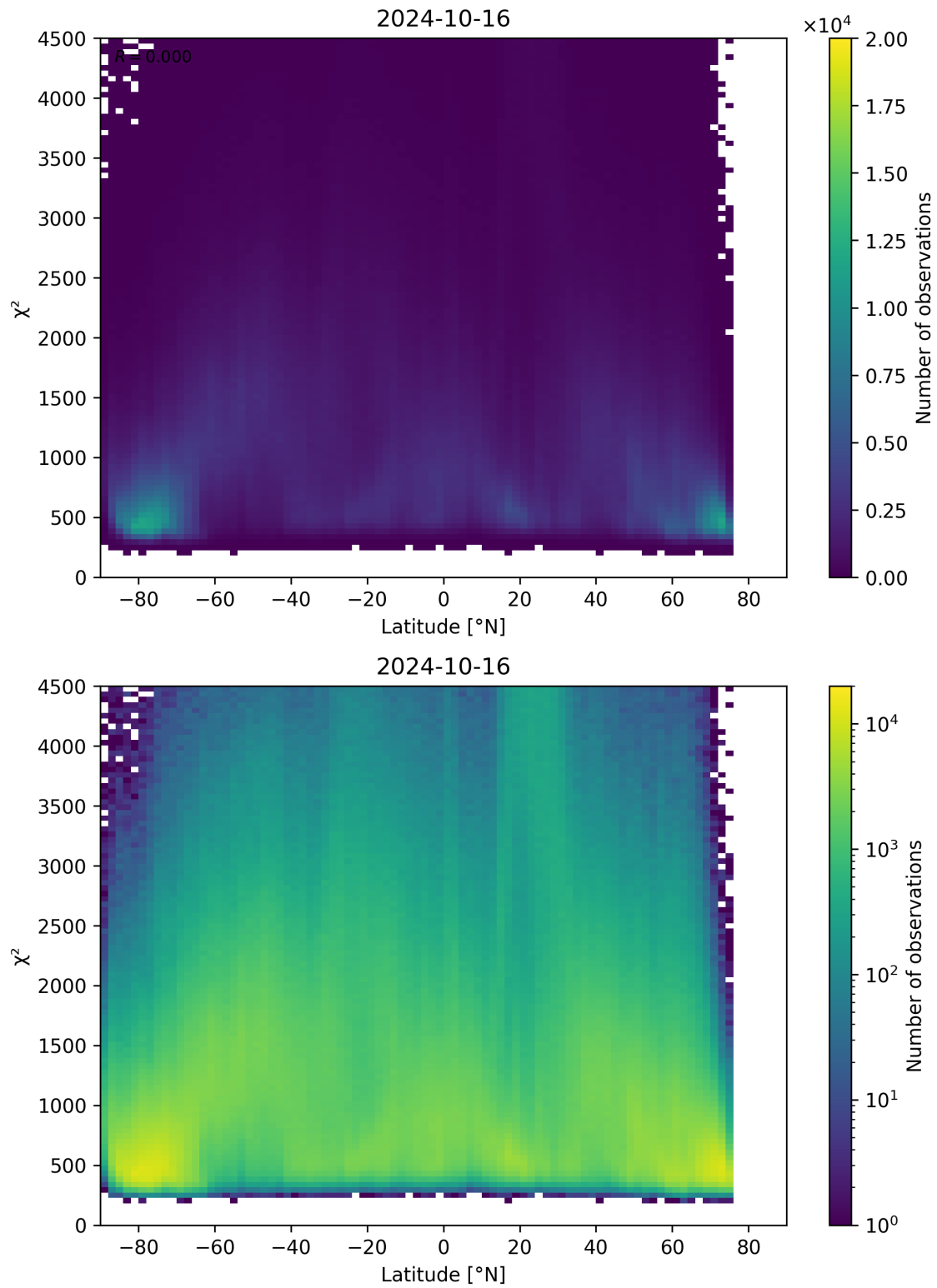
Figure 54: Scatter density plot of “Latitude” against “ \chi^2 ” for 2024-10-15 to 2024-10-17.
