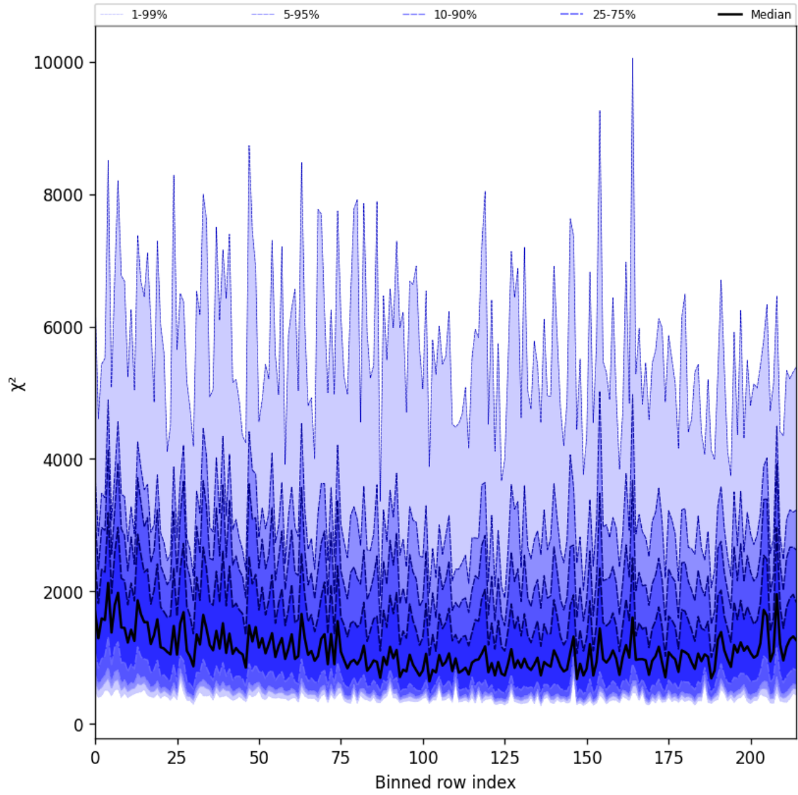
Figure 30: Along track statistics of “ \chi^2 ” for 2024-10-15 to 2024-10-17
