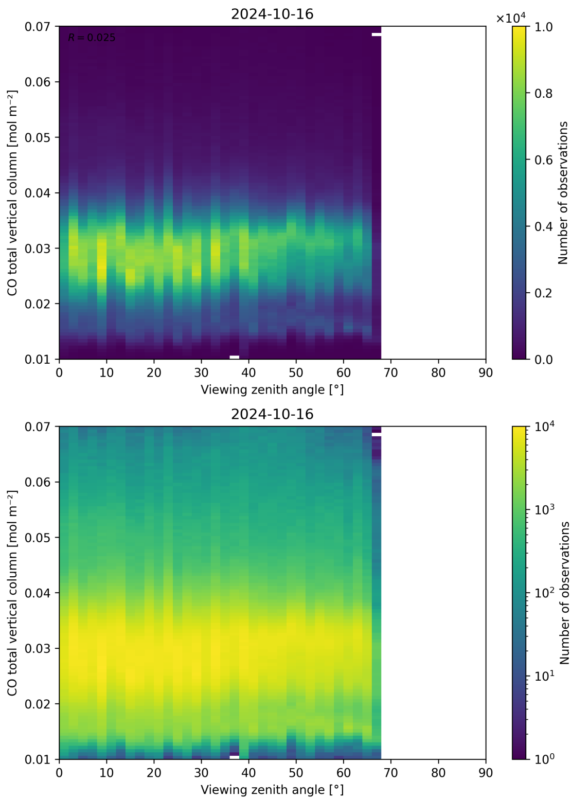
Figure 69: Scatter density plot of “Viewing zenith angle” against “CO total vertical column” for 2024-10-15 to 2024-10-17.
