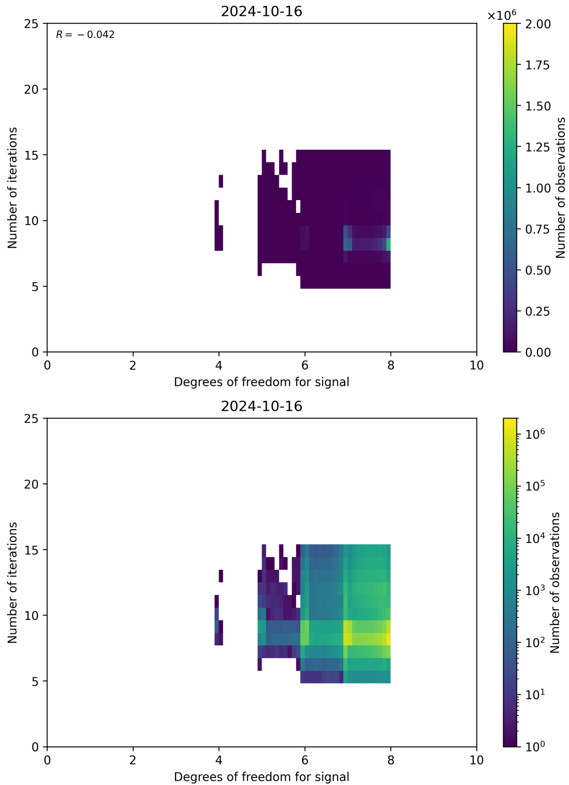
Figure 50: Scatter density plot of “Degrees of freedom for signal” against “Number of iterations” for 2024-10-15 to 2024-10-17.
