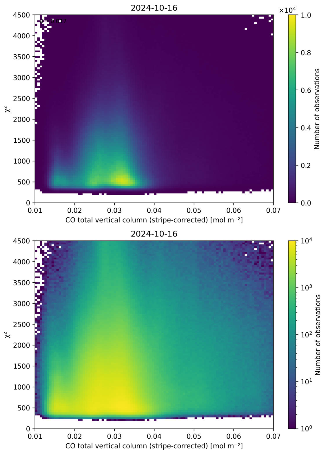
Figure 37: Scatter density plot of “CO total vertical column (stripe-corrected)” against “ \chi^2 ” for 2024-10-15 to 2024-10-17.
