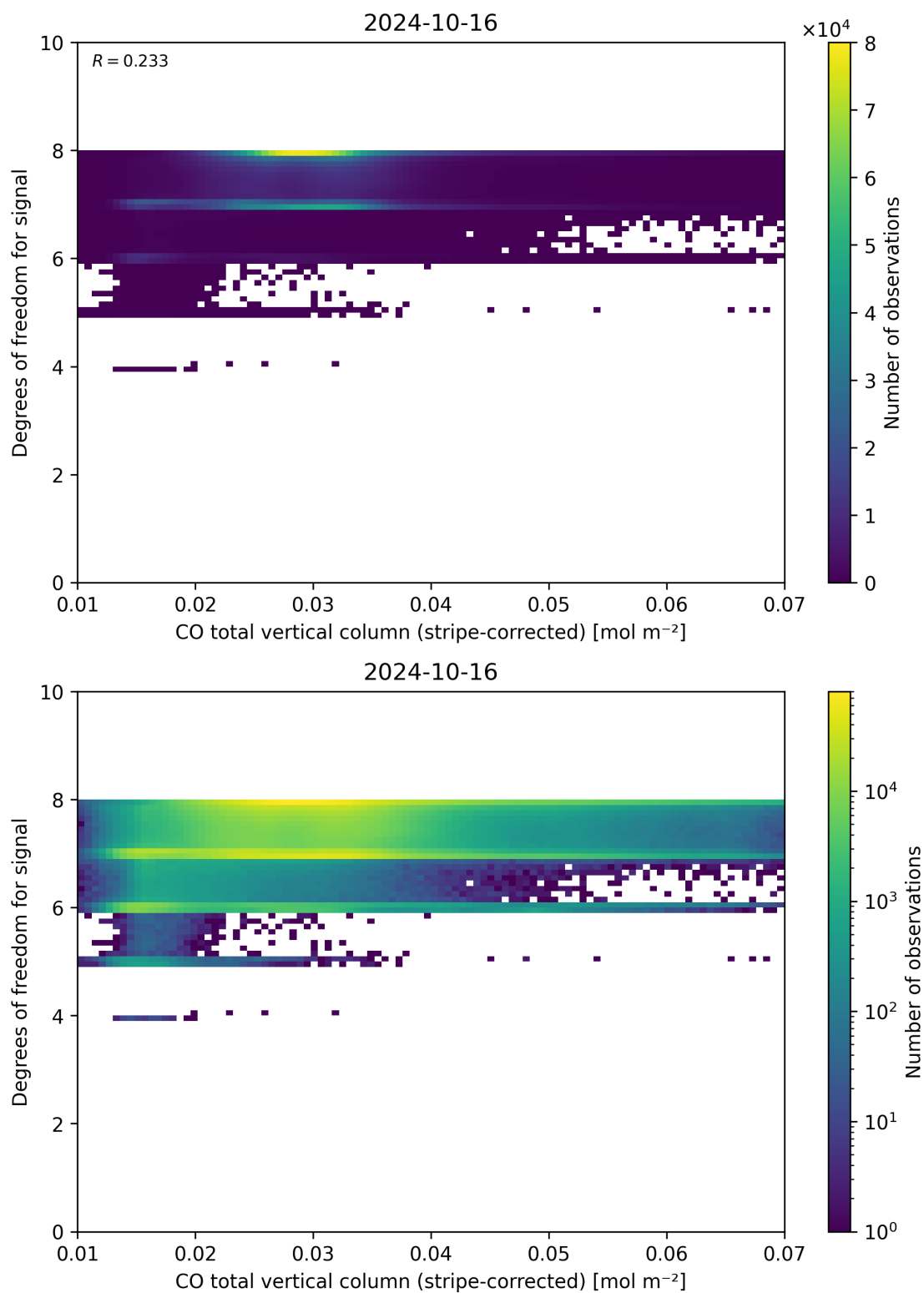
Figure 38: Scatter density plot of “CO total vertical column (stripe-corrected)” against “Degrees of freedom for signal” for 2024-10-15 to 2024-10-17.
