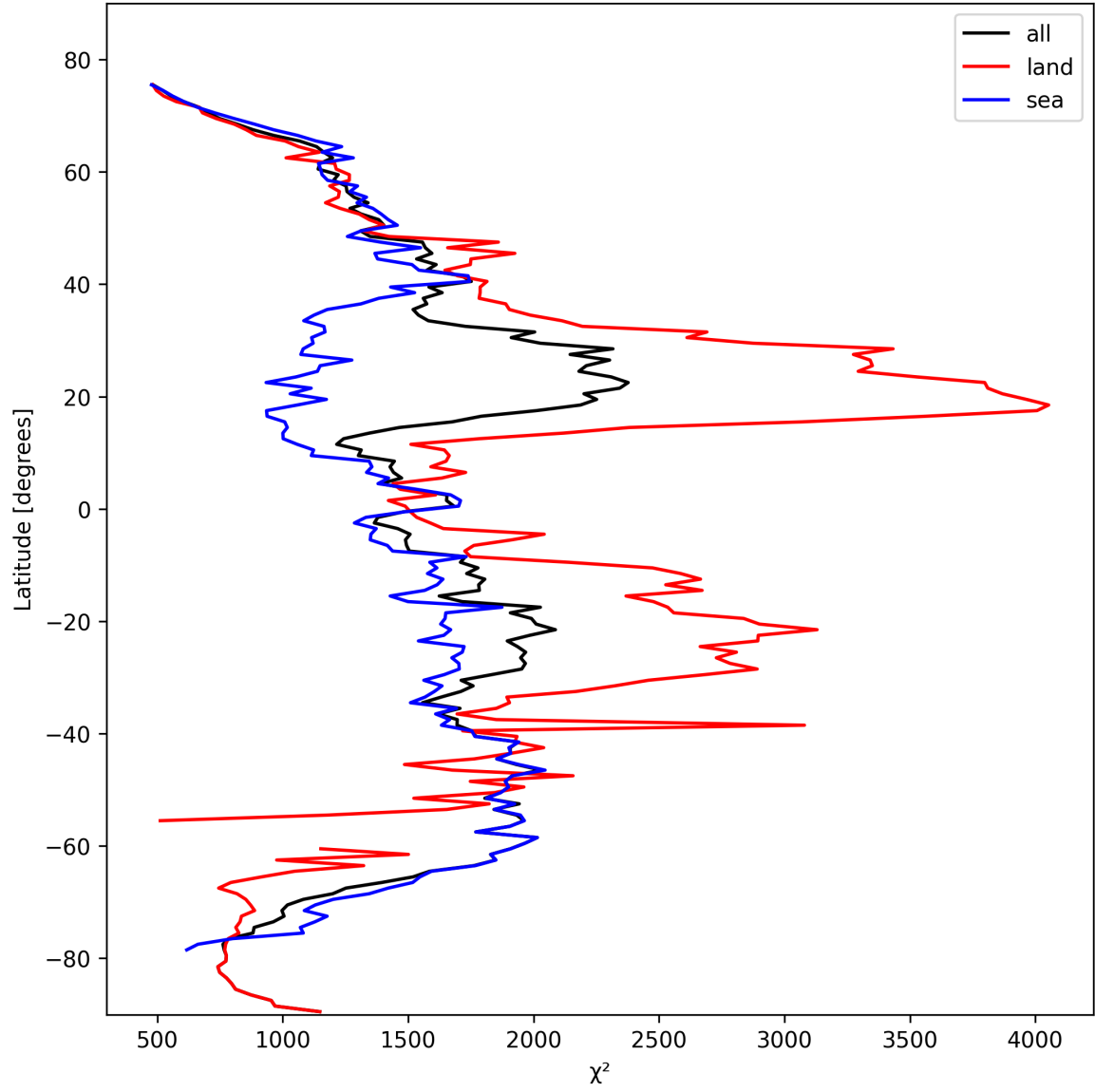
Figure 14: Zonal average of “ \chi^2 ” for 2024-10-15 to 2024-10-17.
