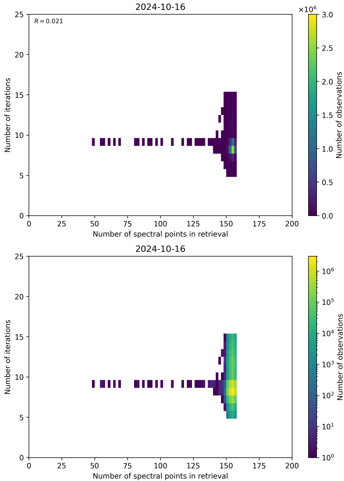
Figure 60: Scatter density plot of “Number of spectral points in retrieval” against “Number of iterations” for 2024-10-15 to 2024-10-17.
