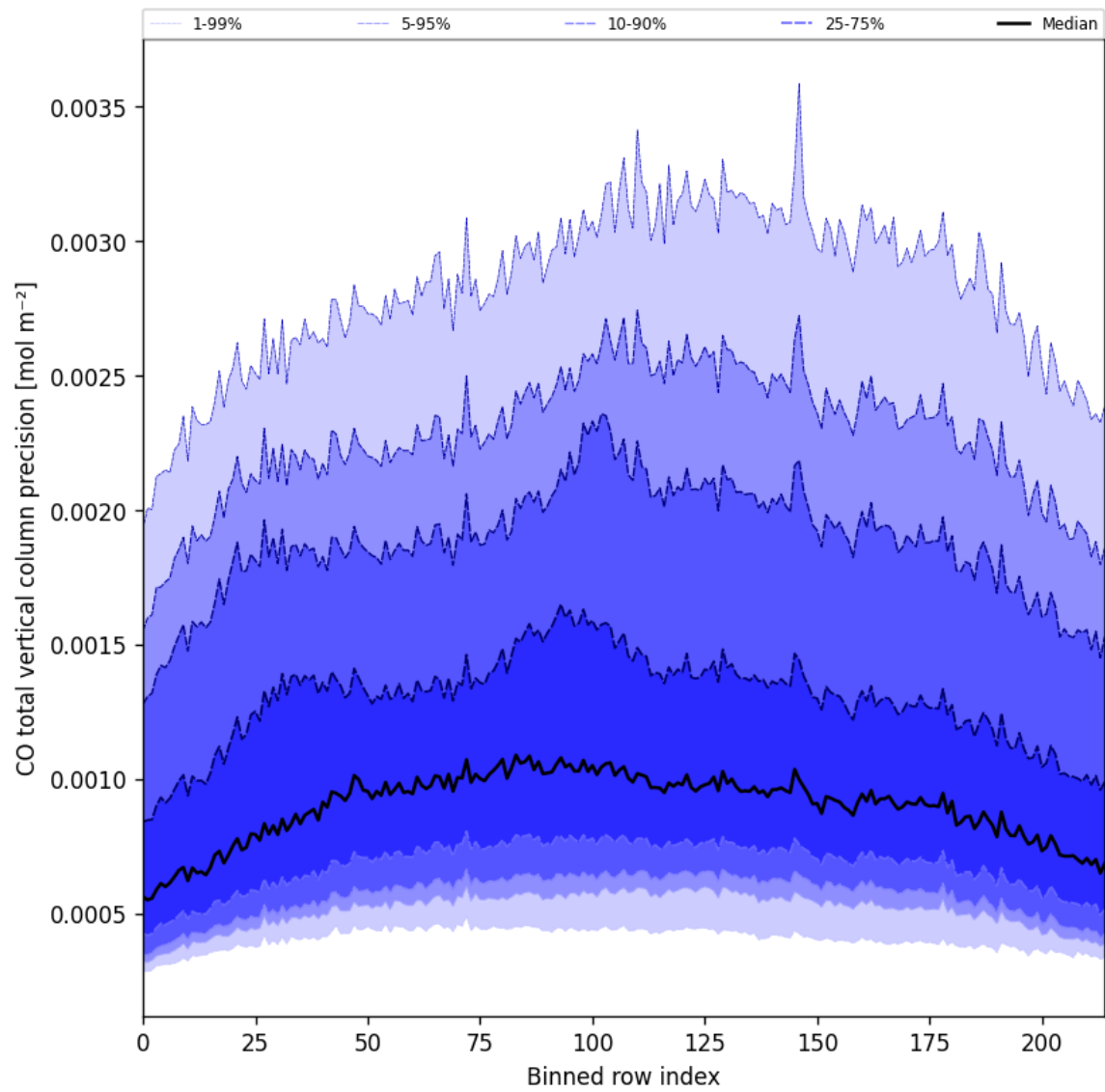
Figure 28: Along track statistics of “CO total vertical column precision” for 2024-10-15 to 2024-10-17
