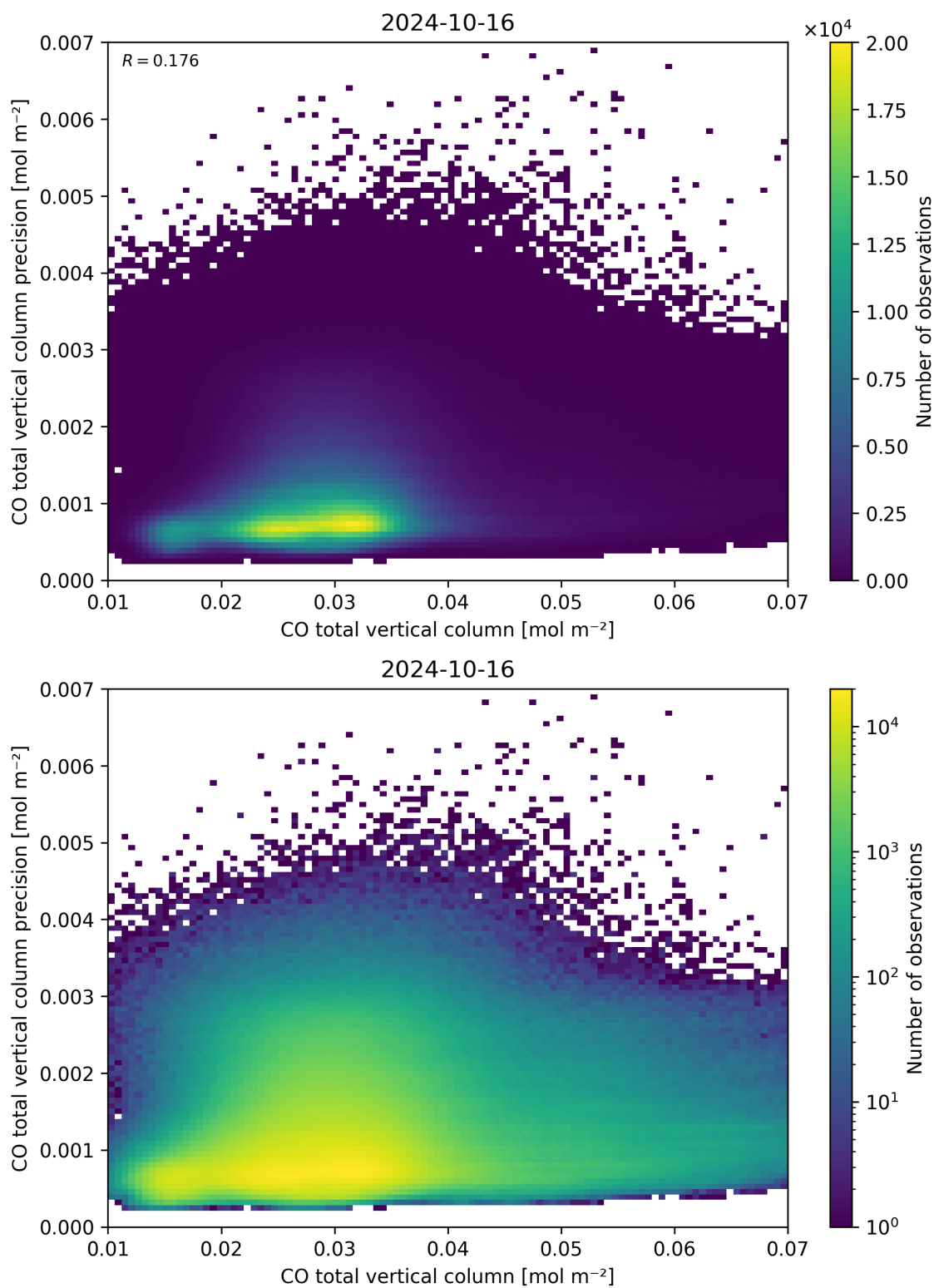
Figure 34: Scatter density plot of “CO total vertical column” against “CO total vertical column precision” for 2024-10-15 to 2024-10-17.
