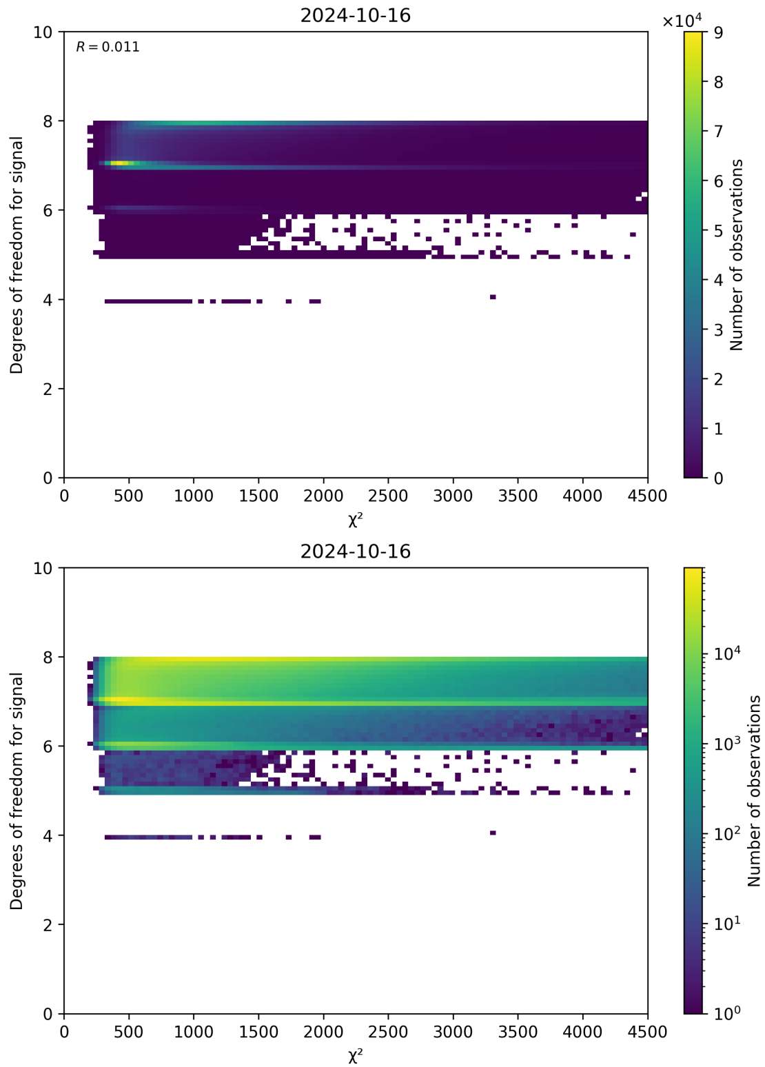
Figure 48: Scatter density plot of “ \chi^2 ” against “Degrees of freedom for signal” for 2024-10-15 to 2024-10-17.
