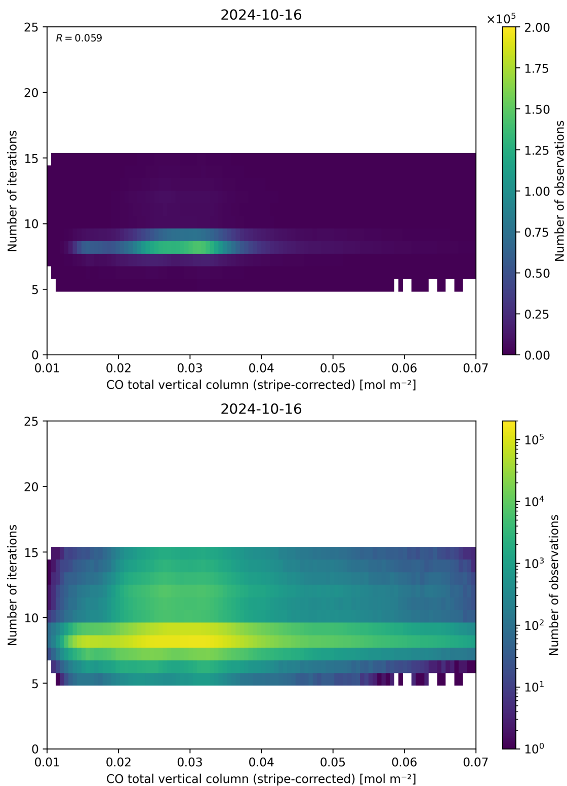
Figure 39: Scatter density plot of “CO total vertical column (stripe-corrected)” against “Number of iterations” for 2024-10-15 to 2024-10-17.
