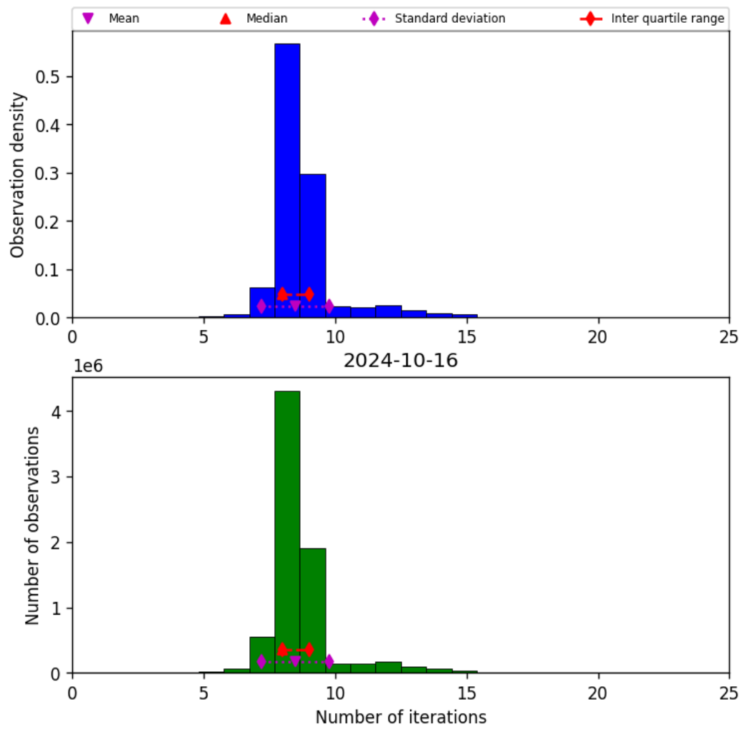
Figure 24: Histogram of “Number of iterations” for 2024-10-15 to 2024-10-17
