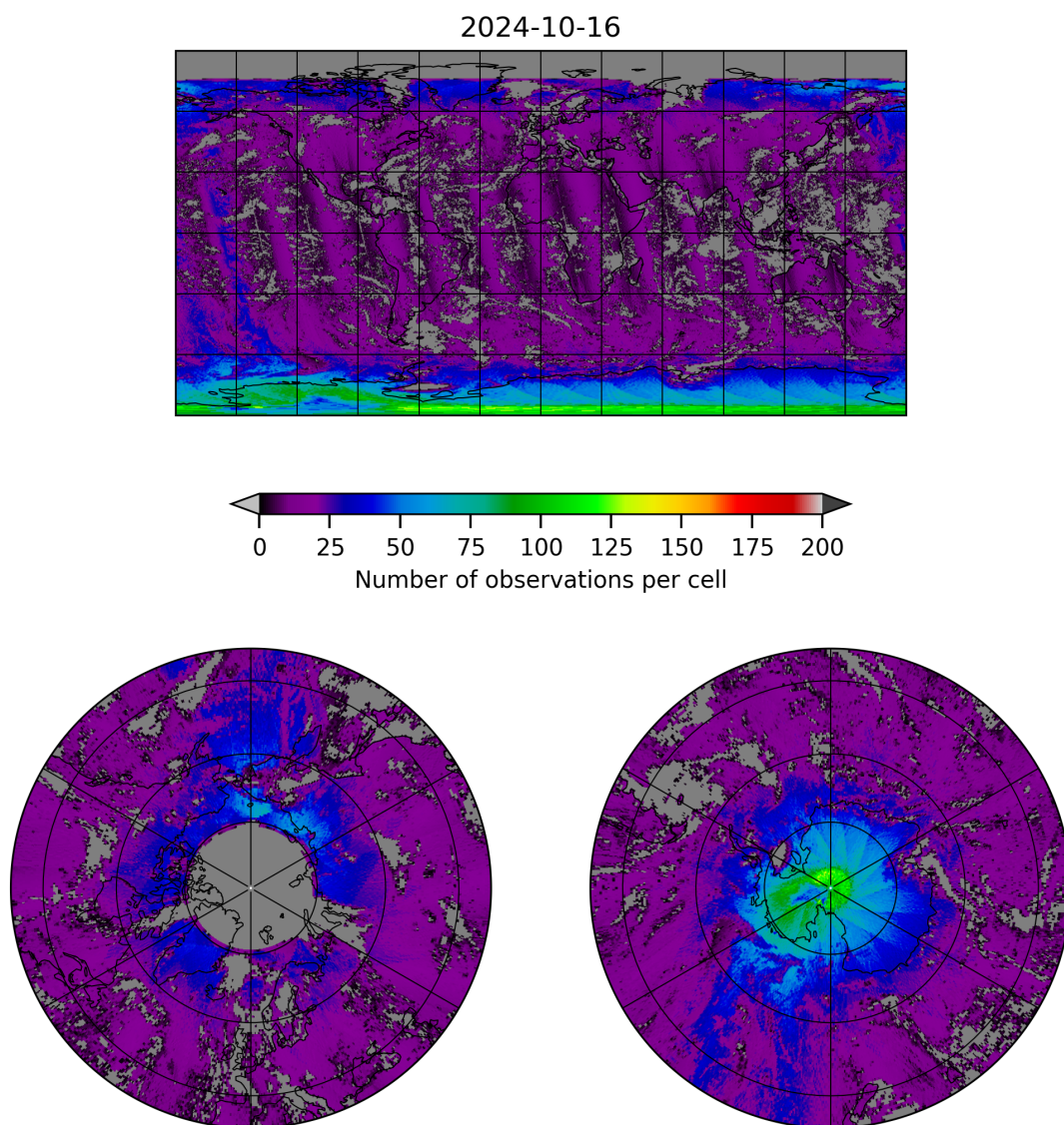
Figure 8: Map of the number of observations for 2024-10-15 to 2024-10-17
