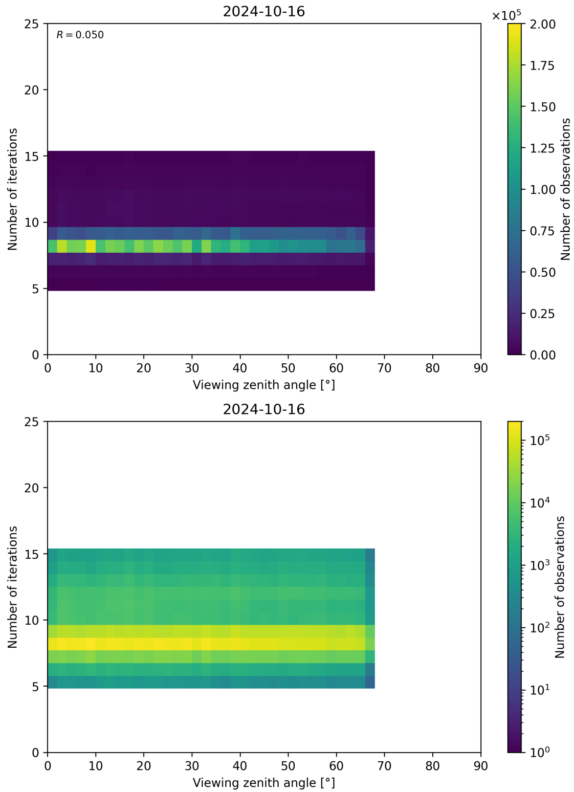
Figure 75: Scatter density plot of “Viewing zenith angle” against “Number of iterations” for 2024-10-15 to 2024-10-17.
