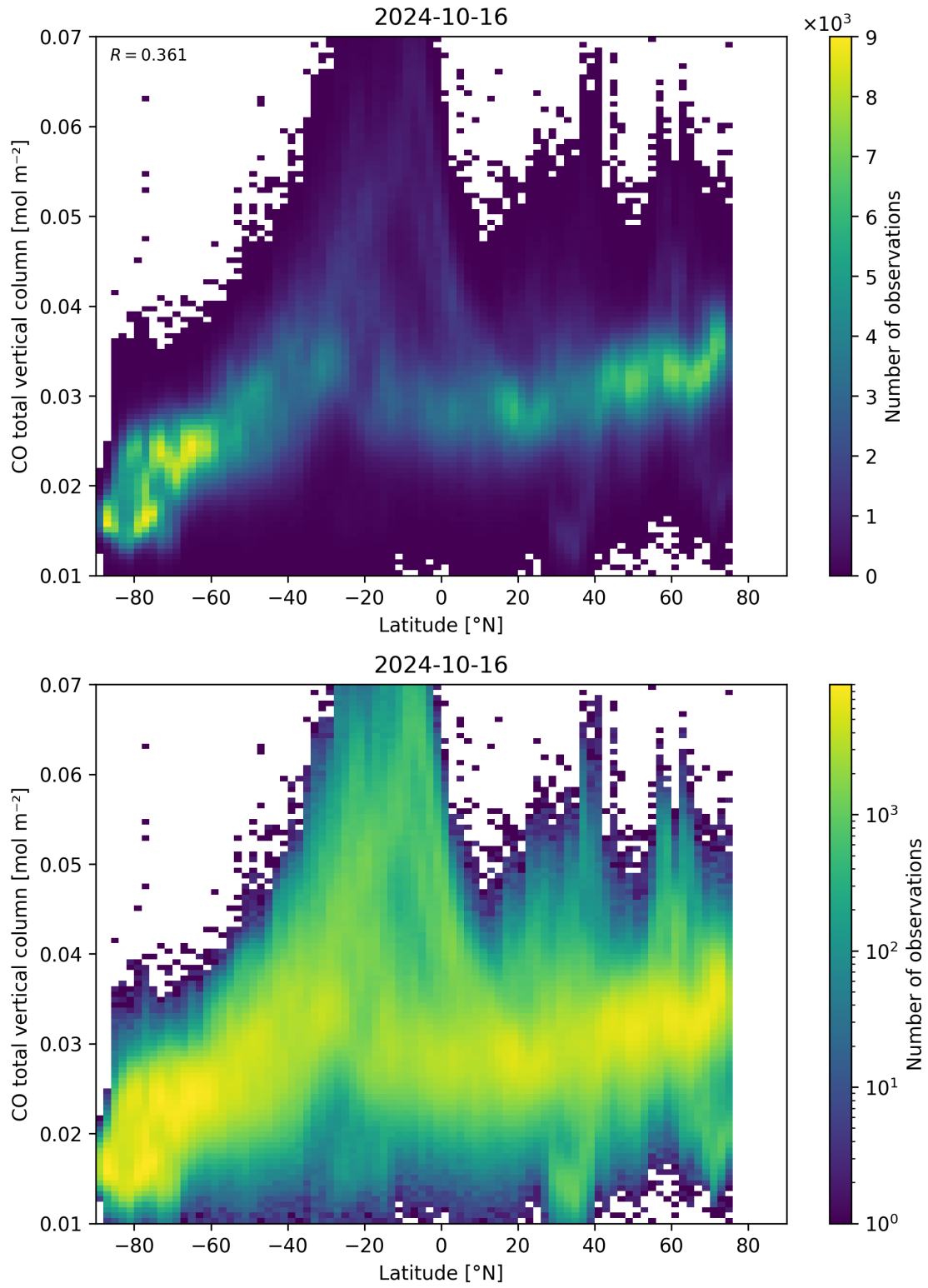
Figure 51: Scatter density plot of “Latitude” against “CO total vertical column” for 2024-10-15 to 2024-10-17.
