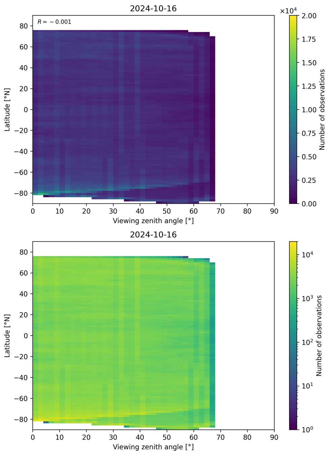
Figure 74: Scatter density plot of “Viewing zenith angle” against “Latitude” for 2024-10-15 to 2024-10-17.
