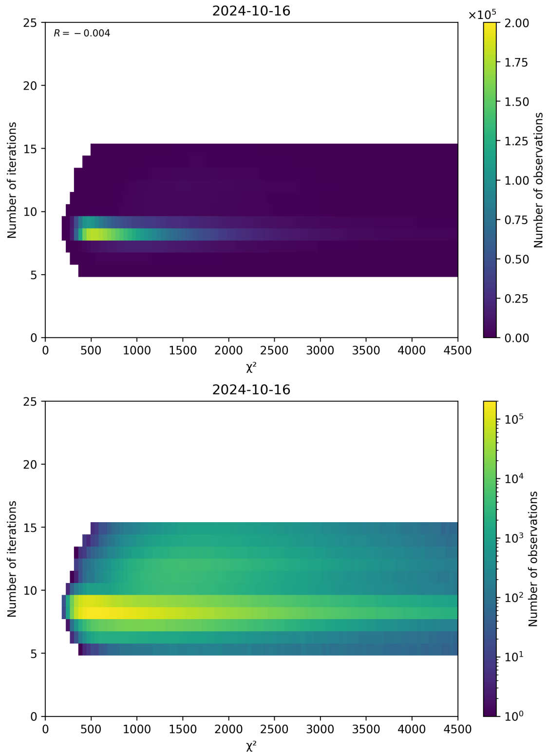
Figure 49: Scatter density plot of “ \chi^2 ” against “Number of iterations” for 2024-10-15 to 2024-10-17.
