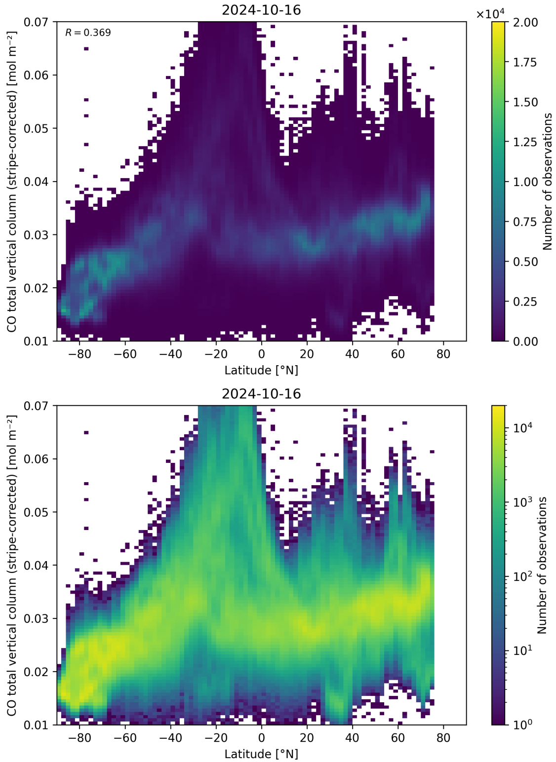
Figure 52: Scatter density plot of “Latitude” against “CO total vertical column (stripe-corrected)” for 2024-10-15 to 2024-10-17.
