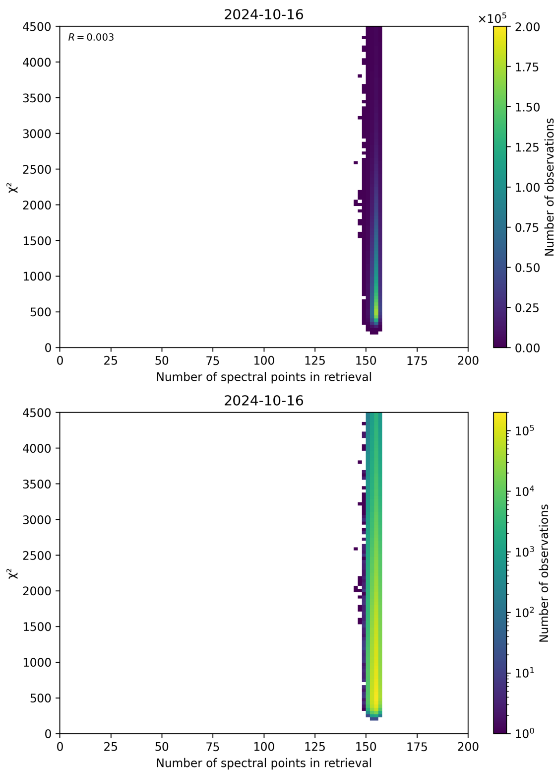
Figure 58: Scatter density plot of “Number of spectral points in retrieval” against “ \chi^2 ” for 2024-10-15 to 2024-10-17.
