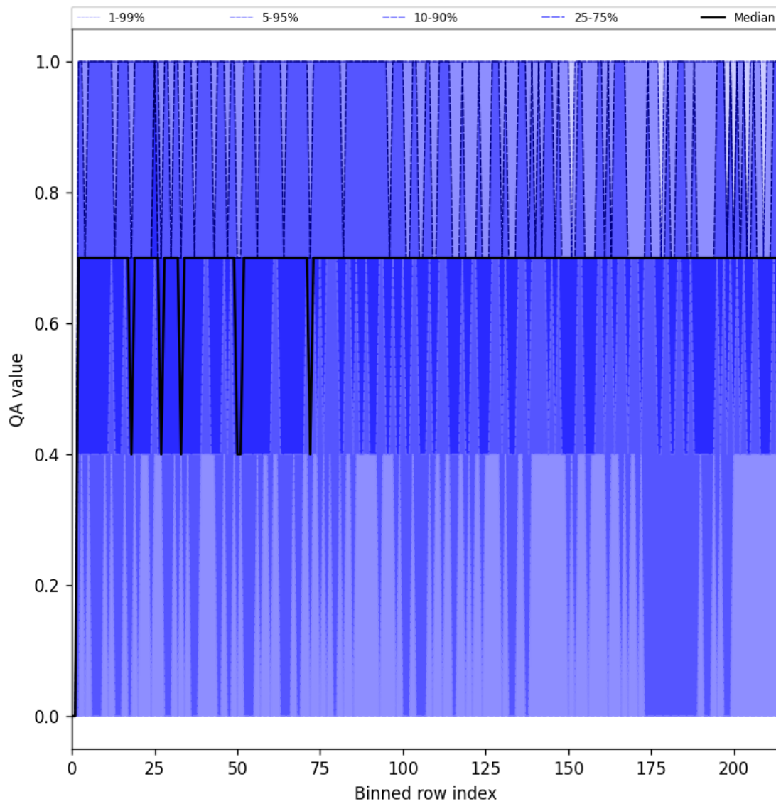
Figure 25: Along track statistics of “QA value” for 2024-10-16 to 2024-10-18
