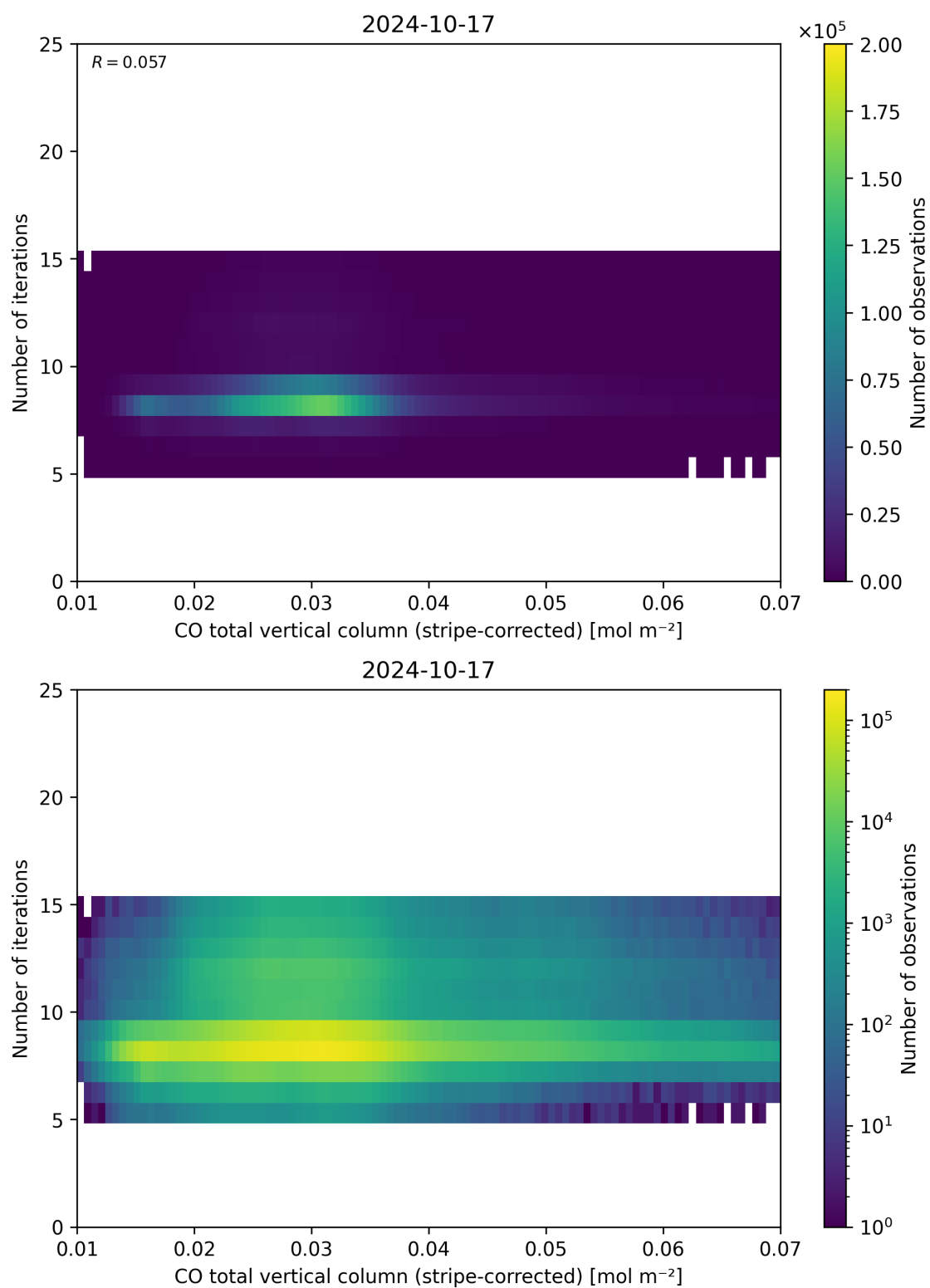
Figure 39: Scatter density plot of “CO total vertical column (stripe-corrected)” against “Number of iterations” for 2024-10-16 to 2024-10-18.
