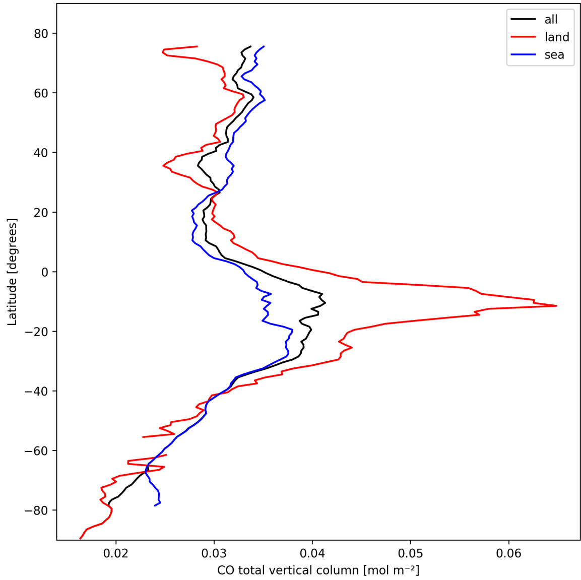
Figure 10: Zonal average of “CO total vertical column” for 2024-10-16 to 2024-10-18.
