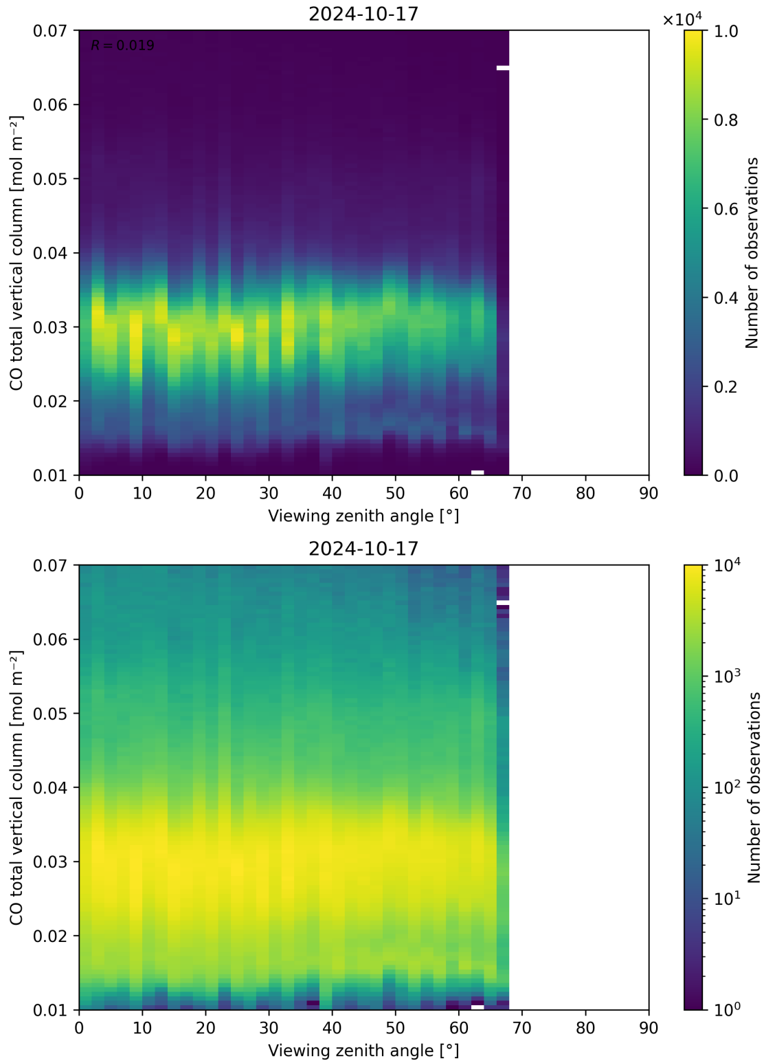
Figure 69: Scatter density plot of “Viewing zenith angle” against “CO total vertical column” for 2024-10-16 to 2024-10-18.
