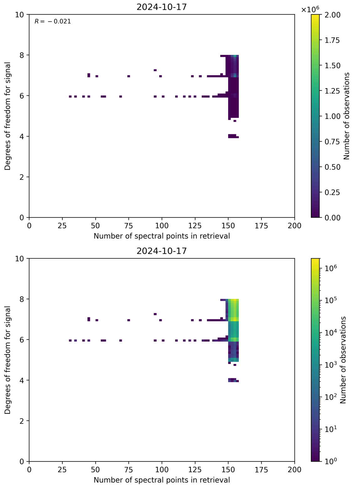
Figure 59: Scatter density plot of “Number of spectral points in retrieval” against “Degrees of freedom for signal” for 2024-10-16 to 2024-10-18.
