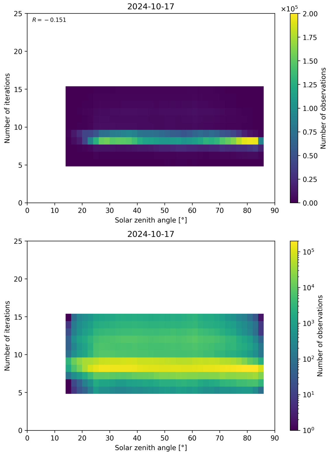
Figure 67: Scatter density plot of “Solar zenith angle” against “Number of iterations” for 2024-10-16 to 2024-10-18.
