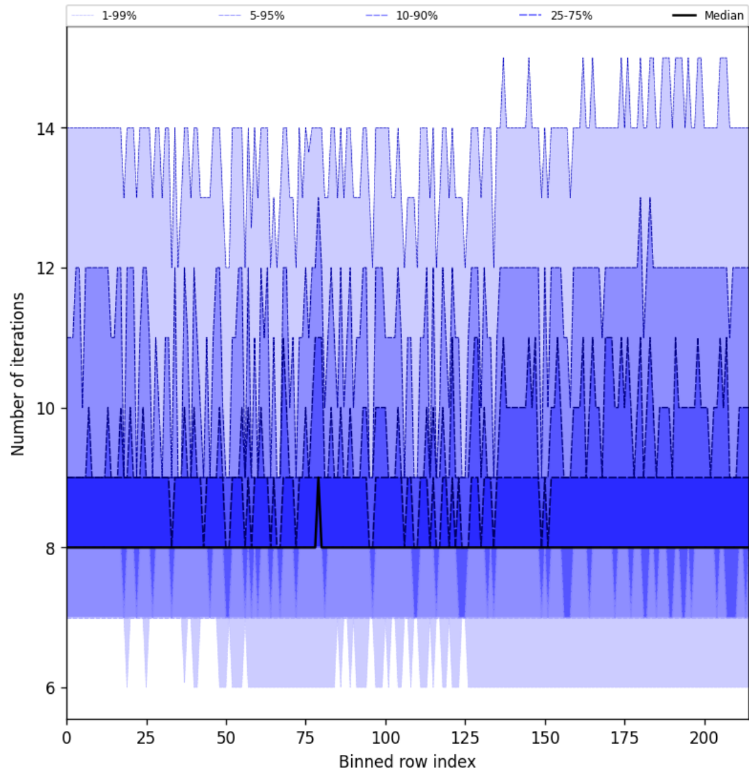
Figure 32: Along track statistics of “Number of iterations” for 2024-10-16 to 2024-10-18
