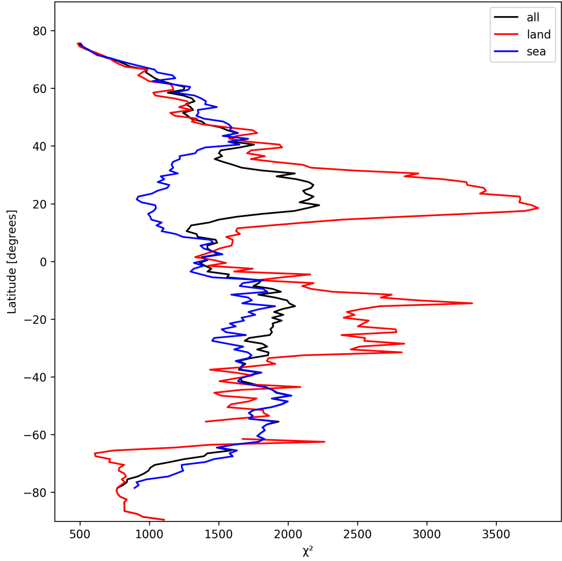
Figure 14: Zonal average of “ \chi^2 ” for 2024-10-16 to 2024-10-18.
