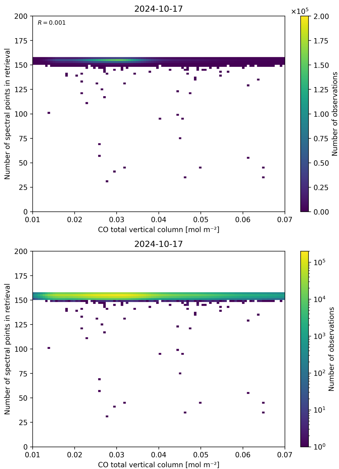
Figure 43: Scatter density plot of “CO total vertical column” against “Number of spectral points in retrieval” for 2024-10-16 to 2024-10-18.
