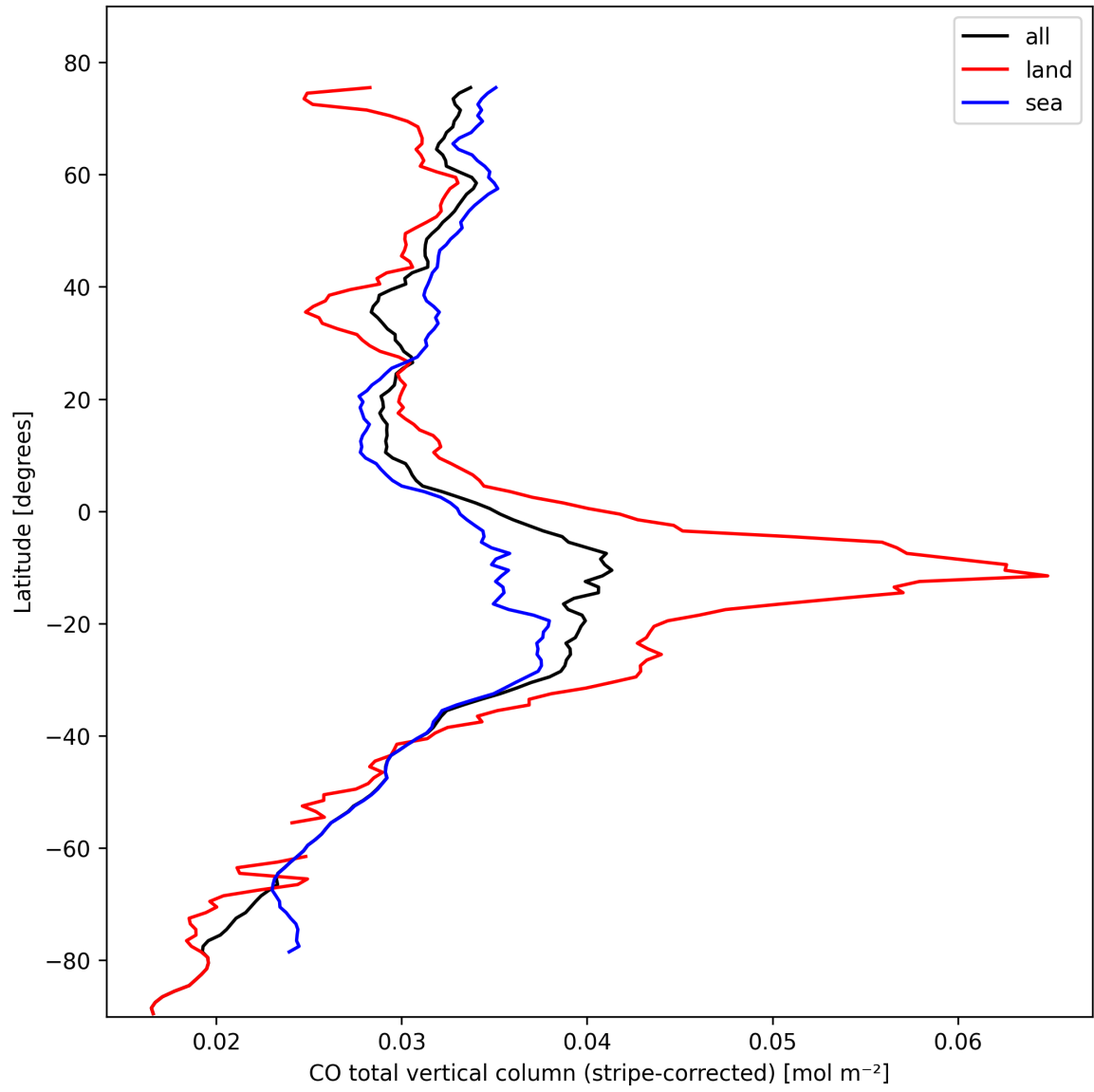
Figure 11: Zonal average of “CO total vertical column (stripe-corrected)” for 2024-10-16 to 2024-10-18.
