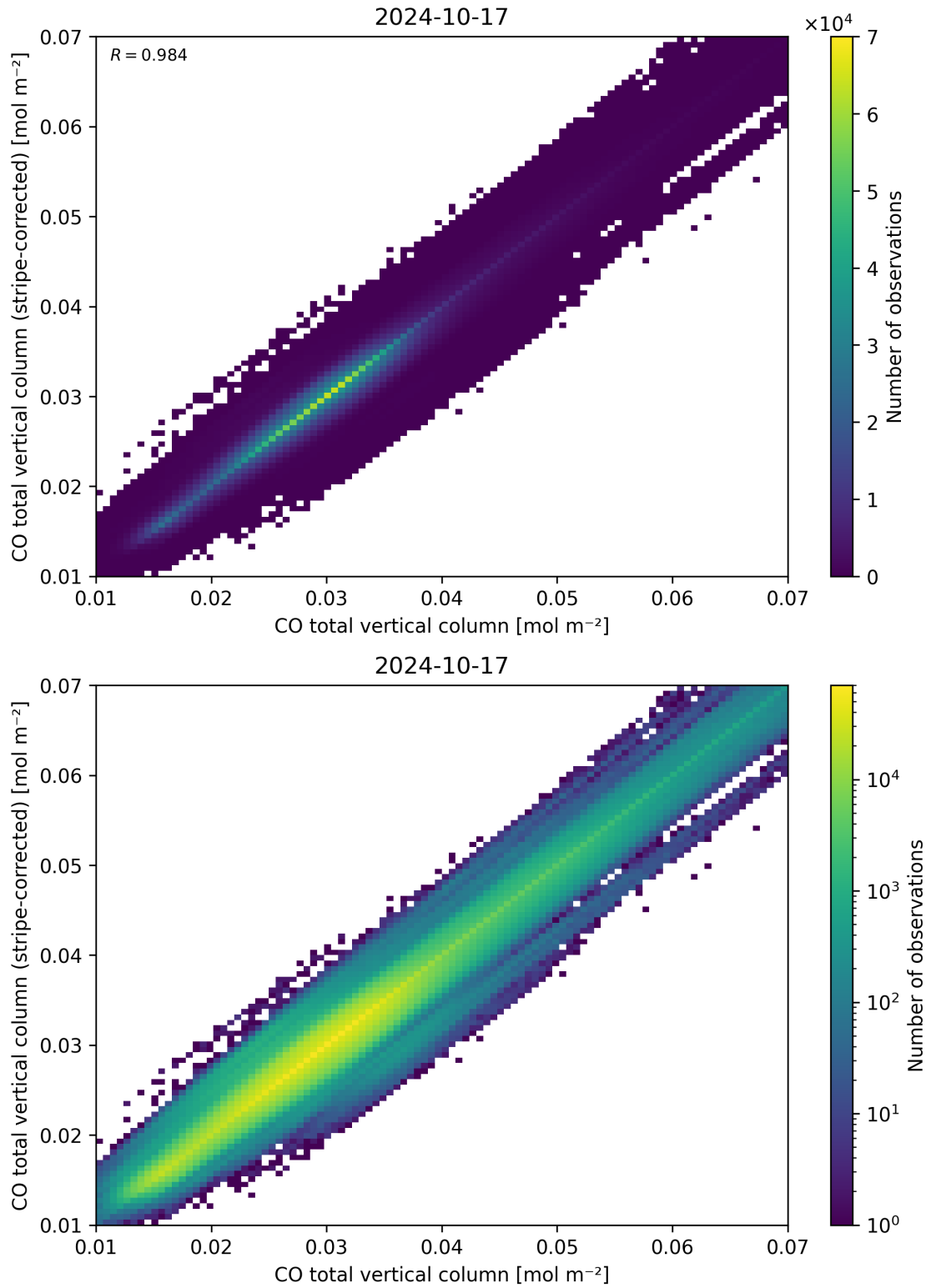
Figure 33: Scatter density plot of “CO total vertical column” against “CO total vertical column (stripe-corrected)” for 2024-10-16 to 2024-10-18.
