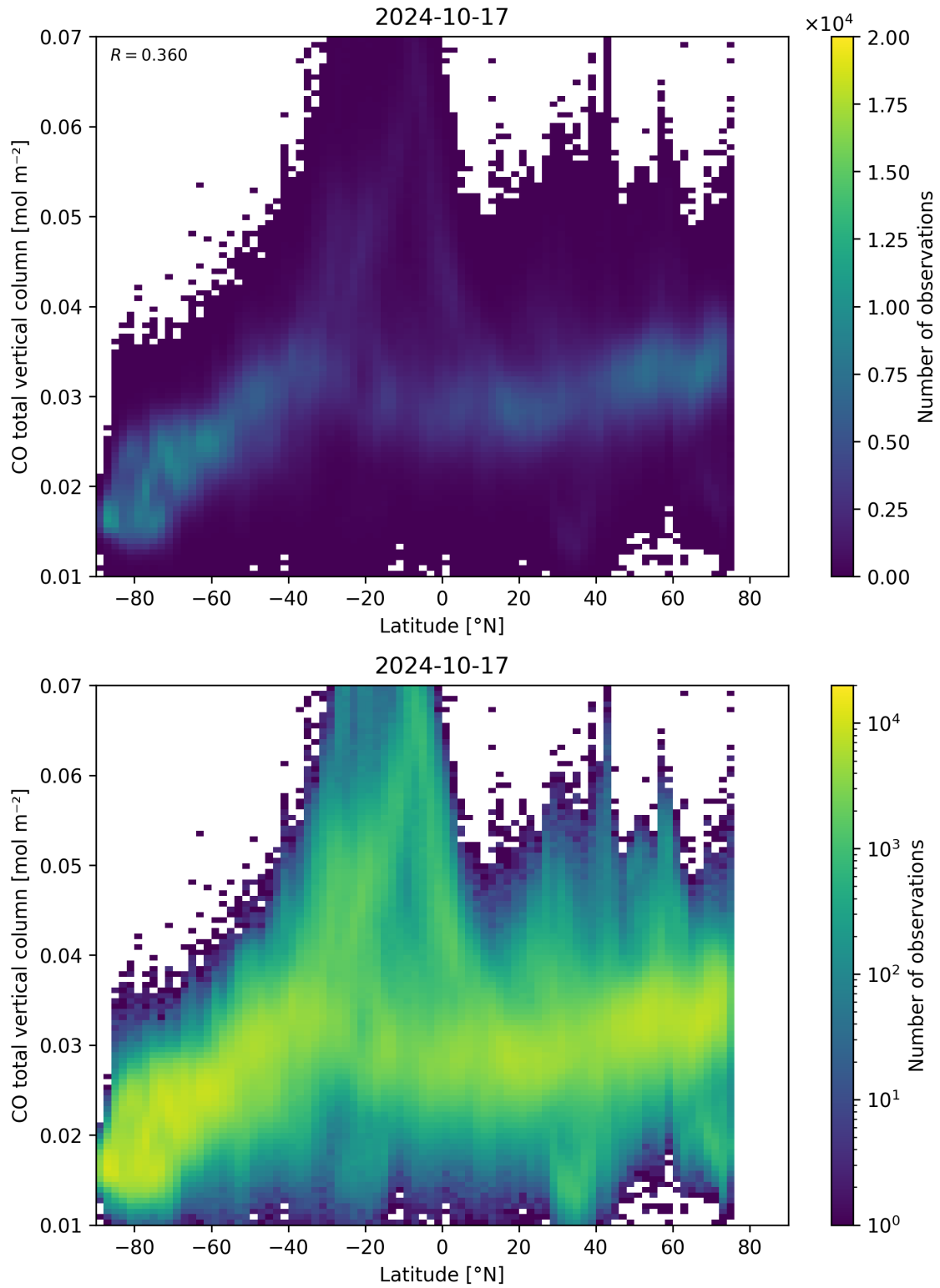
Figure 51: Scatter density plot of “Latitude” against “CO total vertical column” for 2024-10-16 to 2024-10-18.
