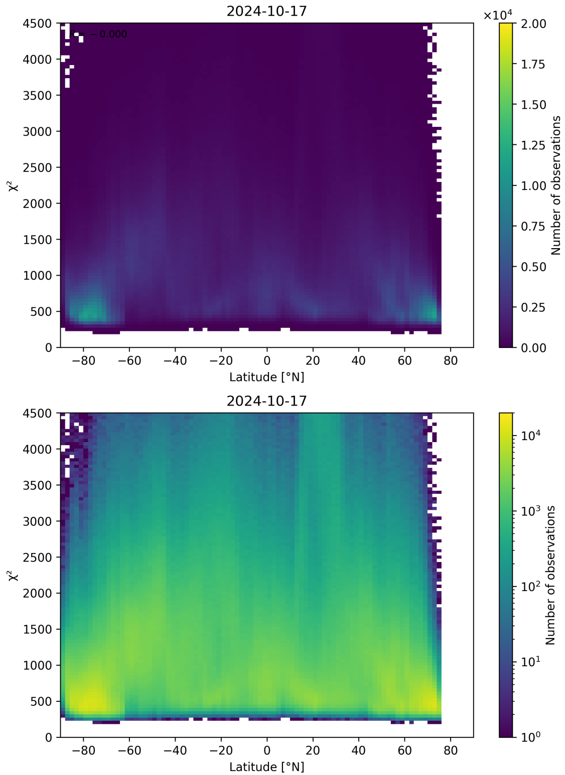
Figure 54: Scatter density plot of “Latitude” against “ \chi^2 ” for 2024-10-16 to 2024-10-18.
