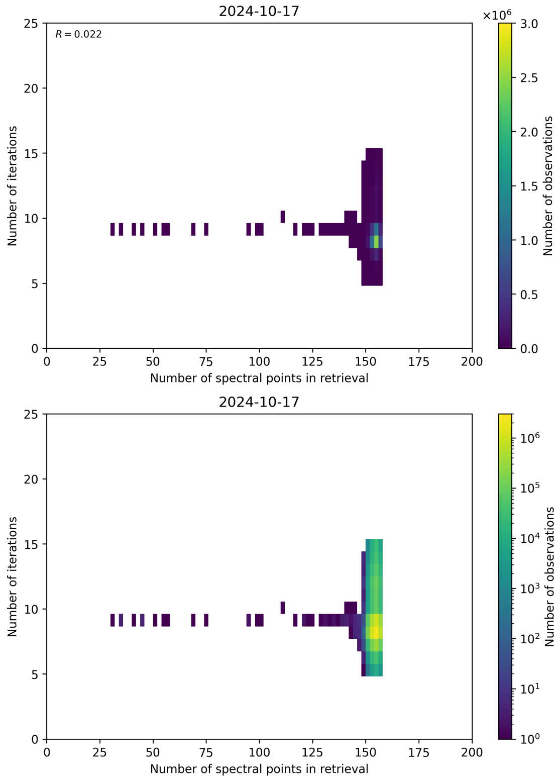
Figure 60: Scatter density plot of “Number of spectral points in retrieval” against “Number of iterations” for 2024-10-16 to 2024-10-18.
