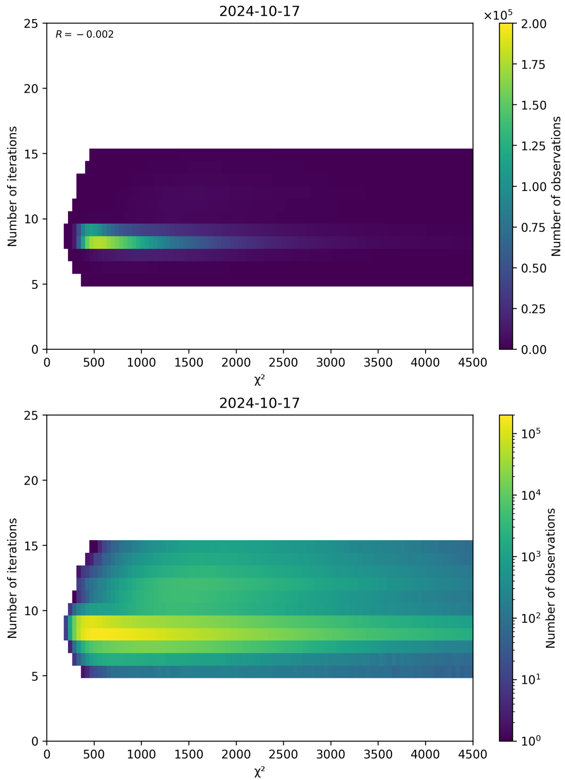
Figure 49: Scatter density plot of “ \chi^2 ” against “Number of iterations” for 2024-10-16 to 2024-10-18.
