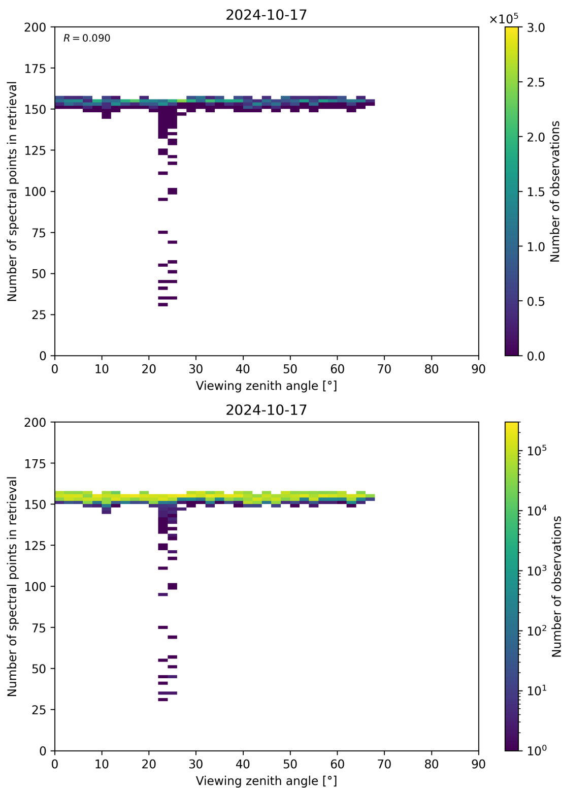
Figure 76: Scatter density plot of “Viewing zenith angle” against “Number of spectral points in retrieval” for 2024-10-16 to 2024-10-18.
