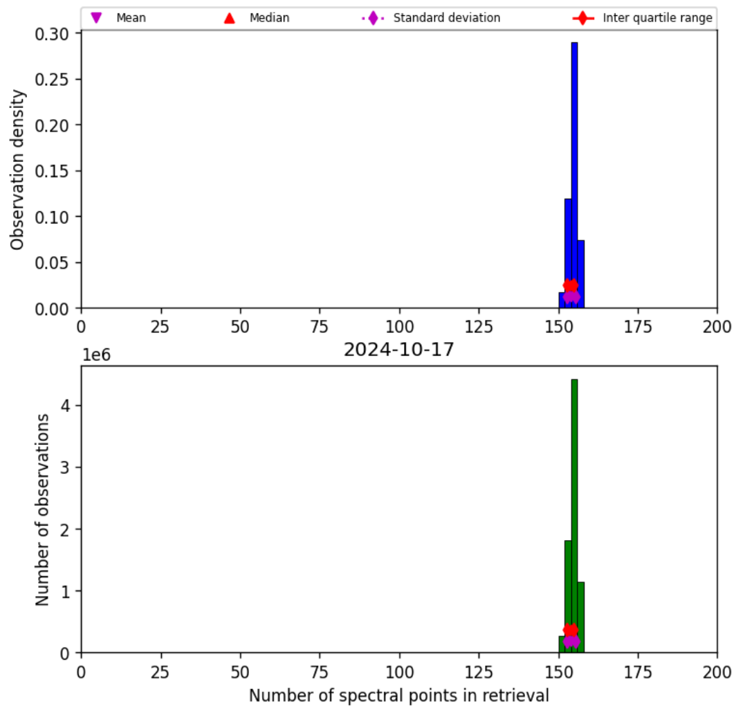
Figure 21: Histogram of “Number of spectral points in retrieval” for 2024-10-16 to 2024-10-18
