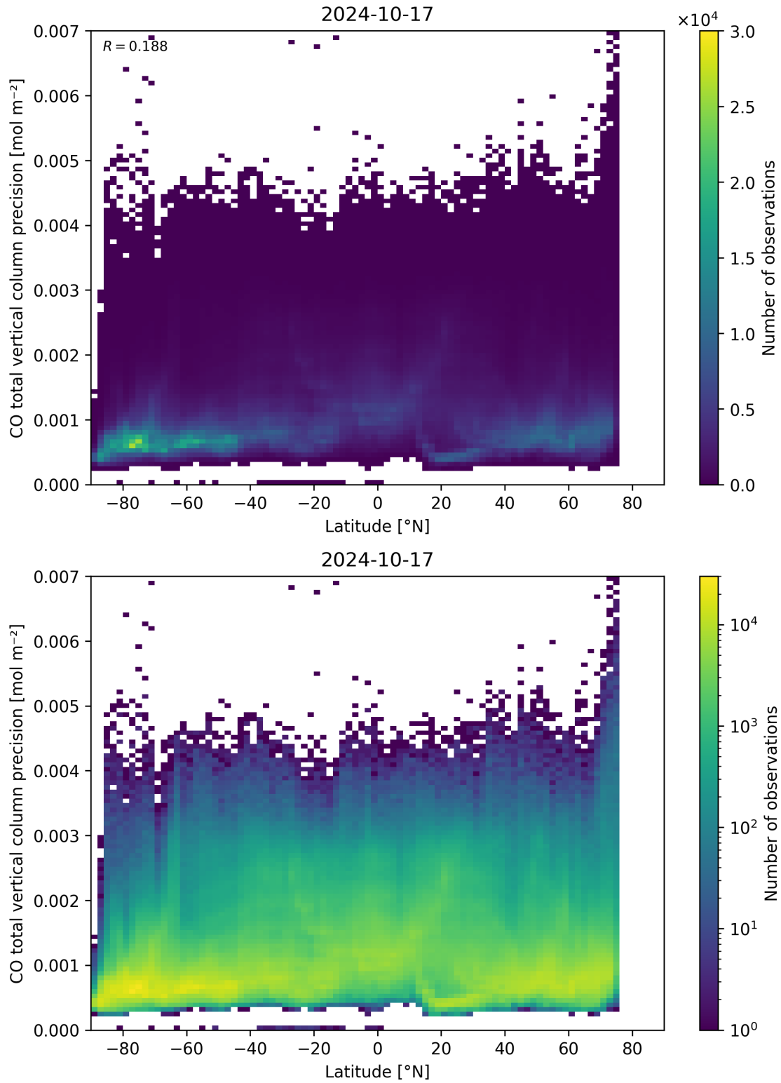
Figure 53: Scatter density plot of “Latitude” against “CO total vertical column precision” for 2024-10-16 to 2024-10-18.
