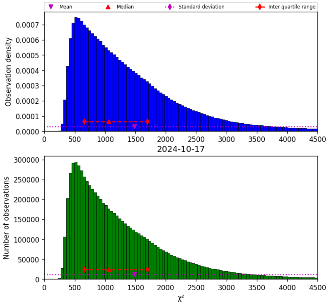
Figure 22: Histogram of “ \chi^2 ” for 2024-10-16 to 2024-10-18
