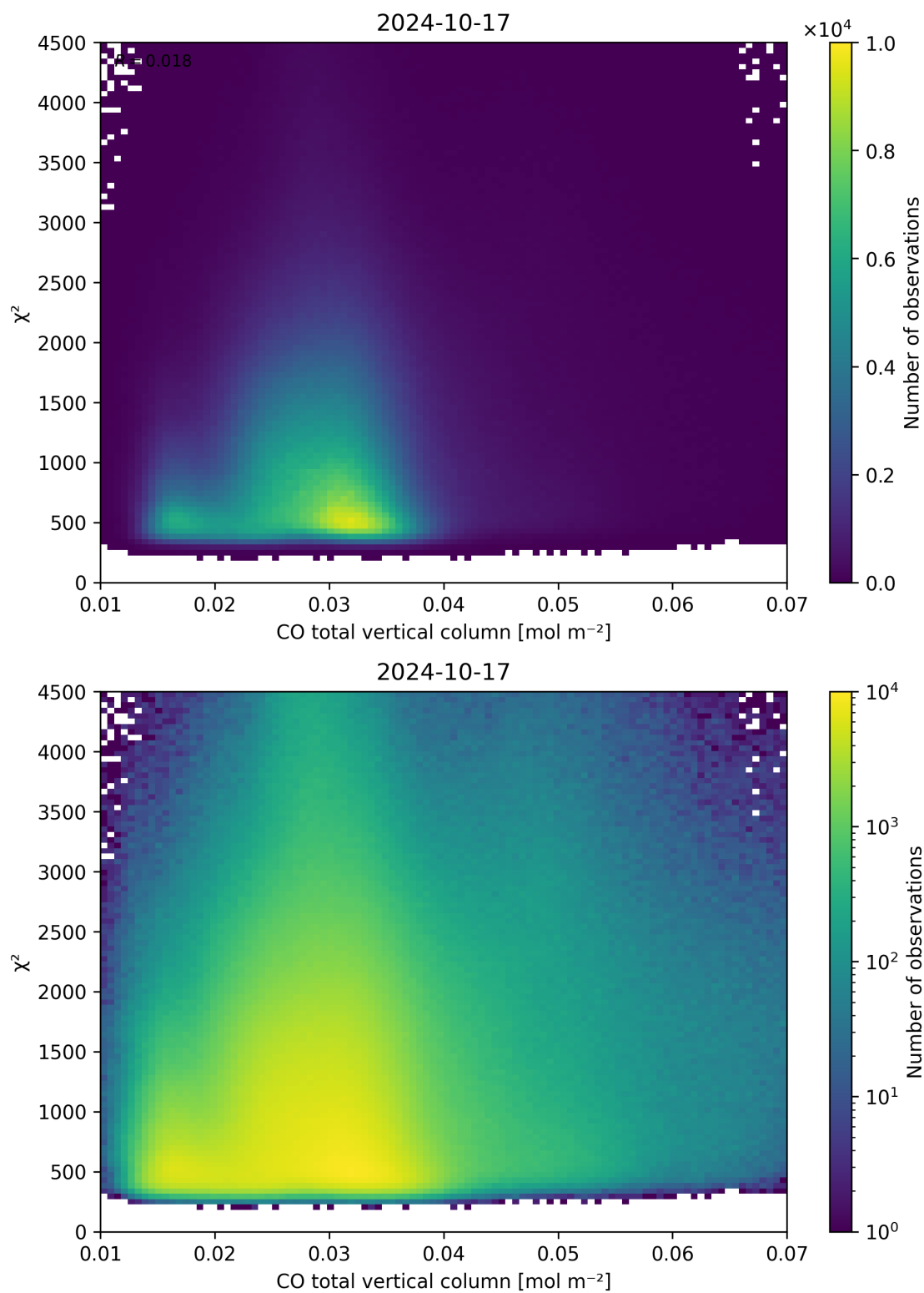
Figure 35: Scatter density plot of “CO total vertical column” against “ \chi^2 ” for 2024-10-16 to 2024-10-18.
