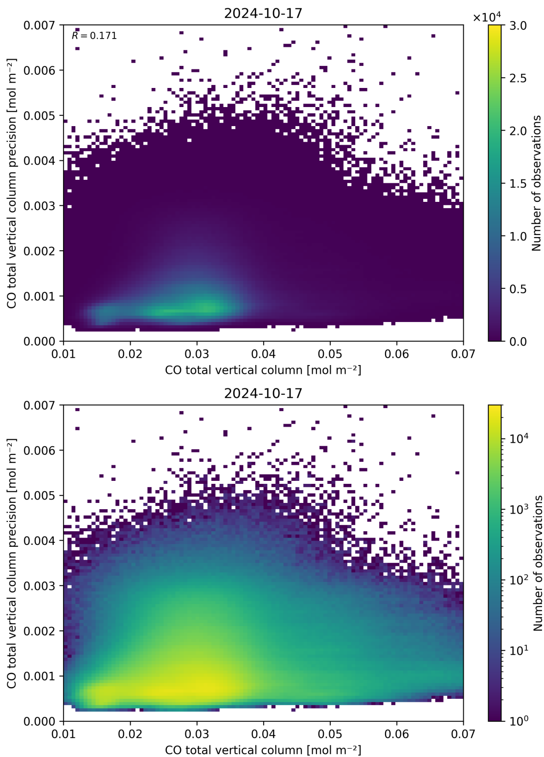
Figure 34: Scatter density plot of “CO total vertical column” against “CO total vertical column precision” for 2024-10-16 to 2024-10-18.
