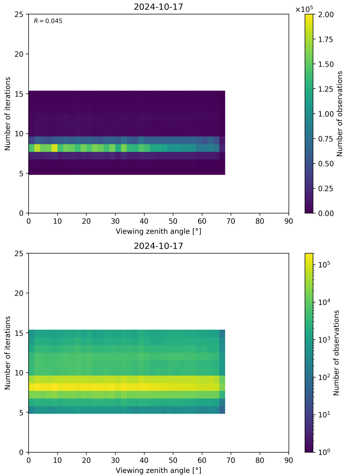
Figure 75: Scatter density plot of “Viewing zenith angle” against “Number of iterations” for 2024-10-16 to 2024-10-18.
