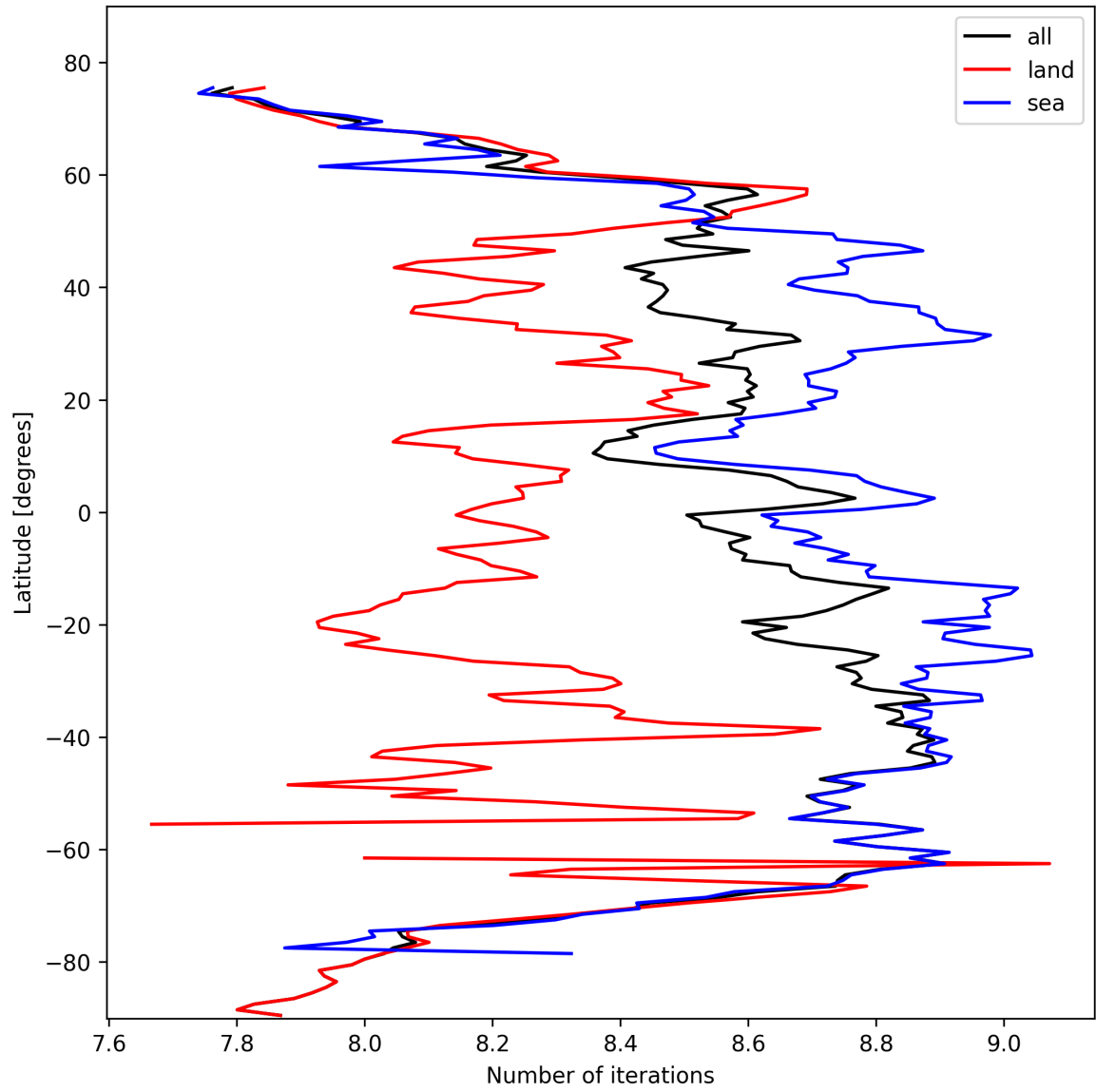
Figure 16: Zonal average of “Number of iterations” for 2024-10-16 to 2024-10-18.
