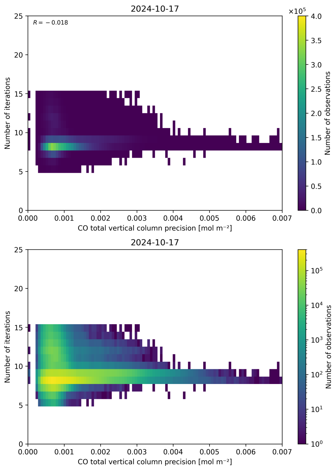
Figure 46: Scatter density plot of “CO total vertical column precision” against “Number of iterations” for 2024-10-16 to 2024-10-18.
