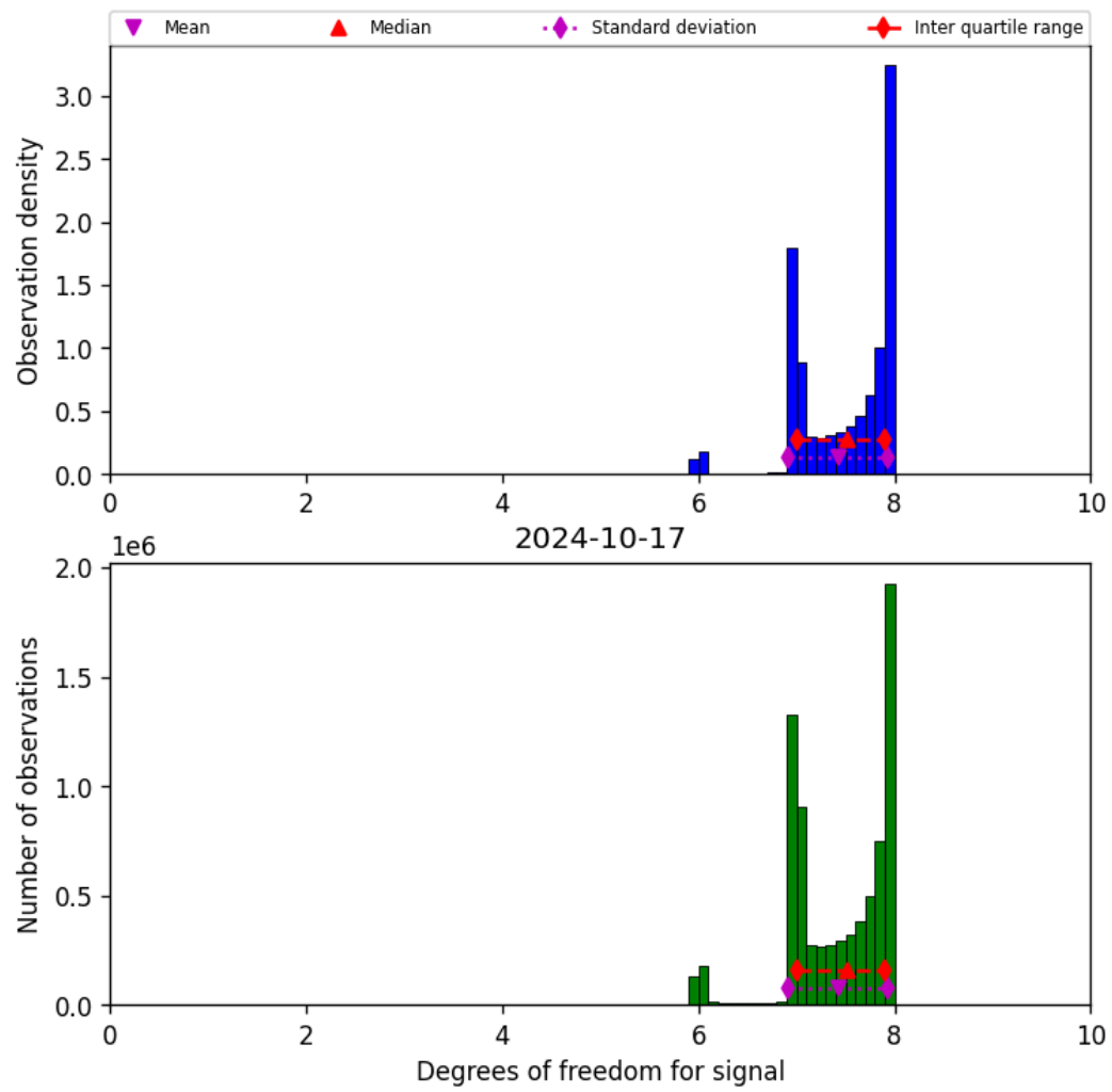
Figure 23: Histogram of “Degrees of freedom for signal” for 2024-10-16 to 2024-10-18
