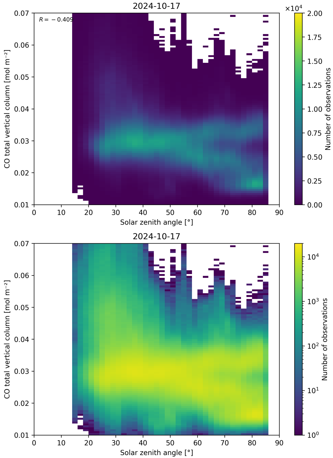
Figure 61: Scatter density plot of “Solar zenith angle” against “CO total vertical column” for 2024-10-16 to 2024-10-18.
