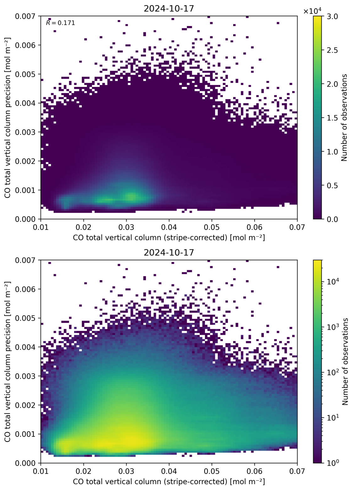
Figure 36: Scatter density plot of “CO total vertical column (stripe-corrected)” against “CO total vertical column precision” for 2024-10-16 to 2024-10-18.
