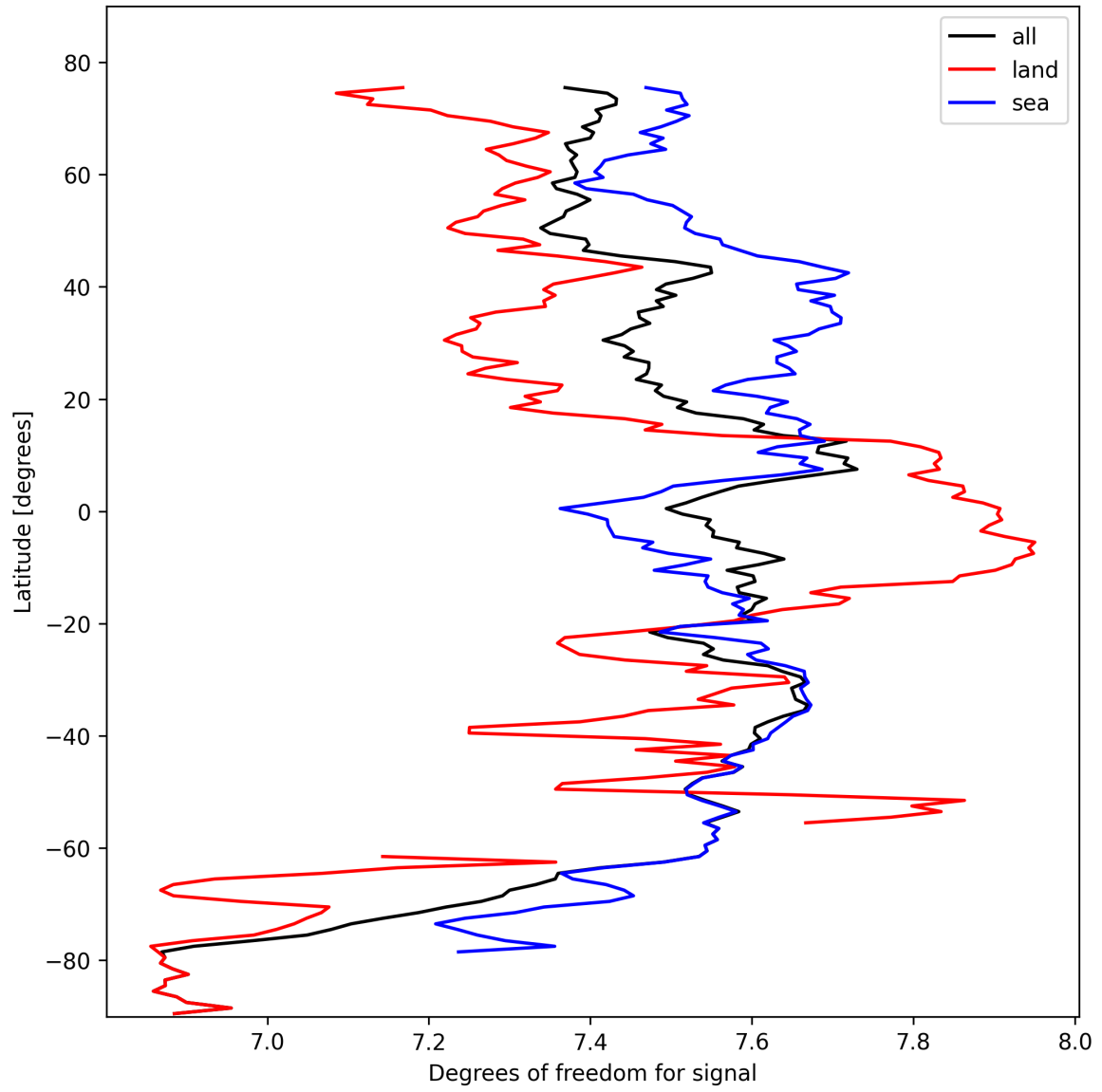
Figure 15: Zonal average of “Degrees of freedom for signal” for 2024-10-16 to 2024-10-18.
