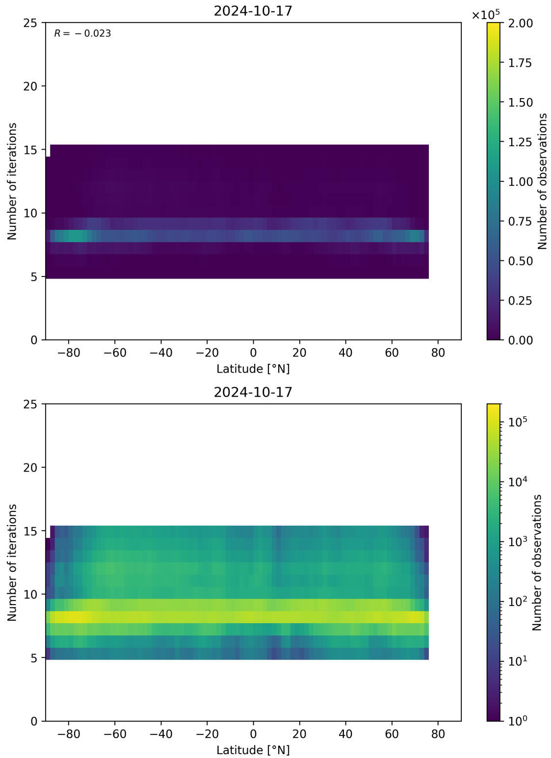
Figure 56: Scatter density plot of “Latitude” against “Number of iterations” for 2024-10-16 to 2024-10-18.
