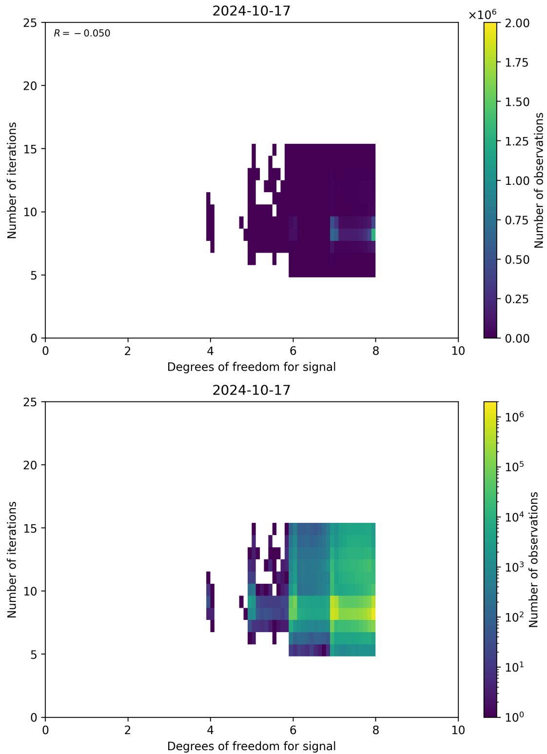
Figure 50: Scatter density plot of “Degrees of freedom for signal” against “Number of iterations” for 2024-10-16 to 2024-10-18.
