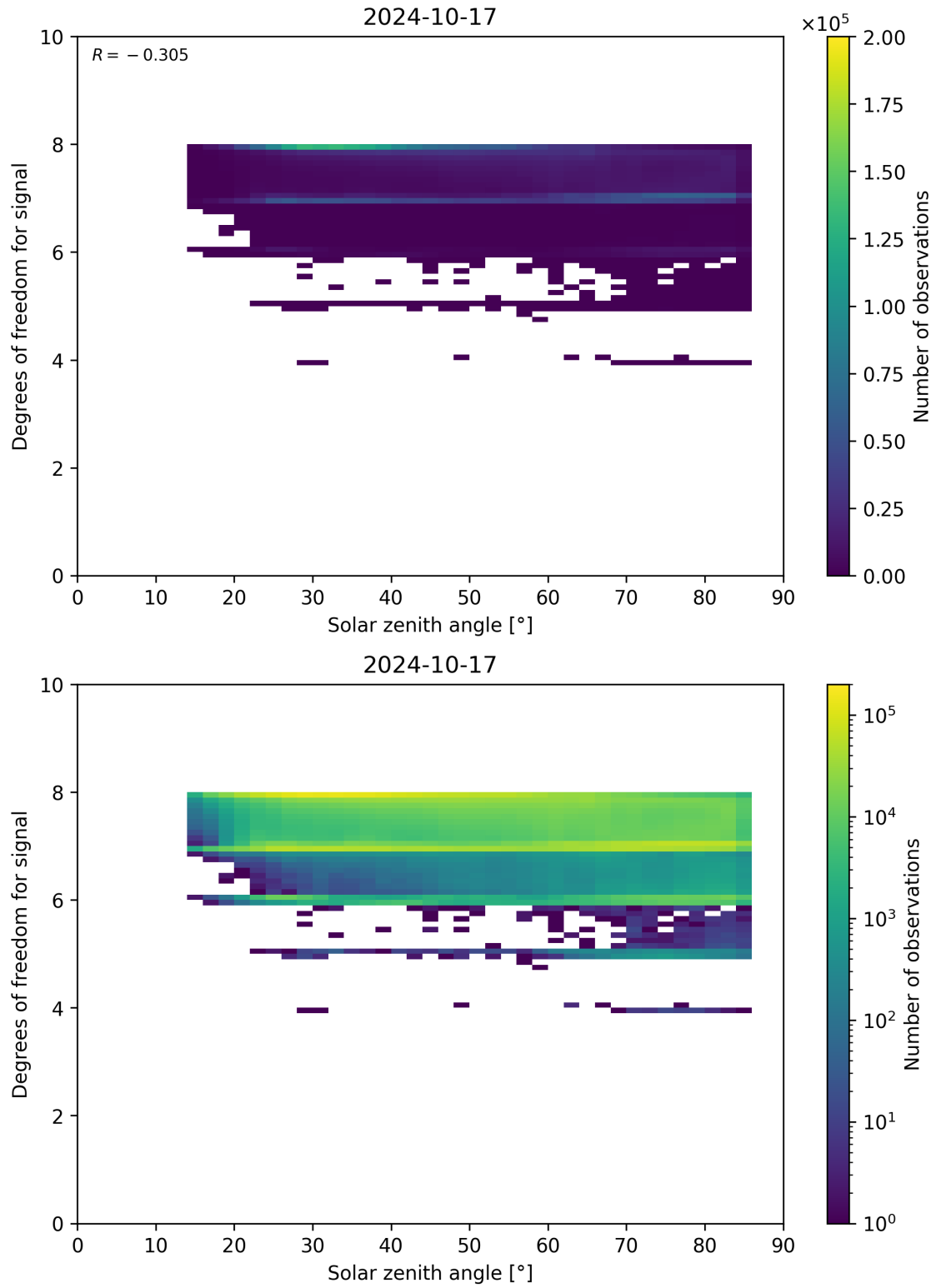
Figure 65: Scatter density plot of “Solar zenith angle” against “Degrees of freedom for signal” for 2024-10-16 to 2024-10-18.
