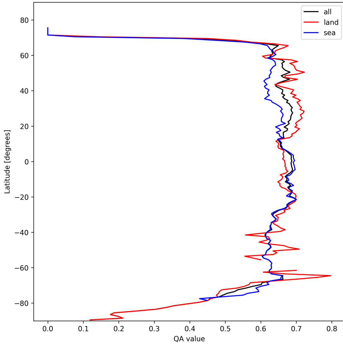
Figure 9: Zonal average of “QA value” for 2024-10-16 to 2024-10-18.
