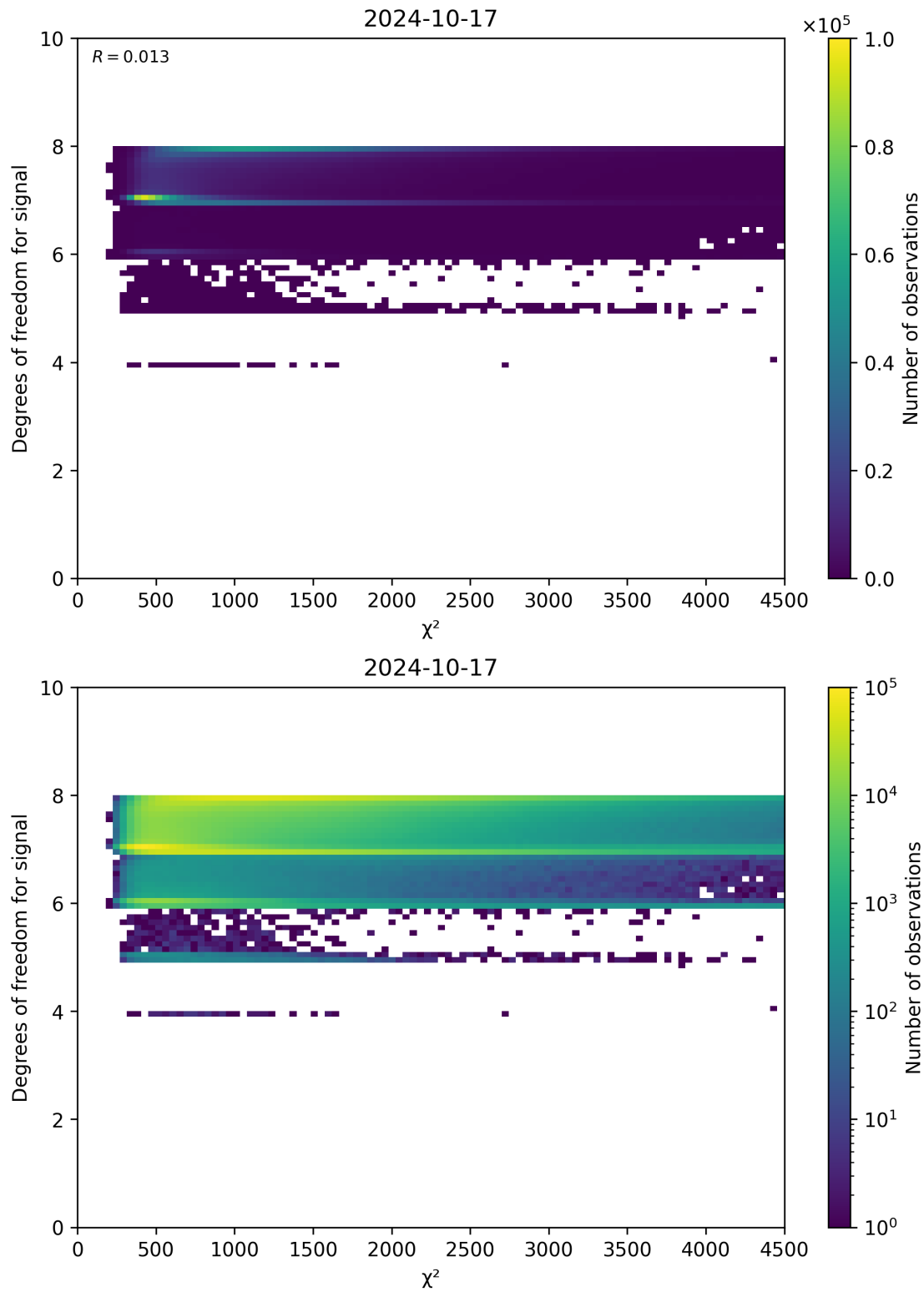
Figure 48: Scatter density plot of “ \chi^2 ” against “Degrees of freedom for signal” for 2024-10-16 to 2024-10-18.
