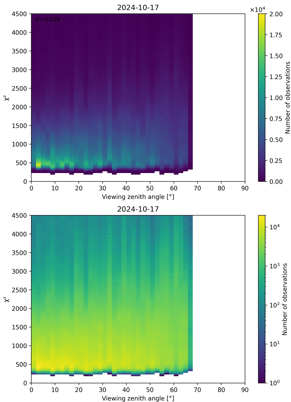
Figure 72: Scatter density plot of “Viewing zenith angle” against “ \chi^2 ” for 2024-10-16 to 2024-10-18.
