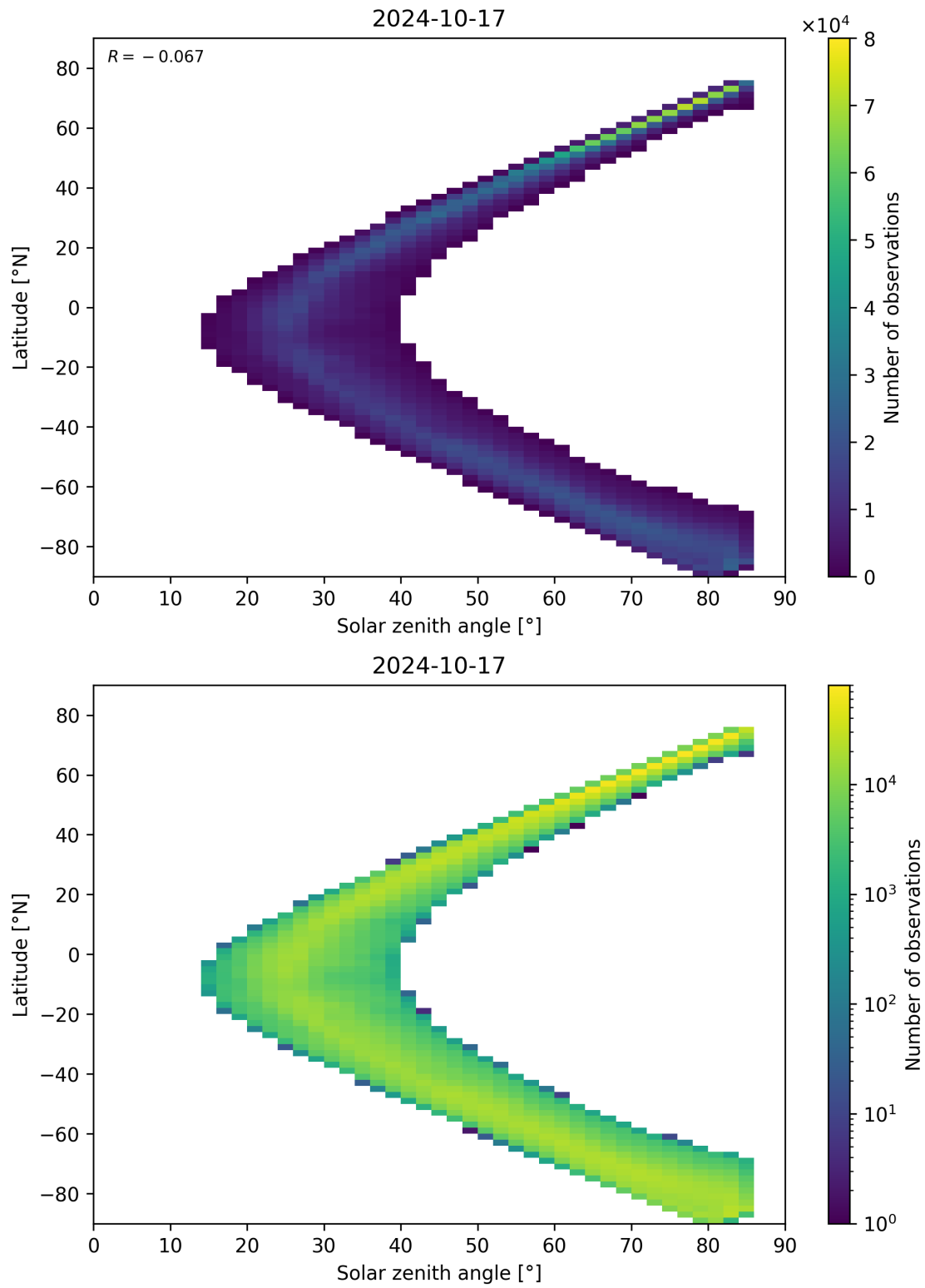
Figure 66: Scatter density plot of “Solar zenith angle” against “Latitude” for 2024-10-16 to 2024-10-18.
