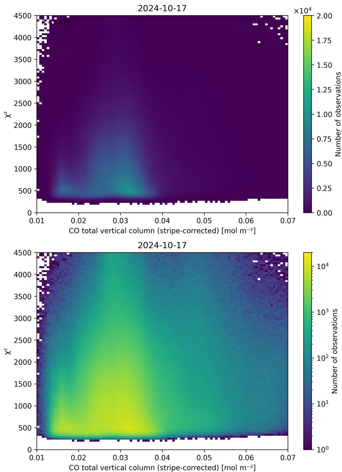
Figure 37: Scatter density plot of “CO total vertical column (stripe-corrected)” against “ \chi^2 ” for 2024-10-16 to 2024-10-18.
