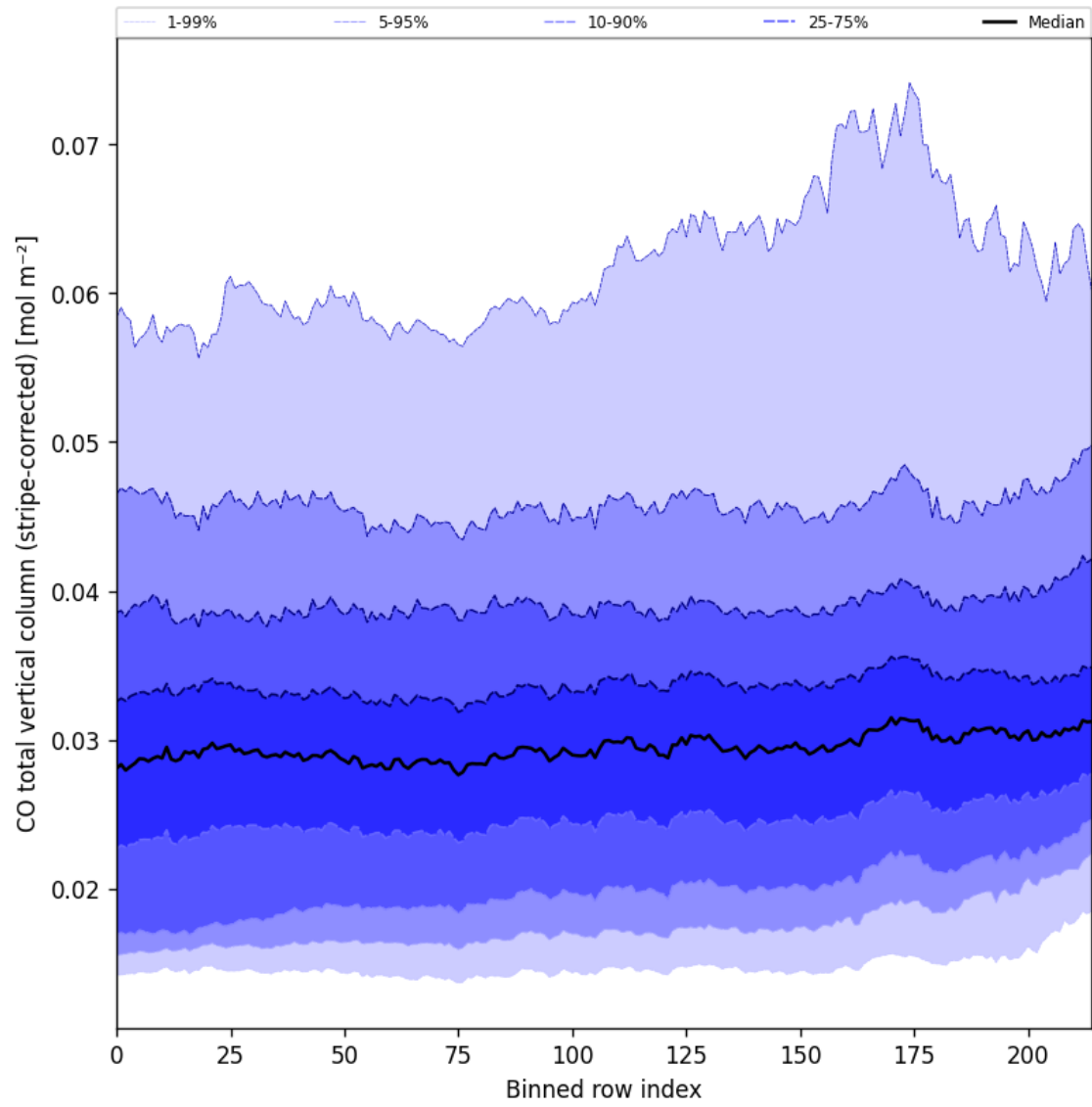
Figure 27: Along track statistics of “CO total vertical column (stripe-corrected)” for 2024-10-16 to 2024-10-18
