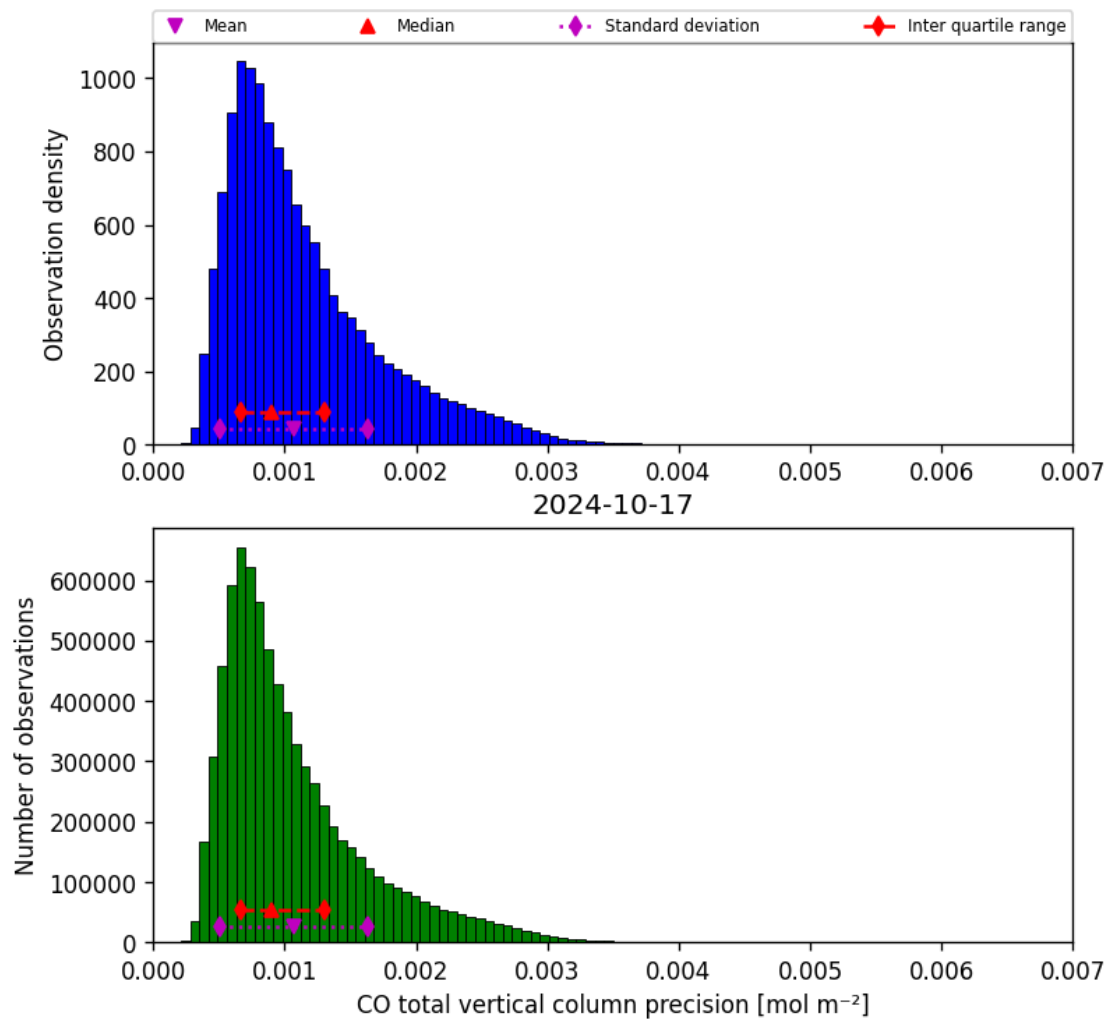
Figure 20: Histogram of “CO total vertical column precision” for 2024-10-16 to 2024-10-18
