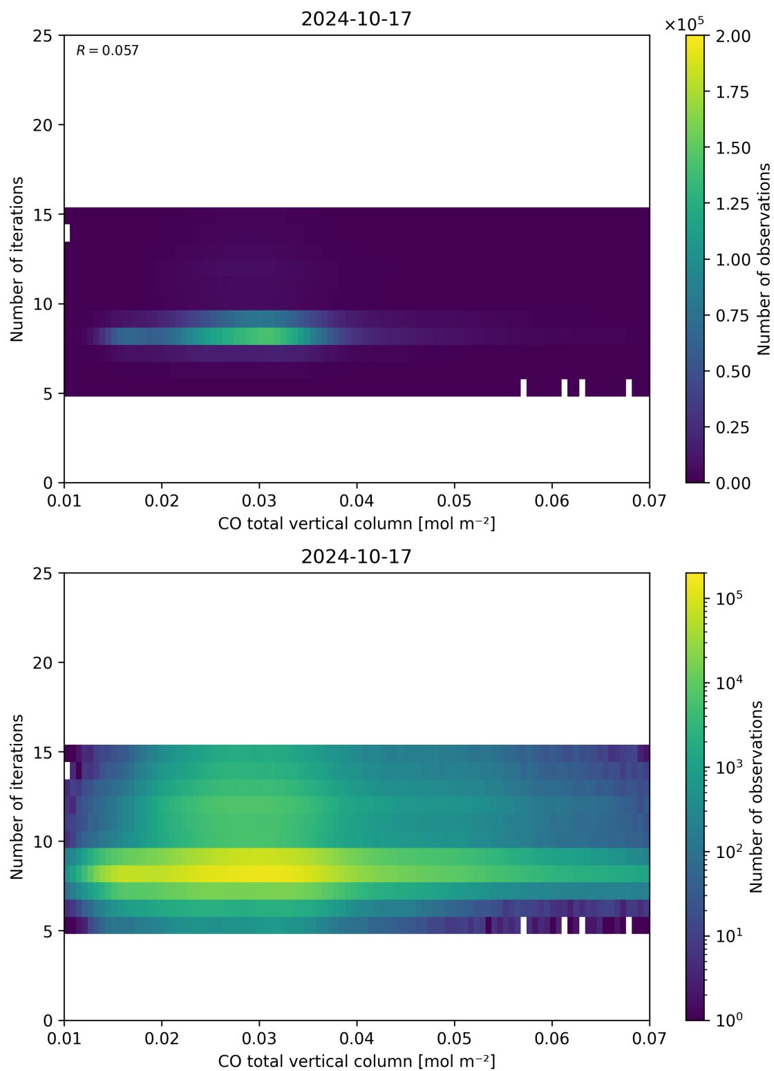
Figure 42: Scatter density plot of “CO total vertical column” against “Number of iterations” for 2024-10-16 to 2024-10-18.
