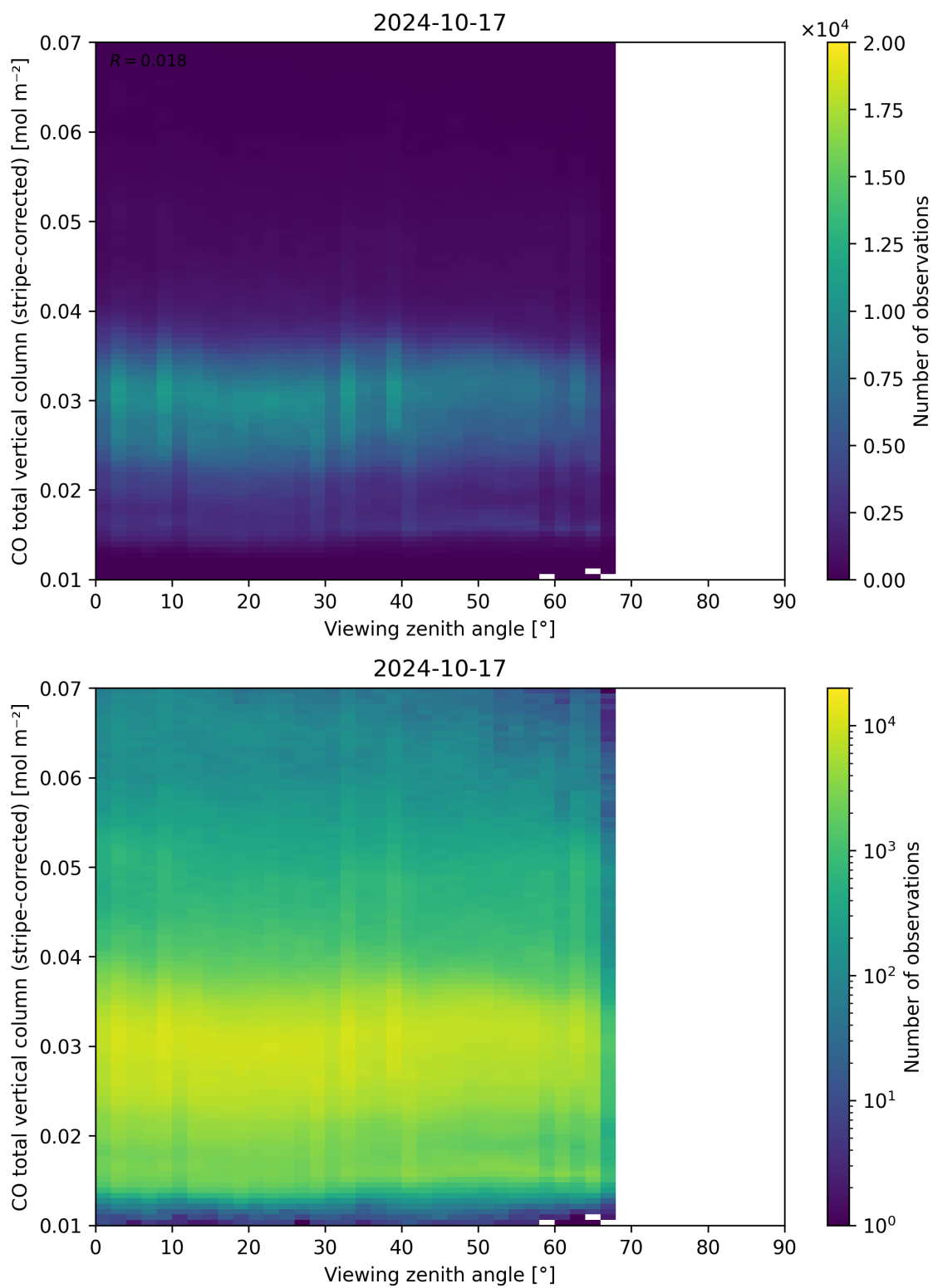
Figure 70: Scatter density plot of “Viewing zenith angle” against “CO total vertical column (stripe-corrected)” for 2024-10-16 to 2024-10-18.
