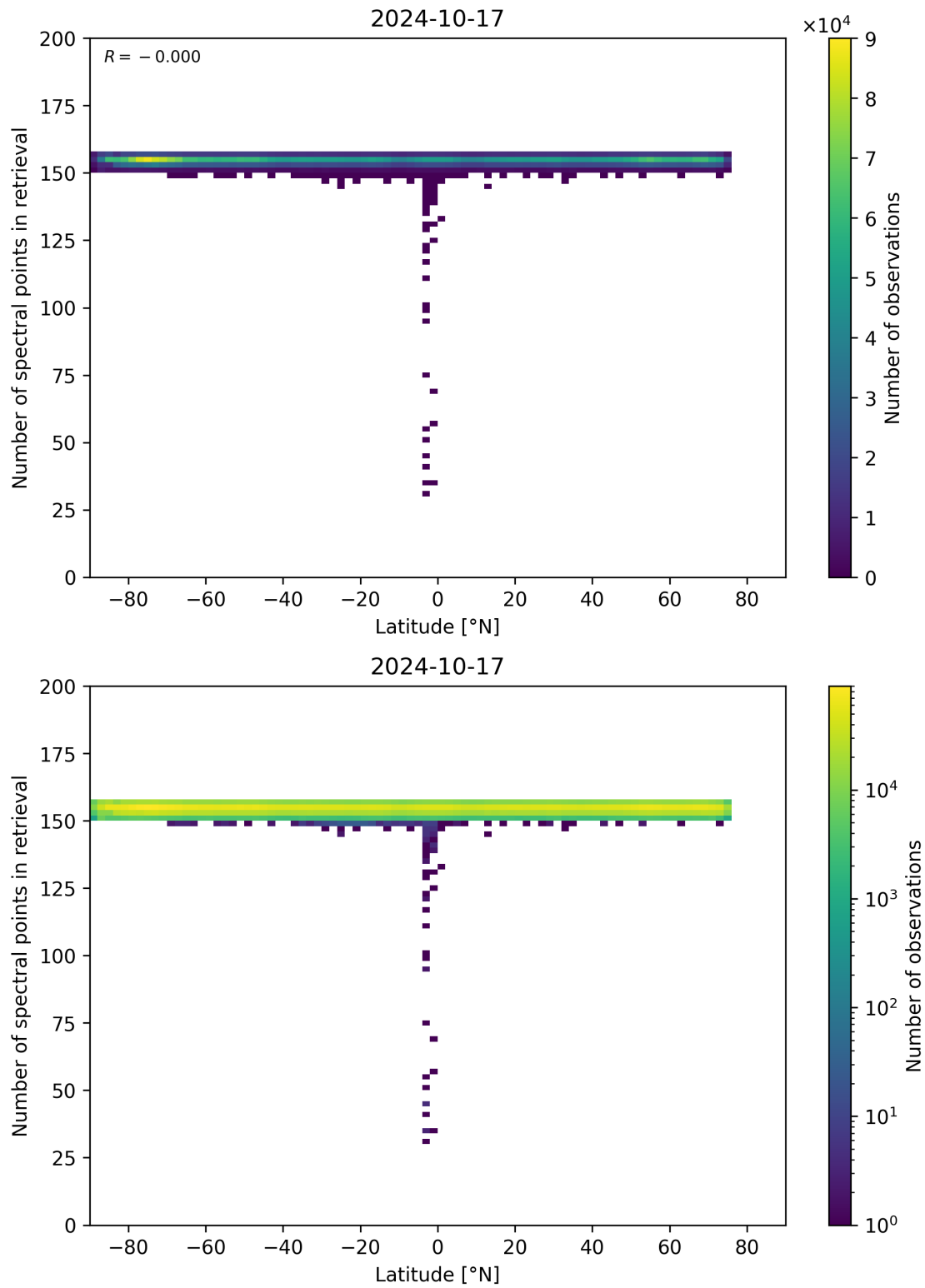
Figure 57: Scatter density plot of “Latitude” against “Number of spectral points in retrieval” for 2024-10-16 to 2024-10-18.
