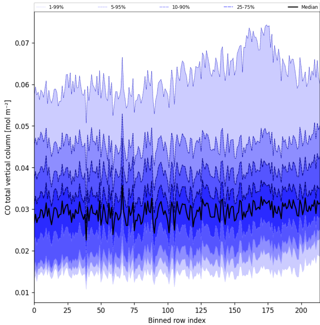
Figure 26: Along track statistics of “CO total vertical column” for 2024-10-16 to 2024-10-18
