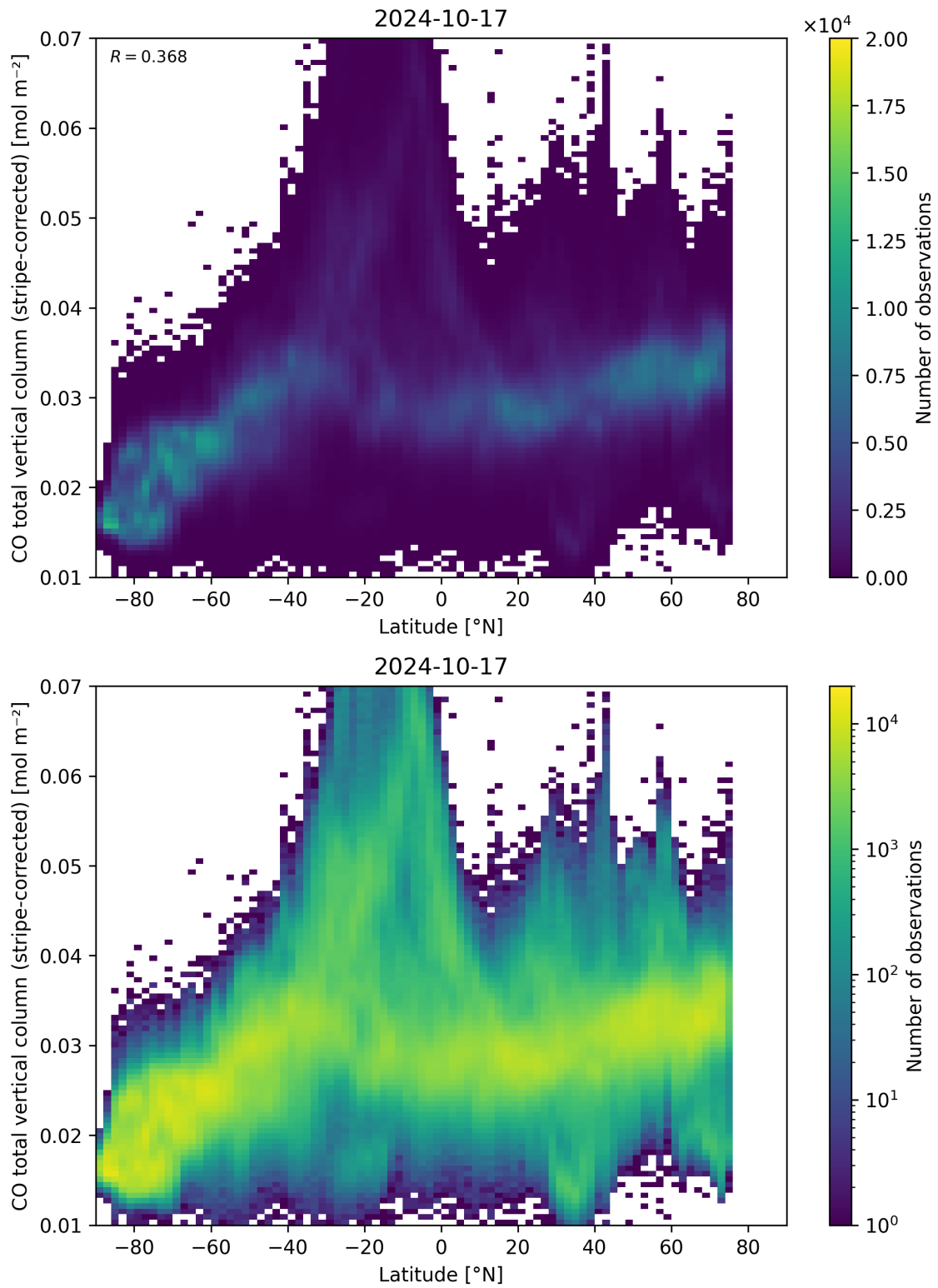
Figure 52: Scatter density plot of “Latitude” against “CO total vertical column (stripe-corrected)” for 2024-10-16 to 2024-10-18.
