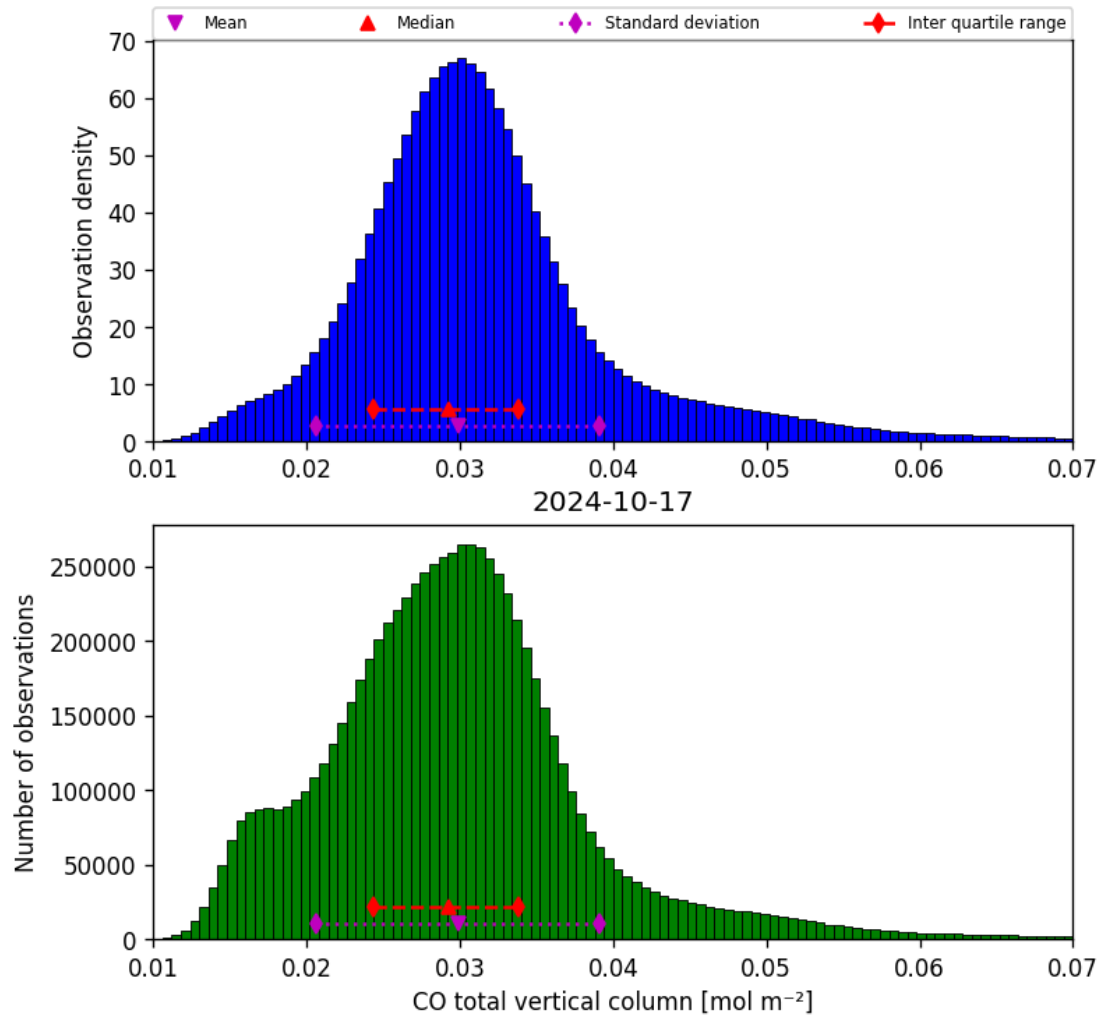
Figure 18: Histogram of “CO total vertical column” for 2024-10-16 to 2024-10-18
