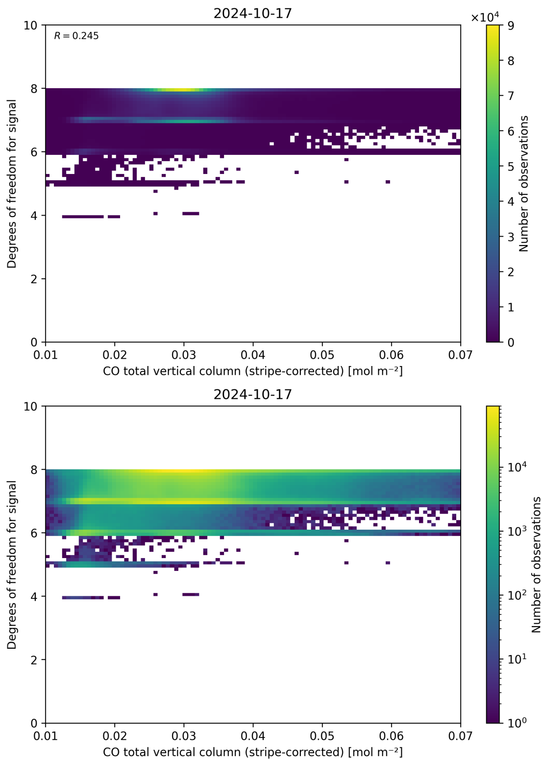
Figure 38: Scatter density plot of “CO total vertical column (stripe-corrected)” against “Degrees of freedom for signal” for 2024-10-16 to 2024-10-18.
