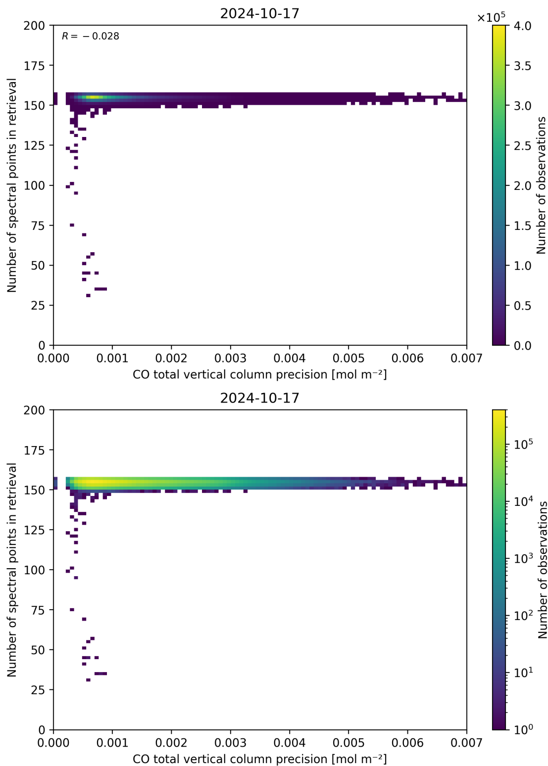
Figure 47: Scatter density plot of “CO total vertical column precision” against “Number of spectral points in retrieval” for 2024-10-16 to 2024-10-18.
