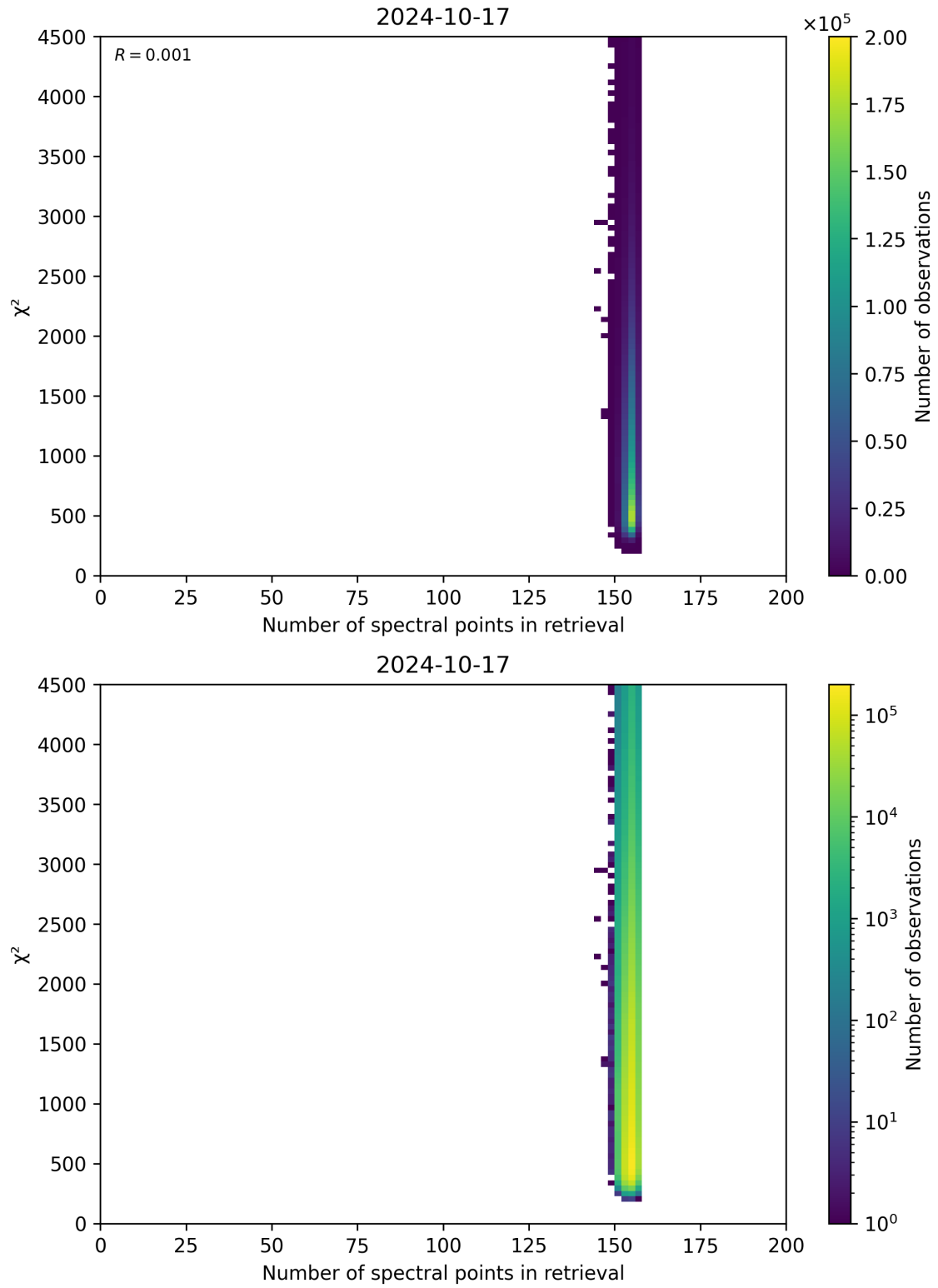
Figure 58: Scatter density plot of “Number of spectral points in retrieval” against “ \chi^2 ” for 2024-10-16 to 2024-10-18.
