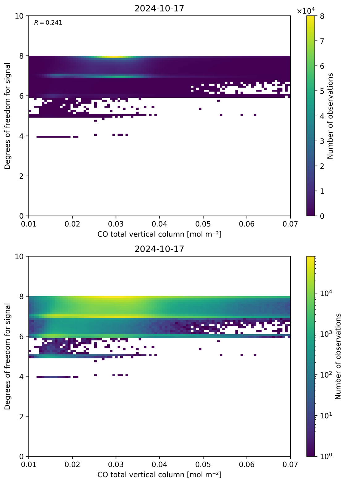
Figure 41: Scatter density plot of “CO total vertical column” against “Degrees of freedom for signal” for 2024-10-16 to 2024-10-18.
