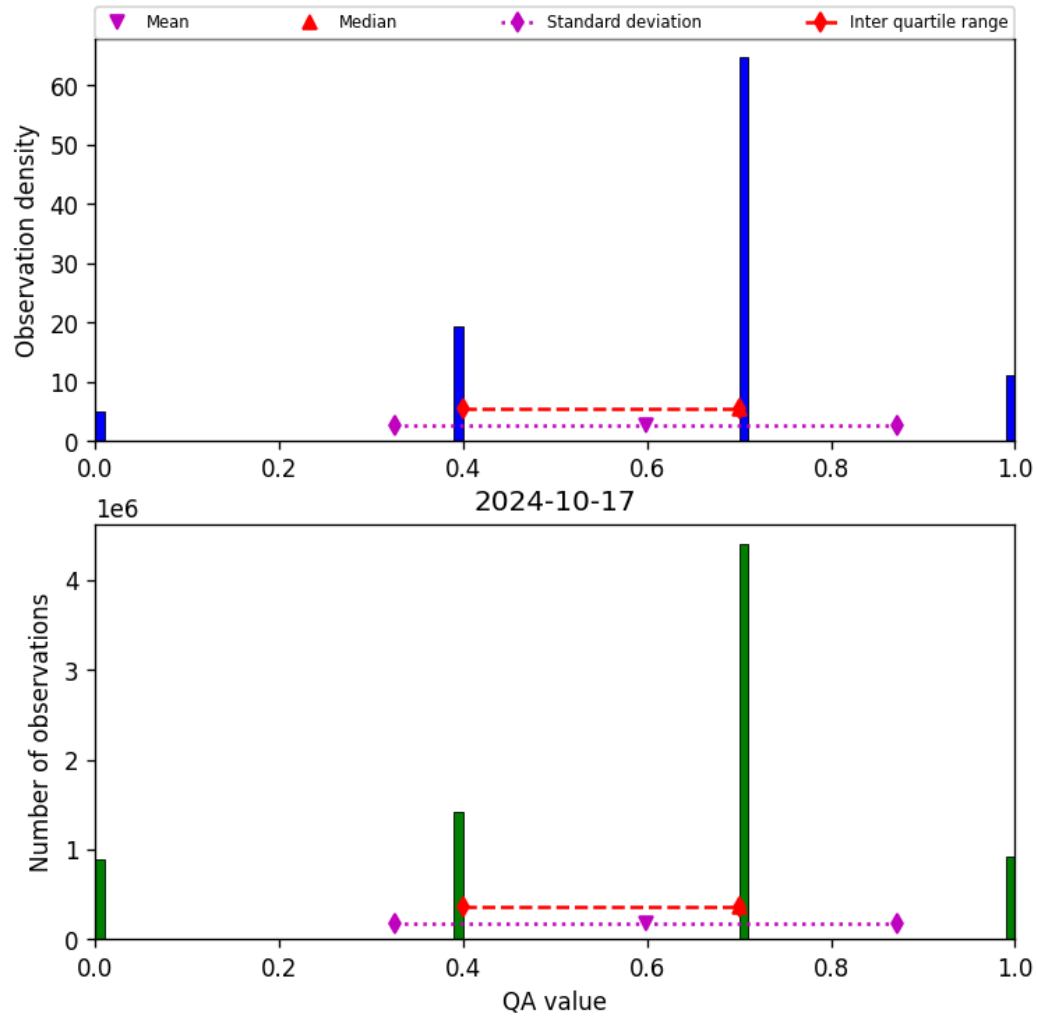
Figure 17: Histogram of “QA value” for 2024-10-16 to 2024-10-18
