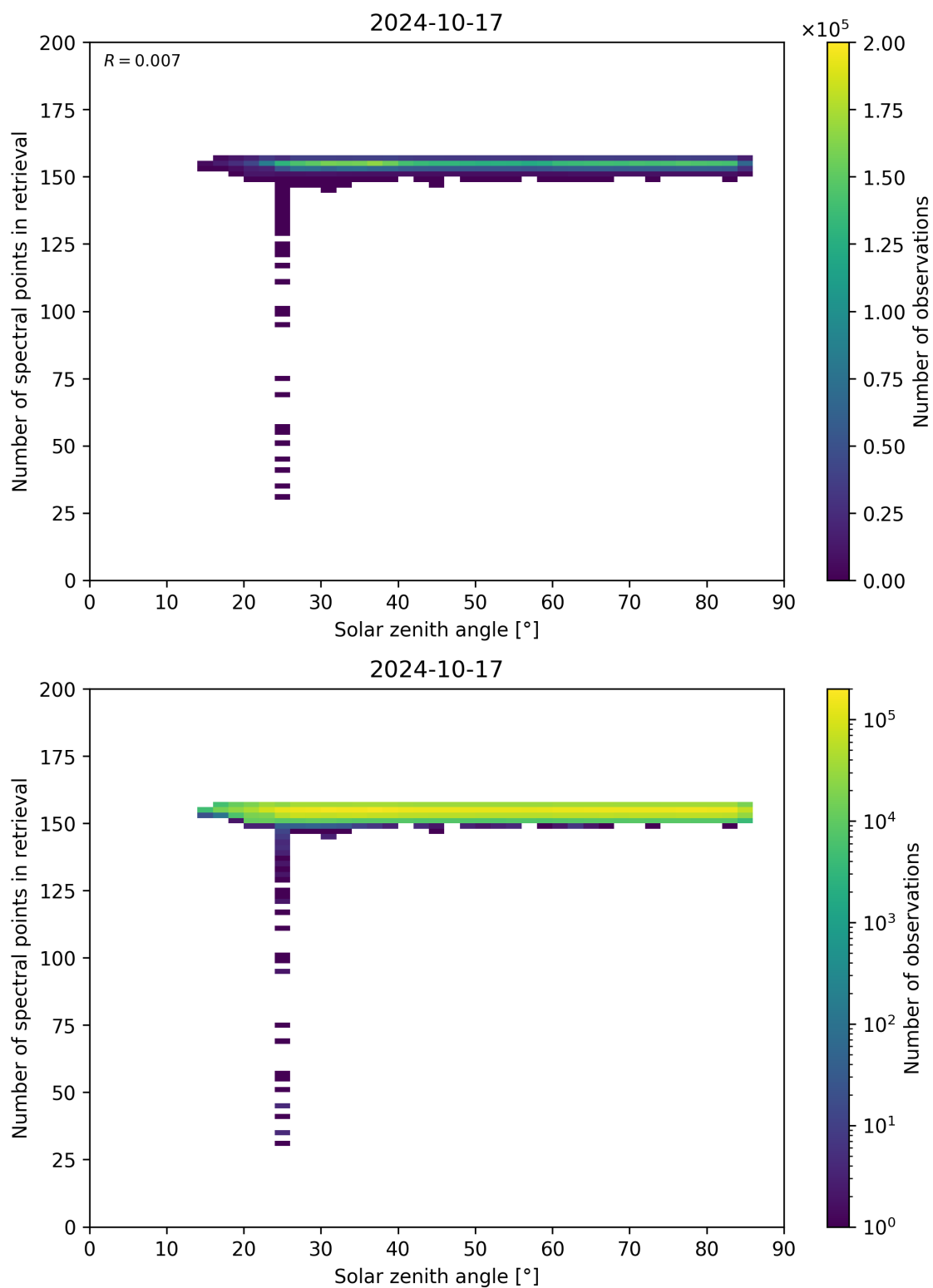
Figure 68: Scatter density plot of “Solar zenith angle” against “Number of spectral points in retrieval” for 2024-10-16 to 2024-10-18.
