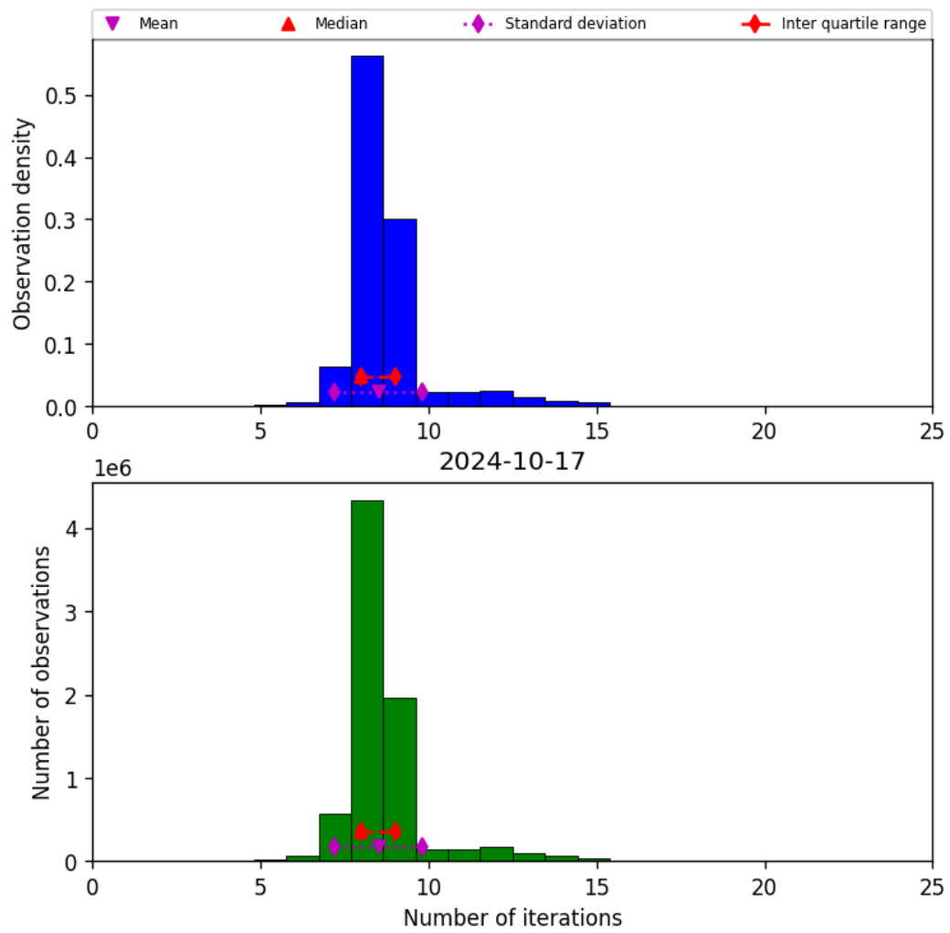
Figure 24: Histogram of “Number of iterations” for 2024-10-16 to 2024-10-18
