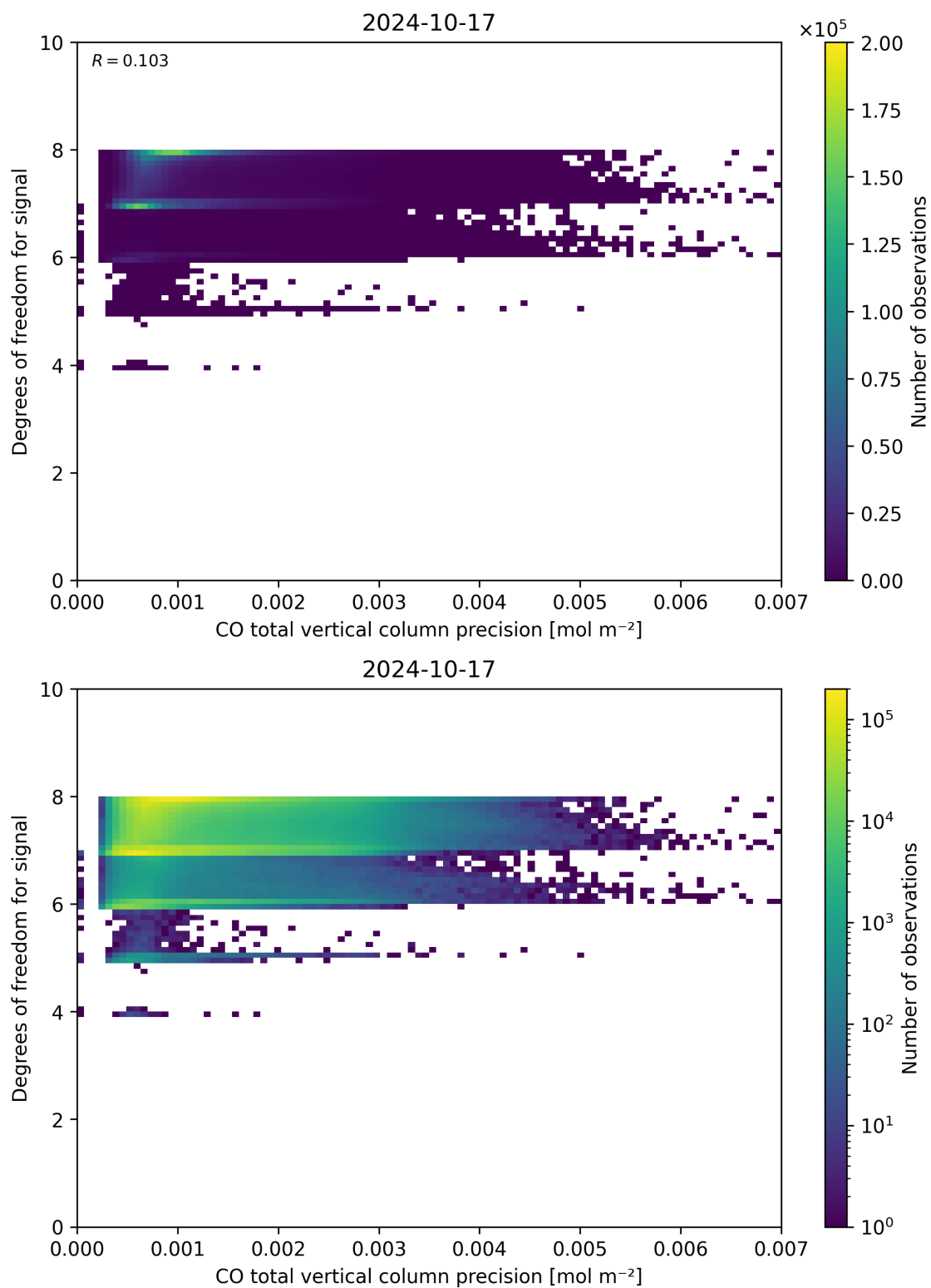
Figure 45: Scatter density plot of “CO total vertical column precision” against “Degrees of freedom for signal” for 2024-10-16 to 2024-10-18.
