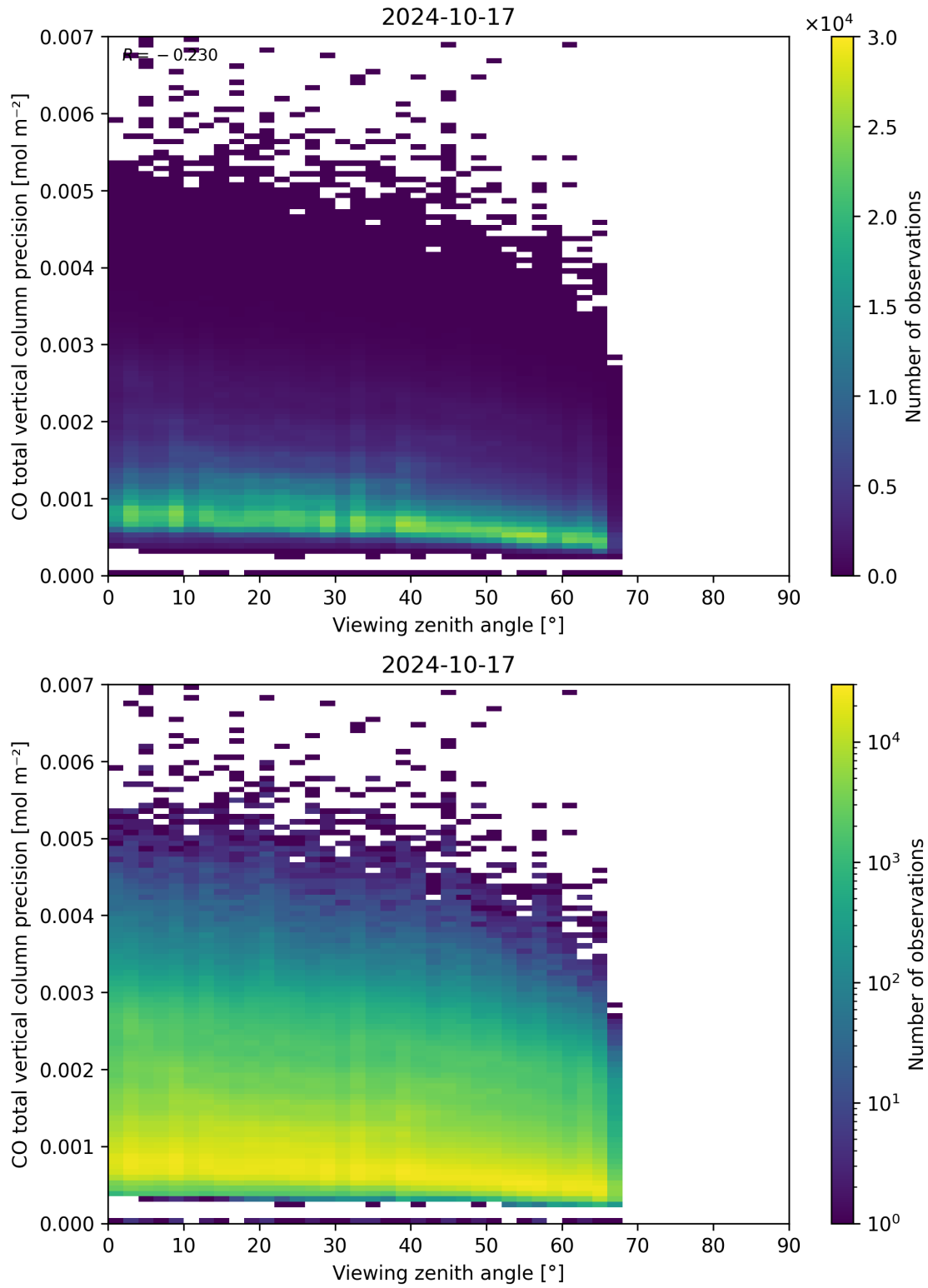
Figure 71: Scatter density plot of “Viewing zenith angle” against “CO total vertical column precision” for 2024-10-16 to 2024-10-18.
