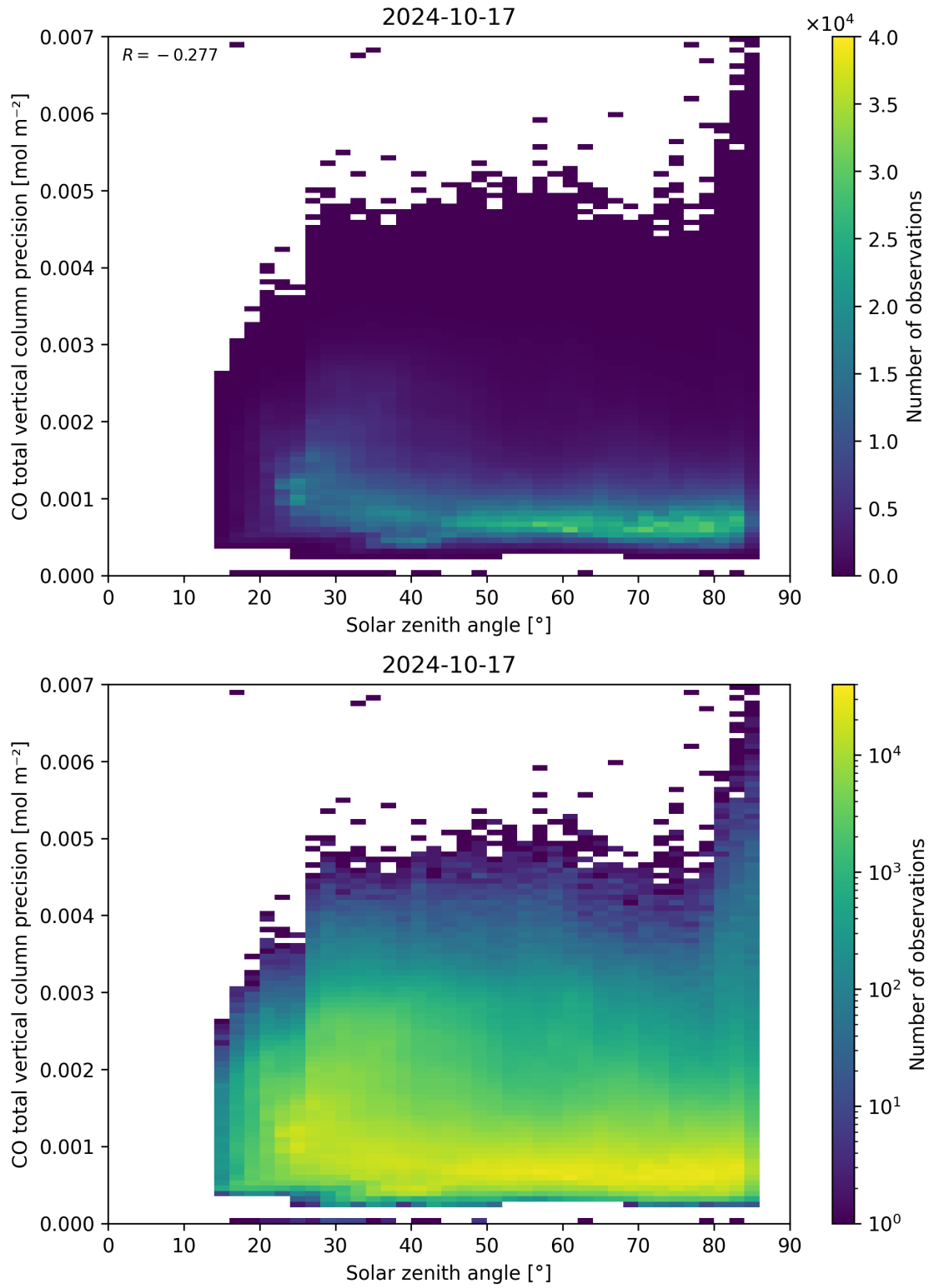
Figure 63: Scatter density plot of “Solar zenith angle” against “CO total vertical column precision” for 2024-10-16 to 2024-10-18.
