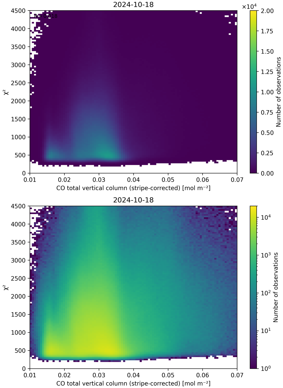
Figure 37: Scatter density plot of “CO total vertical column (stripe-corrected)” against “ \chi^2 ” for 2024-10-17 to 2024-10-19.
