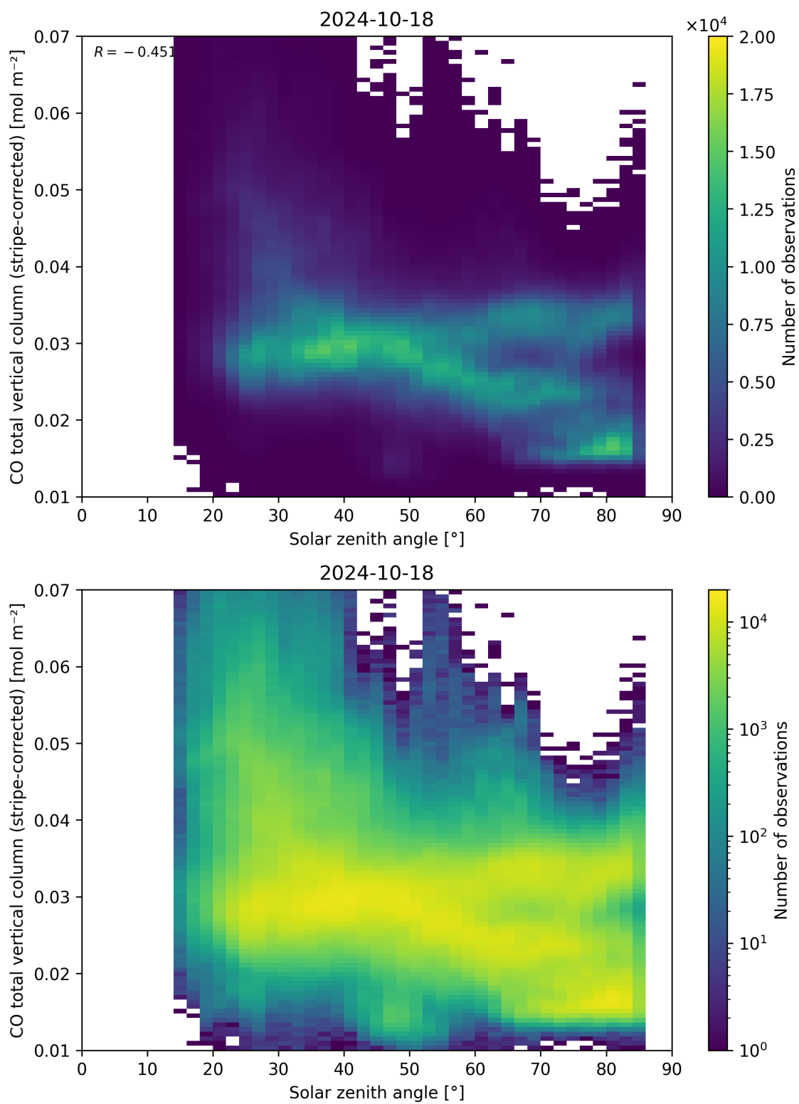
Figure 62: Scatter density plot of “Solar zenith angle” against “CO total vertical column (stripe-corrected)” for 2024-10-17 to 2024-10-19.
