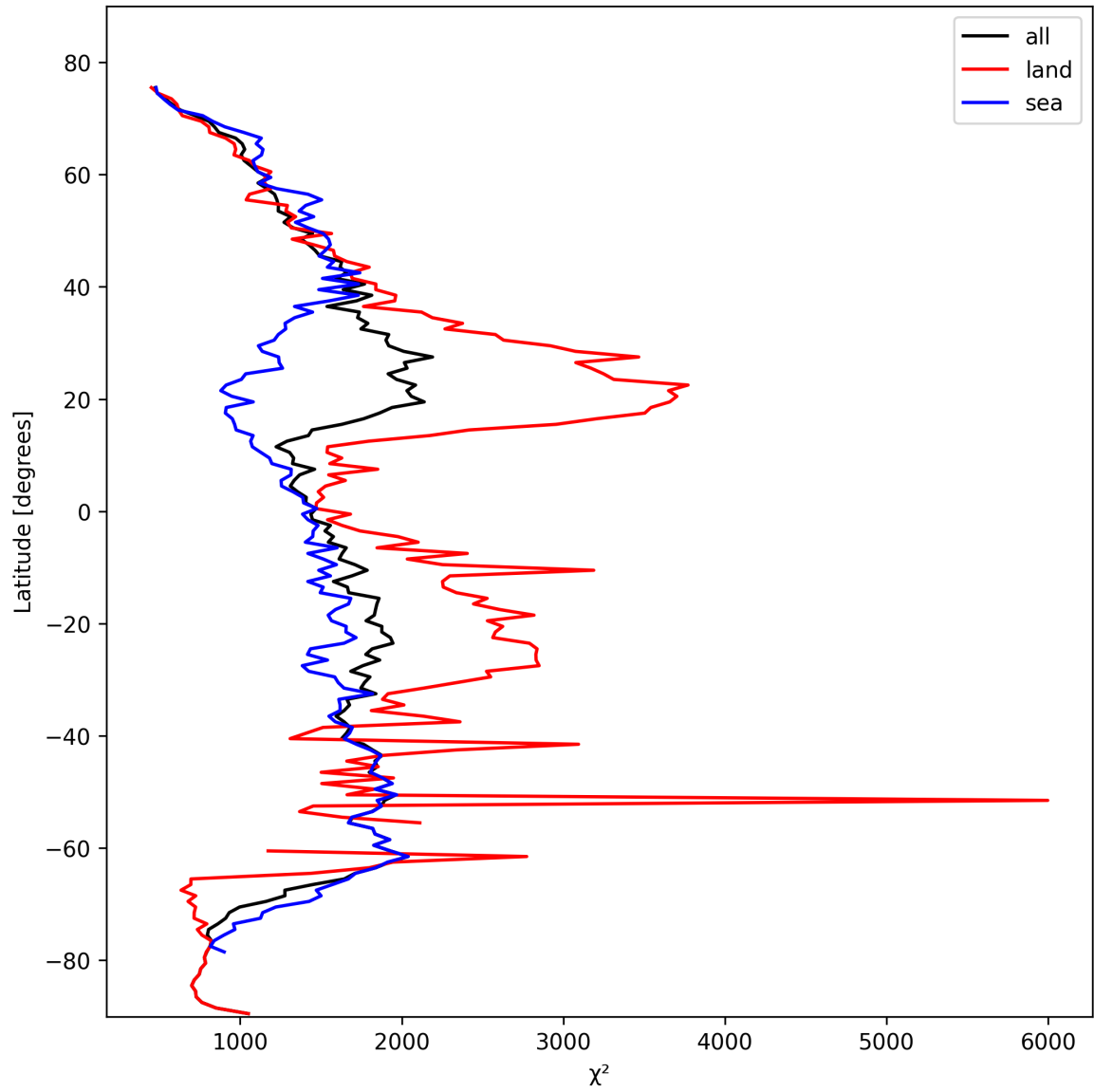
Figure 14: Zonal average of “ \chi^2 ” for 2024-10-17 to 2024-10-19.
