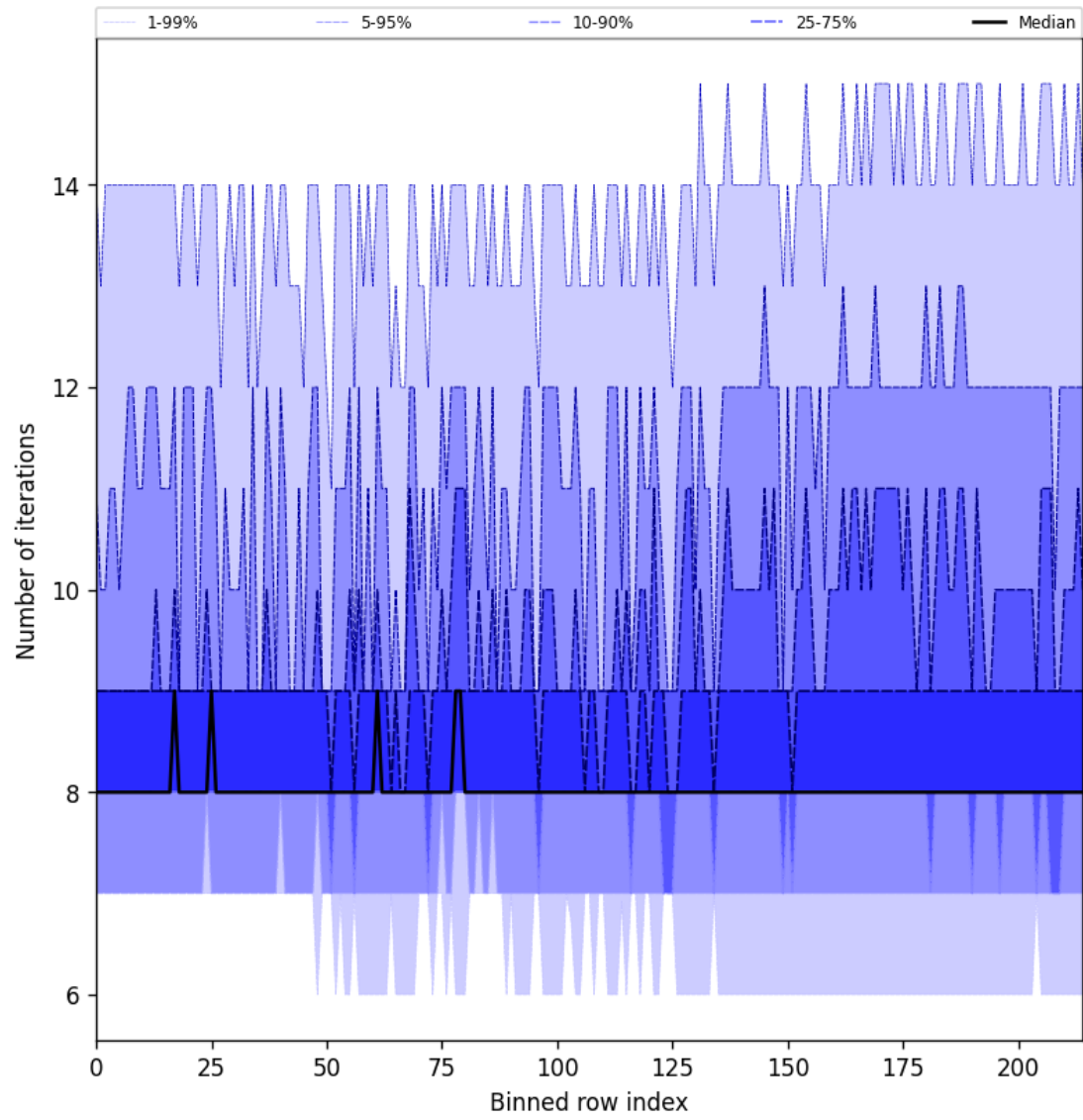
Figure 32: Along track statistics of “Number of iterations” for 2024-10-17 to 2024-10-19
