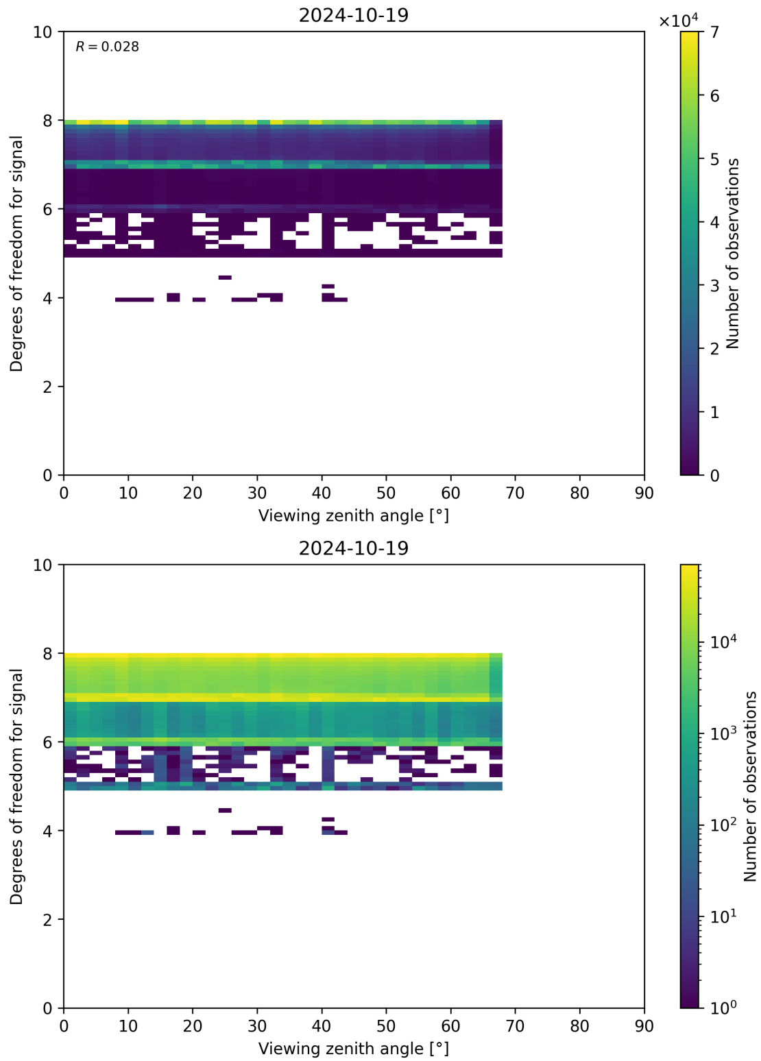
Figure 73: Scatter density plot of “Viewing zenith angle” against “Degrees of freedom for signal” for 2024-10-19 to 2024-10-20.
