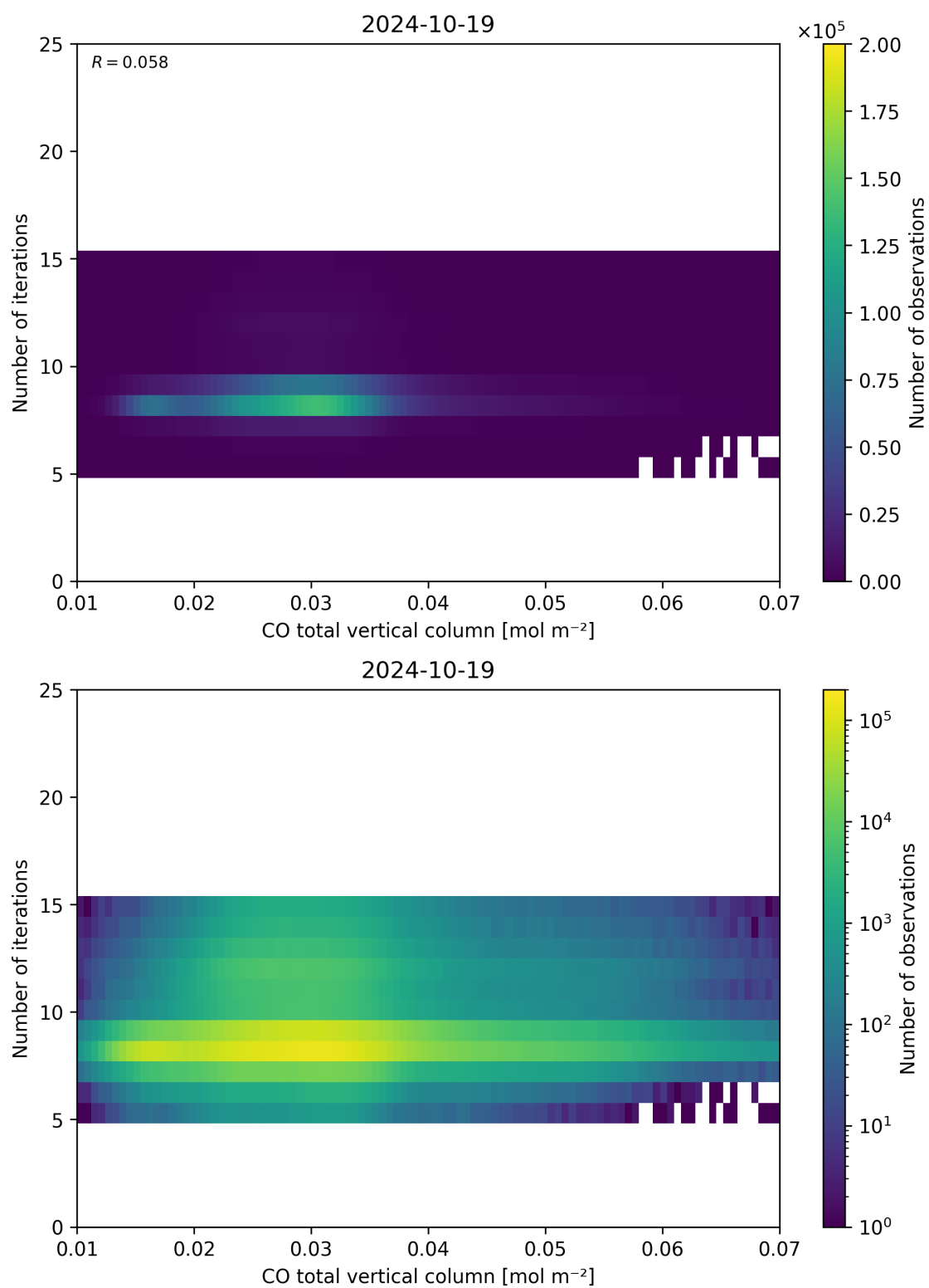
Figure 42: Scatter density plot of “CO total vertical column” against “Number of iterations” for 2024-10-19 to 2024-10-20.
