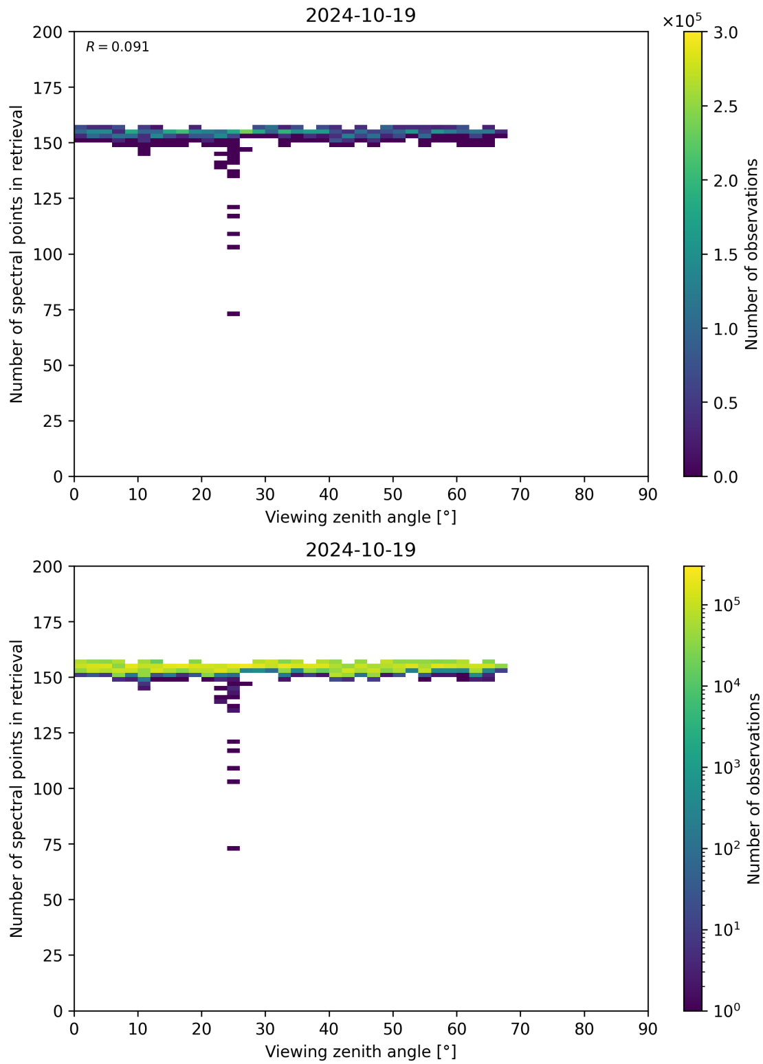
Figure 76: Scatter density plot of “Viewing zenith angle” against “Number of spectral points in retrieval” for 2024-10-19 to 2024-10-20.
