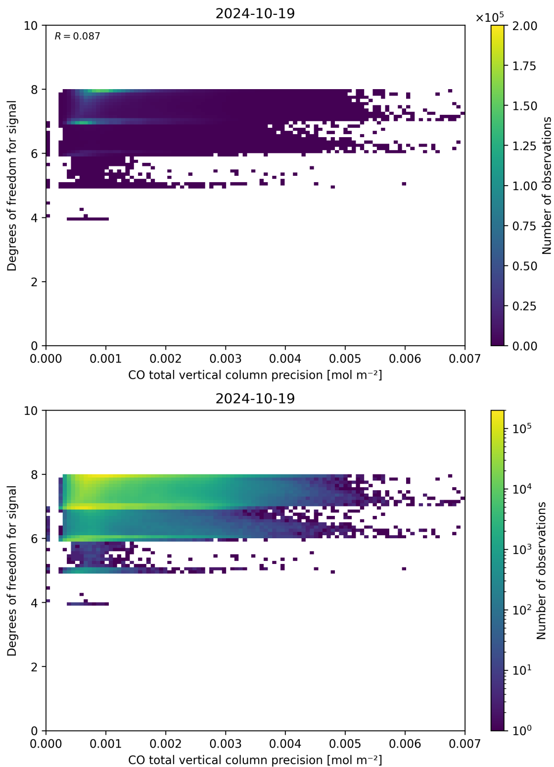
Figure 45: Scatter density plot of “CO total vertical column precision” against “Degrees of freedom for signal” for 2024-10-19 to 2024-10-20.
