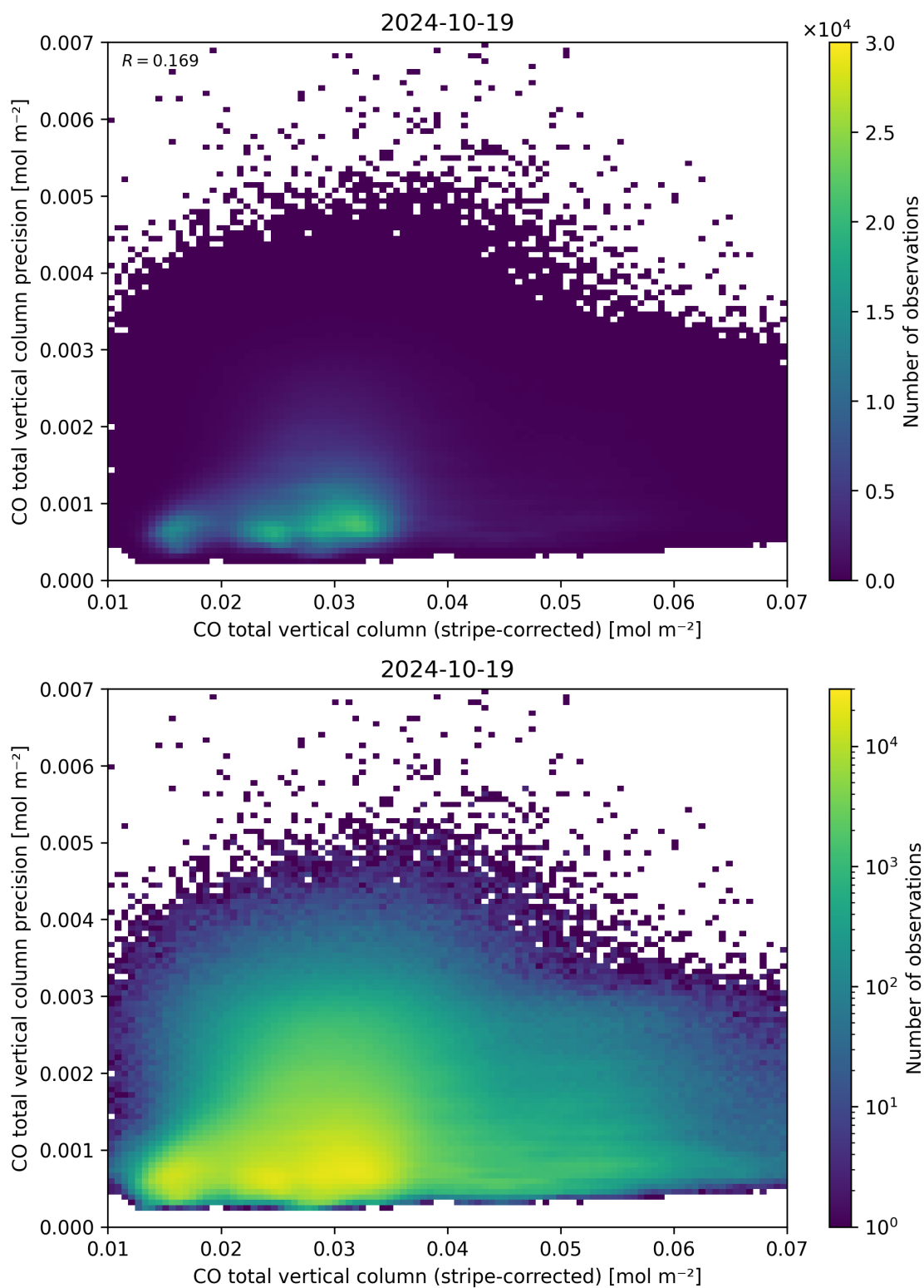
Figure 36: Scatter density plot of “CO total vertical column (stripe-corrected)” against “CO total vertical column precision” for 2024-10-19 to 2024-10-20.
