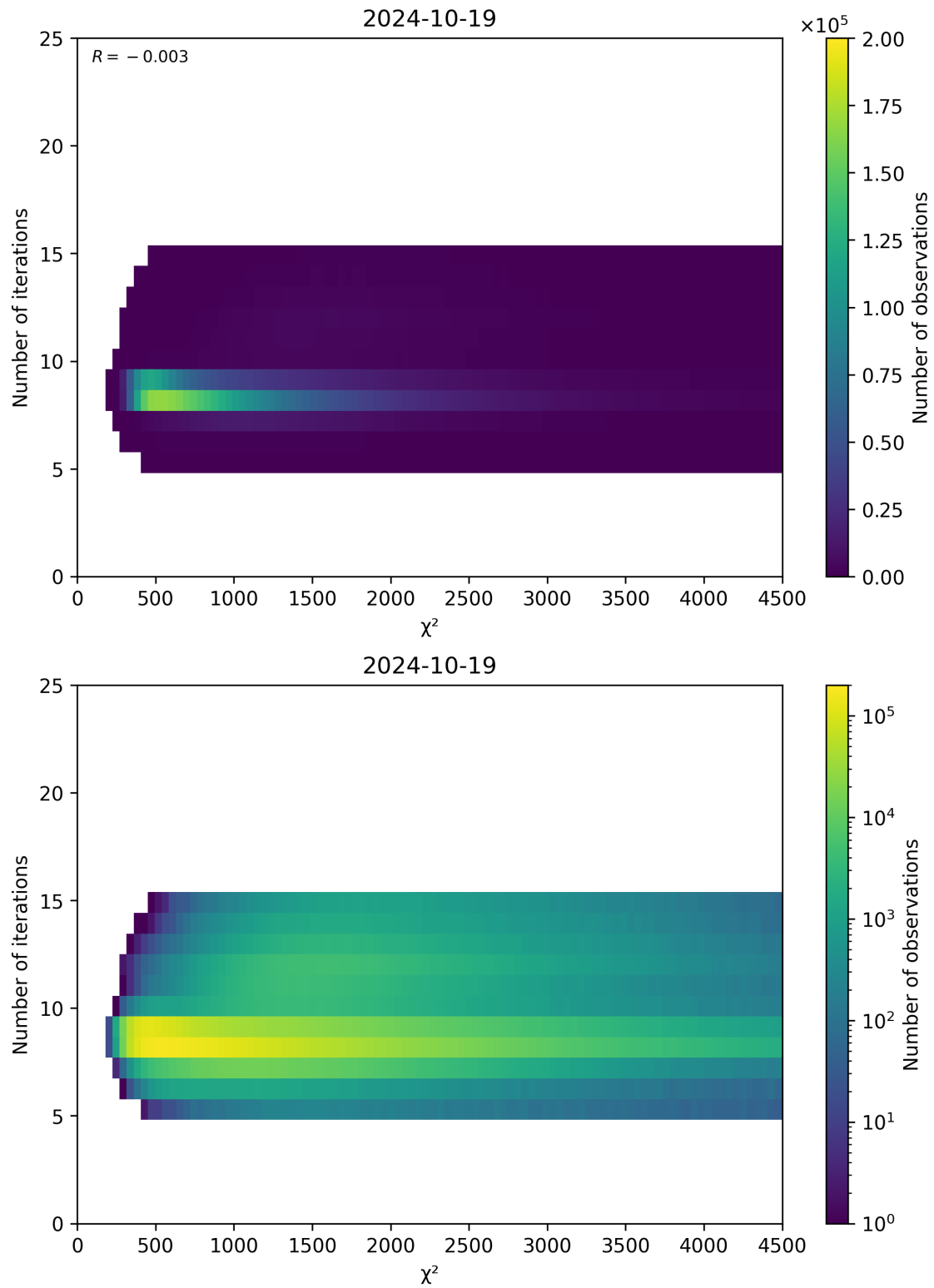
Figure 49: Scatter density plot of “ \chi^2 ” against “Number of iterations” for 2024-10-19 to 2024-10-20.
