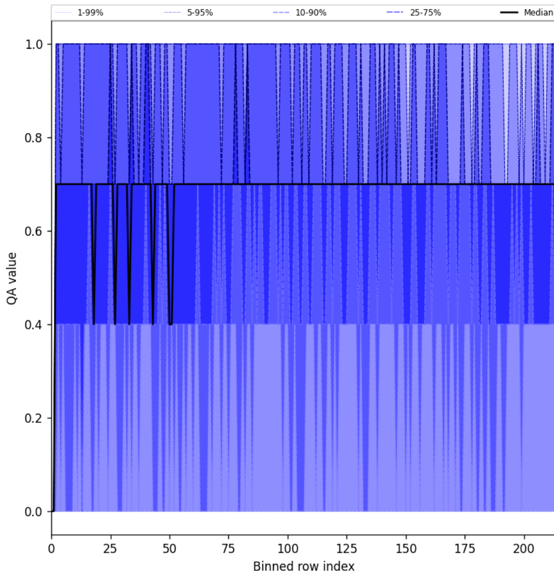
Figure 25: Along track statistics of “QA value” for 2024-10-19 to 2024-10-20
