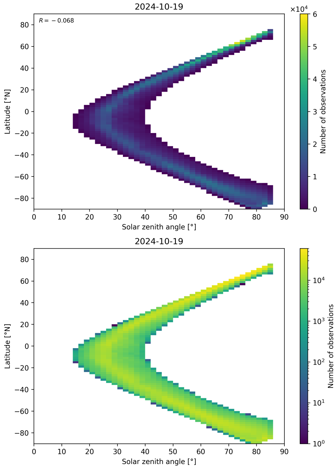
Figure 66: Scatter density plot of “Solar zenith angle” against “Latitude” for 2024-10-19 to 2024-10-20.
