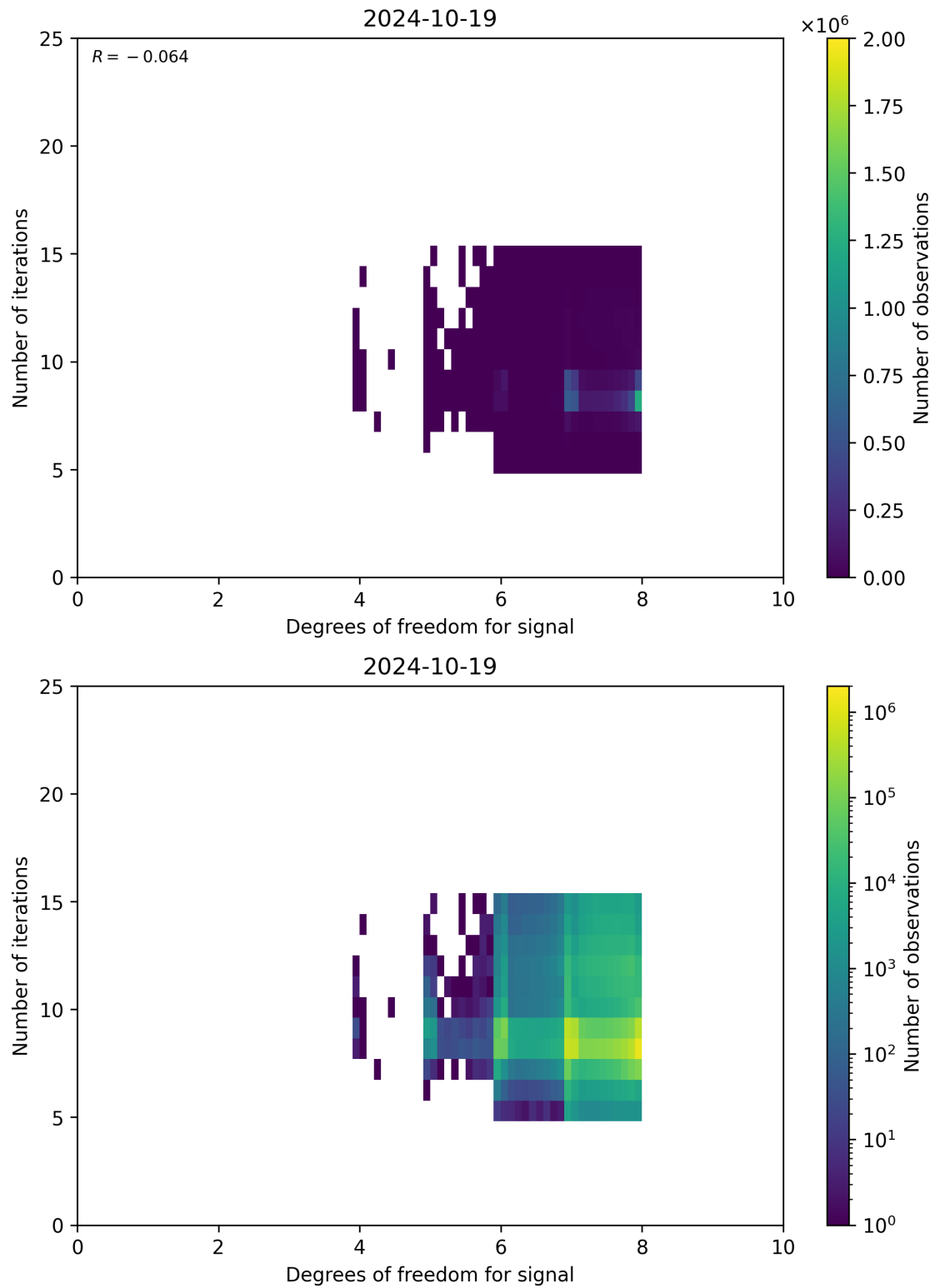
Figure 50: Scatter density plot of “Degrees of freedom for signal” against “Number of iterations” for 2024-10-19 to 2024-10-20.
