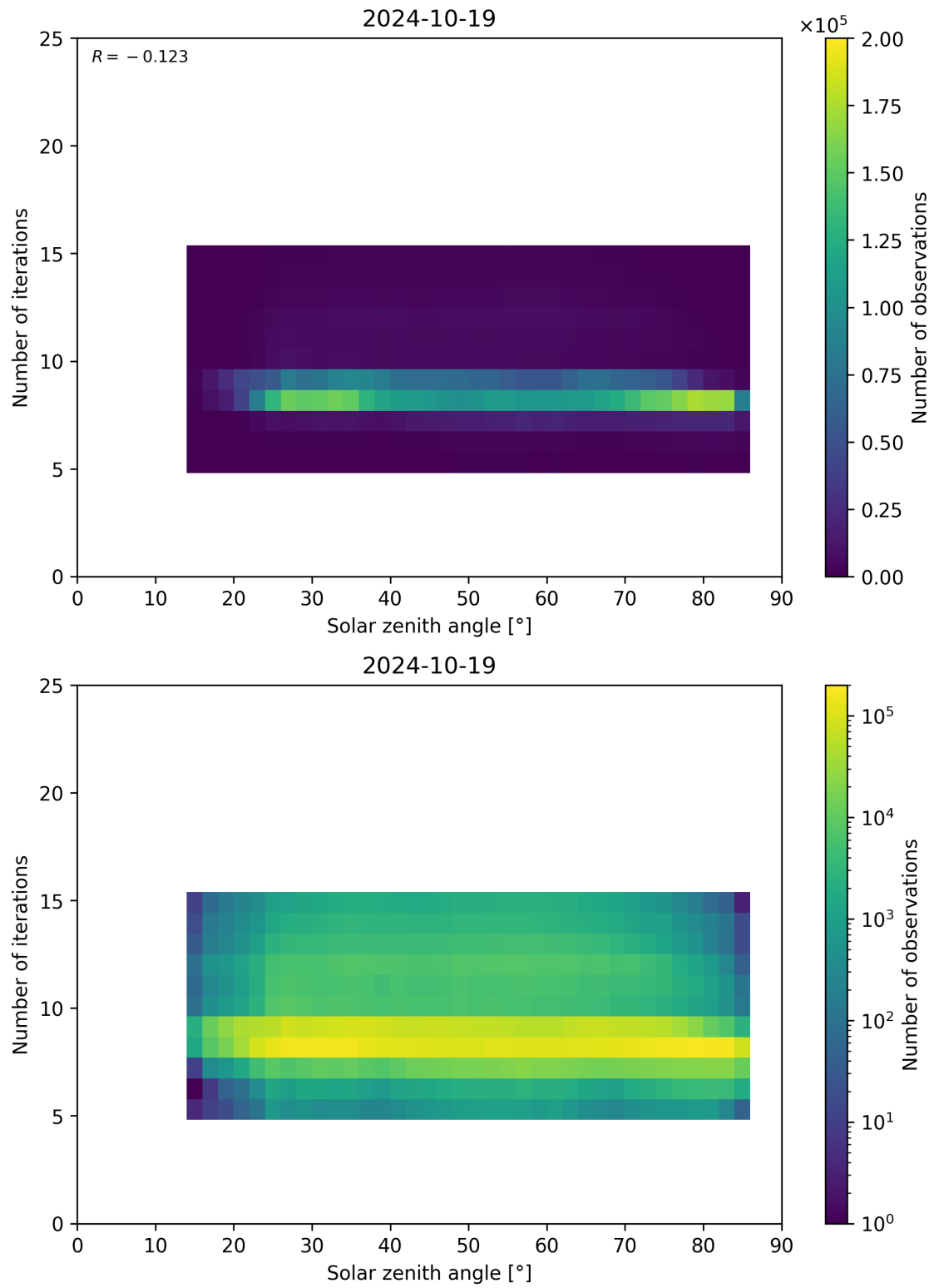
Figure 67: Scatter density plot of “Solar zenith angle” against “Number of iterations” for 2024-10-19 to 2024-10-20.
