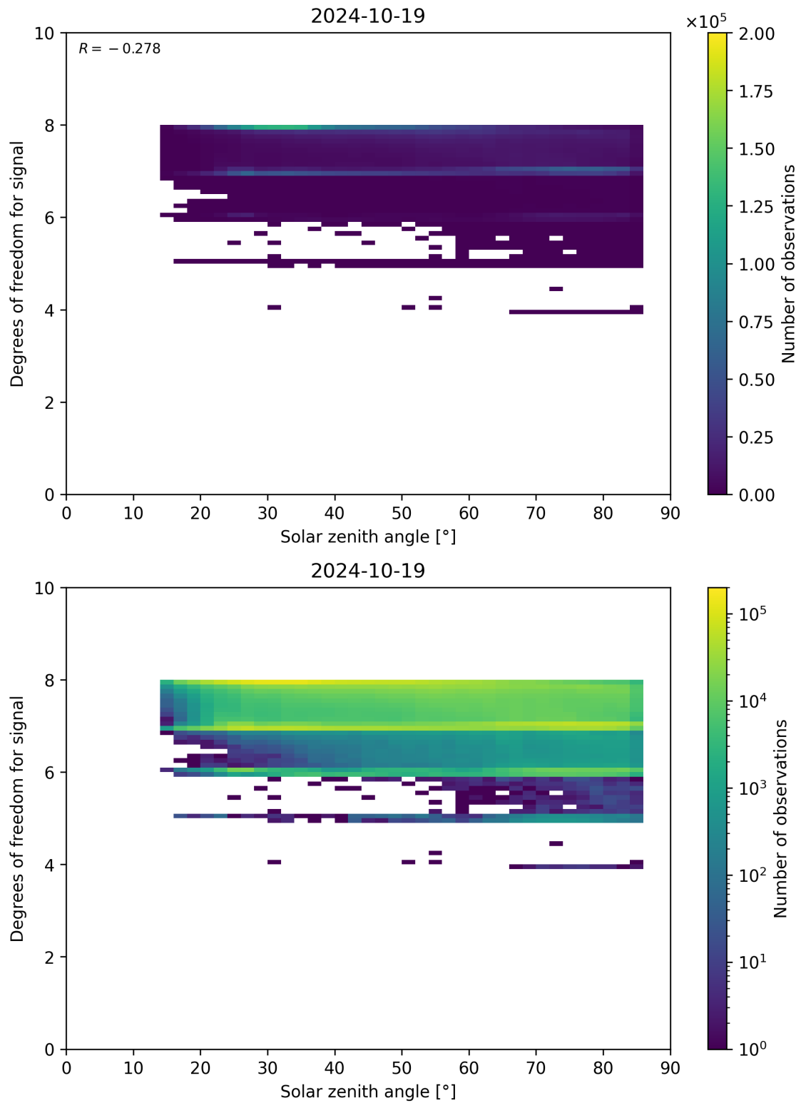
Figure 65: Scatter density plot of “Solar zenith angle” against “Degrees of freedom for signal” for 2024-10-19 to 2024-10-20.
