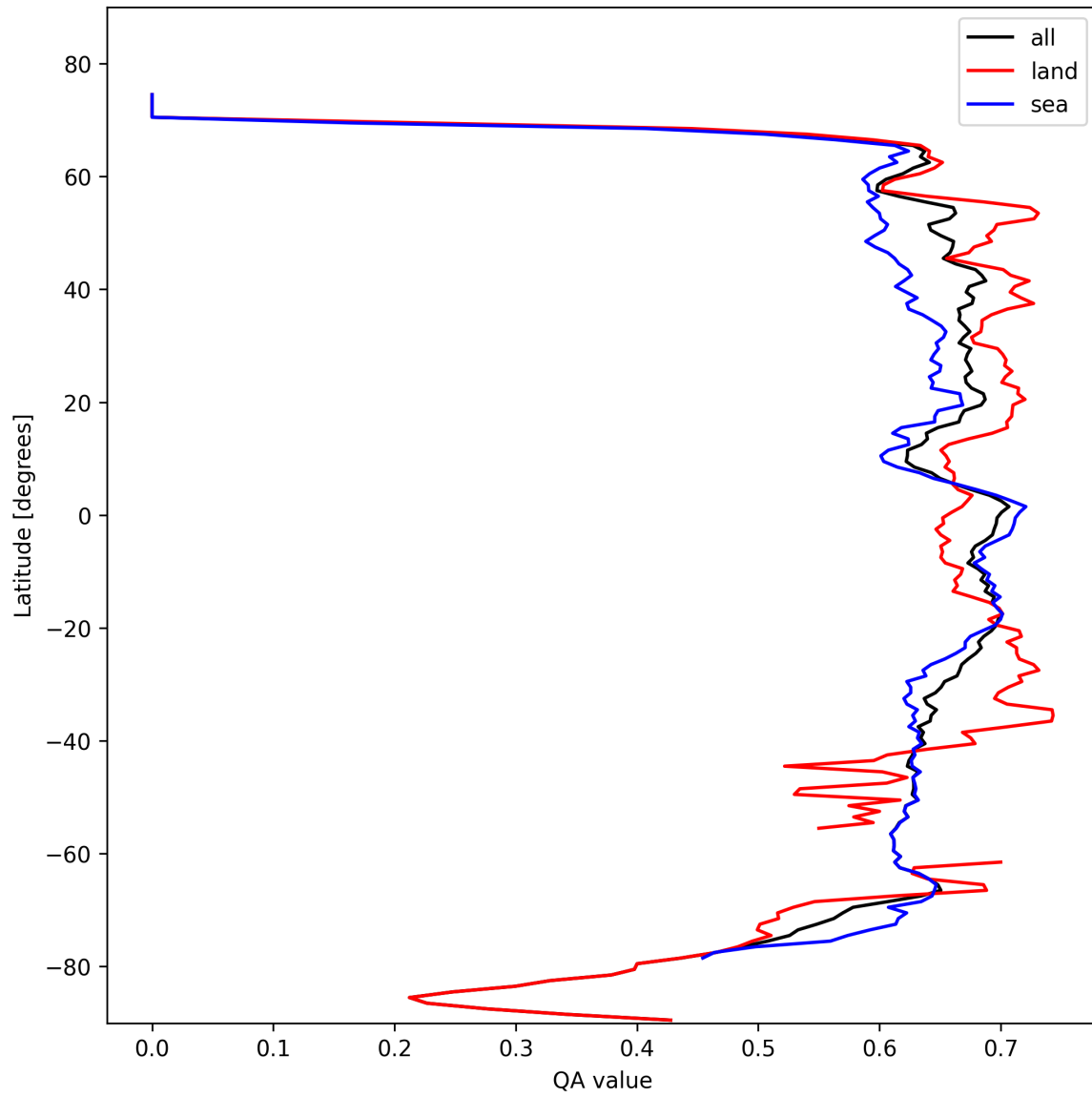
Figure 9: Zonal average of “QA value” for 2024-10-19 to 2024-10-20.
