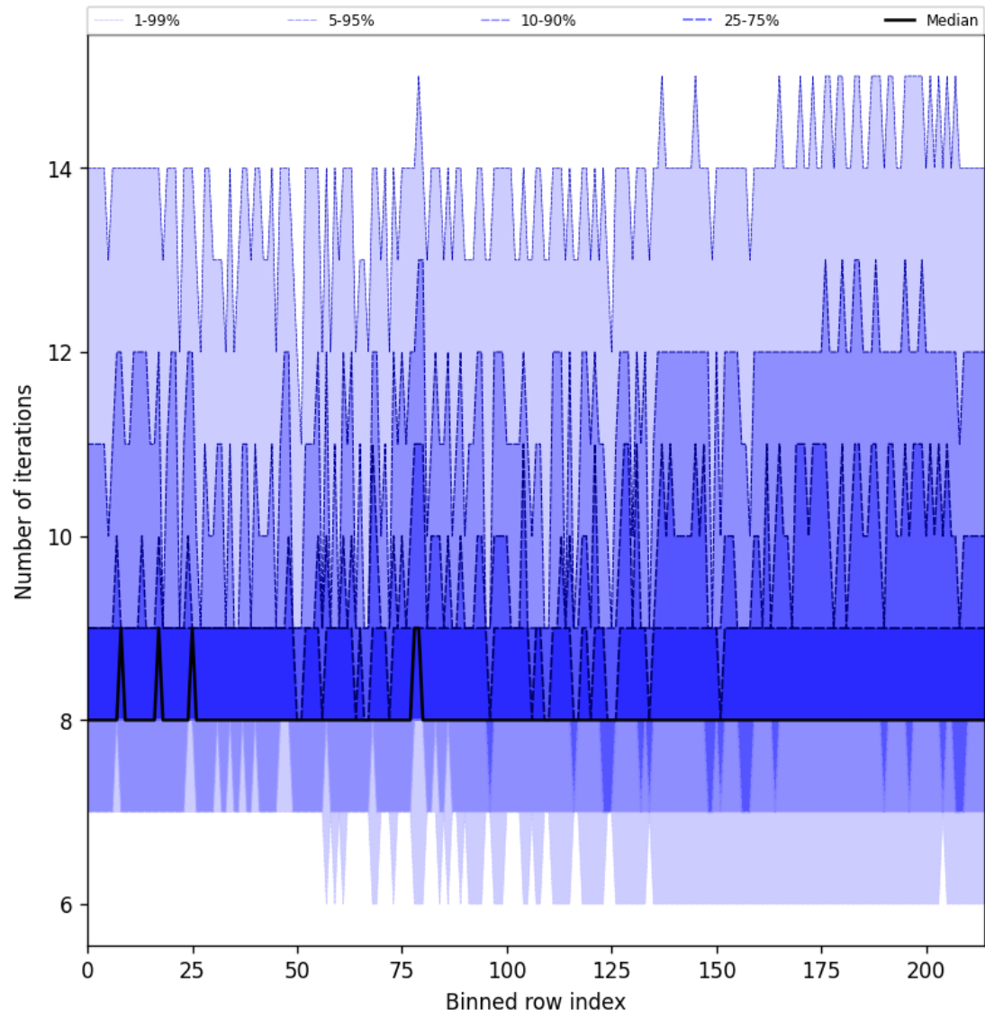
Figure 32: Along track statistics of “Number of iterations” for 2024-10-19 to 2024-10-20
