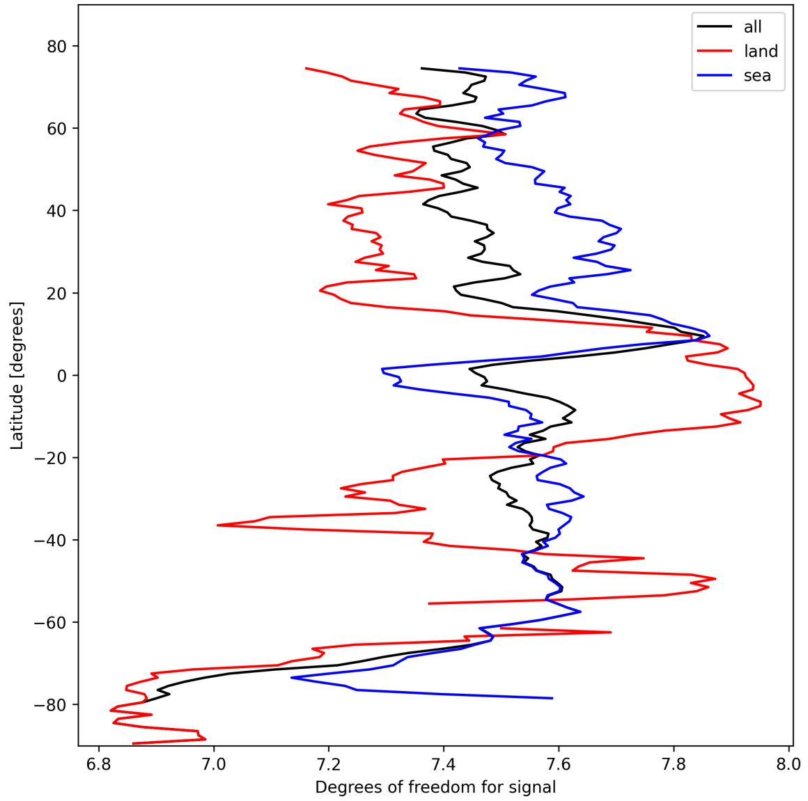
Figure 15: Zonal average of “Degrees of freedom for signal” for 2024-10-19 to 2024-10-20.
