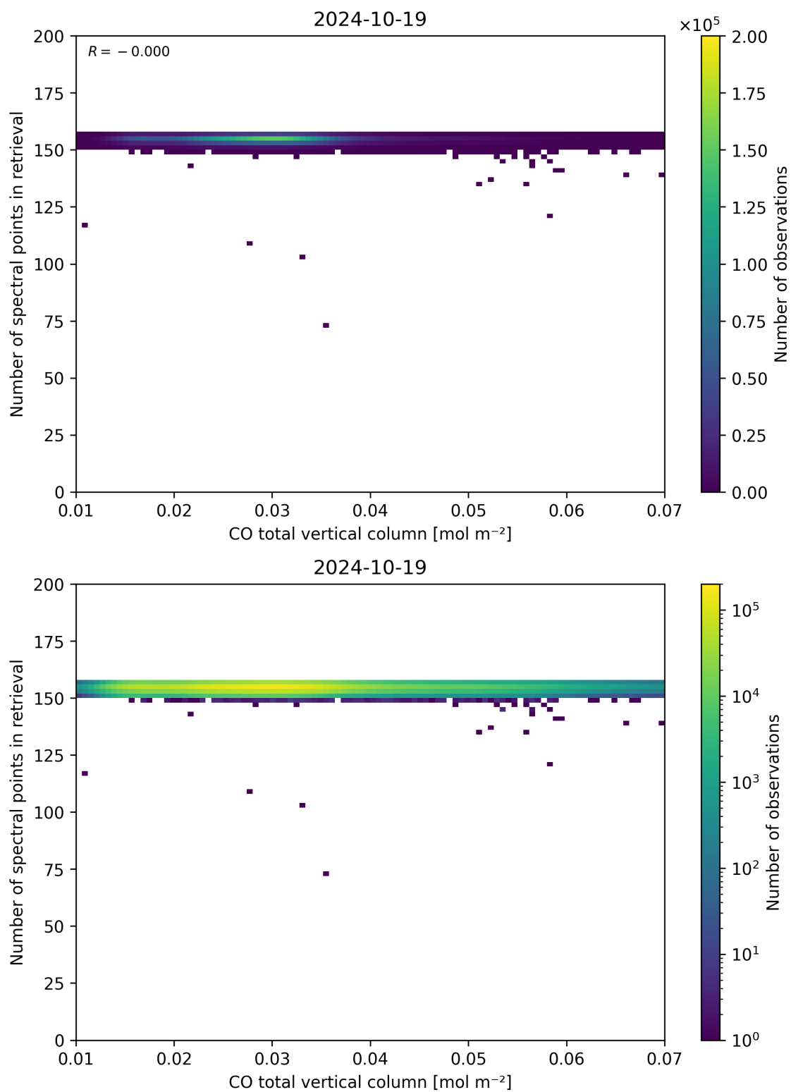
Figure 43: Scatter density plot of “CO total vertical column” against “Number of spectral points in retrieval” for 2024-10-19 to 2024-10-20.
