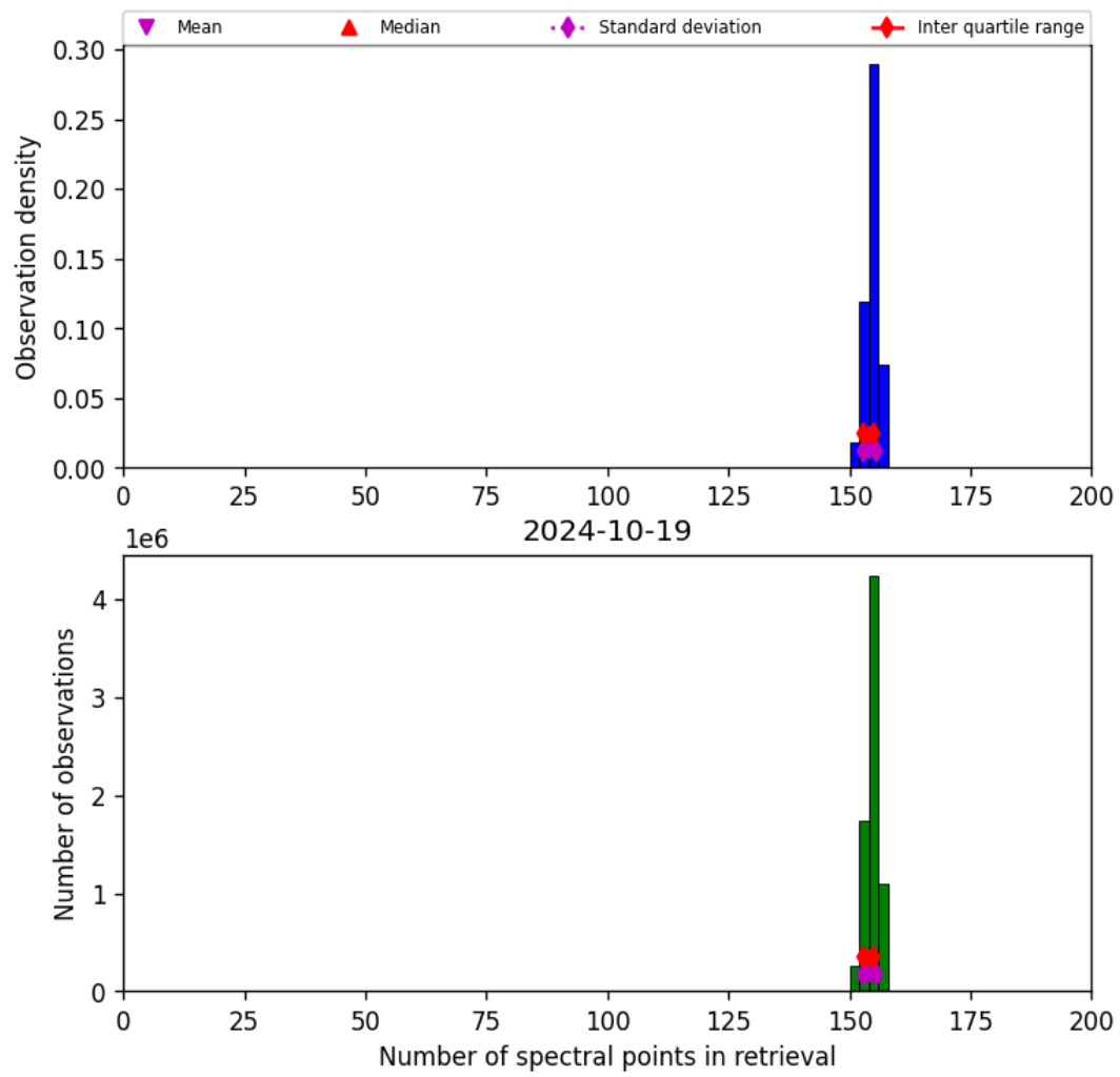
Figure 21: Histogram of “Number of spectral points in retrieval” for 2024-10-19 to 2024-10-20
