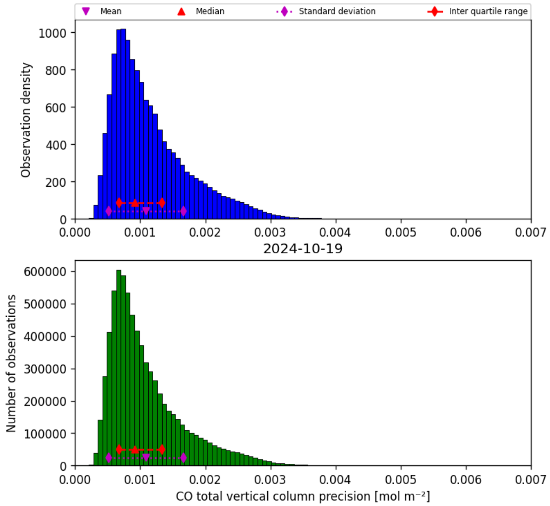
Figure 20: Histogram of “CO total vertical column precision” for 2024-10-19 to 2024-10-20
