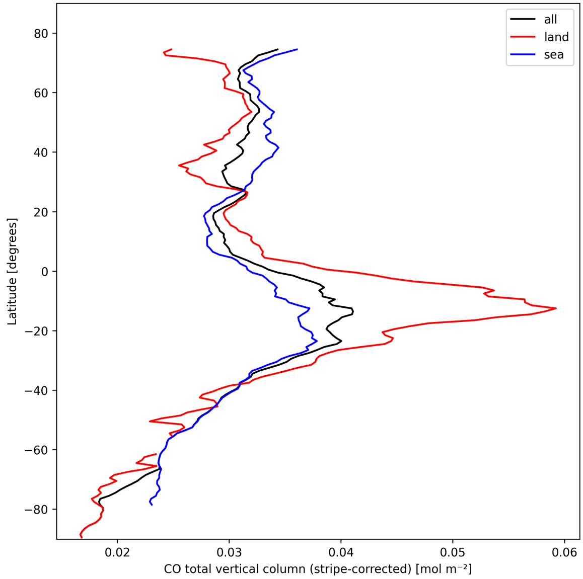
Figure 11: Zonal average of “CO total vertical column (stripe-corrected)” for 2024-10-19 to 2024-10-20.
