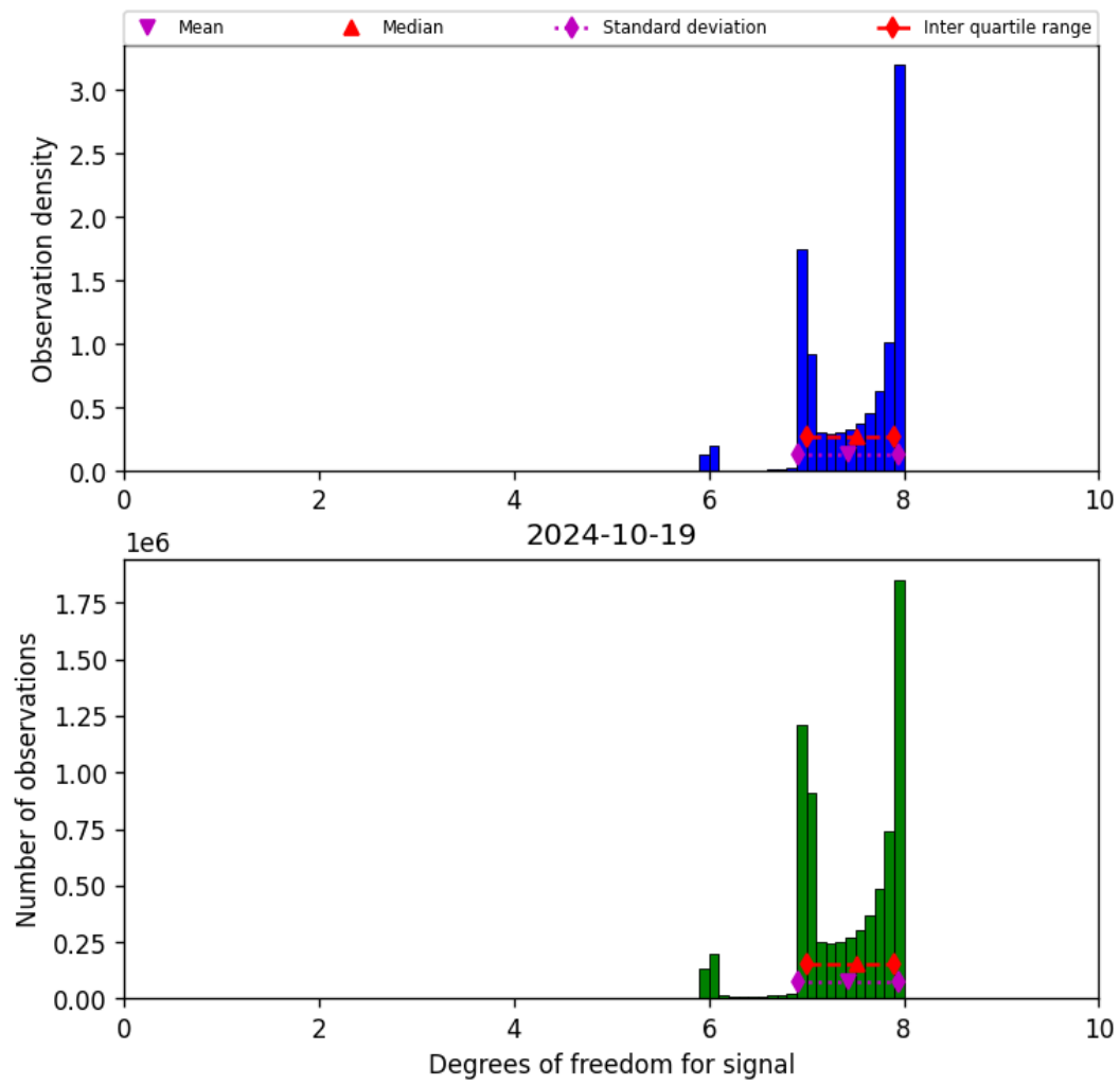
Figure 23: Histogram of “Degrees of freedom for signal” for 2024-10-19 to 2024-10-20
