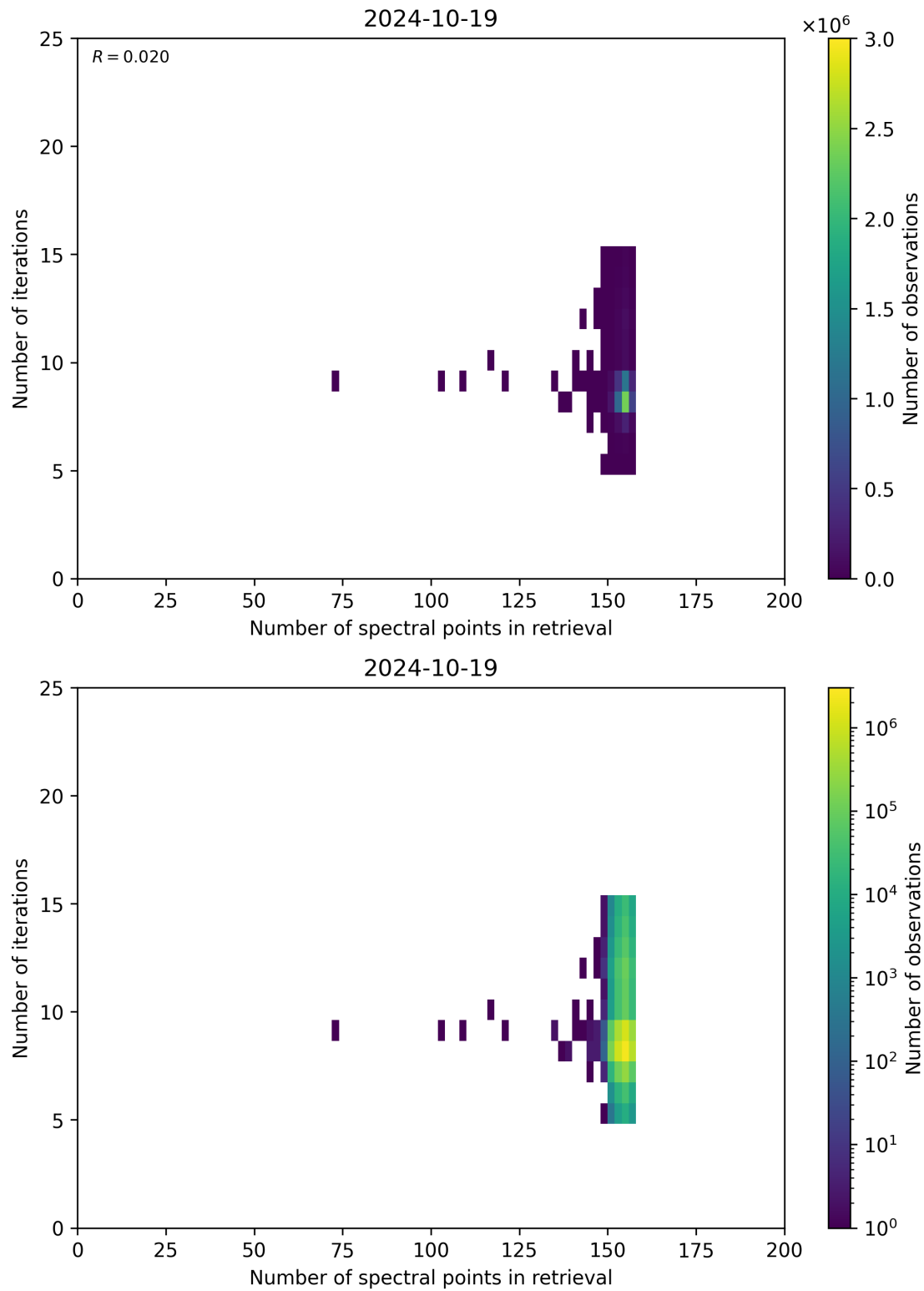
Figure 60: Scatter density plot of “Number of spectral points in retrieval” against “Number of iterations” for 2024-10-19 to 2024-10-20.
