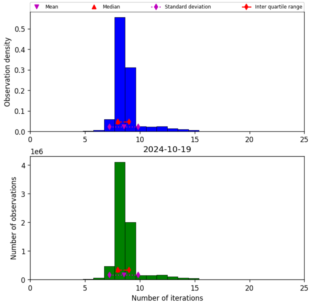
Figure 24: Histogram of “Number of iterations” for 2024-10-19 to 2024-10-20
