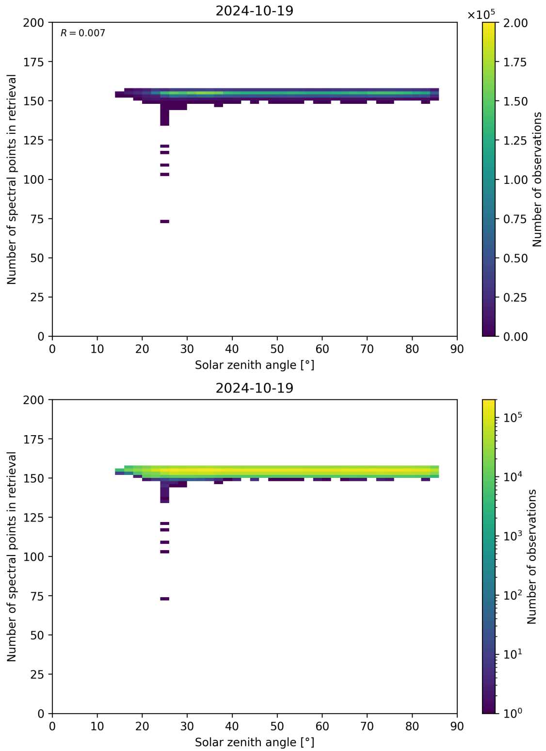
Figure 68: Scatter density plot of “Solar zenith angle” against “Number of spectral points in retrieval” for 2024-10-19 to 2024-10-20.
