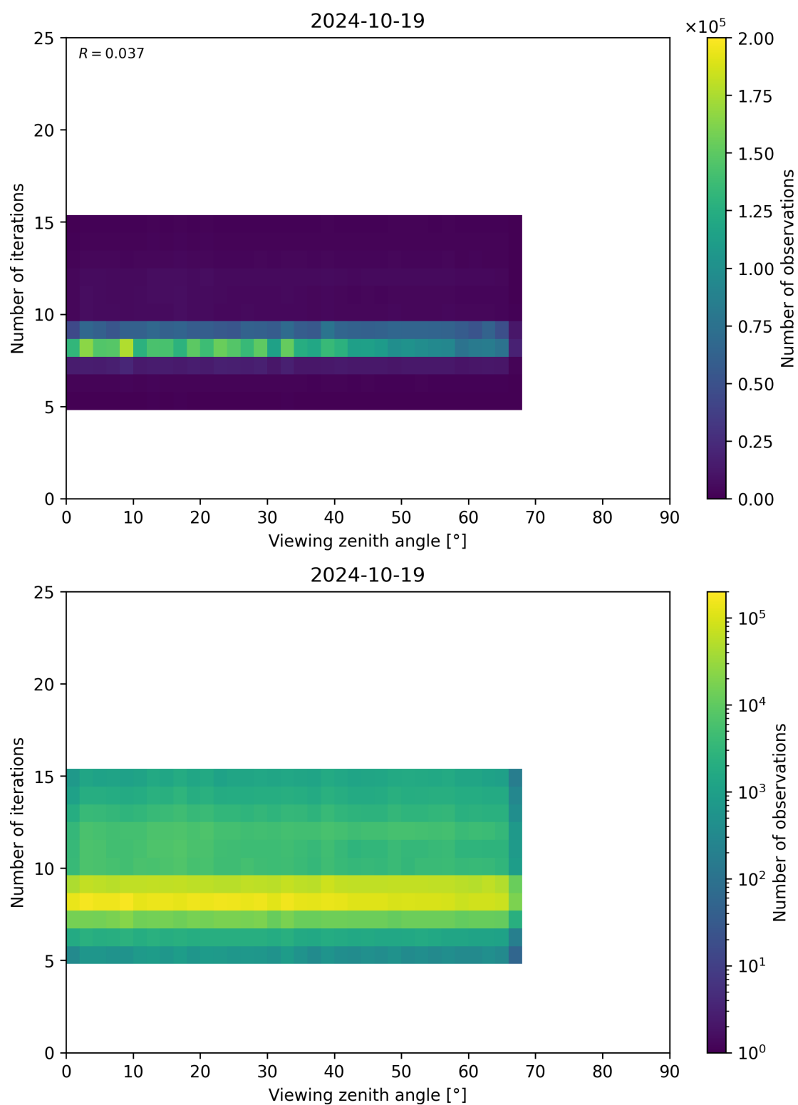
Figure 75: Scatter density plot of “Viewing zenith angle” against “Number of iterations” for 2024-10-19 to 2024-10-20.
