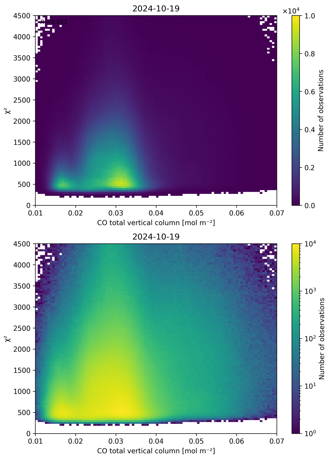
Figure 35: Scatter density plot of “CO total vertical column” against “ \chi^2 ” for 2024-10-19 to 2024-10-20.
