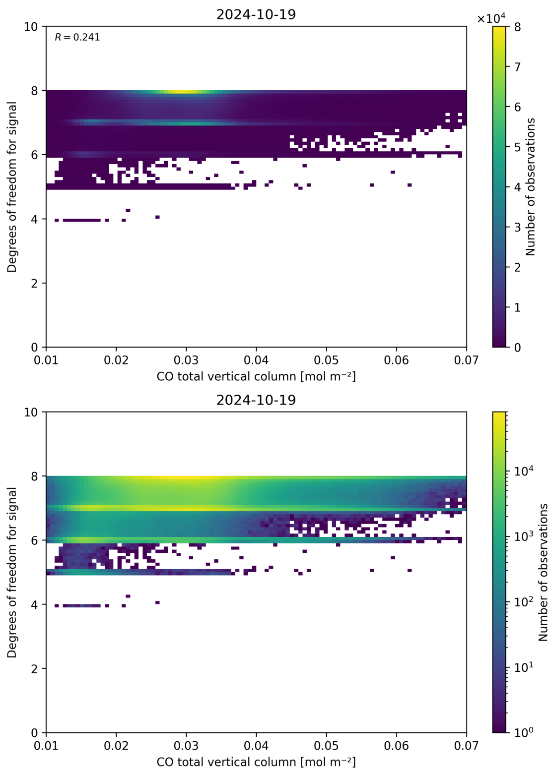
Figure 41: Scatter density plot of “CO total vertical column” against “Degrees of freedom for signal” for 2024-10-19 to 2024-10-20.
