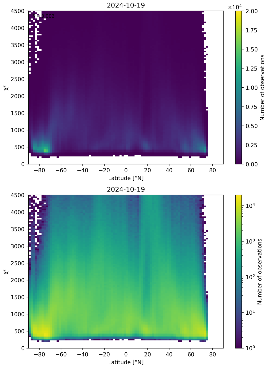
Figure 54: Scatter density plot of “Latitude” against “ \chi^2 ” for 2024-10-19 to 2024-10-20.
