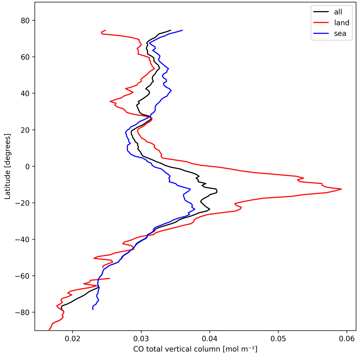
Figure 10: Zonal average of “CO total vertical column” for 2024-10-19 to 2024-10-20.
