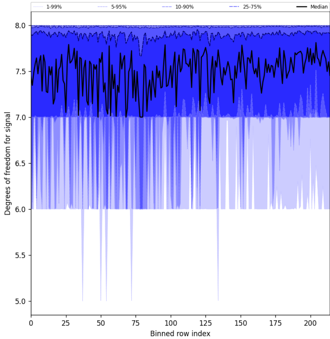
Figure 31: Along track statistics of “Degrees of freedom for signal” for 2024-10-19 to 2024-10-20
