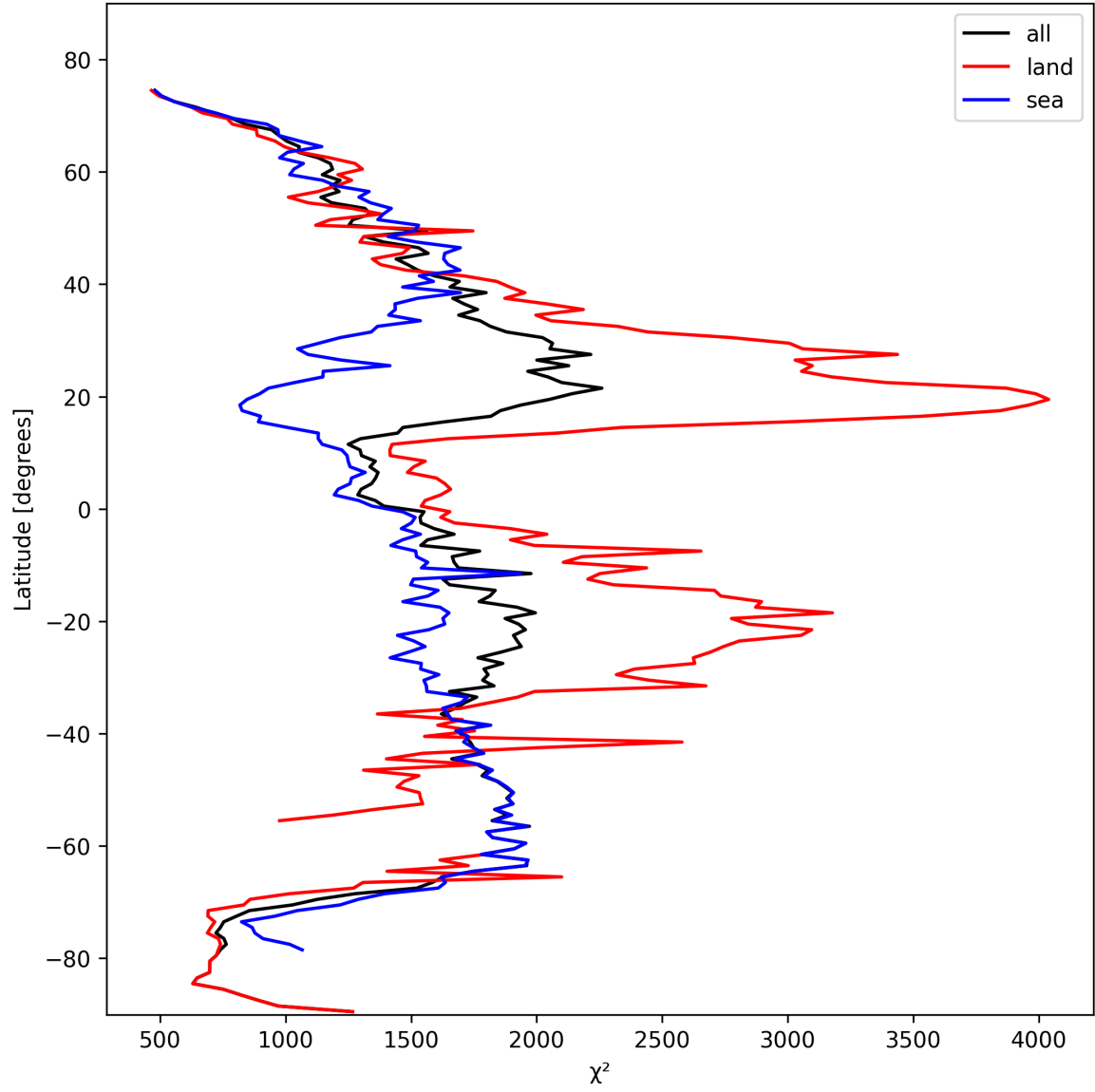
Figure 14: Zonal average of “ \chi^2 ” for 2024-10-19 to 2024-10-20.
