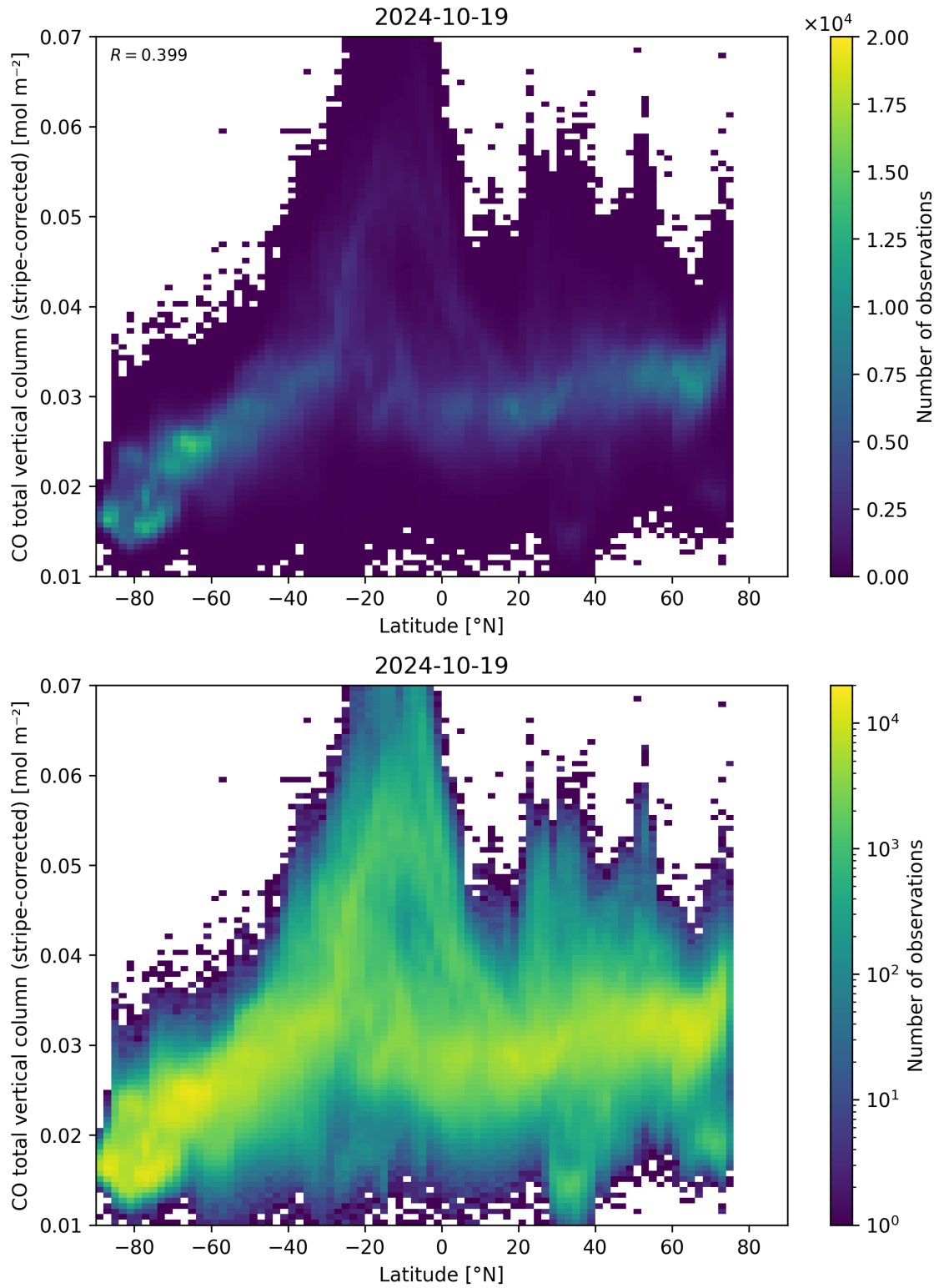
Figure 52: Scatter density plot of “Latitude” against “CO total vertical column (stripe-corrected)” for 2024-10-19 to 2024-10-20.
