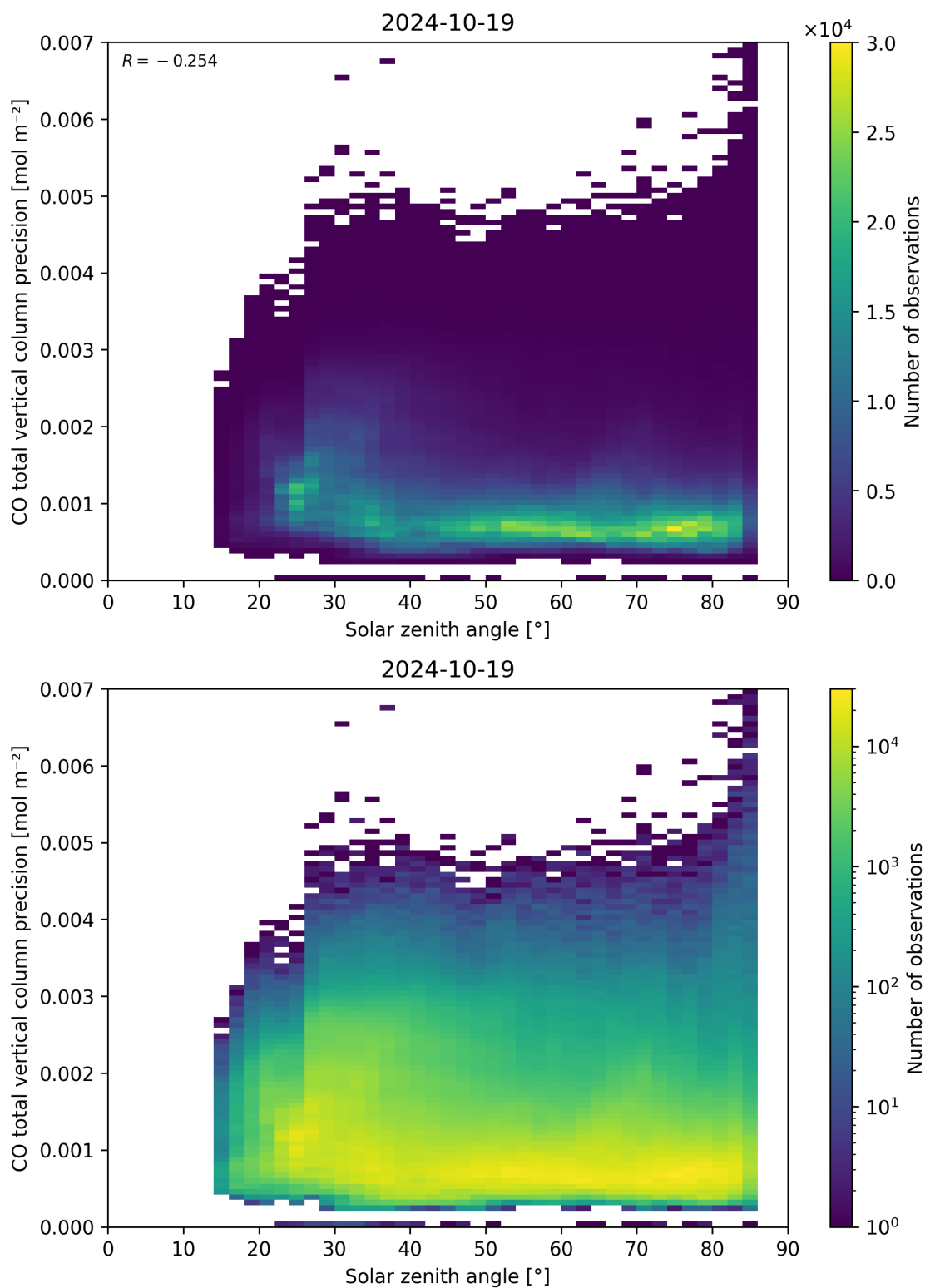
Figure 63: Scatter density plot of “Solar zenith angle” against “CO total vertical column precision” for 2024-10-19 to 2024-10-20.
