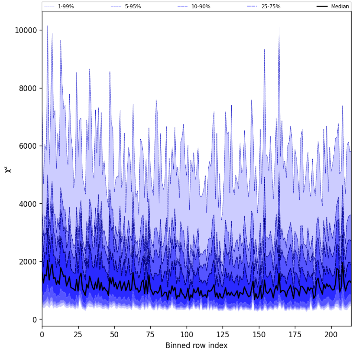
Figure 30: Along track statistics of “ \chi^2 ” for 2024-10-19 to 2024-10-20
