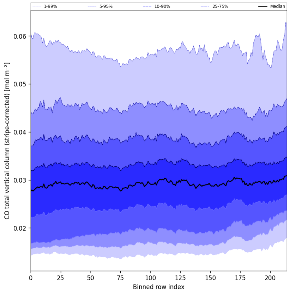
Figure 27: Along track statistics of “CO total vertical column (stripe-corrected)” for 2024-10-19 to 2024-10-20
