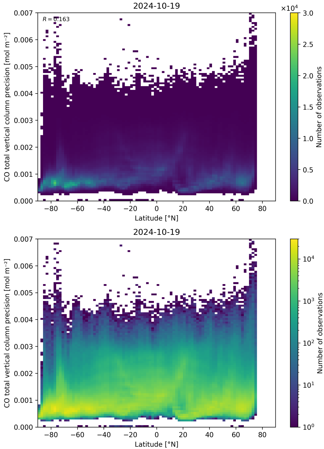
Figure 53: Scatter density plot of “Latitude” against “CO total vertical column precision” for 2024-10-19 to 2024-10-20.
