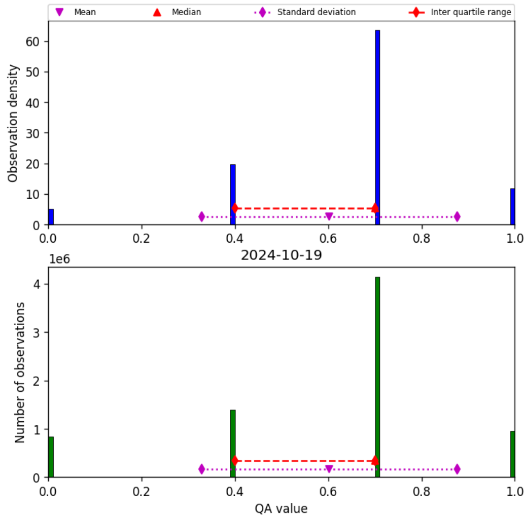
Figure 17: Histogram of “QA value” for 2024-10-19 to 2024-10-20
