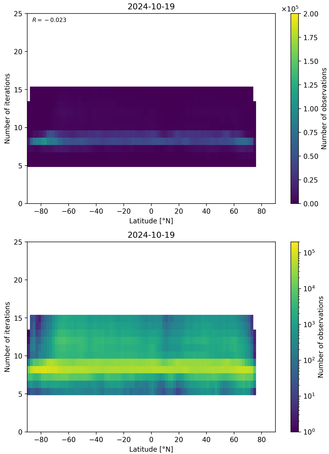
Figure 56: Scatter density plot of “Latitude” against “Number of iterations” for 2024-10-19 to 2024-10-20.
