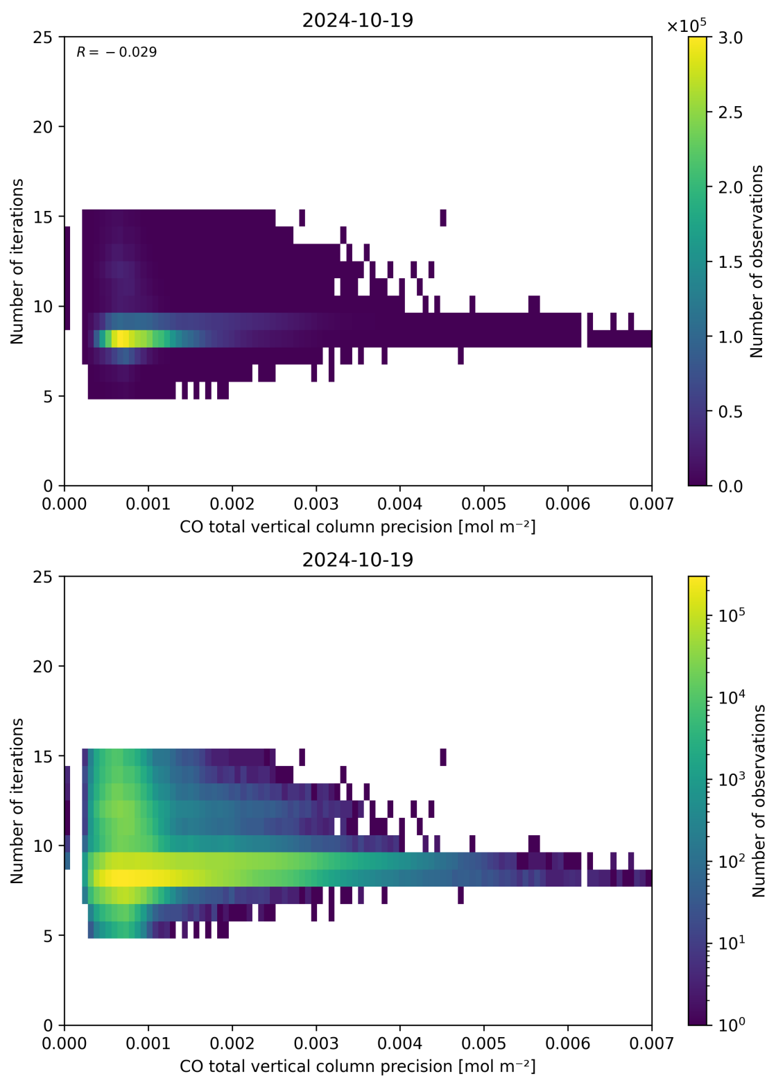
Figure 46: Scatter density plot of “CO total vertical column precision” against “Number of iterations” for 2024-10-19 to 2024-10-20.
