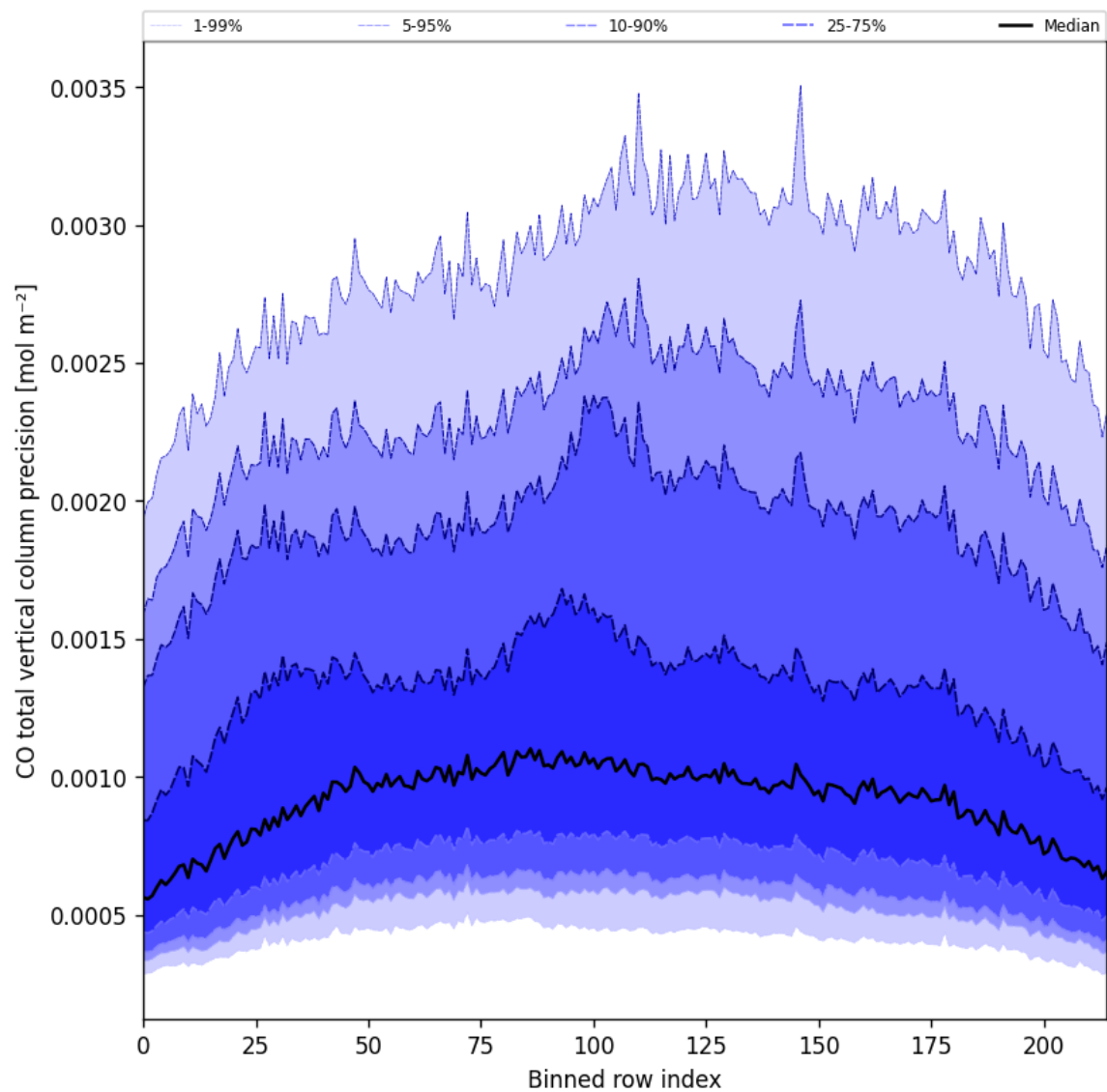
Figure 28: Along track statistics of “CO total vertical column precision” for 2024-10-19 to 2024-10-20
