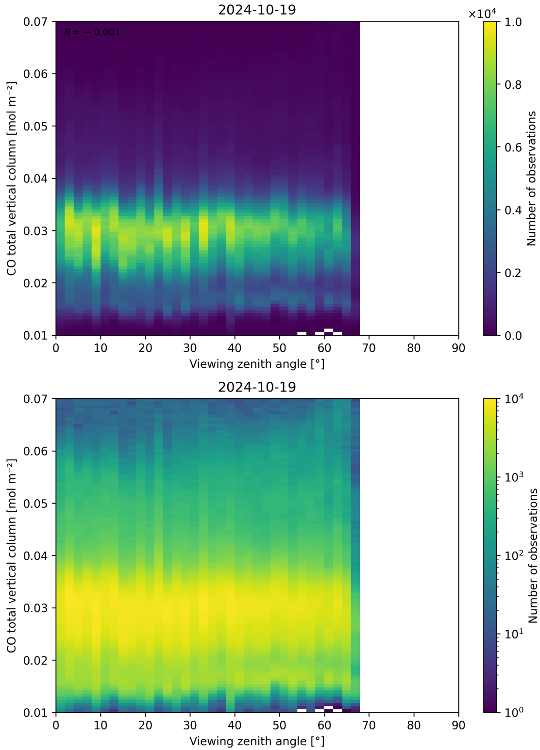
Figure 69: Scatter density plot of “Viewing zenith angle” against “CO total vertical column” for 2024-10-19 to 2024-10-20.
