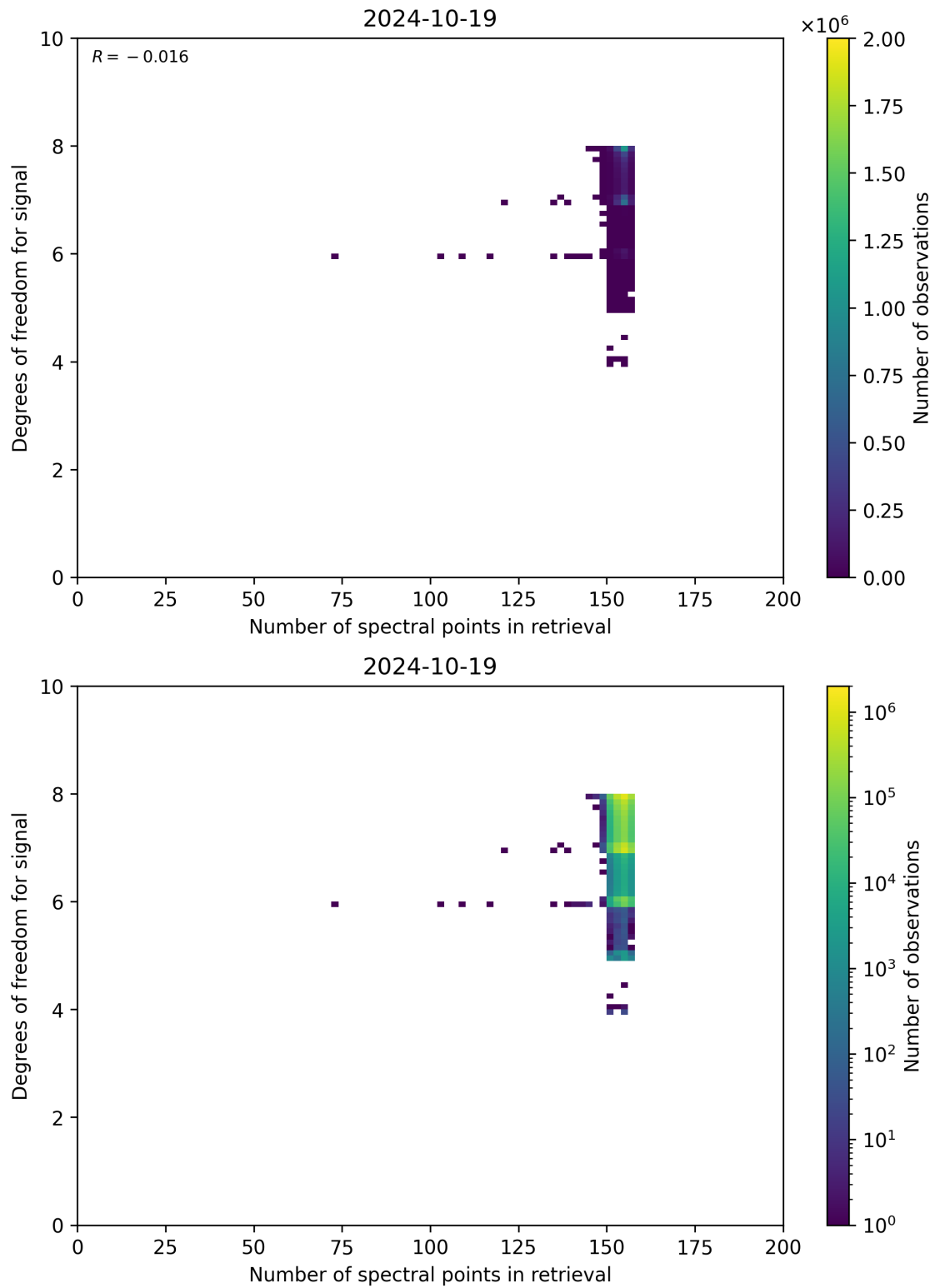
Figure 59: Scatter density plot of “Number of spectral points in retrieval” against “Degrees of freedom for signal” for 2024-10-19 to 2024-10-20.
