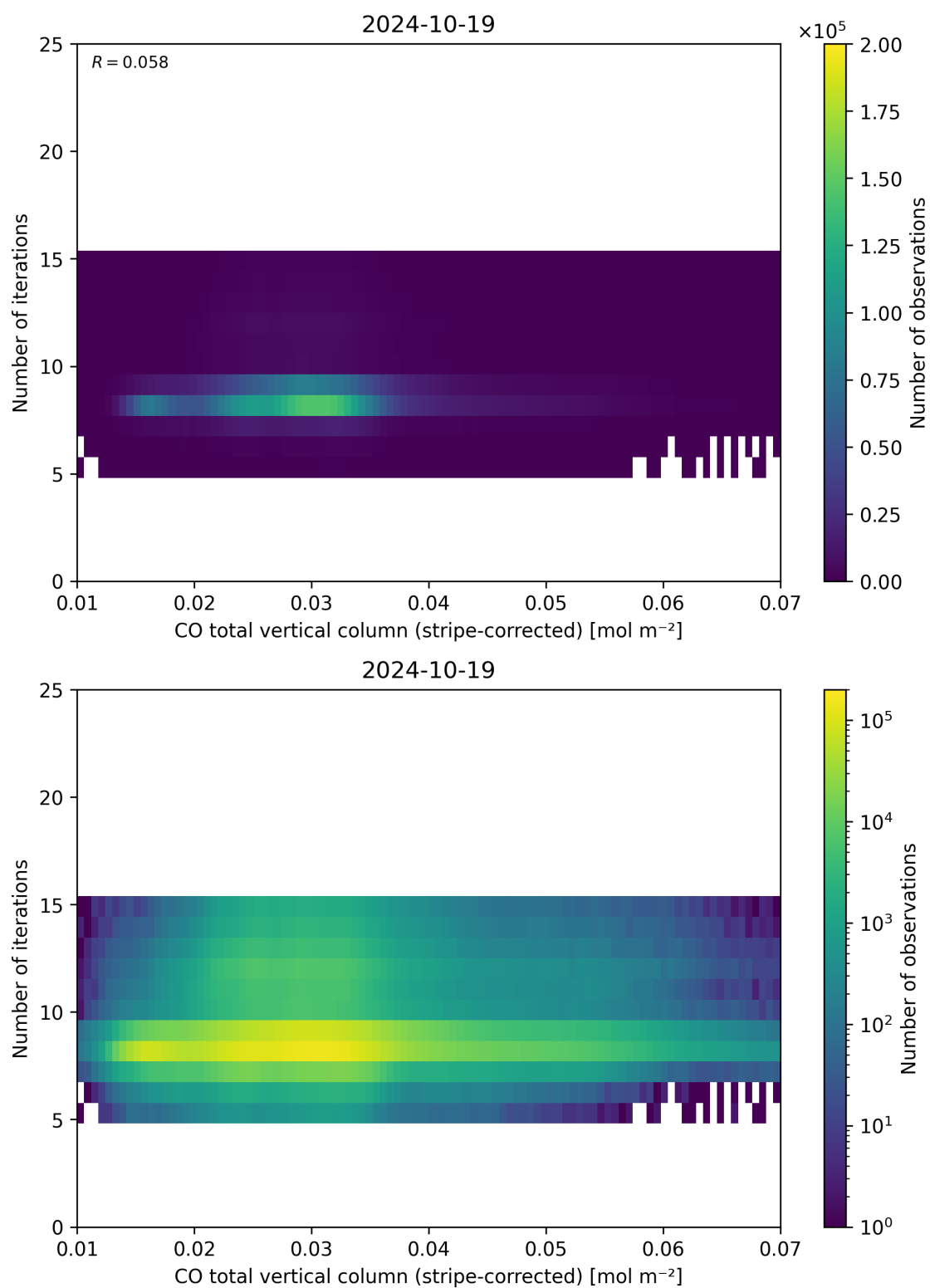
Figure 39: Scatter density plot of “CO total vertical column (stripe-corrected)” against “Number of iterations” for 2024-10-19 to 2024-10-20.
