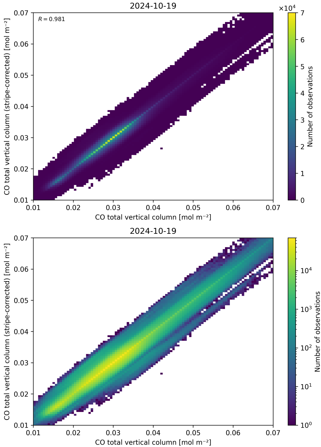
Figure 33: Scatter density plot of “CO total vertical column” against “CO total vertical column (stripe-corrected)” for 2024-10-19 to 2024-10-20.
