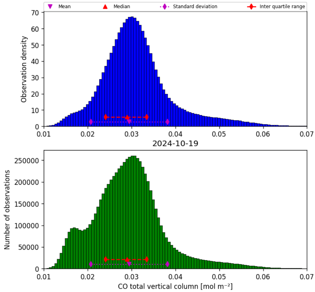
Figure 18: Histogram of “CO total vertical column” for 2024-10-19 to 2024-10-20
