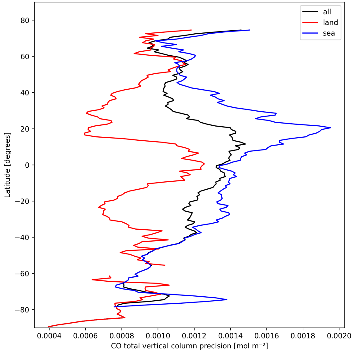
Figure 12: Zonal average of “CO total vertical column precision” for 2024-10-19 to 2024-10-20.
