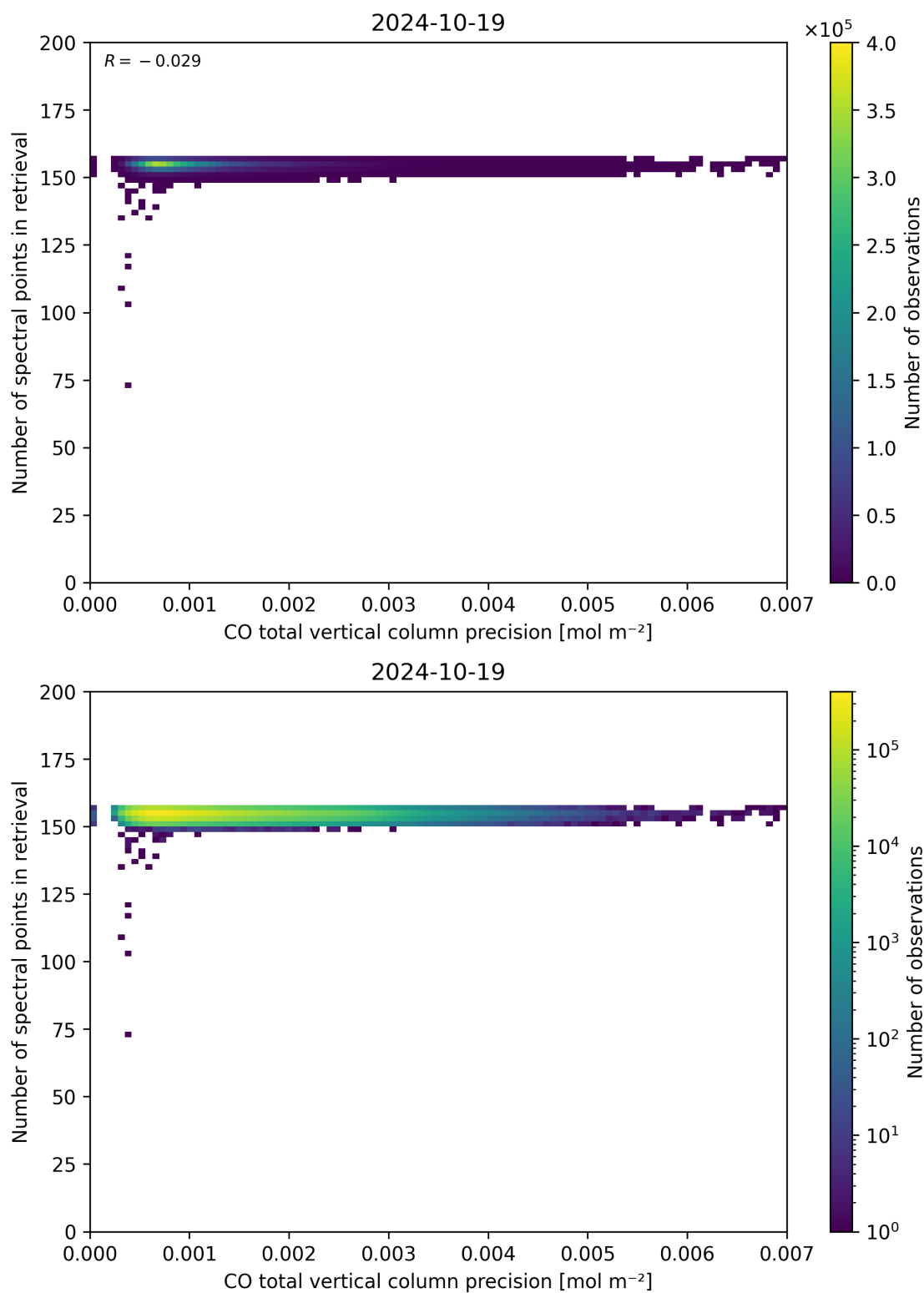
Figure 47: Scatter density plot of “CO total vertical column precision” against “Number of spectral points in retrieval” for 2024-10-19 to 2024-10-20.
