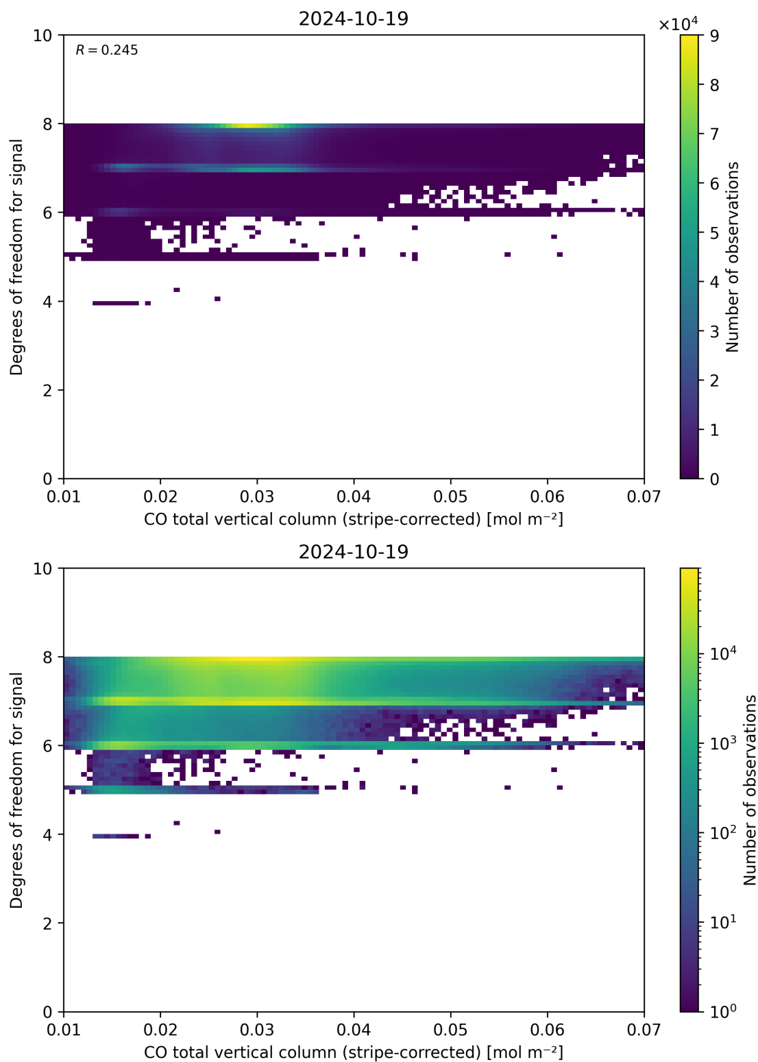
Figure 38: Scatter density plot of “CO total vertical column (stripe-corrected)” against “Degrees of freedom for signal” for 2024-10-19 to 2024-10-20.
