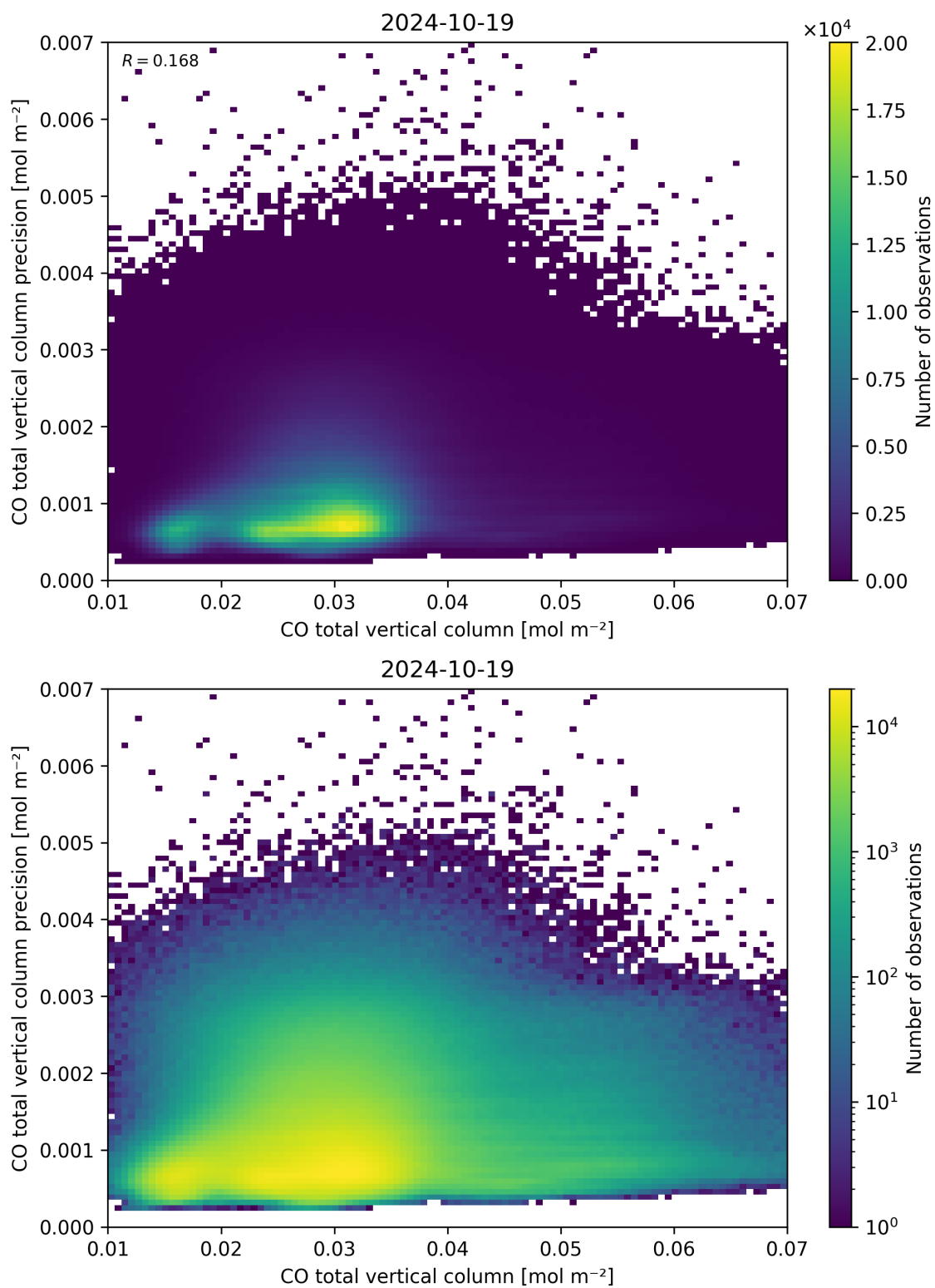
Figure 34: Scatter density plot of “CO total vertical column” against “CO total vertical column precision” for 2024-10-19 to 2024-10-20.
