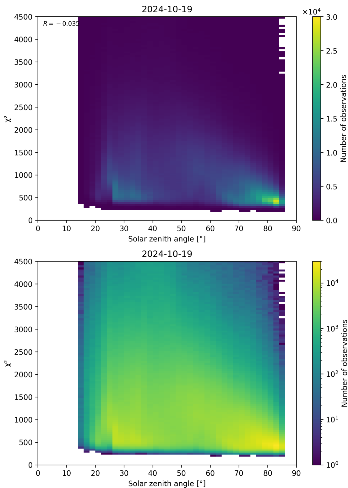
Figure 64: Scatter density plot of “Solar zenith angle” against “ \chi^2 ” for 2024-10-19 to 2024-10-20.
