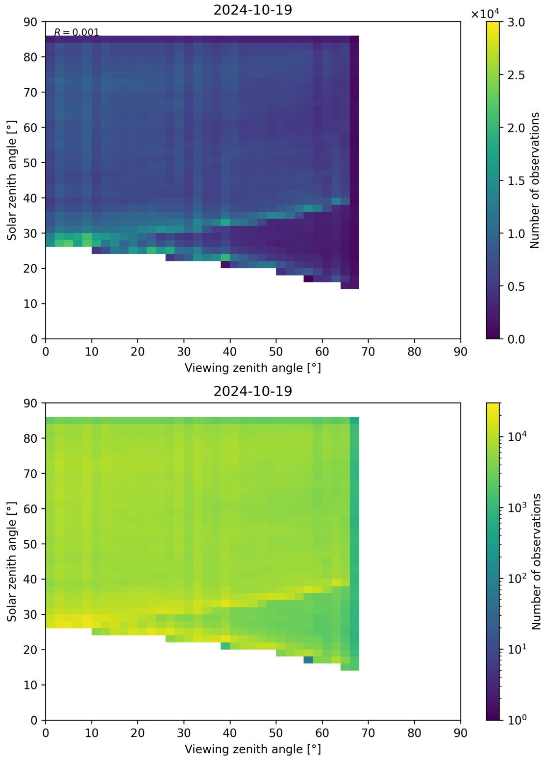
Figure 77: Scatter density plot of “Viewing zenith angle” against “Solar zenith angle” for 2024-10-19 to 2024-10-20.
