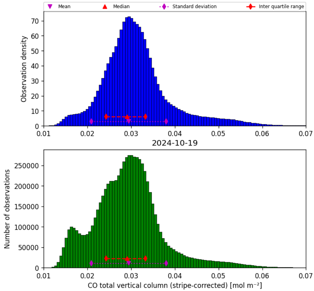
Figure 19: Histogram of “CO total vertical column (stripe-corrected)” for 2024-10-19 to 2024-10-20
