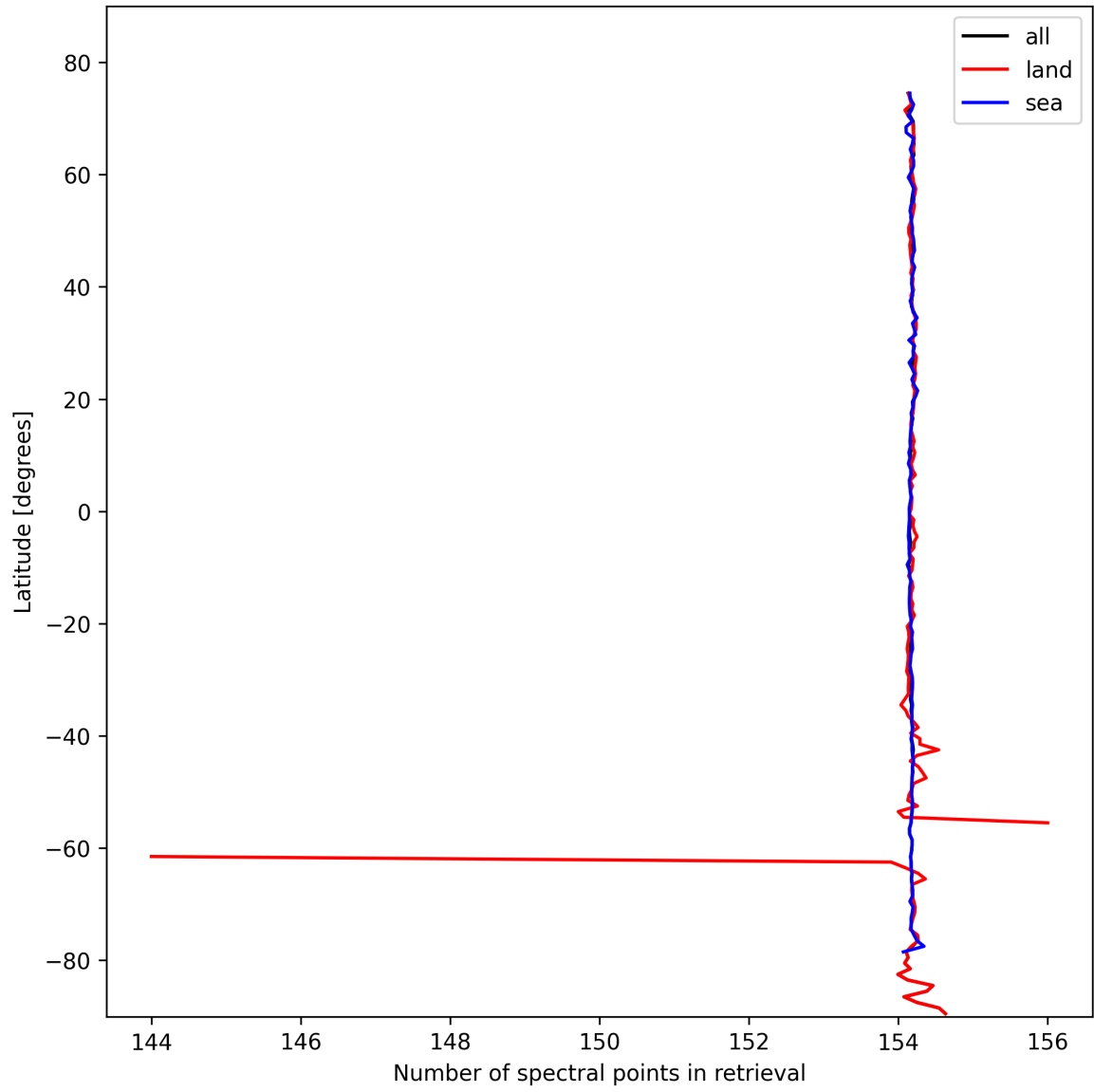
Figure 13: Zonal average of “Number of spectral points in retrieval” for 2024-10-19 to 2024-10-20.
