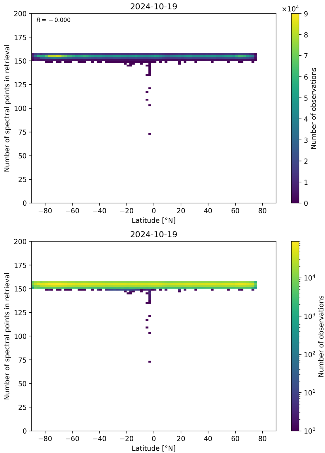
Figure 57: Scatter density plot of “Latitude” against “Number of spectral points in retrieval” for 2024-10-19 to 2024-10-20.
