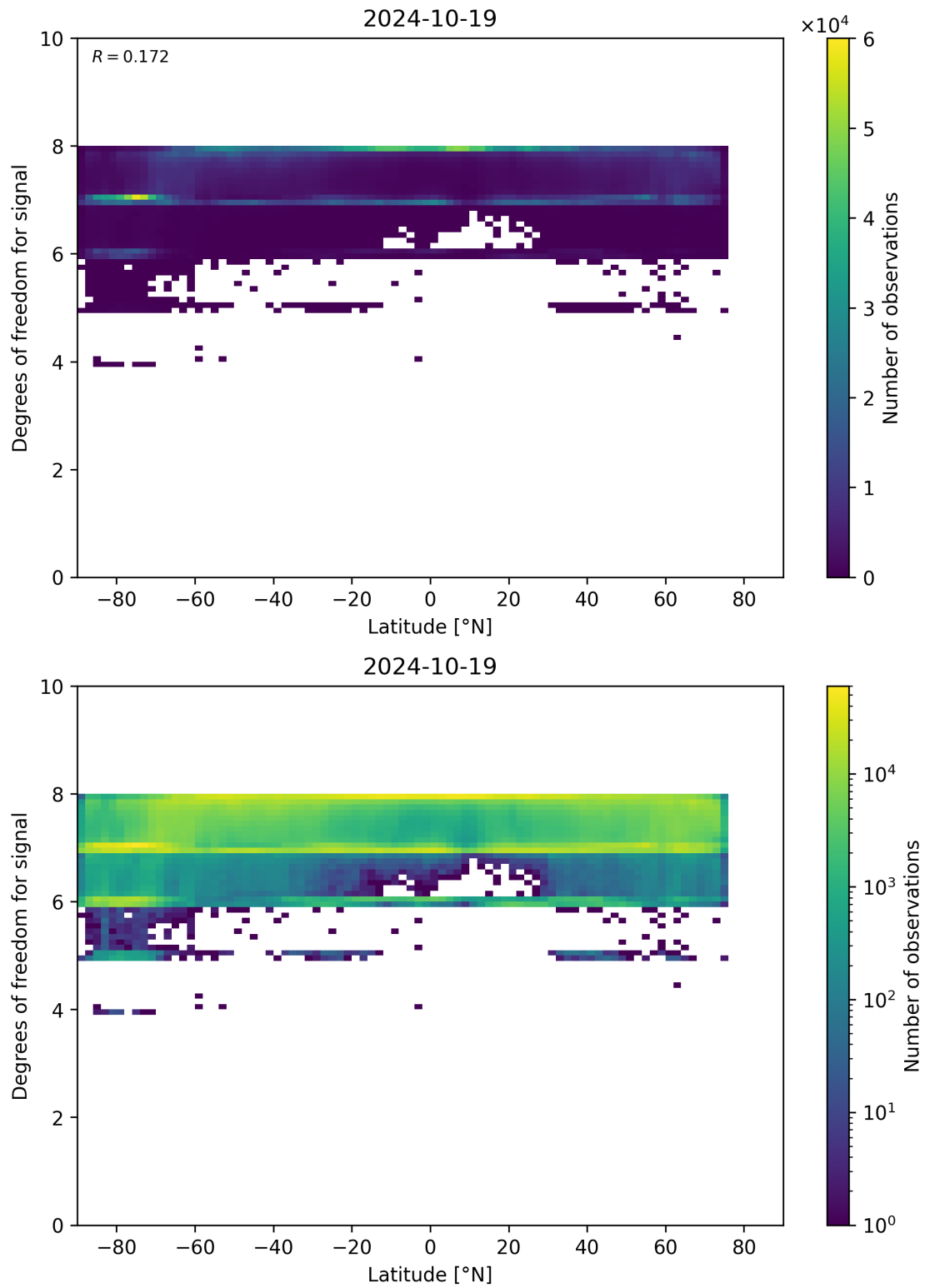
Figure 55: Scatter density plot of “Latitude” against “Degrees of freedom for signal” for 2024-10-19 to 2024-10-20.
