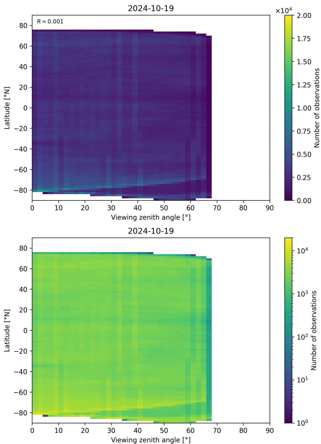
Figure 74: Scatter density plot of “Viewing zenith angle” against “Latitude” for 2024-10-19 to 2024-10-20.
