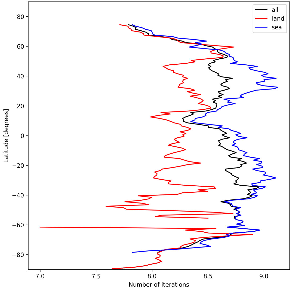
Figure 16: Zonal average of “Number of iterations” for 2024-10-19 to 2024-10-20.
