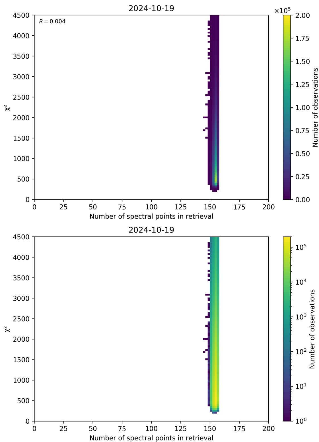
Figure 58: Scatter density plot of “Number of spectral points in retrieval” against “ \chi^2 ” for 2024-10-19 to 2024-10-20.
