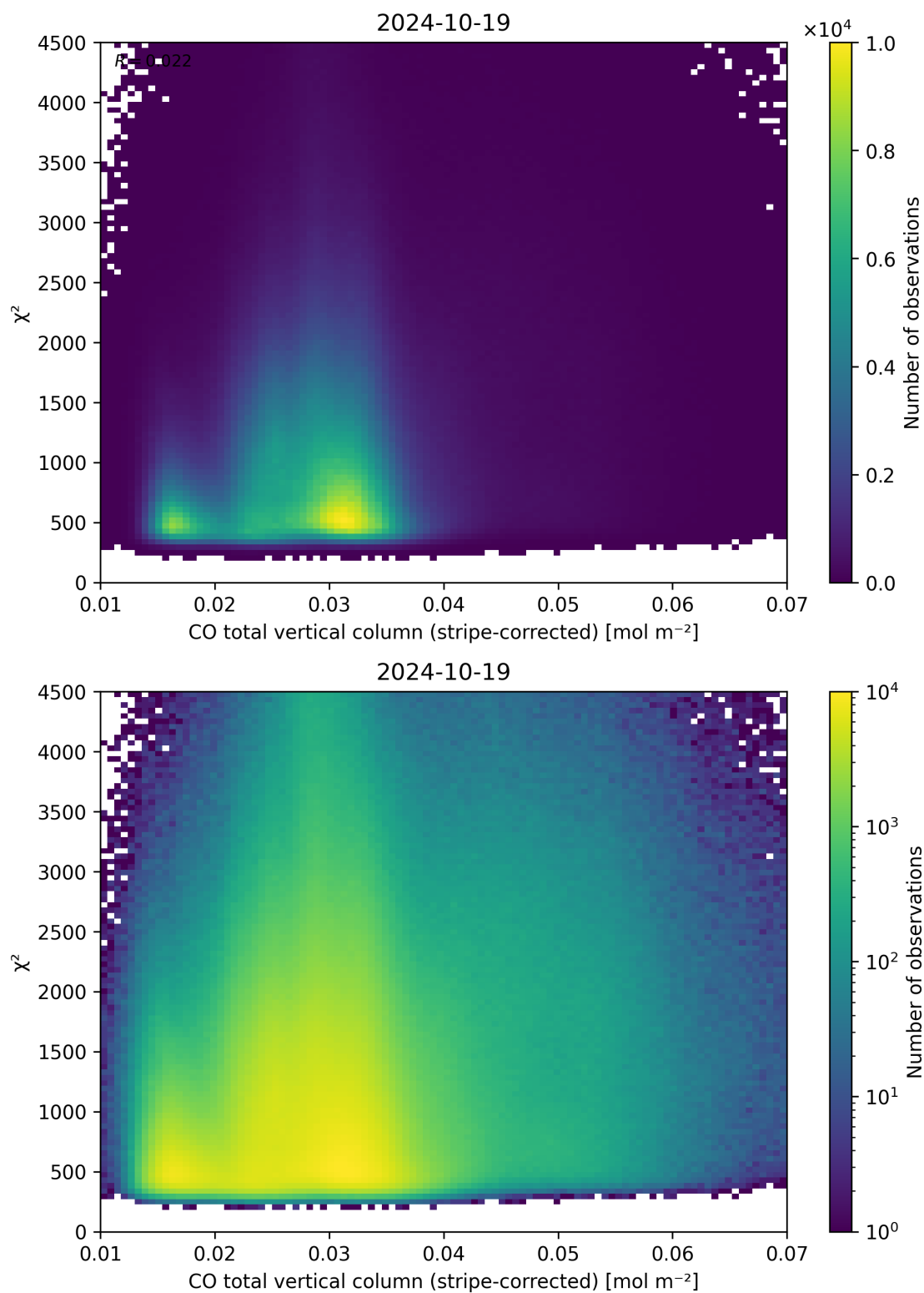
Figure 37: Scatter density plot of “CO total vertical column (stripe-corrected)” against “ \chi^2 ” for 2024-10-19 to 2024-10-20.
