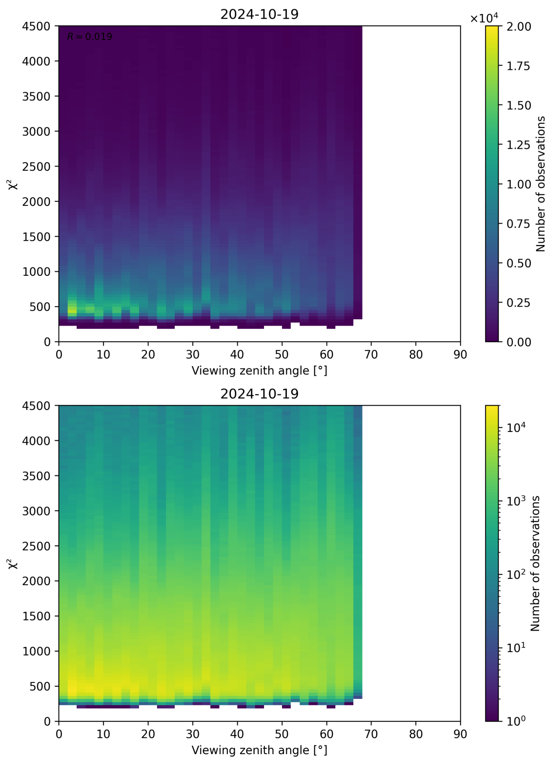
Figure 72: Scatter density plot of “Viewing zenith angle” against “ \chi^2 ” for 2024-10-19 to 2024-10-20.
