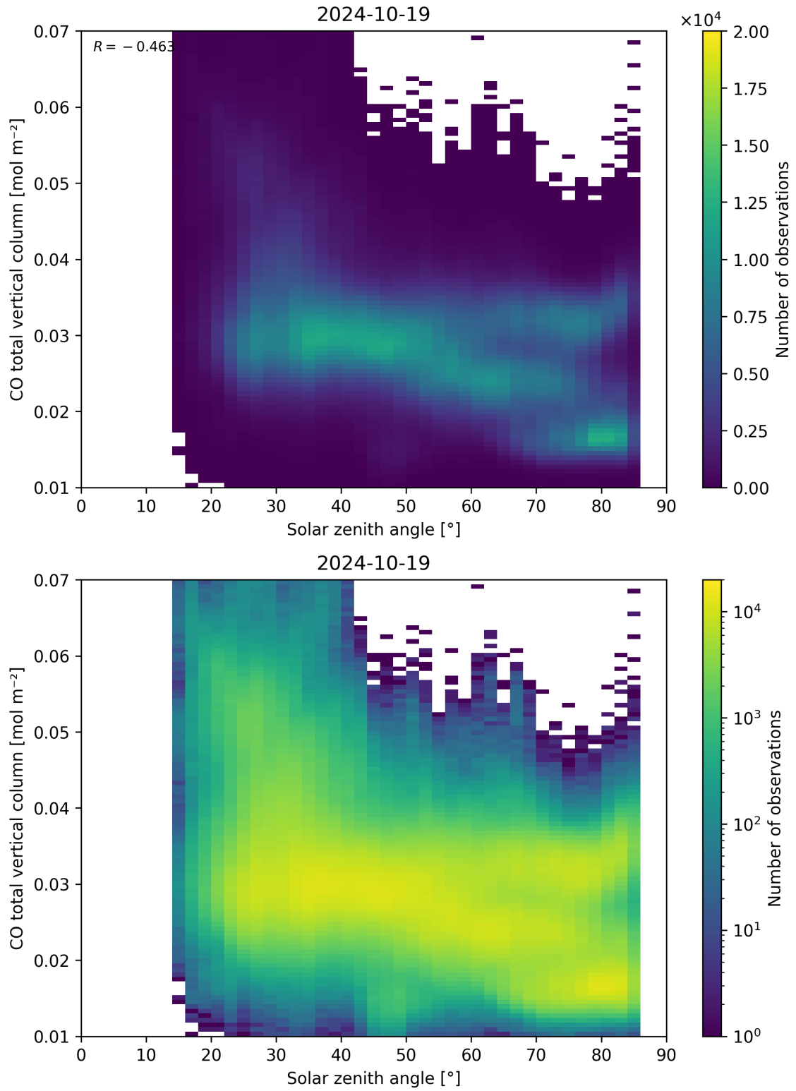
Figure 61: Scatter density plot of “Solar zenith angle” against “CO total vertical column” for 2024-10-19 to 2024-10-20.
