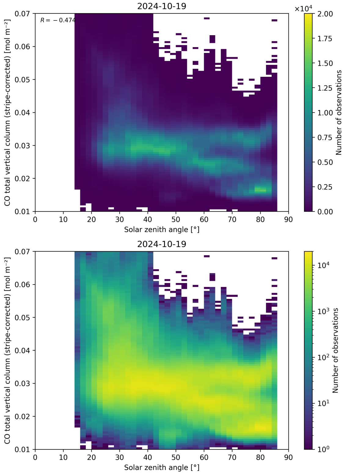
Figure 62: Scatter density plot of “Solar zenith angle” against “CO total vertical column (stripe-corrected)” for 2024-10-19 to 2024-10-20.
