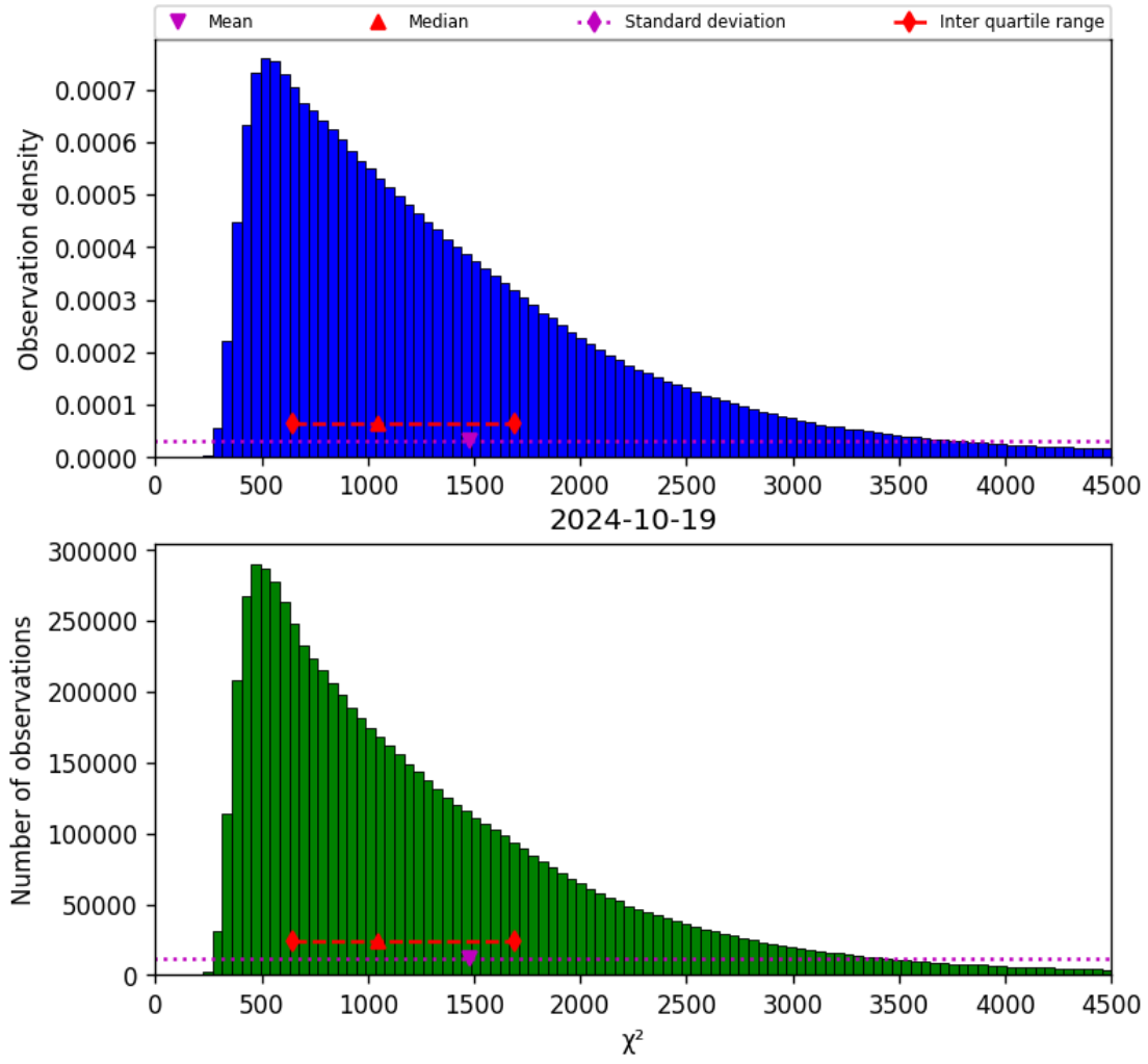
Figure 22: Histogram of “ \chi^2 ” for 2024-10-19 to 2024-10-20
