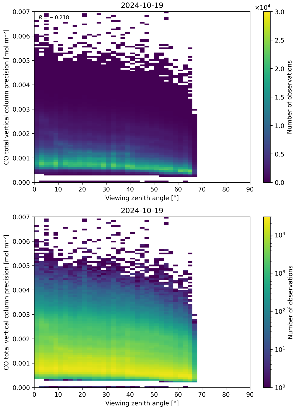
Figure 71: Scatter density plot of “Viewing zenith angle” against “CO total vertical column precision” for 2024-10-19 to 2024-10-20.
