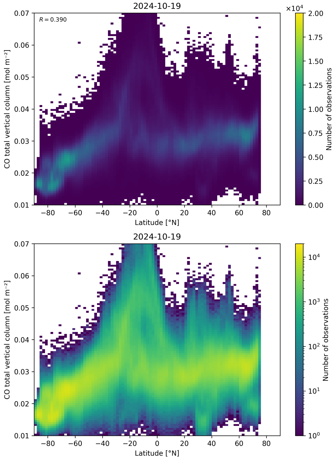
Figure 51: Scatter density plot of “Latitude” against “CO total vertical column” for 2024-10-19 to 2024-10-20.
