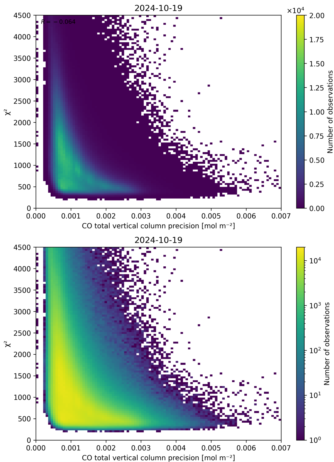
Figure 44: Scatter density plot of “CO total vertical column precision” against “ \chi^2 ” for 2024-10-19 to 2024-10-20.
