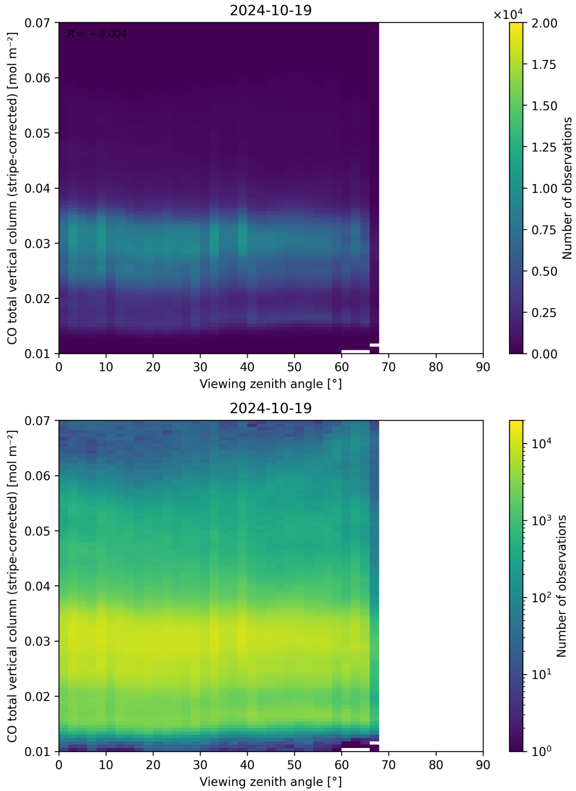
Figure 70: Scatter density plot of “Viewing zenith angle” against “CO total vertical column (stripe-corrected)” for 2024-10-19 to 2024-10-20.
