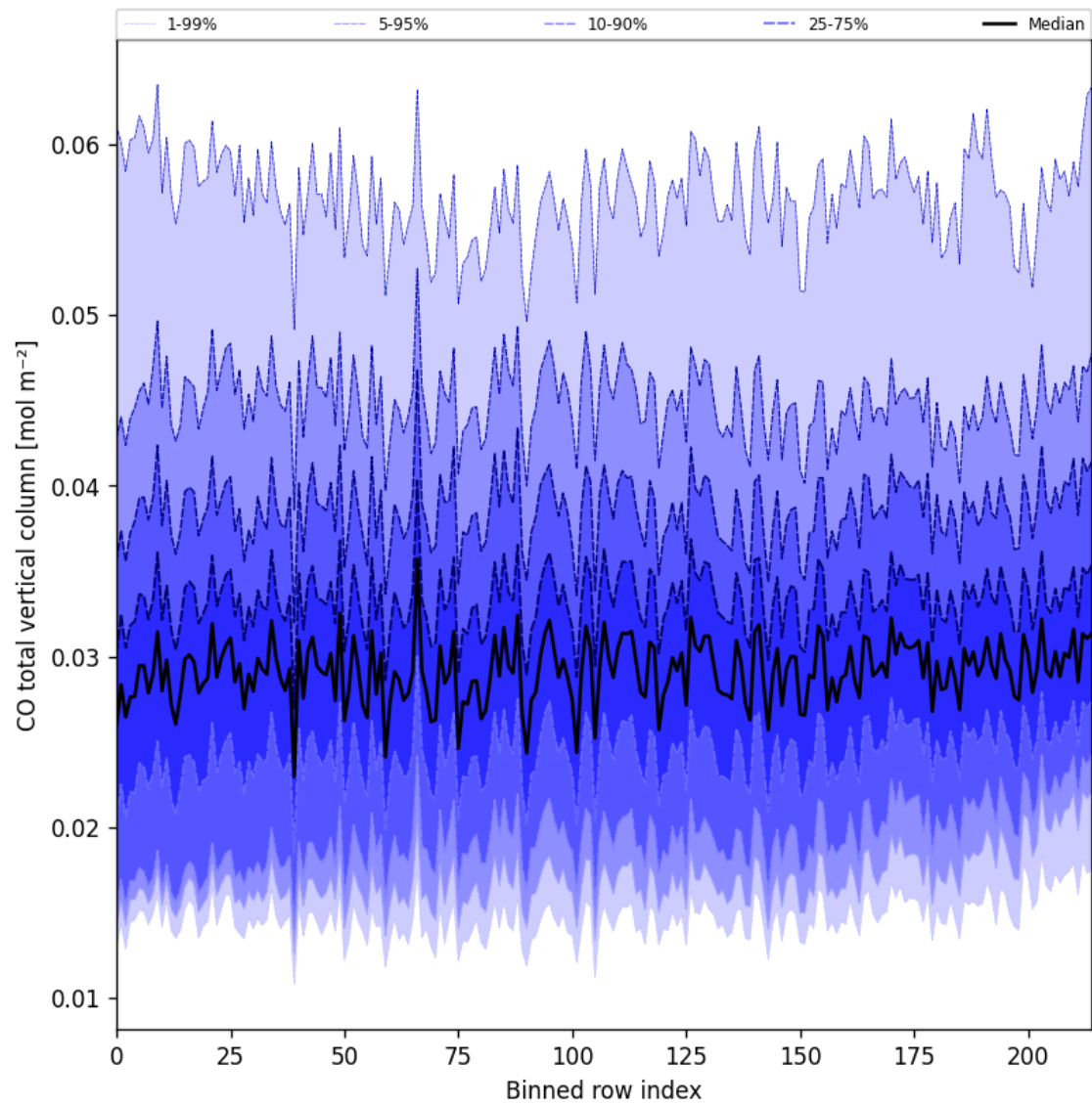
Figure 26: Along track statistics of "CO total vertical column" for 2024-10-19 to 2024-10-20
