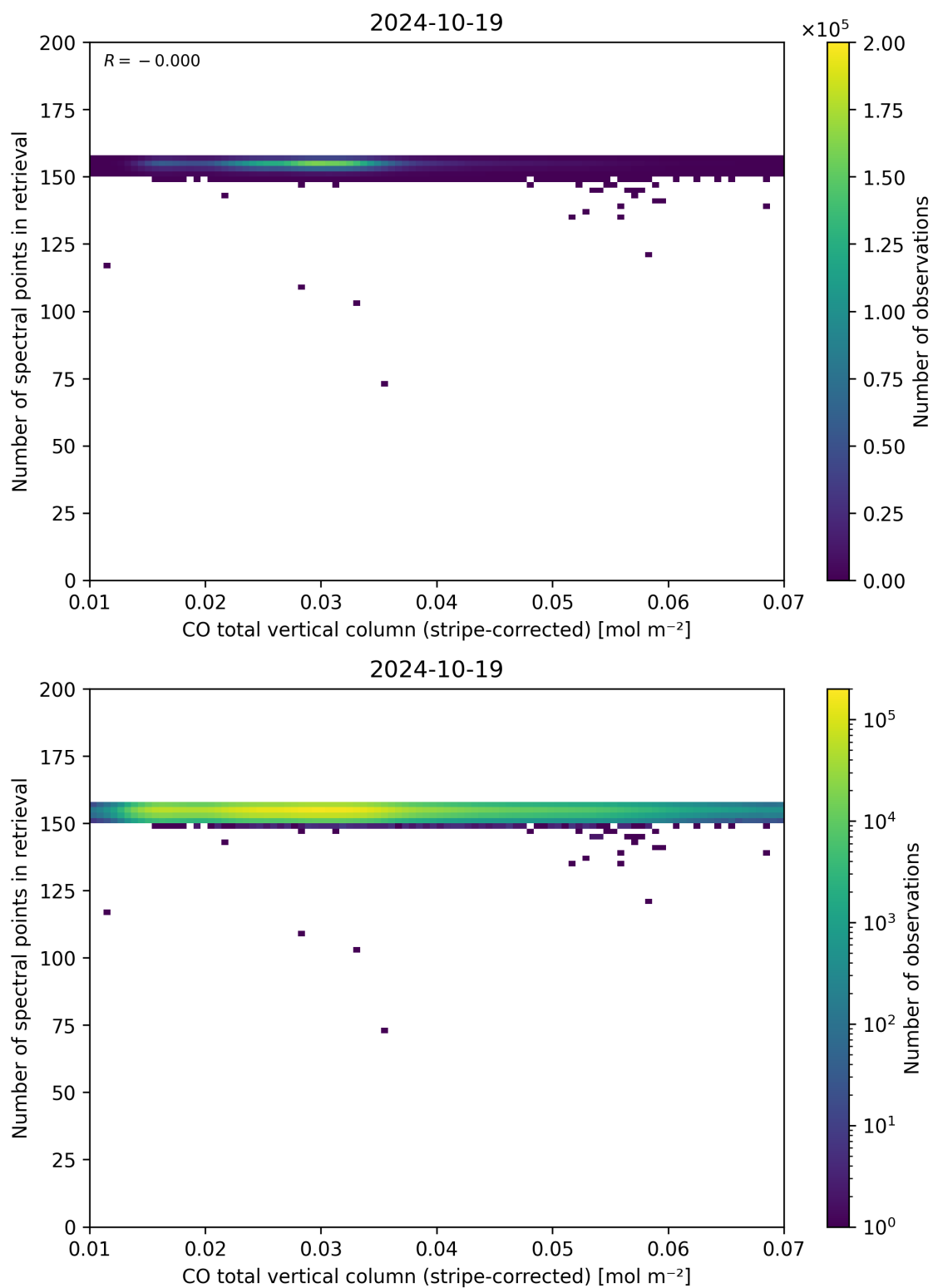
Figure 40: Scatter density plot of “CO total vertical column (stripe-corrected)” against “Number of spectral points in retrieval” for 2024-10-19 to 2024-10-20.
