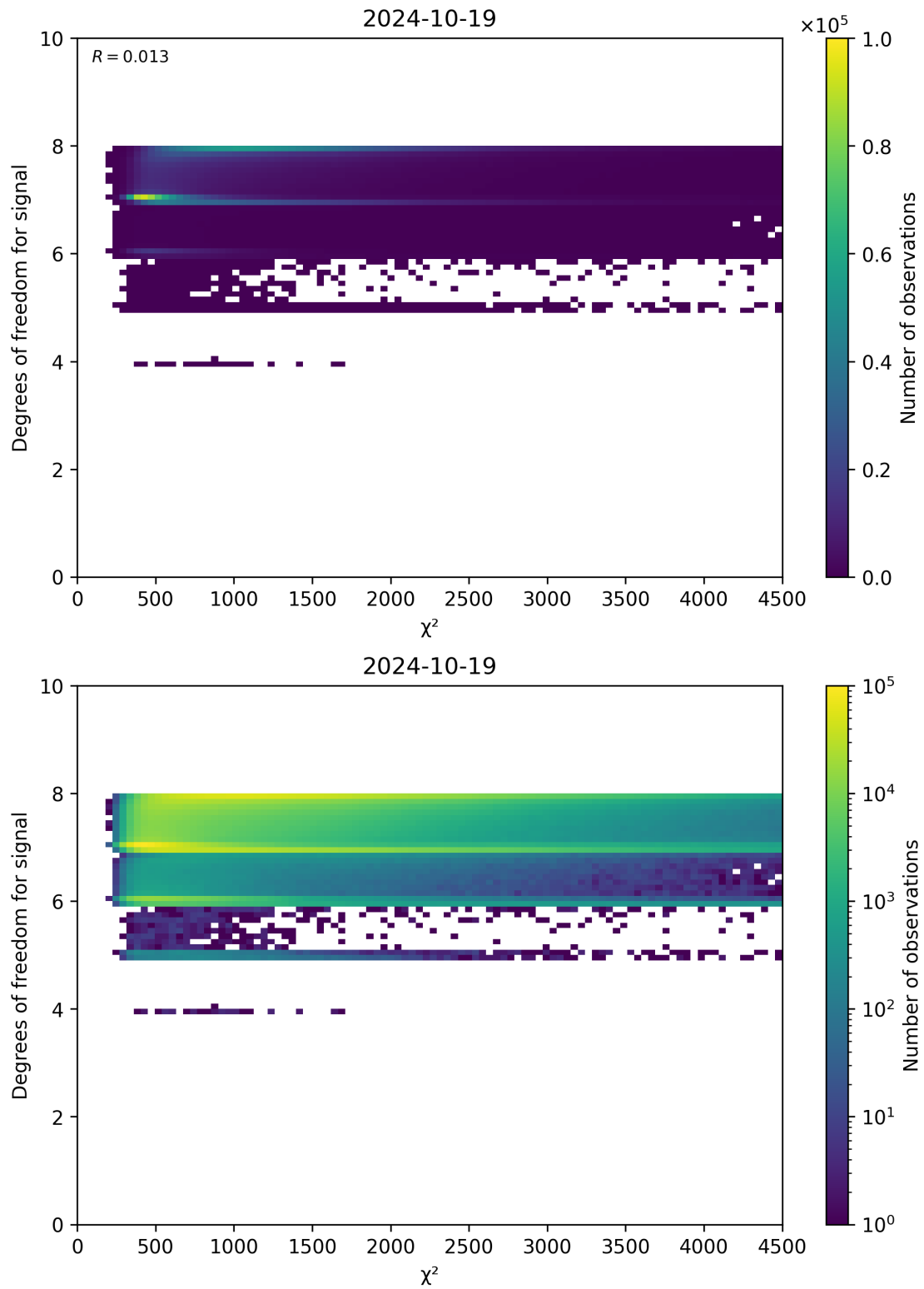
Figure 48: Scatter density plot of “ \chi^2 ” against “Degrees of freedom for signal” for 2024-10-19 to 2024-10-20.
