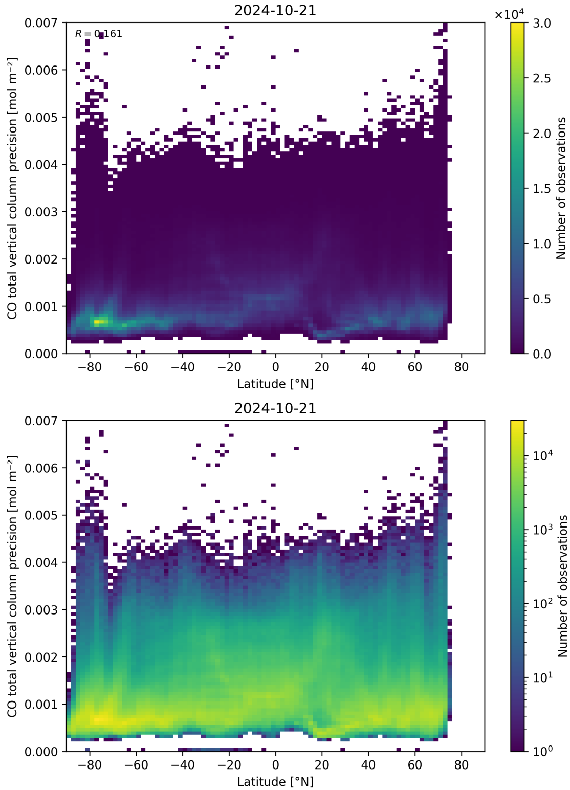
Figure 53: Scatter density plot of “Latitude” against “CO total vertical column precision” for 2024-10-20 to 2024-10-22.
