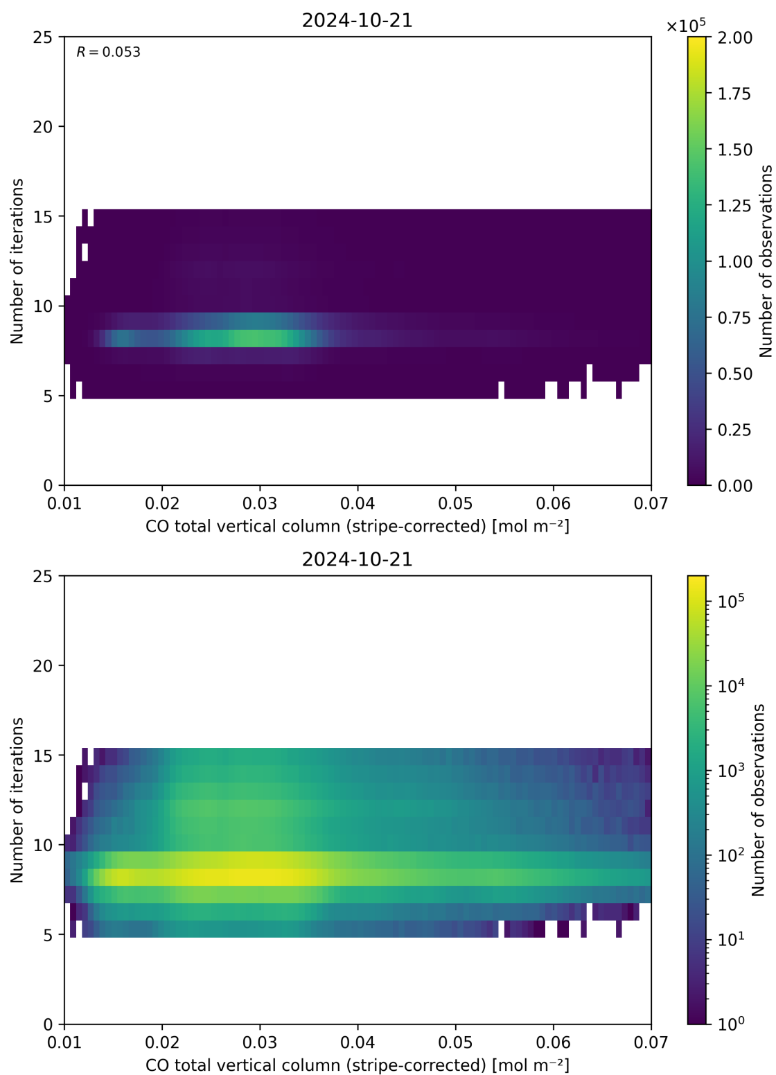
Figure 39: Scatter density plot of “CO total vertical column (stripe-corrected)” against “Number of iterations” for 2024-10-20 to 2024-10-22.
