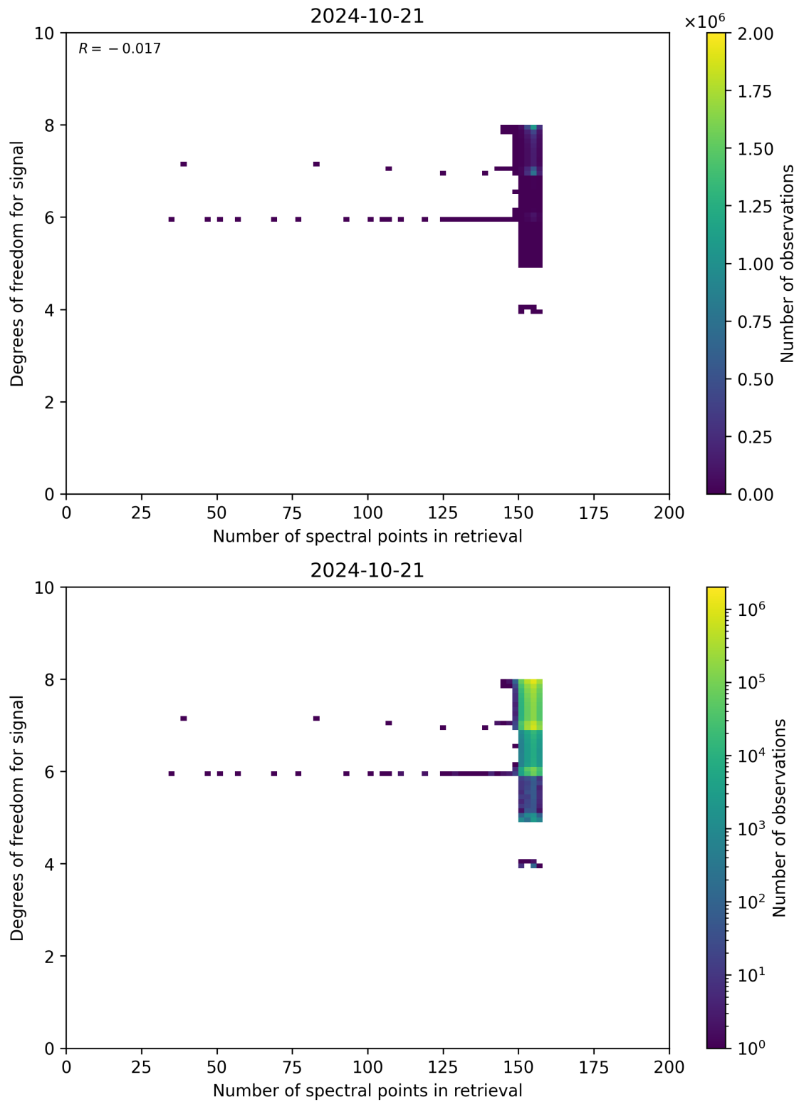
Figure 59: Scatter density plot of “Number of spectral points in retrieval” against “Degrees of freedom for signal” for 2024-10-20 to 2024-10-22.
