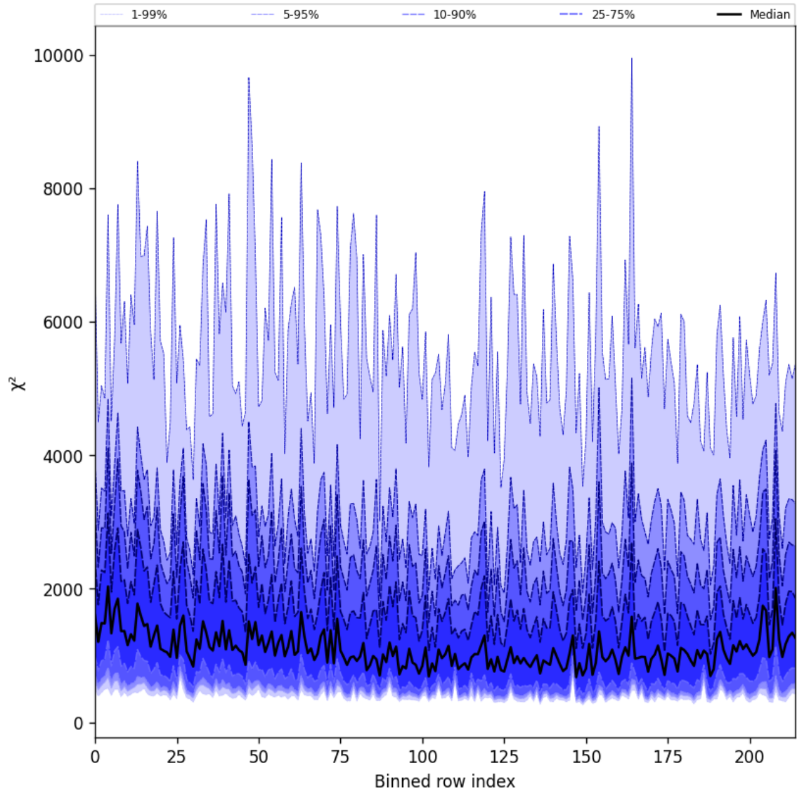
Figure 30: Along track statistics of “ \chi^2 ” for 2024-10-20 to 2024-10-22
