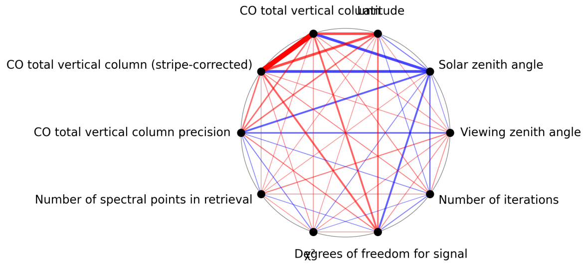
Figure 1: Map of correlation graph for 2024-10-20 to 2024-10-22.
