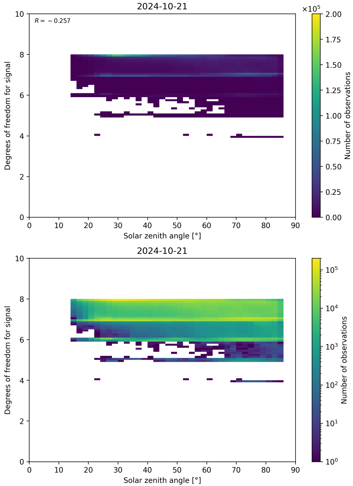
Figure 65: Scatter density plot of “Solar zenith angle” against “Degrees of freedom for signal” for 2024-10-20 to 2024-10-22.
