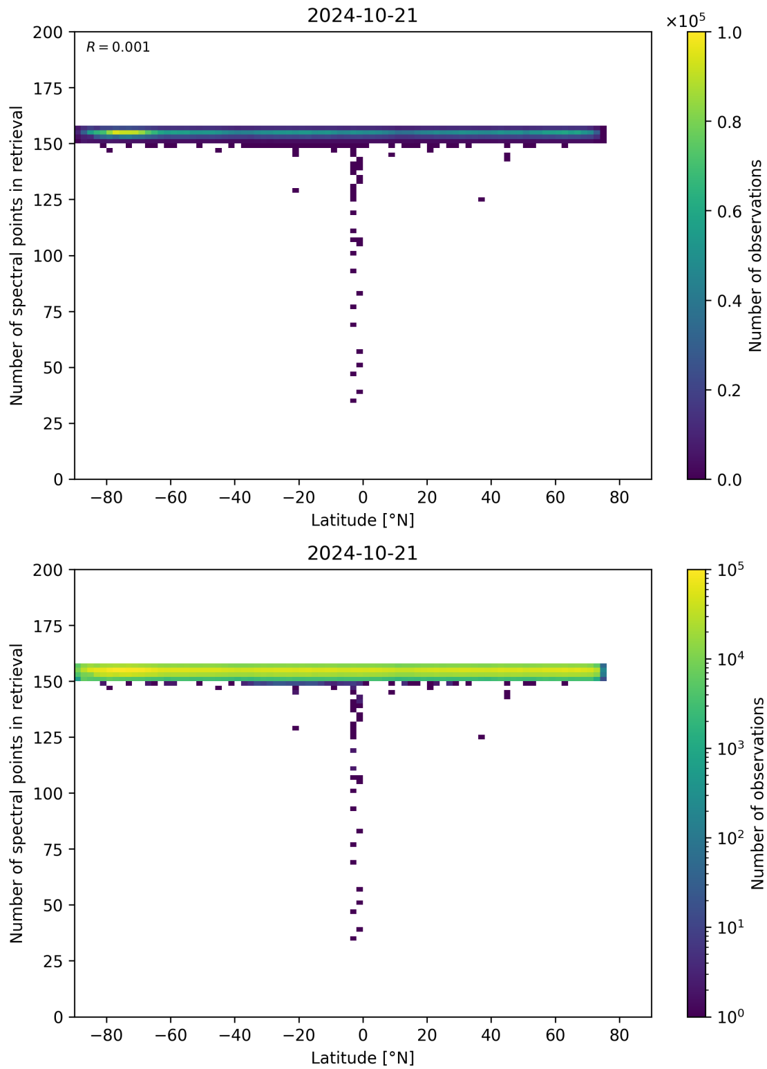
Figure 57: Scatter density plot of “Latitude” against “Number of spectral points in retrieval” for 2024-10-20 to 2024-10-22.
