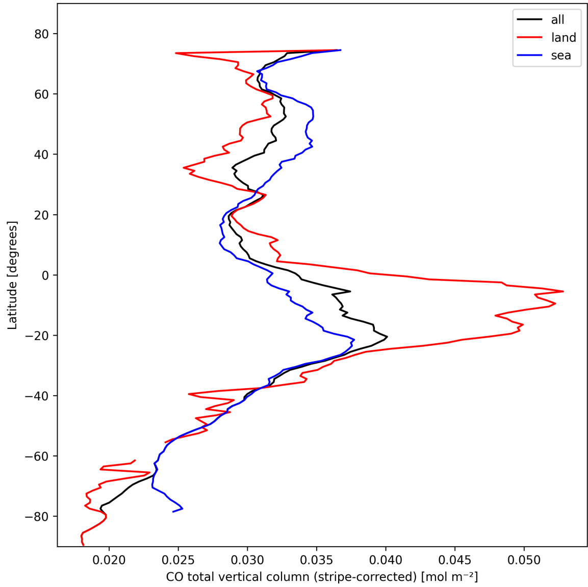
Figure 11: Zonal average of “CO total vertical column (stripe-corrected)” for 2024-10-20 to 2024-10-22.
