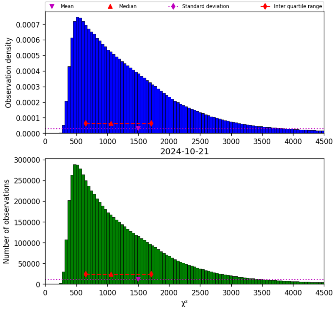
Figure 22: Histogram of “ \chi^2 ” for 2024-10-20 to 2024-10-22
