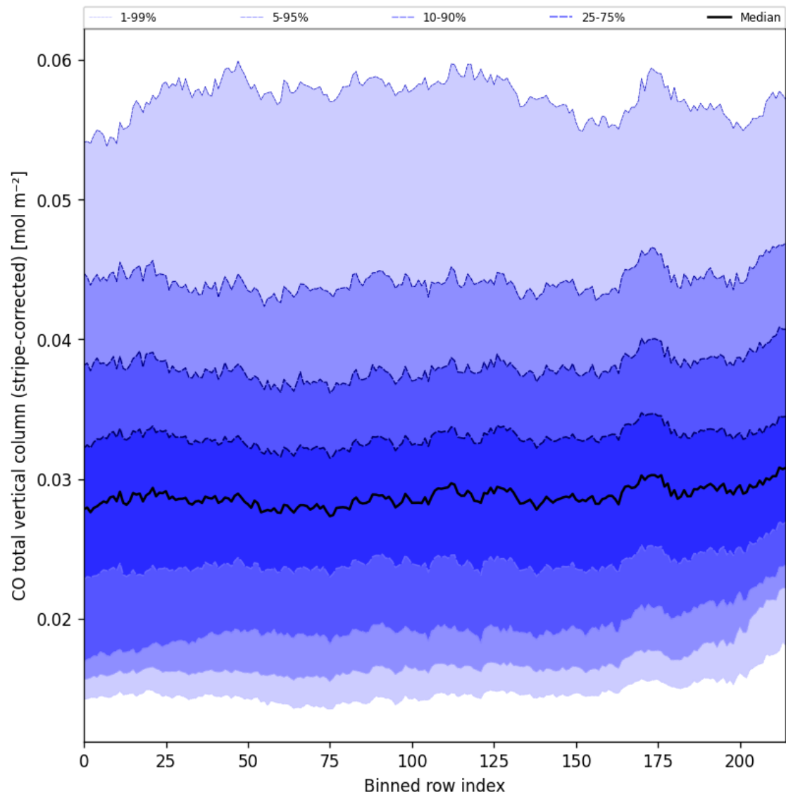
Figure 27: Along track statistics of “CO total vertical column (stripe-corrected)” for 2024-10-20 to 2024-10-22
