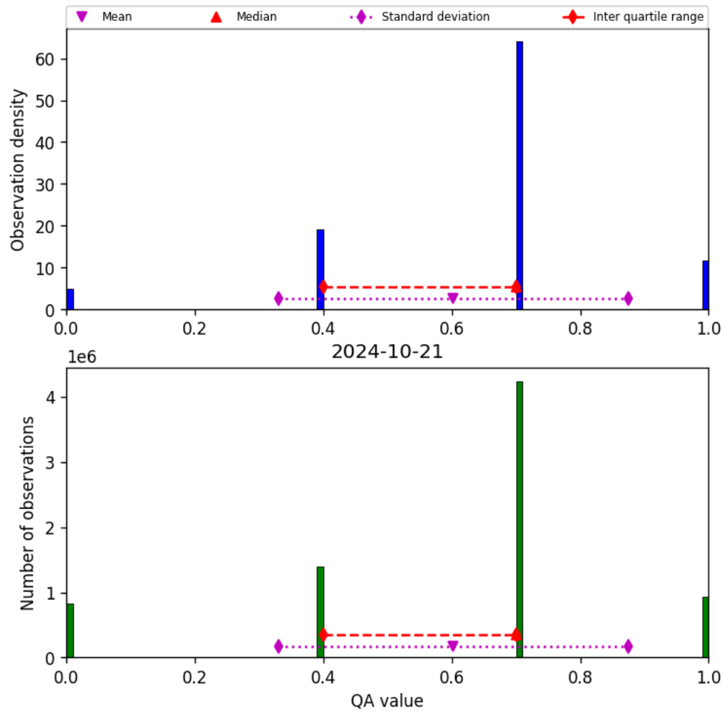
Figure 17: Histogram of “QA value” for 2024-10-20 to 2024-10-22
