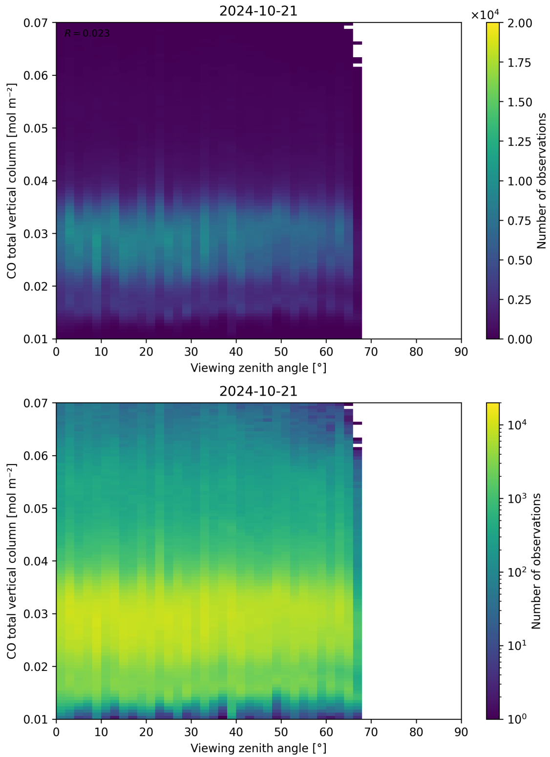
Figure 69: Scatter density plot of “Viewing zenith angle” against “CO total vertical column” for 2024-10-20 to 2024-10-22.
