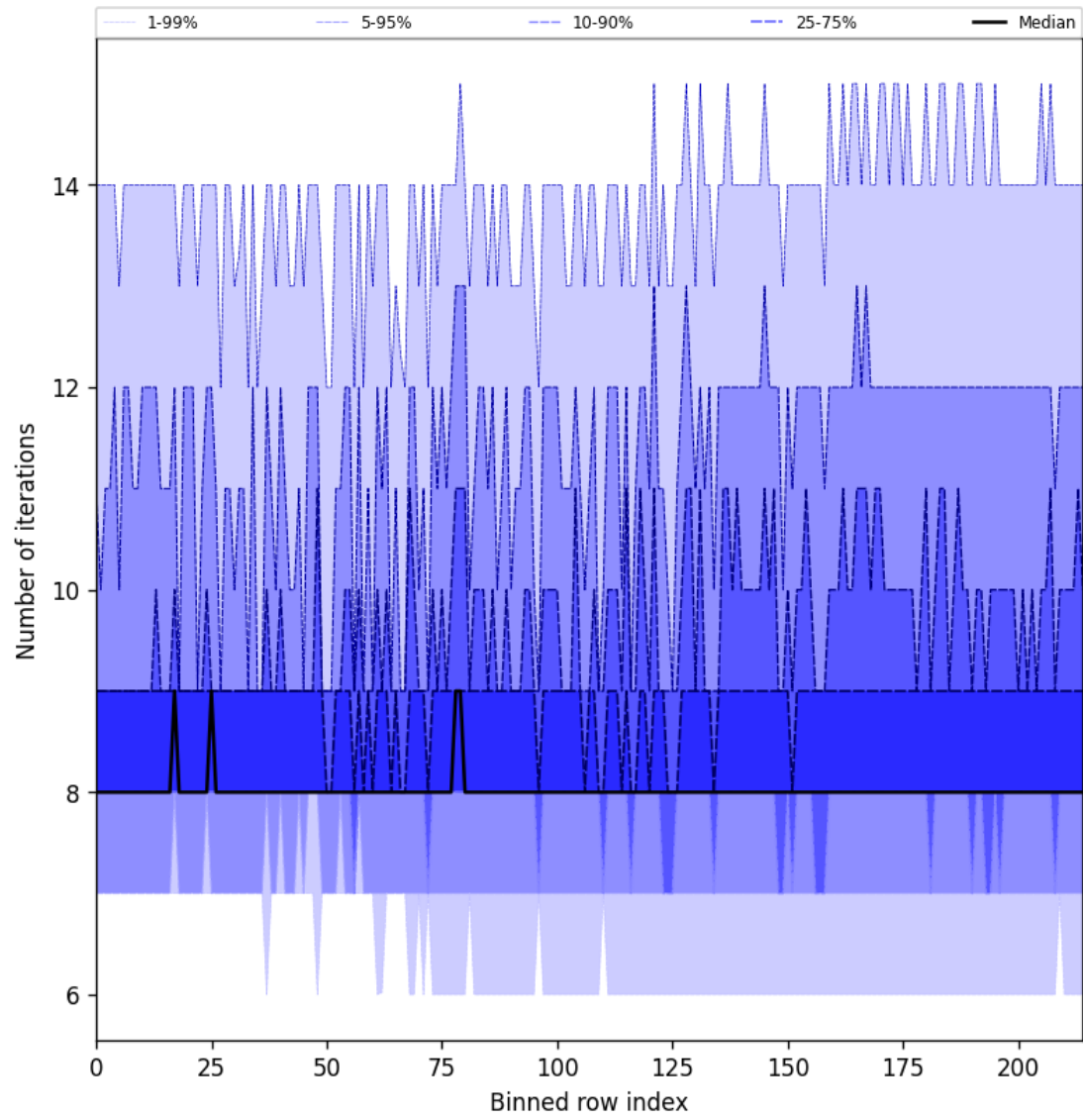
Figure 32: Along track statistics of “Number of iterations” for 2024-10-20 to 2024-10-22
