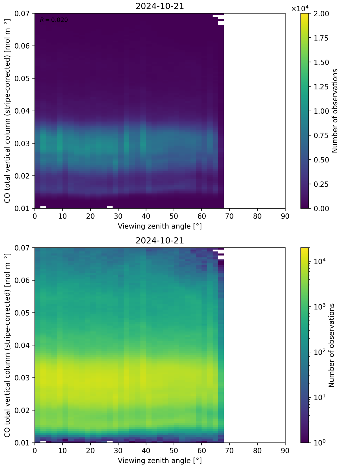
Figure 70: Scatter density plot of “Viewing zenith angle” against “CO total vertical column (stripe-corrected)” for 2024-10-20 to 2024-10-22.
