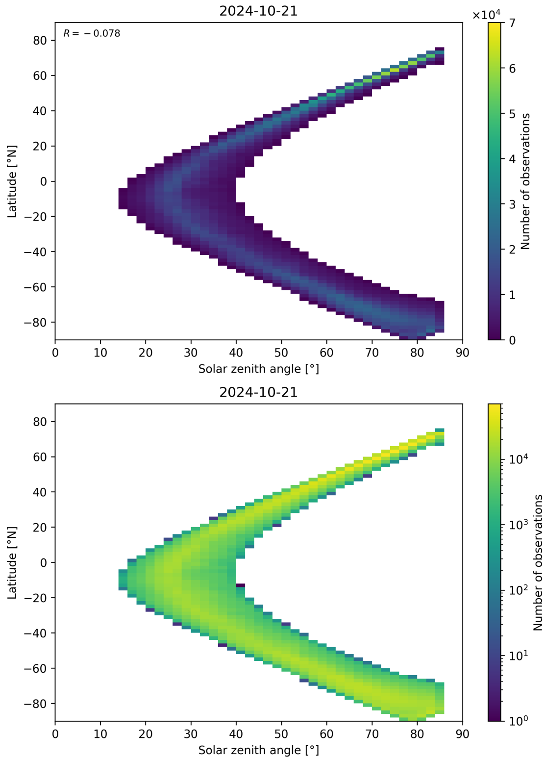
Figure 66: Scatter density plot of “Solar zenith angle” against “Latitude” for 2024-10-20 to 2024-10-22.
