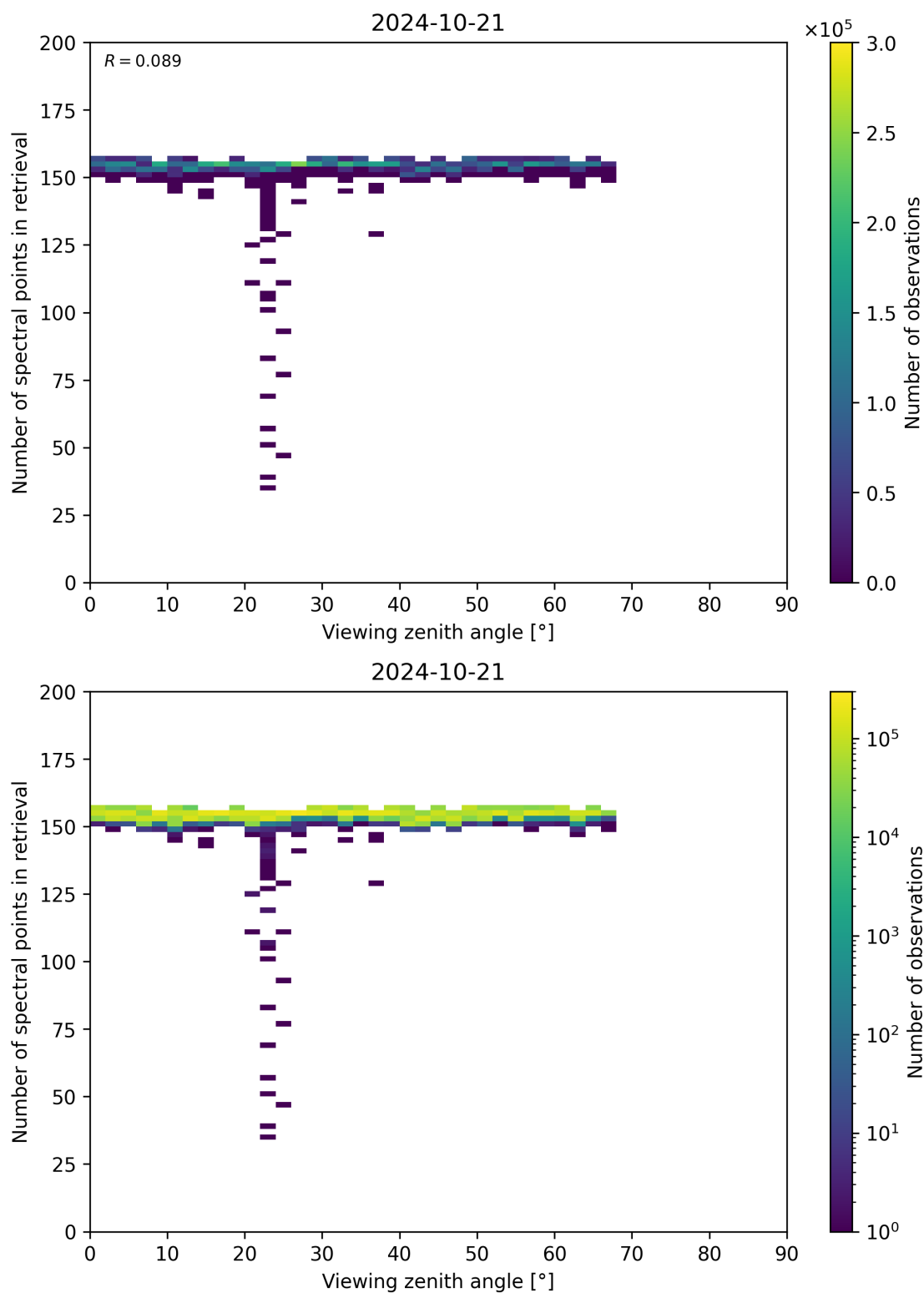
Figure 76: Scatter density plot of “Viewing zenith angle” against “Number of spectral points in retrieval” for 2024-10-20 to 2024-10-22.
