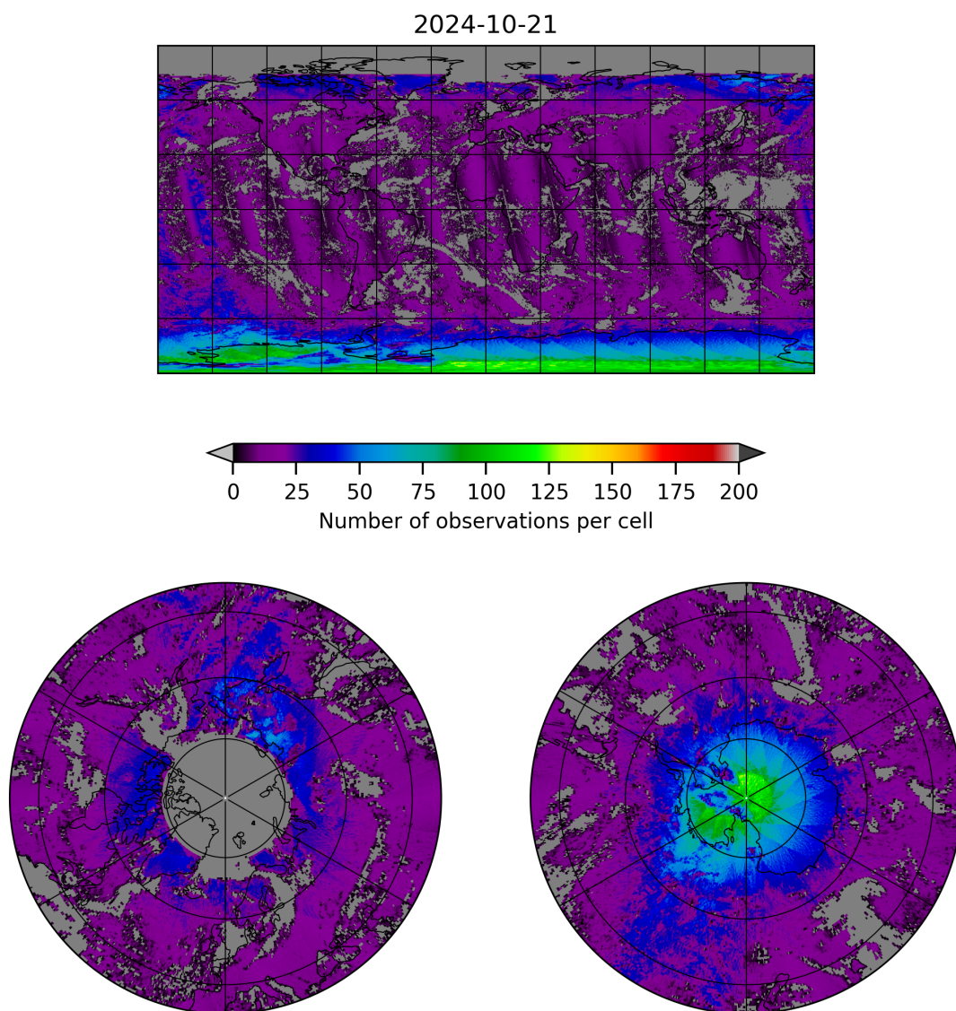
Figure 8: Map of the number of observations for 2024-10-20 to 2024-10-22
