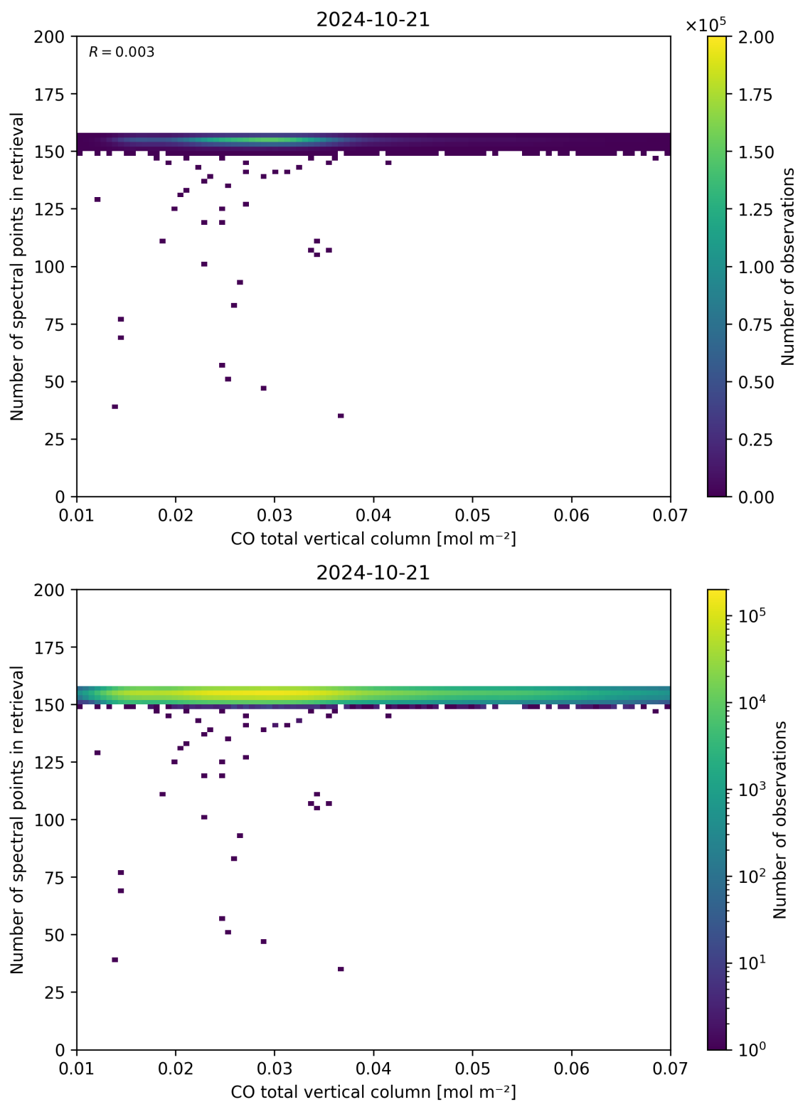
Figure 43: Scatter density plot of “CO total vertical column” against “Number of spectral points in retrieval” for 2024-10-20 to 2024-10-22.
