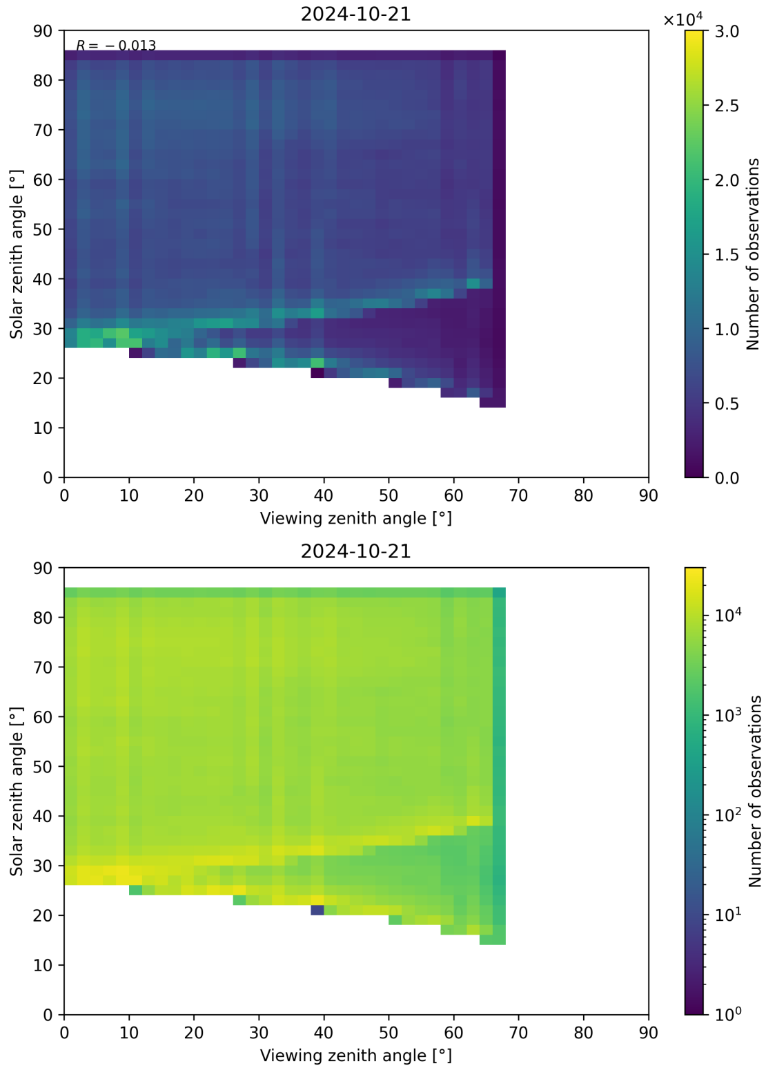
Figure 77: Scatter density plot of “Viewing zenith angle” against “Solar zenith angle” for 2024-10-20 to 2024-10-22.
