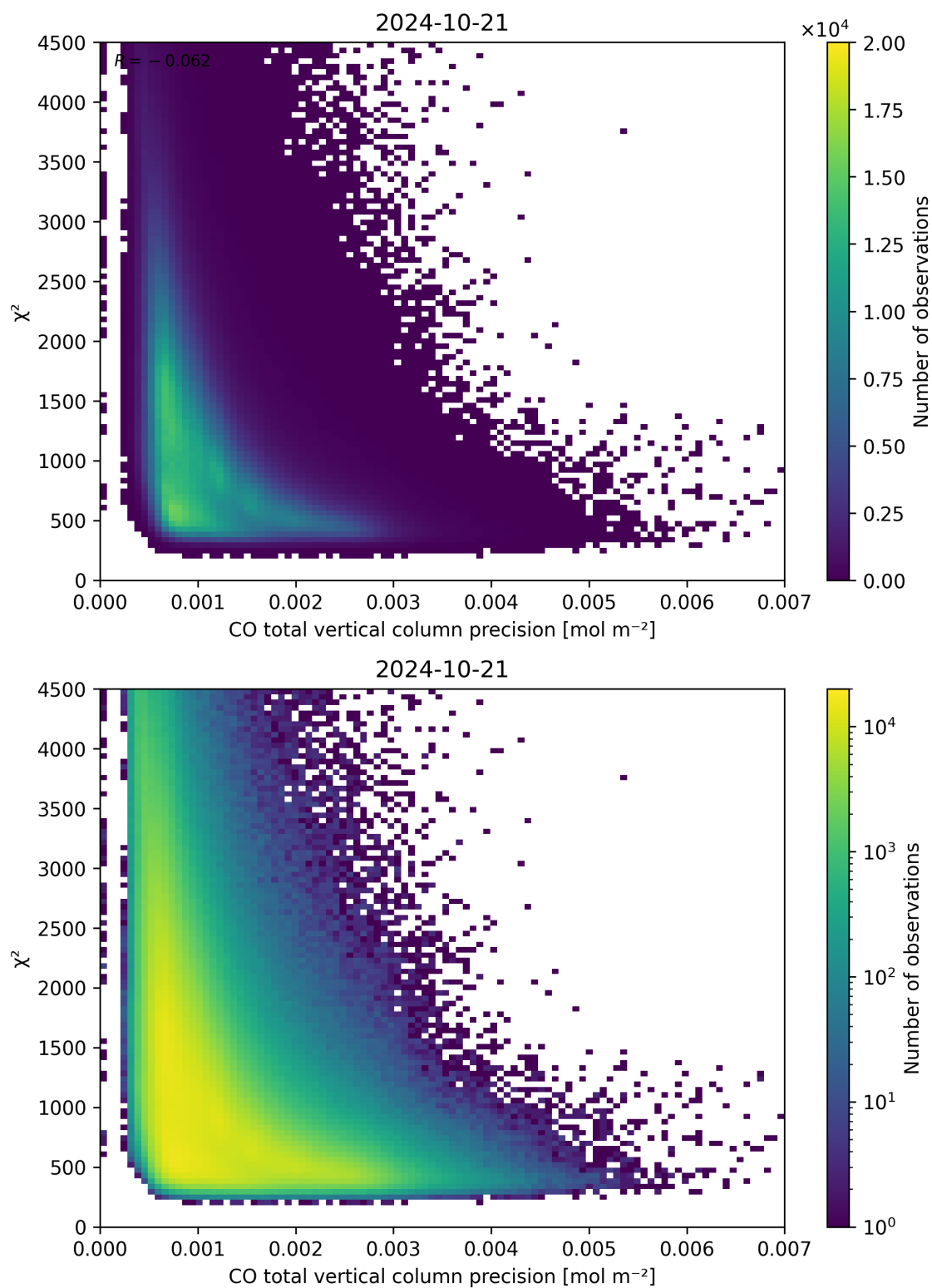
Figure 44: Scatter density plot of “CO total vertical column precision” against “ \chi^2 ” for 2024-10-20 to 2024-10-22.
