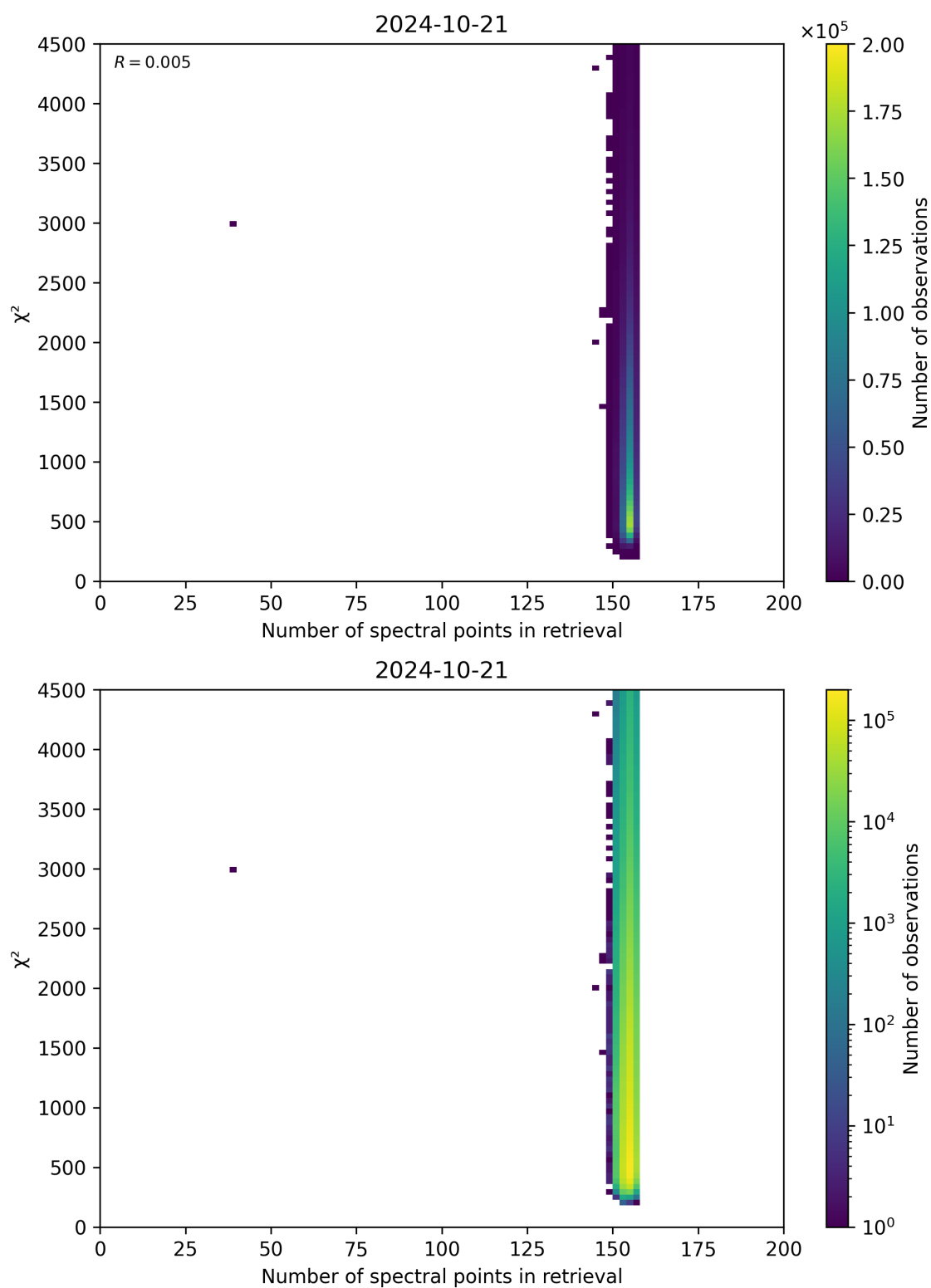
Figure 58: Scatter density plot of “Number of spectral points in retrieval” against “ \chi^2 ” for 2024-10-20 to 2024-10-22.
