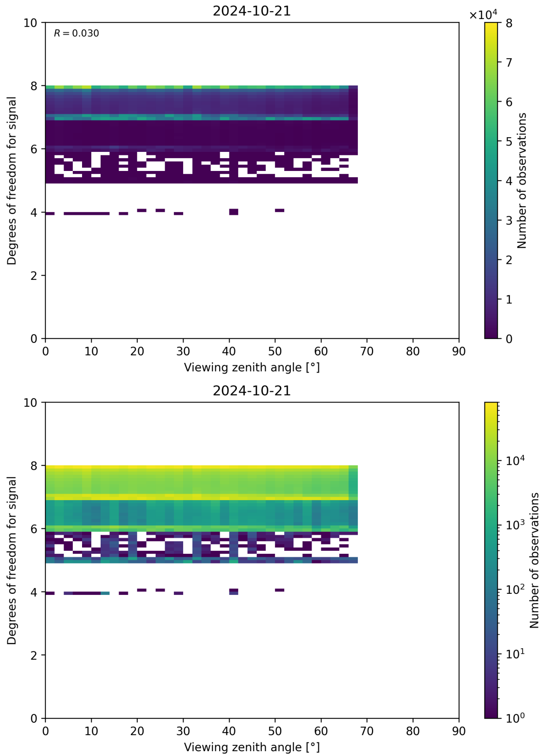
Figure 73: Scatter density plot of “Viewing zenith angle” against “Degrees of freedom for signal” for 2024-10-20 to 2024-10-22.
