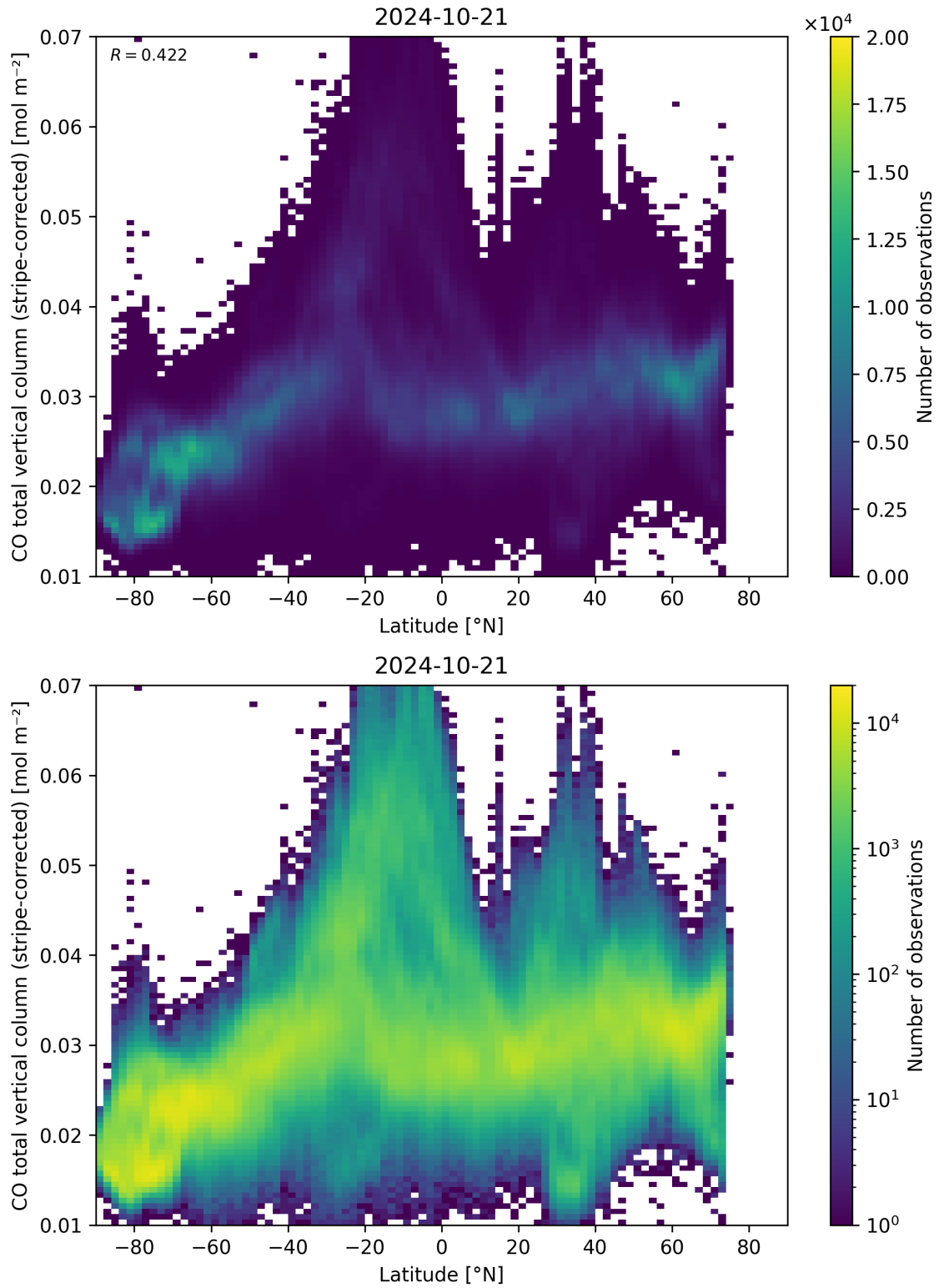
Figure 52: Scatter density plot of “Latitude” against “CO total vertical column (stripe-corrected)” for 2024-10-20 to 2024-10-22.
