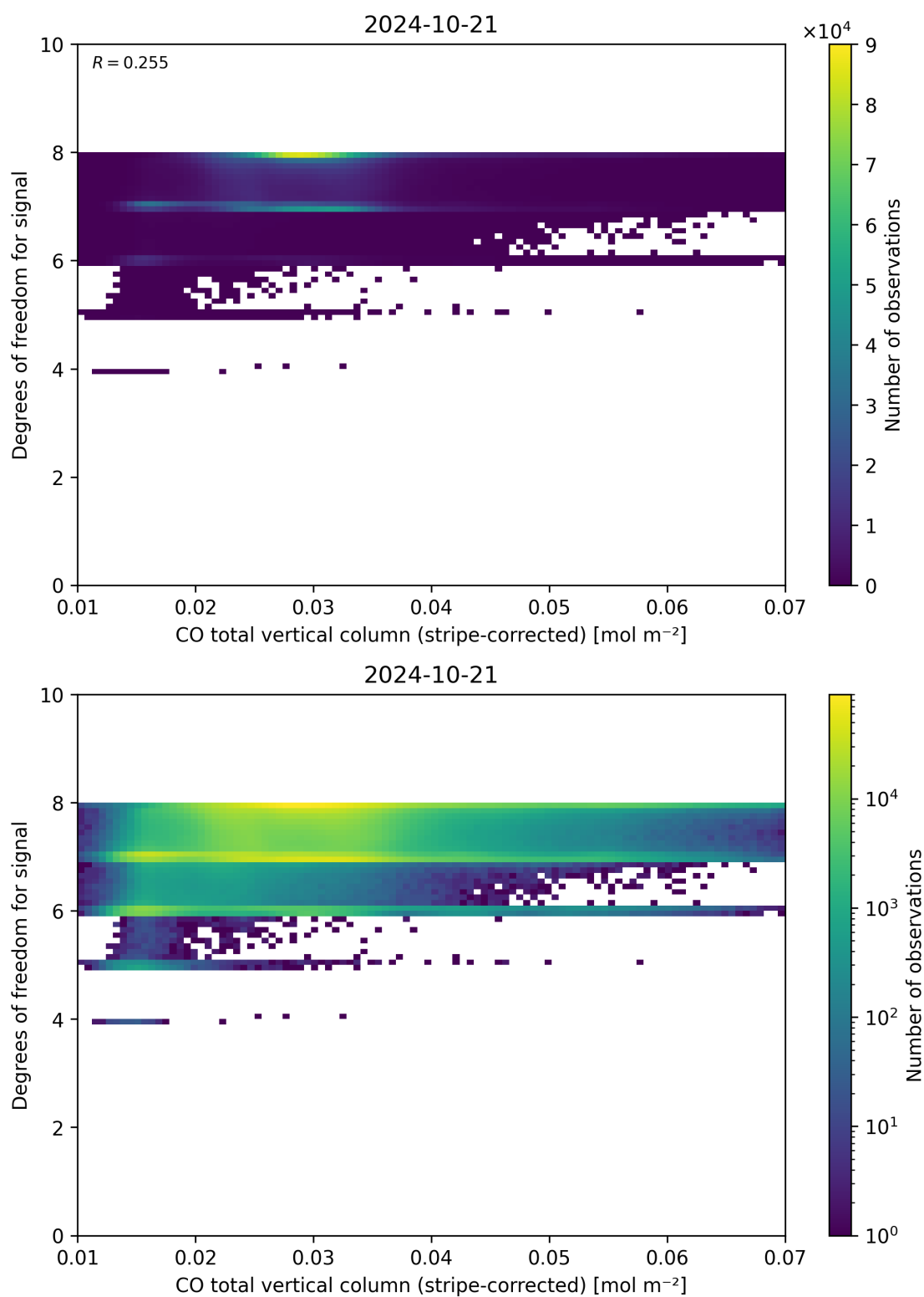
Figure 38: Scatter density plot of “CO total vertical column (stripe-corrected)” against “Degrees of freedom for signal” for 2024-10-20 to 2024-10-22.
