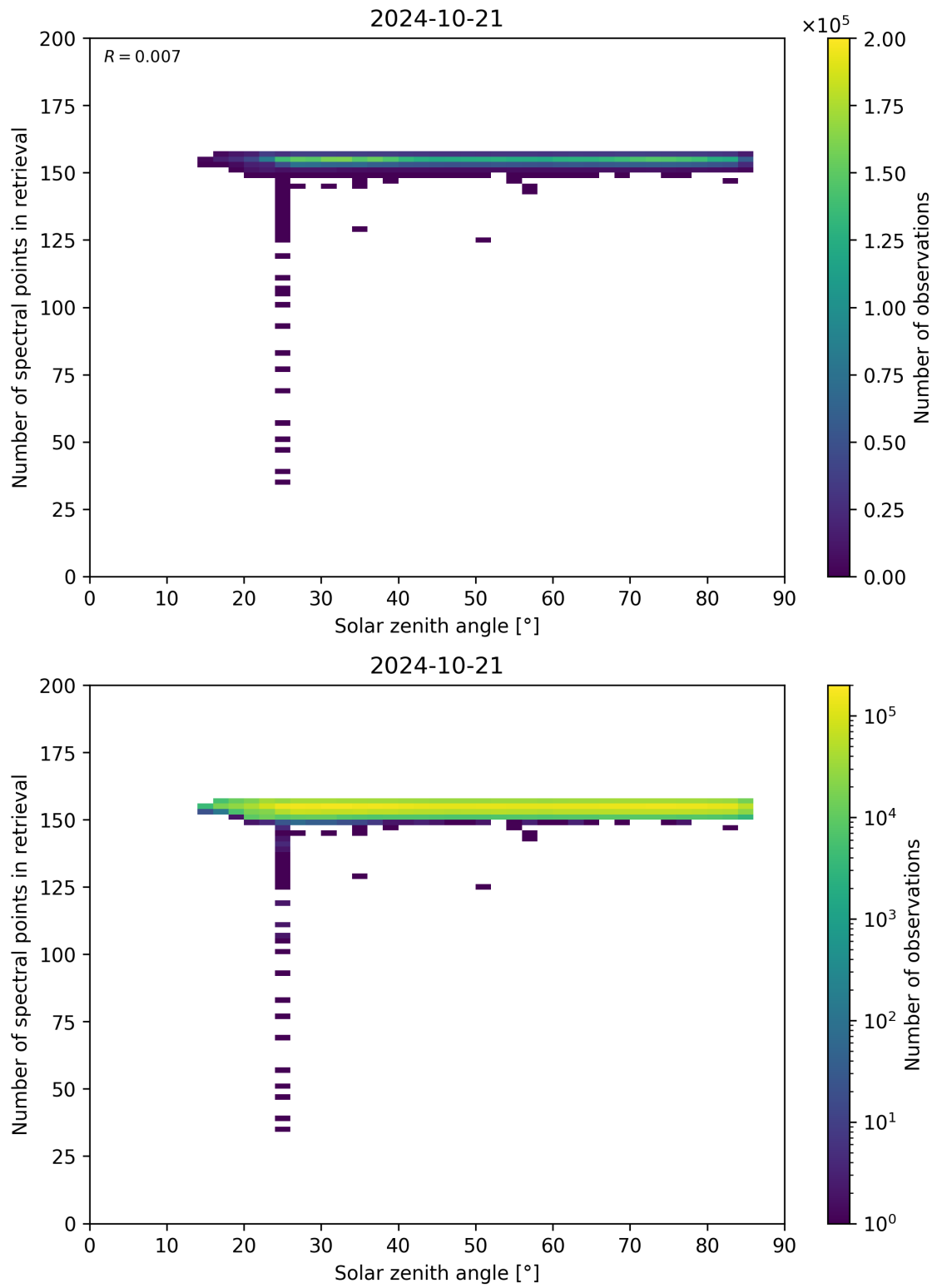
Figure 68: Scatter density plot of “Solar zenith angle” against “Number of spectral points in retrieval” for 2024-10-20 to 2024-10-22.
