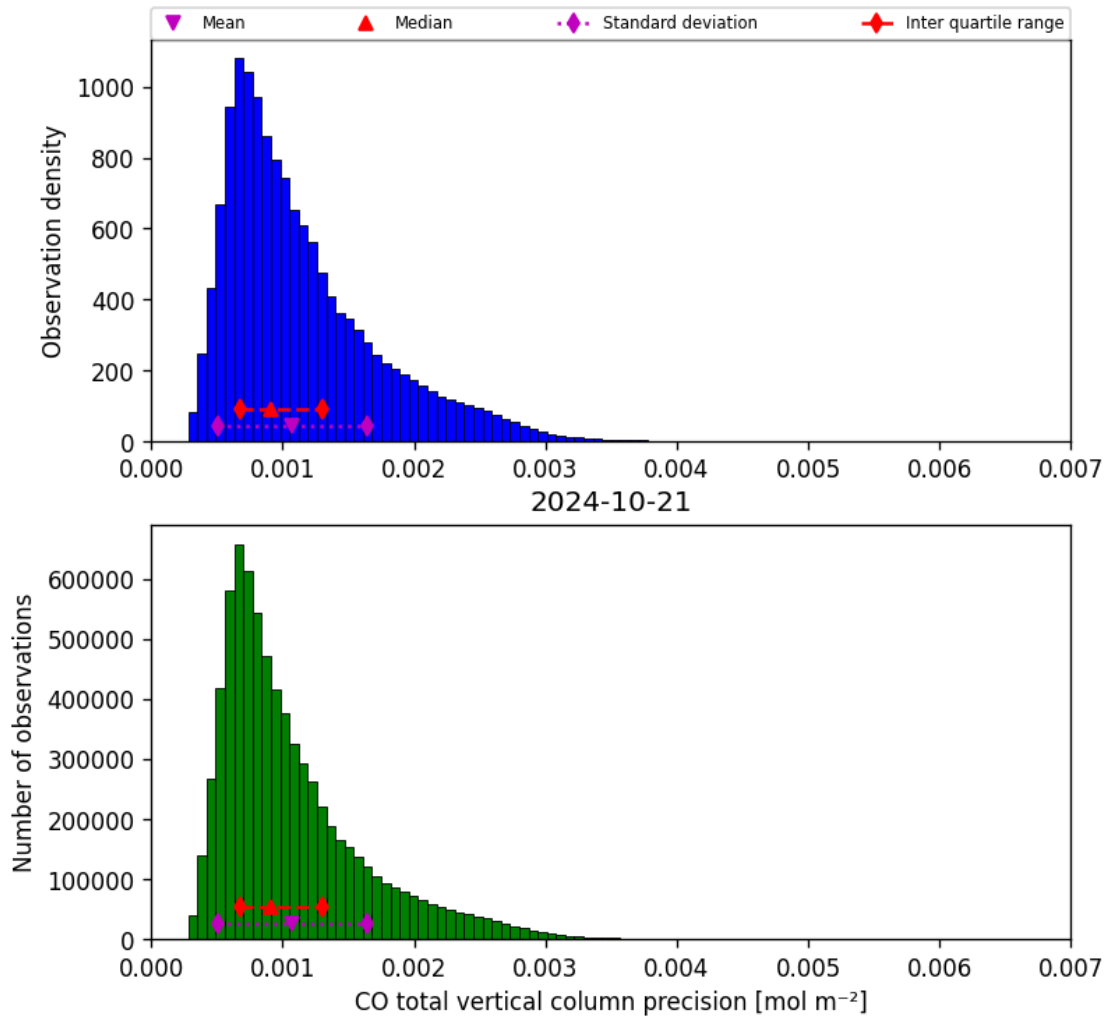
Figure 20: Histogram of “CO total vertical column precision” for 2024-10-20 to 2024-10-22
