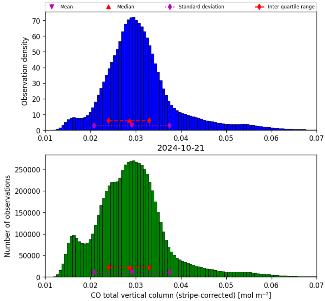
Figure 19: Histogram of “CO total vertical column (stripe-corrected)” for 2024-10-20 to 2024-10-22
