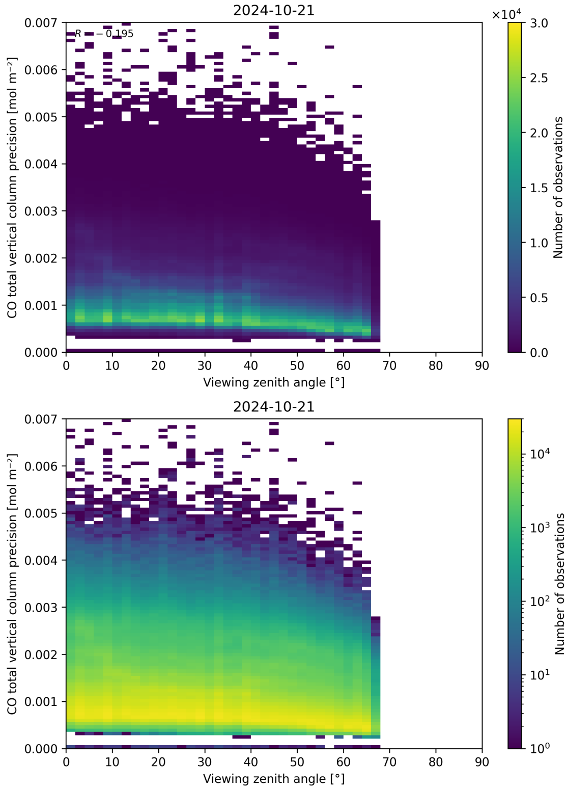
Figure 71: Scatter density plot of “Viewing zenith angle” against “CO total vertical column precision” for 2024-10-20 to 2024-10-22.
