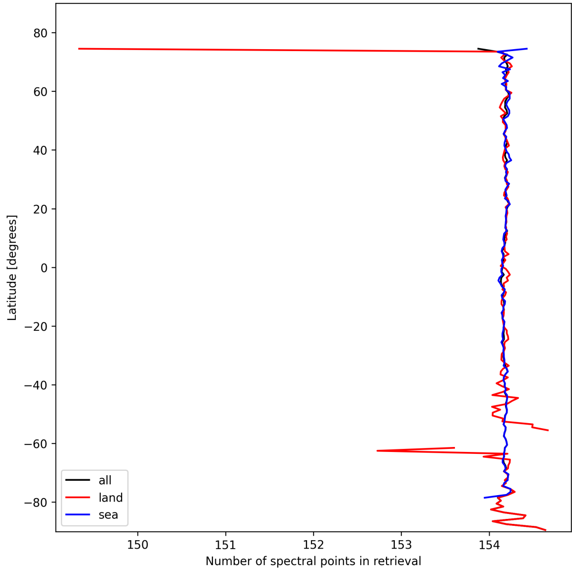
Figure 13: Zonal average of “Number of spectral points in retrieval” for 2024-10-20 to 2024-10-22.
