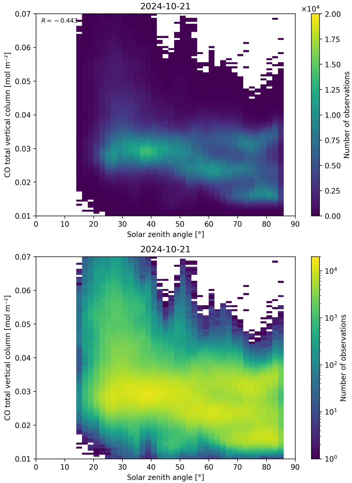
Figure 61: Scatter density plot of “Solar zenith angle” against “CO total vertical column” for 2024-10-20 to 2024-10-22.
