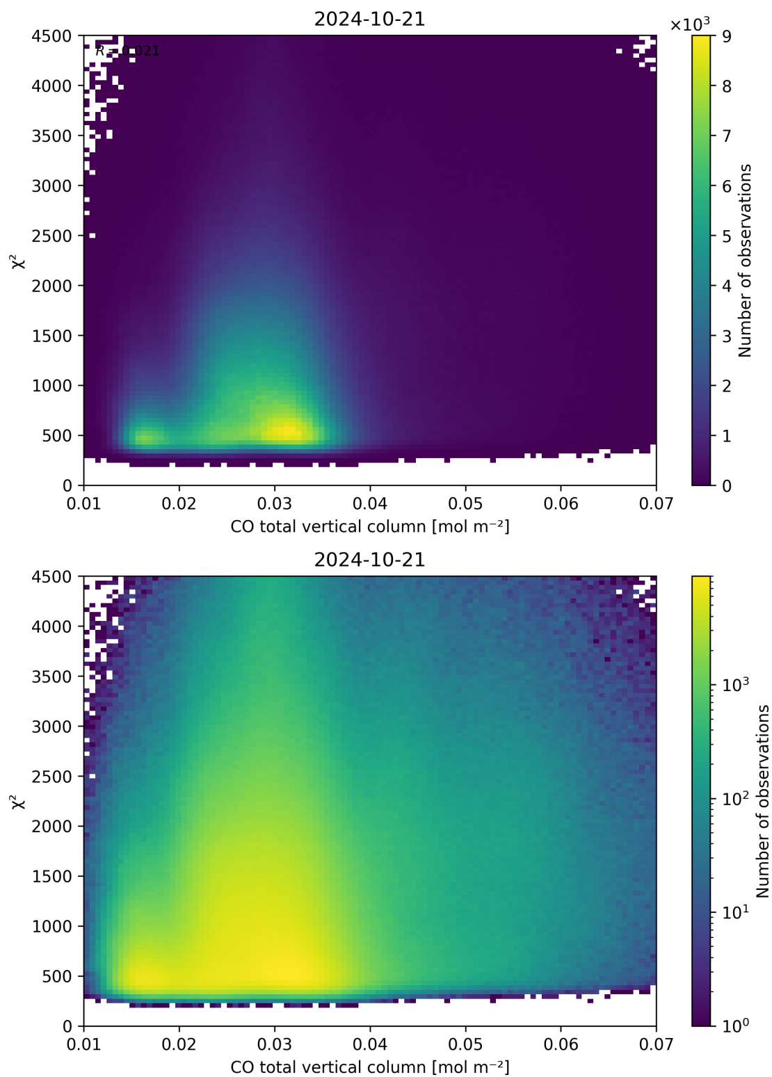
Figure 35: Scatter density plot of “CO total vertical column” against “ \chi^2 ” for 2024-10-20 to 2024-10-22.
