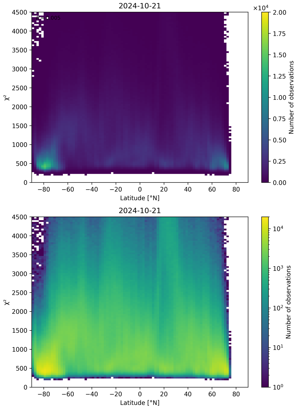
Figure 54: Scatter density plot of “Latitude” against “ \chi^2 ” for 2024-10-20 to 2024-10-22.
