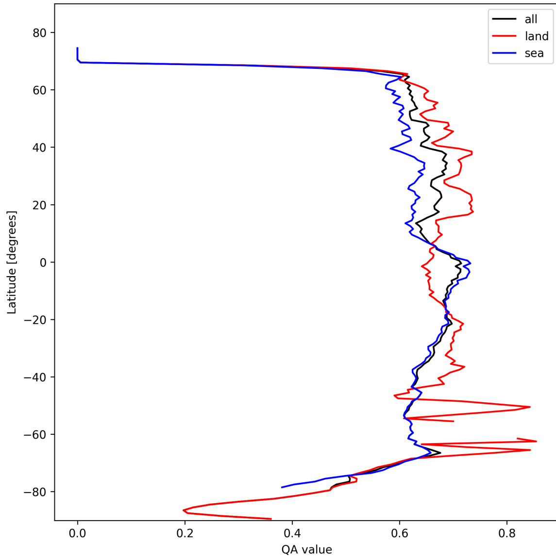
Figure 9: Zonal average of “QA value” for 2024-10-20 to 2024-10-22.
