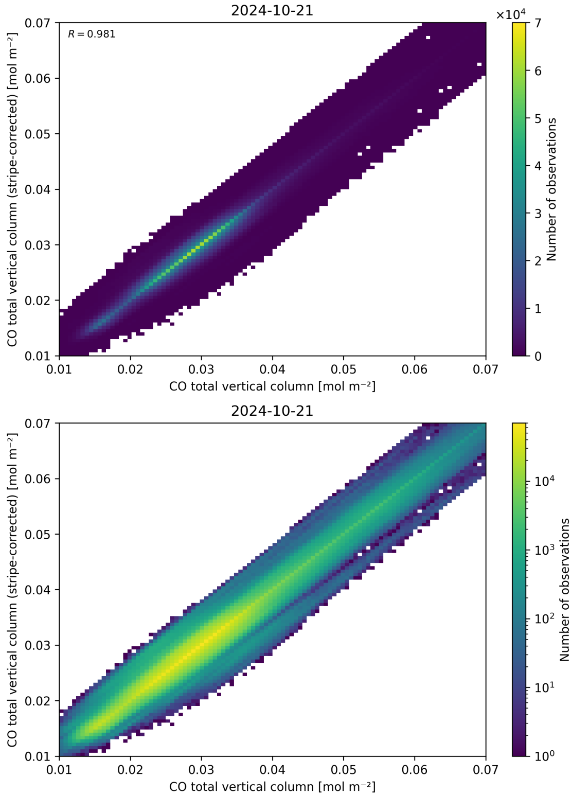
Figure 33: Scatter density plot of “CO total vertical column” against “CO total vertical column (stripe-corrected)” for 2024-10-20 to 2024-10-22.
