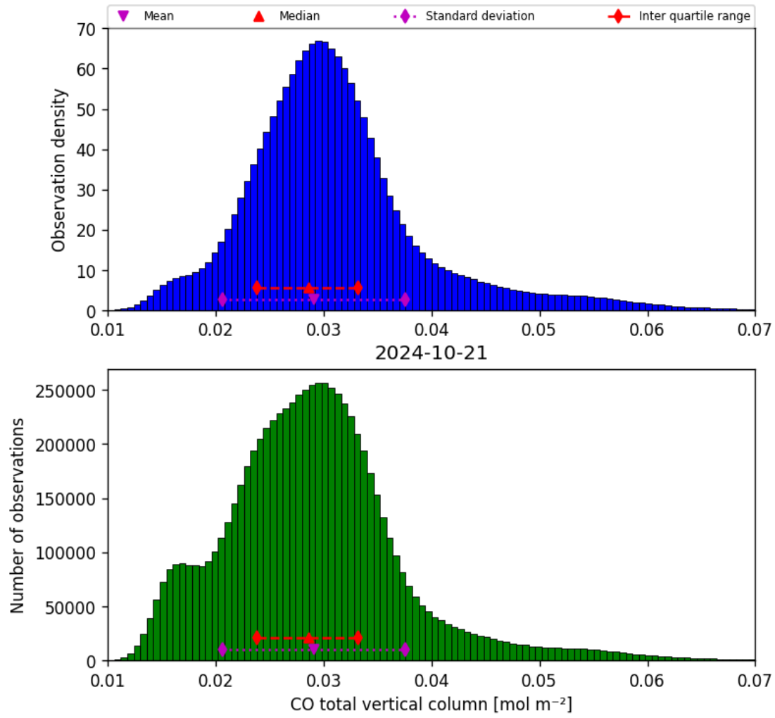
Figure 18: Histogram of “CO total vertical column” for 2024-10-20 to 2024-10-22
