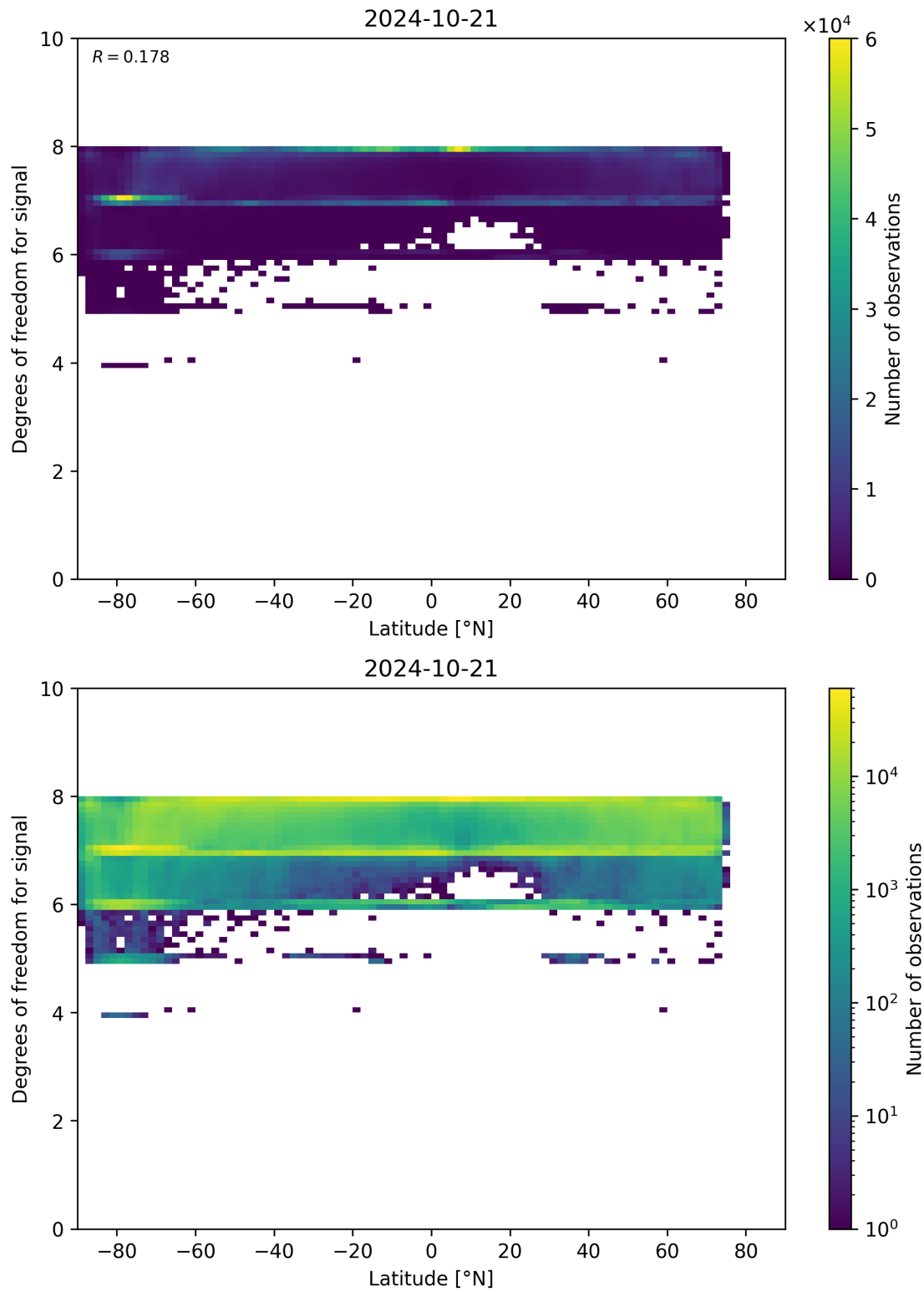
Figure 55: Scatter density plot of “Latitude” against “Degrees of freedom for signal” for 2024-10-20 to 2024-10-22.
