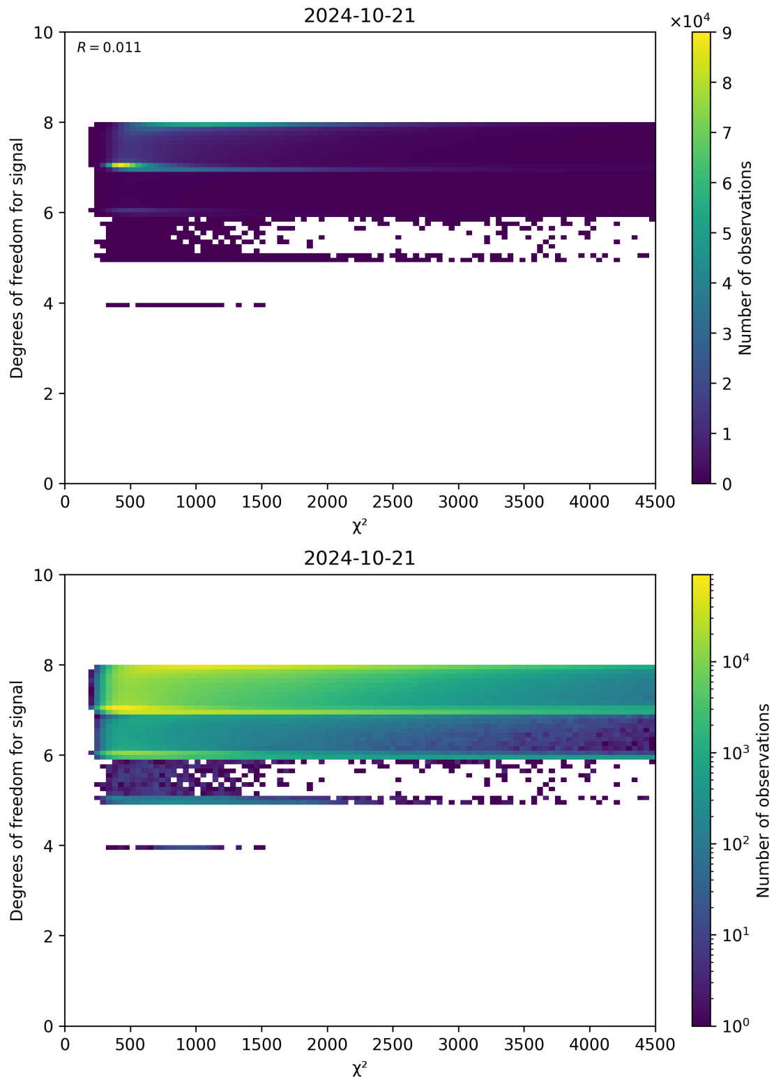
Figure 48: Scatter density plot of “ \chi^2 ” against “Degrees of freedom for signal” for 2024-10-20 to 2024-10-22.
