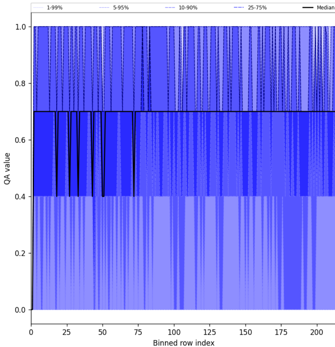
Figure 25: Along track statistics of “QA value” for 2024-10-20 to 2024-10-22
