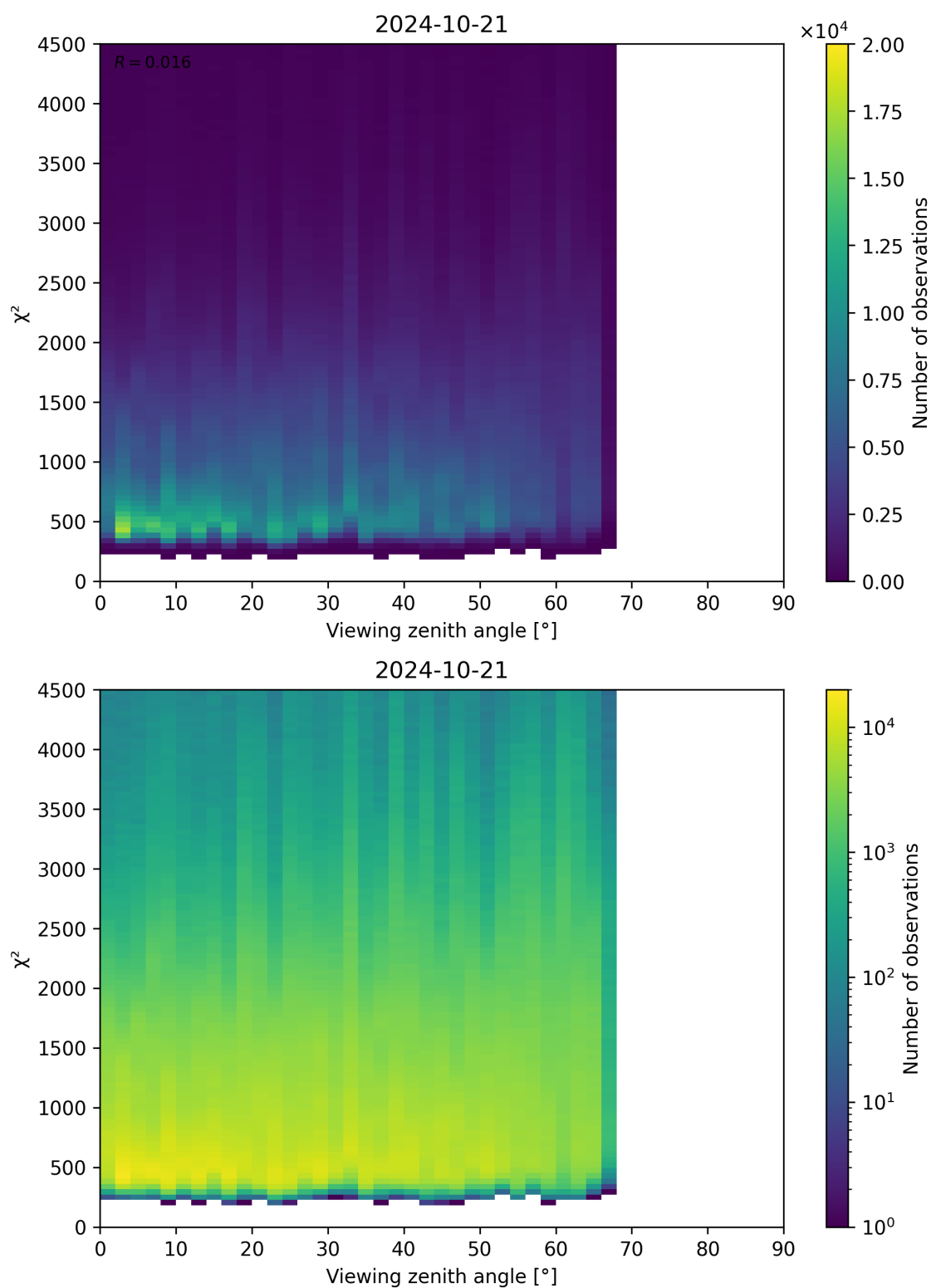
Figure 72: Scatter density plot of “Viewing zenith angle” against “ \chi^2 ” for 2024-10-20 to 2024-10-22.
