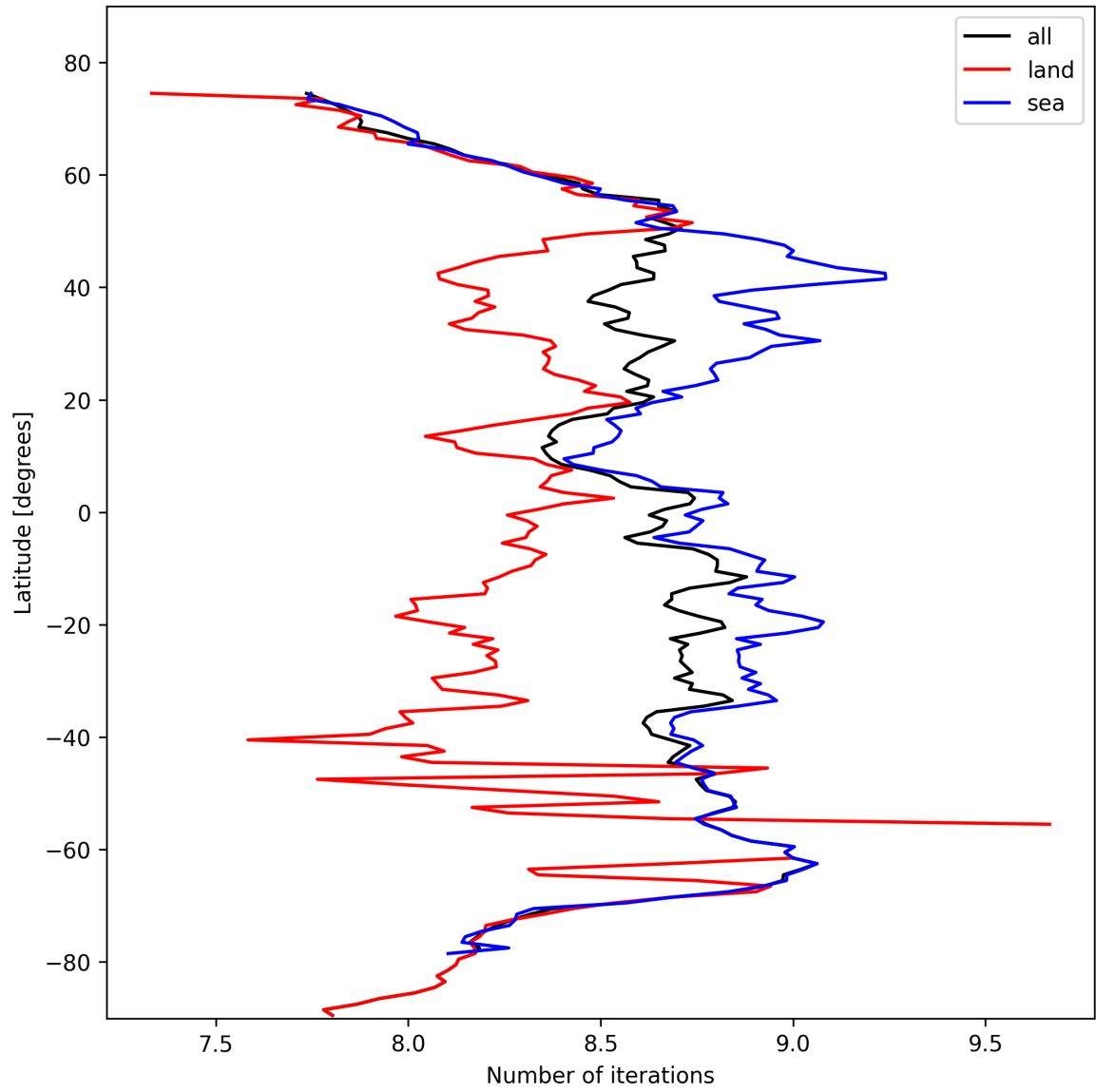
Figure 16: Zonal average of “Number of iterations” for 2024-10-20 to 2024-10-22.
