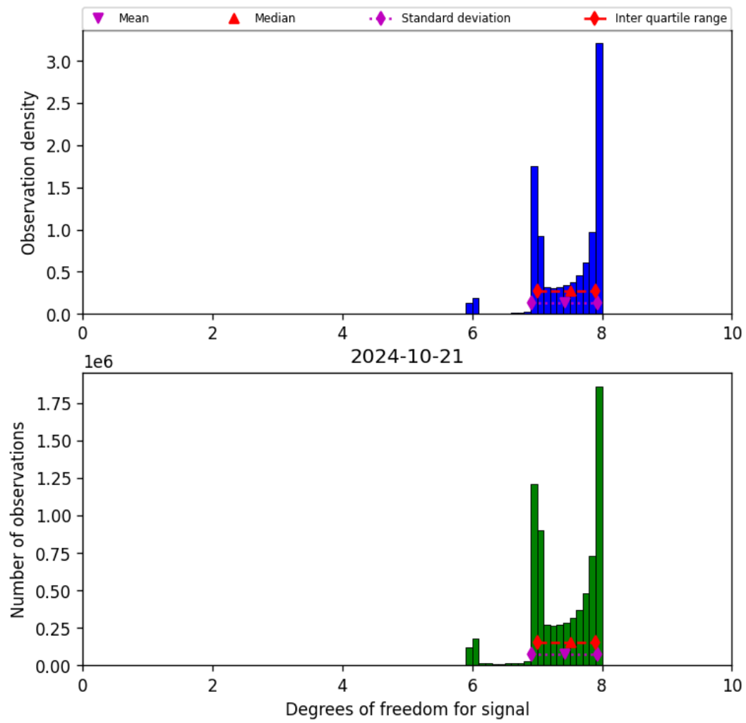
Figure 23: Histogram of “Degrees of freedom for signal” for 2024-10-20 to 2024-10-22
