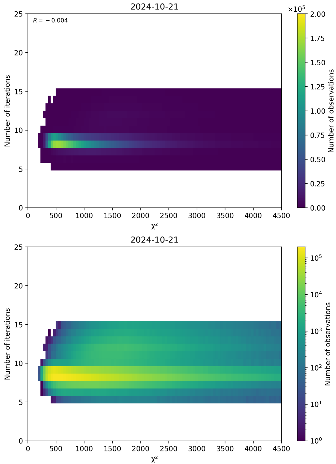
Figure 49: Scatter density plot of “ \chi^2 ” against “Number of iterations” for 2024-10-20 to 2024-10-22.
