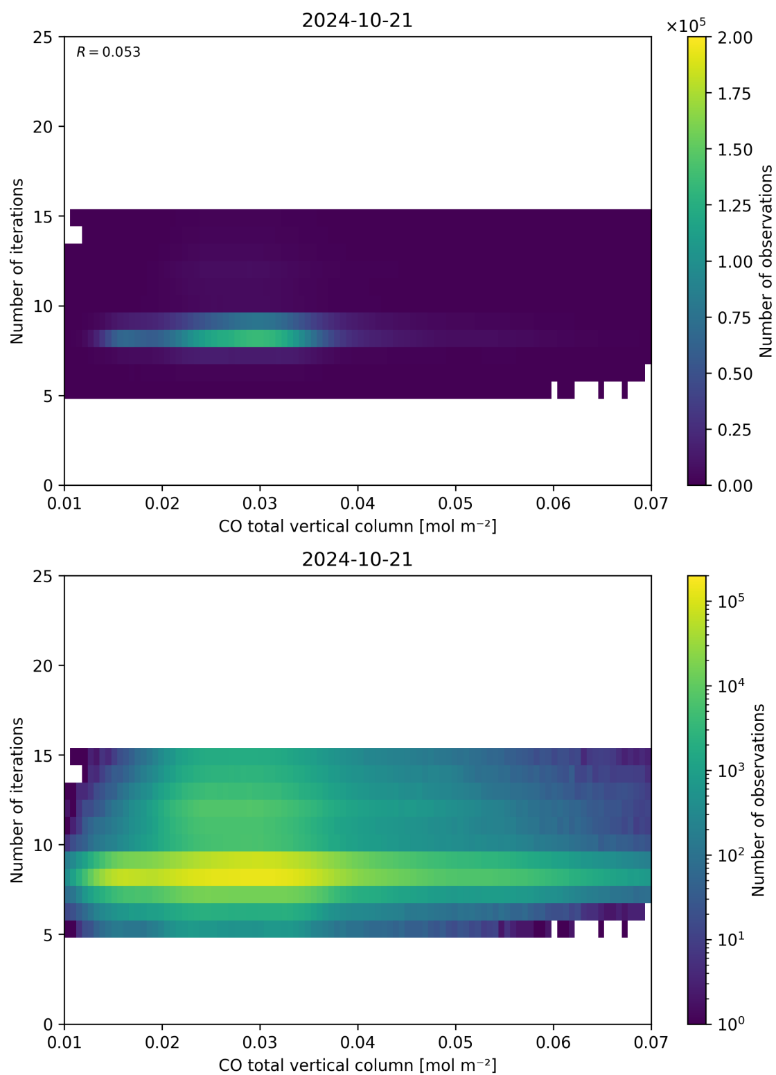
Figure 42: Scatter density plot of “CO total vertical column” against “Number of iterations” for 2024-10-20 to 2024-10-22.
