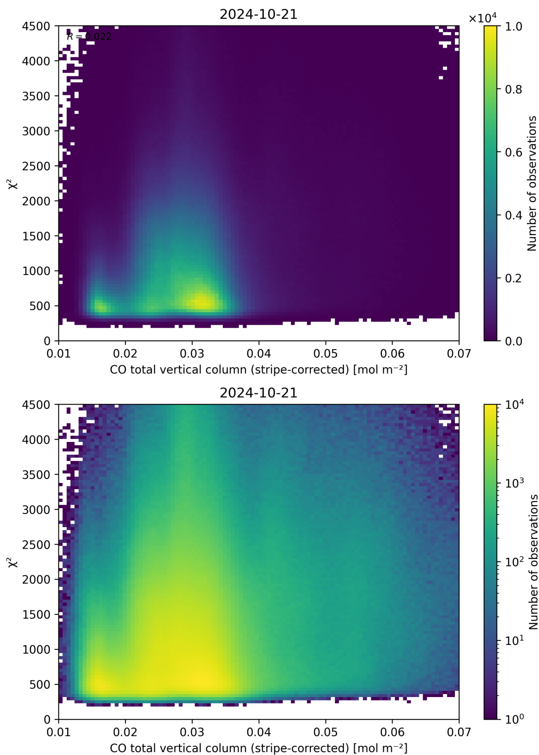
Figure 37: Scatter density plot of “CO total vertical column (stripe-corrected)” against “ \chi^2 ” for 2024-10-20 to 2024-10-22.
