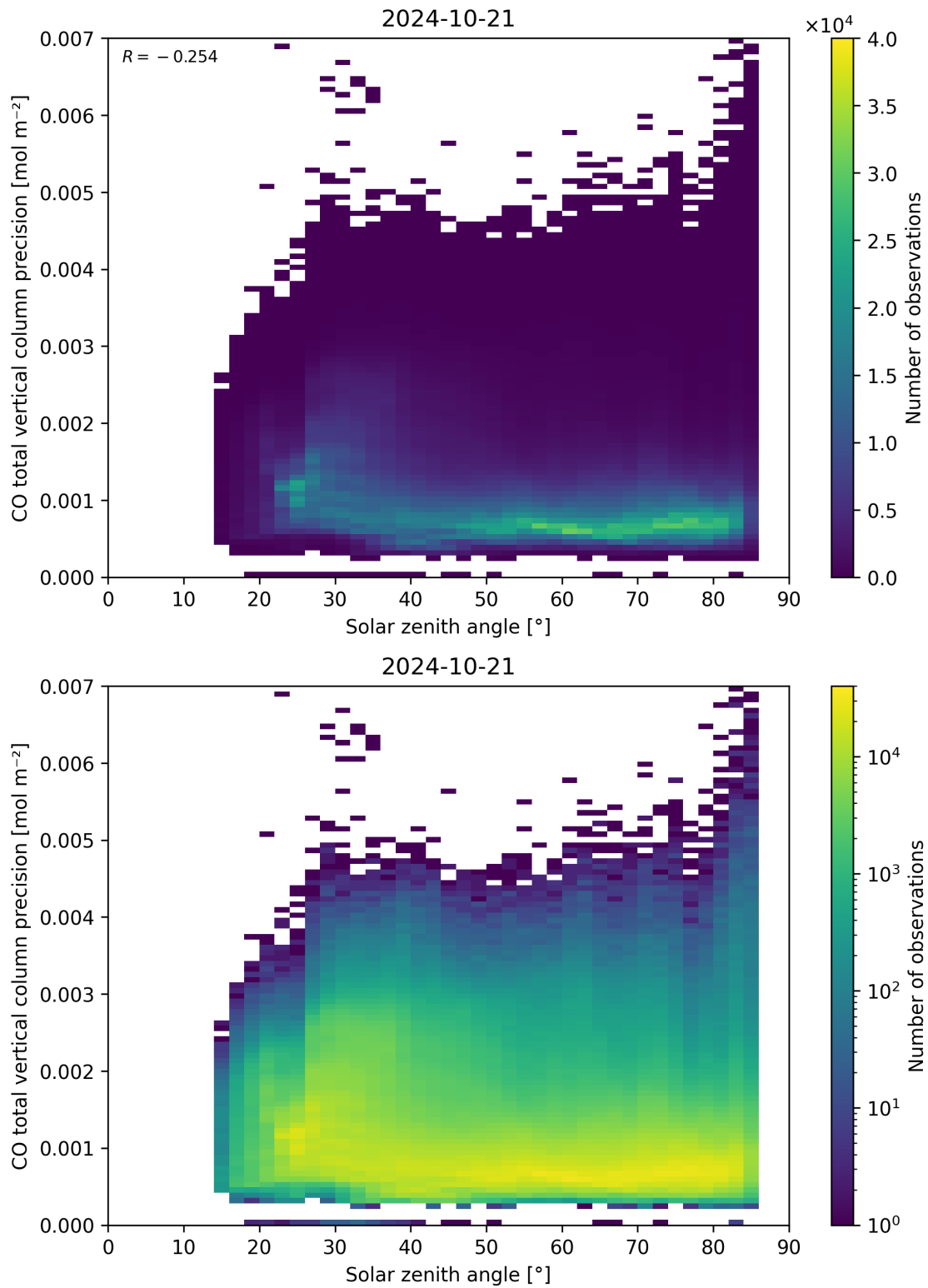
Figure 63: Scatter density plot of “Solar zenith angle” against “CO total vertical column precision” for 2024-10-20 to 2024-10-22.
