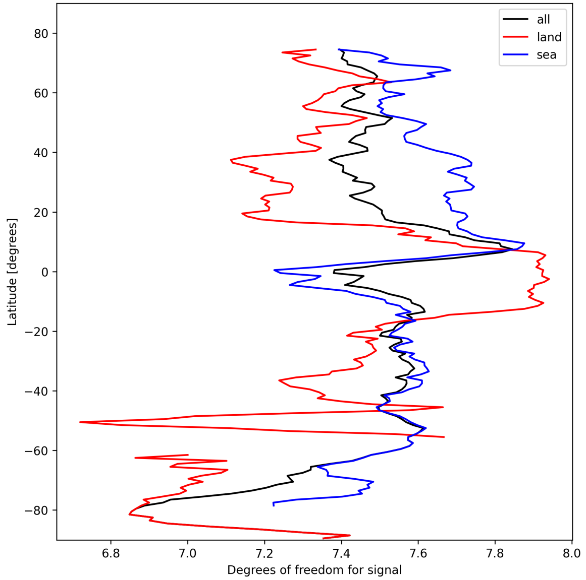
Figure 15: Zonal average of “Degrees of freedom for signal” for 2024-10-20 to 2024-10-22.
