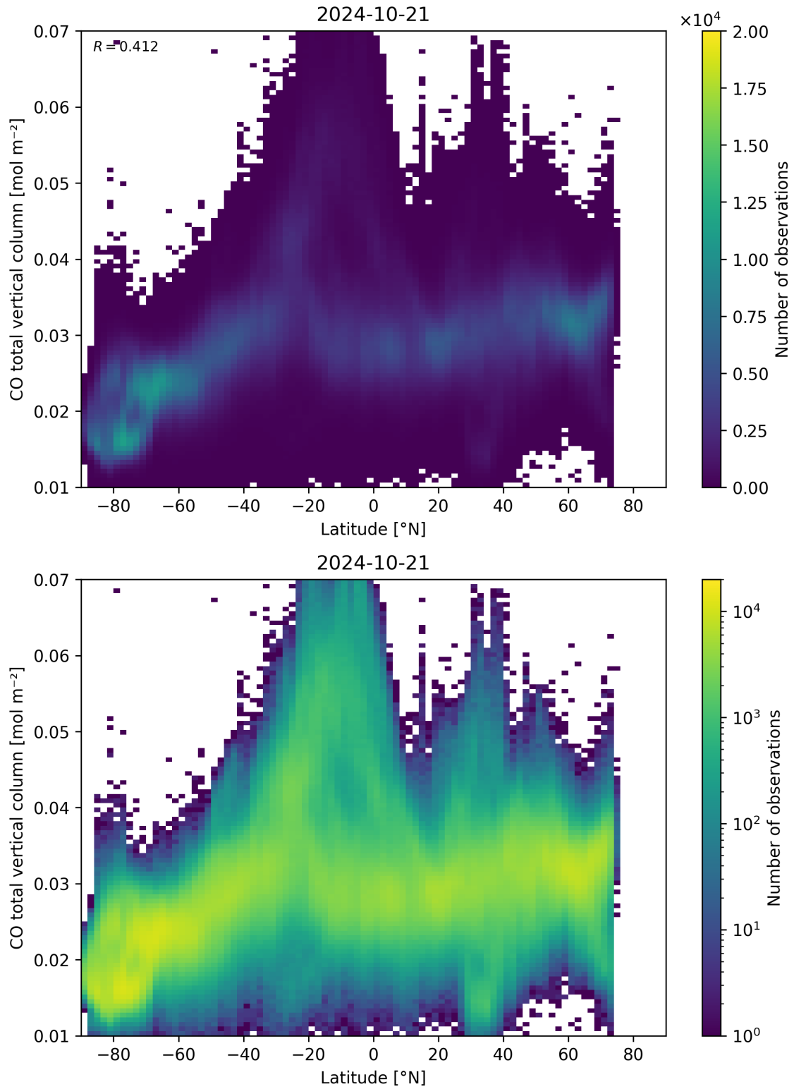
Figure 51: Scatter density plot of “Latitude” against “CO total vertical column” for 2024-10-20 to 2024-10-22.
