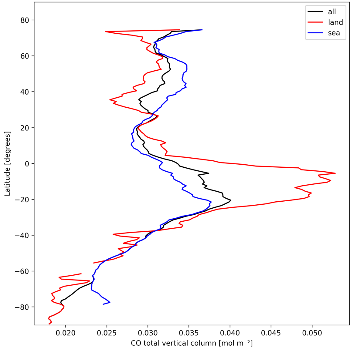
Figure 10: Zonal average of “CO total vertical column” for 2024-10-20 to 2024-10-22.
