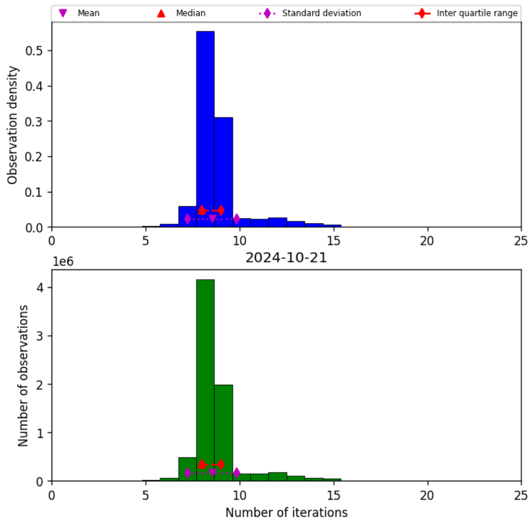
Figure 24: Histogram of “Number of iterations” for 2024-10-20 to 2024-10-22
