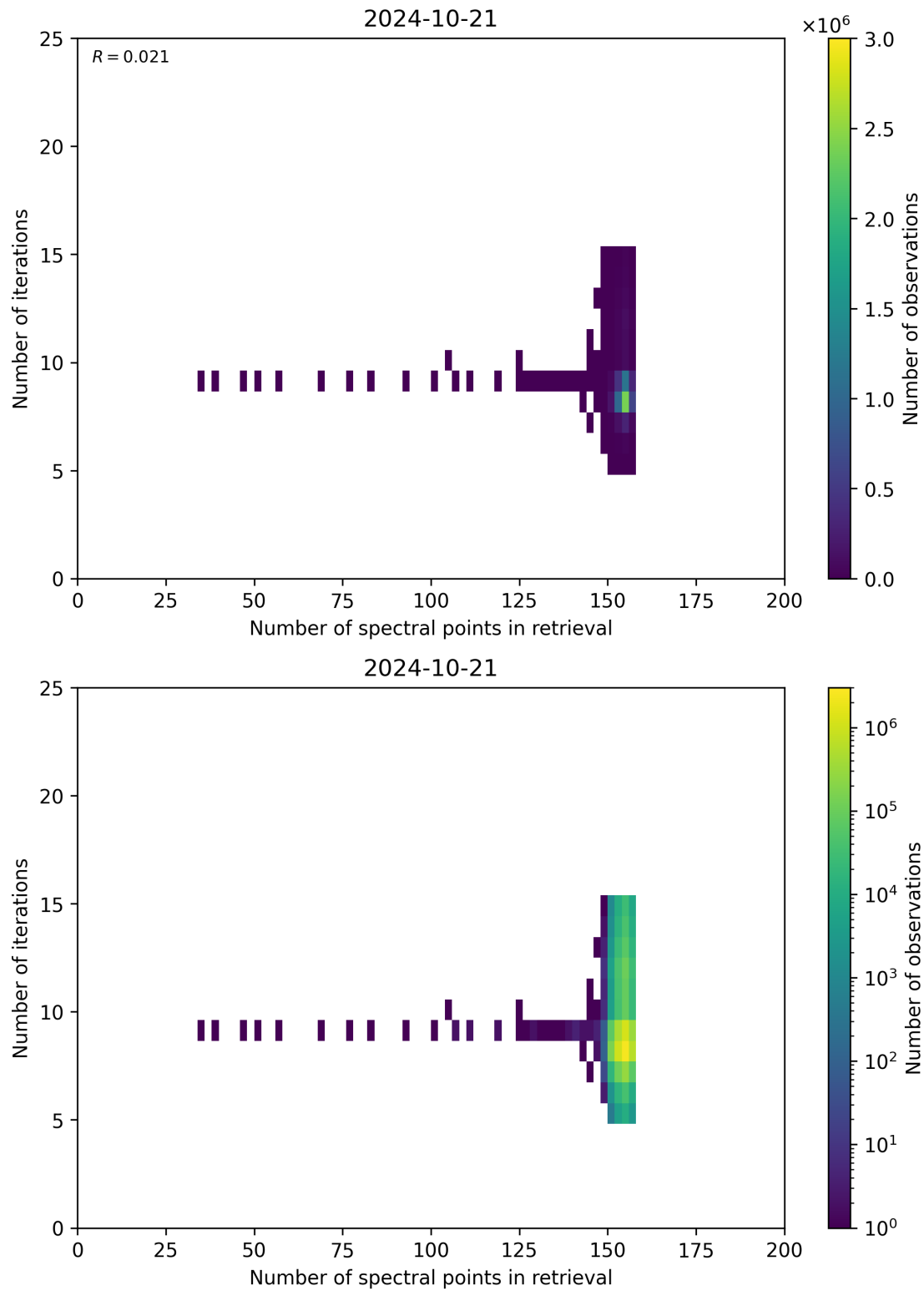
Figure 60: Scatter density plot of “Number of spectral points in retrieval” against “Number of iterations” for 2024-10-20 to 2024-10-22.
