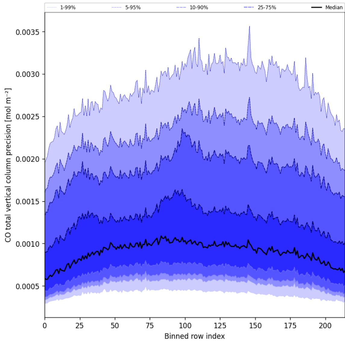
Figure 28: Along track statistics of “CO total vertical column precision” for 2024-10-20 to 2024-10-22
