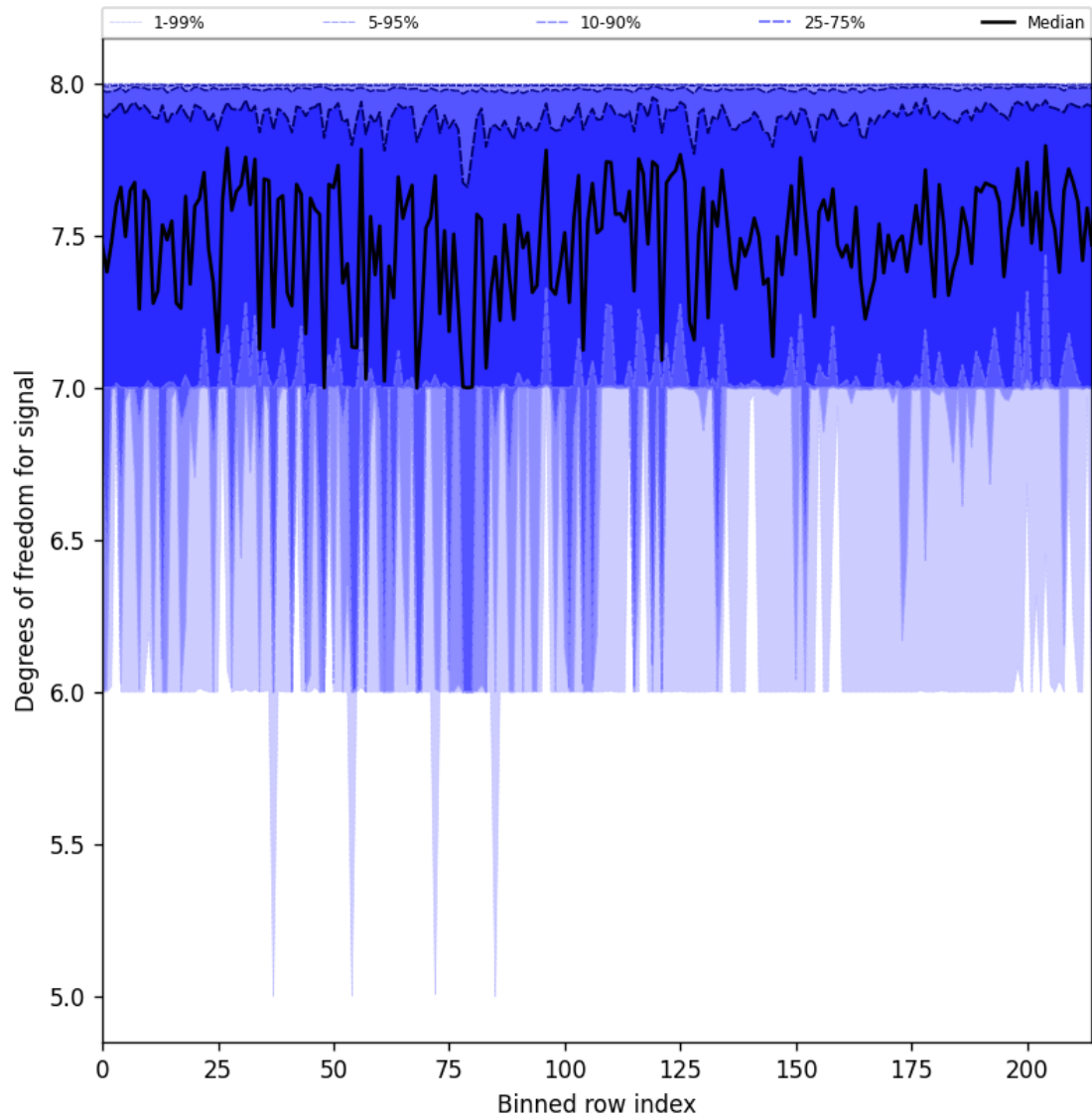
Figure 31: Along track statistics of “Degrees of freedom for signal” for 2024-10-20 to 2024-10-22
