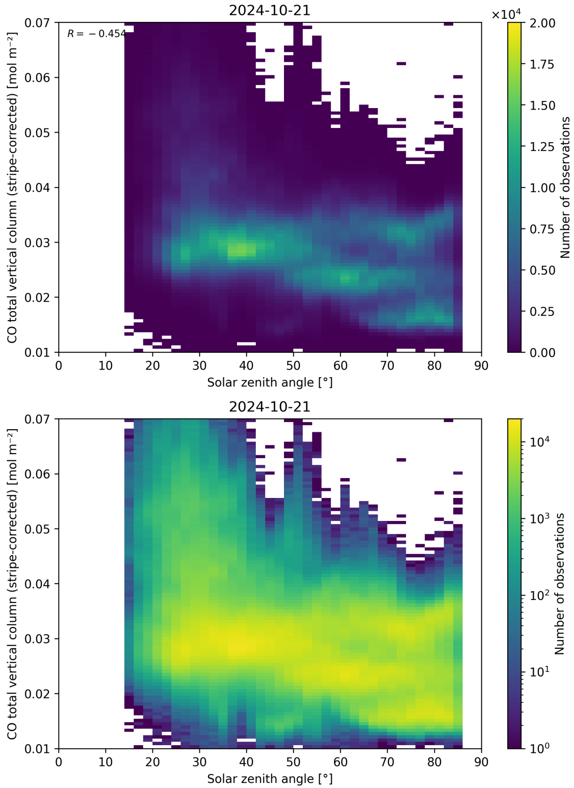
Figure 62: Scatter density plot of “Solar zenith angle” against “CO total vertical column (stripe-corrected)” for 2024-10-20 to 2024-10-22.
