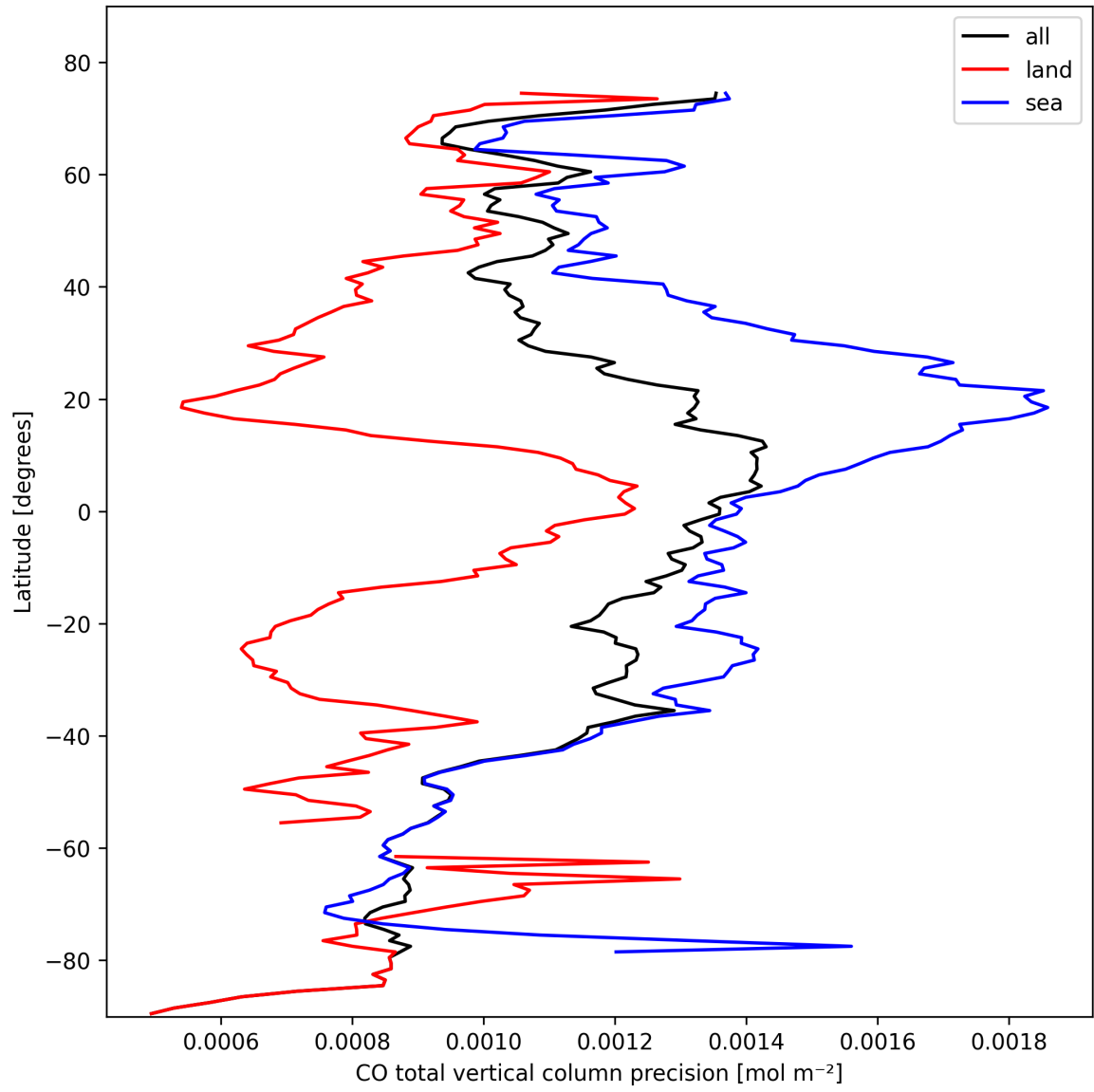
Figure 12: Zonal average of "CO total vertical column precision" for 2024-10-20 to 2024-10-22.
