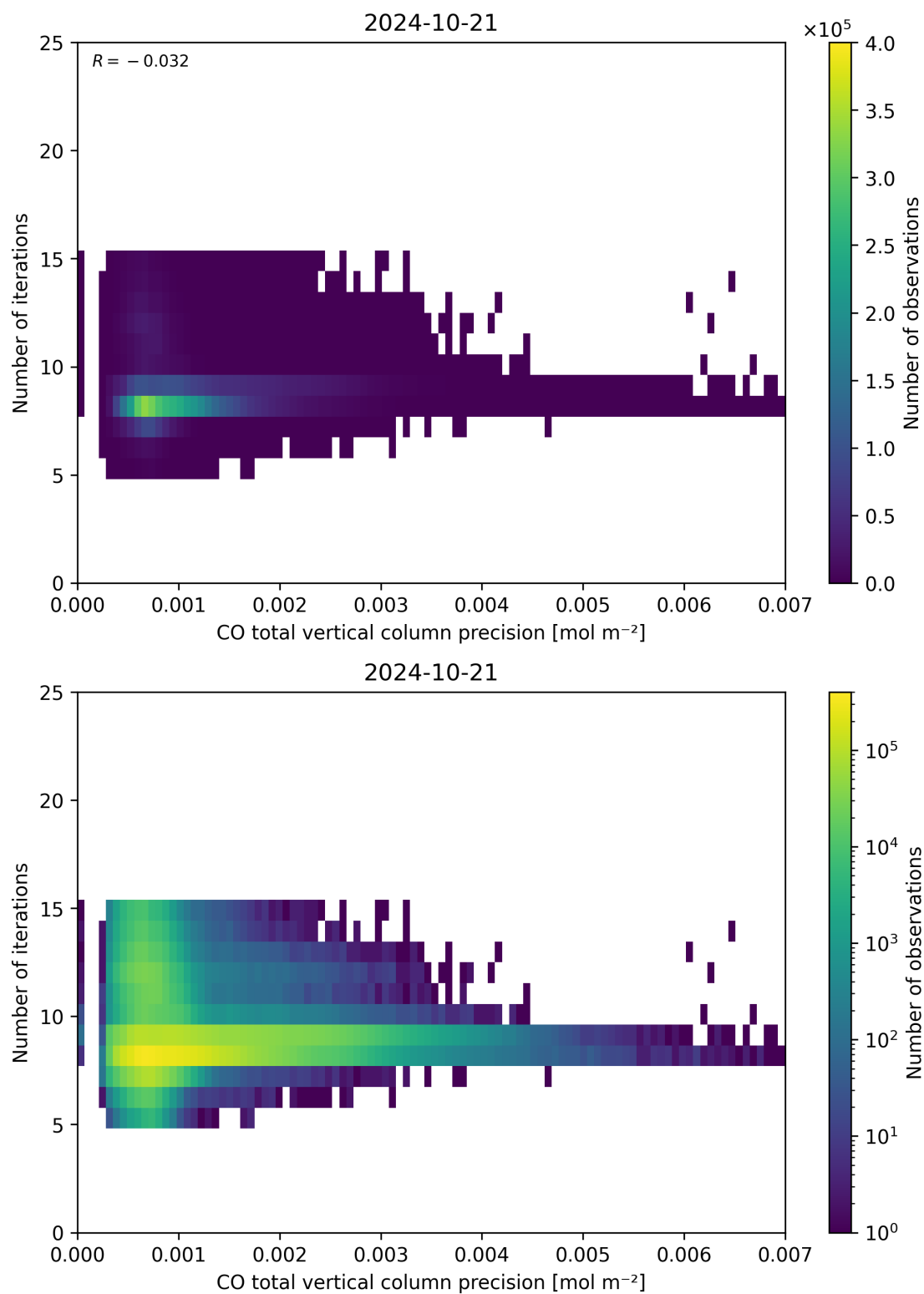
Figure 46: Scatter density plot of “CO total vertical column precision” against “Number of iterations” for 2024-10-20 to 2024-10-22.
