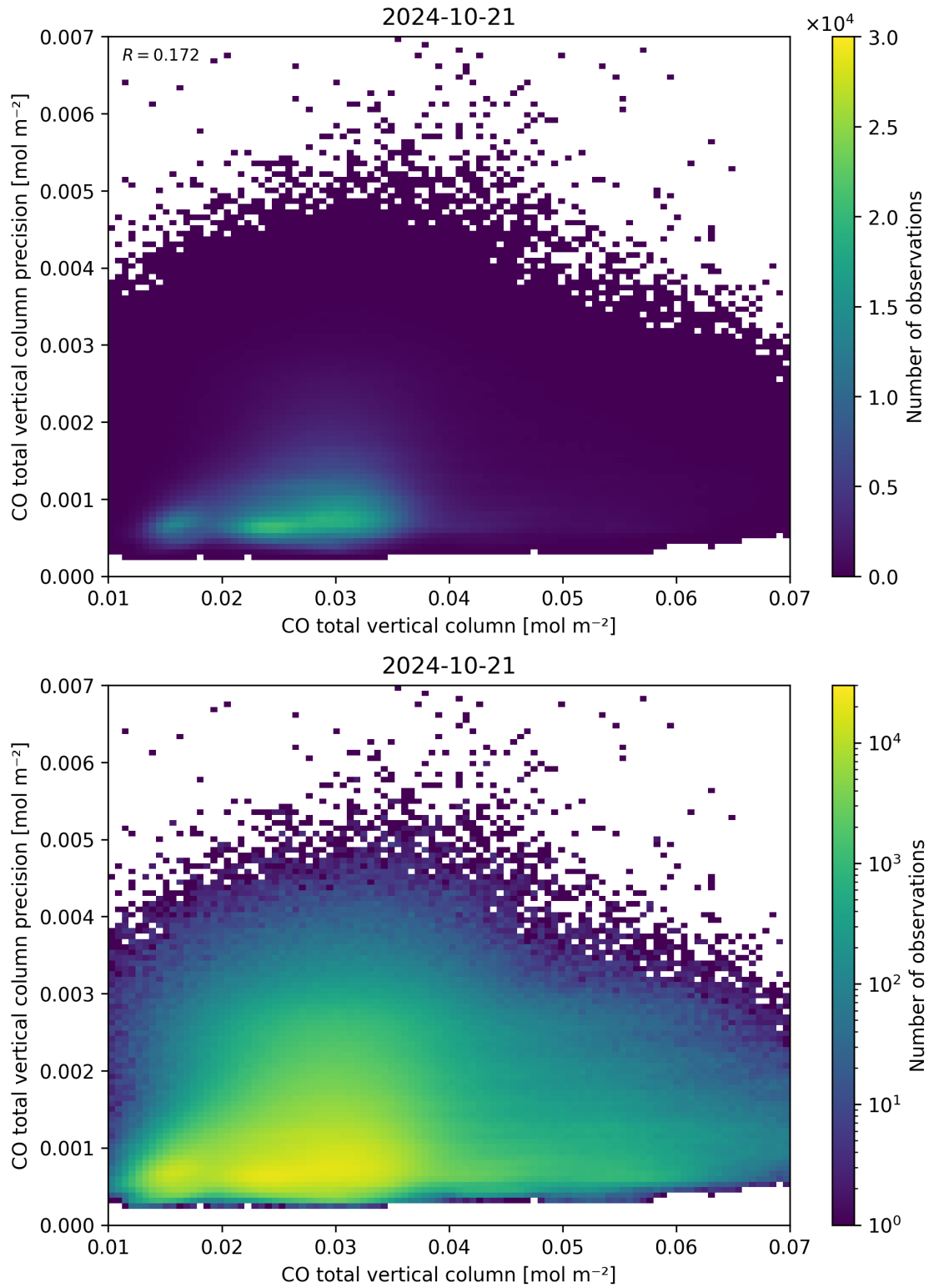
Figure 34: Scatter density plot of “CO total vertical column” against “CO total vertical column precision” for 2024-10-20 to 2024-10-22.
