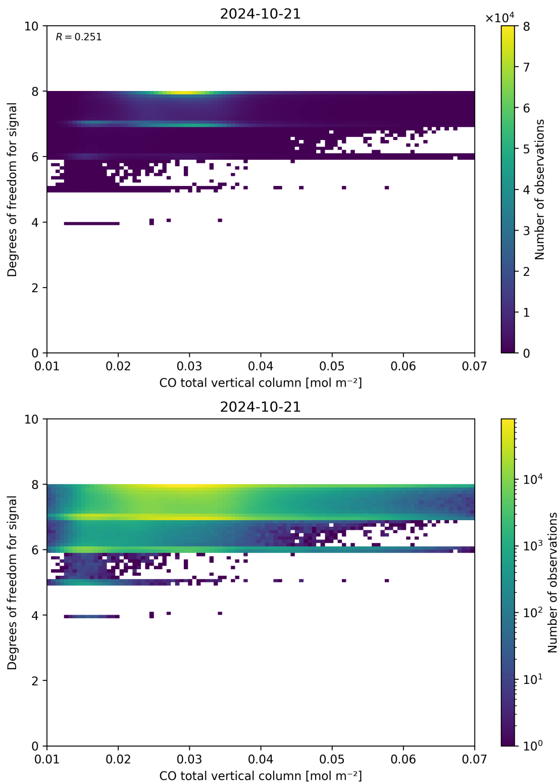
Figure 41: Scatter density plot of “CO total vertical column” against “Degrees of freedom for signal” for 2024-10-20 to 2024-10-22.
