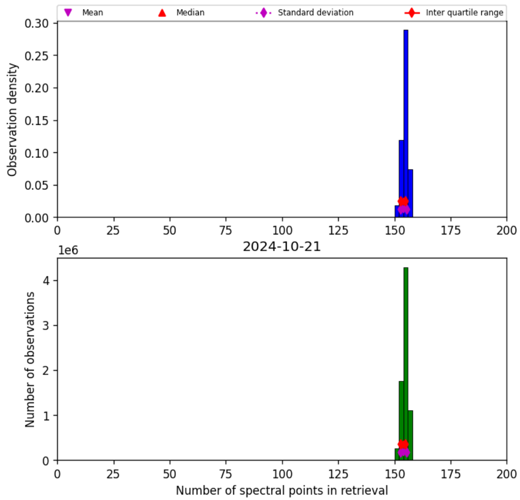
Figure 21: Histogram of “Number of spectral points in retrieval” for 2024-10-20 to 2024-10-22
