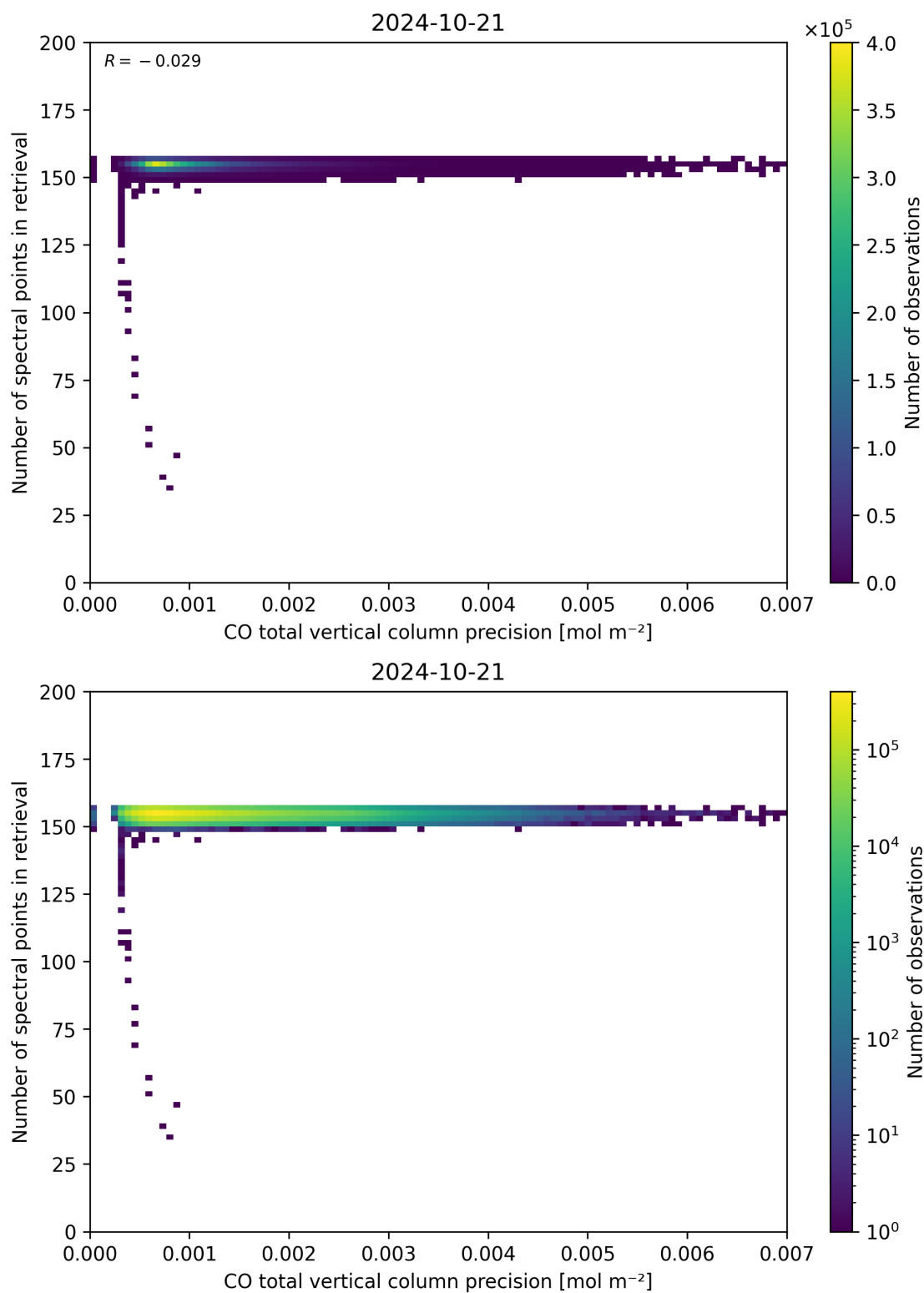
Figure 47: Scatter density plot of “CO total vertical column precision” against “Number of spectral points in retrieval” for 2024-10-20 to 2024-10-22.
