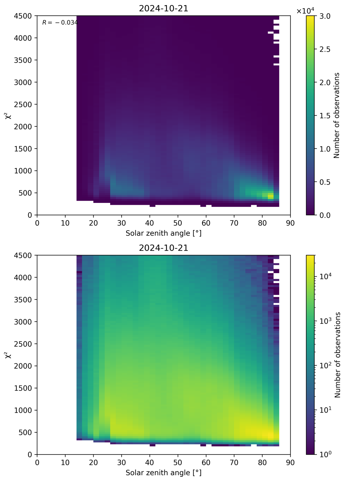
Figure 64: Scatter density plot of “Solar zenith angle” against “ \chi^2 ” for 2024-10-20 to 2024-10-22.
