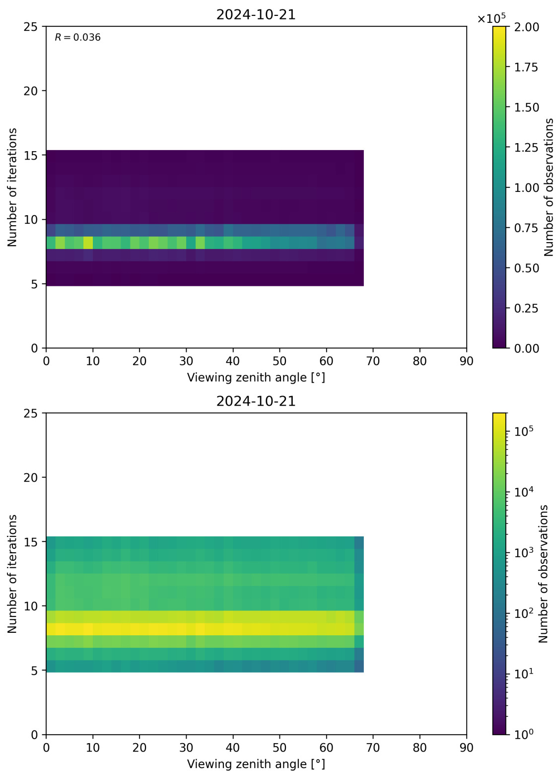
Figure 75: Scatter density plot of “Viewing zenith angle” against “Number of iterations” for 2024-10-20 to 2024-10-22.
