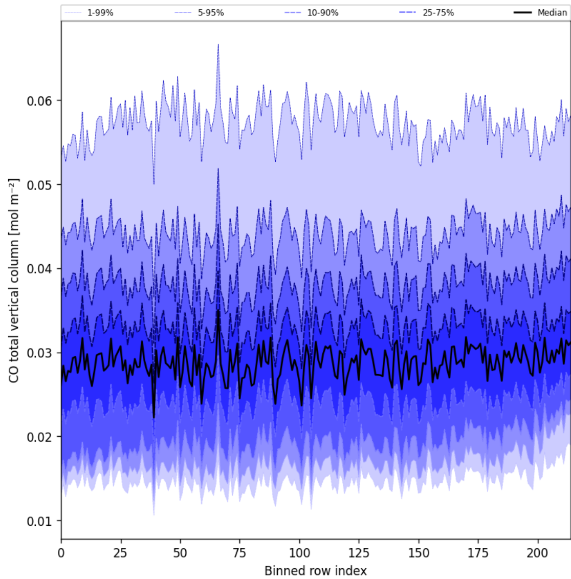
Figure 26: Along track statistics of “CO total vertical column” for 2024-10-20 to 2024-10-22
