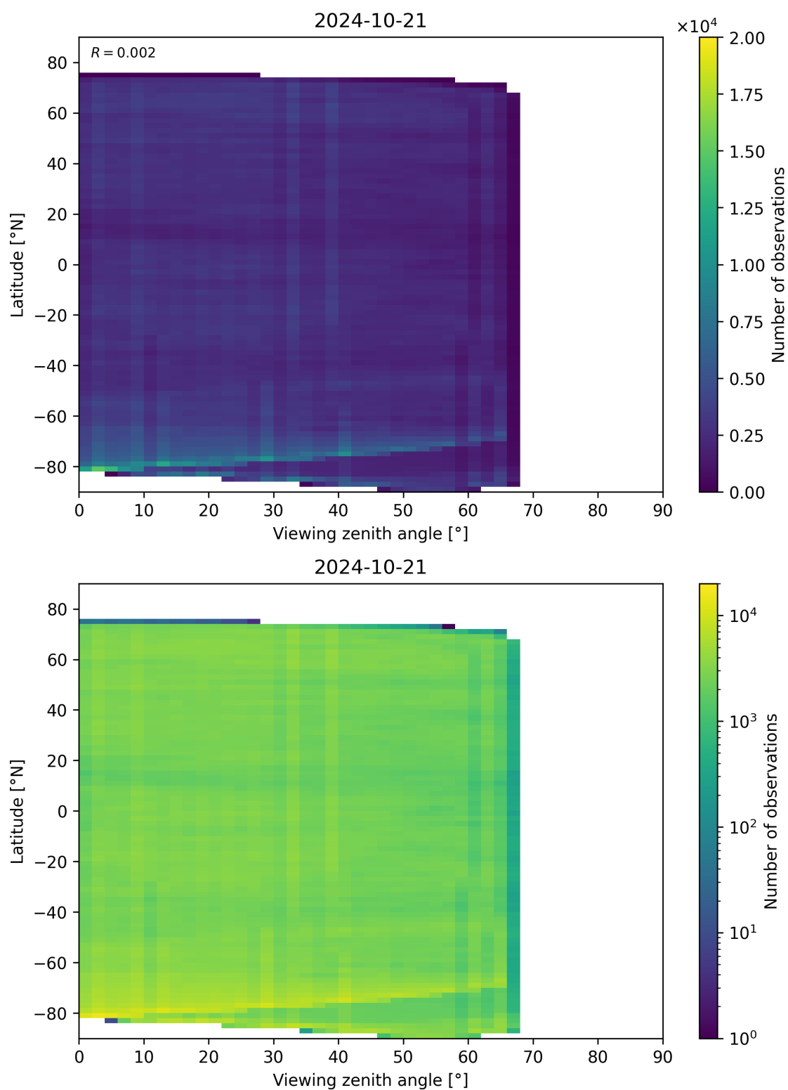
Figure 74: Scatter density plot of “Viewing zenith angle” against “Latitude” for 2024-10-20 to 2024-10-22.
