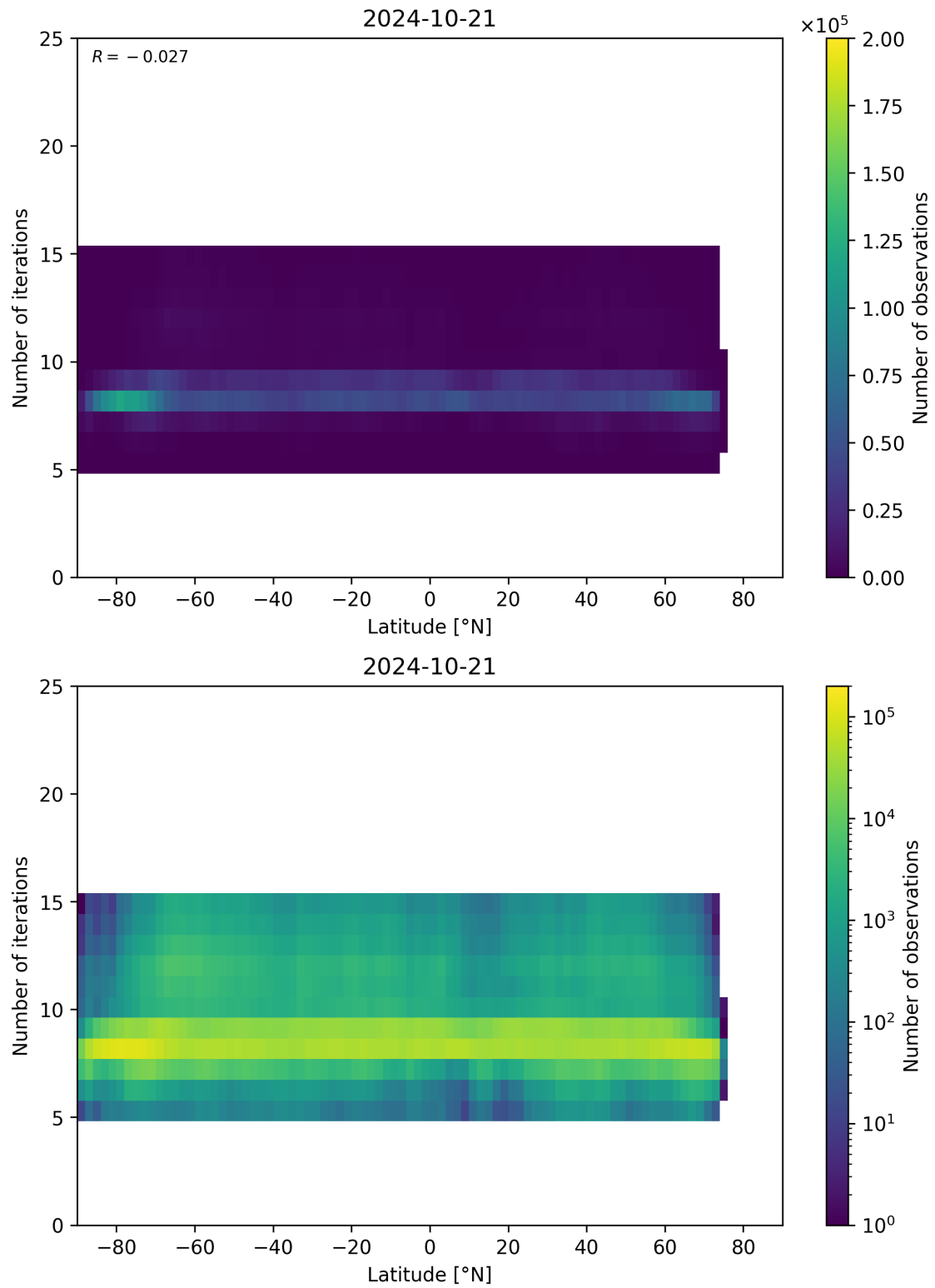
Figure 56: Scatter density plot of “Latitude” against “Number of iterations” for 2024-10-20 to 2024-10-22.
