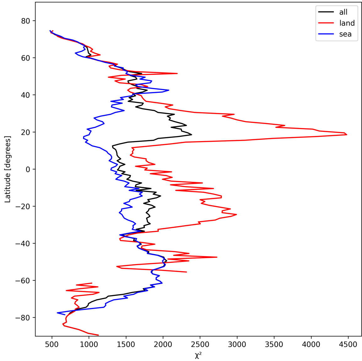
Figure 14: Zonal average of “ \chi^2 ” for 2024-10-20 to 2024-10-22.
