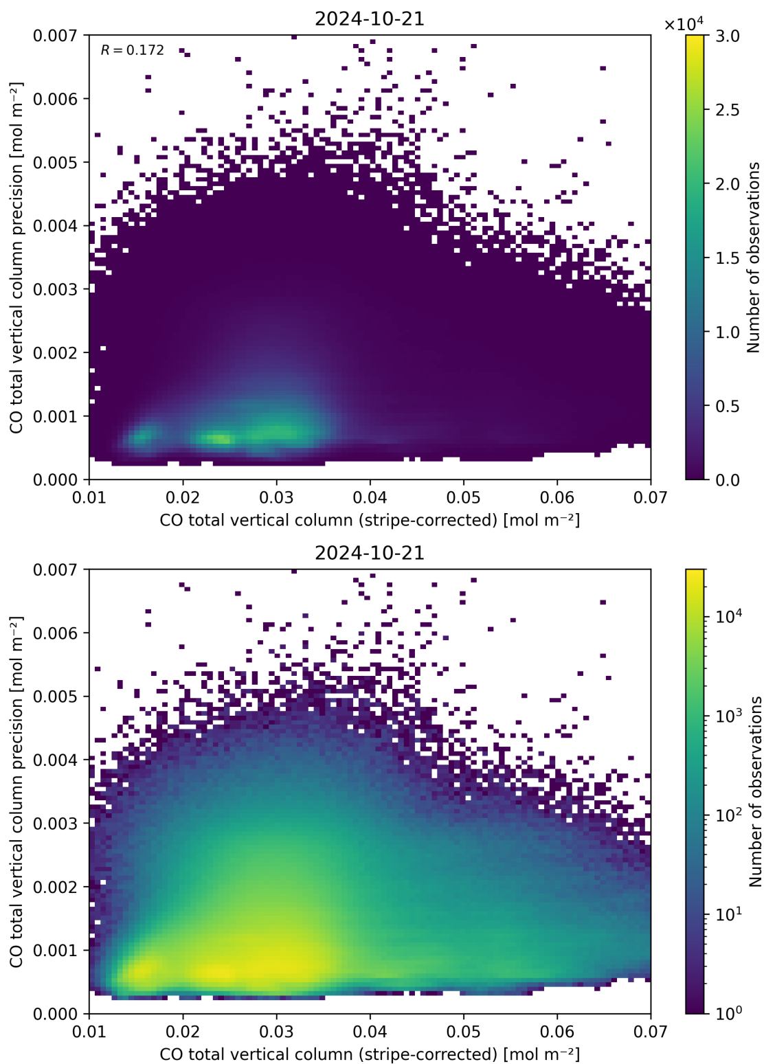
Figure 36: Scatter density plot of “CO total vertical column (stripe-corrected)” against “CO total vertical column precision” for 2024-10-20 to 2024-10-22.
