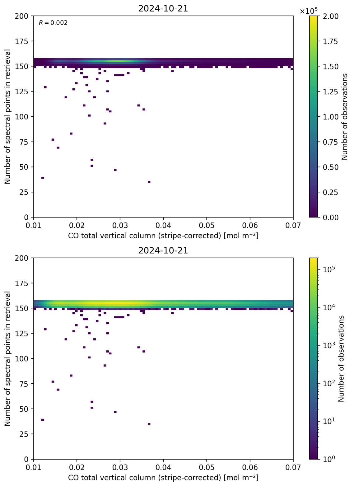
Figure 40: Scatter density plot of “CO total vertical column (stripe-corrected)” against “Number of spectral points in retrieval” for 2024-10-20 to 2024-10-22.
