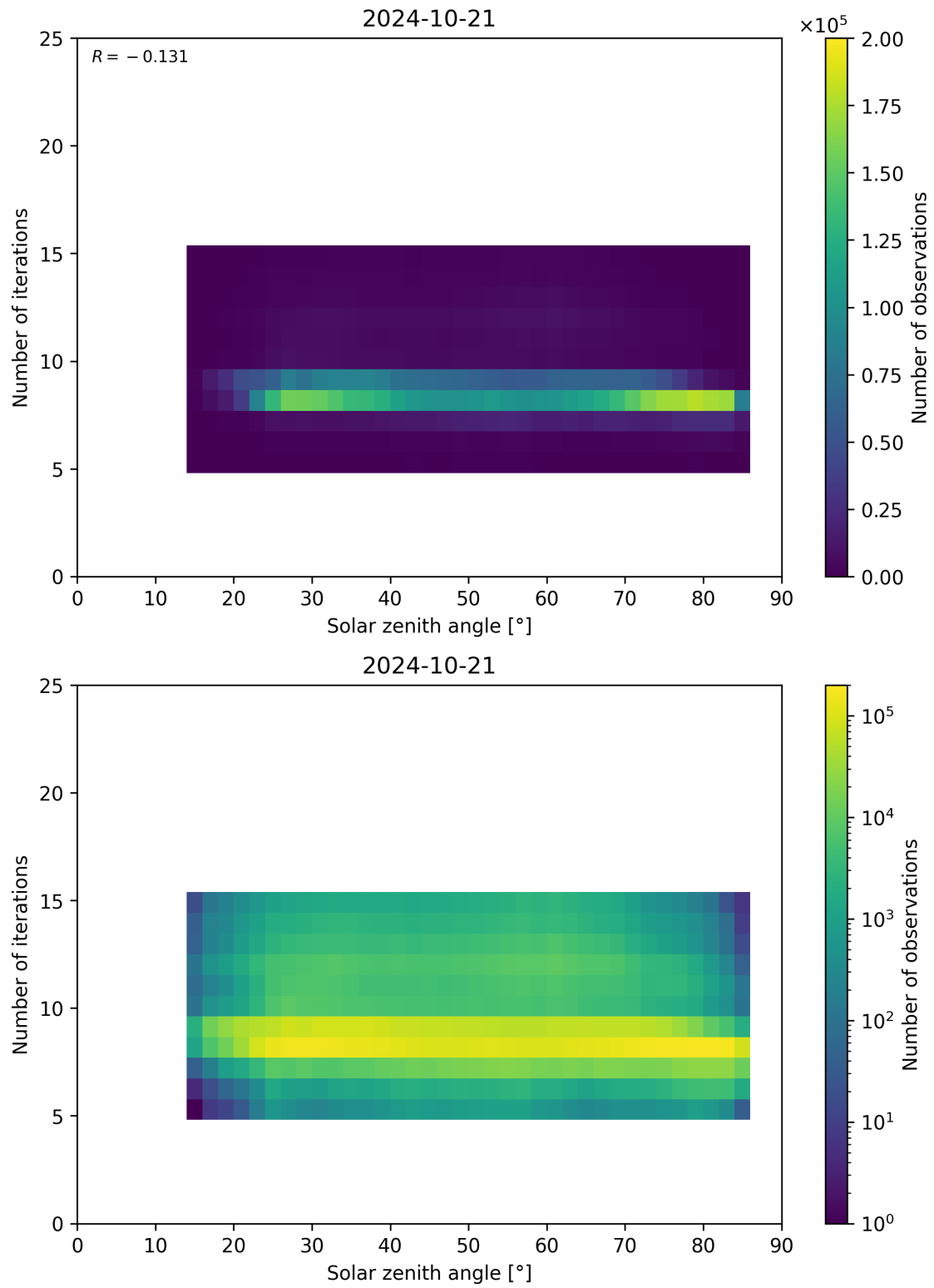
Figure 67: Scatter density plot of “Solar zenith angle” against “Number of iterations” for 2024-10-20 to 2024-10-22.
