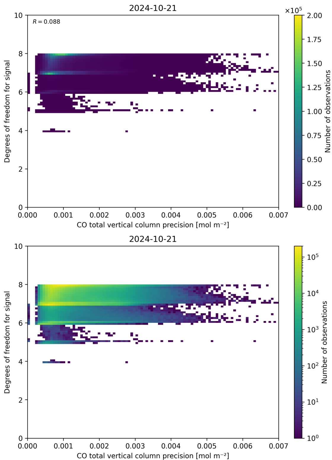
Figure 45: Scatter density plot of “CO total vertical column precision” against “Degrees of freedom for signal” for 2024-10-20 to 2024-10-22.
