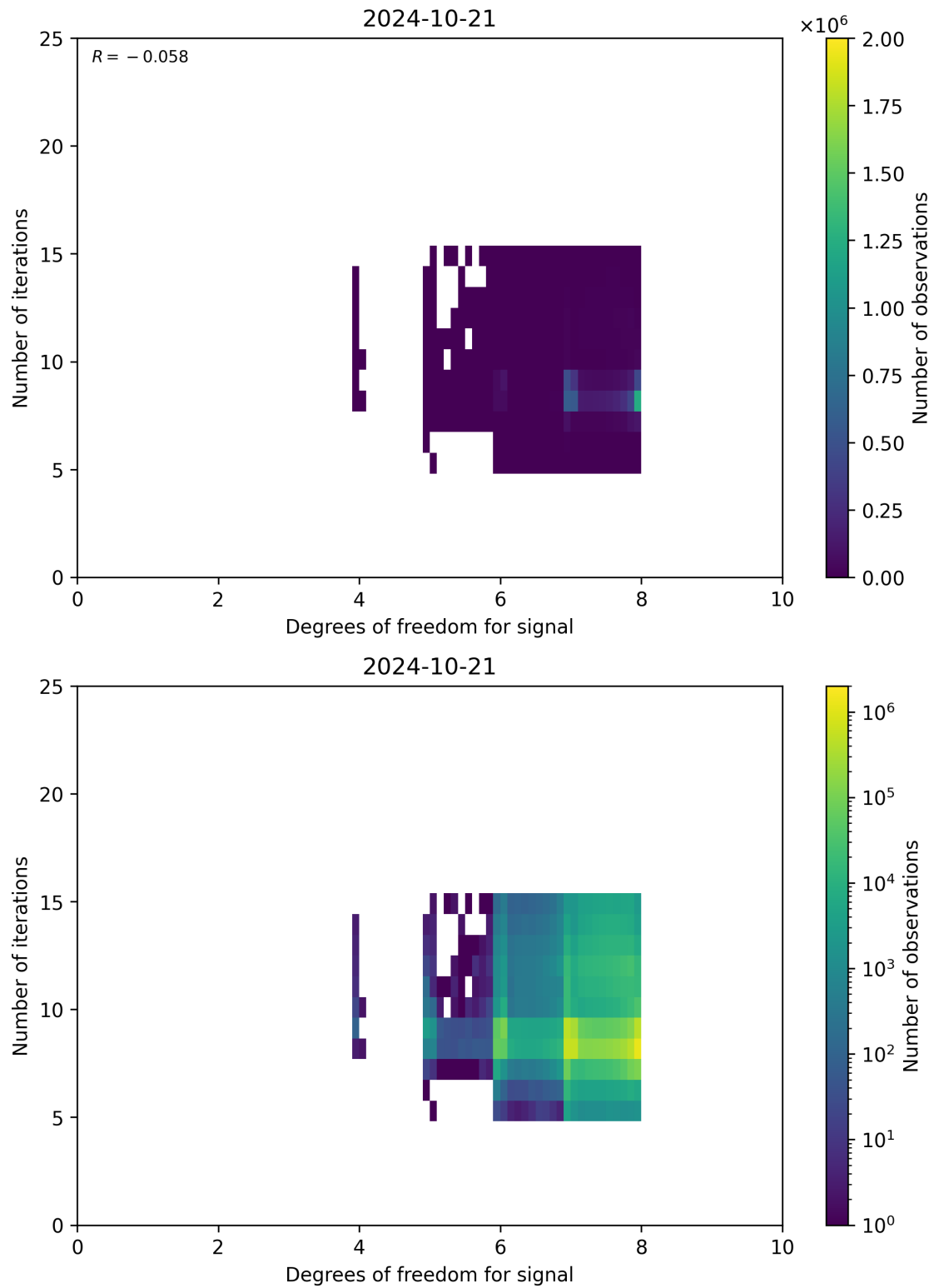
Figure 50: Scatter density plot of “Degrees of freedom for signal” against “Number of iterations” for 2024-10-20 to 2024-10-22.
