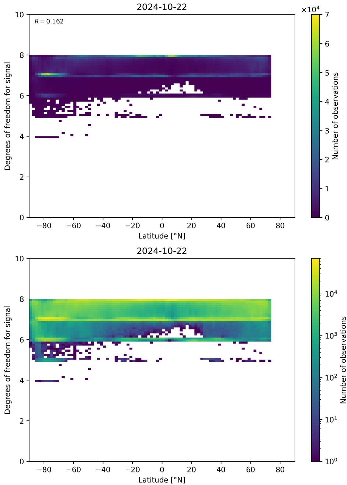
Figure 55: Scatter density plot of “Latitude” against “Degrees of freedom for signal” for 2024-10-21 to 2024-10-23.
