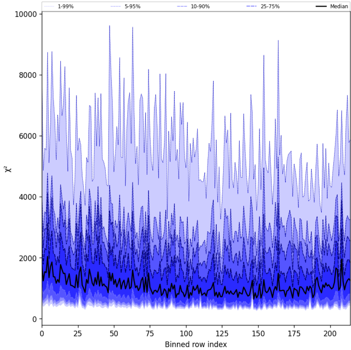
Figure 30: Along track statistics of “ \chi^2 ” for 2024-10-21 to 2024-10-23
