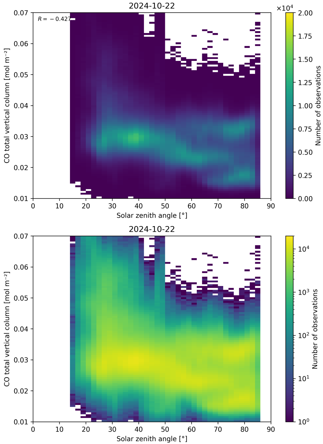
Figure 61: Scatter density plot of “Solar zenith angle” against “CO total vertical column” for 2024-10-21 to 2024-10-23.
