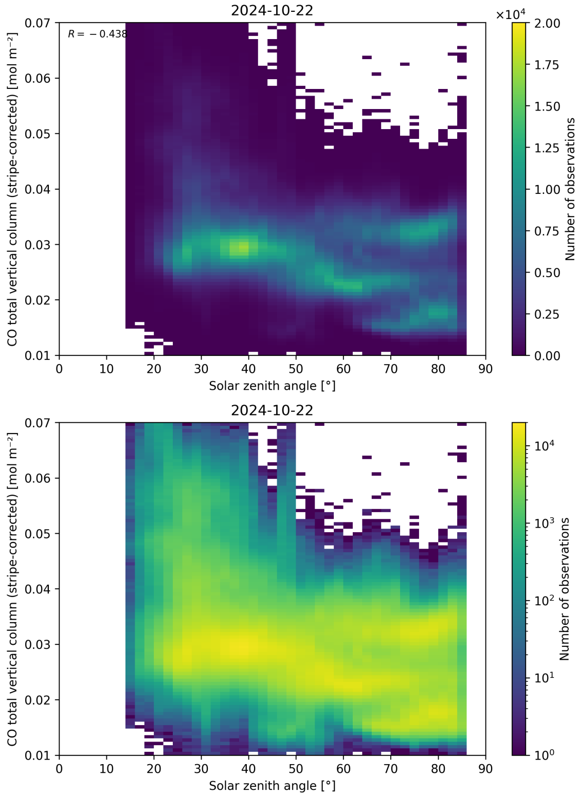
Figure 62: Scatter density plot of “Solar zenith angle” against “CO total vertical column (stripe-corrected)” for 2024-10-21 to 2024-10-23.
