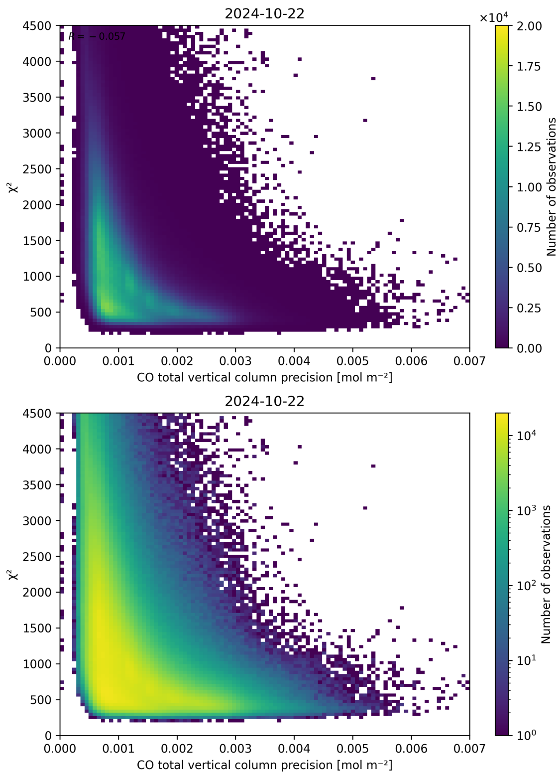
Figure 44: Scatter density plot of “CO total vertical column precision” against “ \chi^2 ” for 2024-10-21 to 2024-10-23.
