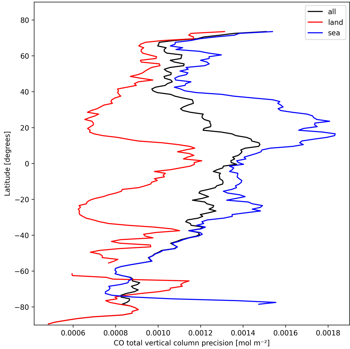
Figure 12: Zonal average of “CO total vertical column precision” for 2024-10-21 to 2024-10-23.
