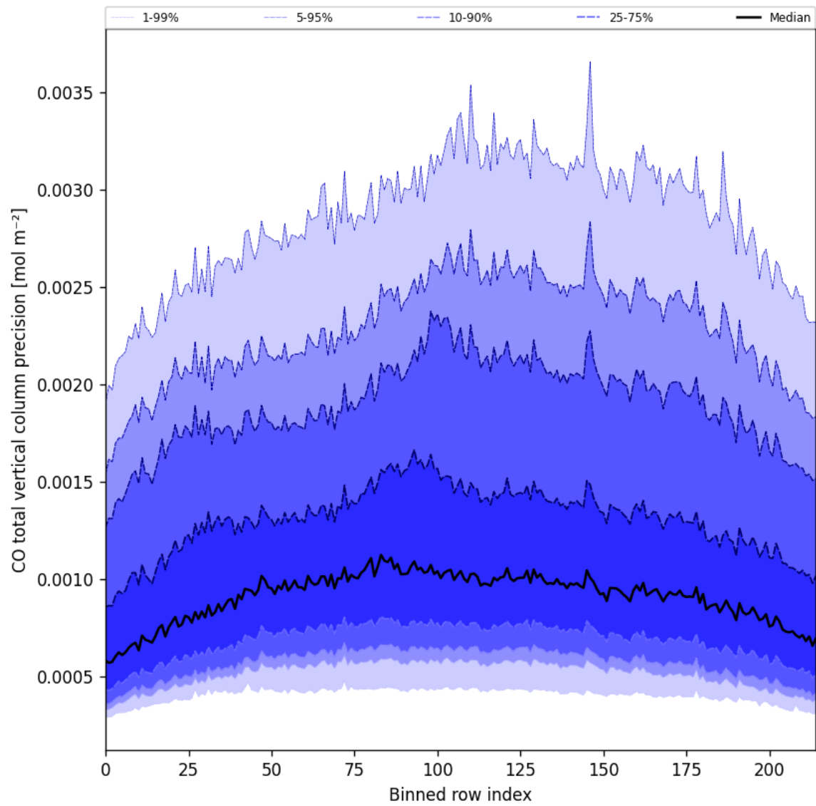
Figure 28: Along track statistics of “CO total vertical column precision” for 2024-10-21 to 2024-10-23
