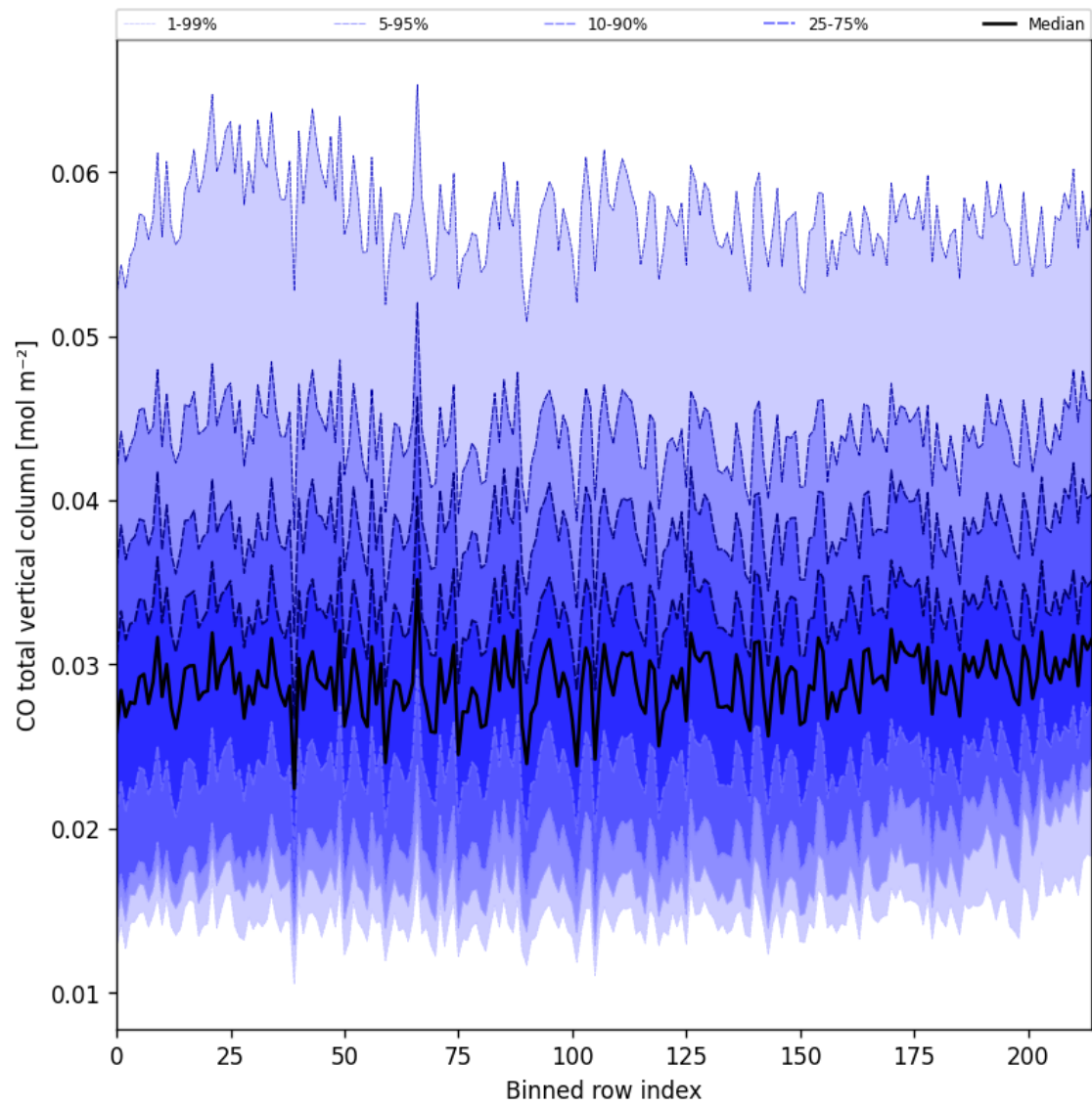
Figure 26: Along track statistics of “CO total vertical column” for 2024-10-21 to 2024-10-23
