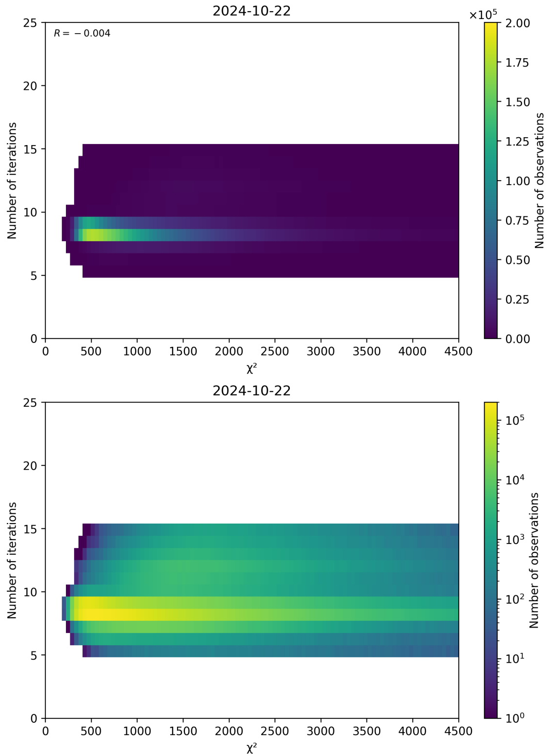
Figure 49: Scatter density plot of “ \chi^2 ” against “Number of iterations” for 2024-10-21 to 2024-10-23.
