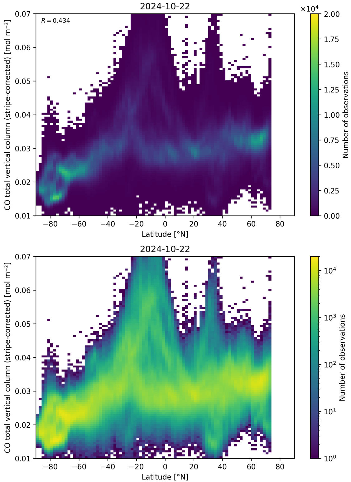
Figure 52: Scatter density plot of “Latitude” against “CO total vertical column (stripe-corrected)” for 2024-10-21 to 2024-10-23.
