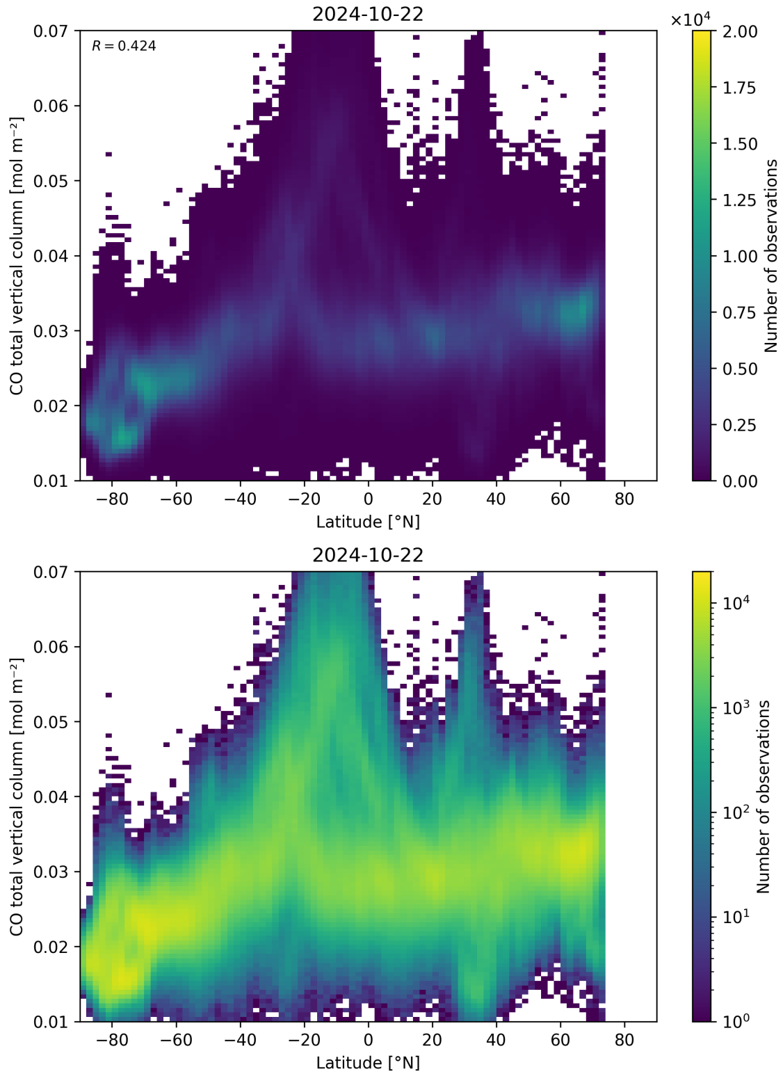
Figure 51: Scatter density plot of “Latitude” against “CO total vertical column” for 2024-10-21 to 2024-10-23.
