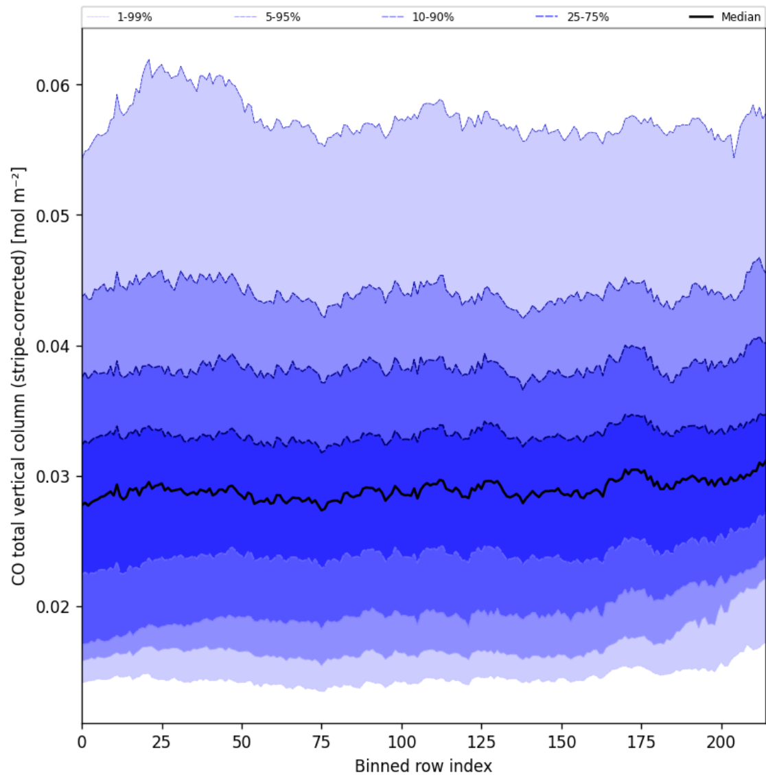
Figure 27: Along track statistics of “CO total vertical column (stripe-corrected)” for 2024-10-21 to 2024-10-23
