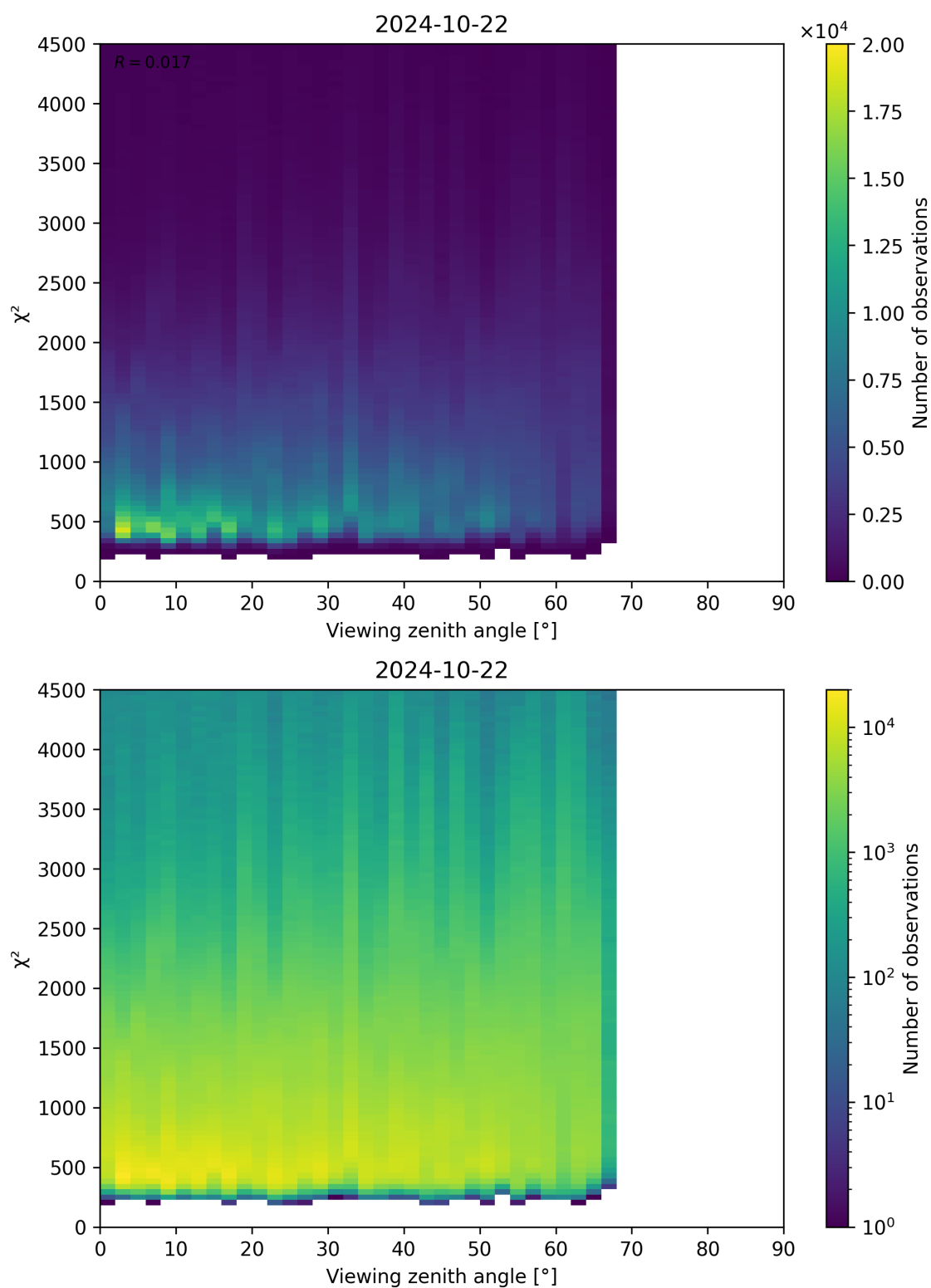
Figure 72: Scatter density plot of “Viewing zenith angle” against “ \chi^2 ” for 2024-10-21 to 2024-10-23.
