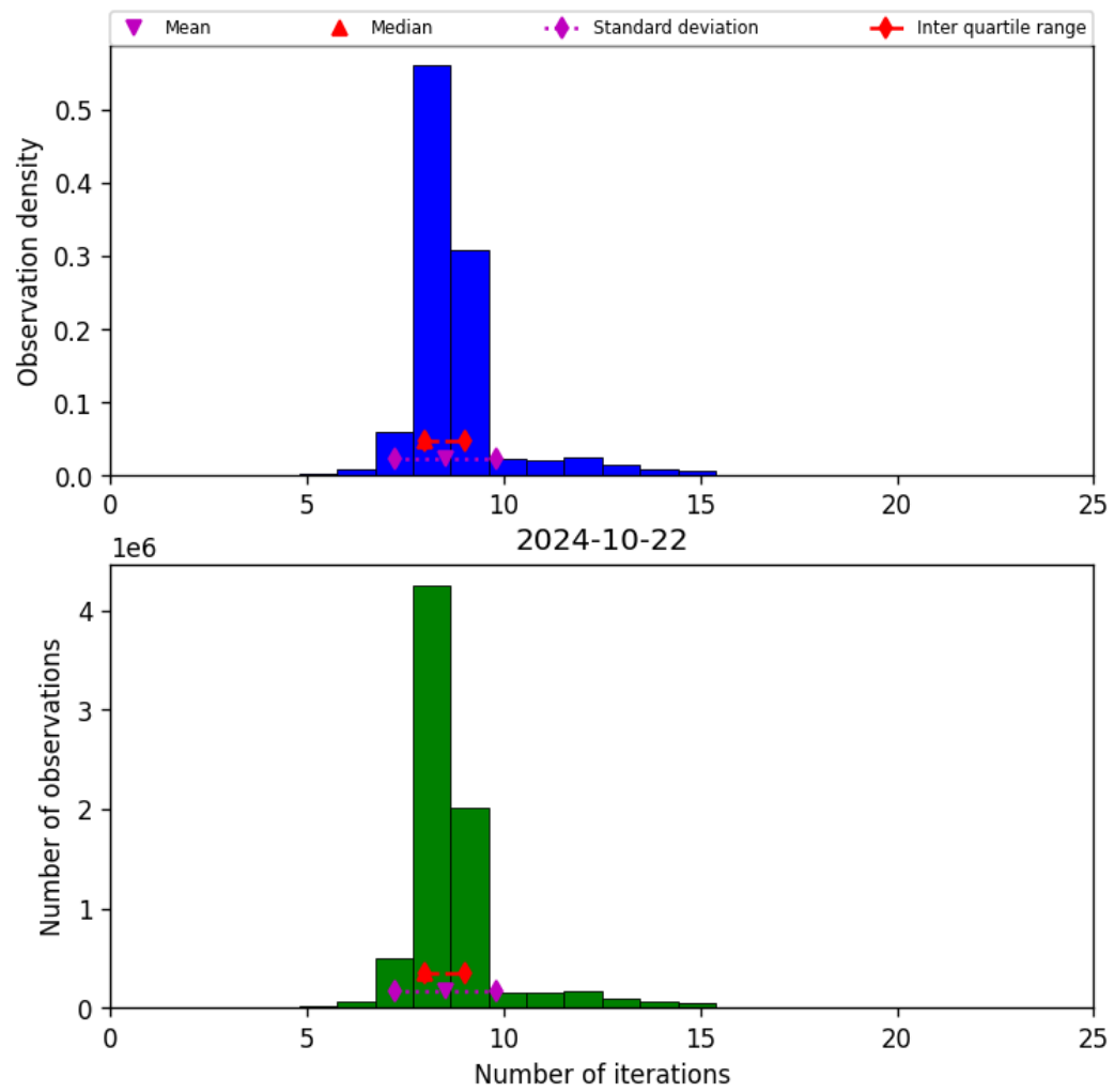
Figure 24: Histogram of “Number of iterations” for 2024-10-21 to 2024-10-23
