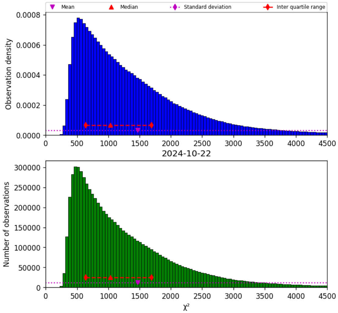
Figure 22: Histogram of “ \chi^2 ” for 2024-10-21 to 2024-10-23
