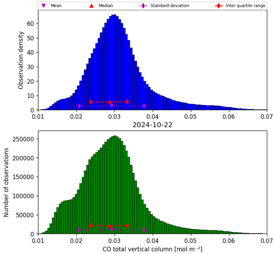
Figure 18: Histogram of “CO total vertical column” for 2024-10-21 to 2024-10-23
