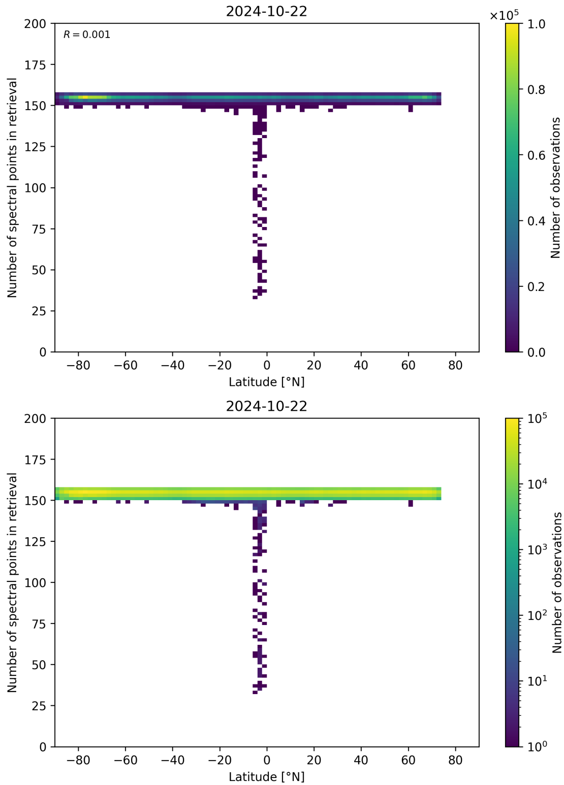
Figure 57: Scatter density plot of “Latitude” against “Number of spectral points in retrieval” for 2024-10-21 to 2024-10-23.
