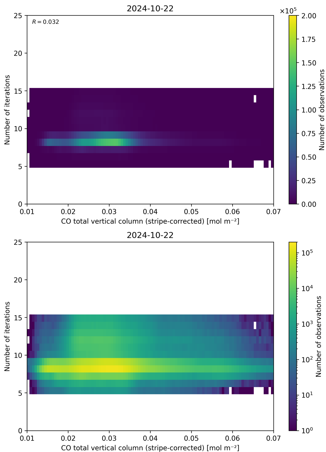
Figure 39: Scatter density plot of “CO total vertical column (stripe-corrected)” against “Number of iterations” for 2024-10-21 to 2024-10-23.
