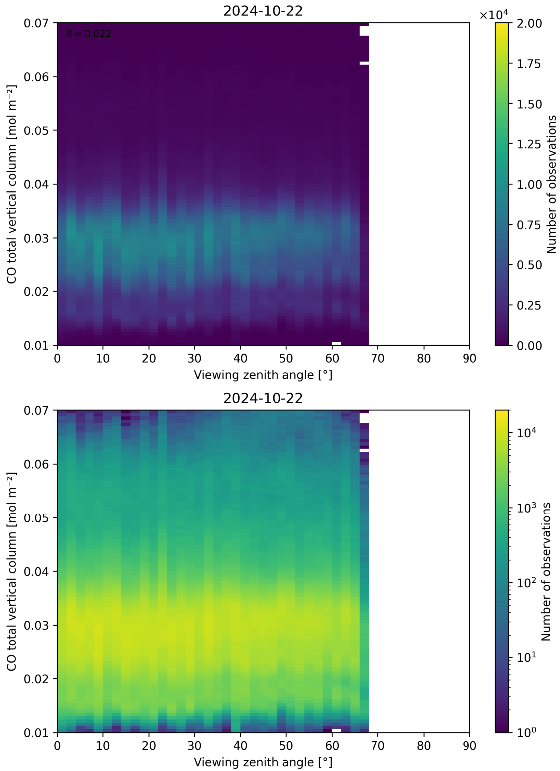
Figure 69: Scatter density plot of “Viewing zenith angle” against “CO total vertical column” for 2024-10-21 to 2024-10-23.
