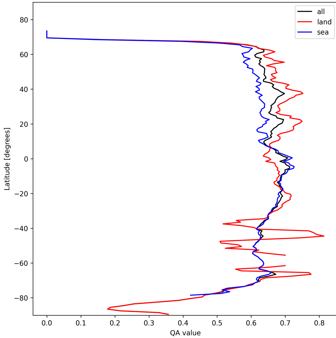
Figure 9: Zonal average of “QA value” for 2024-10-21 to 2024-10-23.
