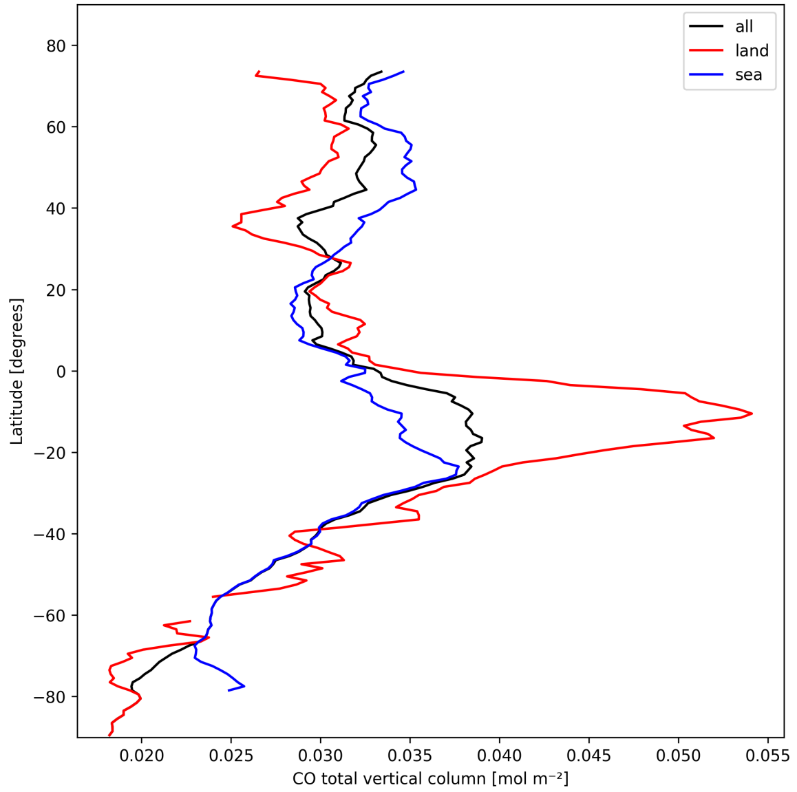
Figure 10: Zonal average of “CO total vertical column” for 2024-10-21 to 2024-10-23.
