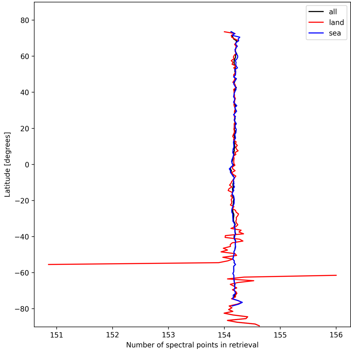
Figure 13: Zonal average of “Number of spectral points in retrieval” for 2024-10-21 to 2024-10-23.
