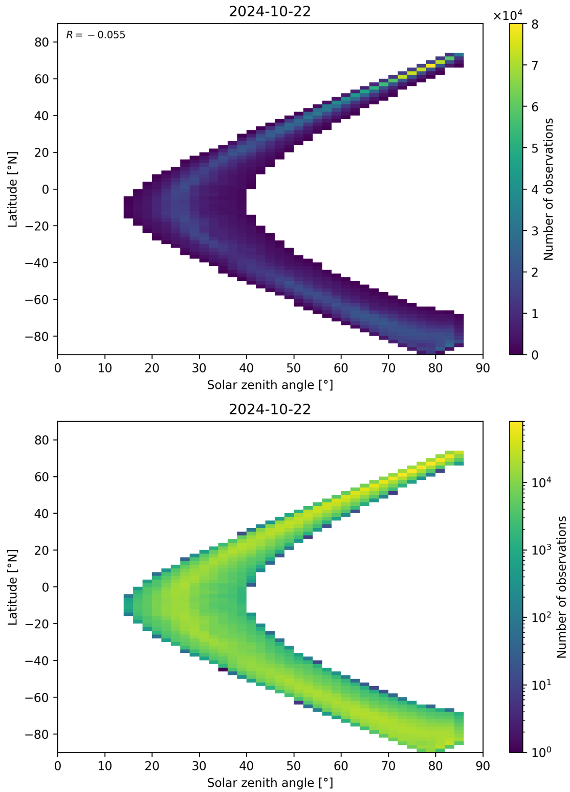
Figure 66: Scatter density plot of “Solar zenith angle” against “Latitude” for 2024-10-21 to 2024-10-23.
