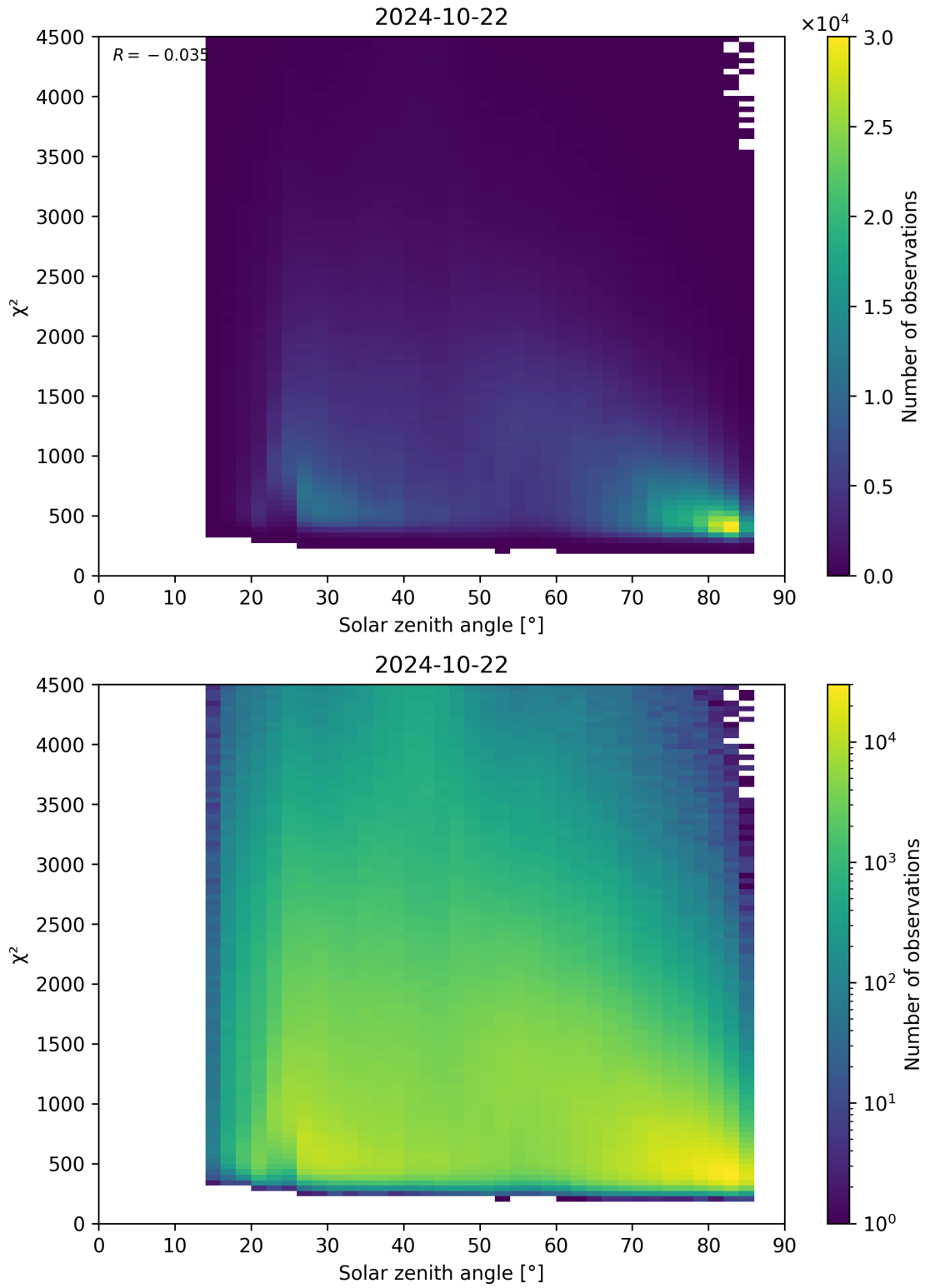
Figure 64: Scatter density plot of “Solar zenith angle” against “ \chi^2 ” for 2024-10-21 to 2024-10-23.
