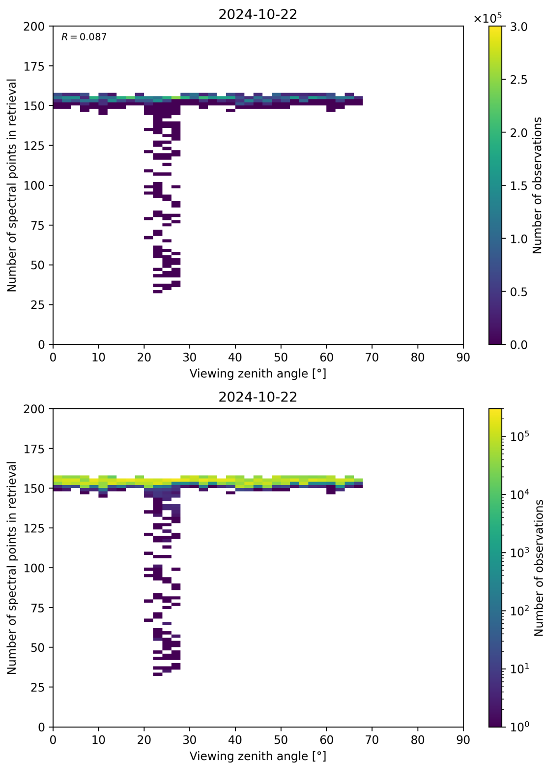
Figure 76: Scatter density plot of “Viewing zenith angle” against “Number of spectral points in retrieval” for 2024-10-21 to 2024-10-23.
