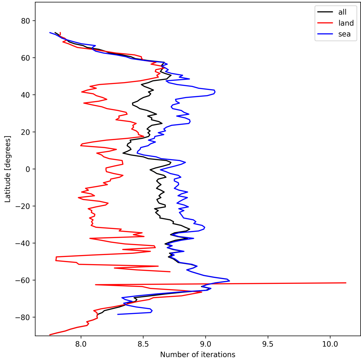
Figure 16: Zonal average of “Number of iterations” for 2024-10-21 to 2024-10-23.
