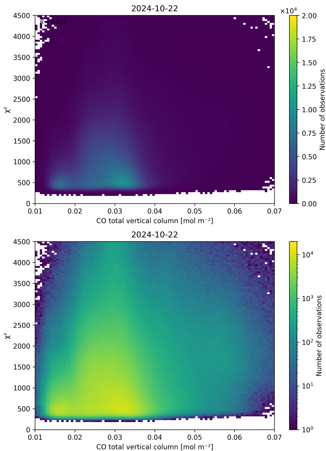
Figure 35: Scatter density plot of “CO total vertical column” against “ \chi^2 ” for 2024-10-21 to 2024-10-23.
