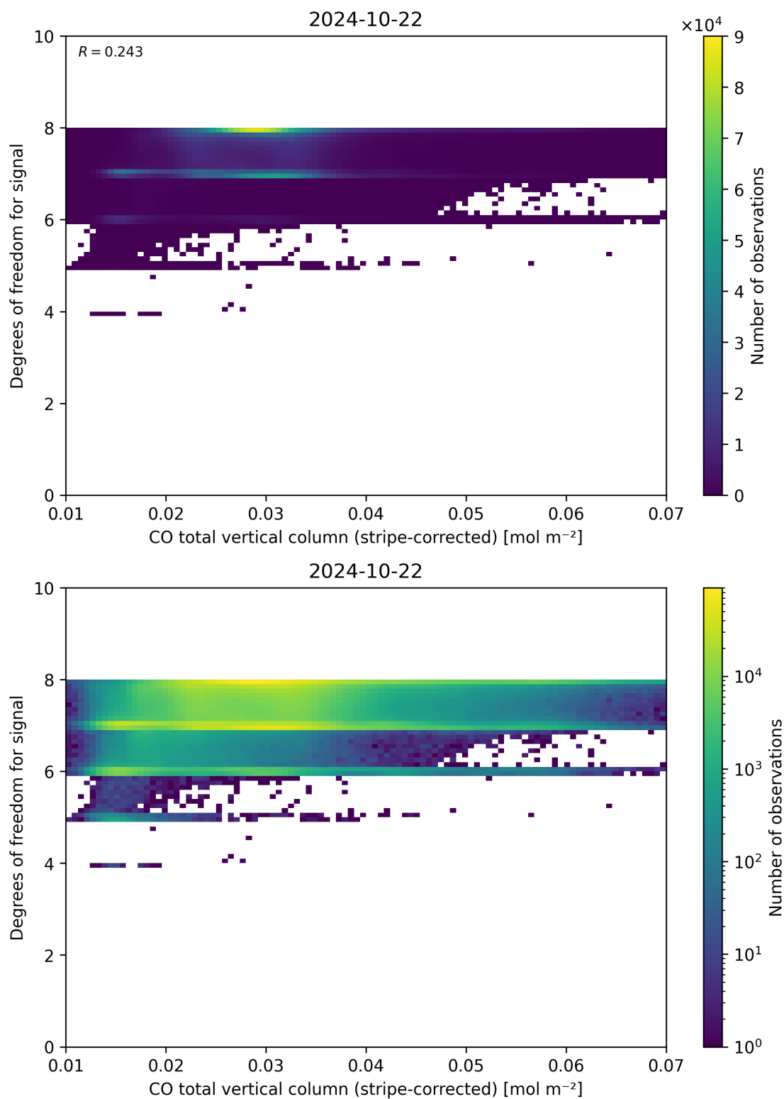
Figure 38: Scatter density plot of “CO total vertical column (stripe-corrected)” against “Degrees of freedom for signal” for 2024-10-21 to 2024-10-23.
