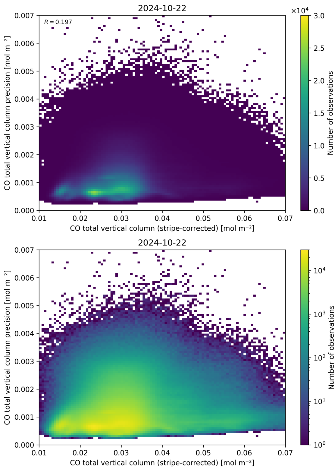
Figure 36: Scatter density plot of “CO total vertical column (stripe-corrected)” against “CO total vertical column precision” for 2024-10-21 to 2024-10-23.
