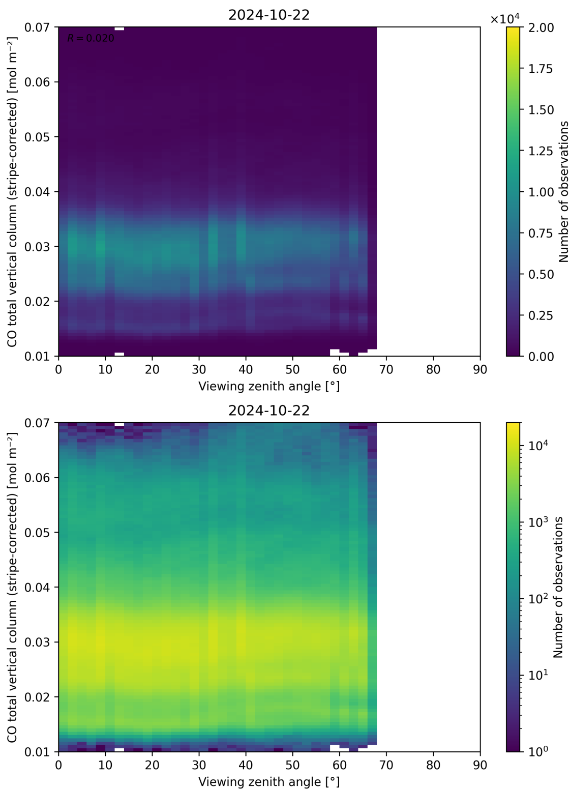
Figure 70: Scatter density plot of “Viewing zenith angle” against “CO total vertical column (stripe-corrected)” for 2024-10-21 to 2024-10-23.
