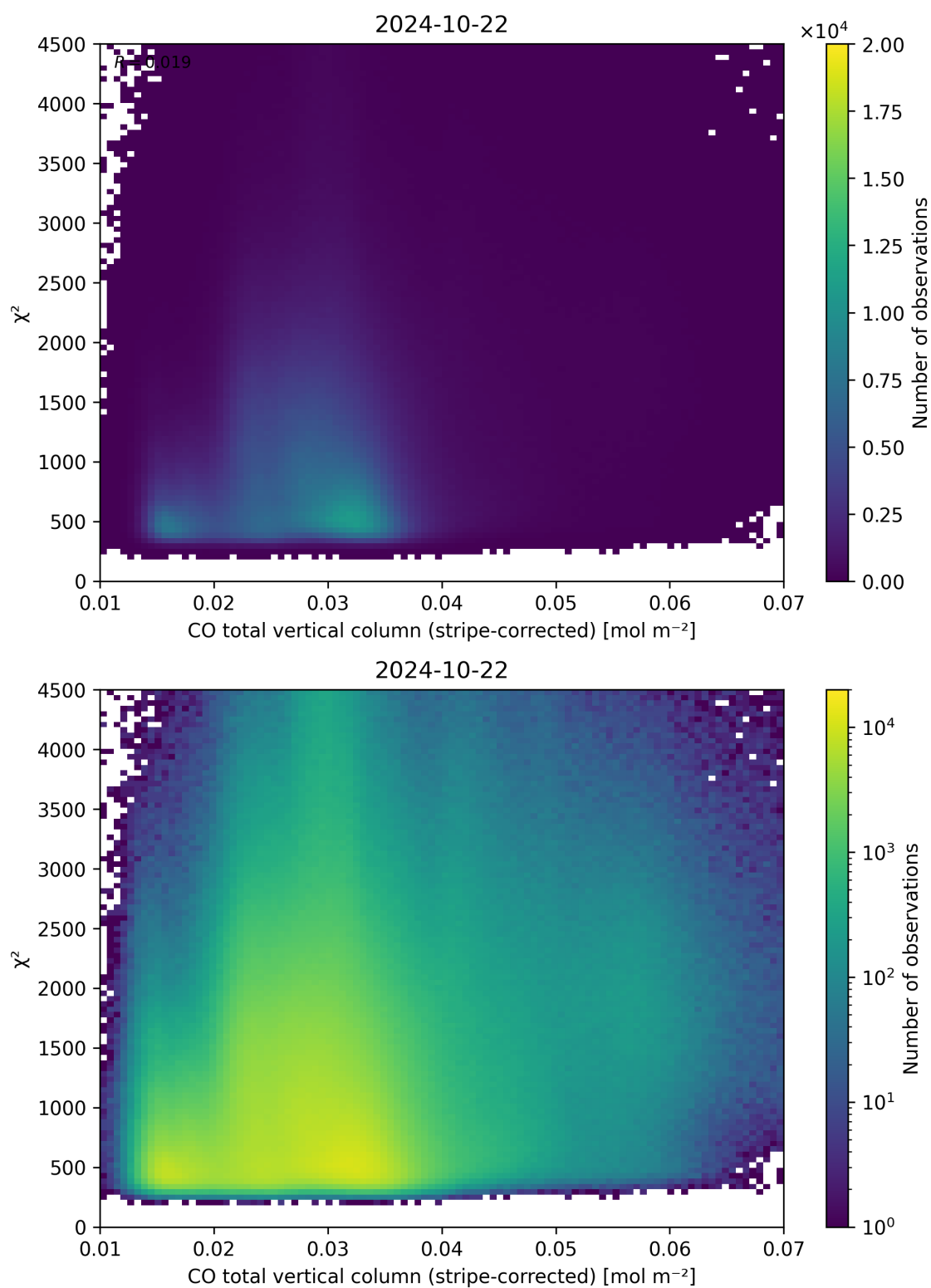
Figure 37: Scatter density plot of “CO total vertical column (stripe-corrected)” against “ \chi^2 ” for 2024-10-21 to 2024-10-23.
