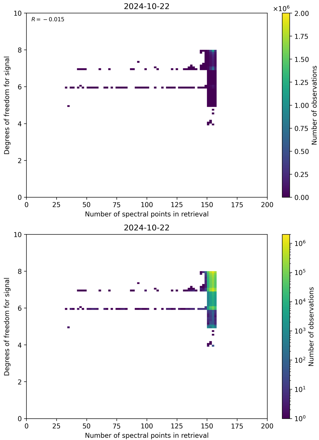
Figure 59: Scatter density plot of “Number of spectral points in retrieval” against “Degrees of freedom for signal” for 2024-10-21 to 2024-10-23.
