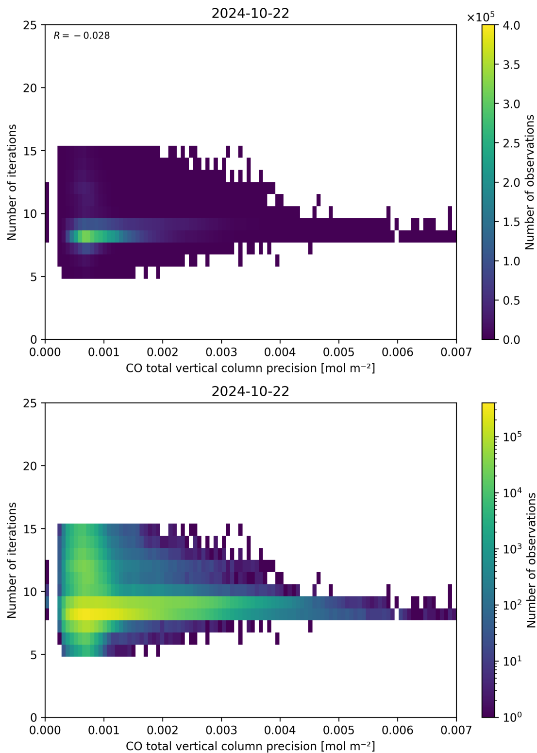
Figure 46: Scatter density plot of “CO total vertical column precision” against “Number of iterations” for 2024-10-21 to 2024-10-23.
