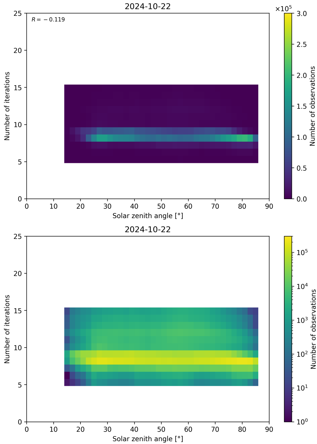
Figure 67: Scatter density plot of “Solar zenith angle” against “Number of iterations” for 2024-10-21 to 2024-10-23.
