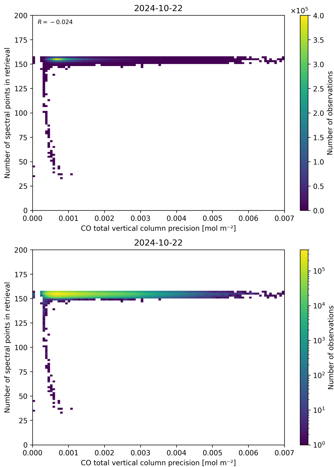
Figure 47: Scatter density plot of “CO total vertical column precision” against “Number of spectral points in retrieval” for 2024-10-21 to 2024-10-23.
