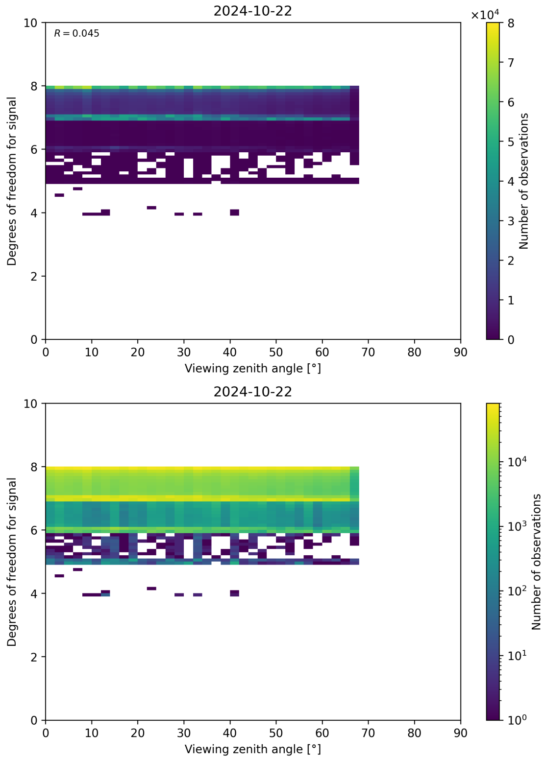
Figure 73: Scatter density plot of “Viewing zenith angle” against “Degrees of freedom for signal” for 2024-10-21 to 2024-10-23.
