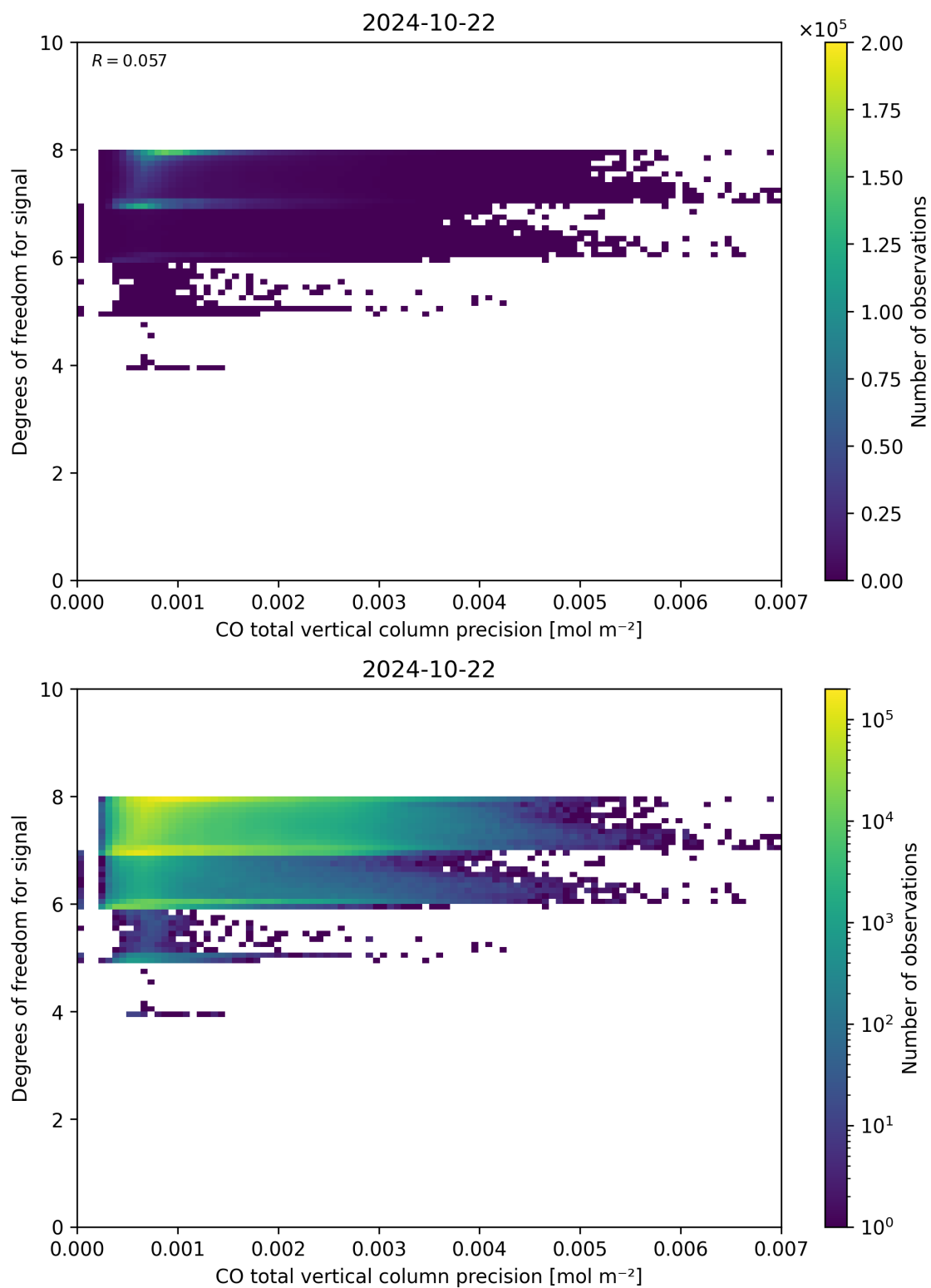
Figure 45: Scatter density plot of “CO total vertical column precision” against “Degrees of freedom for signal” for 2024-10-21 to 2024-10-23.
