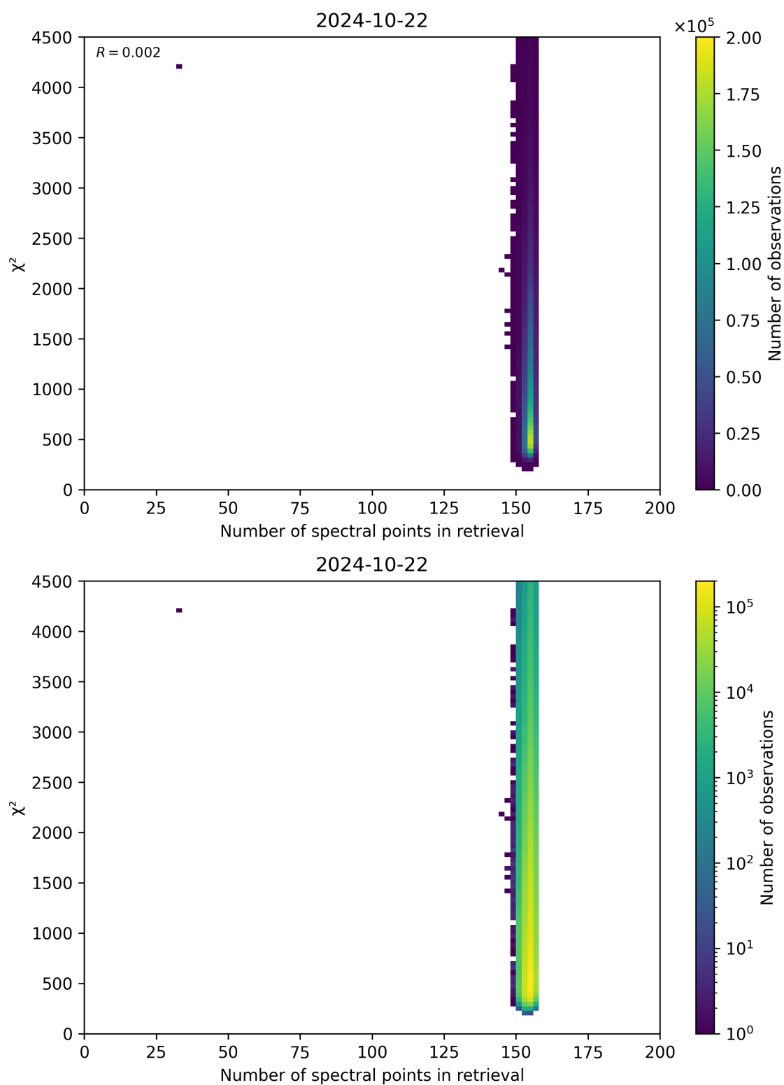
Figure 58: Scatter density plot of “Number of spectral points in retrieval” against “ \chi^2 ” for 2024-10-21 to 2024-10-23.
