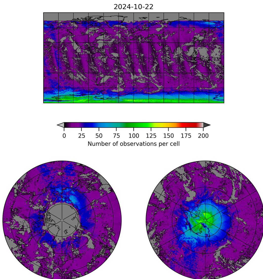
Figure 8: Map of the number of observations for 2024-10-21 to 2024-10-23
