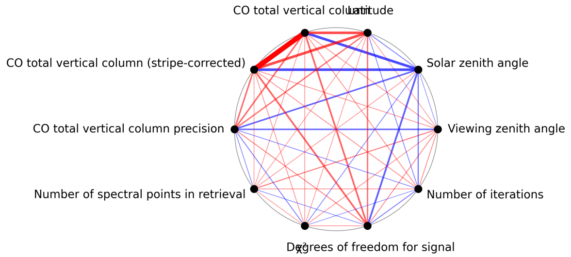
Figure 1: Map of correlation graph for 2024-10-21 to 2024-10-23.
