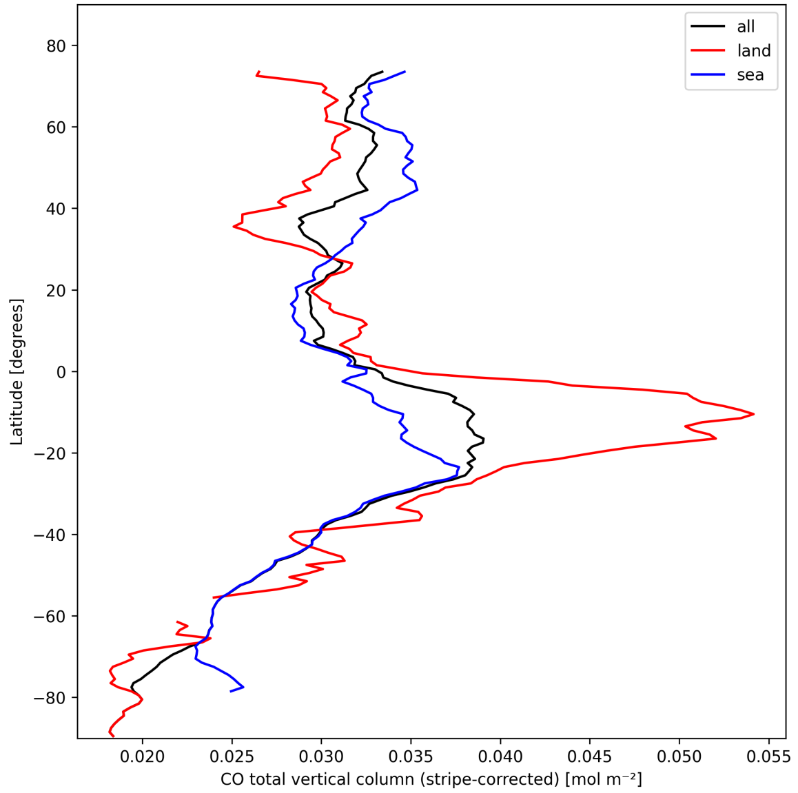
Figure 11: Zonal average of “CO total vertical column (stripe-corrected)” for 2024-10-21 to 2024-10-23.
