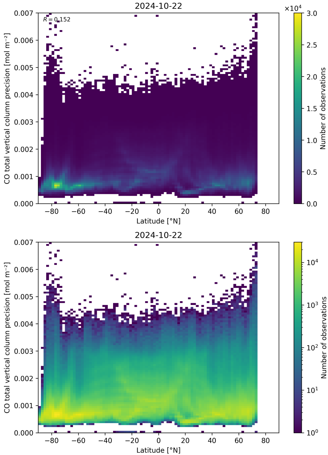
Figure 53: Scatter density plot of “Latitude” against “CO total vertical column precision” for 2024-10-21 to 2024-10-23.
