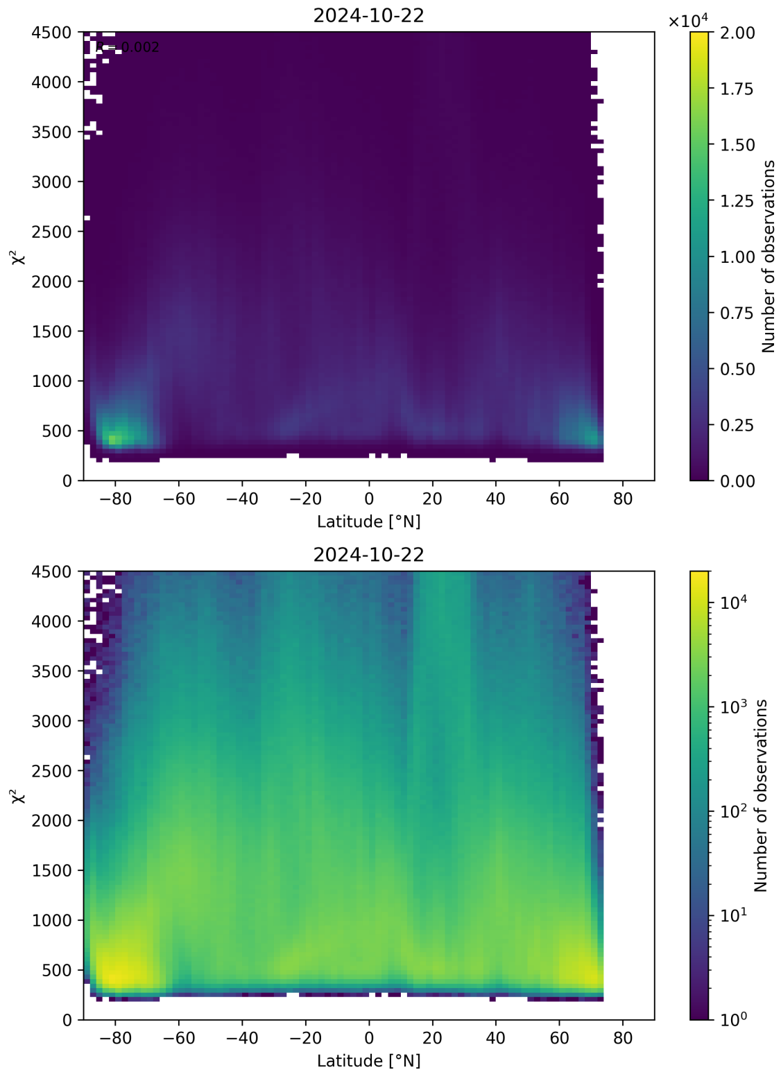
Figure 54: Scatter density plot of “Latitude” against “ \chi^2 ” for 2024-10-21 to 2024-10-23.
