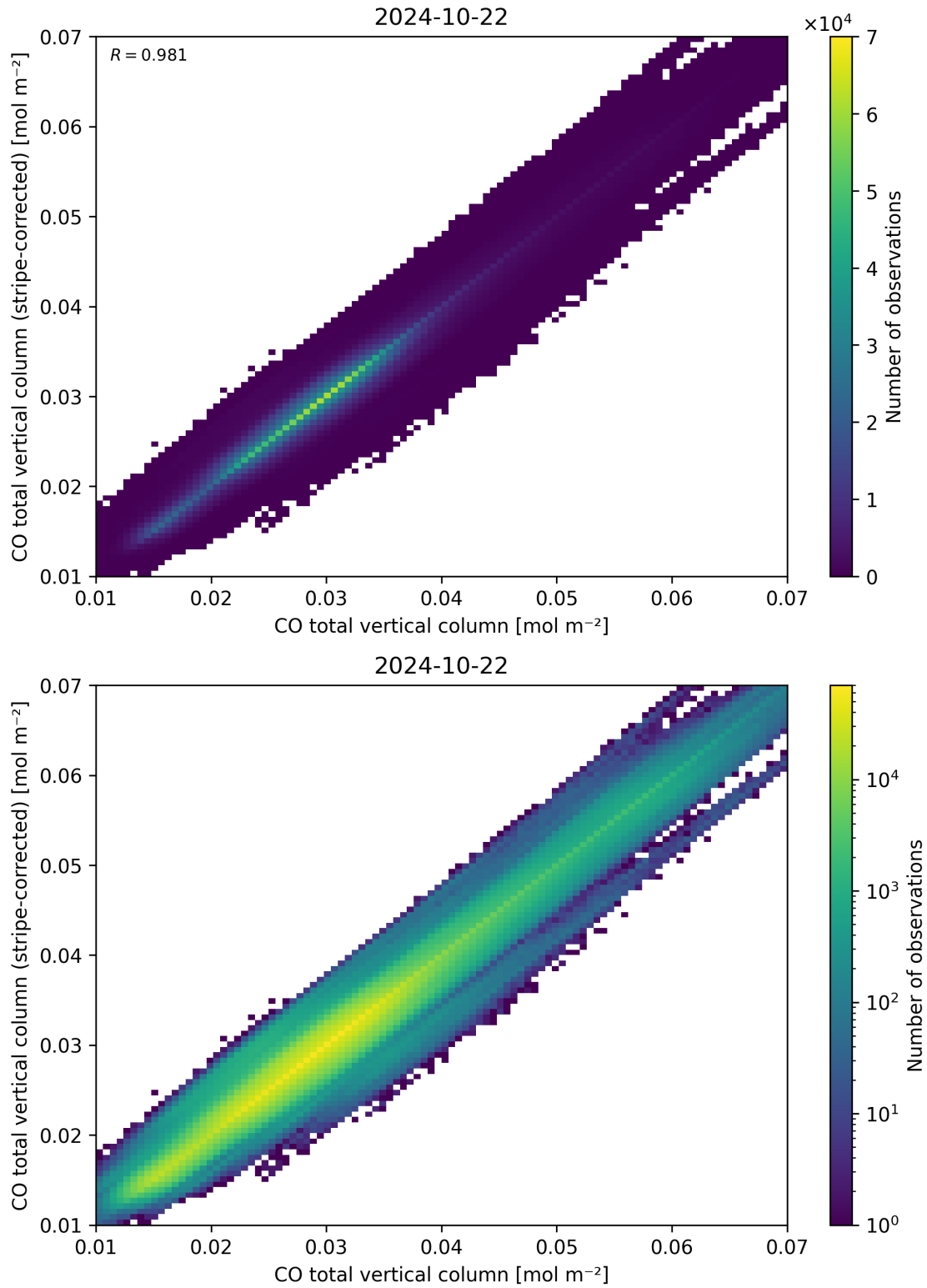
Figure 33: Scatter density plot of “CO total vertical column” against “CO total vertical column (stripe-corrected)” for 2024-10-21 to 2024-10-23.
