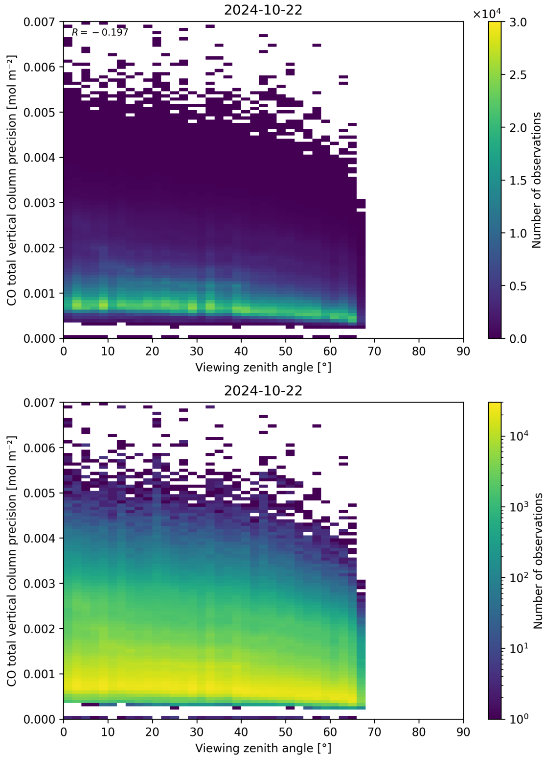
Figure 71: Scatter density plot of “Viewing zenith angle” against “CO total vertical column precision” for 2024-10-21 to 2024-10-23.
