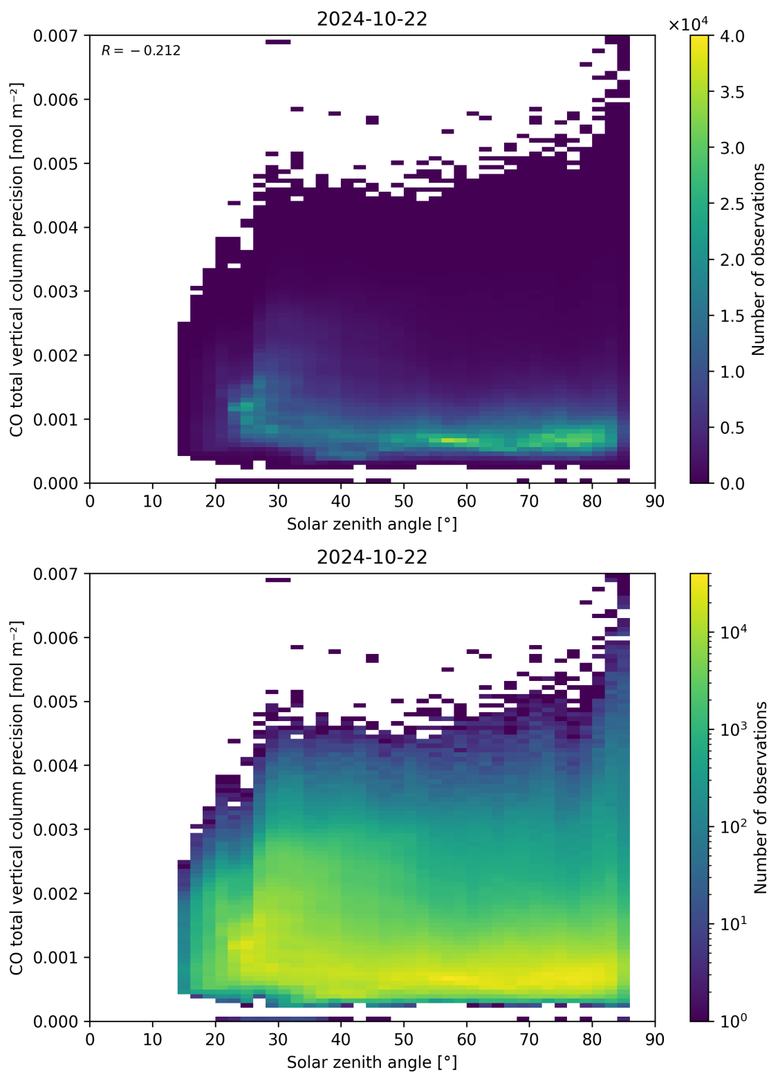
Figure 63: Scatter density plot of “Solar zenith angle” against “CO total vertical column precision” for 2024-10-21 to 2024-10-23.
