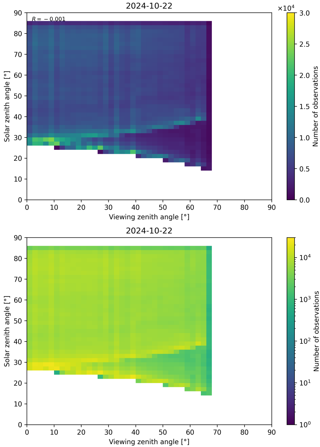
Figure 77: Scatter density plot of “Viewing zenith angle” against “Solar zenith angle” for 2024-10-21 to 2024-10-23.
