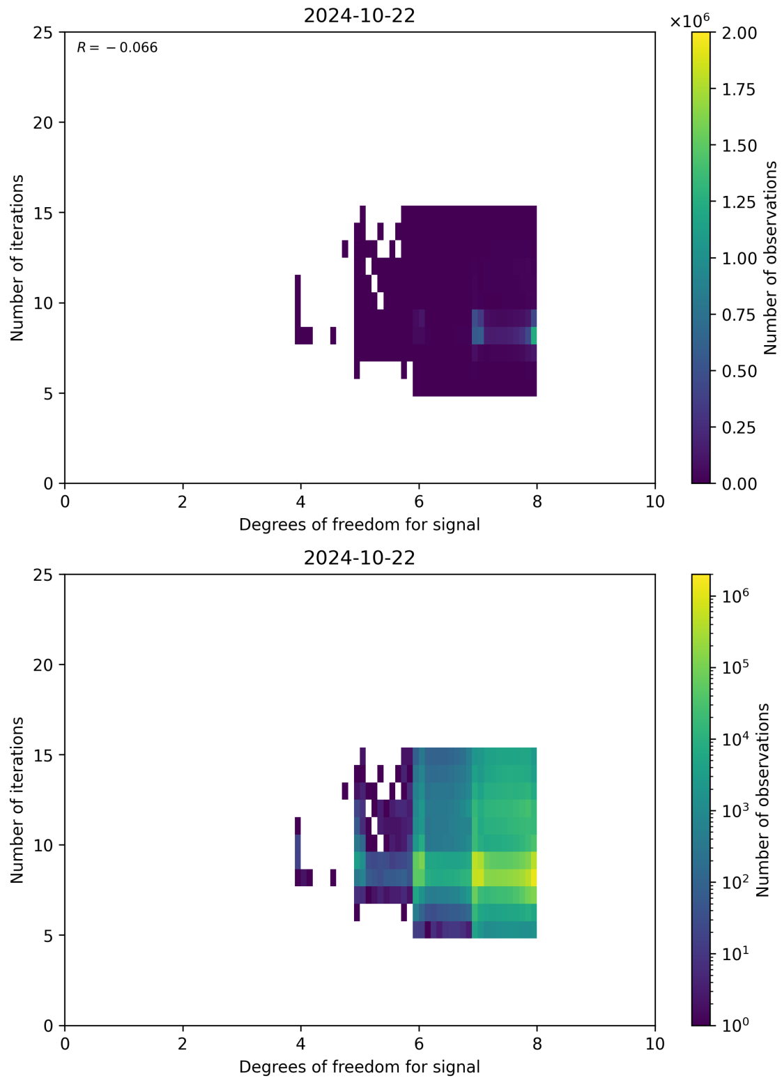
Figure 50: Scatter density plot of “Degrees of freedom for signal” against “Number of iterations” for 2024-10-21 to 2024-10-23.
