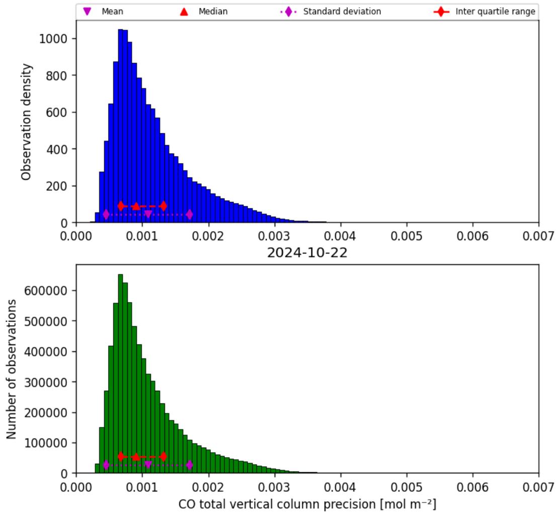
Figure 20: Histogram of “CO total vertical column precision” for 2024-10-21 to 2024-10-23
