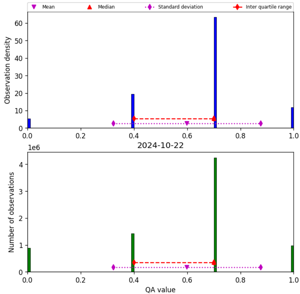
Figure 17: Histogram of “QA value” for 2024-10-21 to 2024-10-23
