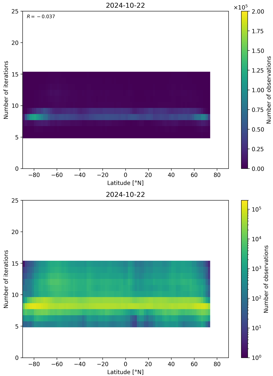
Figure 56: Scatter density plot of “Latitude” against “Number of iterations” for 2024-10-21 to 2024-10-23.
