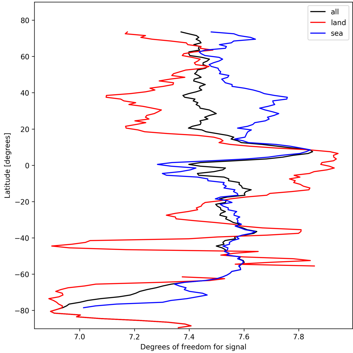
Figure 15: Zonal average of “Degrees of freedom for signal” for 2024-10-21 to 2024-10-23.
