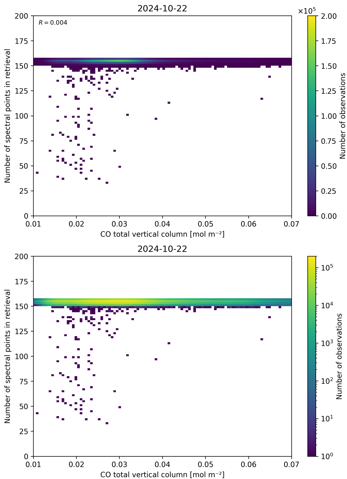
Figure 43: Scatter density plot of “CO total vertical column” against “Number of spectral points in retrieval” for 2024-10-21 to 2024-10-23.
