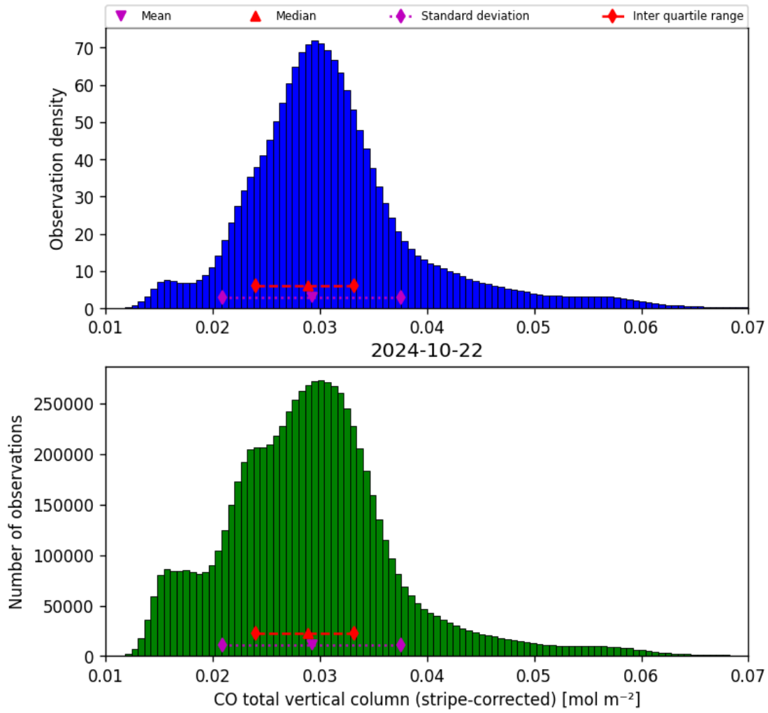
Figure 19: Histogram of “CO total vertical column (stripe-corrected)” for 2024-10-21 to 2024-10-23
