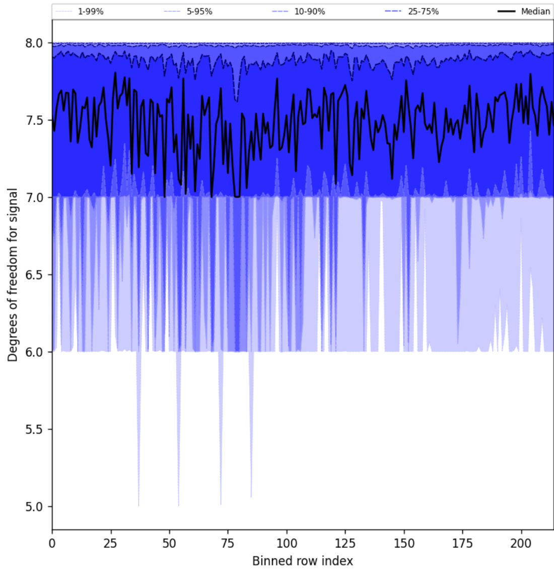
Figure 31: Along track statistics of “Degrees of freedom for signal” for 2024-10-21 to 2024-10-23
