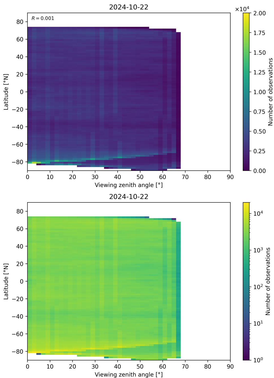
Figure 74: Scatter density plot of “Viewing zenith angle” against “Latitude” for 2024-10-21 to 2024-10-23.
