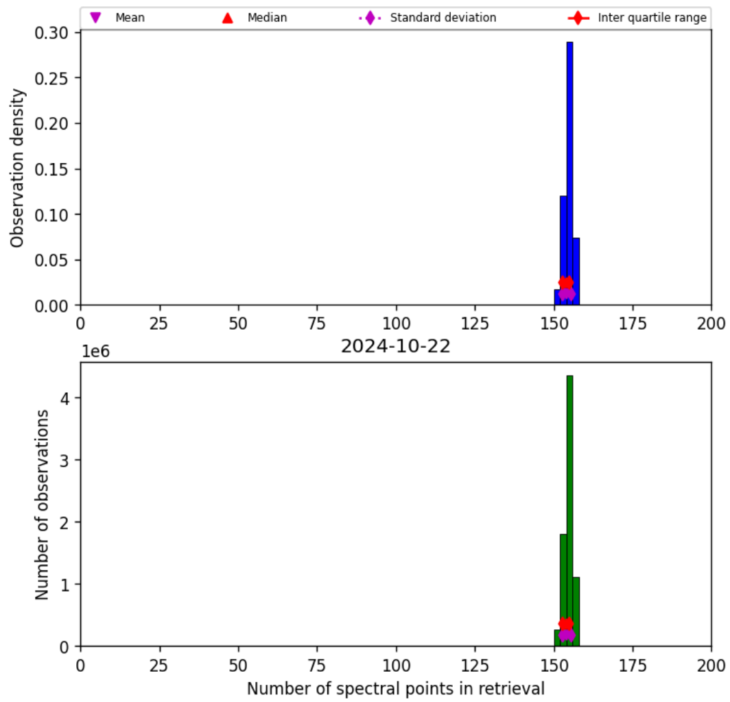
Figure 21: Histogram of “Number of spectral points in retrieval” for 2024-10-21 to 2024-10-23
