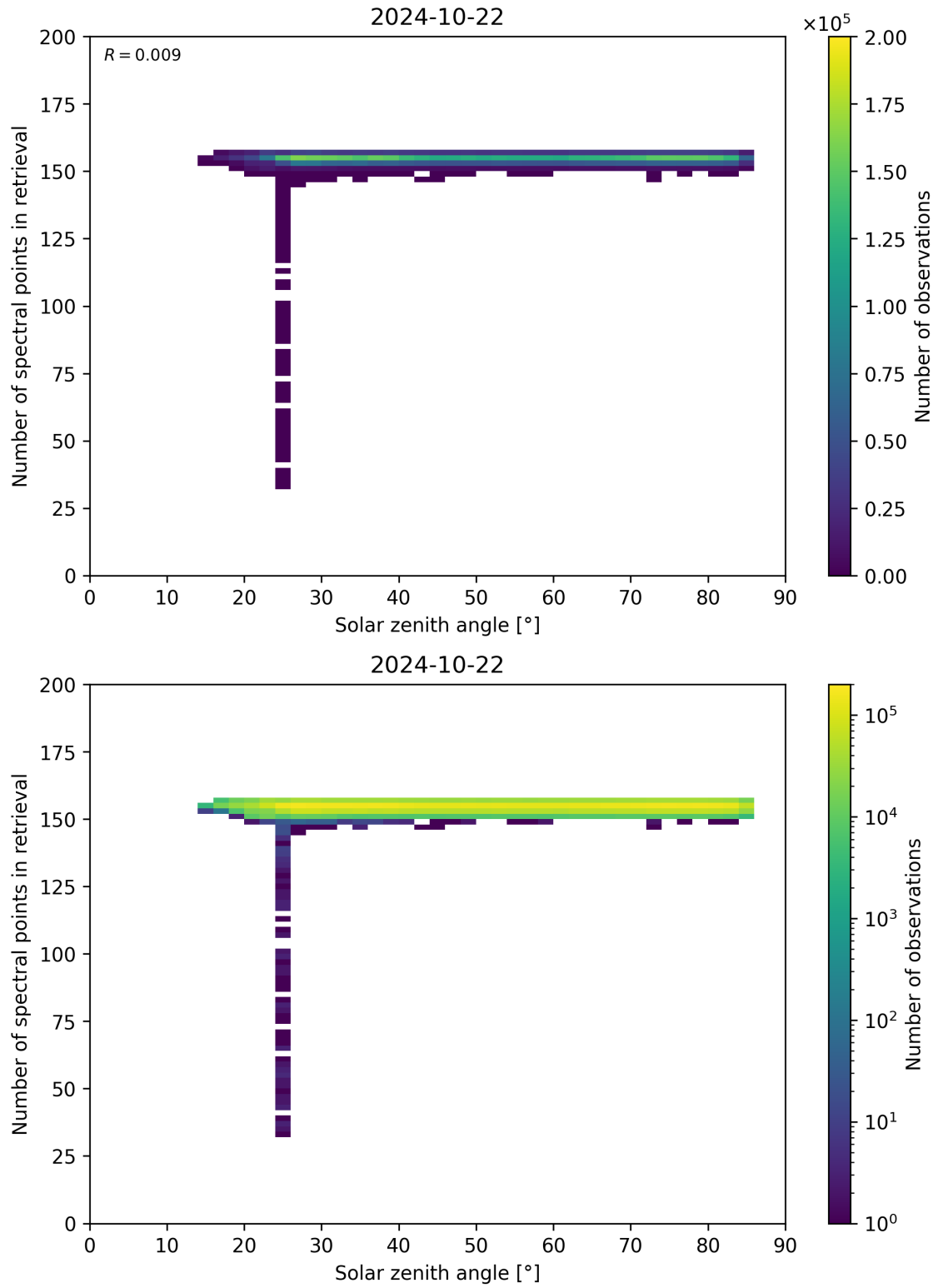
Figure 68: Scatter density plot of “Solar zenith angle” against “Number of spectral points in retrieval” for 2024-10-21 to 2024-10-23.
