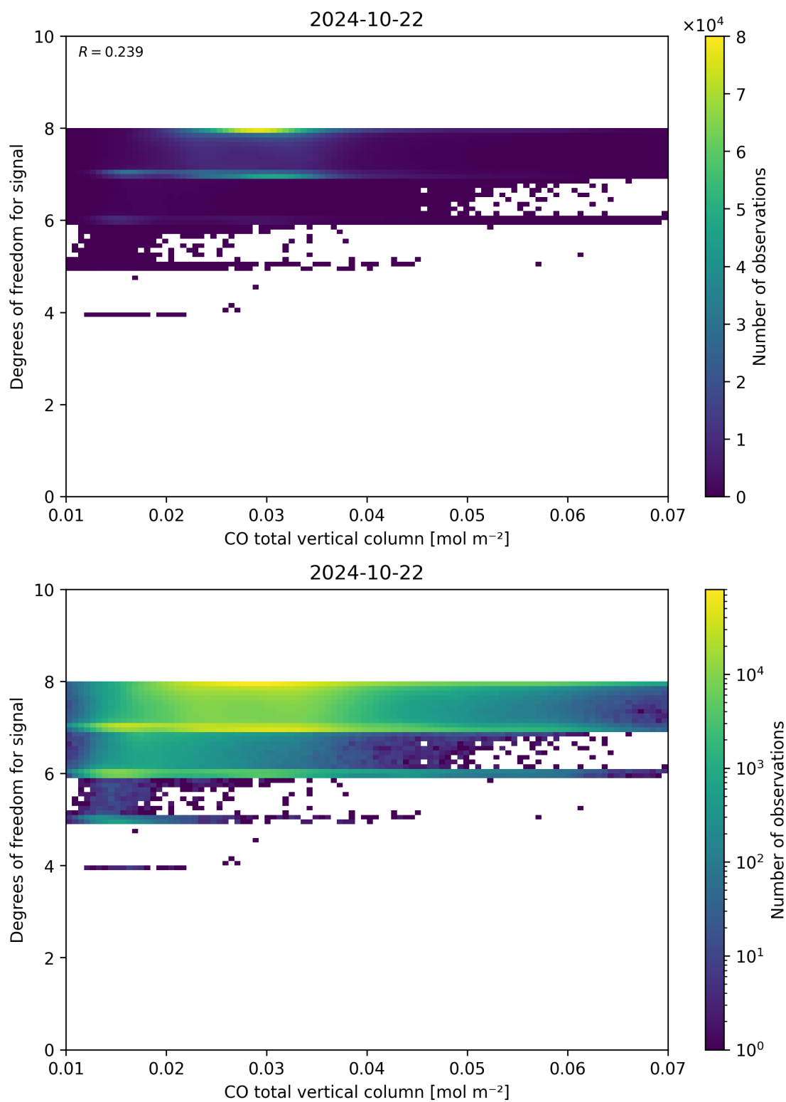
Figure 41: Scatter density plot of “CO total vertical column” against “Degrees of freedom for signal” for 2024-10-21 to 2024-10-23.
