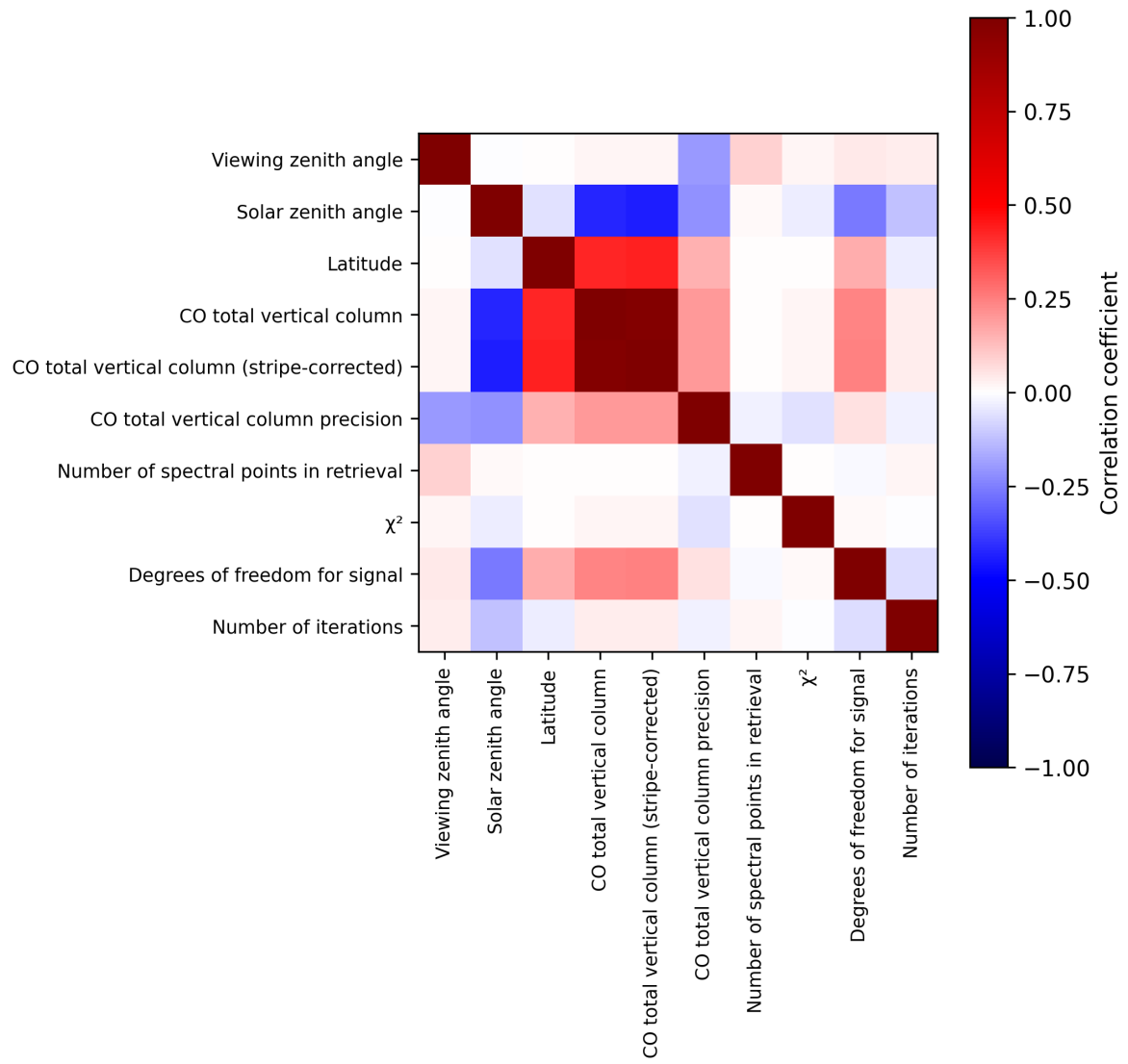
Figure 2: Map of correlation matrix for 2024-10-21 to 2024-10-23.
