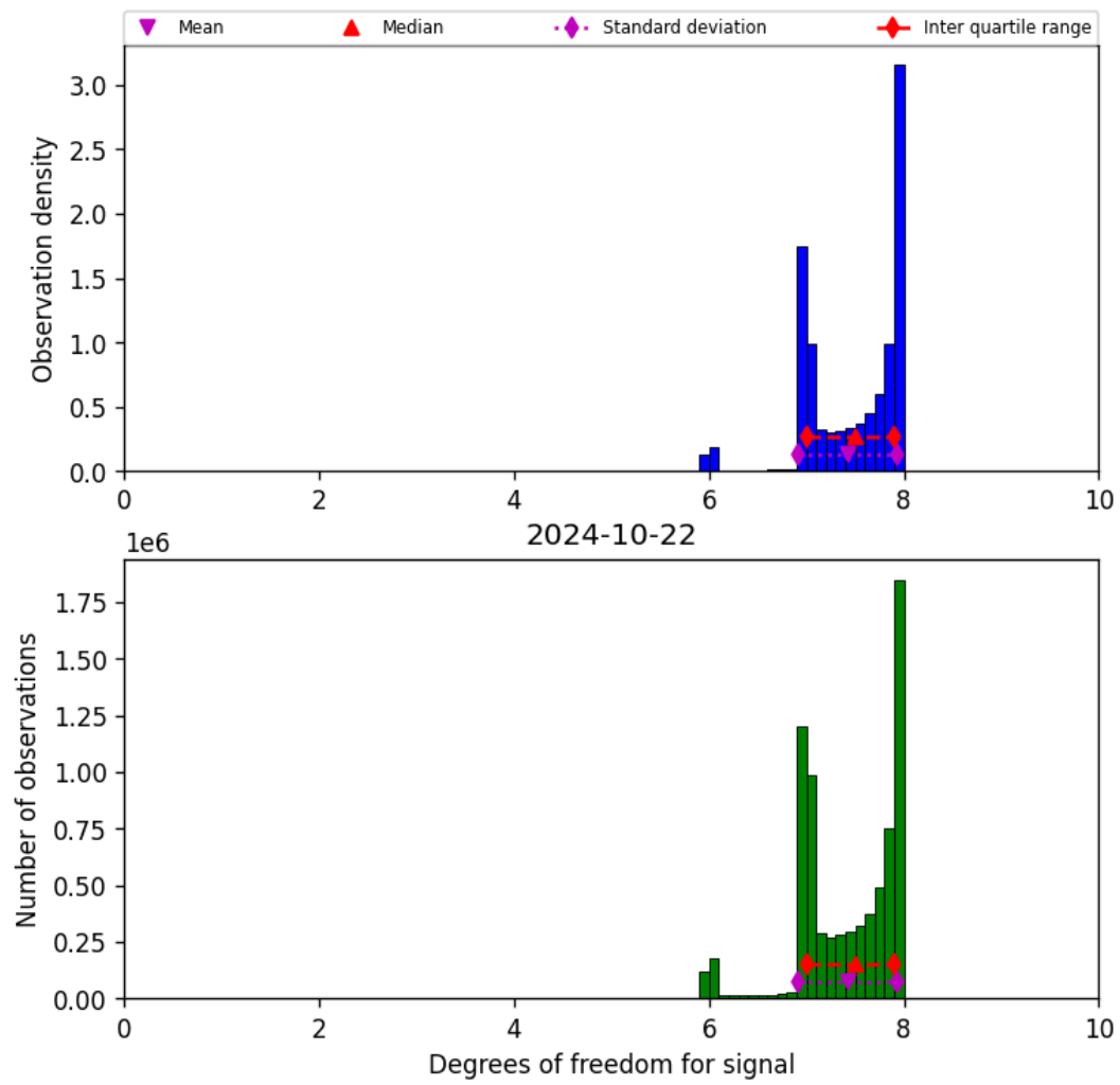
Figure 23: Histogram of “Degrees of freedom for signal” for 2024-10-21 to 2024-10-23
