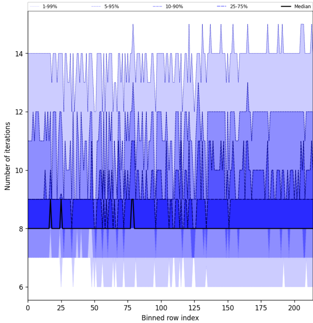
Figure 32: Along track statistics of “Number of iterations” for 2024-10-21 to 2024-10-23
