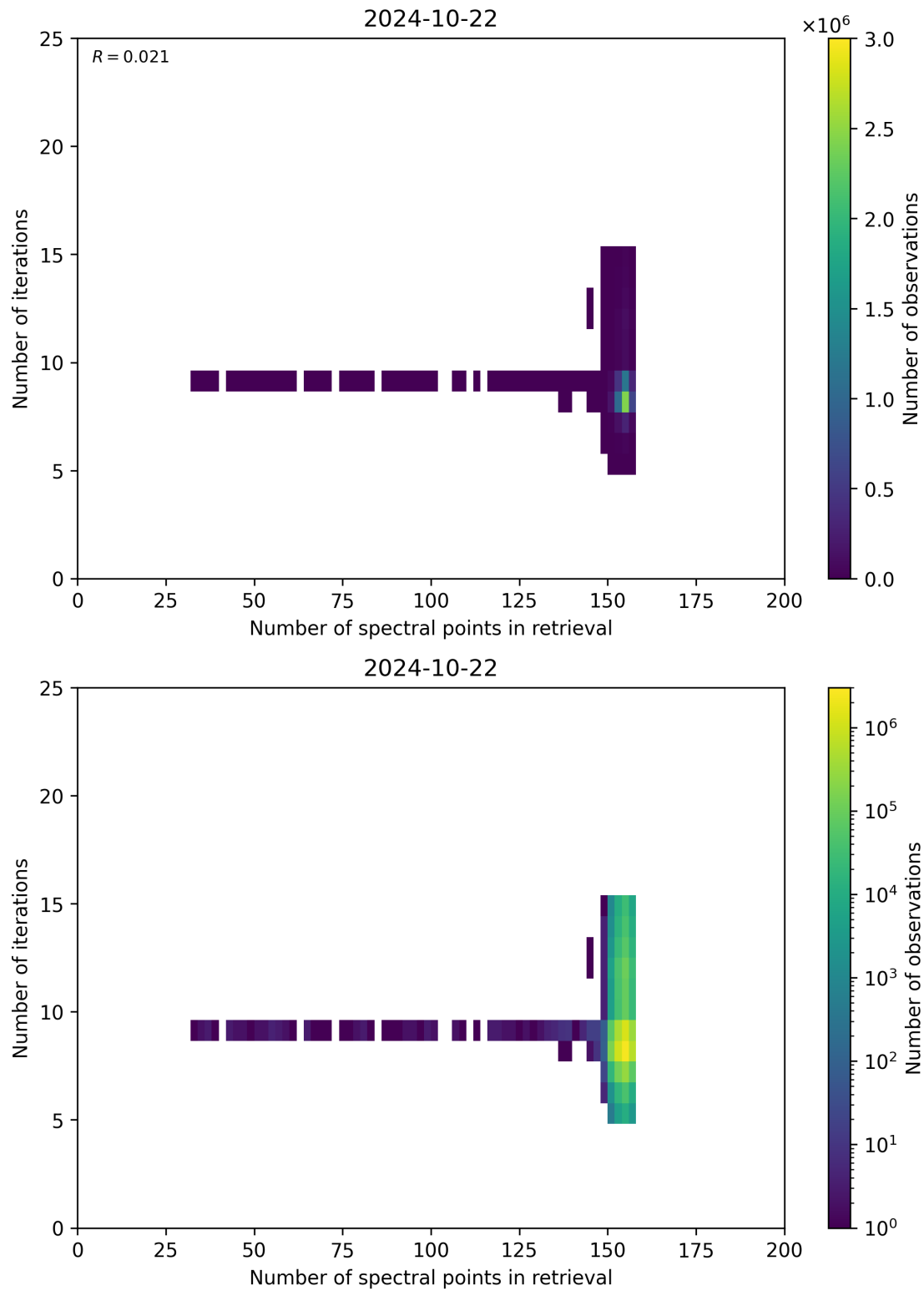
Figure 60: Scatter density plot of “Number of spectral points in retrieval” against “Number of iterations” for 2024-10-21 to 2024-10-23.
