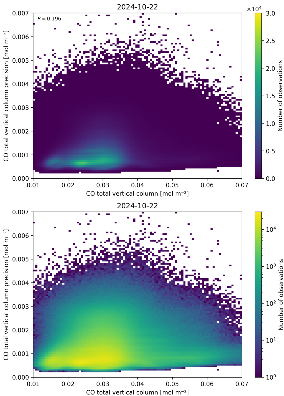
Figure 34: Scatter density plot of “CO total vertical column” against “CO total vertical column precision” for 2024-10-21 to 2024-10-23.
