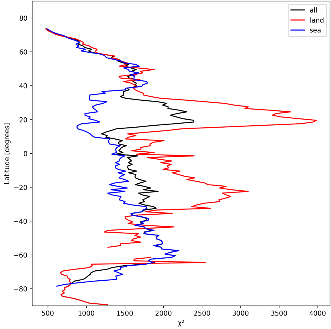
Figure 14: Zonal average of “ \chi^2 ” for 2024-10-21 to 2024-10-23.
