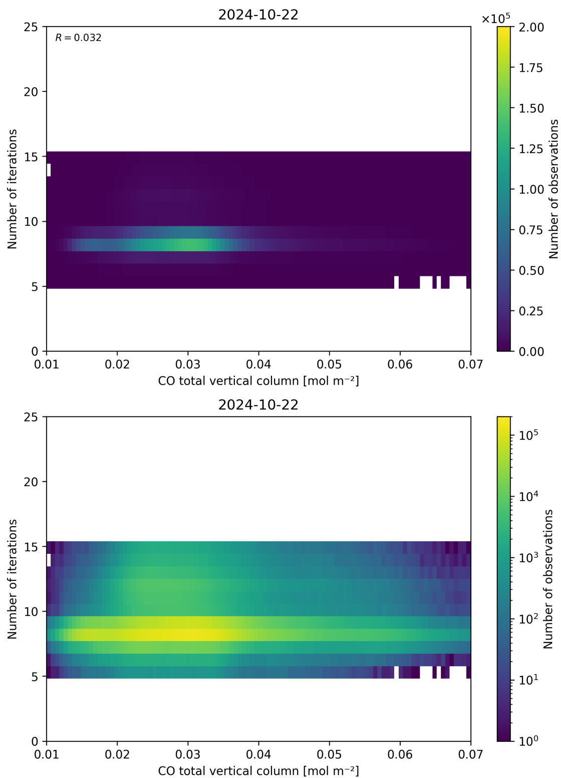
Figure 42: Scatter density plot of “CO total vertical column” against “Number of iterations” for 2024-10-21 to 2024-10-23.
