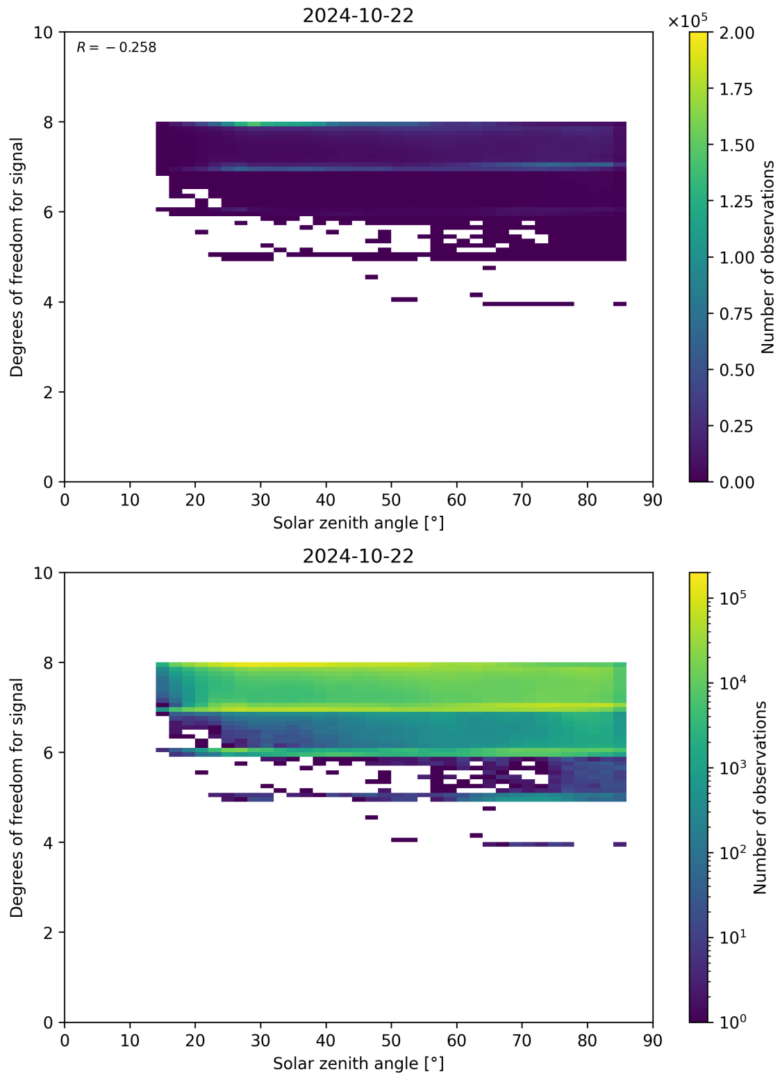
Figure 65: Scatter density plot of “Solar zenith angle” against “Degrees of freedom for signal” for 2024-10-21 to 2024-10-23.
