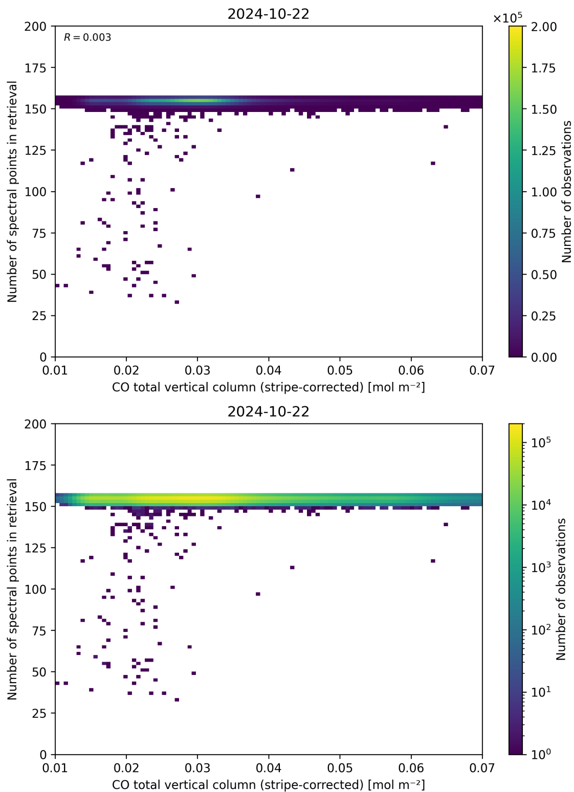
Figure 40: Scatter density plot of “CO total vertical column (stripe-corrected)” against “Number of spectral points in retrieval” for 2024-10-21 to 2024-10-23.
