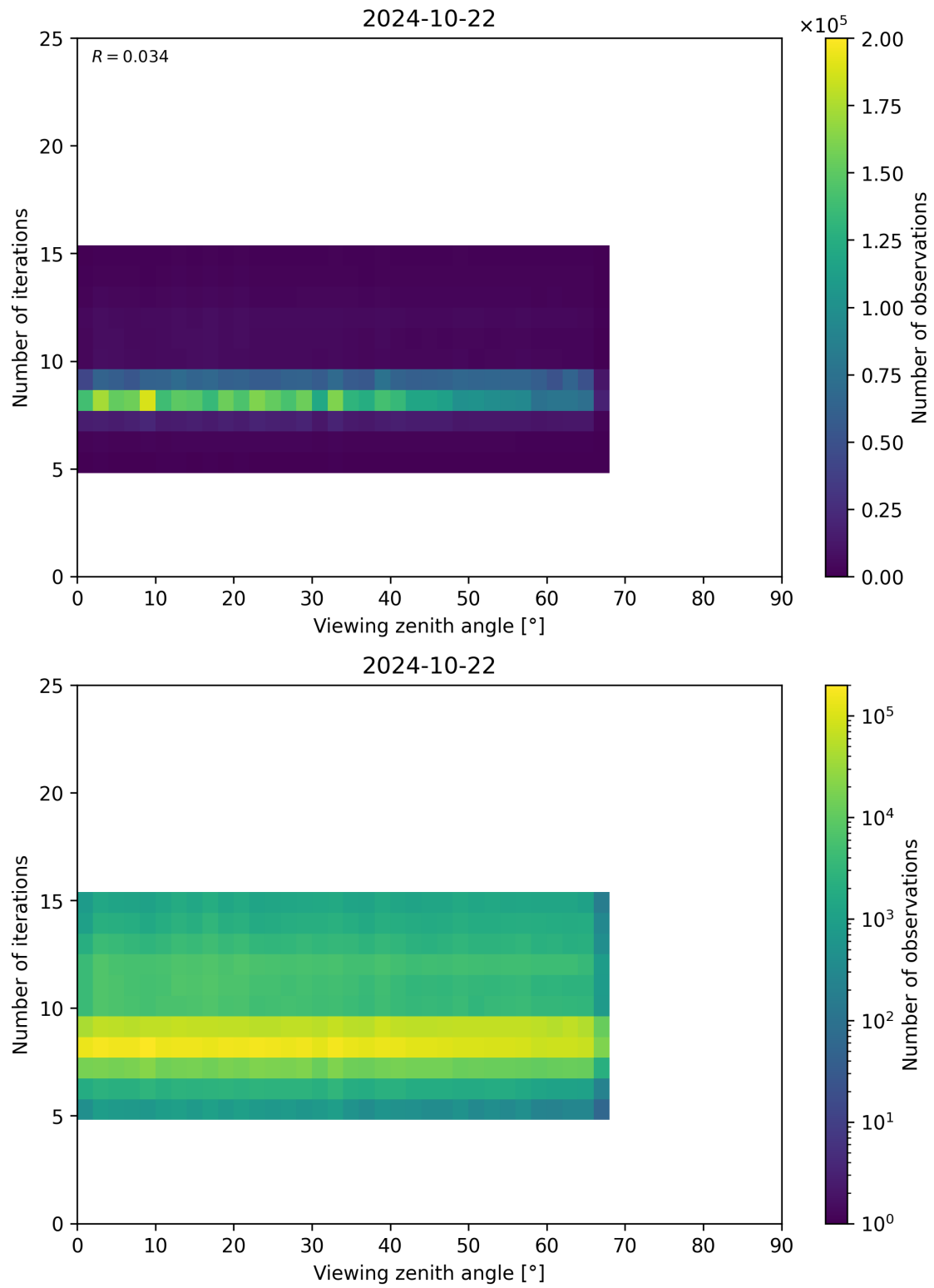
Figure 75: Scatter density plot of “Viewing zenith angle” against “Number of iterations” for 2024-10-21 to 2024-10-23.
