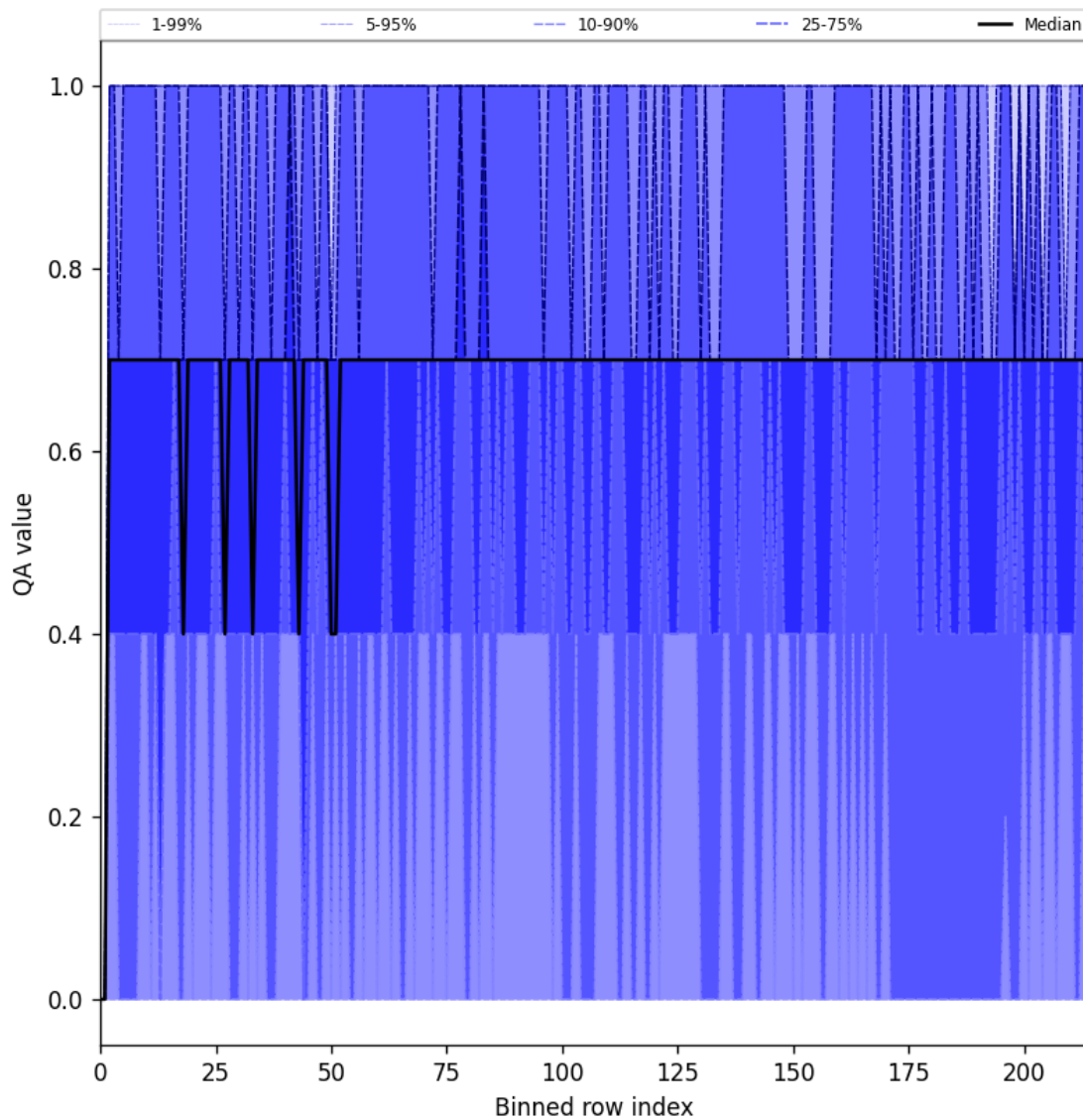
Figure 25: Along track statistics of “QA value” for 2024-10-21 to 2024-10-23
