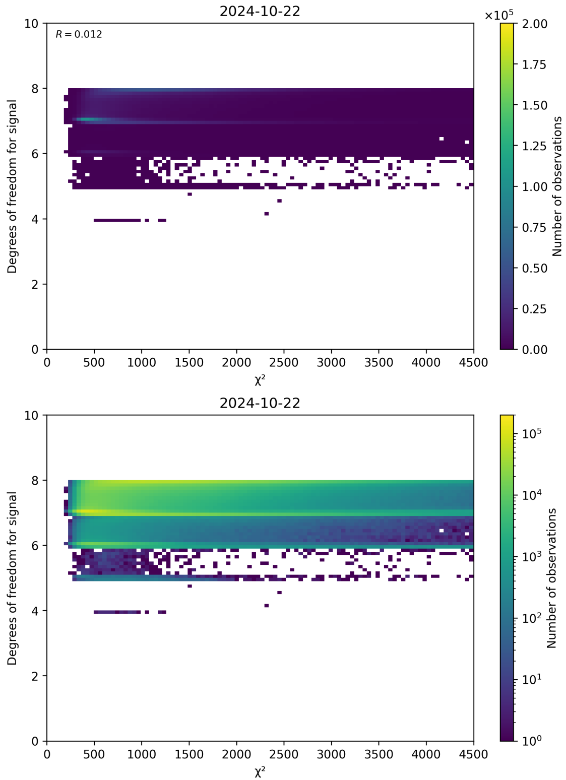
Figure 48: Scatter density plot of “ \chi^2 ” against “Degrees of freedom for signal” for 2024-10-21 to 2024-10-23.
