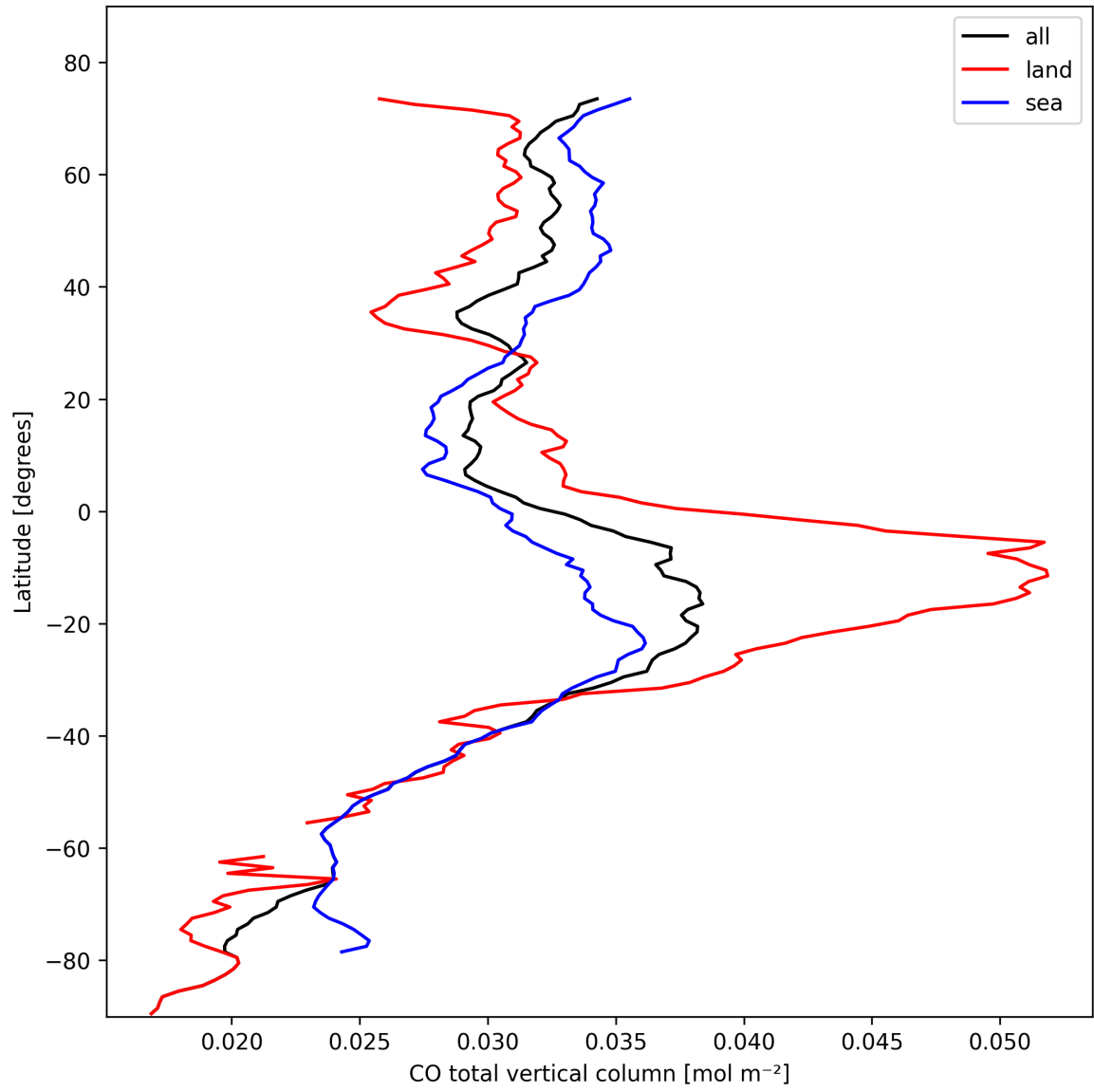
Figure 10: Zonal average of “CO total vertical column” for 2024-10-22 to 2024-10-24.
