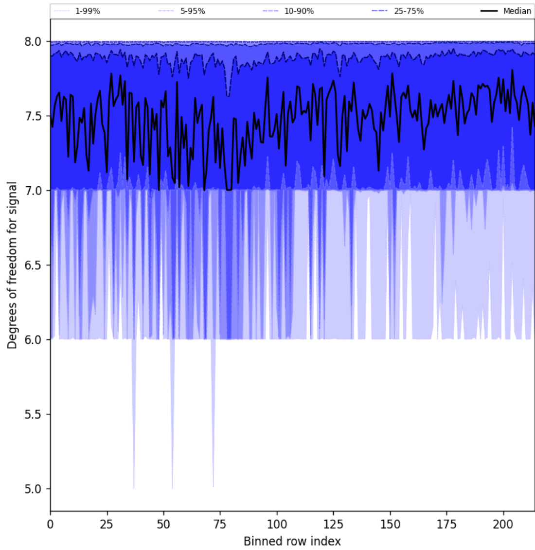
Figure 31: Along track statistics of “Degrees of freedom for signal” for 2024-10-22 to 2024-10-24
