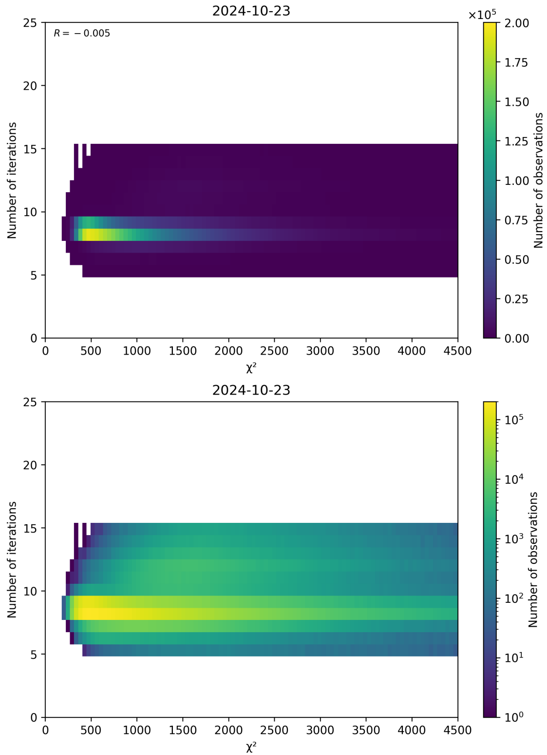
Figure 49: Scatter density plot of “ \chi^2 ” against “Number of iterations” for 2024-10-22 to 2024-10-24.
