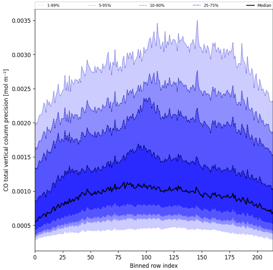
Figure 28: Along track statistics of “CO total vertical column precision” for 2024-10-22 to 2024-10-24
