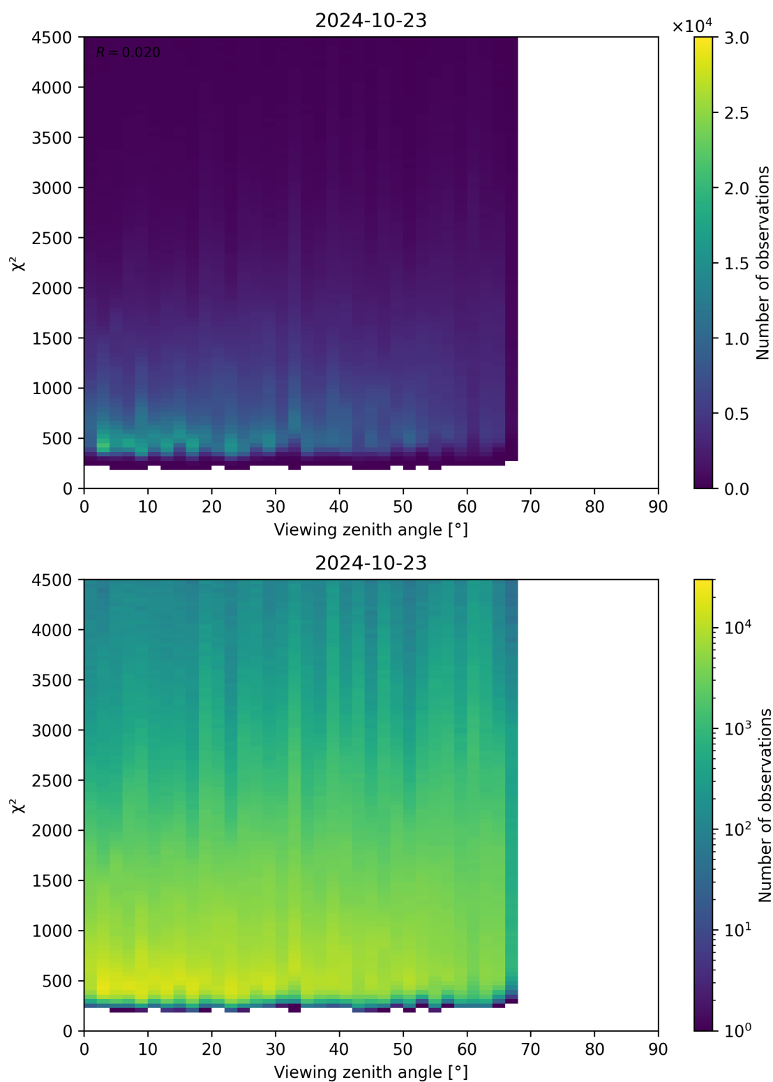
Figure 72: Scatter density plot of “Viewing zenith angle” against “ \chi^2 ” for 2024-10-22 to 2024-10-24.
