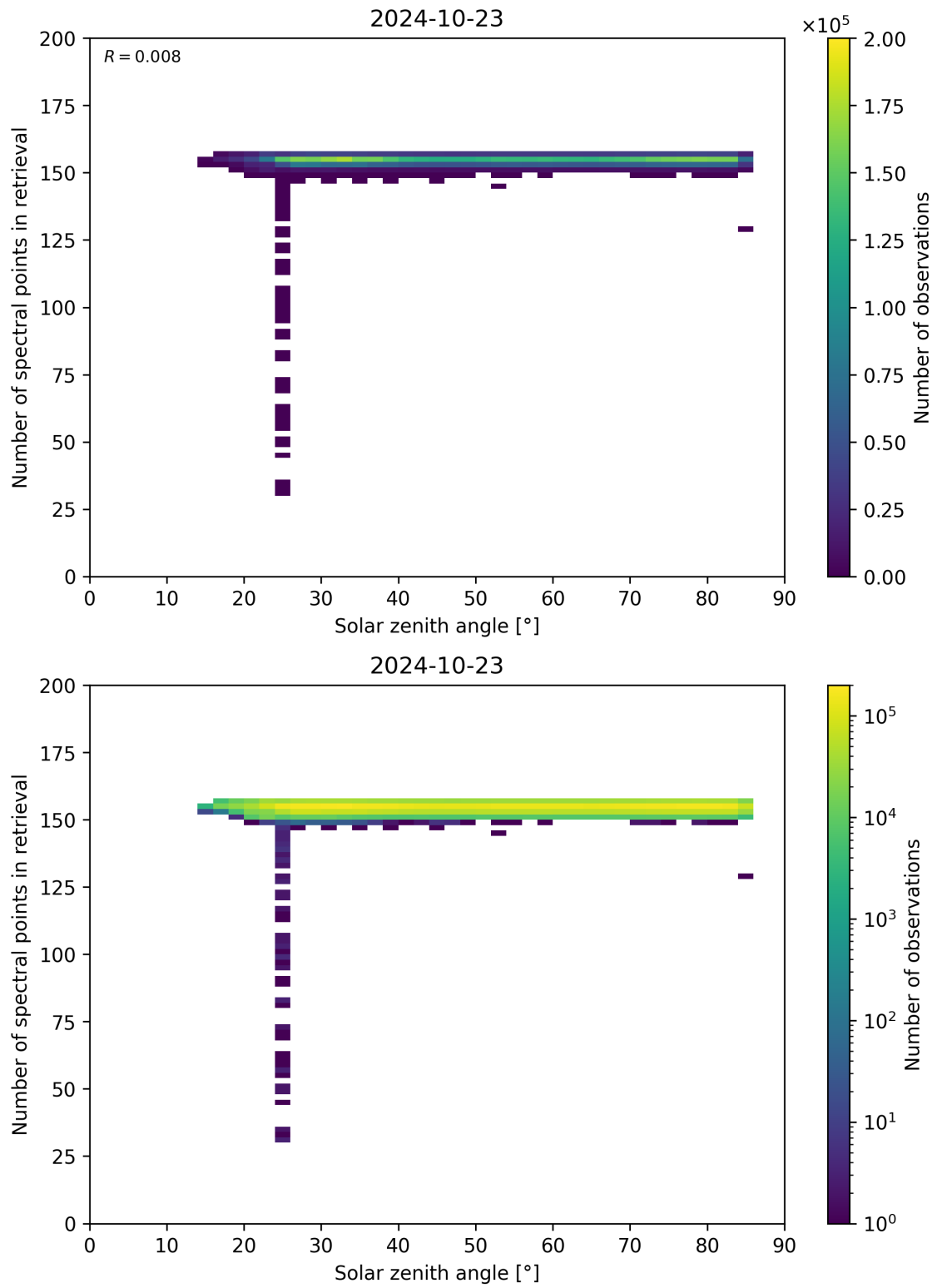
Figure 68: Scatter density plot of “Solar zenith angle” against “Number of spectral points in retrieval” for 2024-10-22 to 2024-10-24.
