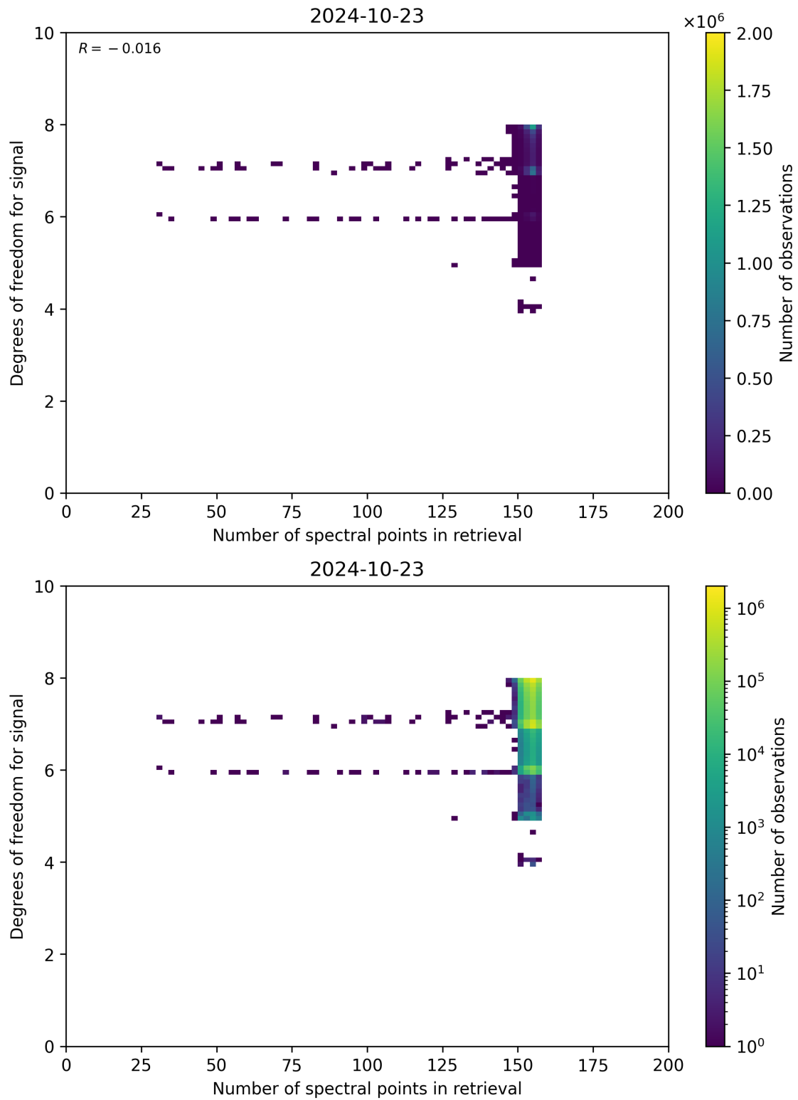
Figure 59: Scatter density plot of “Number of spectral points in retrieval” against “Degrees of freedom for signal” for 2024-10-22 to 2024-10-24.
