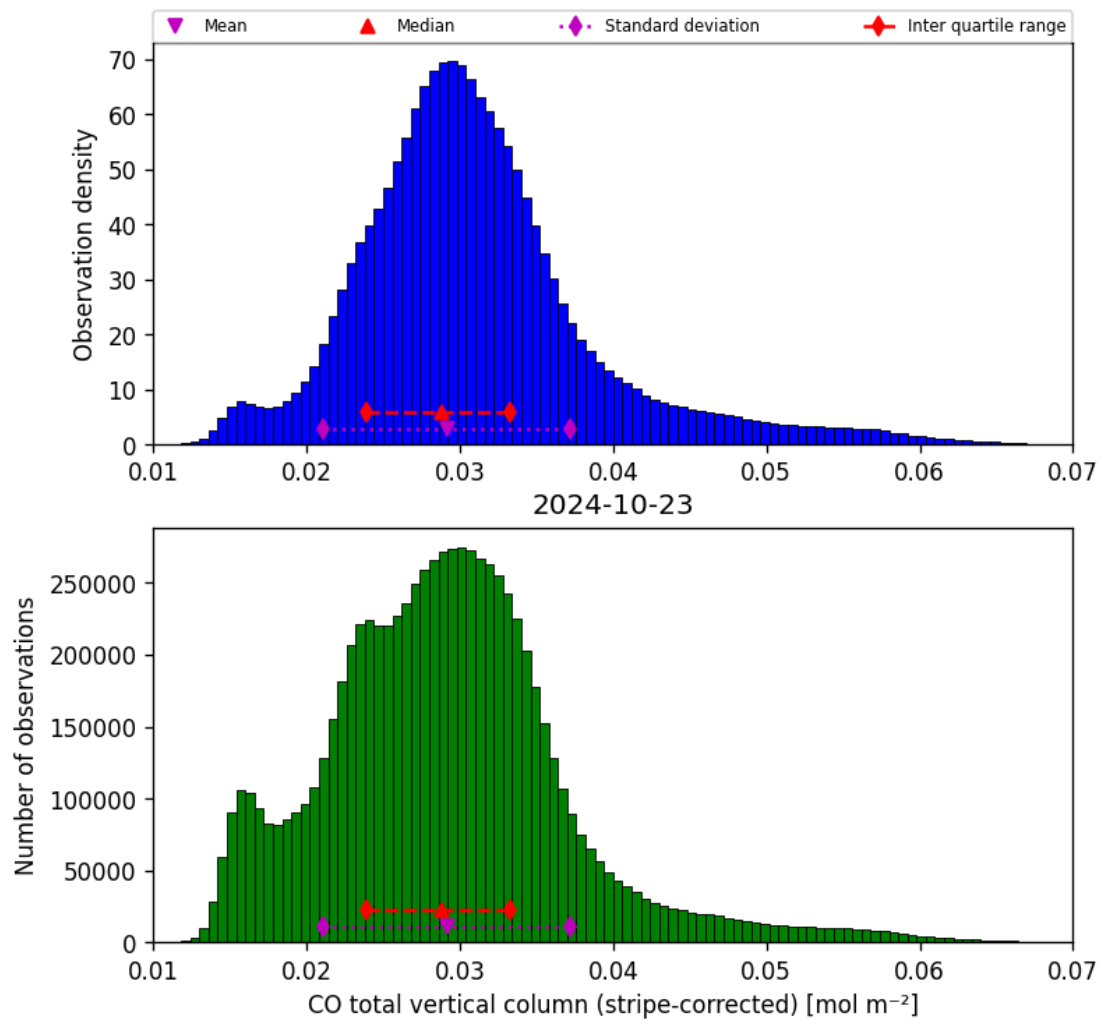
Figure 19: Histogram of “CO total vertical column (stripe-corrected)” for 2024-10-22 to 2024-10-24
