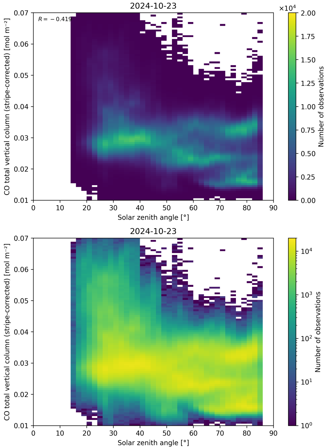
Figure 62: Scatter density plot of “Solar zenith angle” against “CO total vertical column (stripe-corrected)” for 2024-10-22 to 2024-10-24.
