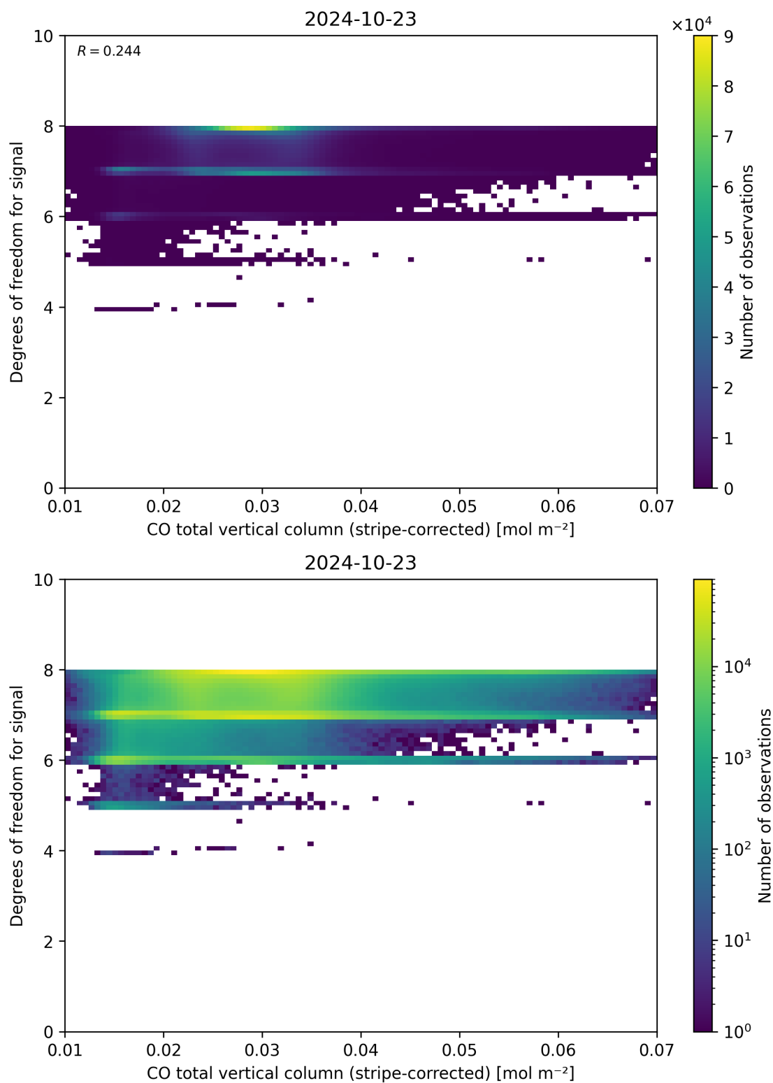
Figure 38: Scatter density plot of “CO total vertical column (stripe-corrected)” against “Degrees of freedom for signal” for 2024-10-22 to 2024-10-24.
