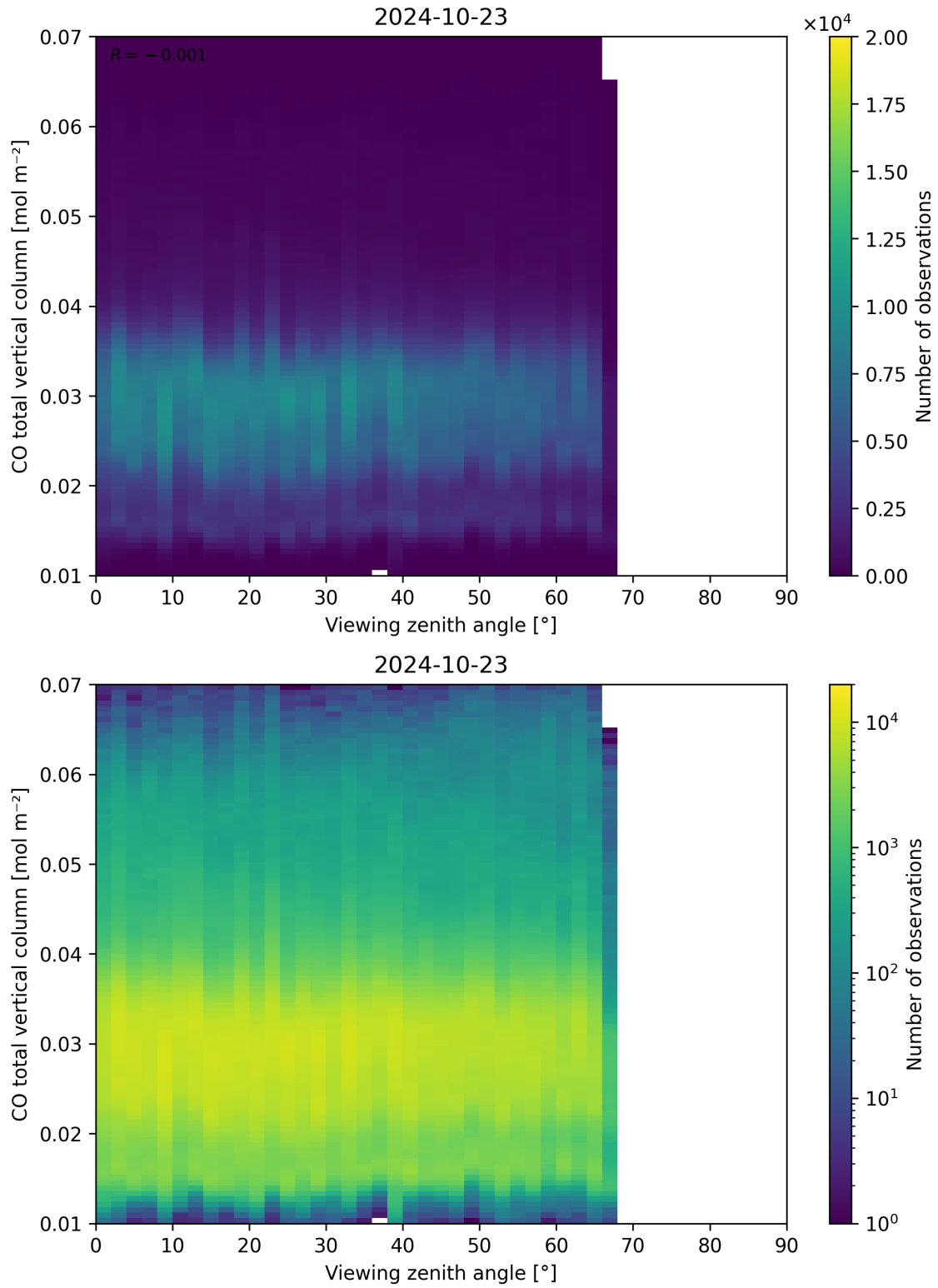
Figure 69: Scatter density plot of “Viewing zenith angle” against “CO total vertical column” for 2024-10-22 to 2024-10-24.
