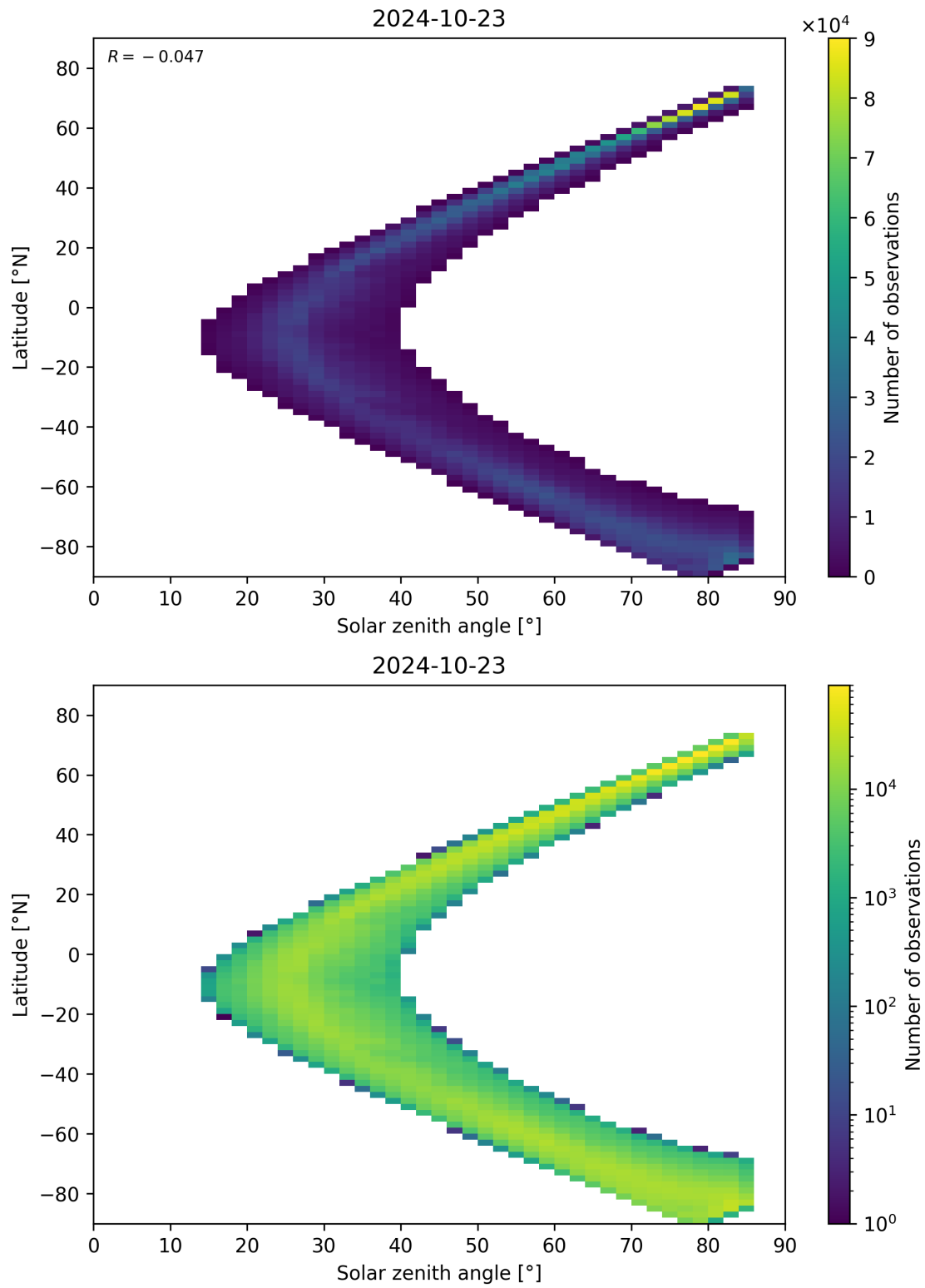
Figure 66: Scatter density plot of “Solar zenith angle” against “Latitude” for 2024-10-22 to 2024-10-24.
