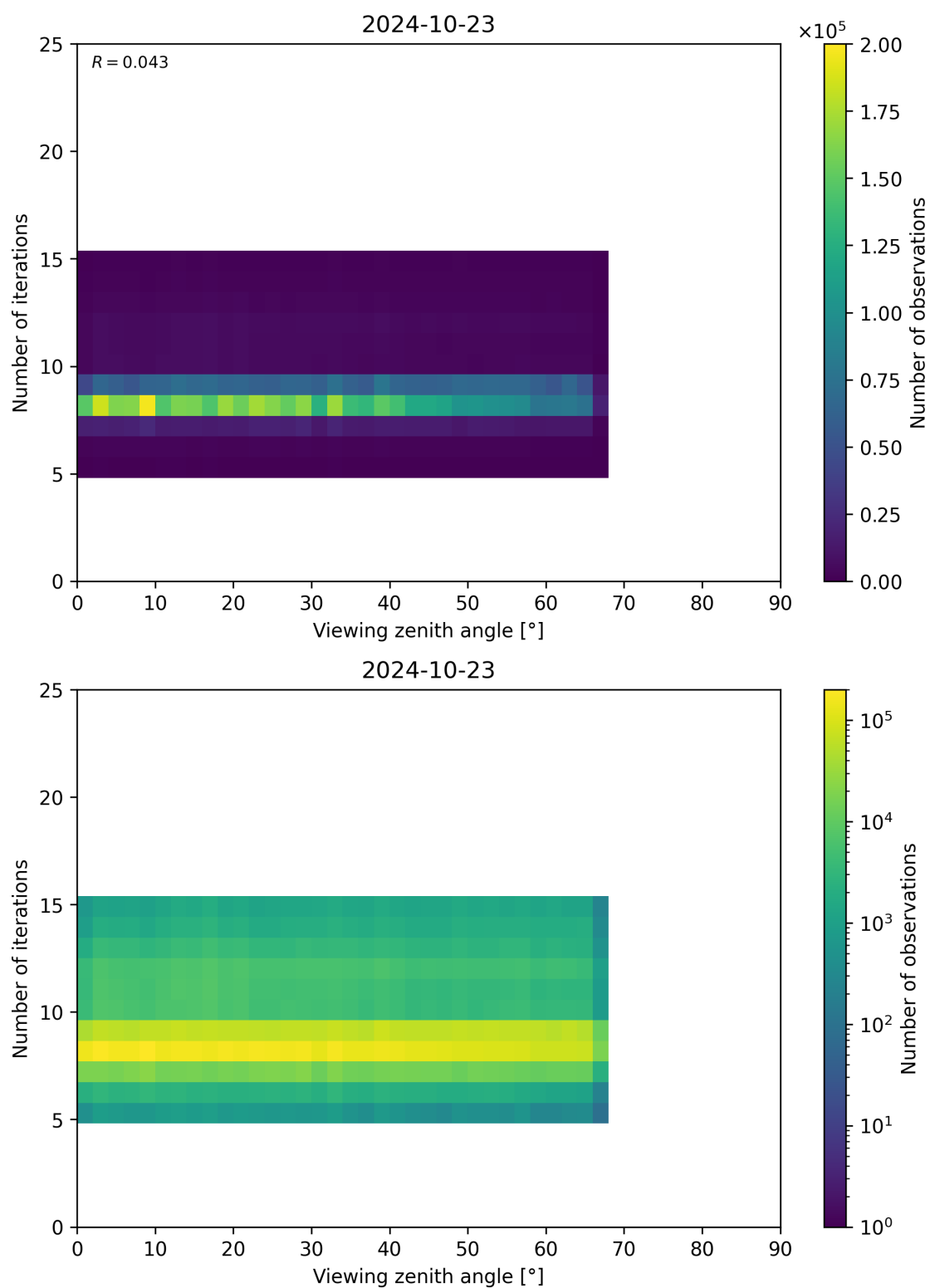
Figure 75: Scatter density plot of “Viewing zenith angle” against “Number of iterations” for 2024-10-22 to 2024-10-24.
