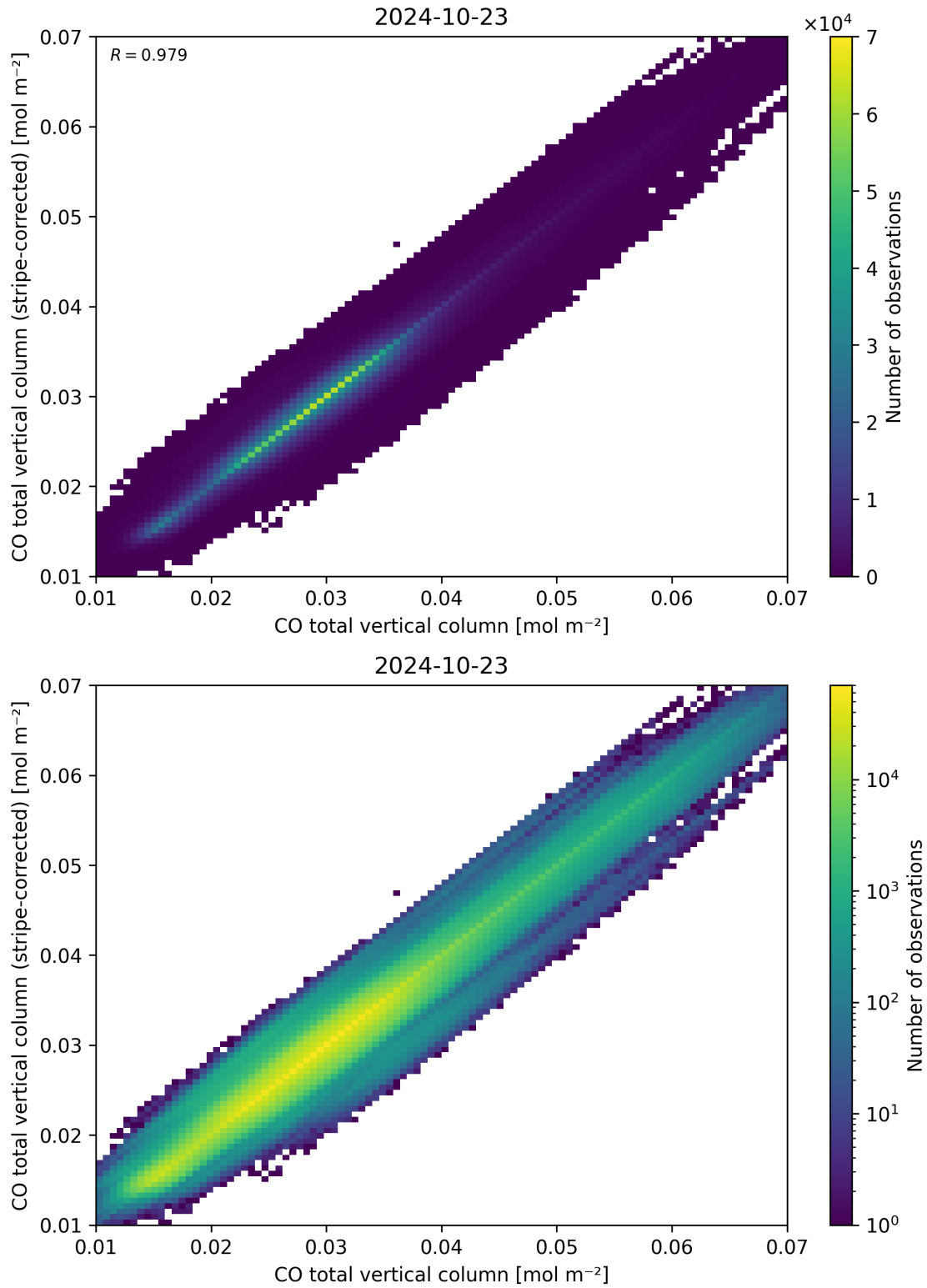
Figure 33: Scatter density plot of “CO total vertical column” against “CO total vertical column (stripe-corrected)” for 2024-10-22 to 2024-10-24.
