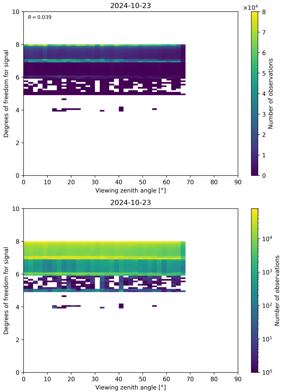
Figure 73: Scatter density plot of “Viewing zenith angle” against “Degrees of freedom for signal” for 2024-10-22 to 2024-10-24.
