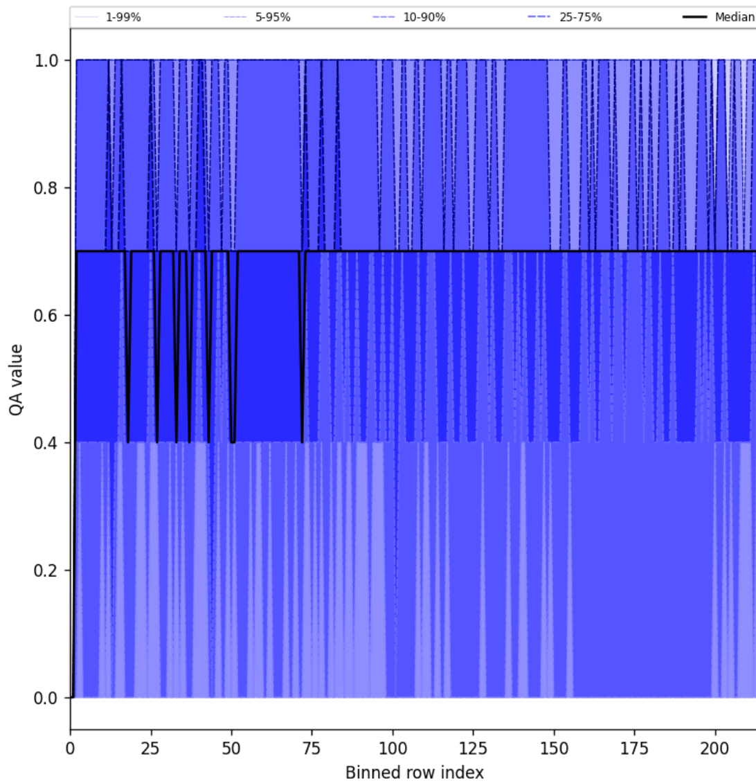
Figure 25: Along track statistics of “QA value” for 2024-10-22 to 2024-10-24
