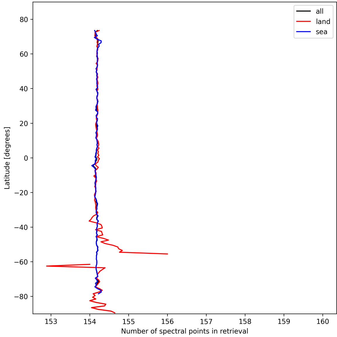
Figure 13: Zonal average of “Number of spectral points in retrieval” for 2024-10-22 to 2024-10-24.
