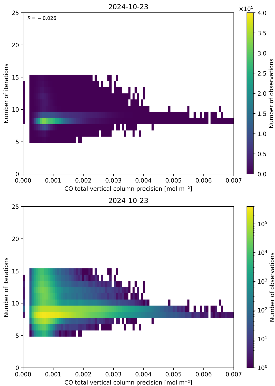
Figure 46: Scatter density plot of “CO total vertical column precision” against “Number of iterations” for 2024-10-22 to 2024-10-24.
