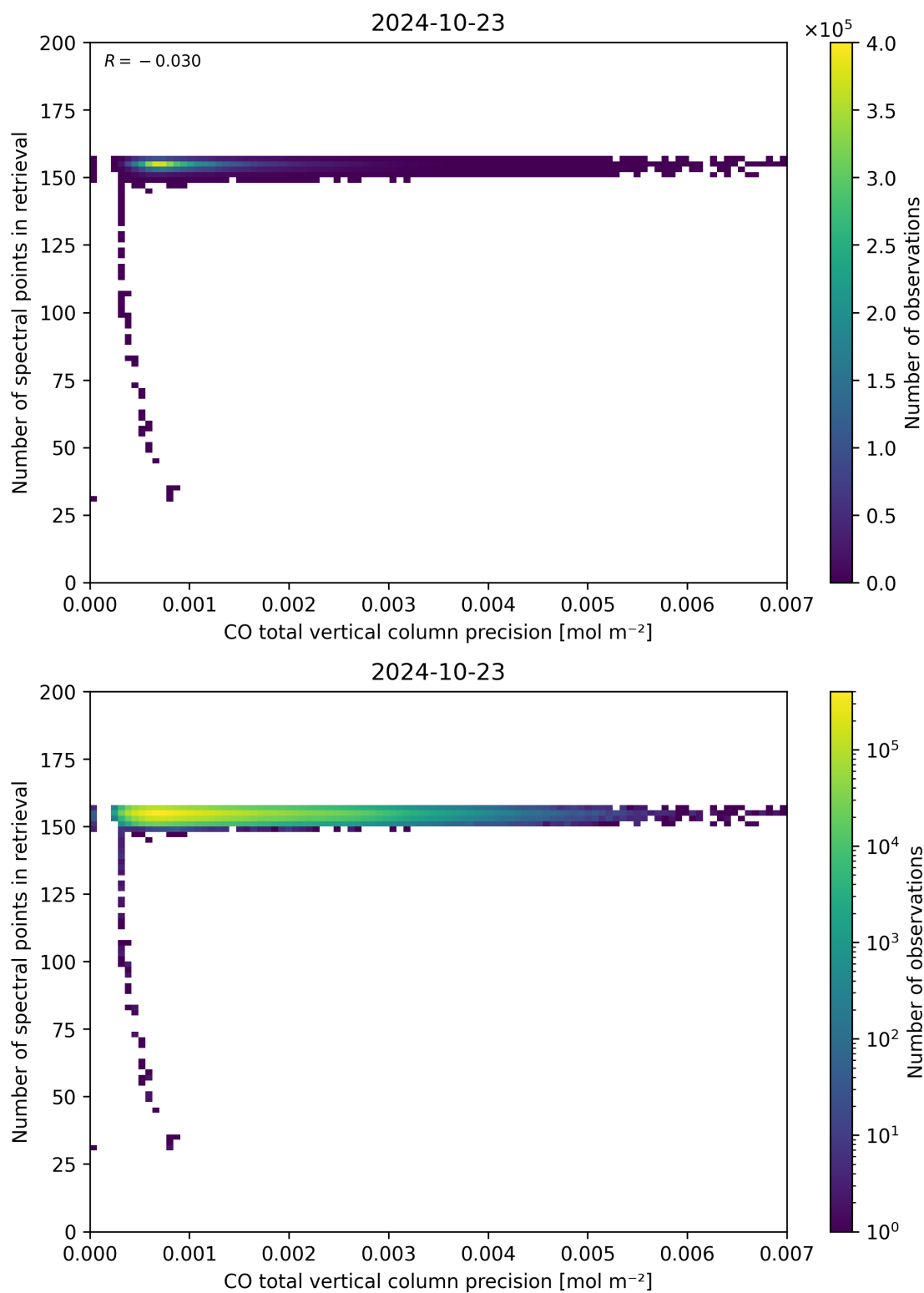
Figure 47: Scatter density plot of “CO total vertical column precision” against “Number of spectral points in retrieval” for 2024-10-22 to 2024-10-24.
