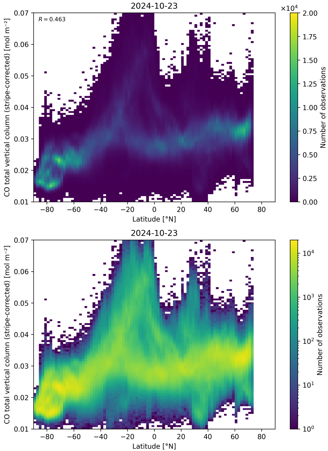
Figure 52: Scatter density plot of “Latitude” against “CO total vertical column (stripe-corrected)” for 2024-10-22 to 2024-10-24.
