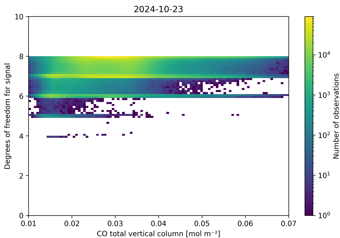
Figure 41: Scatter density plot of “CO total vertical column” against “Degrees of freedom for signal” for 2024-10-22 to 2024-10-24.
