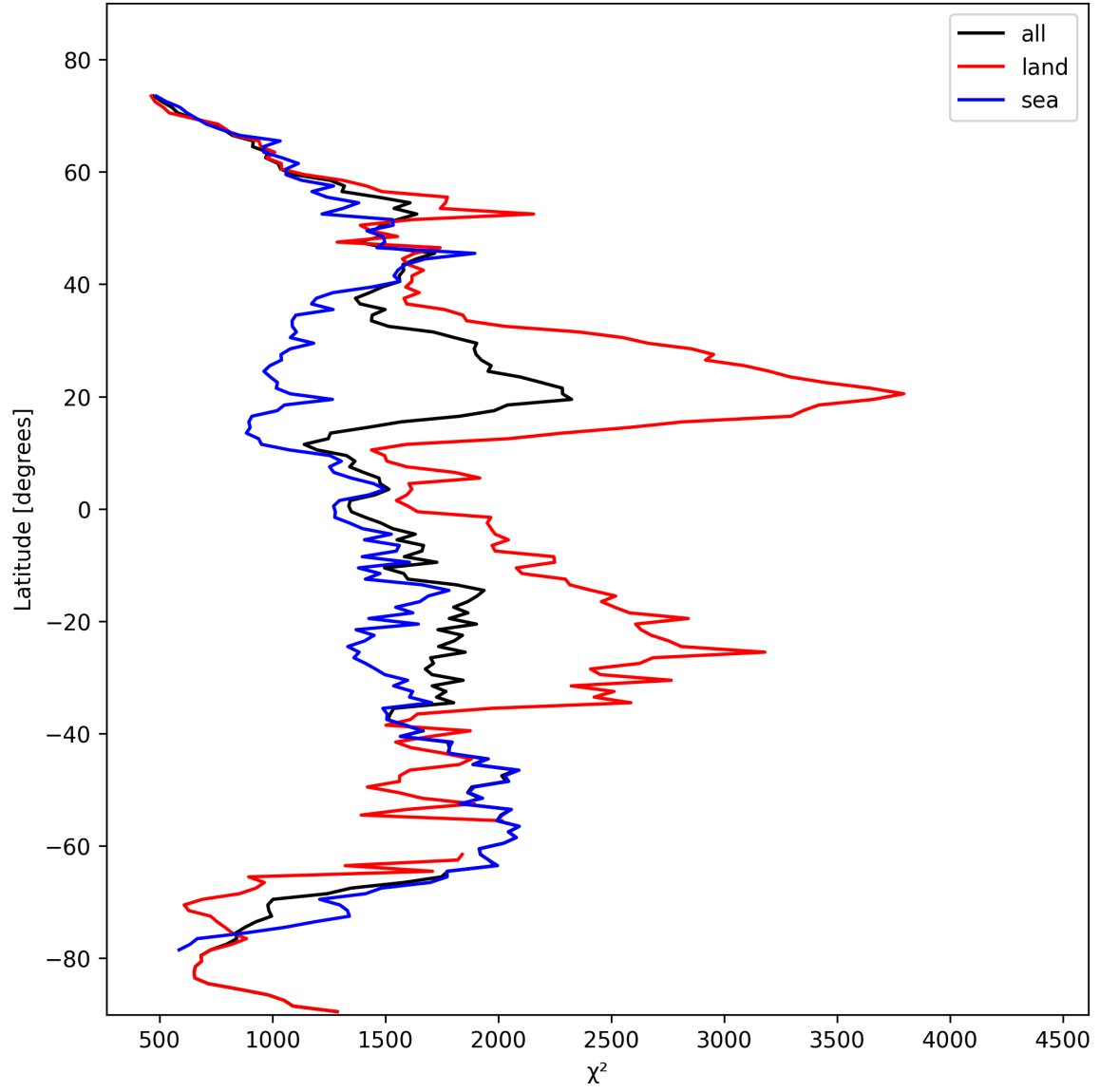
Figure 14: Zonal average of “ \chi^2 ” for 2024-10-22 to 2024-10-24.
