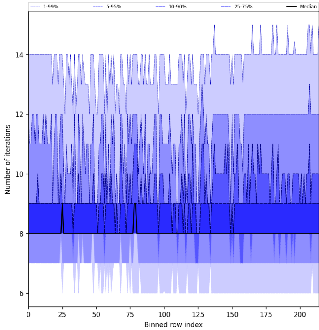
Figure 32: Along track statistics of “Number of iterations” for 2024-10-22 to 2024-10-24
