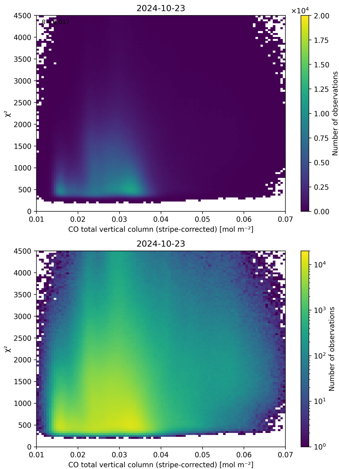
Figure 37: Scatter density plot of “CO total vertical column (stripe-corrected)” against “ \chi^2 ” for 2024-10-22 to 2024-10-24.
