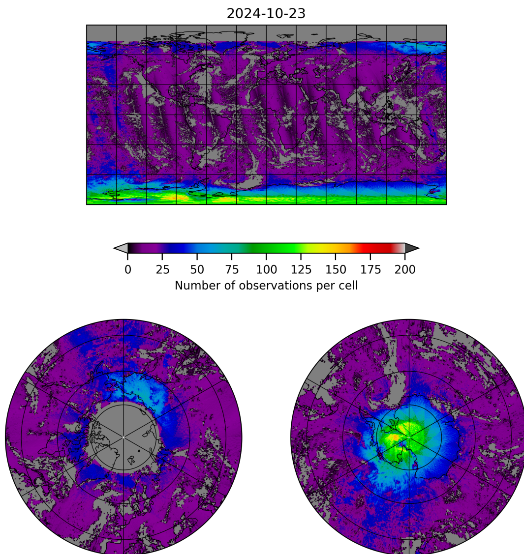
Figure 8: Map of the number of observations for 2024-10-22 to 2024-10-24
