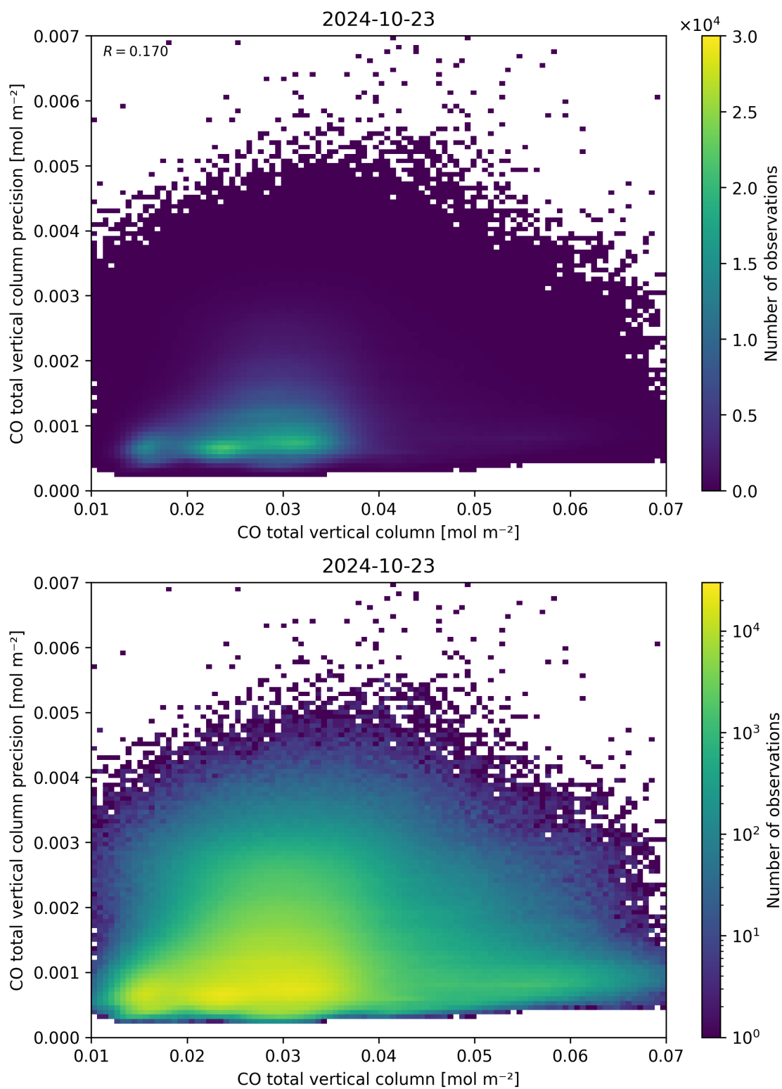
Figure 34: Scatter density plot of “CO total vertical column” against “CO total vertical column precision” for 2024-10-22 to 2024-10-24.
