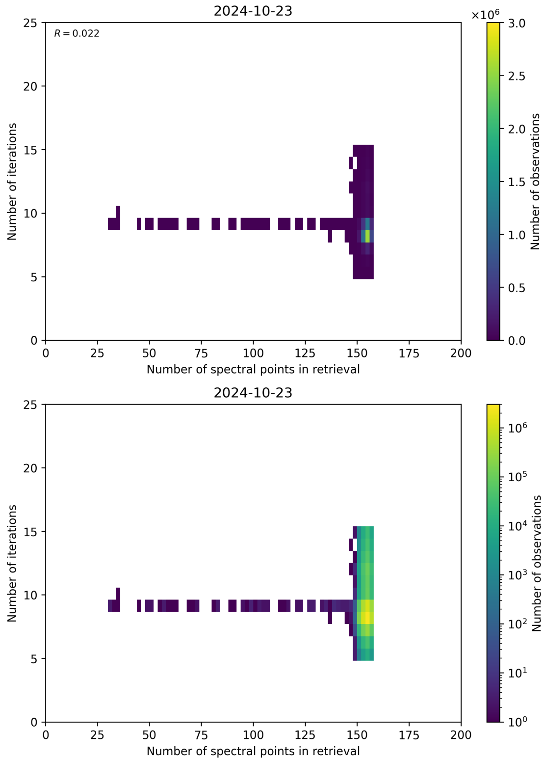
Figure 60: Scatter density plot of “Number of spectral points in retrieval” against “Number of iterations” for 2024-10-22 to 2024-10-24.
