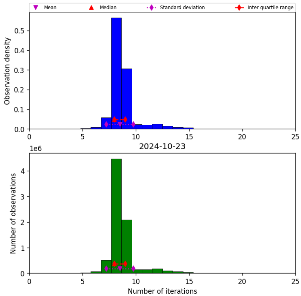
Figure 24: Histogram of “Number of iterations” for 2024-10-22 to 2024-10-24
