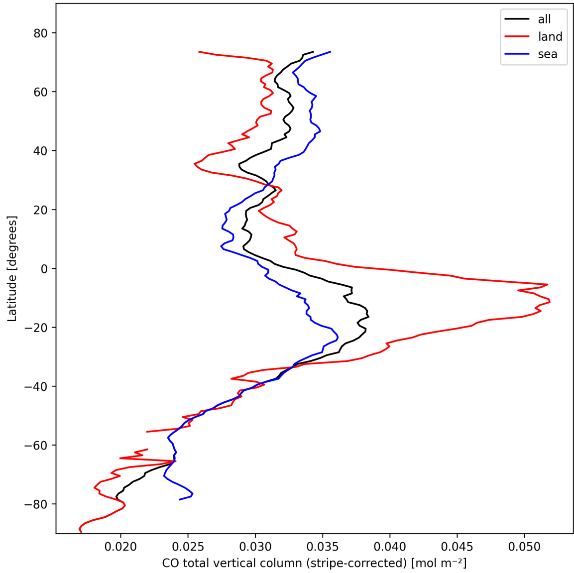
Figure 11: Zonal average of “CO total vertical column (stripe-corrected)” for 2024-10-22 to 2024-10-24.
