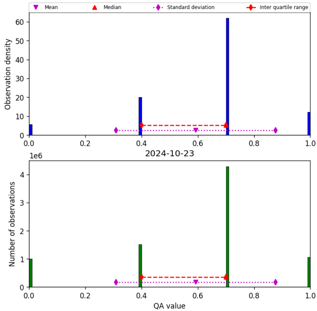
Figure 17: Histogram of “QA value” for 2024-10-22 to 2024-10-24
