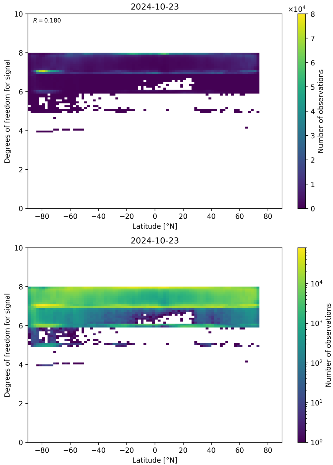
Figure 55: Scatter density plot of “Latitude” against “Degrees of freedom for signal” for 2024-10-22 to 2024-10-24.
