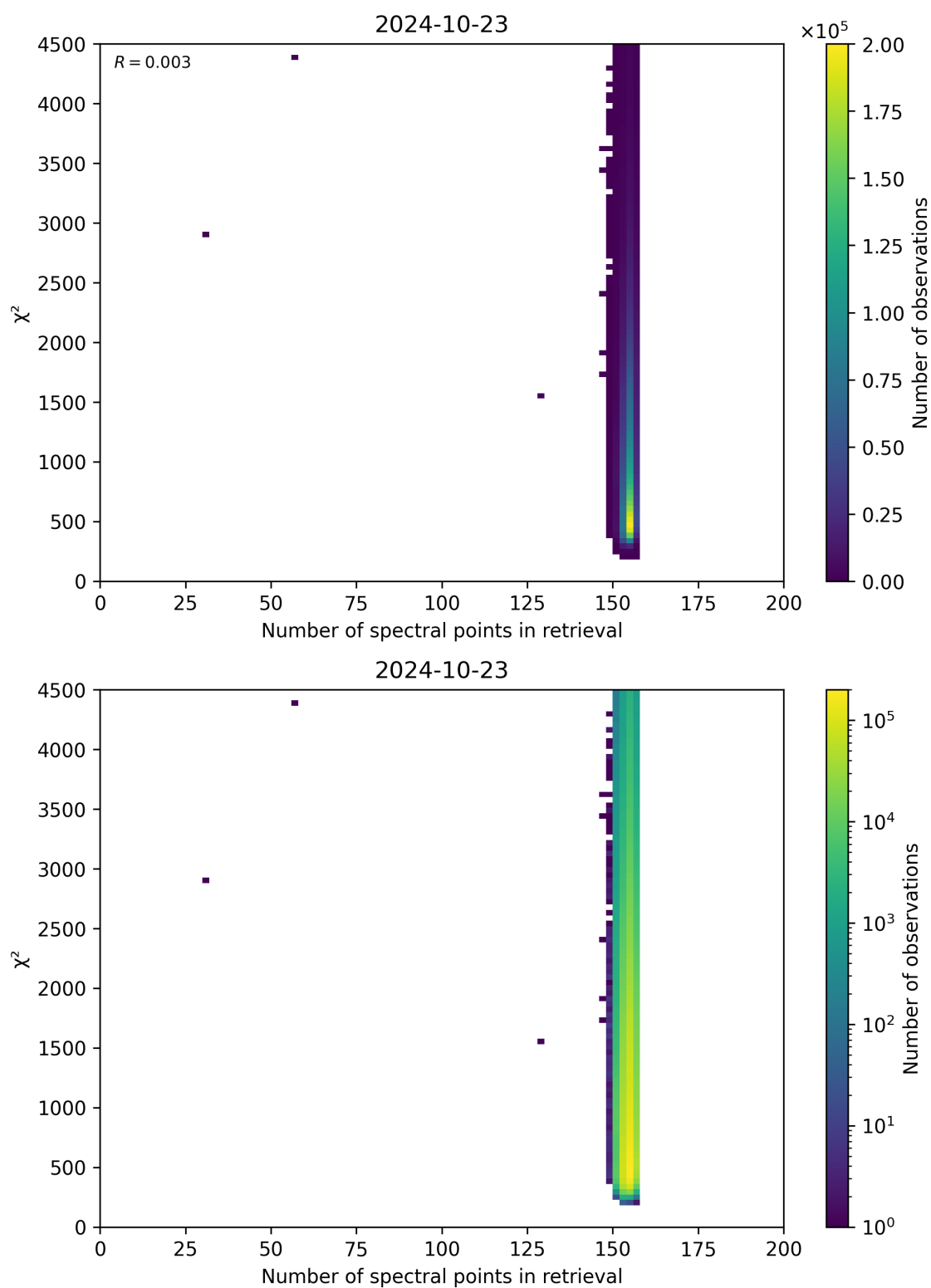
Figure 58: Scatter density plot of “Number of spectral points in retrieval” against “ \chi^2 ” for 2024-10-22 to 2024-10-24.
