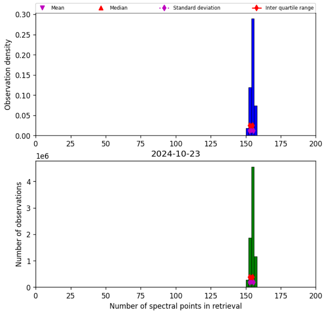
Figure 21: Histogram of “Number of spectral points in retrieval” for 2024-10-22 to 2024-10-24
