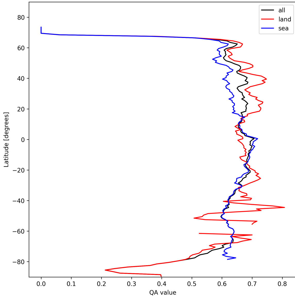
Figure 9: Zonal average of “QA value” for 2024-10-22 to 2024-10-24.
