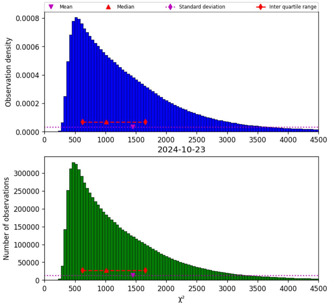
Figure 22: Histogram of “ \chi^2 ” for 2024-10-22 to 2024-10-24
