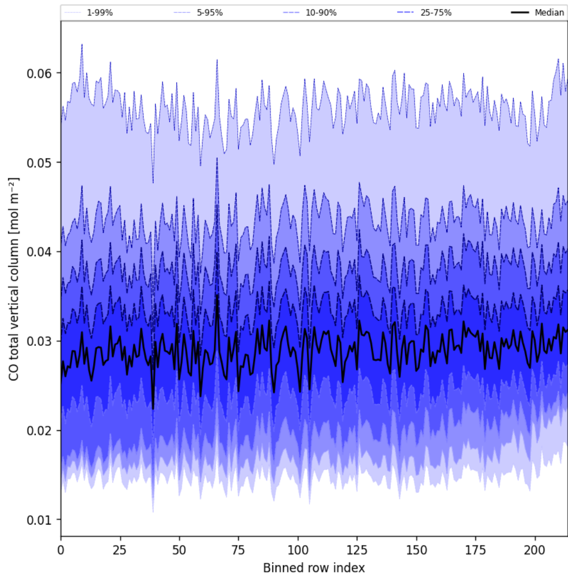
Figure 26: Along track statistics of “CO total vertical column” for 2024-10-22 to 2024-10-24
