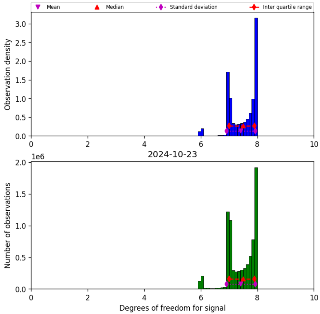
Figure 23: Histogram of “Degrees of freedom for signal” for 2024-10-22 to 2024-10-24
