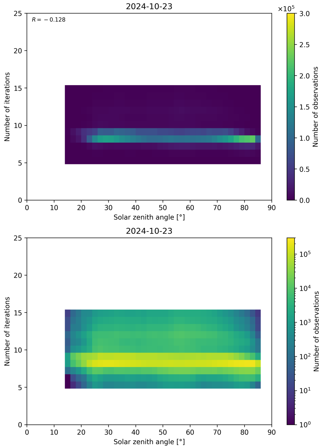
Figure 67: Scatter density plot of “Solar zenith angle” against “Number of iterations” for 2024-10-22 to 2024-10-24.
