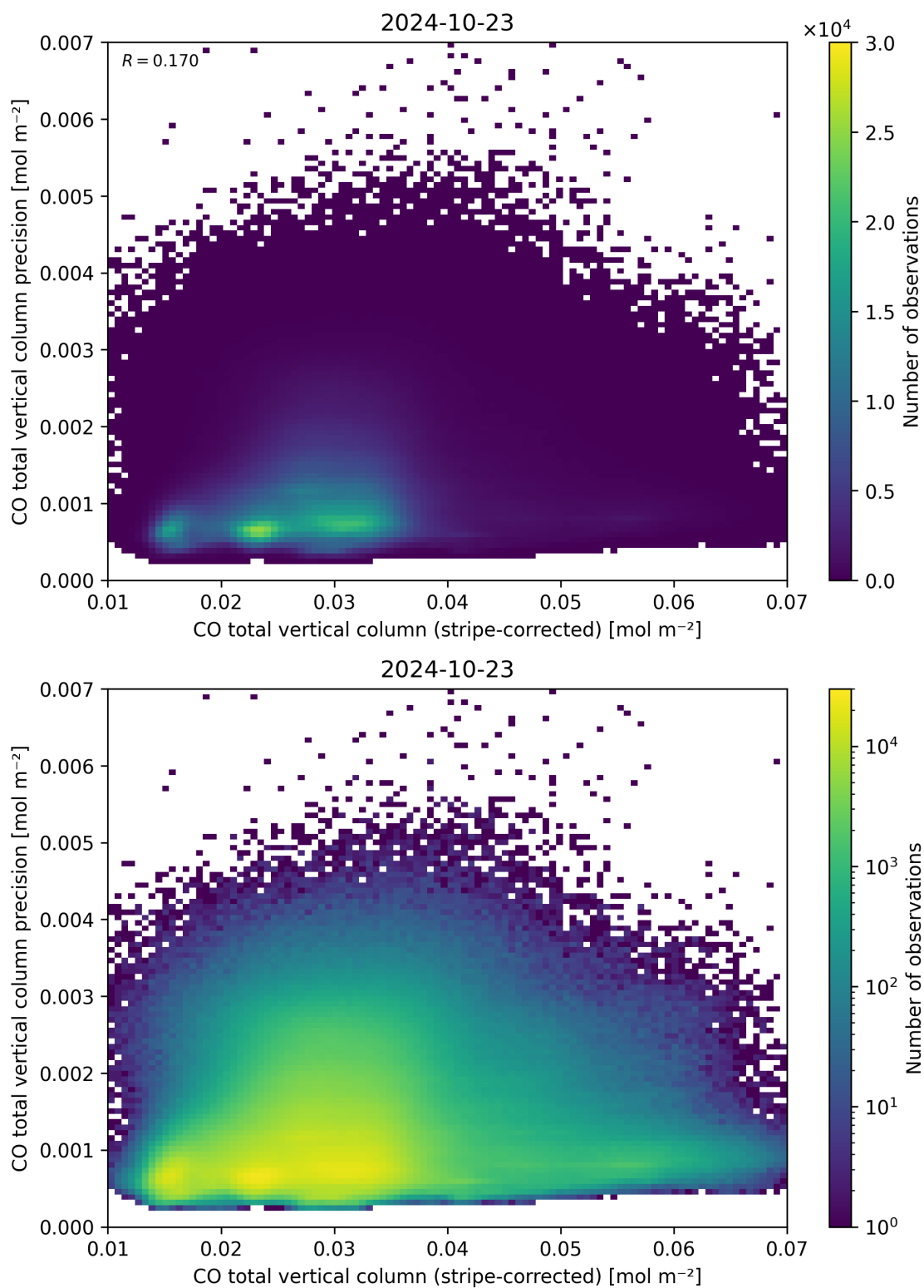
Figure 36: Scatter density plot of “CO total vertical column (stripe-corrected)” against “CO total vertical column precision” for 2024-10-22 to 2024-10-24.
