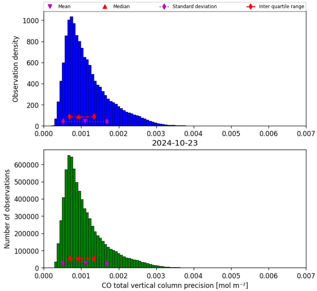
Figure 20: Histogram of “CO total vertical column precision” for 2024-10-22 to 2024-10-24
