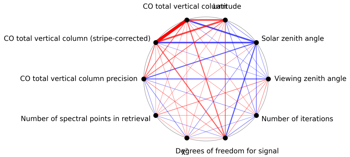
Figure 1: Map of correlation graph for 2024-10-22 to 2024-10-24.
