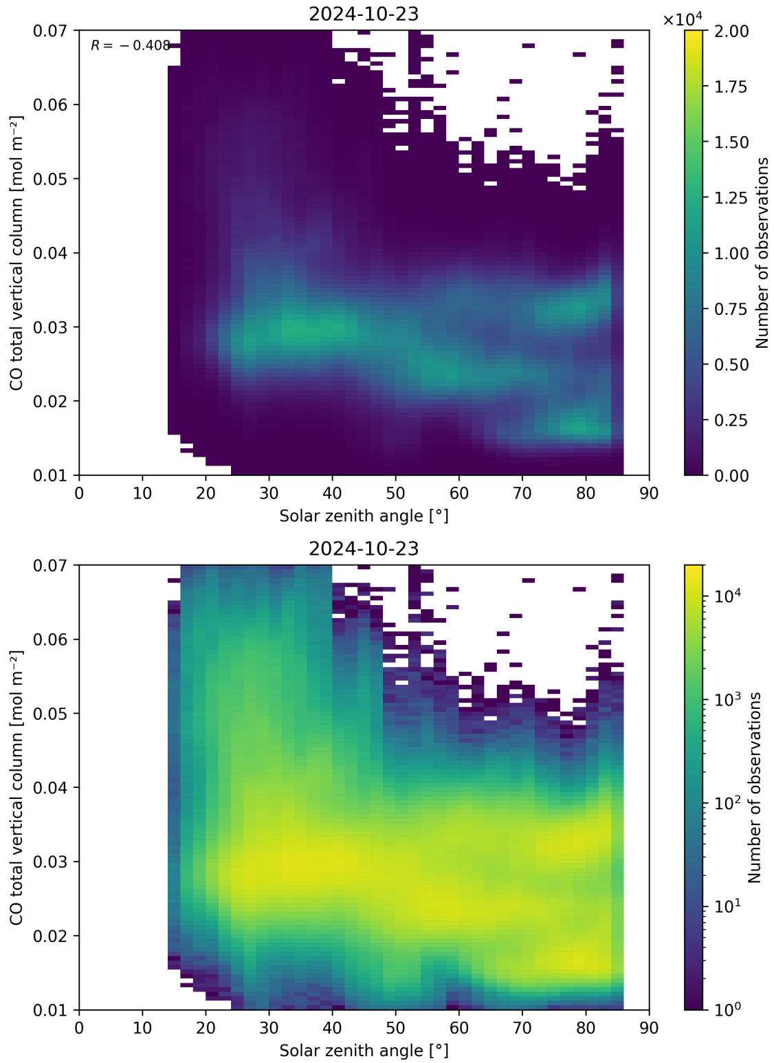
Figure 61: Scatter density plot of “Solar zenith angle” against “CO total vertical column” for 2024-10-22 to 2024-10-24.
