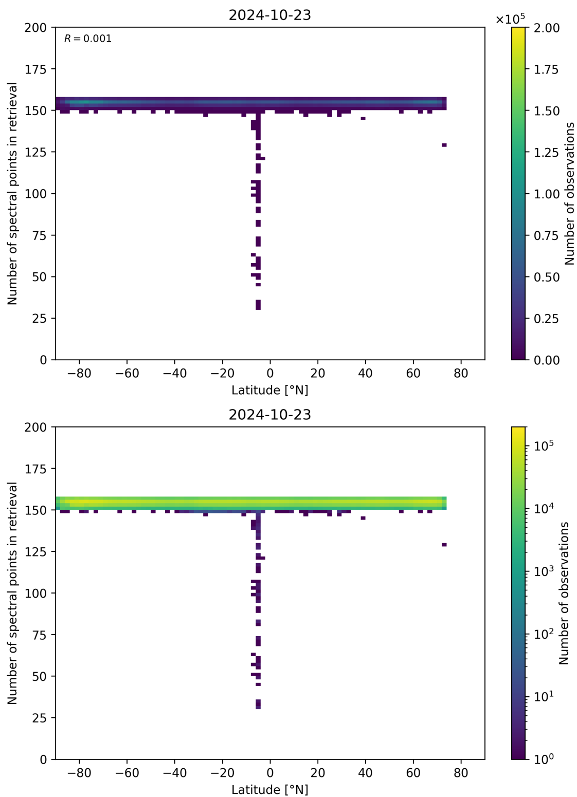
Figure 57: Scatter density plot of “Latitude” against “Number of spectral points in retrieval” for 2024-10-22 to 2024-10-24.
