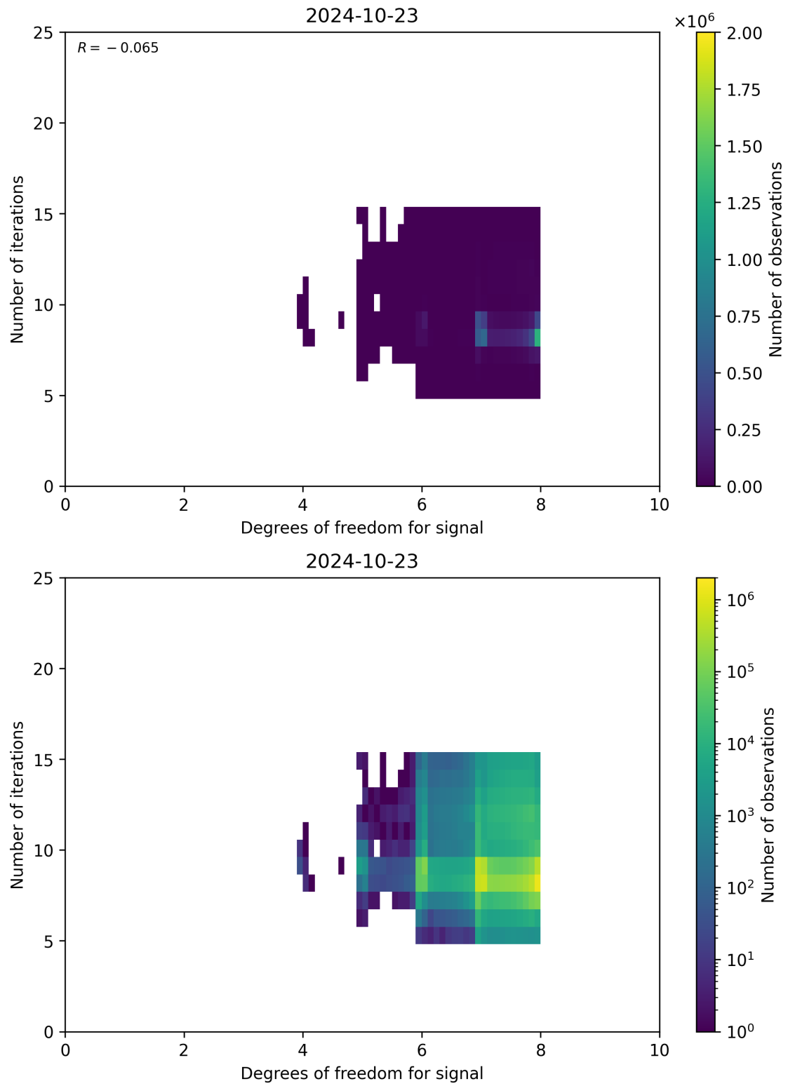
Figure 50: Scatter density plot of “Degrees of freedom for signal” against “Number of iterations” for 2024-10-22 to 2024-10-24.
