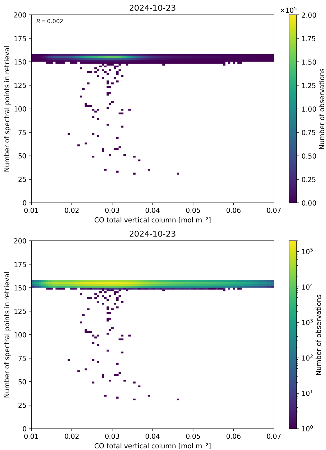
Figure 43: Scatter density plot of “CO total vertical column” against “Number of spectral points in retrieval” for 2024-10-22 to 2024-10-24.
