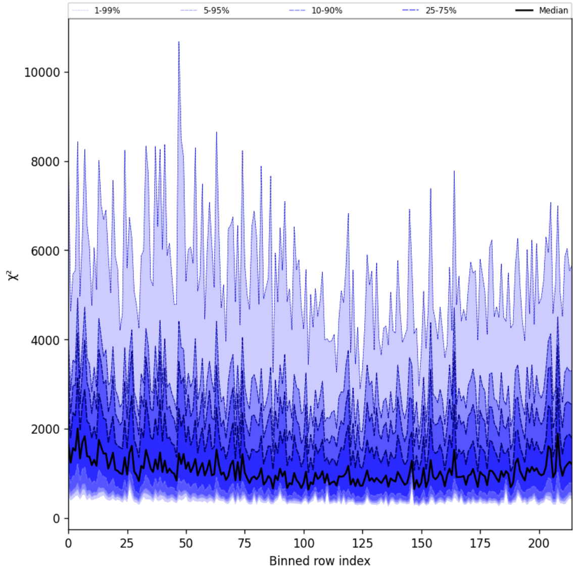
Figure 30: Along track statistics of “ \chi^2 ” for 2024-10-22 to 2024-10-24
