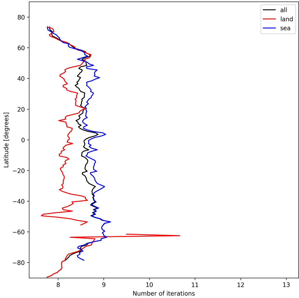
Figure 16: Zonal average of “Number of iterations” for 2024-10-22 to 2024-10-24.
