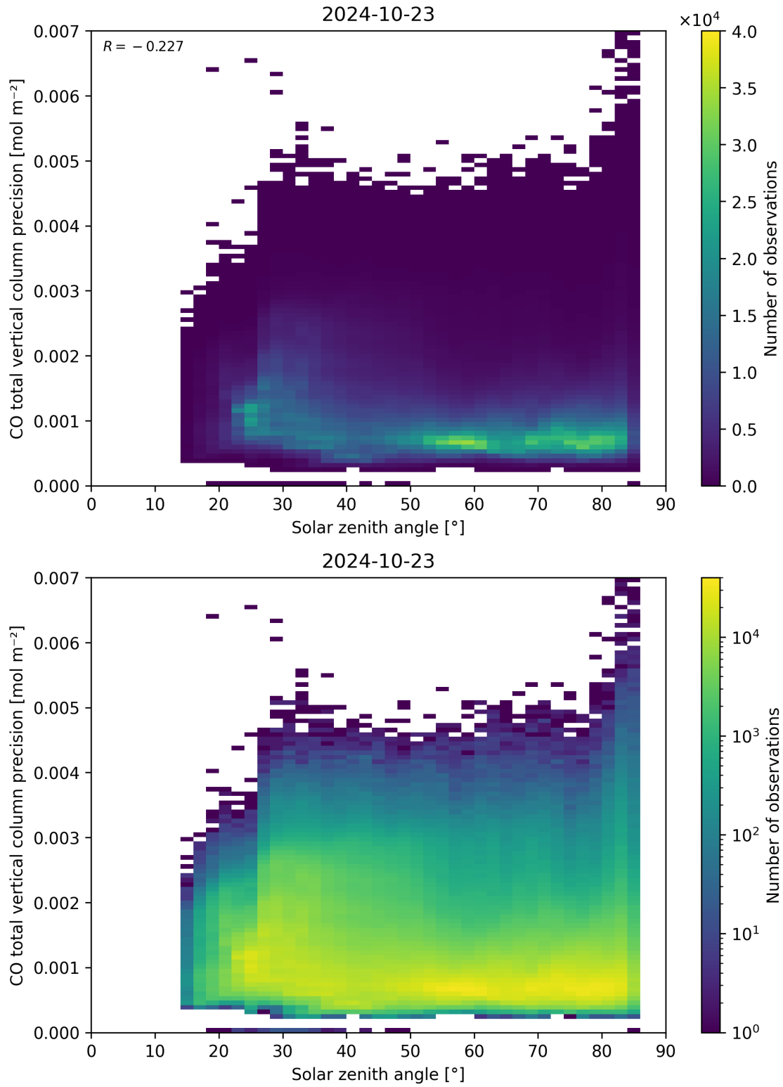
Figure 63: Scatter density plot of “Solar zenith angle” against “CO total vertical column precision” for 2024-10-22 to 2024-10-24.
