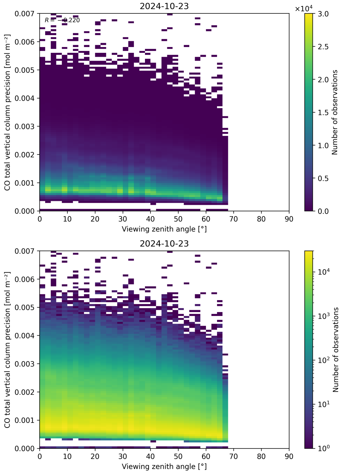
Figure 71: Scatter density plot of “Viewing zenith angle” against “CO total vertical column precision” for 2024-10-22 to 2024-10-24.
