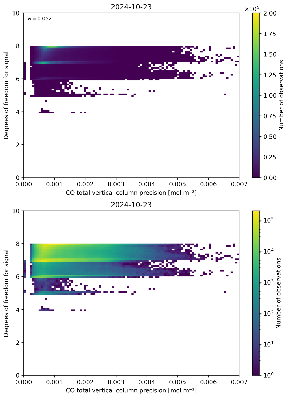
Figure 45: Scatter density plot of “CO total vertical column precision” against “Degrees of freedom for signal” for 2024-10-22 to 2024-10-24.
