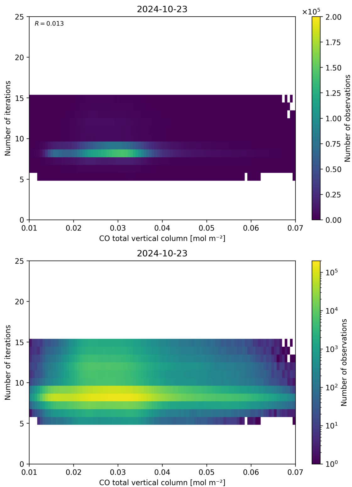
Figure 42: Scatter density plot of “CO total vertical column” against “Number of iterations” for 2024-10-22 to 2024-10-24.
