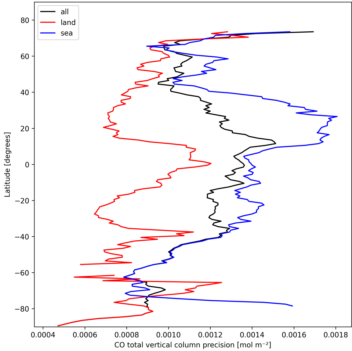
Figure 12: Zonal average of “CO total vertical column precision” for 2024-10-22 to 2024-10-24.
