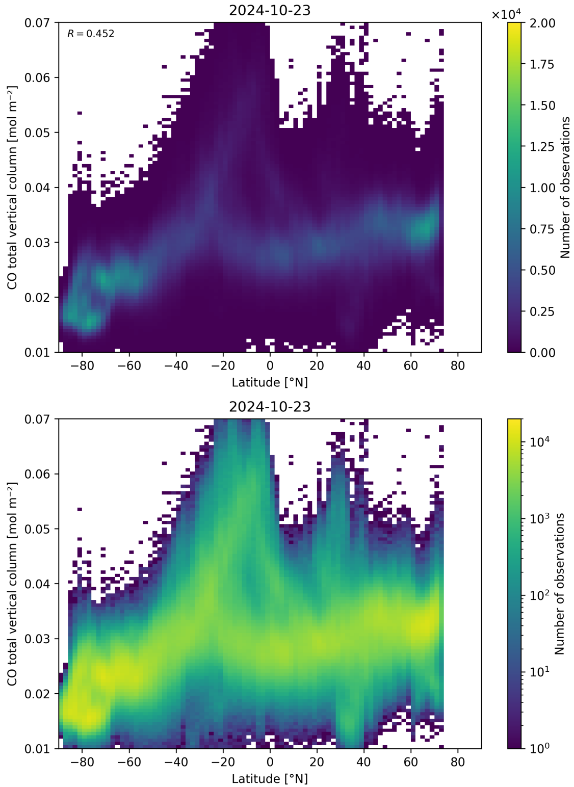
Figure 51: Scatter density plot of “Latitude” against “CO total vertical column” for 2024-10-22 to 2024-10-24.
