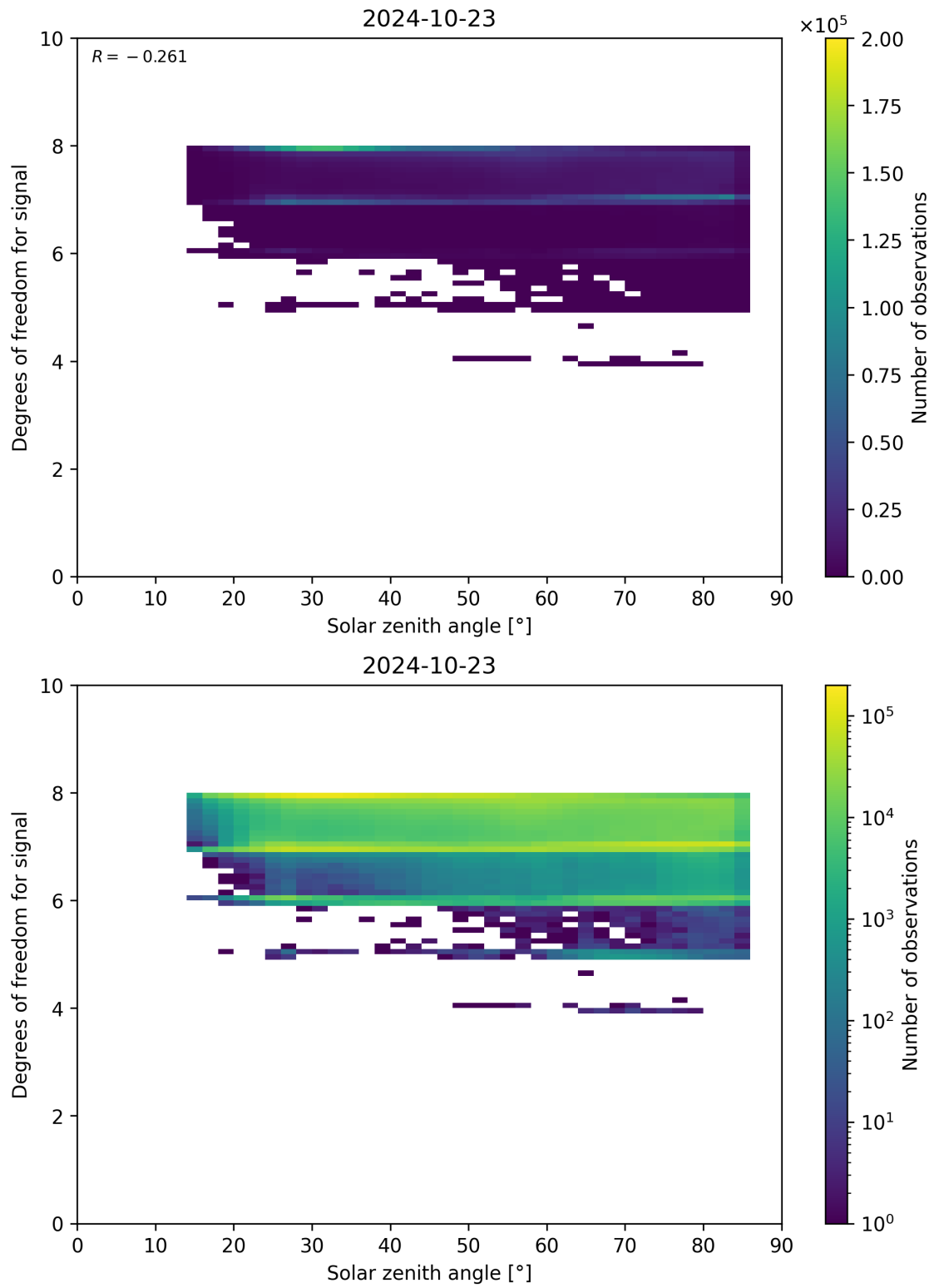
Figure 65: Scatter density plot of “Solar zenith angle” against “Degrees of freedom for signal” for 2024-10-22 to 2024-10-24.
