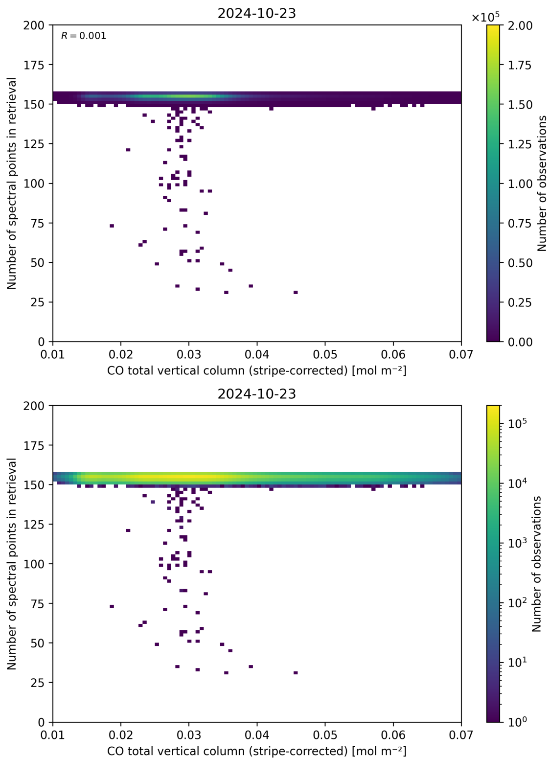
Figure 40: Scatter density plot of “CO total vertical column (stripe-corrected)” against “Number of spectral points in retrieval” for 2024-10-22 to 2024-10-24.
