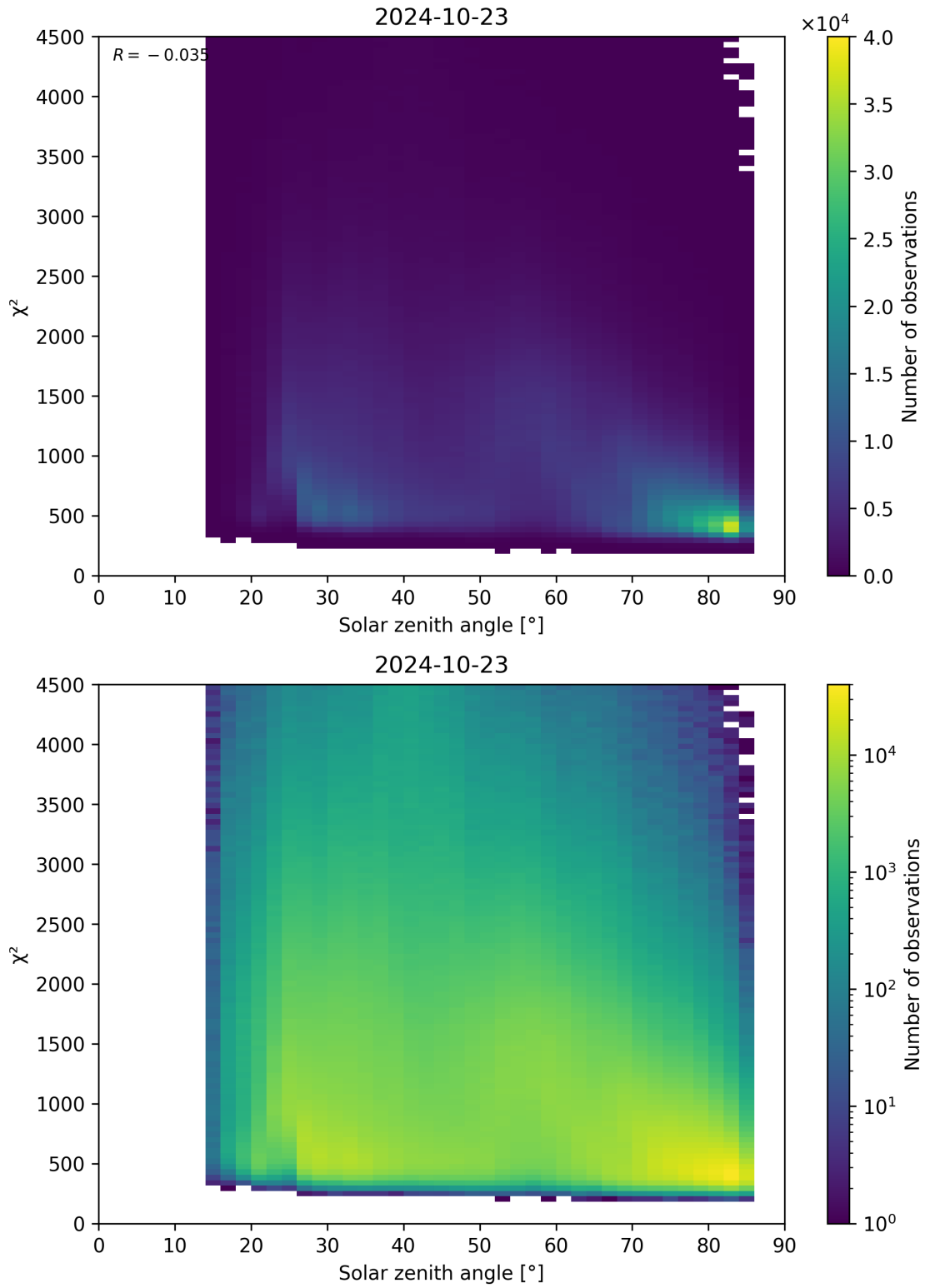
Figure 64: Scatter density plot of “Solar zenith angle” against “ \chi^2 ” for 2024-10-22 to 2024-10-24.
