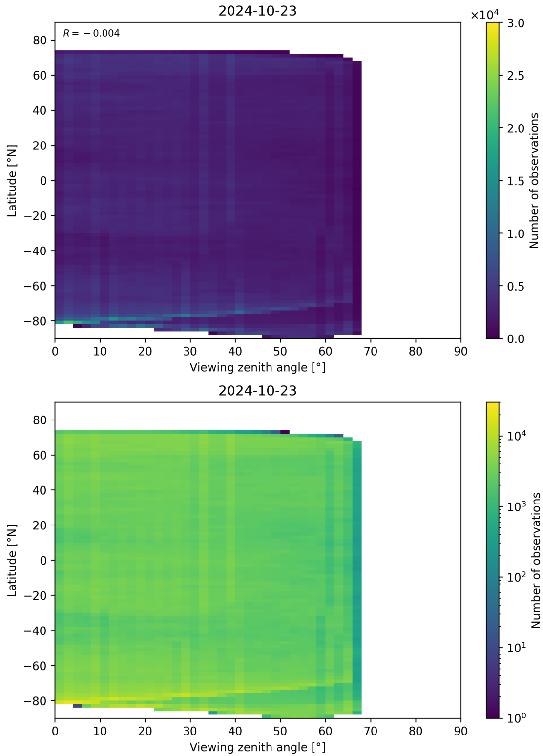
Figure 74: Scatter density plot of “Viewing zenith angle” against “Latitude” for 2024-10-22 to 2024-10-24.
