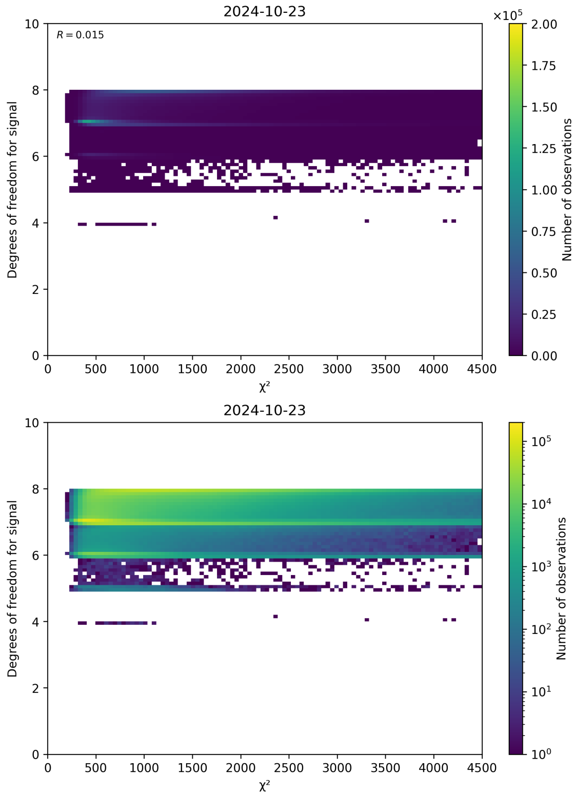
Figure 48: Scatter density plot of “ \chi^2 ” against “Degrees of freedom for signal” for 2024-10-22 to 2024-10-24.
