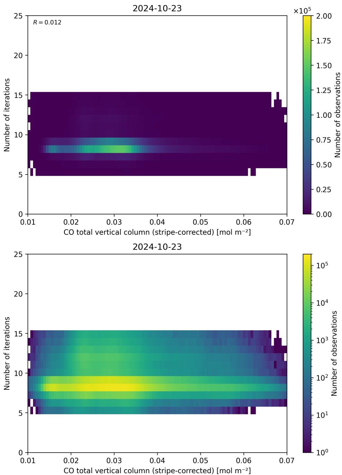
Figure 39: Scatter density plot of “CO total vertical column (stripe-corrected)” against “Number of iterations” for 2024-10-22 to 2024-10-24.
