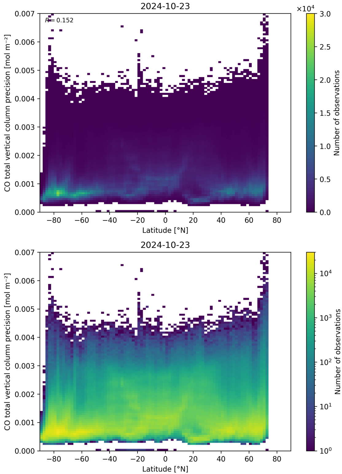
Figure 53: Scatter density plot of “Latitude” against “CO total vertical column precision” for 2024-10-22 to 2024-10-24.
