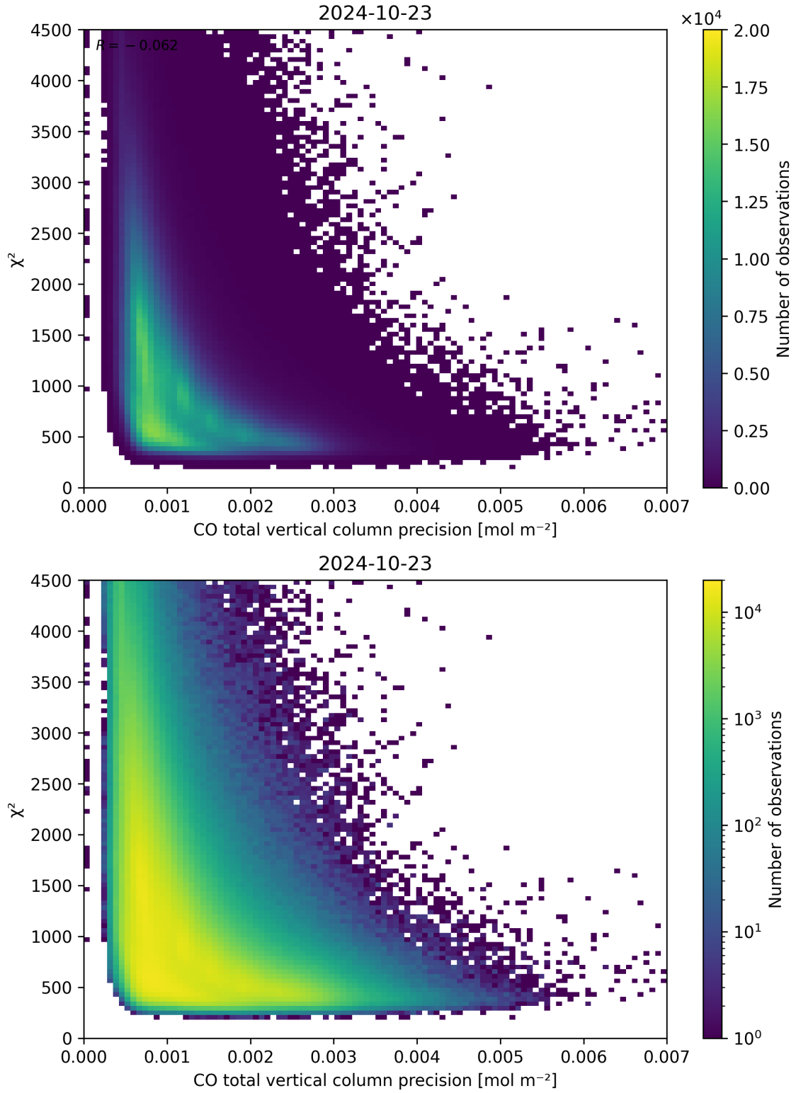
Figure 44: Scatter density plot of “CO total vertical column precision” against “ \chi^2 ” for 2024-10-22 to 2024-10-24.
