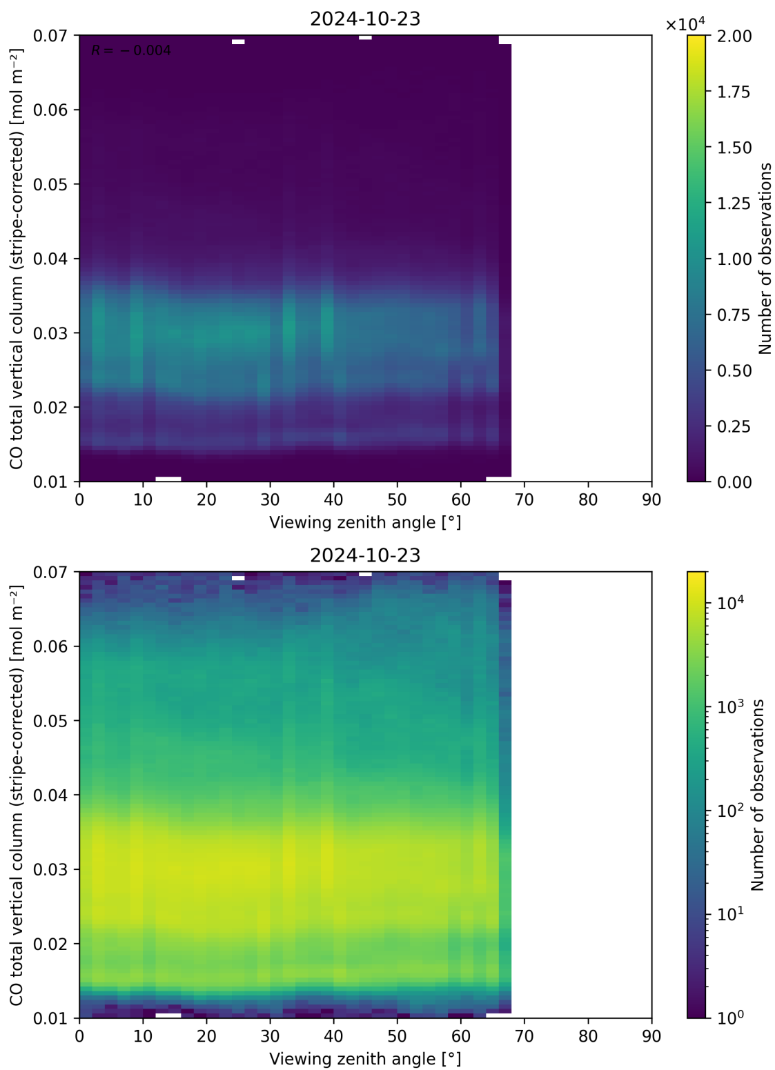
Figure 70: Scatter density plot of “Viewing zenith angle” against “CO total vertical column (stripe-corrected)” for 2024-10-22 to 2024-10-24.
