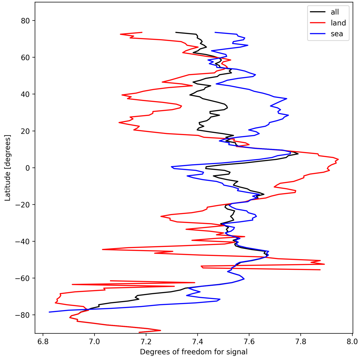
Figure 15: Zonal average of “Degrees of freedom for signal” for 2024-10-22 to 2024-10-24.
