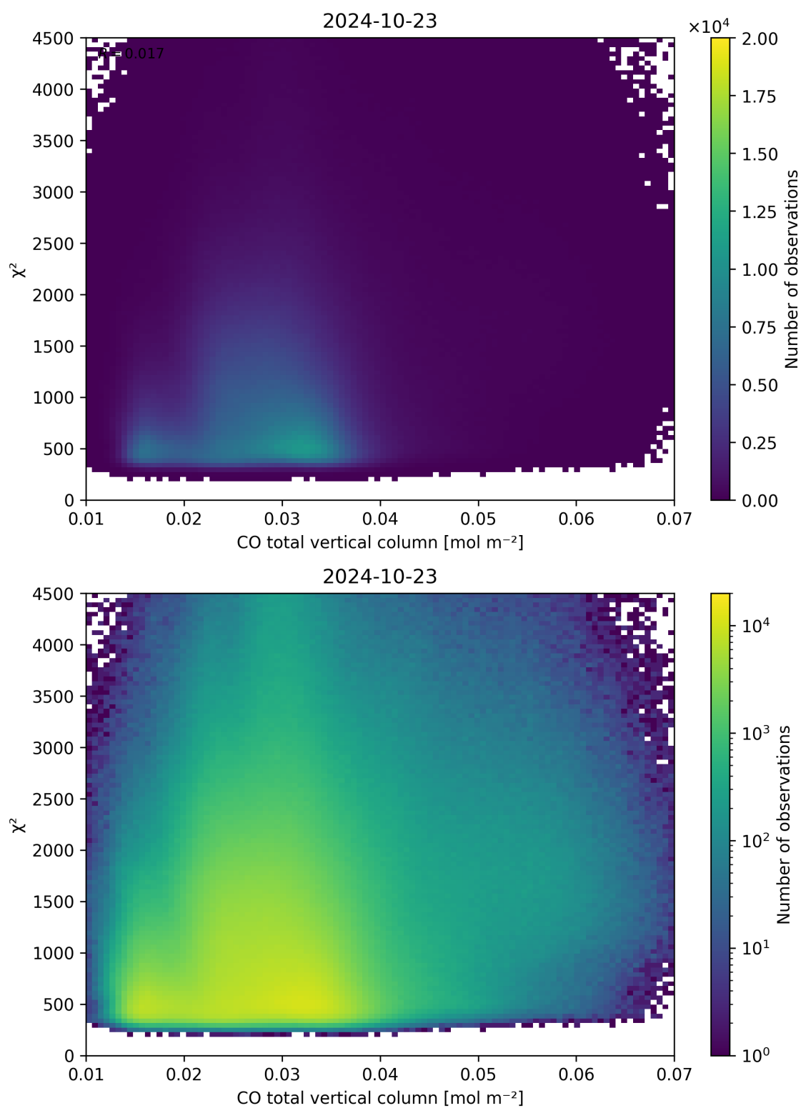
Figure 35: Scatter density plot of “CO total vertical column” against “ \chi^2 ” for 2024-10-22 to 2024-10-24.
