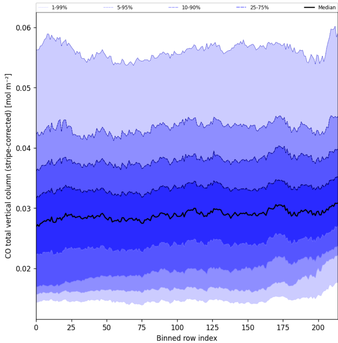
Figure 27: Along track statistics of “CO total vertical column (stripe-corrected)” for 2024-10-22 to 2024-10-24
