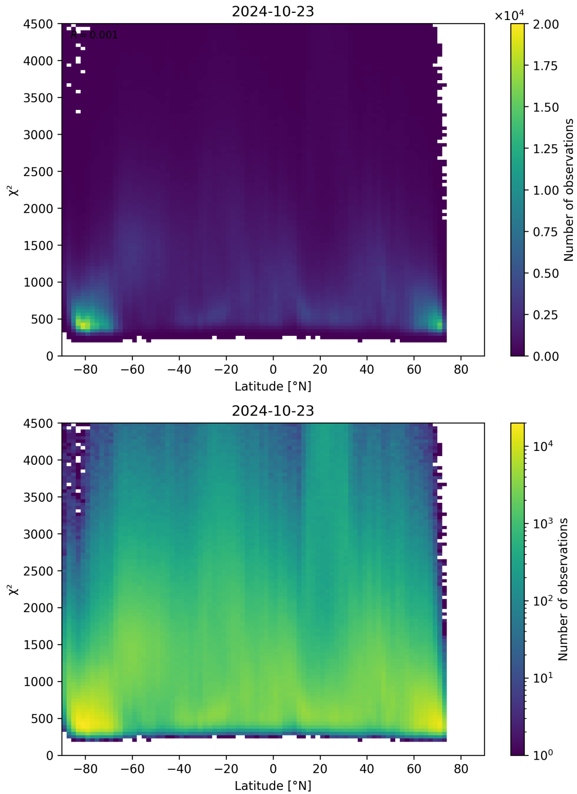
Figure 54: Scatter density plot of “Latitude” against “ \chi^2 ” for 2024-10-22 to 2024-10-24.
