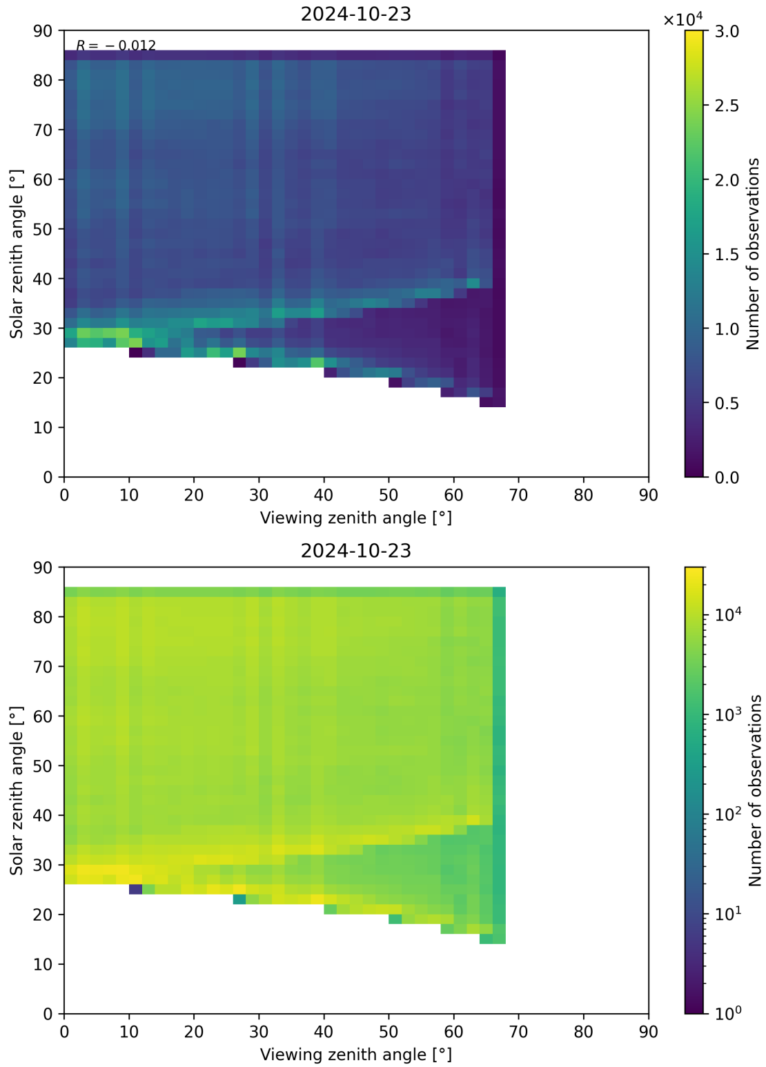
Figure 77: Scatter density plot of “Viewing zenith angle” against “Solar zenith angle” for 2024-10-22 to 2024-10-24.
