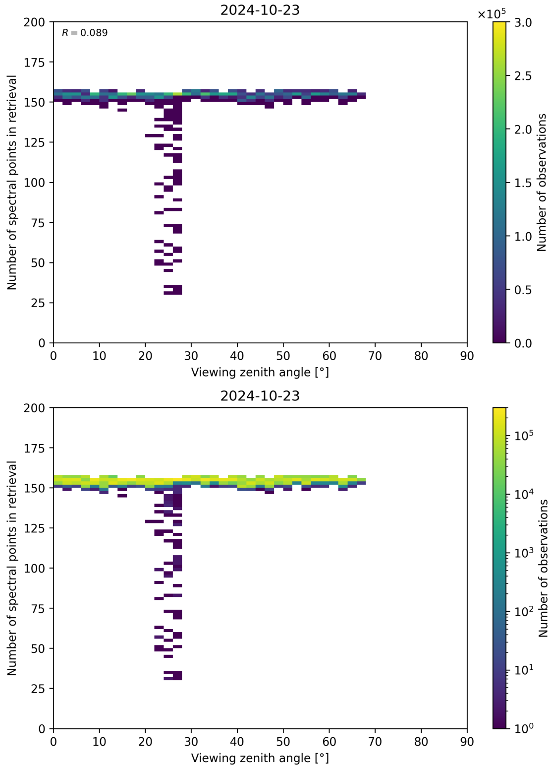
Figure 76: Scatter density plot of “Viewing zenith angle” against “Number of spectral points in retrieval” for 2024-10-22 to 2024-10-24.
