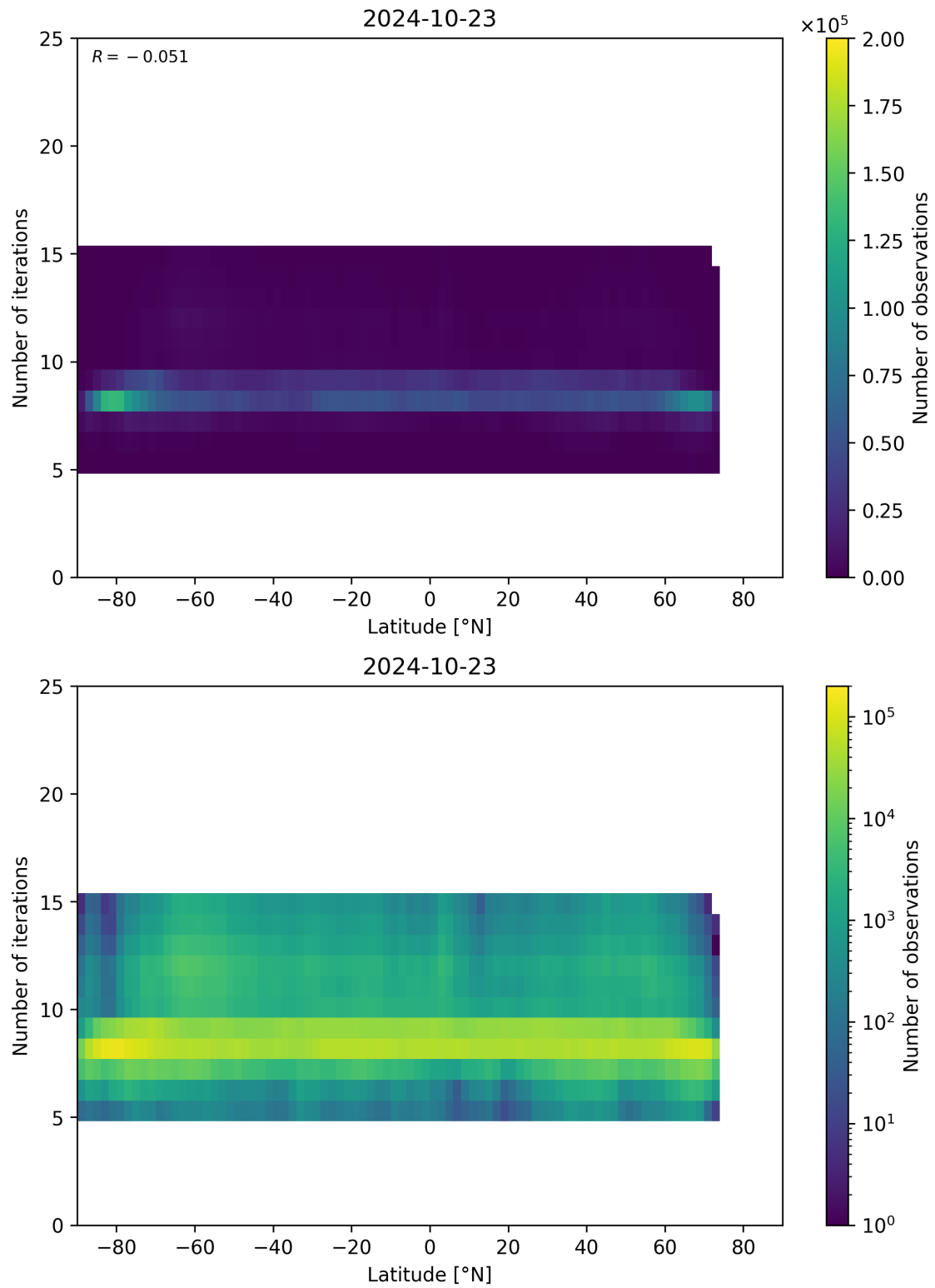
Figure 56: Scatter density plot of “Latitude” against “Number of iterations” for 2024-10-22 to 2024-10-24.
