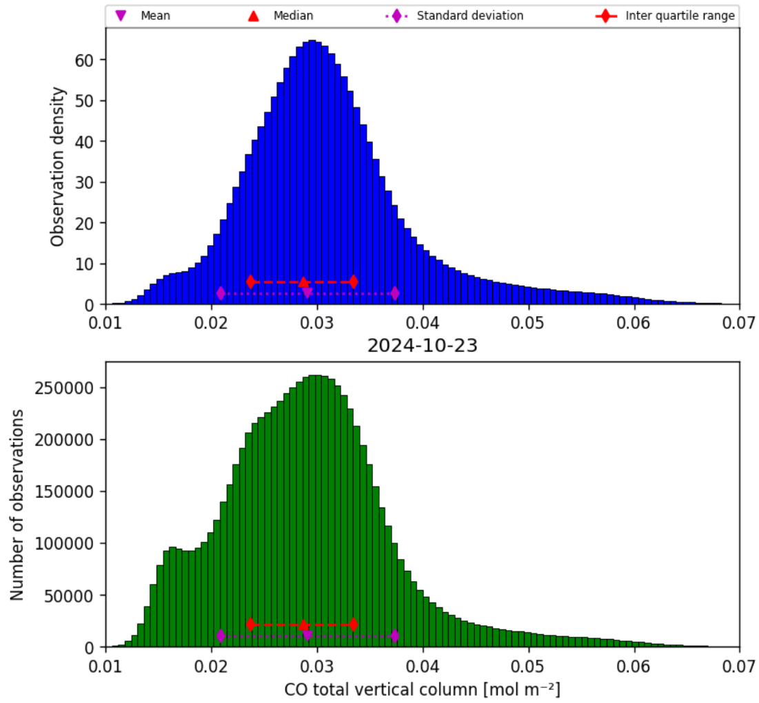
Figure 18: Histogram of “CO total vertical column” for 2024-10-22 to 2024-10-24
