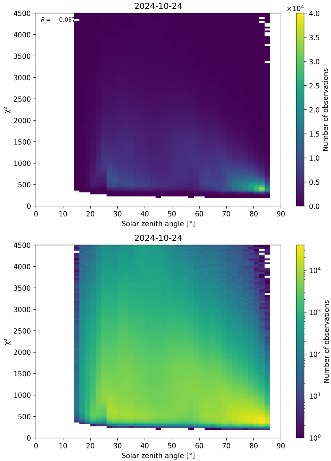
Figure 64: Scatter density plot of “Solar zenith angle” against “ \chi^2 ” for 2024-10-24 to 2024-10-25.
