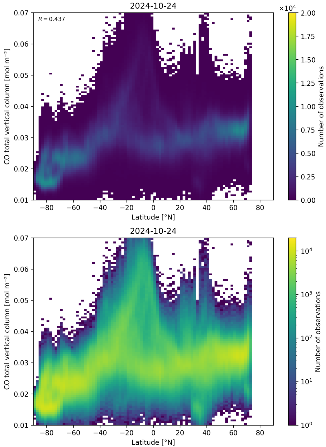
Figure 51: Scatter density plot of “Latitude” against “CO total vertical column” for 2024-10-24 to 2024-10-25.
