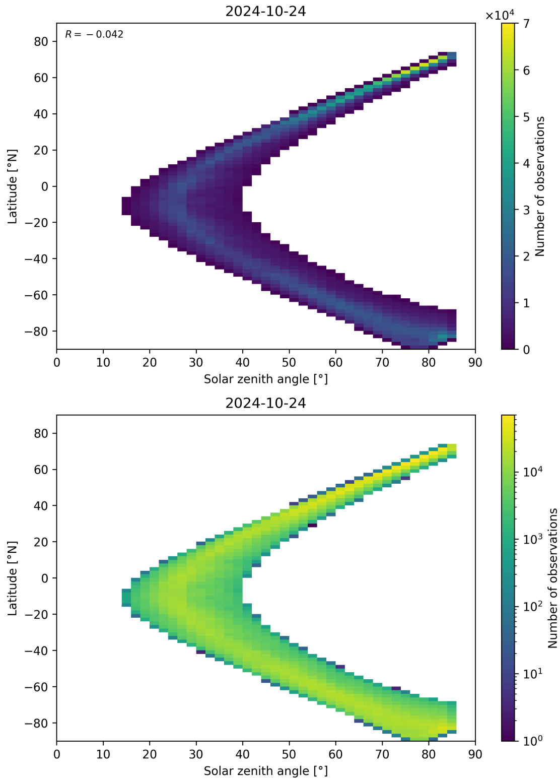
Figure 66: Scatter density plot of “Solar zenith angle” against “Latitude” for 2024-10-24 to 2024-10-25.
