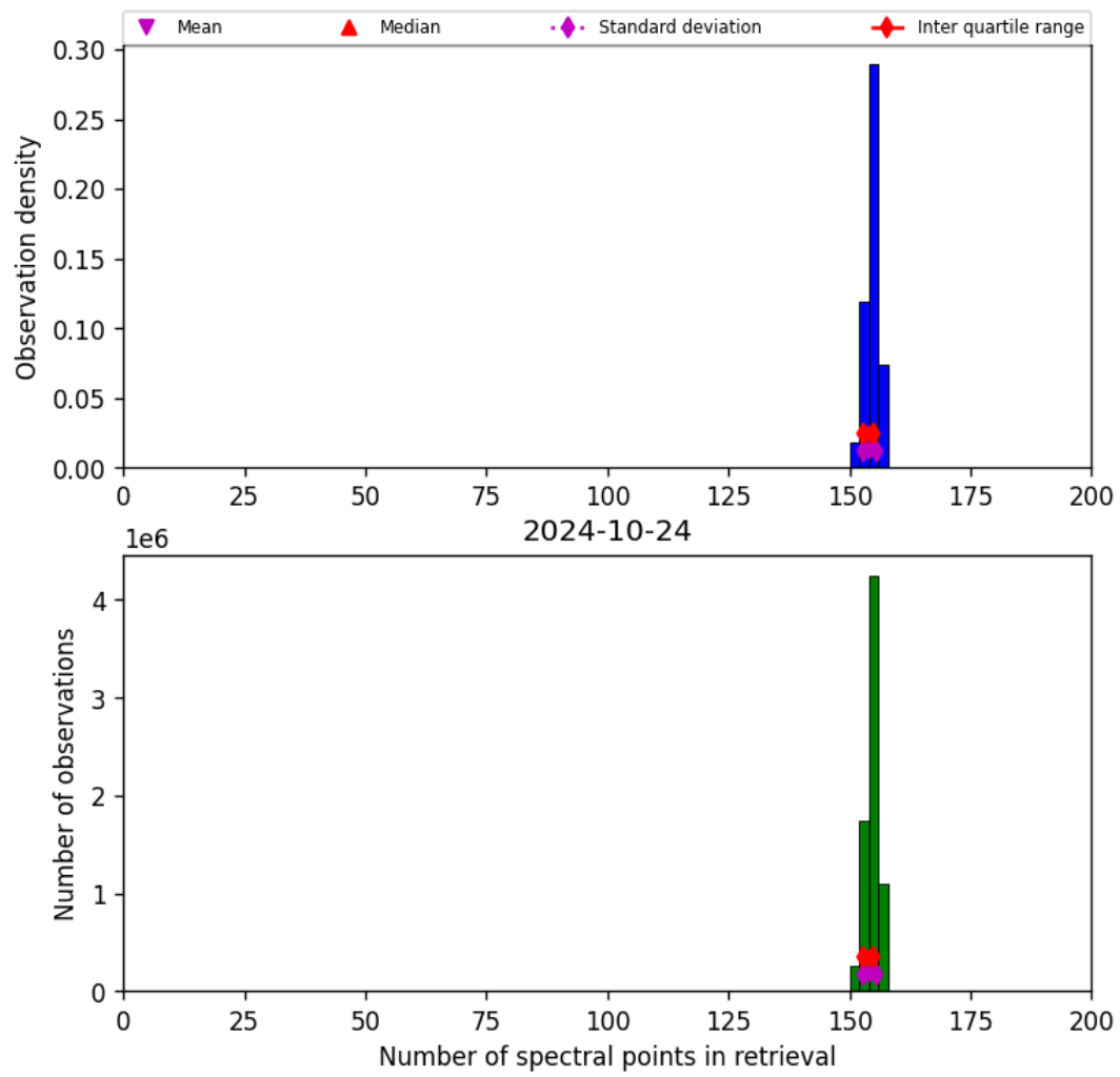
Figure 21: Histogram of “Number of spectral points in retrieval” for 2024-10-24 to 2024-10-25
