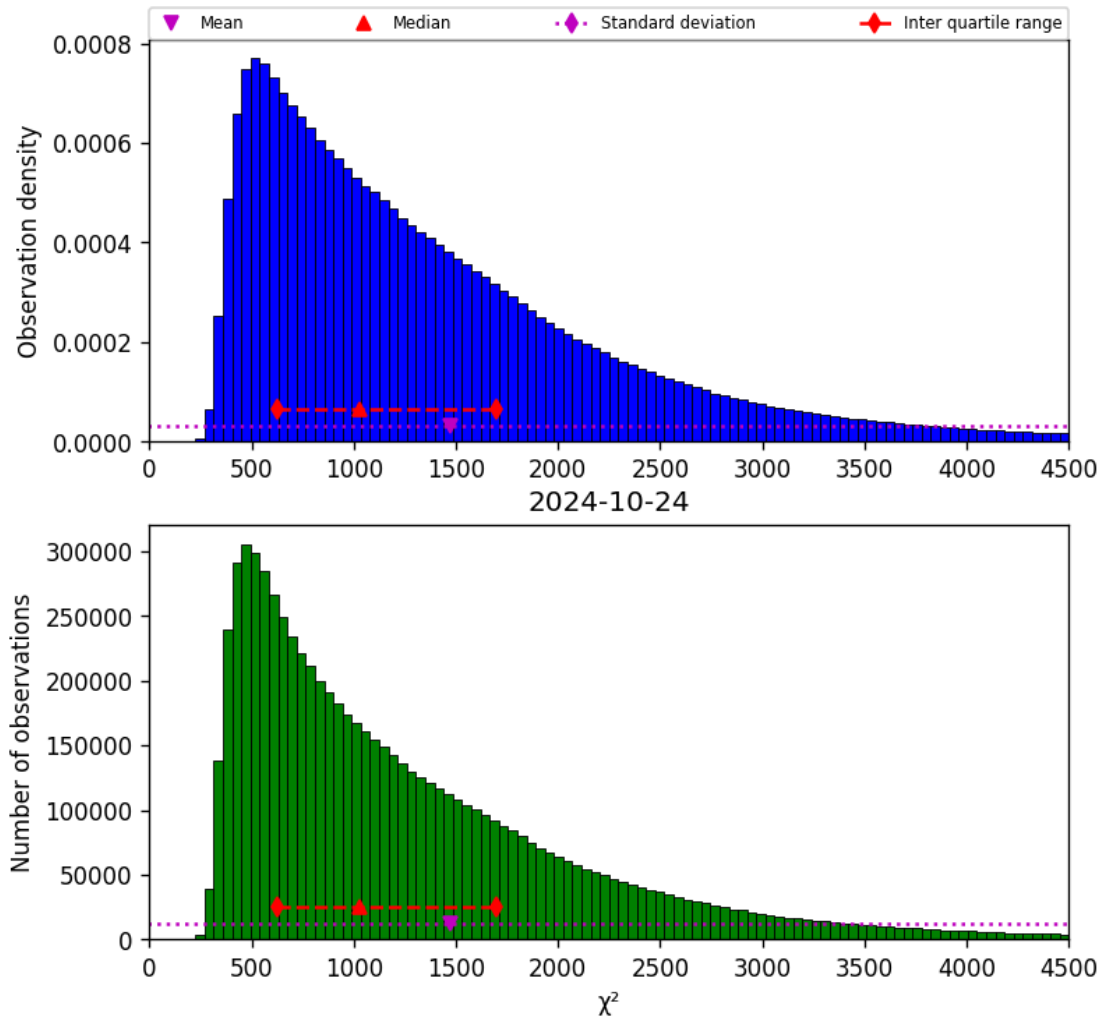
Figure 22: Histogram of “ \chi^2 ” for 2024-10-24 to 2024-10-25
