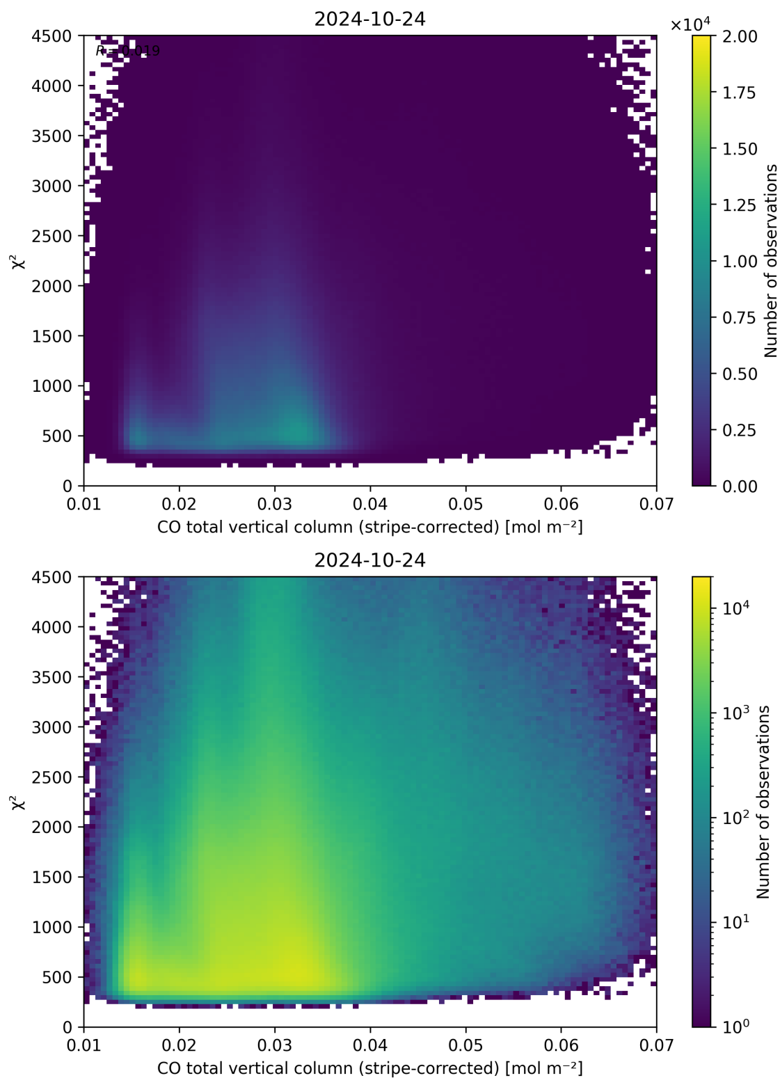
Figure 37: Scatter density plot of “CO total vertical column (stripe-corrected)” against “ \chi^2 ” for 2024-10-24 to 2024-10-25.
