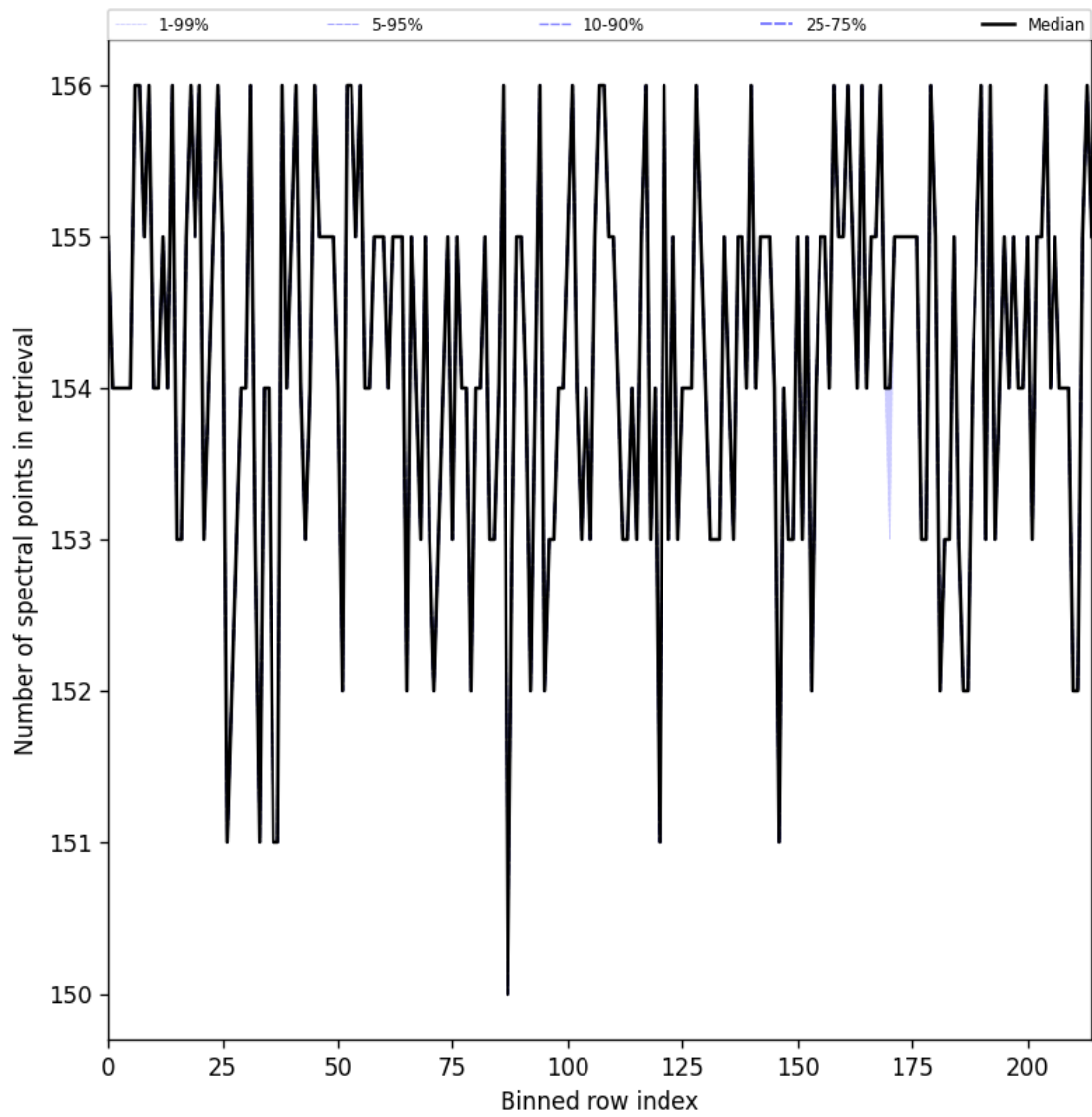
Figure 29: Along track statistics of “Number of spectral points in retrieval” for 2024-10-24 to 2024-10-25
