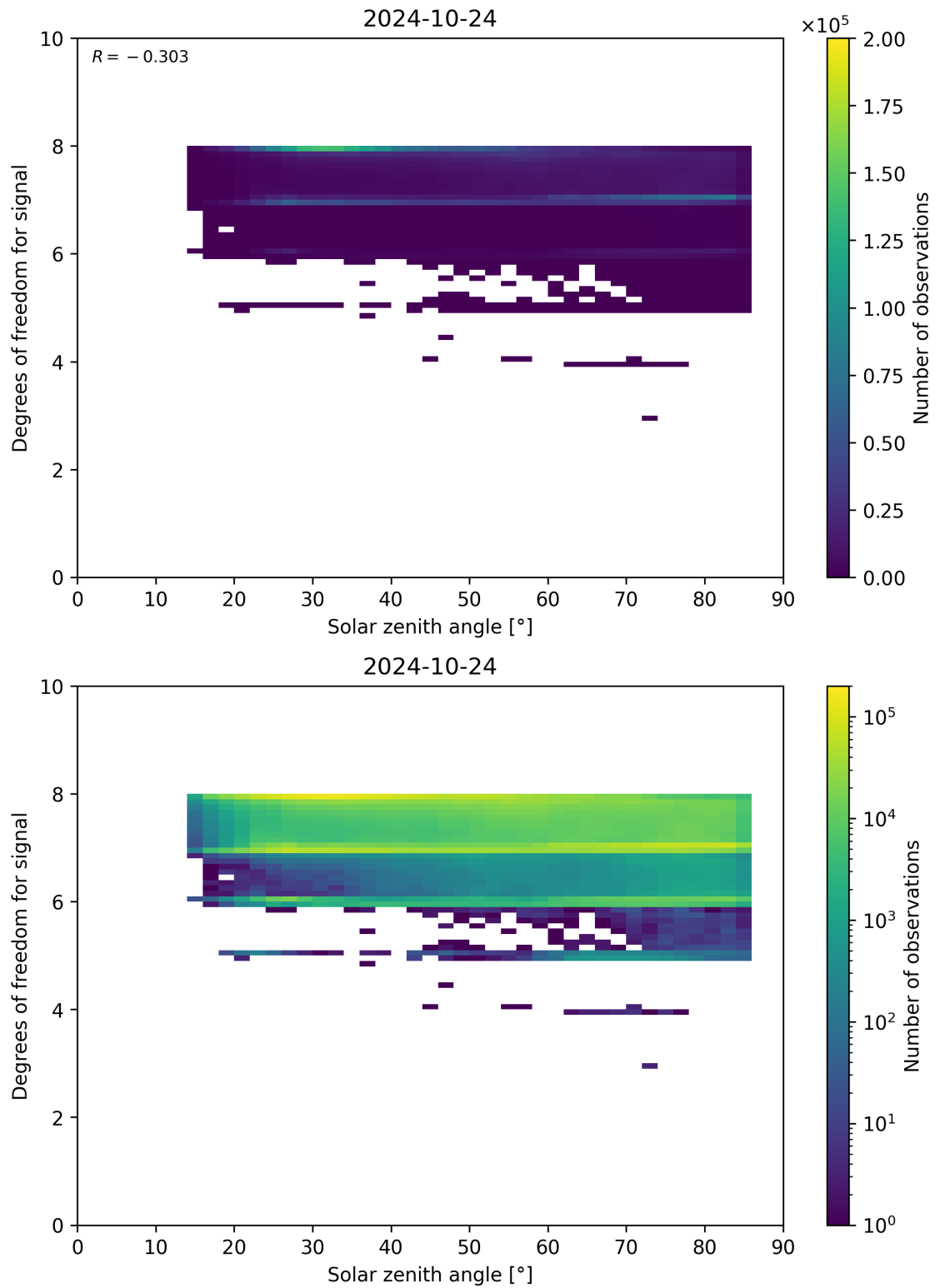
Figure 65: Scatter density plot of “Solar zenith angle” against “Degrees of freedom for signal” for 2024-10-24 to 2024-10-25.
