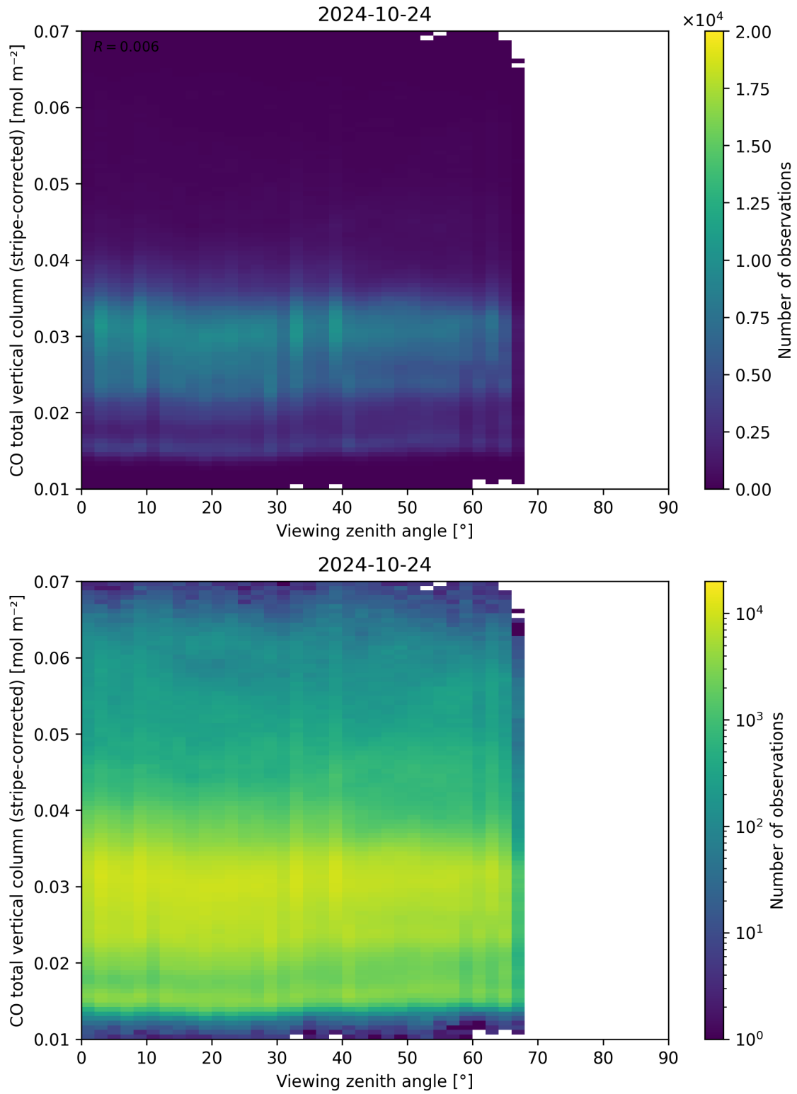
Figure 70: Scatter density plot of “Viewing zenith angle” against “CO total vertical column (stripe-corrected)” for 2024-10-24 to 2024-10-25.
