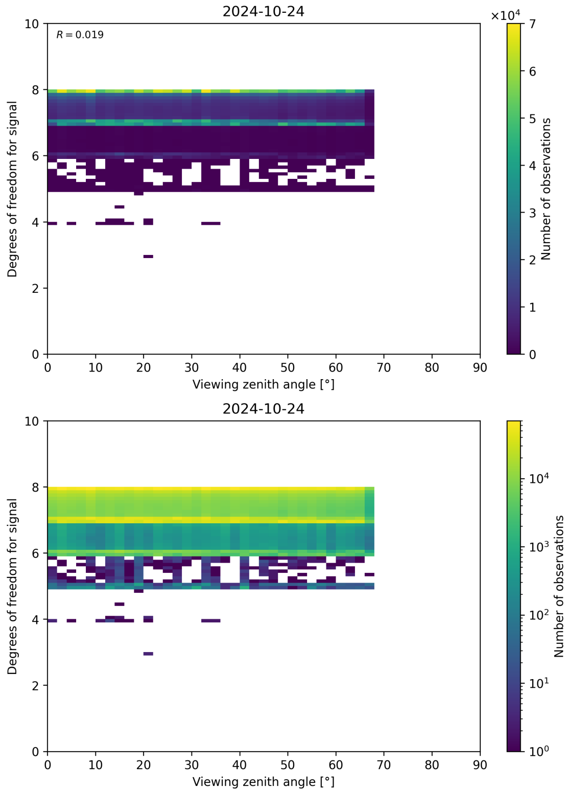
Figure 73: Scatter density plot of “Viewing zenith angle” against “Degrees of freedom for signal” for 2024-10-24 to 2024-10-25.
