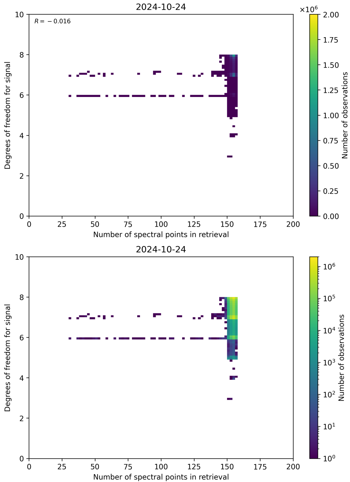
Figure 59: Scatter density plot of “Number of spectral points in retrieval” against “Degrees of freedom for signal” for 2024-10-24 to 2024-10-25.
