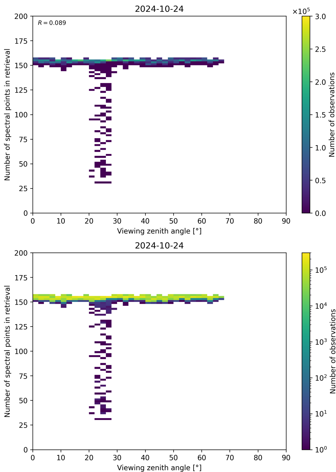
Figure 76: Scatter density plot of “Viewing zenith angle” against “Number of spectral points in retrieval” for 2024-10-24 to 2024-10-25.
