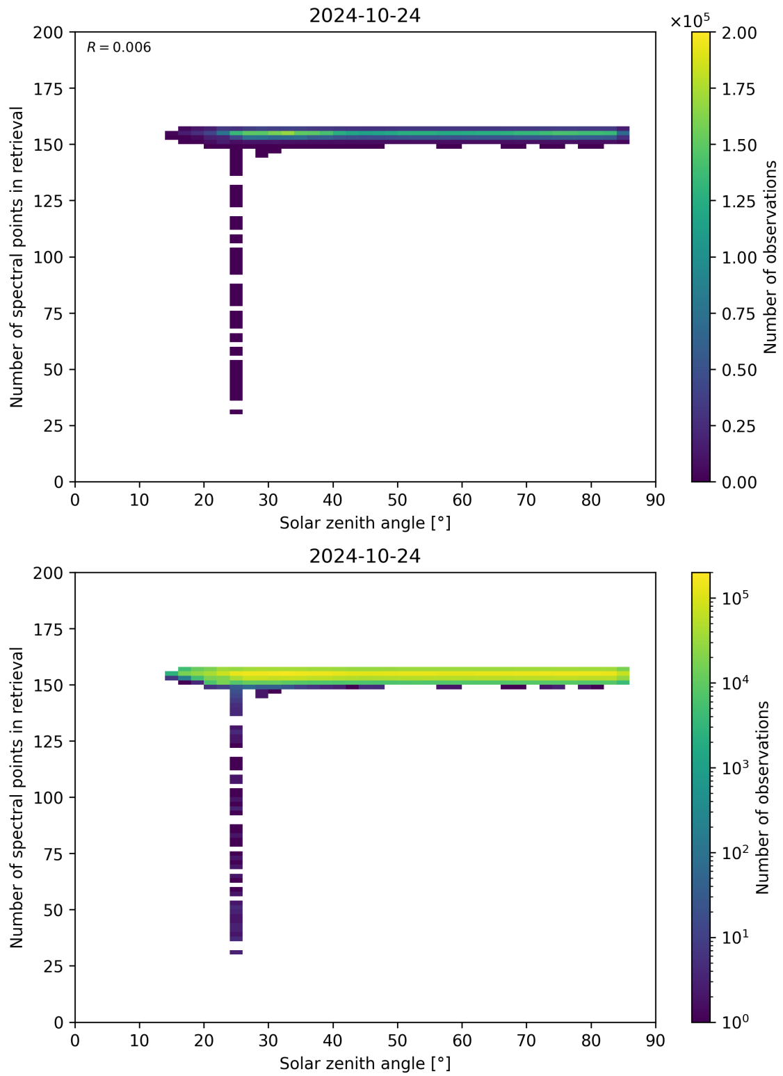
Figure 68: Scatter density plot of “Solar zenith angle” against “Number of spectral points in retrieval” for 2024-10-24 to 2024-10-25.
