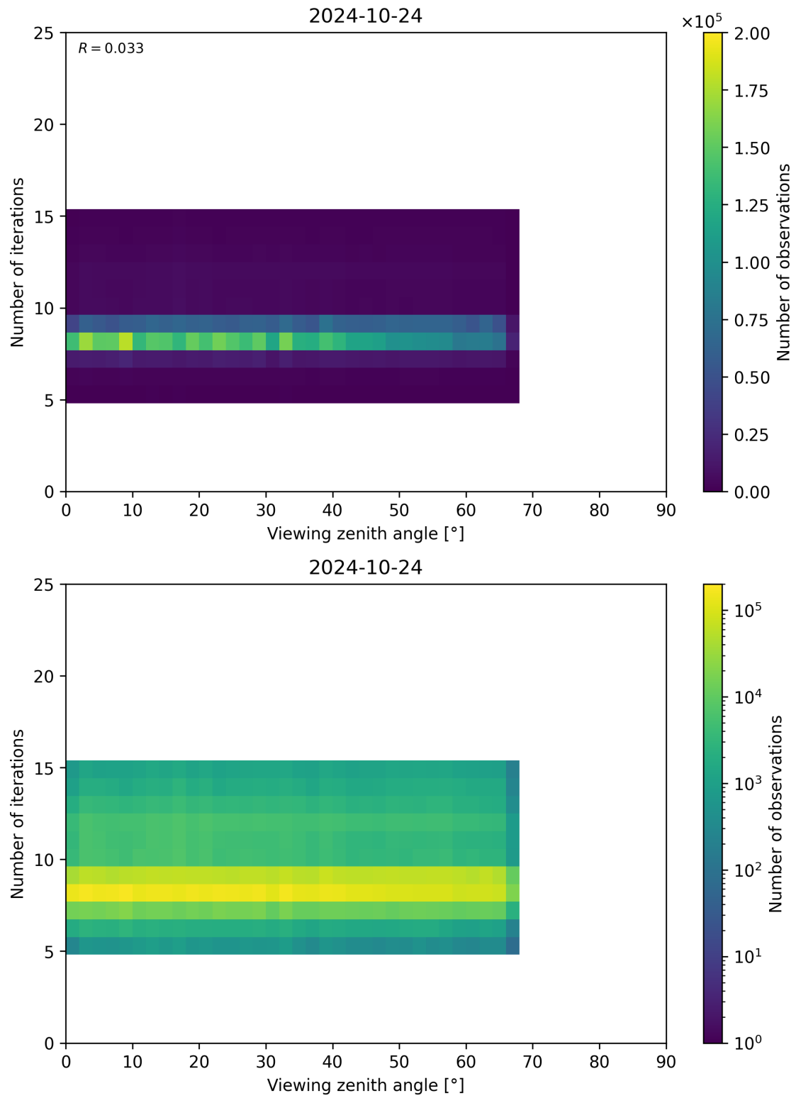
Figure 75: Scatter density plot of “Viewing zenith angle” against “Number of iterations” for 2024-10-24 to 2024-10-25.
