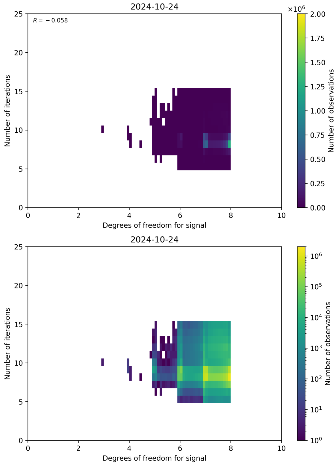
Figure 50: Scatter density plot of “Degrees of freedom for signal” against “Number of iterations” for 2024-10-24 to 2024-10-25.
