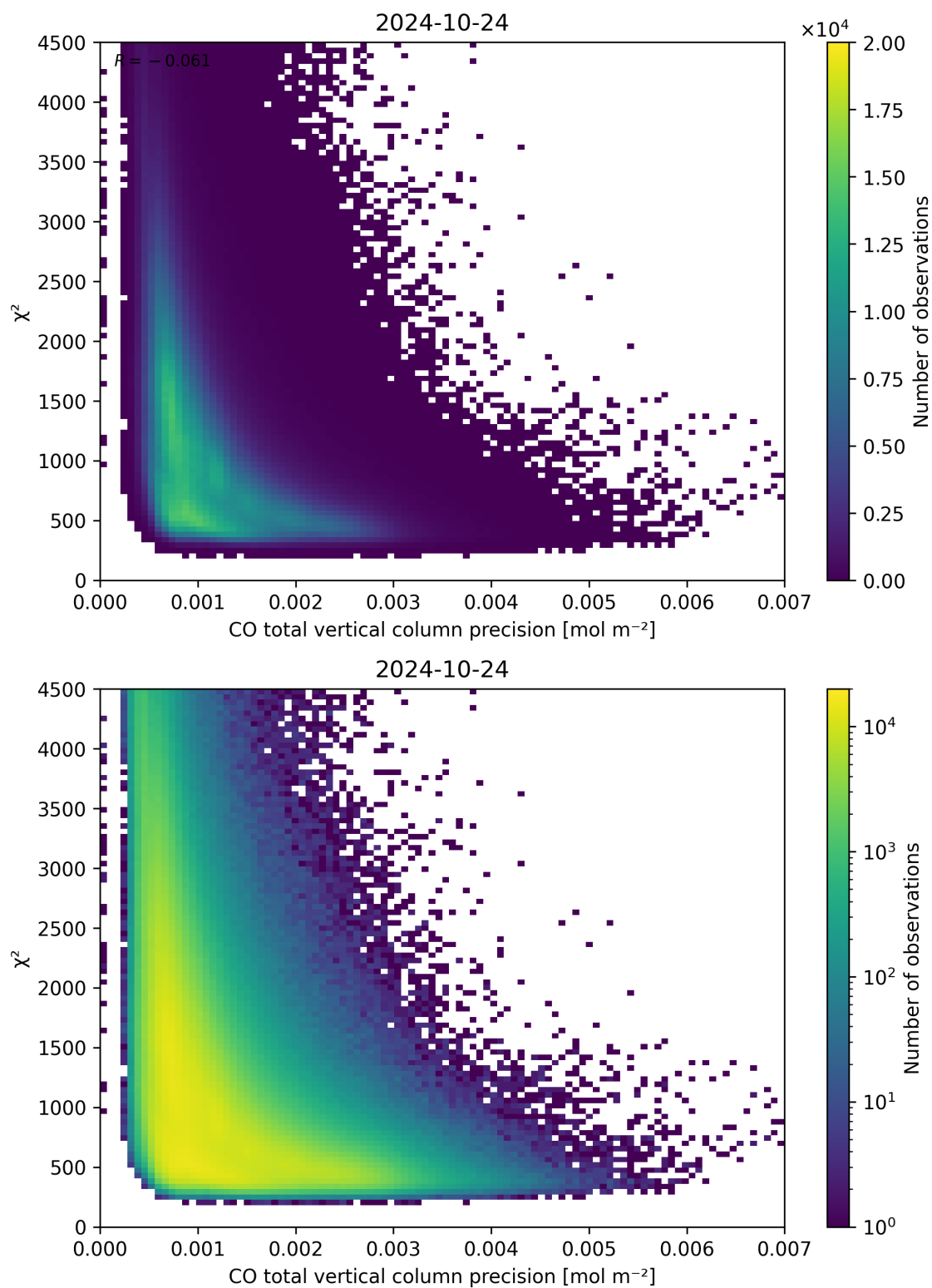
Figure 44: Scatter density plot of “CO total vertical column precision” against “ \chi^2 ” for 2024-10-24 to 2024-10-25.
