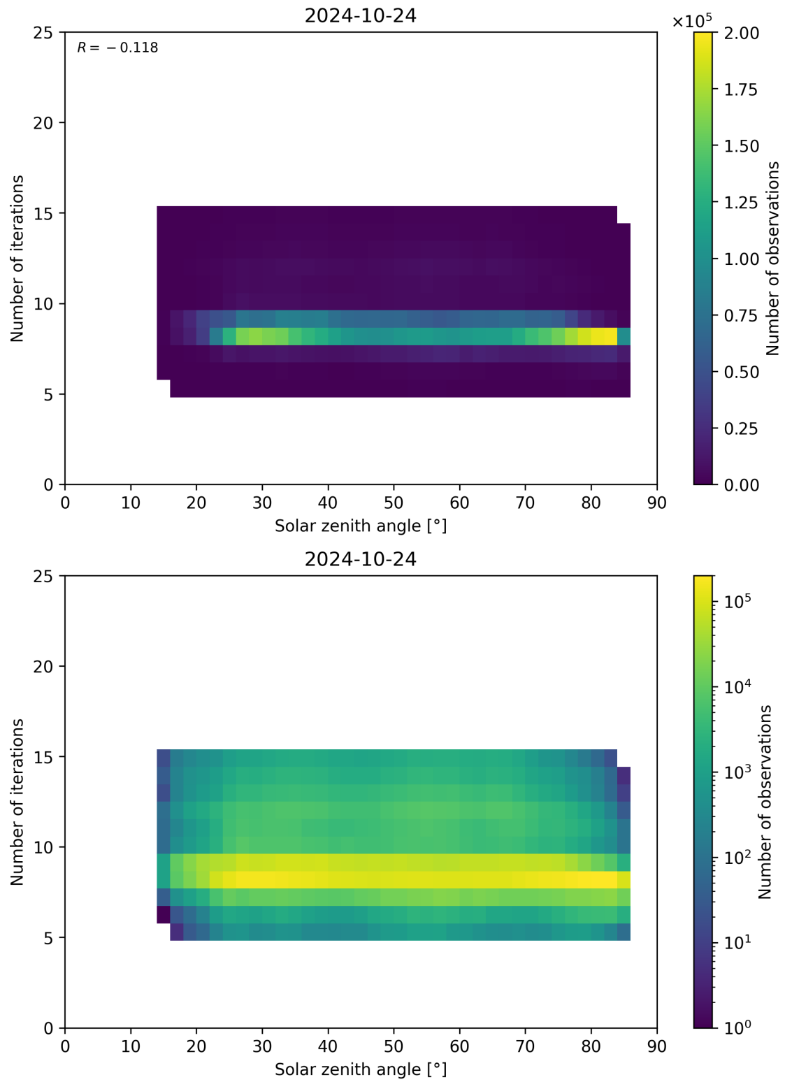
Figure 67: Scatter density plot of “Solar zenith angle” against “Number of iterations” for 2024-10-24 to 2024-10-25.
