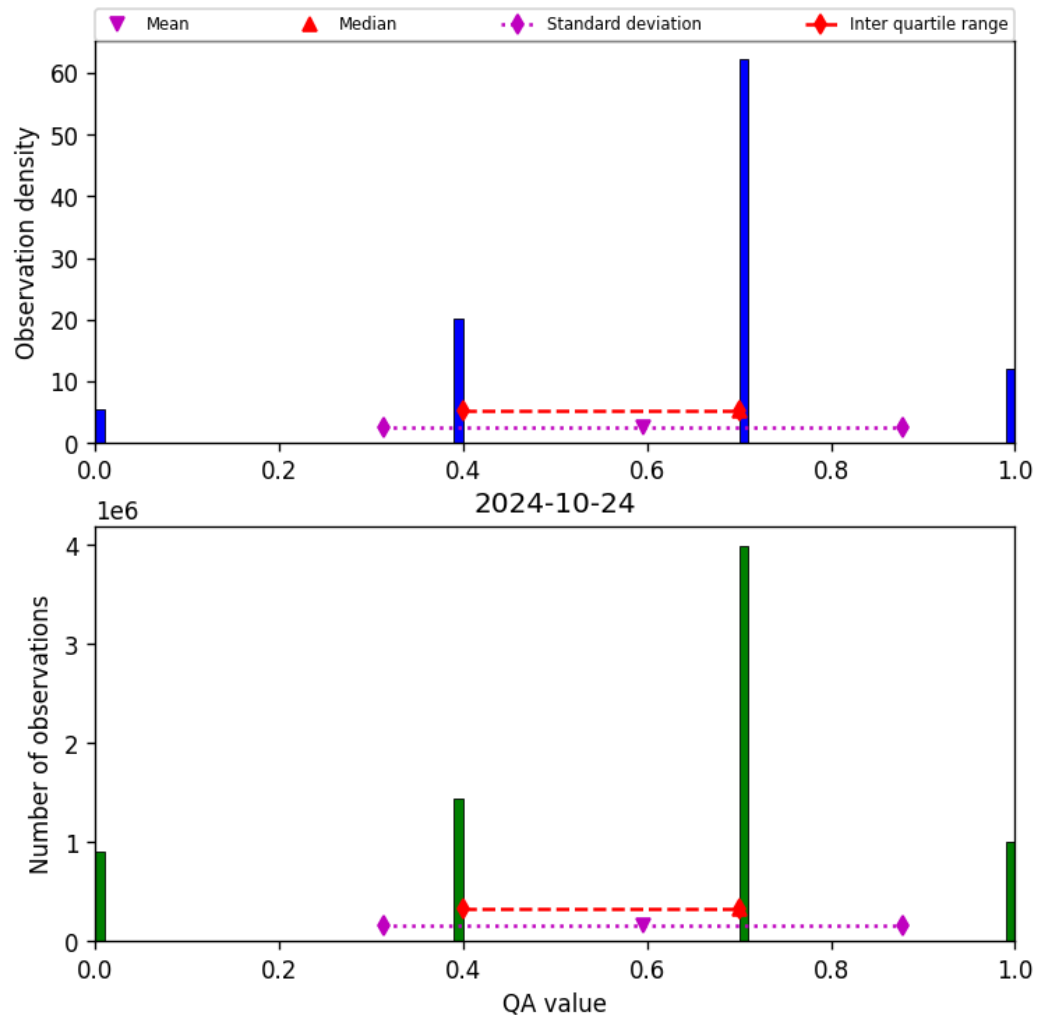
Figure 17: Histogram of “QA value” for 2024-10-24 to 2024-10-25
