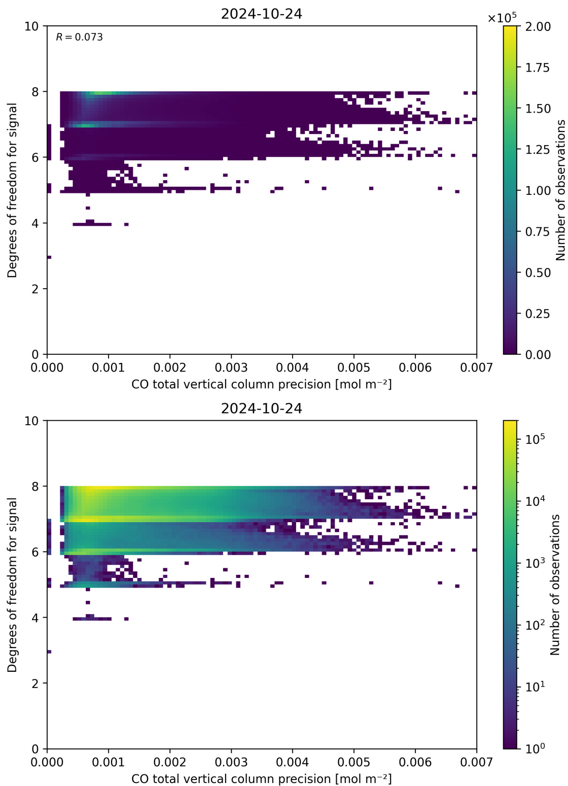
Figure 45: Scatter density plot of “CO total vertical column precision” against “Degrees of freedom for signal” for 2024-10-24 to 2024-10-25.
