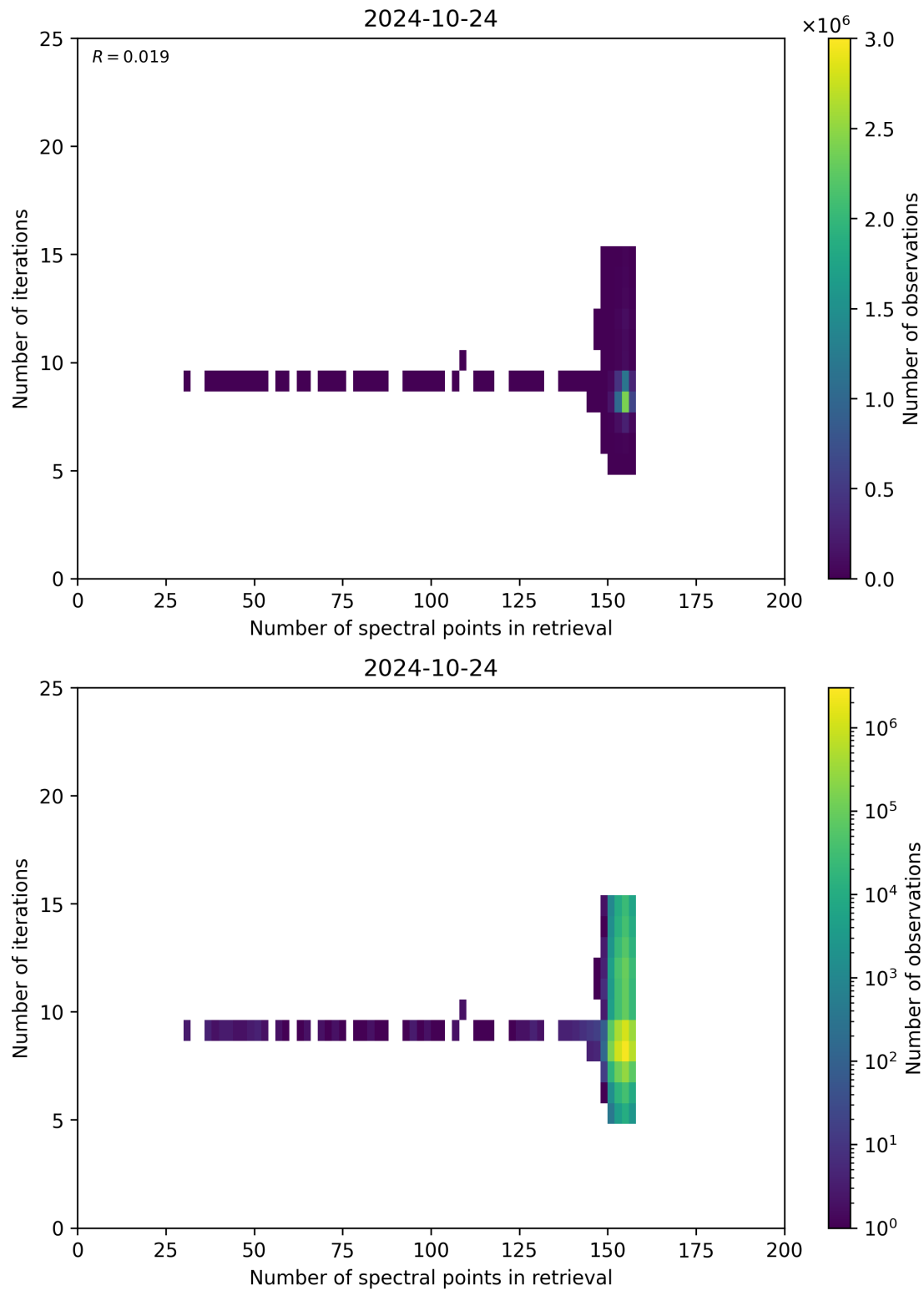
Figure 60: Scatter density plot of “Number of spectral points in retrieval” against “Number of iterations” for 2024-10-24 to 2024-10-25.
