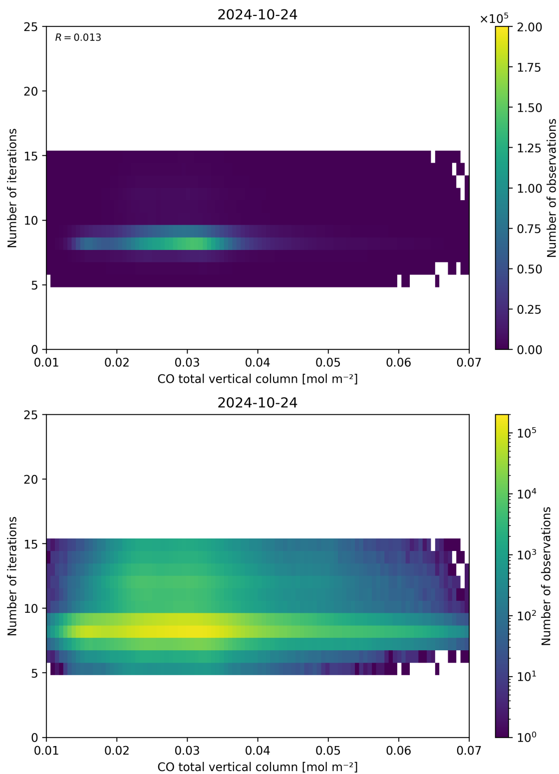
Figure 42: Scatter density plot of “CO total vertical column” against “Number of iterations” for 2024-10-24 to 2024-10-25.
