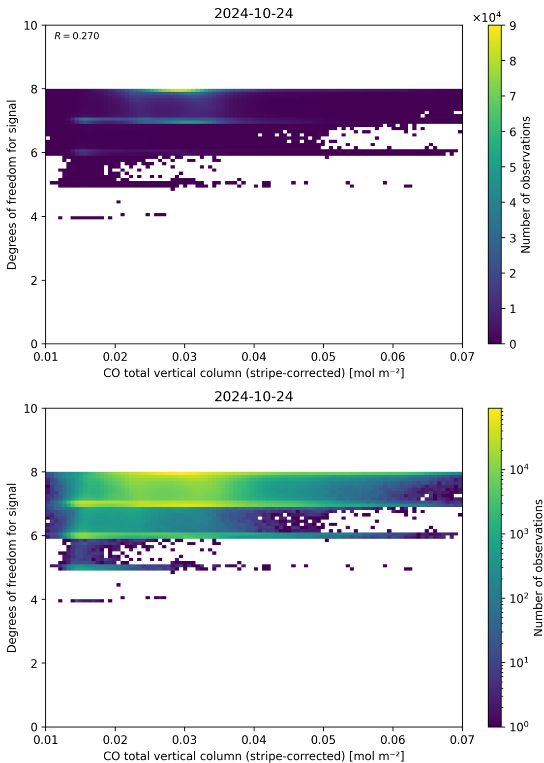
Figure 38: Scatter density plot of “CO total vertical column (stripe-corrected)” against “Degrees of freedom for signal” for 2024-10-24 to 2024-10-25.
