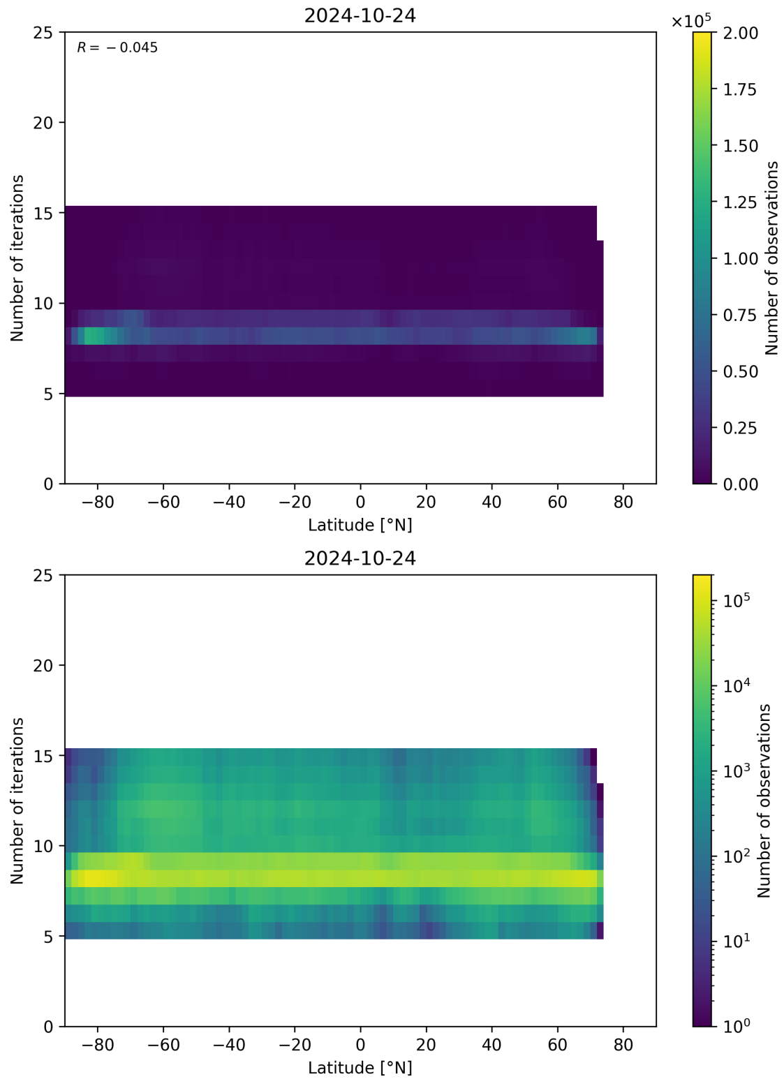
Figure 56: Scatter density plot of “Latitude” against “Number of iterations” for 2024-10-24 to 2024-10-25.
