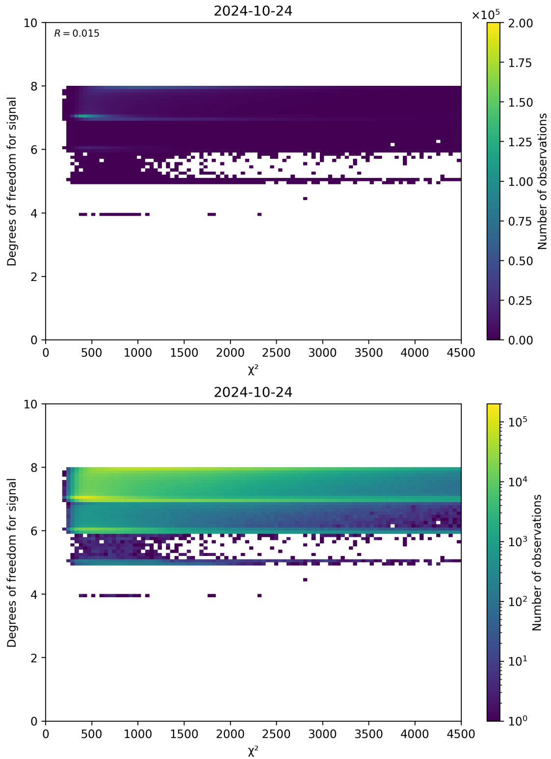
Figure 48: Scatter density plot of “ \chi^2 ” against “Degrees of freedom for signal” for 2024-10-24 to 2024-10-25.
