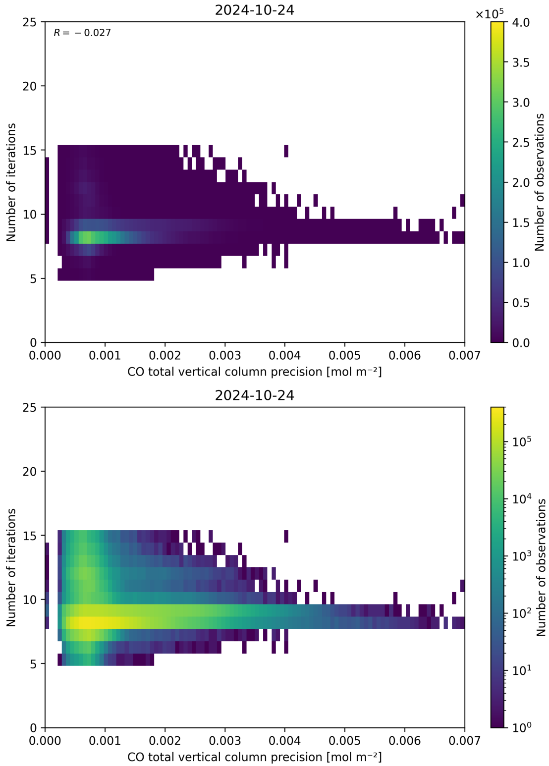
Figure 46: Scatter density plot of “CO total vertical column precision” against “Number of iterations” for 2024-10-24 to 2024-10-25.
