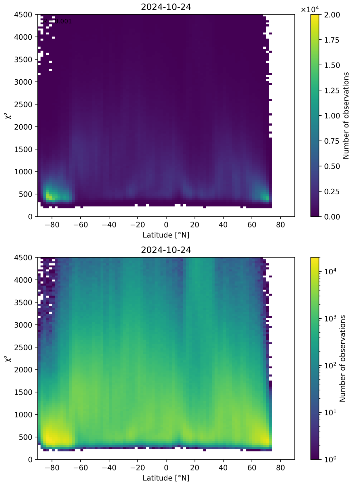
Figure 54: Scatter density plot of “Latitude” against “ \chi^2 ” for 2024-10-24 to 2024-10-25.
