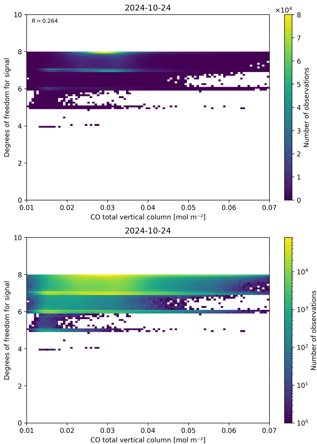
Figure 41: Scatter density plot of “CO total vertical column” against “Degrees of freedom for signal” for 2024-10-24 to 2024-10-25.
