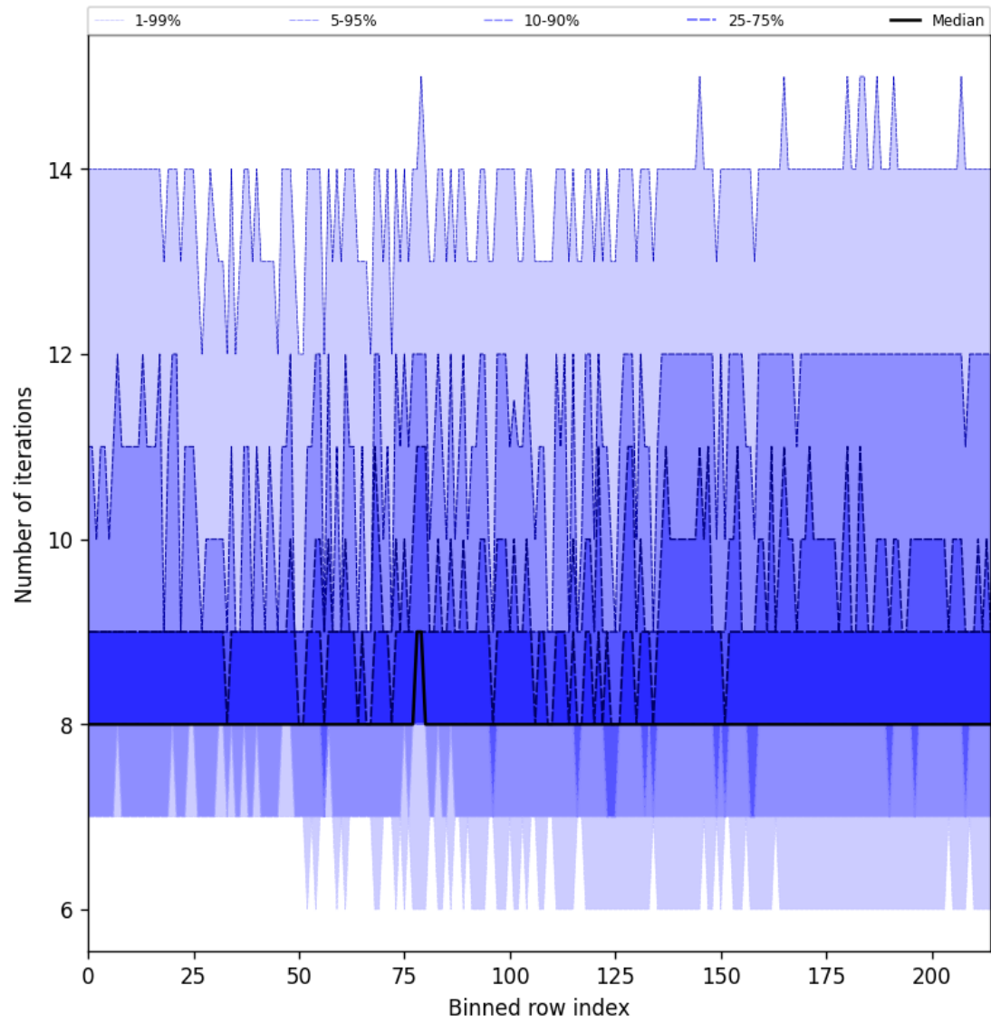
Figure 32: Along track statistics of “Number of iterations” for 2024-10-24 to 2024-10-25
