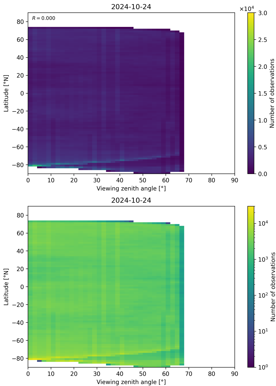
Figure 74: Scatter density plot of “Viewing zenith angle” against “Latitude” for 2024-10-24 to 2024-10-25.
