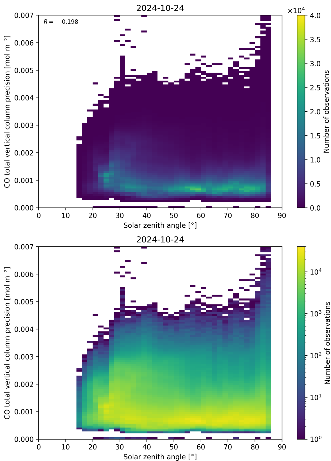
Figure 63: Scatter density plot of “Solar zenith angle” against “CO total vertical column precision” for 2024-10-24 to 2024-10-25.
