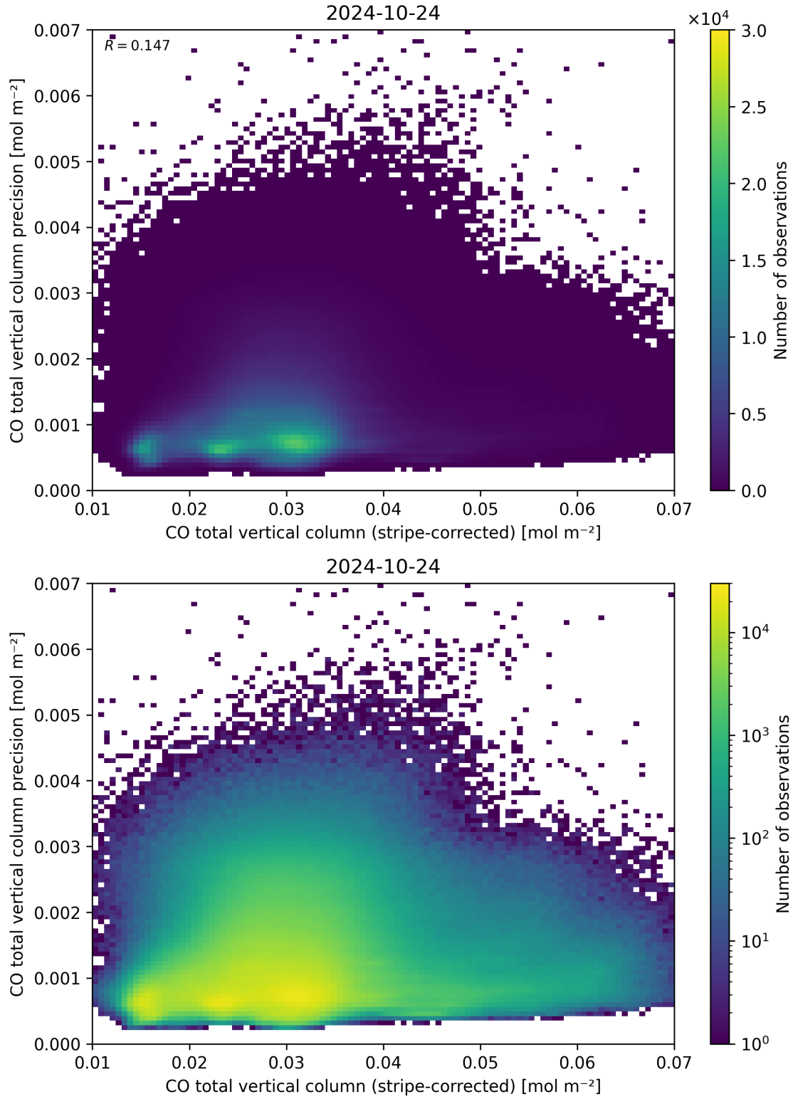
Figure 36: Scatter density plot of “CO total vertical column (stripe-corrected)” against “CO total vertical column precision” for 2024-10-24 to 2024-10-25.
