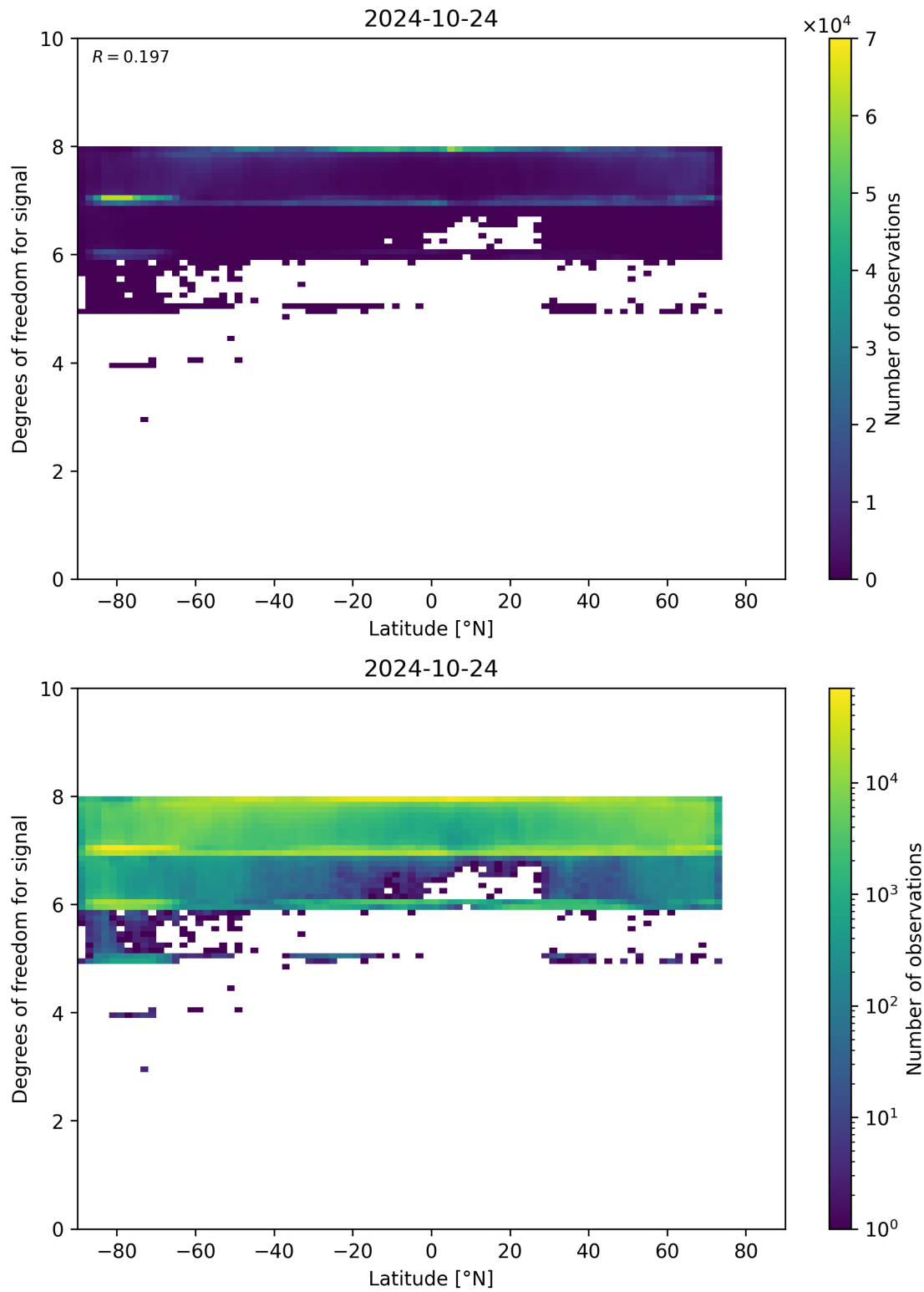
Figure 55: Scatter density plot of “Latitude” against “Degrees of freedom for signal” for 2024-10-24 to 2024-10-25.
