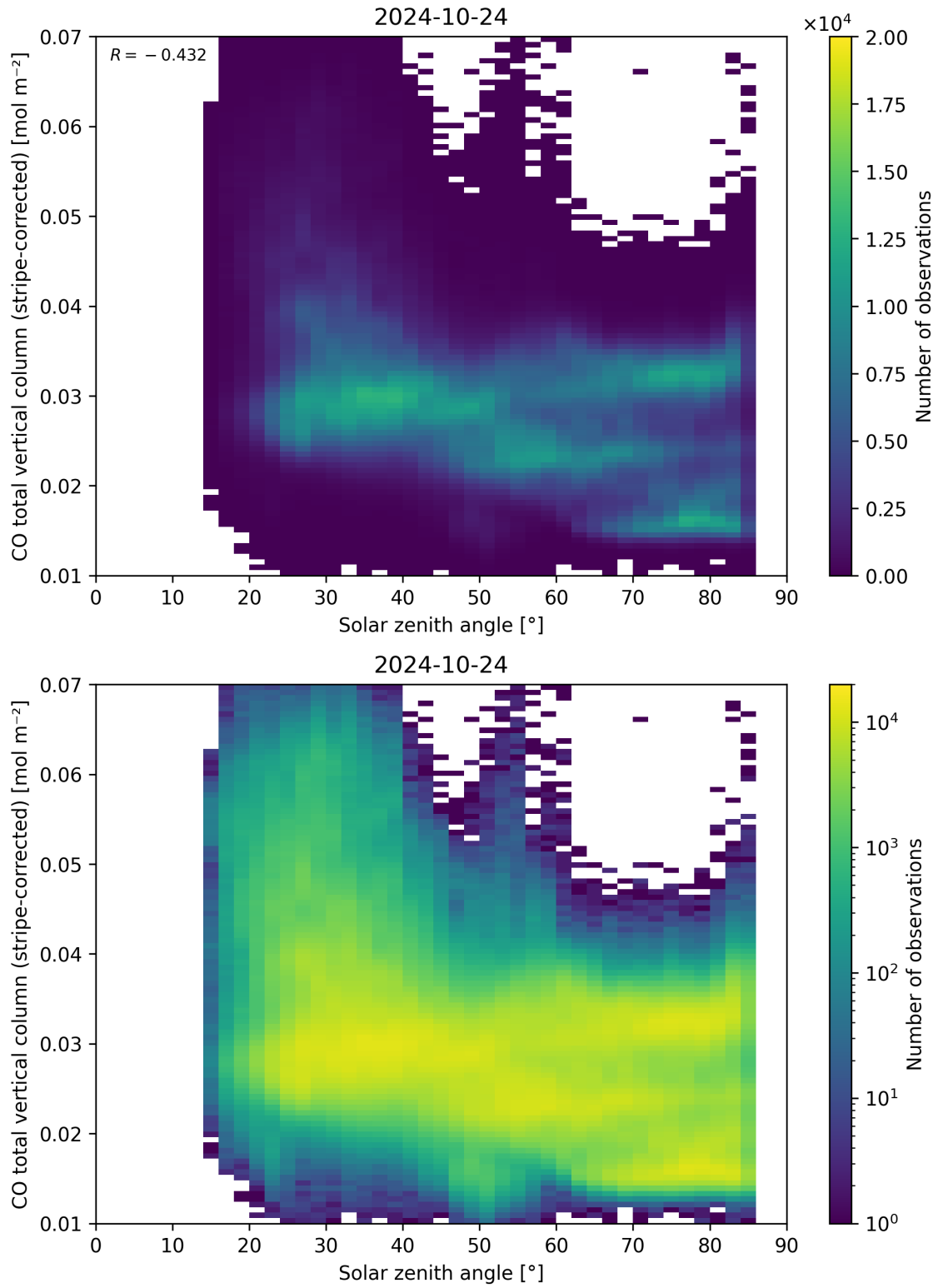
Figure 62: Scatter density plot of “Solar zenith angle” against “CO total vertical column (stripe-corrected)” for 2024-10-24 to 2024-10-25.
