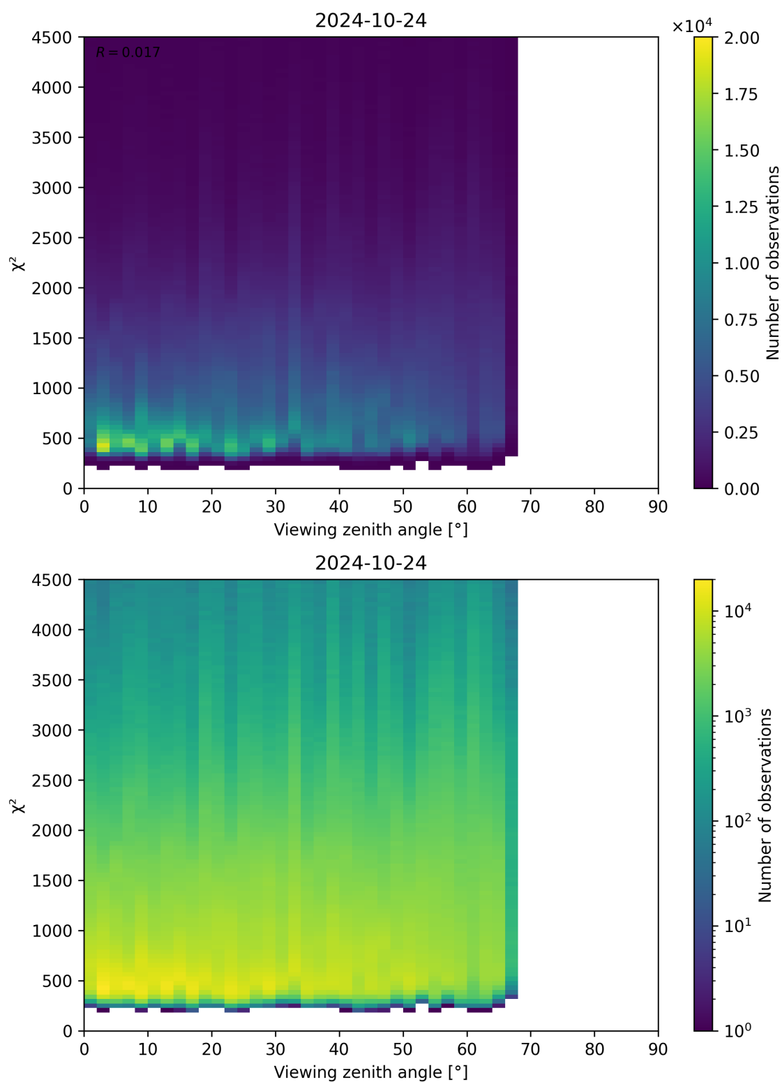
Figure 72: Scatter density plot of “Viewing zenith angle” against “ \chi^2 ” for 2024-10-24 to 2024-10-25.
