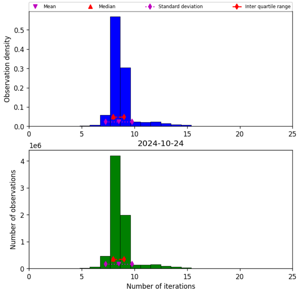
Figure 24: Histogram of “Number of iterations” for 2024-10-24 to 2024-10-25
