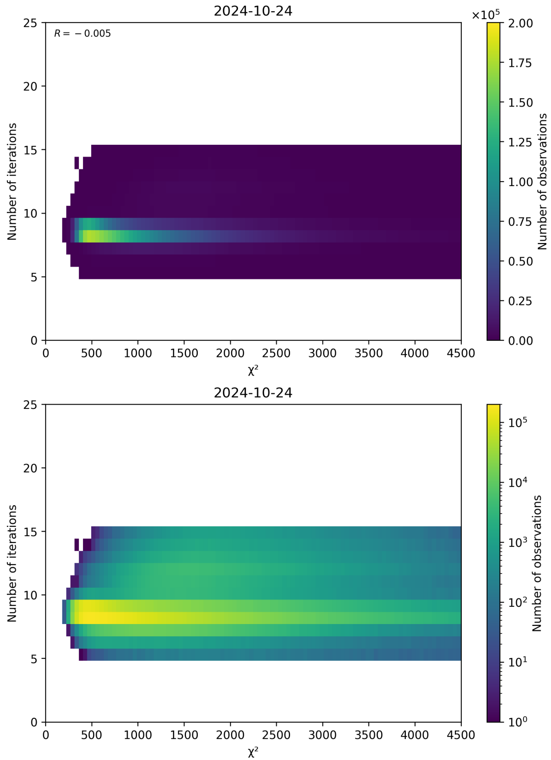
Figure 49: Scatter density plot of “ \chi^2 ” against “Number of iterations” for 2024-10-24 to 2024-10-25.
