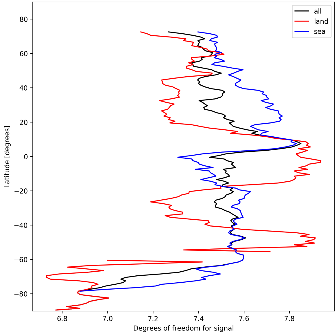
Figure 15: Zonal average of “Degrees of freedom for signal” for 2024-10-24 to 2024-10-26.
