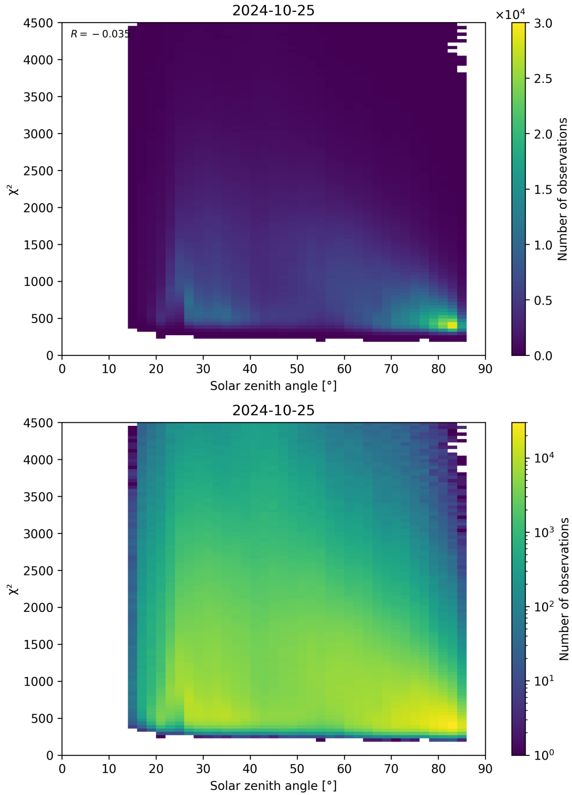
Figure 64: Scatter density plot of “Solar zenith angle” against “ \chi^2 ” for 2024-10-24 to 2024-10-26.
