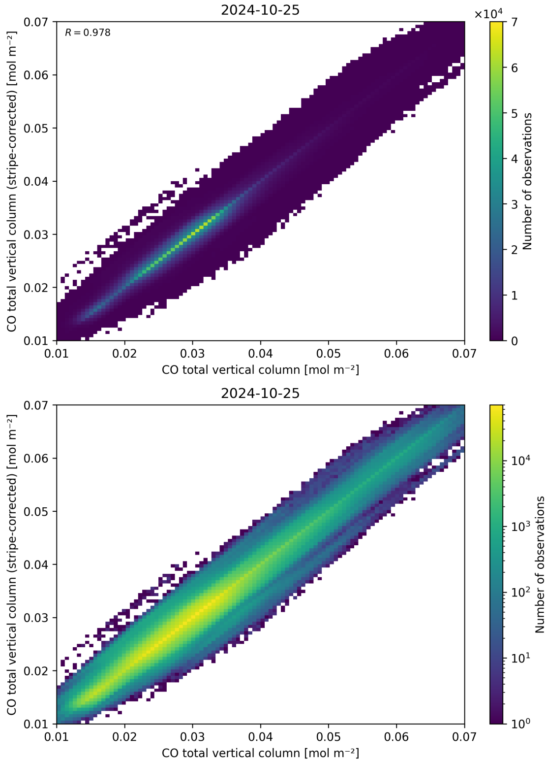
Figure 33: Scatter density plot of “CO total vertical column” against “CO total vertical column (stripe-corrected)” for 2024-10-24 to 2024-10-26.
