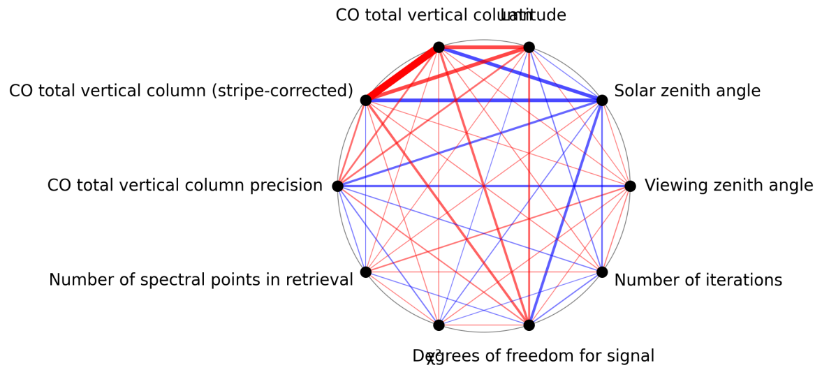
Figure 1: Map of correlation graph for 2024-10-24 to 2024-10-26.
