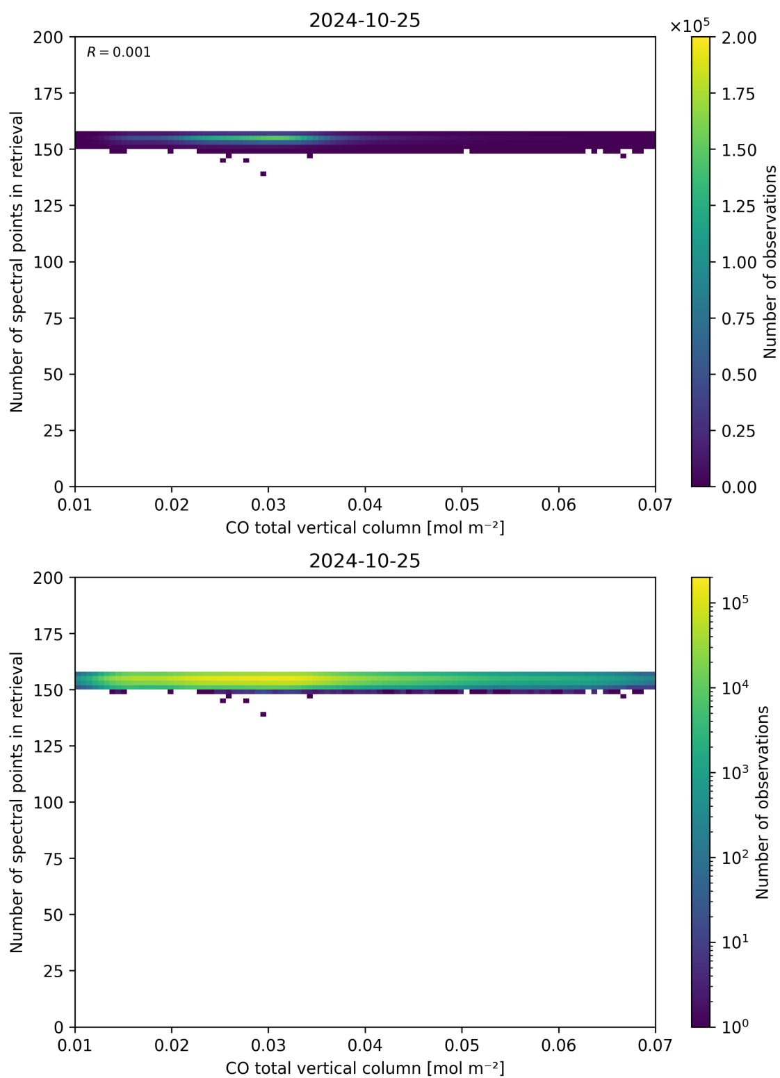
Figure 43: Scatter density plot of “CO total vertical column” against “Number of spectral points in retrieval” for 2024-10-24 to 2024-10-26.
