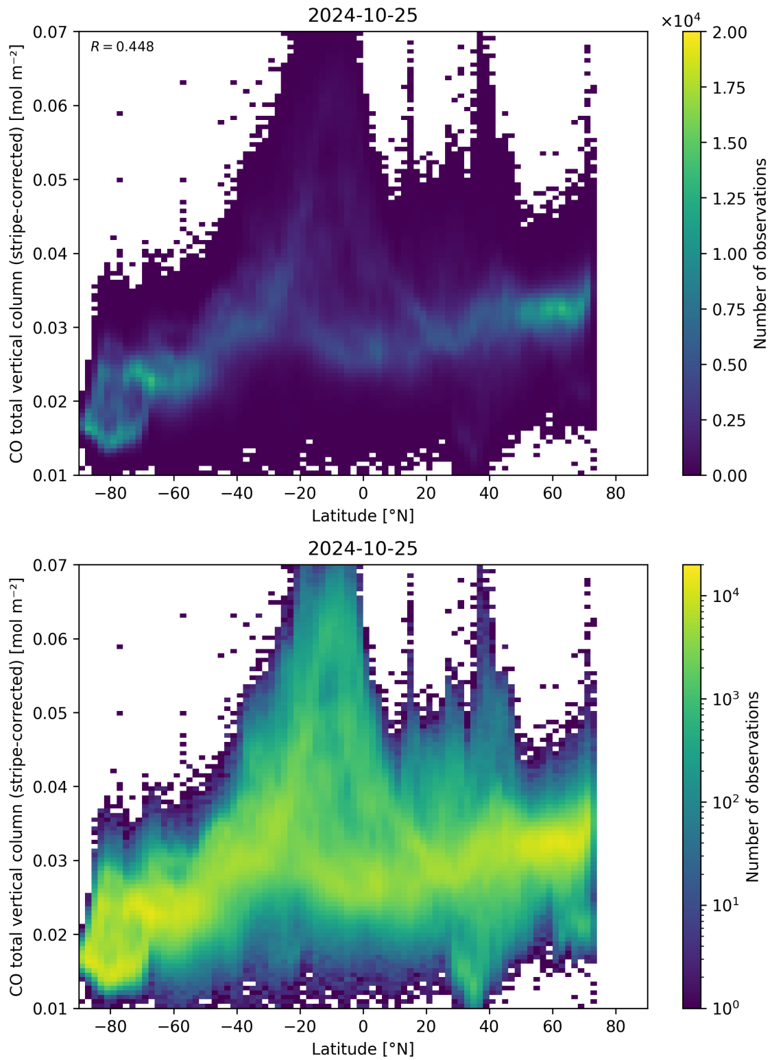
Figure 52: Scatter density plot of “Latitude” against “CO total vertical column (stripe-corrected)” for 2024-10-24 to 2024-10-26.
