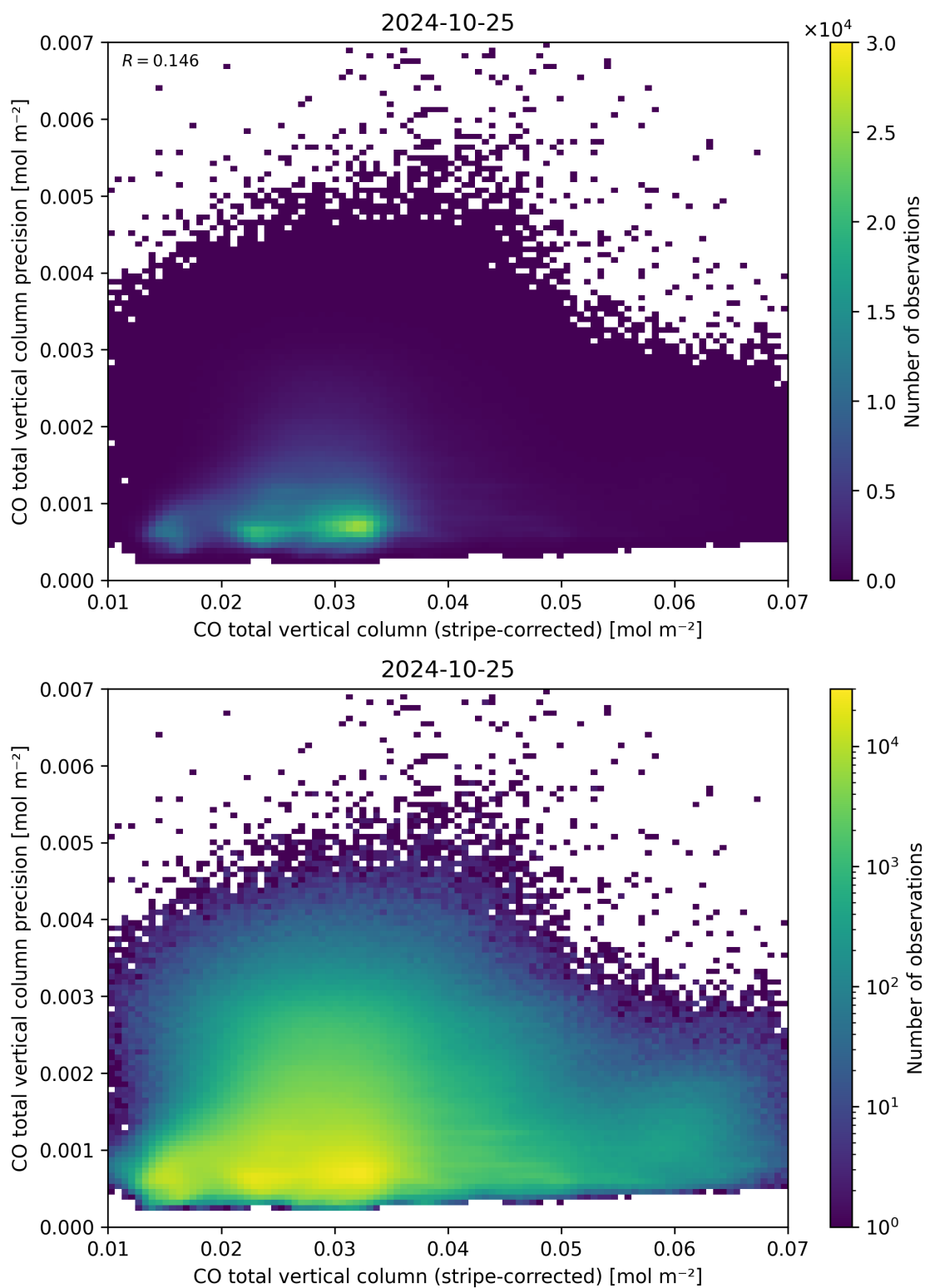
Figure 36: Scatter density plot of “CO total vertical column (stripe-corrected)” against “CO total vertical column precision” for 2024-10-24 to 2024-10-26.
