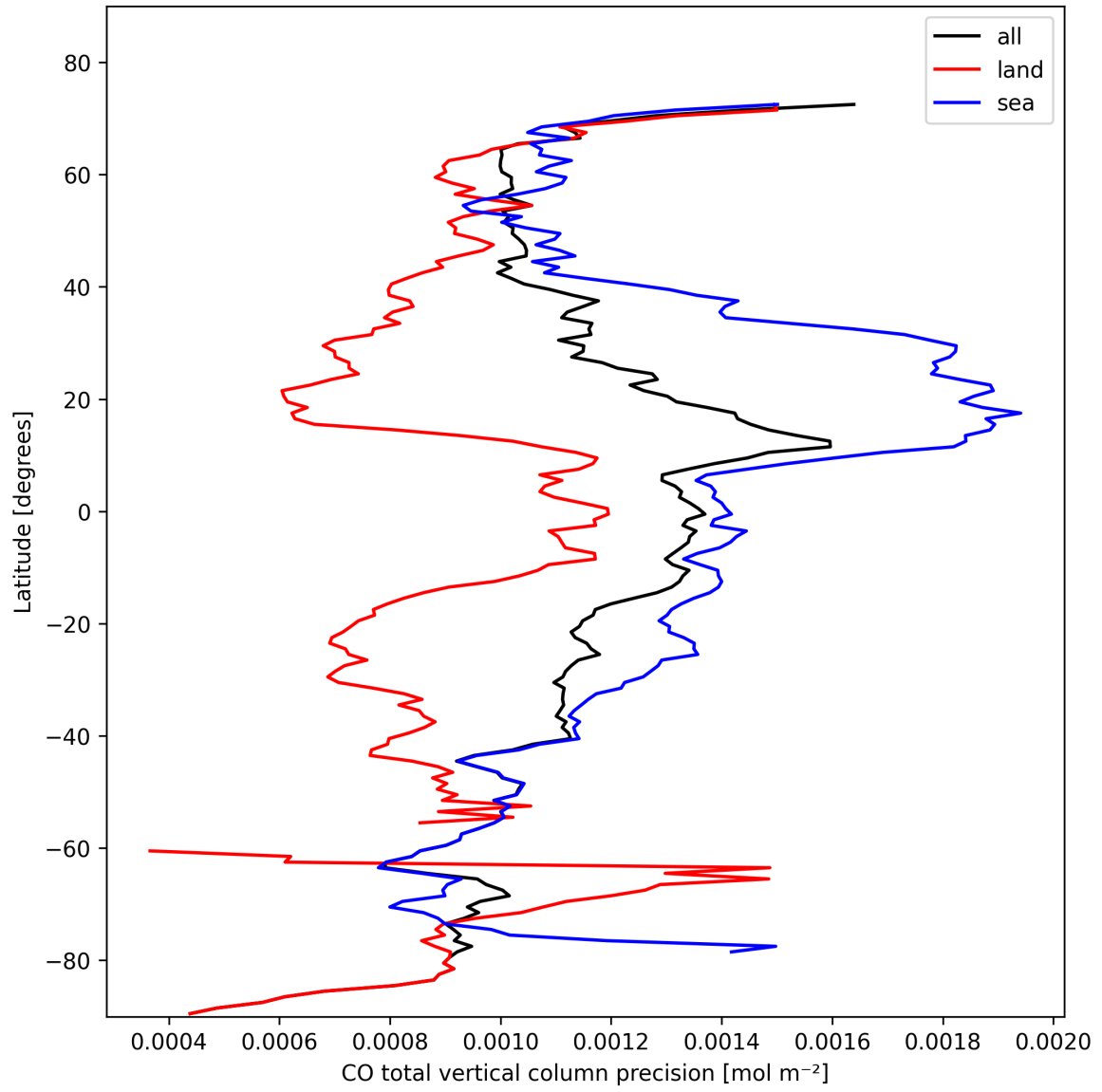
Figure 12: Zonal average of “CO total vertical column precision” for 2024-10-24 to 2024-10-26.
