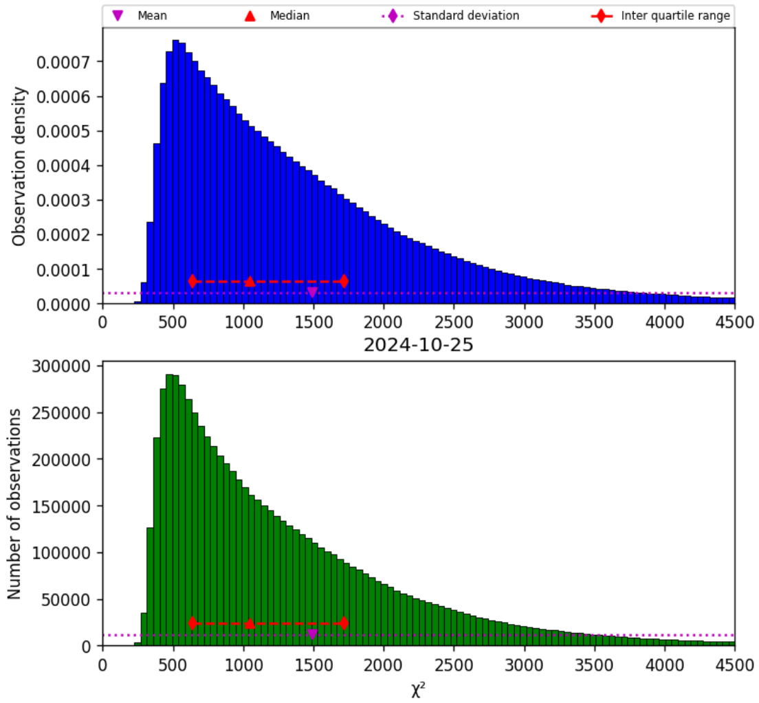
Figure 22: Histogram of “ \chi^2 ” for 2024-10-24 to 2024-10-26
