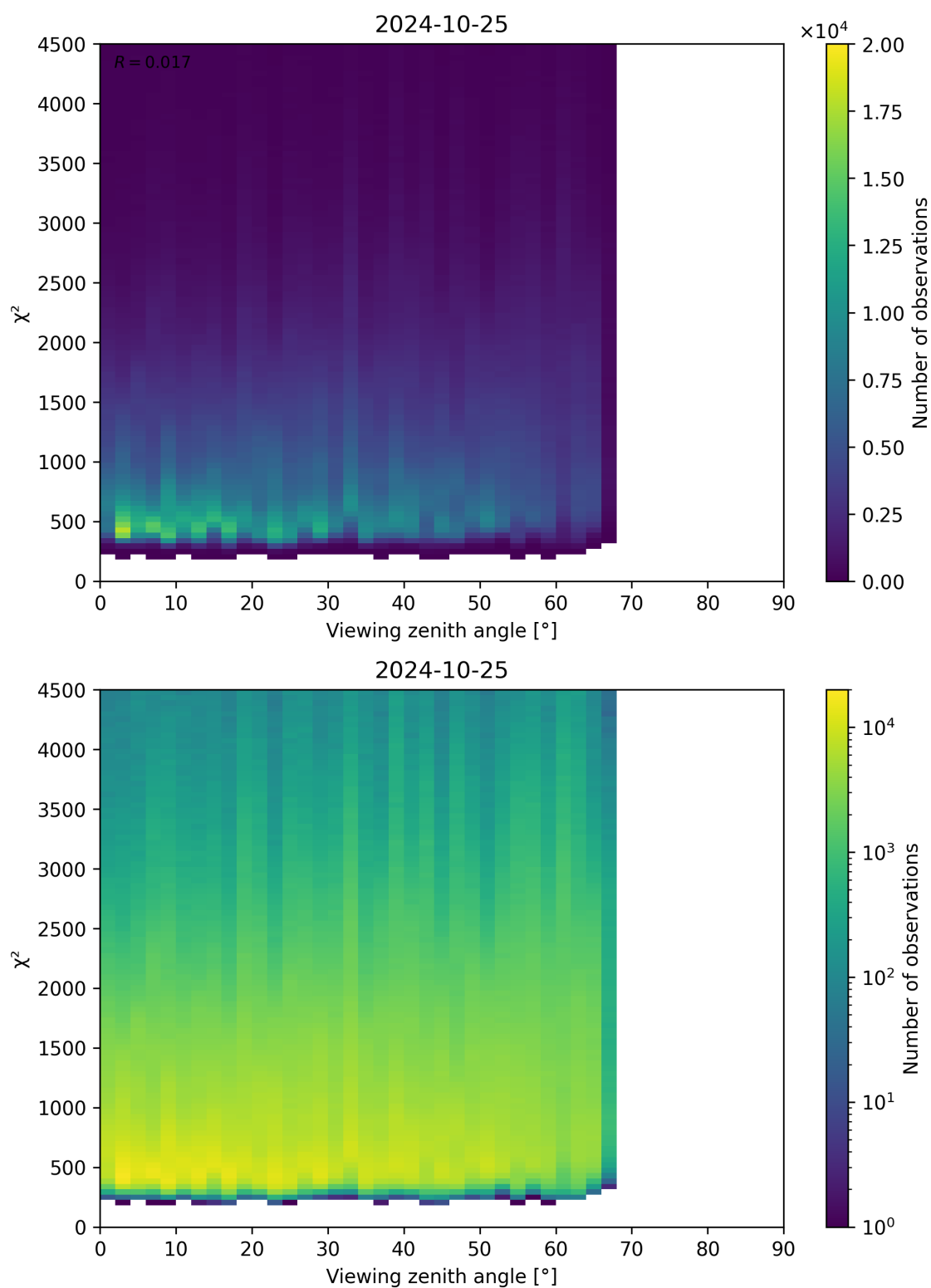
Figure 72: Scatter density plot of “Viewing zenith angle” against “ \chi^2 ” for 2024-10-24 to 2024-10-26.
