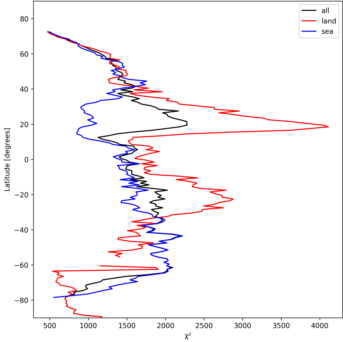
Figure 14: Zonal average of “ \chi^2 ” for 2024-10-24 to 2024-10-26.
