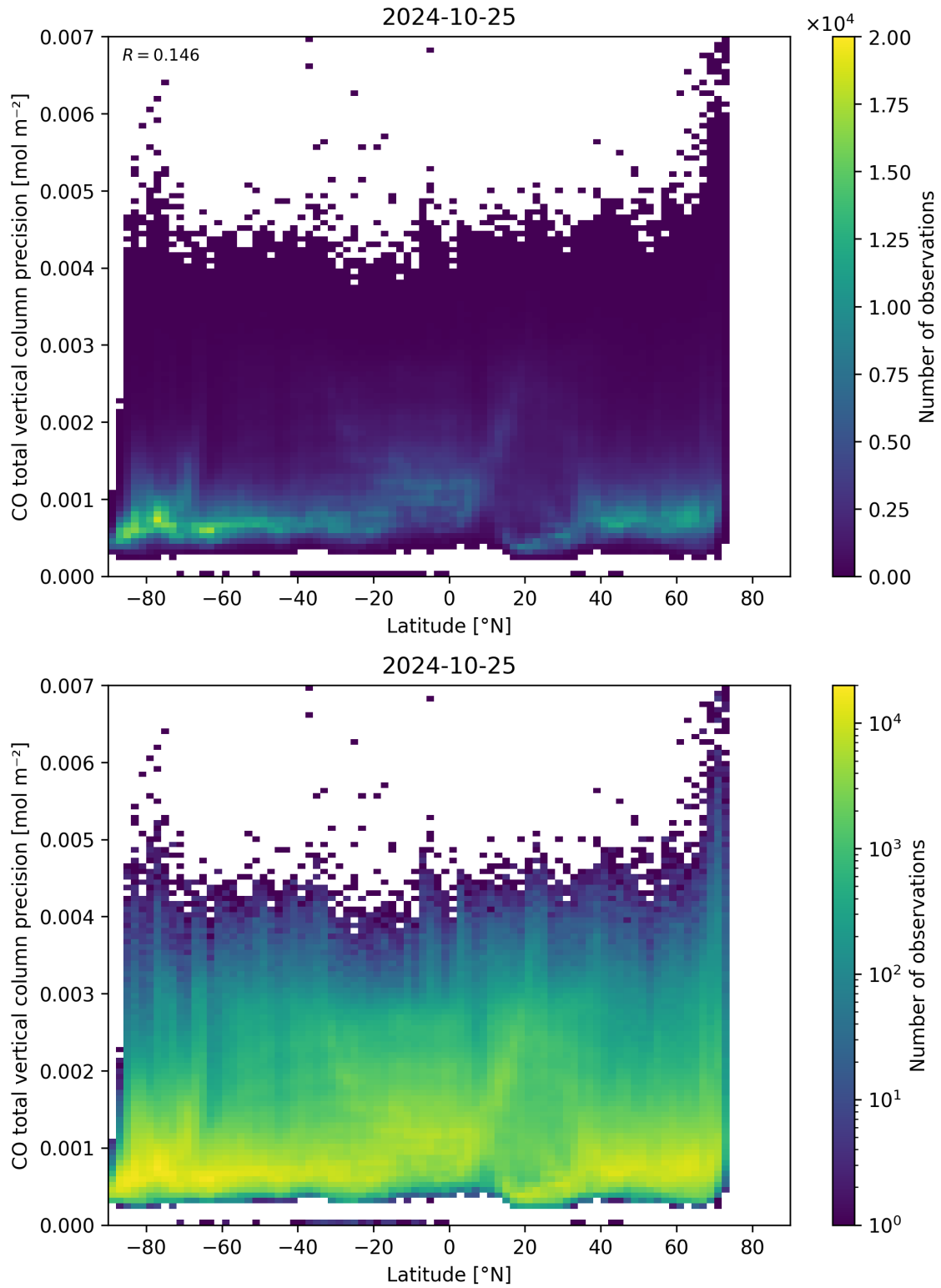
Figure 53: Scatter density plot of “Latitude” against “CO total vertical column precision” for 2024-10-24 to 2024-10-26.
