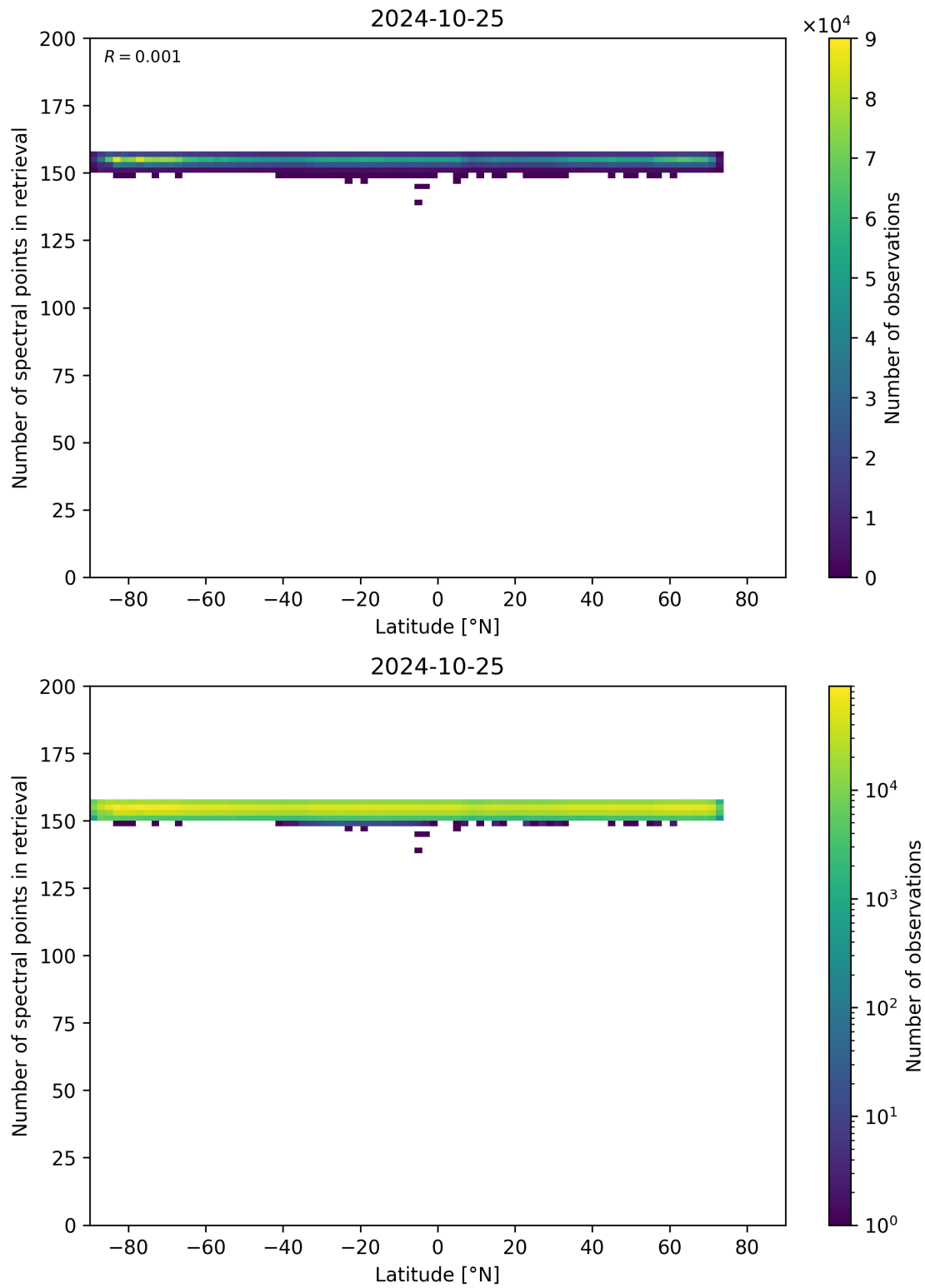
Figure 57: Scatter density plot of “Latitude” against “Number of spectral points in retrieval” for 2024-10-24 to 2024-10-26.
