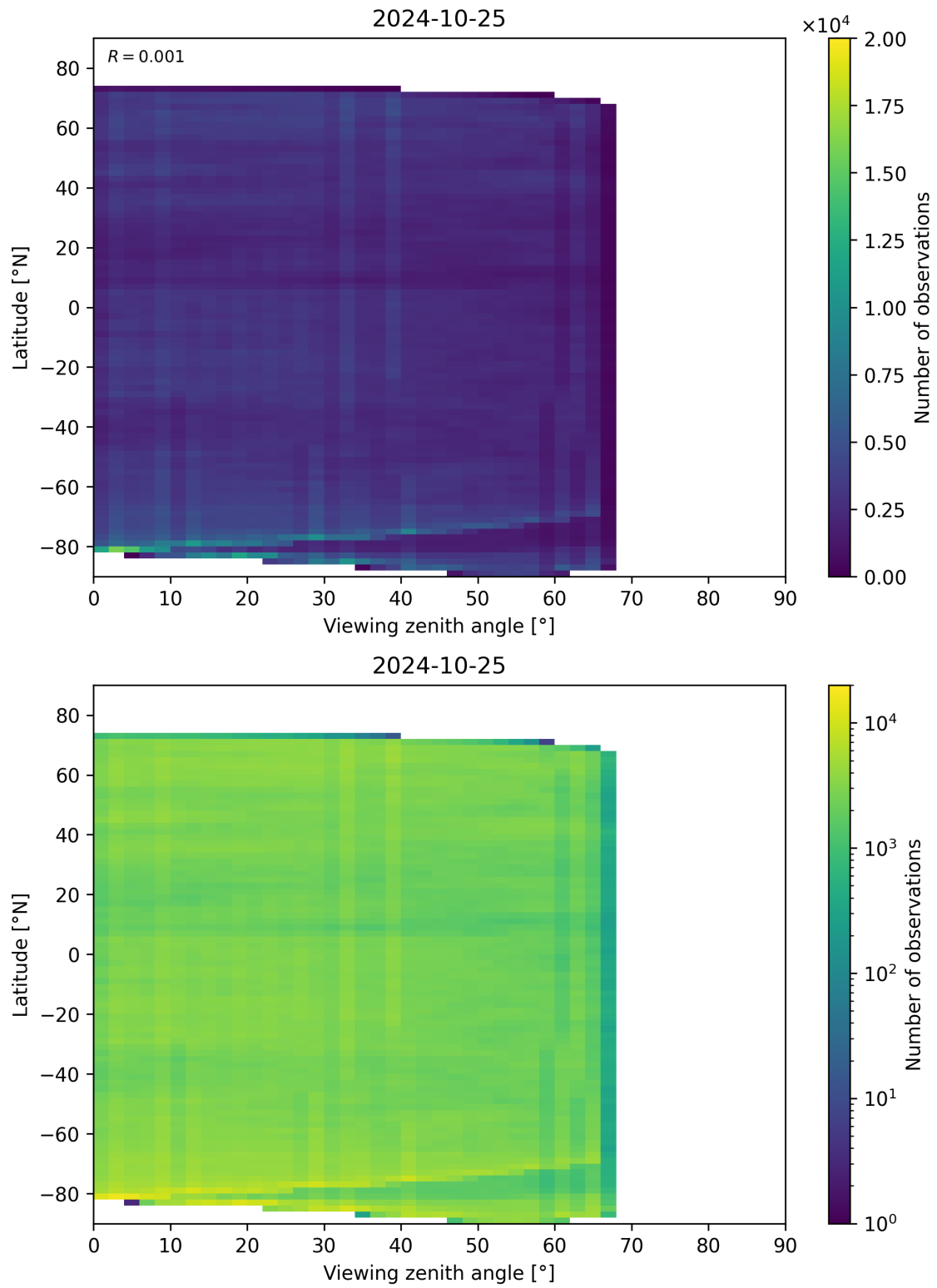
Figure 74: Scatter density plot of “Viewing zenith angle” against “Latitude” for 2024-10-24 to 2024-10-26.
