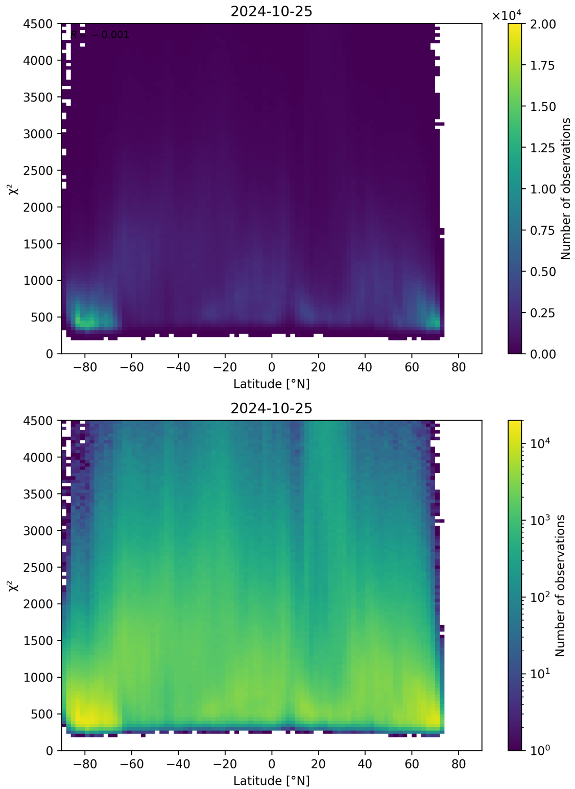
Figure 54: Scatter density plot of “Latitude” against “ \chi^2 ” for 2024-10-24 to 2024-10-26.
