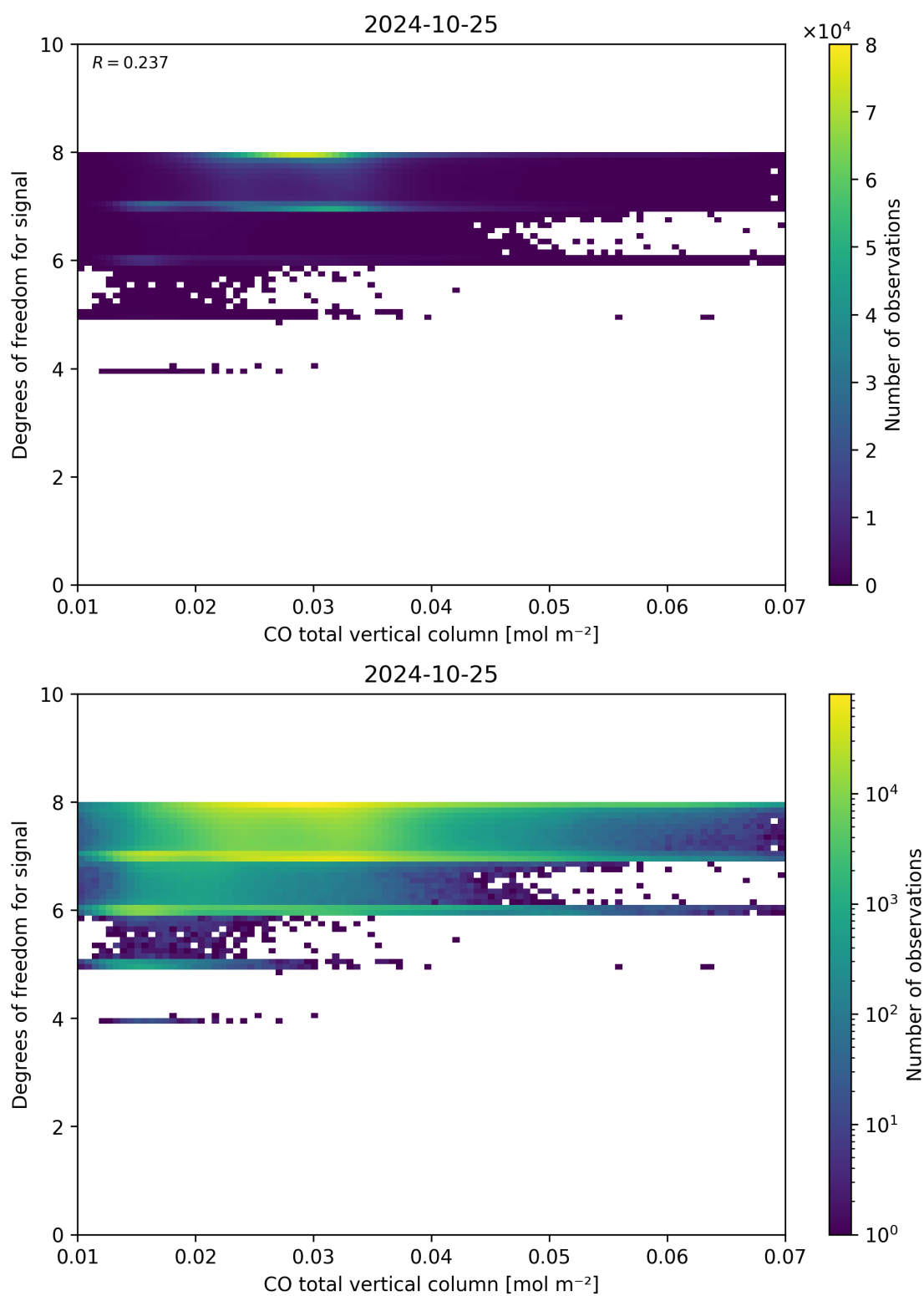
Figure 41: Scatter density plot of “CO total vertical column” against “Degrees of freedom for signal” for 2024-10-24 to 2024-10-26.
