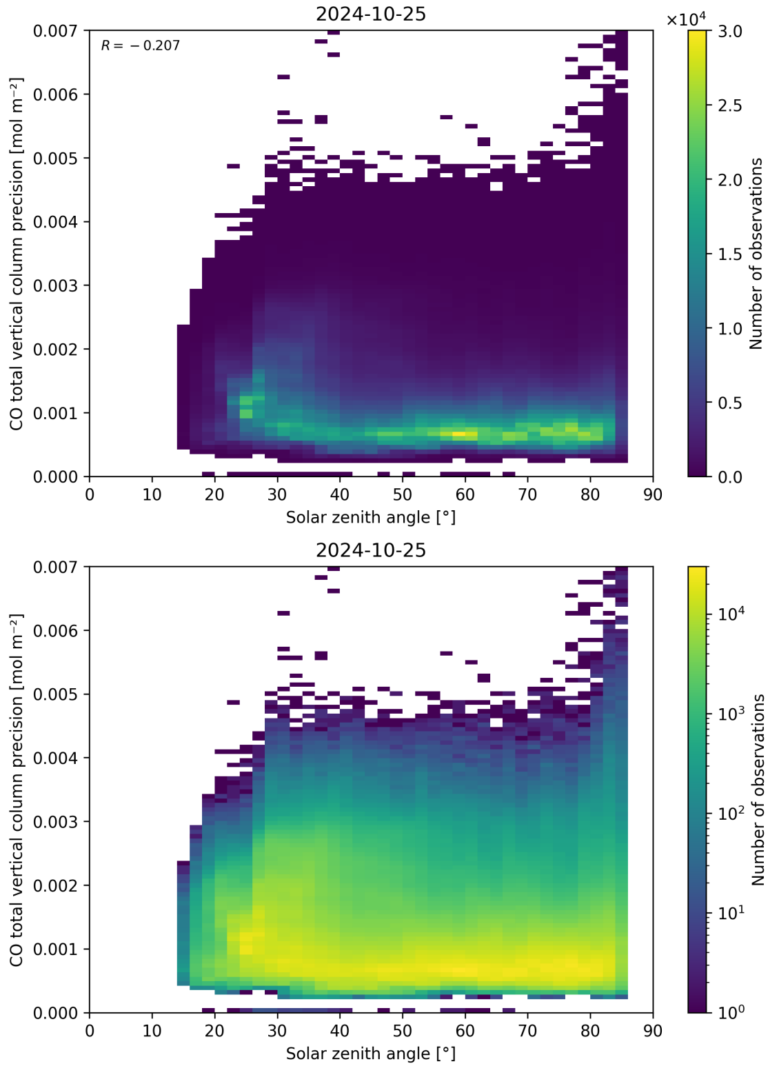
Figure 63: Scatter density plot of “Solar zenith angle” against “CO total vertical column precision” for 2024-10-24 to 2024-10-26.
