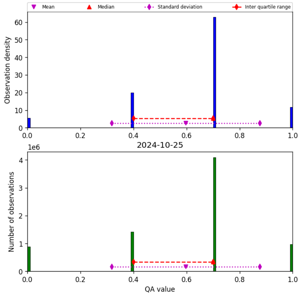
Figure 17: Histogram of “QA value” for 2024-10-24 to 2024-10-26
