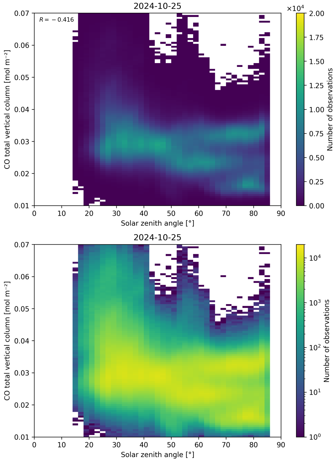
Figure 61: Scatter density plot of “Solar zenith angle” against “CO total vertical column” for 2024-10-24 to 2024-10-26.
