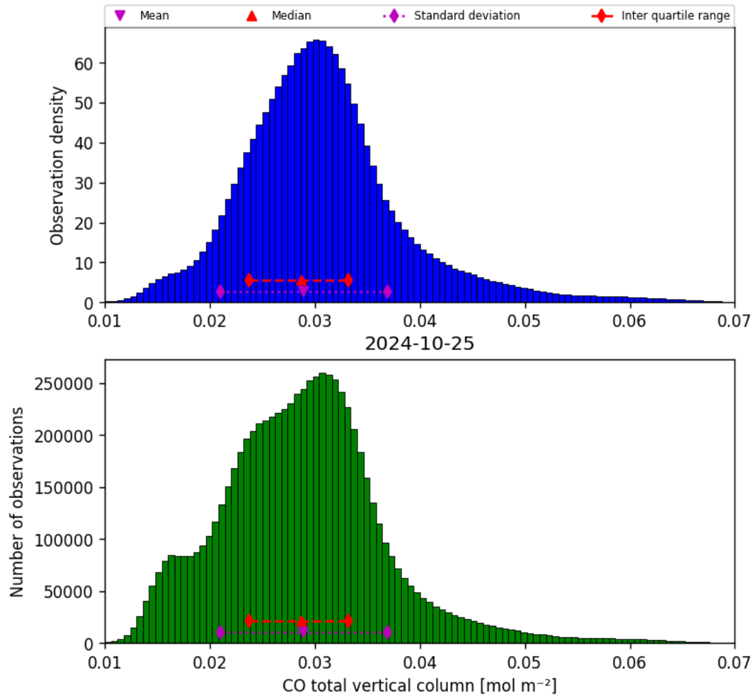
Figure 18: Histogram of “CO total vertical column” for 2024-10-24 to 2024-10-26
