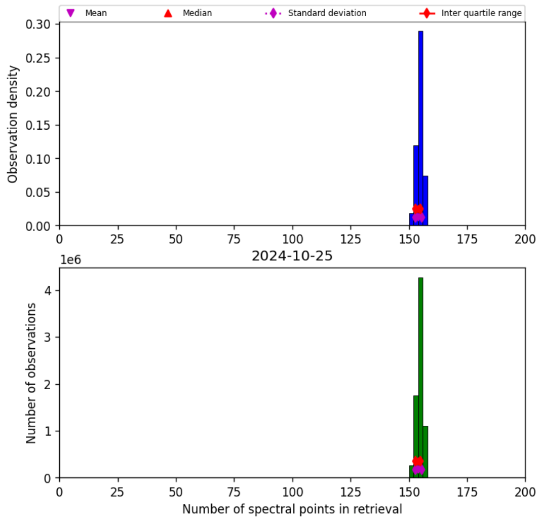
Figure 21: Histogram of “Number of spectral points in retrieval” for 2024-10-24 to 2024-10-26
