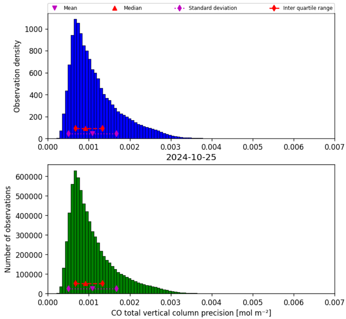
Figure 20: Histogram of “CO total vertical column precision” for 2024-10-24 to 2024-10-26
