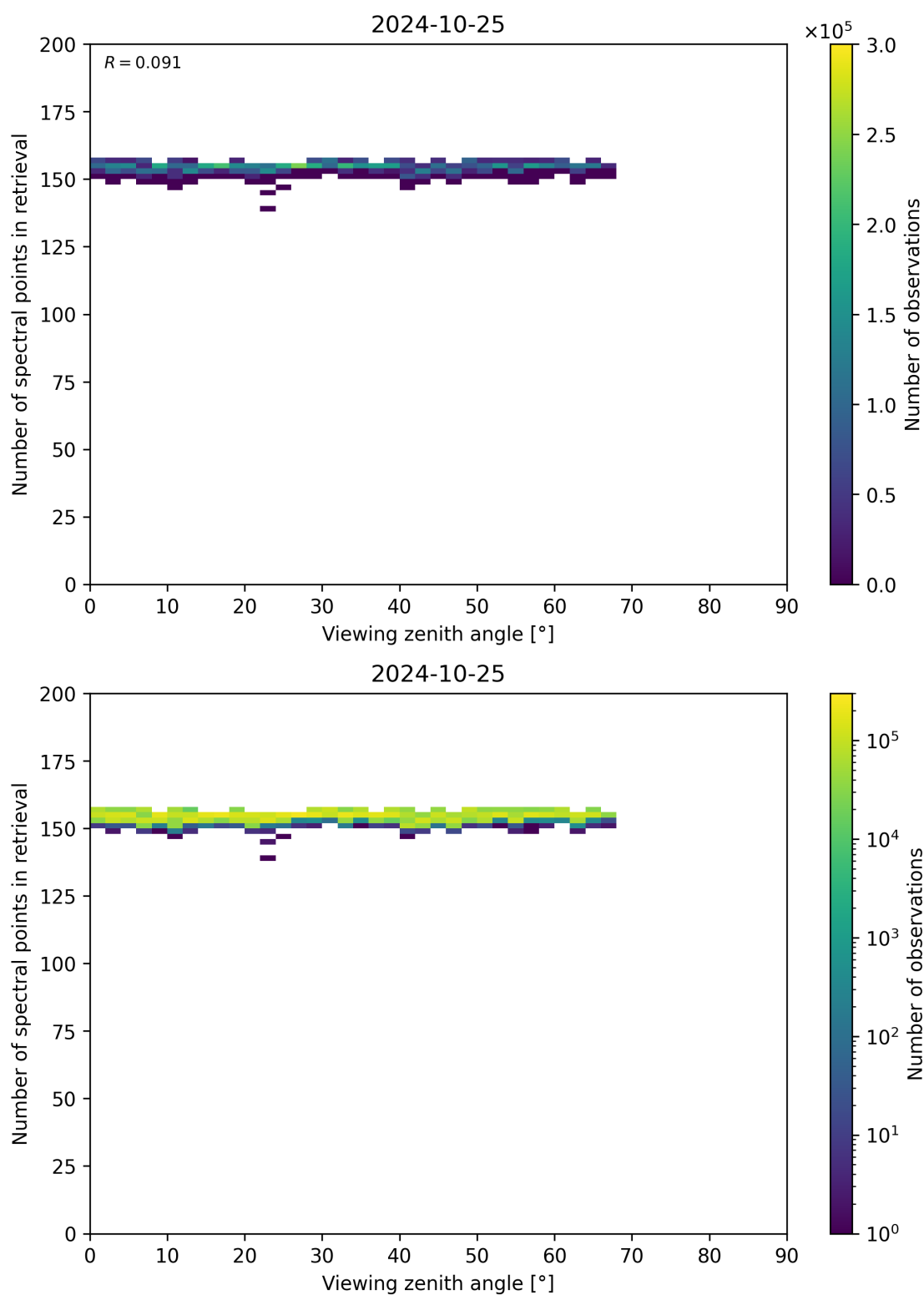
Figure 76: Scatter density plot of “Viewing zenith angle” against “Number of spectral points in retrieval” for 2024-10-24 to 2024-10-26.
