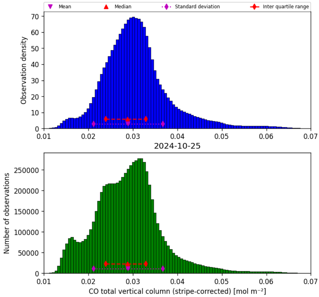
Figure 19: Histogram of “CO total vertical column (stripe-corrected)” for 2024-10-24 to 2024-10-26
