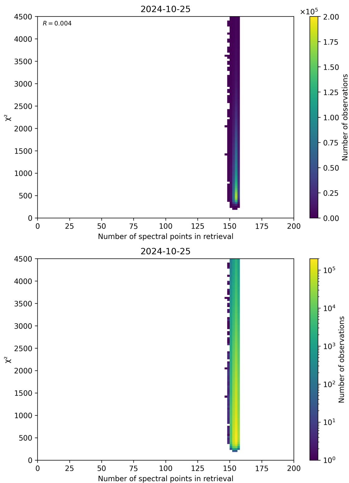
Figure 58: Scatter density plot of “Number of spectral points in retrieval” against “ \chi^2 ” for 2024-10-24 to 2024-10-26.
