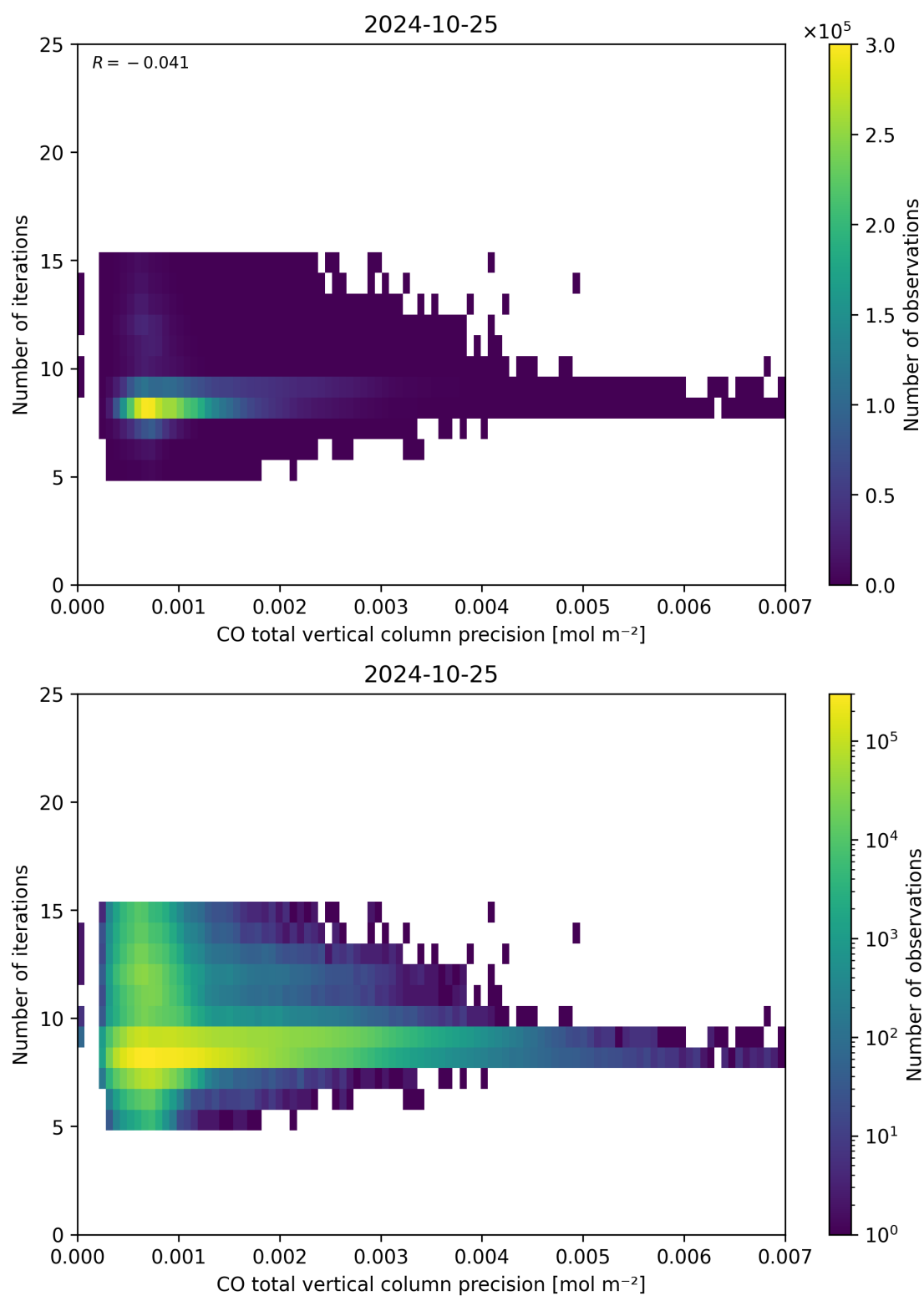
Figure 46: Scatter density plot of “CO total vertical column precision” against “Number of iterations” for 2024-10-24 to 2024-10-26.
