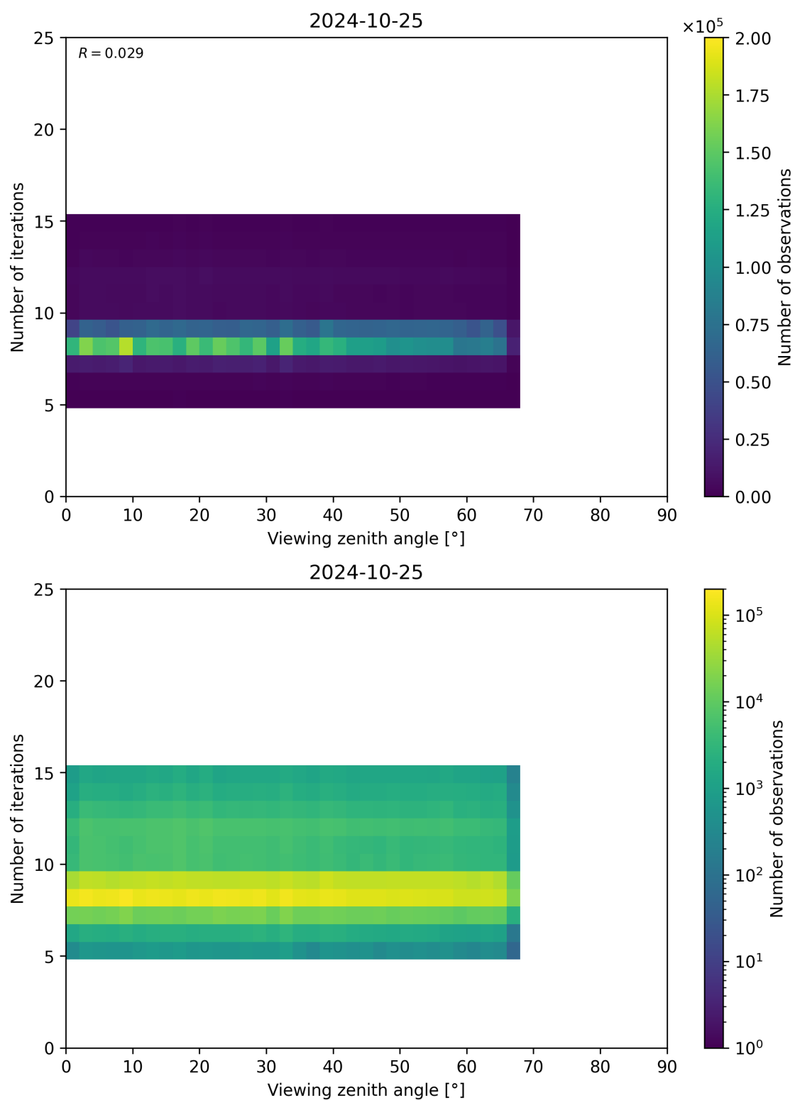
Figure 75: Scatter density plot of “Viewing zenith angle” against “Number of iterations” for 2024-10-24 to 2024-10-26.
