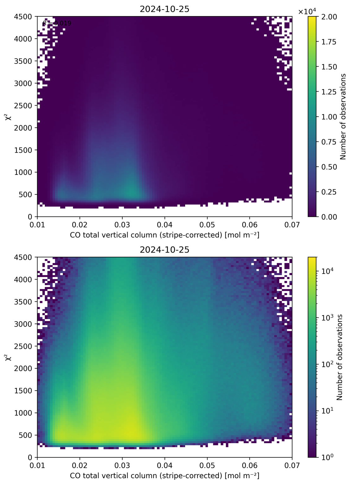
Figure 37: Scatter density plot of “CO total vertical column (stripe-corrected)” against “ \chi^2 ” for 2024-10-24 to 2024-10-26.
