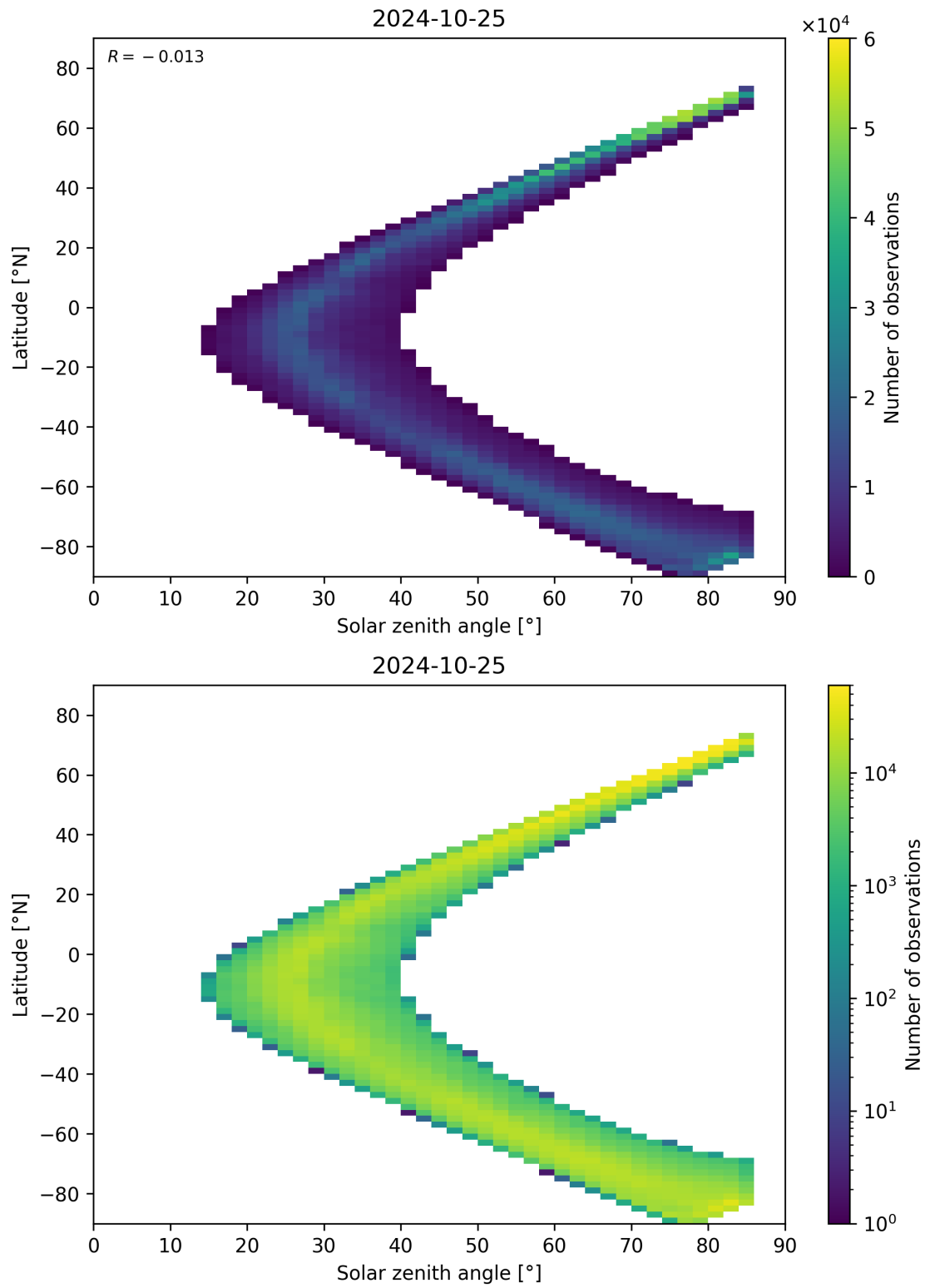
Figure 66: Scatter density plot of “Solar zenith angle” against “Latitude” for 2024-10-24 to 2024-10-26.
