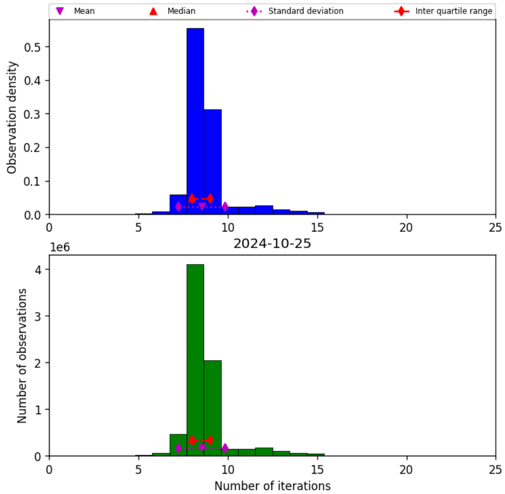
Figure 24: Histogram of “Number of iterations” for 2024-10-24 to 2024-10-26
