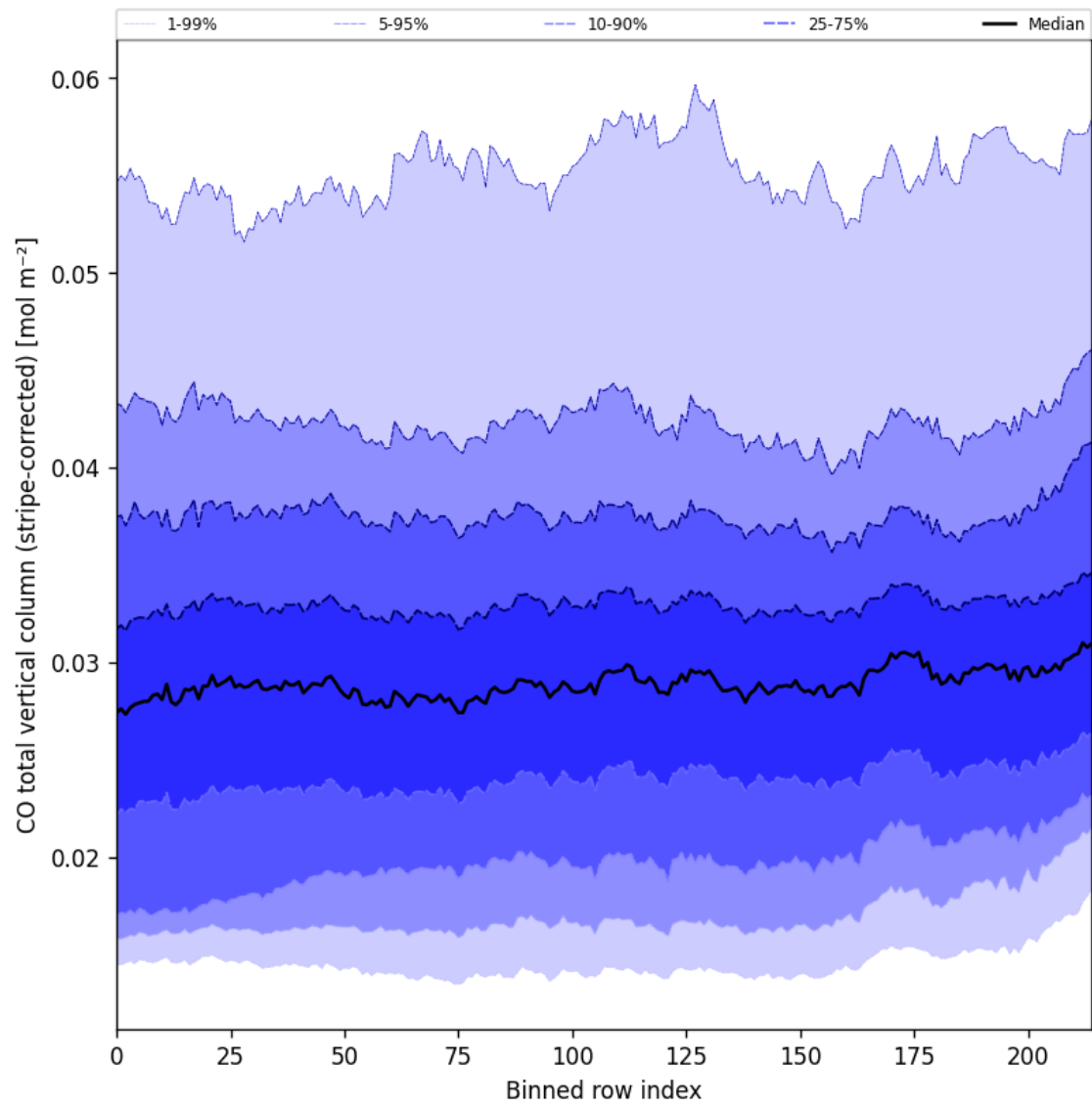
Figure 27: Along track statistics of “CO total vertical column (stripe-corrected)” for 2024-10-24 to 2024-10-26
