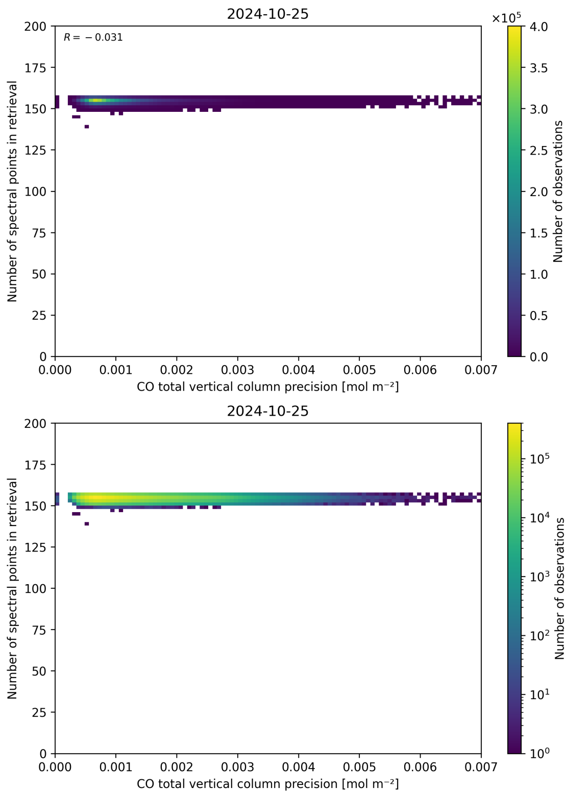
Figure 47: Scatter density plot of “CO total vertical column precision” against “Number of spectral points in retrieval” for 2024-10-24 to 2024-10-26.
