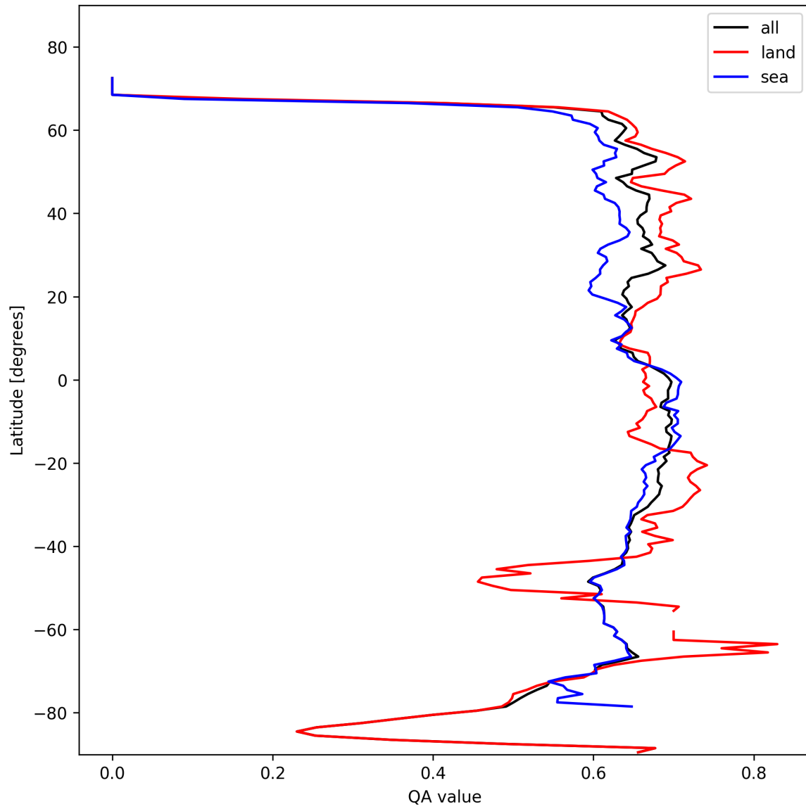
Figure 9: Zonal average of “QA value” for 2024-10-24 to 2024-10-26.
