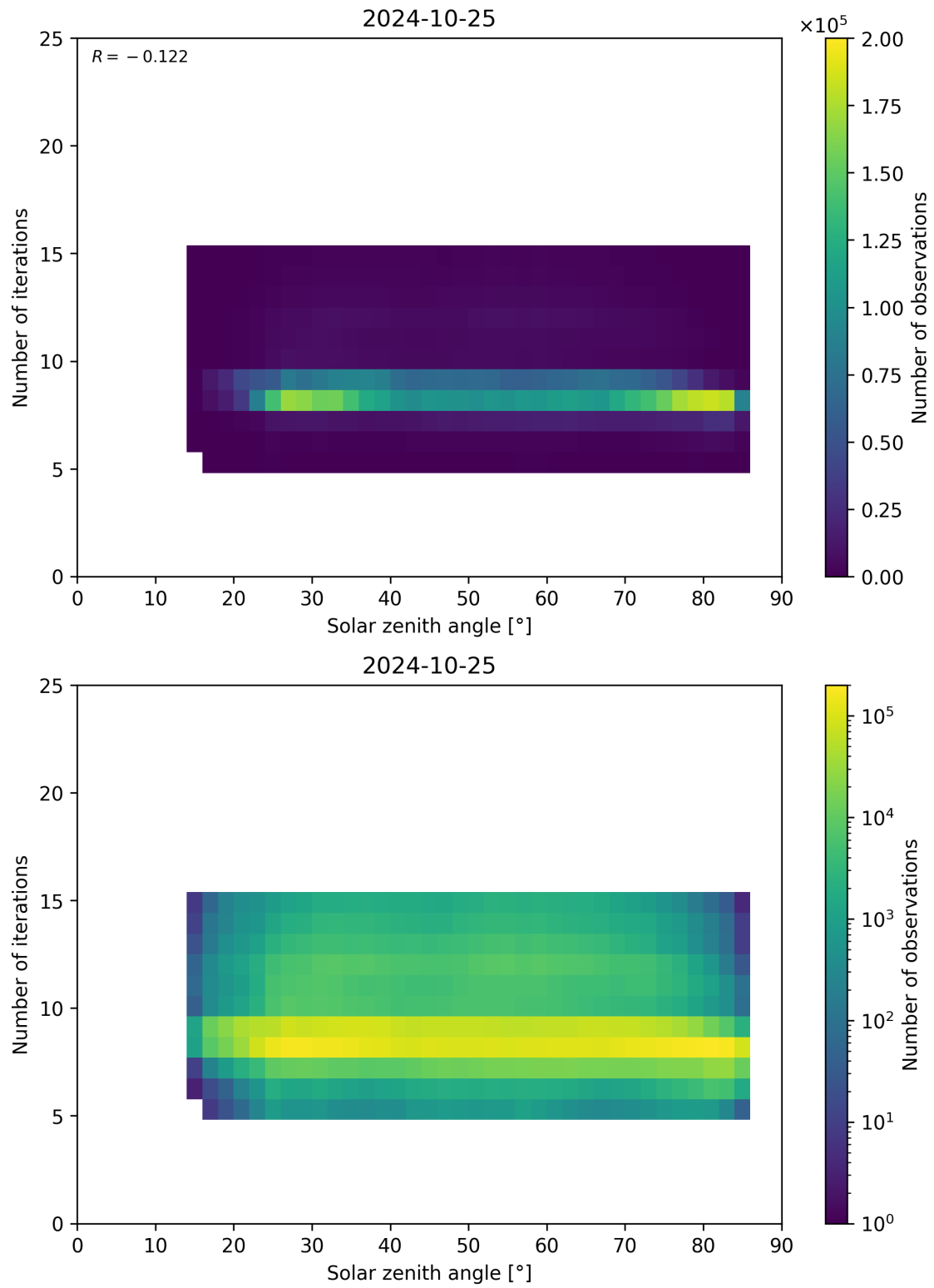
Figure 67: Scatter density plot of “Solar zenith angle” against “Number of iterations” for 2024-10-24 to 2024-10-26.
