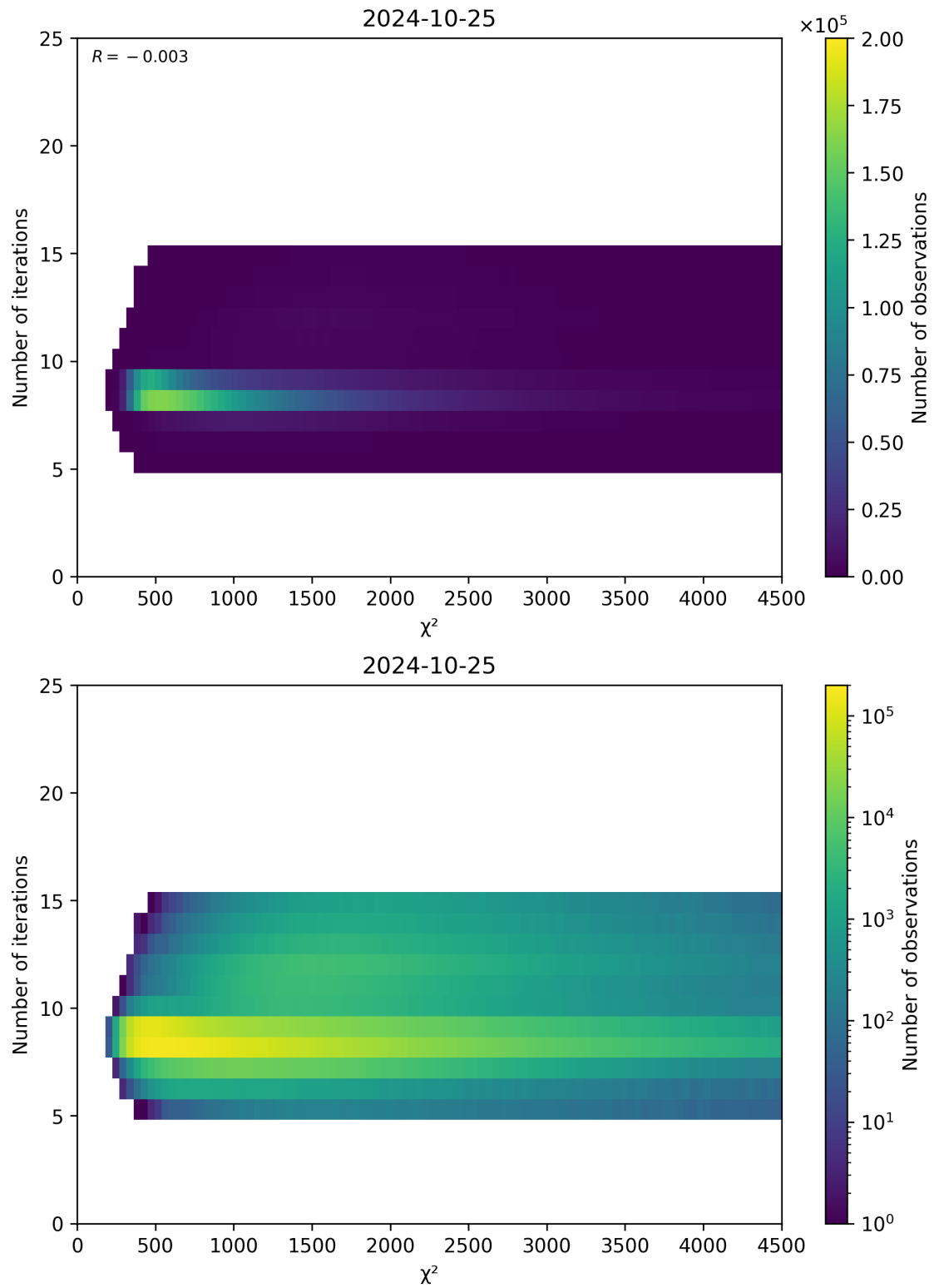
Figure 49: Scatter density plot of “ \chi^2 ” against “Number of iterations” for 2024-10-24 to 2024-10-26.
