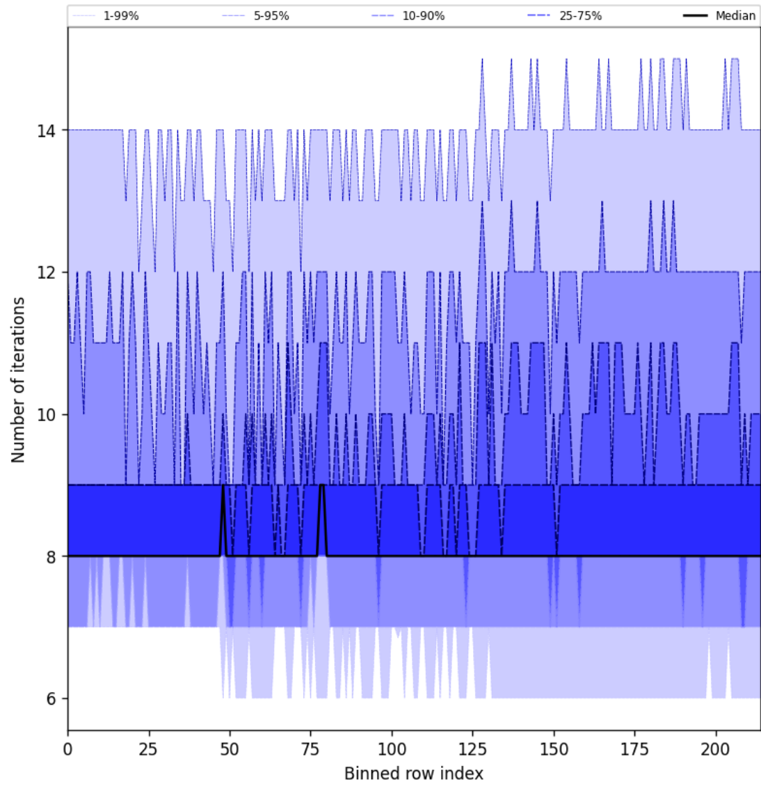
Figure 32: Along track statistics of “Number of iterations” for 2024-10-24 to 2024-10-26
