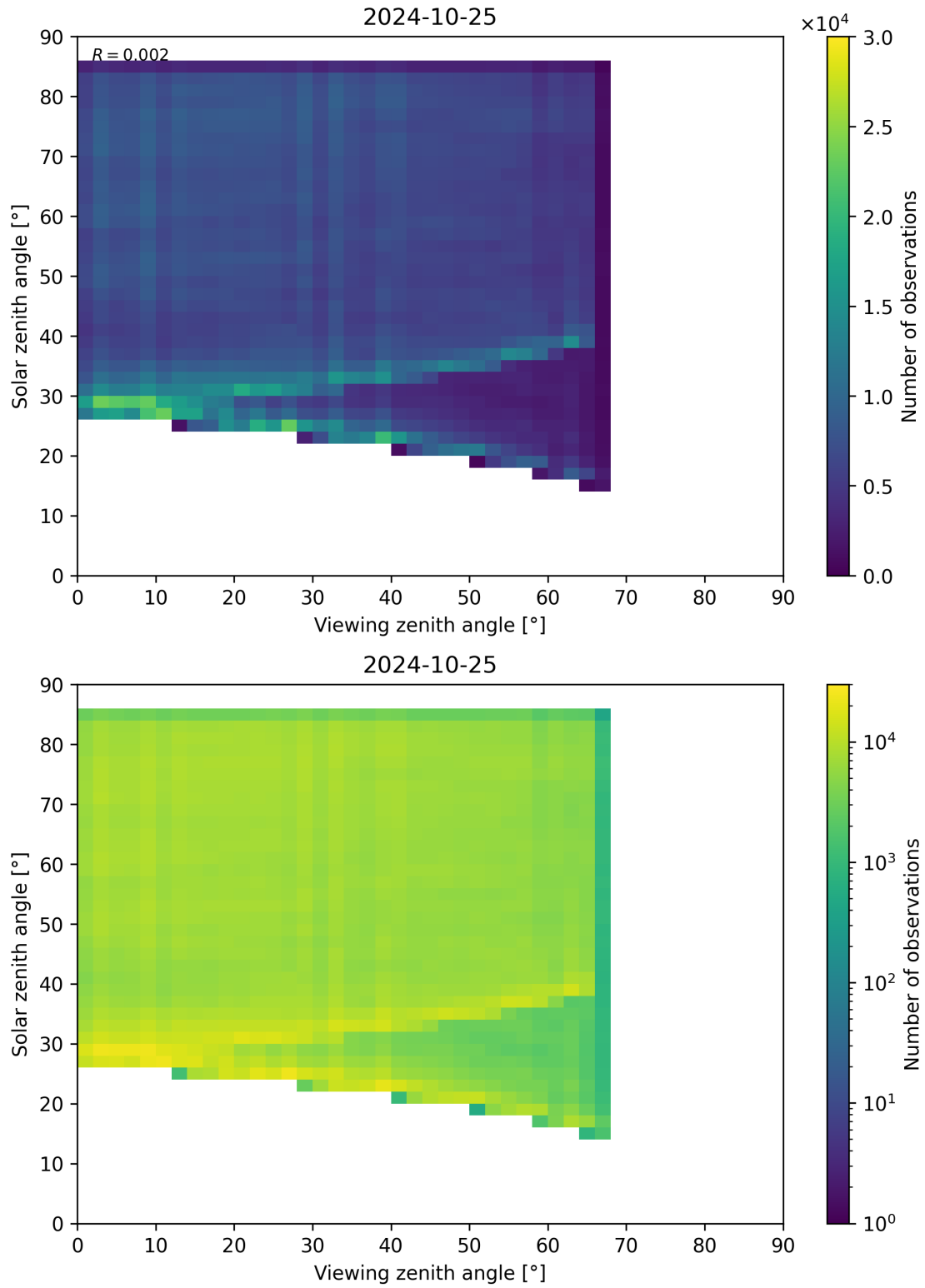
Figure 77: Scatter density plot of “Viewing zenith angle” against “Solar zenith angle” for 2024-10-24 to 2024-10-26.
