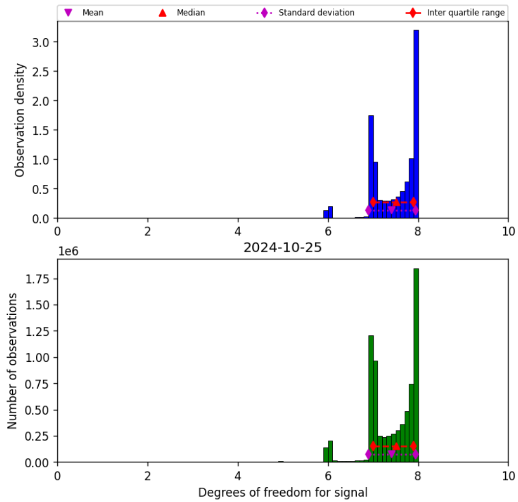
Figure 23: Histogram of “Degrees of freedom for signal” for 2024-10-24 to 2024-10-26
