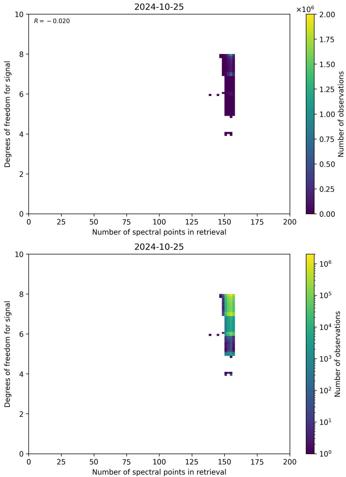
Figure 59: Scatter density plot of “Number of spectral points in retrieval” against “Degrees of freedom for signal” for 2024-10-24 to 2024-10-26.
