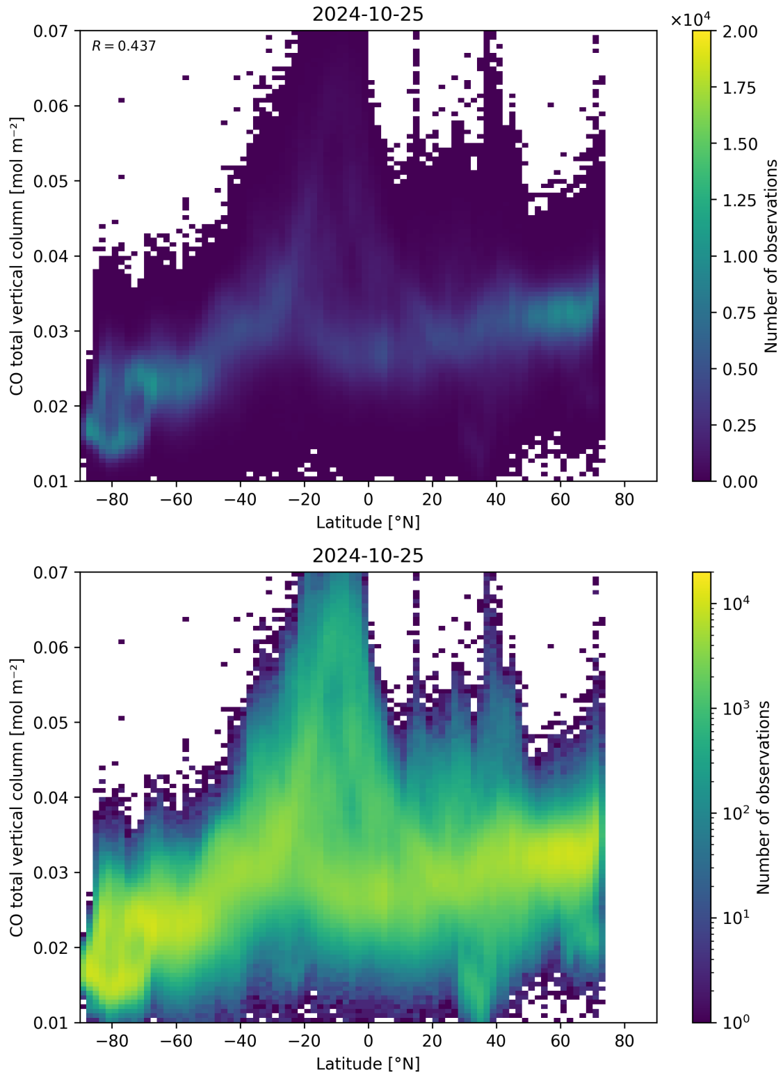
Figure 51: Scatter density plot of “Latitude” against “CO total vertical column” for 2024-10-24 to 2024-10-26.
