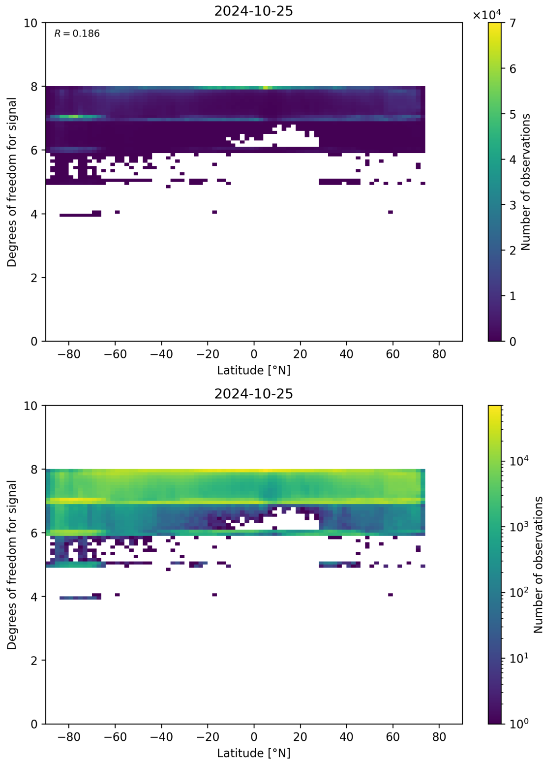
Figure 55: Scatter density plot of “Latitude” against “Degrees of freedom for signal” for 2024-10-24 to 2024-10-26.
