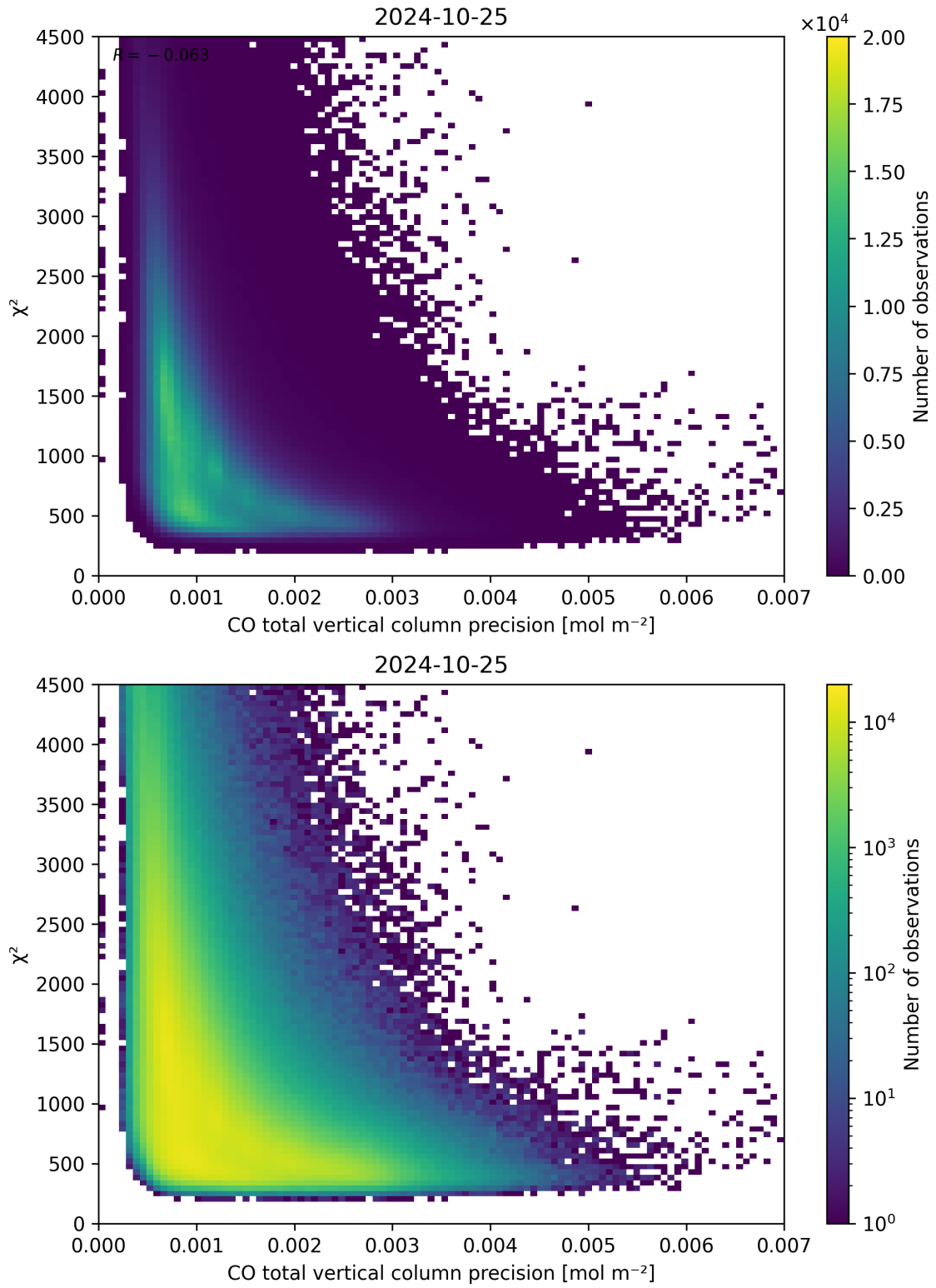
Figure 44: Scatter density plot of “CO total vertical column precision” against “ \chi^2 ” for 2024-10-24 to 2024-10-26.
