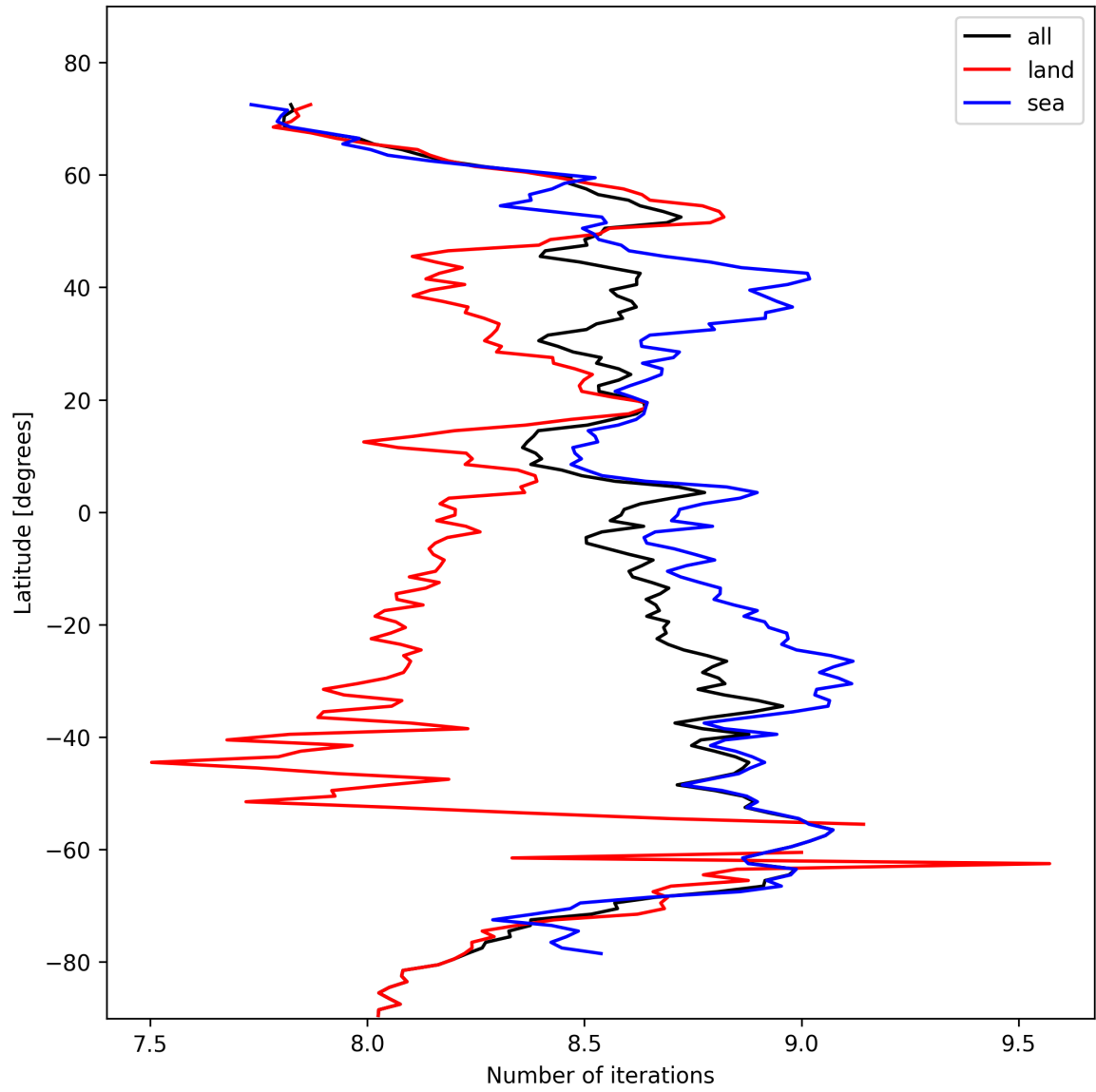
Figure 16: Zonal average of “Number of iterations” for 2024-10-24 to 2024-10-26.
