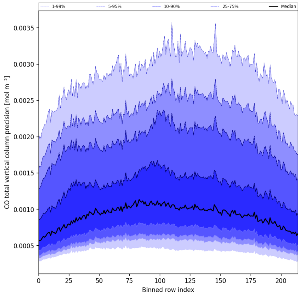
Figure 28: Along track statistics of “CO total vertical column precision” for 2024-10-24 to 2024-10-26
