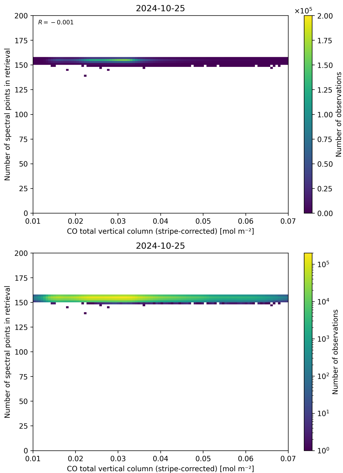
Figure 40: Scatter density plot of “CO total vertical column (stripe-corrected)” against “Number of spectral points in retrieval” for 2024-10-24 to 2024-10-26.
