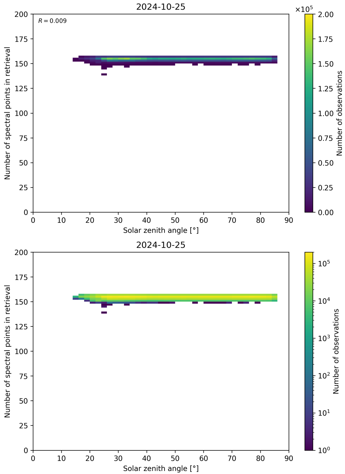
Figure 68: Scatter density plot of “Solar zenith angle” against “Number of spectral points in retrieval” for 2024-10-24 to 2024-10-26.
