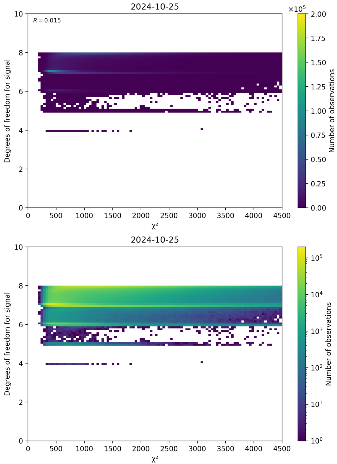
Figure 48: Scatter density plot of “ \chi^2 ” against “Degrees of freedom for signal” for 2024-10-24 to 2024-10-26.
