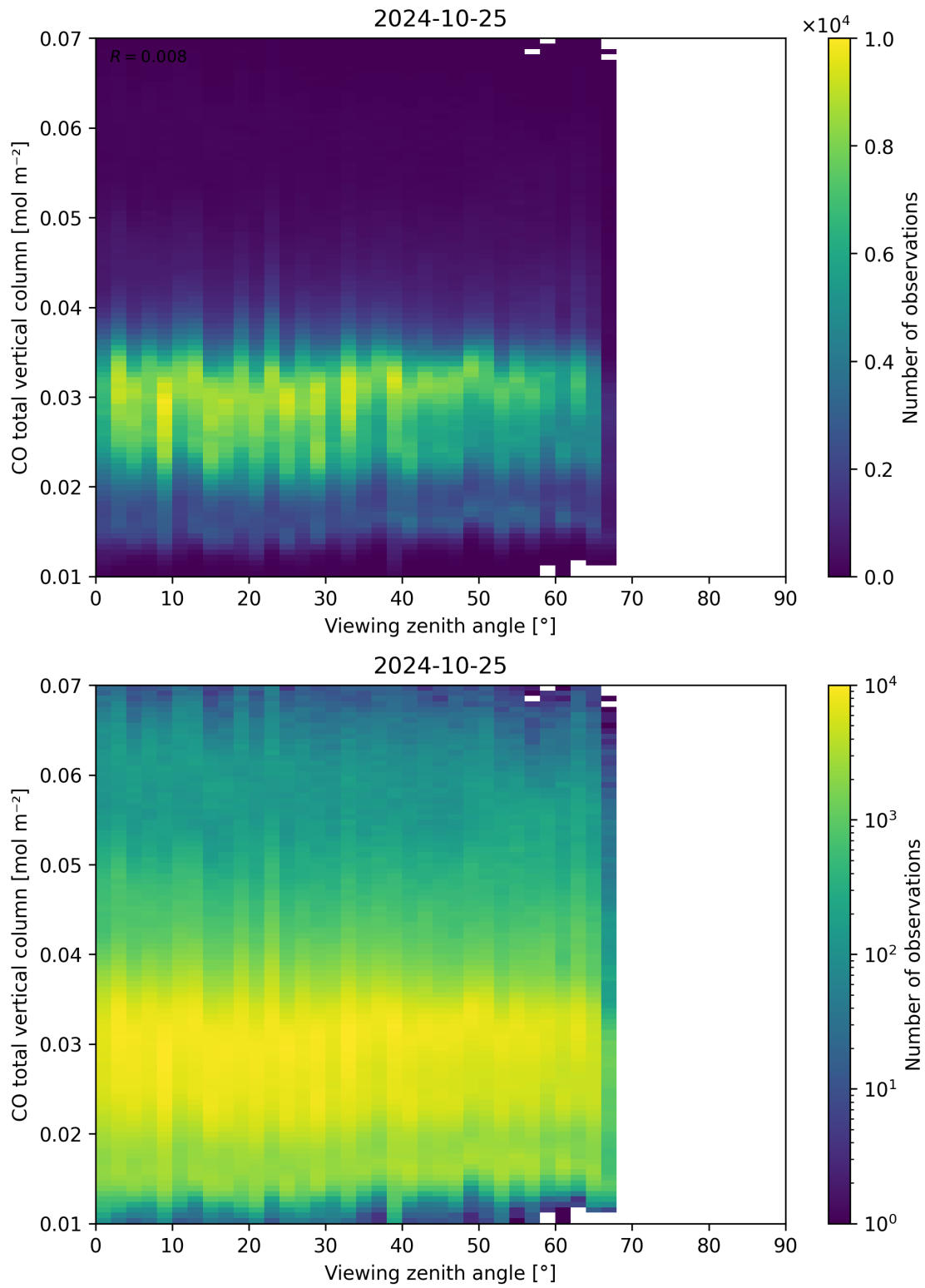
Figure 69: Scatter density plot of “Viewing zenith angle” against “CO total vertical column” for 2024-10-24 to 2024-10-26.
