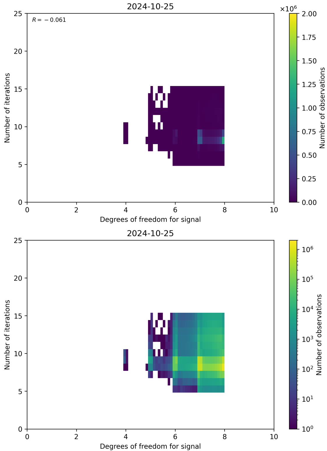
Figure 50: Scatter density plot of “Degrees of freedom for signal” against “Number of iterations” for 2024-10-24 to 2024-10-26.
