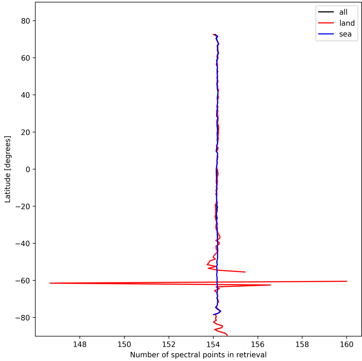
Figure 13: Zonal average of “Number of spectral points in retrieval” for 2024-10-24 to 2024-10-26.
