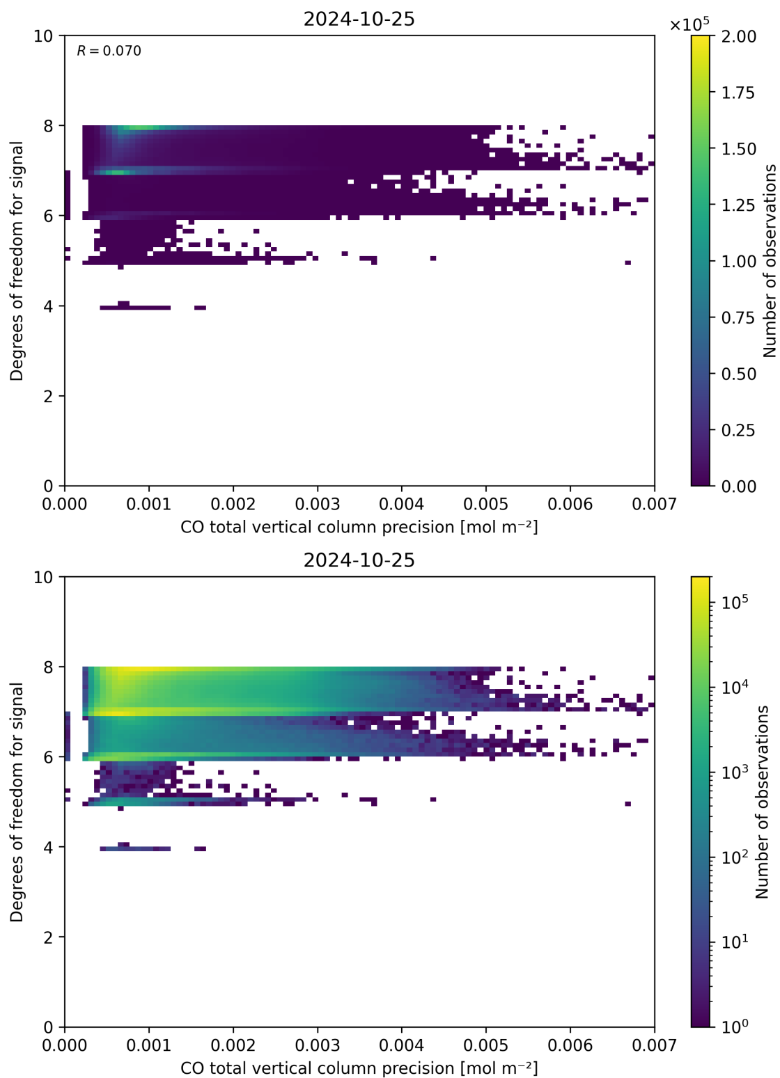
Figure 45: Scatter density plot of “CO total vertical column precision” against “Degrees of freedom for signal” for 2024-10-24 to 2024-10-26.
