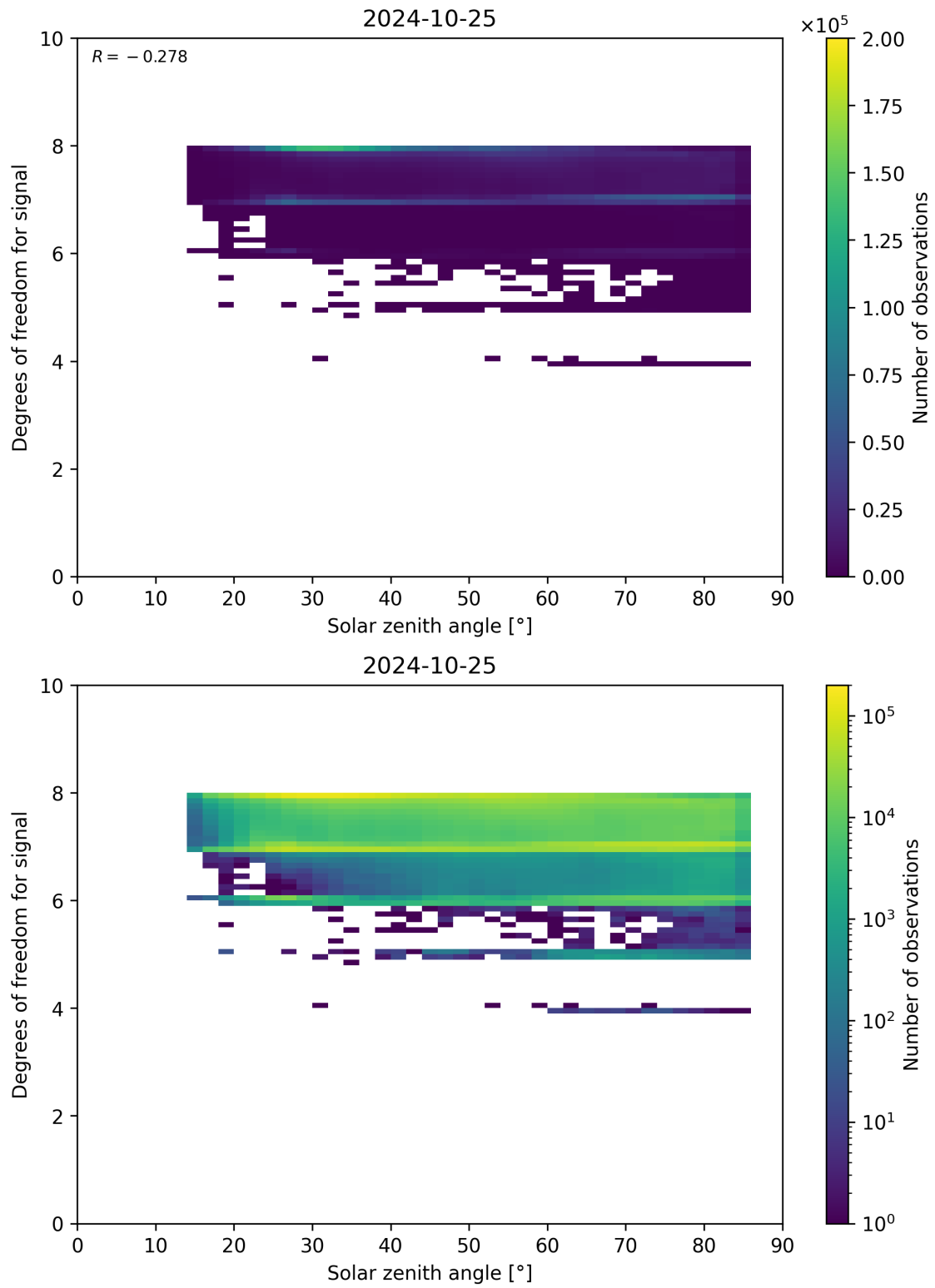
Figure 65: Scatter density plot of “Solar zenith angle” against “Degrees of freedom for signal” for 2024-10-24 to 2024-10-26.
