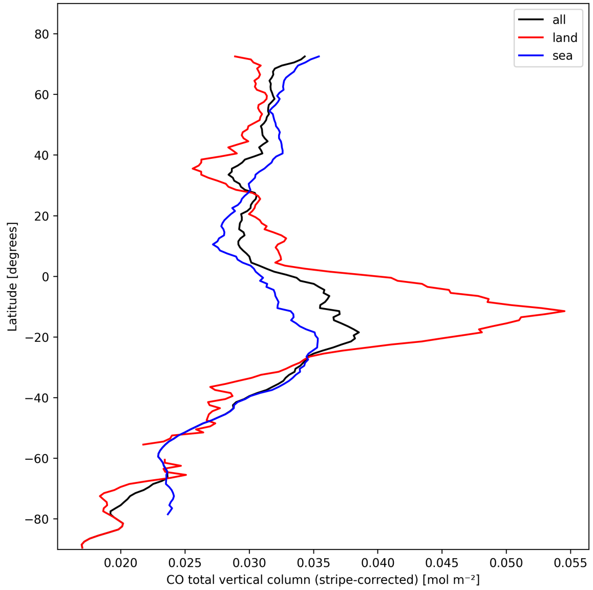
Figure 11: Zonal average of “CO total vertical column (stripe-corrected)” for 2024-10-24 to 2024-10-26.
