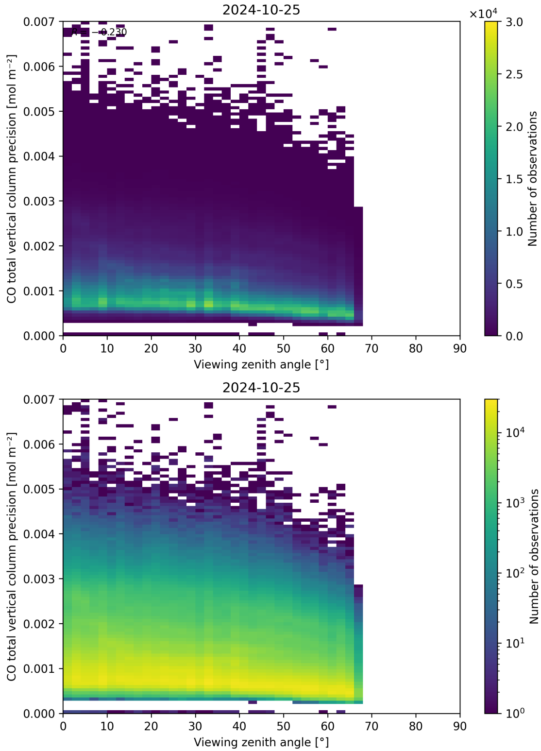
Figure 71: Scatter density plot of “Viewing zenith angle” against “CO total vertical column precision” for 2024-10-24 to 2024-10-26.
