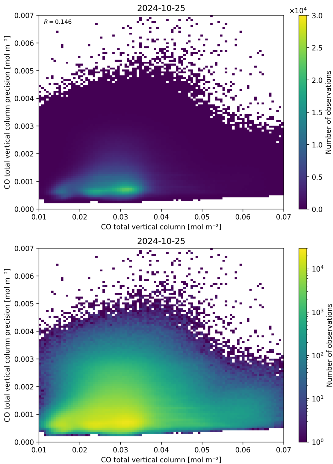
Figure 34: Scatter density plot of “CO total vertical column” against “CO total vertical column precision” for 2024-10-24 to 2024-10-26.
