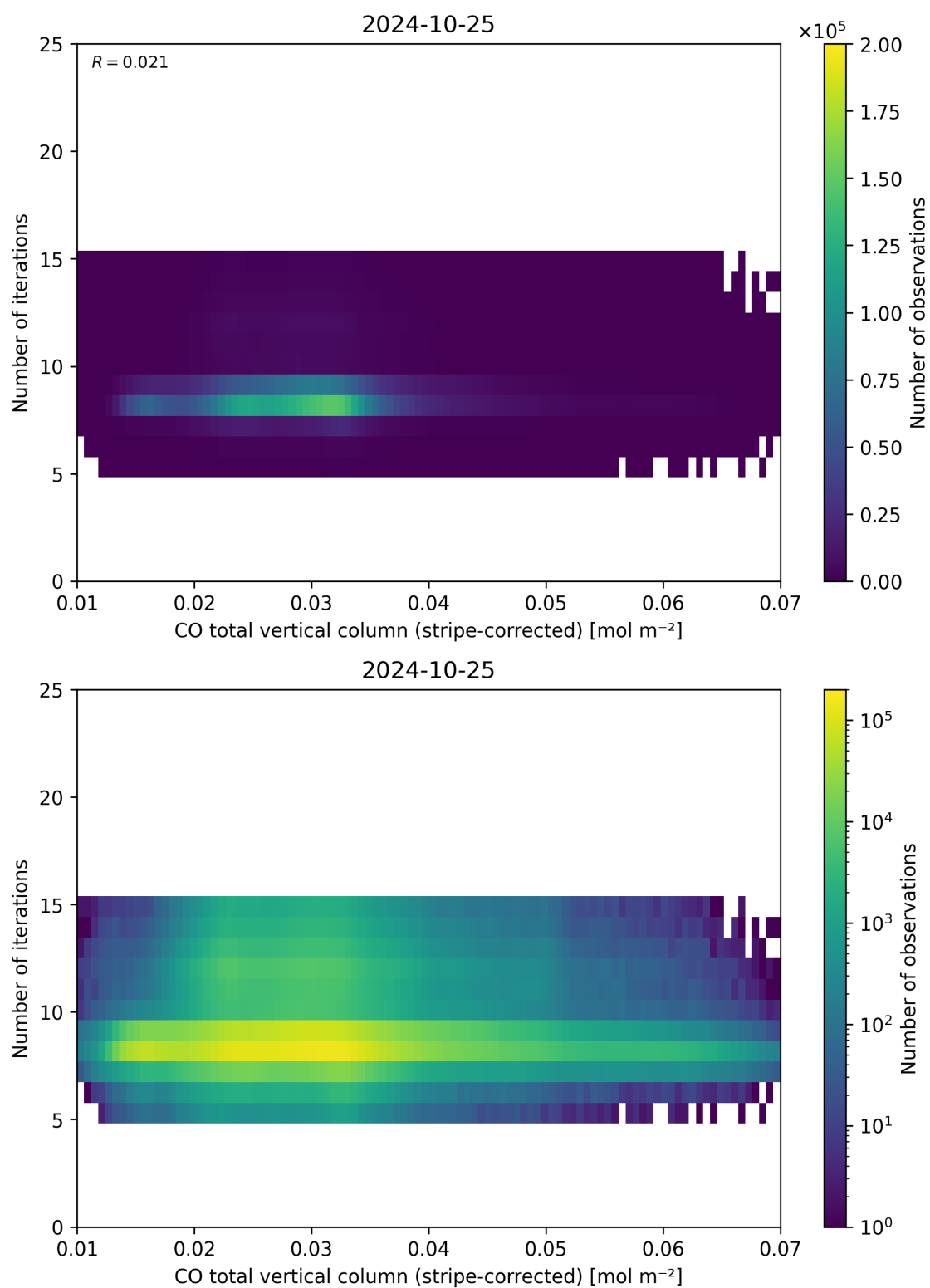
Figure 39: Scatter density plot of “CO total vertical column (stripe-corrected)” against “Number of iterations” for 2024-10-24 to 2024-10-26.
