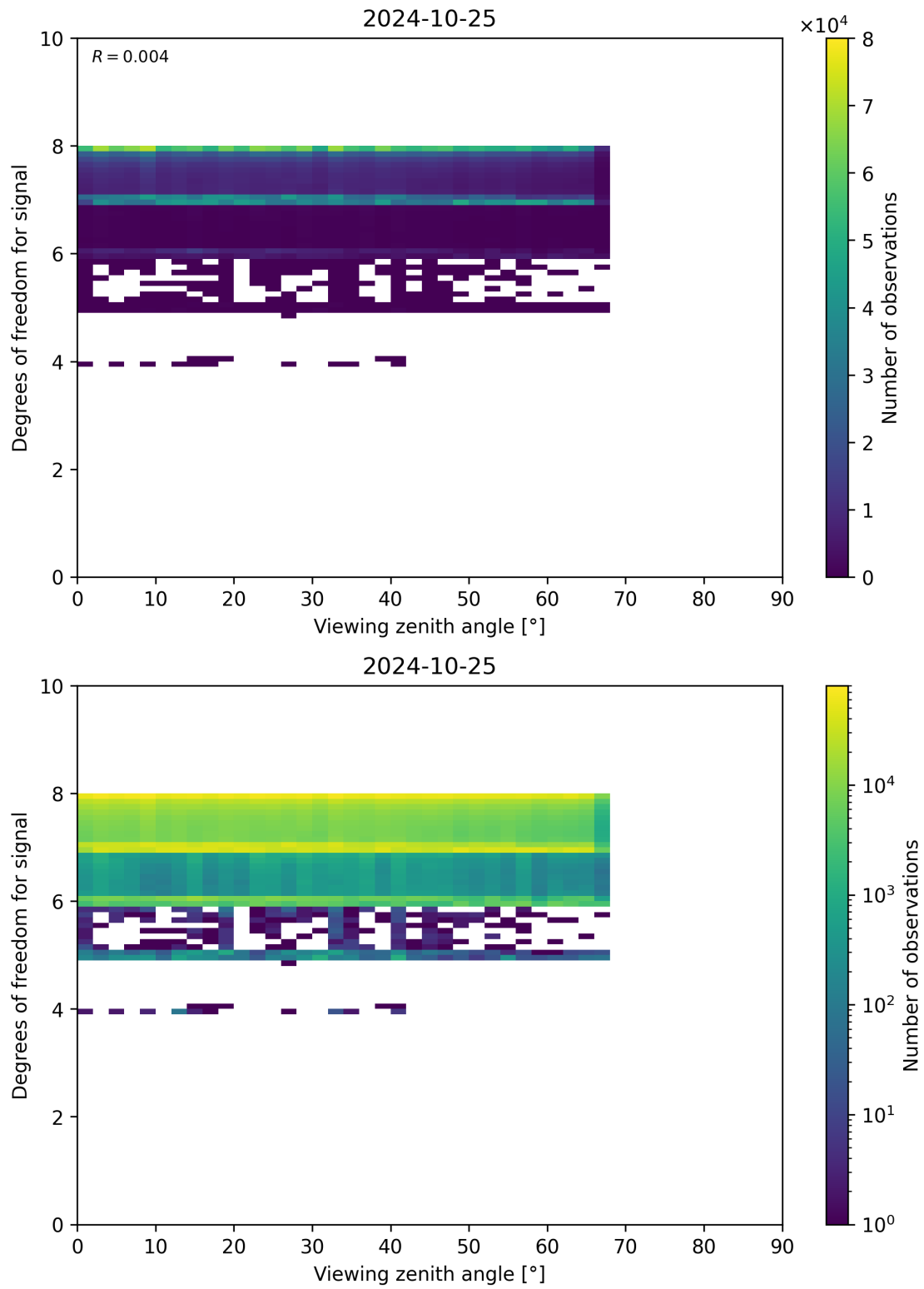
Figure 73: Scatter density plot of “Viewing zenith angle” against “Degrees of freedom for signal” for 2024-10-24 to 2024-10-26.
