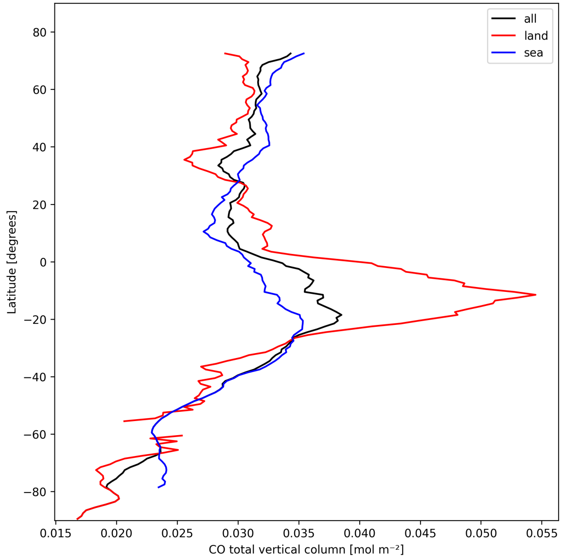
Figure 10: Zonal average of “CO total vertical column” for 2024-10-24 to 2024-10-26.
