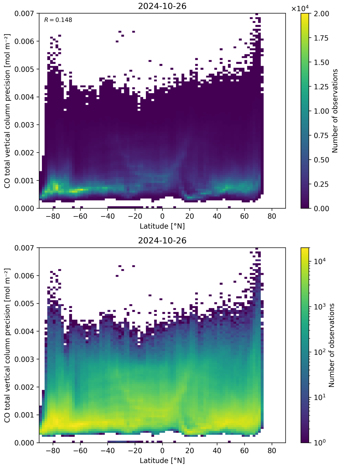
Figure 53: Scatter density plot of “Latitude” against “CO total vertical column precision” for 2024-10-25 to 2024-10-27.
