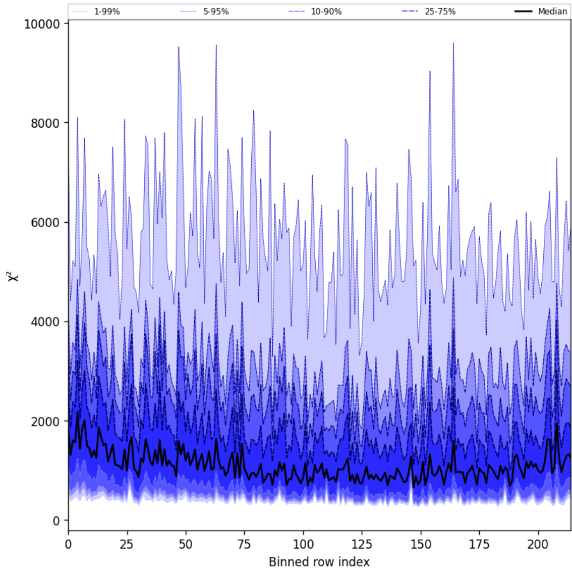
Figure 30: Along track statistics of “ \chi^2 ” for 2024-10-25 to 2024-10-27
