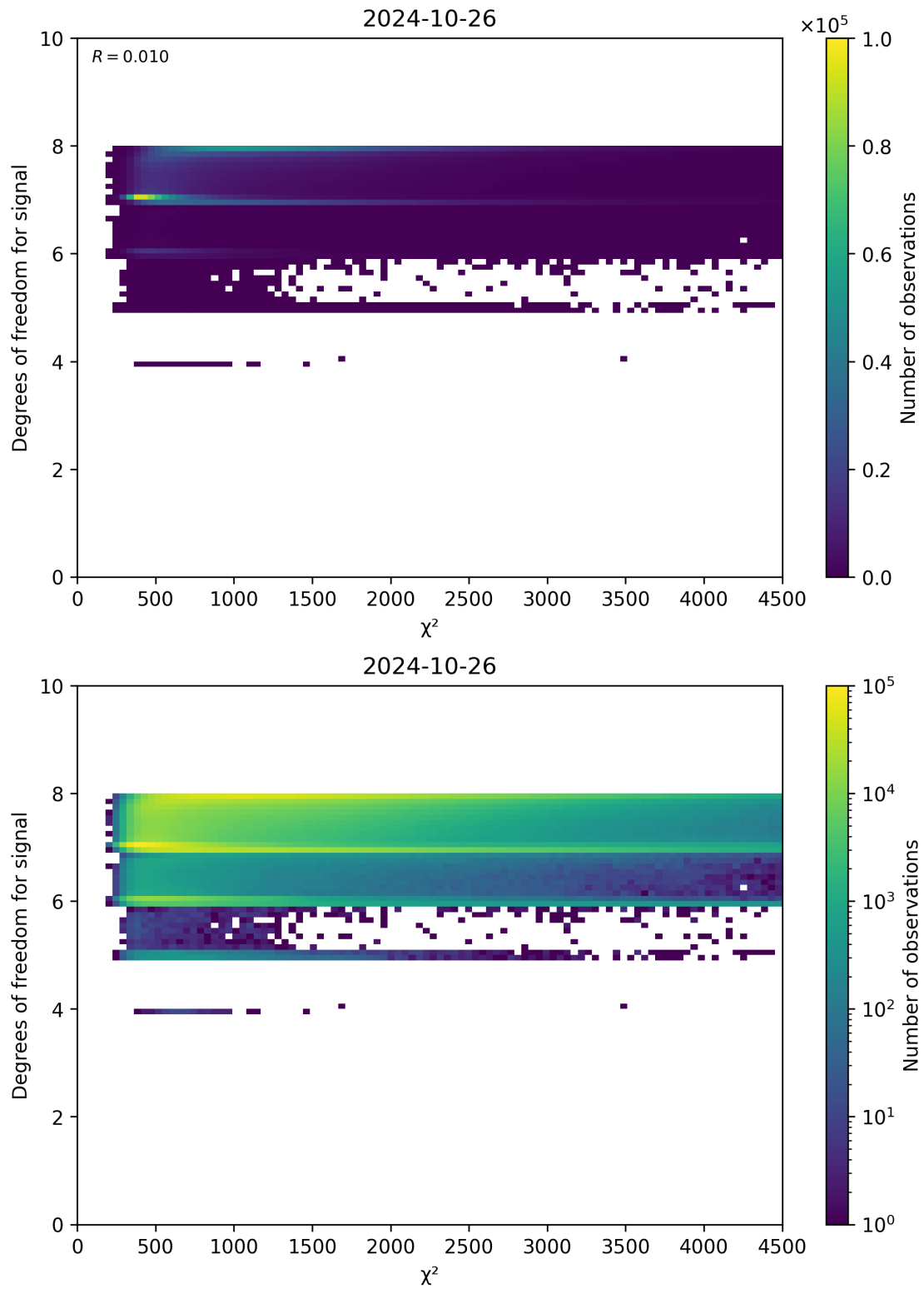
Figure 48: Scatter density plot of “ \chi^2 ” against “Degrees of freedom for signal” for 2024-10-25 to 2024-10-27.
