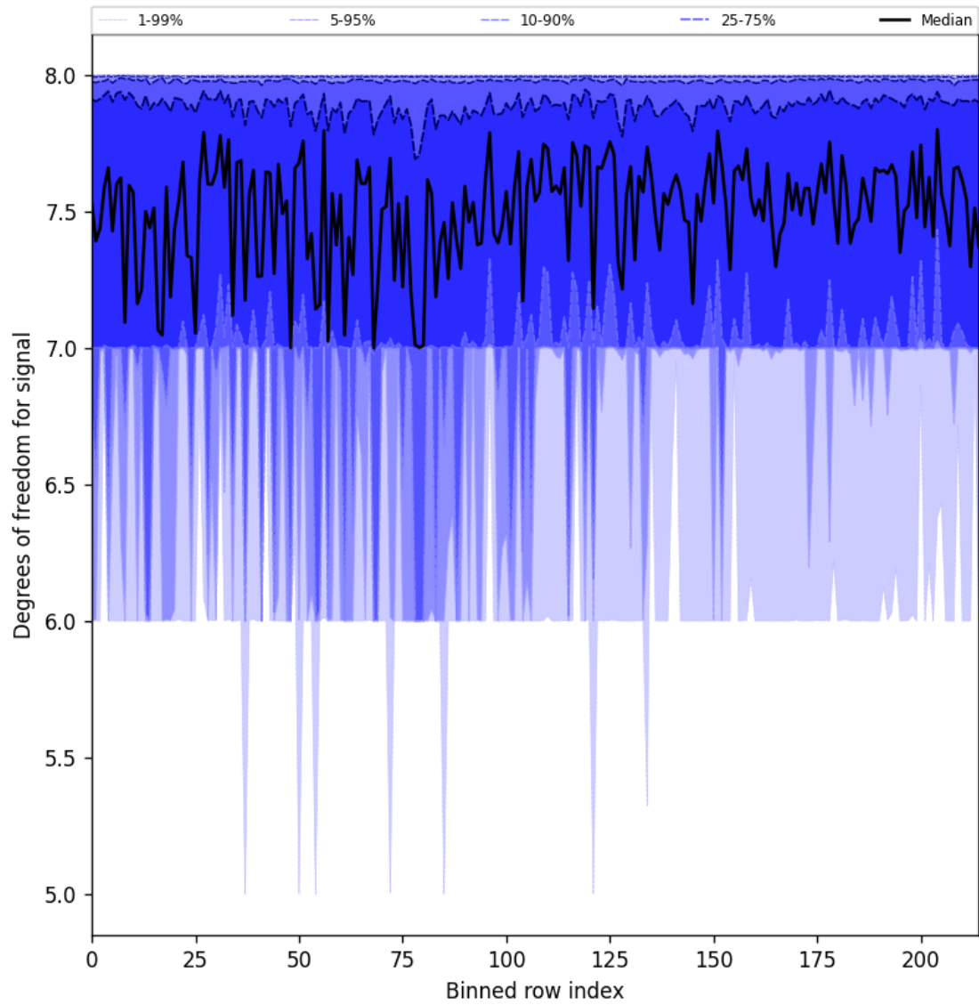
Figure 31: Along track statistics of “Degrees of freedom for signal” for 2024-10-25 to 2024-10-27
