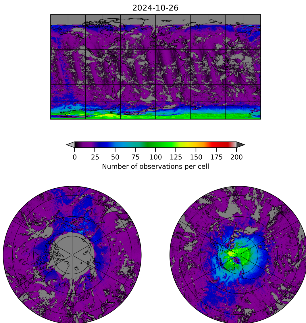
Figure 8: Map of the number of observations for 2024-10-25 to 2024-10-27
