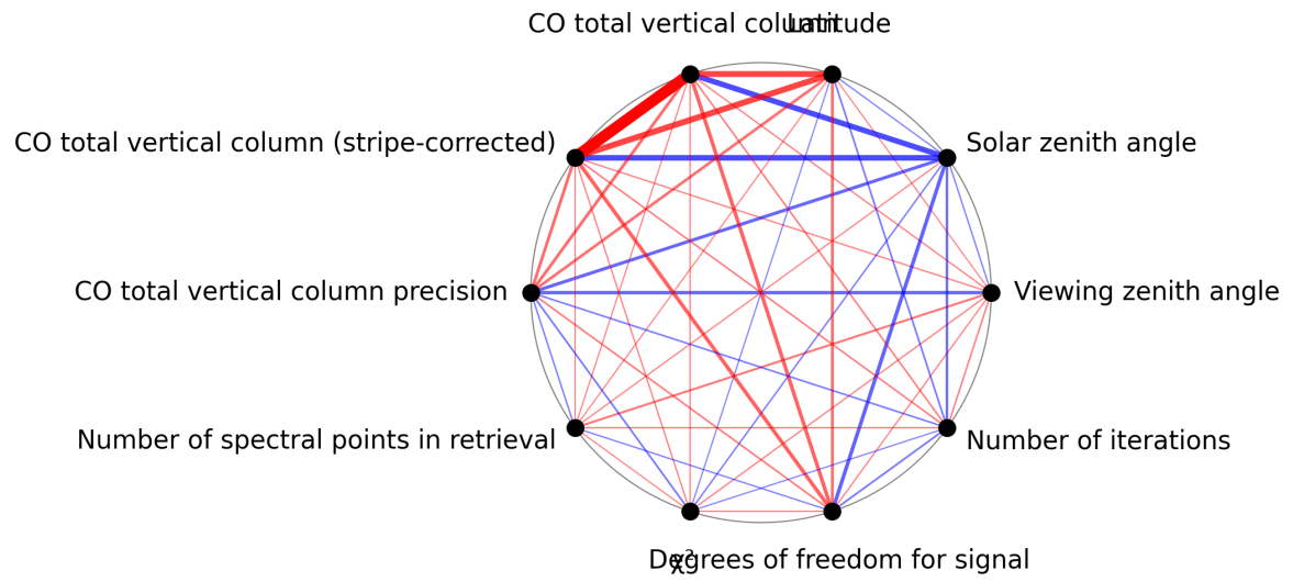
Figure 1: Map of correlation graph for 2024-10-25 to 2024-10-27.
