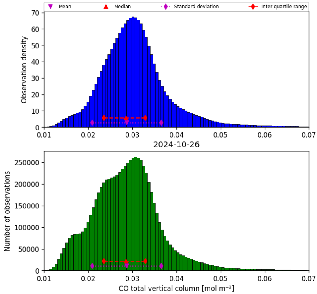
Figure 18: Histogram of “CO total vertical column” for 2024-10-25 to 2024-10-27
