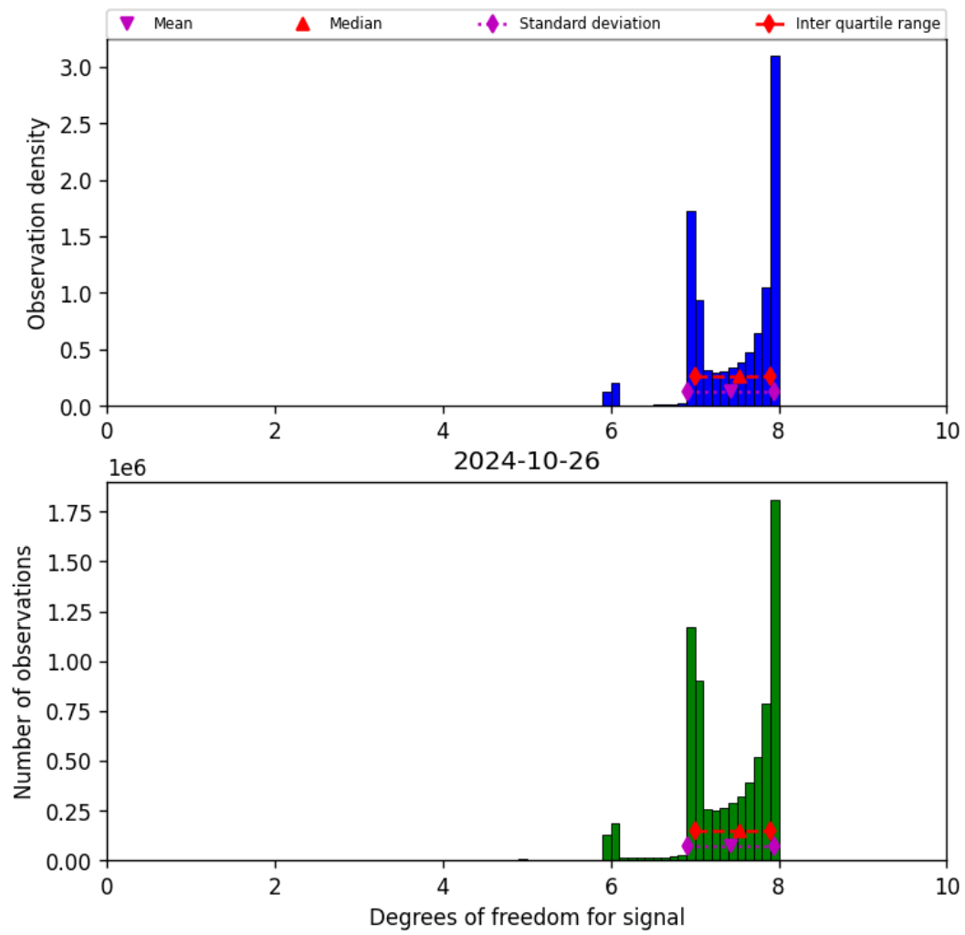
Figure 23: Histogram of “Degrees of freedom for signal” for 2024-10-25 to 2024-10-27
