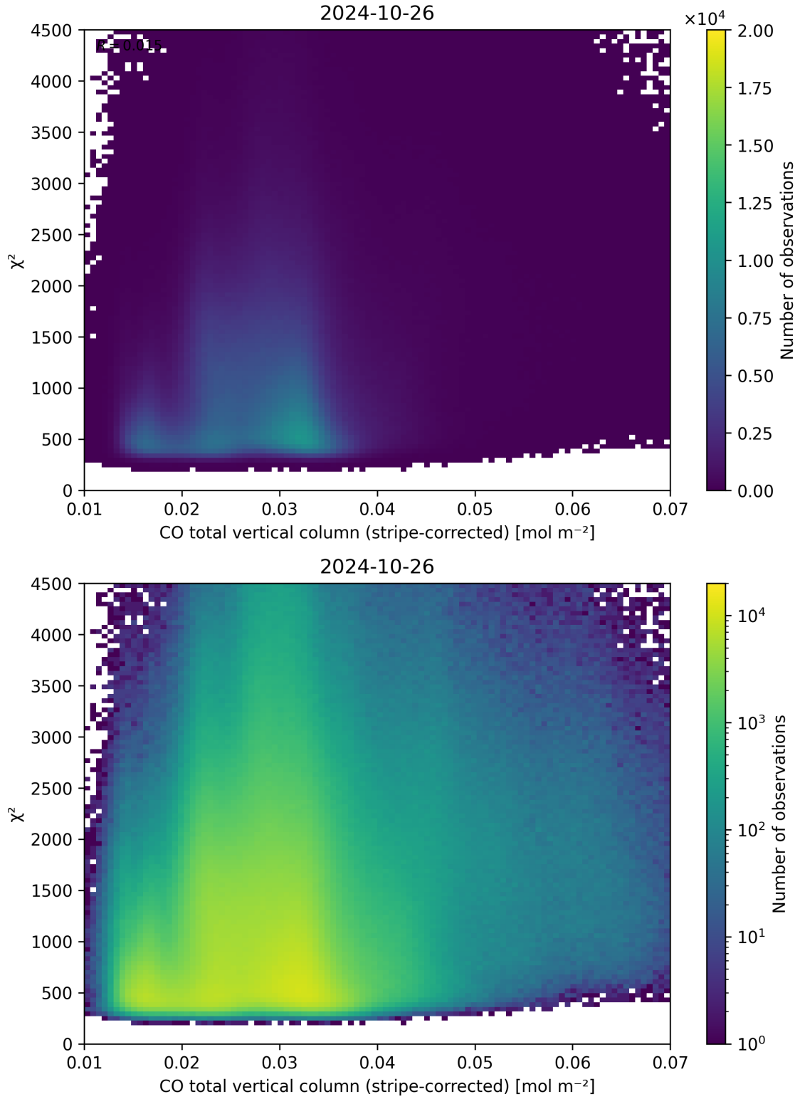
Figure 37: Scatter density plot of “CO total vertical column (stripe-corrected)” against “ \chi^2 ” for 2024-10-25 to 2024-10-27.
