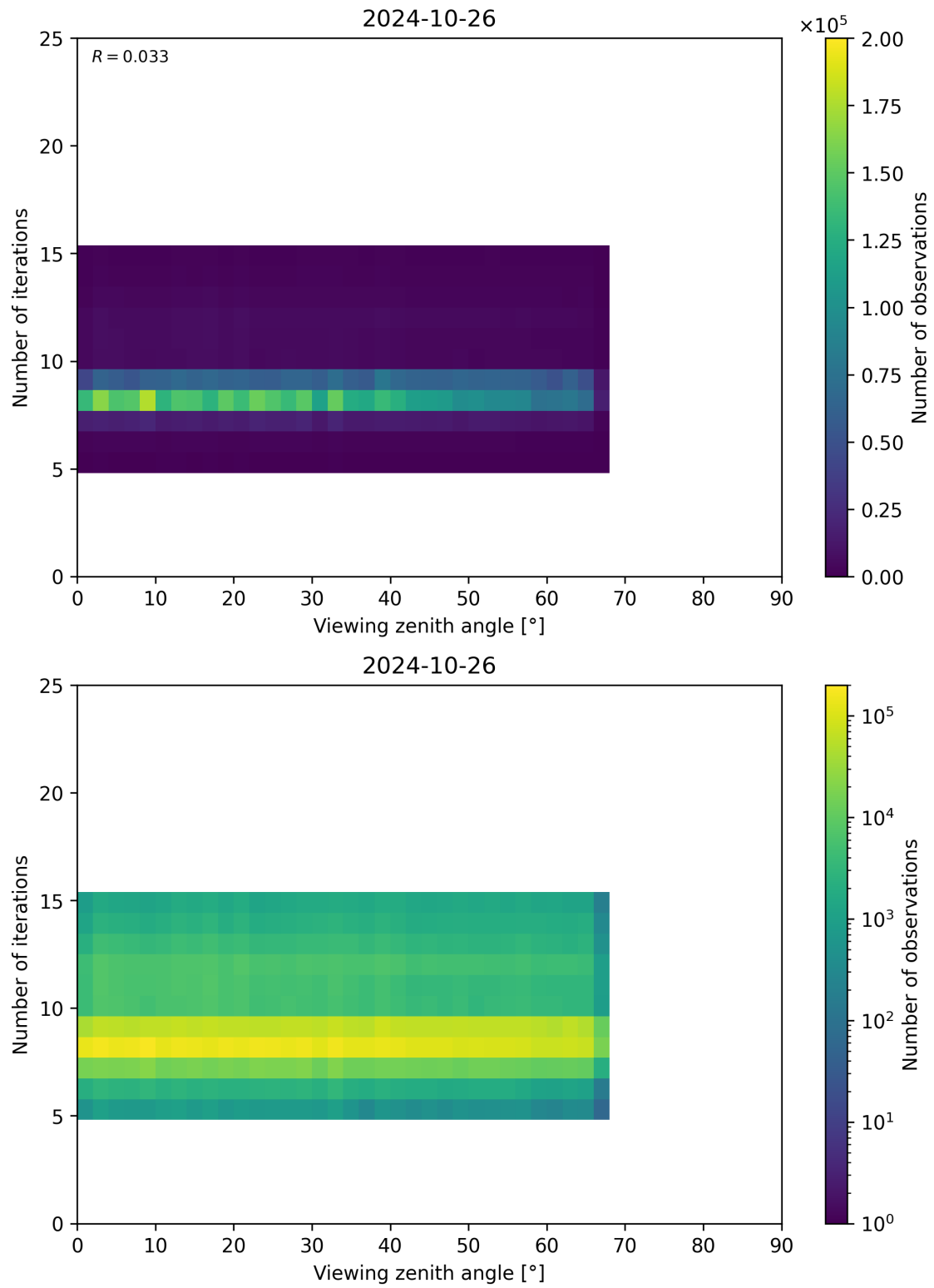
Figure 75: Scatter density plot of “Viewing zenith angle” against “Number of iterations” for 2024-10-25 to 2024-10-27.
