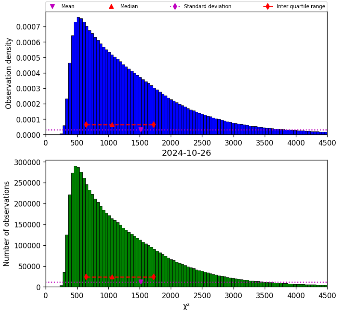
Figure 22: Histogram of “ \chi^2 ” for 2024-10-25 to 2024-10-27
