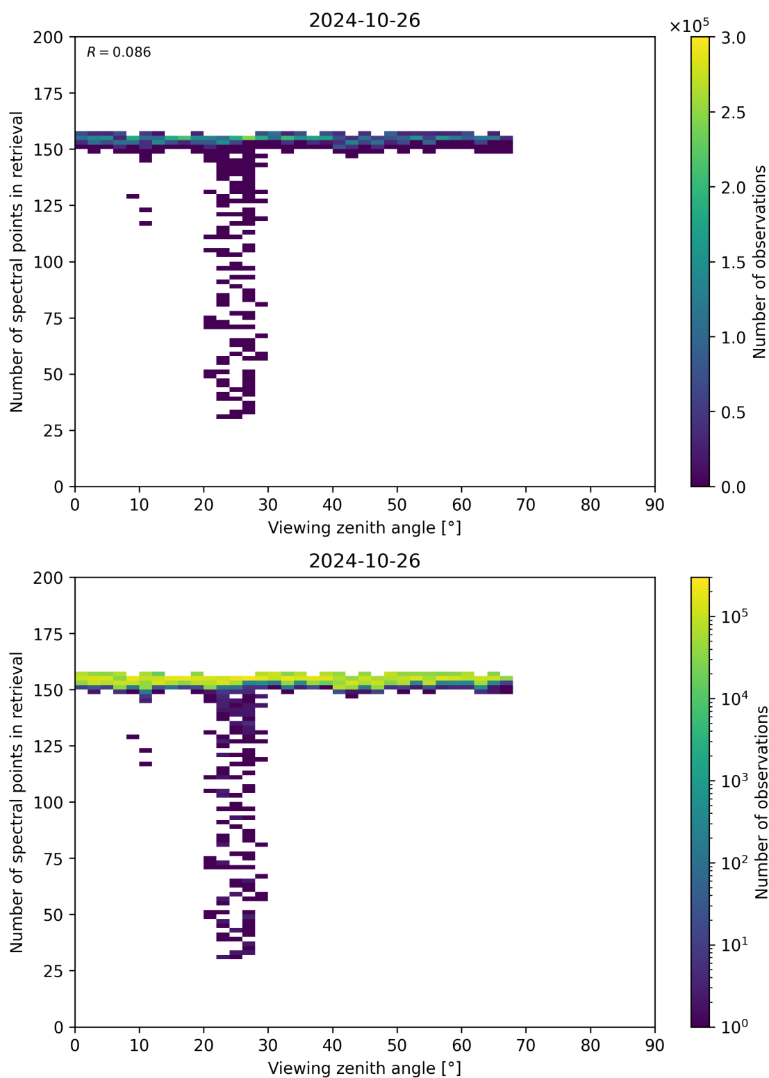
Figure 76: Scatter density plot of “Viewing zenith angle” against “Number of spectral points in retrieval” for 2024-10-25 to 2024-10-27.
