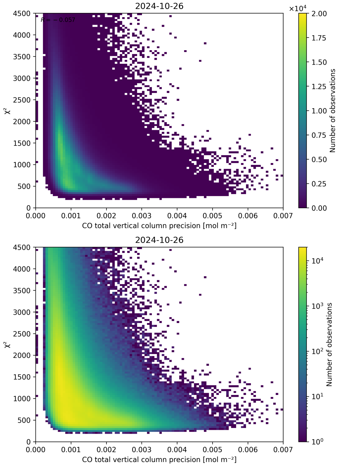
Figure 44: Scatter density plot of “CO total vertical column precision” against “ \chi^2 ” for 2024-10-25 to 2024-10-27.
