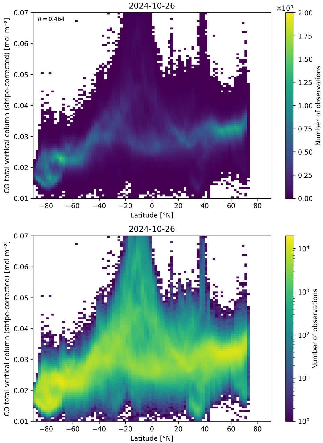
Figure 52: Scatter density plot of “Latitude” against “CO total vertical column (stripe-corrected)” for 2024-10-25 to 2024-10-27.
