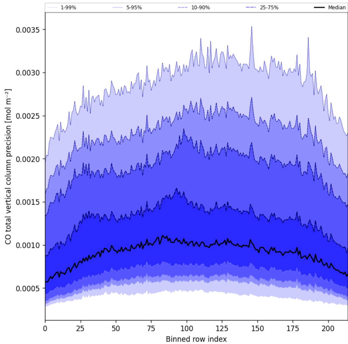
Figure 28: Along track statistics of “CO total vertical column precision” for 2024-10-25 to 2024-10-27
