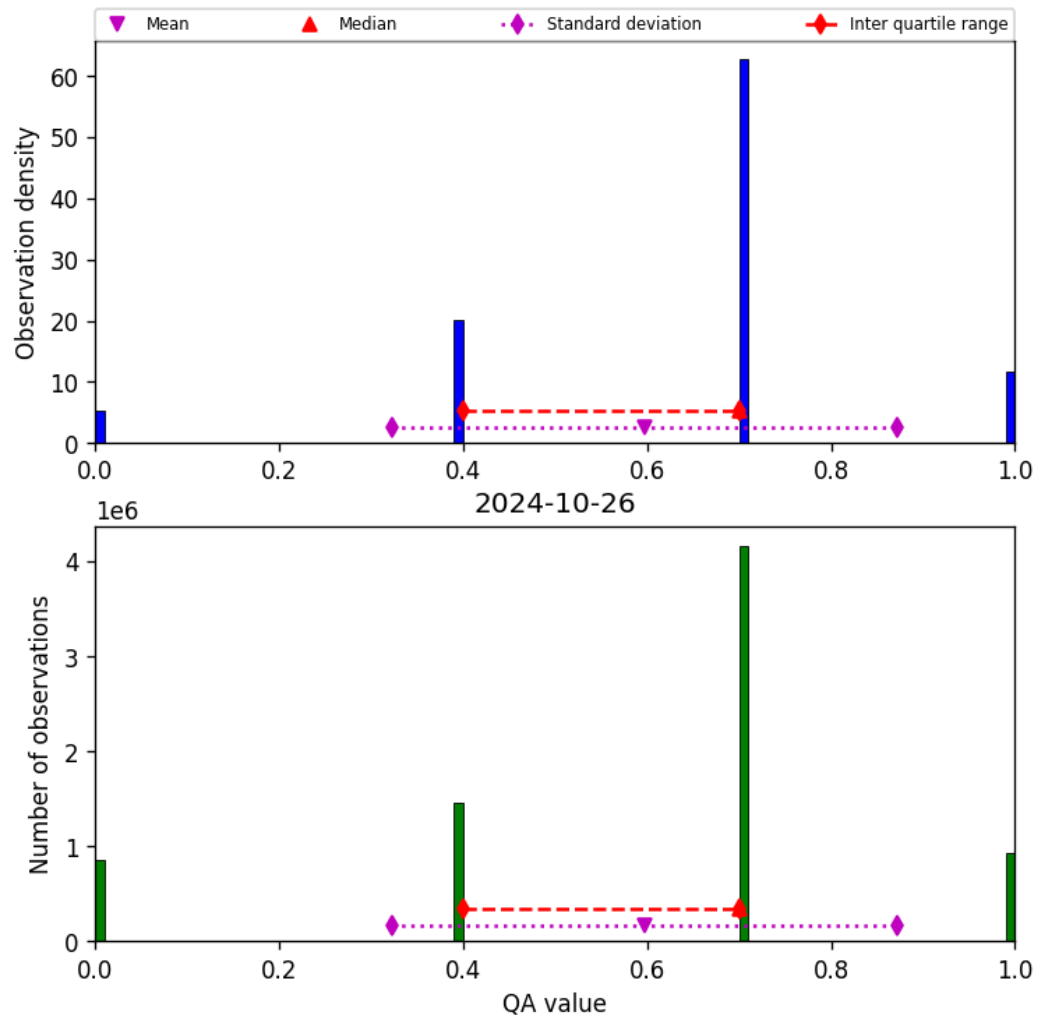
Figure 17: Histogram of “QA value” for 2024-10-25 to 2024-10-27
