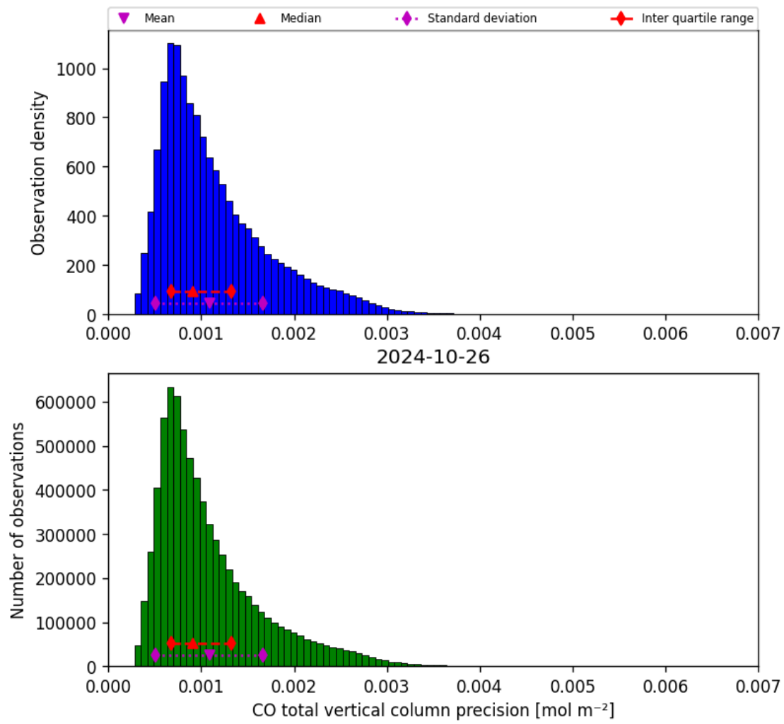
Figure 20: Histogram of “CO total vertical column precision” for 2024-10-25 to 2024-10-27
