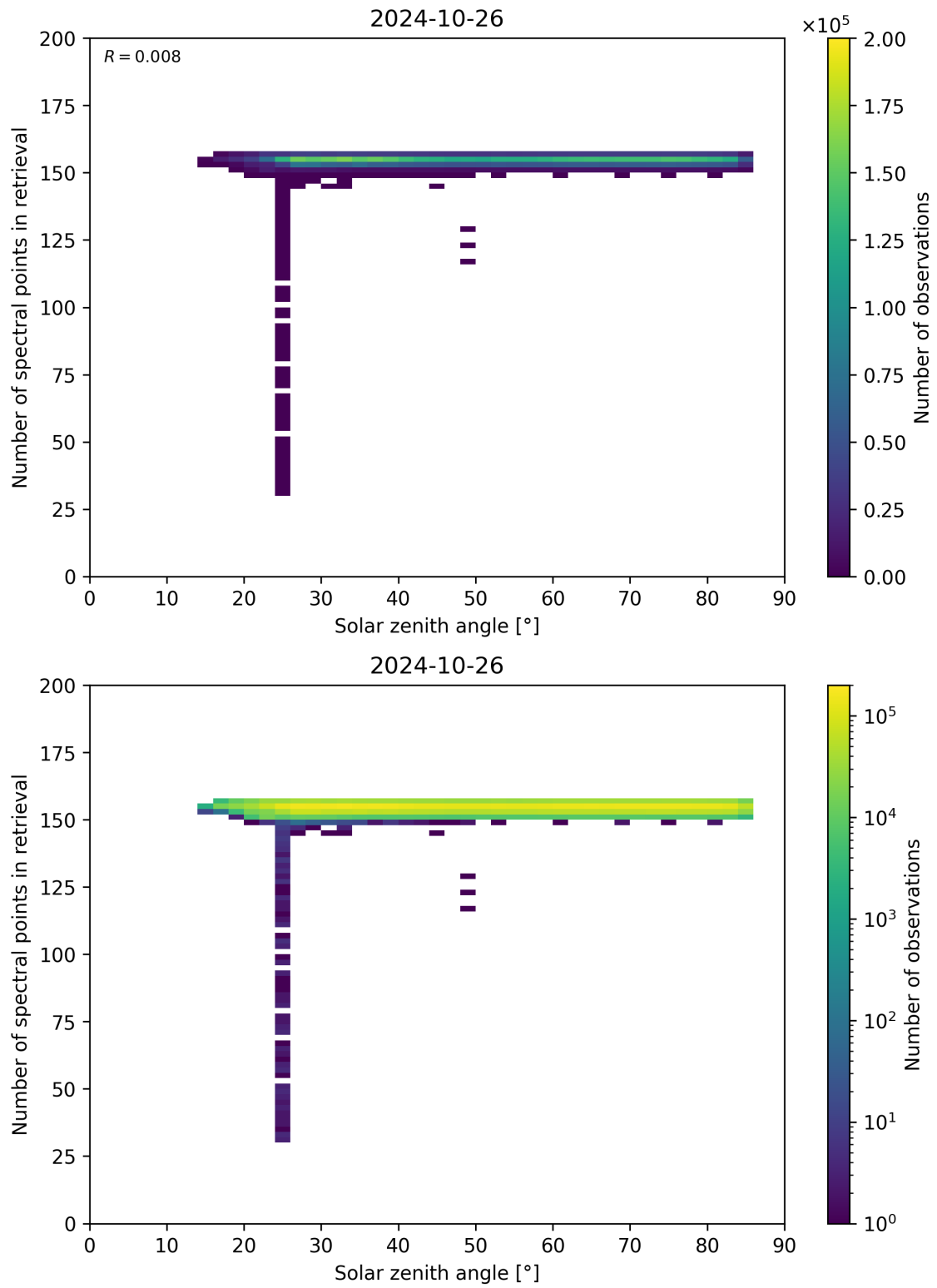
Figure 68: Scatter density plot of “Solar zenith angle” against “Number of spectral points in retrieval” for 2024-10-25 to 2024-10-27.
