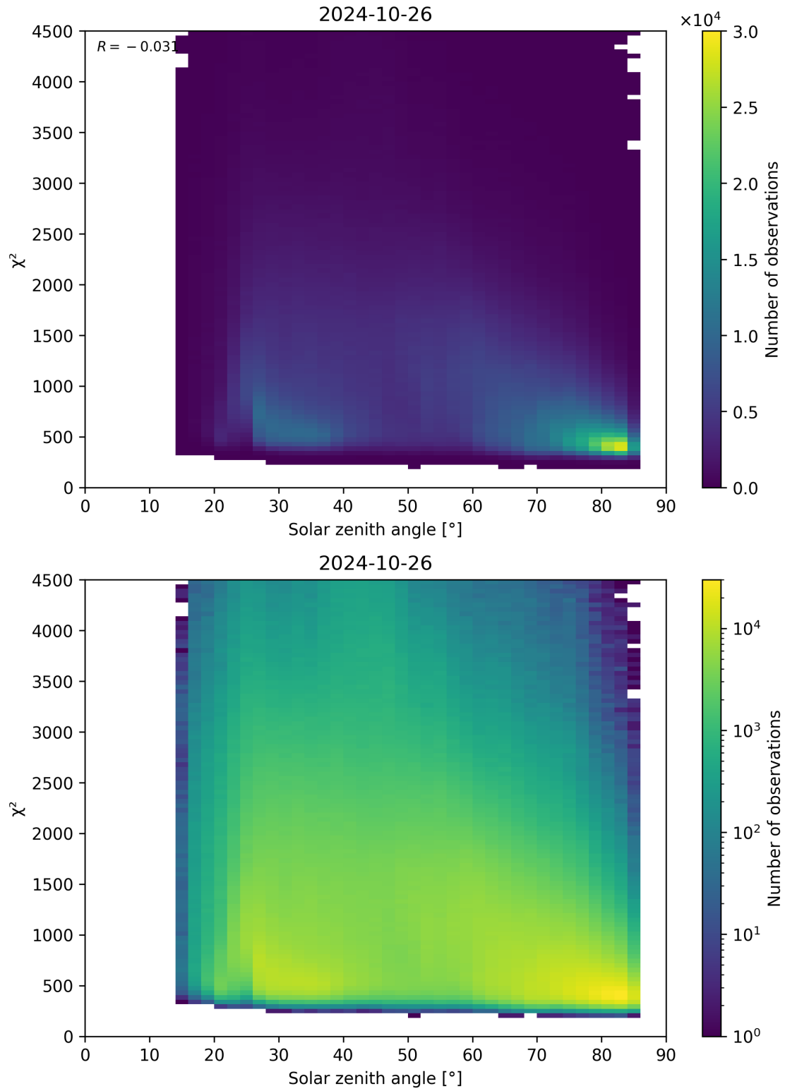
Figure 64: Scatter density plot of “Solar zenith angle” against “ \chi^2 ” for 2024-10-25 to 2024-10-27.
