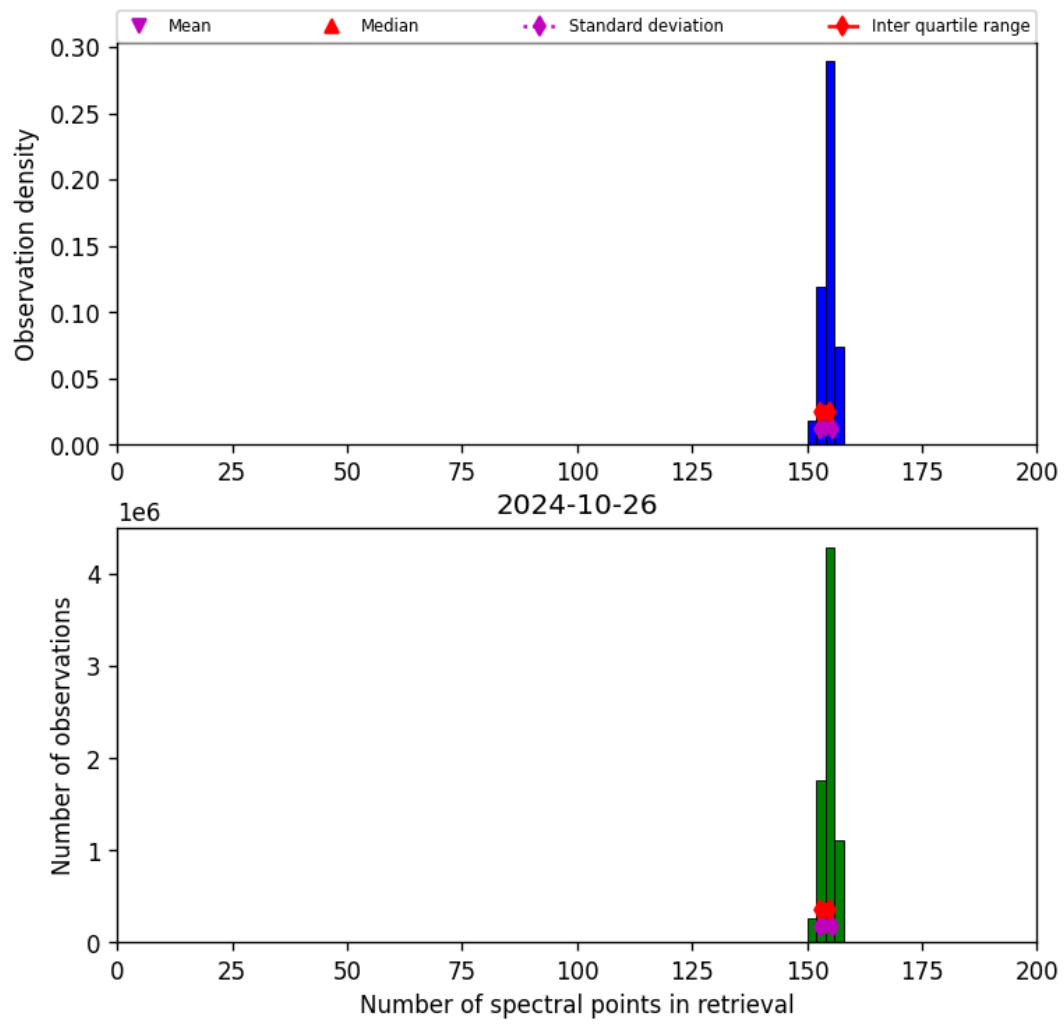
Figure 21: Histogram of “Number of spectral points in retrieval” for 2024-10-25 to 2024-10-27
