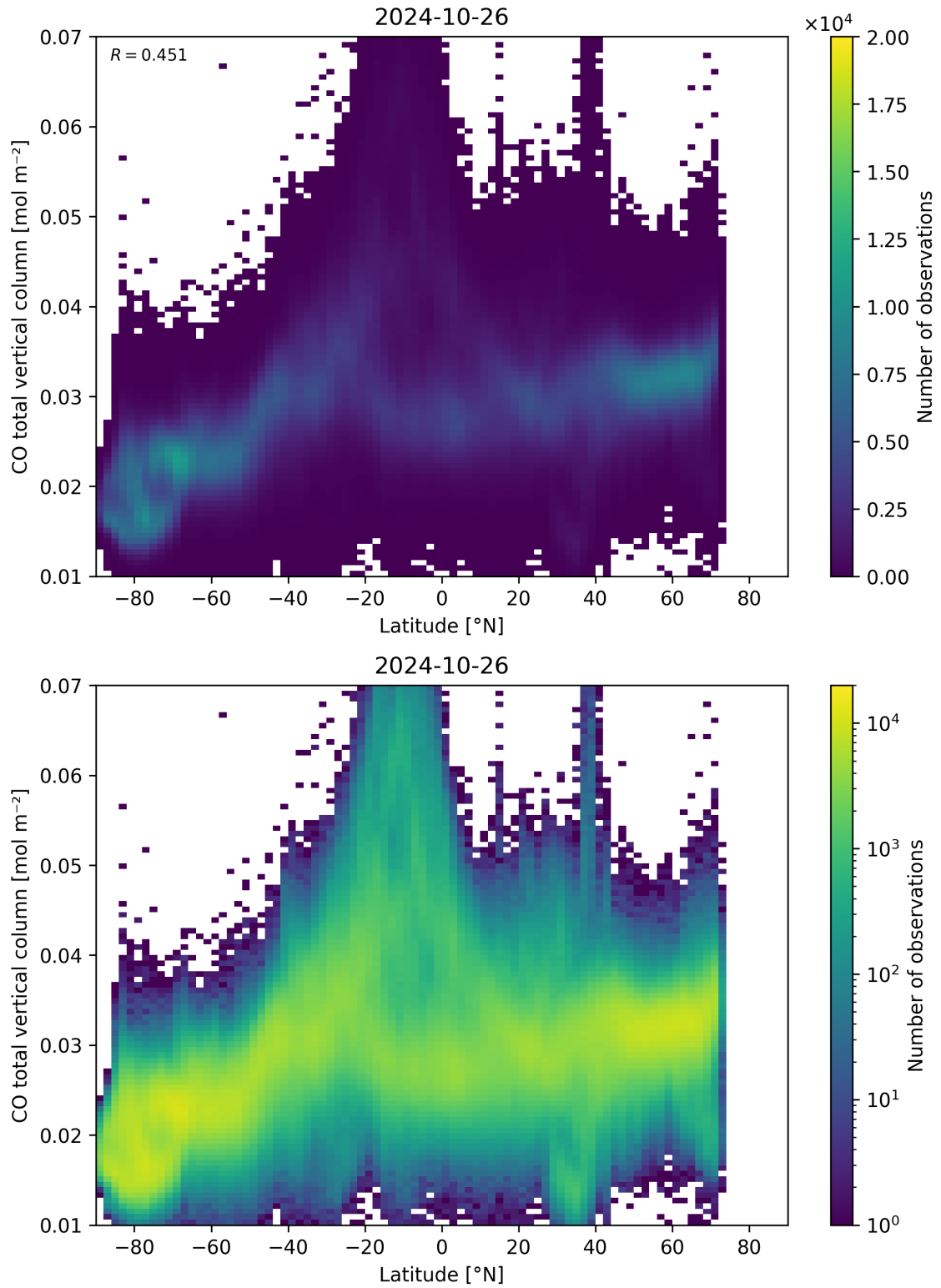
Figure 51: Scatter density plot of “Latitude” against “CO total vertical column” for 2024-10-25 to 2024-10-27.
