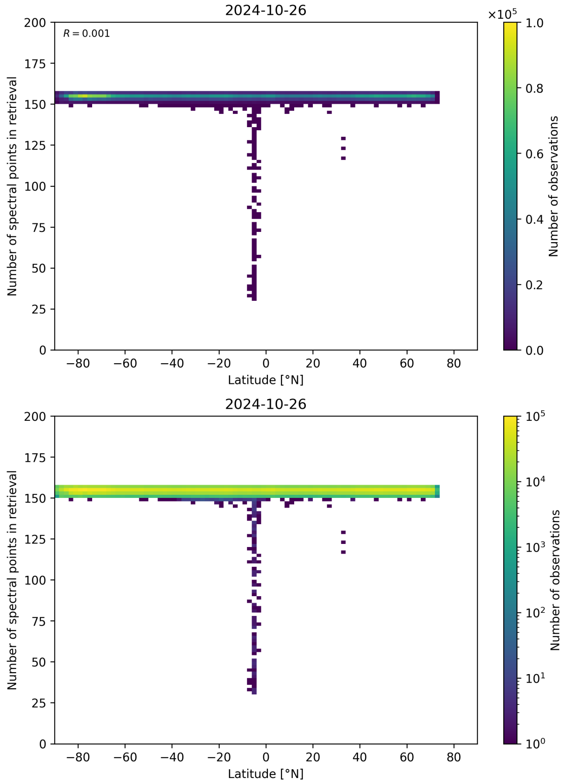
Figure 57: Scatter density plot of “Latitude” against “Number of spectral points in retrieval” for 2024-10-25 to 2024-10-27.
