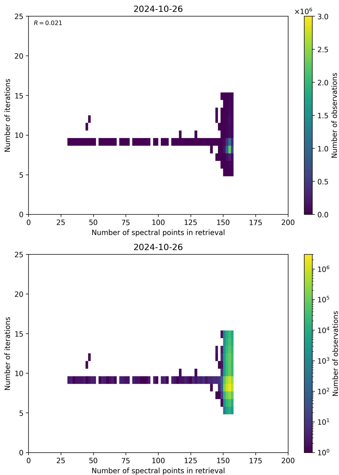
Figure 60: Scatter density plot of “Number of spectral points in retrieval” against “Number of iterations” for 2024-10-25 to 2024-10-27.
