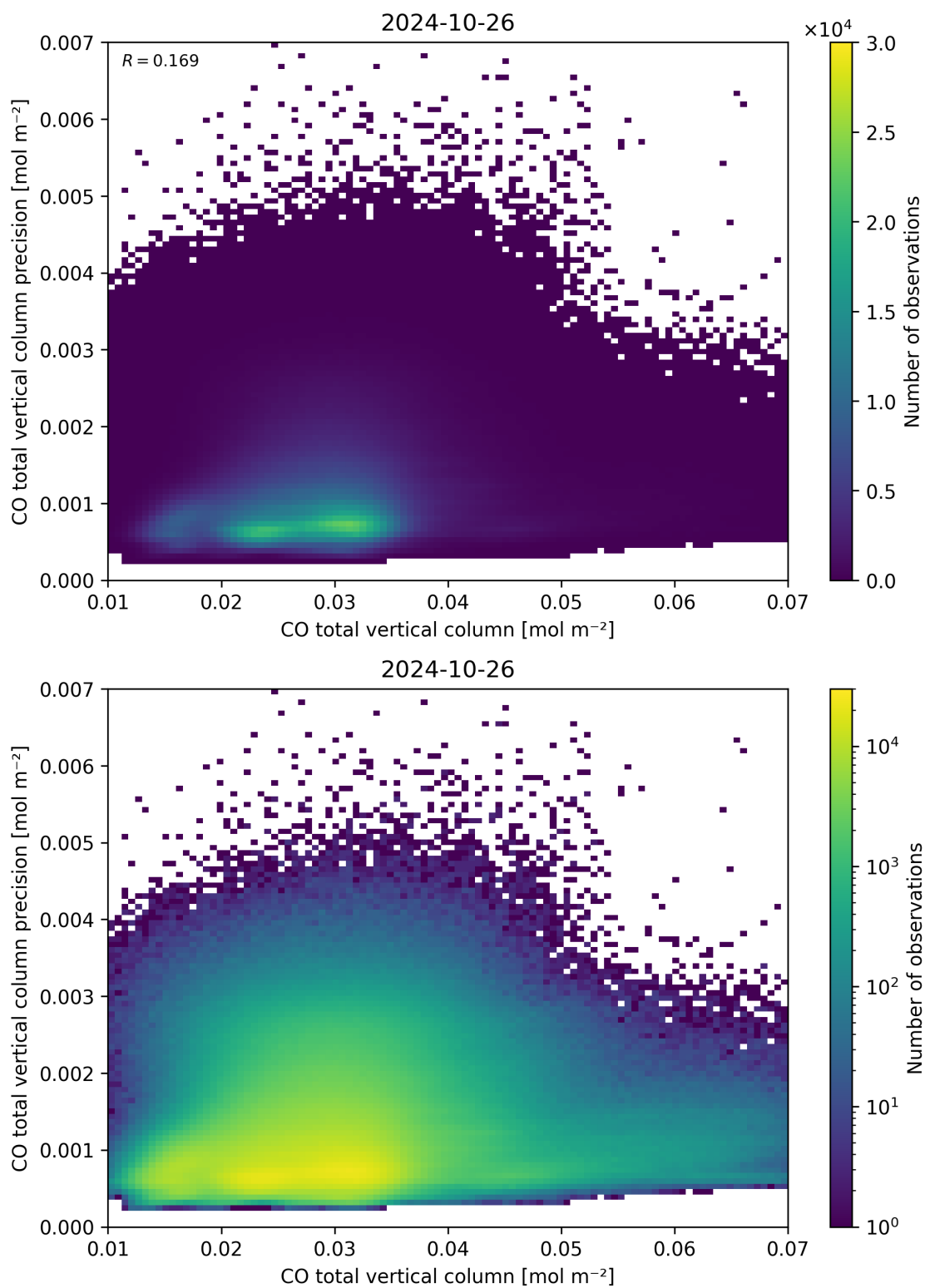
Figure 34: Scatter density plot of “CO total vertical column” against “CO total vertical column precision” for 2024-10-25 to 2024-10-27.
