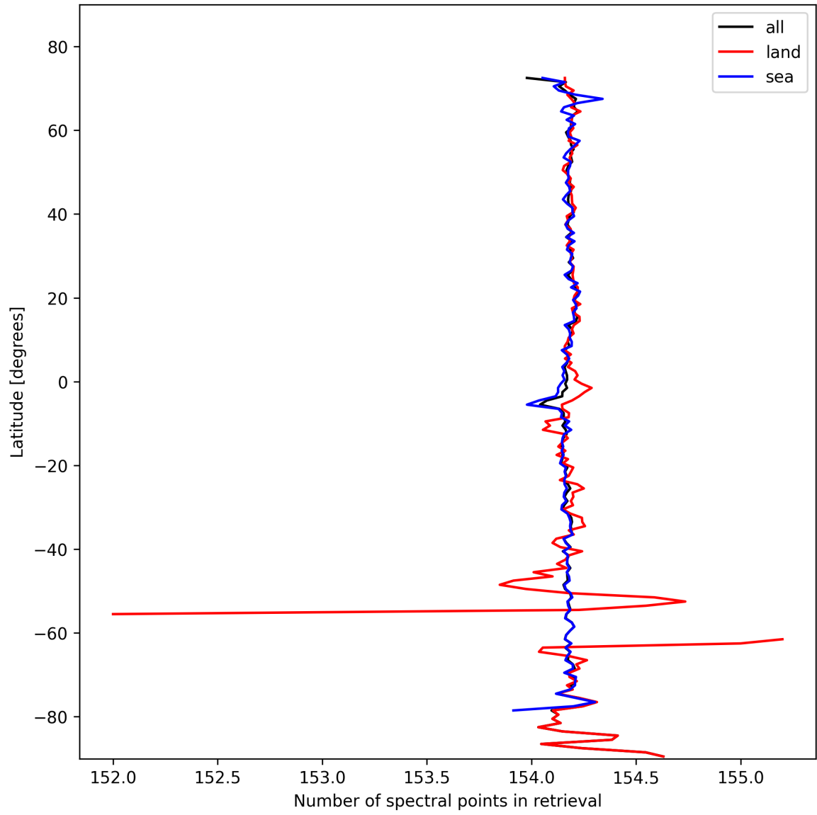
Figure 13: Zonal average of “Number of spectral points in retrieval” for 2024-10-25 to 2024-10-27.
