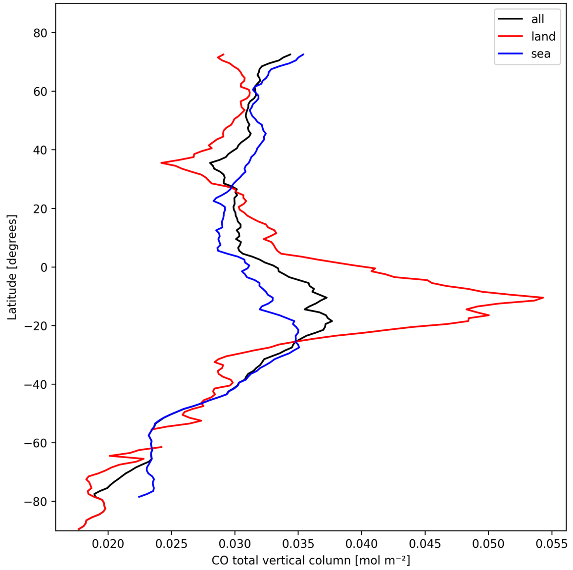
Figure 10: Zonal average of “CO total vertical column” for 2024-10-25 to 2024-10-27.
