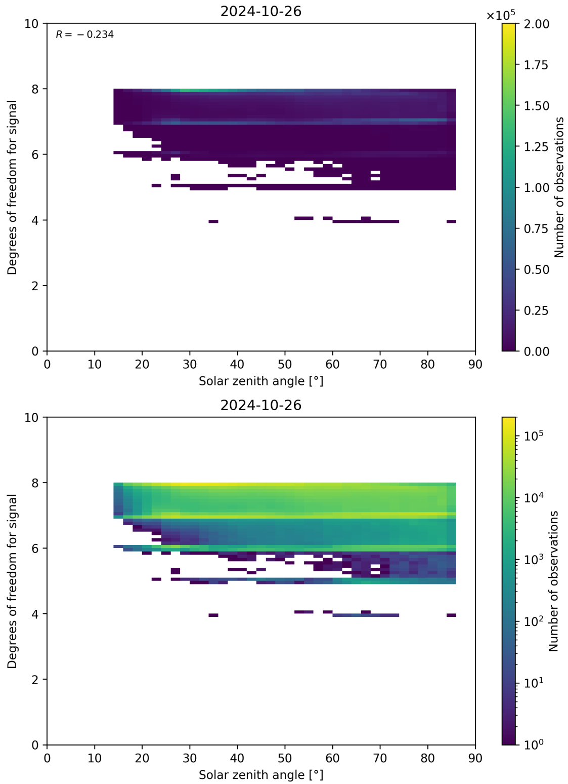
Figure 65: Scatter density plot of “Solar zenith angle” against “Degrees of freedom for signal” for 2024-10-25 to 2024-10-27.
