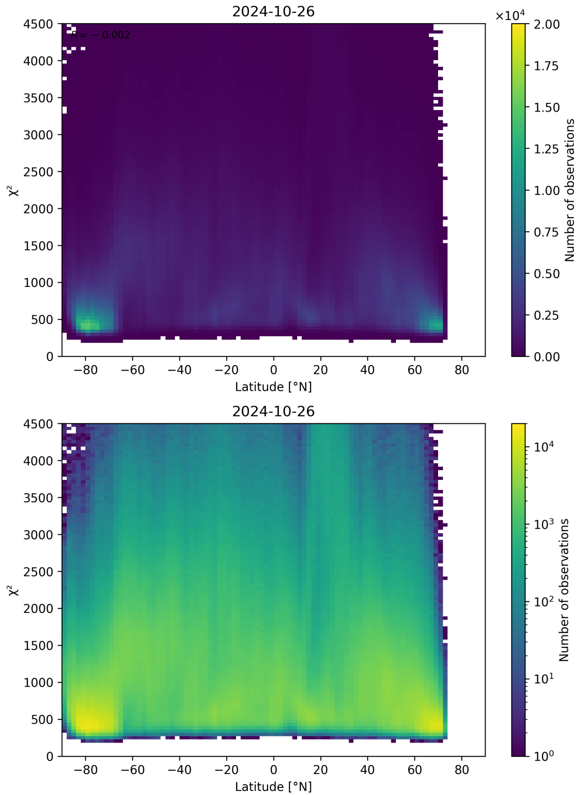
Figure 54: Scatter density plot of “Latitude” against “ \chi^2 ” for 2024-10-25 to 2024-10-27.
