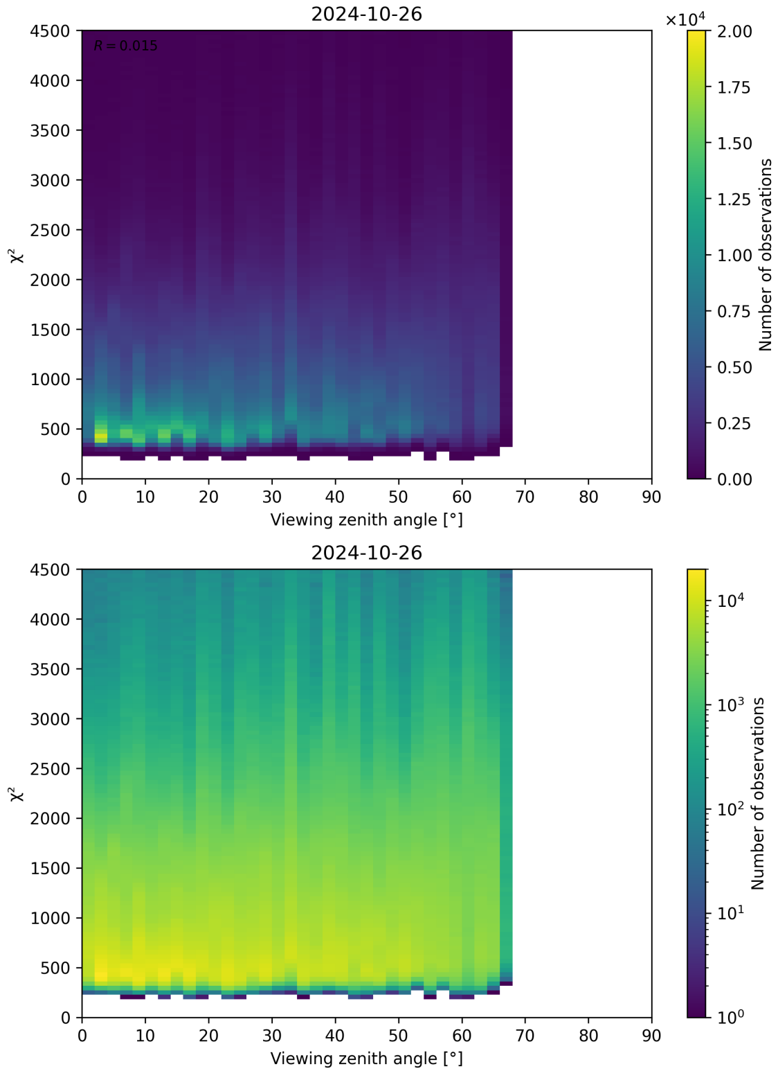
Figure 72: Scatter density plot of “Viewing zenith angle” against “ \chi^2 ” for 2024-10-25 to 2024-10-27.
