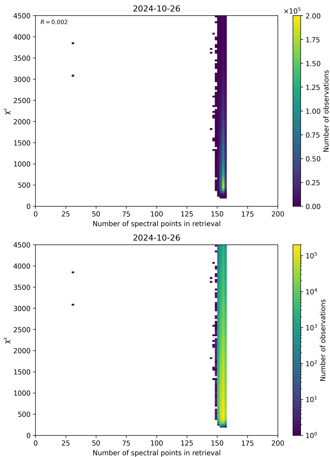
Figure 58: Scatter density plot of “Number of spectral points in retrieval” against “ \chi^2 ” for 2024-10-25 to 2024-10-27.
