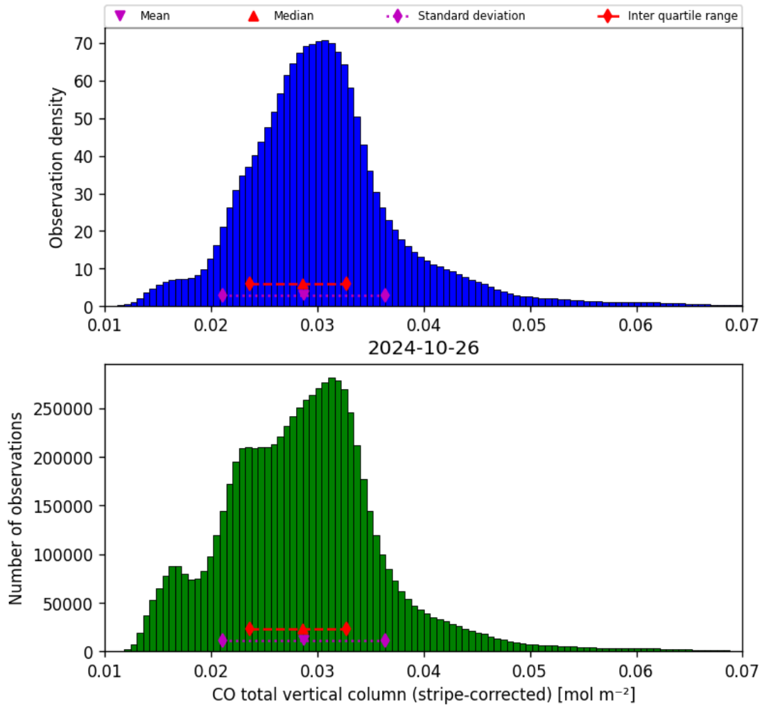
Figure 19: Histogram of “CO total vertical column (stripe-corrected)” for 2024-10-25 to 2024-10-27
