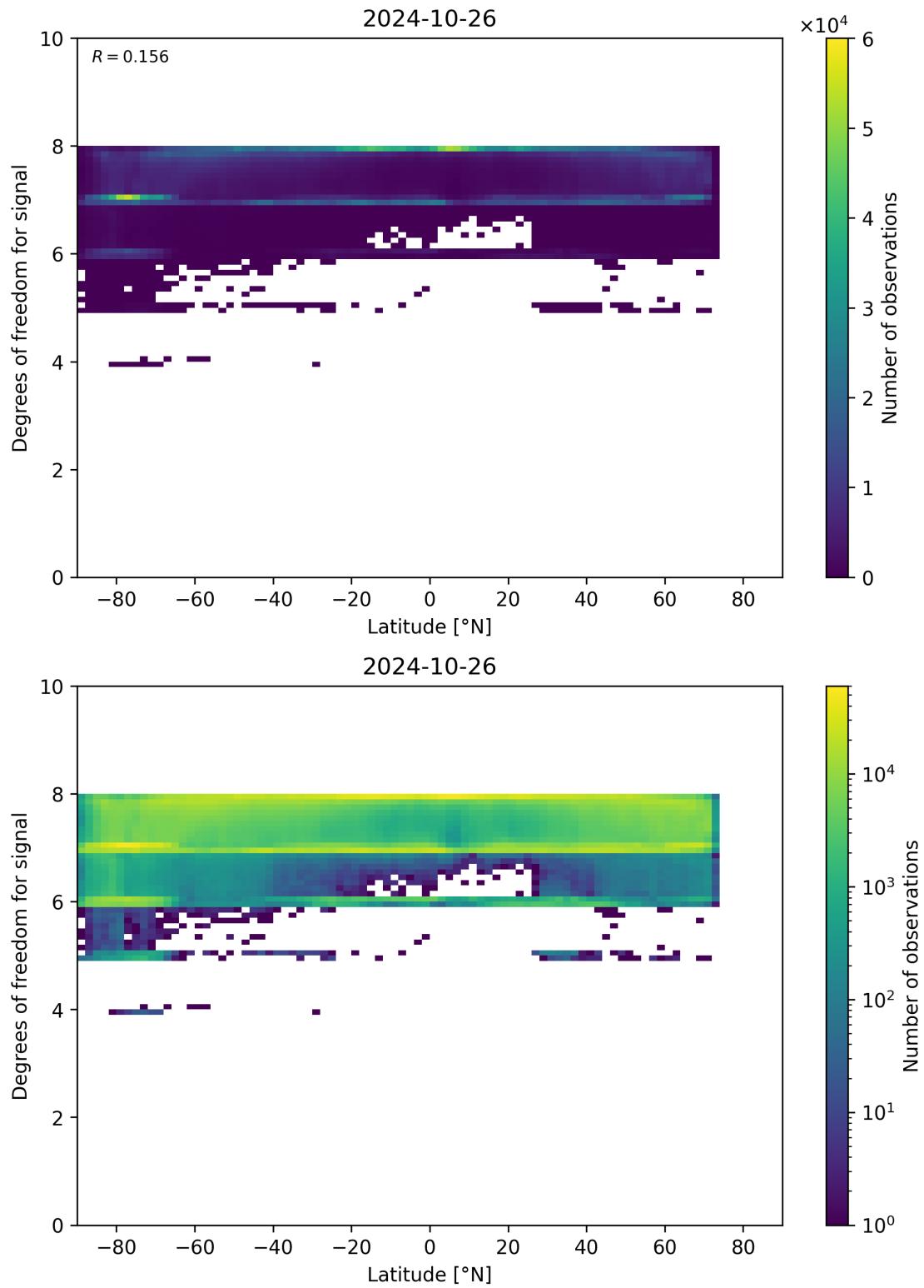
Figure 55: Scatter density plot of “Latitude” against “Degrees of freedom for signal” for 2024-10-25 to 2024-10-27.
