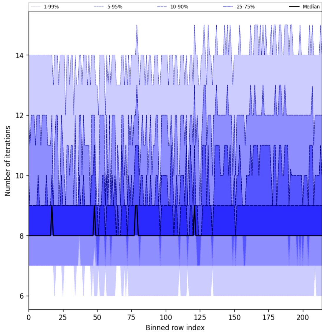
Figure 32: Along track statistics of “Number of iterations” for 2024-10-25 to 2024-10-27
