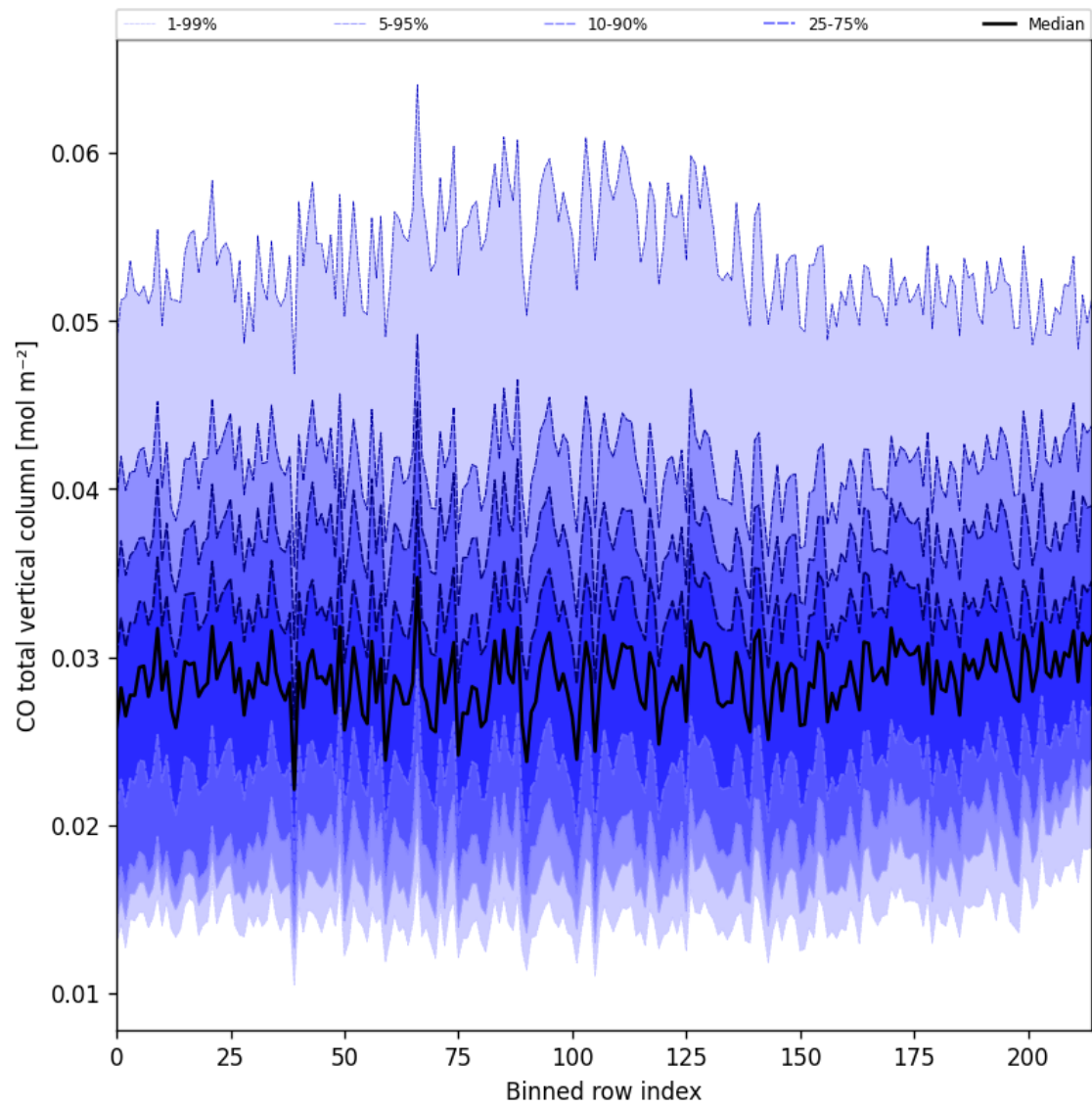
Figure 26: Along track statistics of “CO total vertical column” for 2024-10-25 to 2024-10-27
