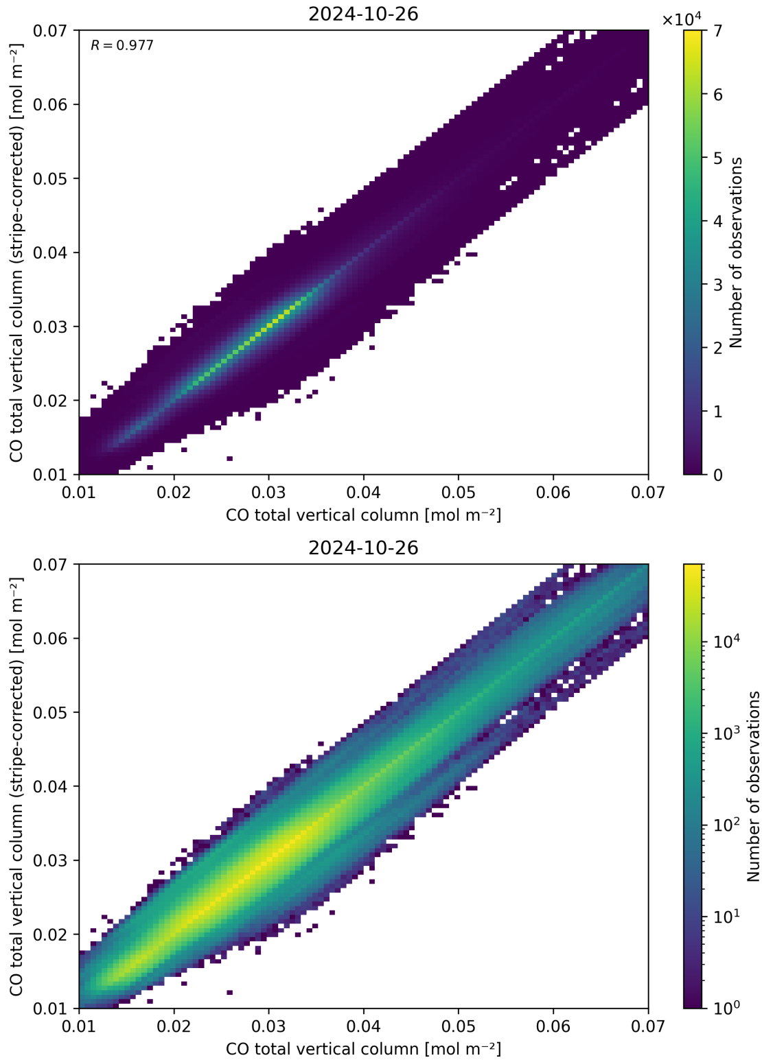
Figure 33: Scatter density plot of “CO total vertical column” against “CO total vertical column (stripe-corrected)” for 2024-10-25 to 2024-10-27.
