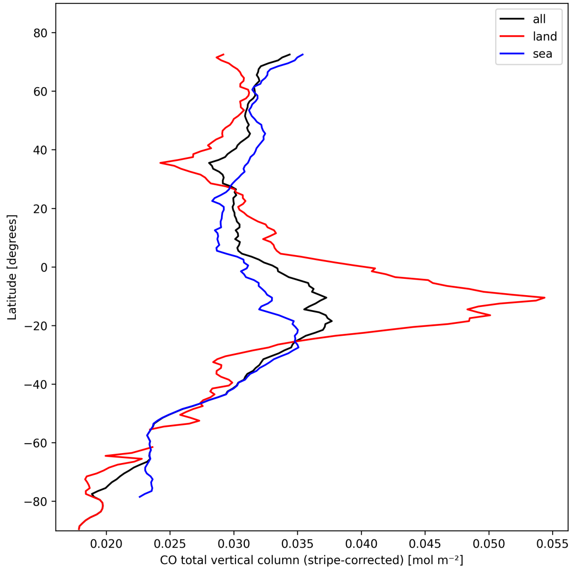
Figure 11: Zonal average of “CO total vertical column (stripe-corrected)” for 2024-10-25 to 2024-10-27.
