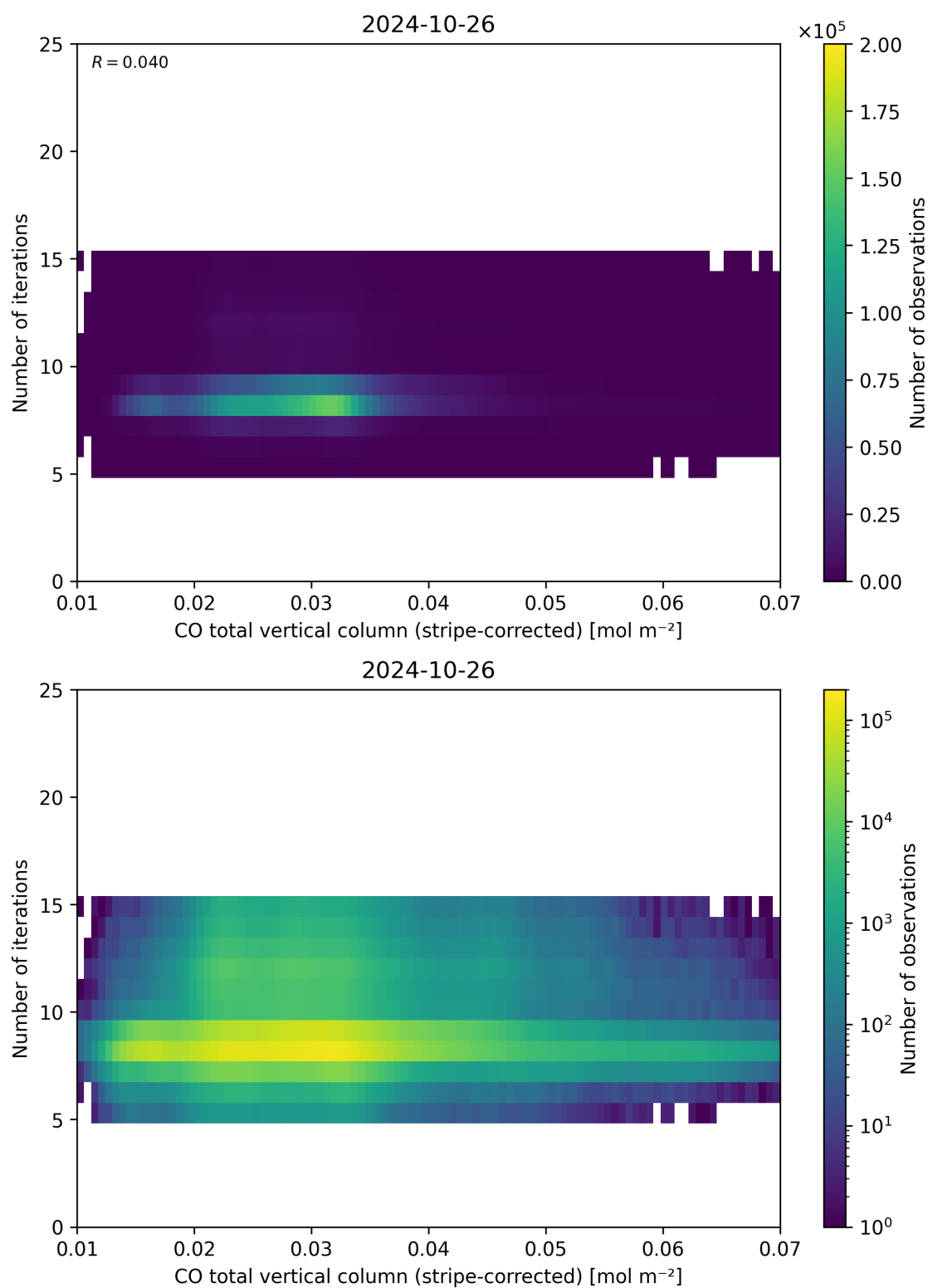
Figure 39: Scatter density plot of “CO total vertical column (stripe-corrected)” against “Number of iterations” for 2024-10-25 to 2024-10-27.
