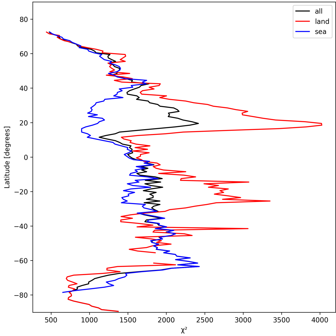
Figure 14: Zonal average of “ \chi^2 ” for 2024-10-25 to 2024-10-27.
