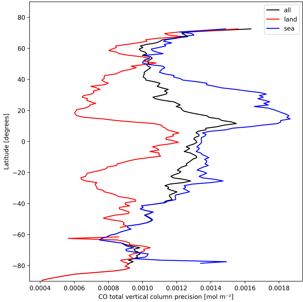
Figure 12: Zonal average of “CO total vertical column precision” for 2024-10-25 to 2024-10-27.
