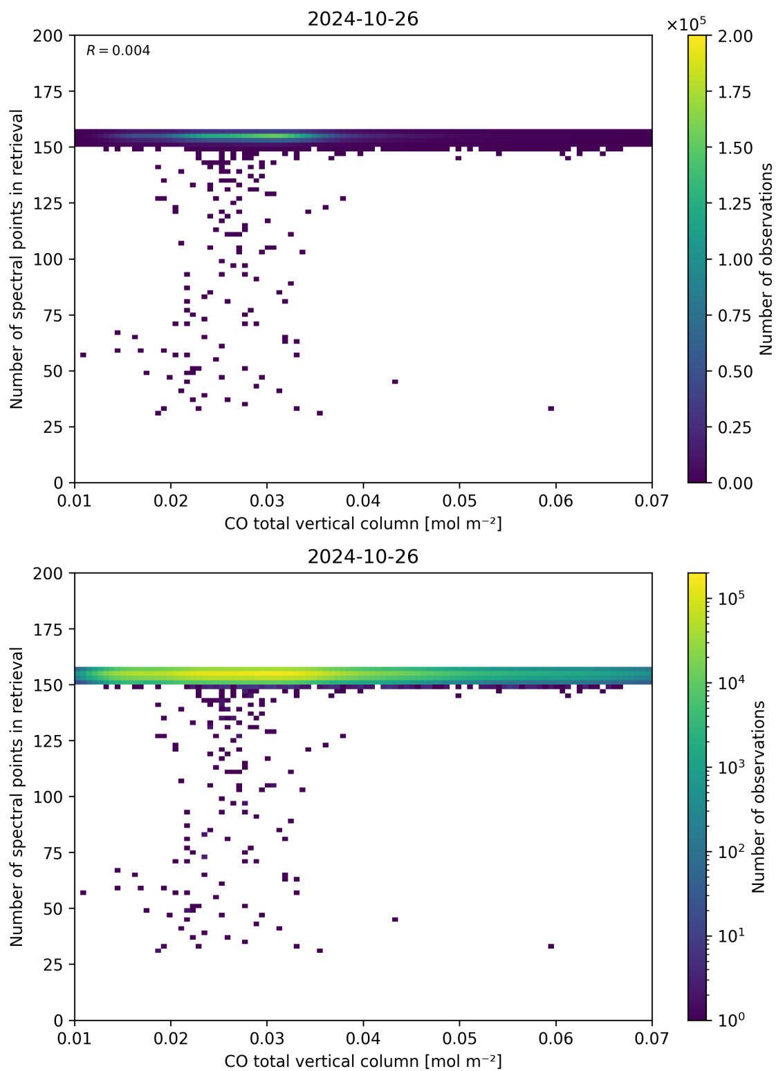
Figure 43: Scatter density plot of “CO total vertical column” against “Number of spectral points in retrieval” for 2024-10-25 to 2024-10-27.
