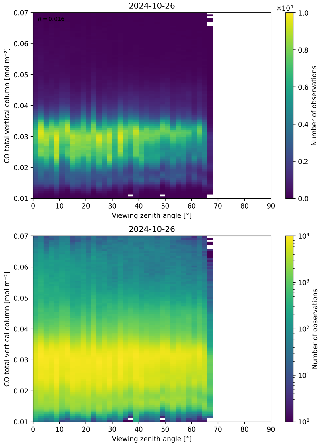
Figure 69: Scatter density plot of “Viewing zenith angle” against “CO total vertical column” for 2024-10-25 to 2024-10-27.
