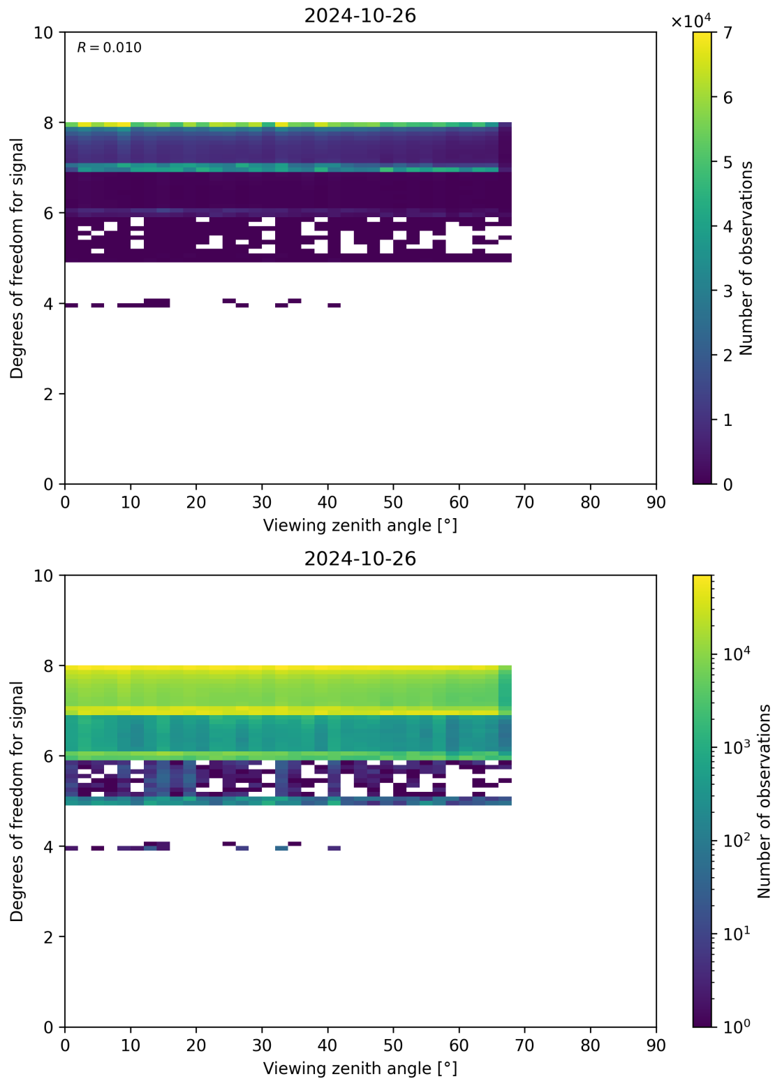
Figure 73: Scatter density plot of “Viewing zenith angle” against “Degrees of freedom for signal” for 2024-10-25 to 2024-10-27.
