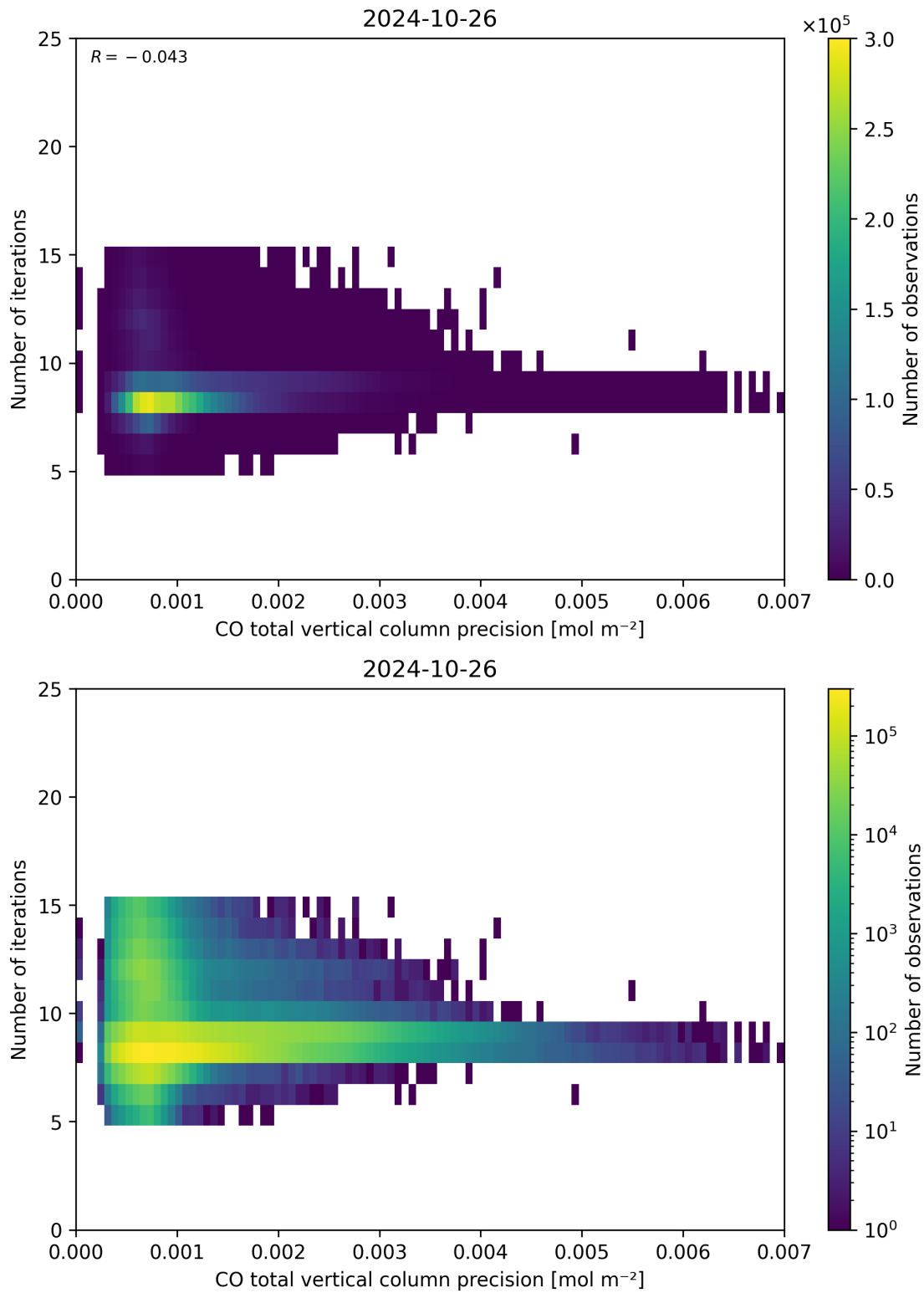
Figure 46: Scatter density plot of “CO total vertical column precision” against “Number of iterations” for 2024-10-25 to 2024-10-27.
