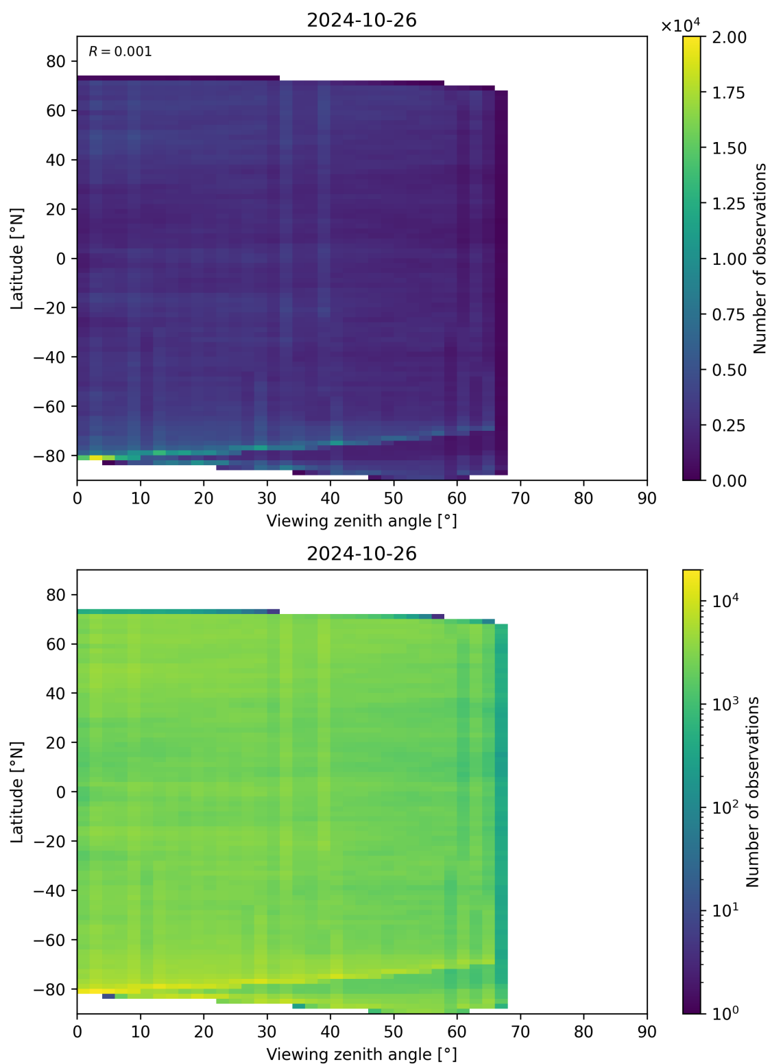
Figure 74: Scatter density plot of “Viewing zenith angle” against “Latitude” for 2024-10-25 to 2024-10-27.
