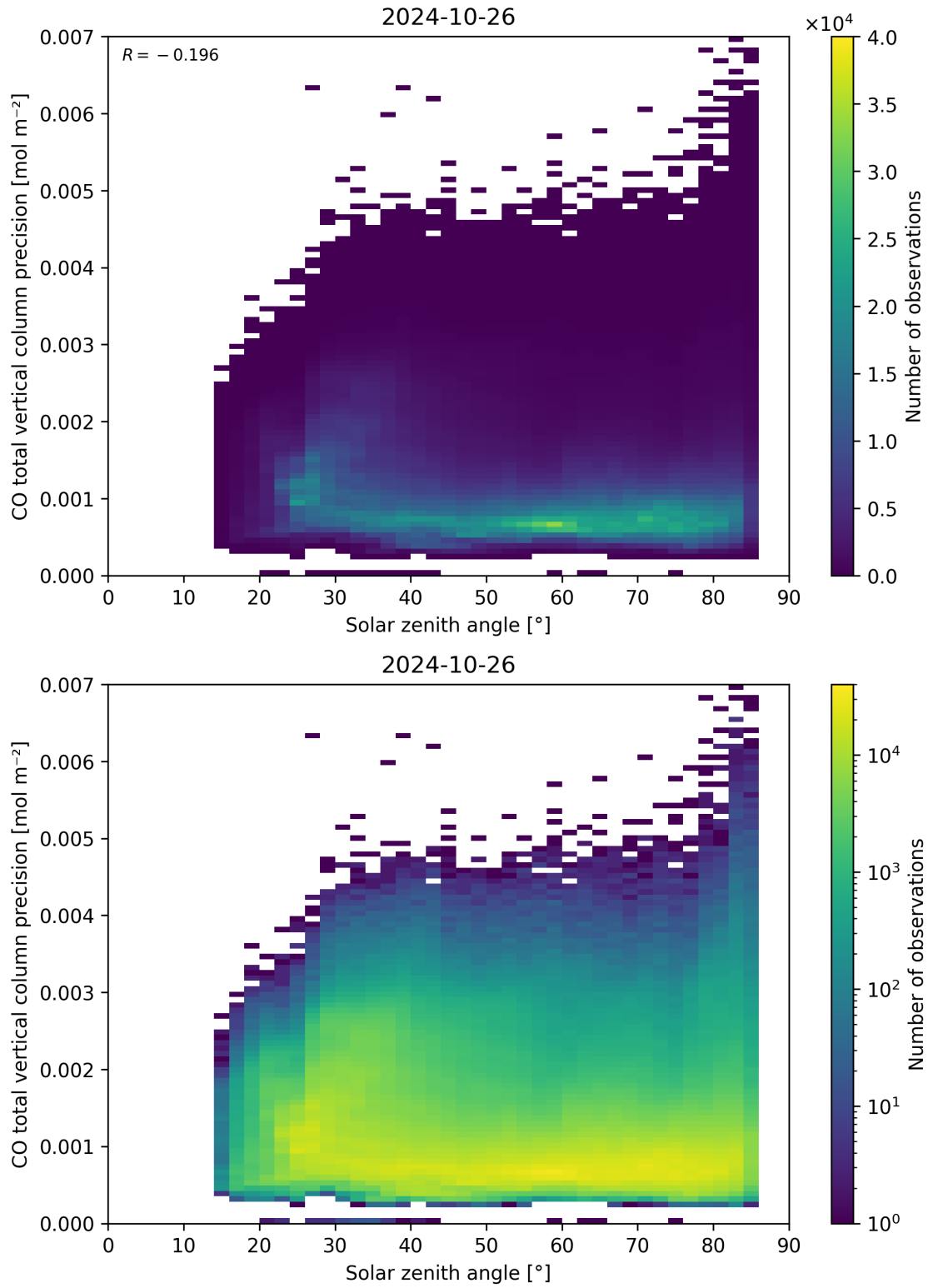
Figure 63: Scatter density plot of “Solar zenith angle” against “CO total vertical column precision” for 2024-10-25 to 2024-10-27.
