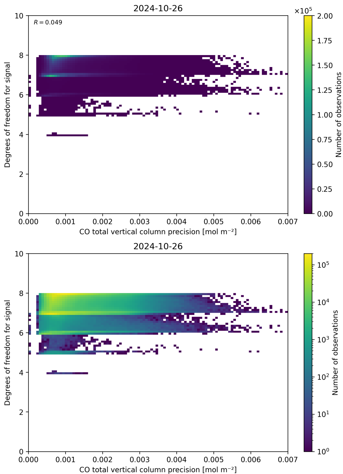
Figure 45: Scatter density plot of “CO total vertical column precision” against “Degrees of freedom for signal” for 2024-10-25 to 2024-10-27.
