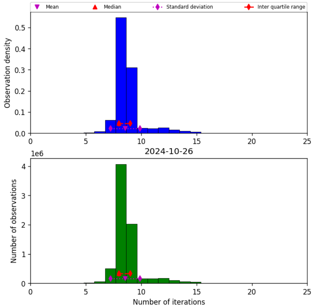
Figure 24: Histogram of “Number of iterations” for 2024-10-25 to 2024-10-27
