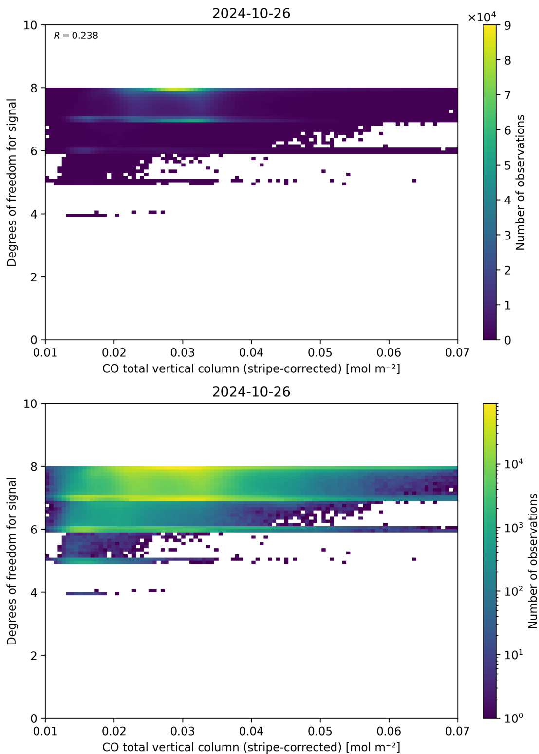
Figure 38: Scatter density plot of “CO total vertical column (stripe-corrected)” against “Degrees of freedom for signal” for 2024-10-25 to 2024-10-27.
