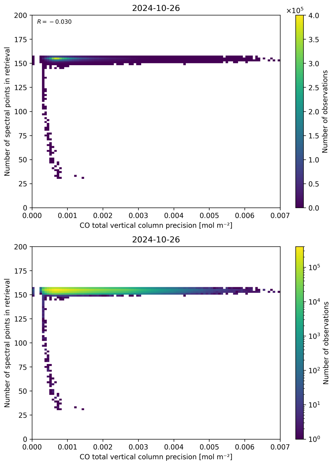
Figure 47: Scatter density plot of “CO total vertical column precision” against “Number of spectral points in retrieval” for 2024-10-25 to 2024-10-27.
