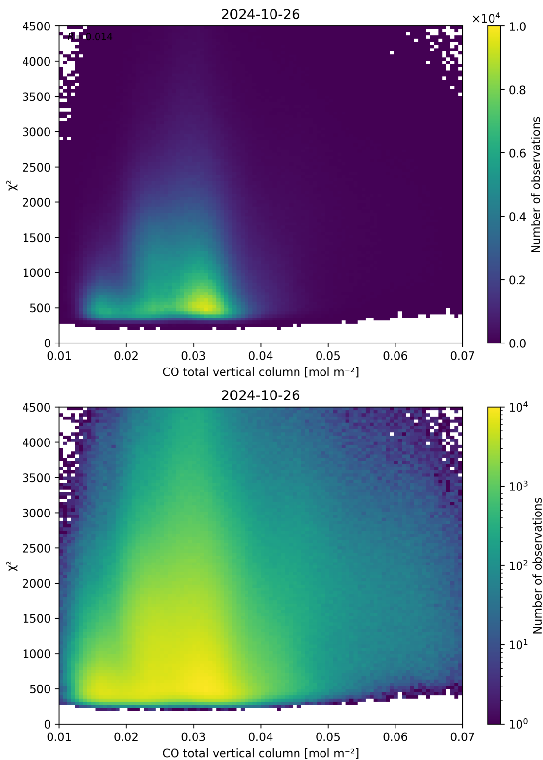
Figure 35: Scatter density plot of “CO total vertical column” against “ \chi^2 ” for 2024-10-25 to 2024-10-27.
