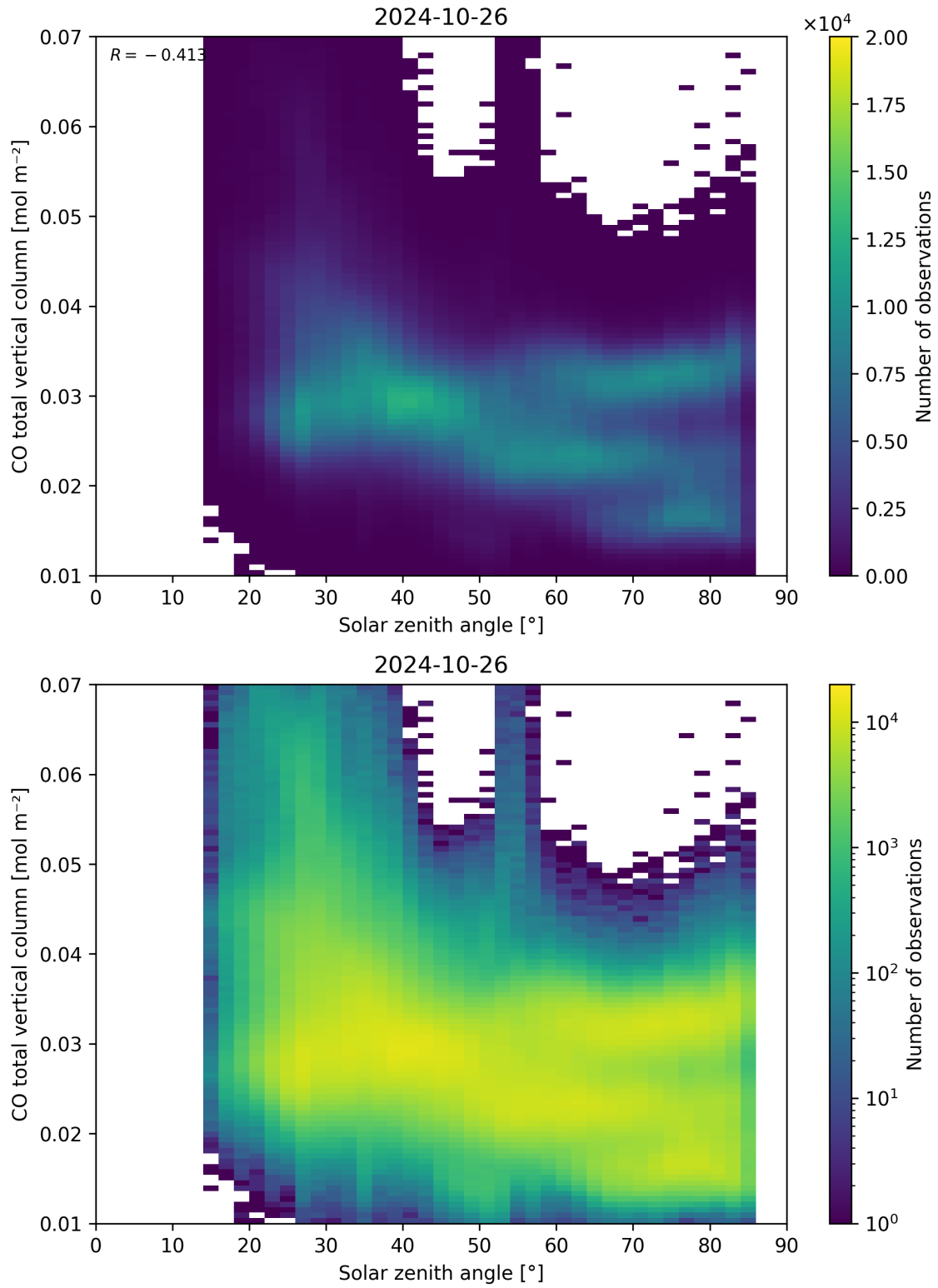
Figure 61: Scatter density plot of “Solar zenith angle” against “CO total vertical column” for 2024-10-25 to 2024-10-27.
