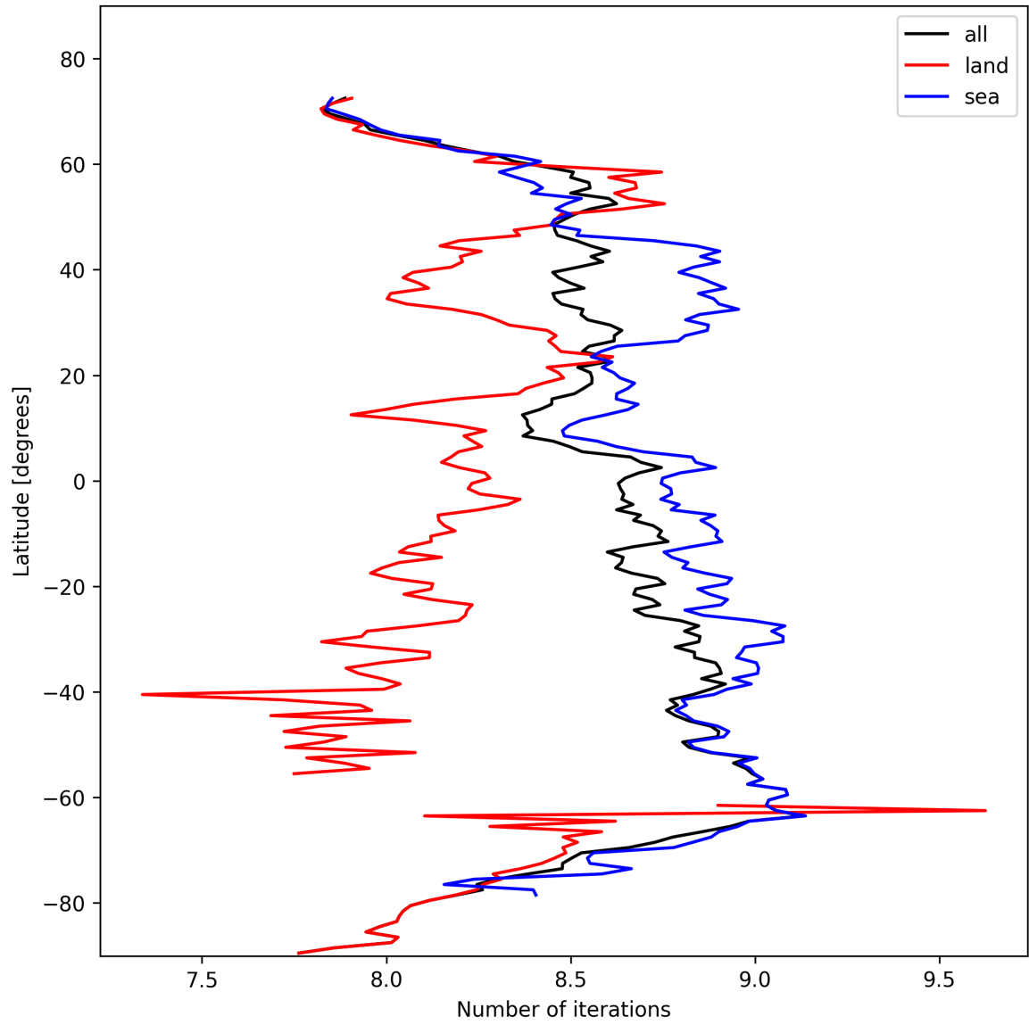
Figure 16: Zonal average of “Number of iterations” for 2024-10-25 to 2024-10-27.
