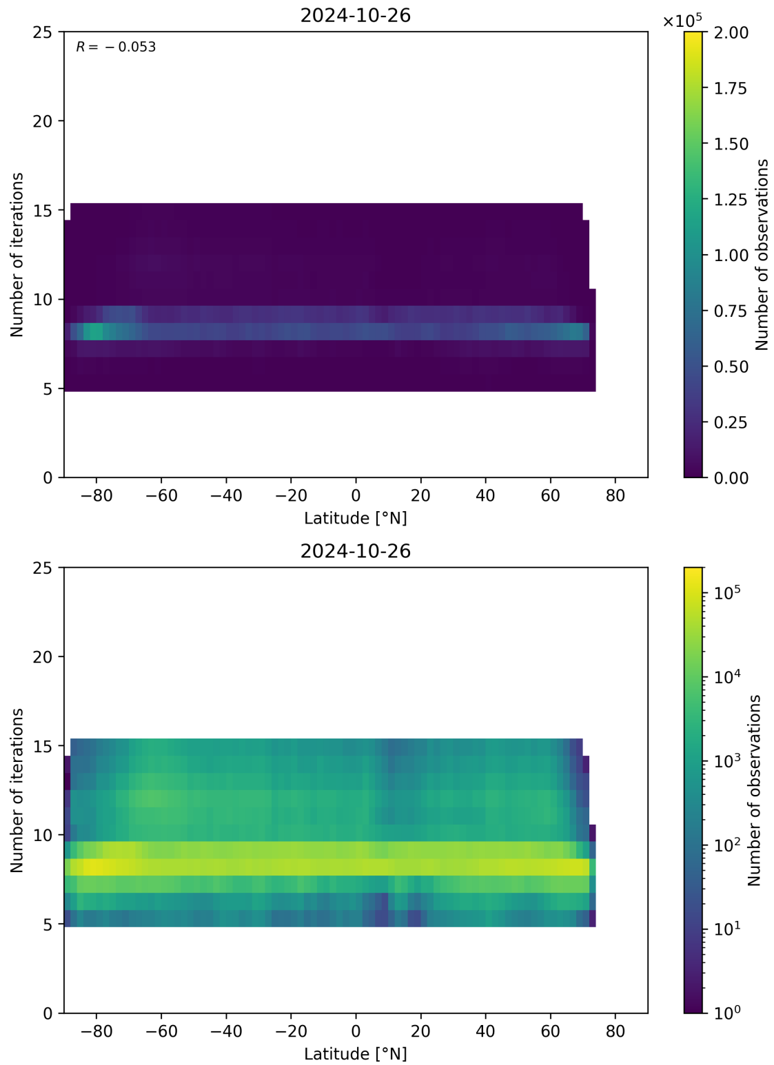
Figure 56: Scatter density plot of “Latitude” against “Number of iterations” for 2024-10-25 to 2024-10-27.
