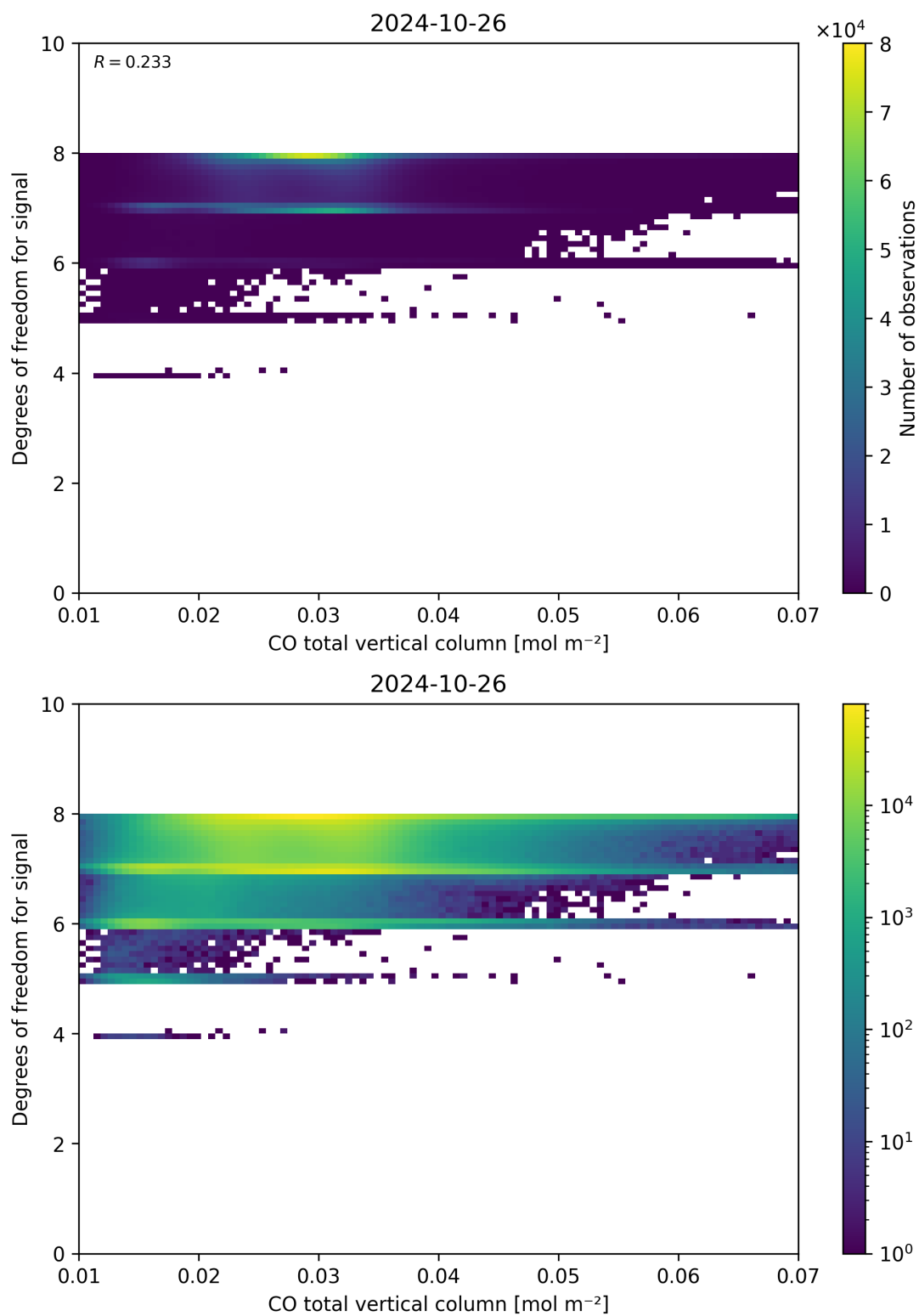
Figure 41: Scatter density plot of “CO total vertical column” against “Degrees of freedom for signal” for 2024-10-25 to 2024-10-27.
