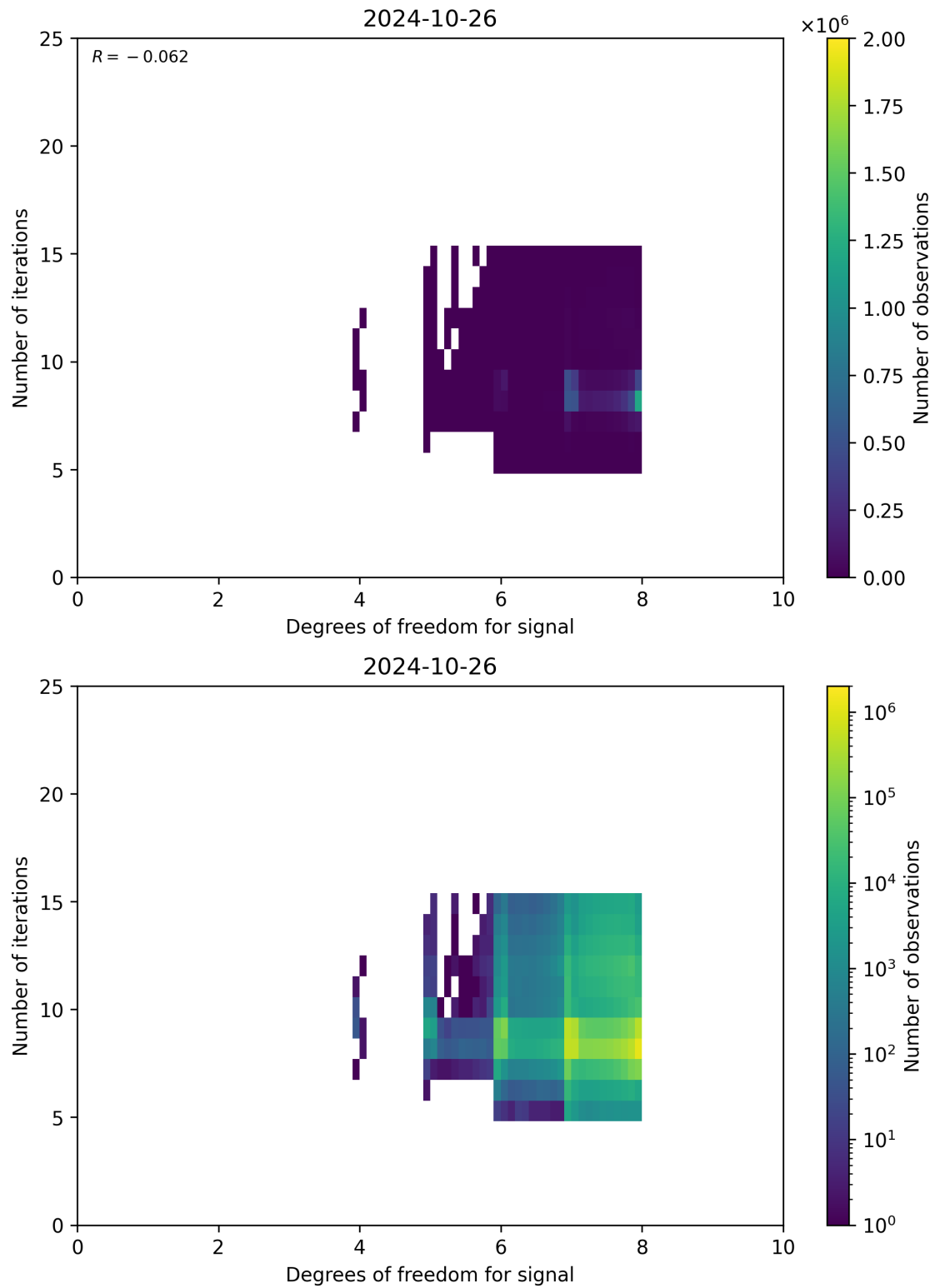
Figure 50: Scatter density plot of “Degrees of freedom for signal” against “Number of iterations” for 2024-10-25 to 2024-10-27.
