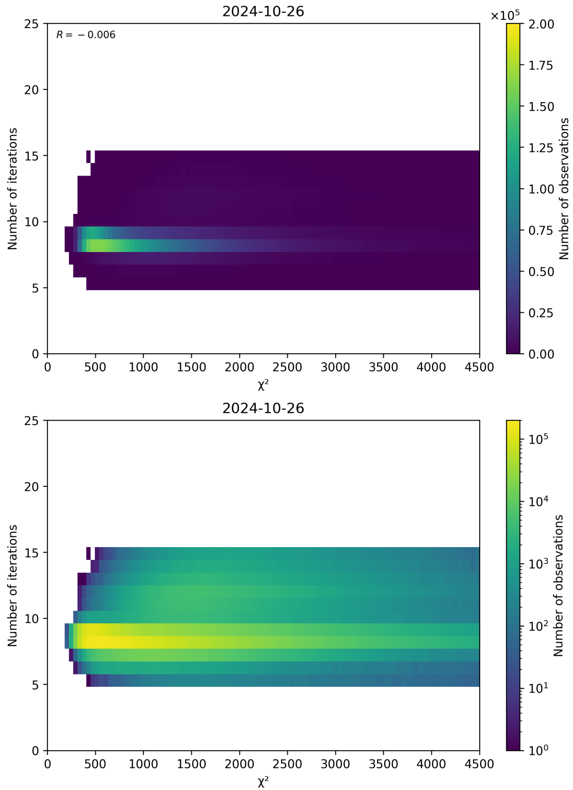
Figure 49: Scatter density plot of “ \chi^2 ” against “Number of iterations” for 2024-10-25 to 2024-10-27.
