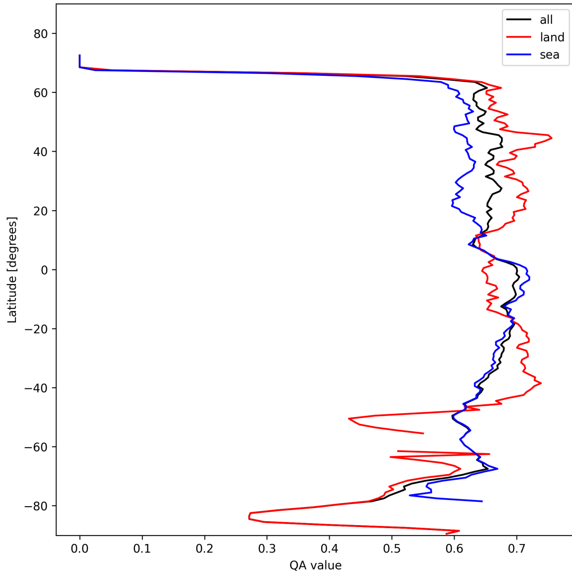
Figure 9: Zonal average of “QA value” for 2024-10-25 to 2024-10-27.
