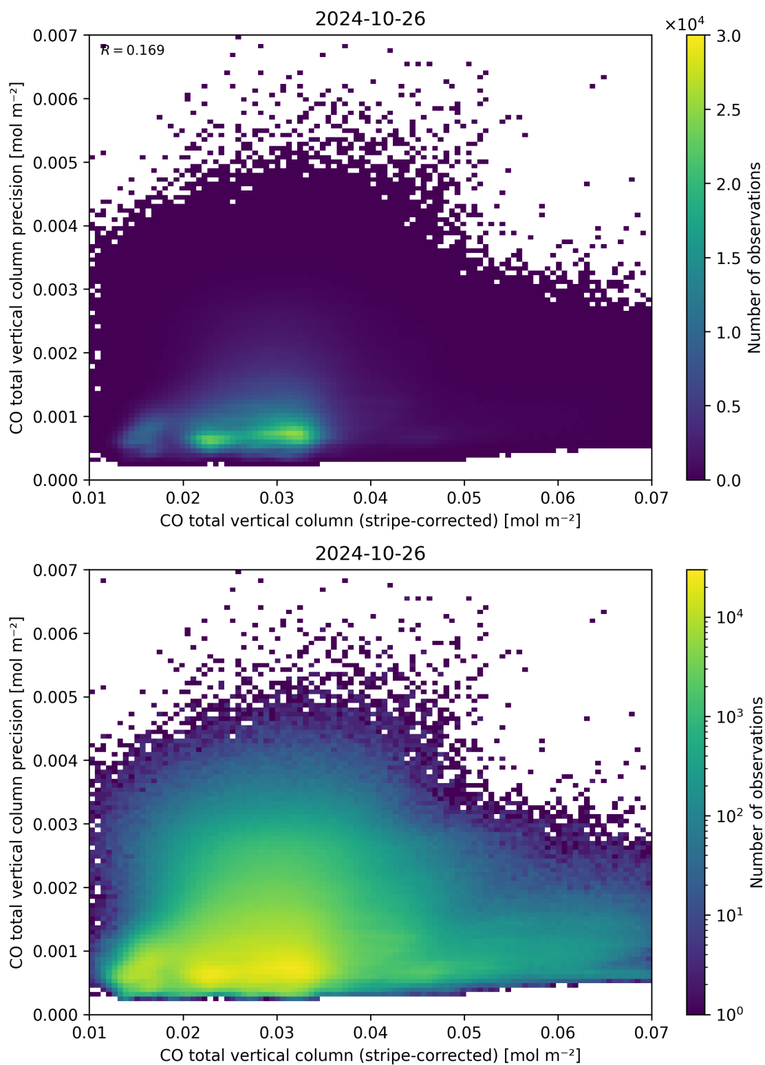
Figure 36: Scatter density plot of “CO total vertical column (stripe-corrected)” against “CO total vertical column precision” for 2024-10-25 to 2024-10-27.
