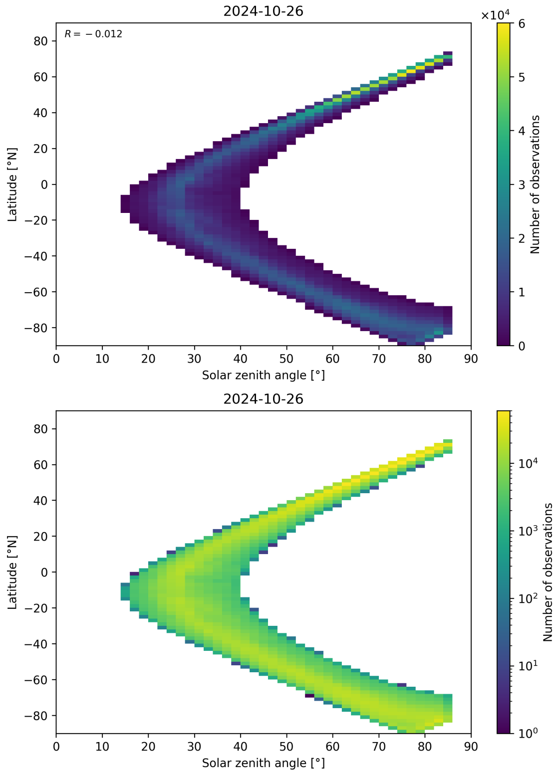
Figure 66: Scatter density plot of “Solar zenith angle” against “Latitude” for 2024-10-25 to 2024-10-27.
