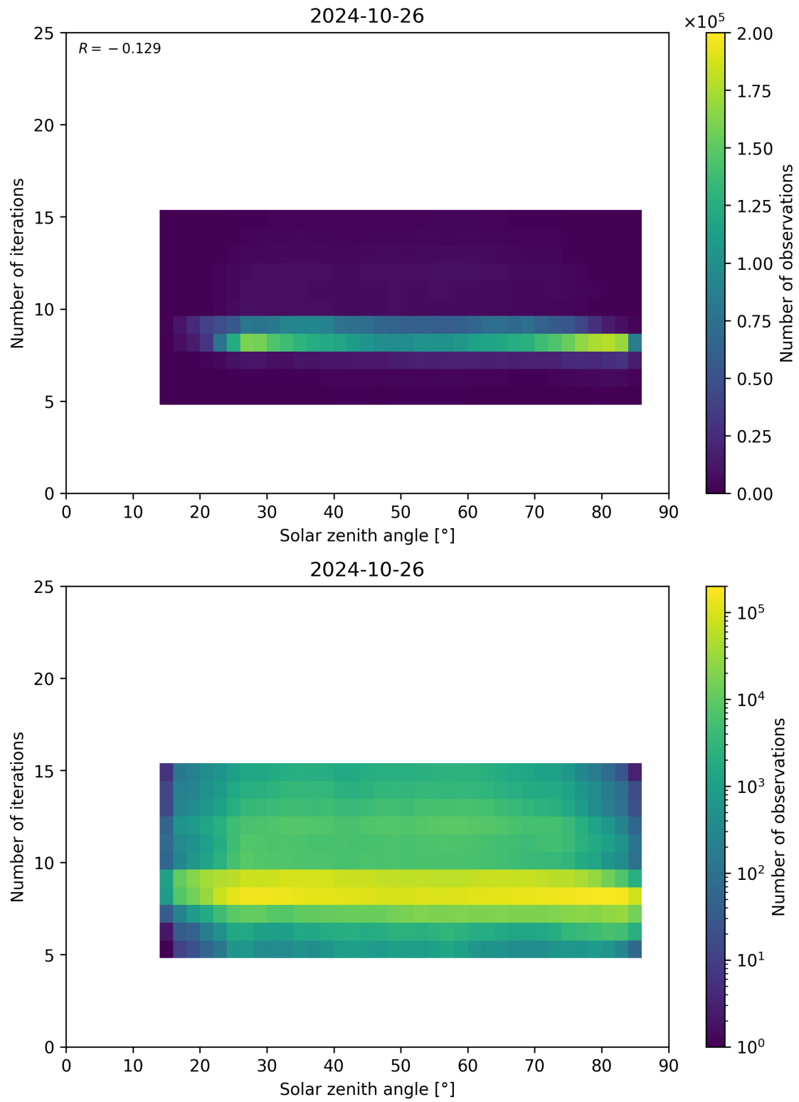
Figure 67: Scatter density plot of “Solar zenith angle” against “Number of iterations” for 2024-10-25 to 2024-10-27.
