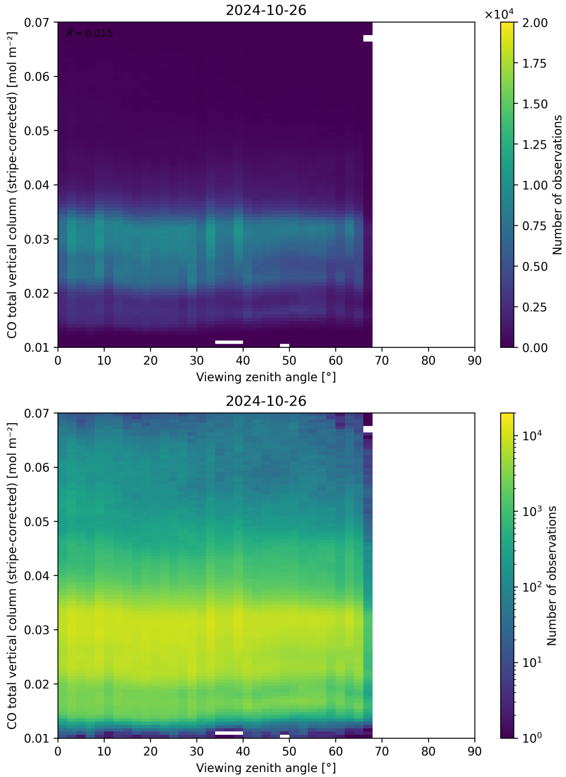
Figure 70: Scatter density plot of “Viewing zenith angle” against “CO total vertical column (stripe-corrected)” for 2024-10-25 to 2024-10-27.
