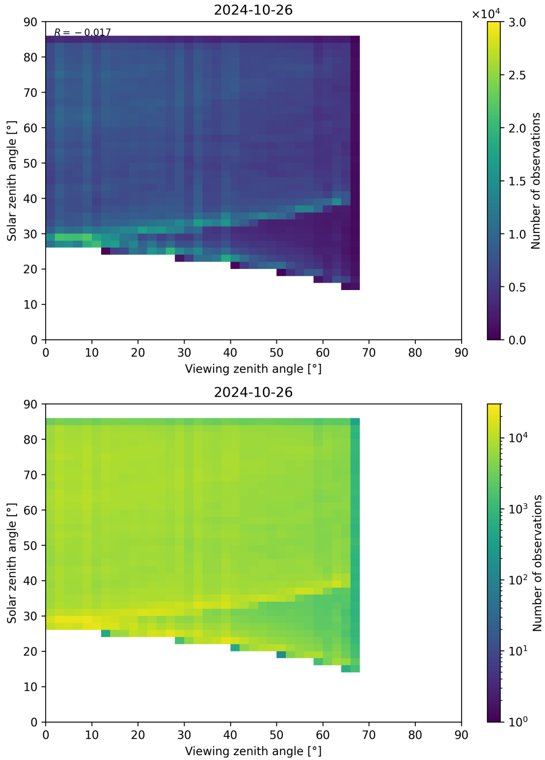
Figure 77: Scatter density plot of “Viewing zenith angle” against “Solar zenith angle” for 2024-10-25 to 2024-10-27.
