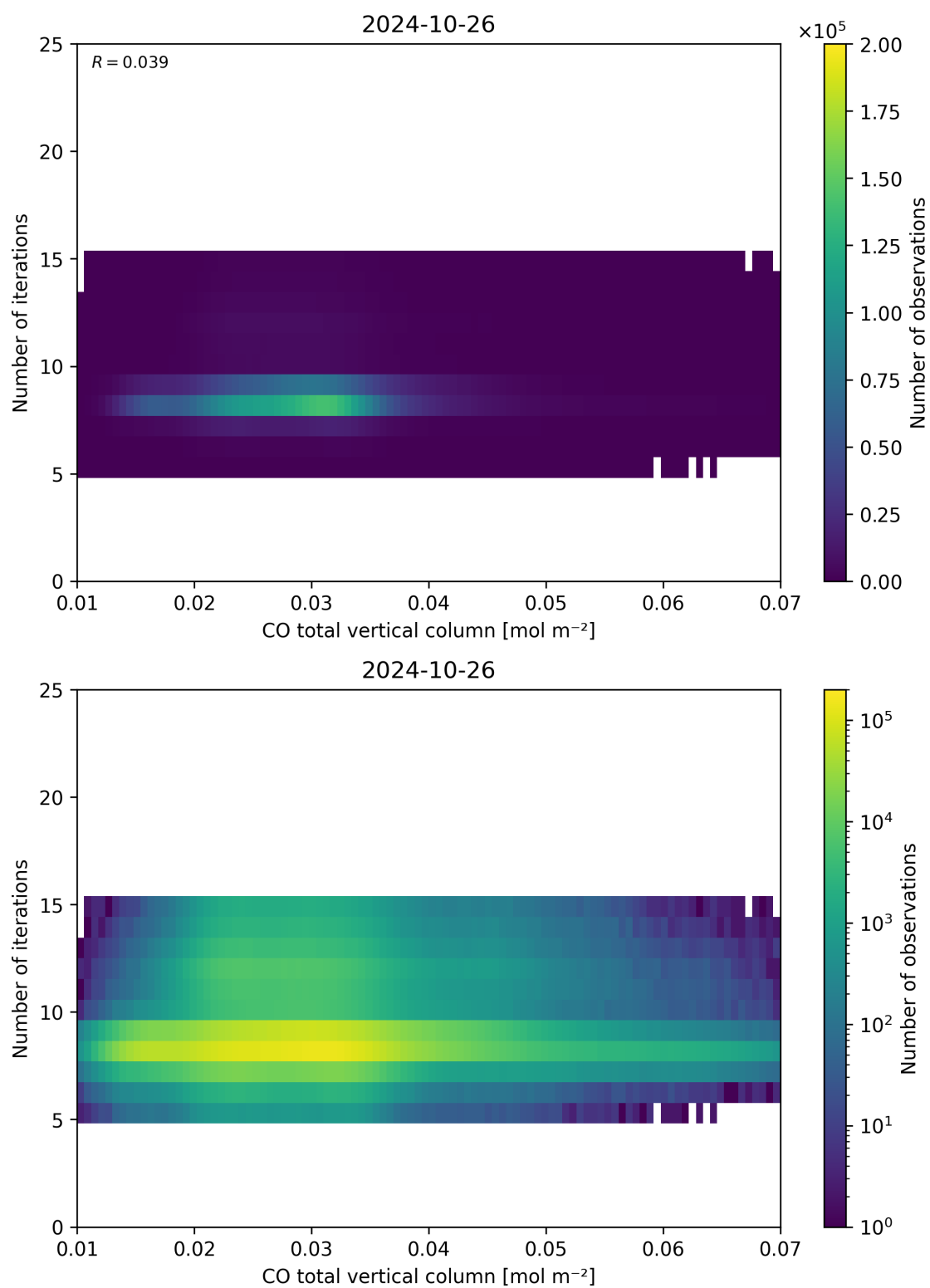
Figure 42: Scatter density plot of “CO total vertical column” against “Number of iterations” for 2024-10-25 to 2024-10-27.
