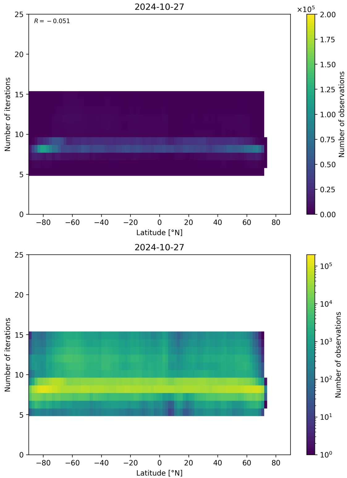
Figure 56: Scatter density plot of “Latitude” against “Number of iterations” for 2024-10-26 to 2024-10-28.
