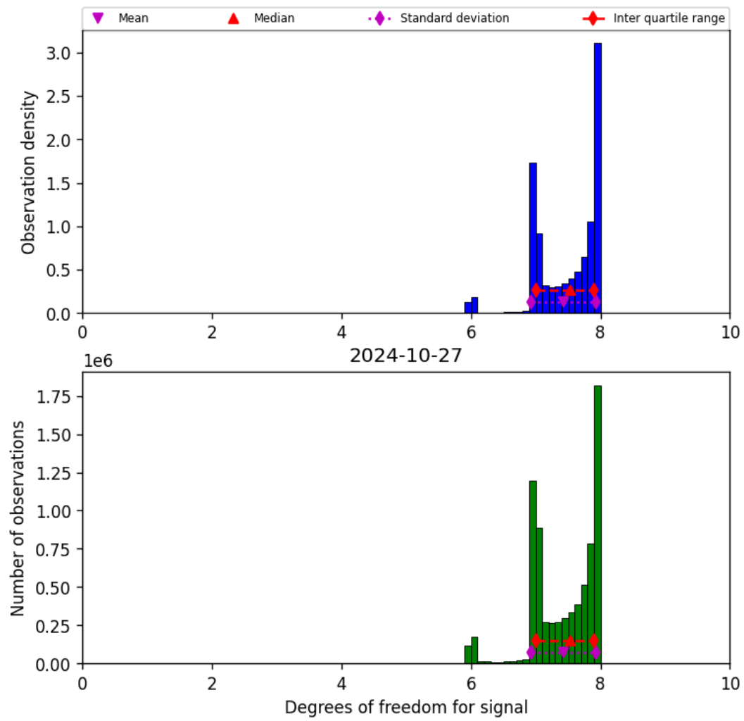
Figure 23: Histogram of “Degrees of freedom for signal” for 2024-10-26 to 2024-10-28
