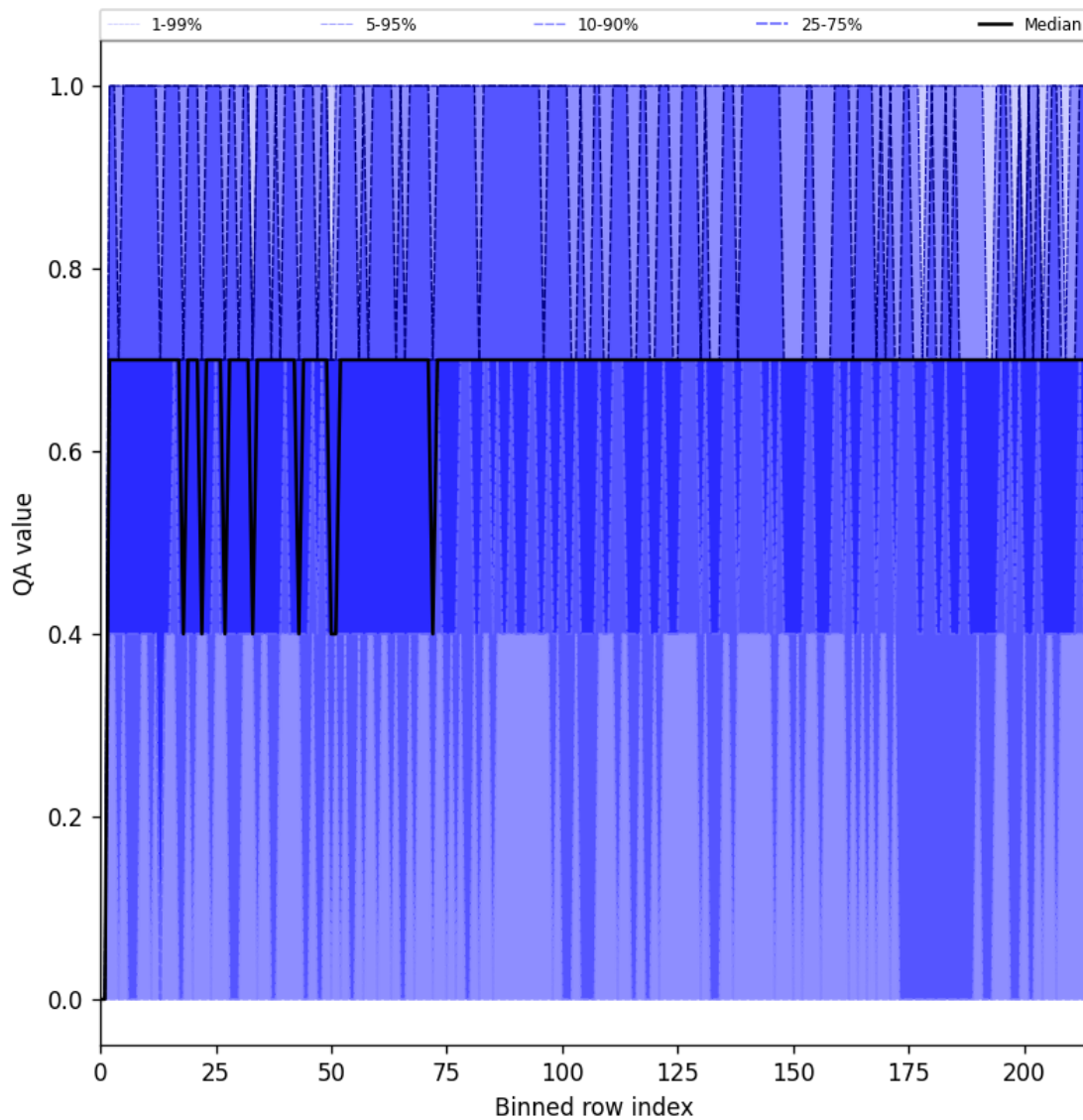
Figure 25: Along track statistics of “QA value” for 2024-10-26 to 2024-10-28
