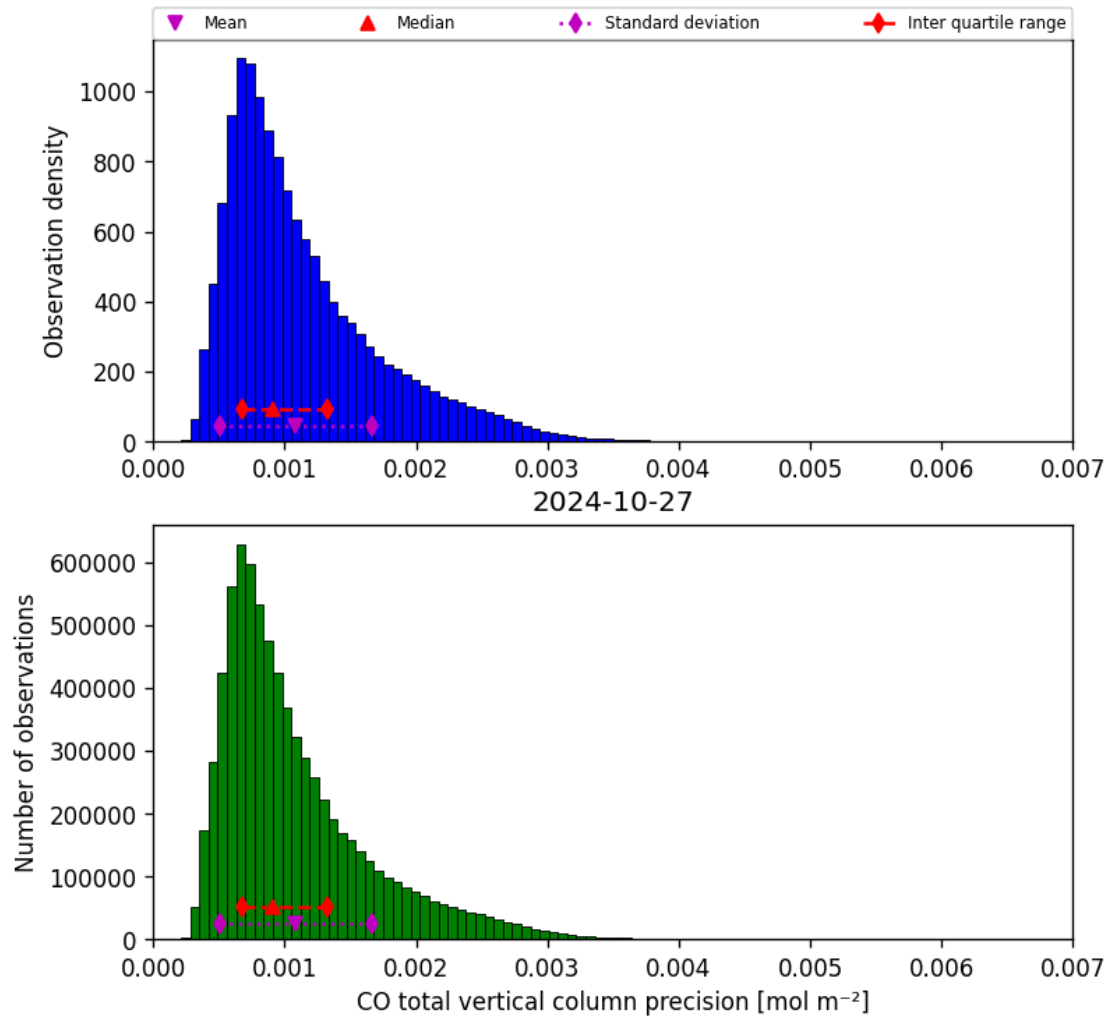
Figure 20: Histogram of “CO total vertical column precision” for 2024-10-26 to 2024-10-28
