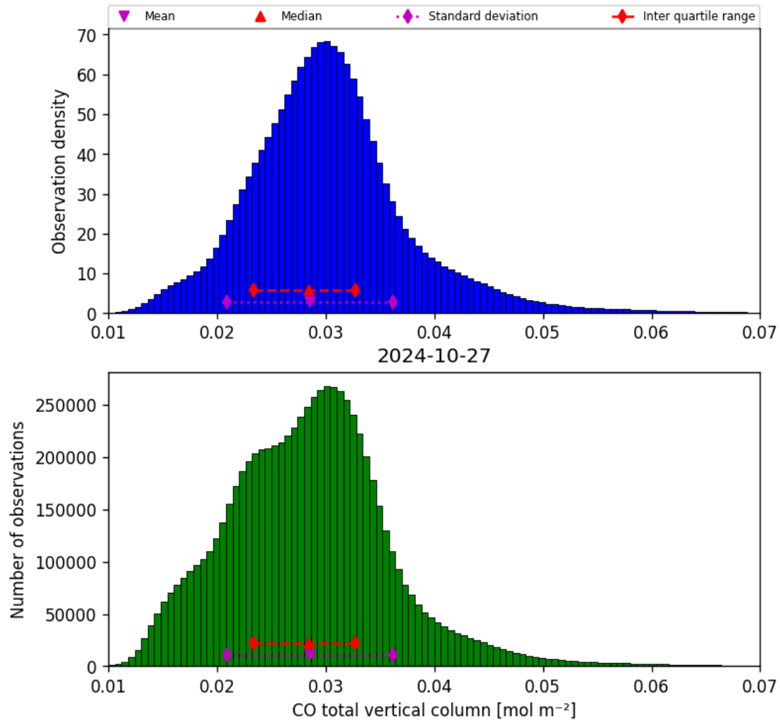
Figure 18: Histogram of “CO total vertical column” for 2024-10-26 to 2024-10-28
