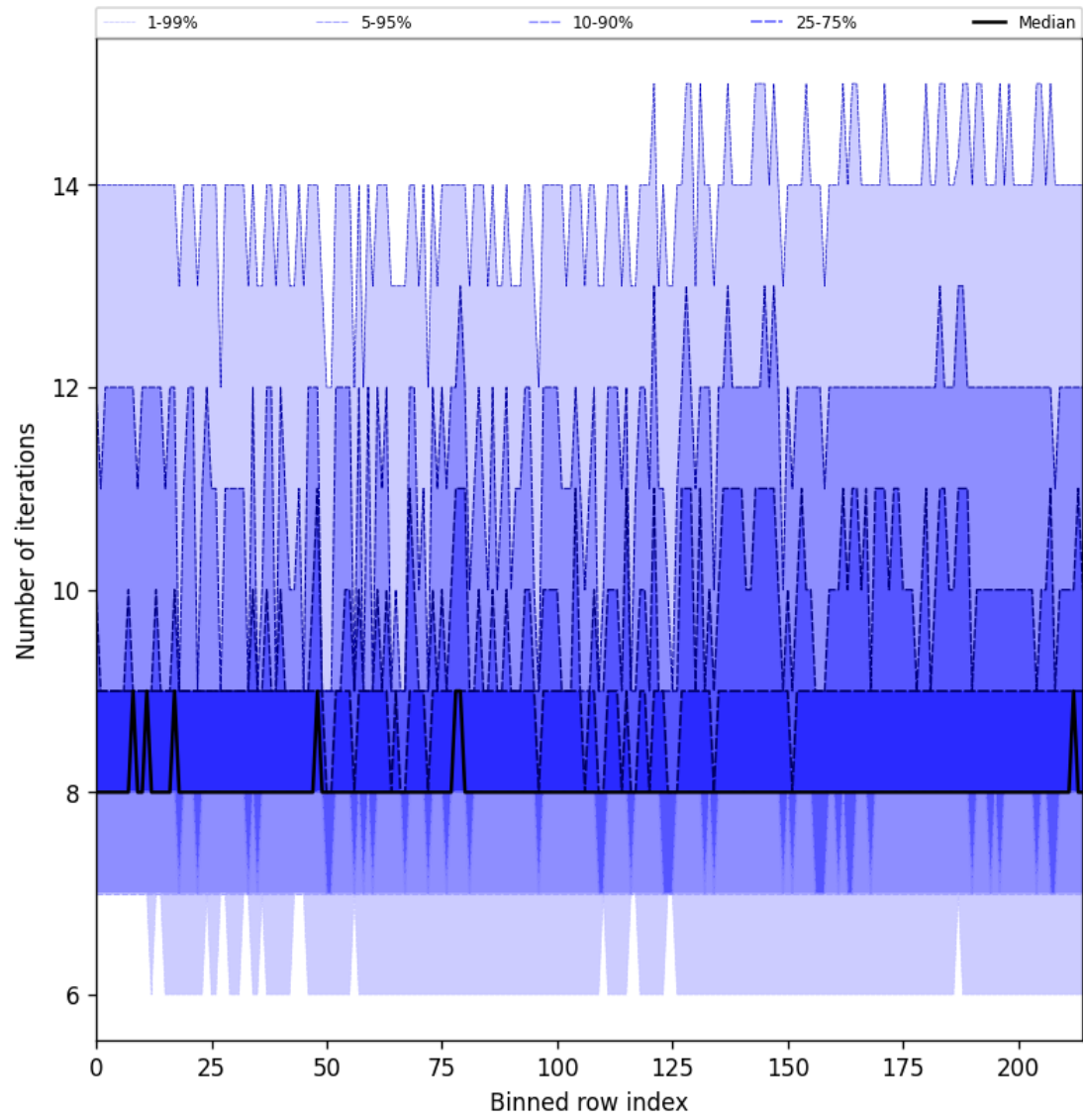
Figure 32: Along track statistics of “Number of iterations” for 2024-10-26 to 2024-10-28
