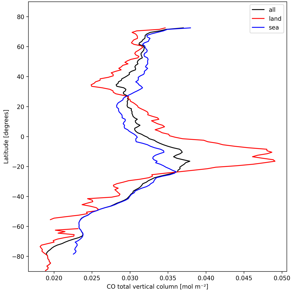
Figure 10: Zonal average of “CO total vertical column” for 2024-10-26 to 2024-10-28.
