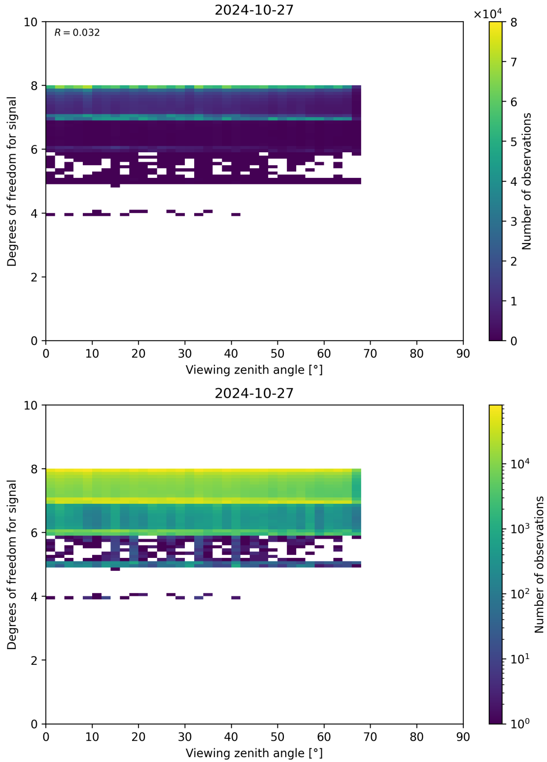
Figure 73: Scatter density plot of “Viewing zenith angle” against “Degrees of freedom for signal” for 2024-10-26 to 2024-10-28.
