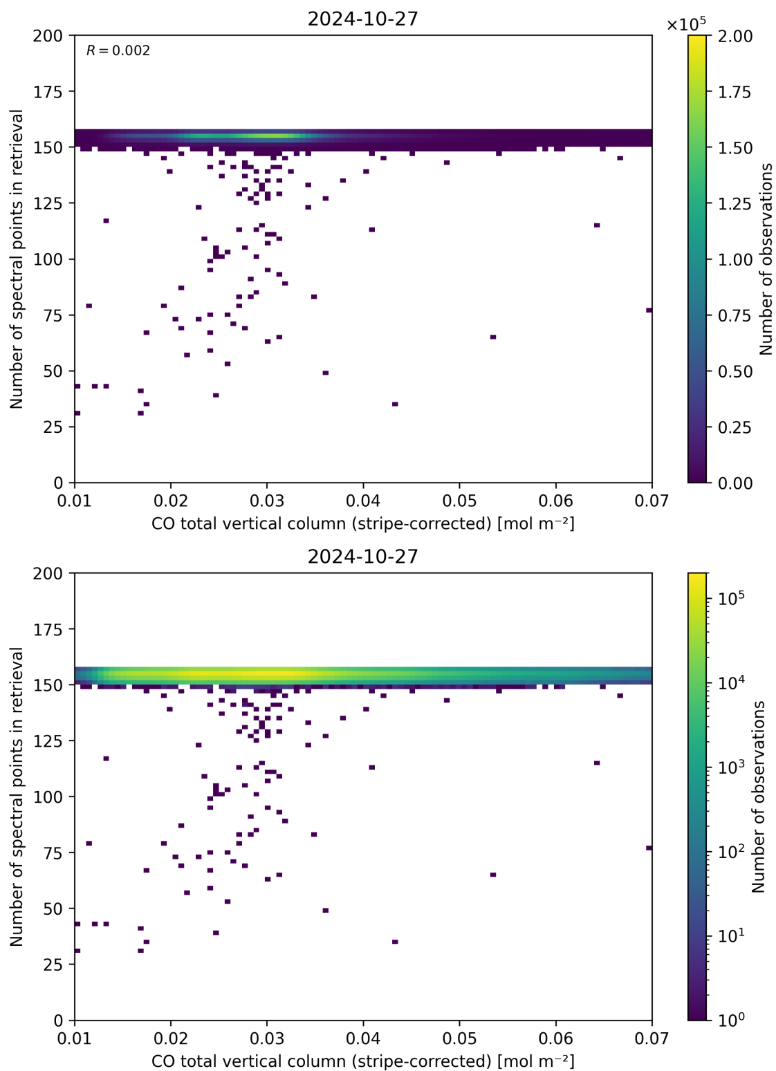
Figure 40: Scatter density plot of “CO total vertical column (stripe-corrected)” against “Number of spectral points in retrieval” for 2024-10-26 to 2024-10-28.
