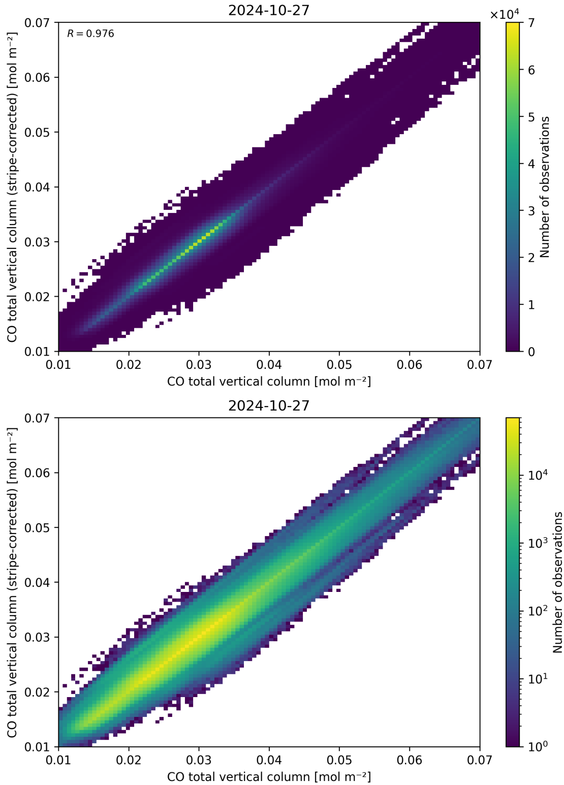
Figure 33: Scatter density plot of “CO total vertical column” against “CO total vertical column (stripe-corrected)” for 2024-10-26 to 2024-10-28.
