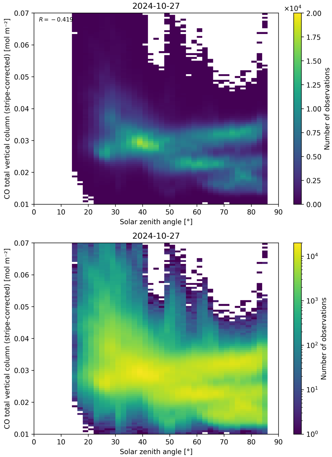
Figure 62: Scatter density plot of “Solar zenith angle” against “CO total vertical column (stripe-corrected)” for 2024-10-26 to 2024-10-28.
