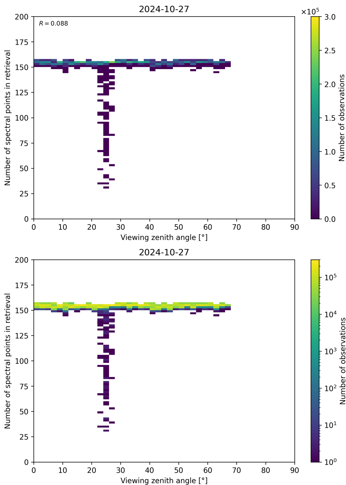
Figure 76: Scatter density plot of “Viewing zenith angle” against “Number of spectral points in retrieval” for 2024-10-26 to 2024-10-28.
