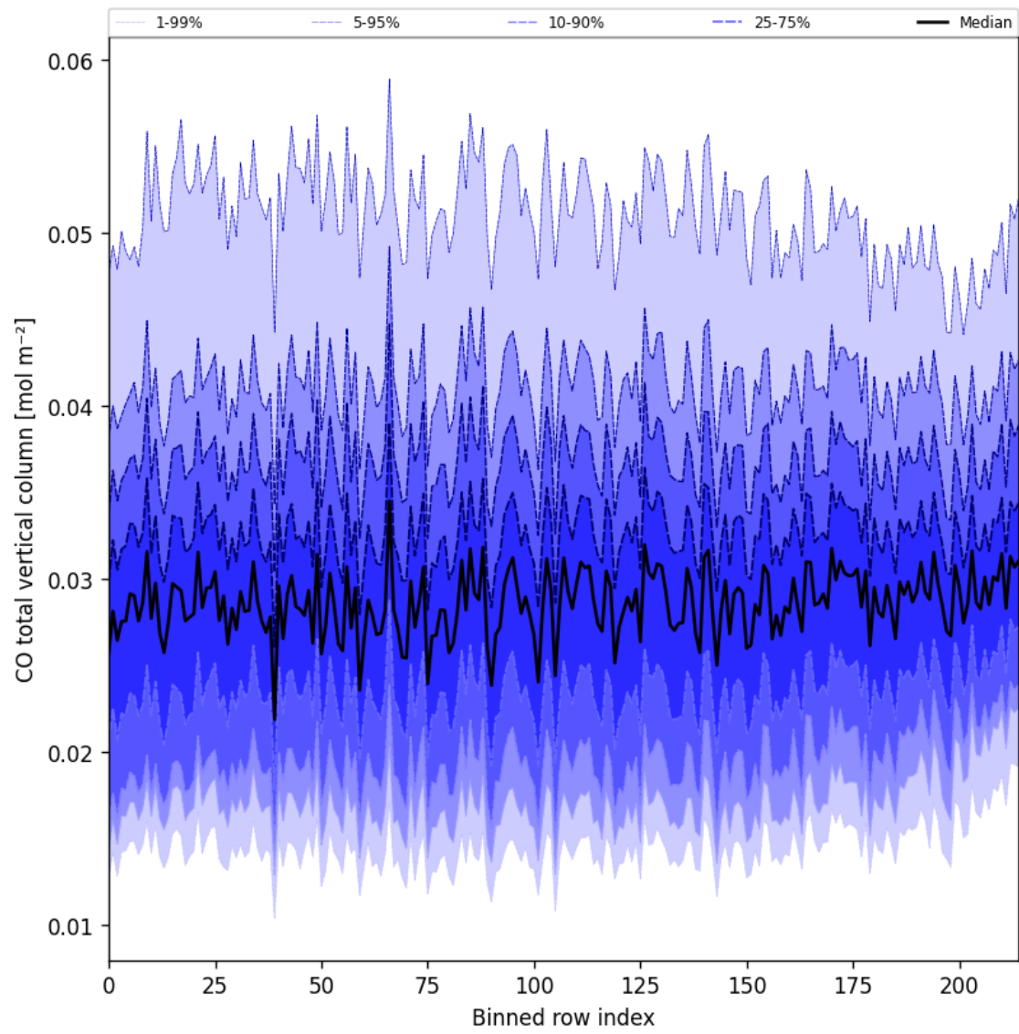
Figure 26: Along track statistics of “CO total vertical column” for 2024-10-26 to 2024-10-28
