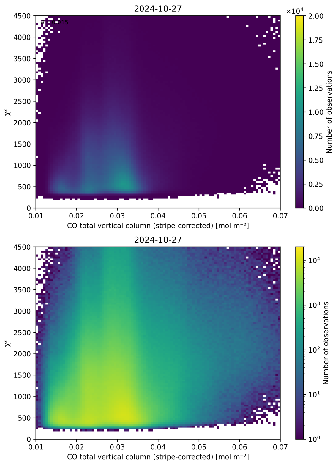
Figure 37: Scatter density plot of “CO total vertical column (stripe-corrected)” against “ \chi^2 ” for 2024-10-26 to 2024-10-28.
