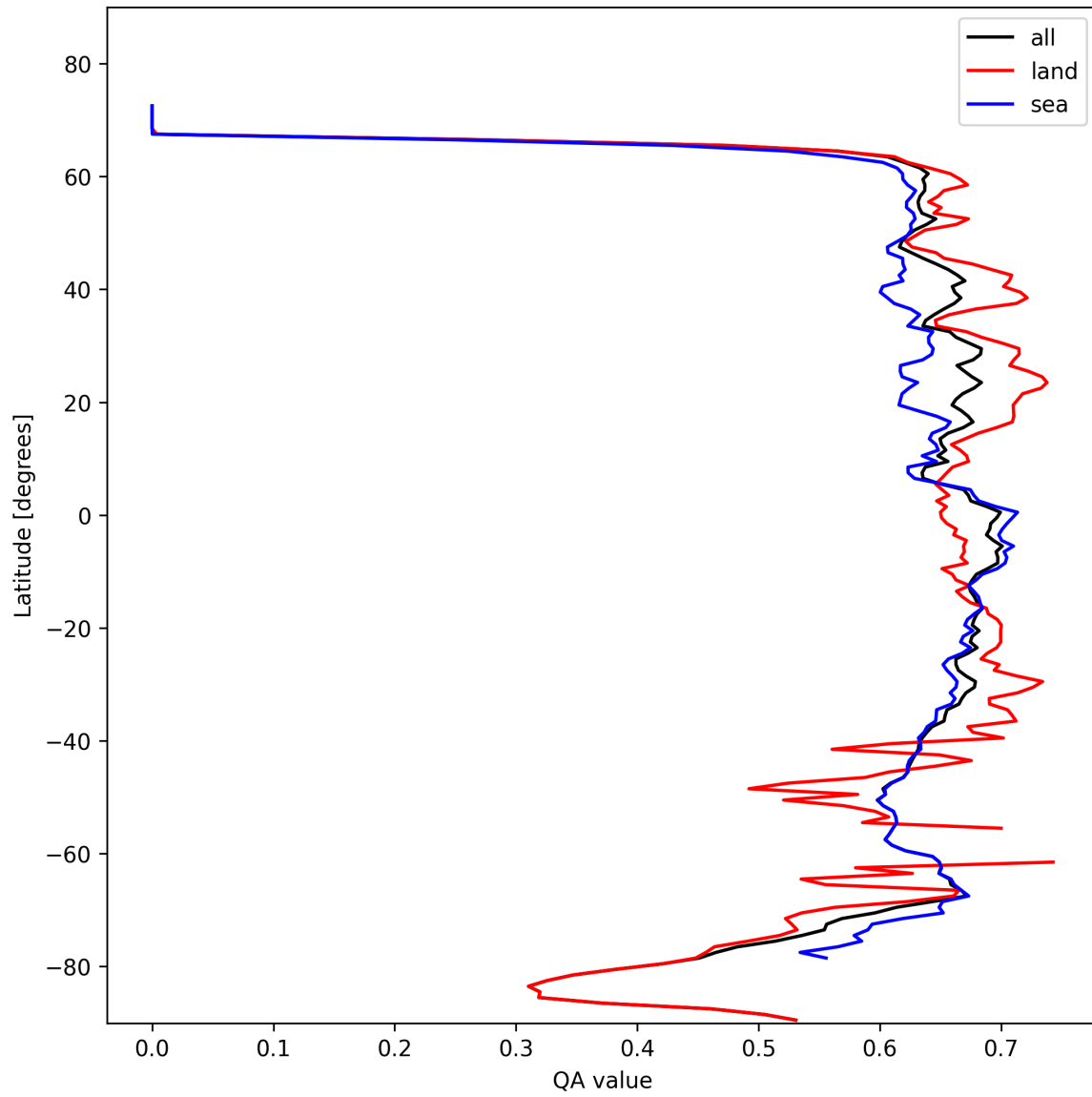
Figure 9: Zonal average of “QA value” for 2024-10-26 to 2024-10-28.
