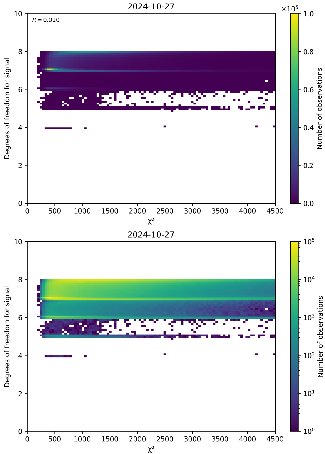
Figure 48: Scatter density plot of “ \chi^2 ” against “Degrees of freedom for signal” for 2024-10-26 to 2024-10-28.
