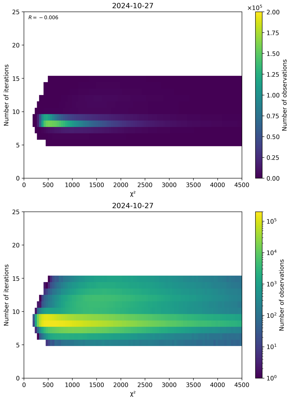
Figure 49: Scatter density plot of “ \chi^2 ” against “Number of iterations” for 2024-10-26 to 2024-10-28.
