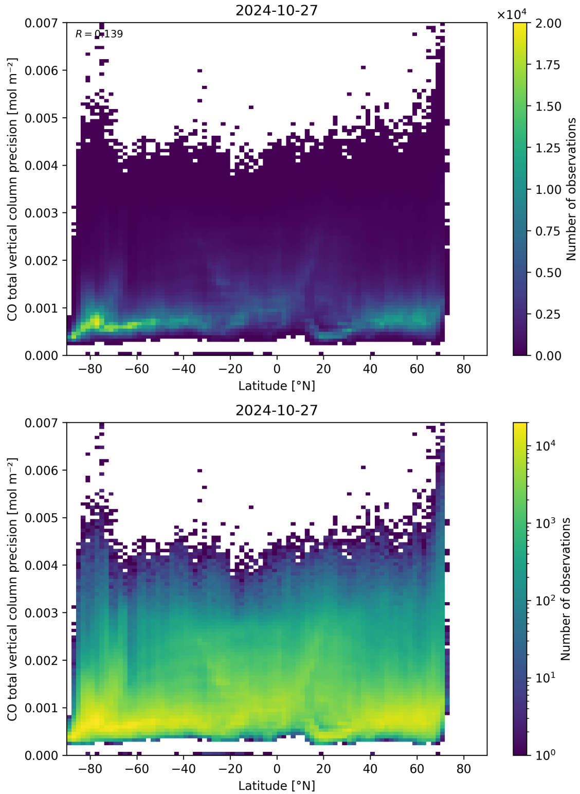
Figure 53: Scatter density plot of “Latitude” against “CO total vertical column precision” for 2024-10-26 to 2024-10-28.
