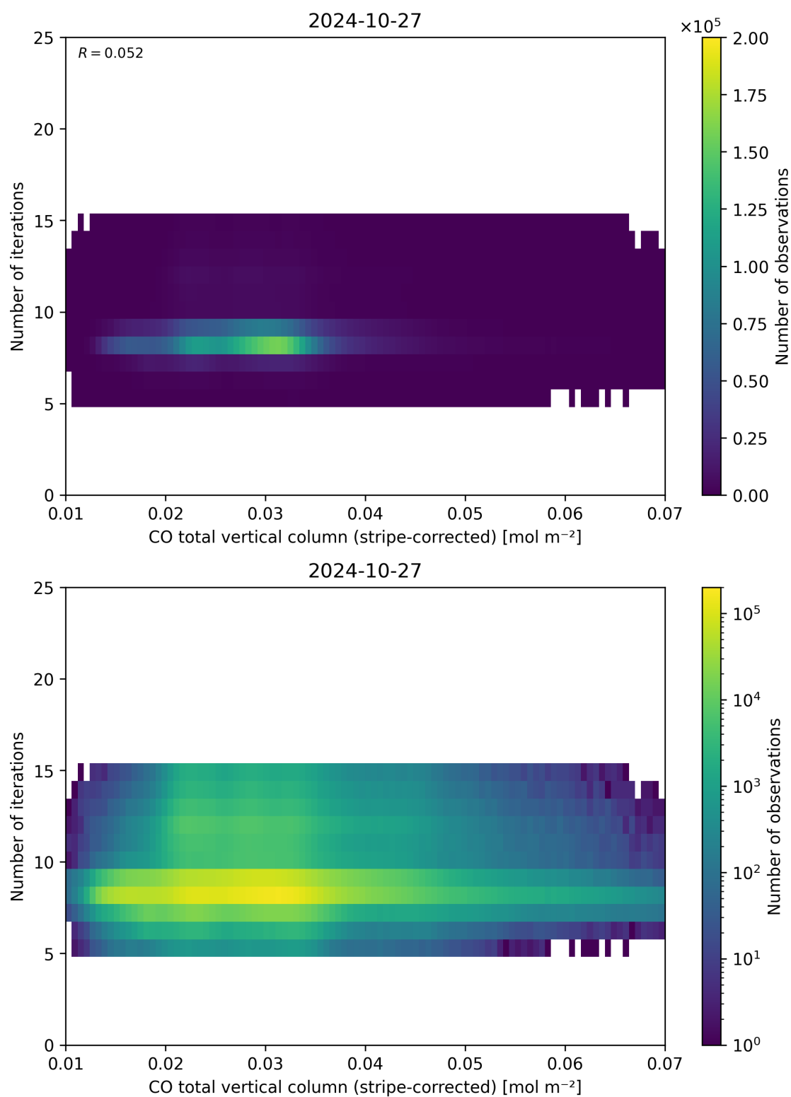
Figure 39: Scatter density plot of “CO total vertical column (stripe-corrected)” against “Number of iterations” for 2024-10-26 to 2024-10-28.
