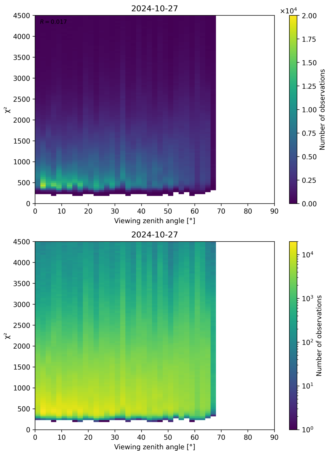
Figure 72: Scatter density plot of “Viewing zenith angle” against “ \chi^2 ” for 2024-10-26 to 2024-10-28.
