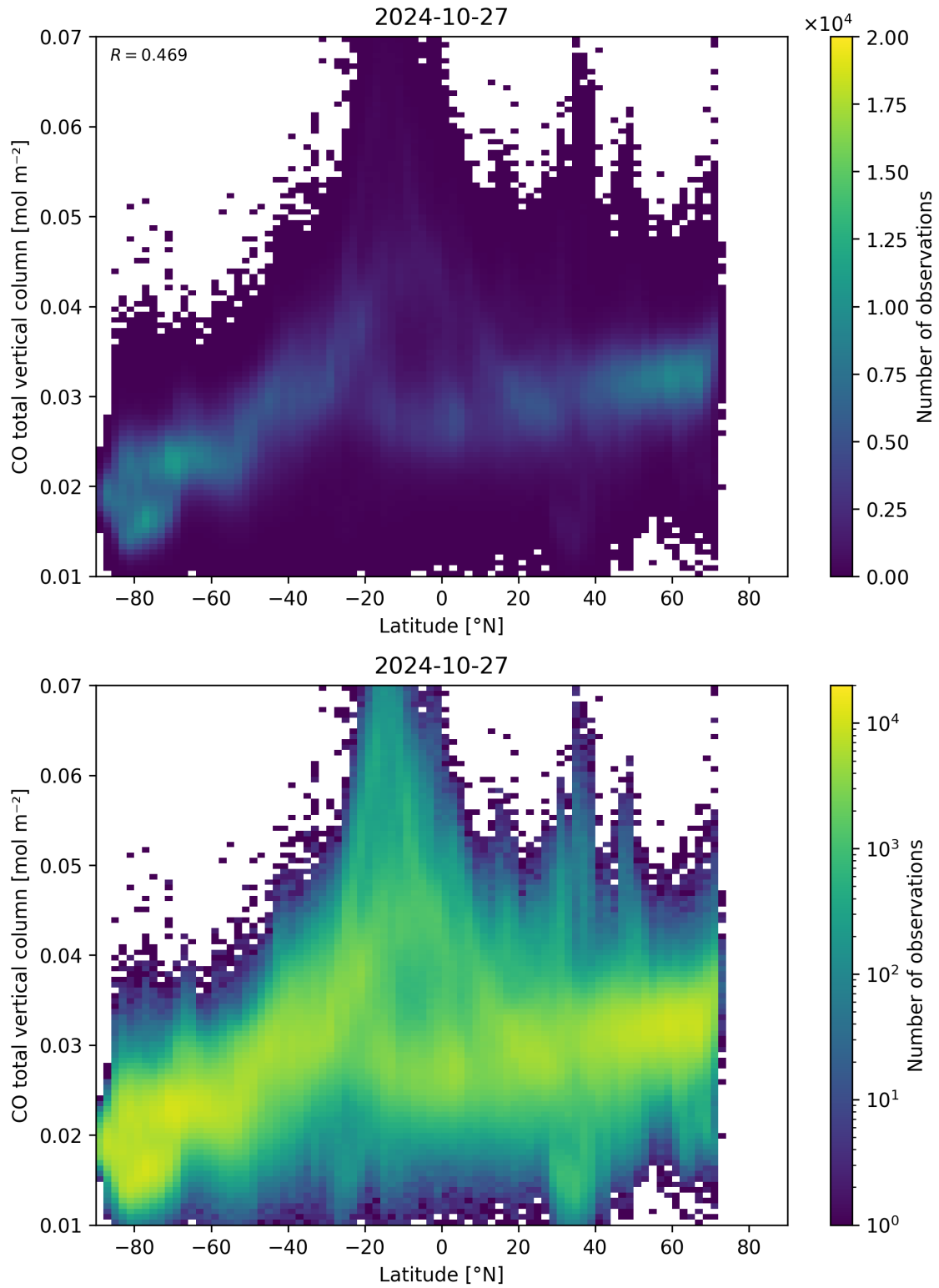
Figure 51: Scatter density plot of “Latitude” against “CO total vertical column” for 2024-10-26 to 2024-10-28.
