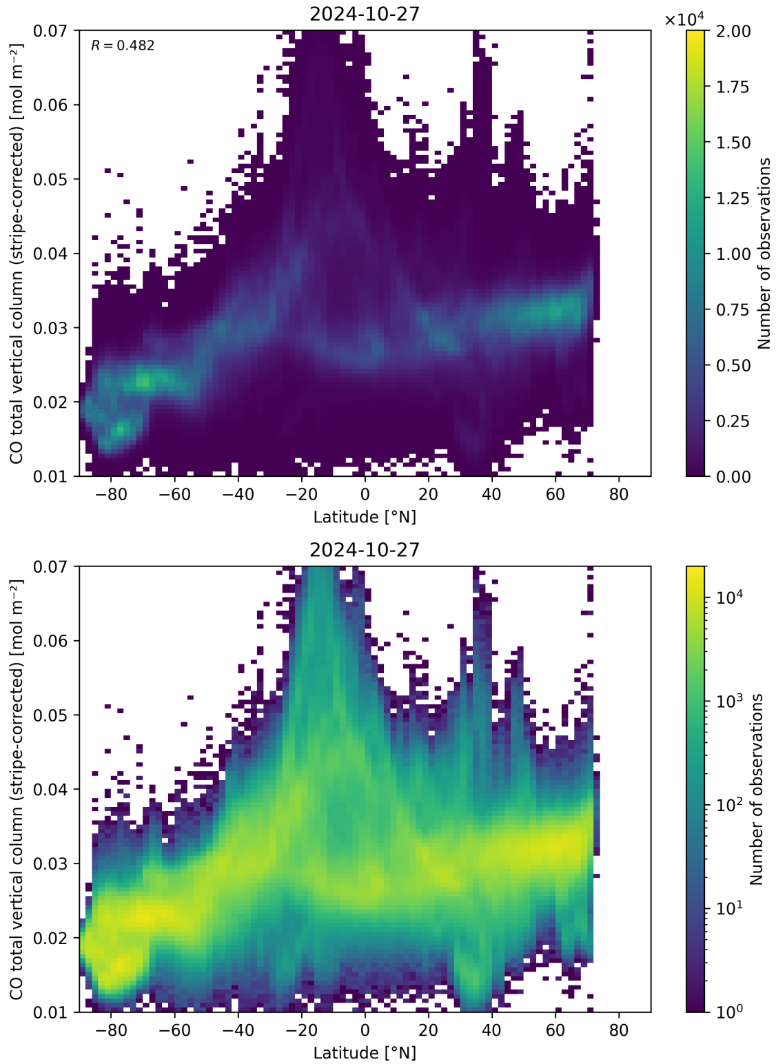
Figure 52: Scatter density plot of “Latitude” against “CO total vertical column (stripe-corrected)” for 2024-10-26 to 2024-10-28.
