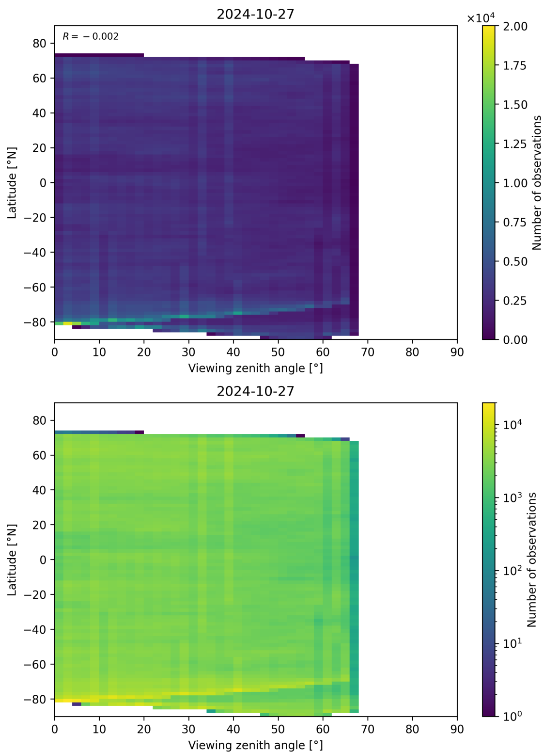
Figure 74: Scatter density plot of “Viewing zenith angle” against “Latitude” for 2024-10-26 to 2024-10-28.
