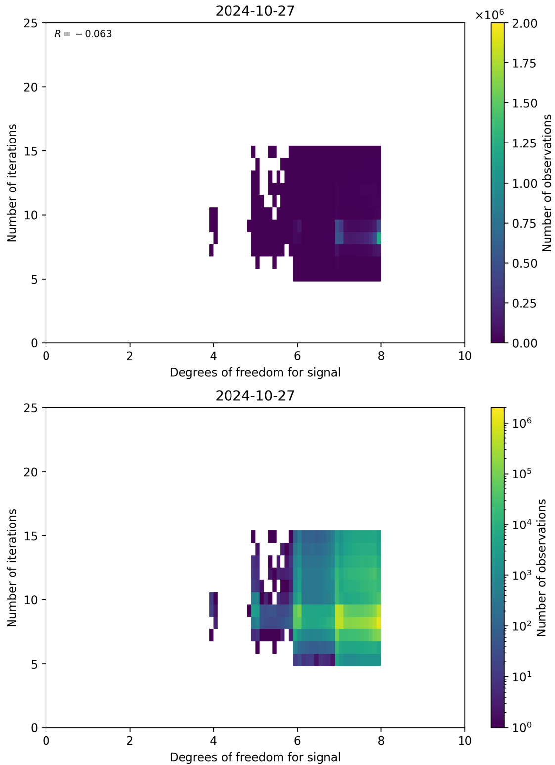
Figure 50: Scatter density plot of “Degrees of freedom for signal” against “Number of iterations” for 2024-10-26 to 2024-10-28.
