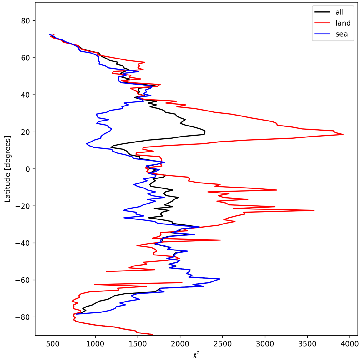
Figure 14: Zonal average of “ \chi^2 ” for 2024-10-26 to 2024-10-28.
