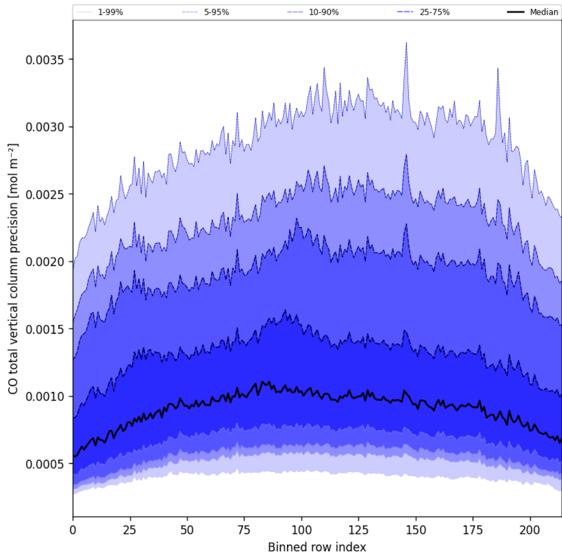
Figure 28: Along track statistics of “CO total vertical column precision” for 2024-10-26 to 2024-10-28
