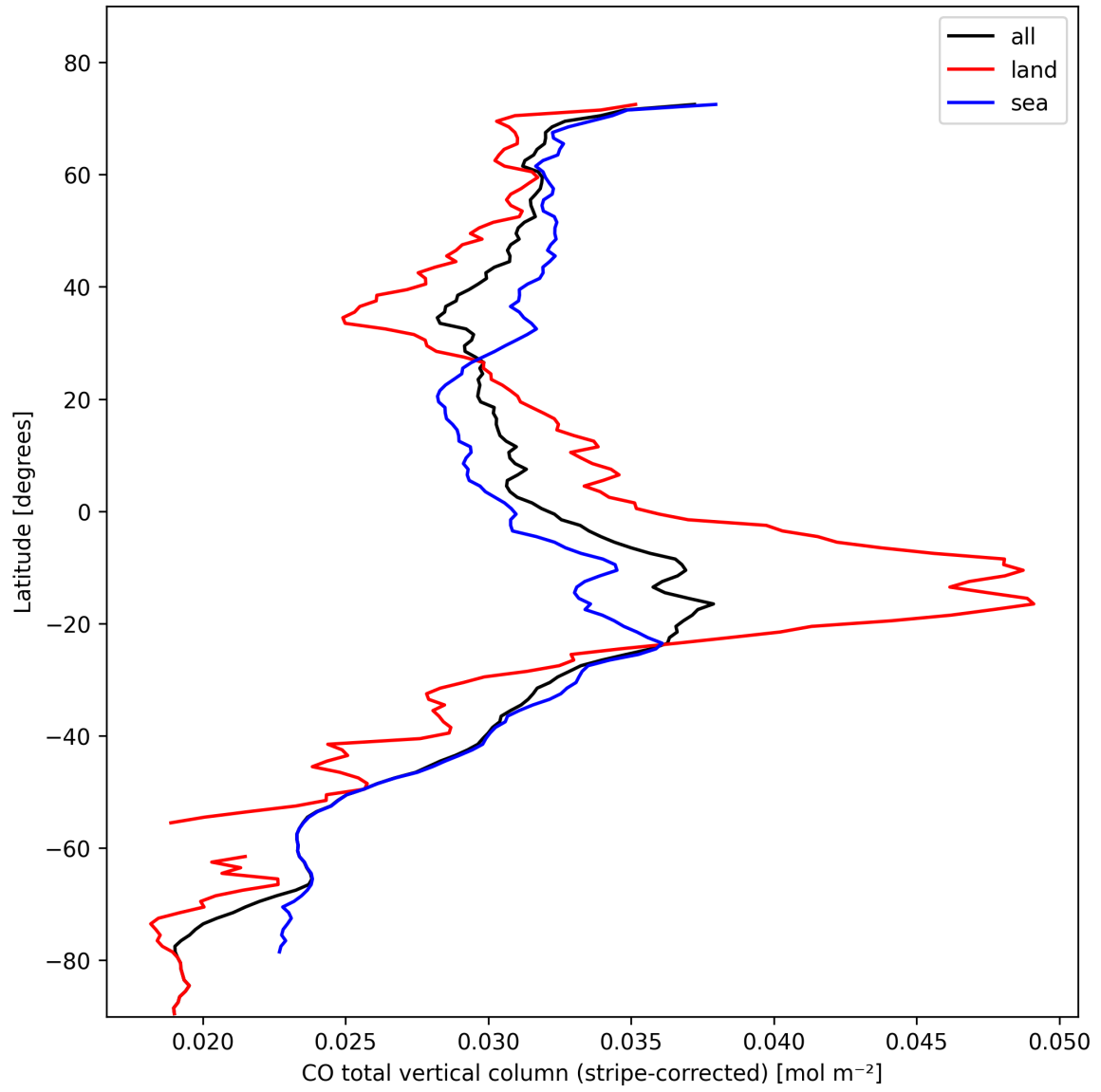
Figure 11: Zonal average of “CO total vertical column (stripe-corrected)” for 2024-10-26 to 2024-10-28.
