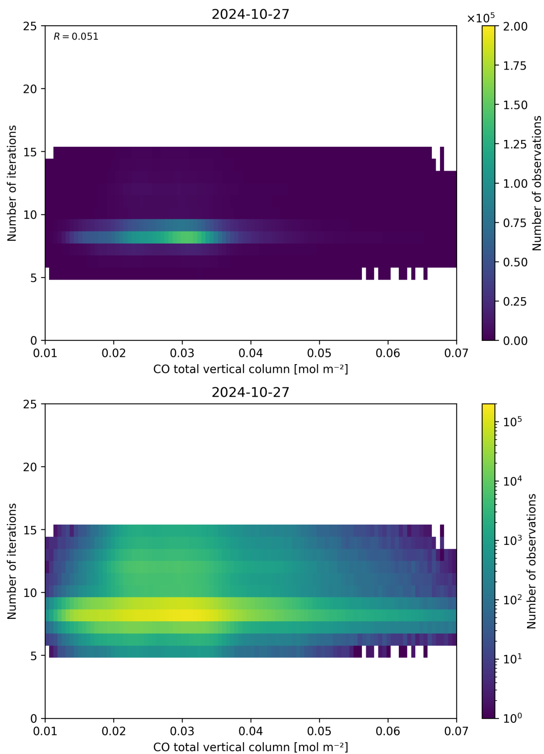
Figure 42: Scatter density plot of “CO total vertical column” against “Number of iterations” for 2024-10-26 to 2024-10-28.
