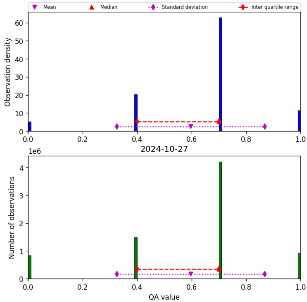
Figure 17: Histogram of “QA value” for 2024-10-26 to 2024-10-28
