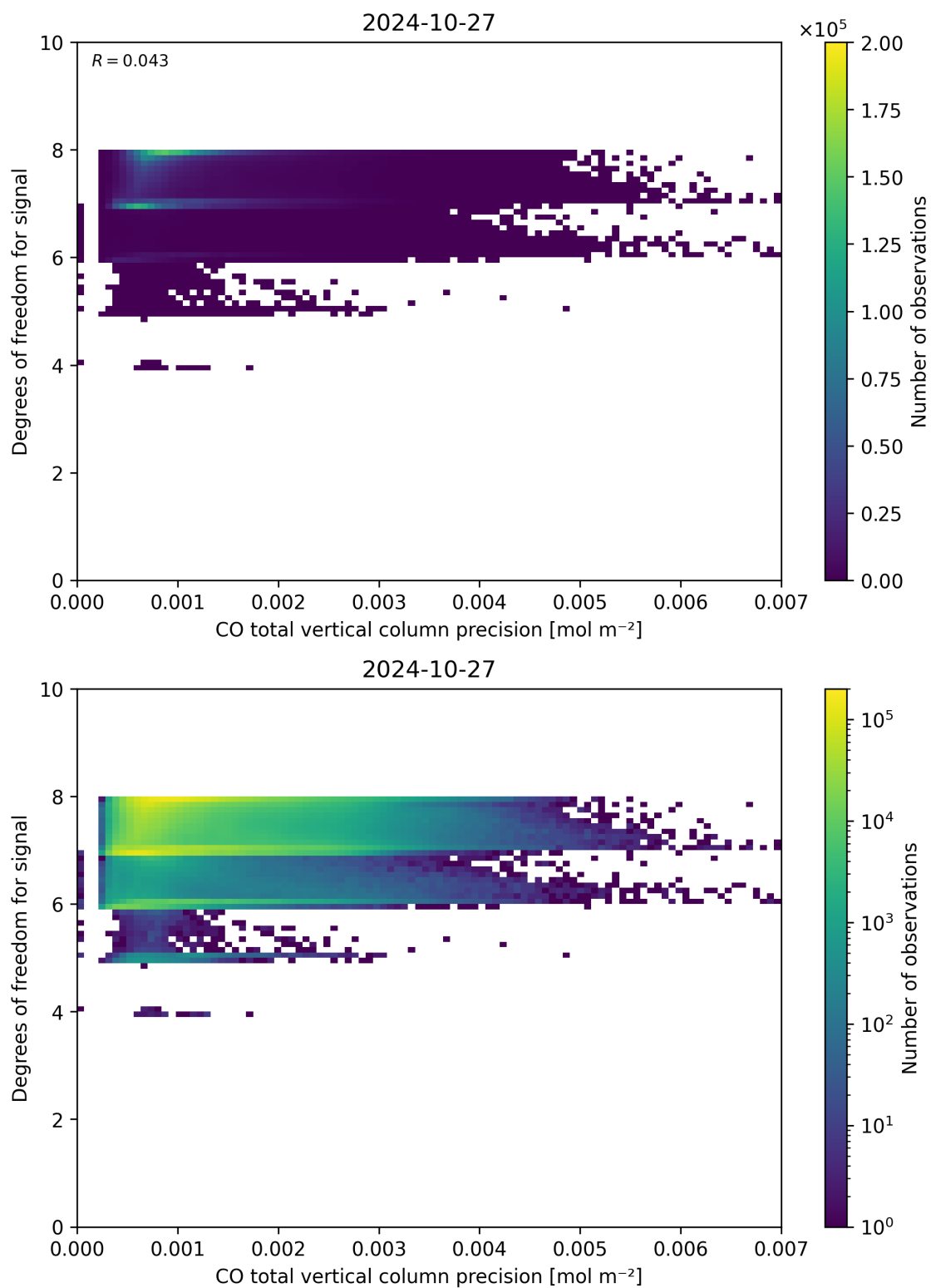
Figure 45: Scatter density plot of “CO total vertical column precision” against “Degrees of freedom for signal” for 2024-10-26 to 2024-10-28.
