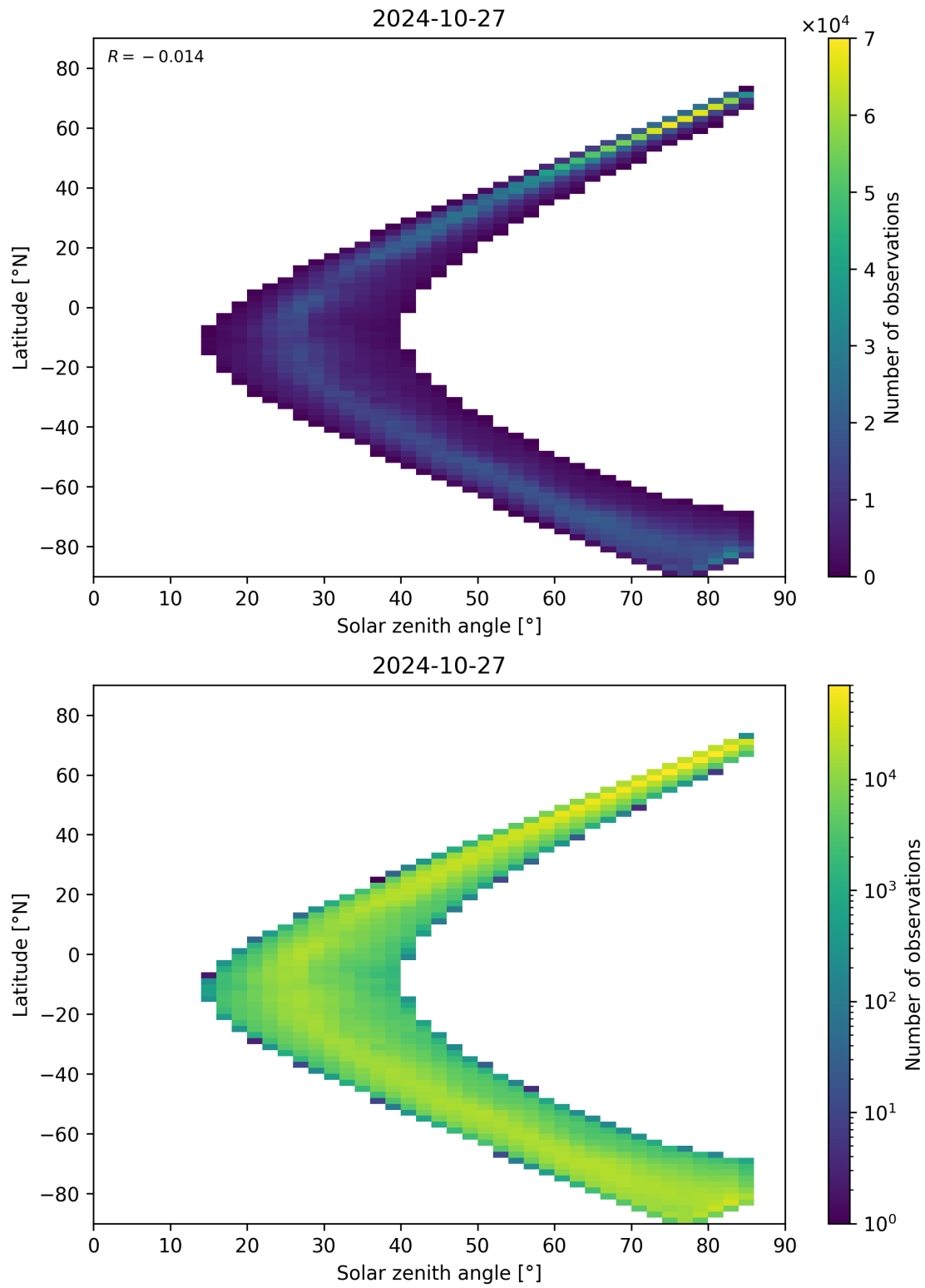
Figure 66: Scatter density plot of “Solar zenith angle” against “Latitude” for 2024-10-26 to 2024-10-28.
