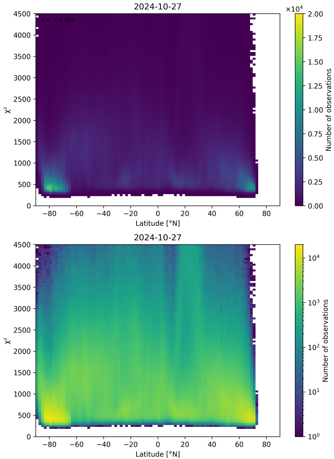
Figure 54: Scatter density plot of “Latitude” against “ \chi^2 ” for 2024-10-26 to 2024-10-28.
