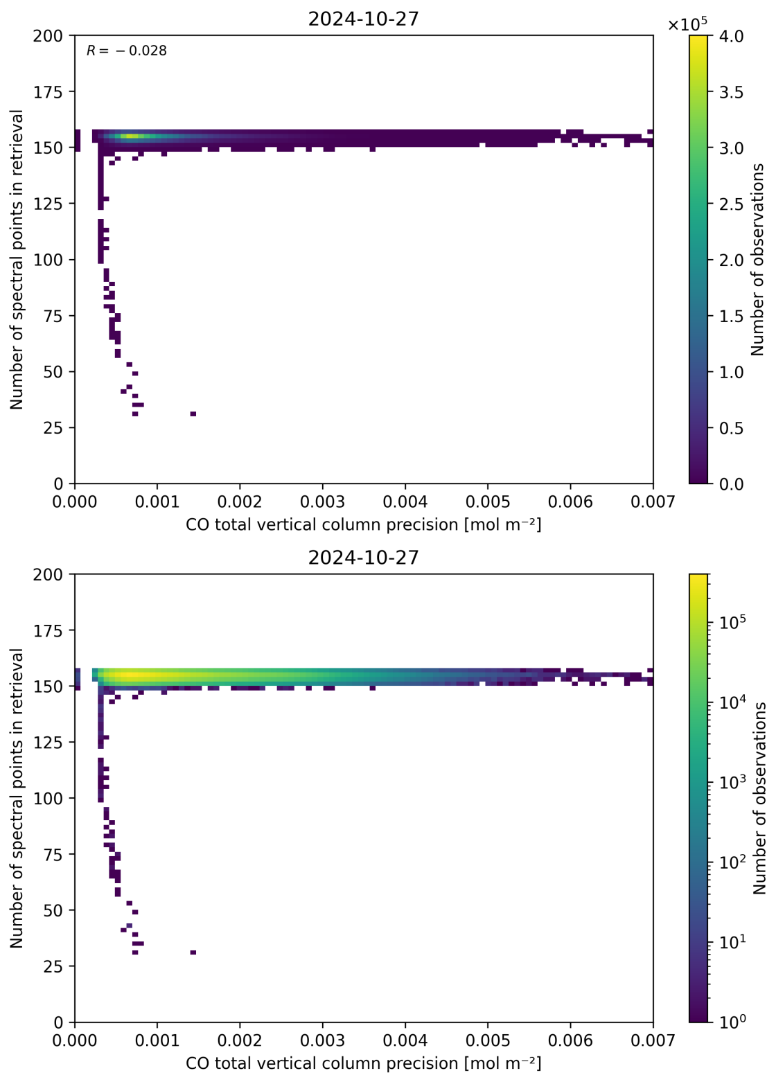
Figure 47: Scatter density plot of “CO total vertical column precision” against “Number of spectral points in retrieval” for 2024-10-26 to 2024-10-28.
