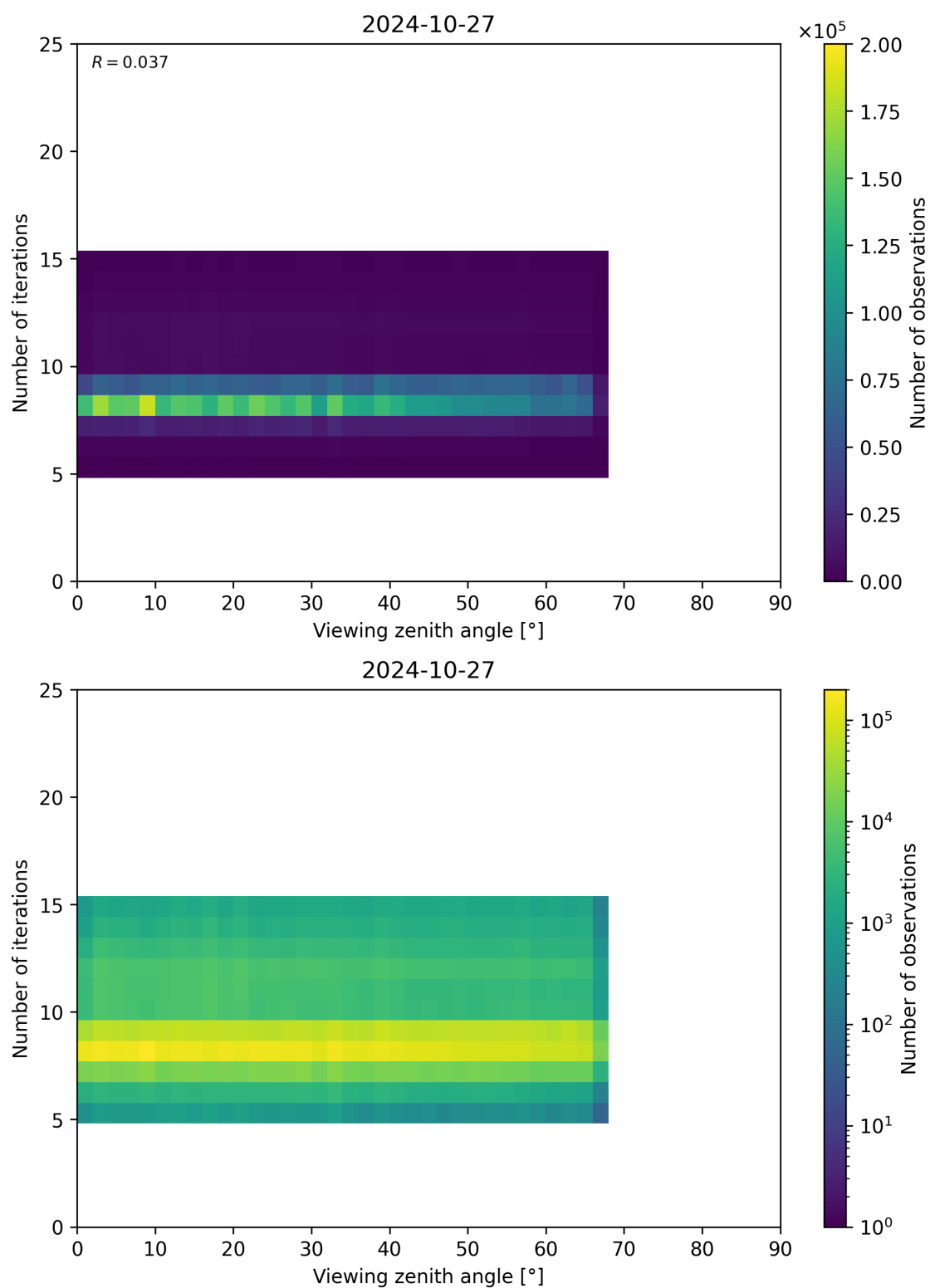
Figure 75: Scatter density plot of “Viewing zenith angle” against “Number of iterations” for 2024-10-26 to 2024-10-28.
