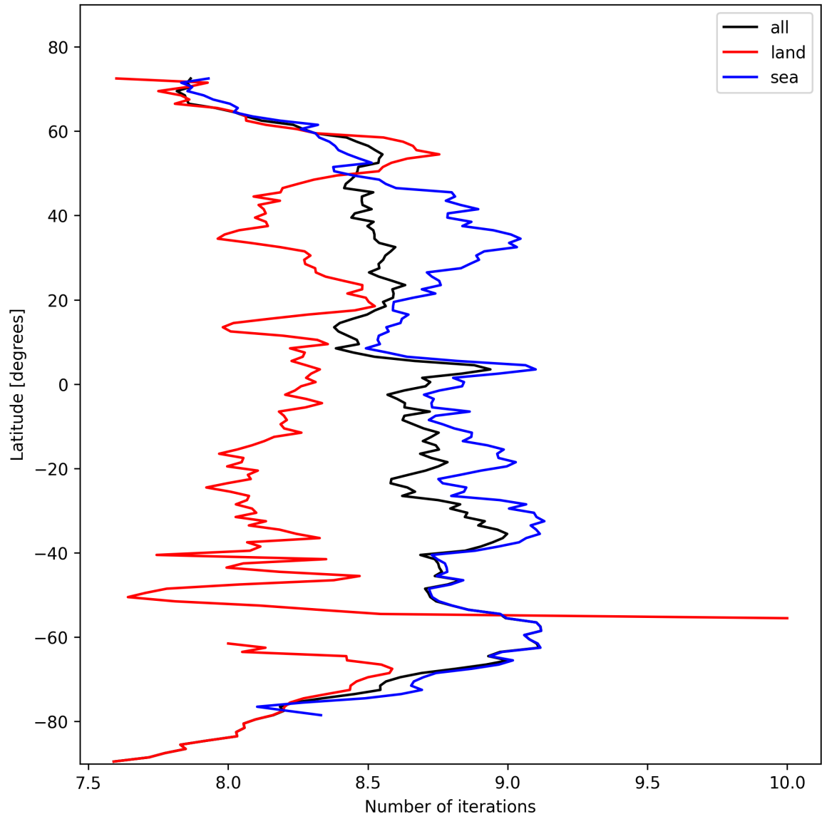
Figure 16: Zonal average of “Number of iterations” for 2024-10-26 to 2024-10-28.
