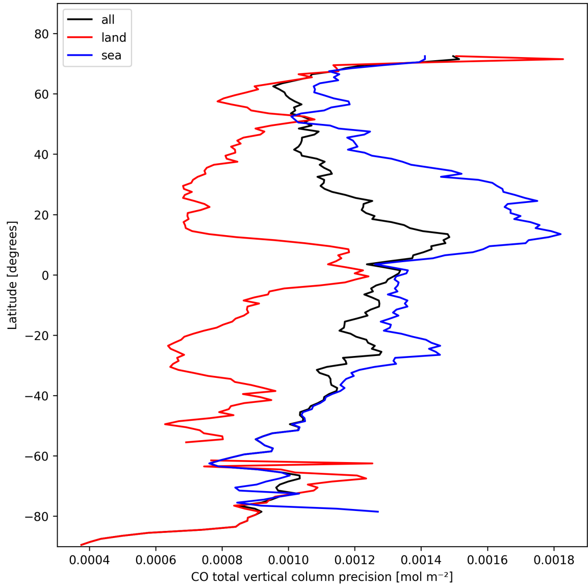
Figure 12: Zonal average of “CO total vertical column precision” for 2024-10-26 to 2024-10-28.
