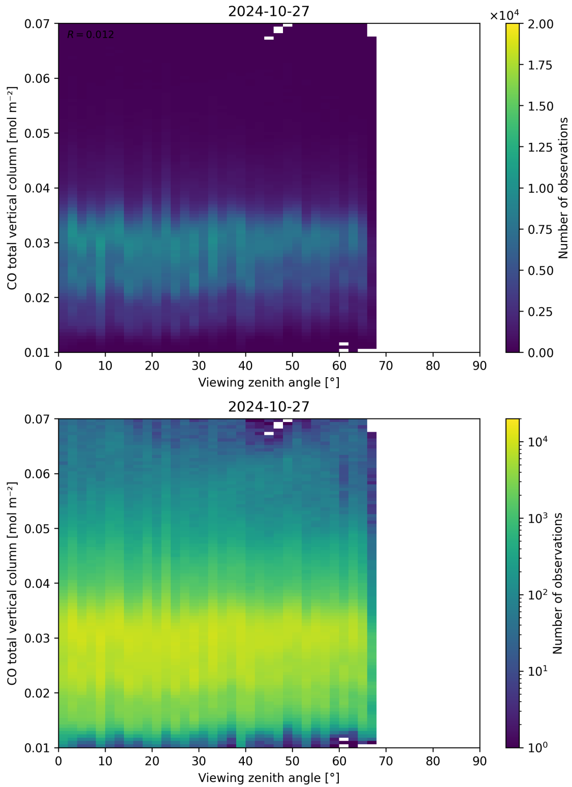
Figure 69: Scatter density plot of “Viewing zenith angle” against “CO total vertical column” for 2024-10-26 to 2024-10-28.
