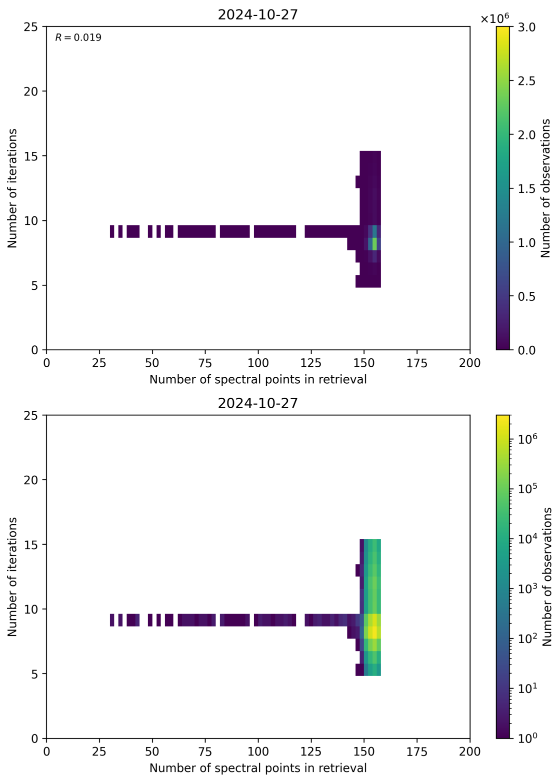
Figure 60: Scatter density plot of “Number of spectral points in retrieval” against “Number of iterations” for 2024-10-26 to 2024-10-28.
