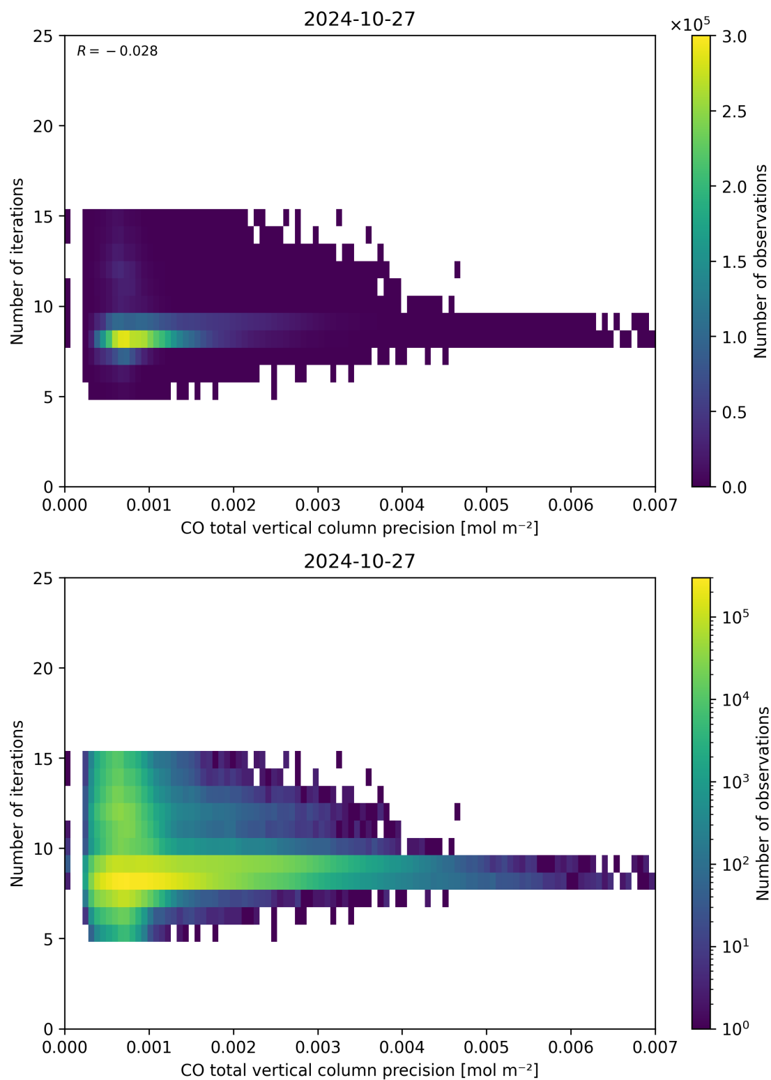
Figure 46: Scatter density plot of “CO total vertical column precision” against “Number of iterations” for 2024-10-26 to 2024-10-28.
