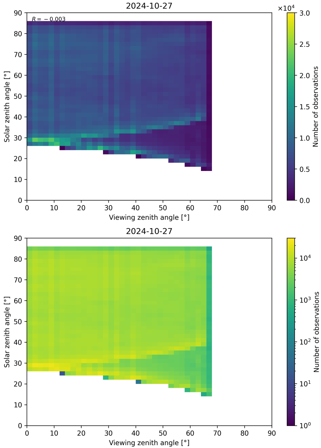
Figure 77: Scatter density plot of “Viewing zenith angle” against “Solar zenith angle” for 2024-10-26 to 2024-10-28.
