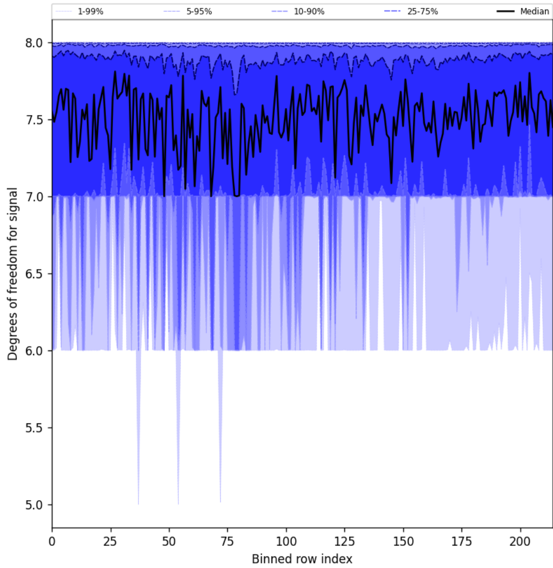
Figure 31: Along track statistics of “Degrees of freedom for signal” for 2024-10-26 to 2024-10-28
