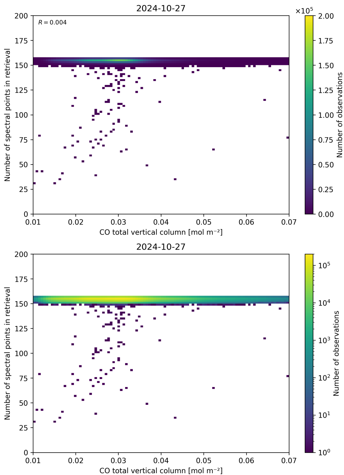
Figure 43: Scatter density plot of “CO total vertical column” against “Number of spectral points in retrieval” for 2024-10-26 to 2024-10-28.
