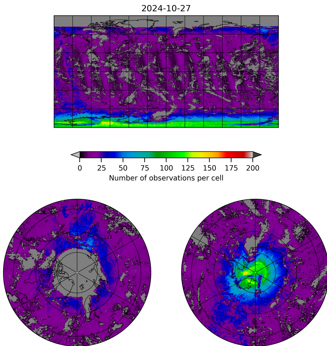
Figure 8: Map of the number of observations for 2024-10-26 to 2024-10-28
