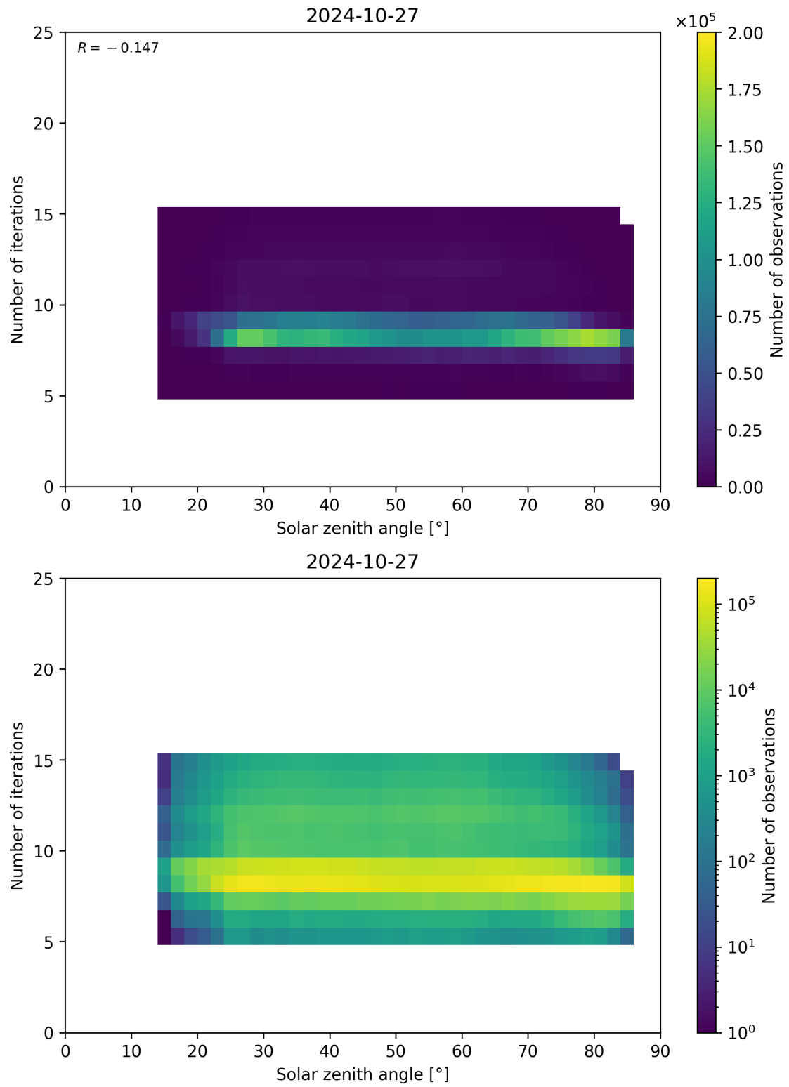
Figure 67: Scatter density plot of “Solar zenith angle” against “Number of iterations” for 2024-10-26 to 2024-10-28.
