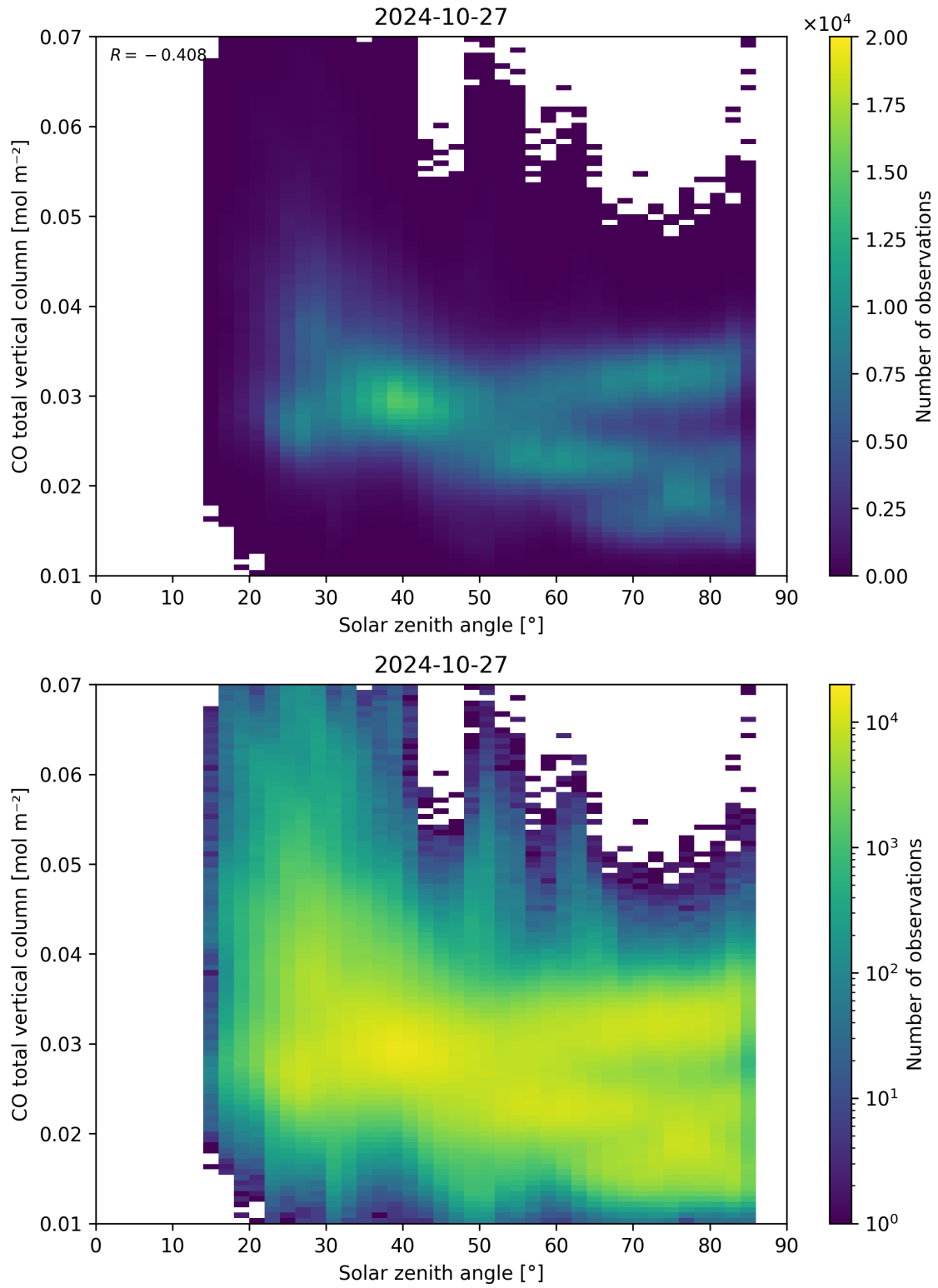
Figure 61: Scatter density plot of “Solar zenith angle” against “CO total vertical column” for 2024-10-26 to 2024-10-28.
