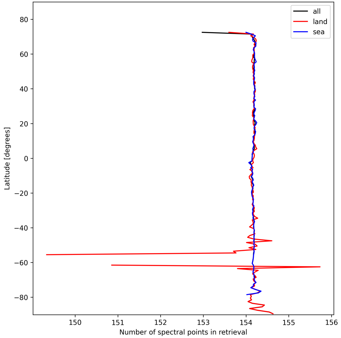
Figure 13: Zonal average of “Number of spectral points in retrieval” for 2024-10-26 to 2024-10-28.
