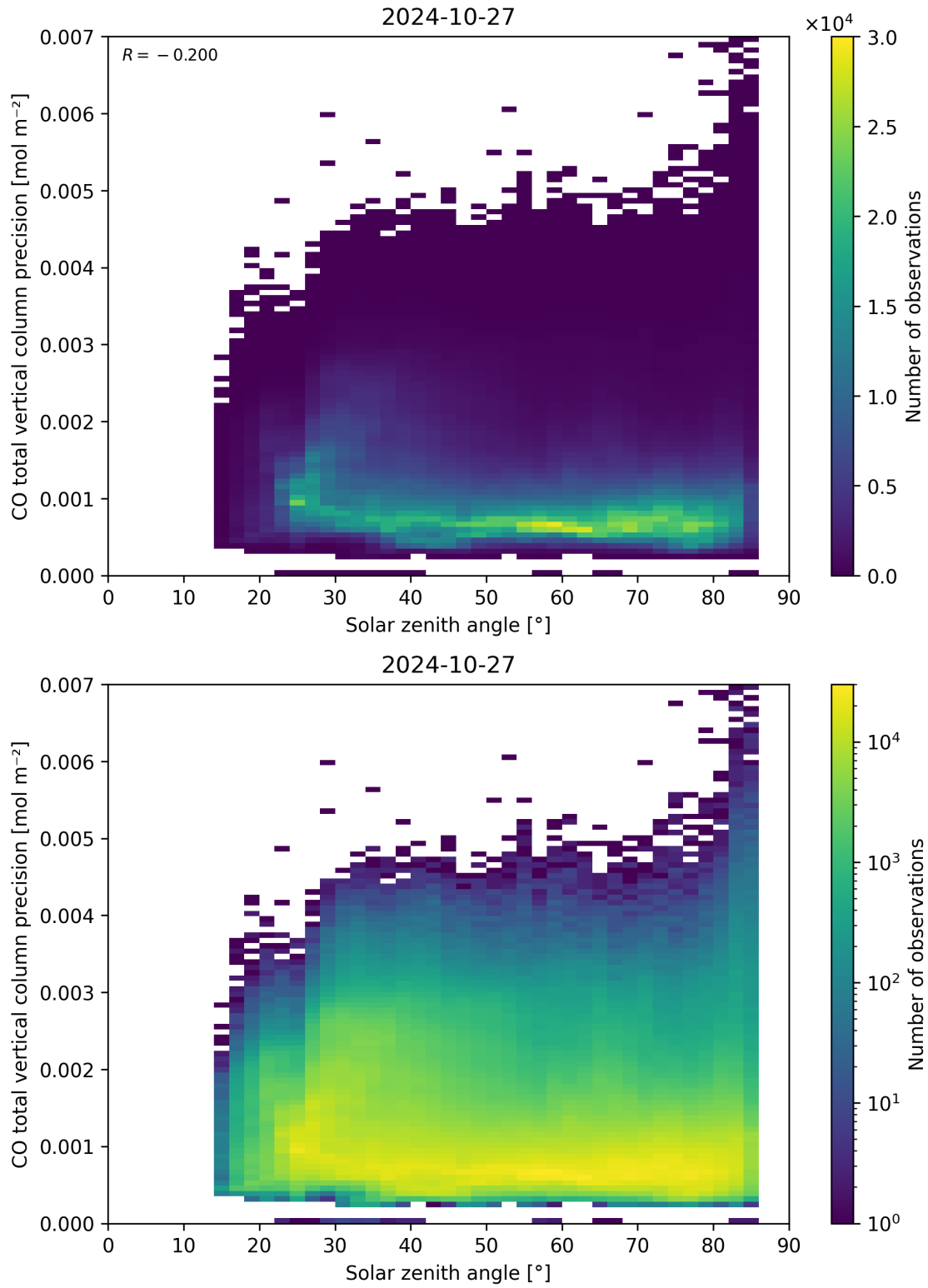
Figure 63: Scatter density plot of “Solar zenith angle” against “CO total vertical column precision” for 2024-10-26 to 2024-10-28.
