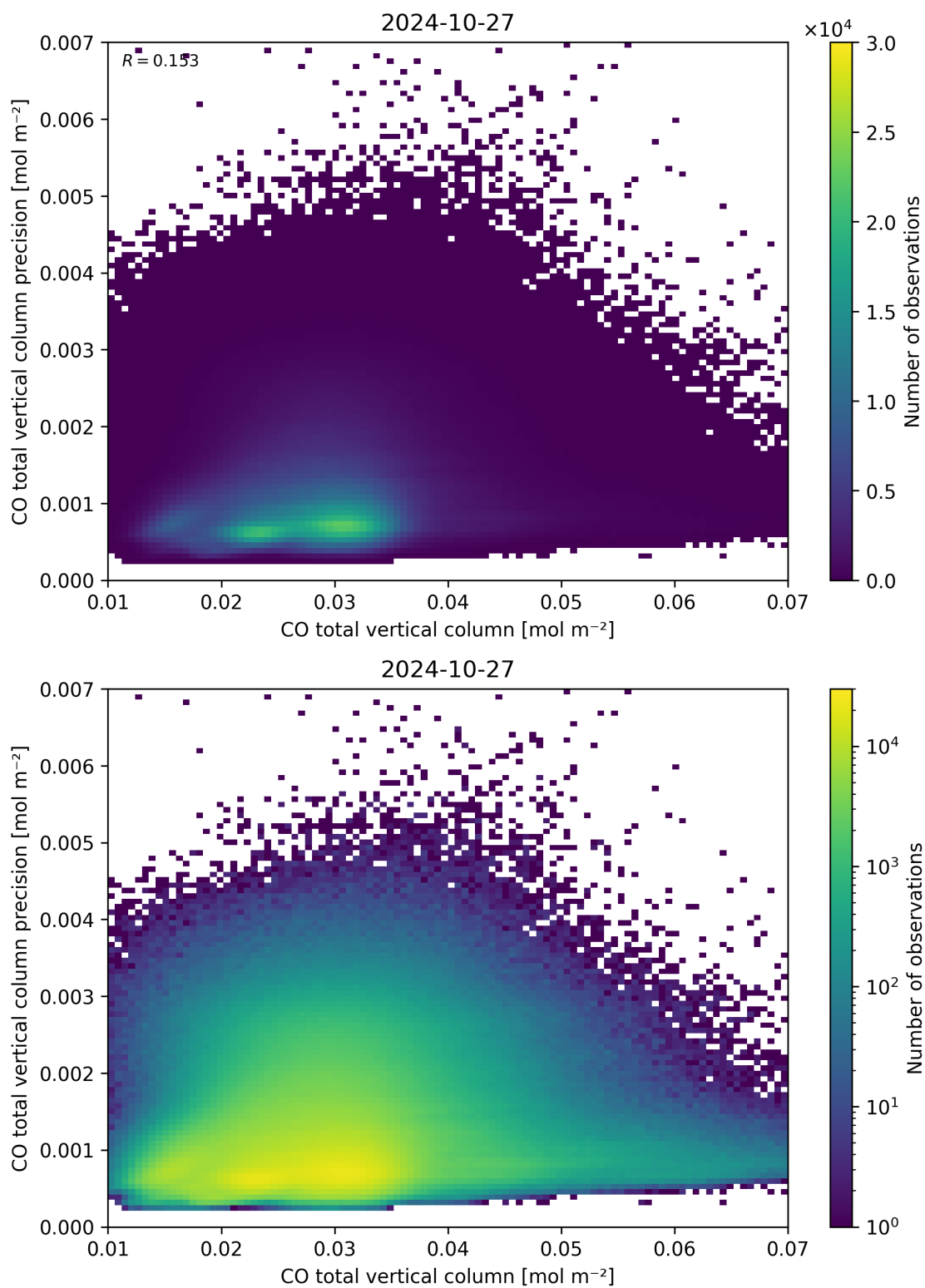
Figure 34: Scatter density plot of “CO total vertical column” against “CO total vertical column precision” for 2024-10-26 to 2024-10-28.
