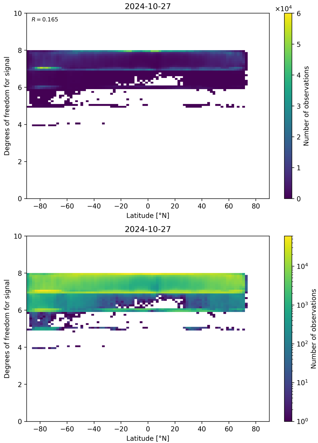
Figure 55: Scatter density plot of “Latitude” against “Degrees of freedom for signal” for 2024-10-26 to 2024-10-28.
