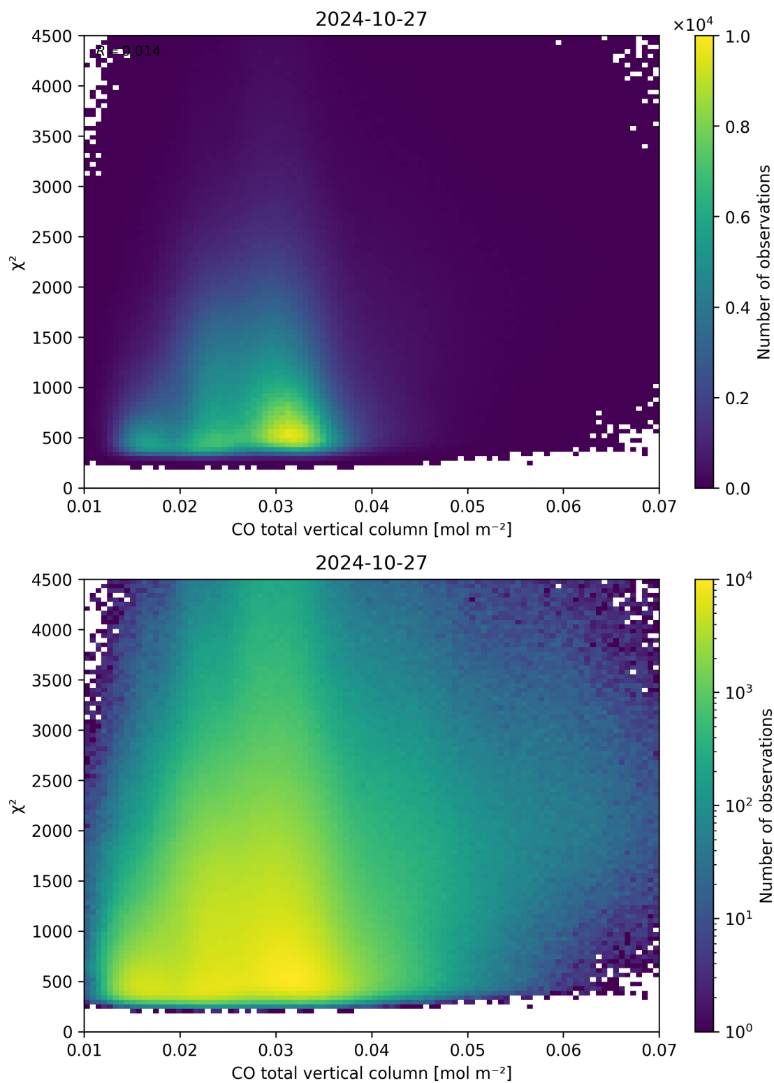
Figure 35: Scatter density plot of “CO total vertical column” against “ \chi^2 ” for 2024-10-26 to 2024-10-28.
