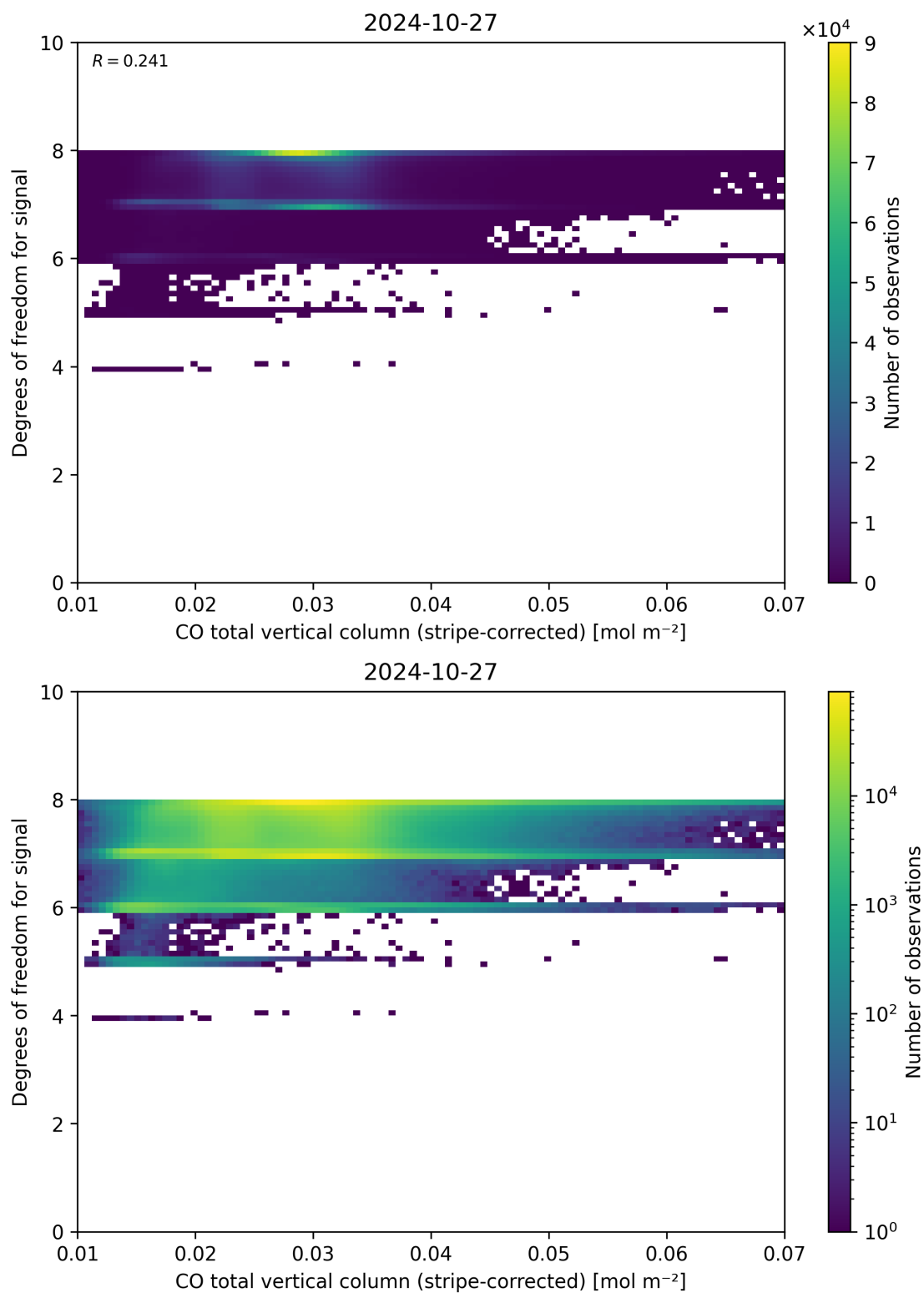
Figure 38: Scatter density plot of “CO total vertical column (stripe-corrected)” against “Degrees of freedom for signal” for 2024-10-26 to 2024-10-28.
