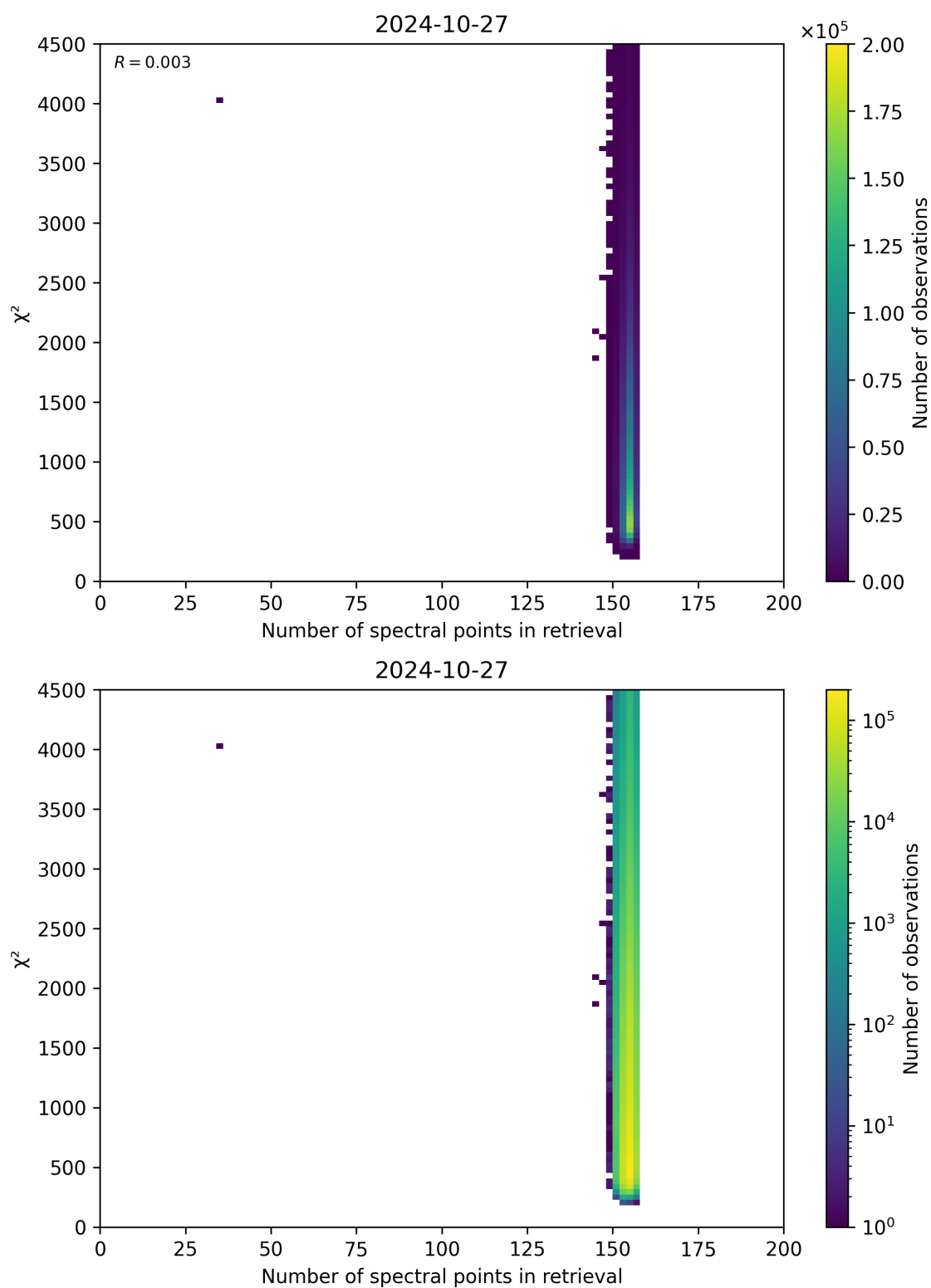
Figure 58: Scatter density plot of “Number of spectral points in retrieval” against “ \chi^2 ” for 2024-10-26 to 2024-10-28.
