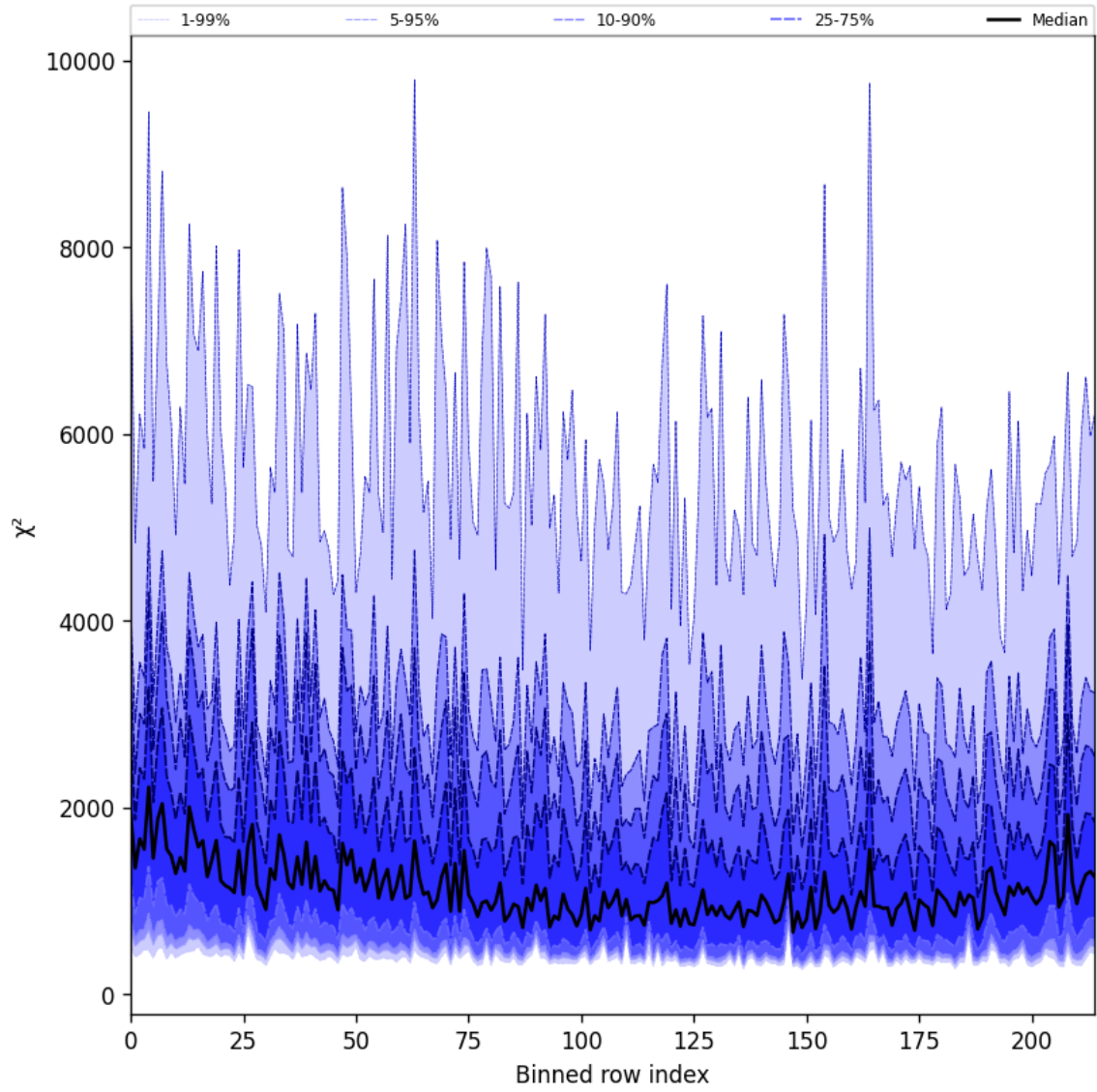
Figure 30: Along track statistics of “ \chi^2 ” for 2024-10-26 to 2024-10-28
