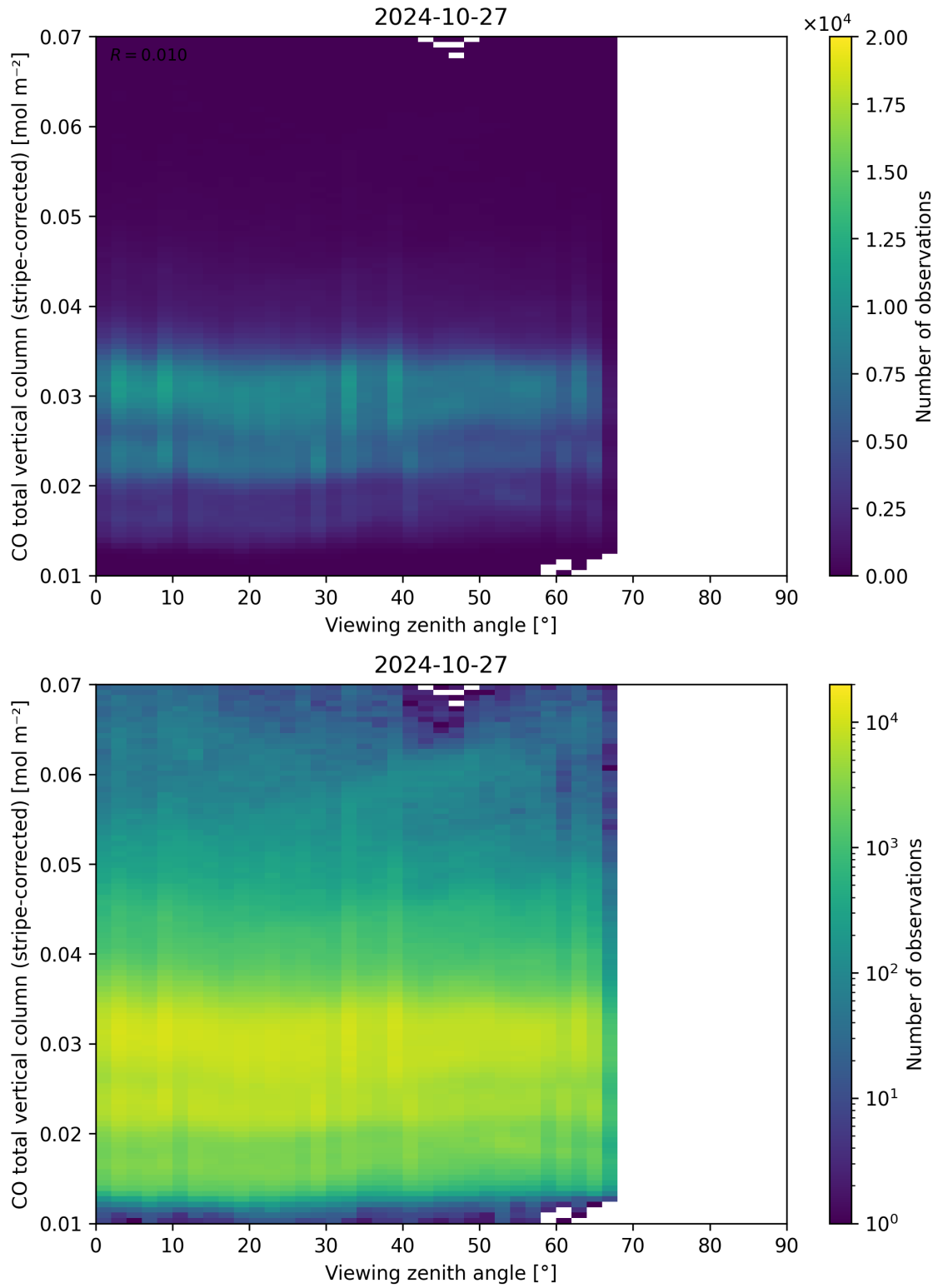
Figure 70: Scatter density plot of “Viewing zenith angle” against “CO total vertical column (stripe-corrected)” for 2024-10-26 to 2024-10-28.
