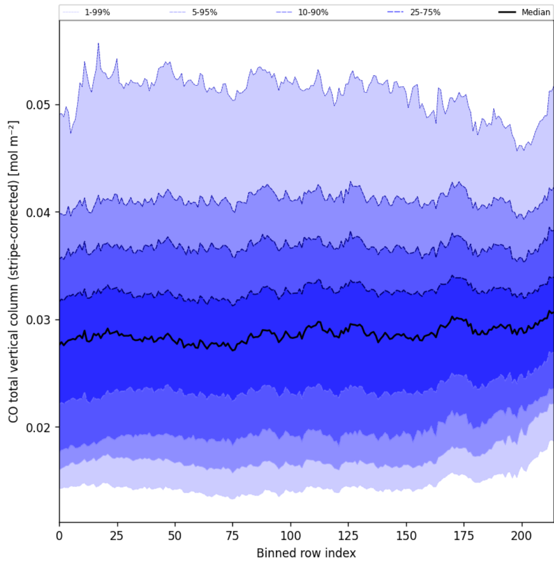
Figure 27: Along track statistics of “CO total vertical column (stripe-corrected)” for 2024-10-26 to 2024-10-28
