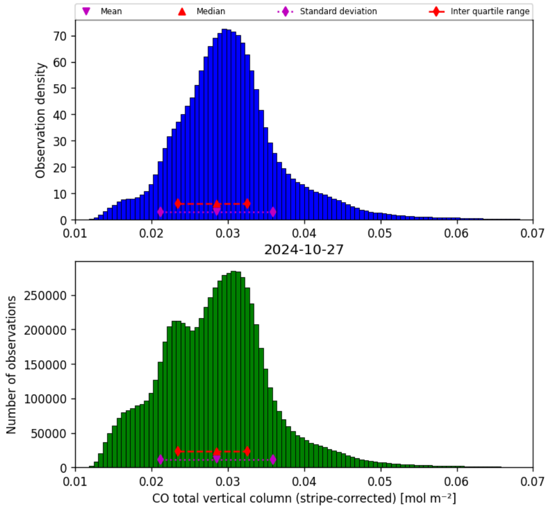
Figure 19: Histogram of “CO total vertical column (stripe-corrected)” for 2024-10-26 to 2024-10-28
