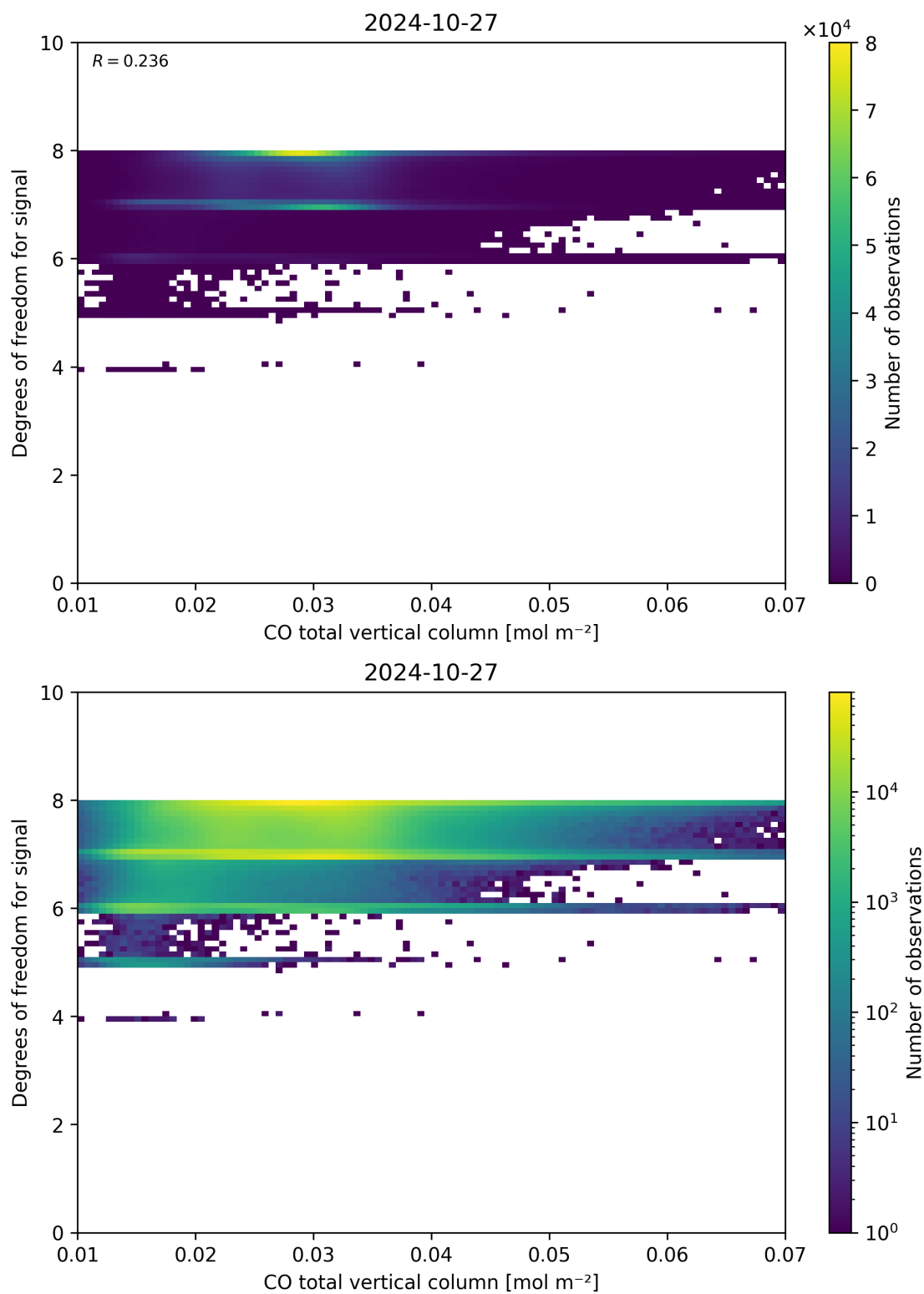
Figure 41: Scatter density plot of “CO total vertical column” against “Degrees of freedom for signal” for 2024-10-26 to 2024-10-28.
