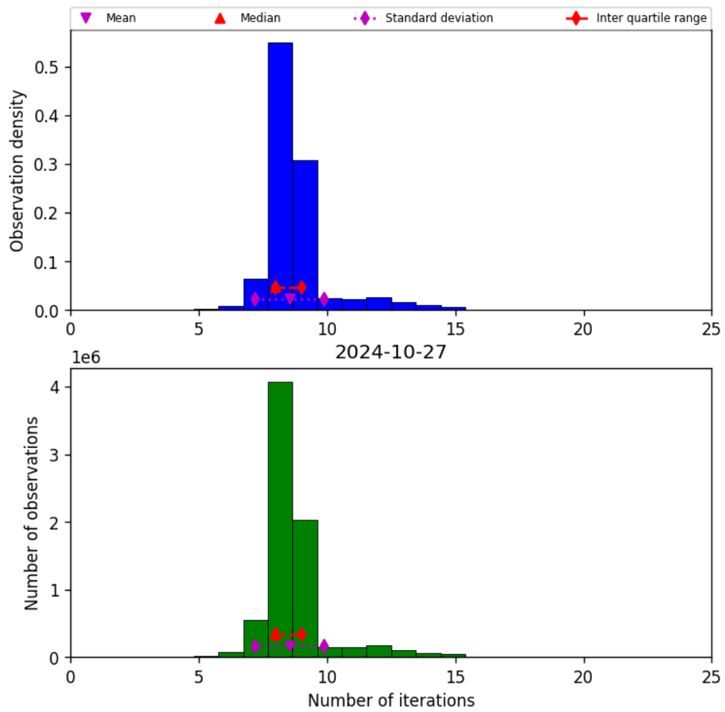
Figure 24: Histogram of “Number of iterations” for 2024-10-26 to 2024-10-28
