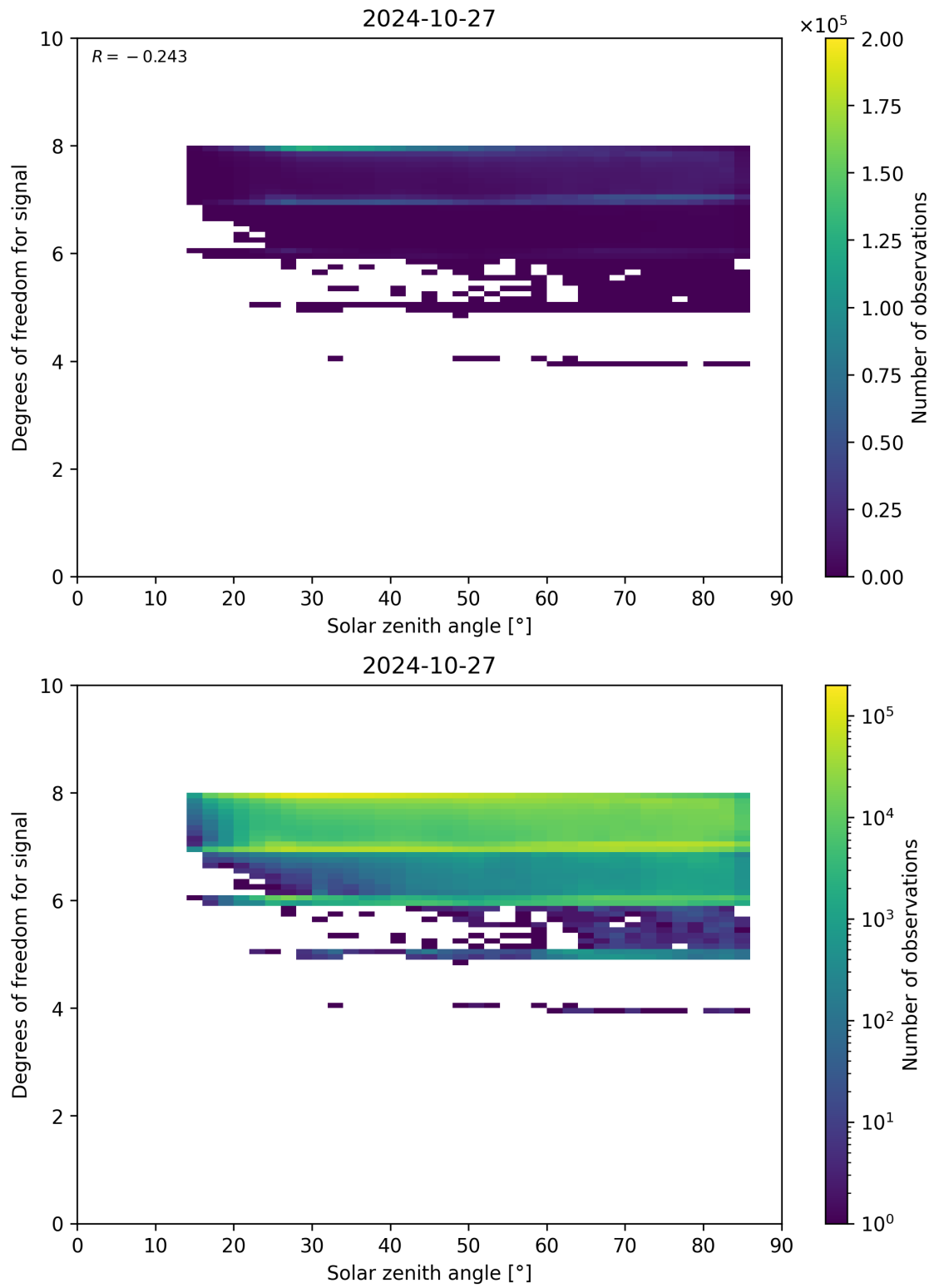
Figure 65: Scatter density plot of “Solar zenith angle” against “Degrees of freedom for signal” for 2024-10-26 to 2024-10-28.
