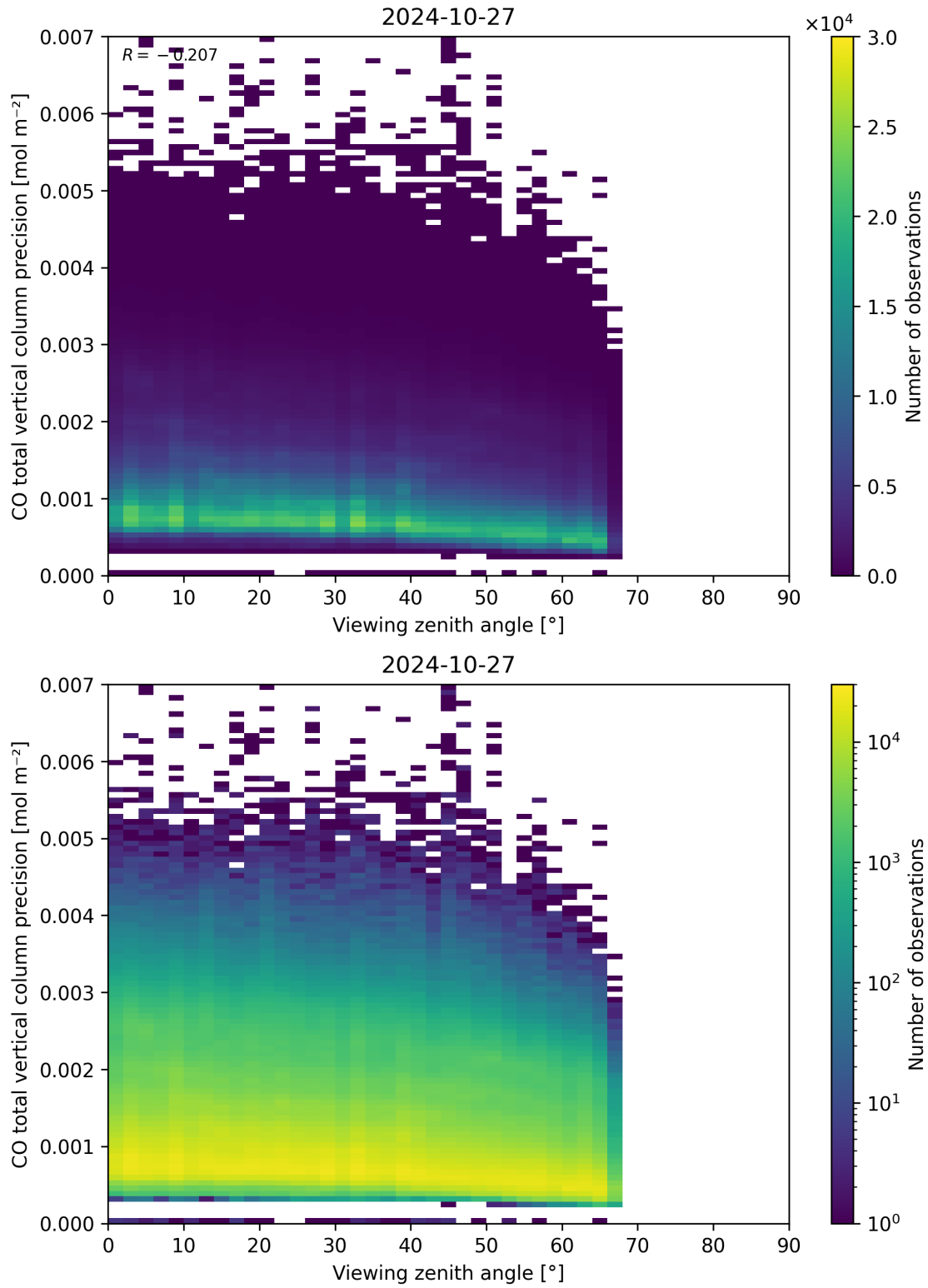
Figure 71: Scatter density plot of “Viewing zenith angle” against “CO total vertical column precision” for 2024-10-26 to 2024-10-28.
