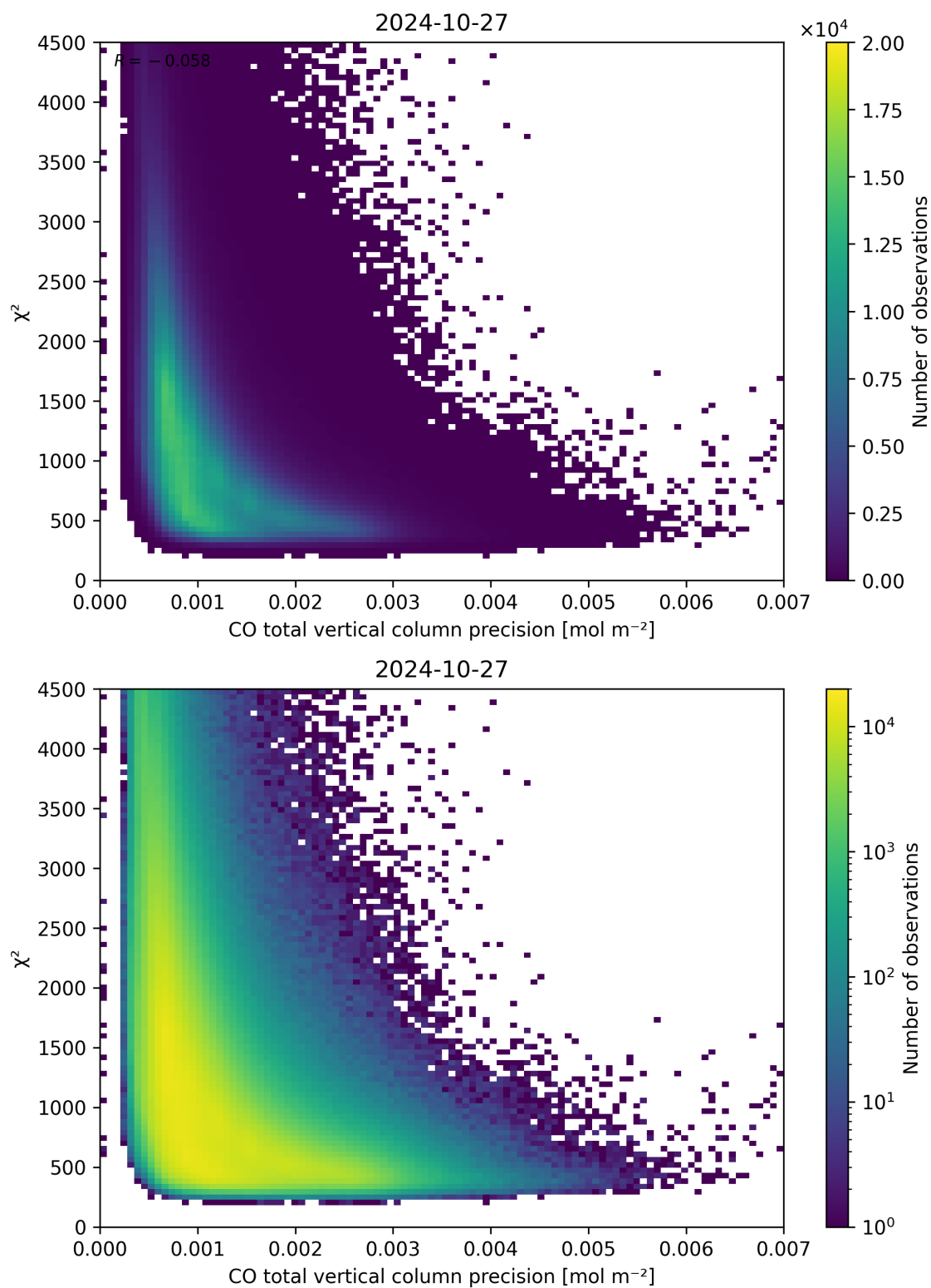
Figure 44: Scatter density plot of “CO total vertical column precision” against “ \chi^2 ” for 2024-10-26 to 2024-10-28.
