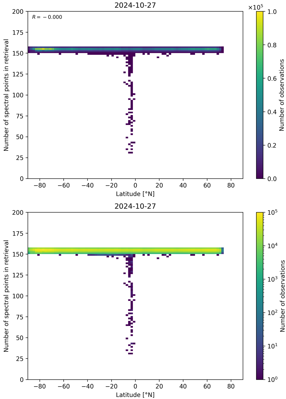
Figure 57: Scatter density plot of “Latitude” against “Number of spectral points in retrieval” for 2024-10-26 to 2024-10-28.
