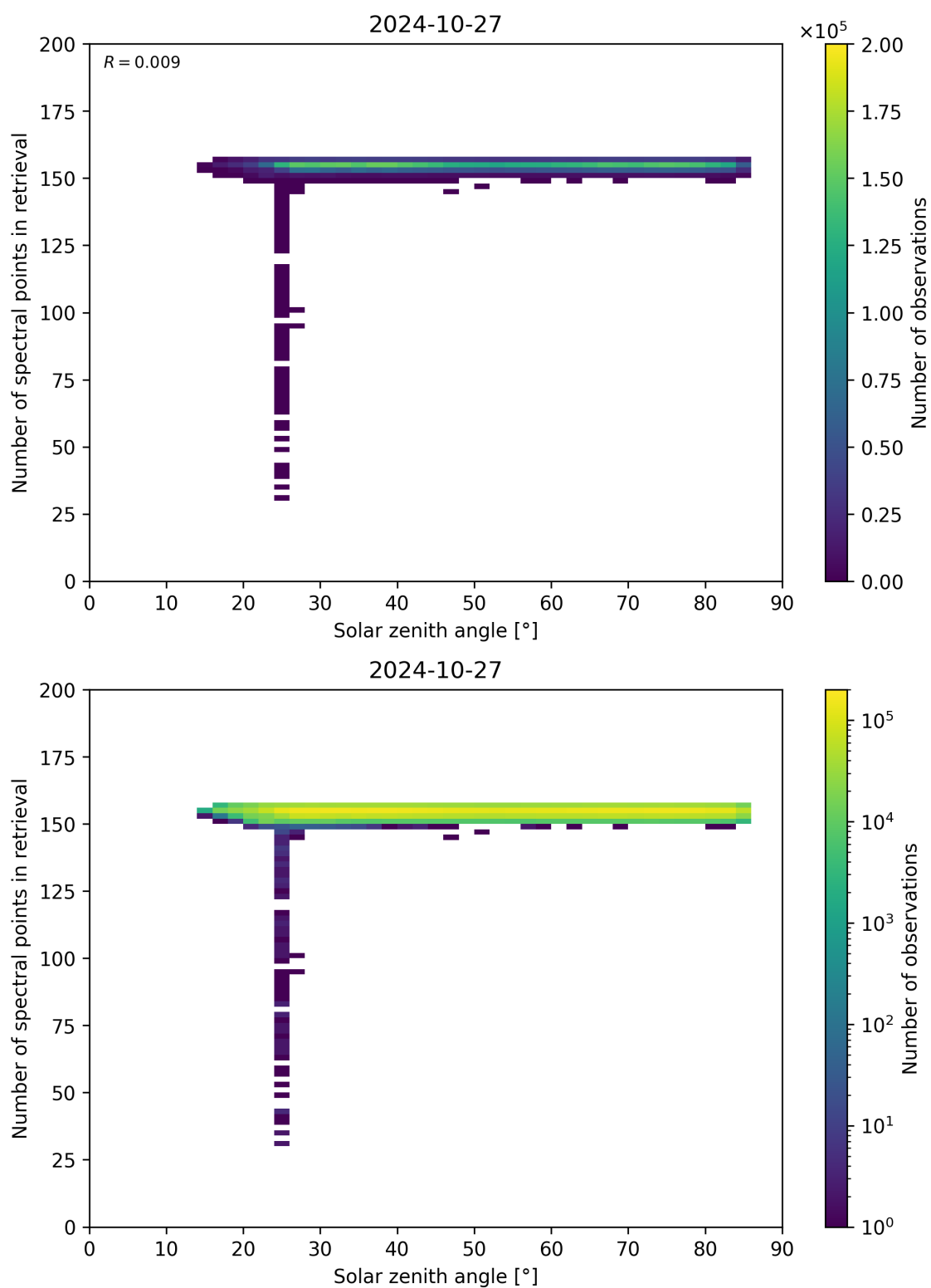
Figure 68: Scatter density plot of “Solar zenith angle” against “Number of spectral points in retrieval” for 2024-10-26 to 2024-10-28.
