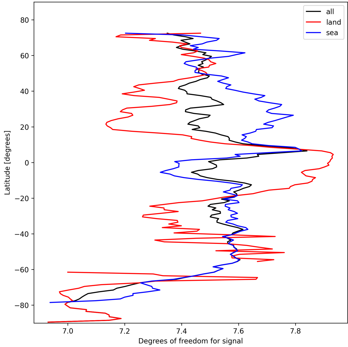
Figure 15: Zonal average of “Degrees of freedom for signal” for 2024-10-26 to 2024-10-28.
