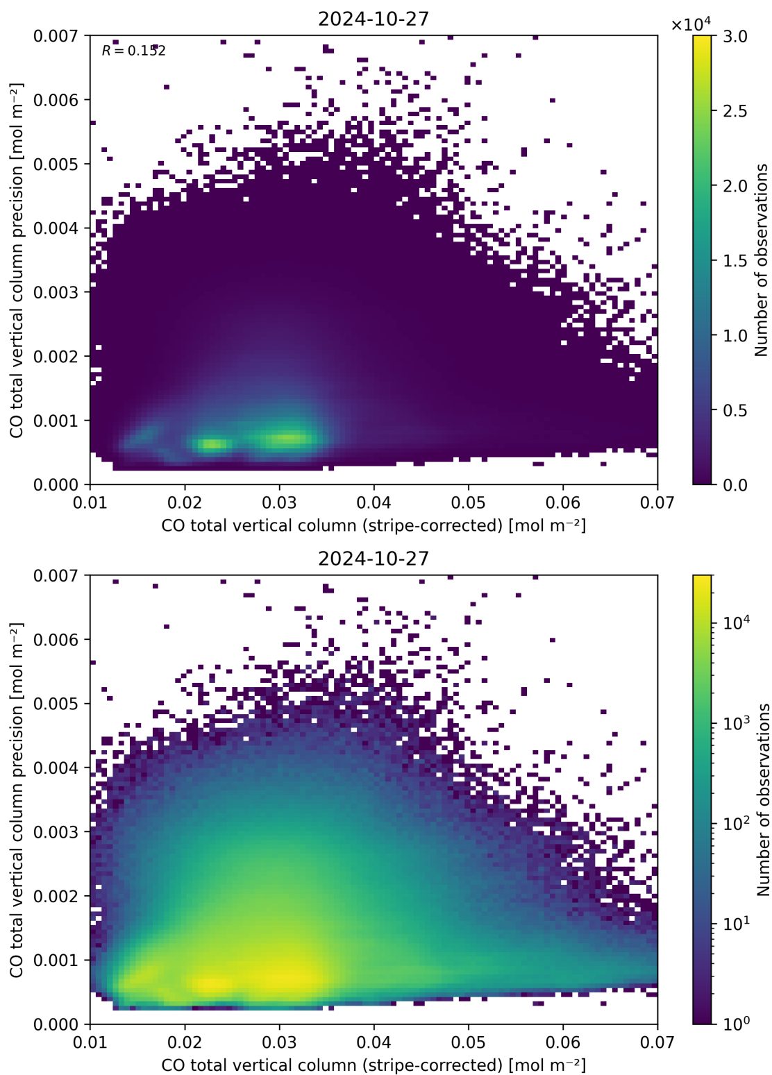
Figure 36: Scatter density plot of “CO total vertical column (stripe-corrected)” against “CO total vertical column precision” for 2024-10-26 to 2024-10-28.
