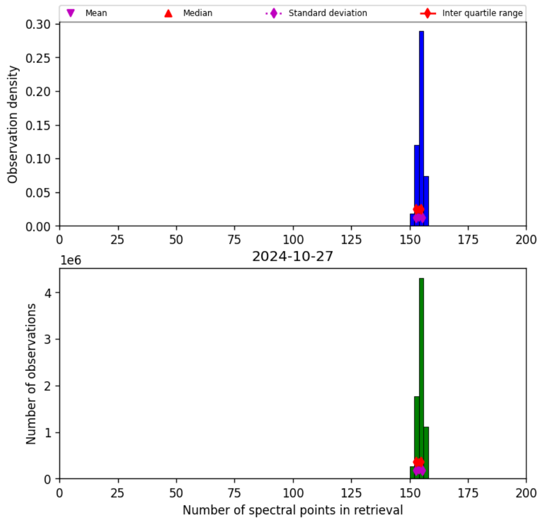
Figure 21: Histogram of “Number of spectral points in retrieval” for 2024-10-26 to 2024-10-28
