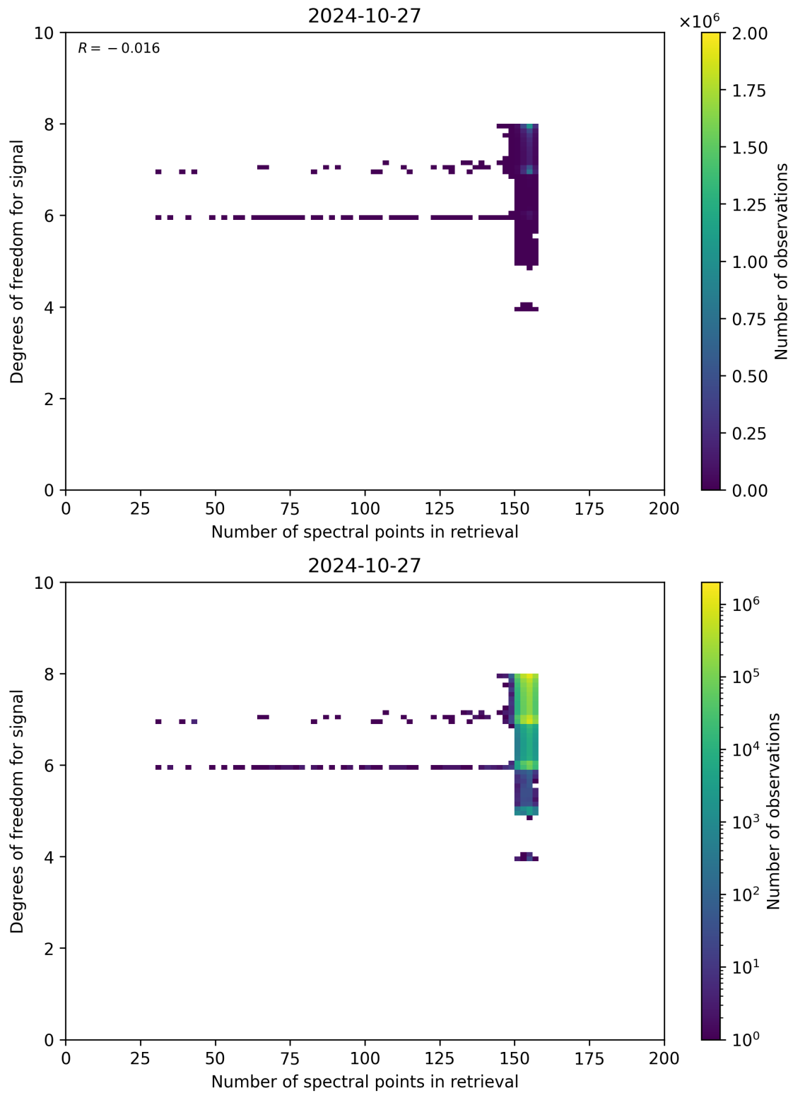
Figure 59: Scatter density plot of “Number of spectral points in retrieval” against “Degrees of freedom for signal” for 2024-10-26 to 2024-10-28.
