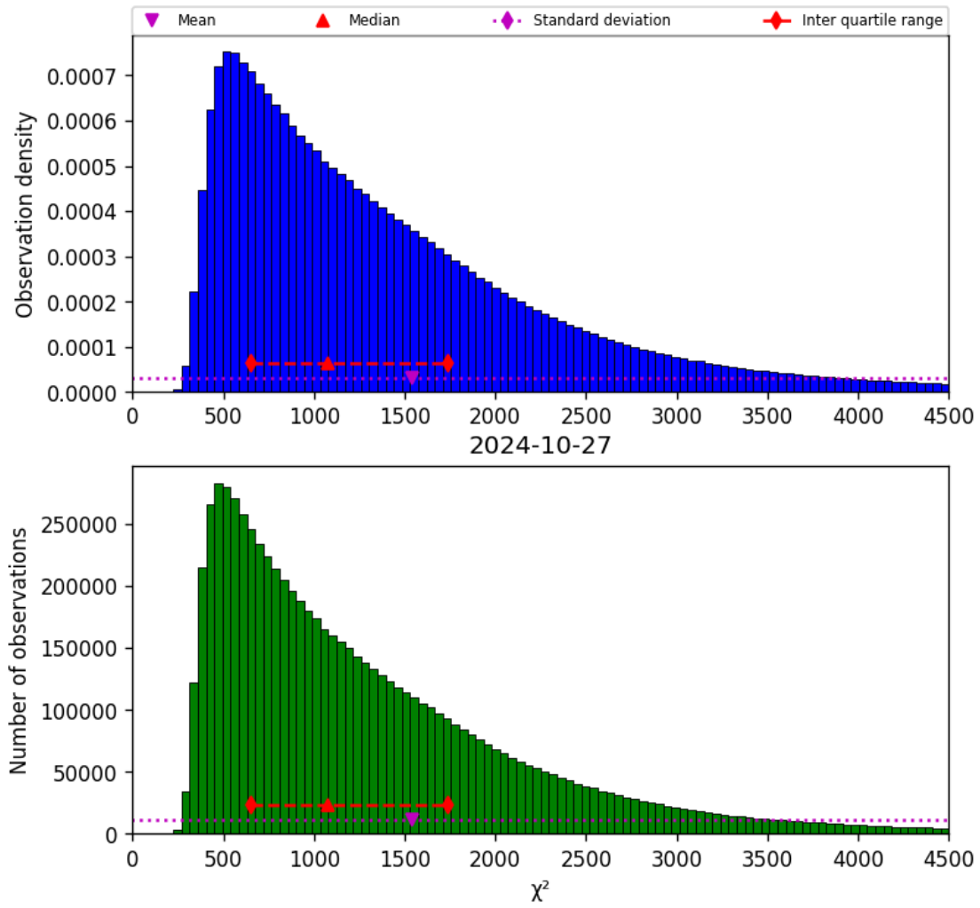
Figure 22: Histogram of “ \chi^2 ” for 2024-10-26 to 2024-10-28
