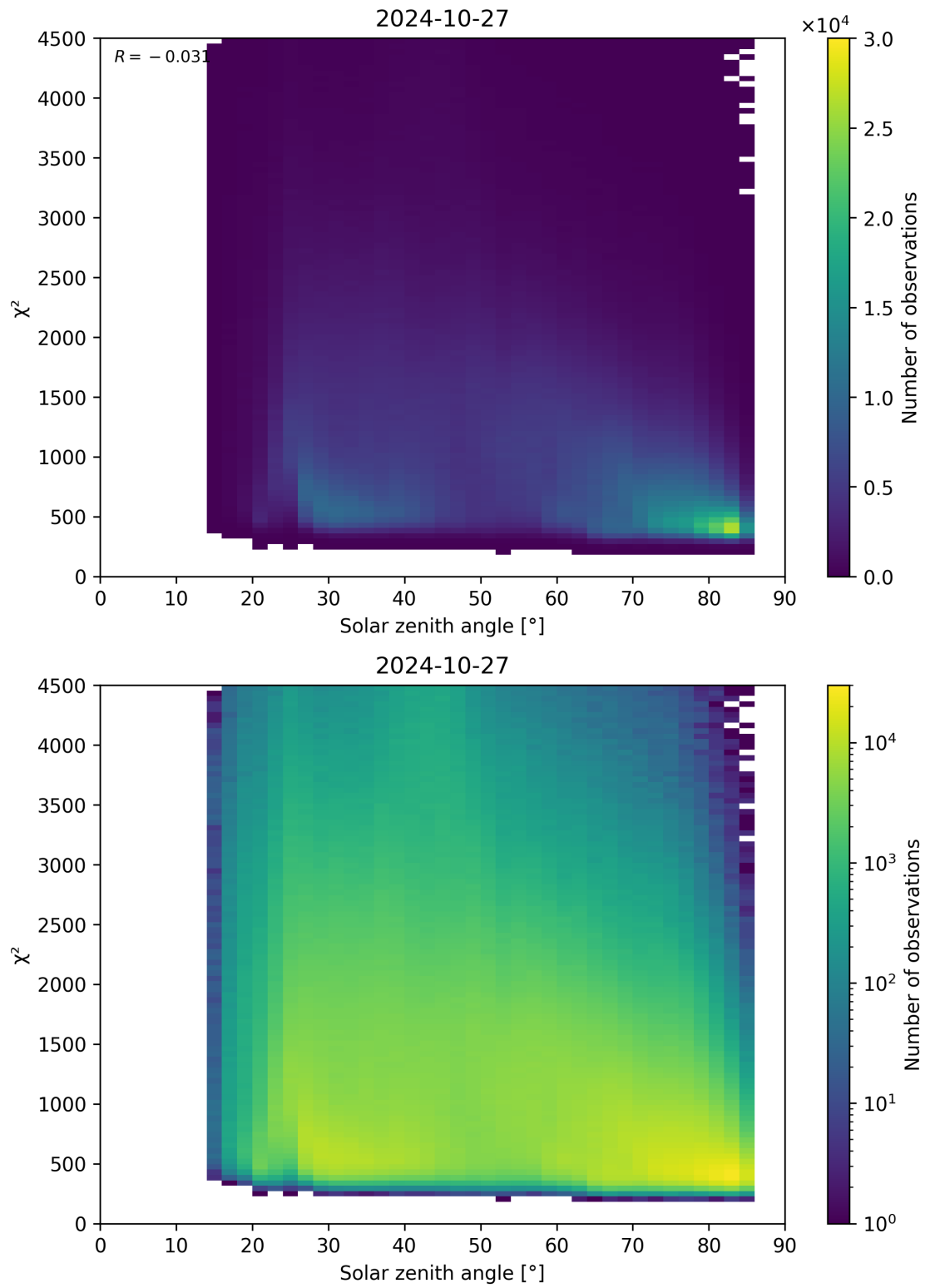
Figure 64: Scatter density plot of “Solar zenith angle” against “ \chi^2 ” for 2024-10-26 to 2024-10-28.
