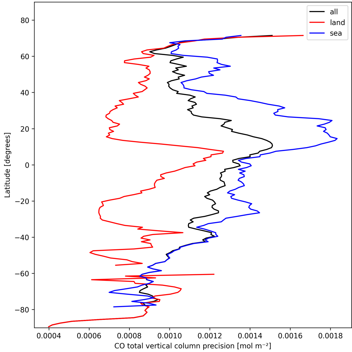
Figure 12: Zonal average of “CO total vertical column precision” for 2024-10-27 to 2024-10-29.
