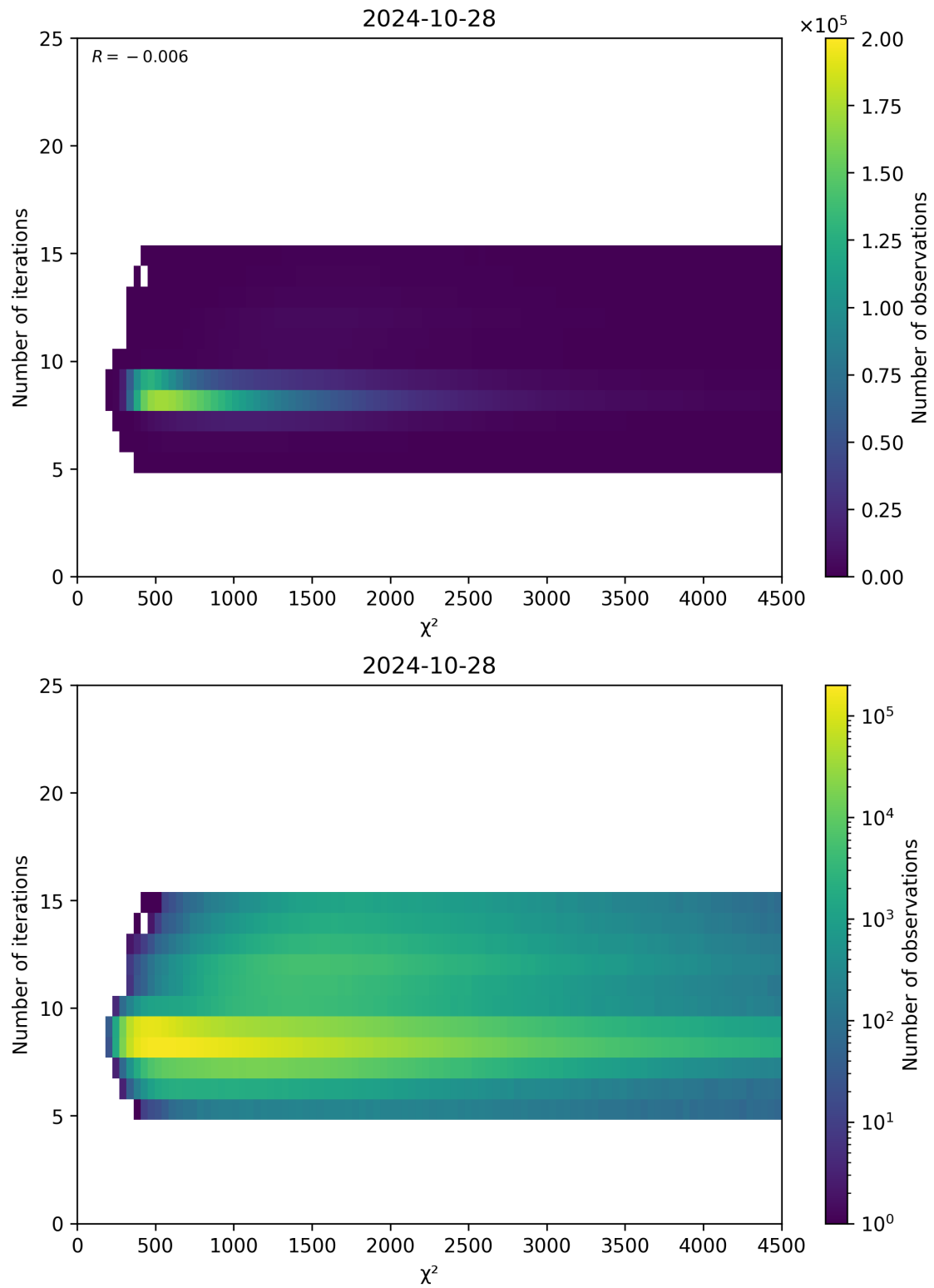
Figure 49: Scatter density plot of “ \chi^2 ” against “Number of iterations” for 2024-10-27 to 2024-10-29.
