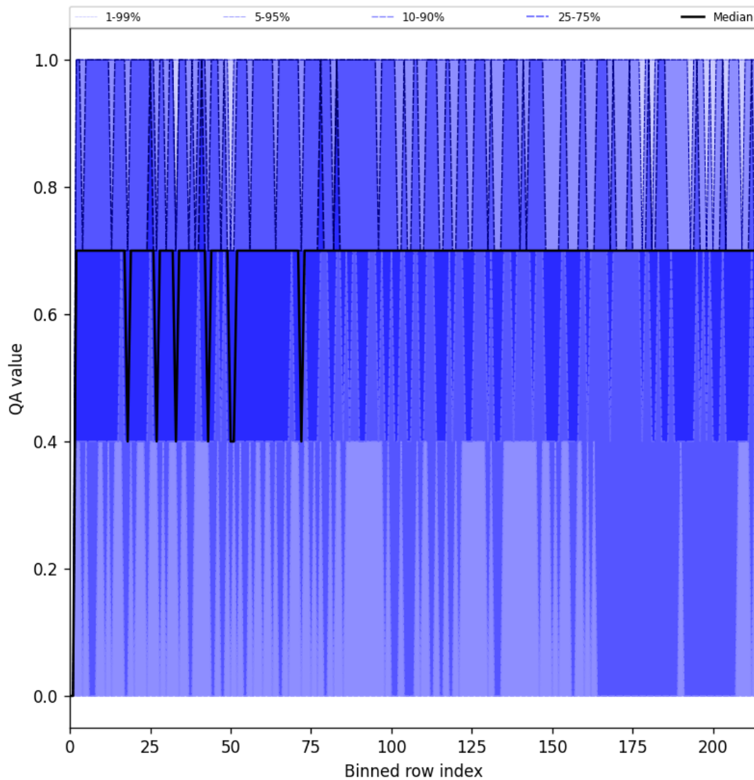
Figure 25: Along track statistics of “QA value” for 2024-10-27 to 2024-10-29
