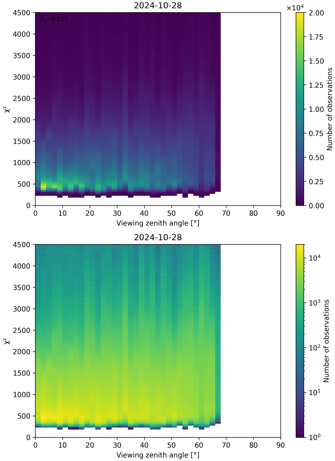
Figure 72: Scatter density plot of “Viewing zenith angle” against “ \chi^2 ” for 2024-10-27 to 2024-10-29.
