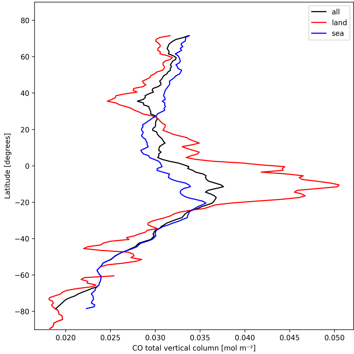
Figure 10: Zonal average of “CO total vertical column” for 2024-10-27 to 2024-10-29.
