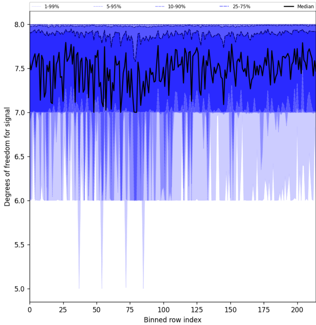
Figure 31: Along track statistics of “Degrees of freedom for signal” for 2024-10-27 to 2024-10-29
