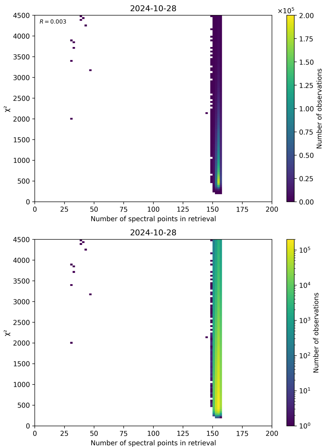
Figure 58: Scatter density plot of “Number of spectral points in retrieval” against “ \chi^2 ” for 2024-10-27 to 2024-10-29.
