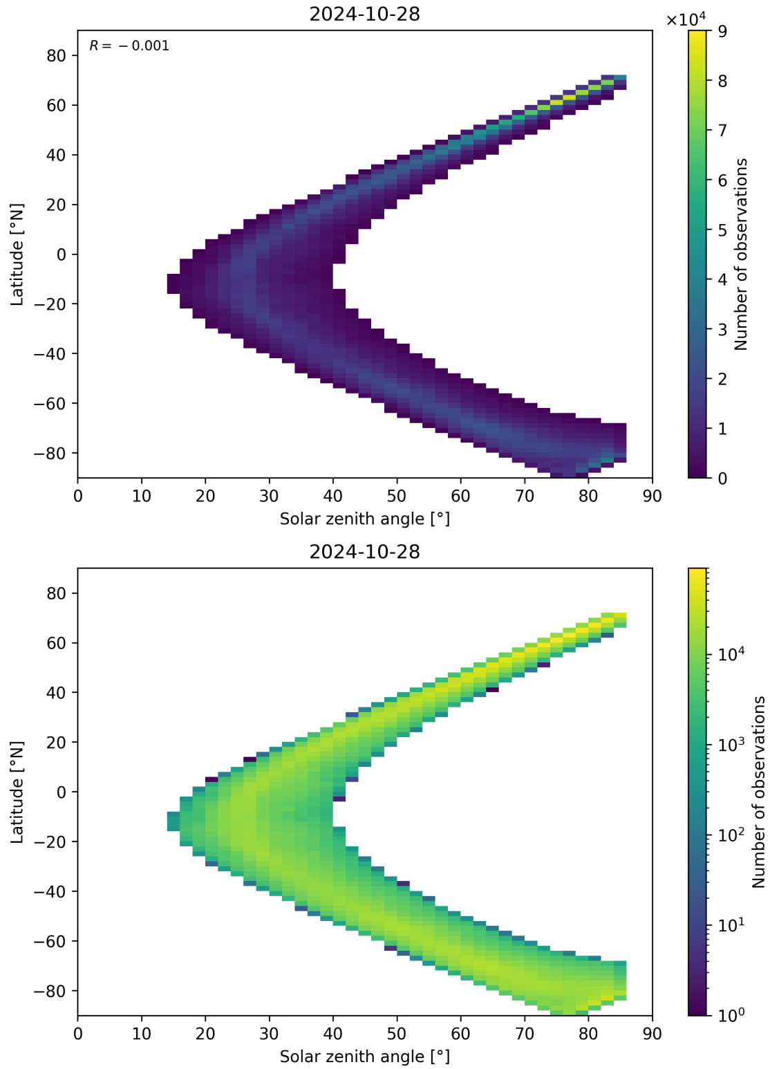
Figure 66: Scatter density plot of “Solar zenith angle” against “Latitude” for 2024-10-27 to 2024-10-29.
