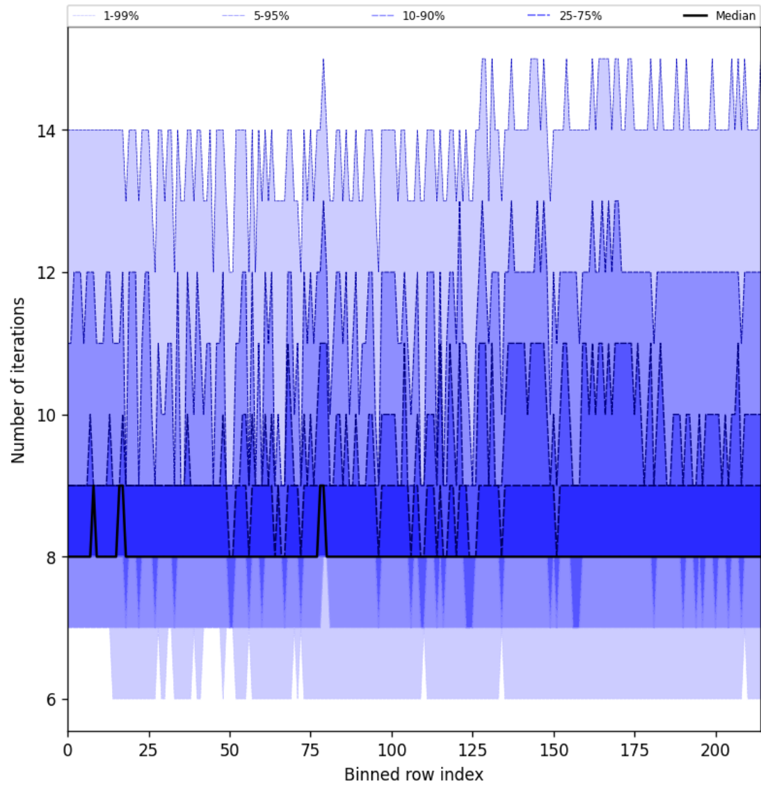
Figure 32: Along track statistics of “Number of iterations” for 2024-10-27 to 2024-10-29
