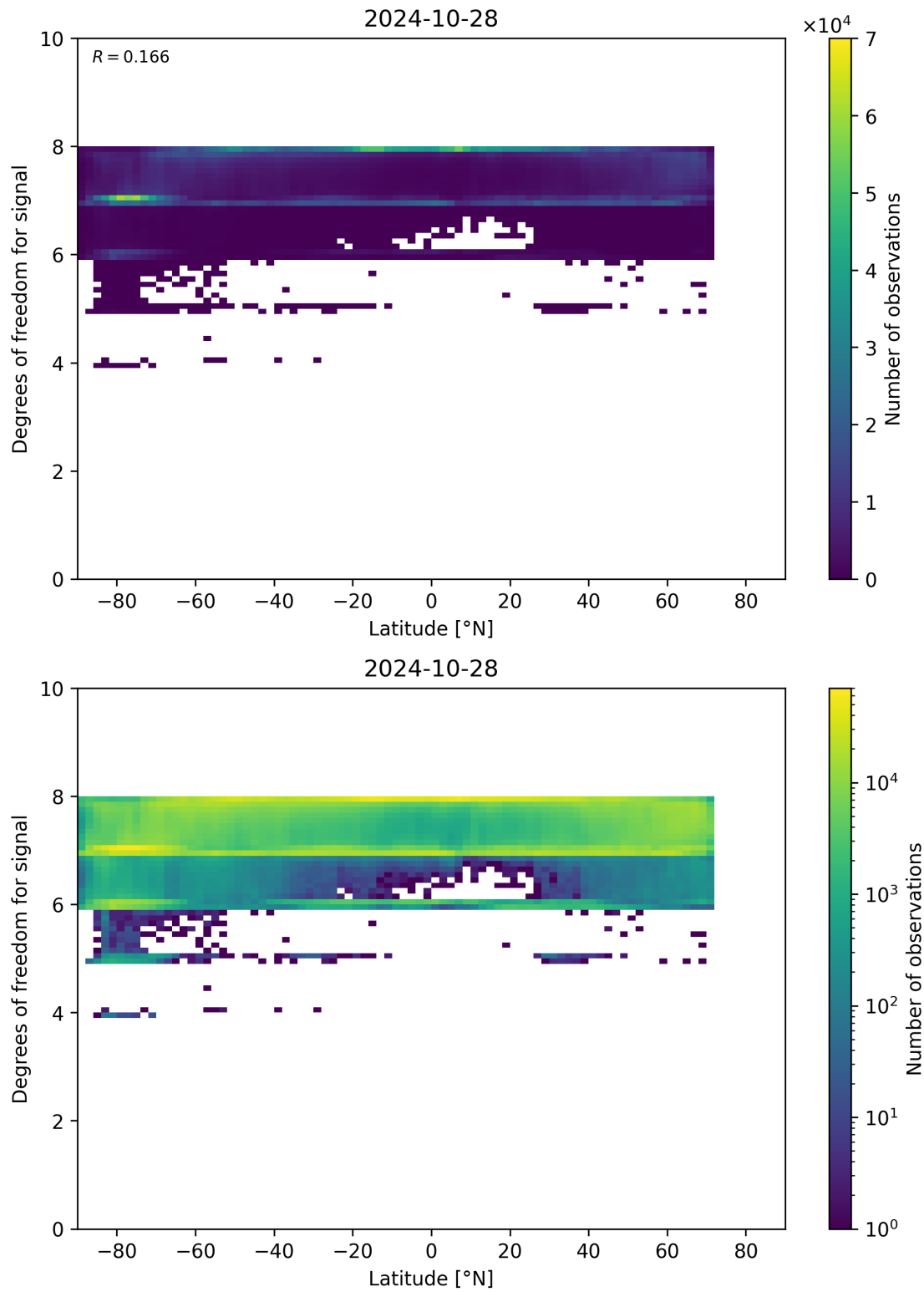
Figure 55: Scatter density plot of “Latitude” against “Degrees of freedom for signal” for 2024-10-27 to 2024-10-29.
