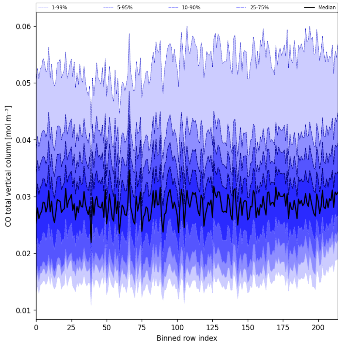
Figure 26: Along track statistics of “CO total vertical column” for 2024-10-27 to 2024-10-29
