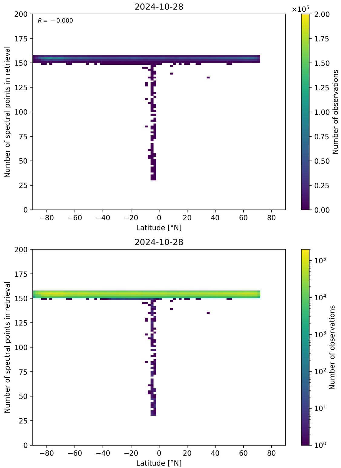
Figure 57: Scatter density plot of “Latitude” against “Number of spectral points in retrieval” for 2024-10-27 to 2024-10-29.
