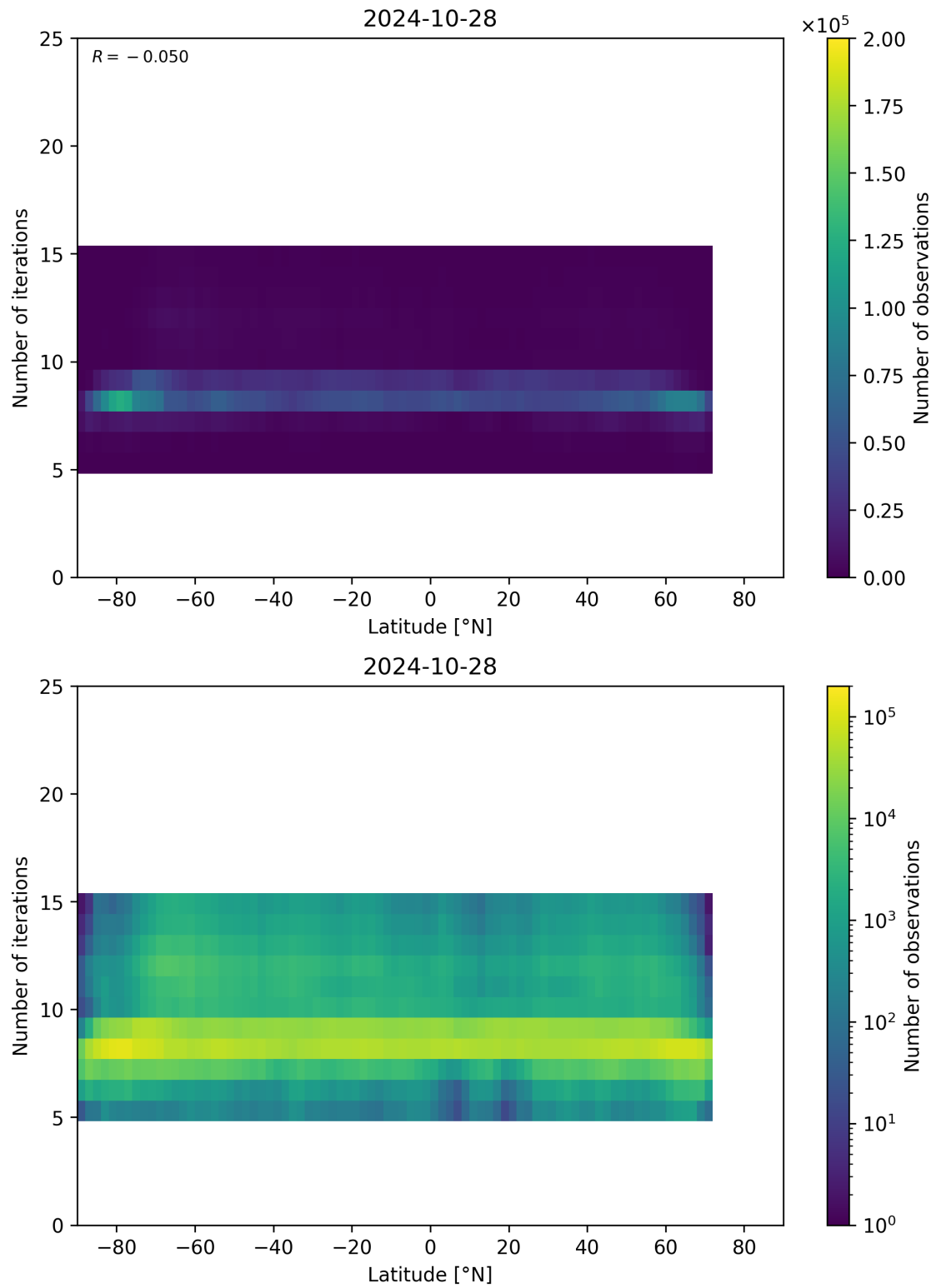
Figure 56: Scatter density plot of “Latitude” against “Number of iterations” for 2024-10-27 to 2024-10-29.
