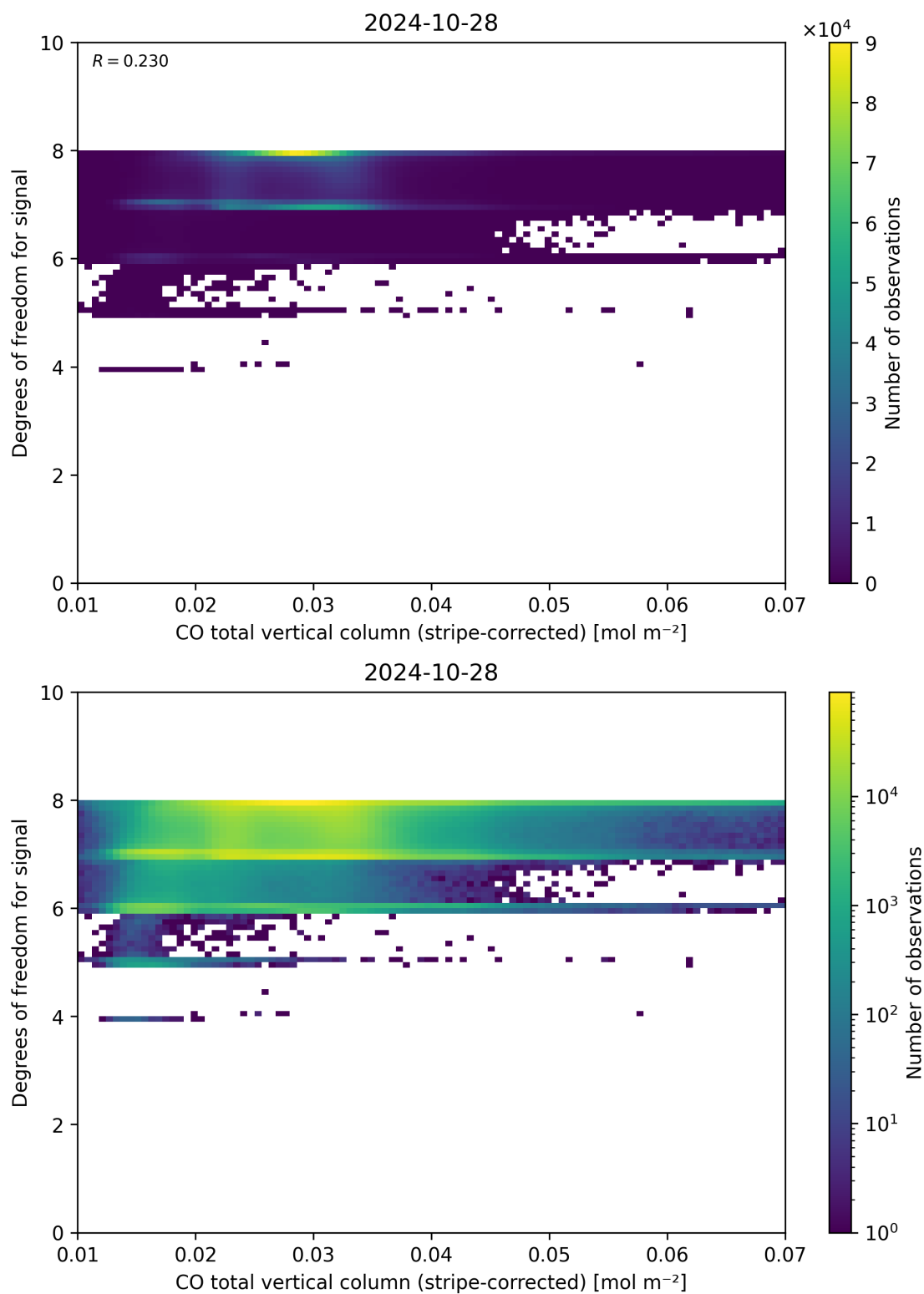
Figure 38: Scatter density plot of “CO total vertical column (stripe-corrected)” against “Degrees of freedom for signal” for 2024-10-27 to 2024-10-29.
