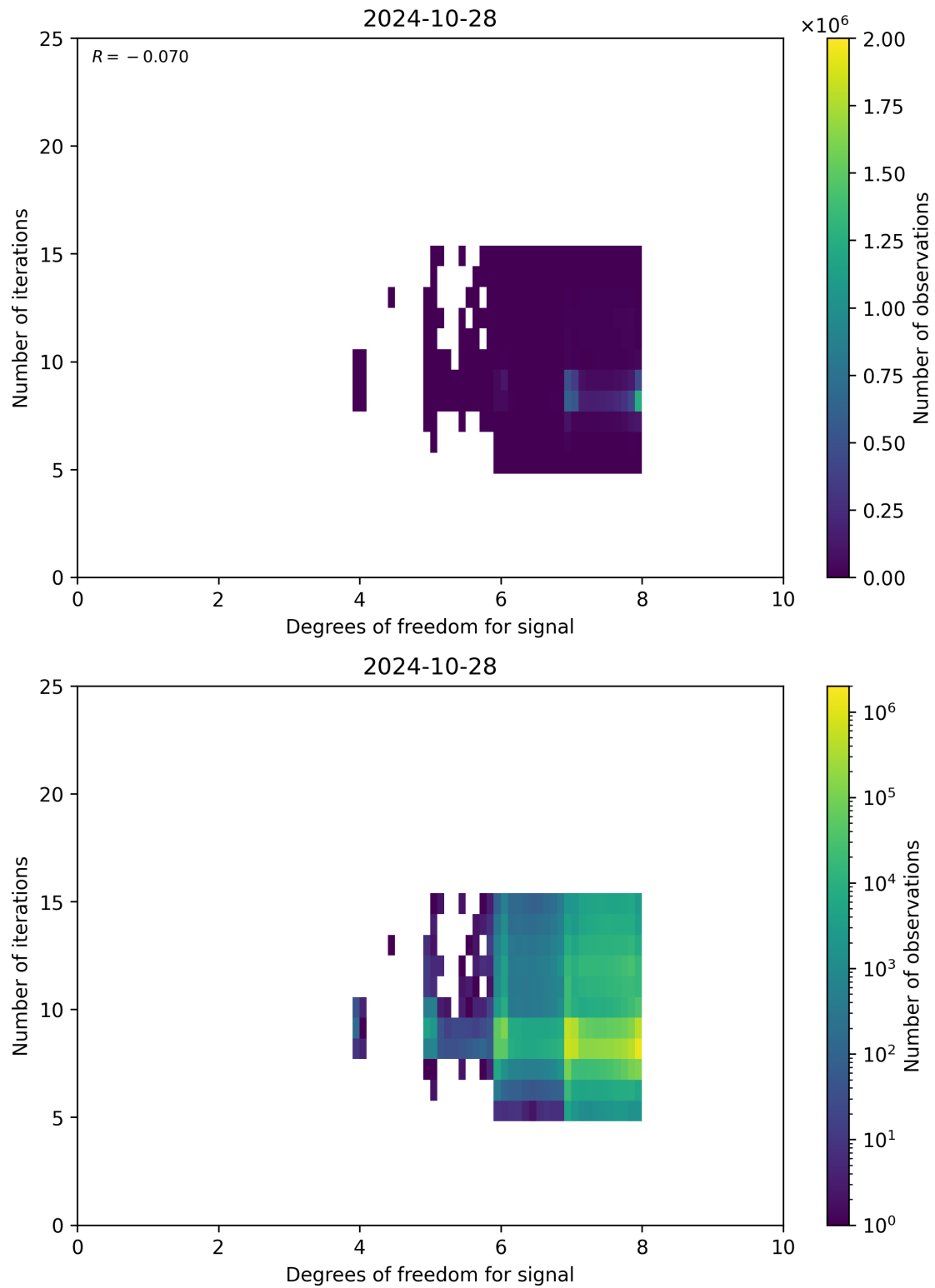
Figure 50: Scatter density plot of “Degrees of freedom for signal” against “Number of iterations” for 2024-10-27 to 2024-10-29.
