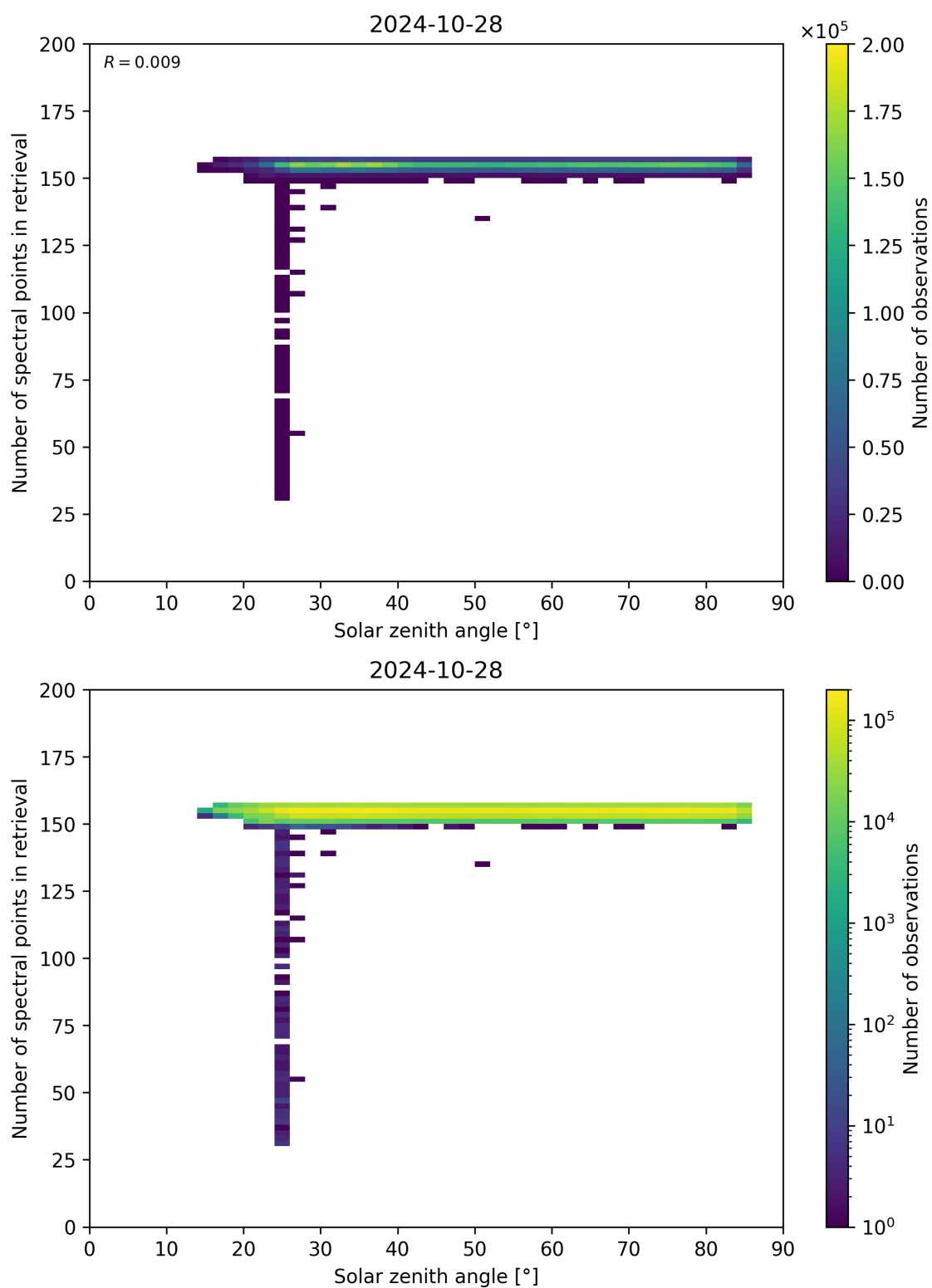
Figure 68: Scatter density plot of “Solar zenith angle” against “Number of spectral points in retrieval” for 2024-10-27 to 2024-10-29.
