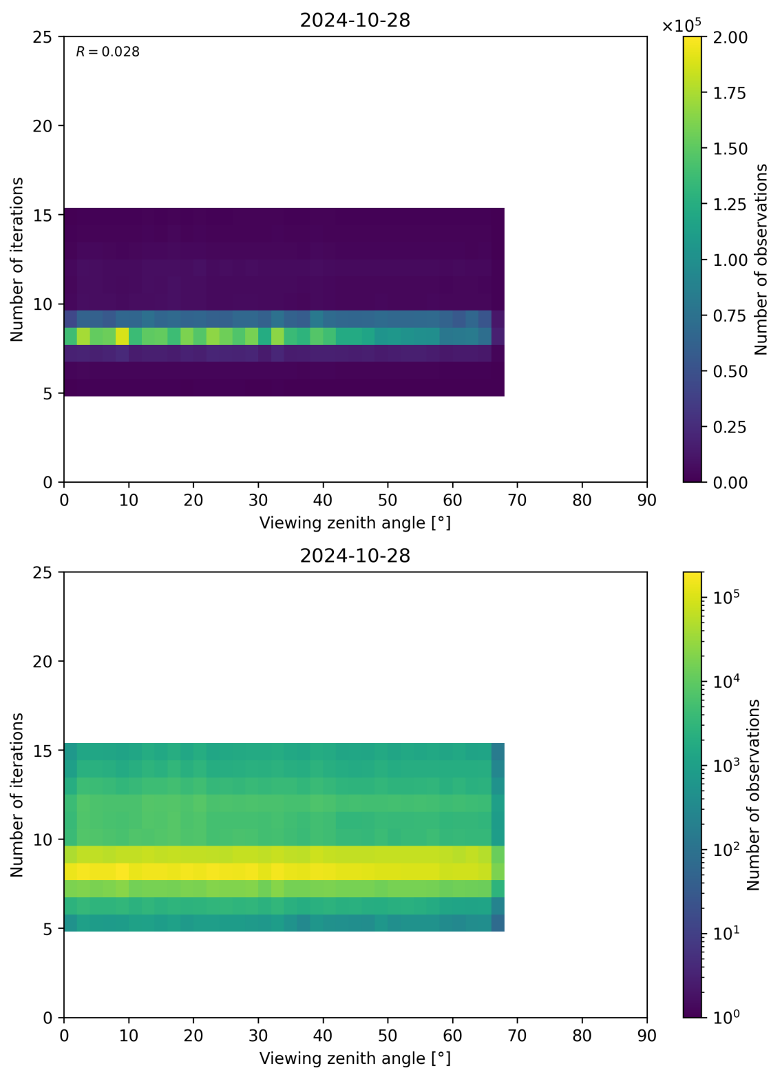
Figure 75: Scatter density plot of “Viewing zenith angle” against “Number of iterations” for 2024-10-27 to 2024-10-29.
