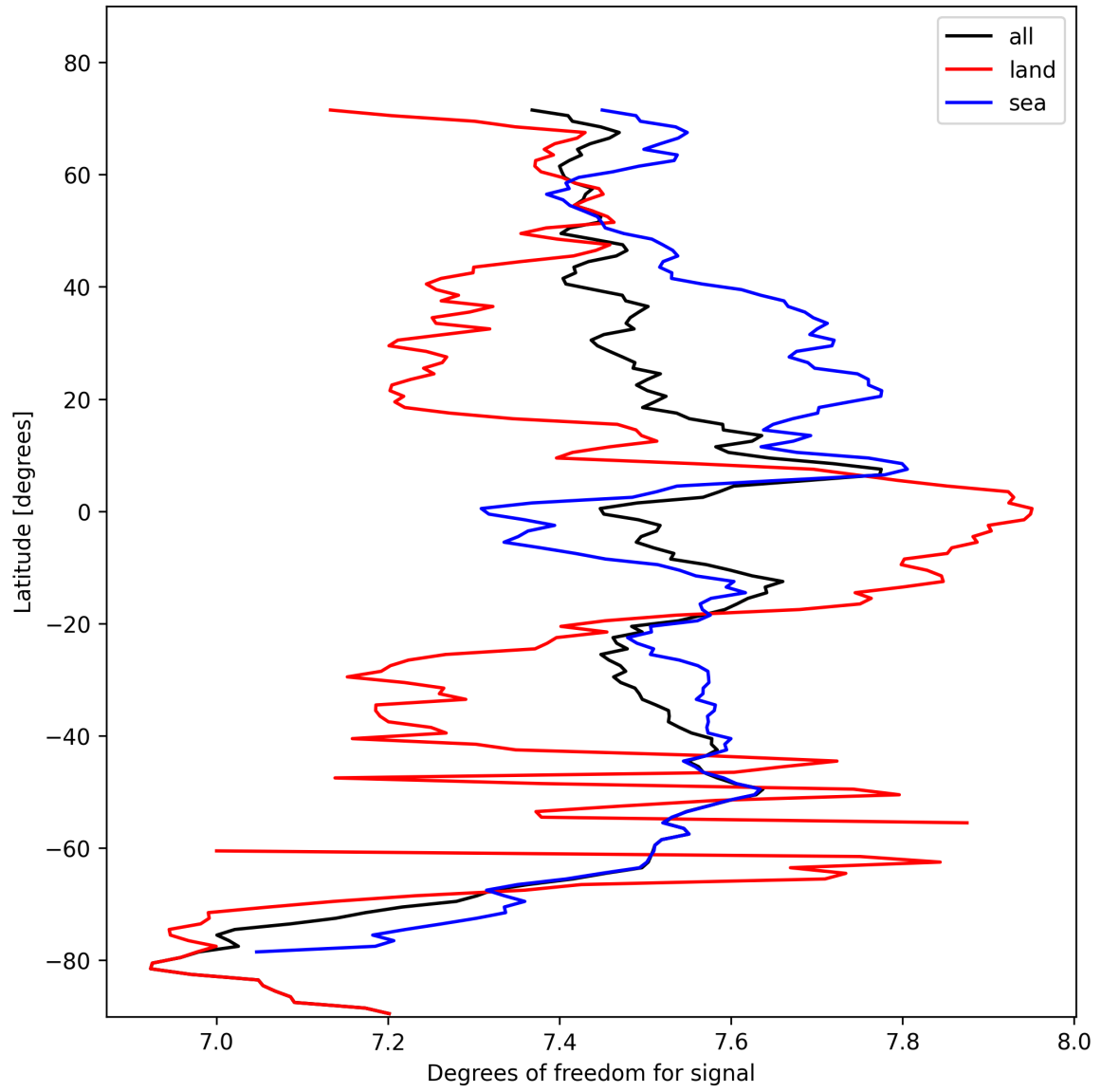
Figure 15: Zonal average of “Degrees of freedom for signal” for 2024-10-27 to 2024-10-29.
