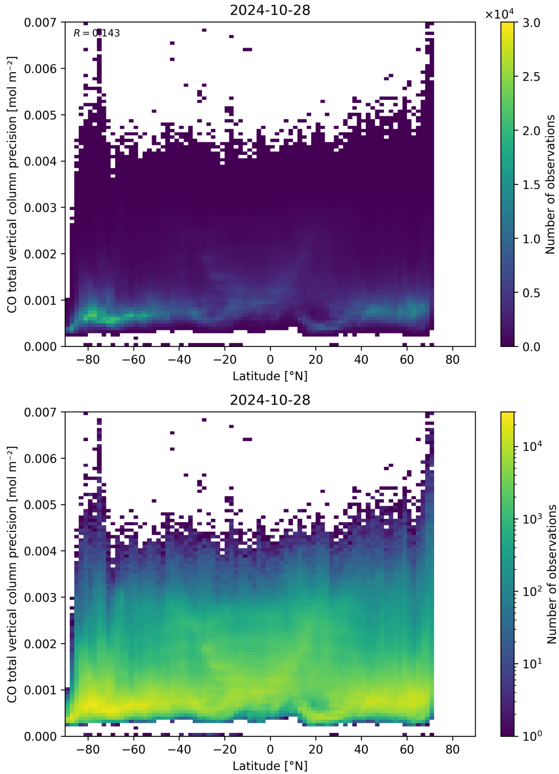
Figure 53: Scatter density plot of “Latitude” against “CO total vertical column precision” for 2024-10-27 to 2024-10-29.
