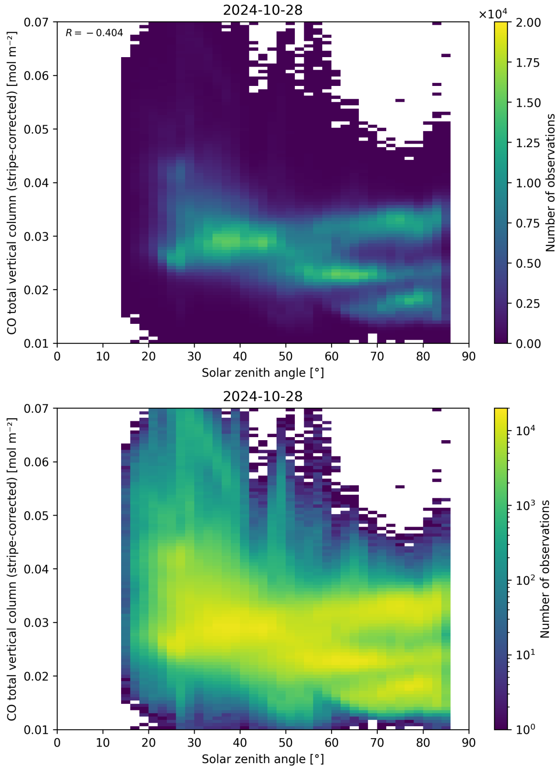
Figure 62: Scatter density plot of “Solar zenith angle” against “CO total vertical column (stripe-corrected)” for 2024-10-27 to 2024-10-29.
