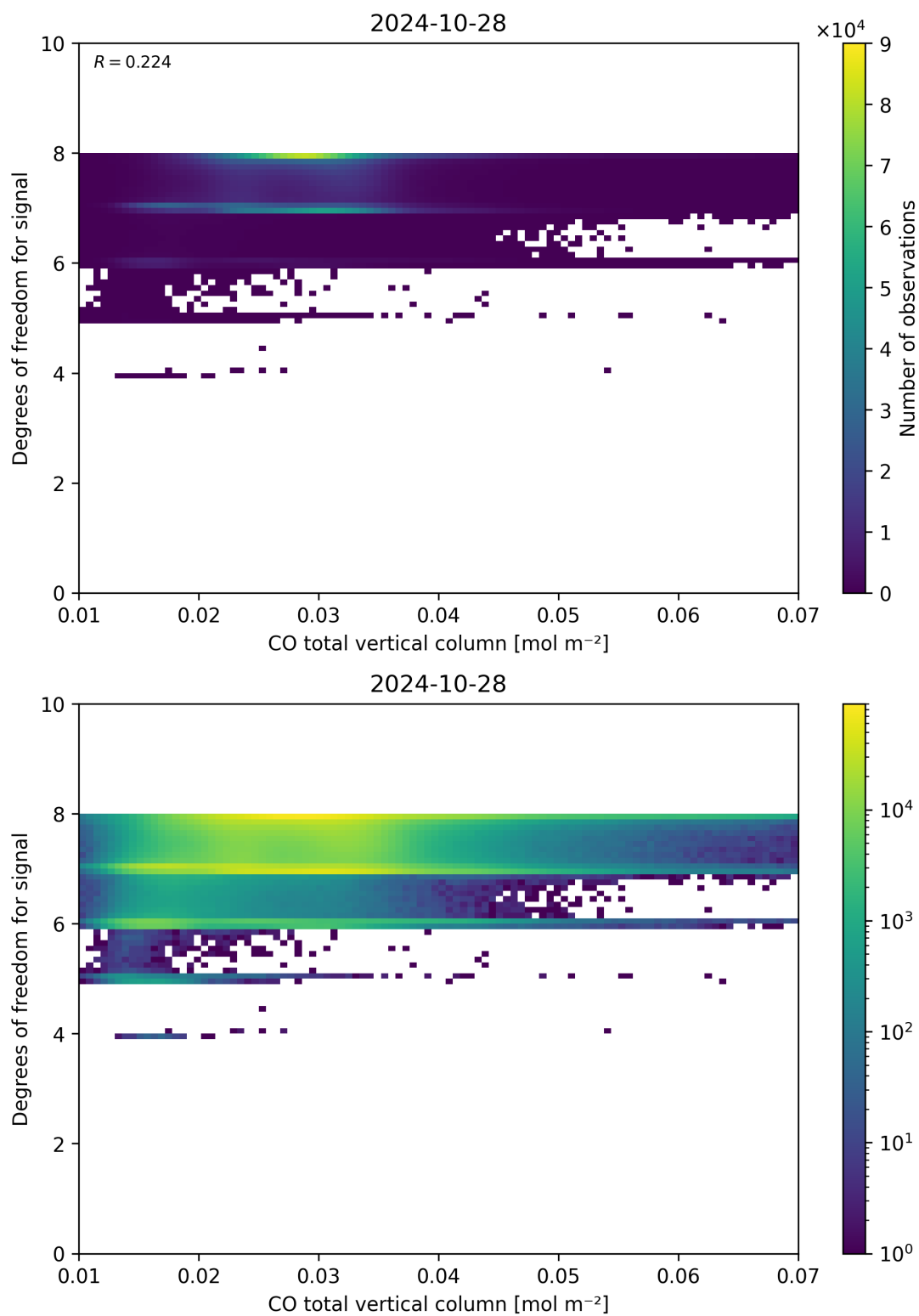
Figure 41: Scatter density plot of “CO total vertical column” against “Degrees of freedom for signal” for 2024-10-27 to 2024-10-29.
