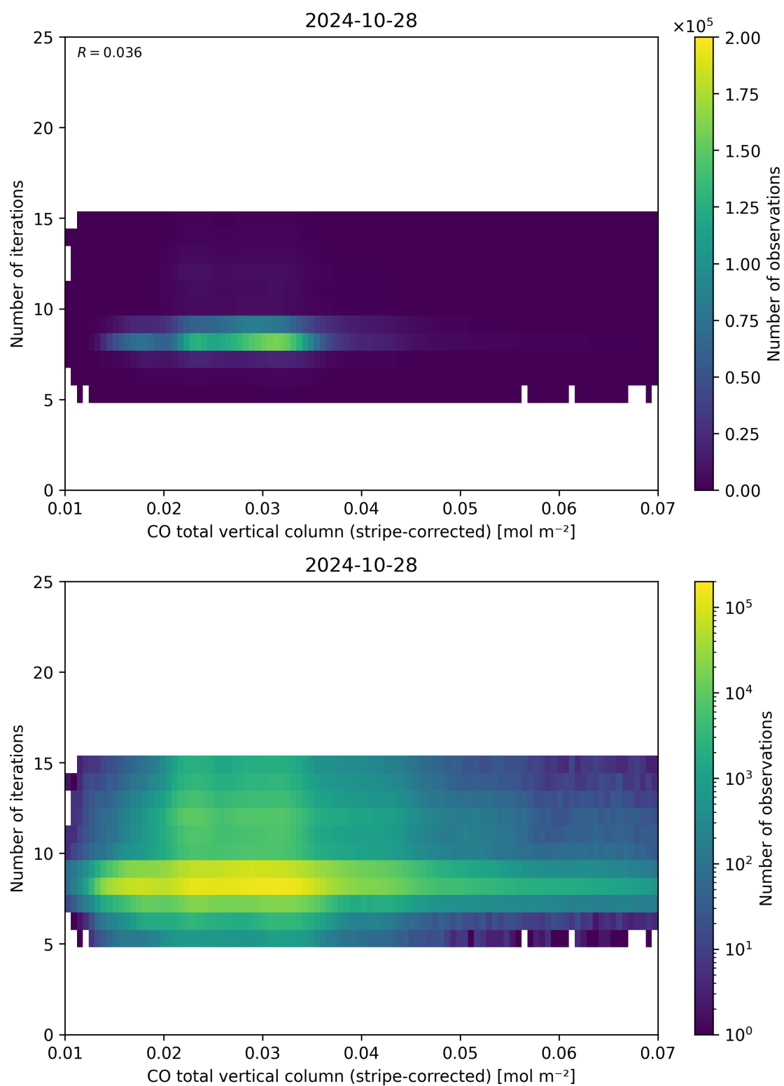
Figure 39: Scatter density plot of “CO total vertical column (stripe-corrected)” against “Number of iterations” for 2024-10-27 to 2024-10-29.
