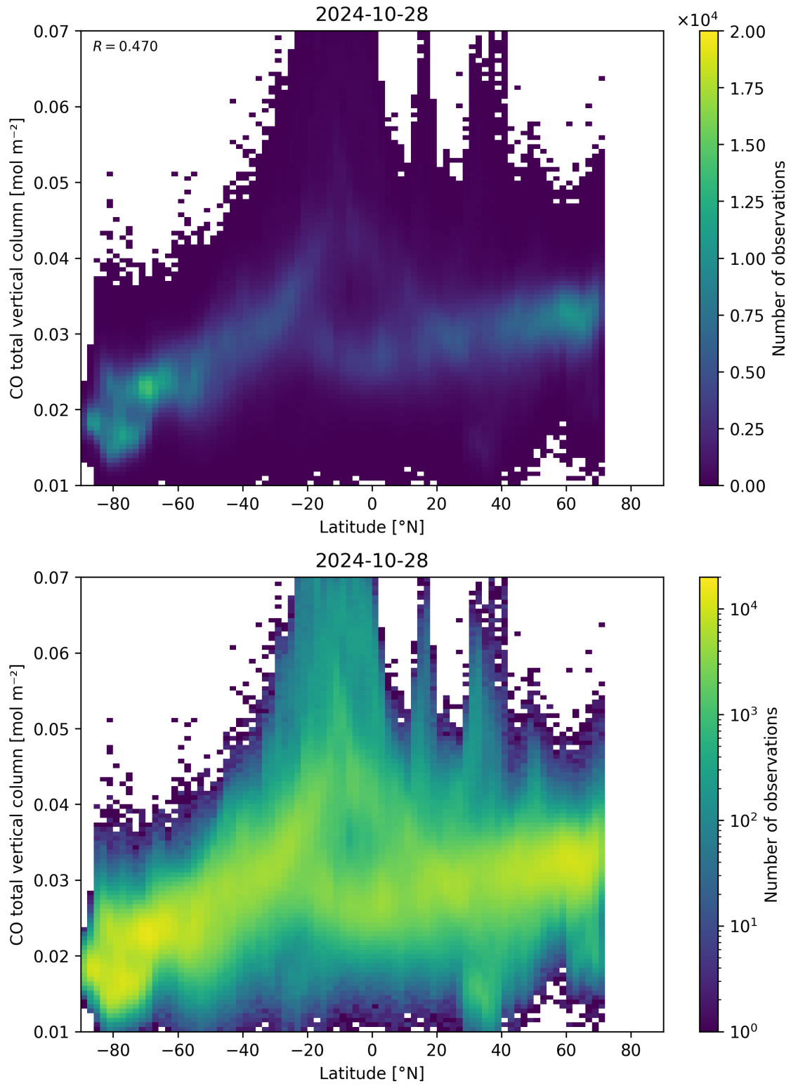
Figure 51: Scatter density plot of “Latitude” against “CO total vertical column” for 2024-10-27 to 2024-10-29.
