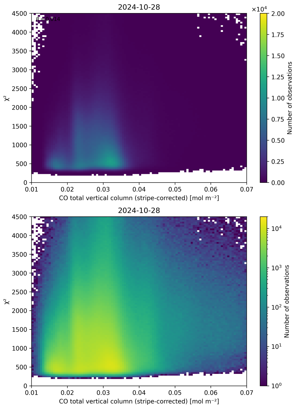
Figure 37: Scatter density plot of “CO total vertical column (stripe-corrected)” against “ \chi^2 ” for 2024-10-27 to 2024-10-29.
