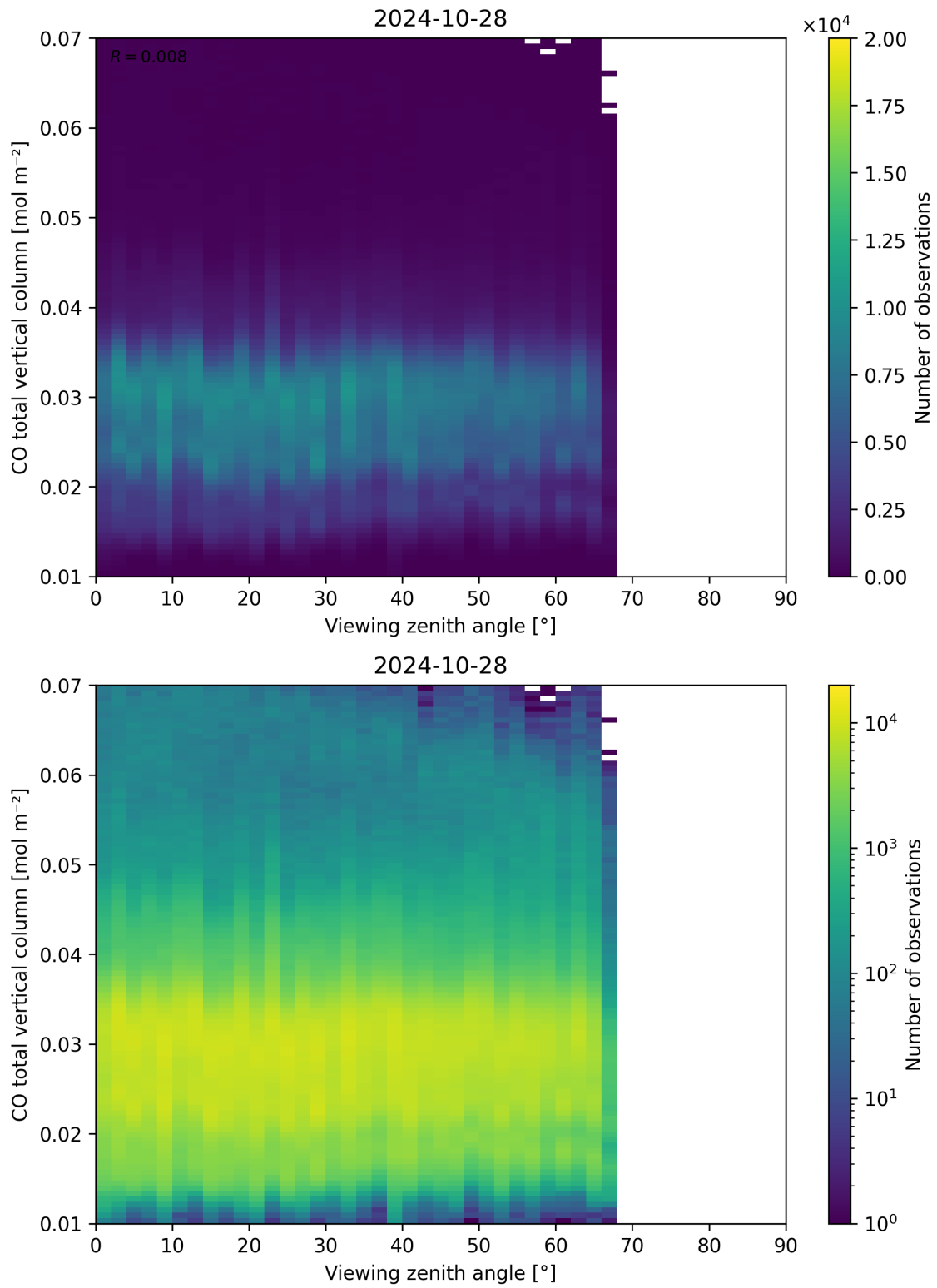
Figure 69: Scatter density plot of “Viewing zenith angle” against “CO total vertical column” for 2024-10-27 to 2024-10-29.
