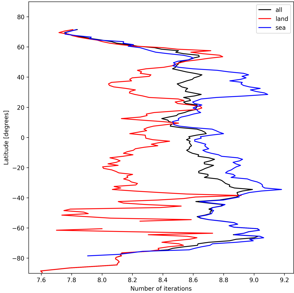
Figure 16: Zonal average of “Number of iterations” for 2024-10-27 to 2024-10-29.
