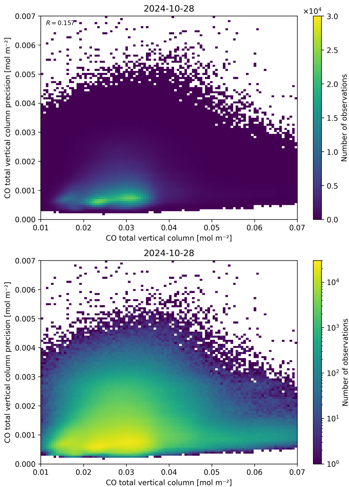
Figure 34: Scatter density plot of “CO total vertical column” against “CO total vertical column precision” for 2024-10-27 to 2024-10-29.
