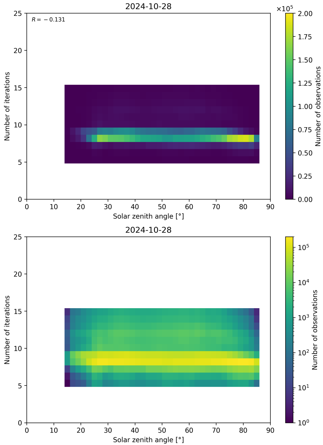
Figure 67: Scatter density plot of “Solar zenith angle” against “Number of iterations” for 2024-10-27 to 2024-10-29.
