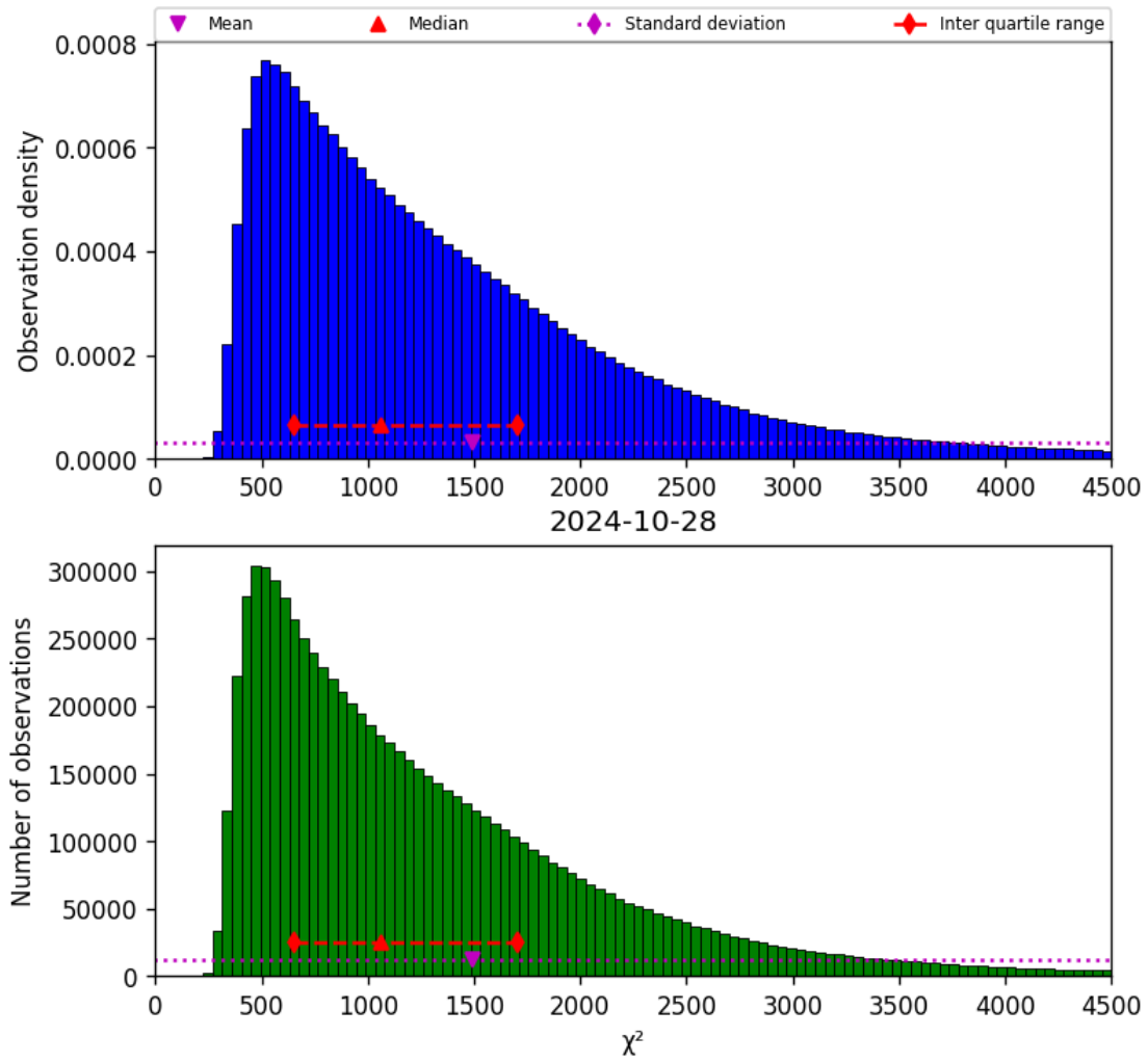
Figure 22: Histogram of “ \chi^2 ” for 2024-10-27 to 2024-10-29
