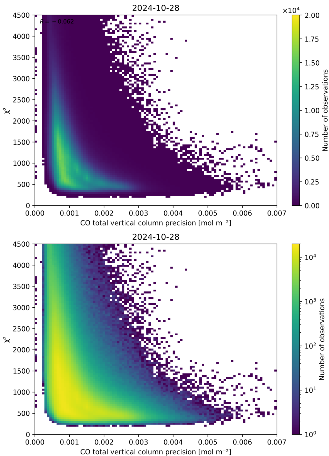
Figure 44: Scatter density plot of “CO total vertical column precision” against “ \chi^2 ” for 2024-10-27 to 2024-10-29.
