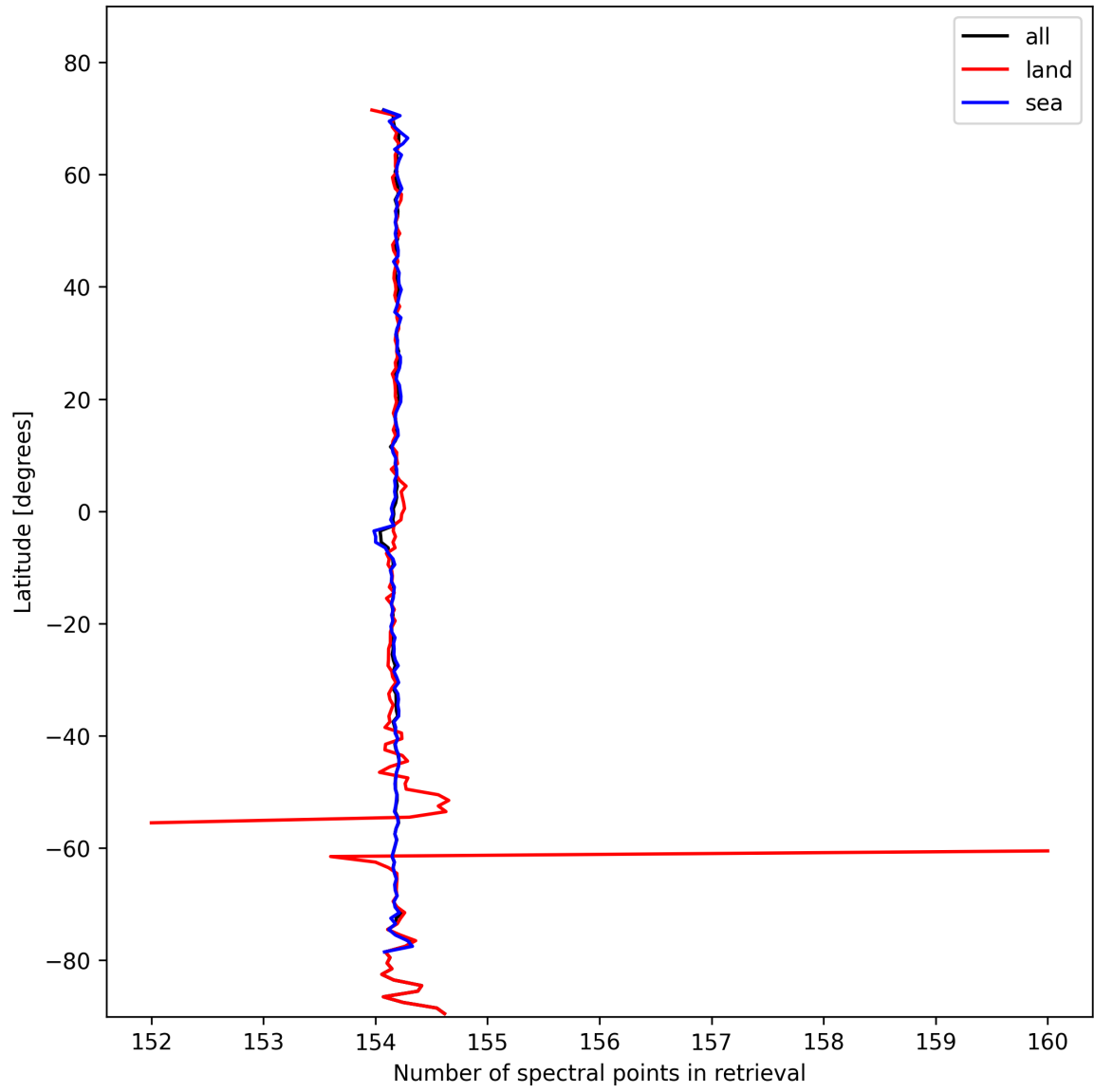
Figure 13: Zonal average of “Number of spectral points in retrieval” for 2024-10-27 to 2024-10-29.
