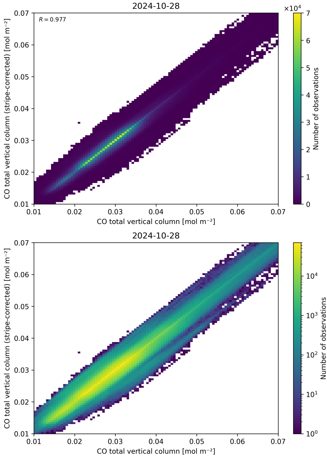
Figure 33: Scatter density plot of “CO total vertical column” against “CO total vertical column (stripe-corrected)” for 2024-10-27 to 2024-10-29.
