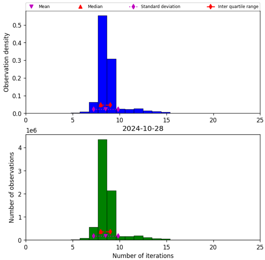
Figure 24: Histogram of “Number of iterations” for 2024-10-27 to 2024-10-29
