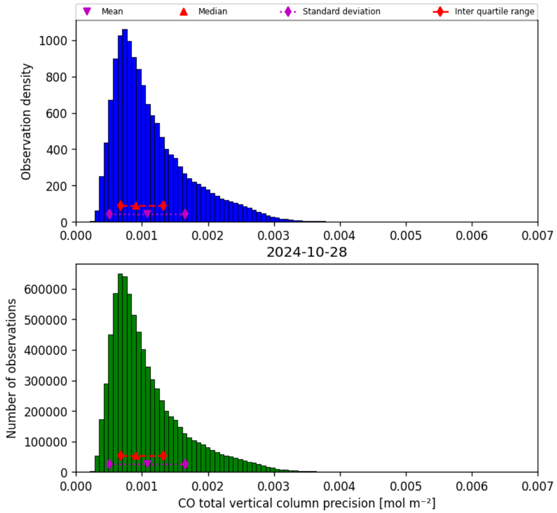
Figure 20: Histogram of “CO total vertical column precision” for 2024-10-27 to 2024-10-29
