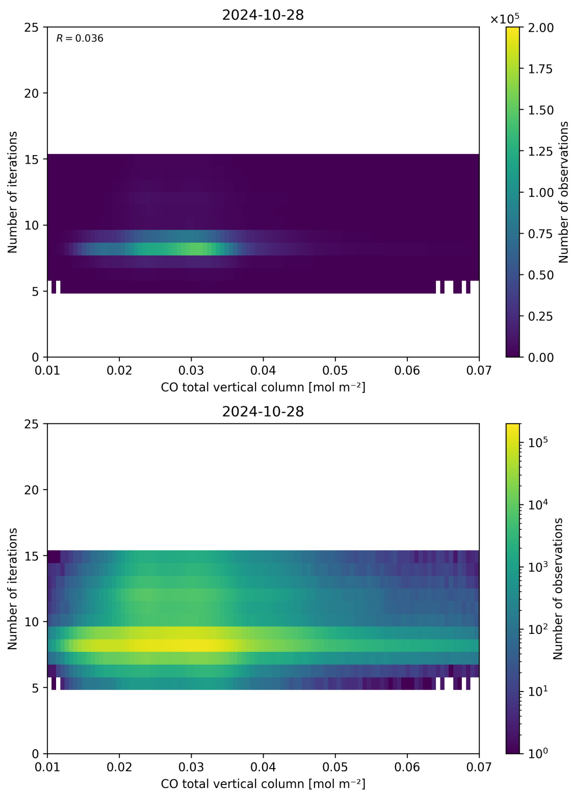
Figure 42: Scatter density plot of “CO total vertical column” against “Number of iterations” for 2024-10-27 to 2024-10-29.
