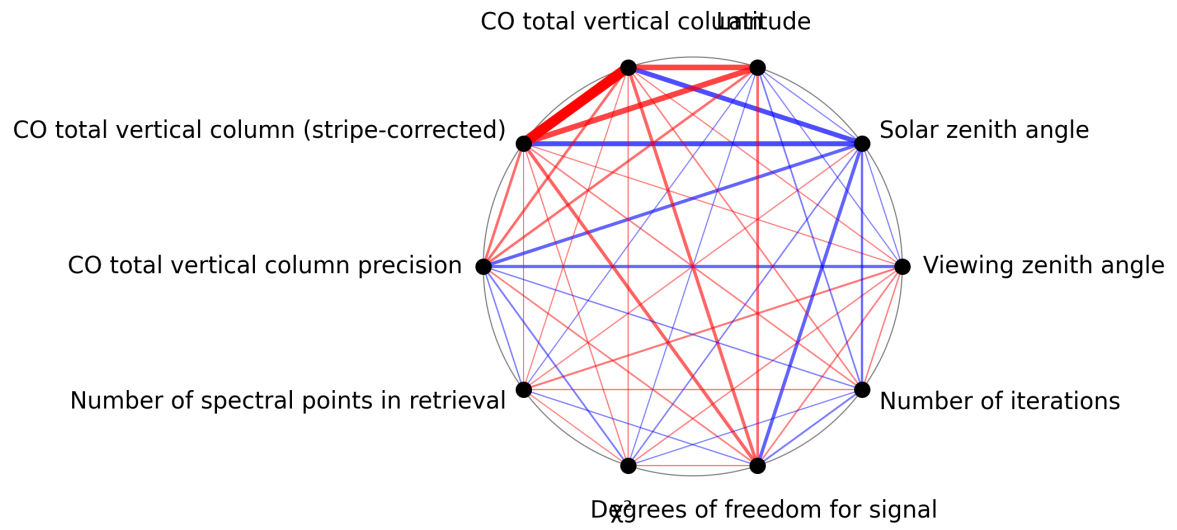
Figure 1: Map of correlation graph for 2024-10-27 to 2024-10-29.
