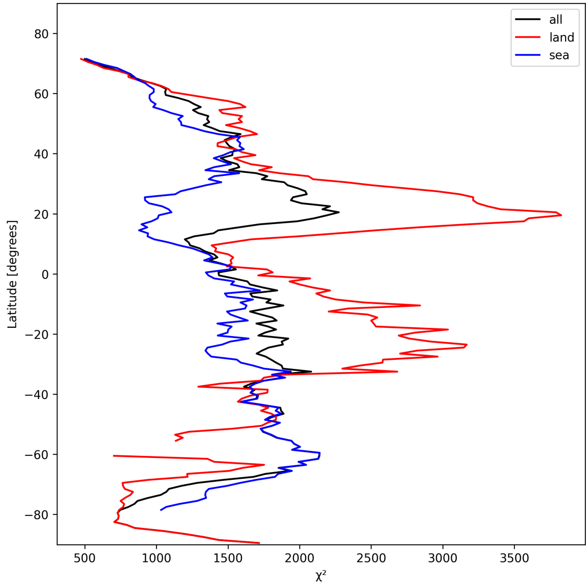
Figure 14: Zonal average of “ \chi^2 ” for 2024-10-27 to 2024-10-29.
