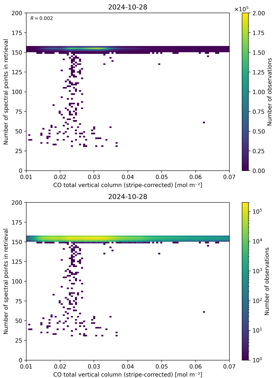
Figure 40: Scatter density plot of “CO total vertical column (stripe-corrected)” against “Number of spectral points in retrieval” for 2024-10-27 to 2024-10-29.
