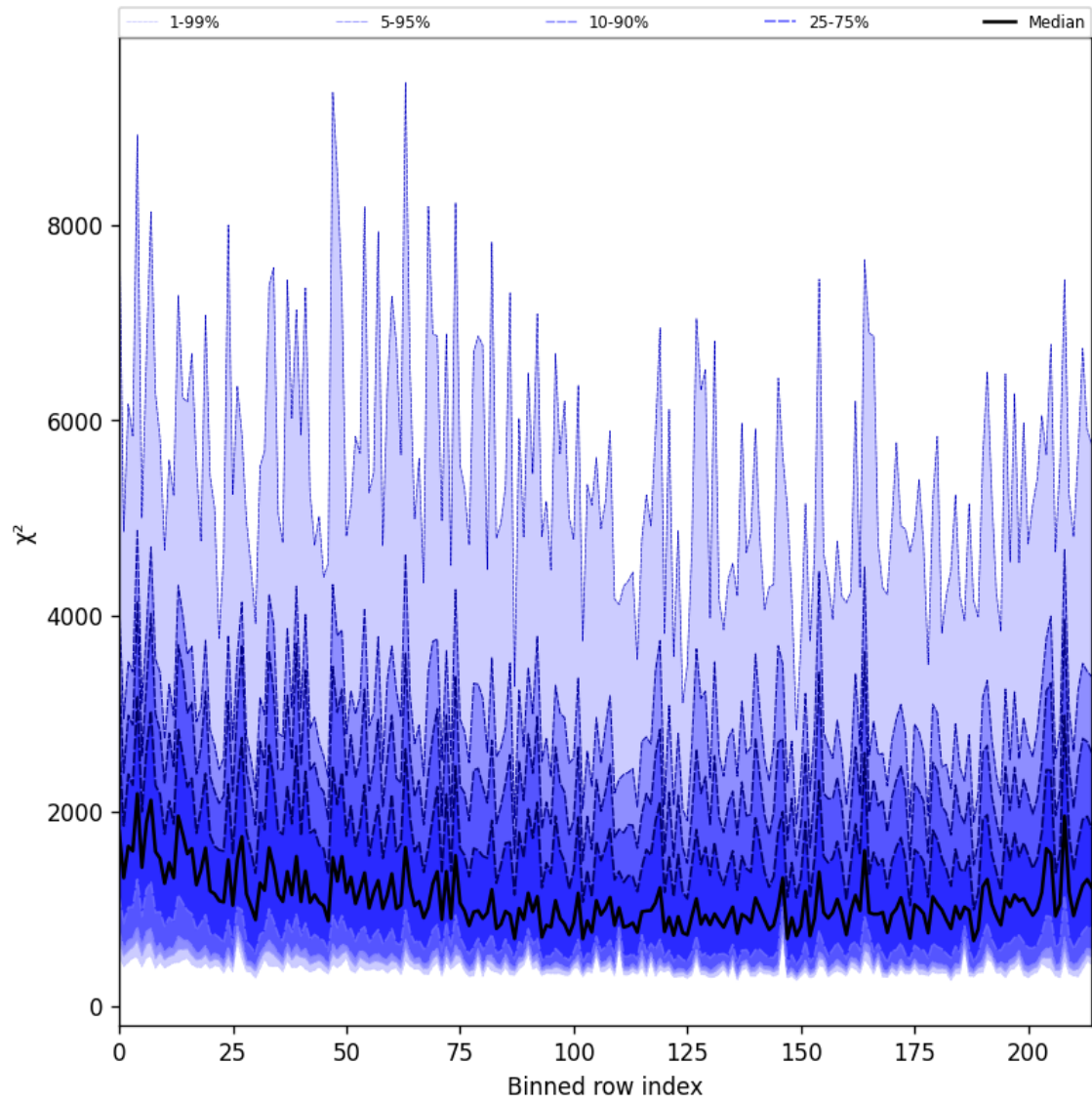
Figure 30: Along track statistics of “ \chi^2 ” for 2024-10-27 to 2024-10-29
