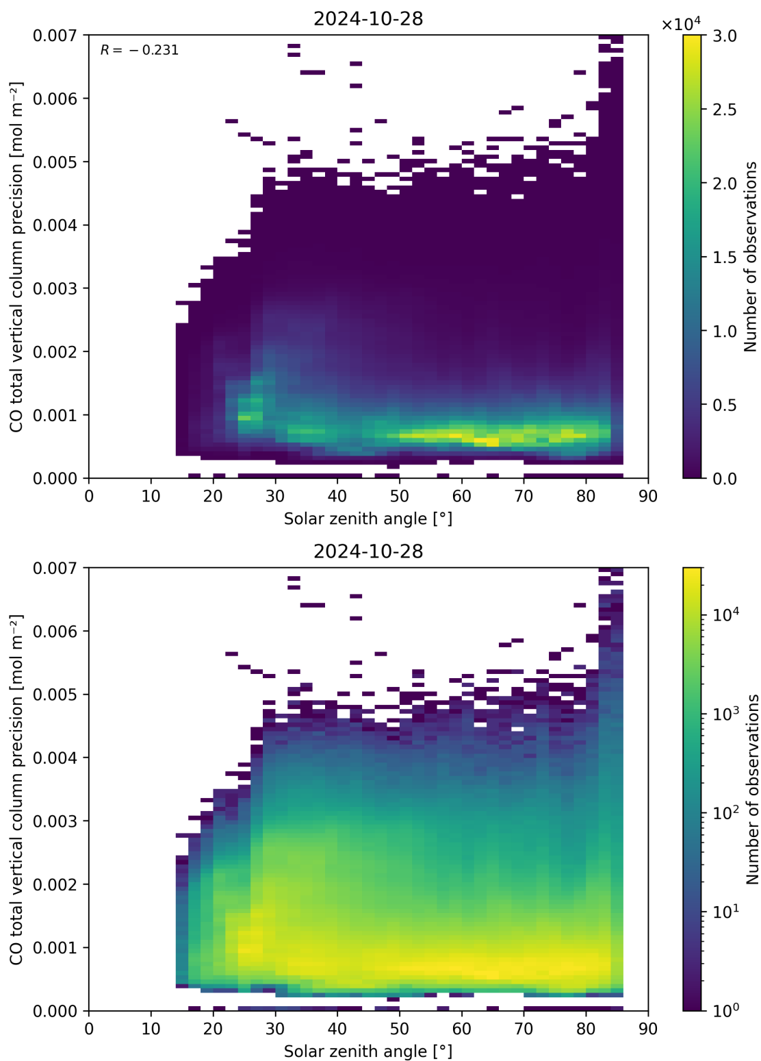
Figure 63: Scatter density plot of “Solar zenith angle” against “CO total vertical column precision” for 2024-10-27 to 2024-10-29.
