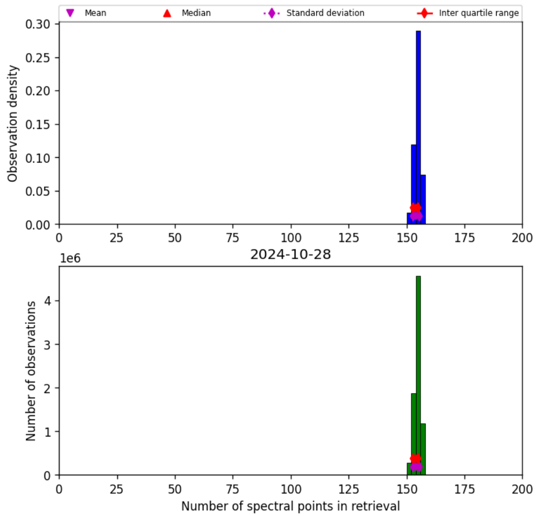
Figure 21: Histogram of “Number of spectral points in retrieval” for 2024-10-27 to 2024-10-29
