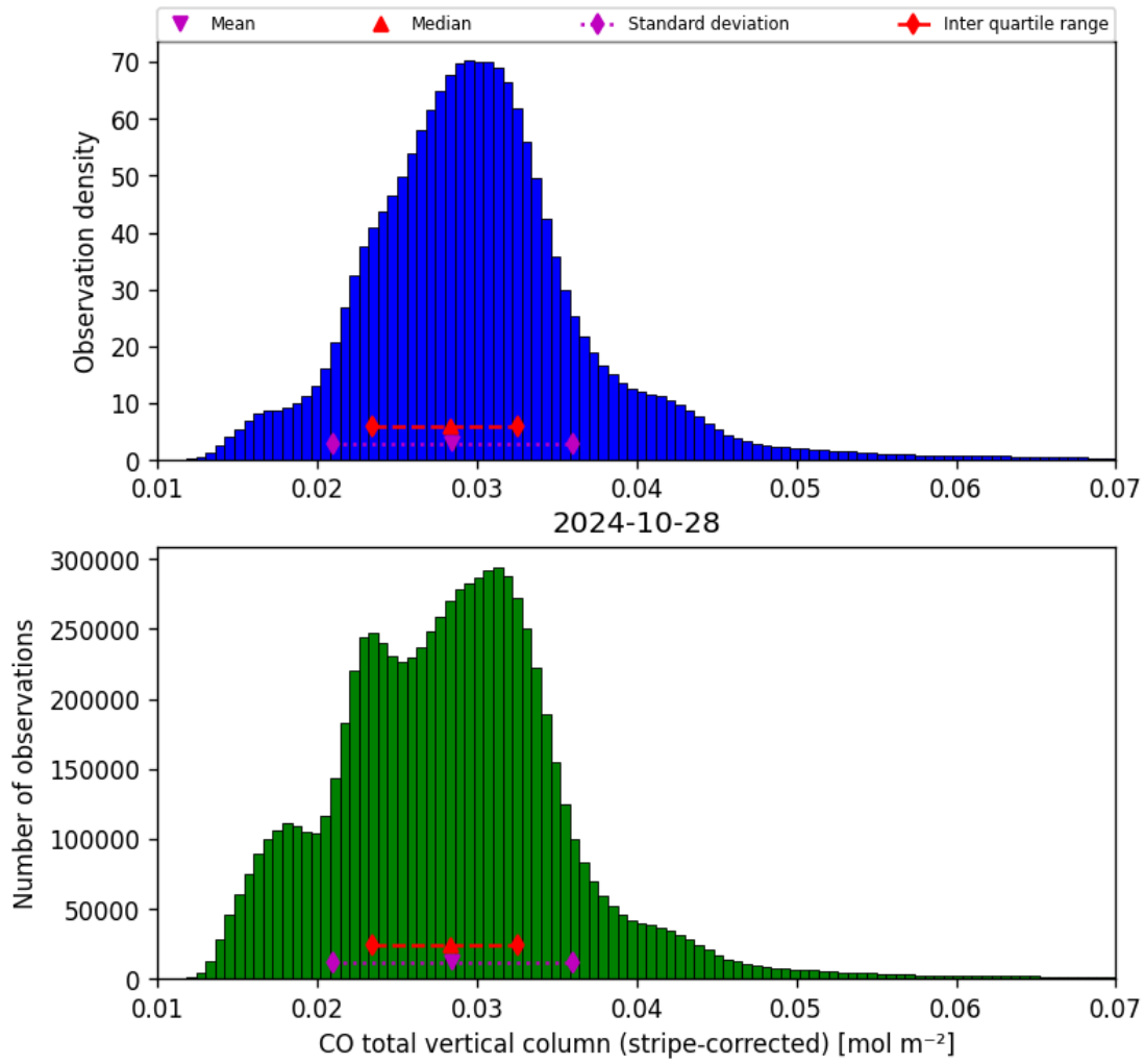
Figure 19: Histogram of “CO total vertical column (stripe-corrected)” for 2024-10-27 to 2024-10-29
