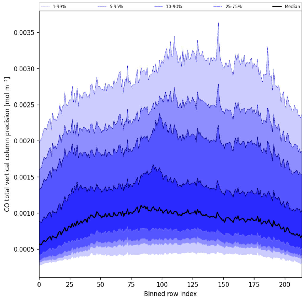
Figure 28: Along track statistics of “CO total vertical column precision” for 2024-10-27 to 2024-10-29
