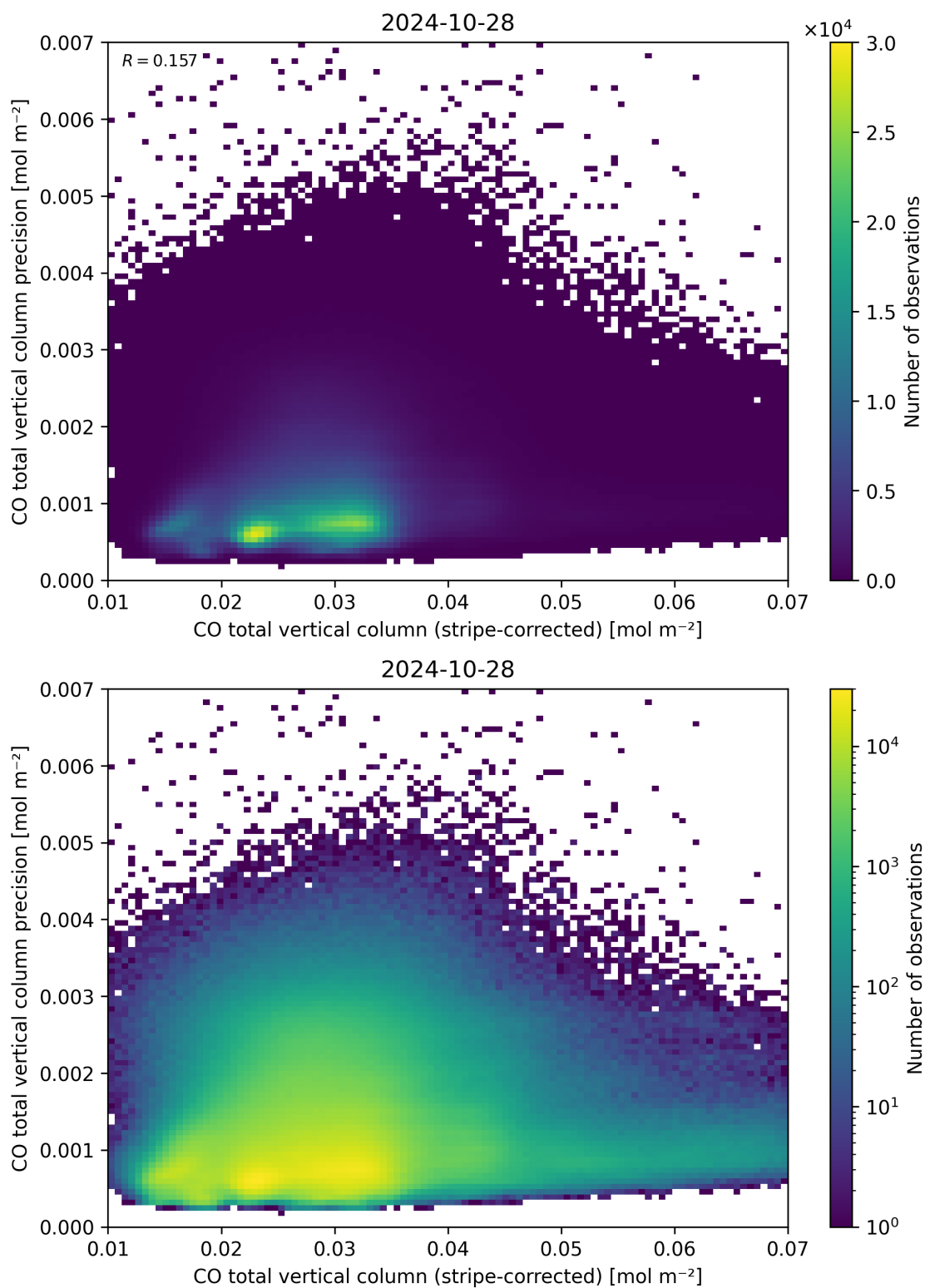
Figure 36: Scatter density plot of “CO total vertical column (stripe-corrected)” against “CO total vertical column precision” for 2024-10-27 to 2024-10-29.
