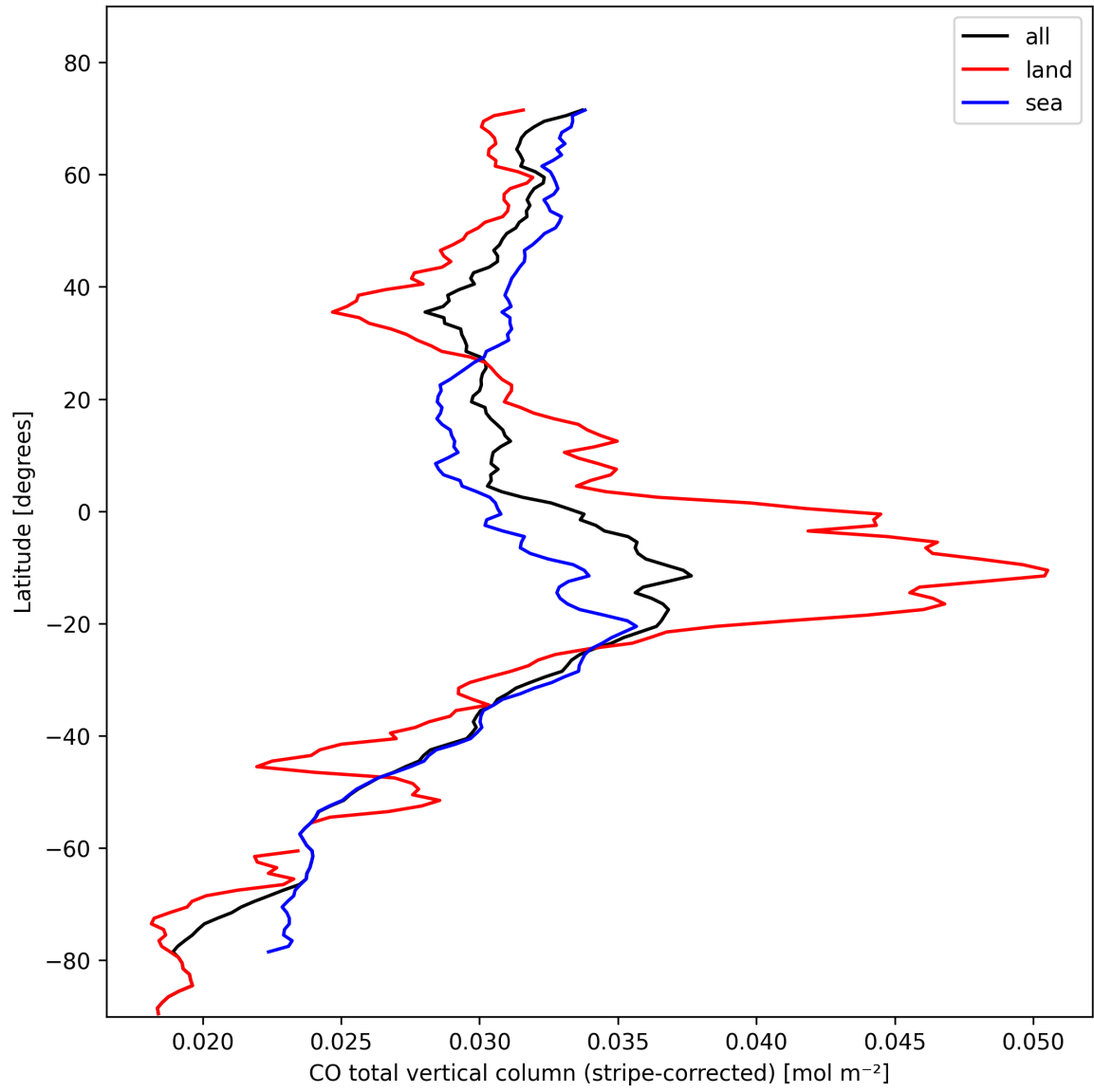
Figure 11: Zonal average of “CO total vertical column (stripe-corrected)” for 2024-10-27 to 2024-10-29.
