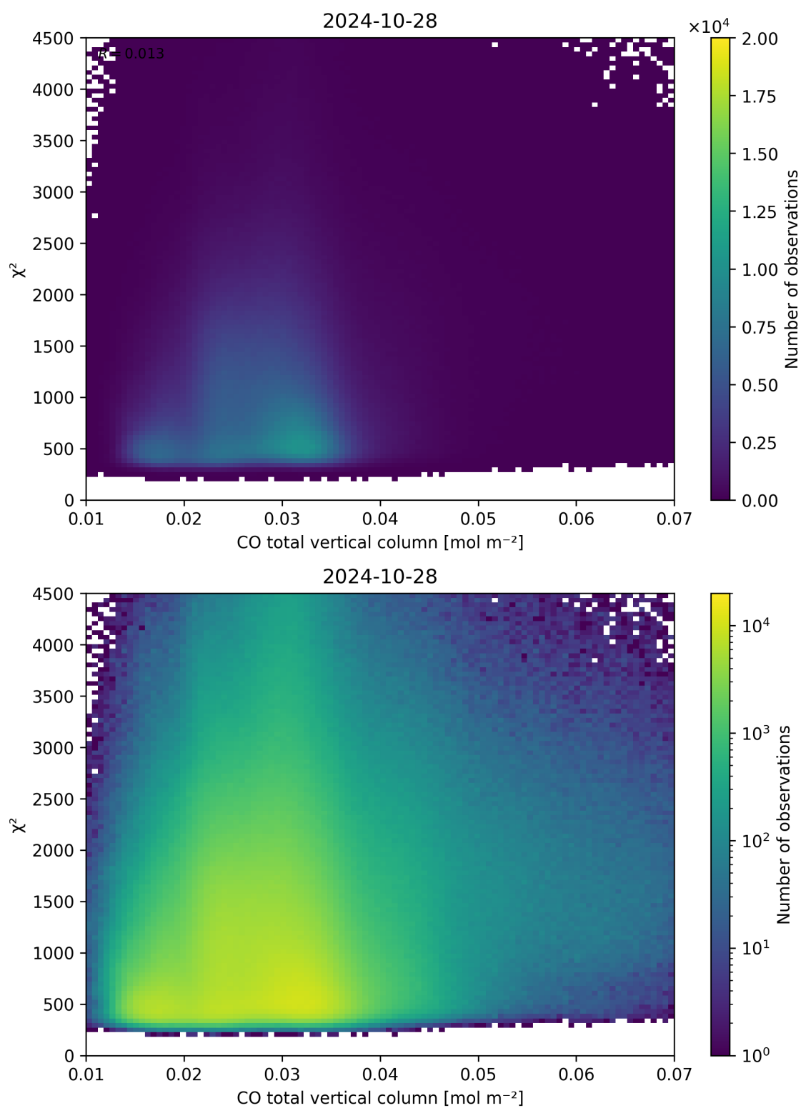
Figure 35: Scatter density plot of “CO total vertical column” against “ \chi^2 ” for 2024-10-27 to 2024-10-29.
