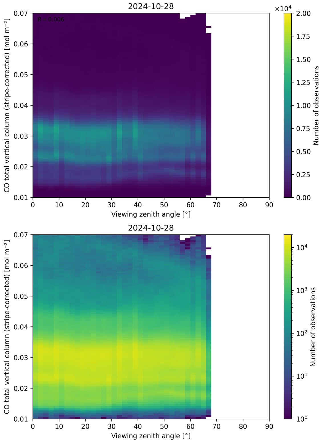
Figure 70: Scatter density plot of “Viewing zenith angle” against “CO total vertical column (stripe-corrected)” for 2024-10-27 to 2024-10-29.
