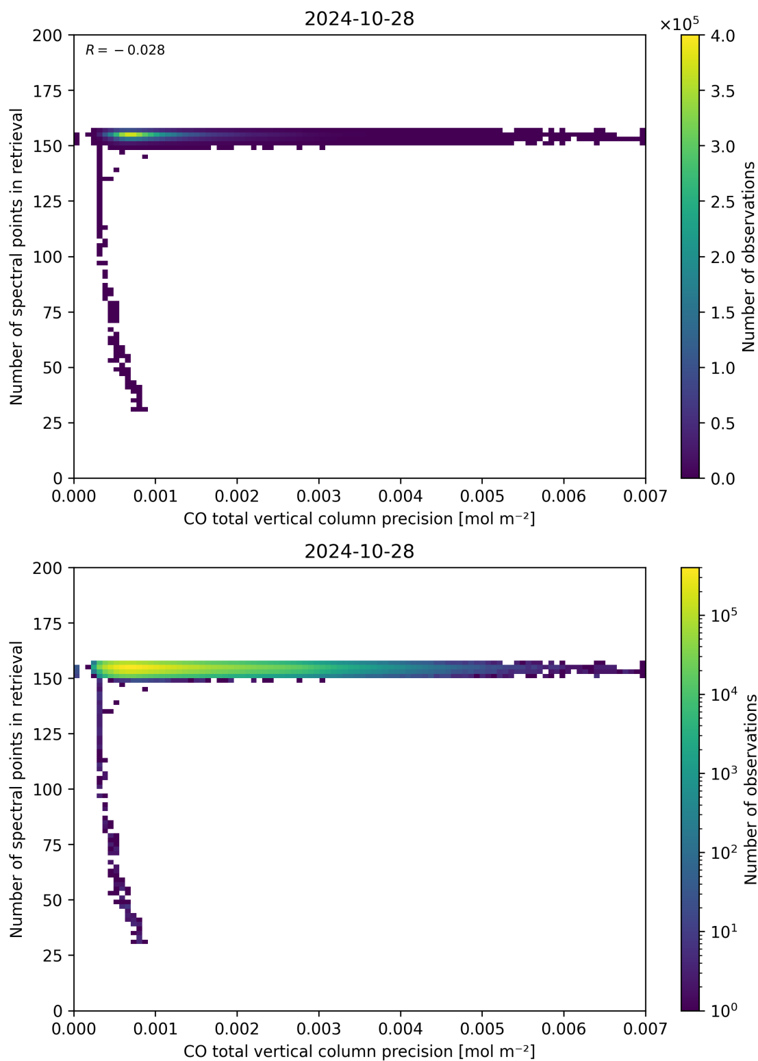
Figure 47: Scatter density plot of “CO total vertical column precision” against “Number of spectral points in retrieval” for 2024-10-27 to 2024-10-29.
