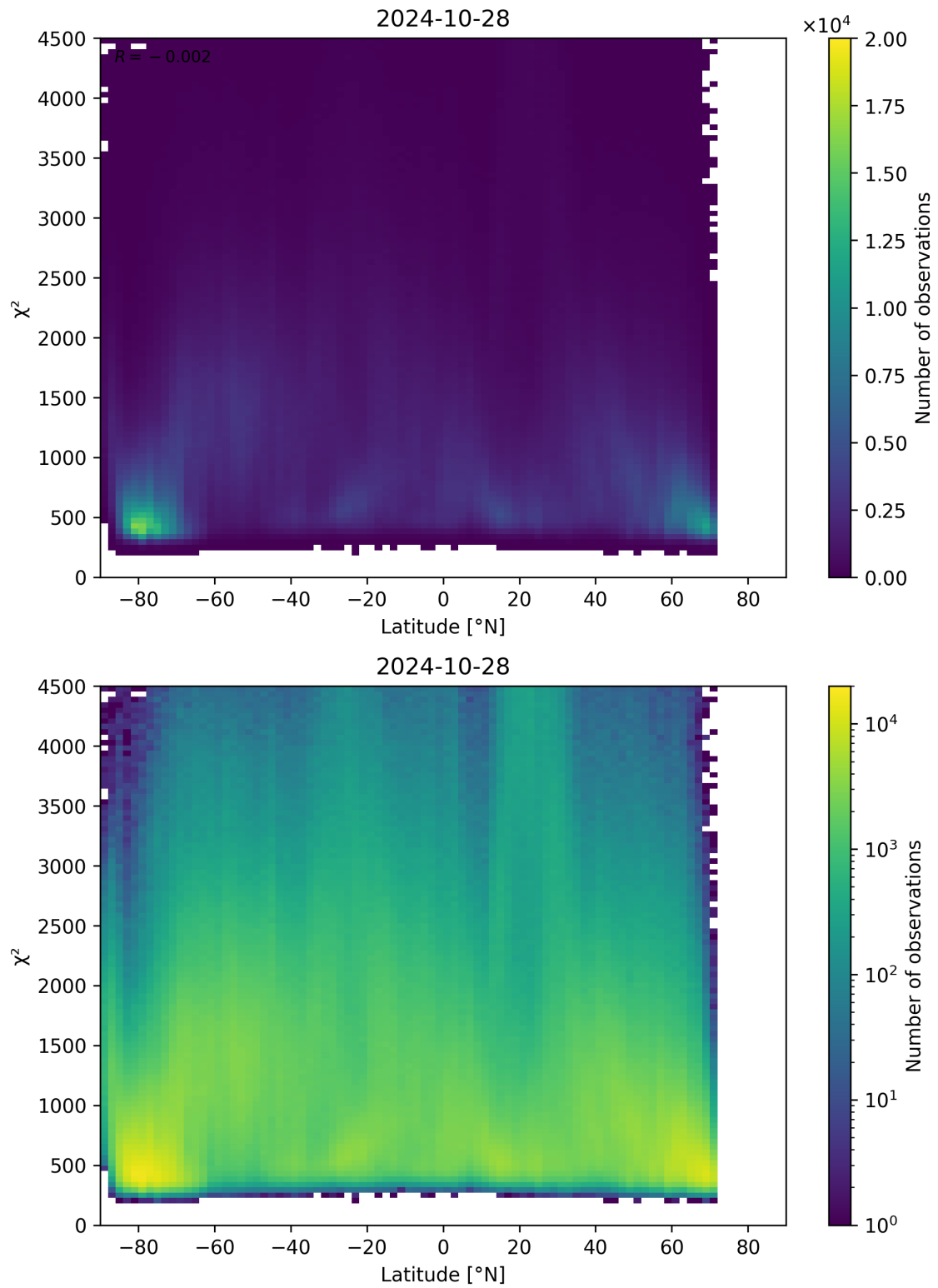
Figure 54: Scatter density plot of “Latitude” against “ \chi^2 ” for 2024-10-27 to 2024-10-29.
