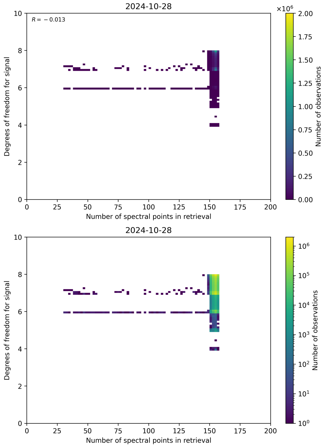
Figure 59: Scatter density plot of “Number of spectral points in retrieval” against “Degrees of freedom for signal” for 2024-10-27 to 2024-10-29.
