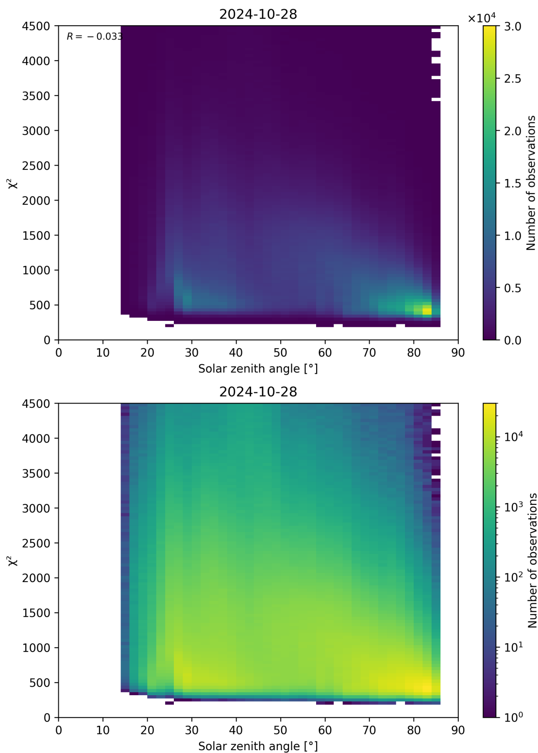
Figure 64: Scatter density plot of “Solar zenith angle” against “ \chi^2 ” for 2024-10-27 to 2024-10-29.
