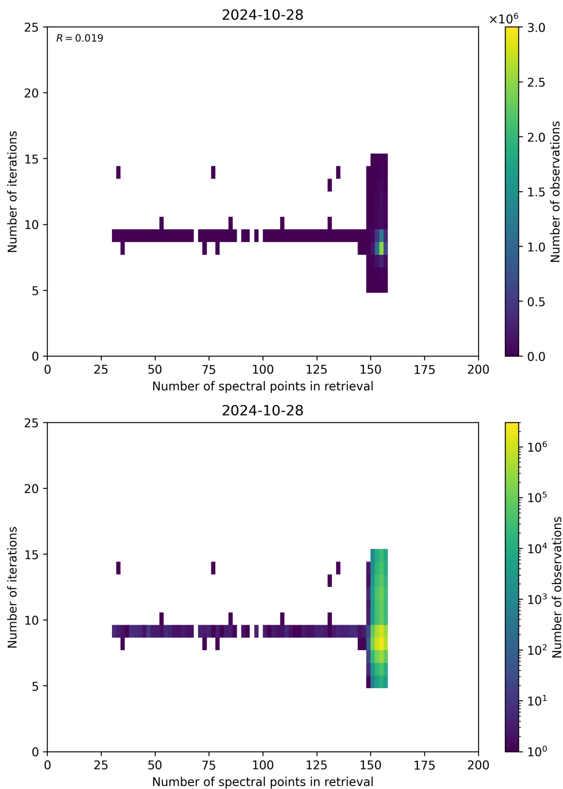
Figure 60: Scatter density plot of “Number of spectral points in retrieval” against “Number of iterations” for 2024-10-27 to 2024-10-29.
