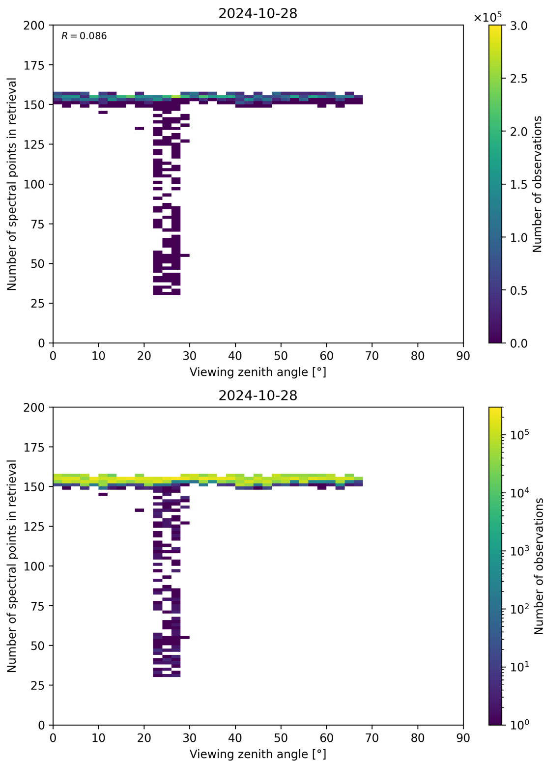
Figure 76: Scatter density plot of “Viewing zenith angle” against “Number of spectral points in retrieval” for 2024-10-27 to 2024-10-29.
