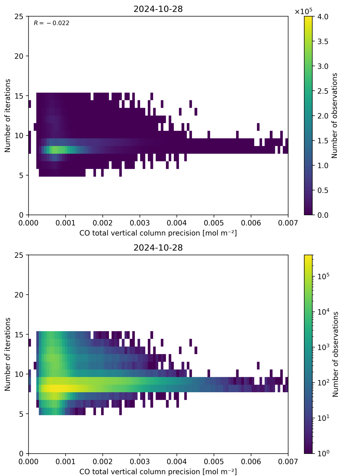
Figure 46: Scatter density plot of “CO total vertical column precision” against “Number of iterations” for 2024-10-27 to 2024-10-29.
