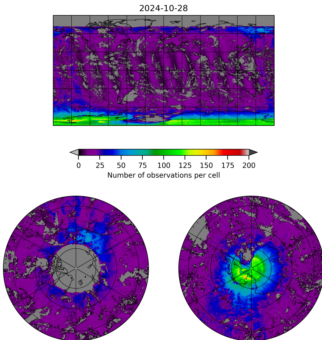
Figure 8: Map of the number of observations for 2024-10-27 to 2024-10-29
