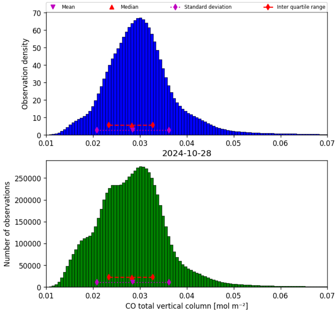
Figure 18: Histogram of “CO total vertical column” for 2024-10-27 to 2024-10-29
