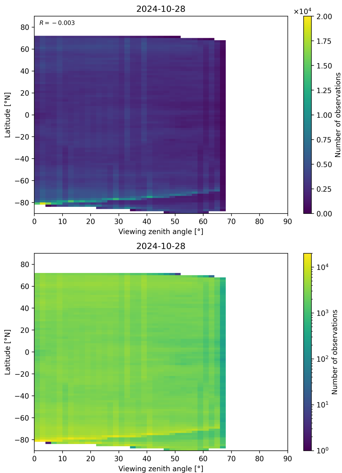
Figure 74: Scatter density plot of “Viewing zenith angle” against “Latitude” for 2024-10-27 to 2024-10-29.
