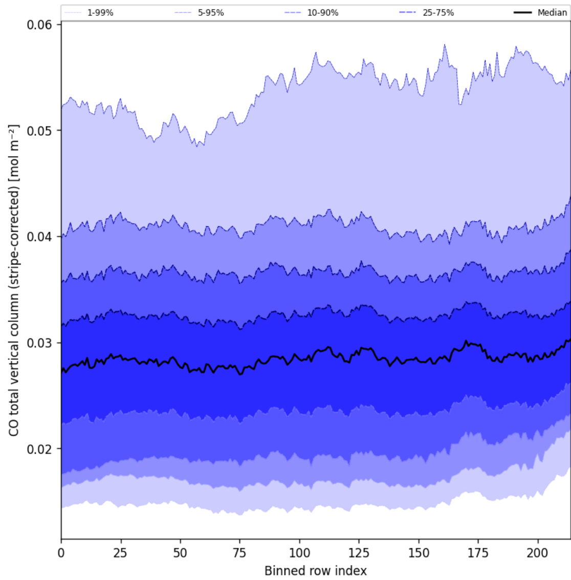
Figure 27: Along track statistics of “CO total vertical column (stripe-corrected)” for 2024-10-27 to 2024-10-29
