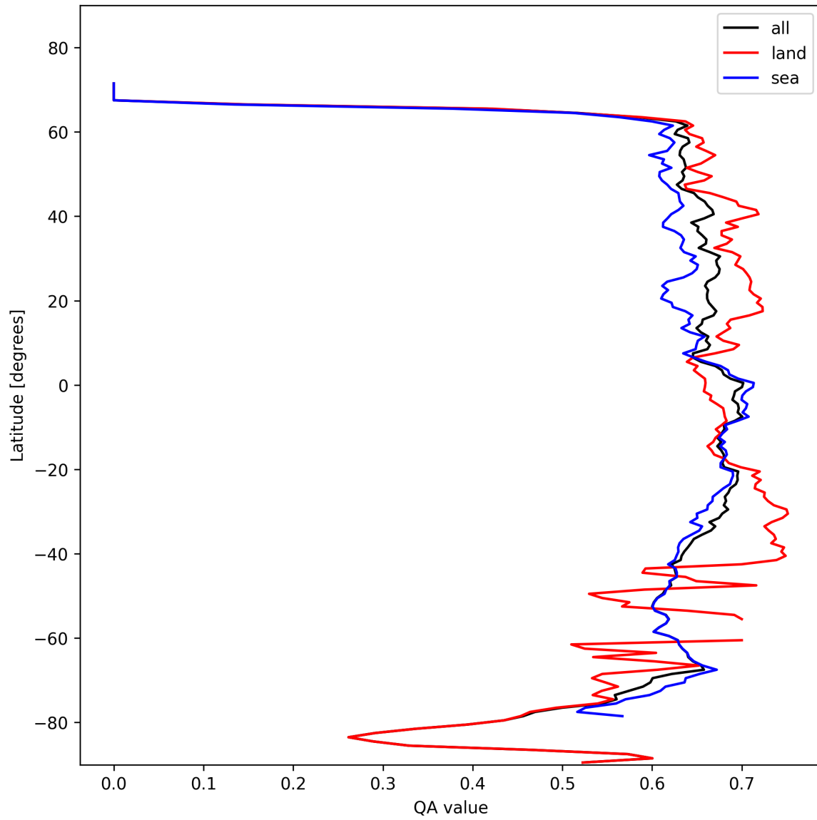
Figure 9: Zonal average of “QA value” for 2024-10-27 to 2024-10-29.
