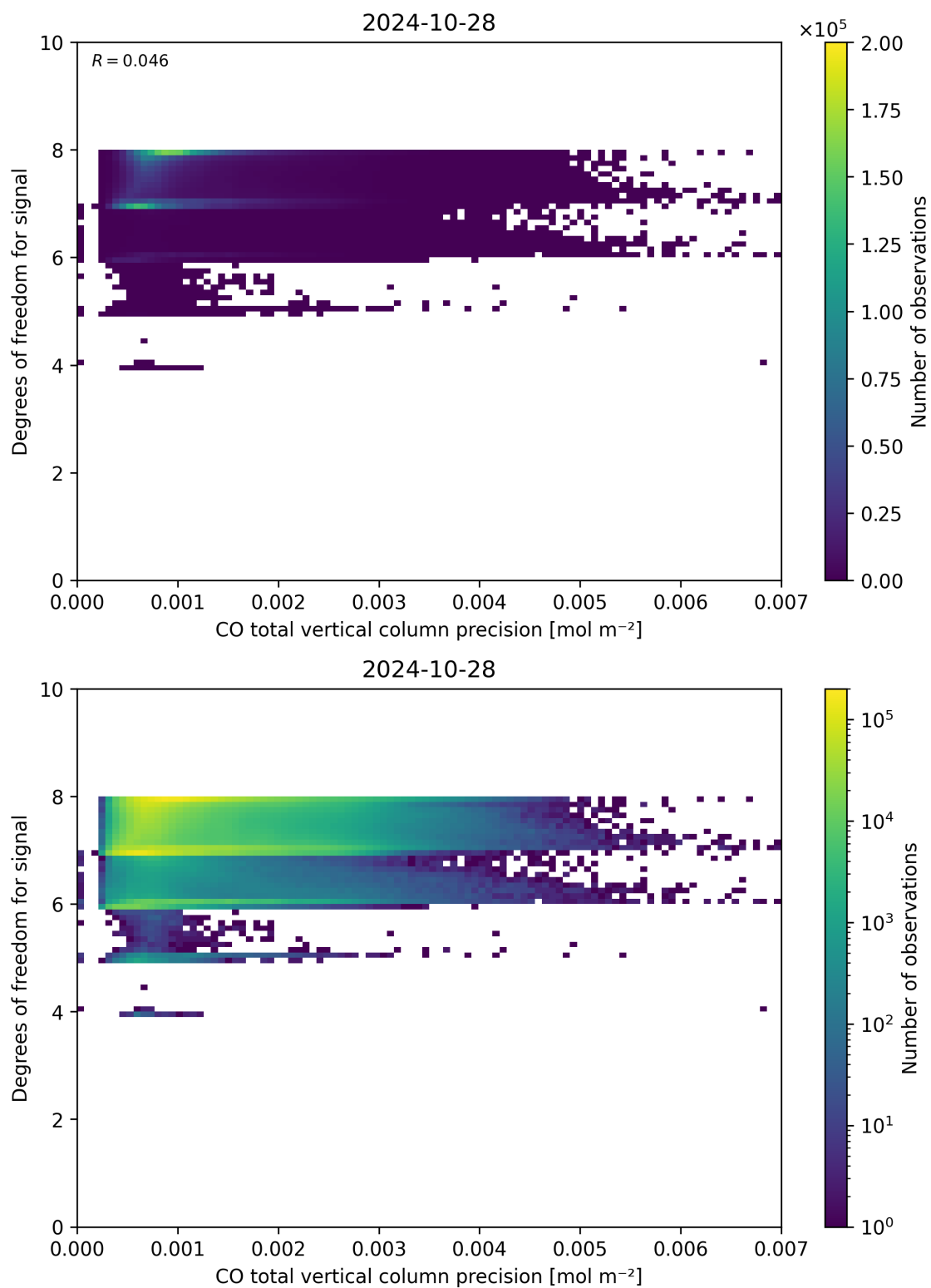
Figure 45: Scatter density plot of “CO total vertical column precision” against “Degrees of freedom for signal” for 2024-10-27 to 2024-10-29.
