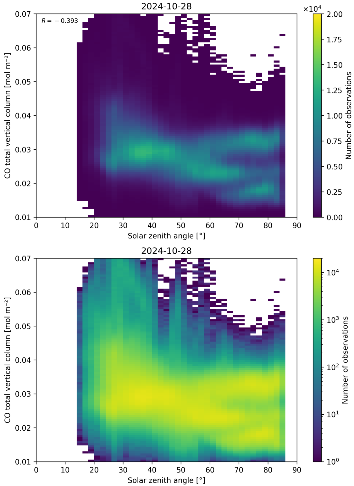
Figure 61: Scatter density plot of “Solar zenith angle” against “CO total vertical column” for 2024-10-27 to 2024-10-29.
