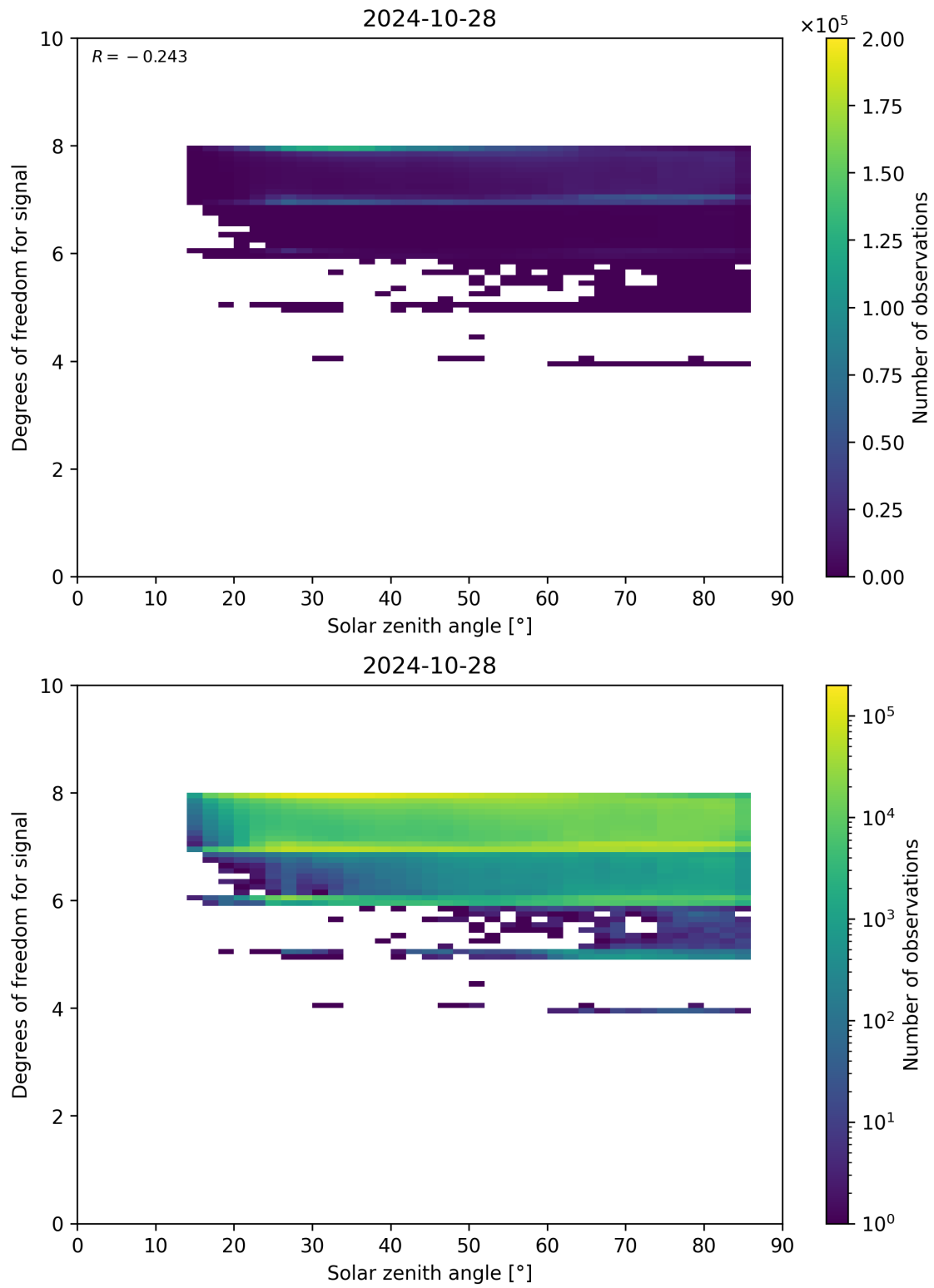
Figure 65: Scatter density plot of “Solar zenith angle” against “Degrees of freedom for signal” for 2024-10-27 to 2024-10-29.
