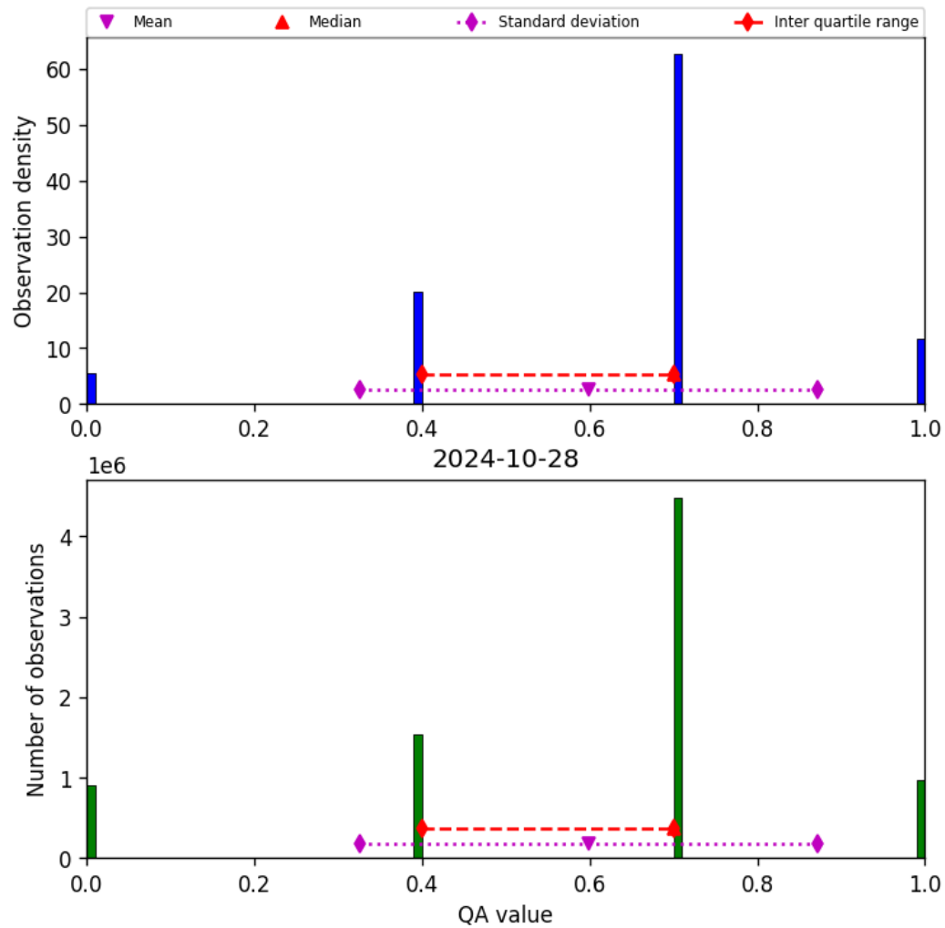
Figure 17: Histogram of “QA value” for 2024-10-27 to 2024-10-29
