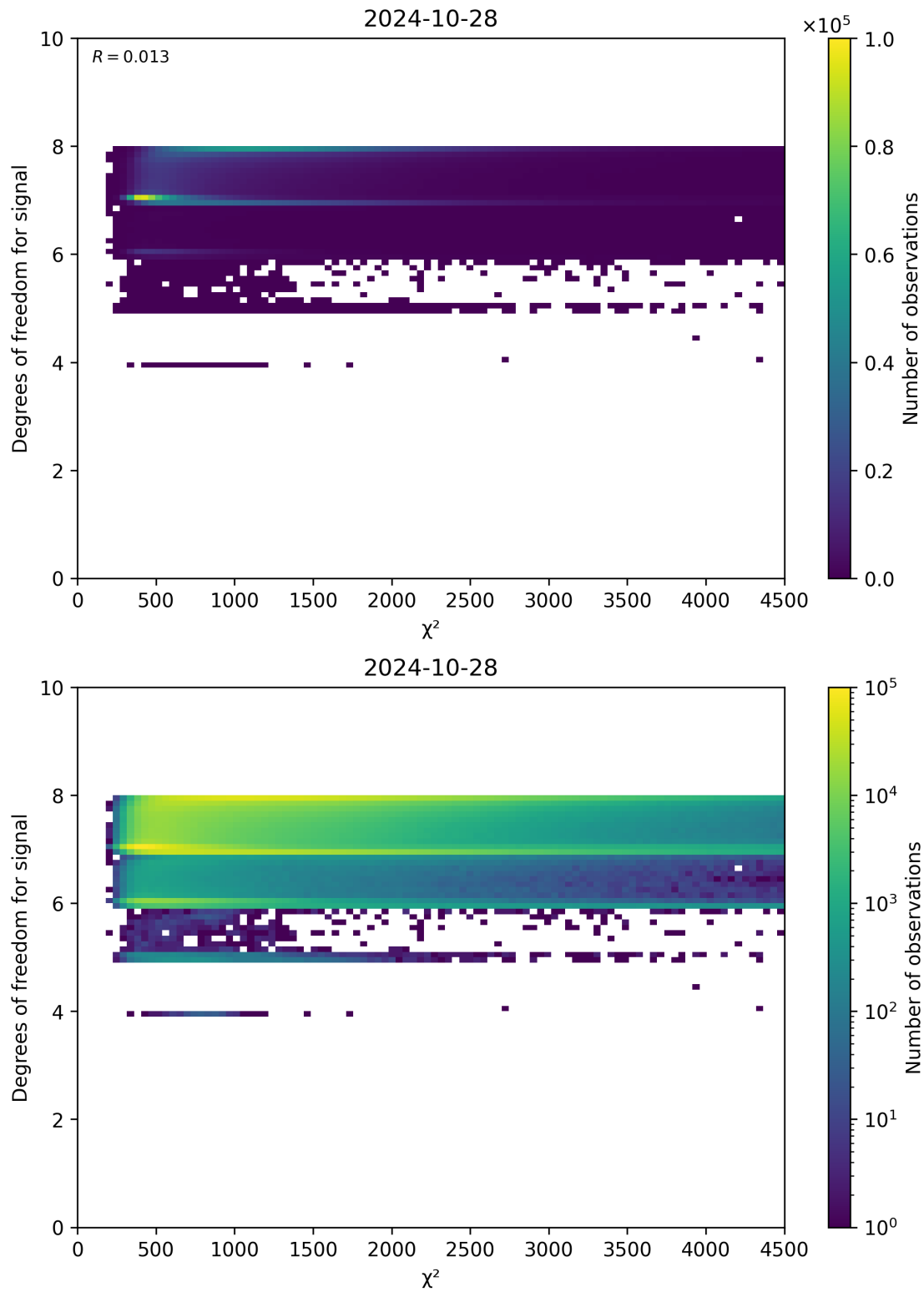
Figure 48: Scatter density plot of “ \chi^2 ” against “Degrees of freedom for signal” for 2024-10-27 to 2024-10-29.
