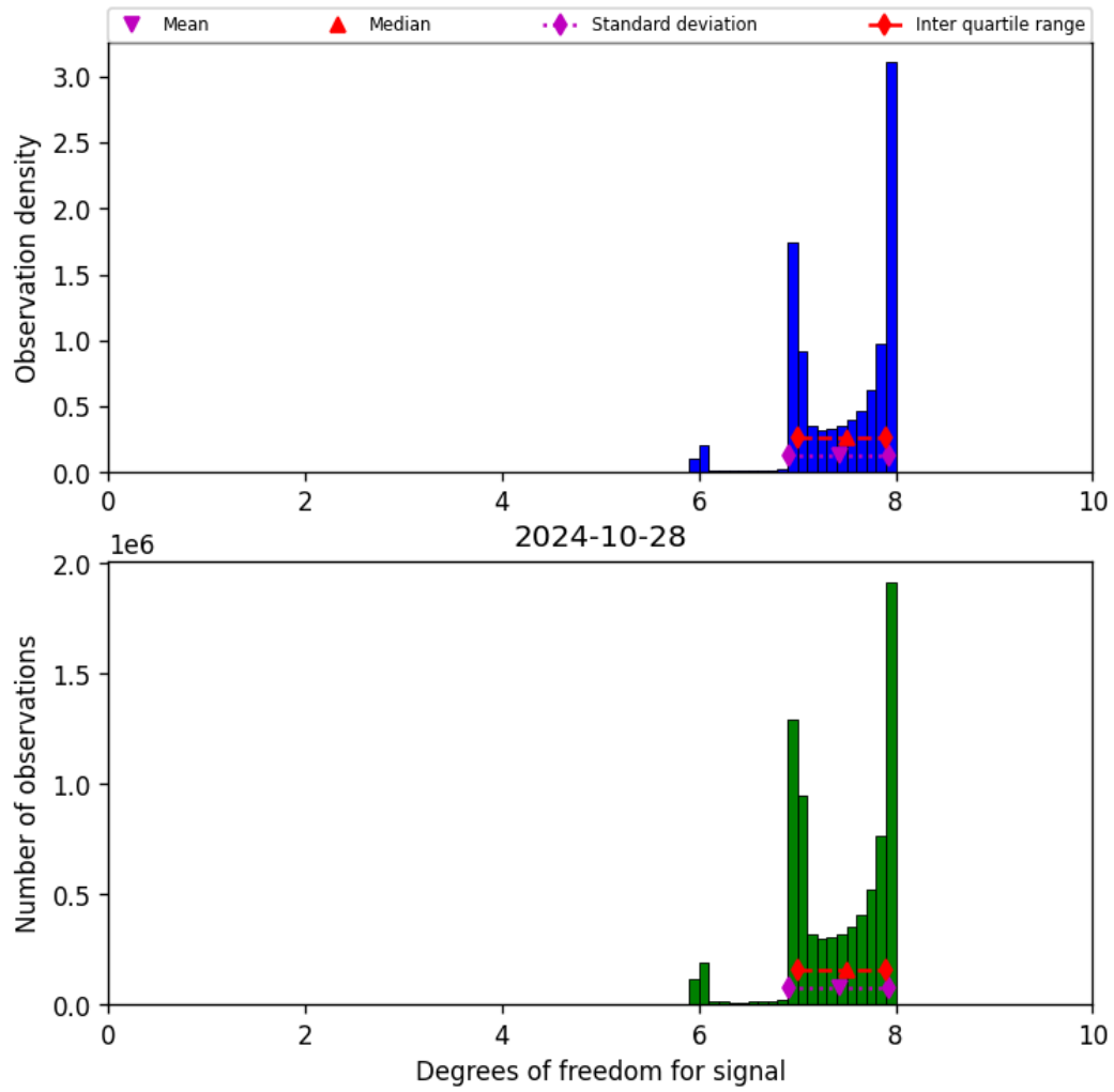
Figure 23: Histogram of “Degrees of freedom for signal” for 2024-10-27 to 2024-10-29
