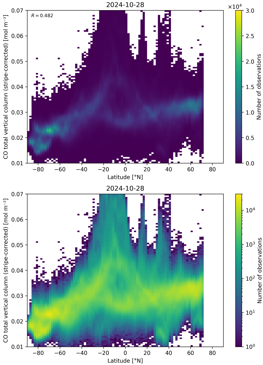
Figure 52: Scatter density plot of “Latitude” against “CO total vertical column (stripe-corrected)” for 2024-10-27 to 2024-10-29.
