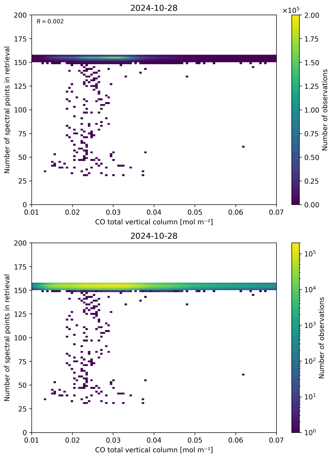
Figure 43: Scatter density plot of “CO total vertical column” against “Number of spectral points in retrieval” for 2024-10-27 to 2024-10-29.
