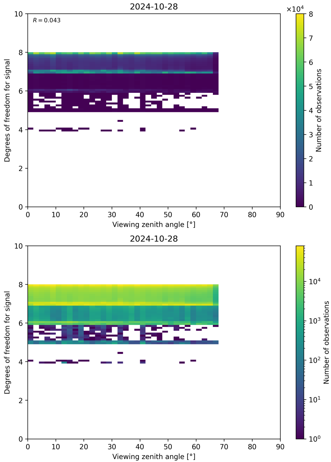
Figure 73: Scatter density plot of “Viewing zenith angle” against “Degrees of freedom for signal” for 2024-10-27 to 2024-10-29.
