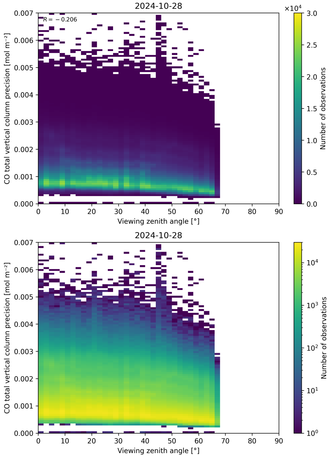
Figure 71: Scatter density plot of “Viewing zenith angle” against “CO total vertical column precision” for 2024-10-27 to 2024-10-29.
