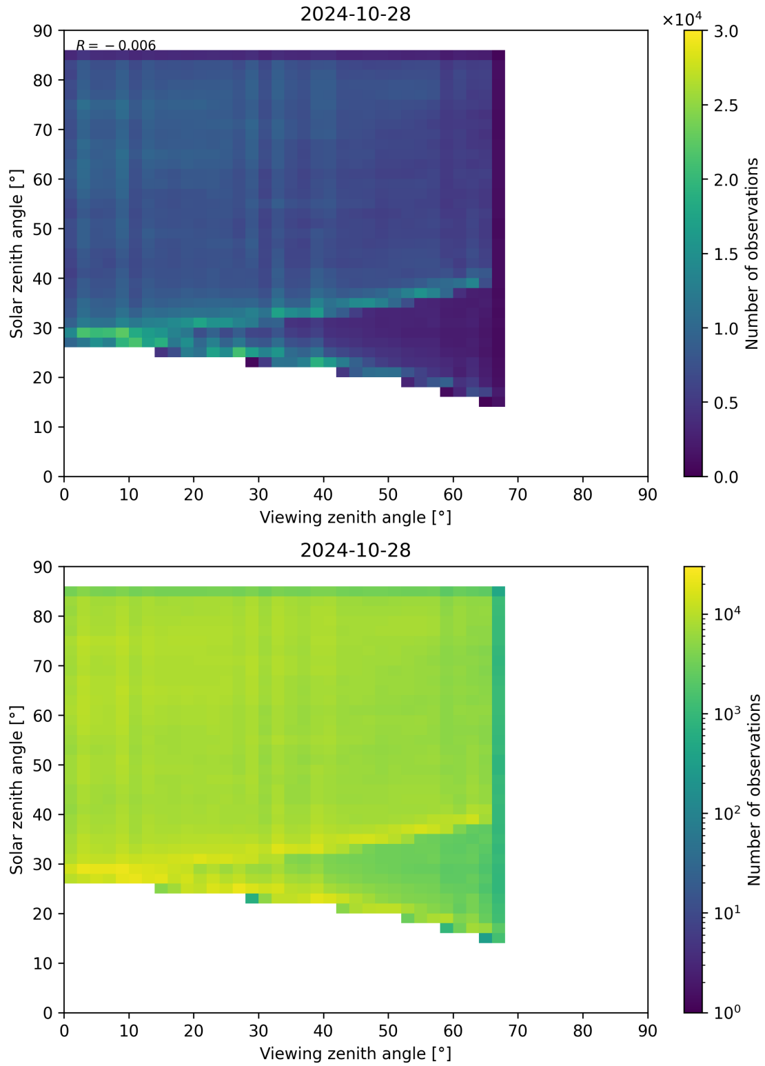
Figure 77: Scatter density plot of “Viewing zenith angle” against “Solar zenith angle” for 2024-10-27 to 2024-10-29.
