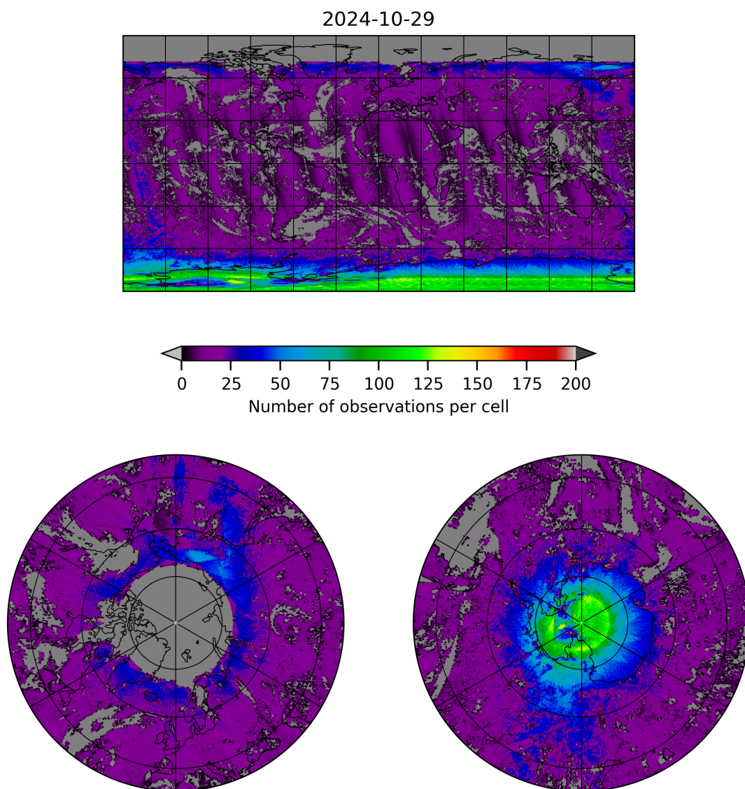
Figure 8: Map of the number of observations for 2024-10-29 to 2024-10-30
