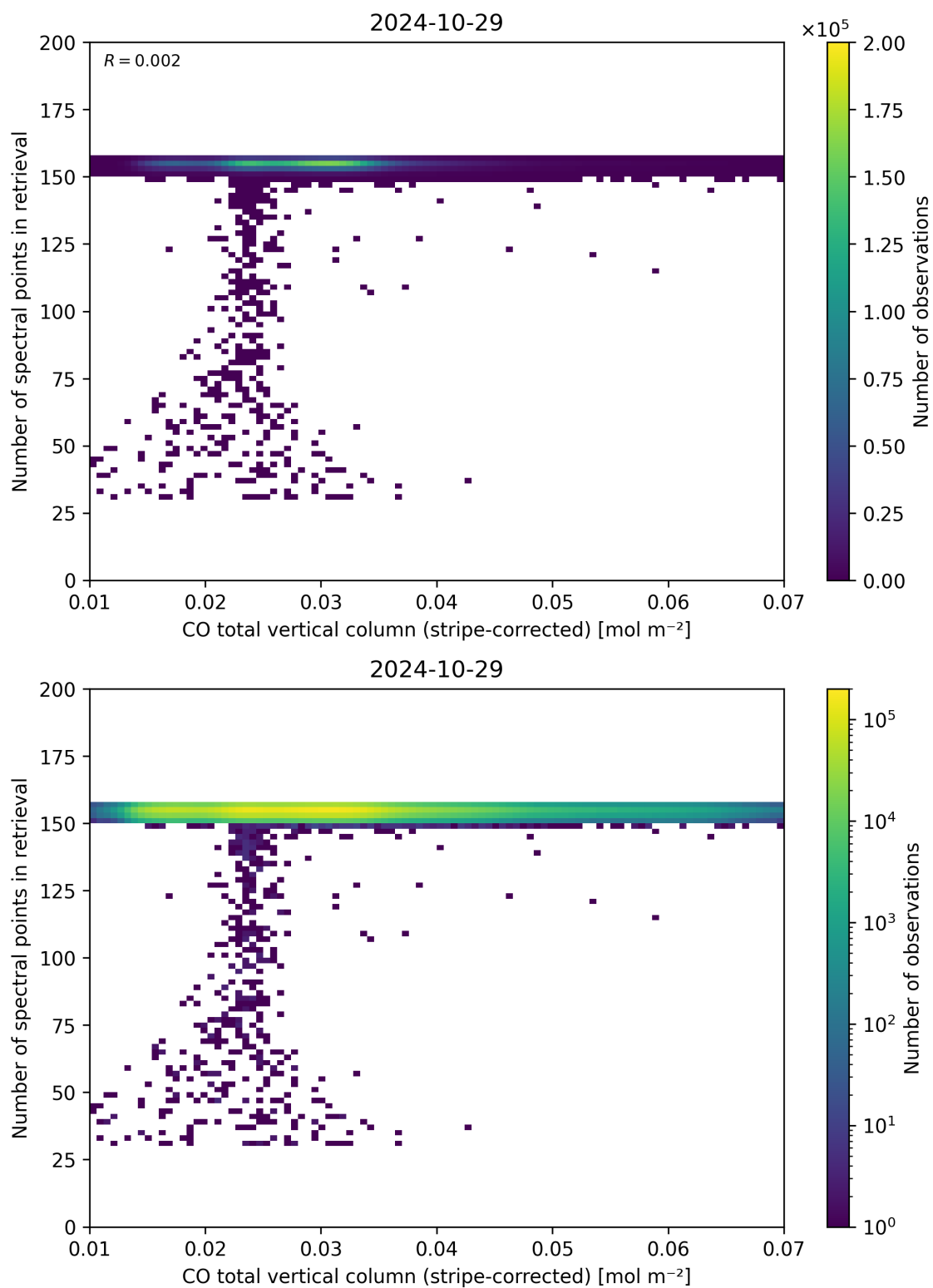
Figure 40: Scatter density plot of “CO total vertical column (stripe-corrected)” against “Number of spectral points in retrieval” for 2024-10-29 to 2024-10-30.
