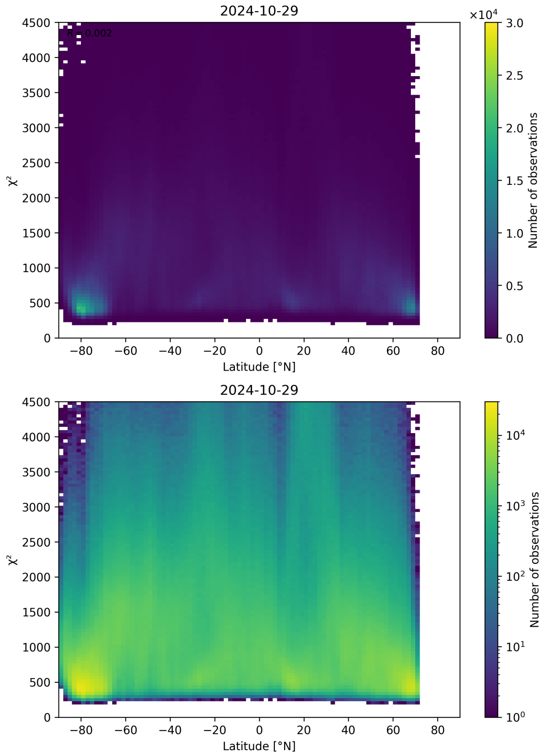
Figure 54: Scatter density plot of “Latitude” against “ \chi^2 ” for 2024-10-29 to 2024-10-30.
