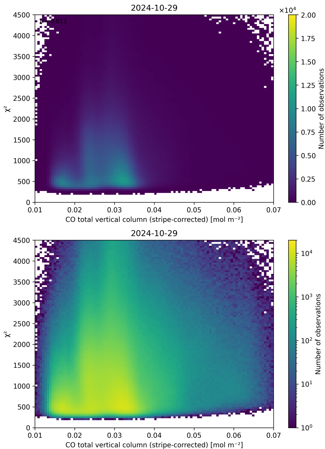
Figure 37: Scatter density plot of “CO total vertical column (stripe-corrected)” against “ \chi^2 ” for 2024-10-29 to 2024-10-30.
