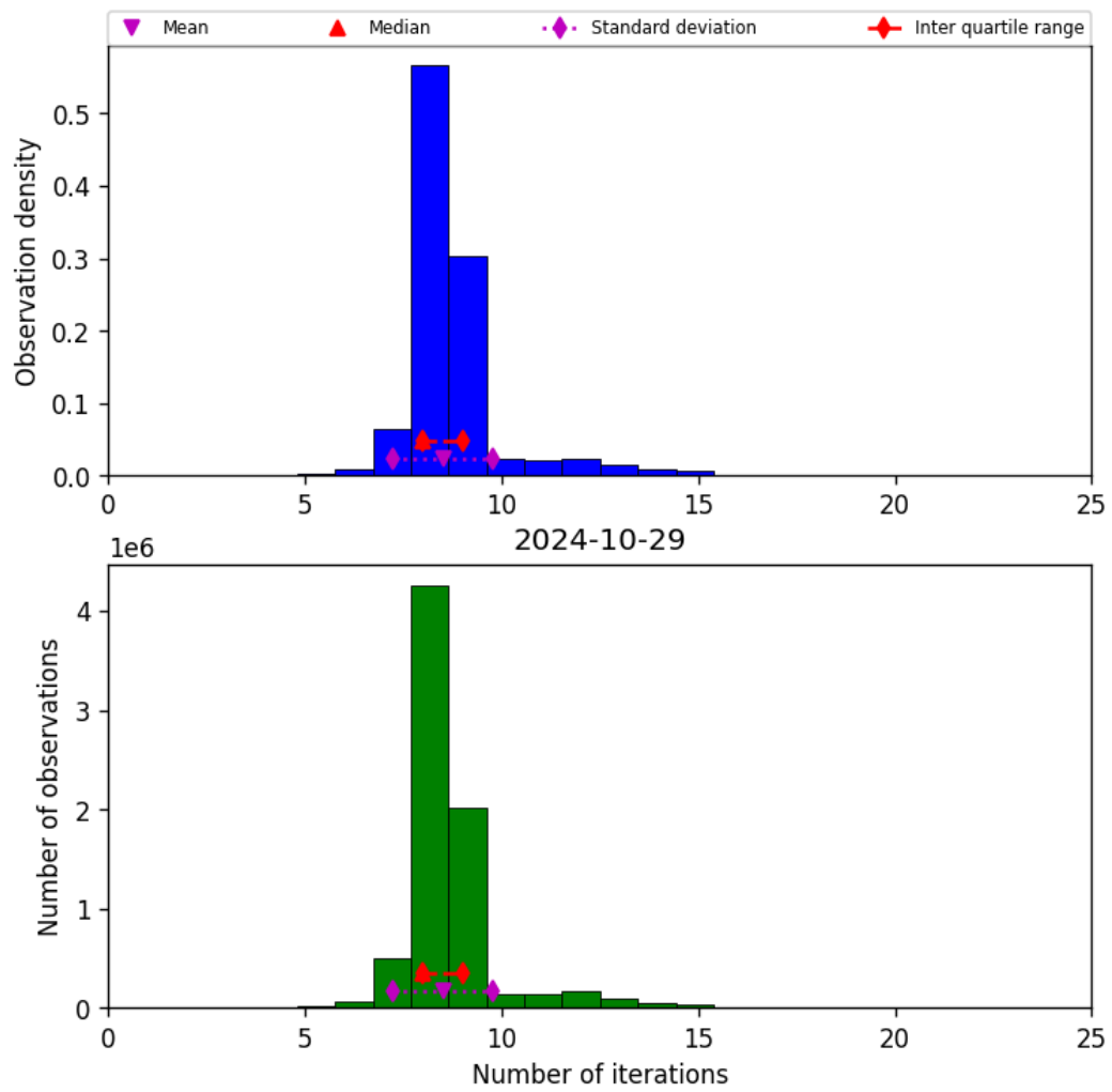
Figure 24: Histogram of “Number of iterations” for 2024-10-29 to 2024-10-30
