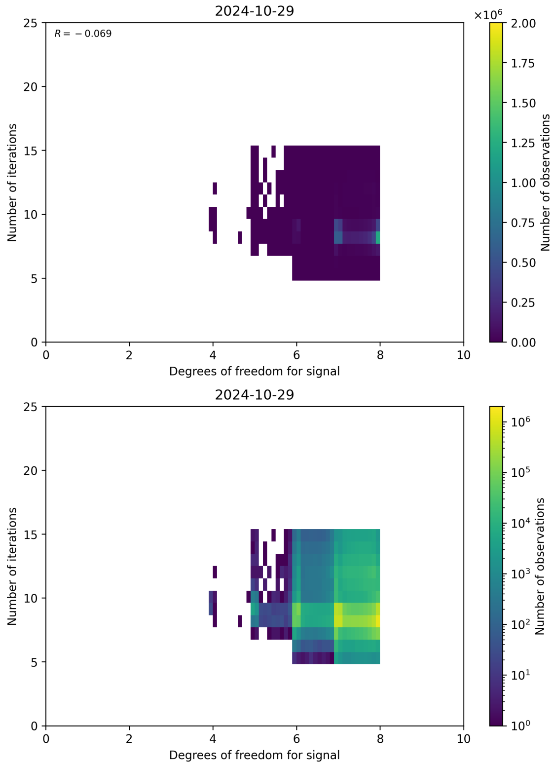
Figure 50: Scatter density plot of “Degrees of freedom for signal” against “Number of iterations” for 2024-10-29 to 2024-10-30.
