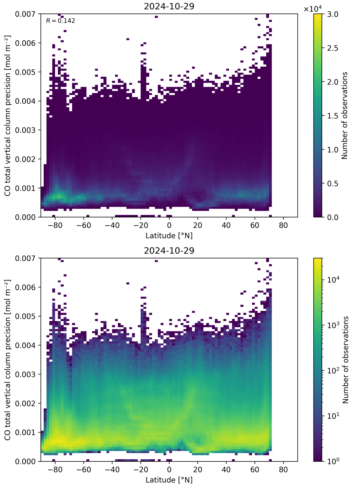
Figure 53: Scatter density plot of “Latitude” against “CO total vertical column precision” for 2024-10-29 to 2024-10-30.
