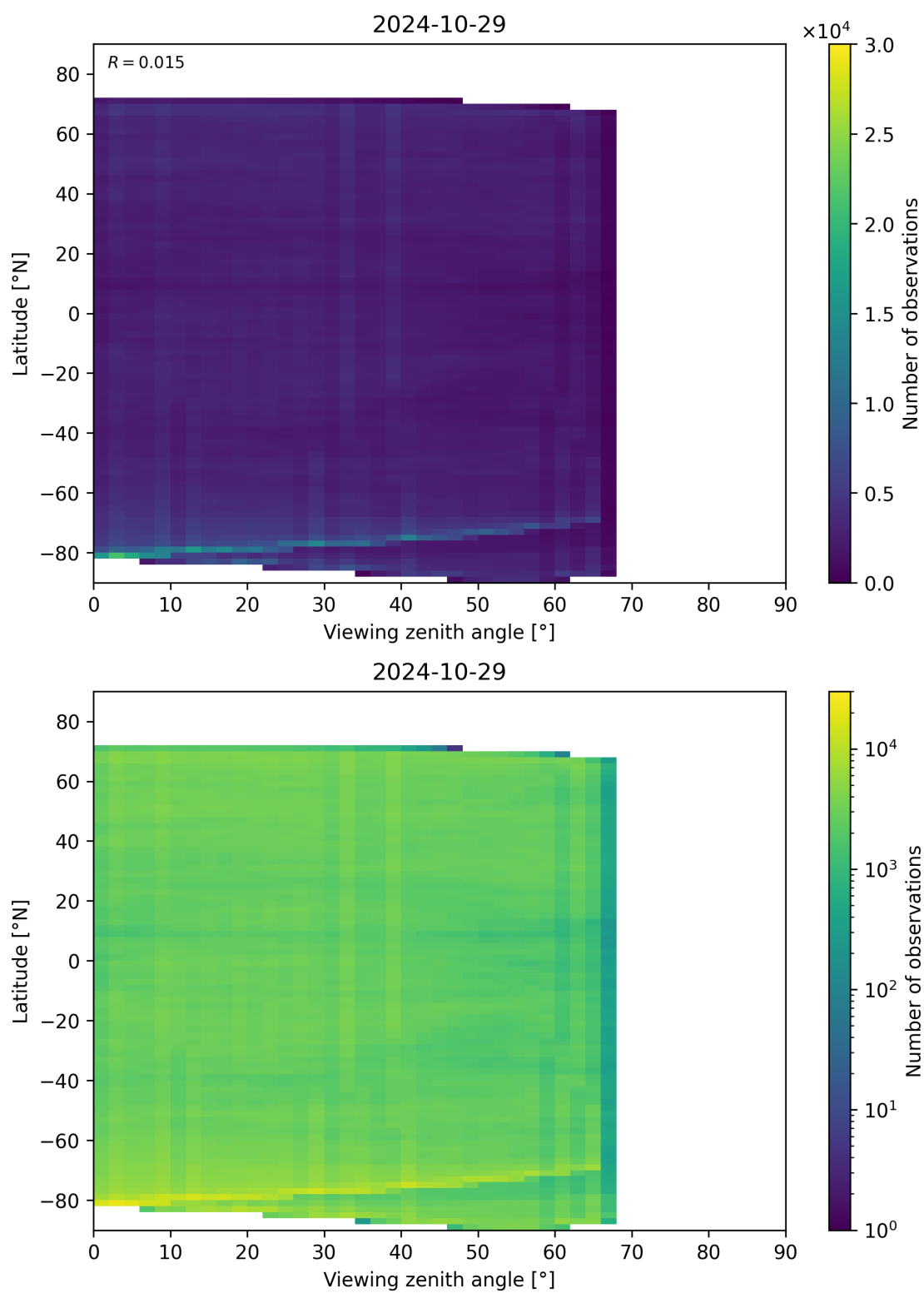
Figure 74: Scatter density plot of “Viewing zenith angle” against “Latitude” for 2024-10-29 to 2024-10-30.
