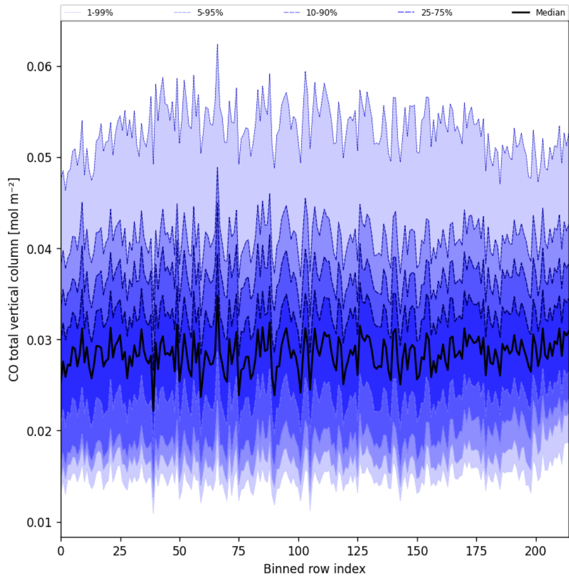
Figure 26: Along track statistics of “CO total vertical column” for 2024-10-29 to 2024-10-30
