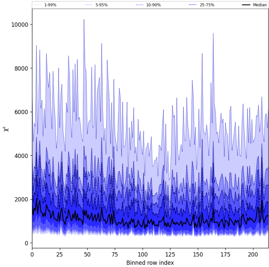
Figure 30: Along track statistics of “ \chi^2 ” for 2024-10-29 to 2024-10-30
