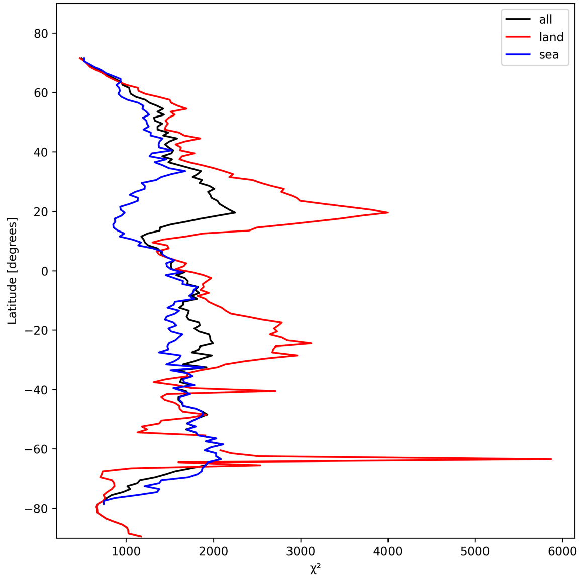
Figure 14: Zonal average of “ \chi^2 ” for 2024-10-29 to 2024-10-30.
