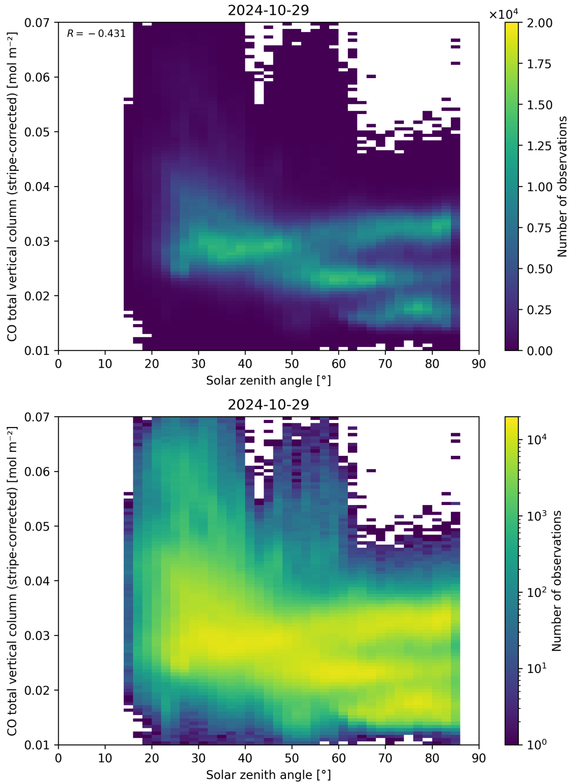
Figure 62: Scatter density plot of “Solar zenith angle” against “CO total vertical column (stripe-corrected)” for 2024-10-29 to 2024-10-30.
