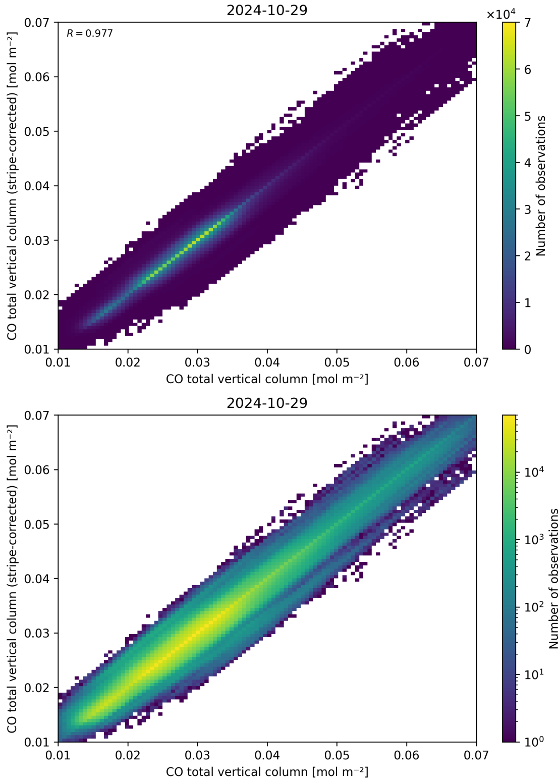
Figure 33: Scatter density plot of “CO total vertical column” against “CO total vertical column (stripe-corrected)” for 2024-10-29 to 2024-10-30.
