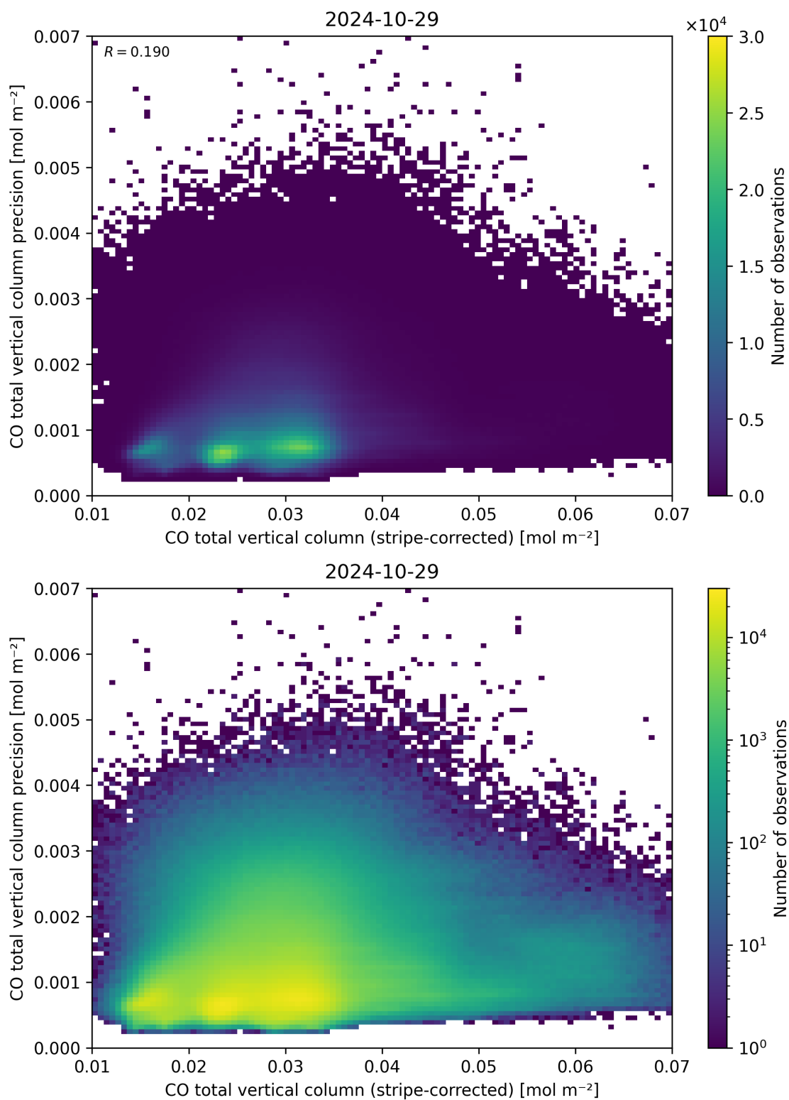
Figure 36: Scatter density plot of “CO total vertical column (stripe-corrected)” against “CO total vertical column precision” for 2024-10-29 to 2024-10-30.
