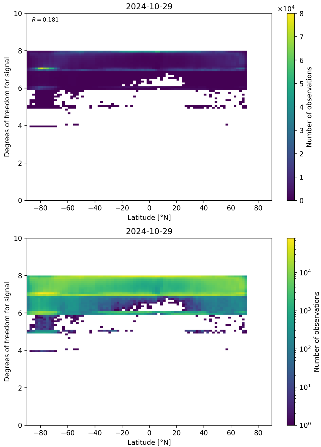
Figure 55: Scatter density plot of “Latitude” against “Degrees of freedom for signal” for 2024-10-29 to 2024-10-30.
