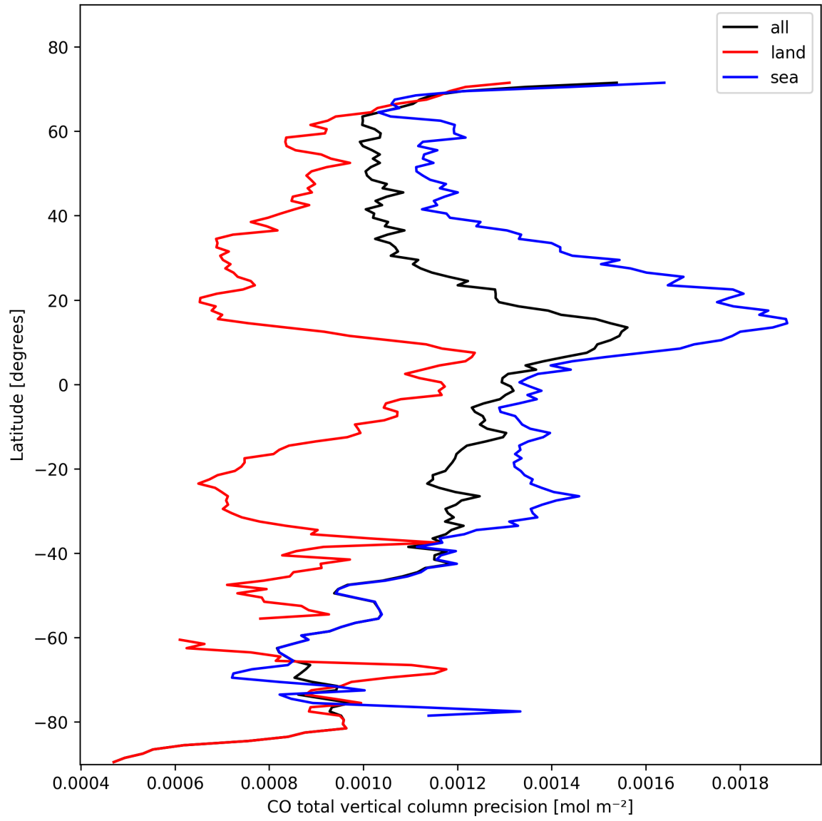
Figure 12: Zonal average of “CO total vertical column precision” for 2024-10-29 to 2024-10-30.
