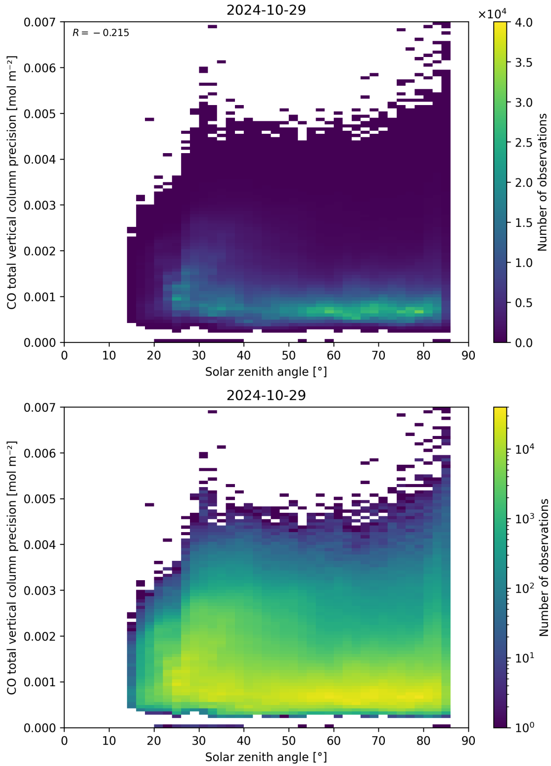
Figure 63: Scatter density plot of “Solar zenith angle” against “CO total vertical column precision” for 2024-10-29 to 2024-10-30.
