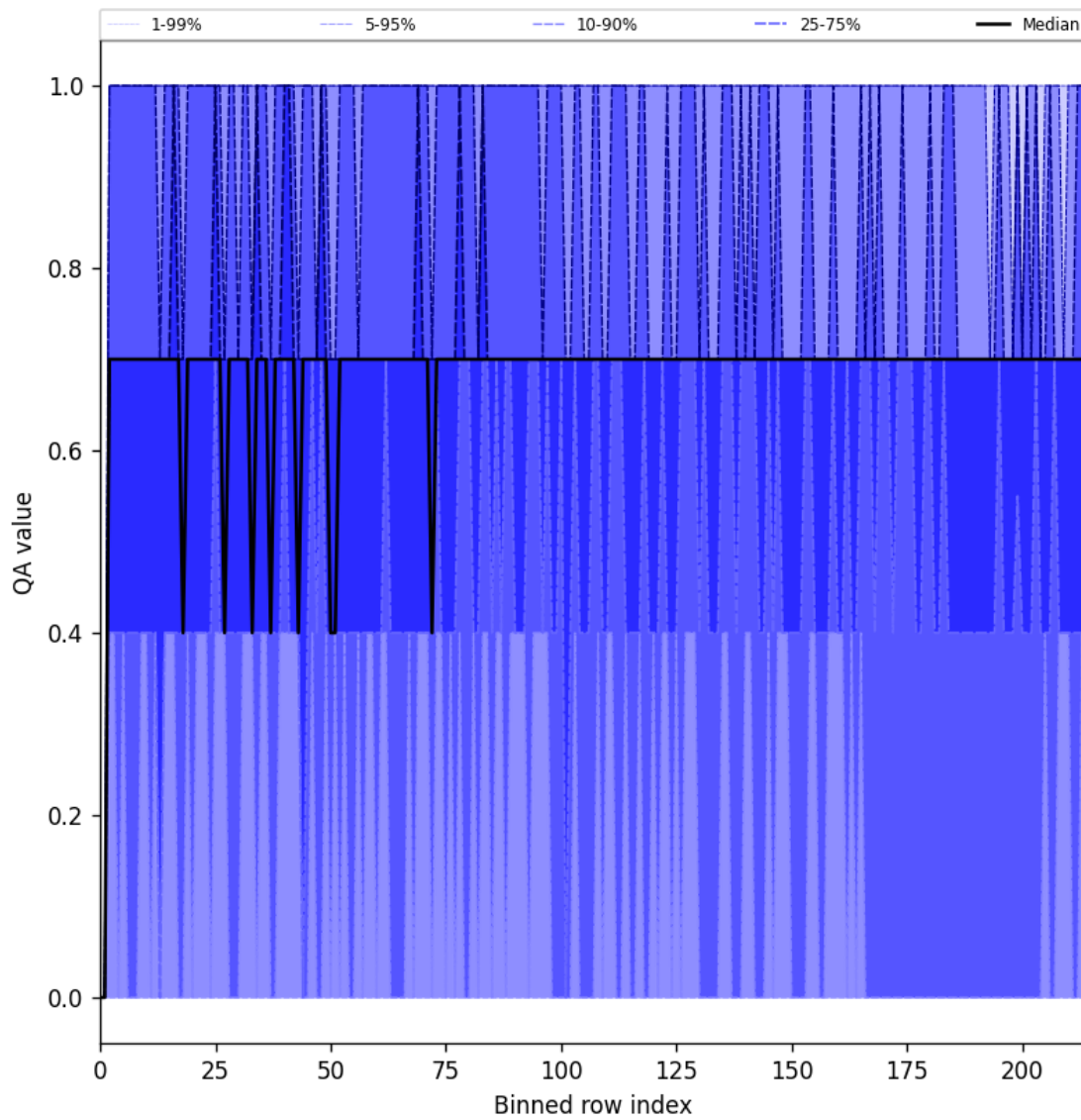
Figure 25: Along track statistics of “QA value” for 2024-10-29 to 2024-10-30
