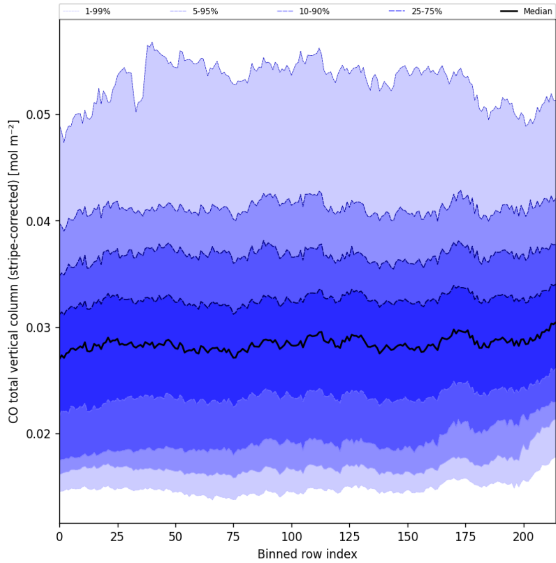
Figure 27: Along track statistics of “CO total vertical column (stripe-corrected)” for 2024-10-29 to 2024-10-30
