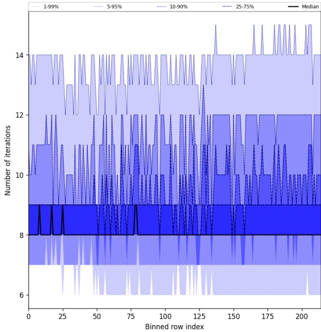
Figure 32: Along track statistics of “Number of iterations” for 2024-10-29 to 2024-10-30
