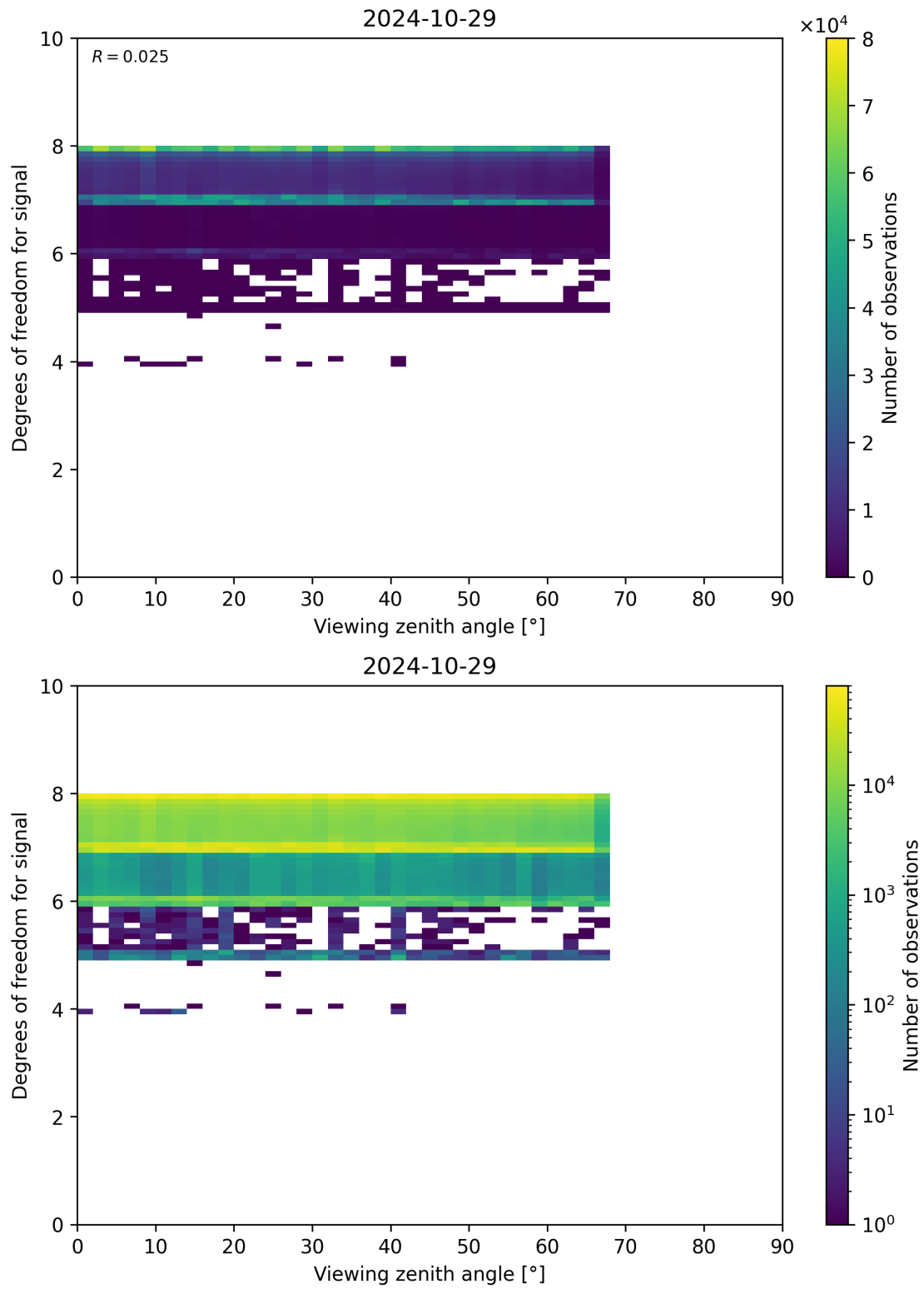
Figure 73: Scatter density plot of “Viewing zenith angle” against “Degrees of freedom for signal” for 2024-10-29 to 2024-10-30.
