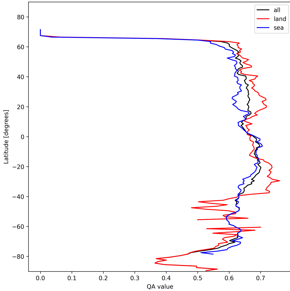
Figure 9: Zonal average of “QA value” for 2024-10-29 to 2024-10-30.
