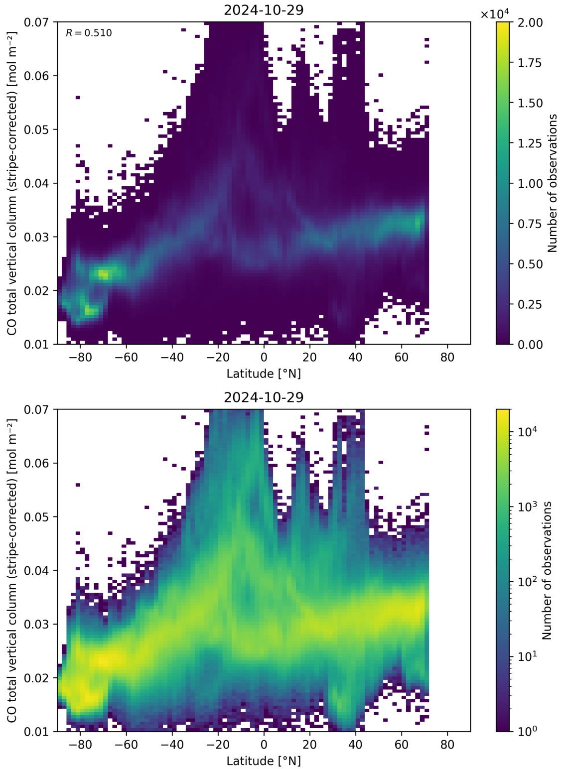
Figure 52: Scatter density plot of “Latitude” against “CO total vertical column (stripe-corrected)” for 2024-10-29 to 2024-10-30.
