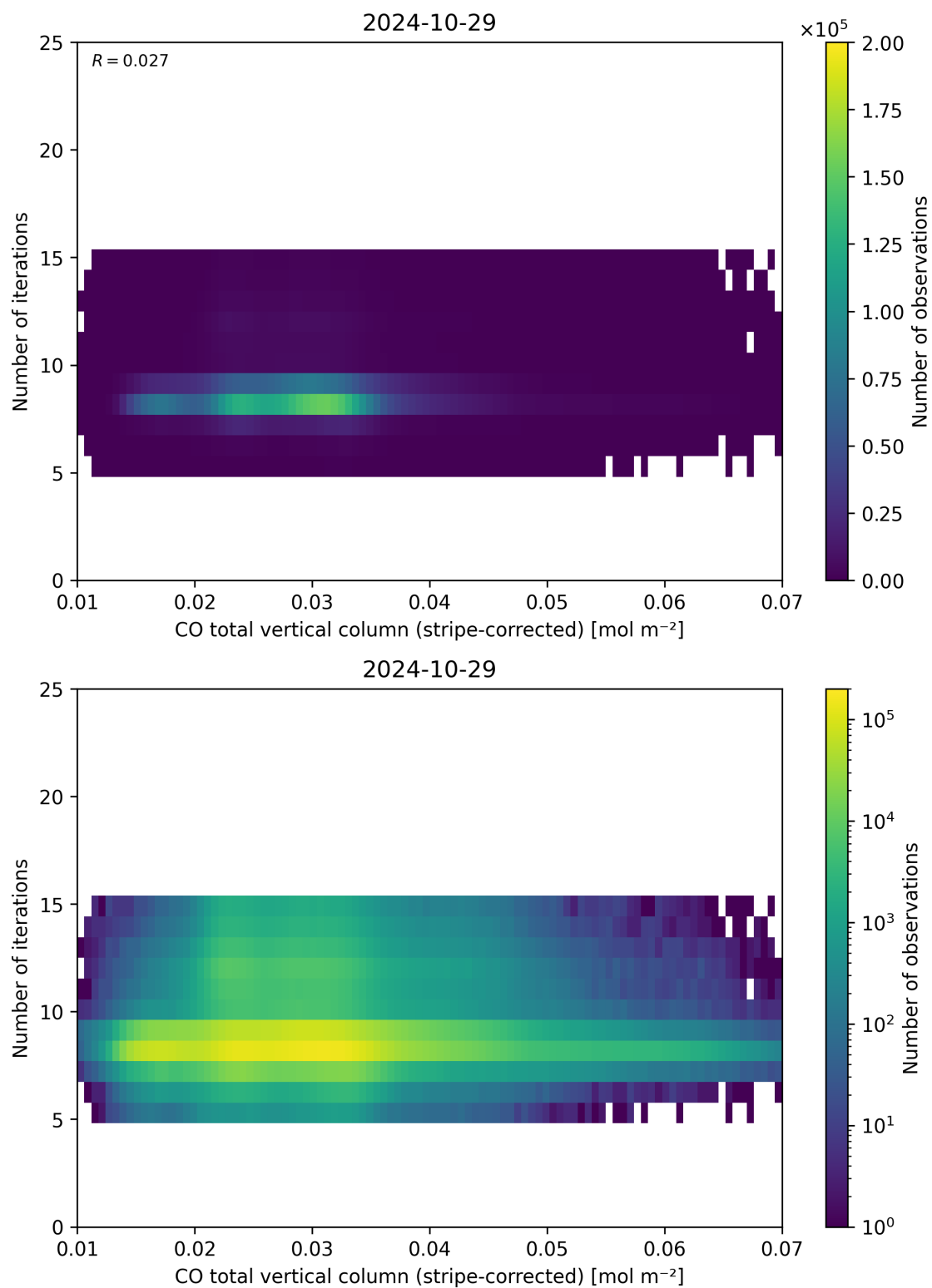
Figure 39: Scatter density plot of “CO total vertical column (stripe-corrected)” against “Number of iterations” for 2024-10-29 to 2024-10-30.
