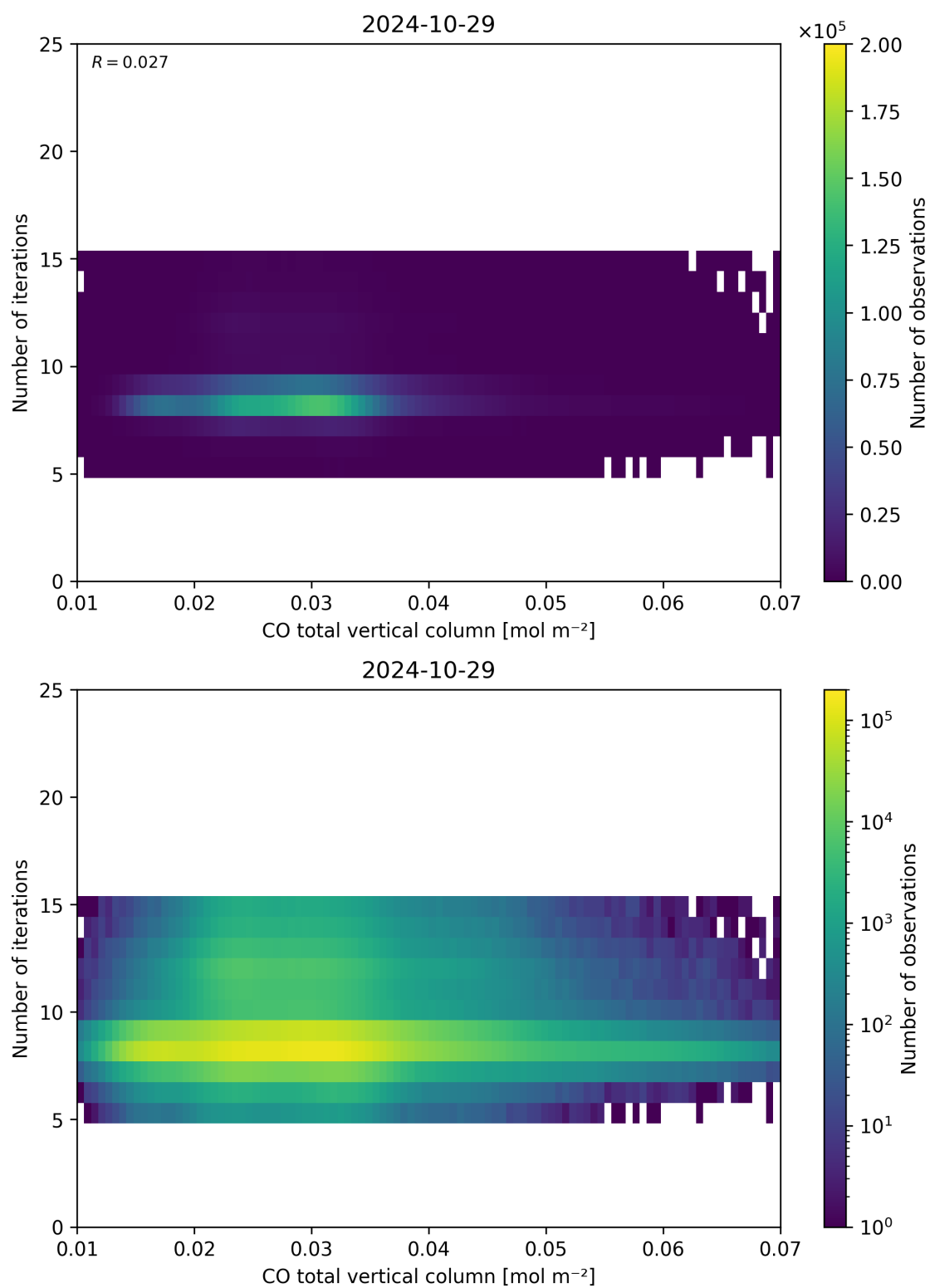
Figure 42: Scatter density plot of “CO total vertical column” against “Number of iterations” for 2024-10-29 to 2024-10-30.
