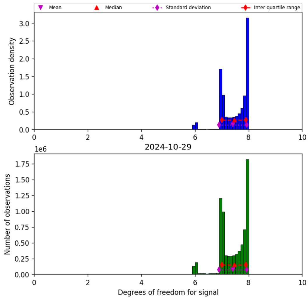
Figure 23: Histogram of “Degrees of freedom for signal” for 2024-10-29 to 2024-10-30
