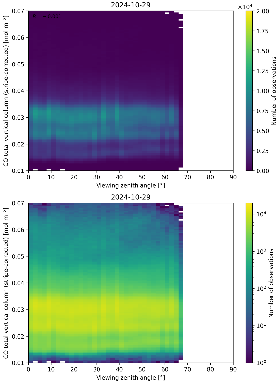
Figure 70: Scatter density plot of “Viewing zenith angle” against “CO total vertical column (stripe-corrected)” for 2024-10-29 to 2024-10-30.
