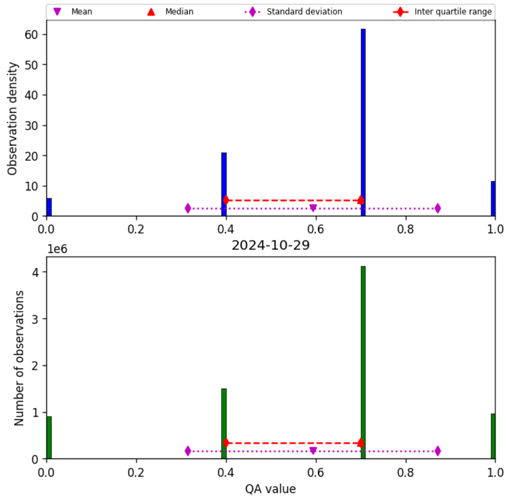
Figure 17: Histogram of “QA value” for 2024-10-29 to 2024-10-30
