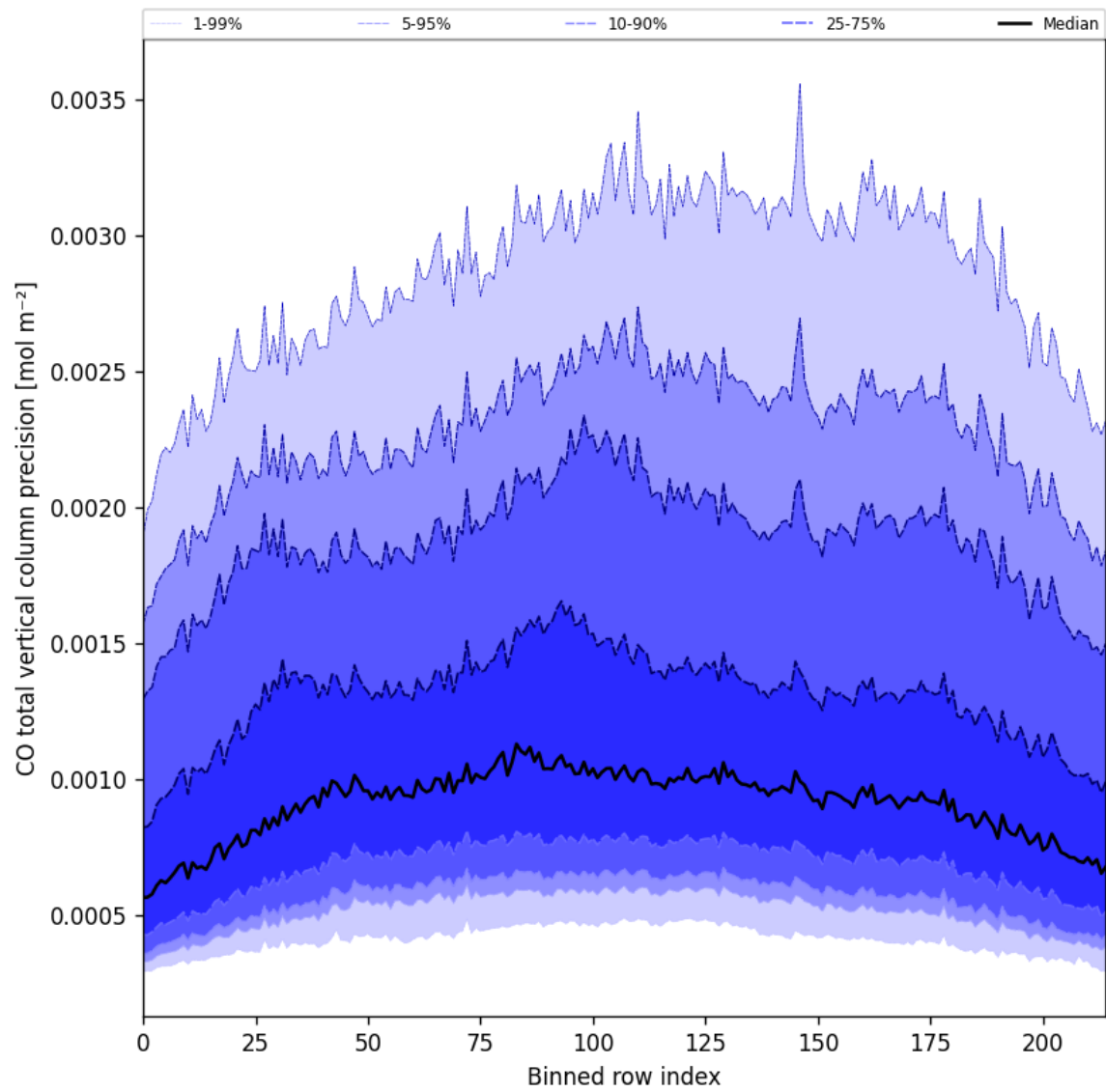
Figure 28: Along track statistics of “CO total vertical column precision” for 2024-10-29 to 2024-10-30
