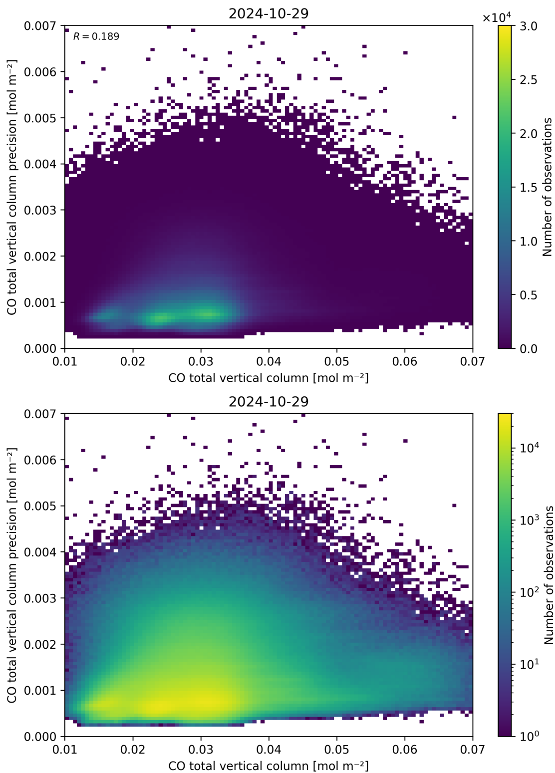
Figure 34: Scatter density plot of “CO total vertical column” against “CO total vertical column precision” for 2024-10-29 to 2024-10-30.
