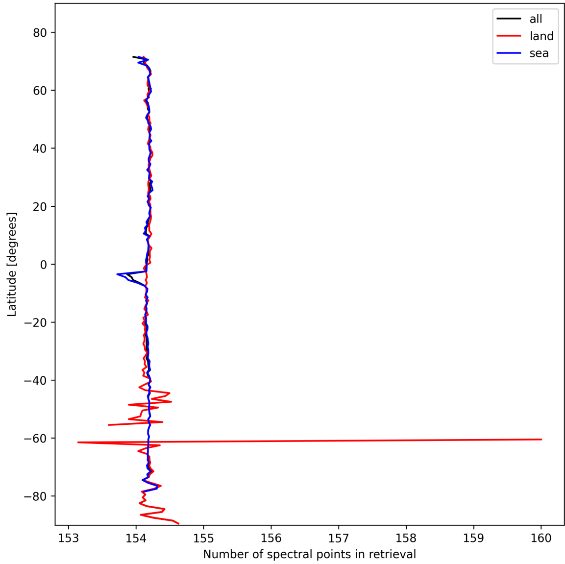
Figure 13: Zonal average of “Number of spectral points in retrieval” for 2024-10-29 to 2024-10-30.
