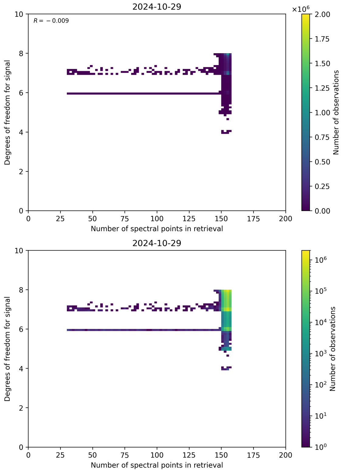
Figure 59: Scatter density plot of “Number of spectral points in retrieval” against “Degrees of freedom for signal” for 2024-10-29 to 2024-10-30.
