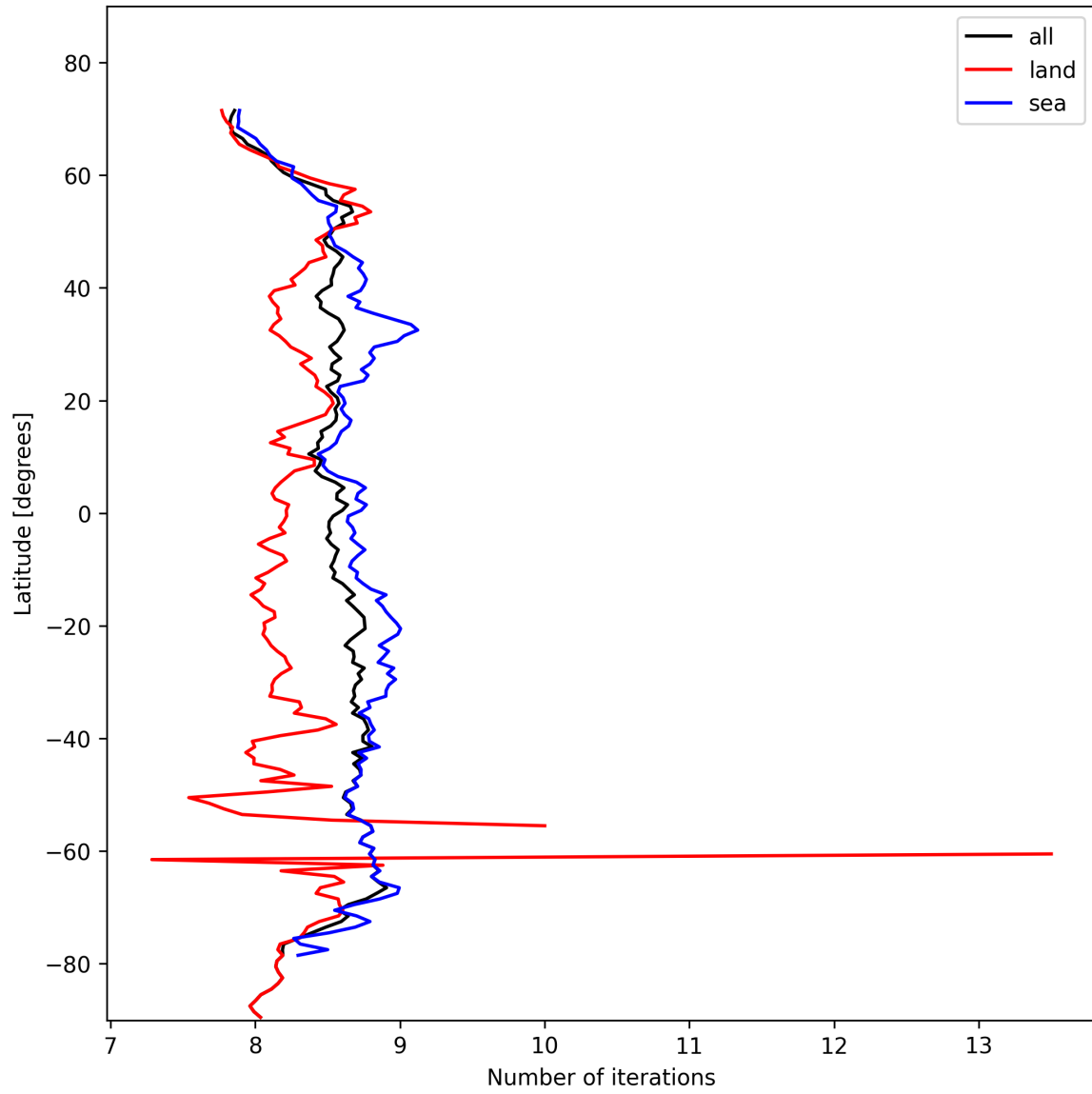
Figure 16: Zonal average of “Number of iterations” for 2024-10-29 to 2024-10-30.
