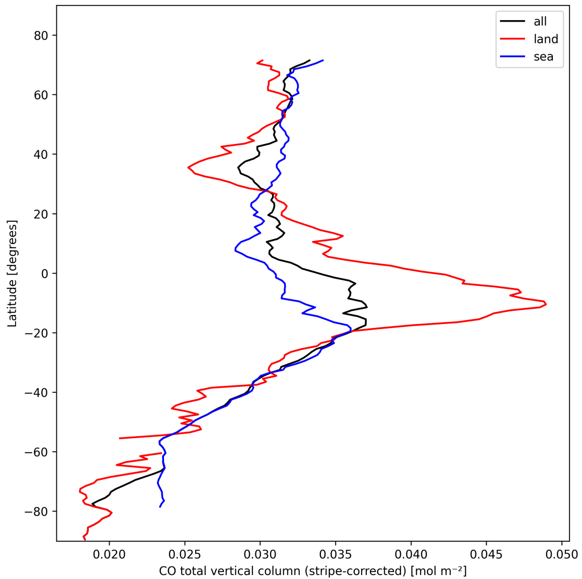
Figure 11: Zonal average of “CO total vertical column (stripe-corrected)” for 2024-10-29 to 2024-10-30.
