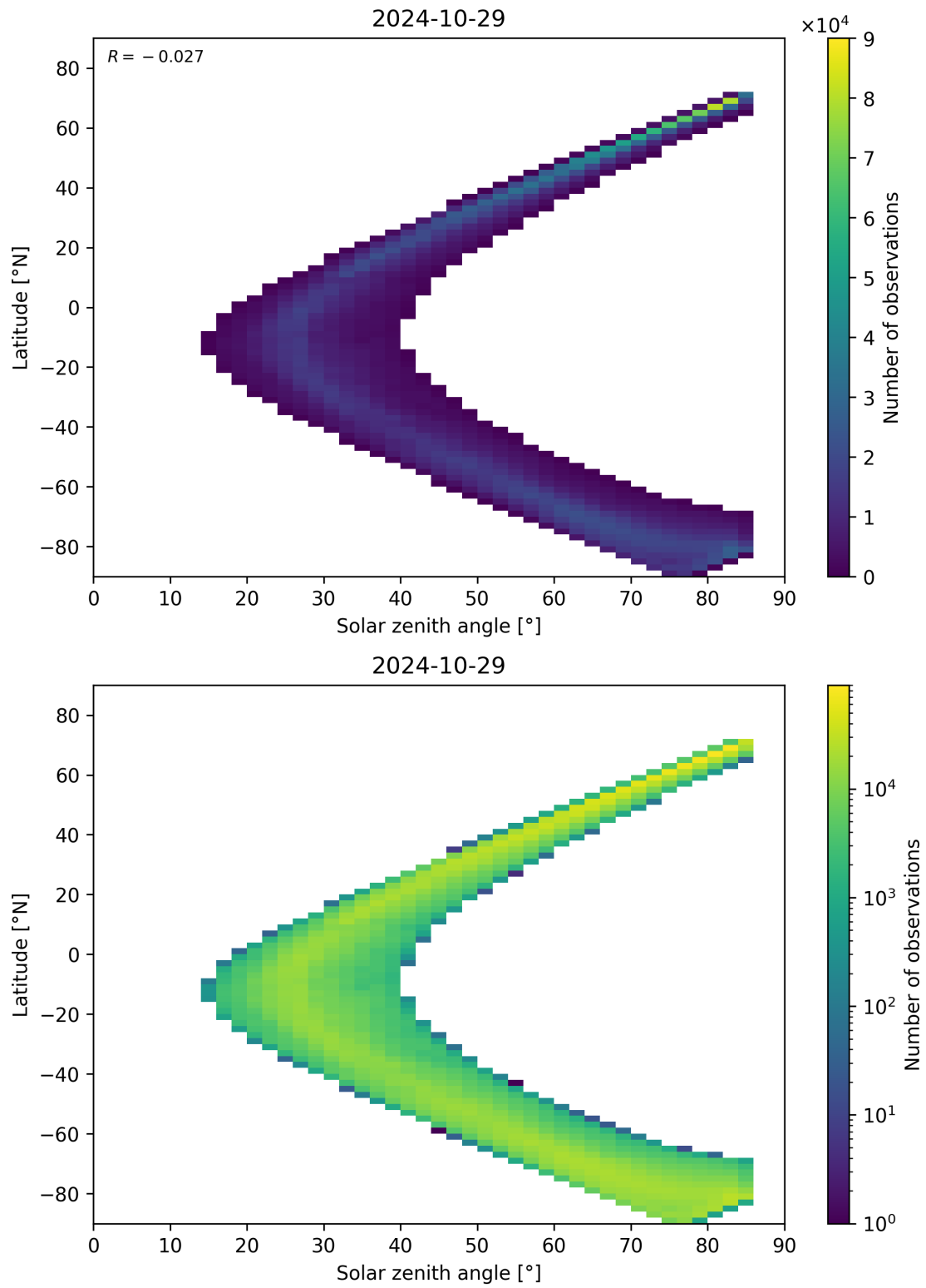
Figure 66: Scatter density plot of “Solar zenith angle” against “Latitude” for 2024-10-29 to 2024-10-30.
