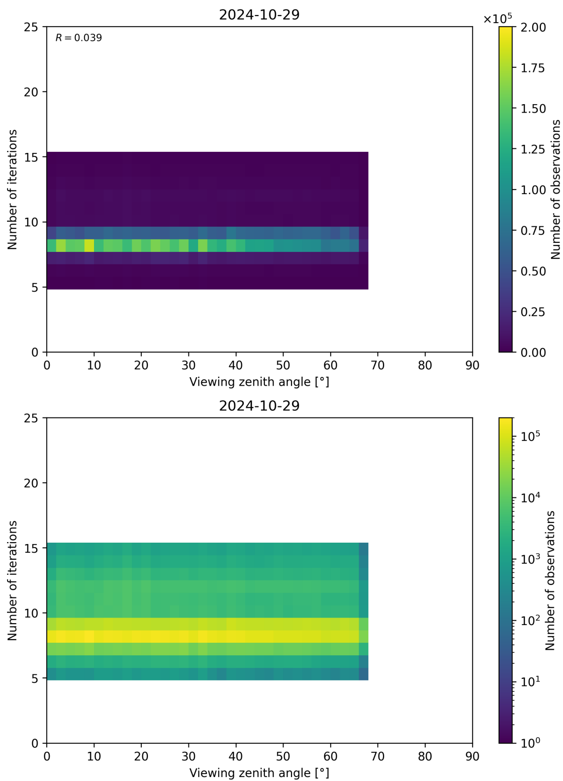
Figure 75: Scatter density plot of “Viewing zenith angle” against “Number of iterations” for 2024-10-29 to 2024-10-30.
