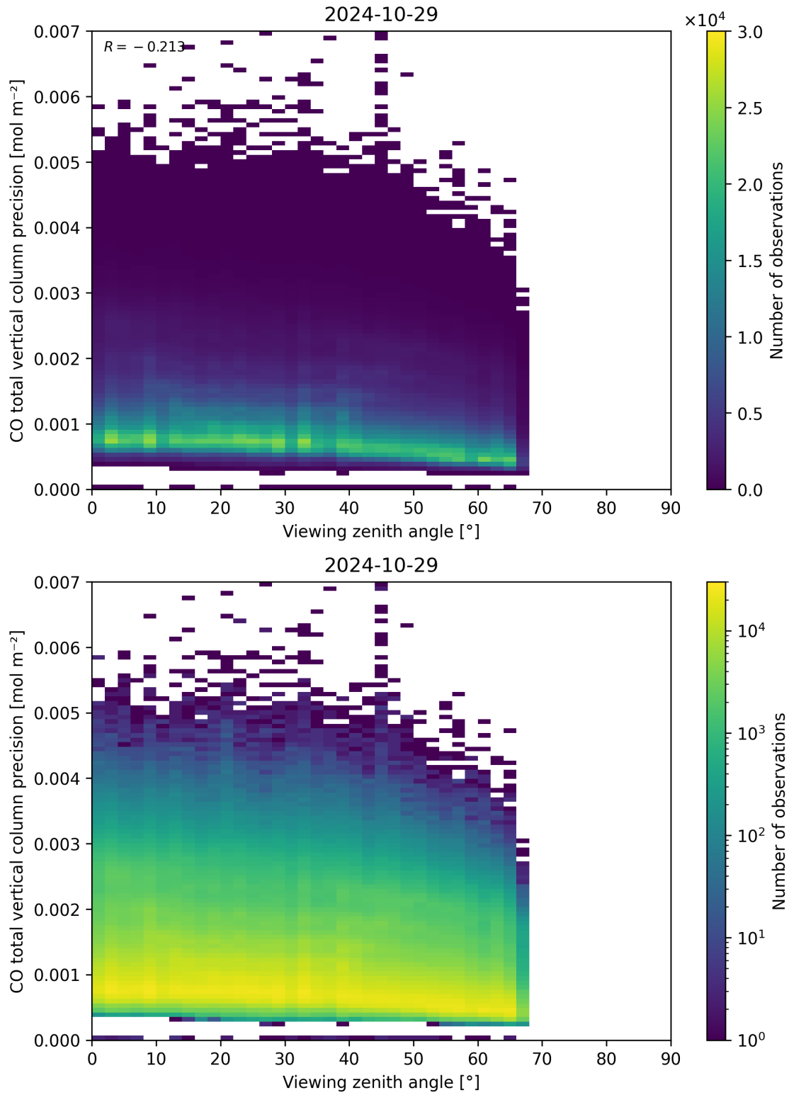
Figure 71: Scatter density plot of “Viewing zenith angle” against “CO total vertical column precision” for 2024-10-29 to 2024-10-30.
