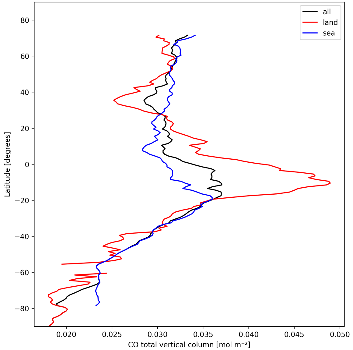
Figure 10: Zonal average of “CO total vertical column” for 2024-10-29 to 2024-10-30.
