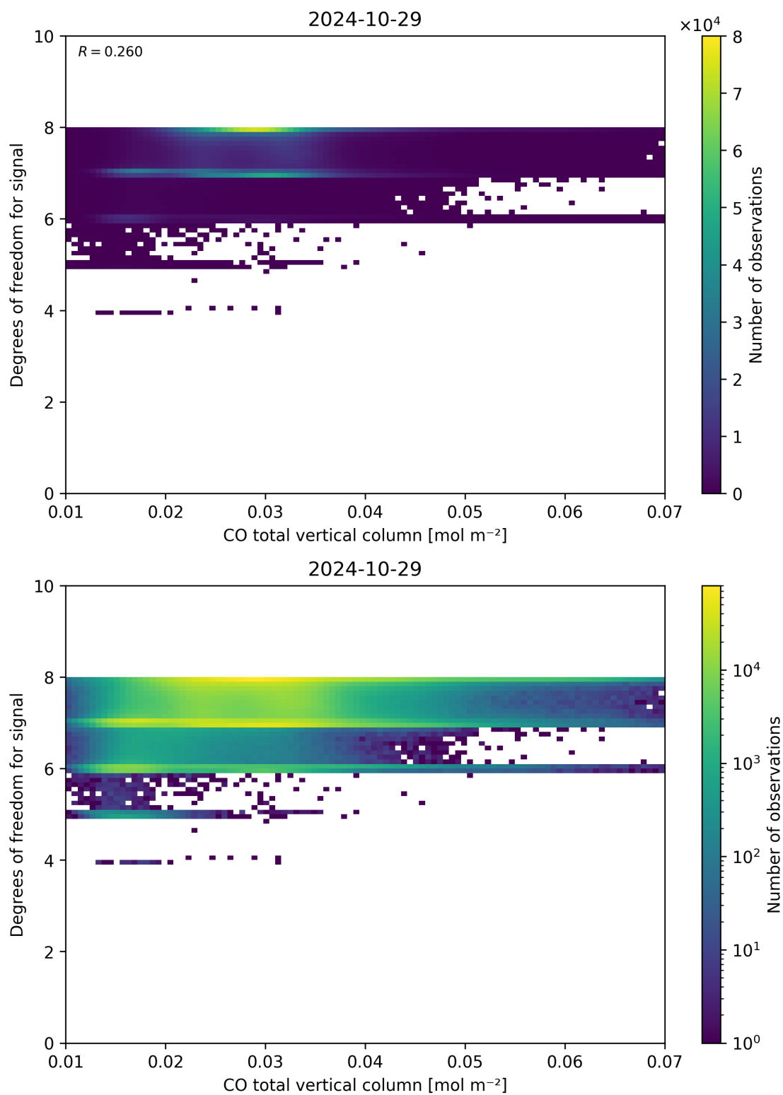
Figure 41: Scatter density plot of “CO total vertical column” against “Degrees of freedom for signal” for 2024-10-29 to 2024-10-30.
