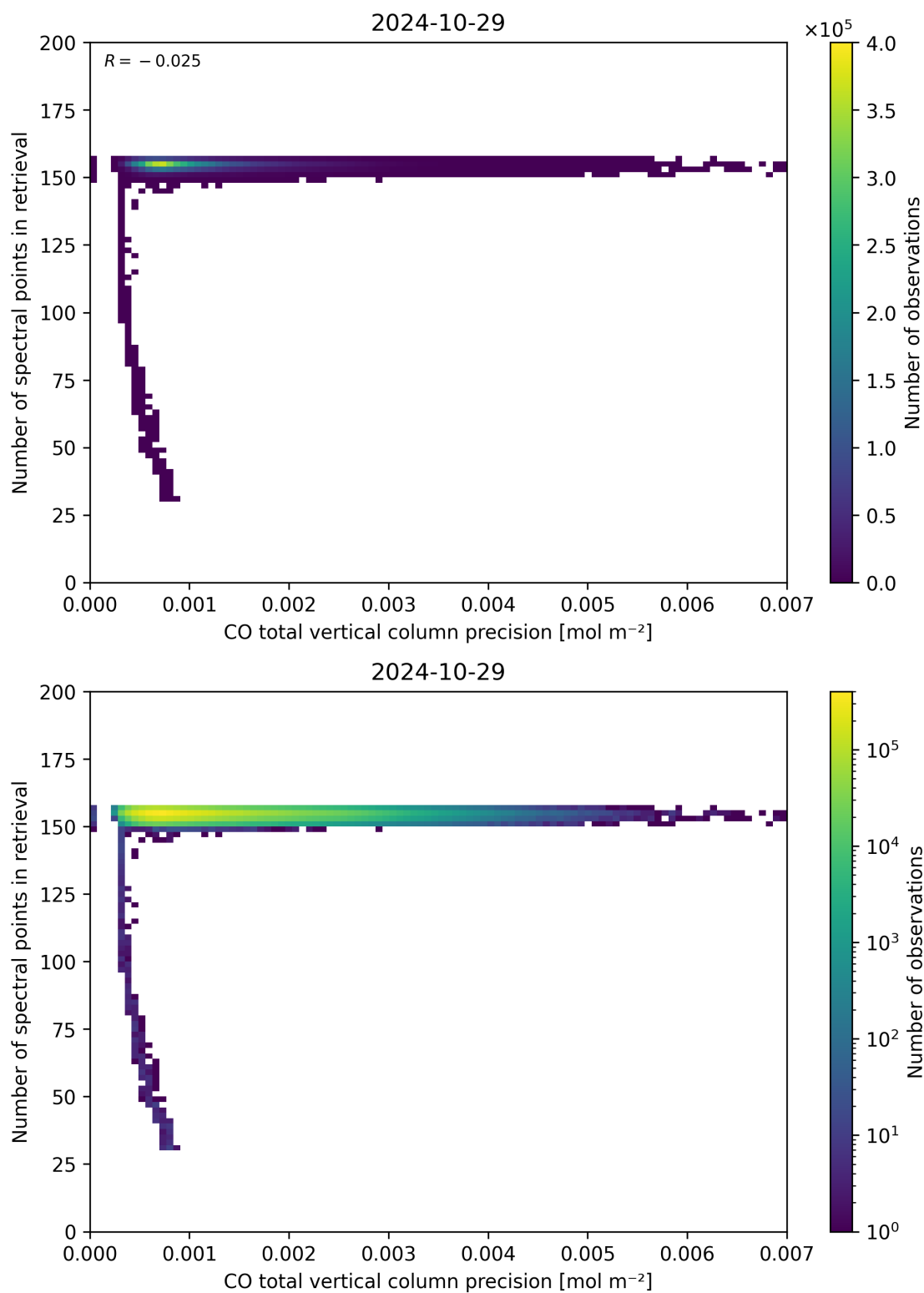
Figure 47: Scatter density plot of “CO total vertical column precision” against “Number of spectral points in retrieval” for 2024-10-29 to 2024-10-30.
