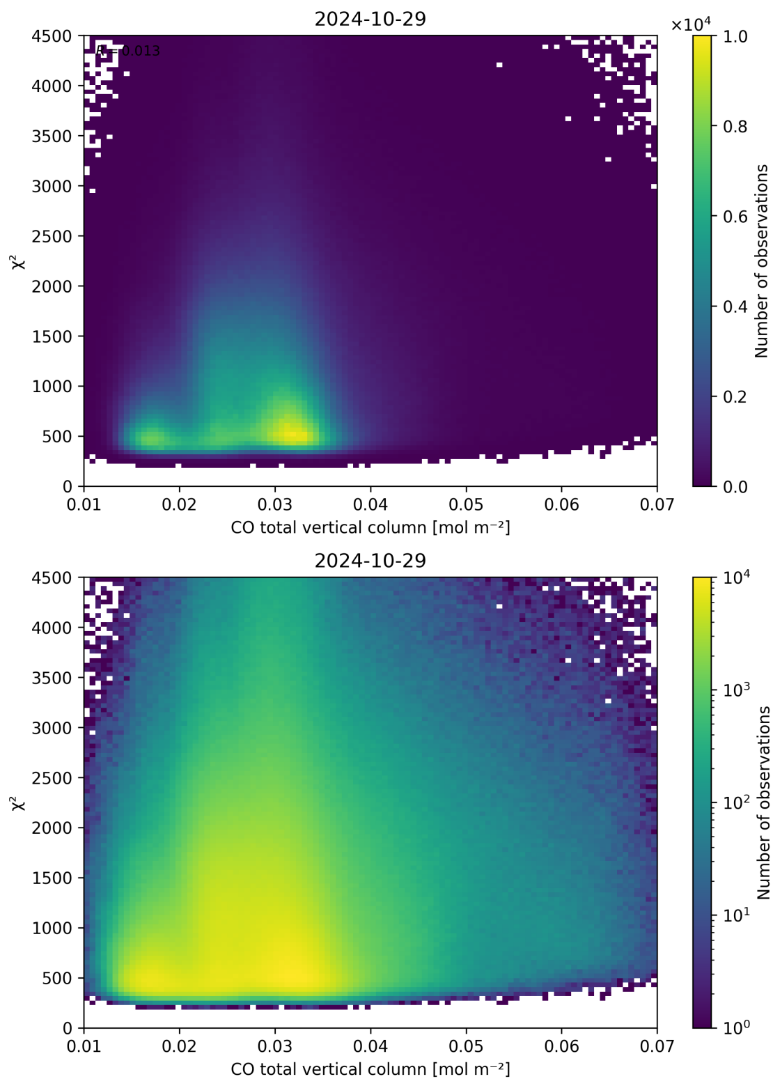
Figure 35: Scatter density plot of “CO total vertical column” against “ \chi^2 ” for 2024-10-29 to 2024-10-30.
