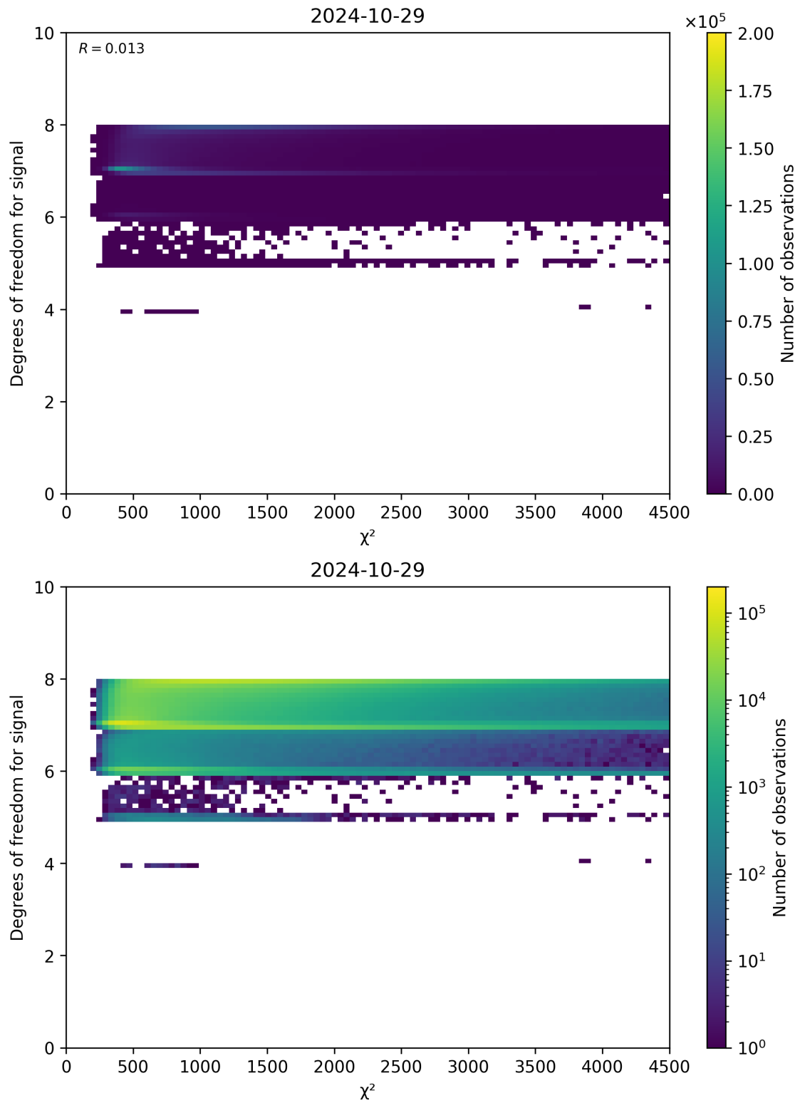
Figure 48: Scatter density plot of “ \chi^2 ” against “Degrees of freedom for signal” for 2024-10-29 to 2024-10-30.
