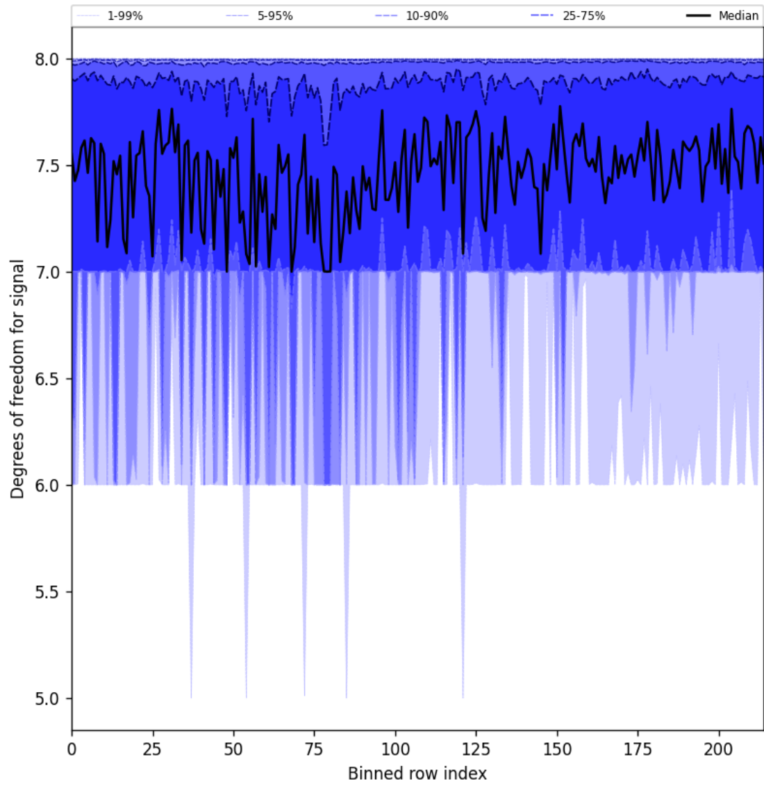
Figure 31: Along track statistics of “Degrees of freedom for signal” for 2024-10-29 to 2024-10-30
