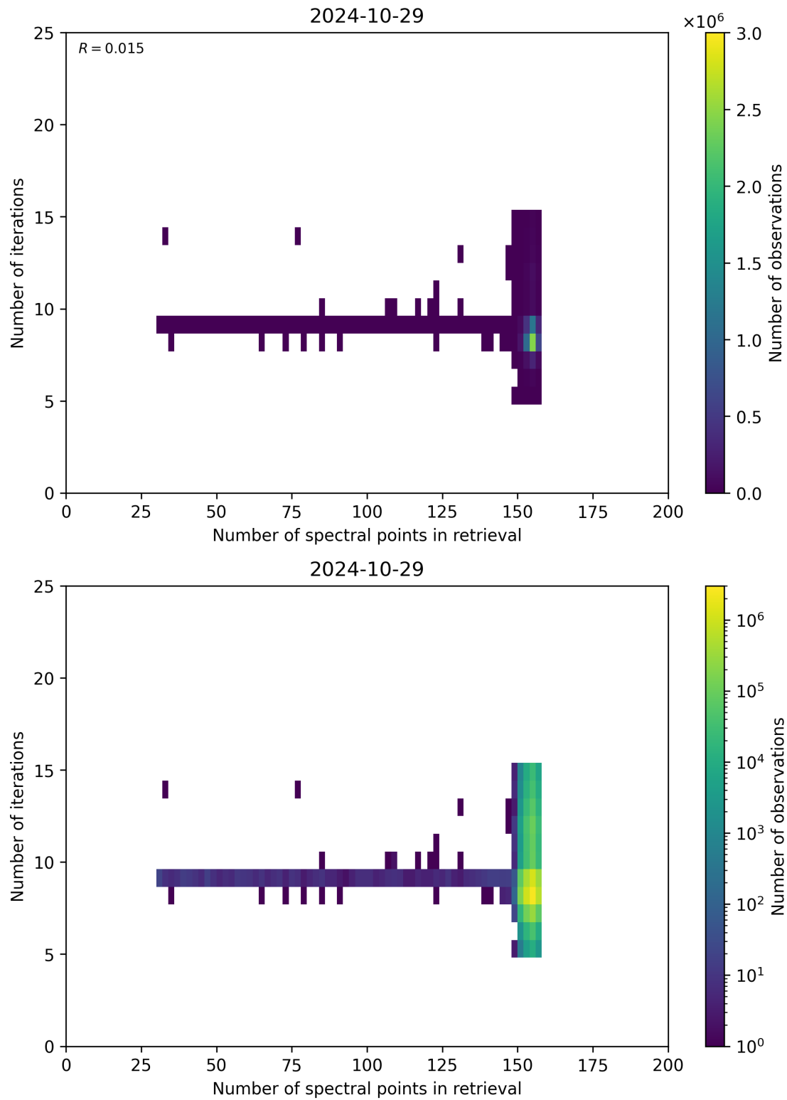
Figure 60: Scatter density plot of “Number of spectral points in retrieval” against “Number of iterations” for 2024-10-29 to 2024-10-30.
