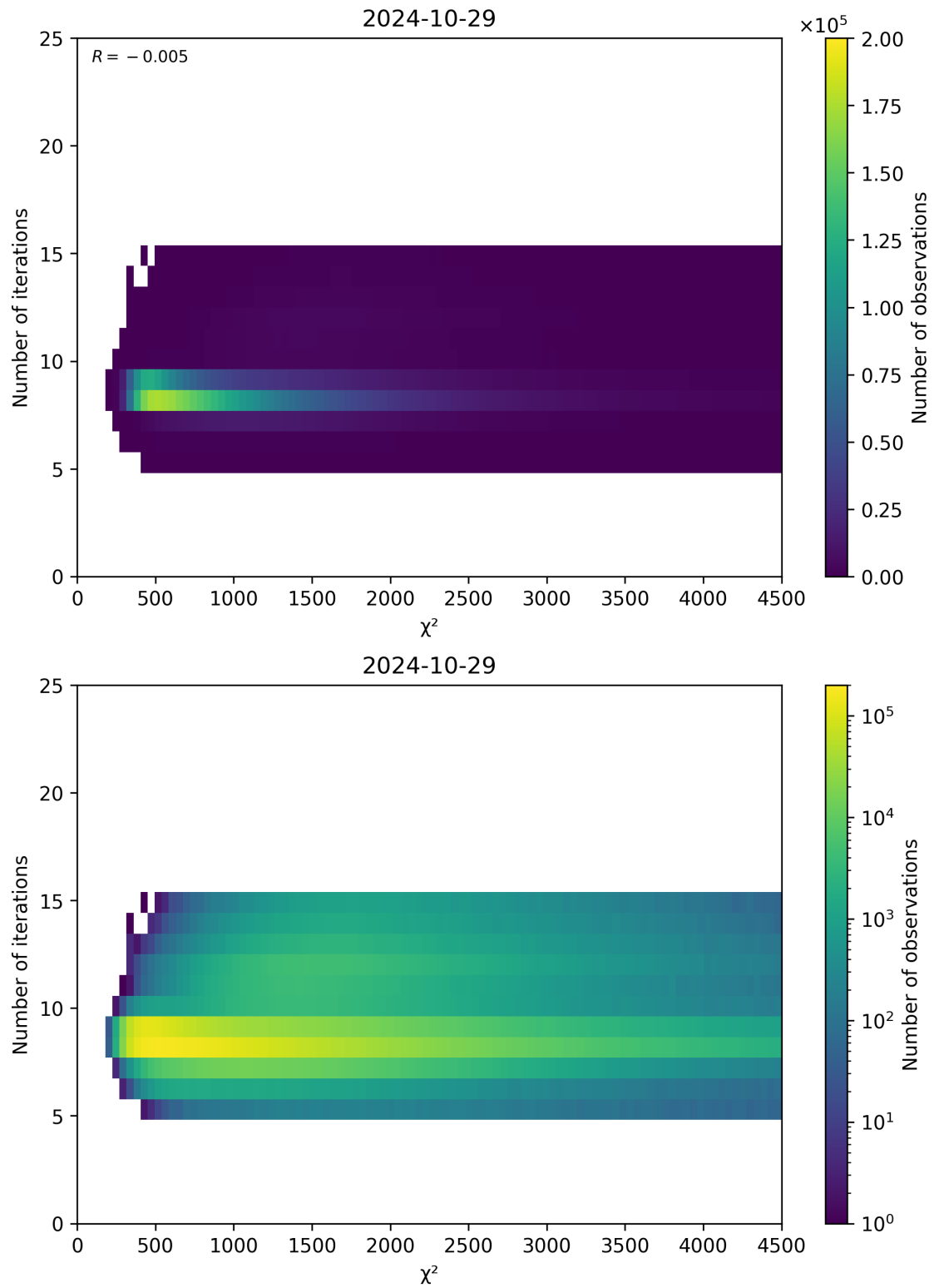
Figure 49: Scatter density plot of “ \chi^2 ” against “Number of iterations” for 2024-10-29 to 2024-10-30.
