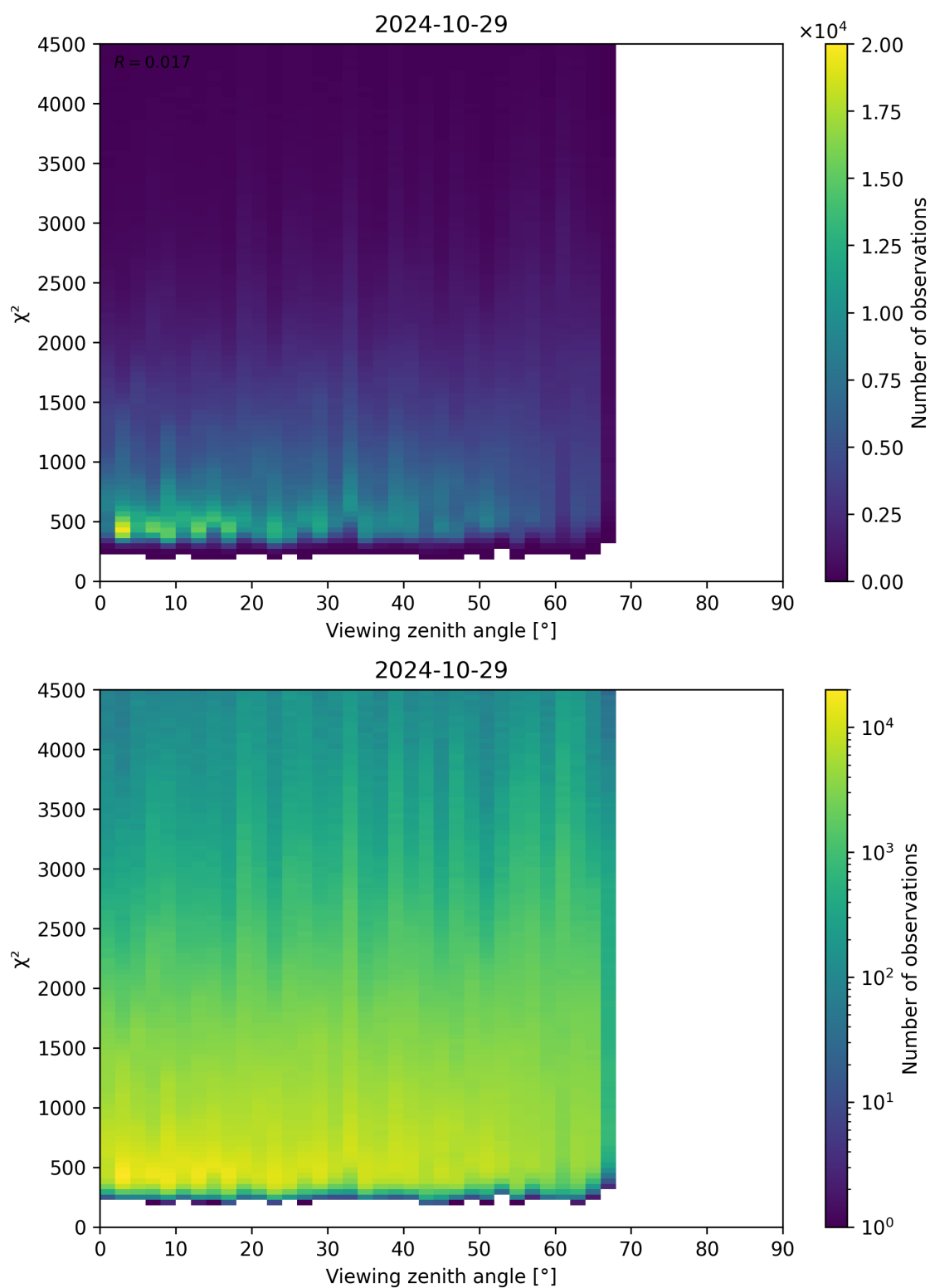
Figure 72: Scatter density plot of “Viewing zenith angle” against “ \chi^2 ” for 2024-10-29 to 2024-10-30.
