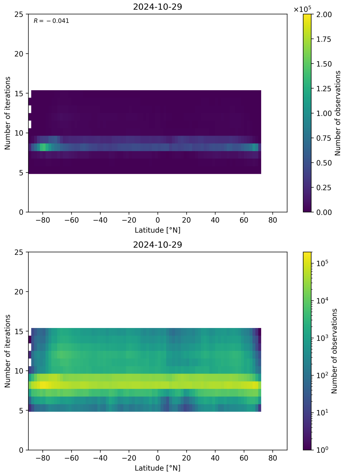
Figure 56: Scatter density plot of “Latitude” against “Number of iterations” for 2024-10-29 to 2024-10-30.
