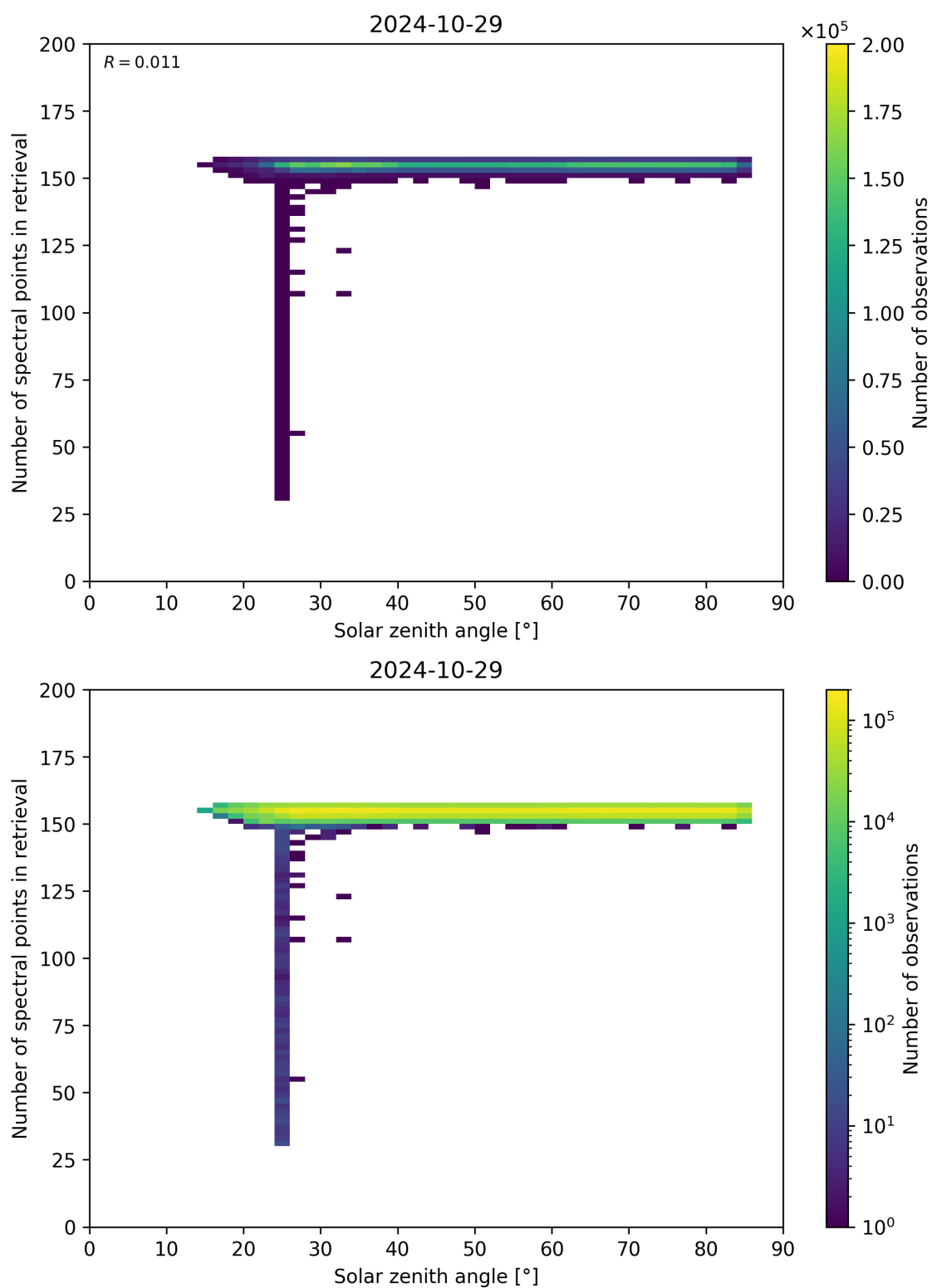
Figure 68: Scatter density plot of “Solar zenith angle” against “Number of spectral points in retrieval” for 2024-10-29 to 2024-10-30.
