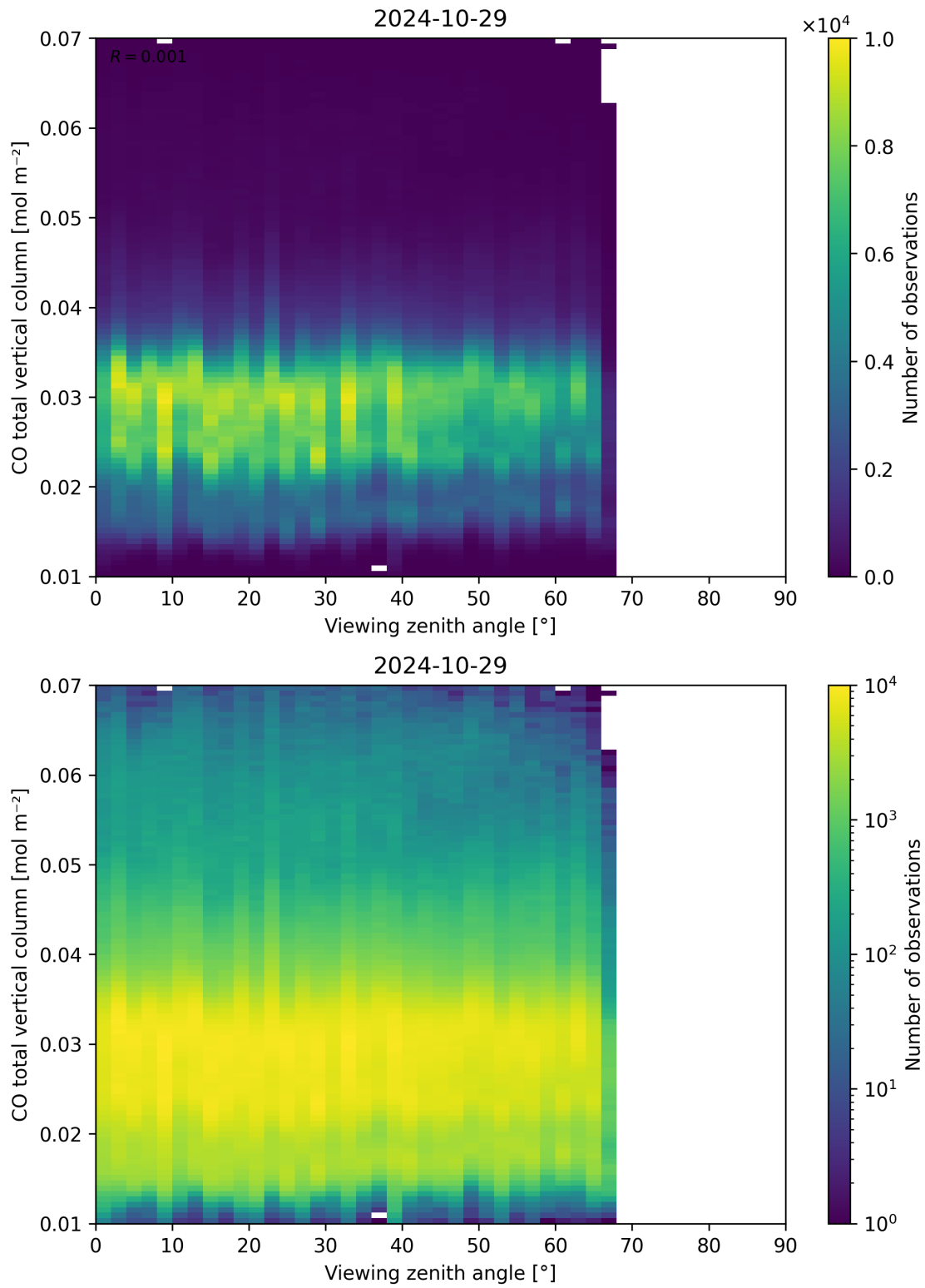
Figure 69: Scatter density plot of “Viewing zenith angle” against “CO total vertical column” for 2024-10-29 to 2024-10-30.
