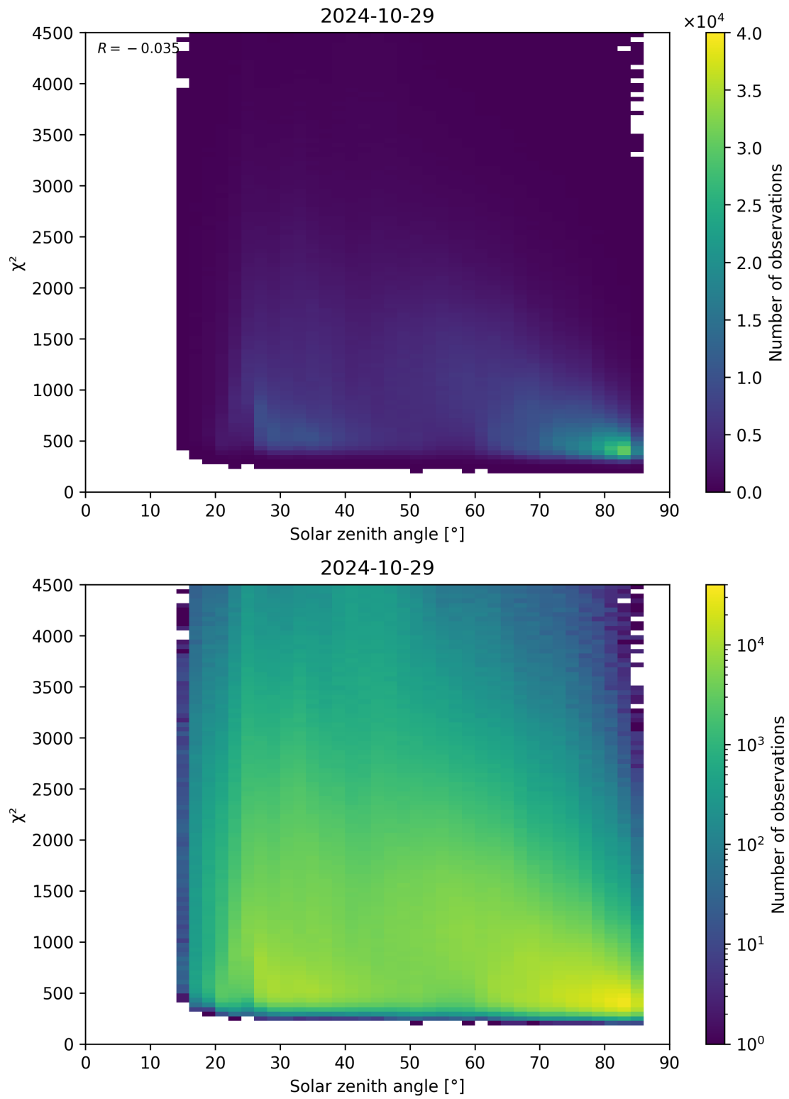
Figure 64: Scatter density plot of “Solar zenith angle” against “ \chi^2 ” for 2024-10-29 to 2024-10-30.
