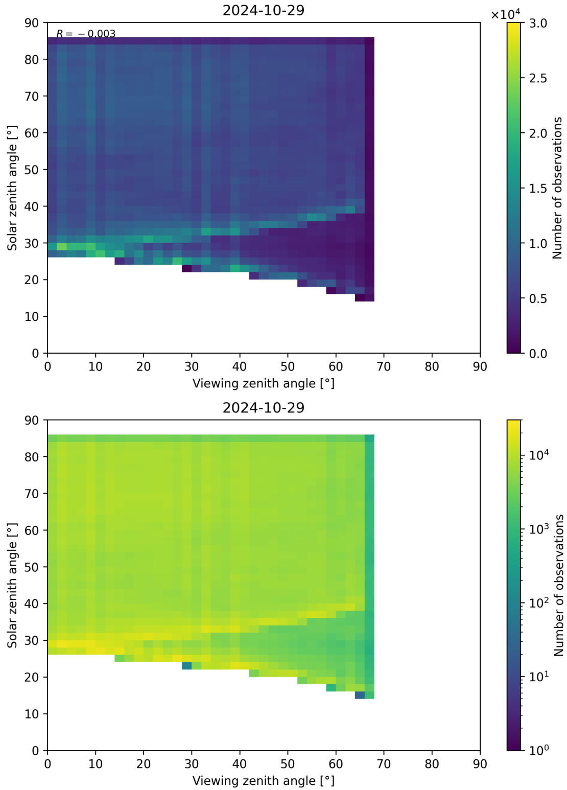
Figure 77: Scatter density plot of “Viewing zenith angle” against “Solar zenith angle” for 2024-10-29 to 2024-10-30.
