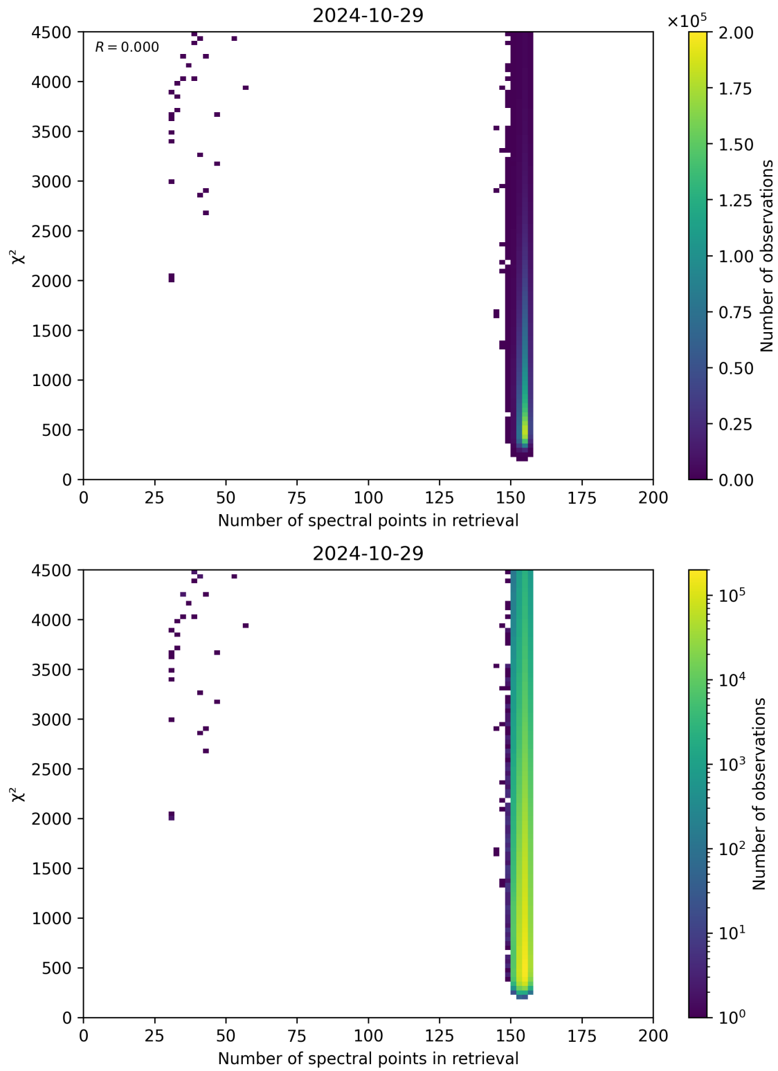
Figure 58: Scatter density plot of “Number of spectral points in retrieval” against “ \chi^2 ” for 2024-10-29 to 2024-10-30.
