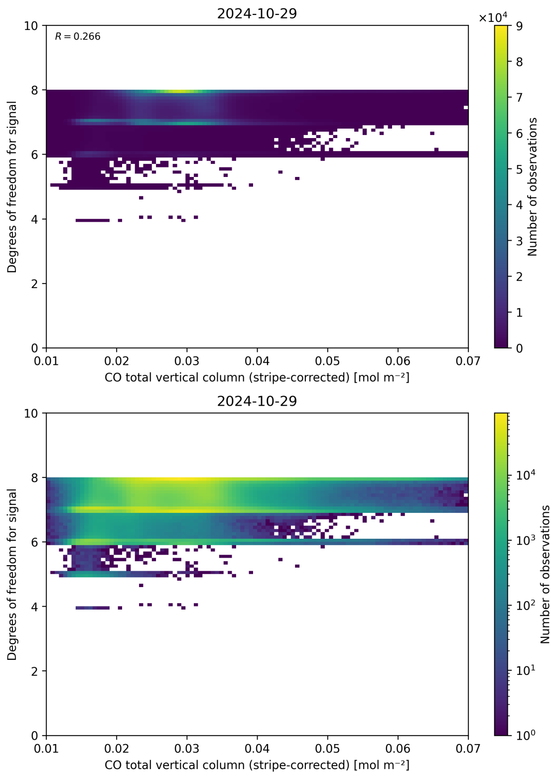
Figure 38: Scatter density plot of “CO total vertical column (stripe-corrected)” against “Degrees of freedom for signal” for 2024-10-29 to 2024-10-30.
