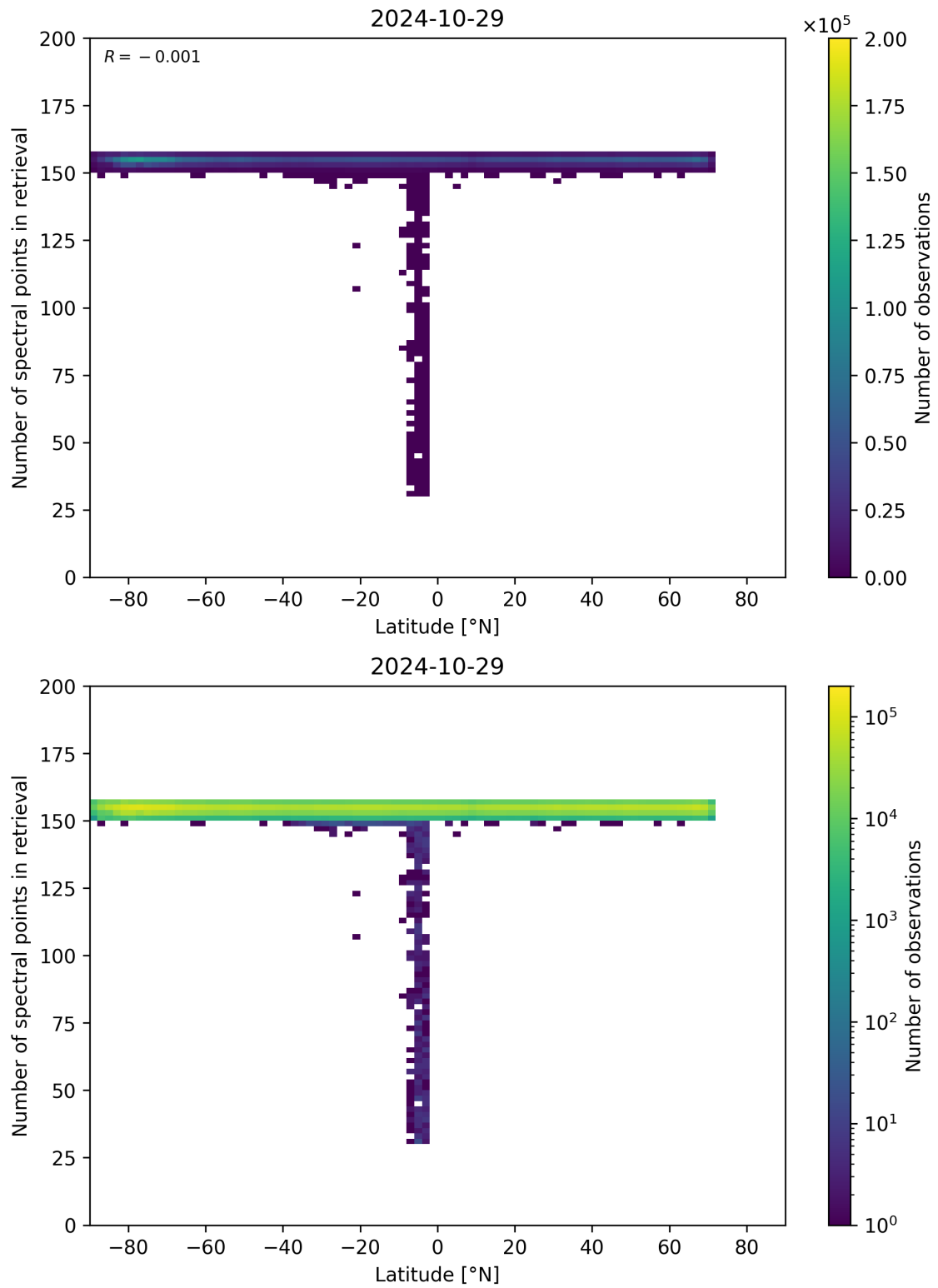
Figure 57: Scatter density plot of “Latitude” against “Number of spectral points in retrieval” for 2024-10-29 to 2024-10-30.
