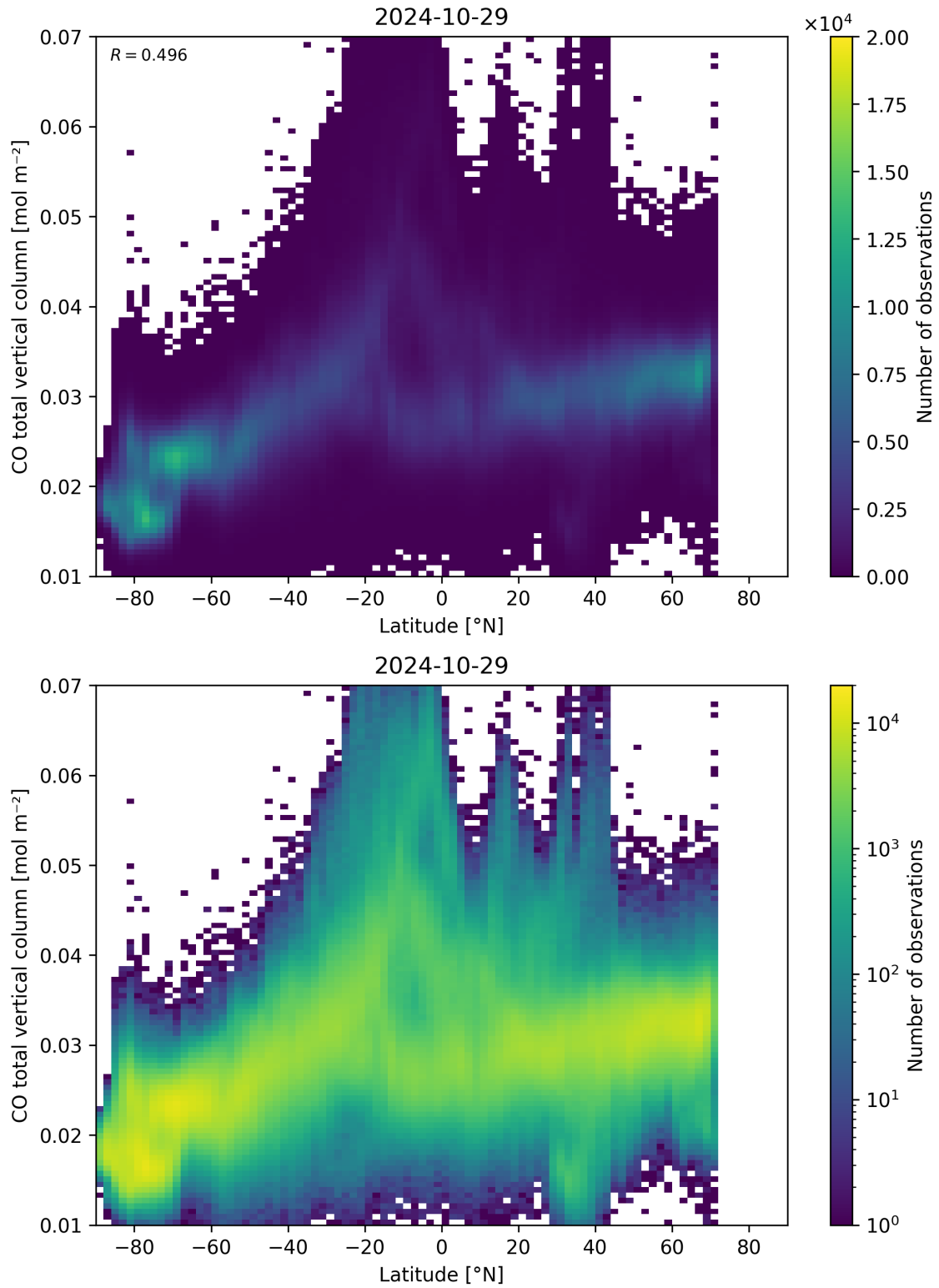
Figure 51: Scatter density plot of “Latitude” against “CO total vertical column” for 2024-10-29 to 2024-10-30.
