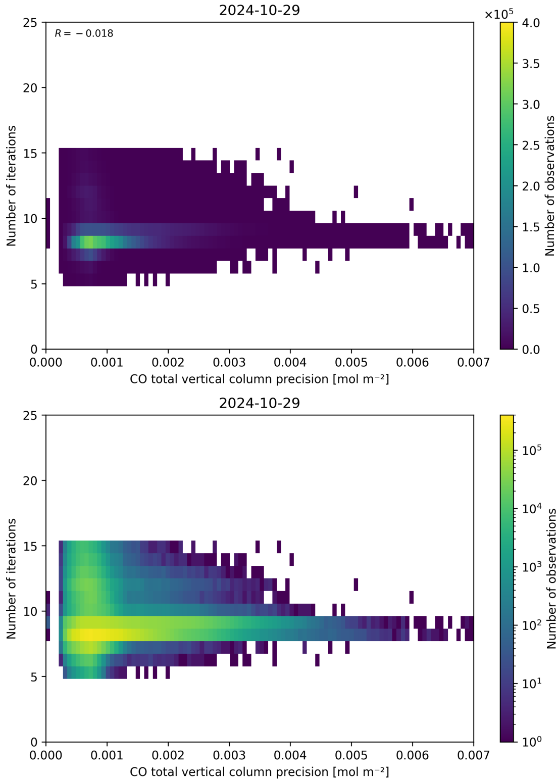
Figure 46: Scatter density plot of “CO total vertical column precision” against “Number of iterations” for 2024-10-29 to 2024-10-30.
