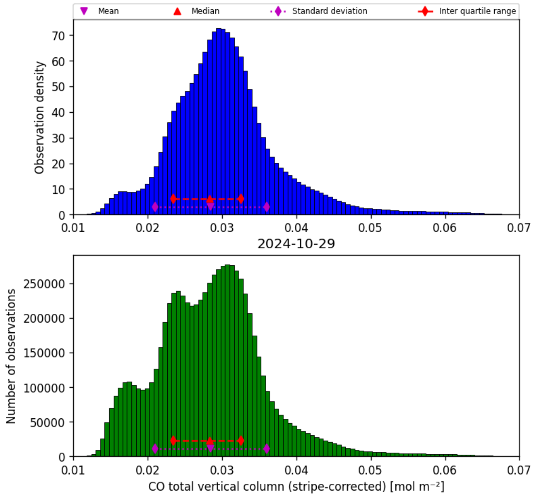
Figure 19: Histogram of “CO total vertical column (stripe-corrected)” for 2024-10-29 to 2024-10-30
