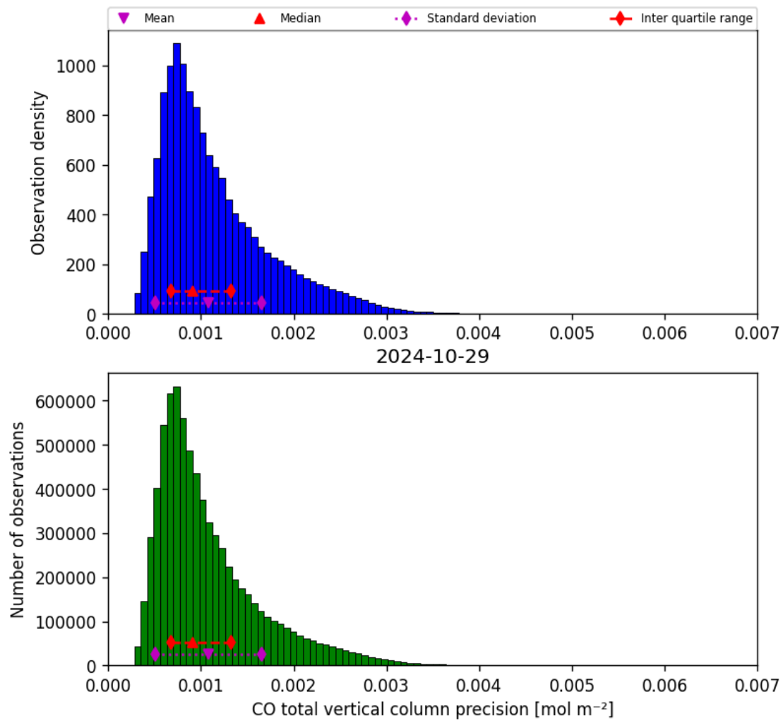
Figure 20: Histogram of “CO total vertical column precision” for 2024-10-29 to 2024-10-30
