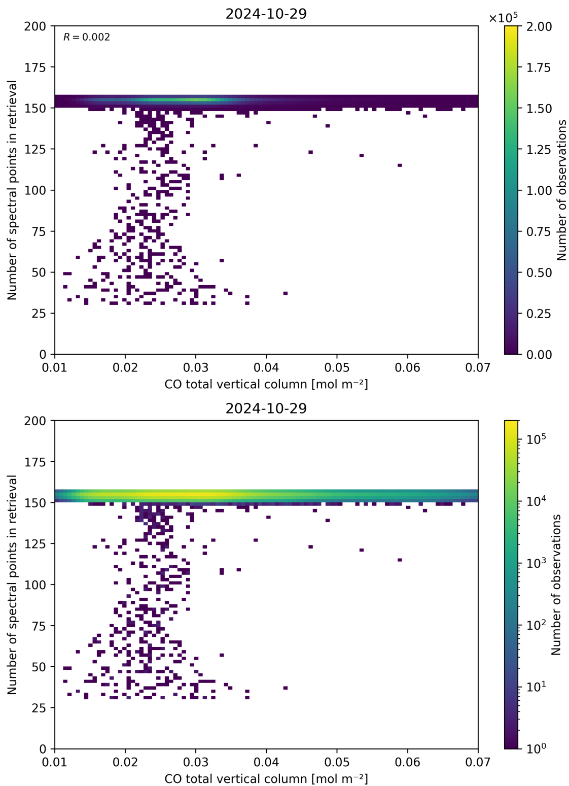
Figure 43: Scatter density plot of “CO total vertical column” against “Number of spectral points in retrieval” for 2024-10-29 to 2024-10-30.
