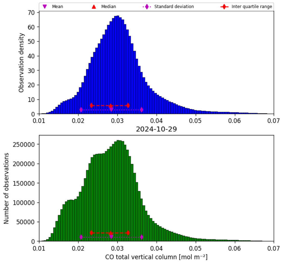
Figure 18: Histogram of “CO total vertical column” for 2024-10-29 to 2024-10-30
