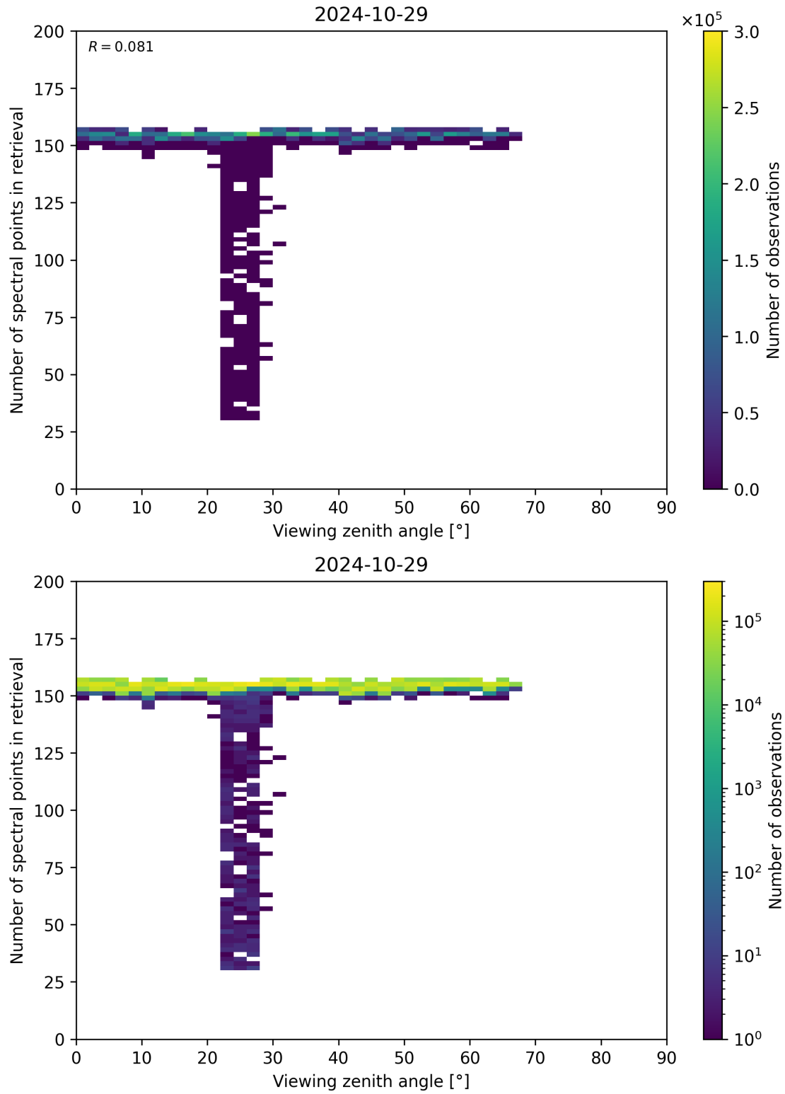
Figure 76: Scatter density plot of “Viewing zenith angle” against “Number of spectral points in retrieval” for 2024-10-29 to 2024-10-30.
