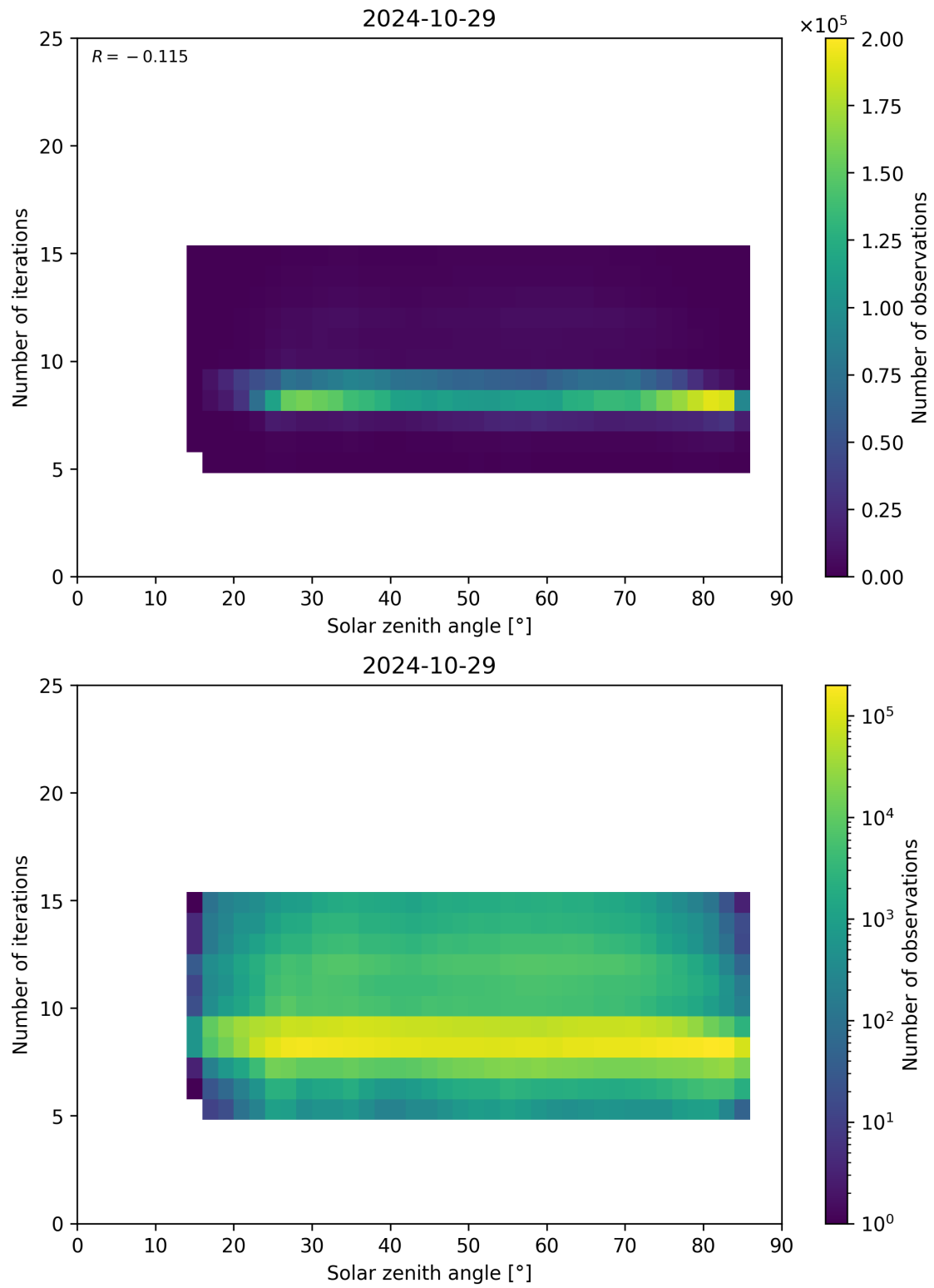
Figure 67: Scatter density plot of “Solar zenith angle” against “Number of iterations” for 2024-10-29 to 2024-10-30.
