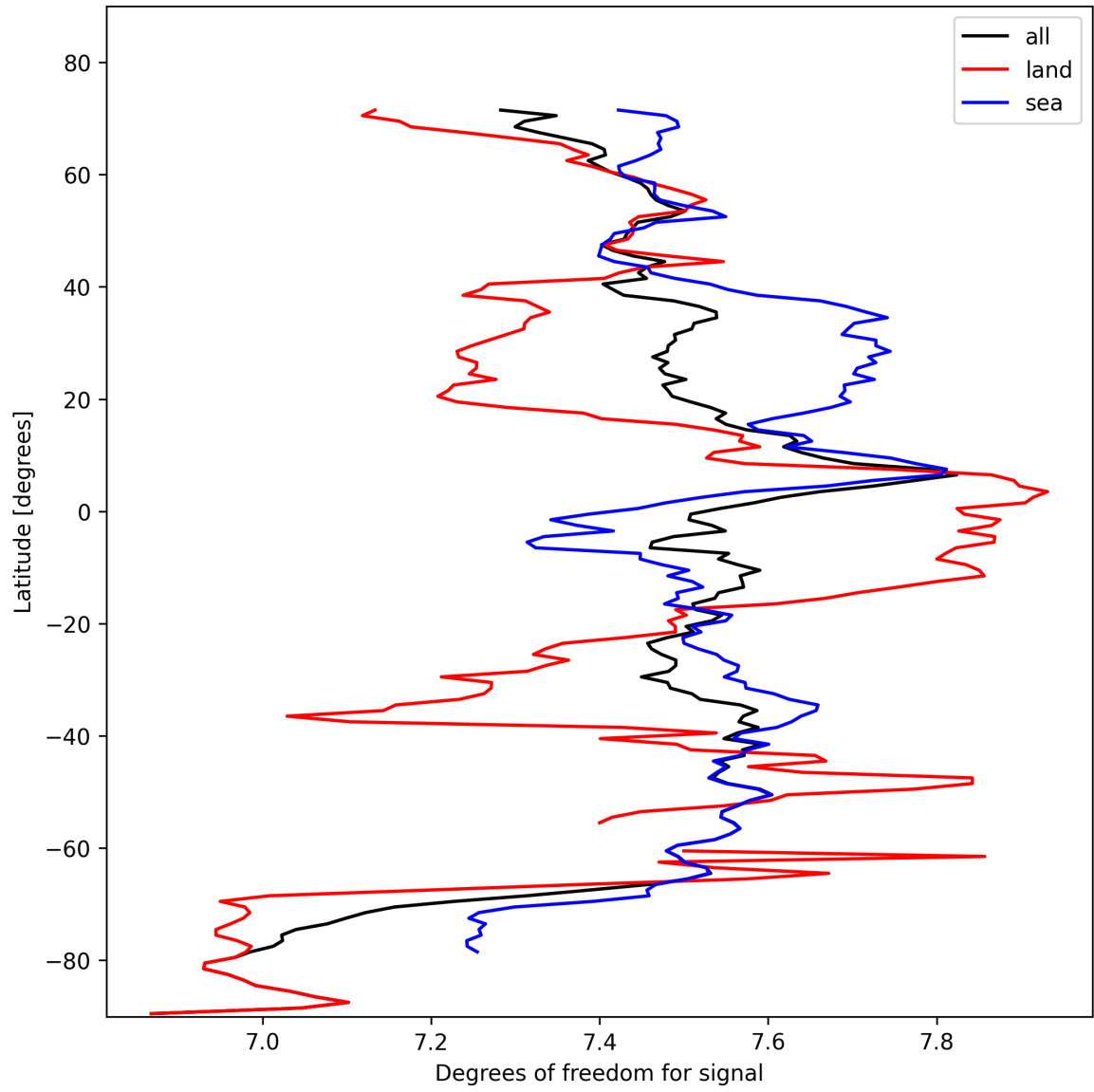
Figure 15: Zonal average of “Degrees of freedom for signal” for 2024-10-29 to 2024-10-30.
