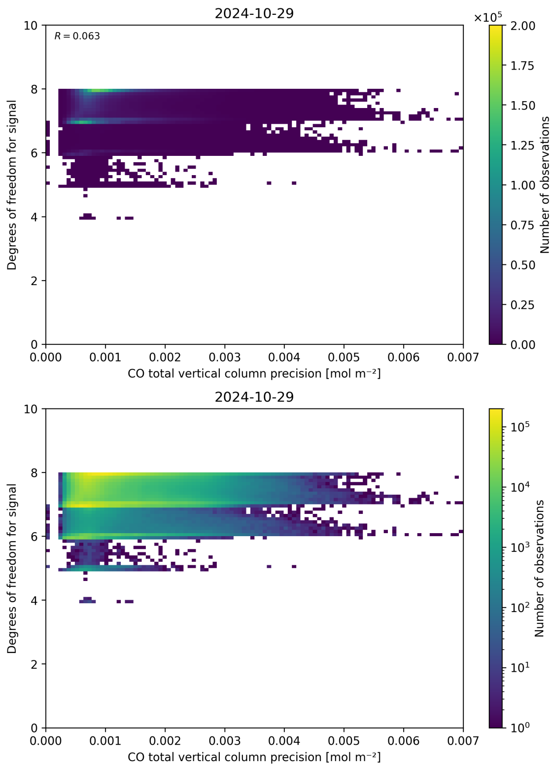
Figure 45: Scatter density plot of “CO total vertical column precision” against “Degrees of freedom for signal” for 2024-10-29 to 2024-10-30.
