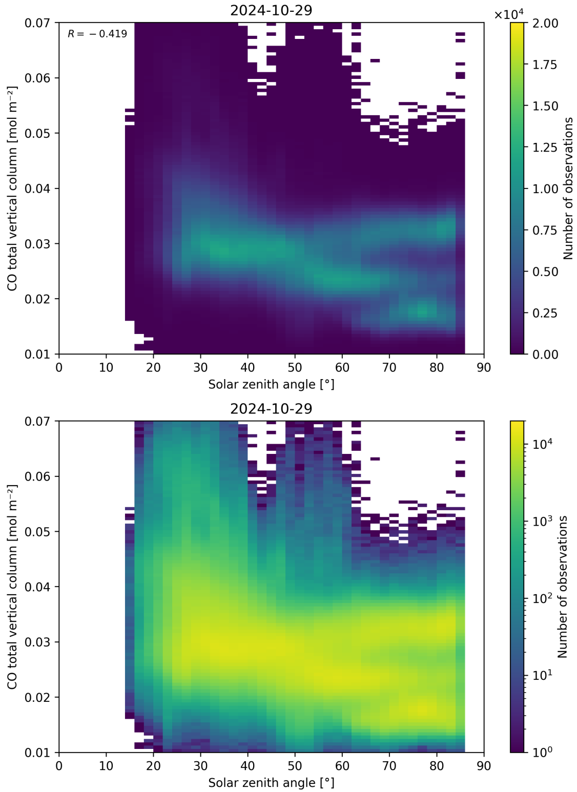
Figure 61: Scatter density plot of “Solar zenith angle” against “CO total vertical column” for 2024-10-29 to 2024-10-30.
