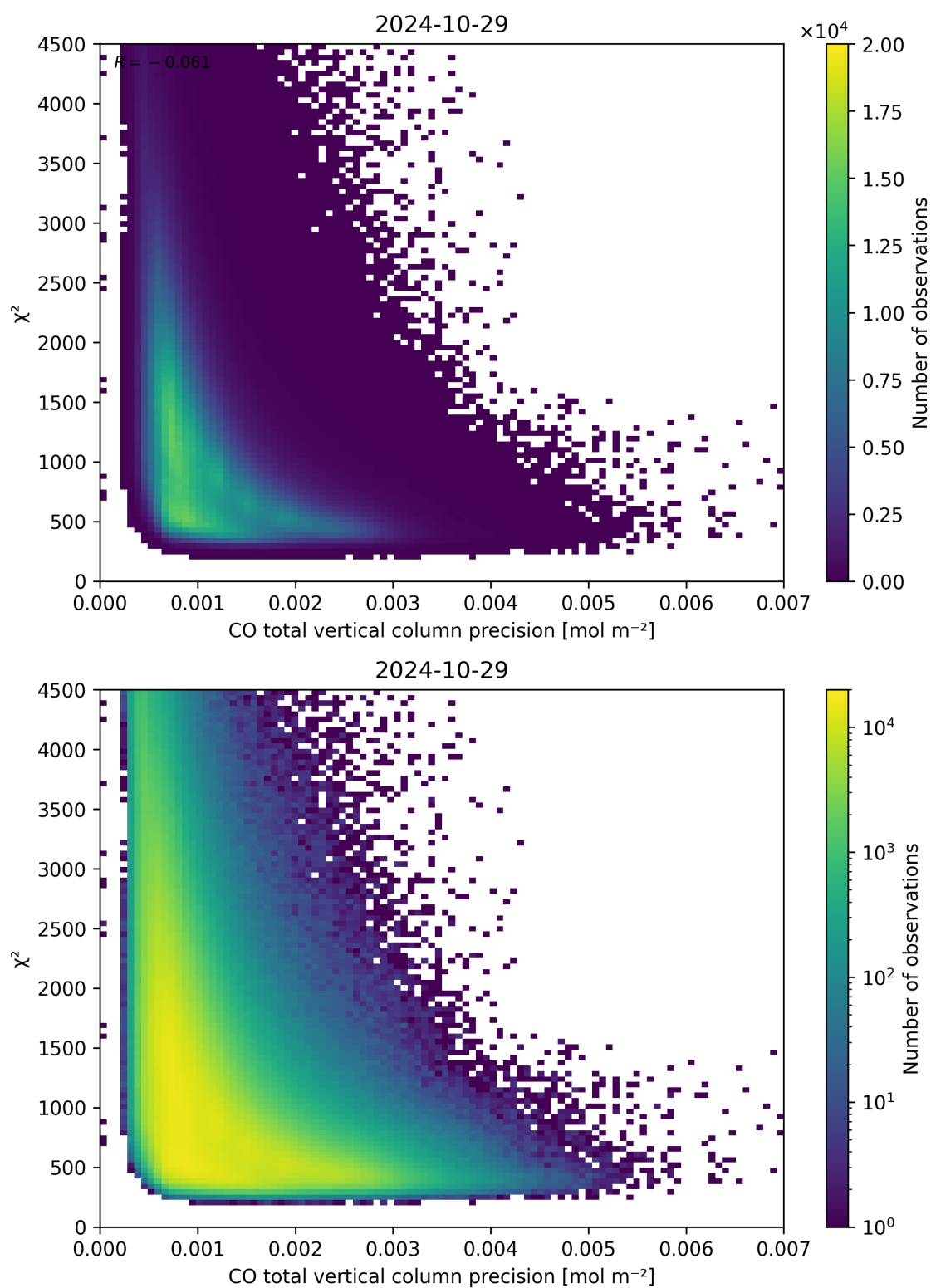
Figure 44: Scatter density plot of “CO total vertical column precision” against “ \chi^2 ” for 2024-10-29 to 2024-10-30.
