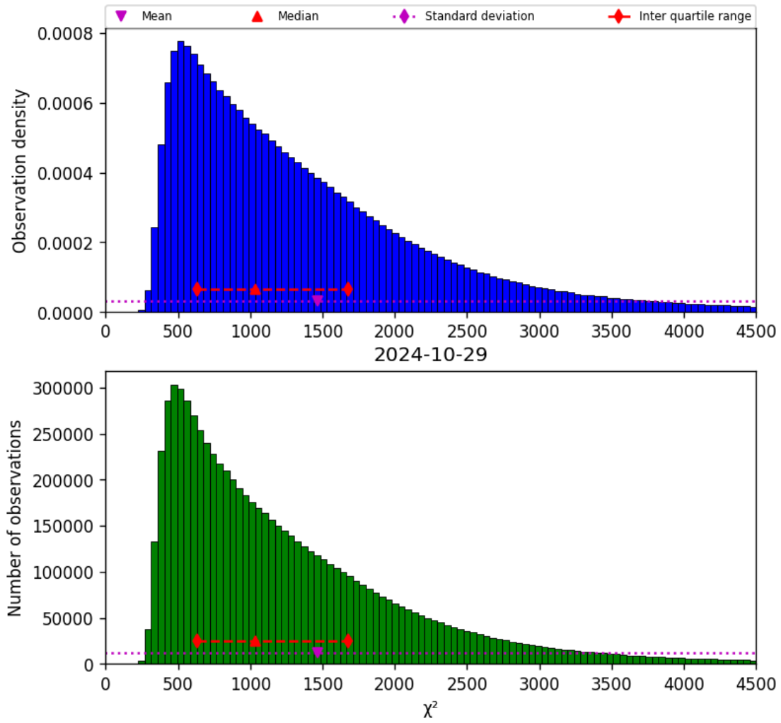
Figure 22: Histogram of “ \chi^2 ” for 2024-10-29 to 2024-10-30
