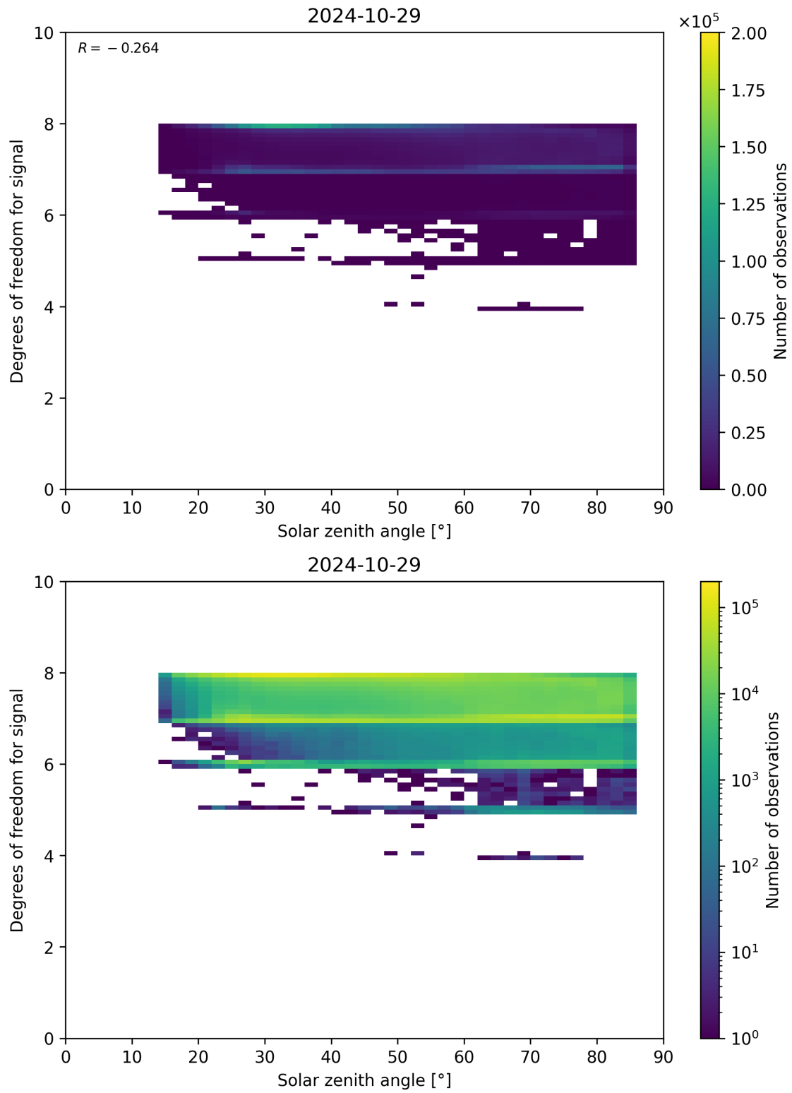
Figure 65: Scatter density plot of “Solar zenith angle” against “Degrees of freedom for signal” for 2024-10-29 to 2024-10-30.
