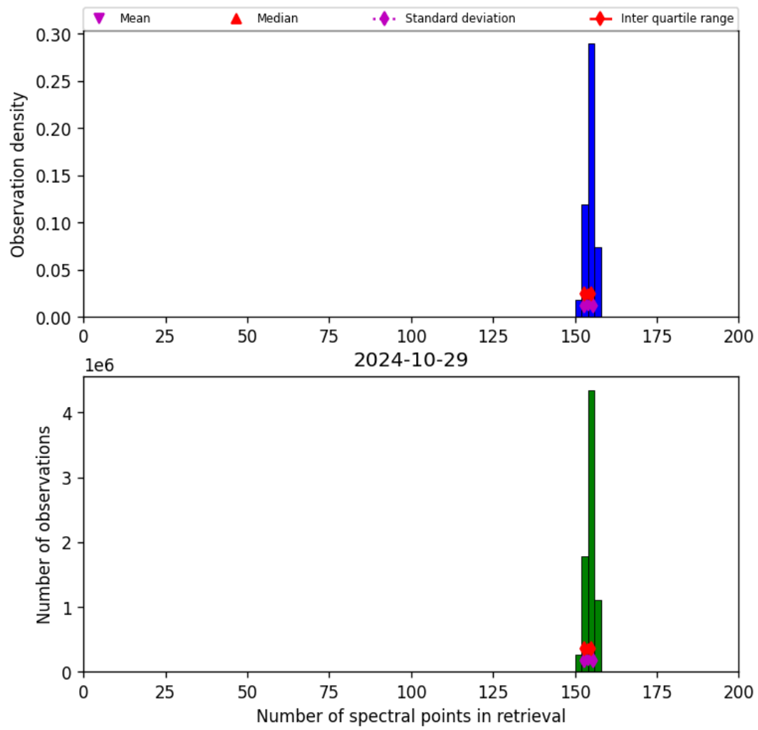
Figure 21: Histogram of “Number of spectral points in retrieval” for 2024-10-29 to 2024-10-30
