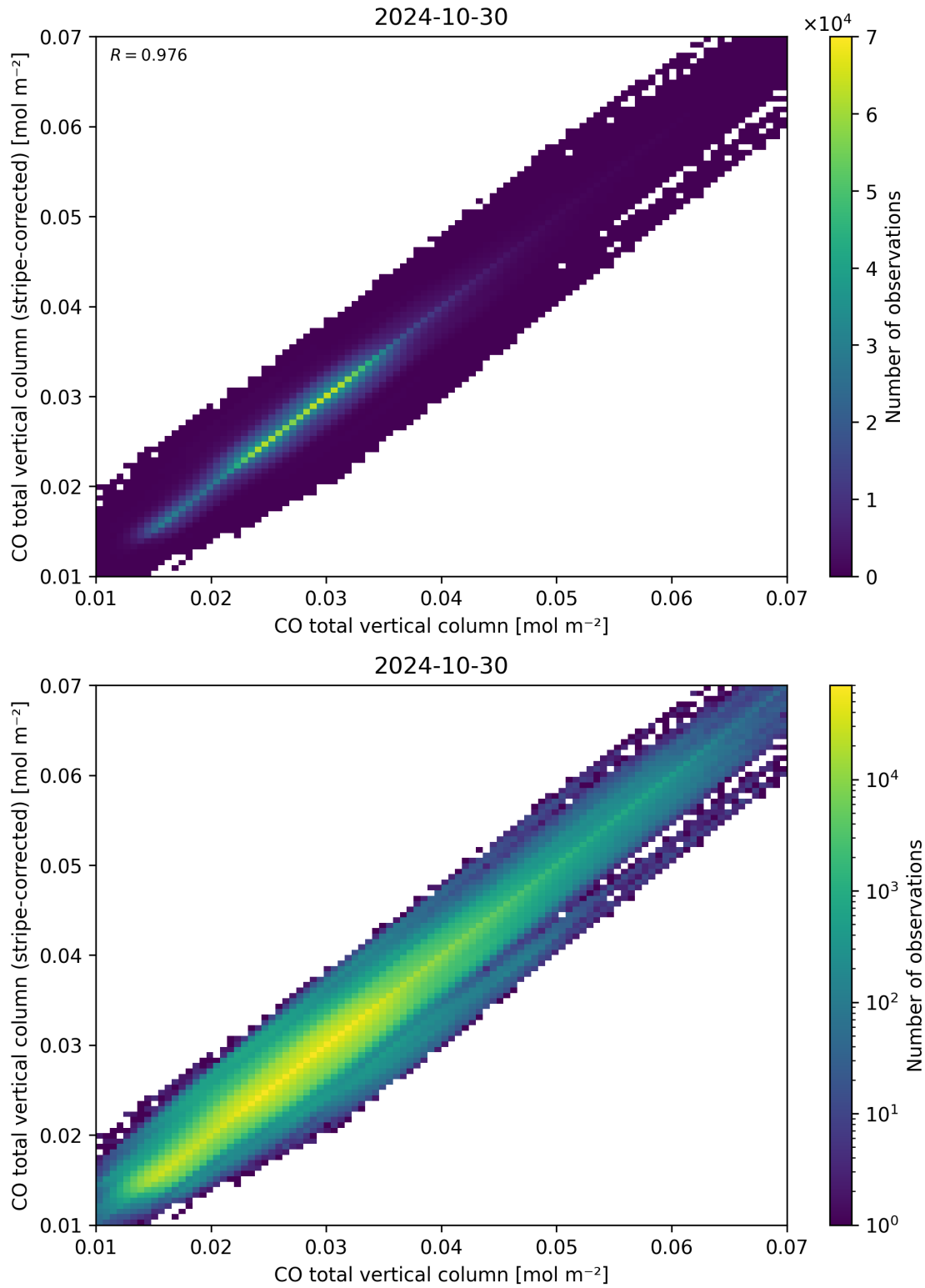
Figure 33: Scatter density plot of “CO total vertical column” against “CO total vertical column (stripe-corrected)” for 2024-10-30 to 2024-10-31.
