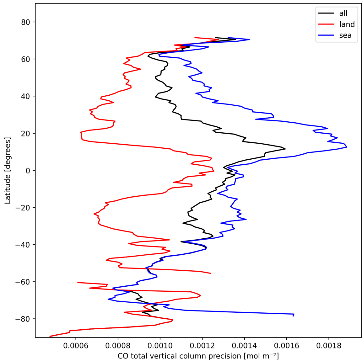
Figure 12: Zonal average of “CO total vertical column precision” for 2024-10-30 to 2024-10-31.
