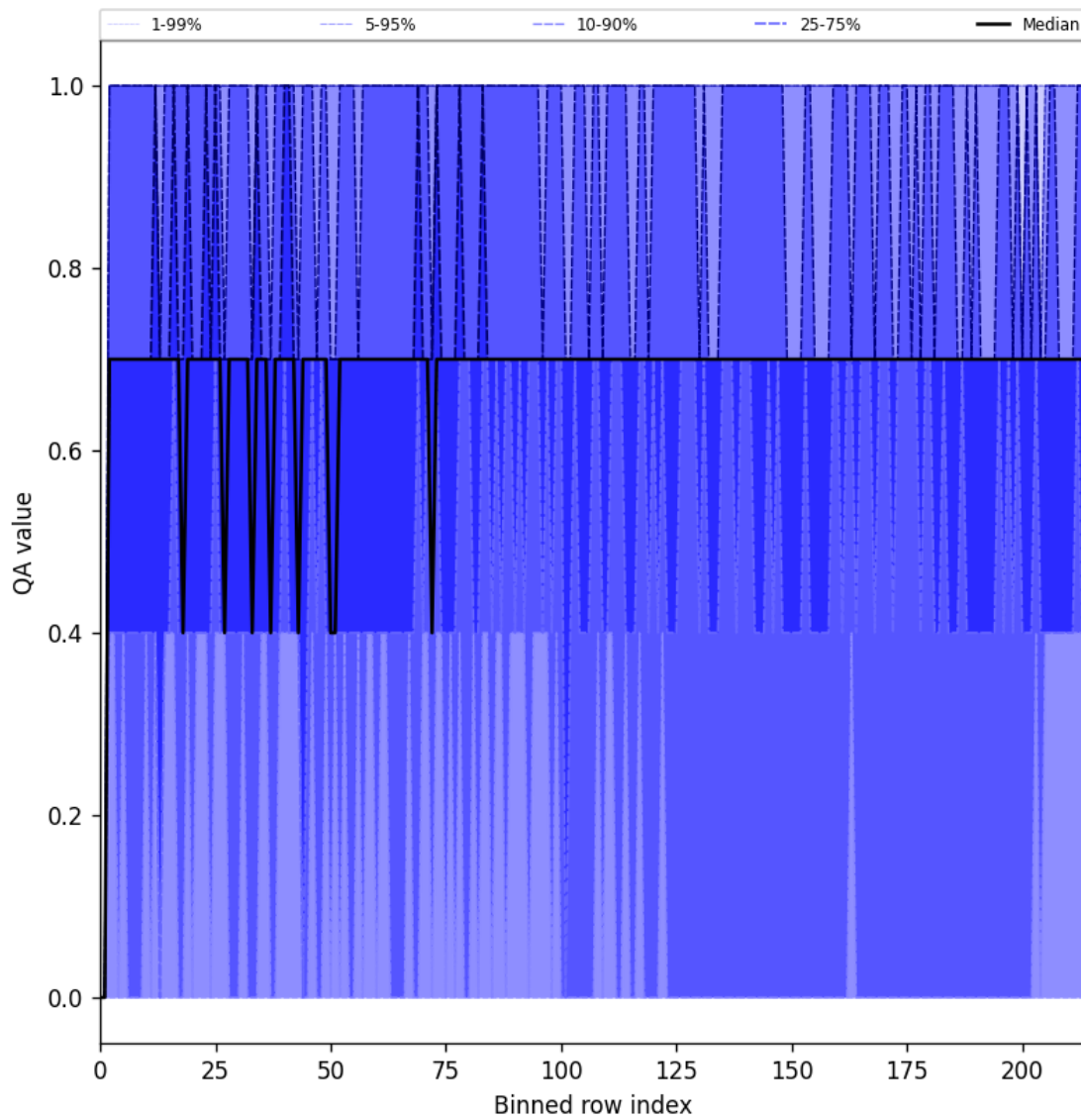
Figure 25: Along track statistics of “QA value” for 2024-10-30 to 2024-10-31
