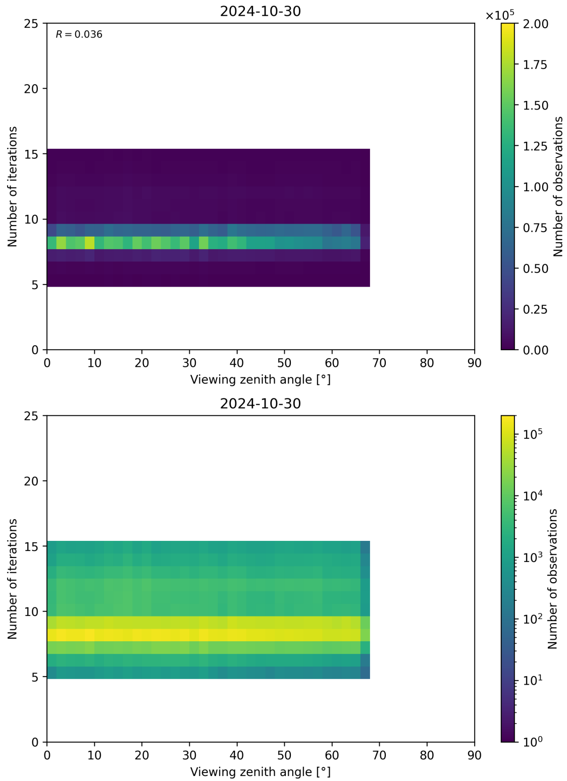
Figure 75: Scatter density plot of “Viewing zenith angle” against “Number of iterations” for 2024-10-30 to 2024-10-31.
