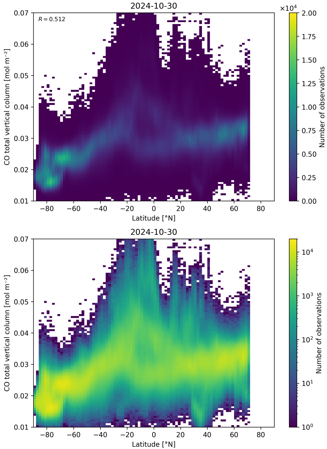
Figure 51: Scatter density plot of “Latitude” against “CO total vertical column” for 2024-10-30 to 2024-10-31.
