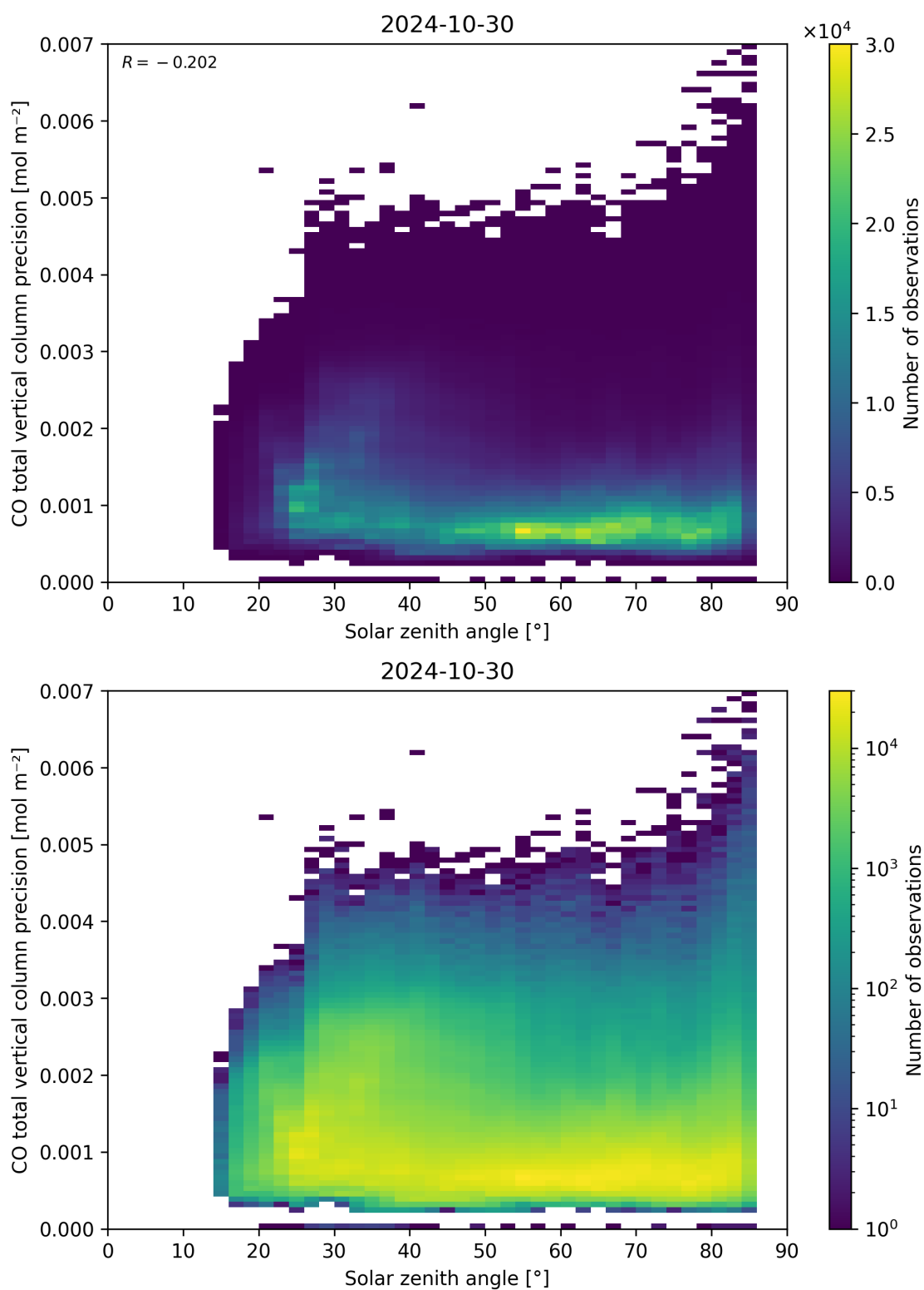
Figure 63: Scatter density plot of “Solar zenith angle” against “CO total vertical column precision” for 2024-10-30 to 2024-10-31.
