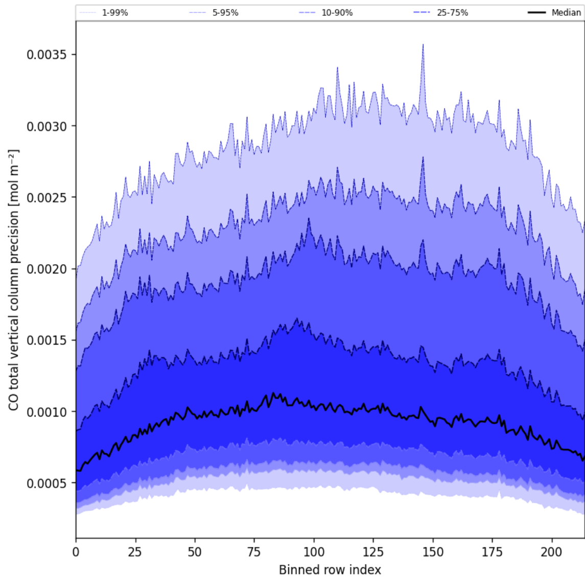
Figure 28: Along track statistics of “CO total vertical column precision” for 2024-10-30 to 2024-10-31
