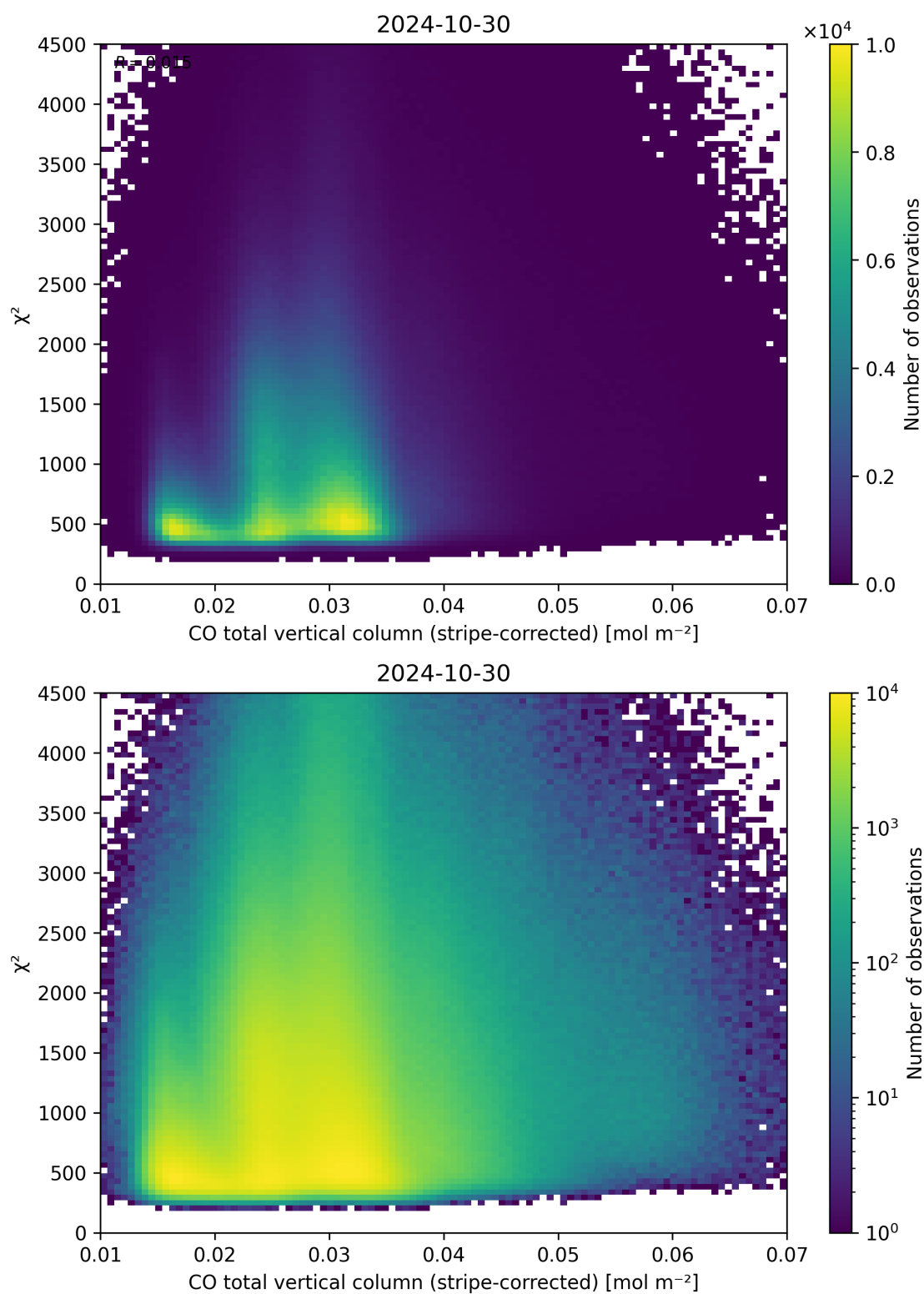
Figure 37: Scatter density plot of “CO total vertical column (stripe-corrected)” against “ \chi^2 ” for 2024-10-30 to 2024-10-31.
