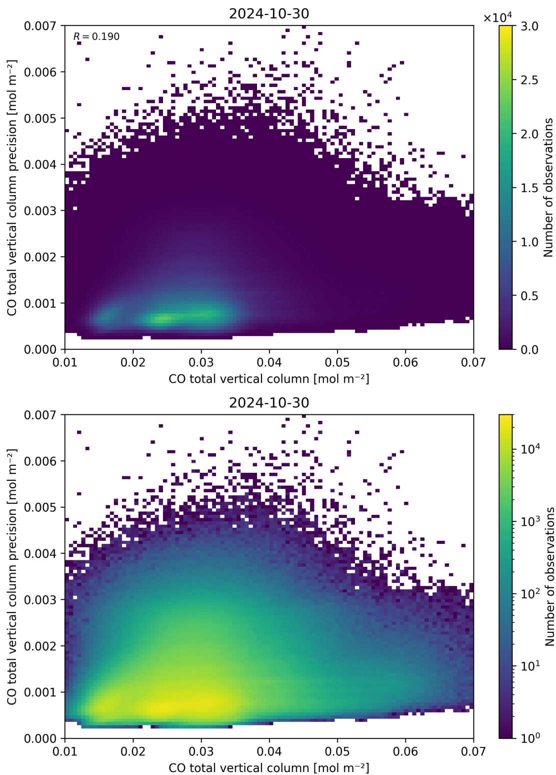
Figure 34: Scatter density plot of “CO total vertical column” against “CO total vertical column precision” for 2024-10-30 to 2024-10-31.
