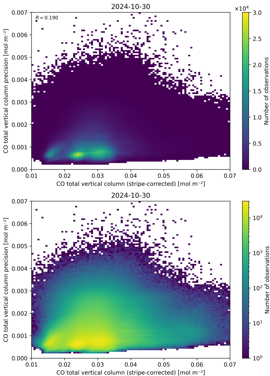
Figure 36: Scatter density plot of “CO total vertical column (stripe-corrected)” against “CO total vertical column precision” for 2024-10-30 to 2024-10-31.
