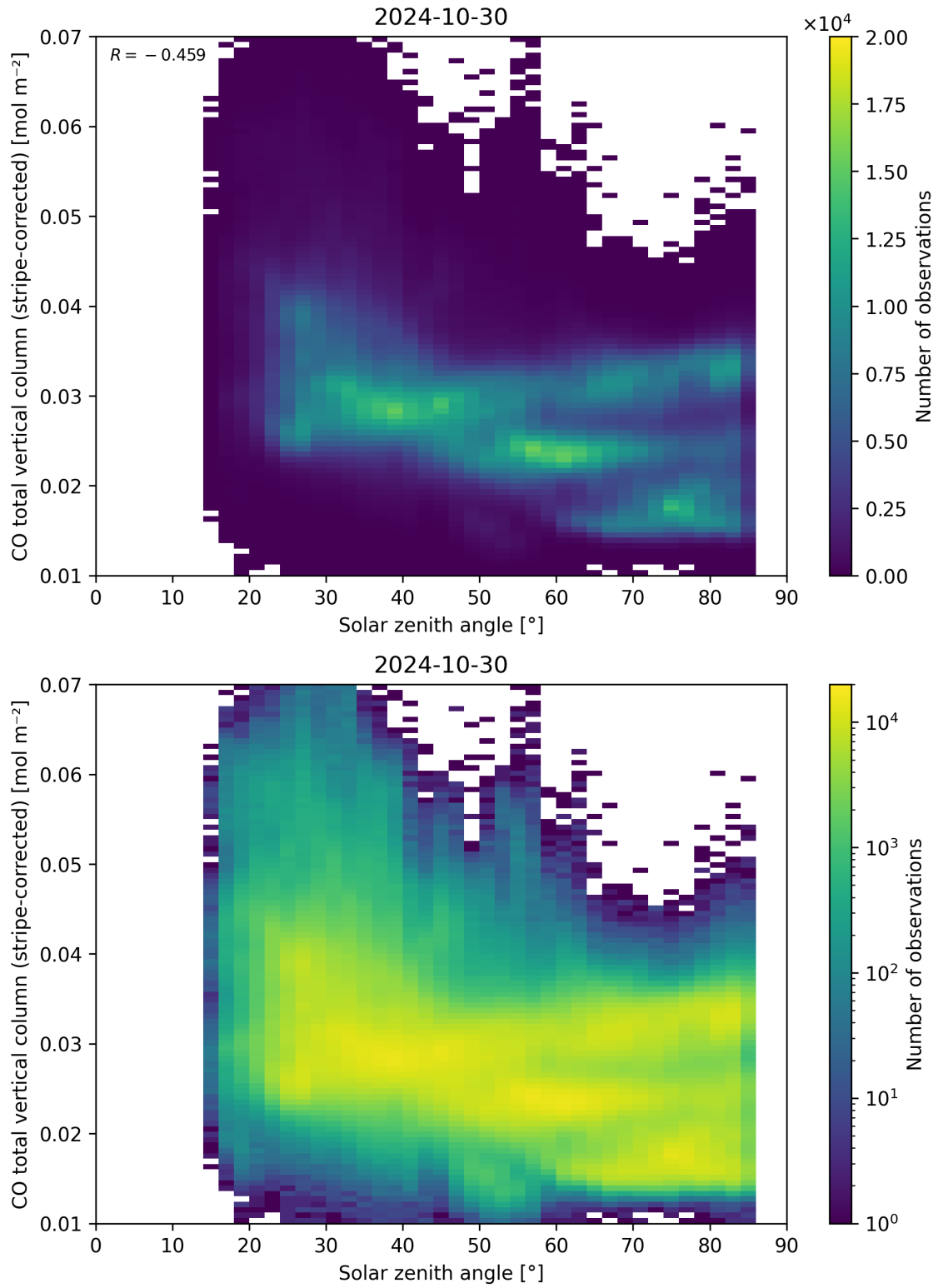
Figure 62: Scatter density plot of “Solar zenith angle” against “CO total vertical column (stripe-corrected)” for 2024-10-30 to 2024-10-31.
