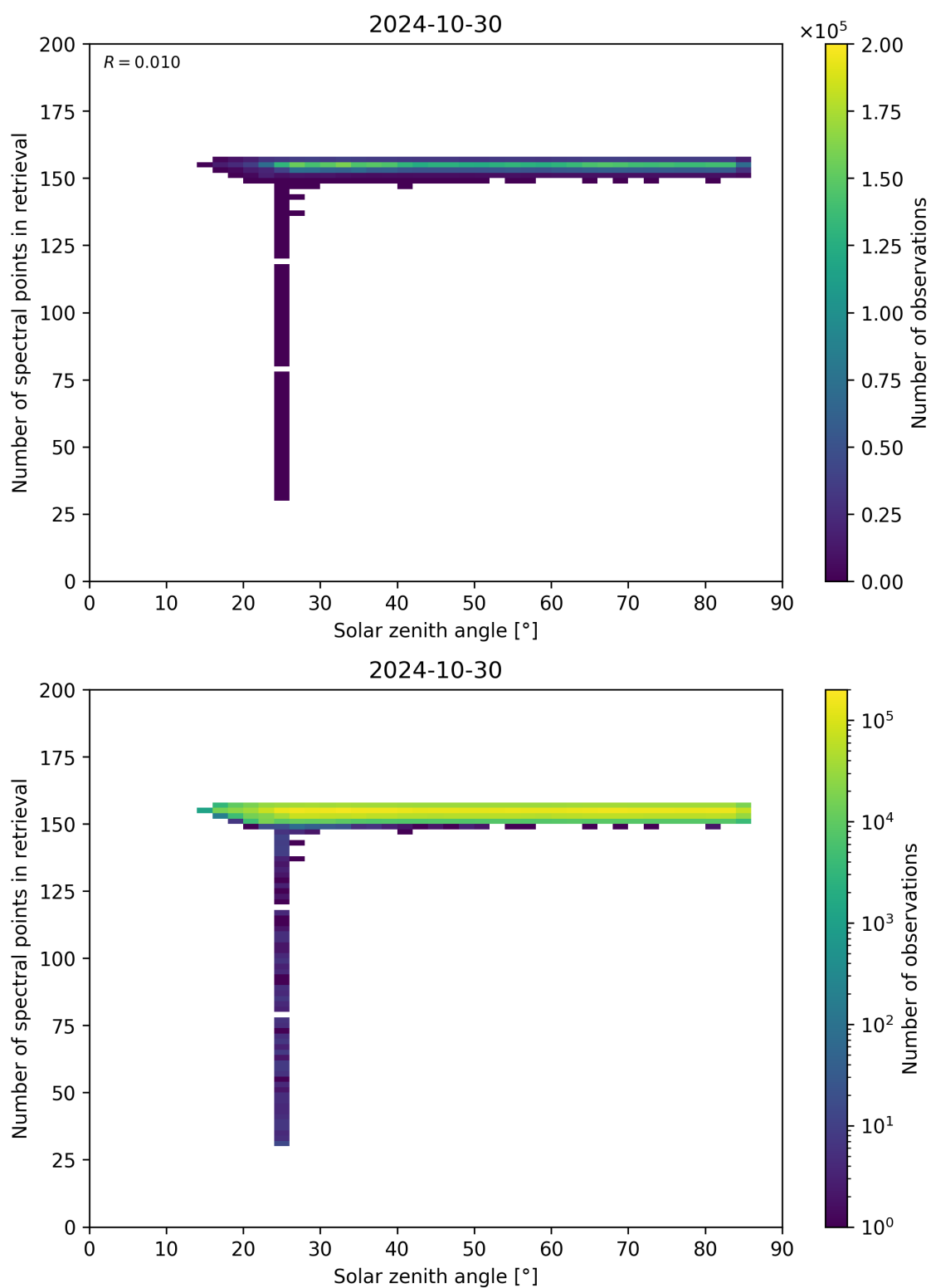
Figure 68: Scatter density plot of “Solar zenith angle” against “Number of spectral points in retrieval” for 2024-10-30 to 2024-10-31.
