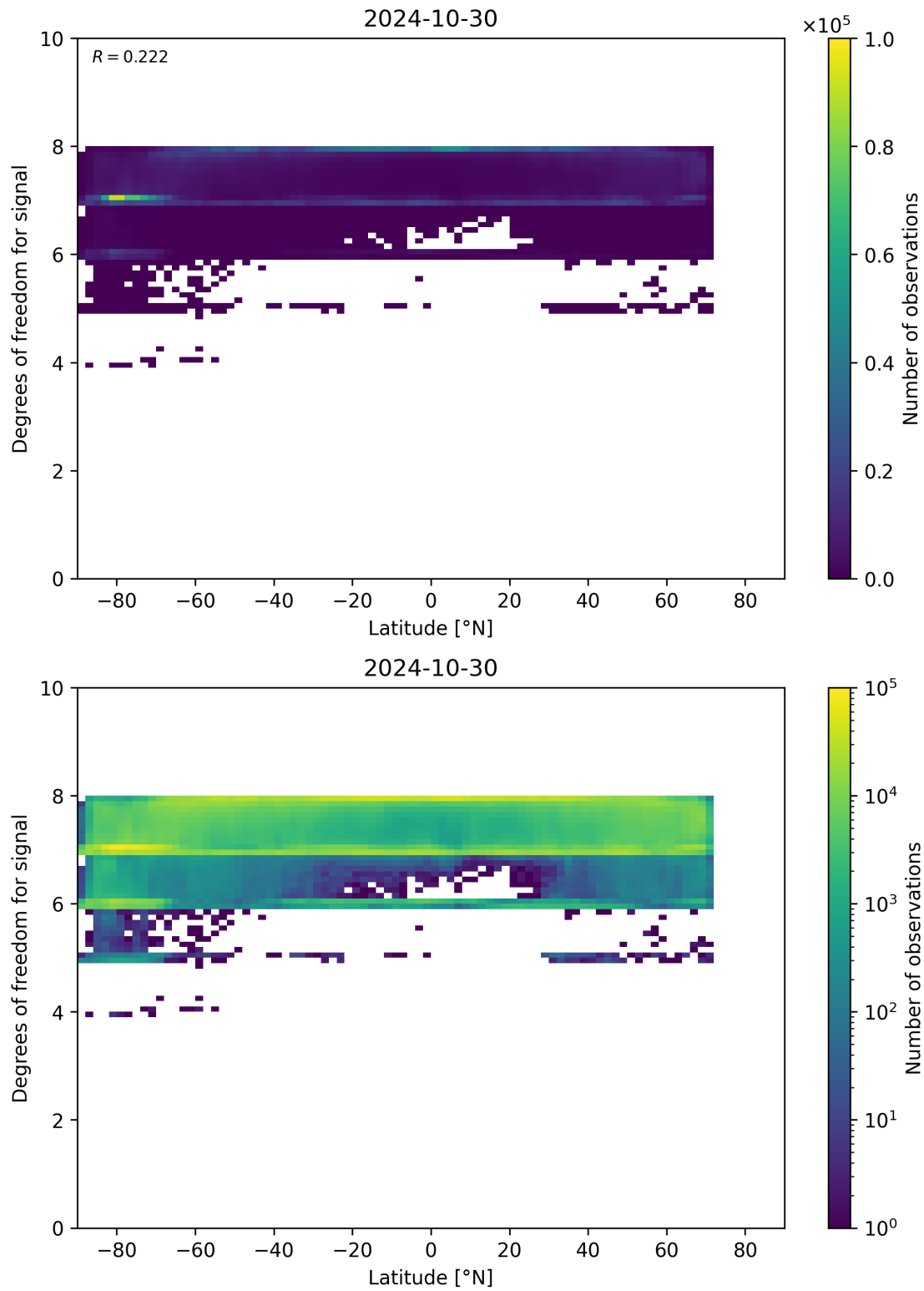
Figure 55: Scatter density plot of “Latitude” against “Degrees of freedom for signal” for 2024-10-30 to 2024-10-31.
