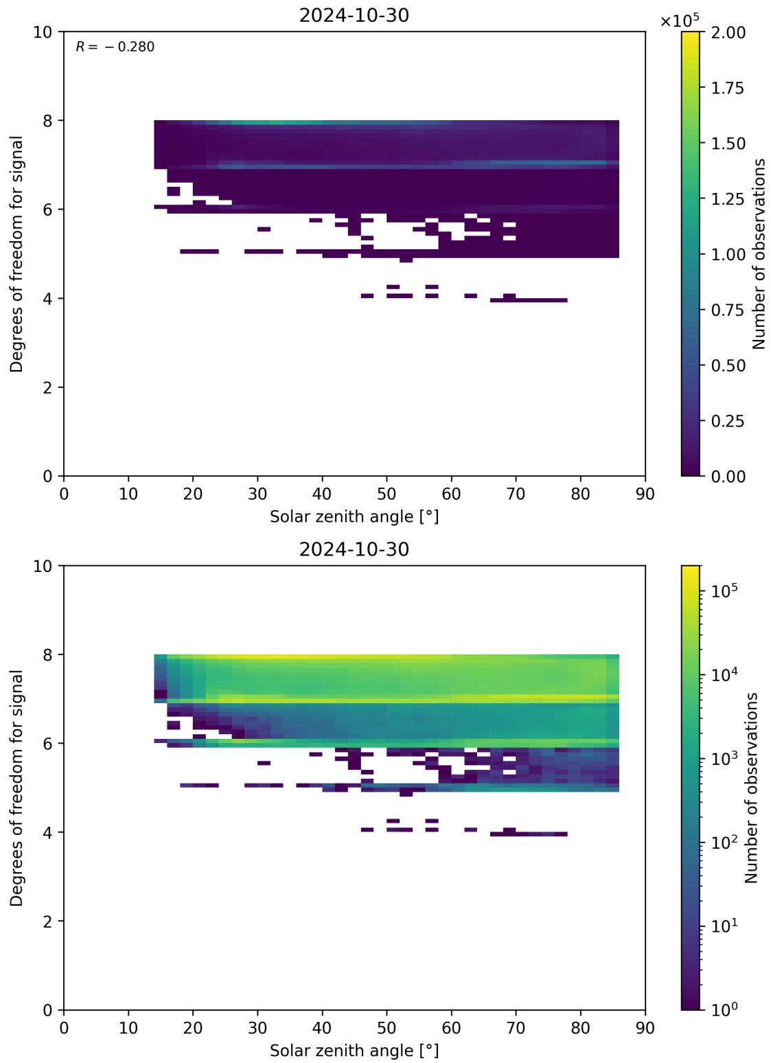
Figure 65: Scatter density plot of “Solar zenith angle” against “Degrees of freedom for signal” for 2024-10-30 to 2024-10-31.
