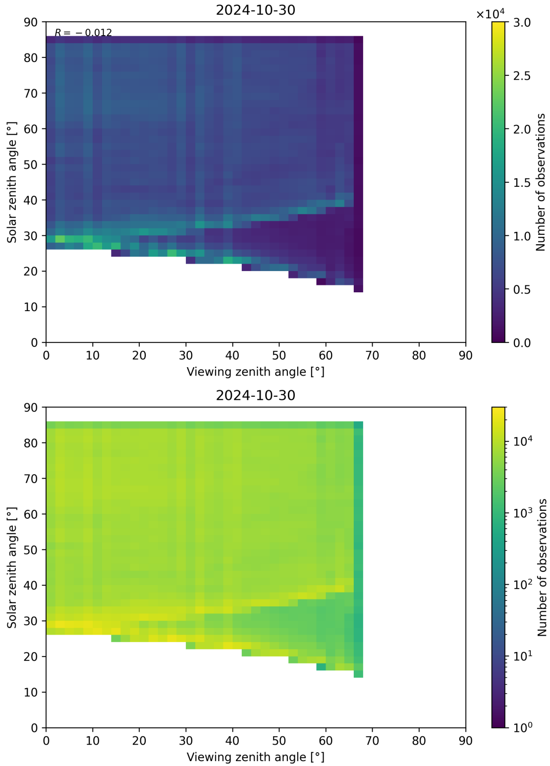
Figure 77: Scatter density plot of “Viewing zenith angle” against “Solar zenith angle” for 2024-10-30 to 2024-10-31.
