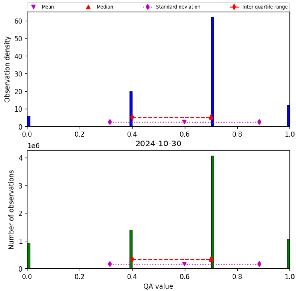
Figure 17: Histogram of “QA value” for 2024-10-30 to 2024-10-31
