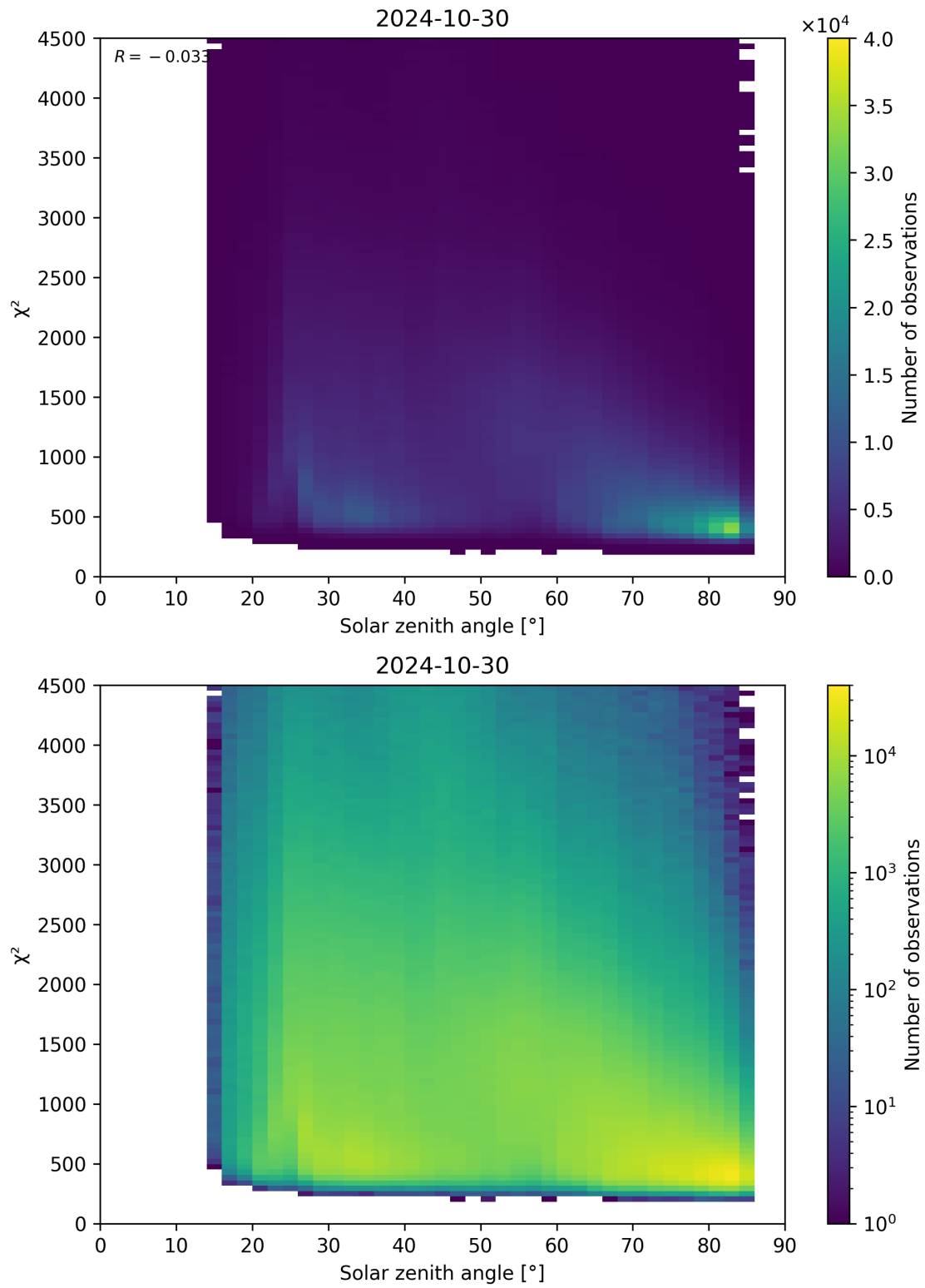
Figure 64: Scatter density plot of “Solar zenith angle” against “ \chi^2 ” for 2024-10-30 to 2024-10-31.
