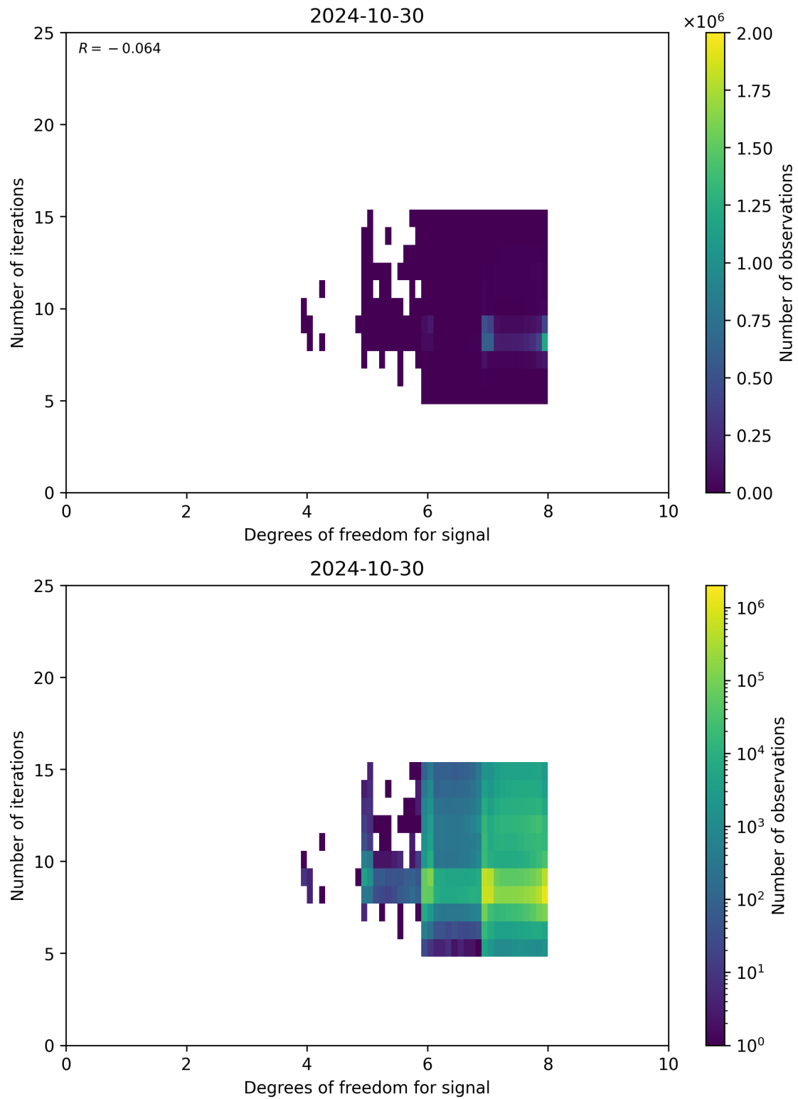
Figure 50: Scatter density plot of “Degrees of freedom for signal” against “Number of iterations” for 2024-10-30 to 2024-10-31.
