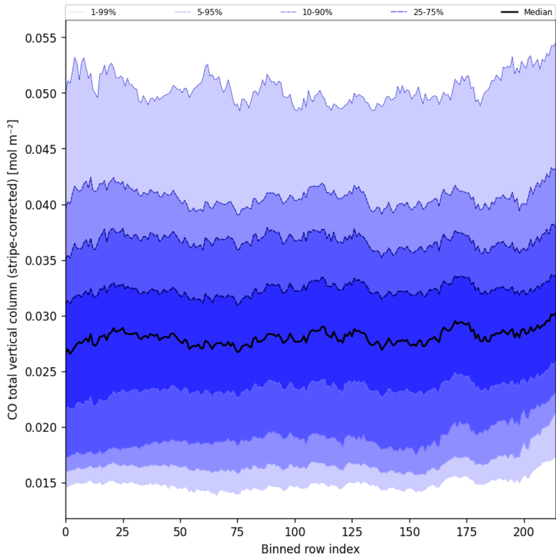
Figure 27: Along track statistics of “CO total vertical column (stripe-corrected)” for 2024-10-30 to 2024-10-31
