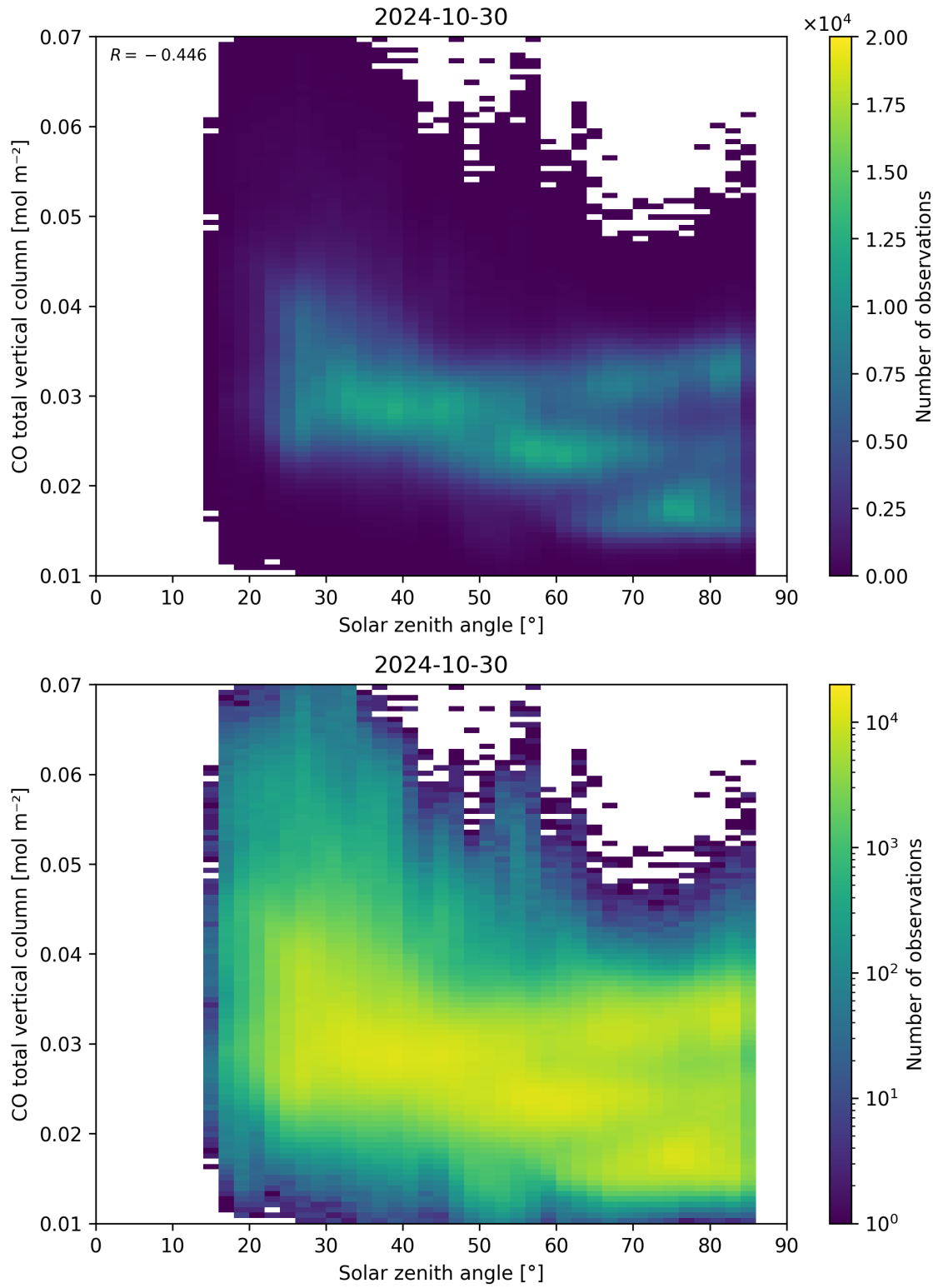
Figure 61: Scatter density plot of “Solar zenith angle” against “CO total vertical column” for 2024-10-30 to 2024-10-31.
