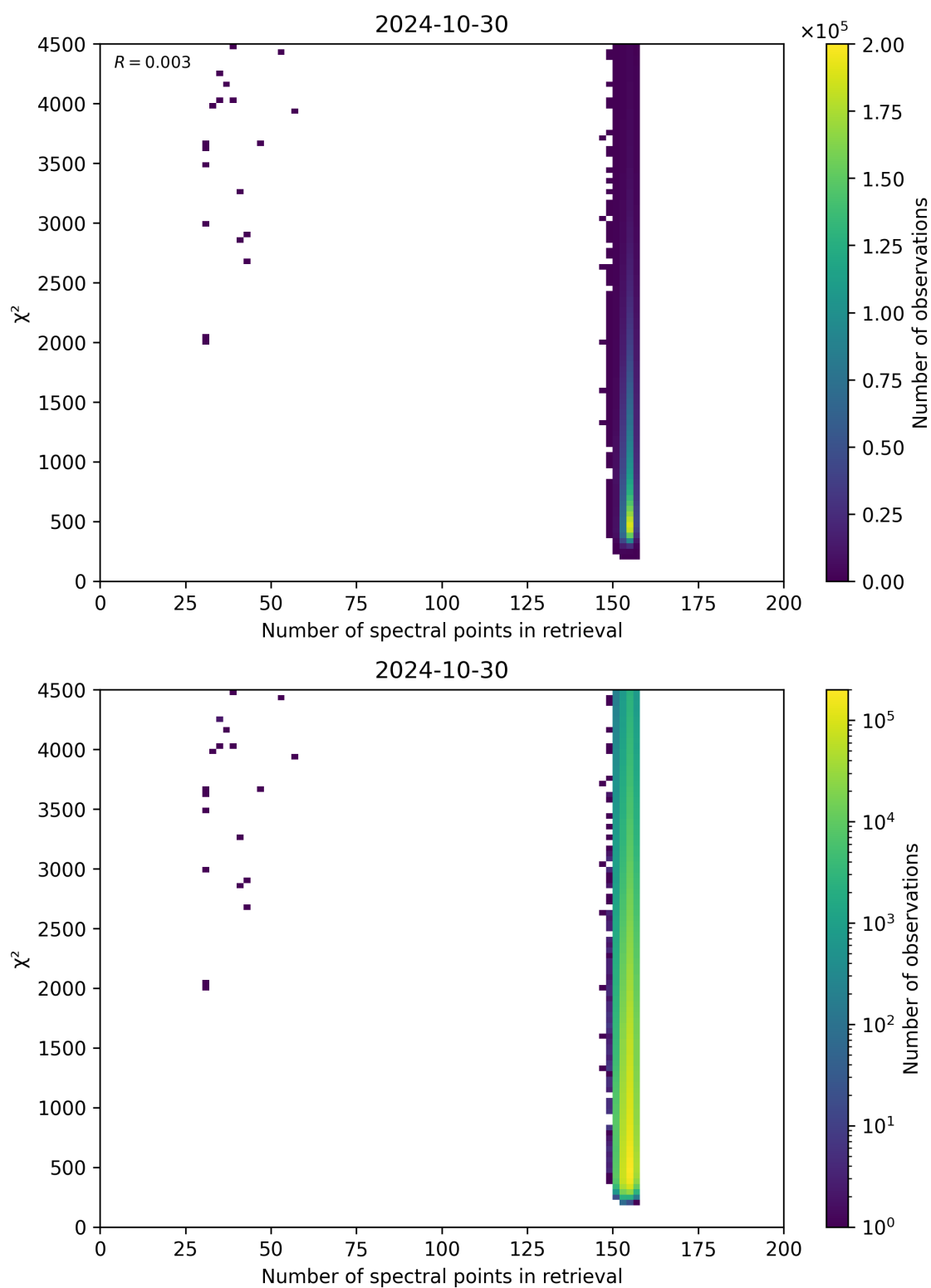
Figure 58: Scatter density plot of “Number of spectral points in retrieval” against “ \chi^2 ” for 2024-10-30 to 2024-10-31.
