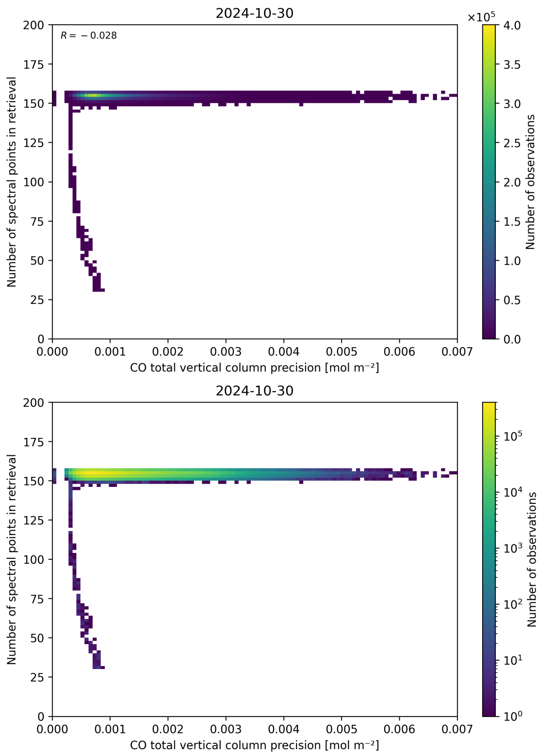
Figure 47: Scatter density plot of “CO total vertical column precision” against “Number of spectral points in retrieval” for 2024-10-30 to 2024-10-31.
