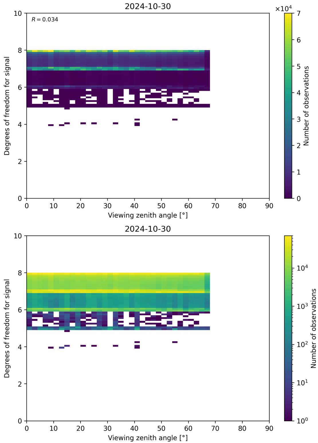
Figure 73: Scatter density plot of “Viewing zenith angle” against “Degrees of freedom for signal” for 2024-10-30 to 2024-10-31.
