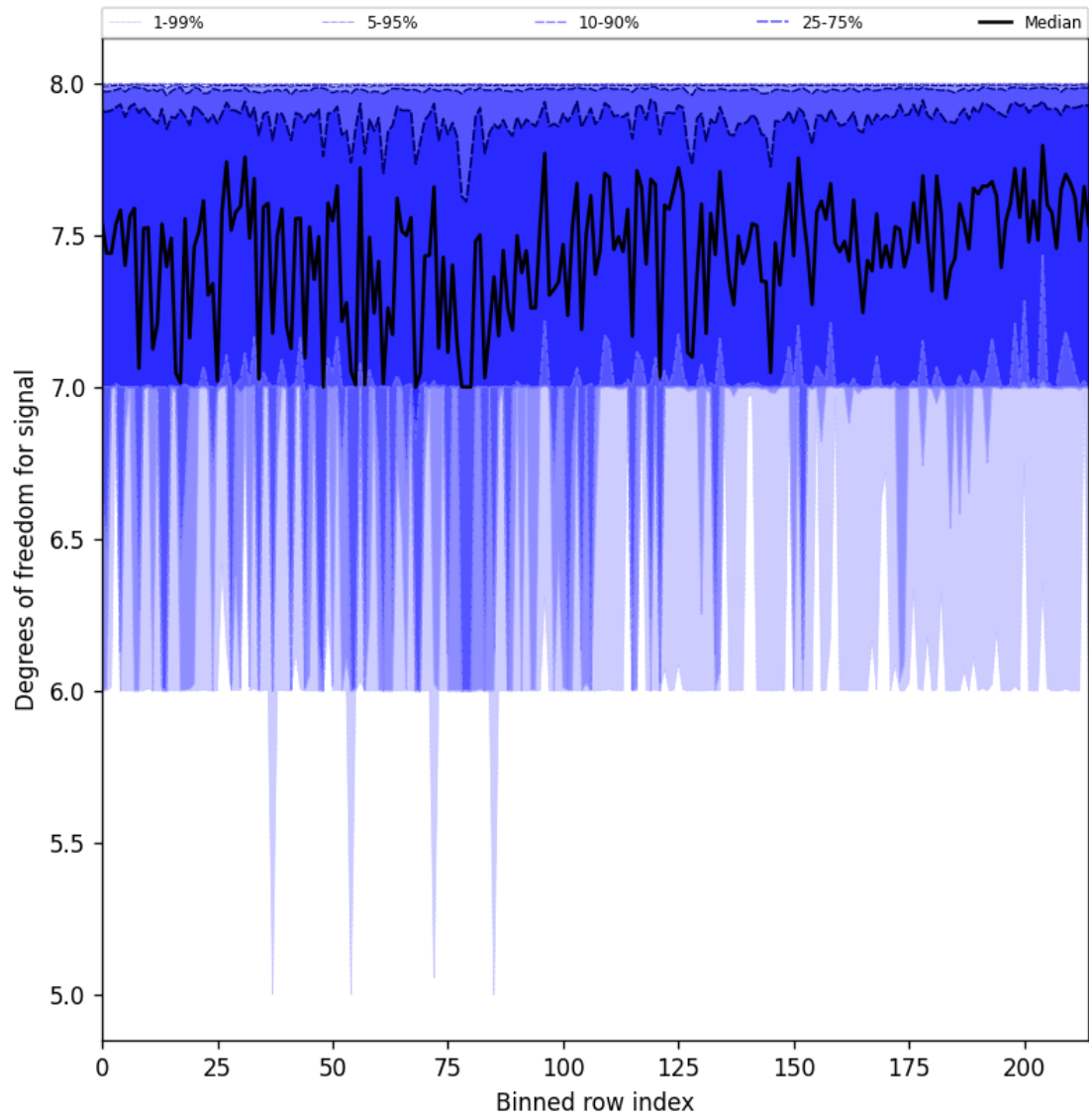
Figure 31: Along track statistics of “Degrees of freedom for signal” for 2024-10-30 to 2024-10-31
