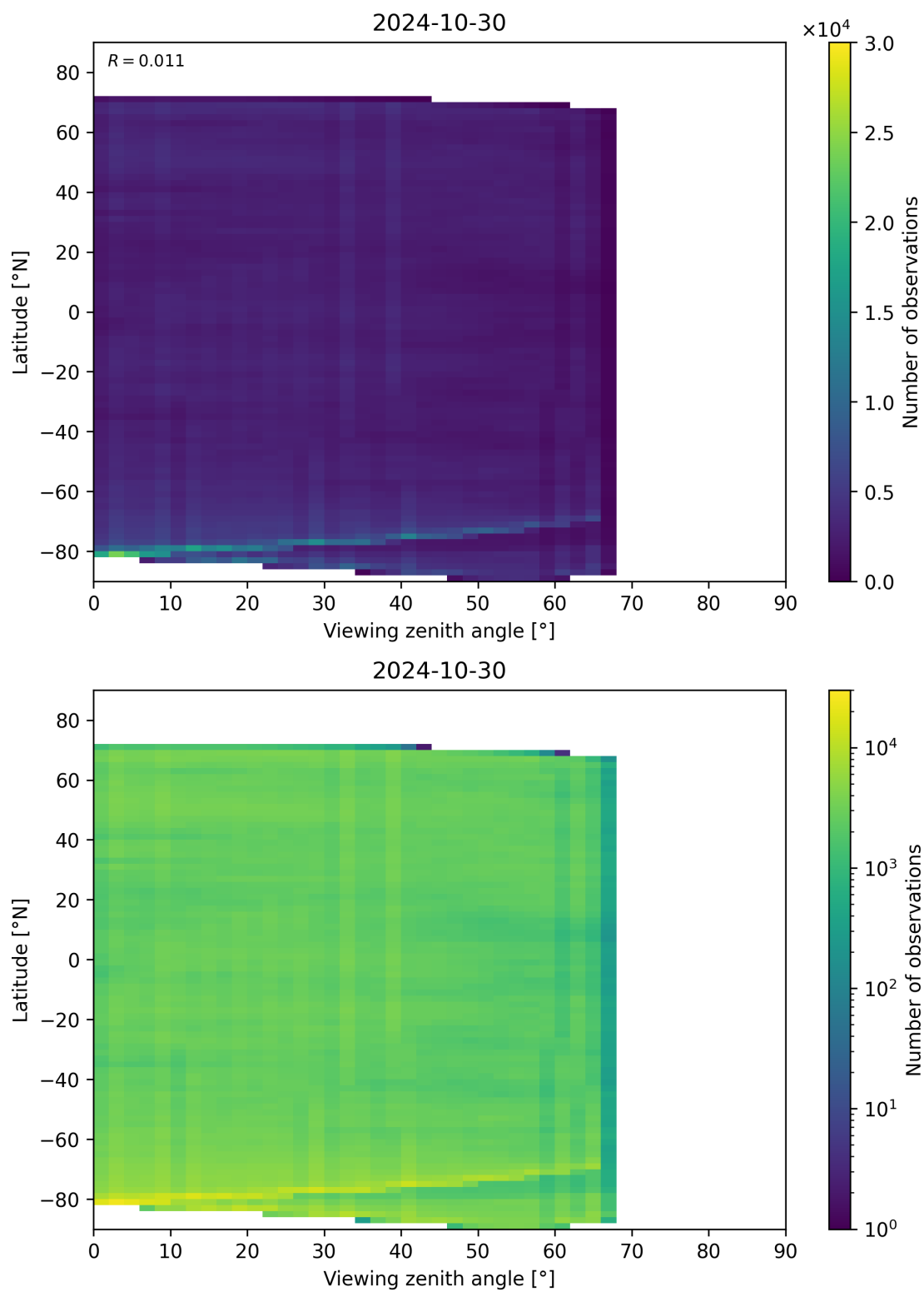
Figure 74: Scatter density plot of “Viewing zenith angle” against “Latitude” for 2024-10-30 to 2024-10-31.
