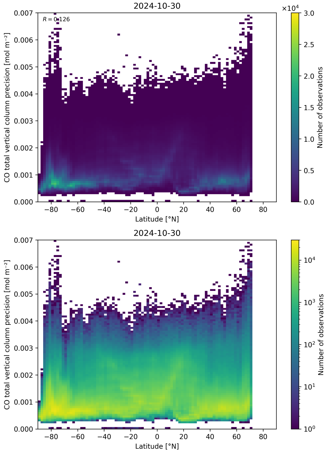
Figure 53: Scatter density plot of “Latitude” against “CO total vertical column precision” for 2024-10-30 to 2024-10-31.
