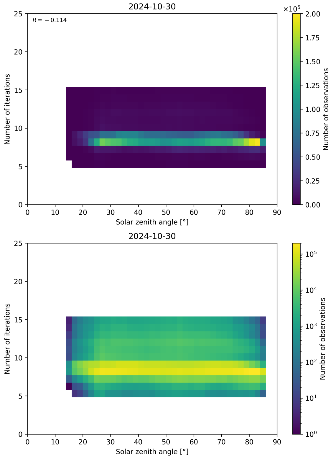
Figure 67: Scatter density plot of “Solar zenith angle” against “Number of iterations” for 2024-10-30 to 2024-10-31.
