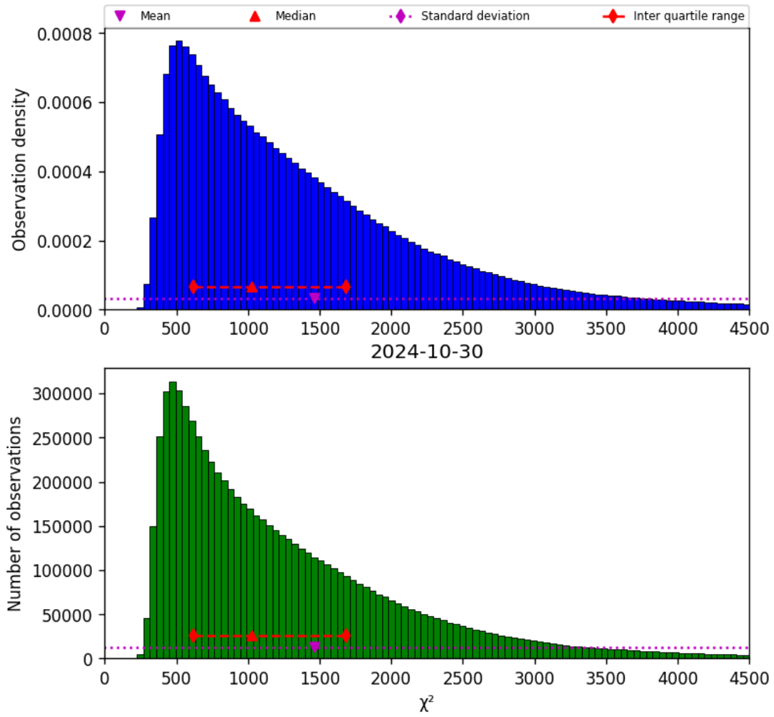
Figure 22: Histogram of “ \chi^2 ” for 2024-10-30 to 2024-10-31
