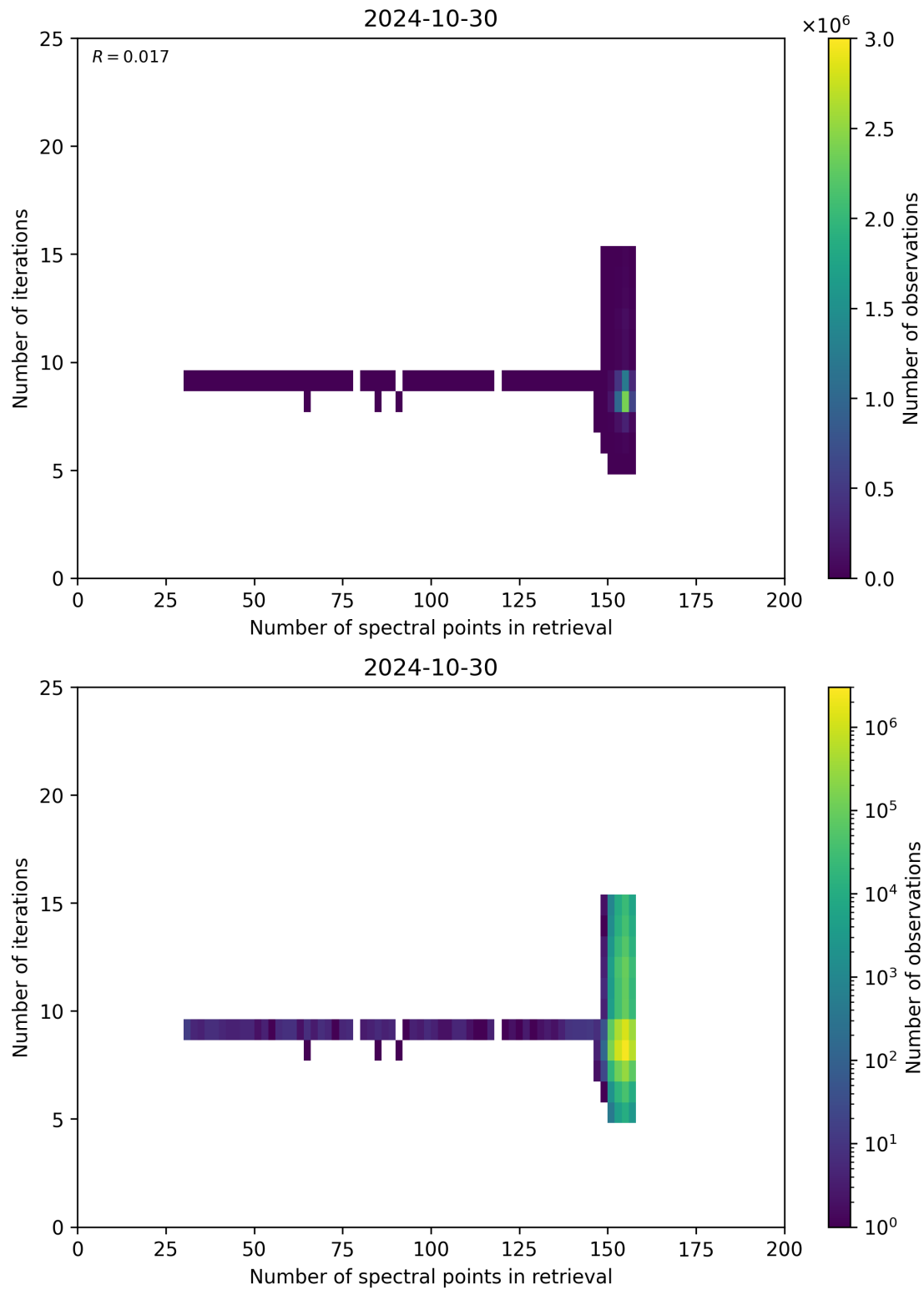
Figure 60: Scatter density plot of “Number of spectral points in retrieval” against “Number of iterations” for 2024-10-30 to 2024-10-31.
