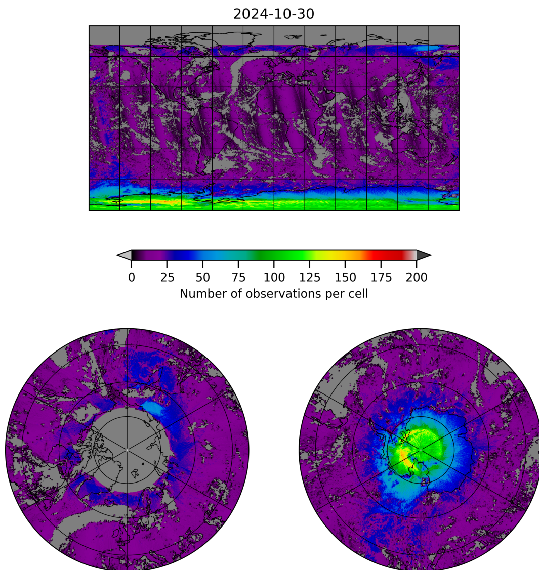
Figure 8: Map of the number of observations for 2024-10-30 to 2024-10-31
