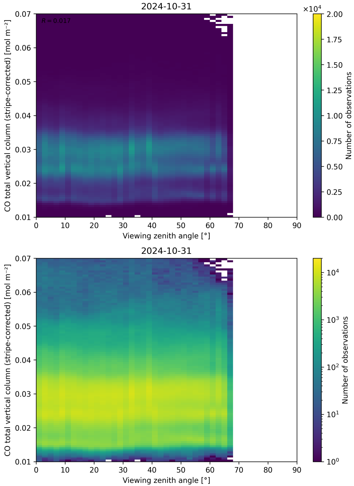
Figure 70: Scatter density plot of “Viewing zenith angle” against “CO total vertical column (stripe-corrected)” for 2024-10-30 to 2024-11-01.
