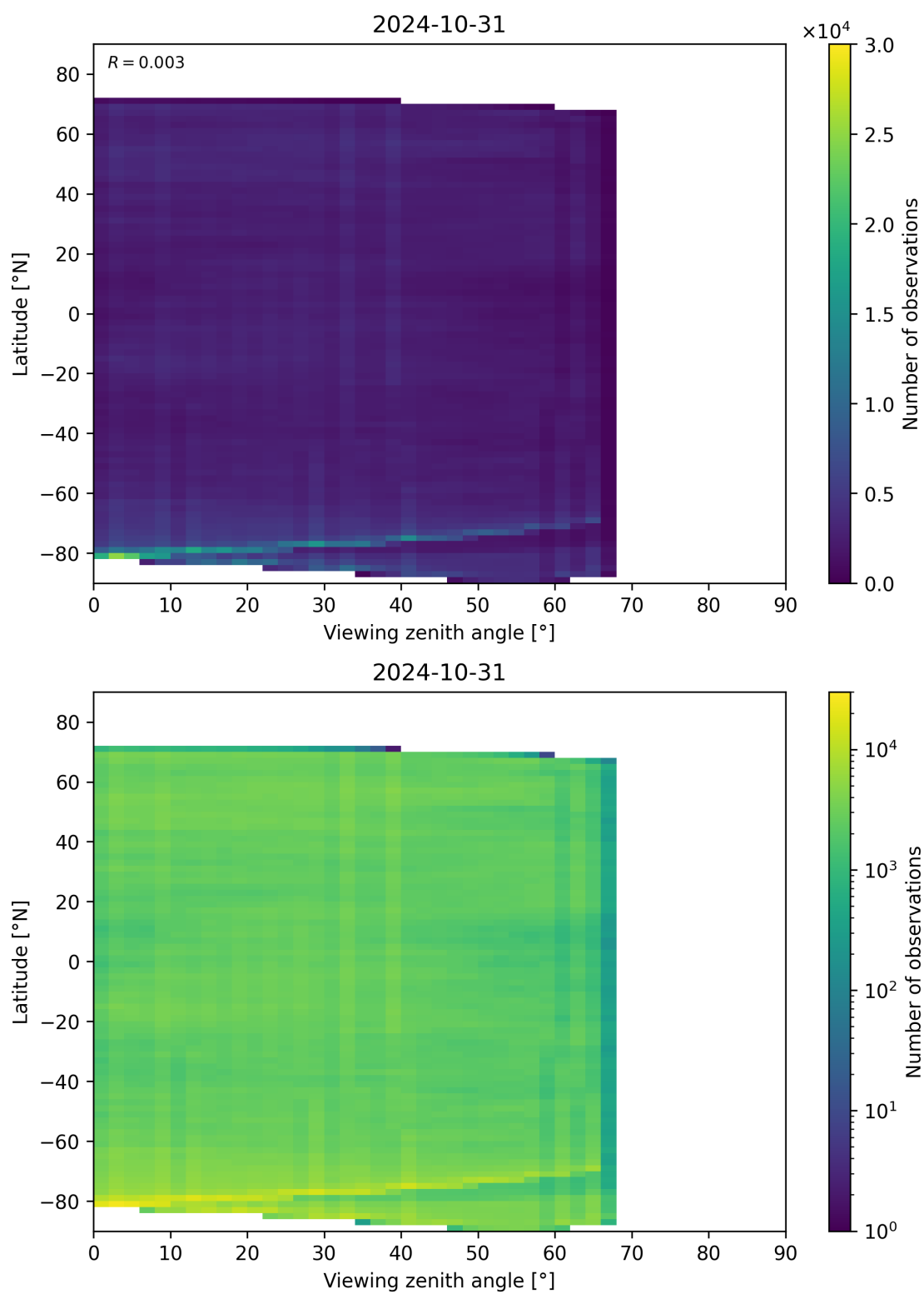
Figure 74: Scatter density plot of “Viewing zenith angle” against “Latitude” for 2024-10-30 to 2024-11-01.
