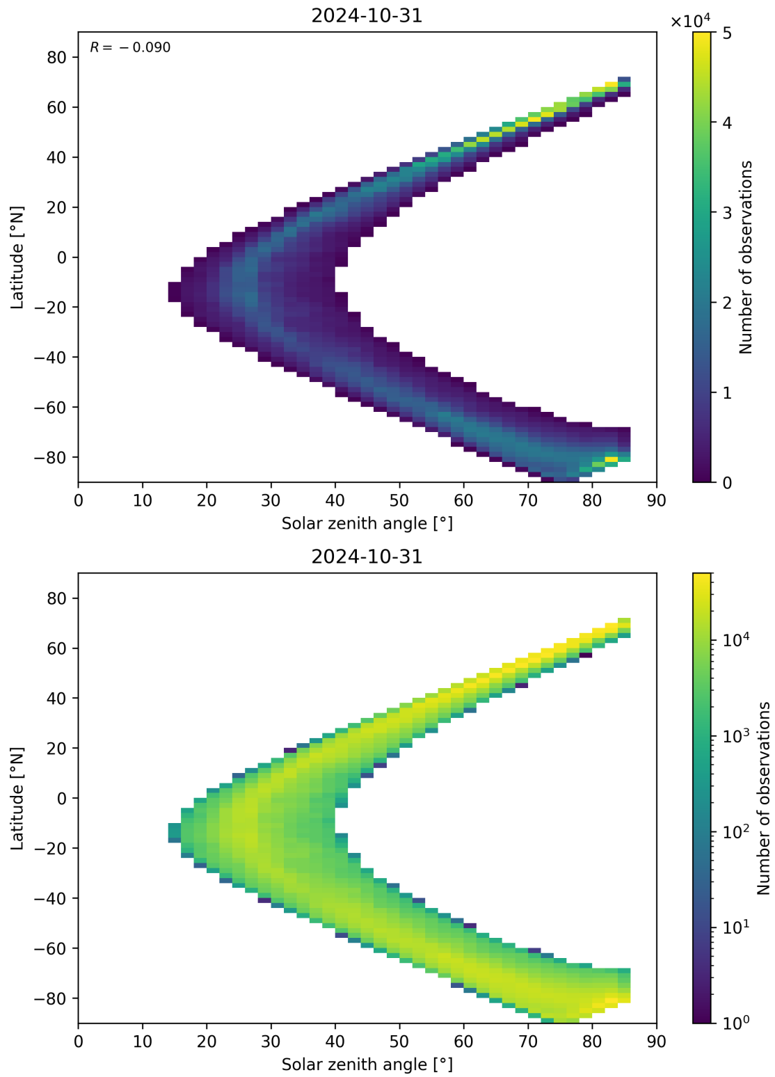
Figure 66: Scatter density plot of “Solar zenith angle” against “Latitude” for 2024-10-30 to 2024-11-01.
