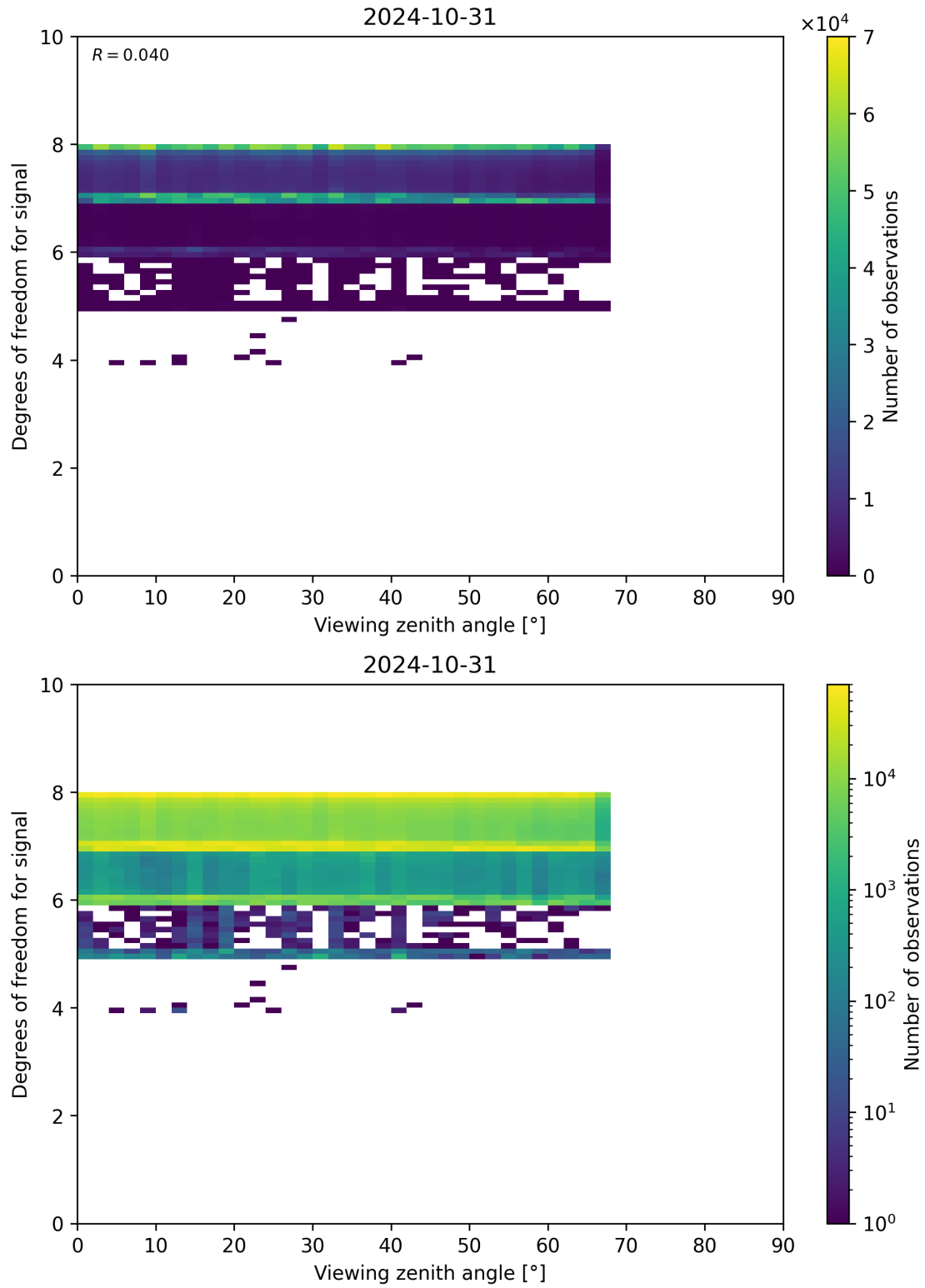
Figure 73: Scatter density plot of “Viewing zenith angle” against “Degrees of freedom for signal” for 2024-10-30 to 2024-11-01.
