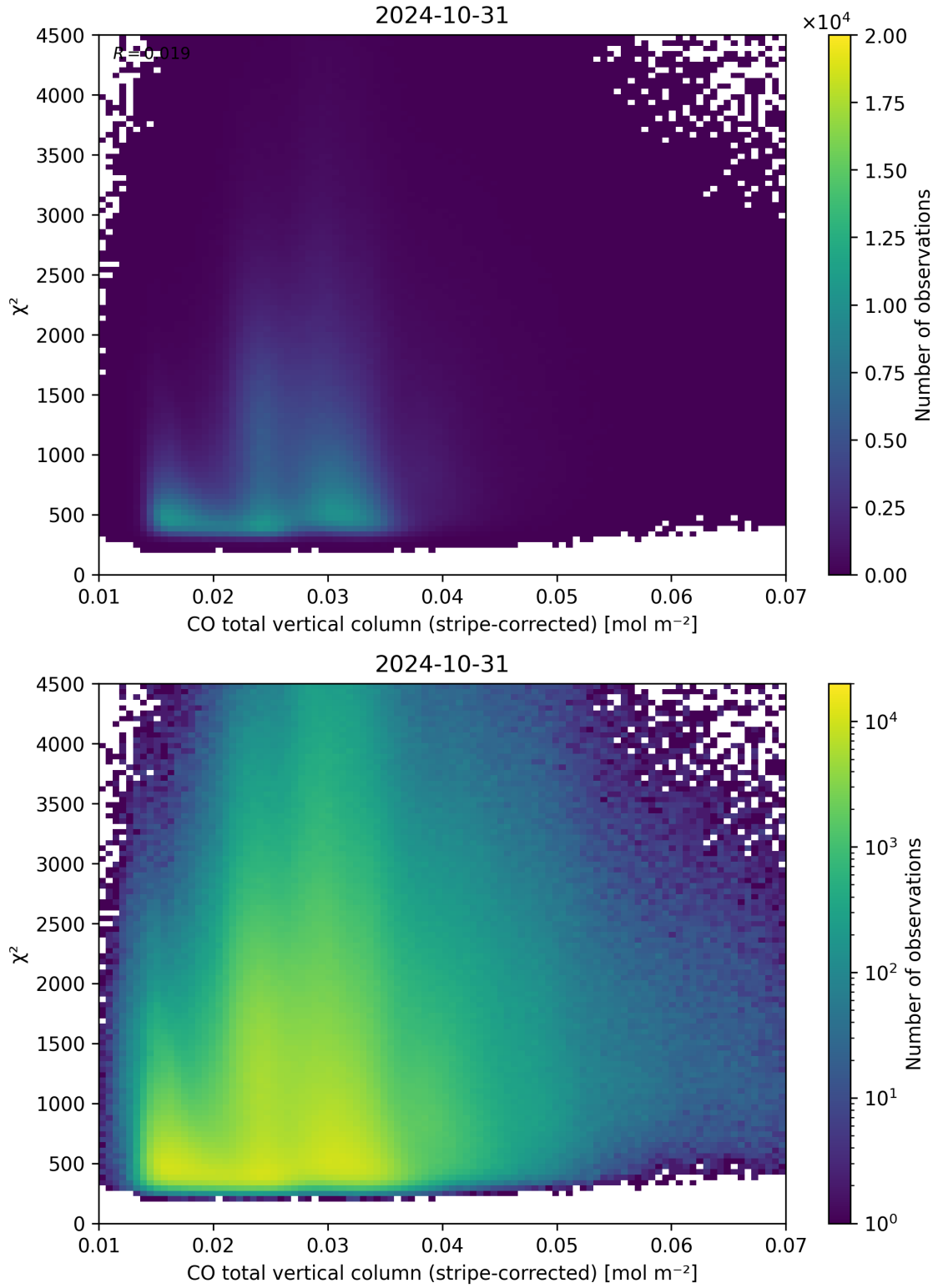
Figure 37: Scatter density plot of “CO total vertical column (stripe-corrected)” against “ \chi^2 ” for 2024-10-30 to 2024-11-01.
