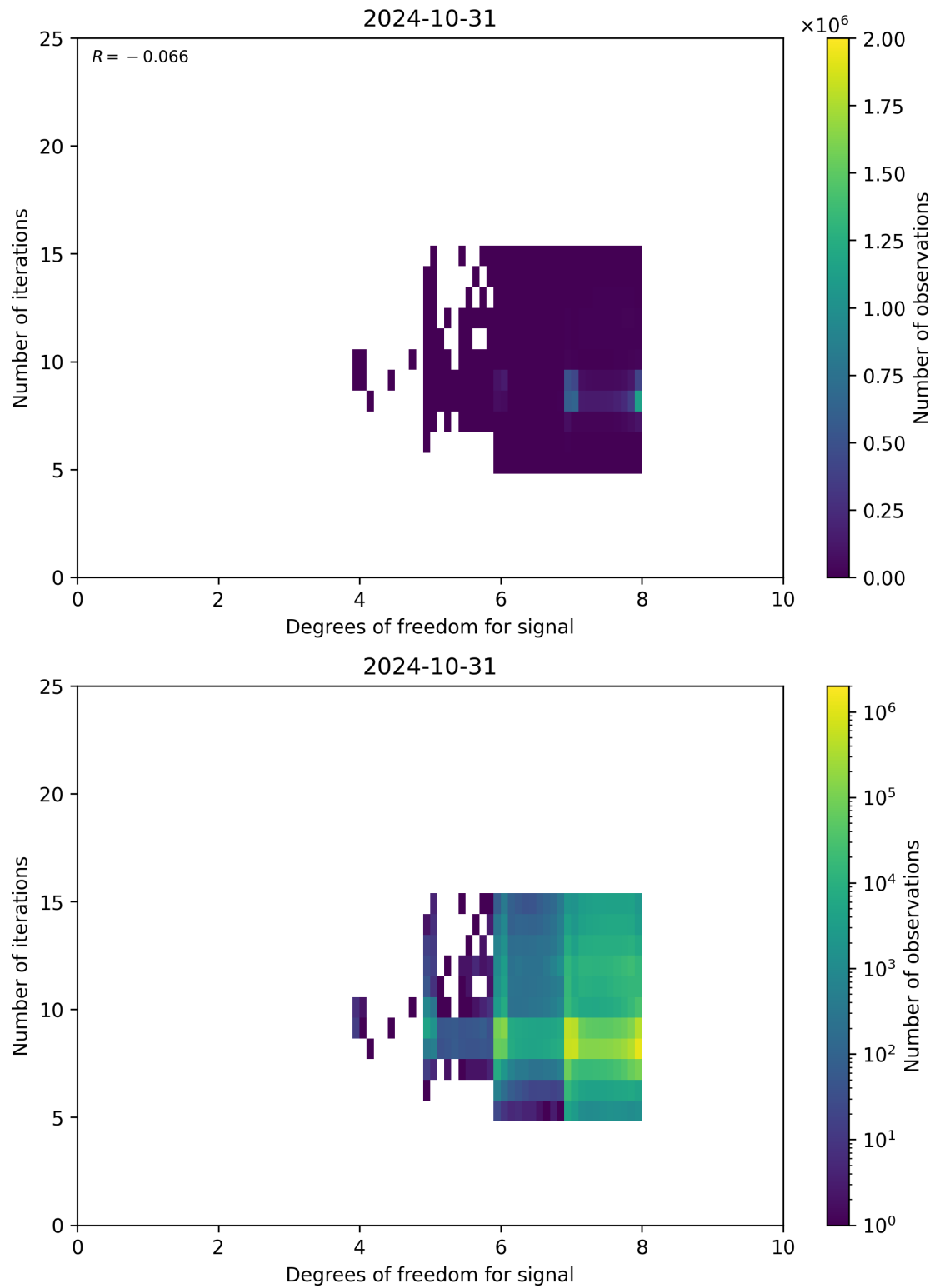
Figure 50: Scatter density plot of “Degrees of freedom for signal” against “Number of iterations” for 2024-10-30 to 2024-11-01.
