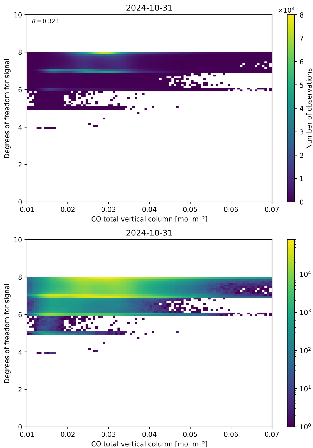
Figure 41: Scatter density plot of “CO total vertical column” against “Degrees of freedom for signal” for 2024-10-30 to 2024-11-01.
