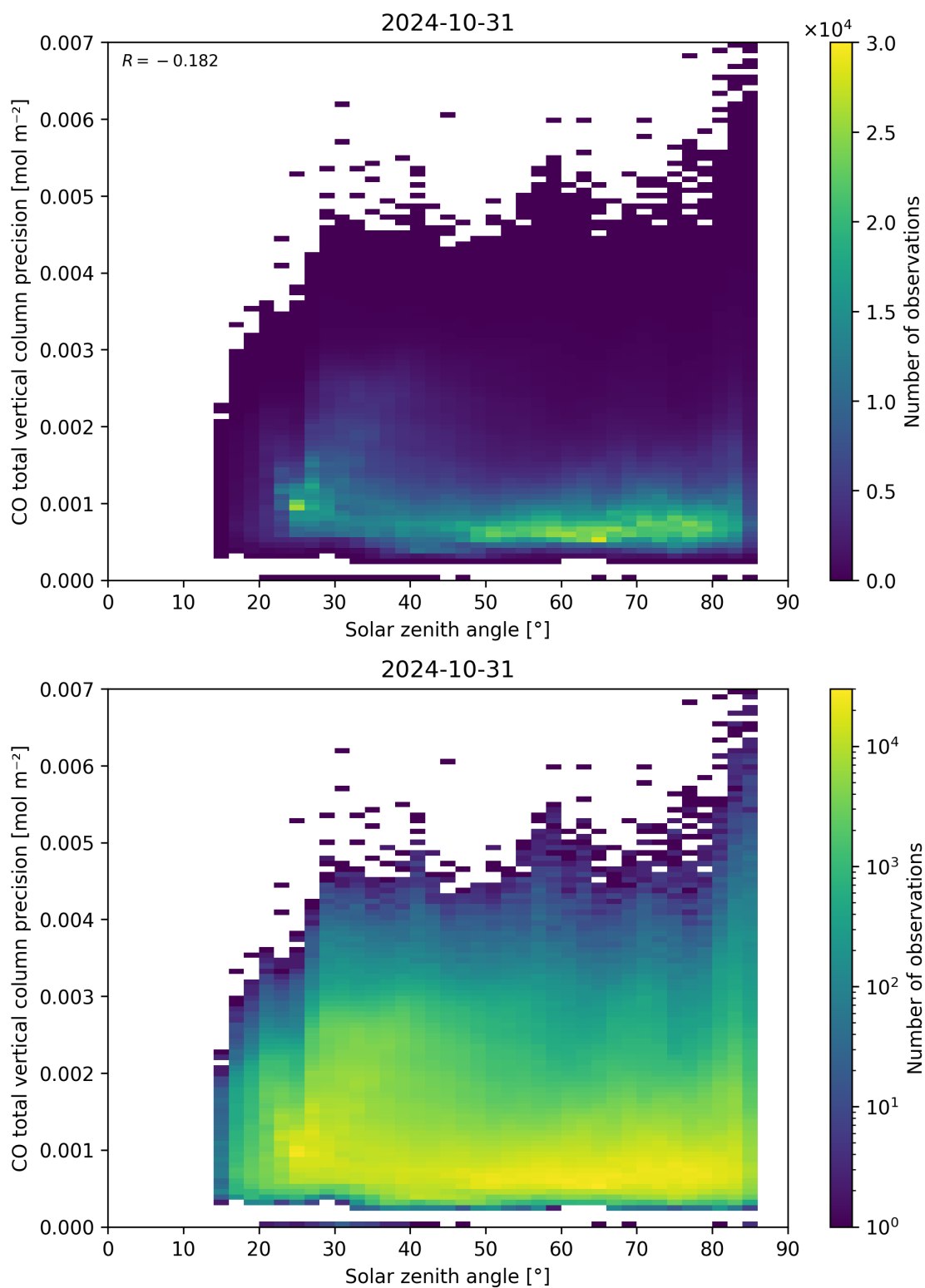
Figure 63: Scatter density plot of “Solar zenith angle” against “CO total vertical column precision” for 2024-10-30 to 2024-11-01.
