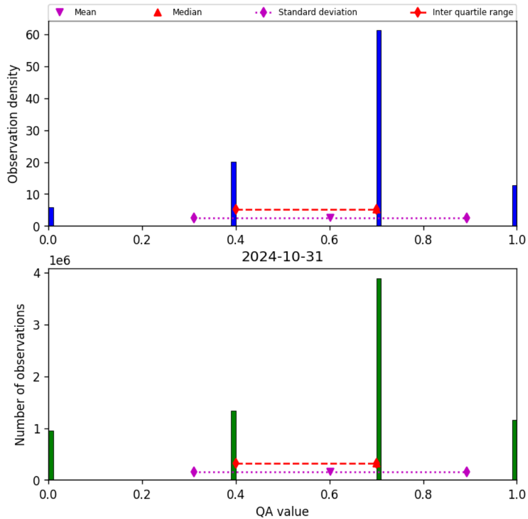
Figure 17: Histogram of “QA value” for 2024-10-30 to 2024-11-01
