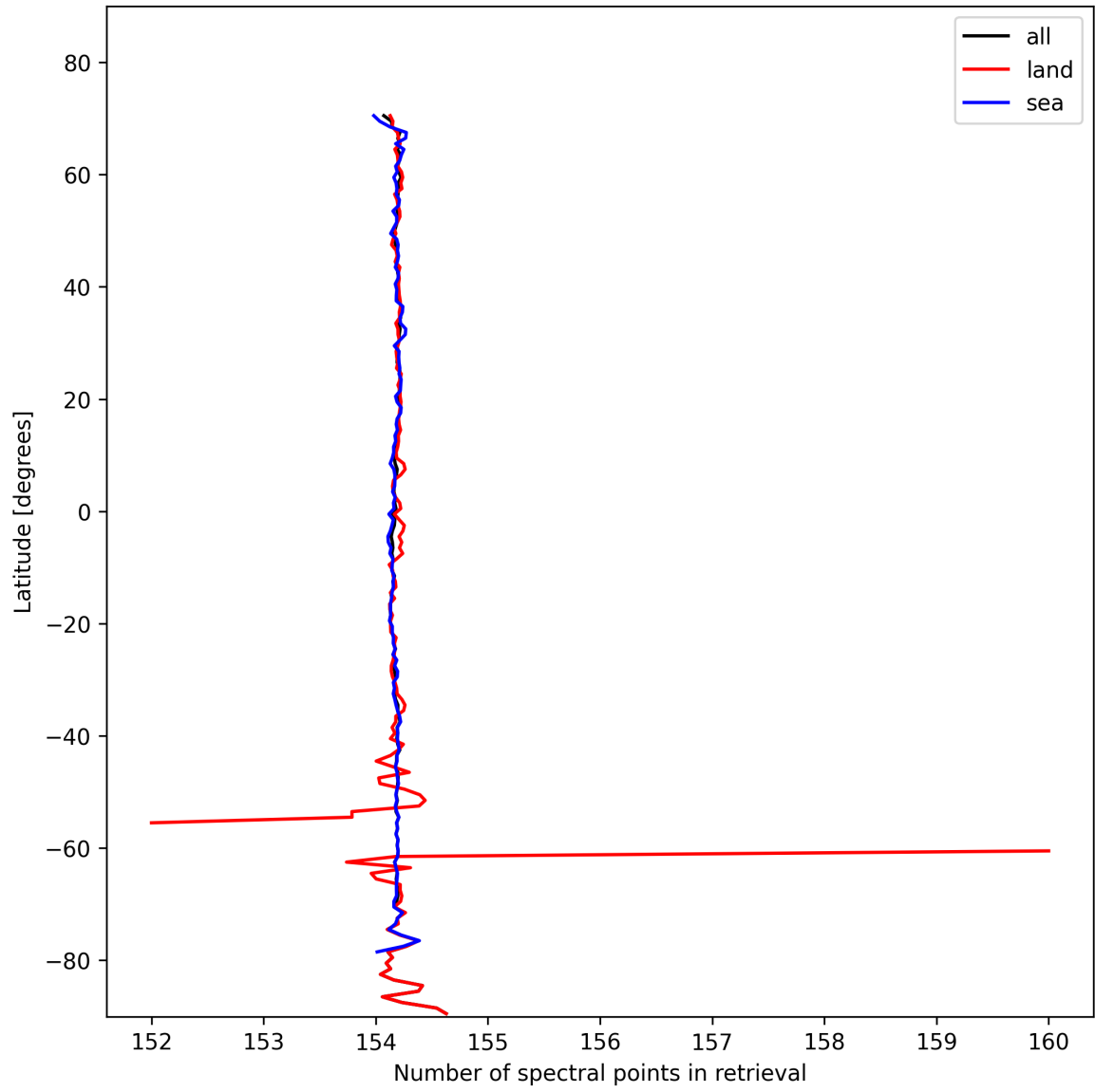
Figure 13: Zonal average of “Number of spectral points in retrieval” for 2024-10-30 to 2024-11-01.
