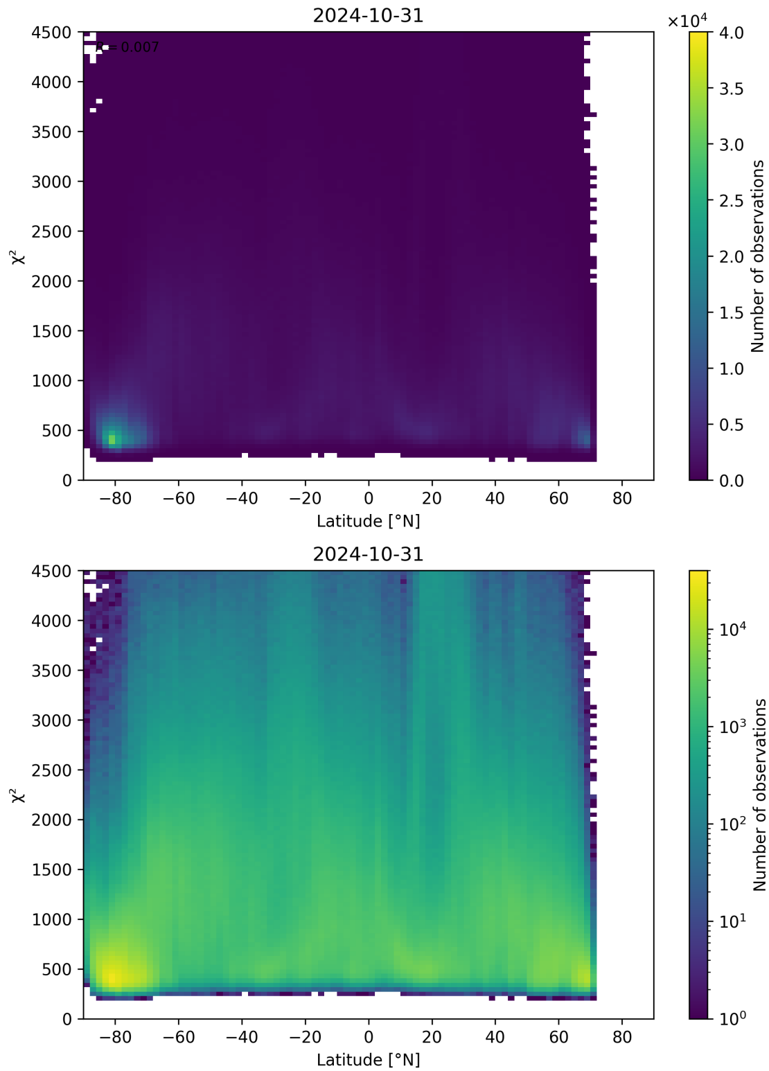
Figure 54: Scatter density plot of “Latitude” against “ \chi^2 ” for 2024-10-30 to 2024-11-01.
