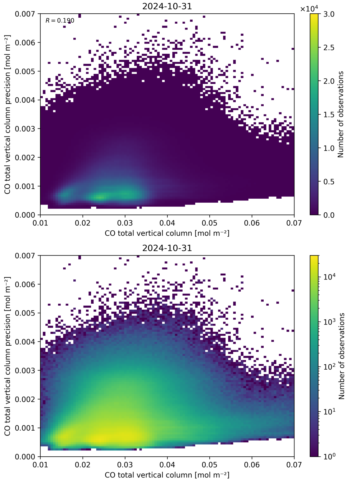
Figure 34: Scatter density plot of “CO total vertical column” against “CO total vertical column precision” for 2024-10-30 to 2024-11-01.
