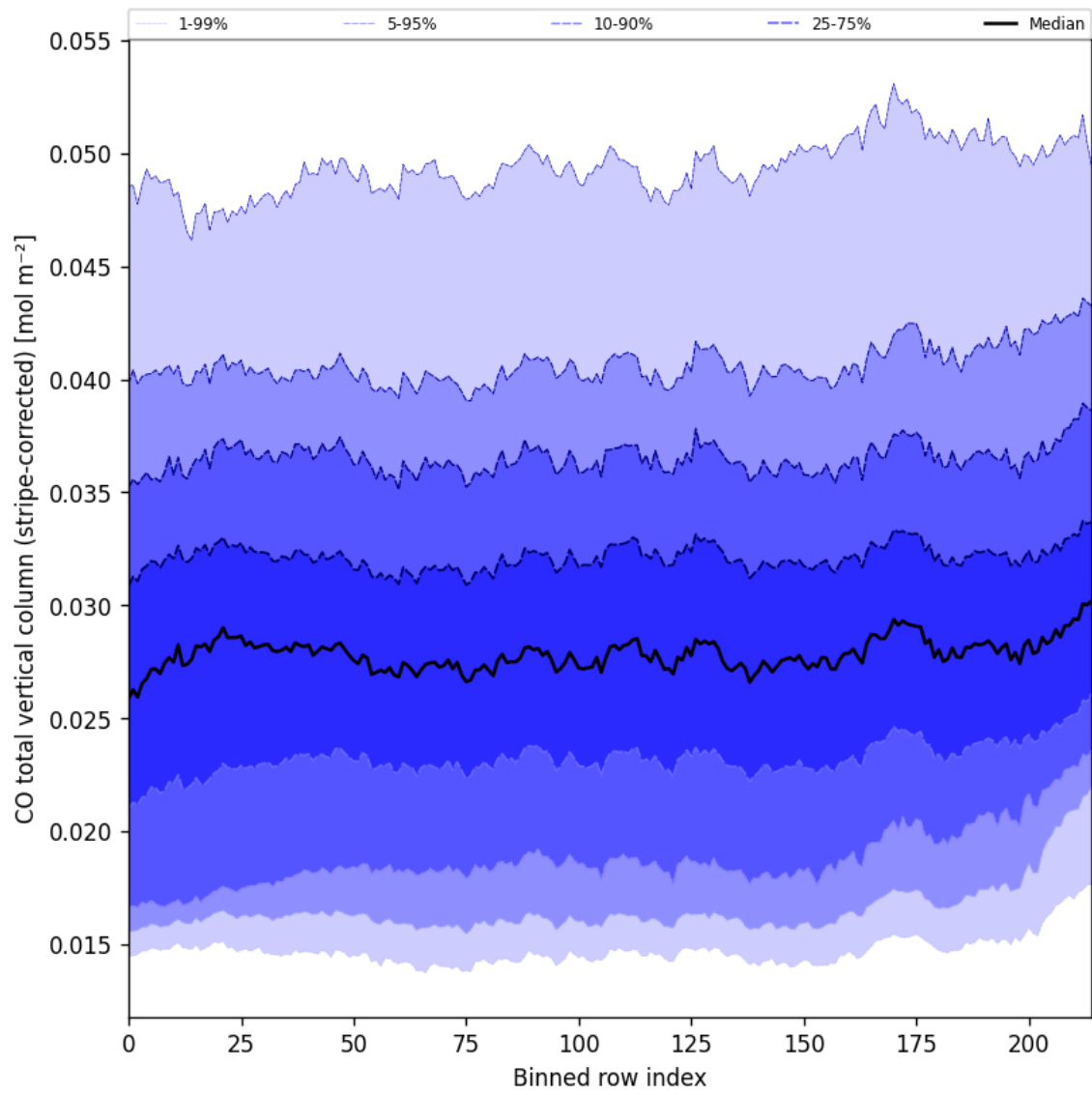
Figure 27: Along track statistics of “CO total vertical column (stripe-corrected)” for 2024-10-30 to 2024-11-01
