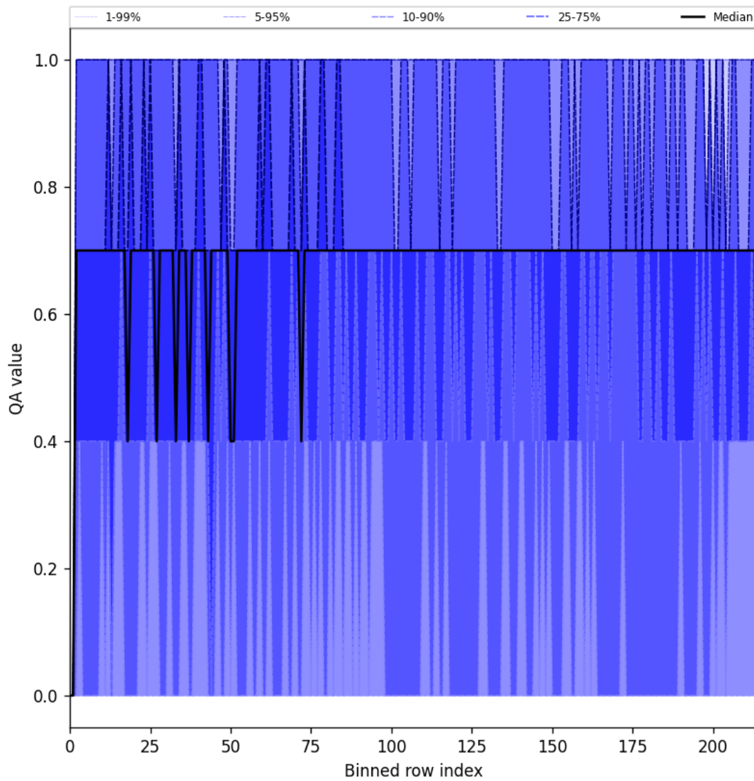
Figure 25: Along track statistics of “QA value” for 2024-10-30 to 2024-11-01
