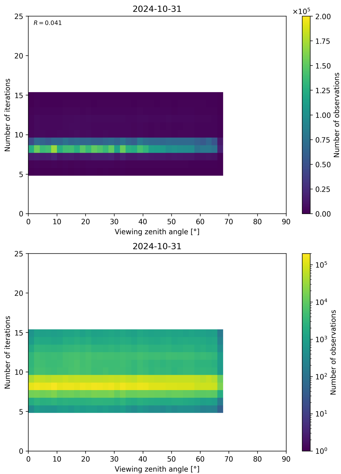
Figure 75: Scatter density plot of “Viewing zenith angle” against “Number of iterations” for 2024-10-30 to 2024-11-01.
