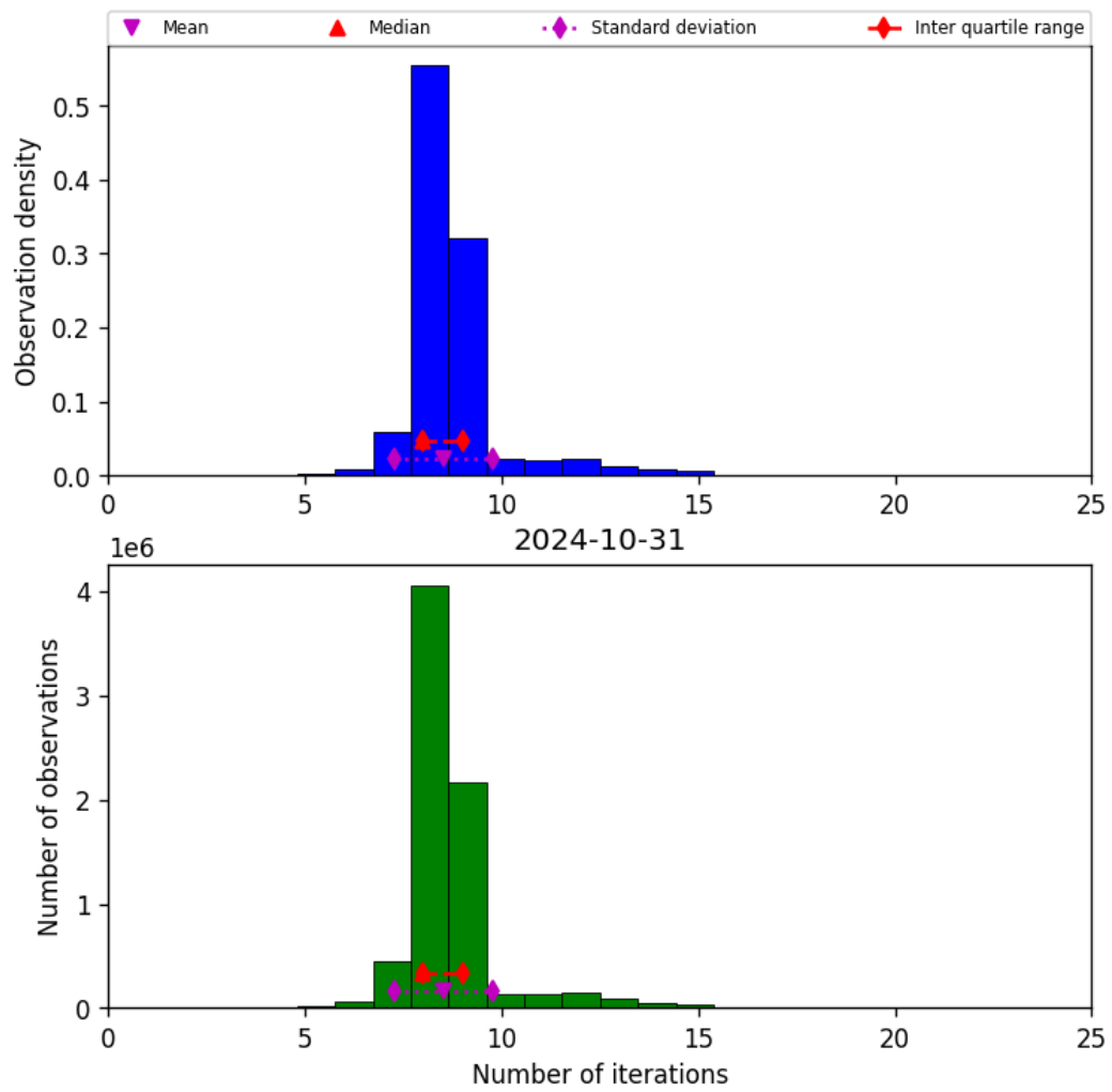
Figure 24: Histogram of “Number of iterations” for 2024-10-30 to 2024-11-01
