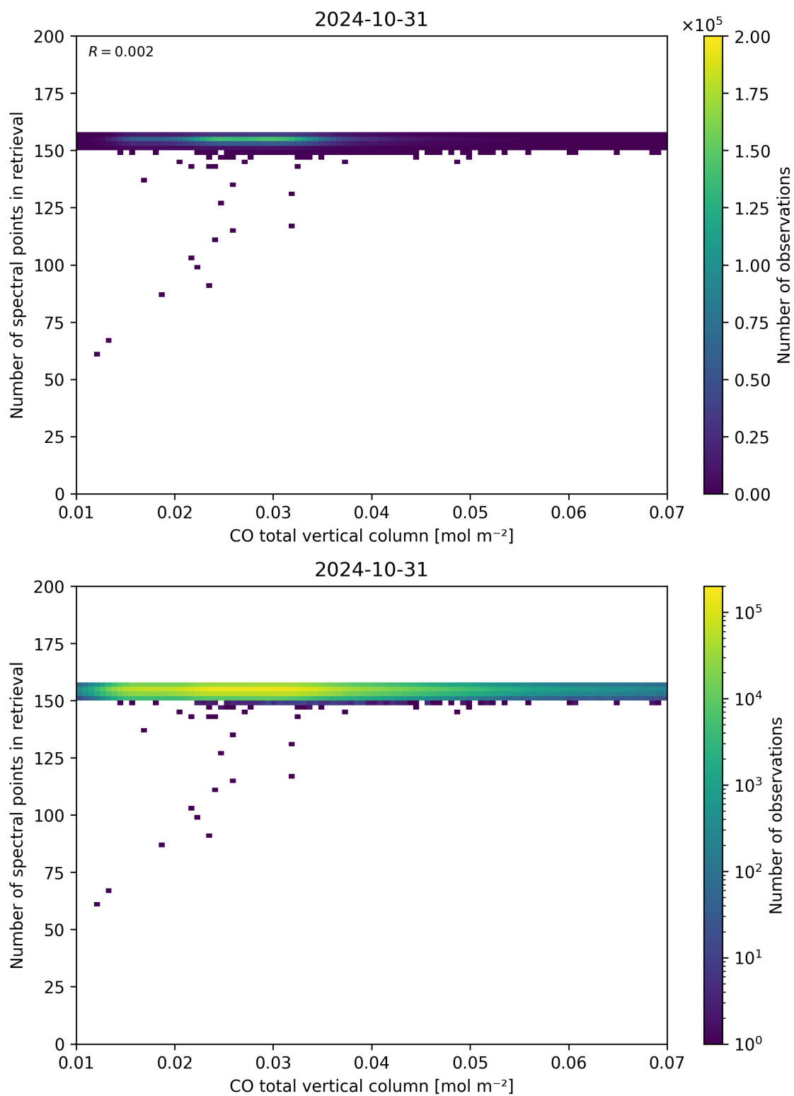
Figure 43: Scatter density plot of “CO total vertical column” against “Number of spectral points in retrieval” for 2024-10-30 to 2024-11-01.
