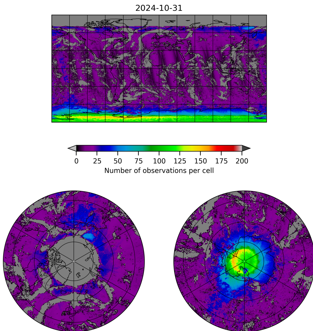
Figure 8: Map of the number of observations for 2024-10-30 to 2024-11-01
