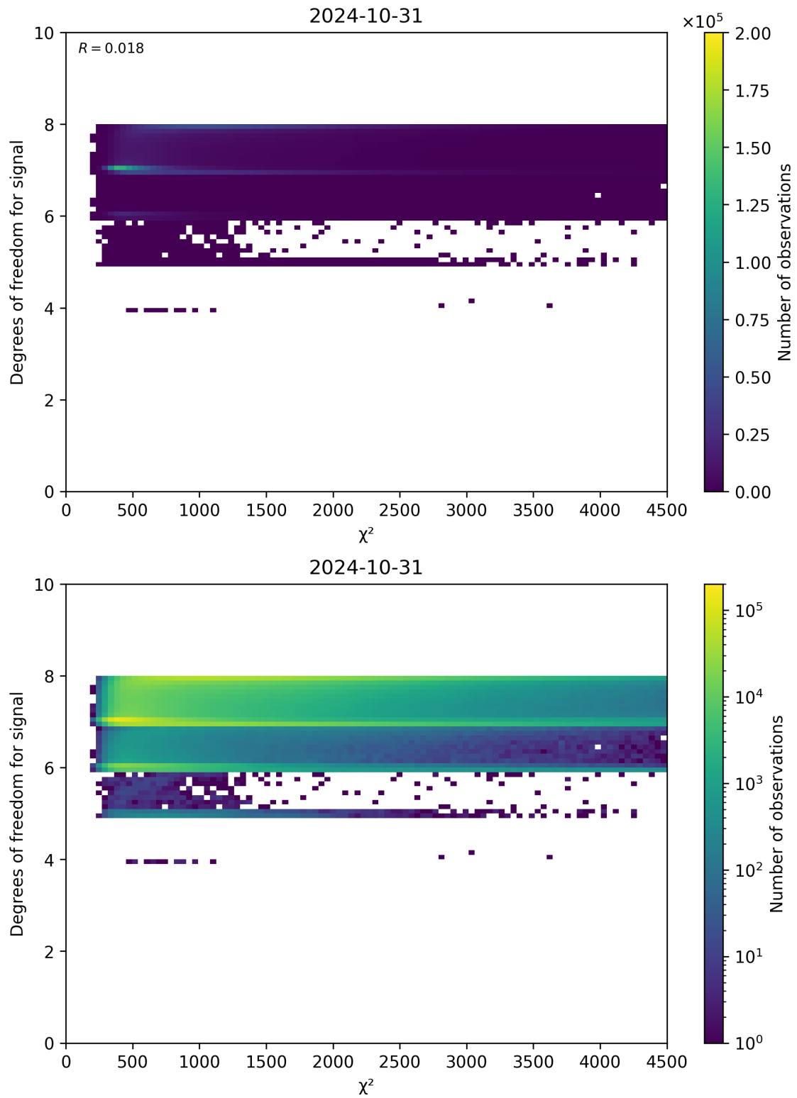
Figure 48: Scatter density plot of “ \chi^2 ” against “Degrees of freedom for signal” for 2024-10-30 to 2024-11-01.
