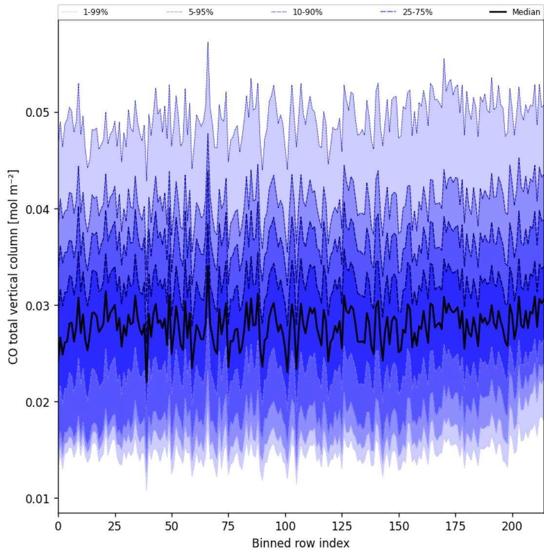
Figure 26: Along track statistics of “CO total vertical column” for 2024-10-30 to 2024-11-01
