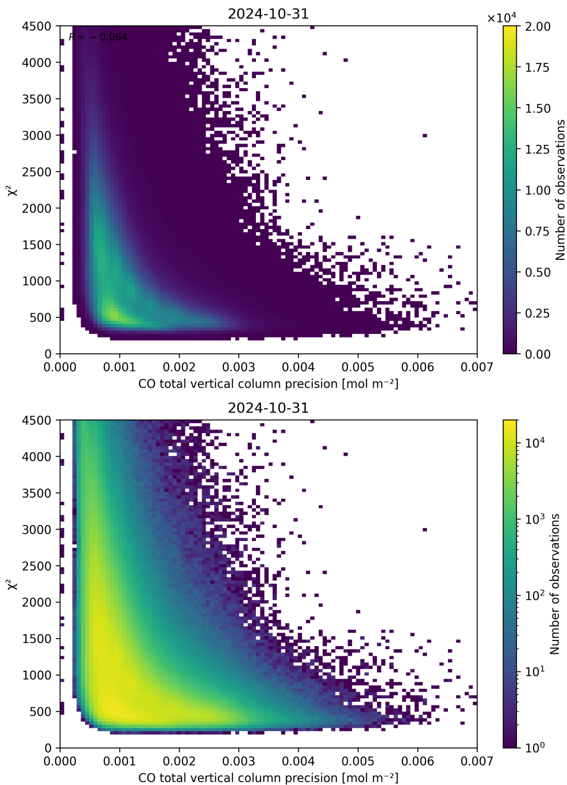
Figure 44: Scatter density plot of “CO total vertical column precision” against “ \chi^2 ” for 2024-10-30 to 2024-11-01.
