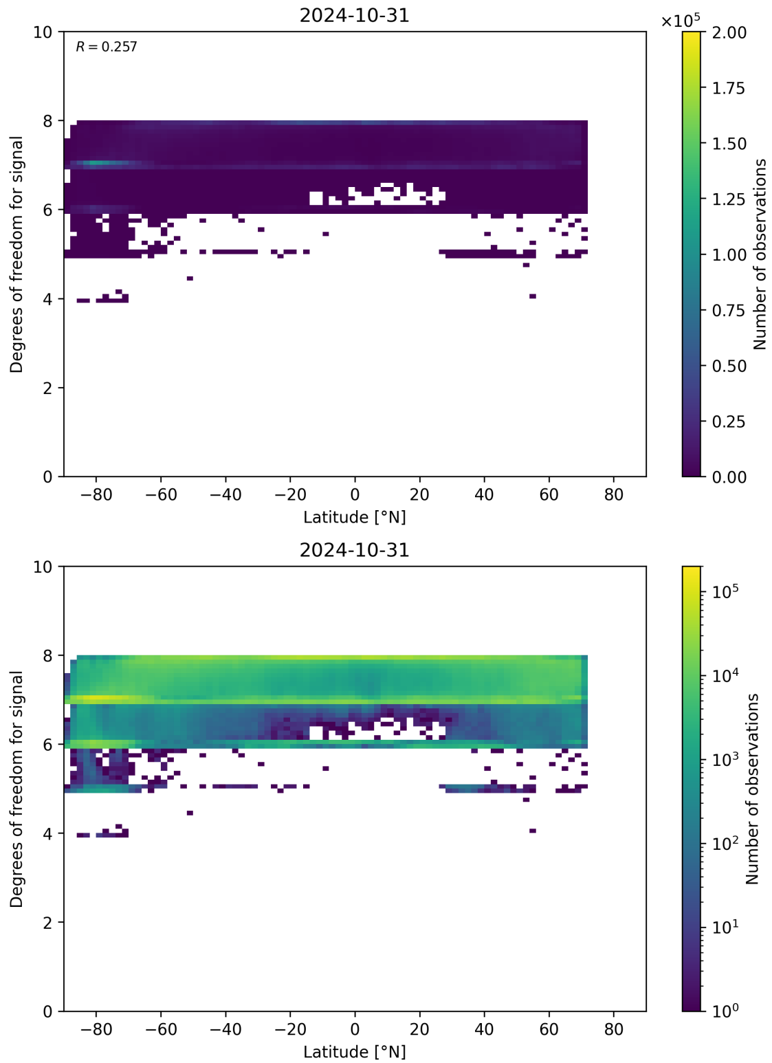
Figure 55: Scatter density plot of “Latitude” against “Degrees of freedom for signal” for 2024-10-30 to 2024-11-01.
