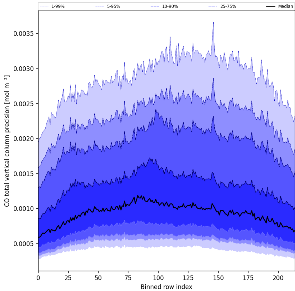
Figure 28: Along track statistics of “CO total vertical column precision” for 2024-10-30 to 2024-11-01
