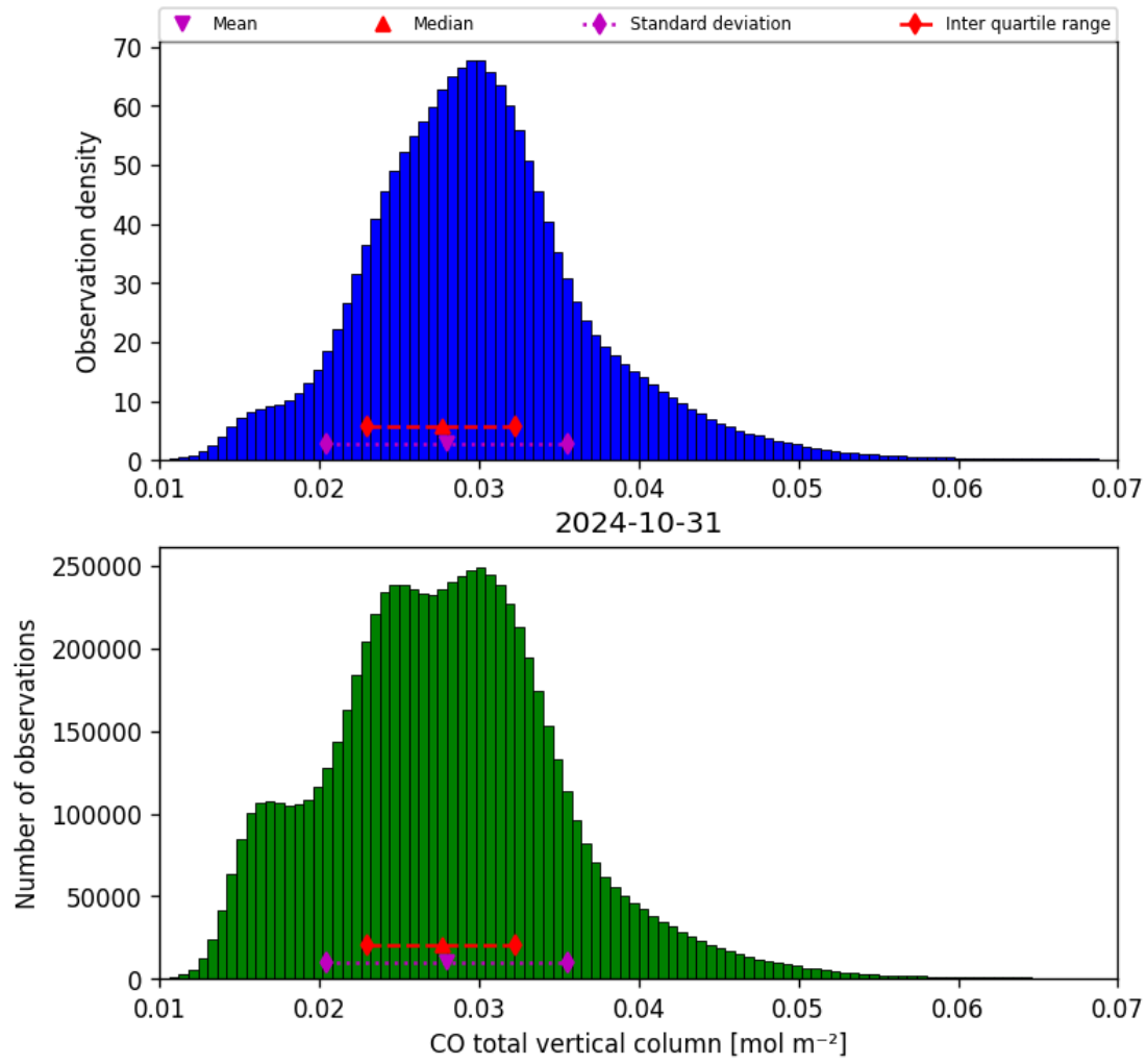
Figure 18: Histogram of “CO total vertical column” for 2024-10-30 to 2024-11-01
