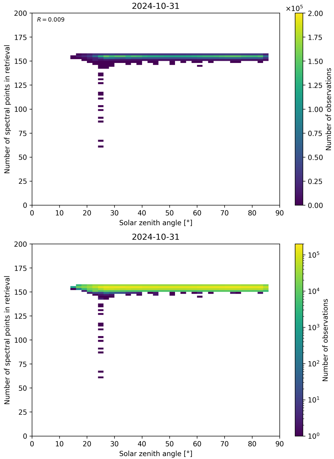
Figure 68: Scatter density plot of “Solar zenith angle” against “Number of spectral points in retrieval” for 2024-10-30 to 2024-11-01.
