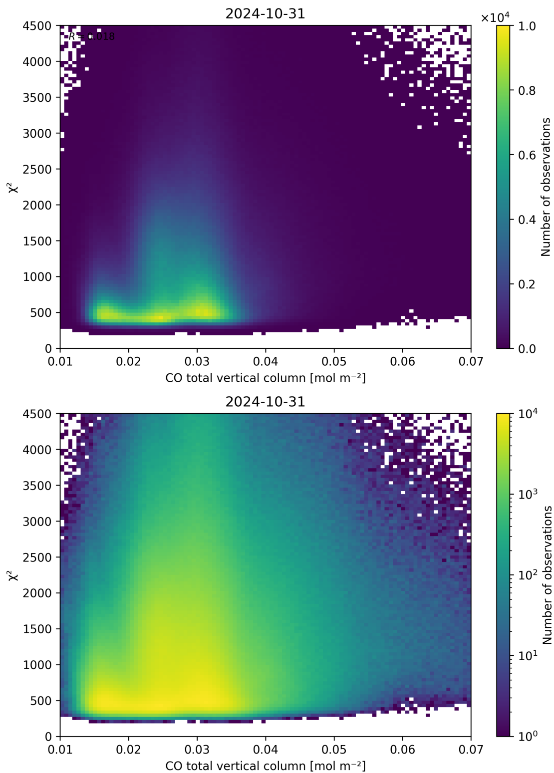
Figure 35: Scatter density plot of “CO total vertical column” against “ \chi^2 ” for 2024-10-30 to 2024-11-01.
