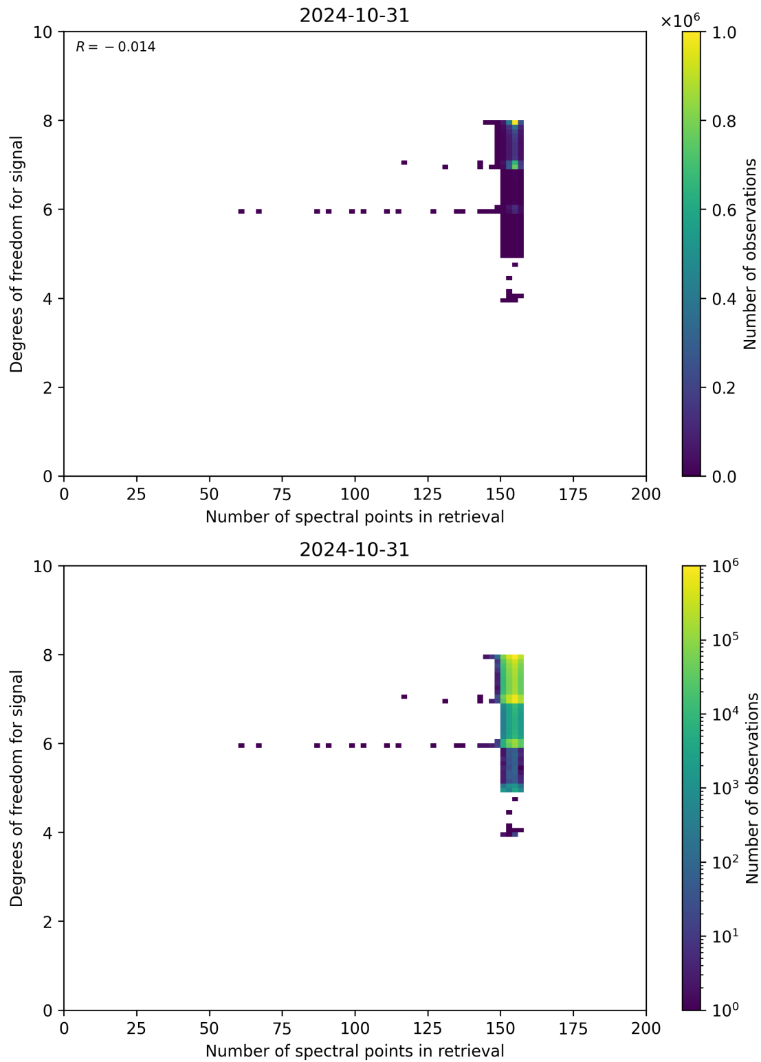
Figure 59: Scatter density plot of “Number of spectral points in retrieval” against “Degrees of freedom for signal” for 2024-10-30 to 2024-11-01.
