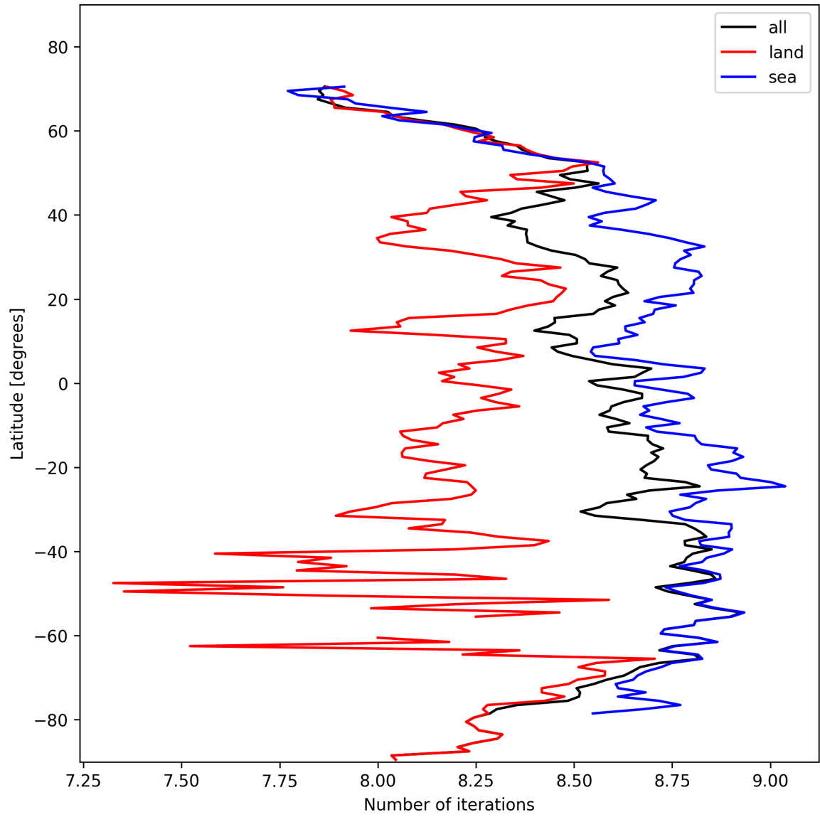
Figure 16: Zonal average of “Number of iterations” for 2024-10-30 to 2024-11-01.
