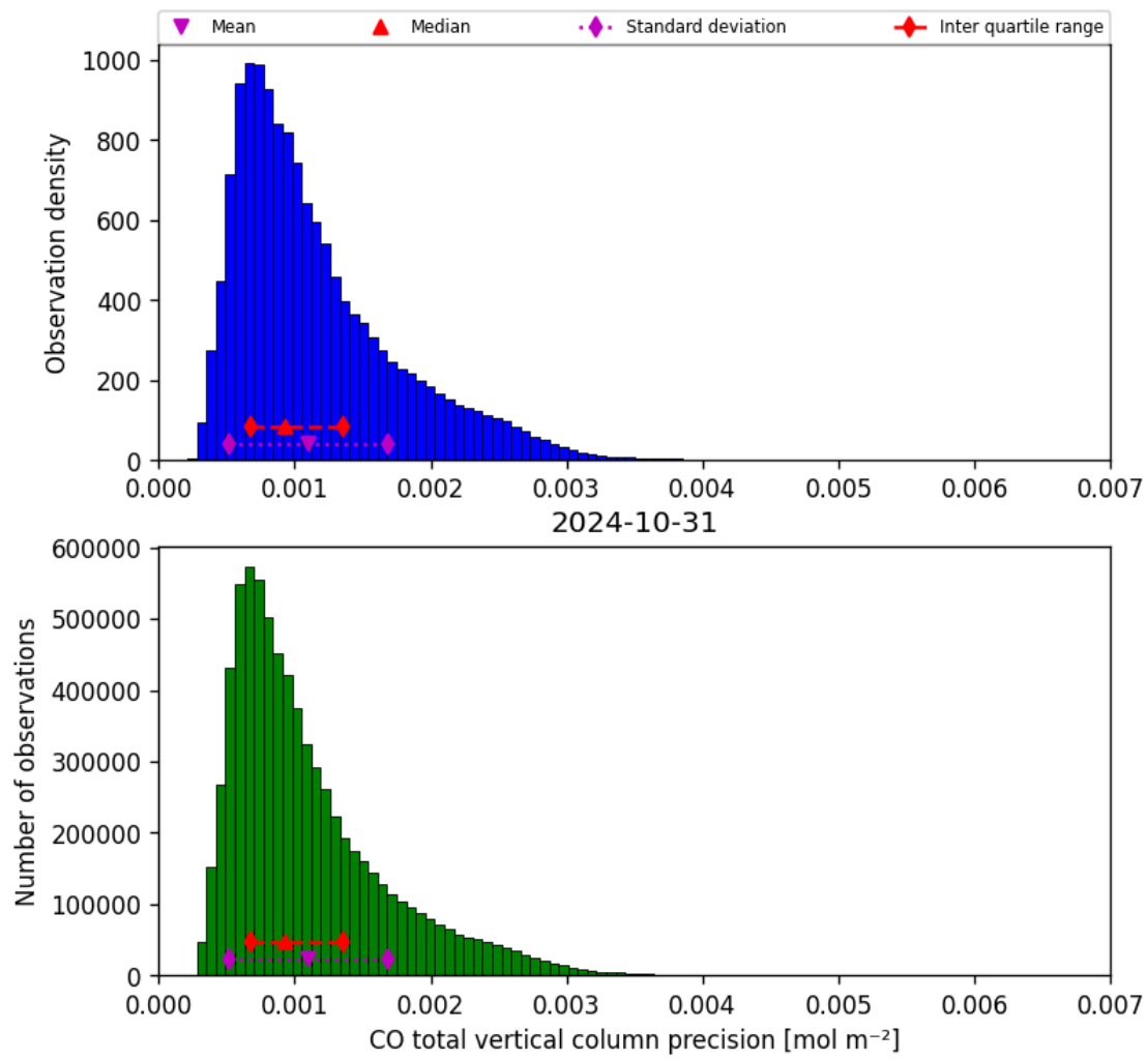
Figure 20: Histogram of “CO total vertical column precision” for 2024-10-30 to 2024-11-01
