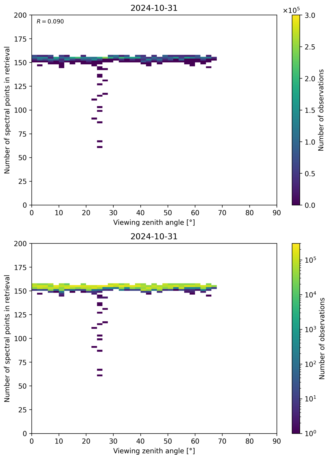
Figure 76: Scatter density plot of “Viewing zenith angle” against “Number of spectral points in retrieval” for 2024-10-30 to 2024-11-01.
