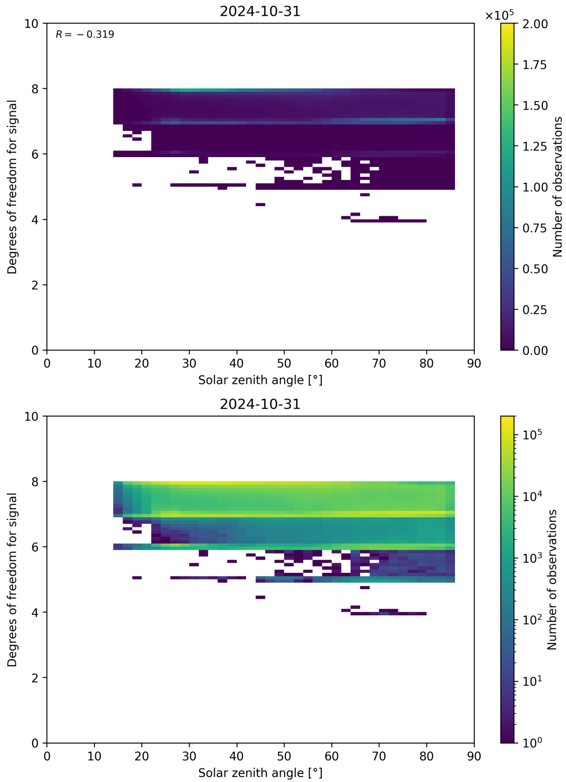
Figure 65: Scatter density plot of “Solar zenith angle” against “Degrees of freedom for signal” for 2024-10-30 to 2024-11-01.
