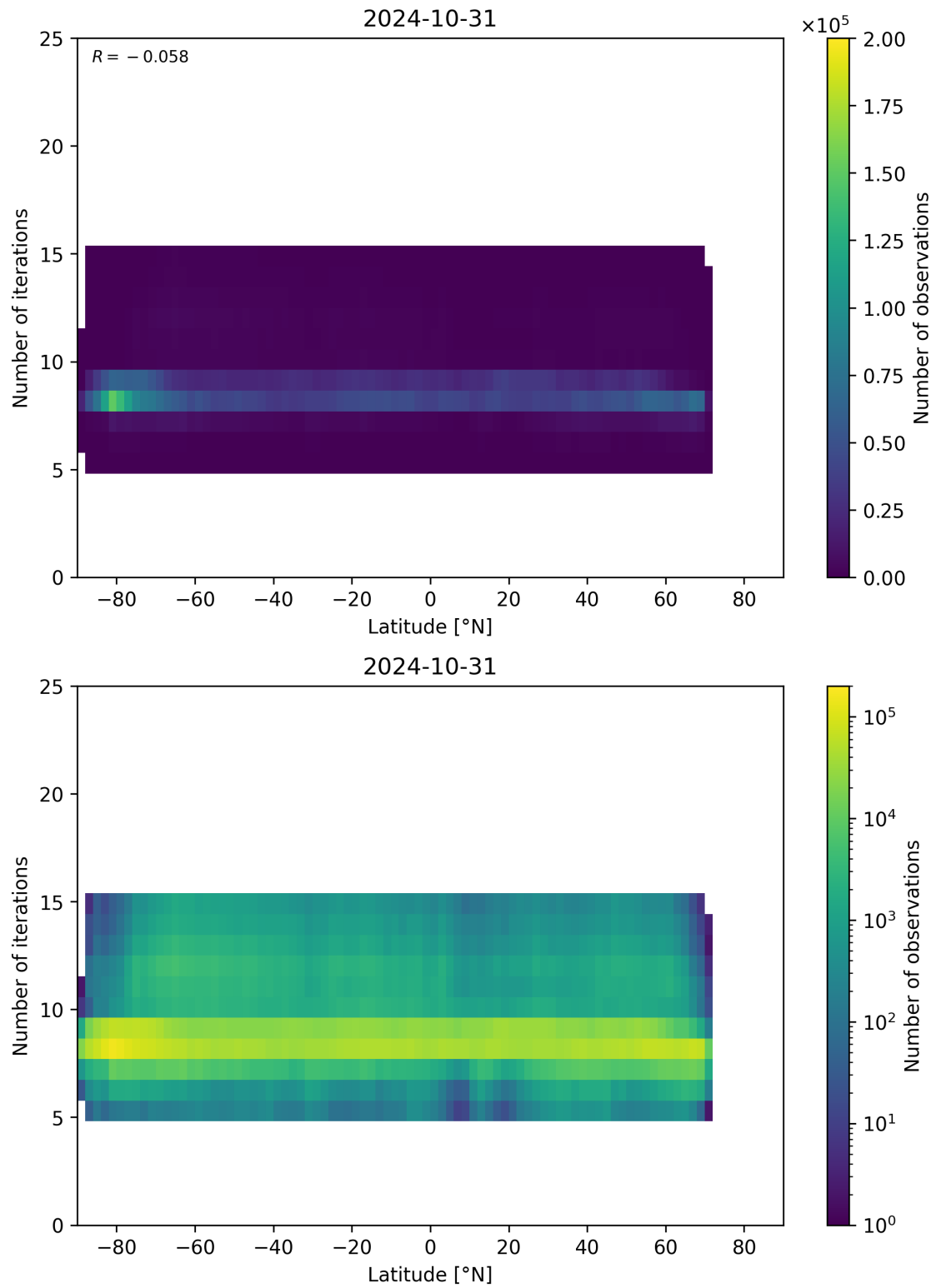
Figure 56: Scatter density plot of “Latitude” against “Number of iterations” for 2024-10-30 to 2024-11-01.
