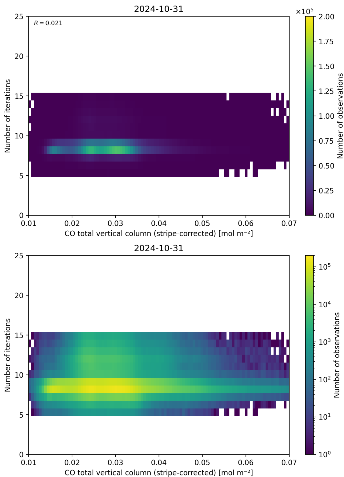
Figure 39: Scatter density plot of “CO total vertical column (stripe-corrected)” against “Number of iterations” for 2024-10-30 to 2024-11-01.
