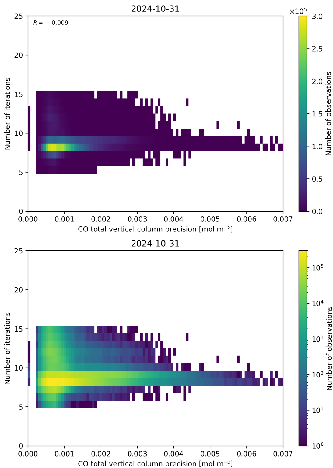
Figure 46: Scatter density plot of “CO total vertical column precision” against “Number of iterations” for 2024-10-30 to 2024-11-01.
