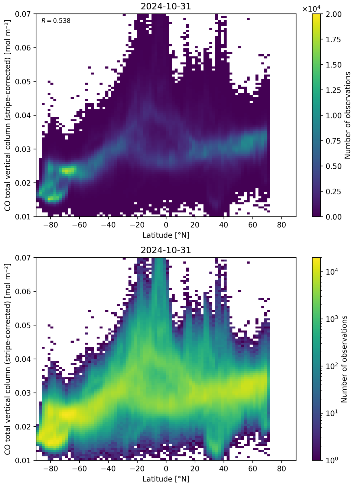
Figure 52: Scatter density plot of “Latitude” against “CO total vertical column (stripe-corrected)” for 2024-10-30 to 2024-11-01.
