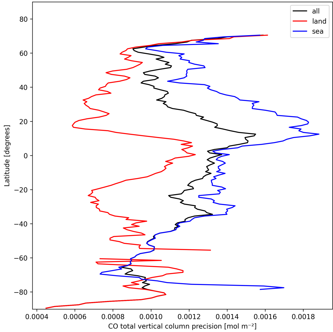
Figure 12: Zonal average of “CO total vertical column precision” for 2024-10-30 to 2024-11-01.
