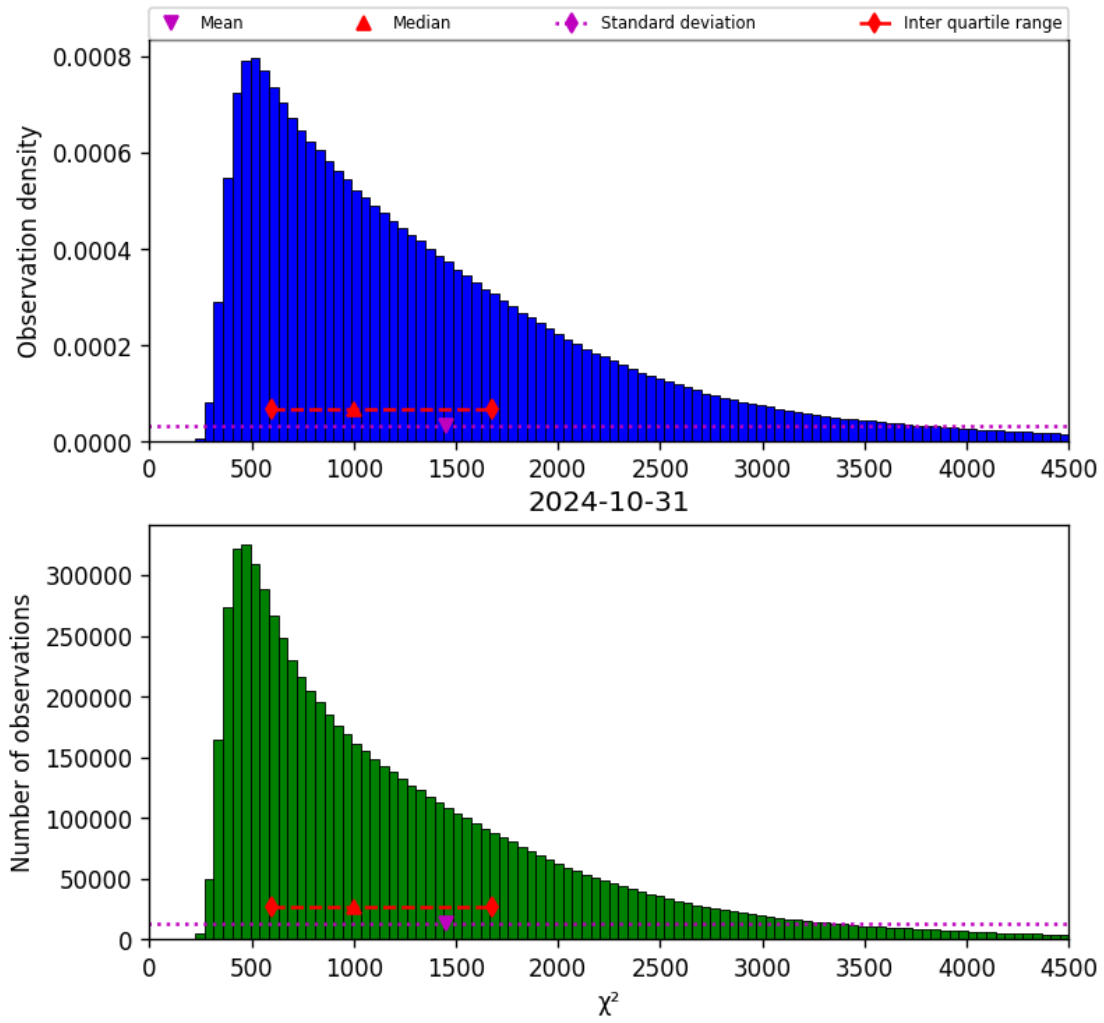
Figure 22: Histogram of “ \chi^2 ” for 2024-10-30 to 2024-11-01
