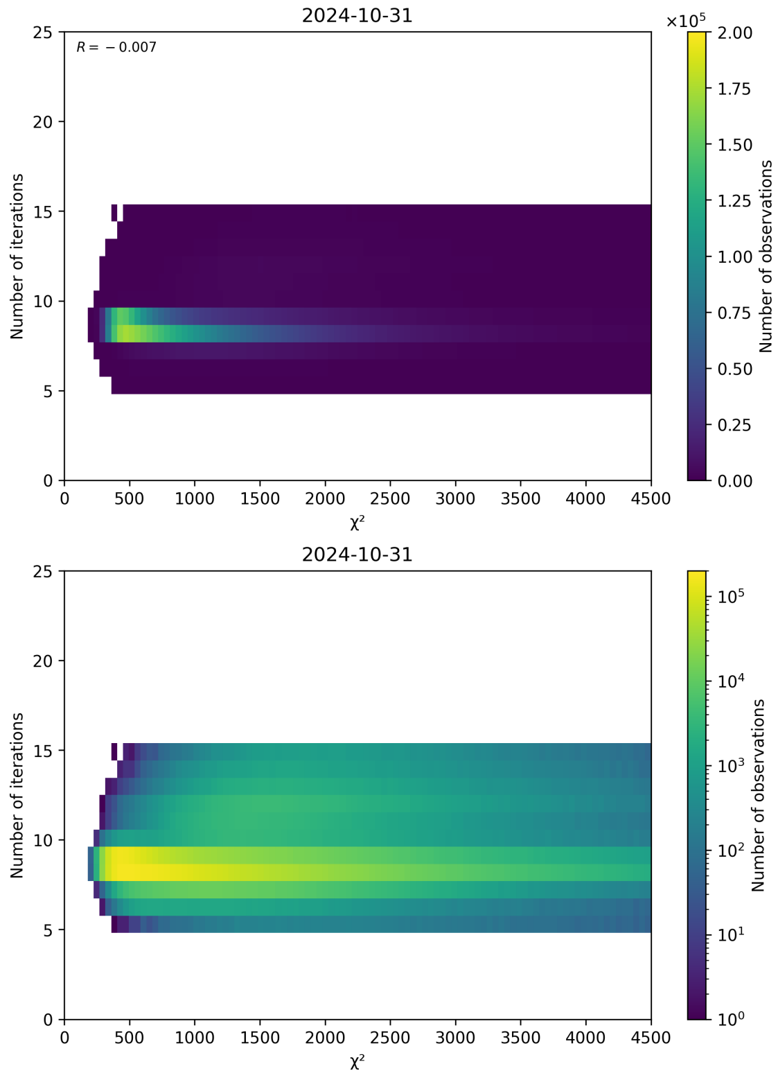
Figure 49: Scatter density plot of “ \chi^2 ” against “Number of iterations” for 2024-10-30 to 2024-11-01.
