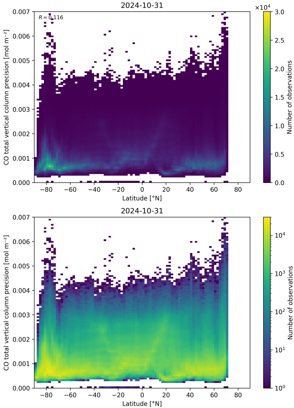
Figure 53: Scatter density plot of “Latitude” against “CO total vertical column precision” for 2024-10-30 to 2024-11-01.
