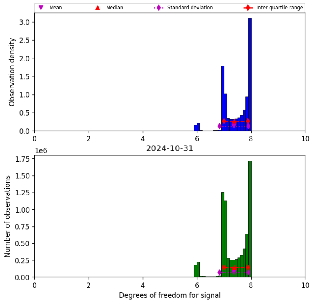
Figure 23: Histogram of “Degrees of freedom for signal” for 2024-10-30 to 2024-11-01
