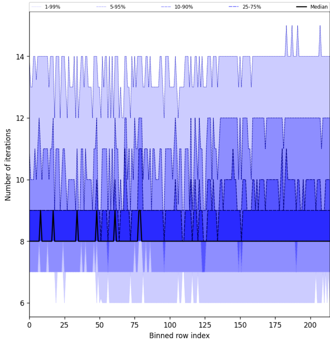
Figure 32: Along track statistics of “Number of iterations” for 2024-10-30 to 2024-11-01
