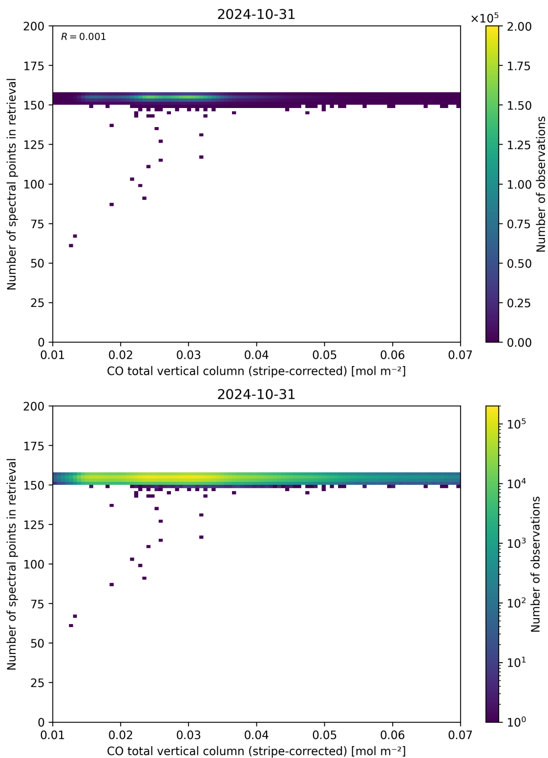
Figure 40: Scatter density plot of “CO total vertical column (stripe-corrected)” against “Number of spectral points in retrieval” for 2024-10-30 to 2024-11-01.
