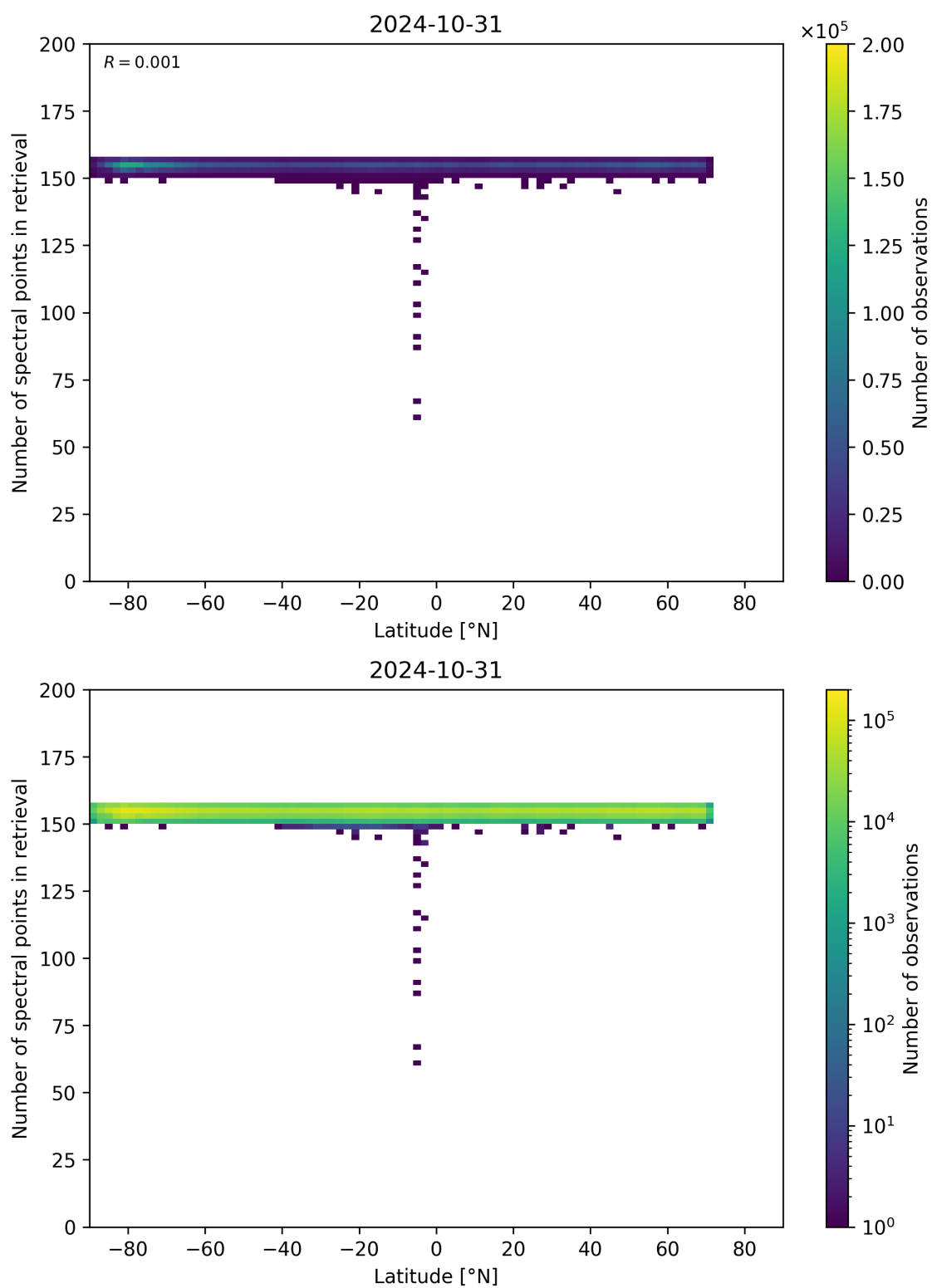
Figure 57: Scatter density plot of “Latitude” against “Number of spectral points in retrieval” for 2024-10-30 to 2024-11-01.
