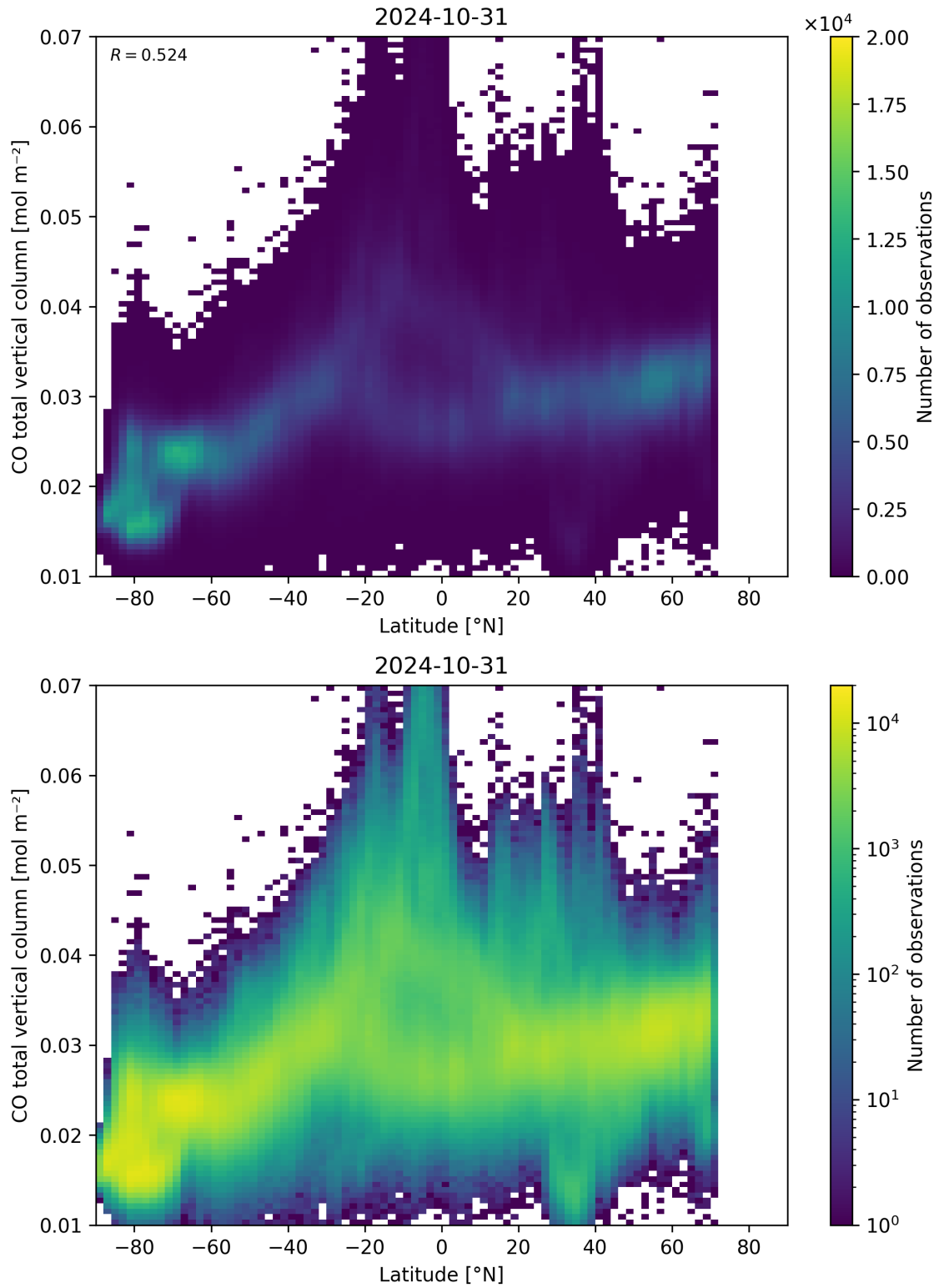
Figure 51: Scatter density plot of “Latitude” against “CO total vertical column” for 2024-10-30 to 2024-11-01.
