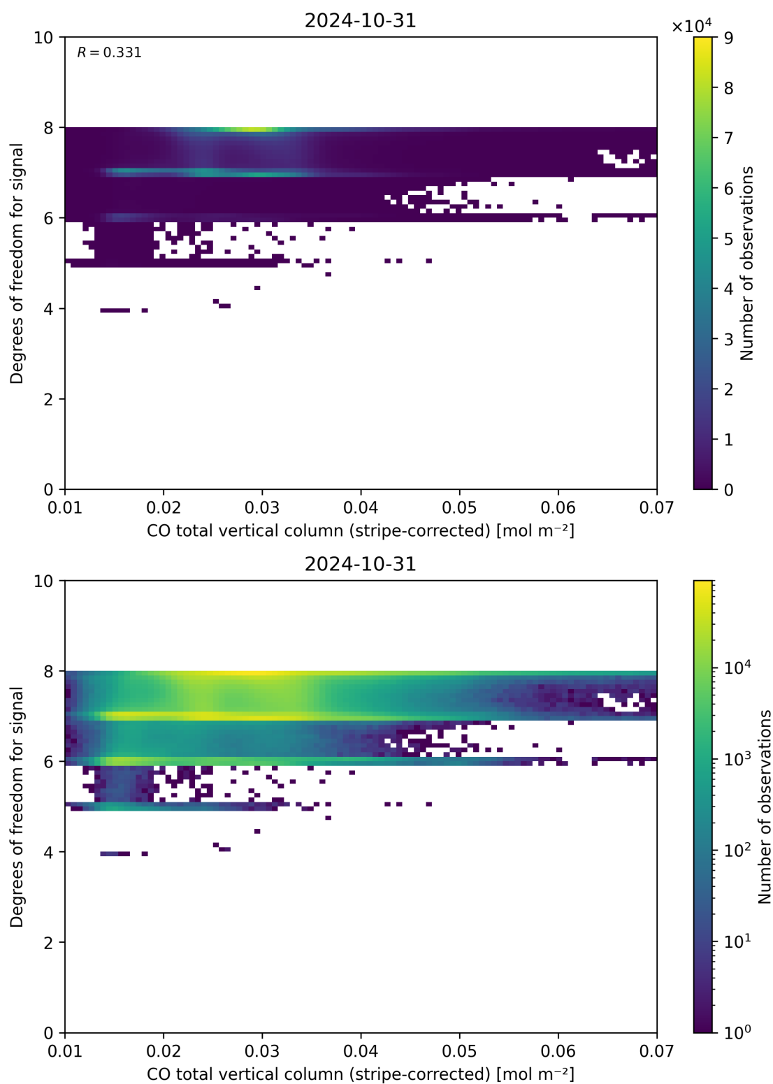
Figure 38: Scatter density plot of “CO total vertical column (stripe-corrected)” against “Degrees of freedom for signal” for 2024-10-30 to 2024-11-01.
