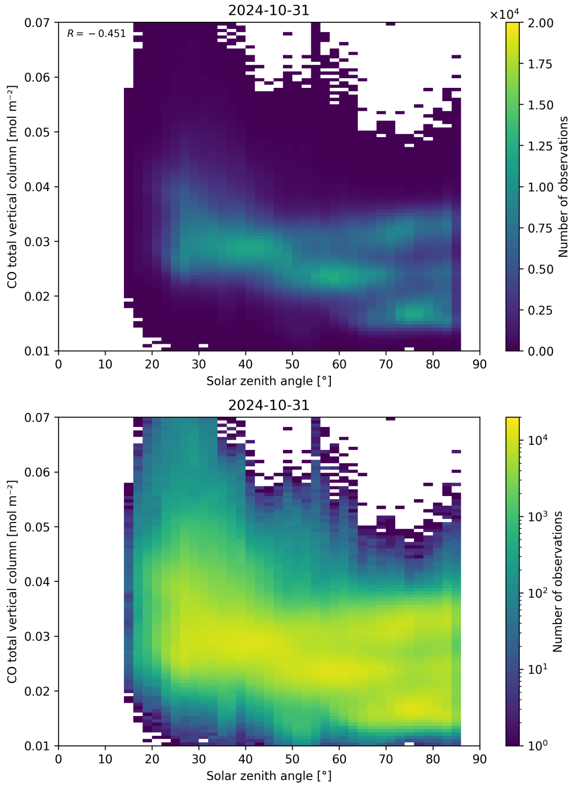
Figure 61: Scatter density plot of “Solar zenith angle” against “CO total vertical column” for 2024-10-30 to 2024-11-01.
