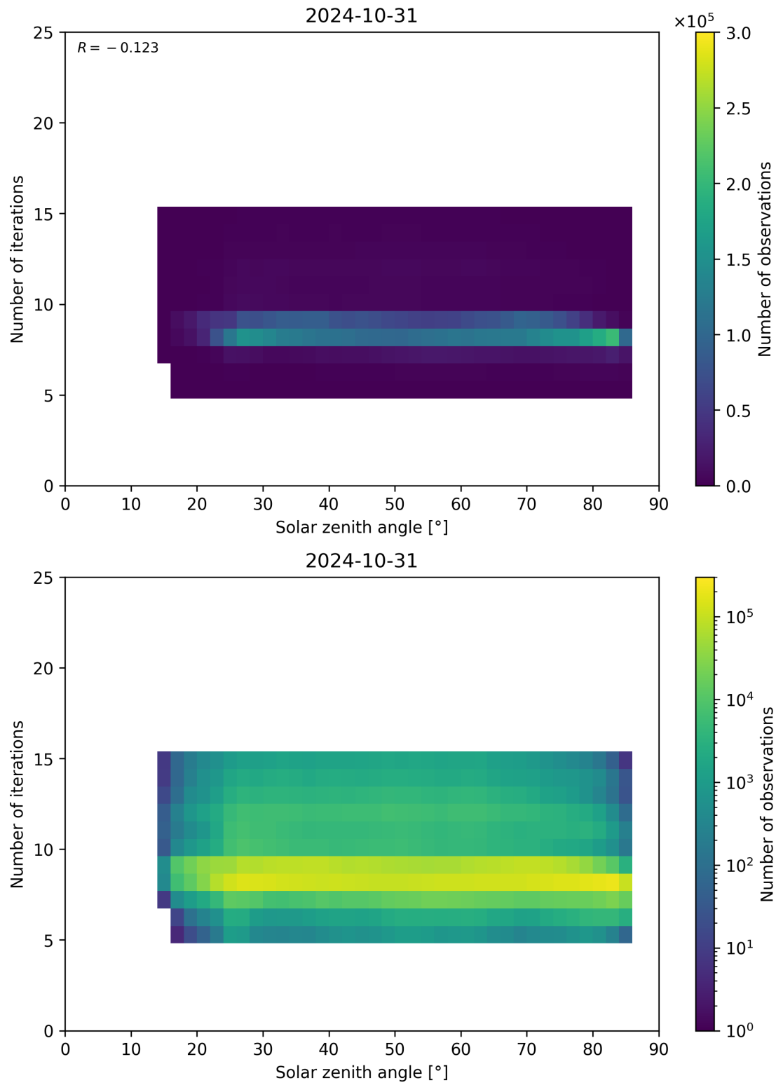
Figure 67: Scatter density plot of “Solar zenith angle” against “Number of iterations” for 2024-10-30 to 2024-11-01.
