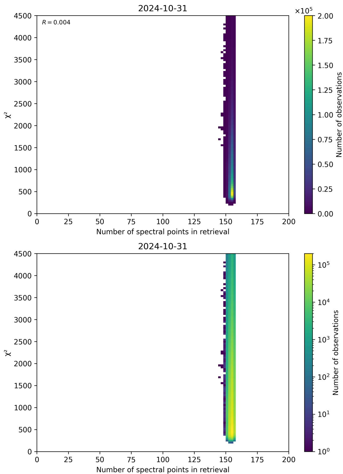
Figure 58: Scatter density plot of “Number of spectral points in retrieval” against “ \chi^2 ” for 2024-10-30 to 2024-11-01.
