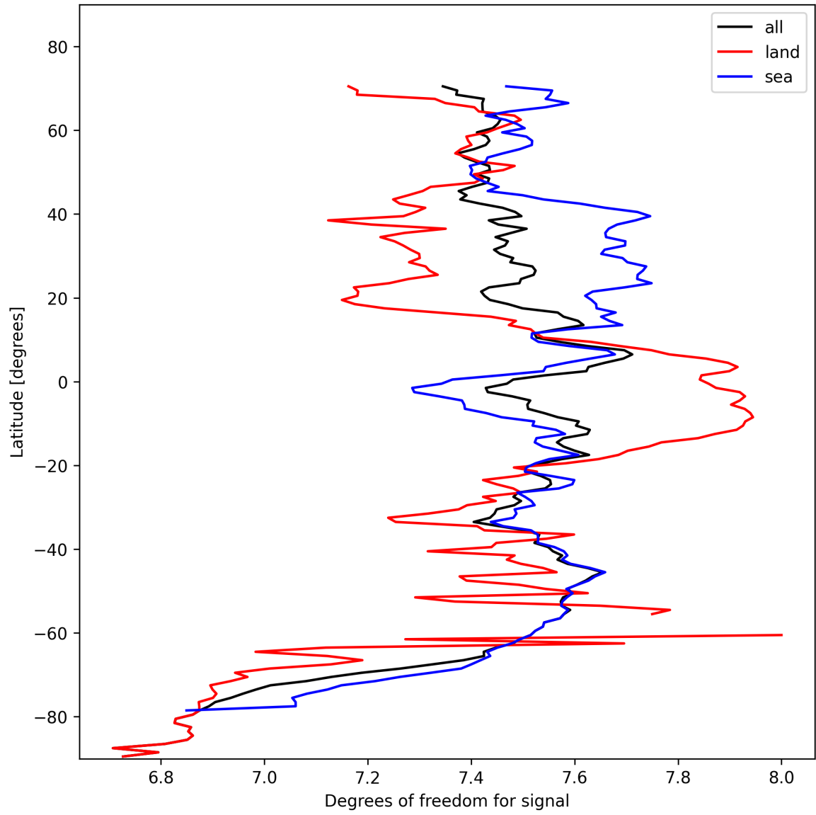
Figure 15: Zonal average of “Degrees of freedom for signal” for 2024-10-30 to 2024-11-01.
