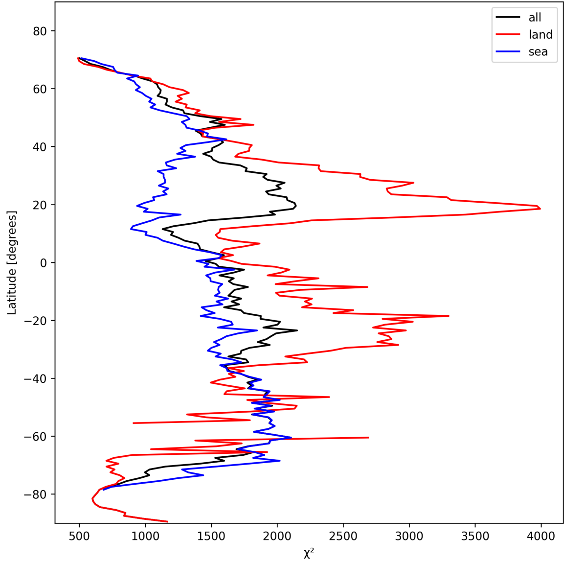
Figure 14: Zonal average of “ \chi^2 ” for 2024-10-30 to 2024-11-01.
