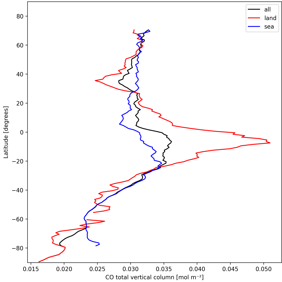
Figure 10: Zonal average of “CO total vertical column” for 2024-10-30 to 2024-11-01.
