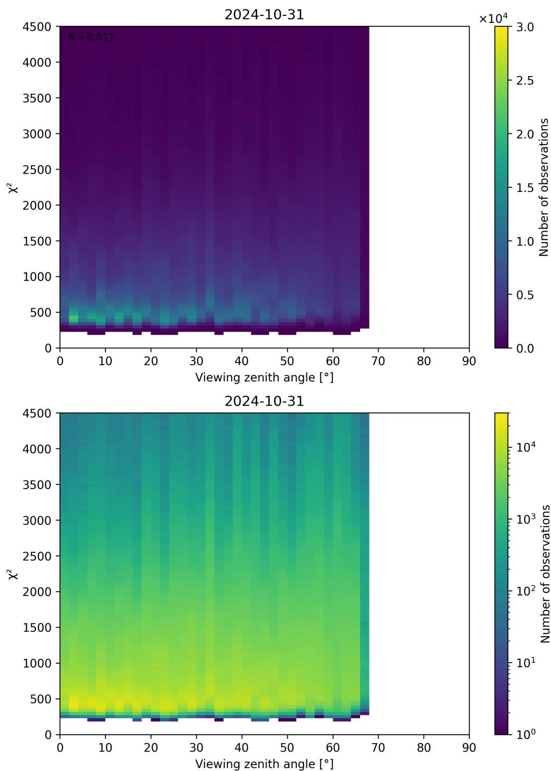
Figure 72: Scatter density plot of “Viewing zenith angle” against “ \chi^2 ” for 2024-10-30 to 2024-11-01.
