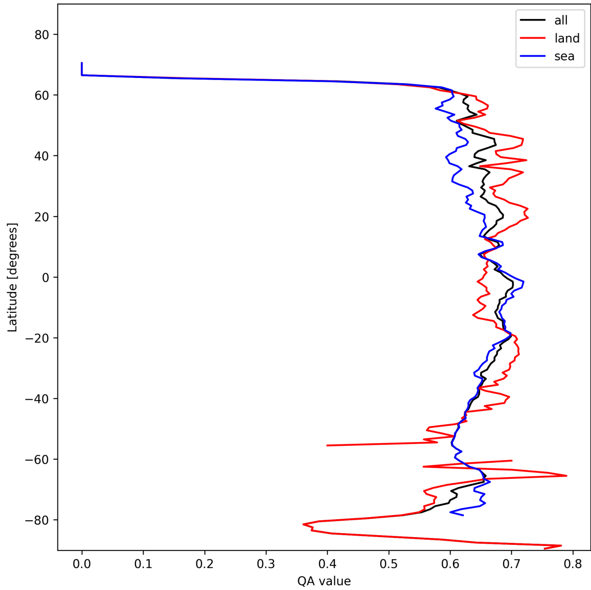
Figure 9: Zonal average of “QA value” for 2024-10-30 to 2024-11-01.
