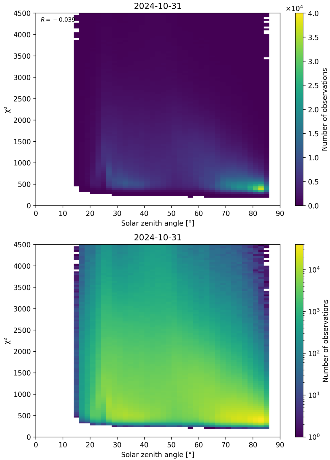
Figure 64: Scatter density plot of “Solar zenith angle” against “ \chi^2 ” for 2024-10-30 to 2024-11-01.
