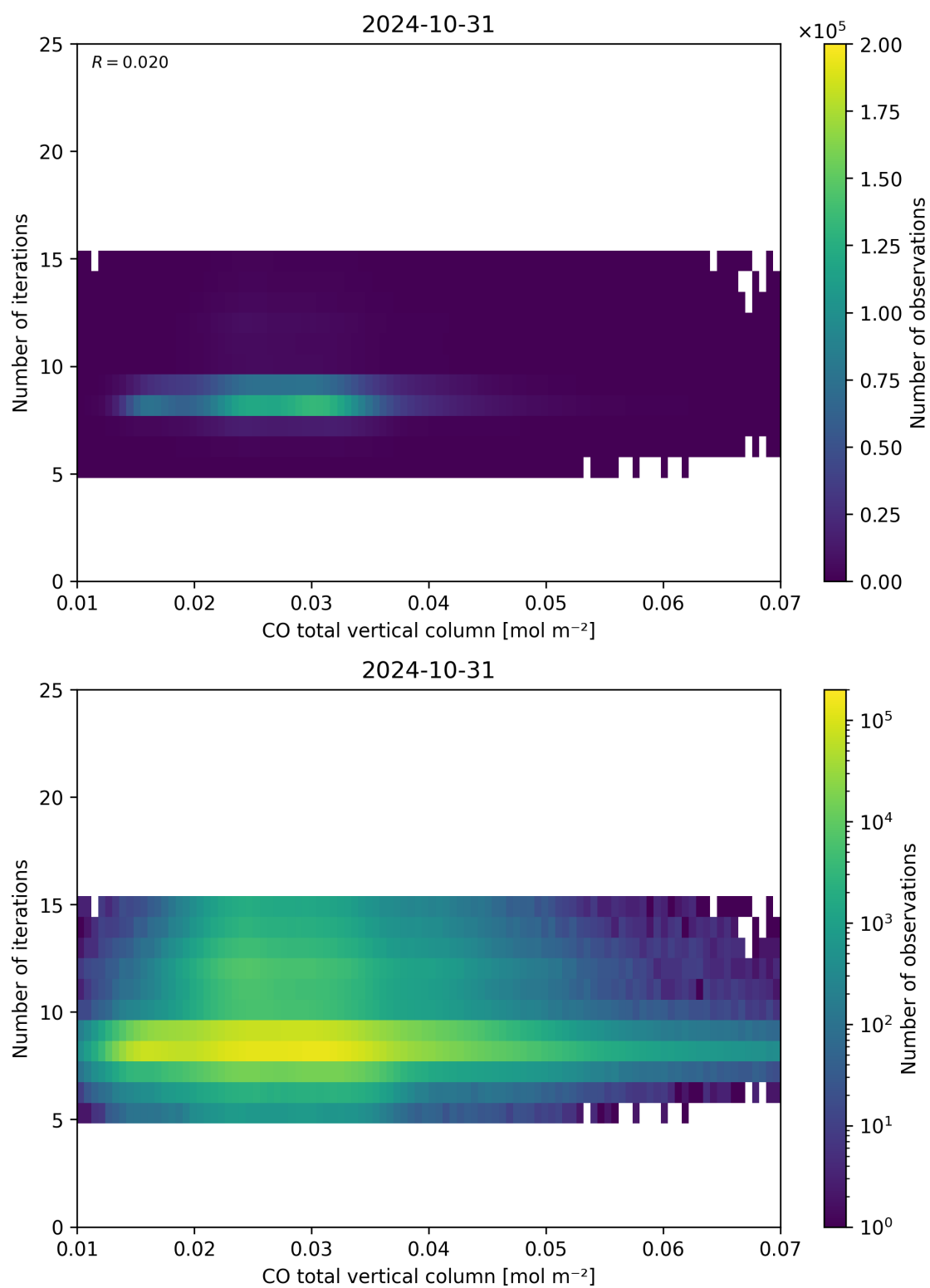
Figure 42: Scatter density plot of “CO total vertical column” against “Number of iterations” for 2024-10-30 to 2024-11-01.
