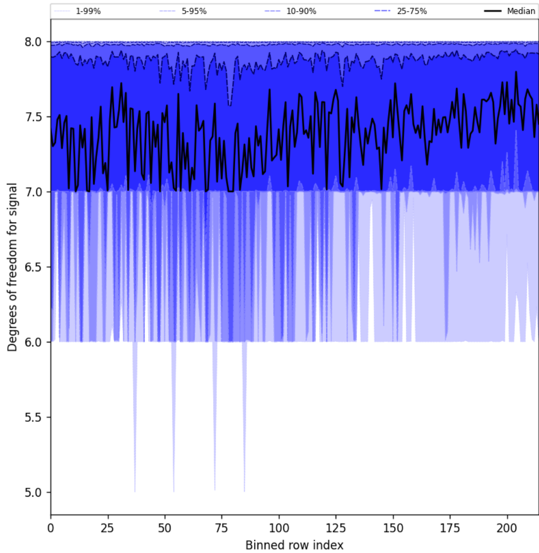
Figure 31: Along track statistics of “Degrees of freedom for signal” for 2024-10-30 to 2024-11-01
