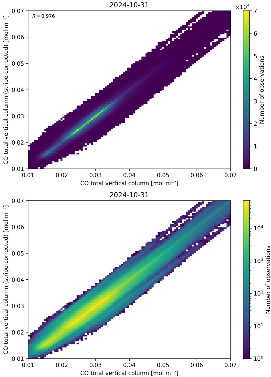
Figure 33: Scatter density plot of “CO total vertical column” against “CO total vertical column (stripe-corrected)” for 2024-10-30 to 2024-11-01.
