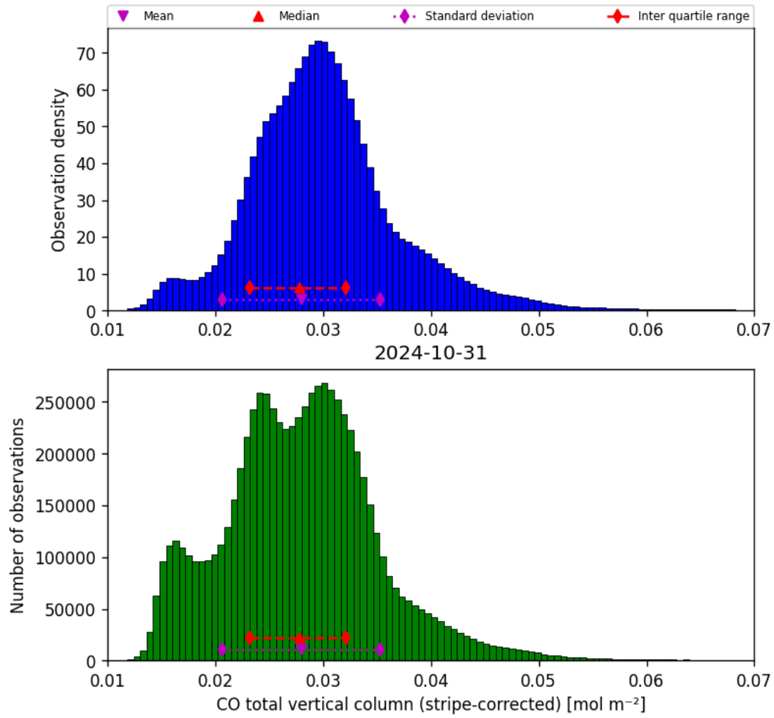
Figure 19: Histogram of “CO total vertical column (stripe-corrected)” for 2024-10-30 to 2024-11-01
