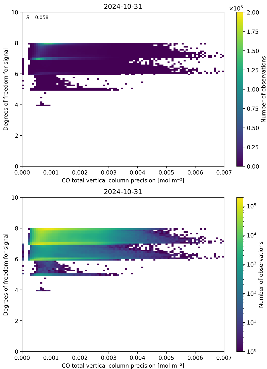
Figure 45: Scatter density plot of “CO total vertical column precision” against “Degrees of freedom for signal” for 2024-10-30 to 2024-11-01.
