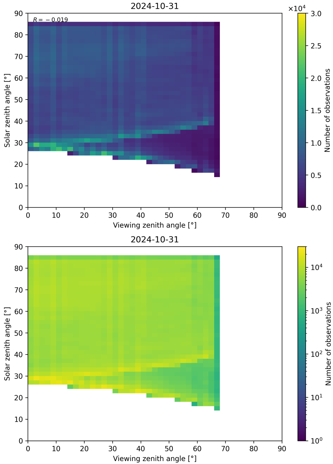
Figure 77: Scatter density plot of “Viewing zenith angle” against “Solar zenith angle” for 2024-10-30 to 2024-11-01.
