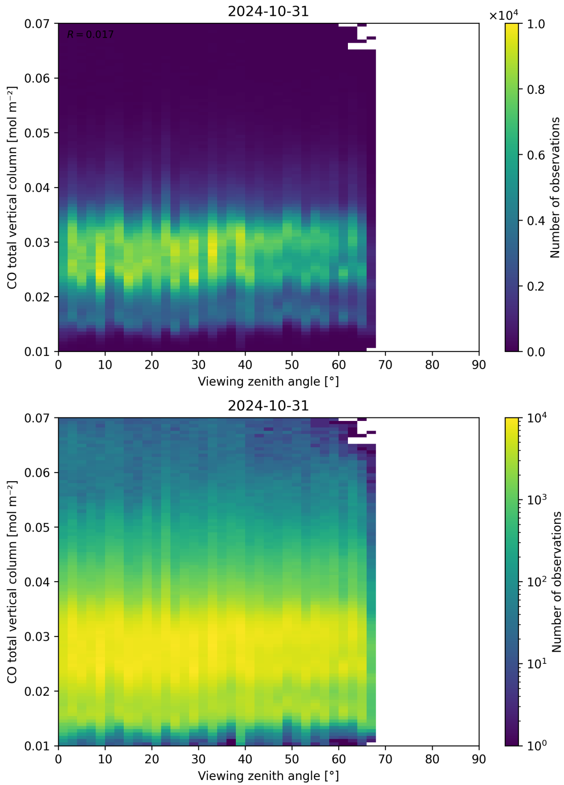
Figure 69: Scatter density plot of “Viewing zenith angle” against “CO total vertical column” for 2024-10-30 to 2024-11-01.
