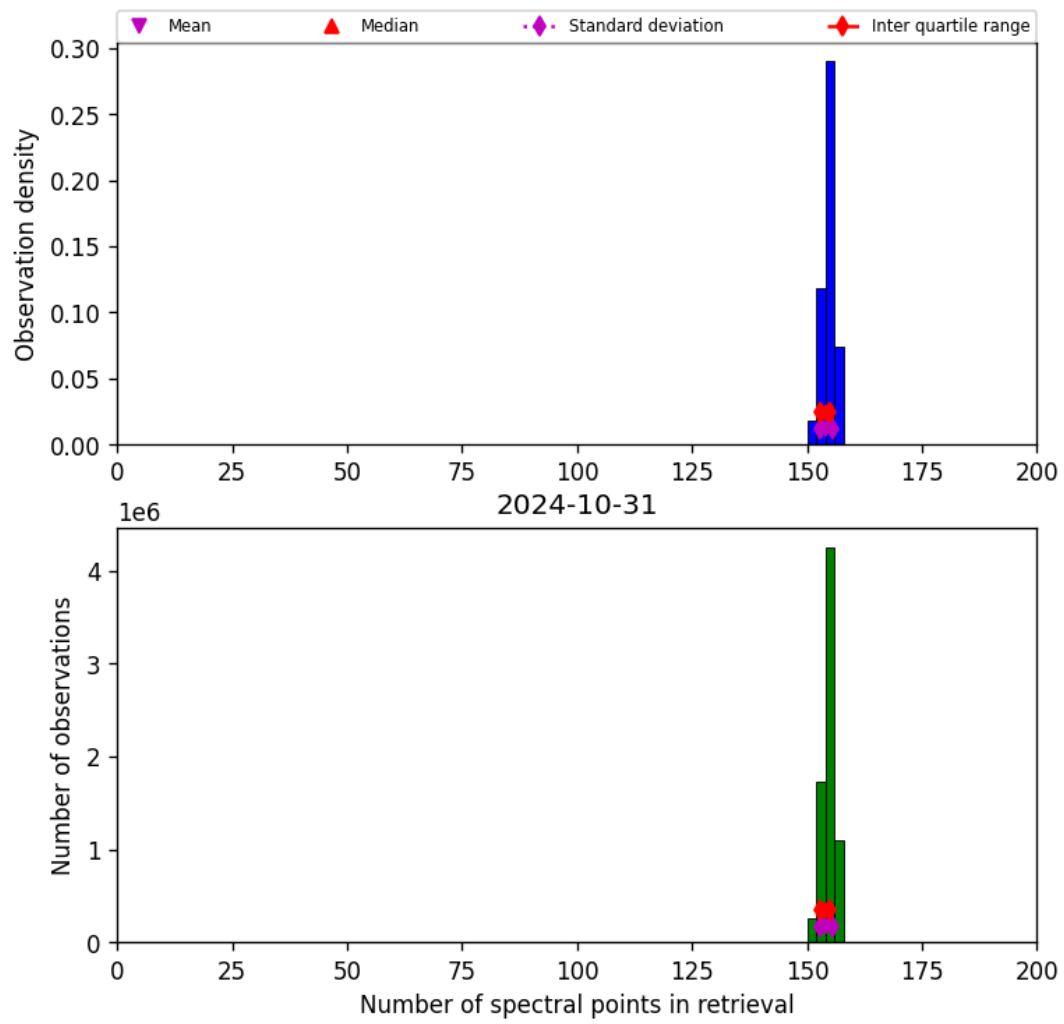
Figure 21: Histogram of “Number of spectral points in retrieval” for 2024-10-30 to 2024-11-01
