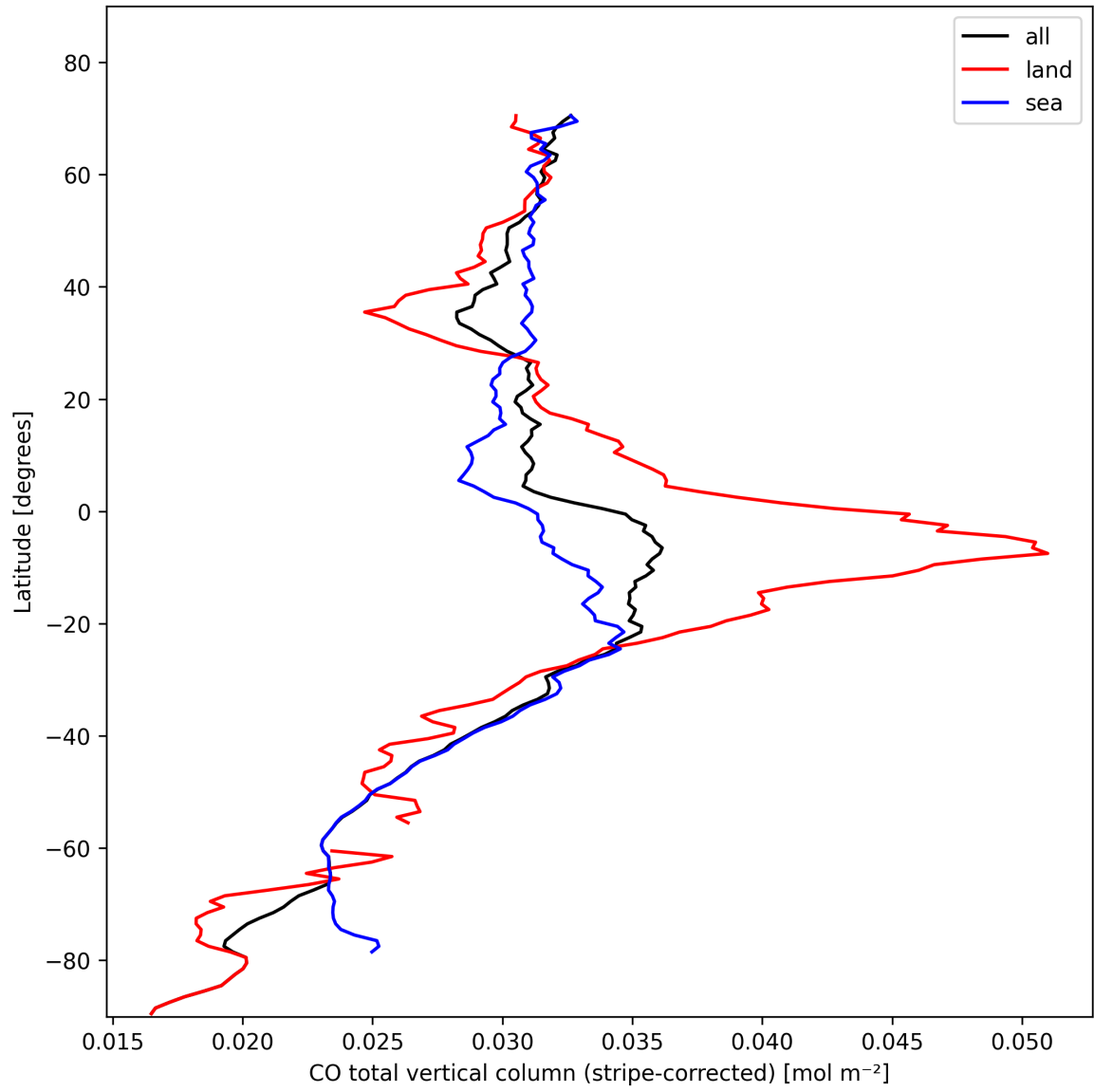
Figure 11: Zonal average of “CO total vertical column (stripe-corrected)” for 2024-10-30 to 2024-11-01.
