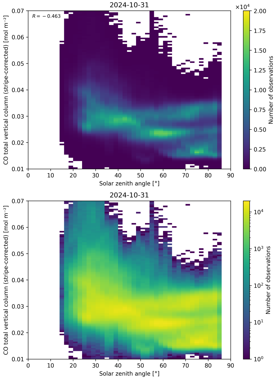
Figure 62: Scatter density plot of “Solar zenith angle” against “CO total vertical column (stripe-corrected)” for 2024-10-30 to 2024-11-01.
