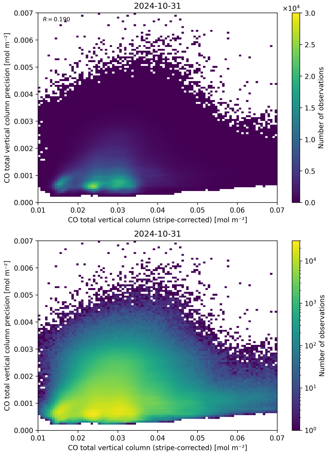
Figure 36: Scatter density plot of “CO total vertical column (stripe-corrected)” against “CO total vertical column precision” for 2024-10-30 to 2024-11-01.
