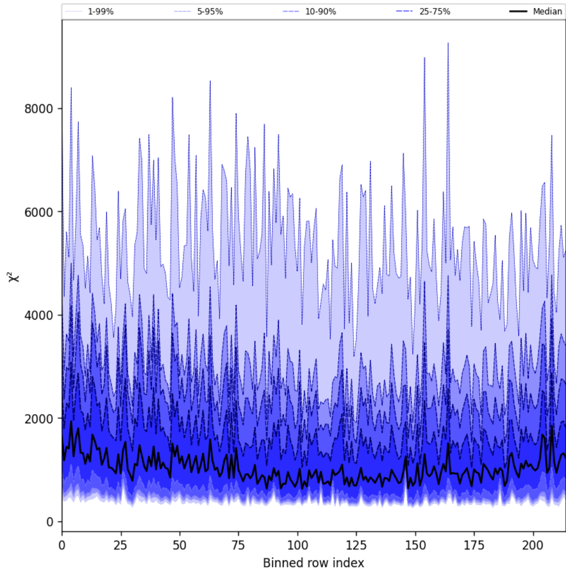
Figure 30: Along track statistics of “ \chi^2 ” for 2024-10-30 to 2024-11-01
