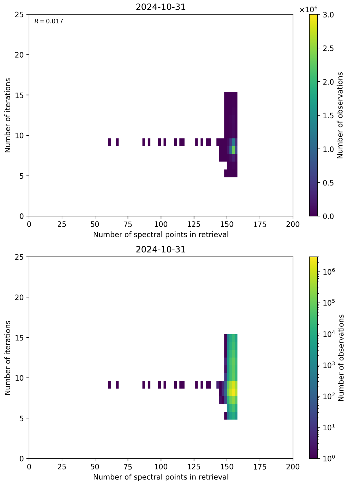
Figure 60: Scatter density plot of “Number of spectral points in retrieval” against “Number of iterations” for 2024-10-30 to 2024-11-01.
