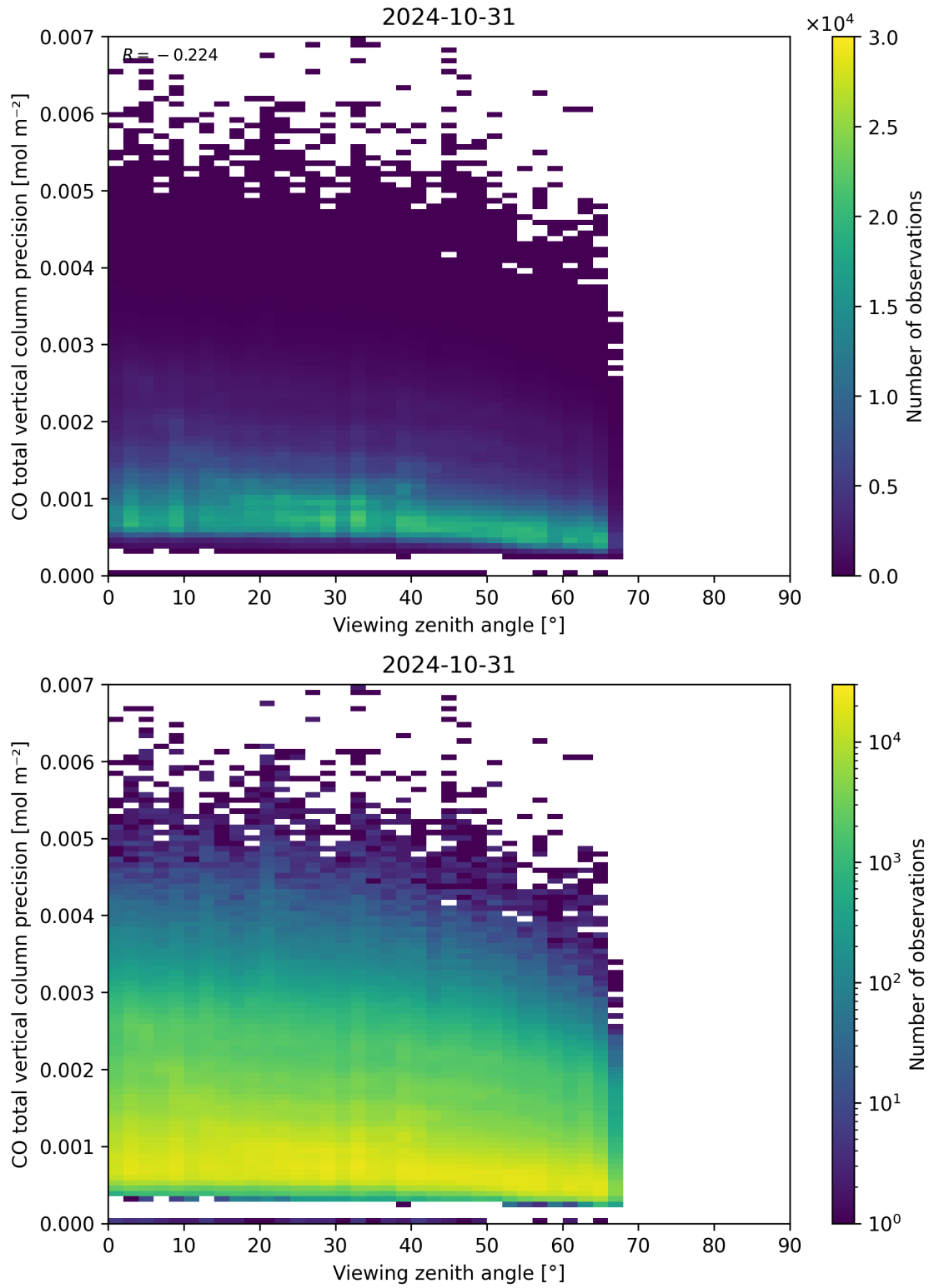
Figure 71: Scatter density plot of “Viewing zenith angle” against “CO total vertical column precision” for 2024-10-30 to 2024-11-01.
