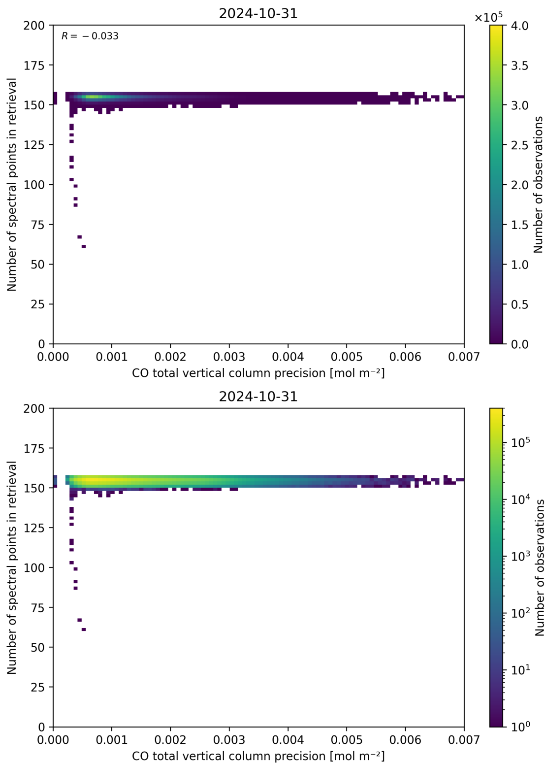
Figure 47: Scatter density plot of “CO total vertical column precision” against “Number of spectral points in retrieval” for 2024-10-30 to 2024-11-01.
