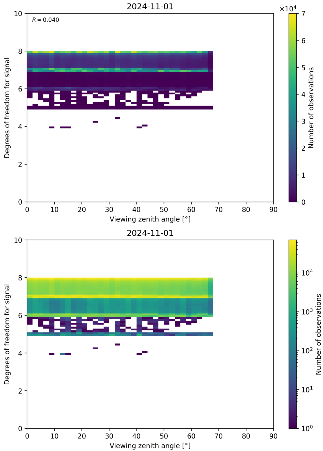
Figure 73: Scatter density plot of “Viewing zenith angle” against “Degrees of freedom for signal” for 2024-10-31 to 2024-11-02.
