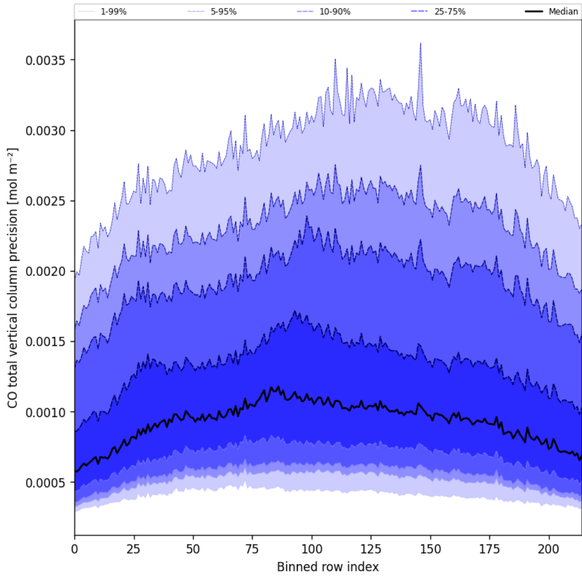
Figure 28: Along track statistics of “CO total vertical column precision” for 2024-10-31 to 2024-11-02
