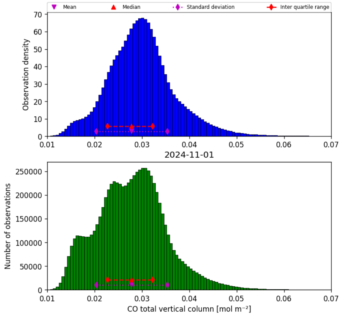
Figure 18: Histogram of “CO total vertical column” for 2024-10-31 to 2024-11-02
