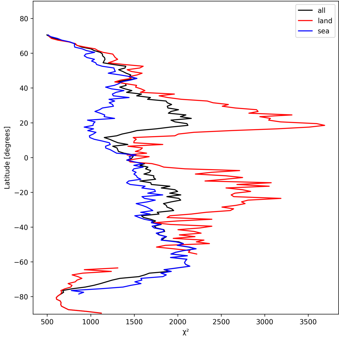
Figure 14: Zonal average of “ \chi^2 ” for 2024-10-31 to 2024-11-02.
