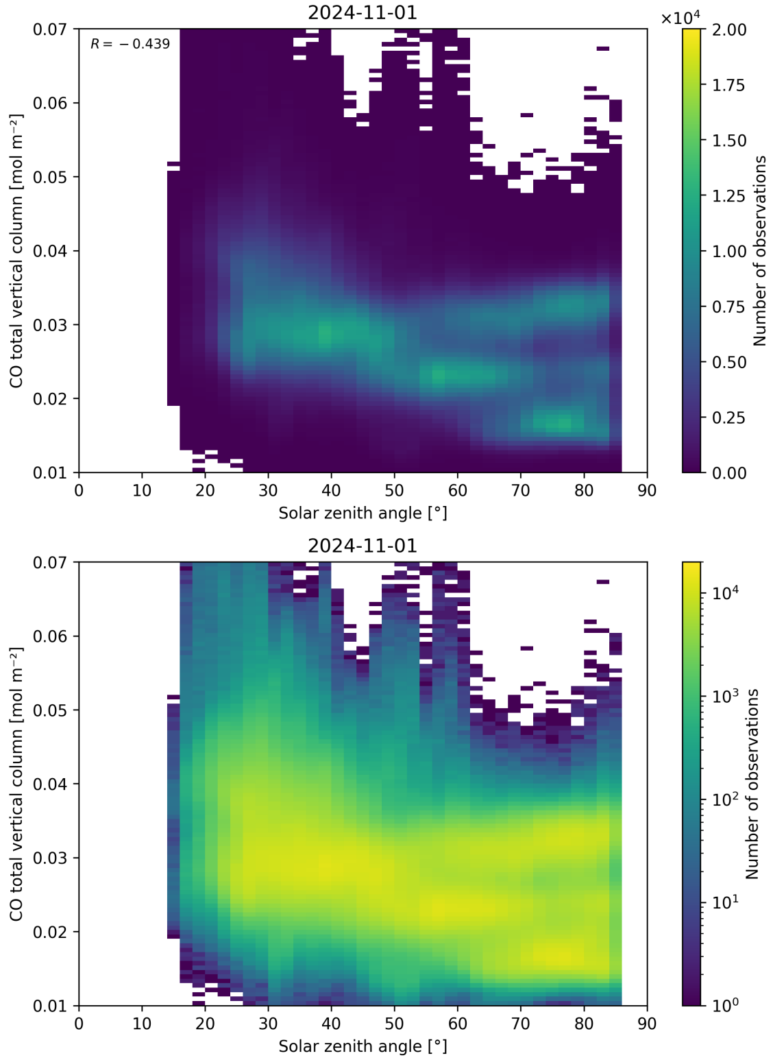
Figure 61: Scatter density plot of “Solar zenith angle” against “CO total vertical column” for 2024-10-31 to 2024-11-02.
