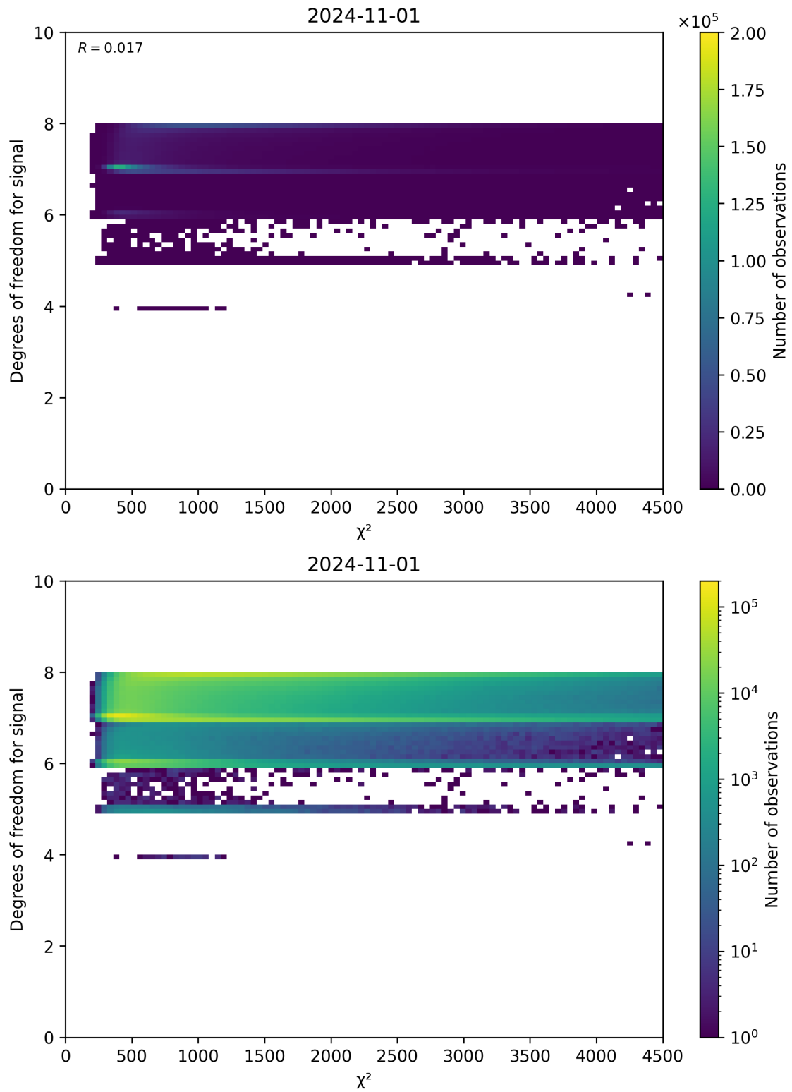
Figure 48: Scatter density plot of “ \chi^2 ” against “Degrees of freedom for signal” for 2024-10-31 to 2024-11-02.
