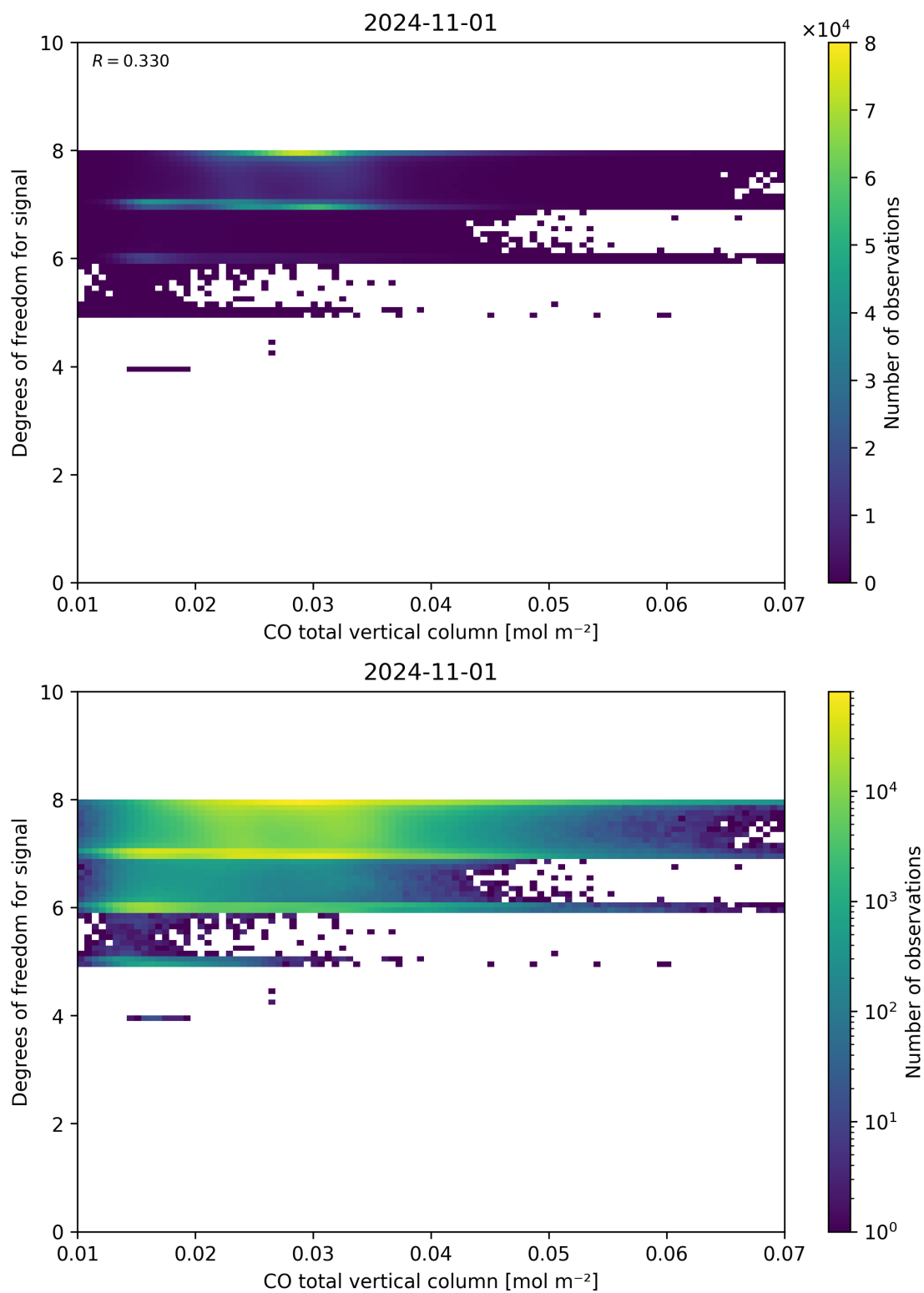
Figure 41: Scatter density plot of “CO total vertical column” against “Degrees of freedom for signal” for 2024-10-31 to 2024-11-02.
