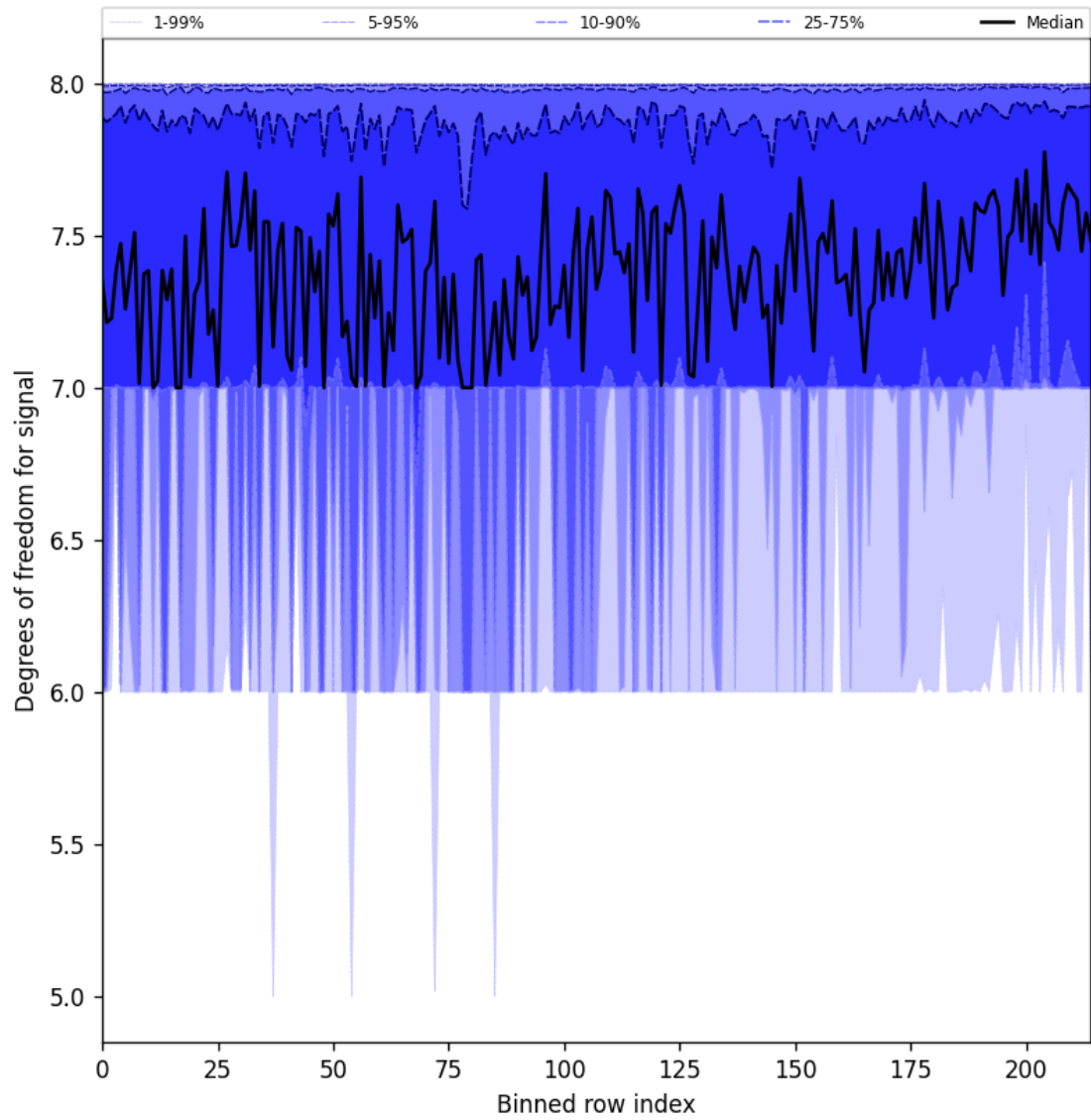
Figure 31: Along track statistics of “Degrees of freedom for signal” for 2024-10-31 to 2024-11-02
