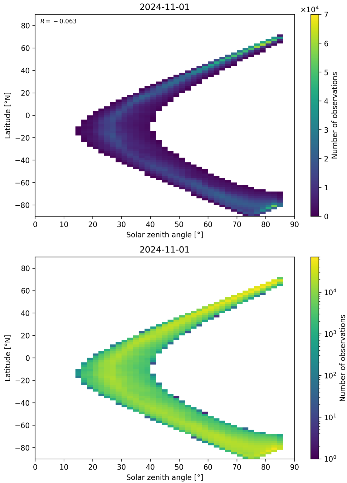
Figure 66: Scatter density plot of “Solar zenith angle” against “Latitude” for 2024-10-31 to 2024-11-02.
