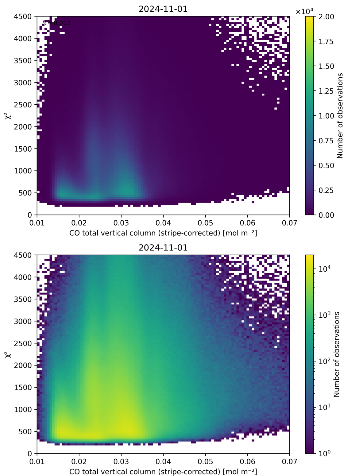
Figure 37: Scatter density plot of “CO total vertical column (stripe-corrected)” against “ \chi^2 ” for 2024-10-31 to 2024-11-02.
