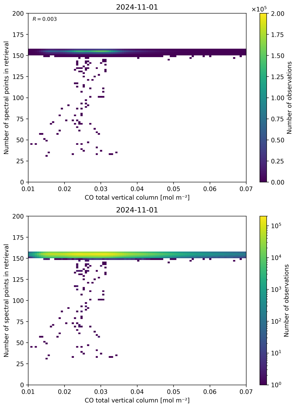
Figure 43: Scatter density plot of “CO total vertical column” against “Number of spectral points in retrieval” for 2024-10-31 to 2024-11-02.
