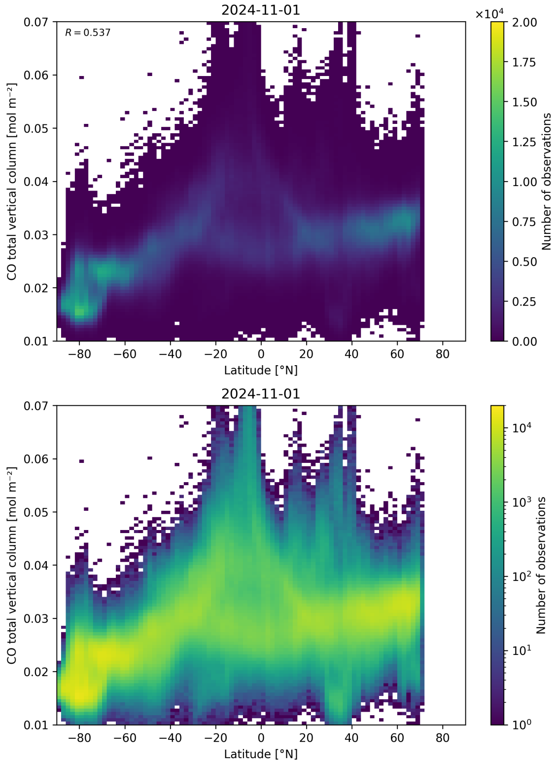
Figure 51: Scatter density plot of “Latitude” against “CO total vertical column” for 2024-10-31 to 2024-11-02.
