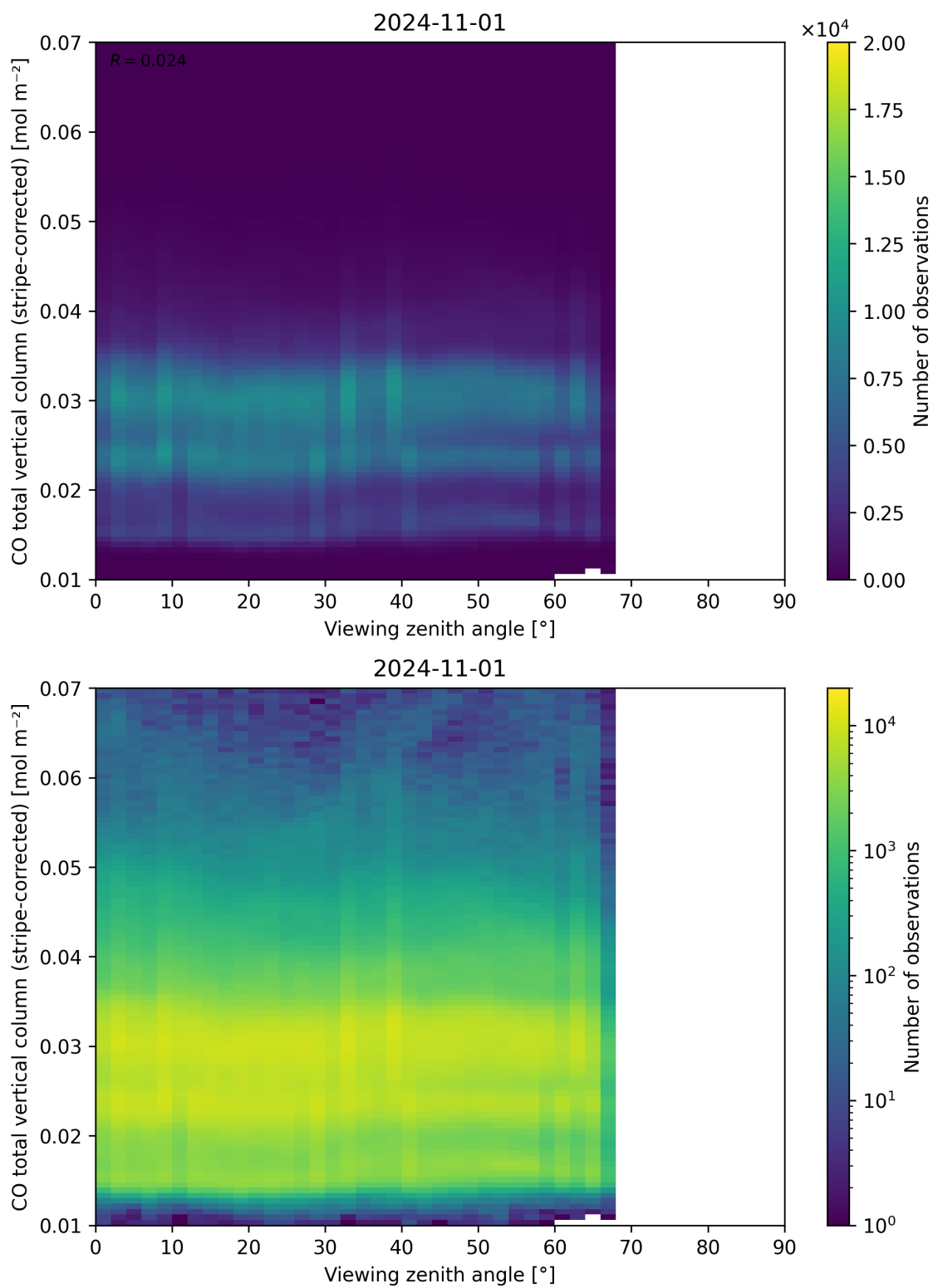
Figure 70: Scatter density plot of “Viewing zenith angle” against “CO total vertical column (stripe-corrected)” for 2024-10-31 to 2024-11-02.
