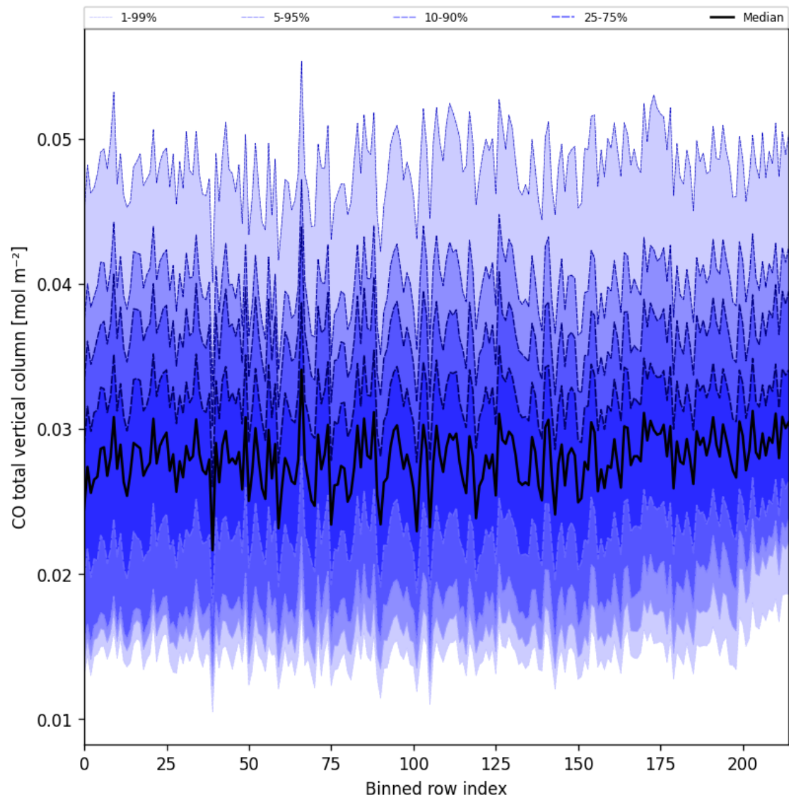
Figure 26: Along track statistics of “CO total vertical column” for 2024-10-31 to 2024-11-02
