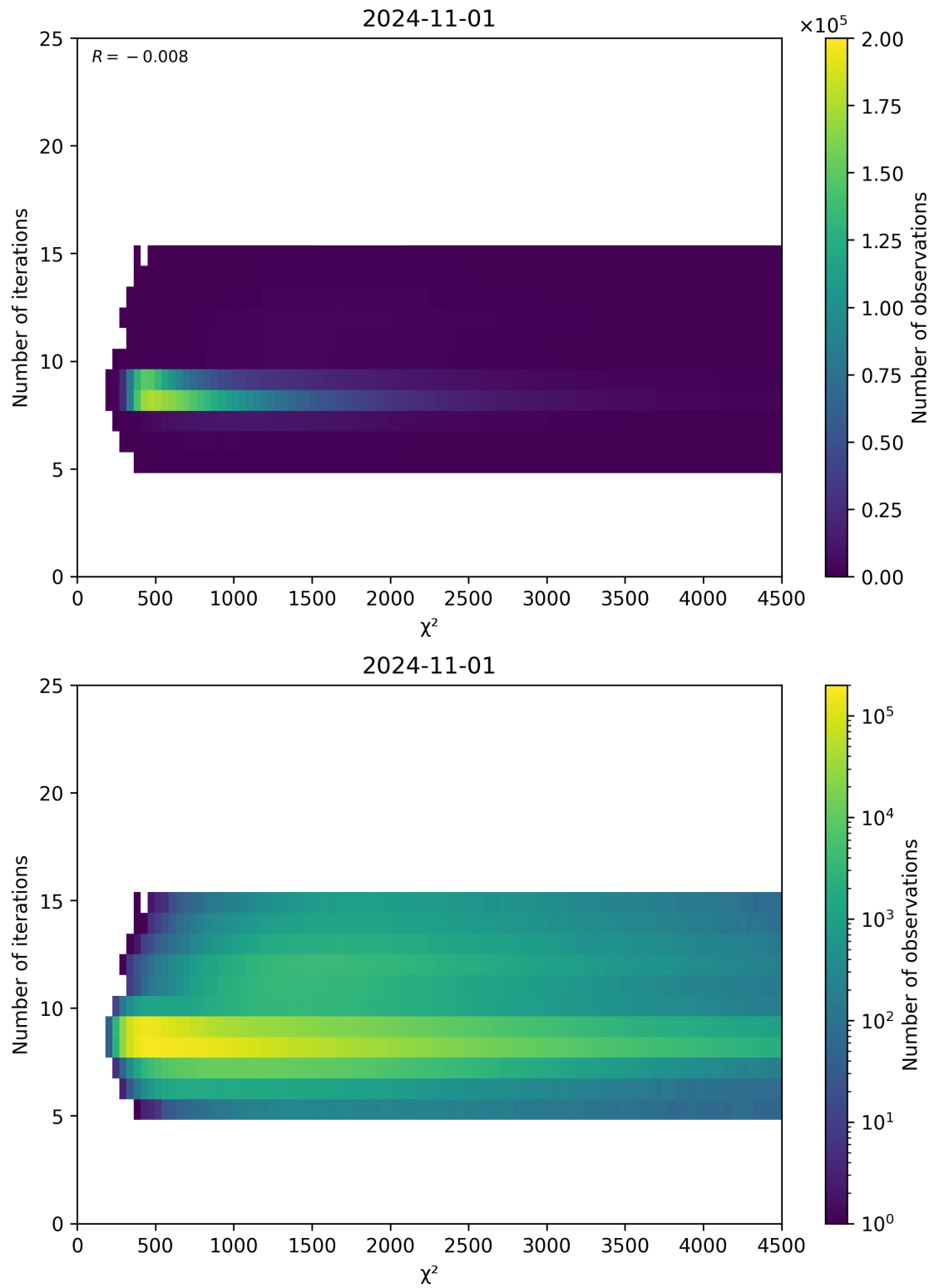
Figure 49: Scatter density plot of “ \chi^2 ” against “Number of iterations” for 2024-10-31 to 2024-11-02.
