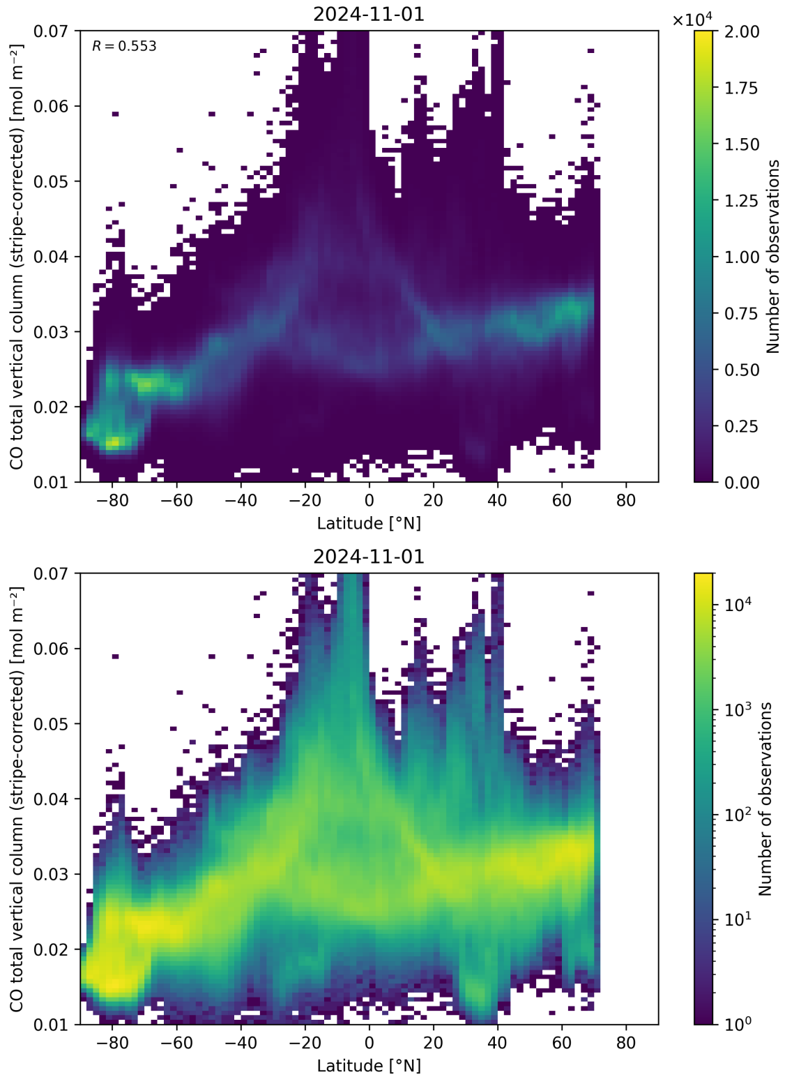
Figure 52: Scatter density plot of “Latitude” against “CO total vertical column (stripe-corrected)” for 2024-10-31 to 2024-11-02.
