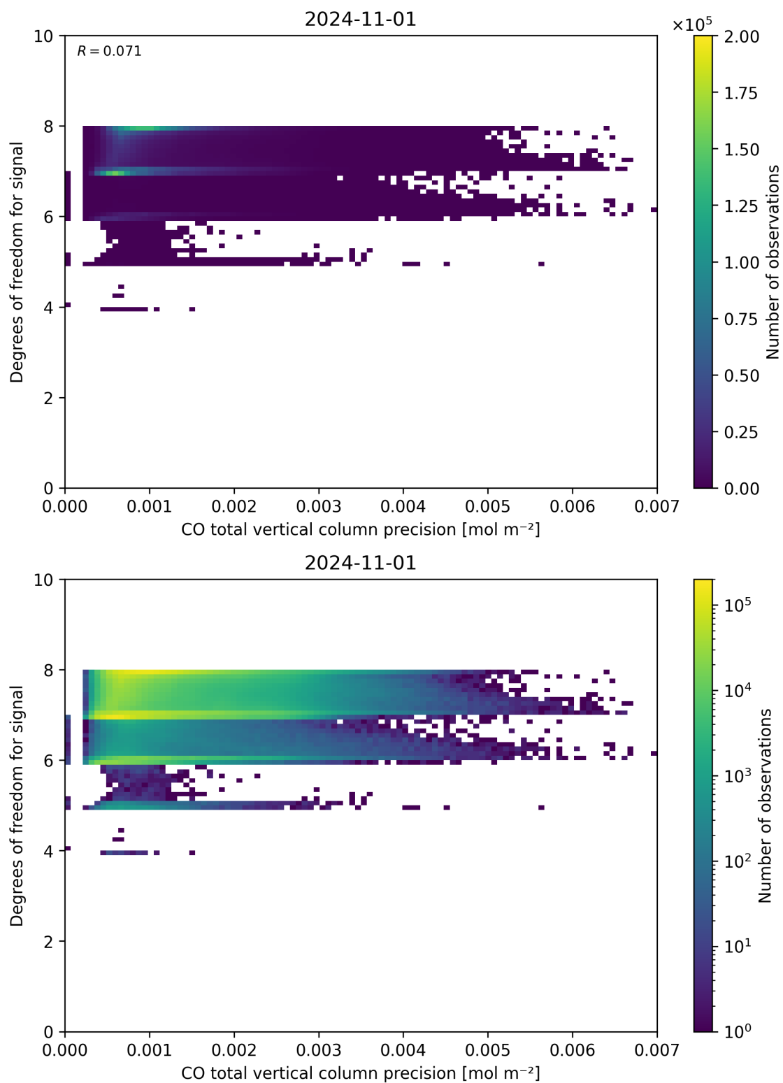
Figure 45: Scatter density plot of “CO total vertical column precision” against “Degrees of freedom for signal” for 2024-10-31 to 2024-11-02.
