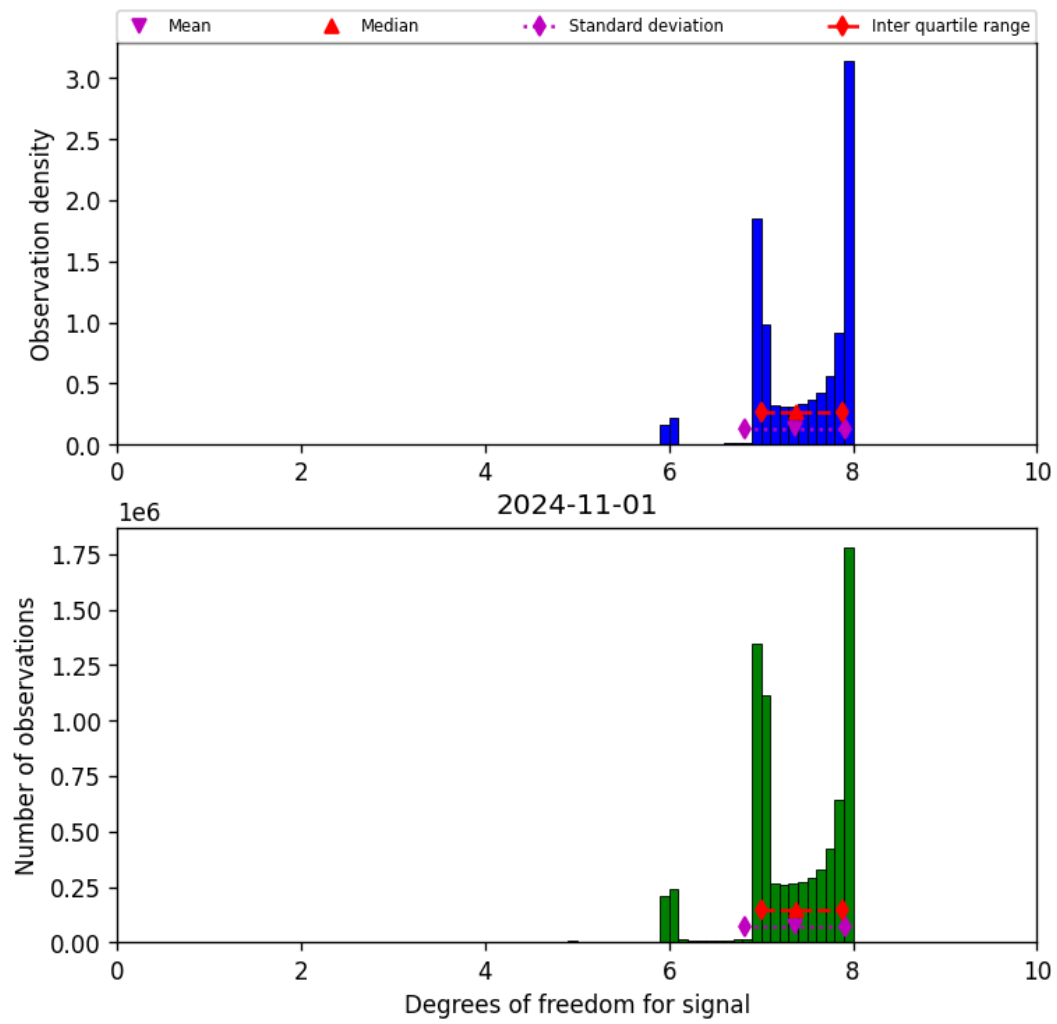
Figure 23: Histogram of “Degrees of freedom for signal” for 2024-10-31 to 2024-11-02
