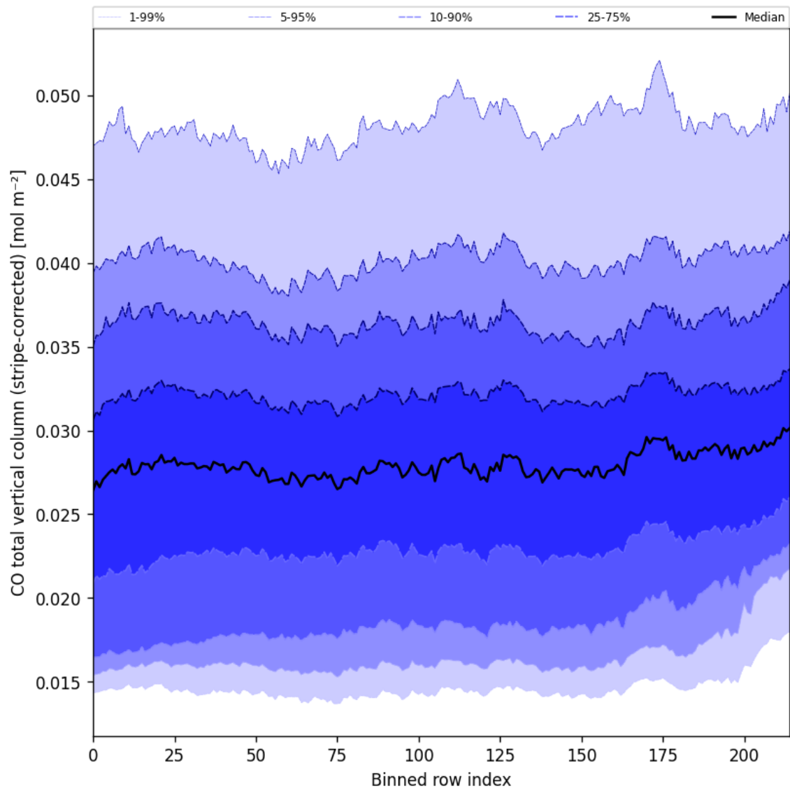
Figure 27: Along track statistics of “CO total vertical column (stripe-corrected)” for 2024-10-31 to 2024-11-02
