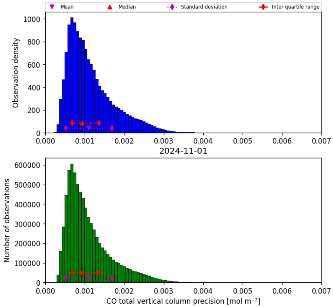
Figure 20: Histogram of “CO total vertical column precision” for 2024-10-31 to 2024-11-02
