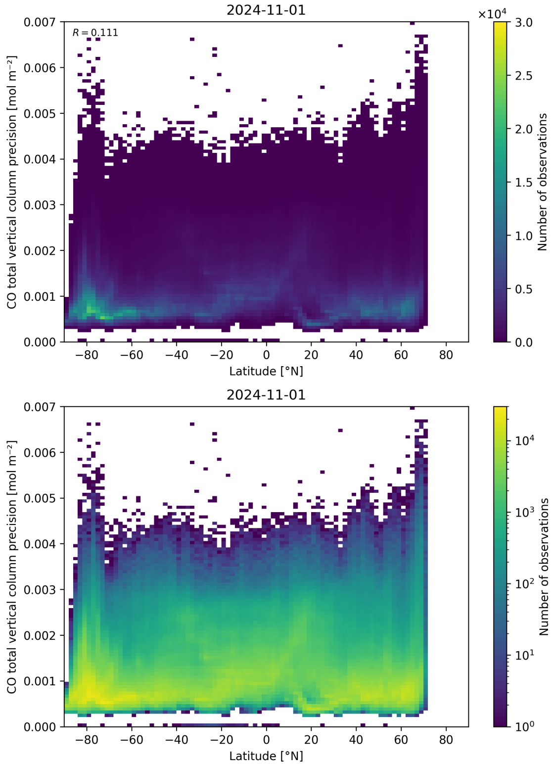
Figure 53: Scatter density plot of “Latitude” against “CO total vertical column precision” for 2024-10-31 to 2024-11-02.
