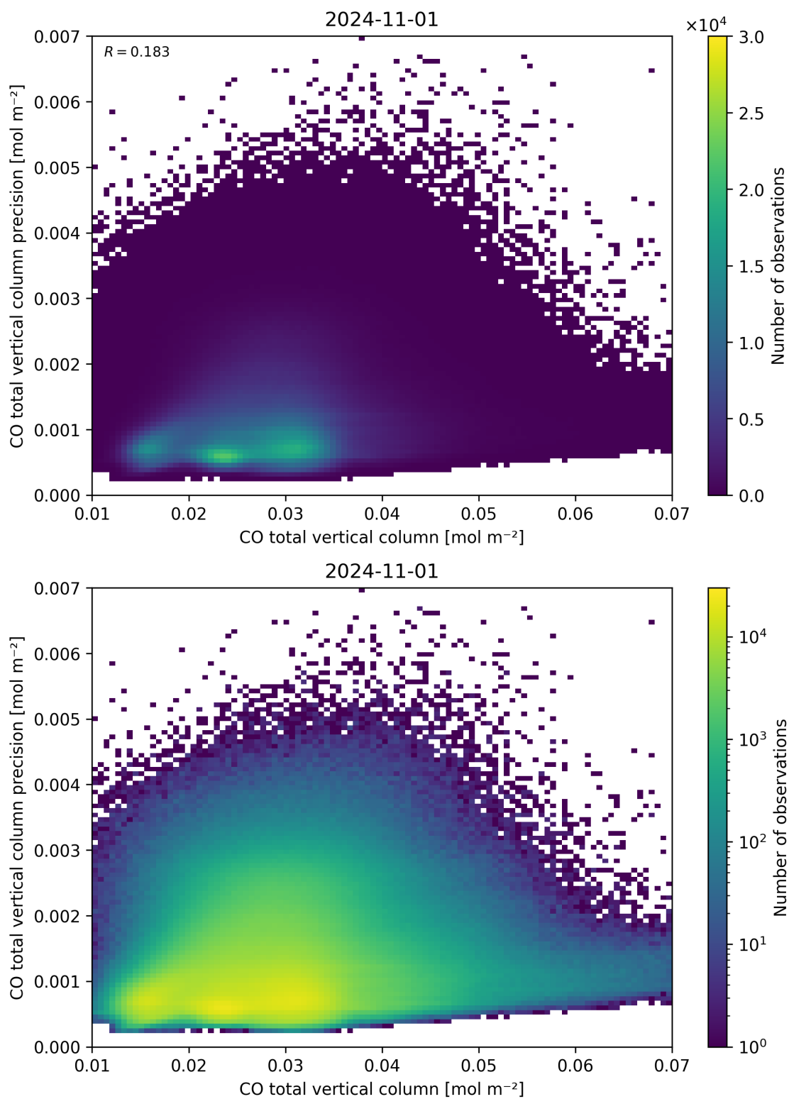
Figure 34: Scatter density plot of “CO total vertical column” against “CO total vertical column precision” for 2024-10-31 to 2024-11-02.
