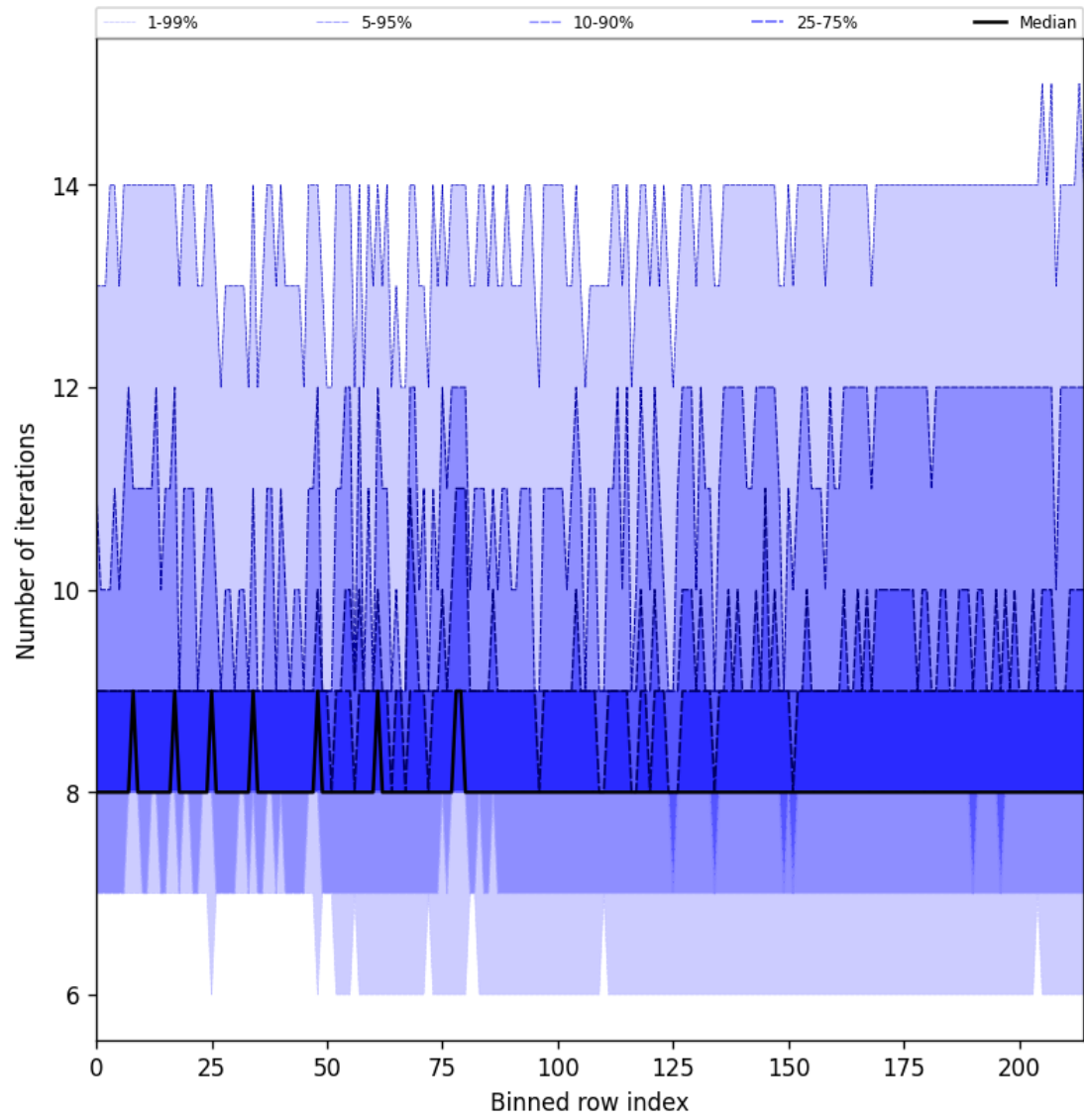
Figure 32: Along track statistics of “Number of iterations” for 2024-10-31 to 2024-11-02
