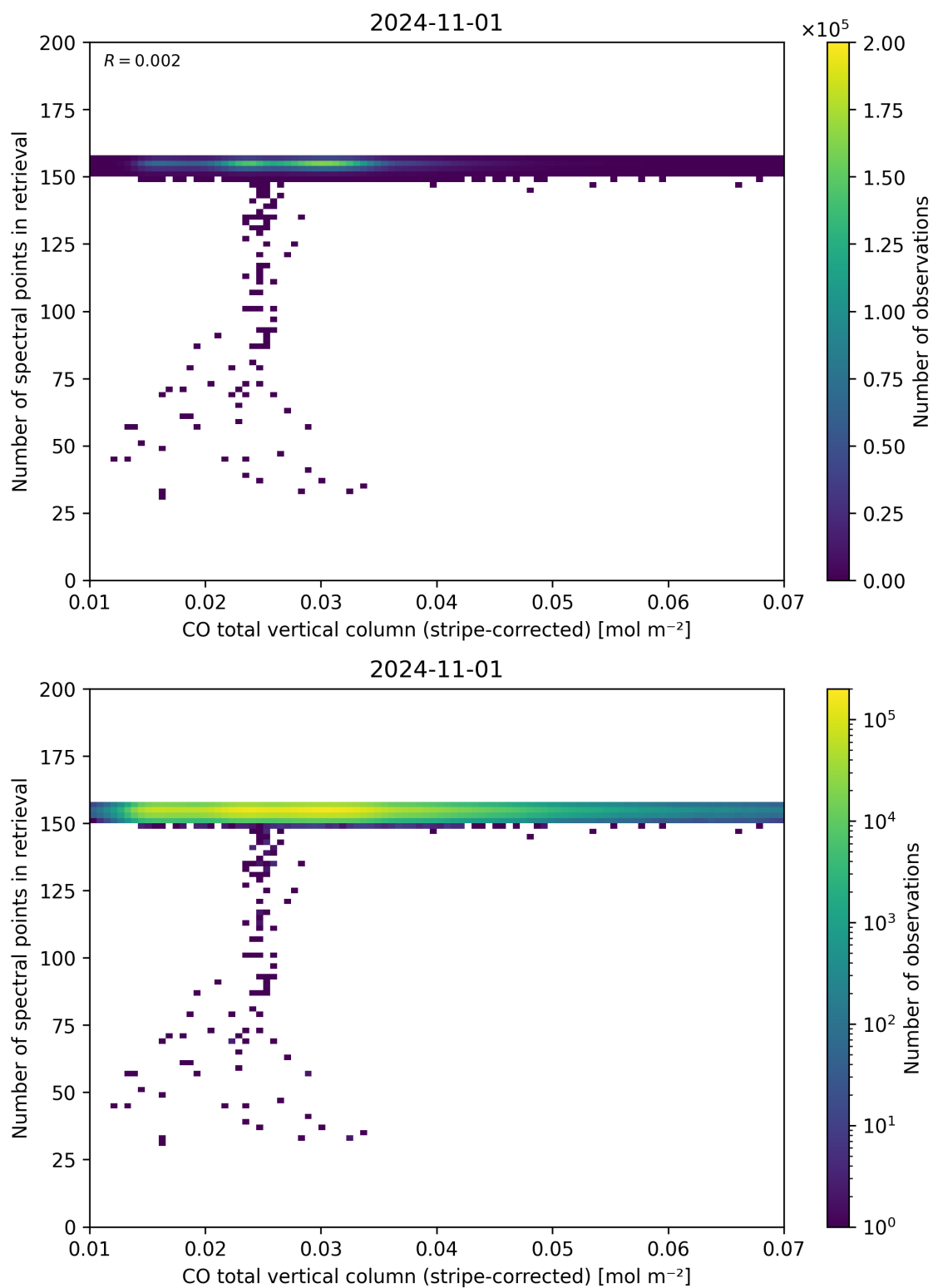
Figure 40: Scatter density plot of “CO total vertical column (stripe-corrected)” against “Number of spectral points in retrieval” for 2024-10-31 to 2024-11-02.
