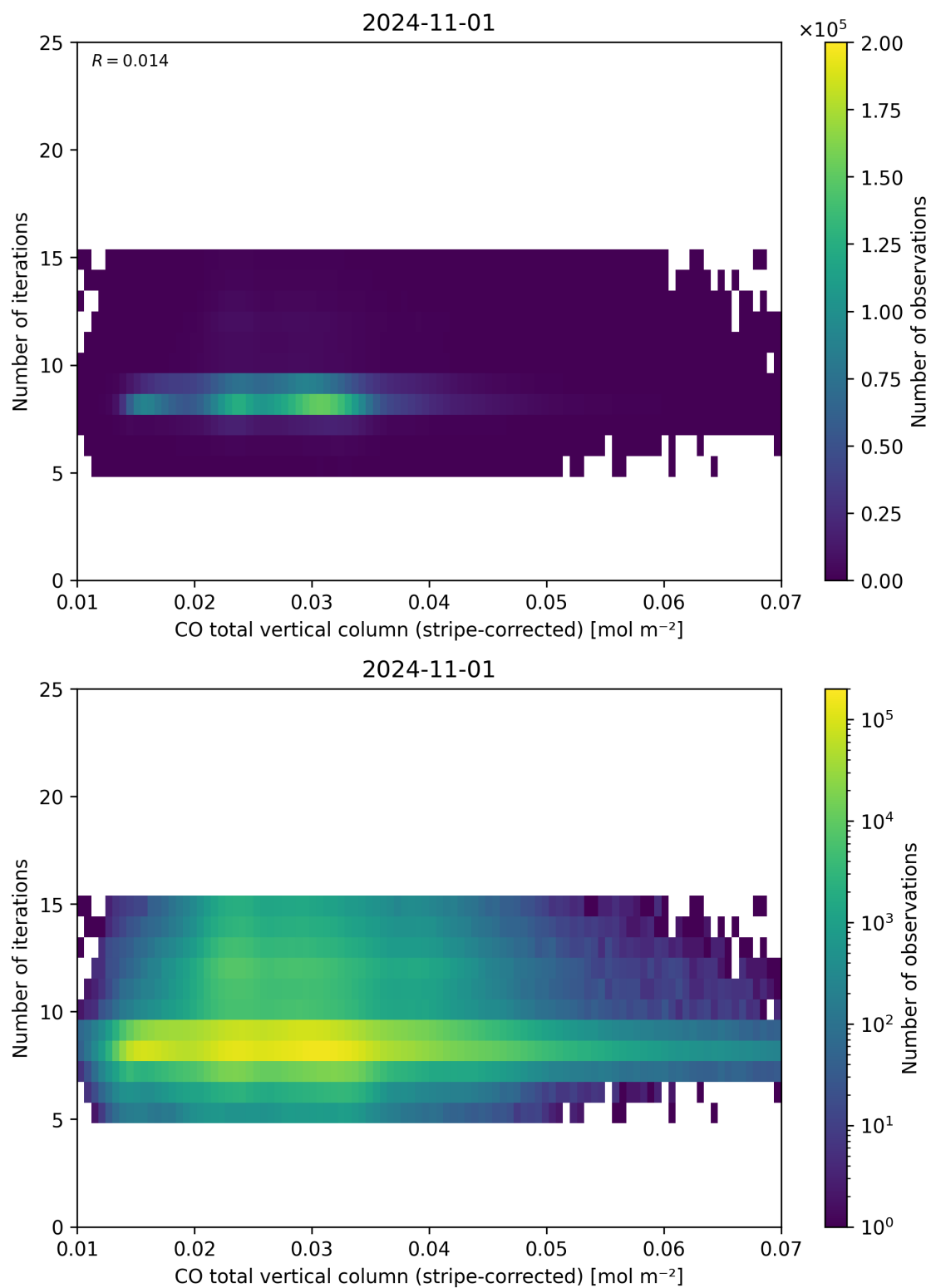
Figure 39: Scatter density plot of “CO total vertical column (stripe-corrected)” against “Number of iterations” for 2024-10-31 to 2024-11-02.
