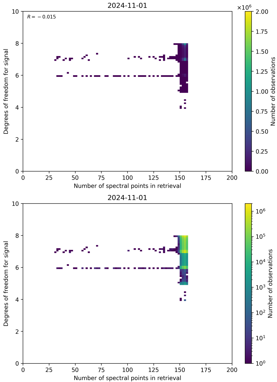
Figure 59: Scatter density plot of “Number of spectral points in retrieval” against “Degrees of freedom for signal” for 2024-10-31 to 2024-11-02.
