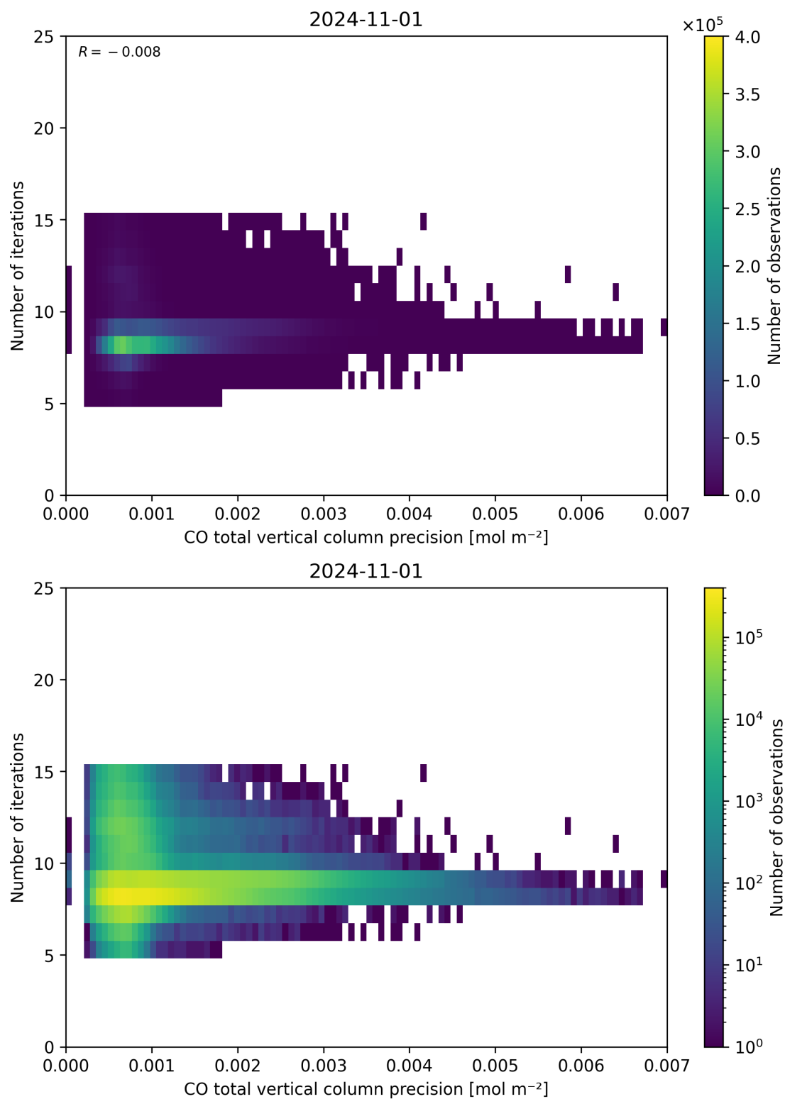
Figure 46: Scatter density plot of “CO total vertical column precision” against “Number of iterations” for 2024-10-31 to 2024-11-02.
