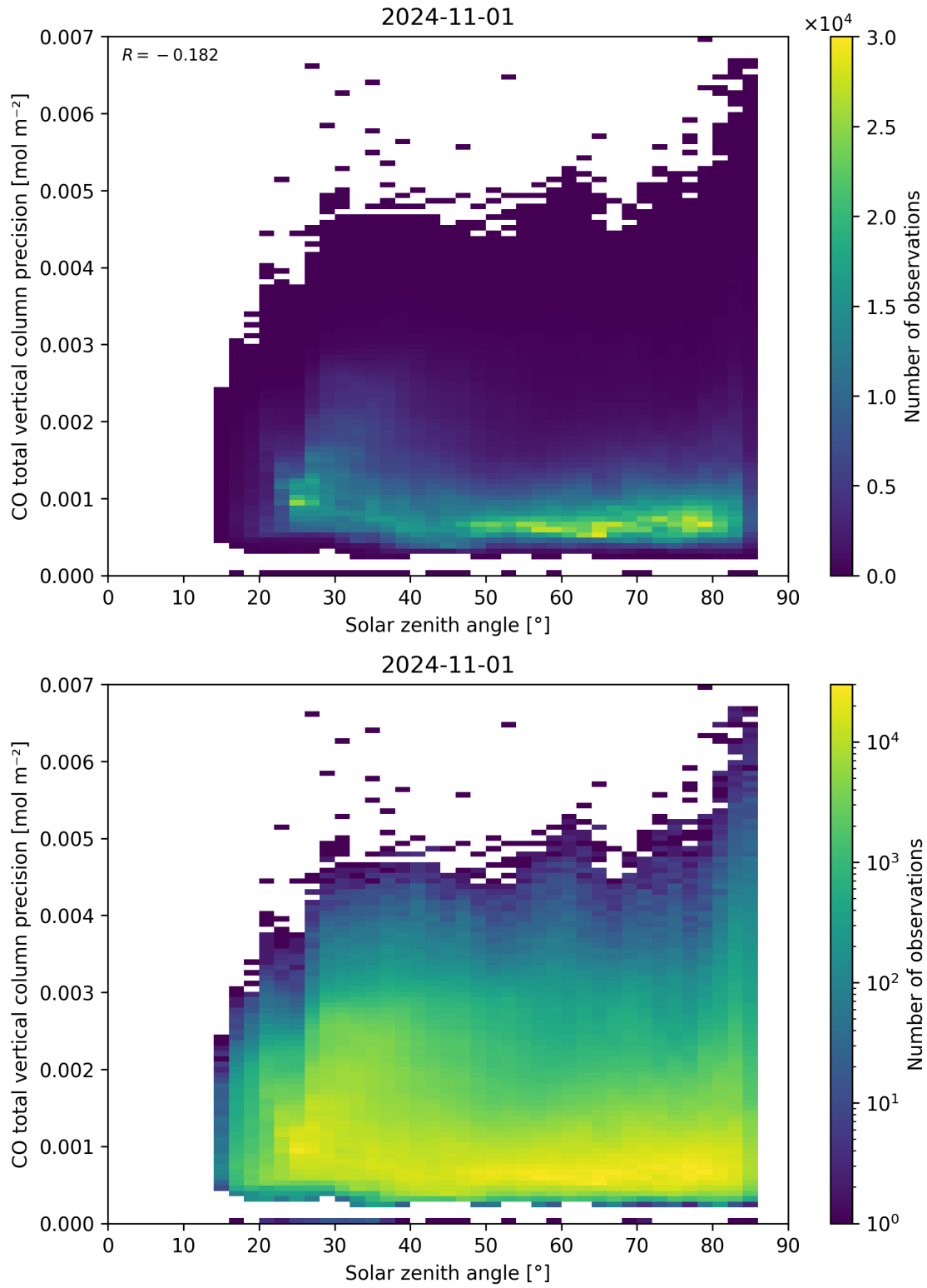
Figure 63: Scatter density plot of “Solar zenith angle” against “CO total vertical column precision” for 2024-10-31 to 2024-11-02.
