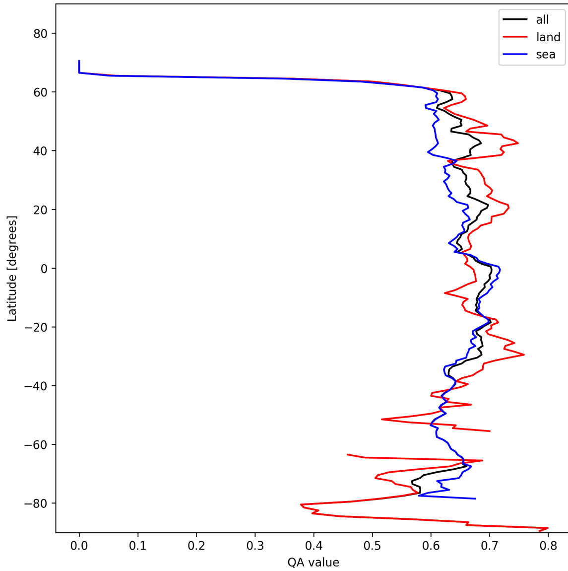
Figure 9: Zonal average of “QA value” for 2024-10-31 to 2024-11-02.
