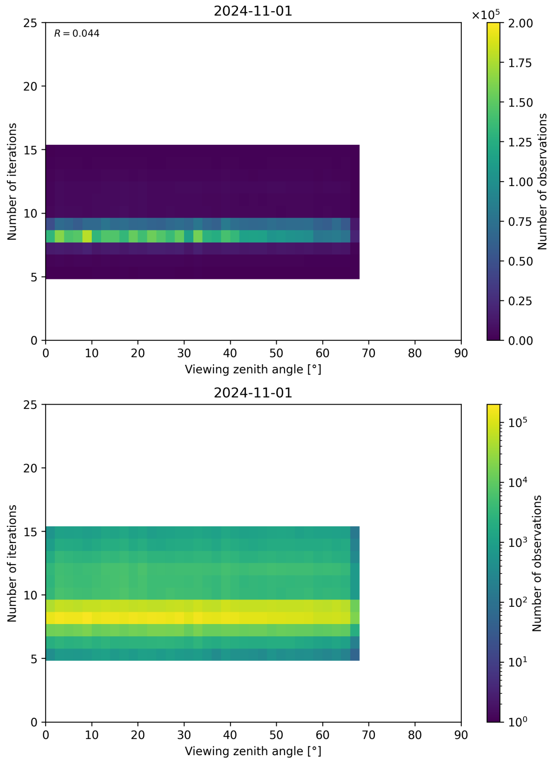
Figure 75: Scatter density plot of “Viewing zenith angle” against “Number of iterations” for 2024-10-31 to 2024-11-02.
