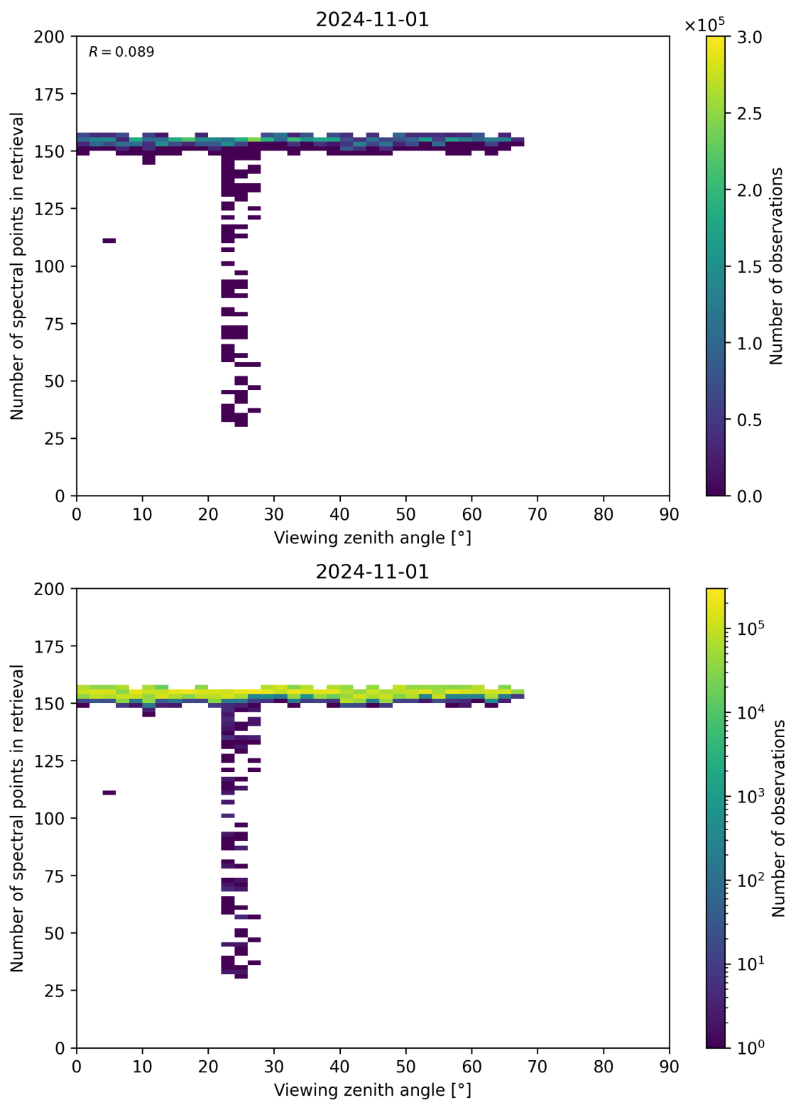
Figure 76: Scatter density plot of “Viewing zenith angle” against “Number of spectral points in retrieval” for 2024-10-31 to 2024-11-02.
