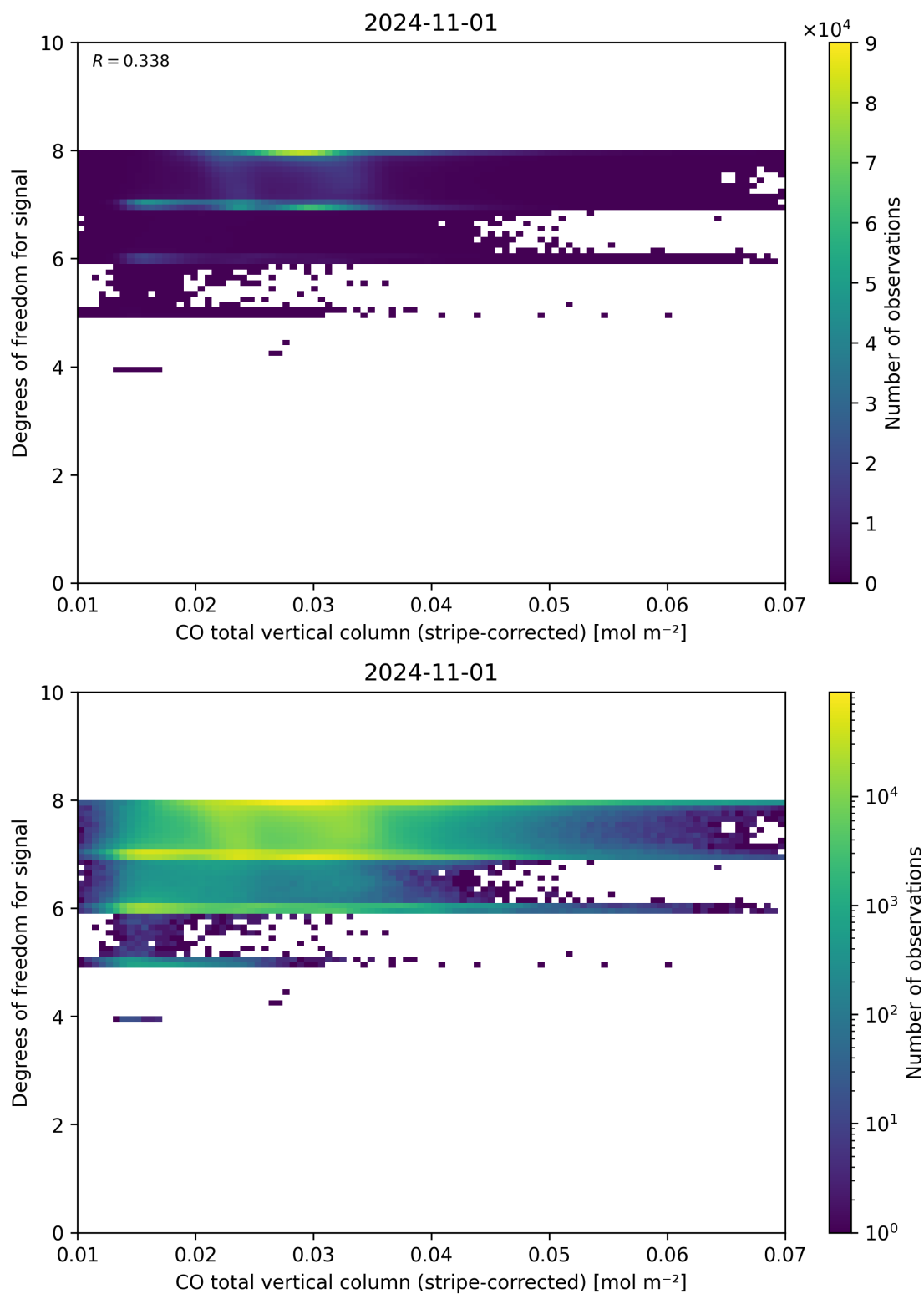
Figure 38: Scatter density plot of “CO total vertical column (stripe-corrected)” against “Degrees of freedom for signal” for 2024-10-31 to 2024-11-02.
