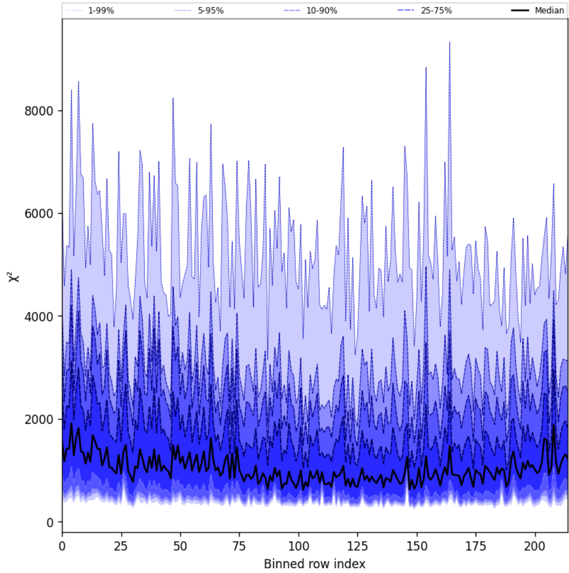
Figure 30: Along track statistics of “ \chi^2 ” for 2024-10-31 to 2024-11-02
