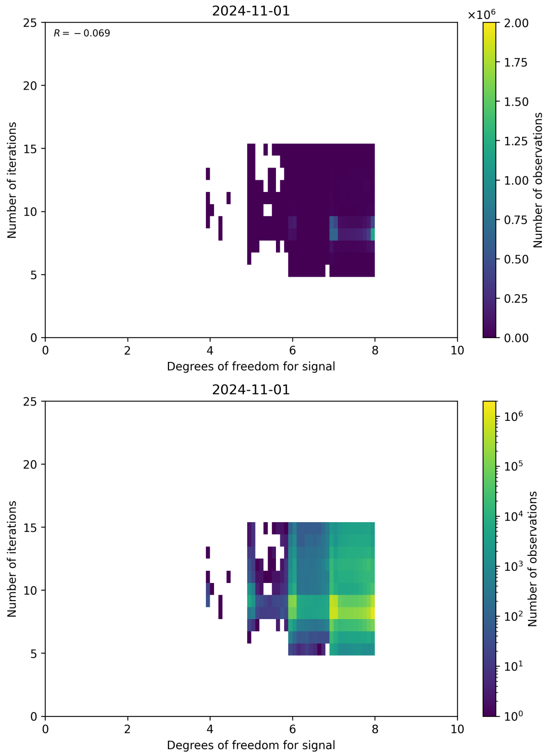
Figure 50: Scatter density plot of “Degrees of freedom for signal” against “Number of iterations” for 2024-10-31 to 2024-11-02.
