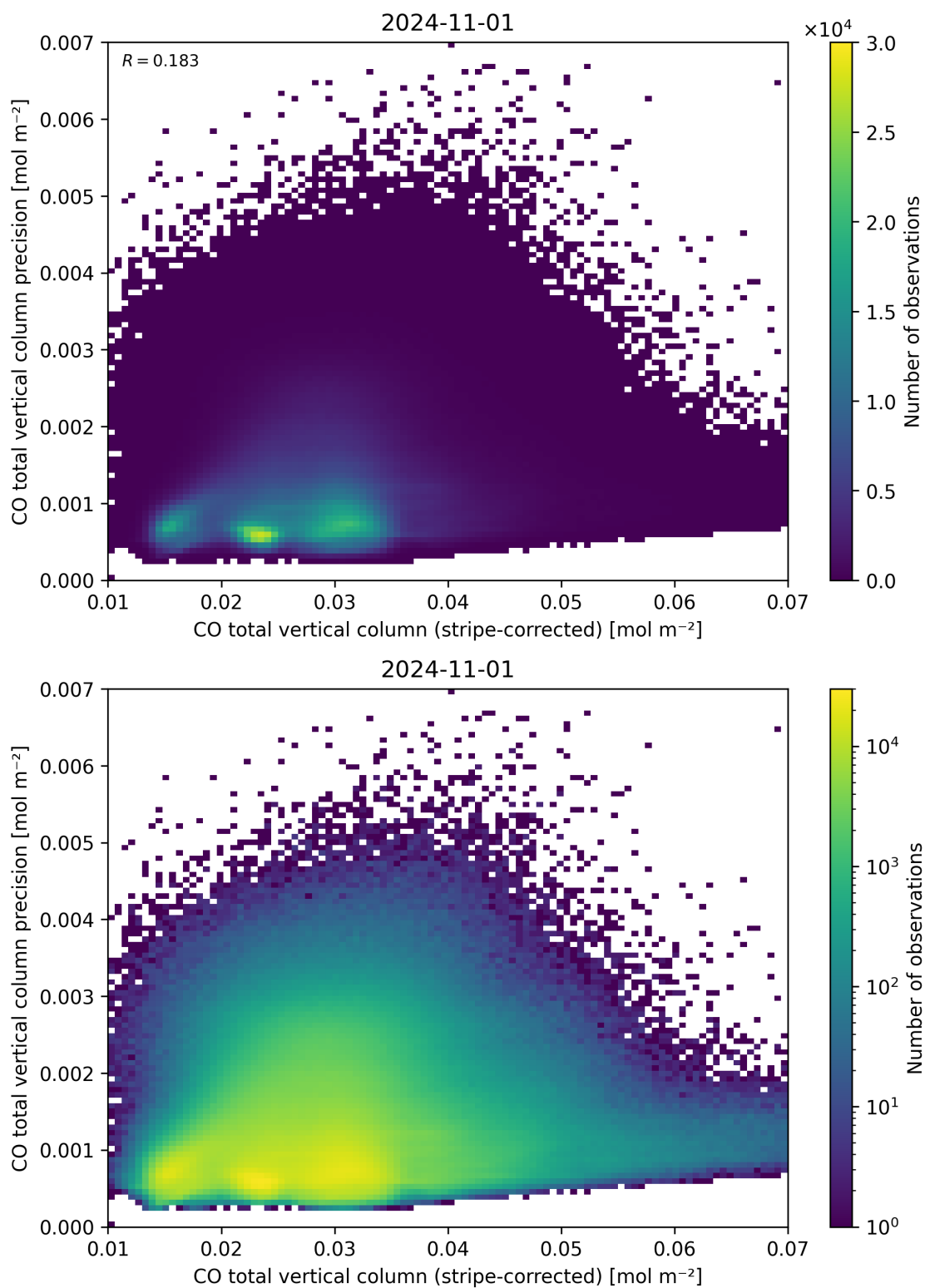
Figure 36: Scatter density plot of “CO total vertical column (stripe-corrected)” against “CO total vertical column precision” for 2024-10-31 to 2024-11-02.
