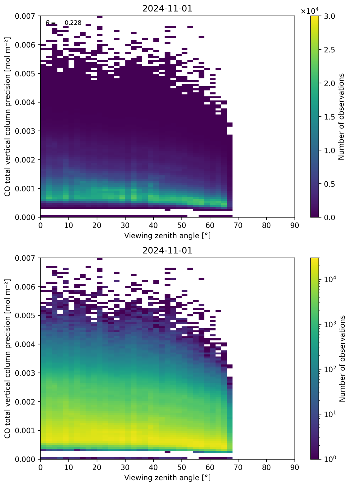
Figure 71: Scatter density plot of “Viewing zenith angle” against “CO total vertical column precision” for 2024-10-31 to 2024-11-02.
