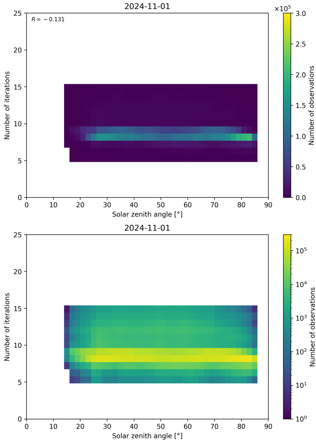
Figure 67: Scatter density plot of “Solar zenith angle” against “Number of iterations” for 2024-10-31 to 2024-11-02.
