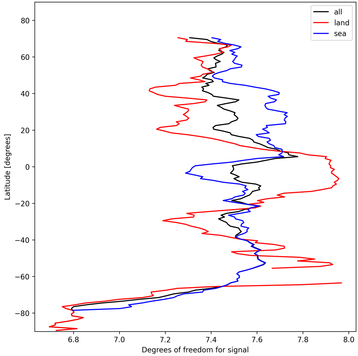
Figure 15: Zonal average of “Degrees of freedom for signal” for 2024-10-31 to 2024-11-02.
