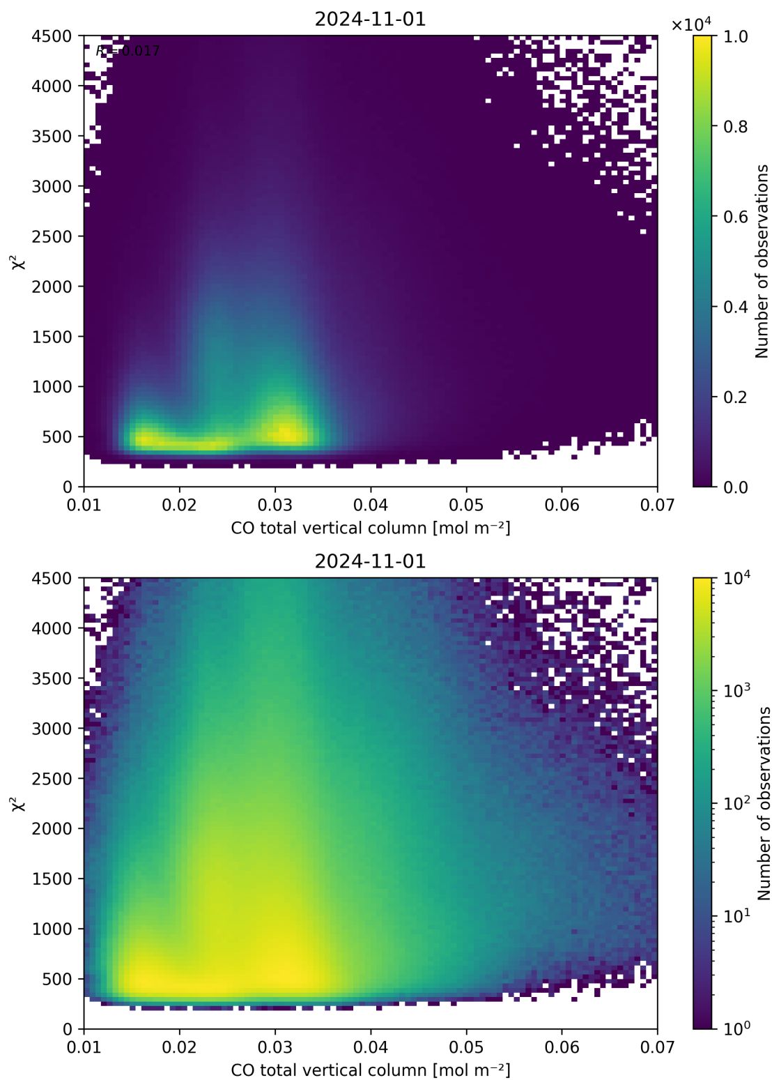
Figure 35: Scatter density plot of “CO total vertical column” against “ \chi^2 ” for 2024-10-31 to 2024-11-02.
