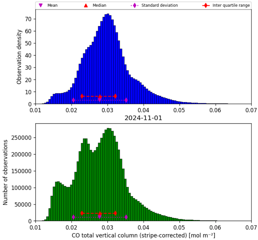
Figure 19: Histogram of “CO total vertical column (stripe-corrected)” for 2024-10-31 to 2024-11-02
