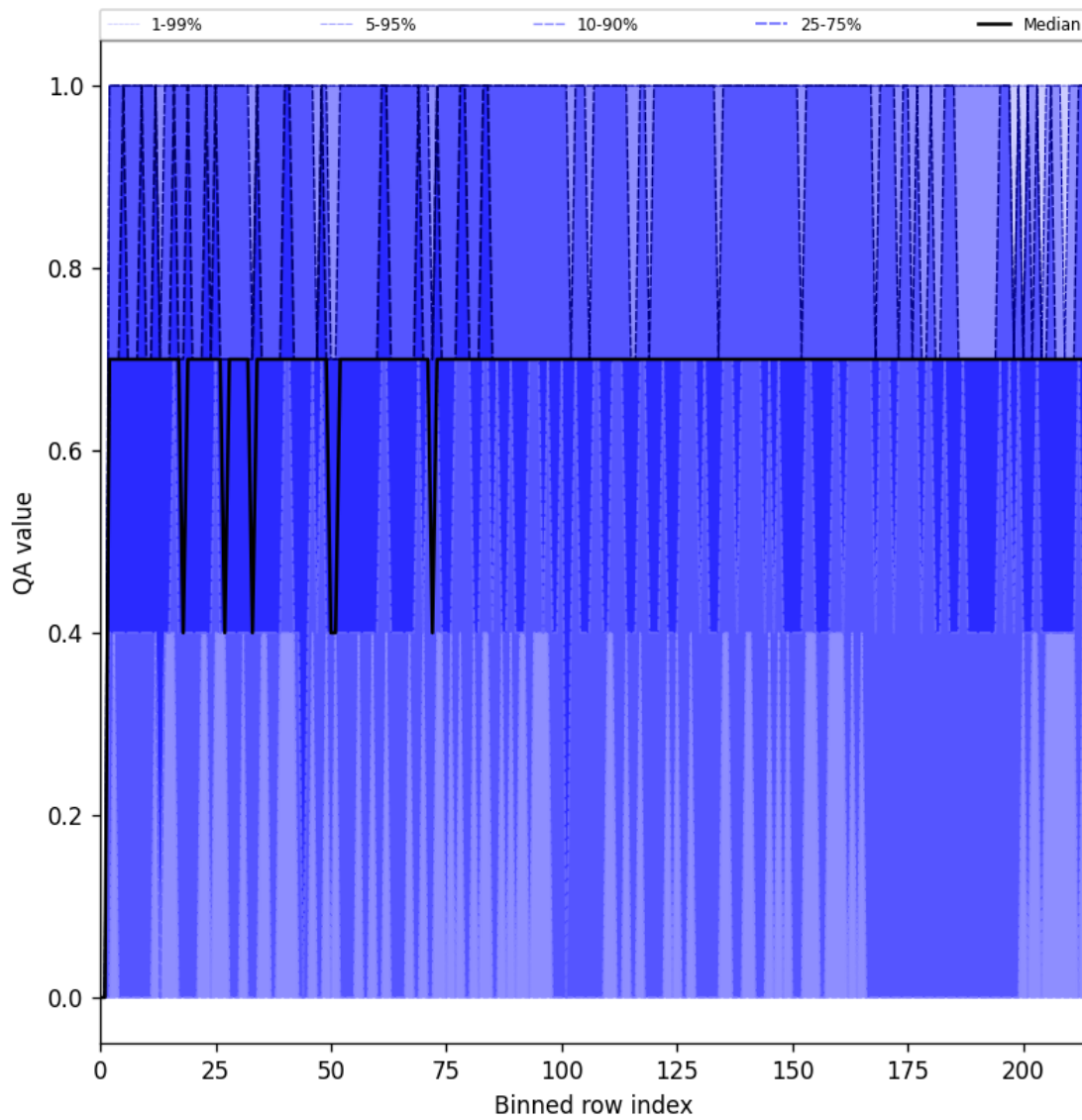
Figure 25: Along track statistics of “QA value” for 2024-10-31 to 2024-11-02
