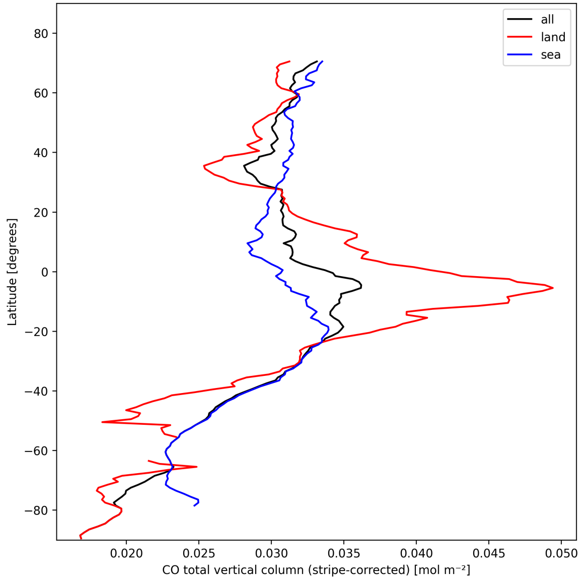
Figure 11: Zonal average of “CO total vertical column (stripe-corrected)” for 2024-10-31 to 2024-11-02.
