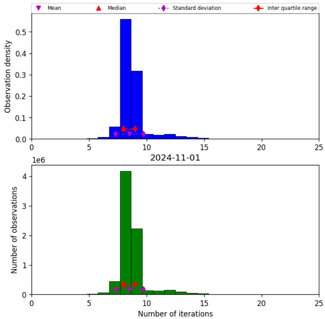
Figure 24: Histogram of “Number of iterations” for 2024-10-31 to 2024-11-02
