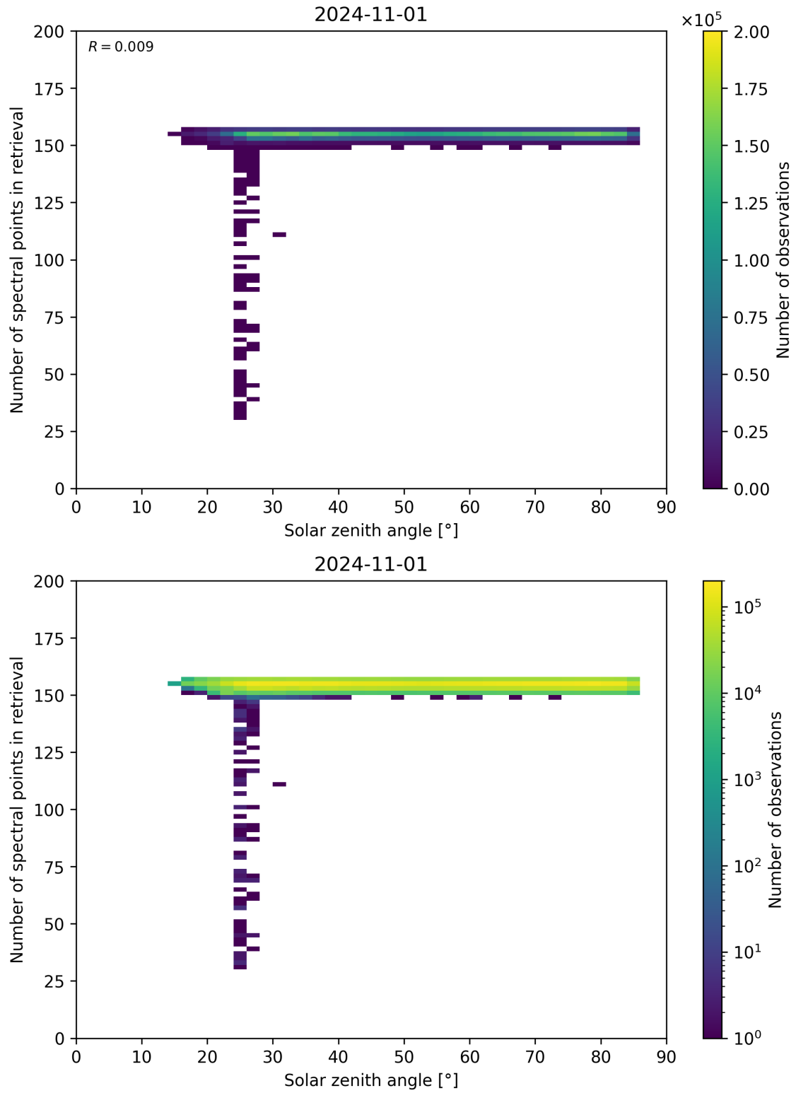
Figure 68: Scatter density plot of “Solar zenith angle” against “Number of spectral points in retrieval” for 2024-10-31 to 2024-11-02.
