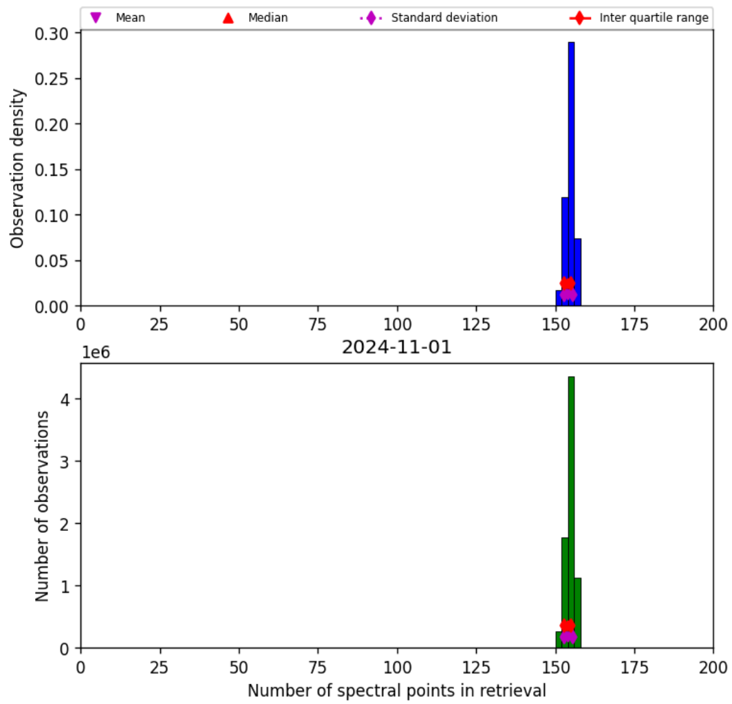
Figure 21: Histogram of “Number of spectral points in retrieval” for 2024-10-31 to 2024-11-02
