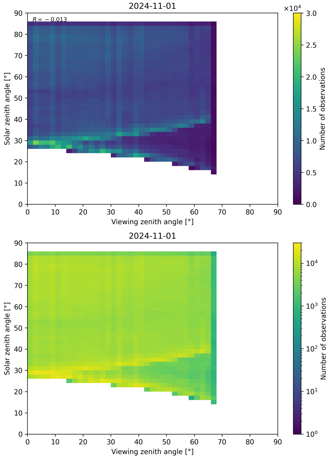
Figure 77: Scatter density plot of “Viewing zenith angle” against “Solar zenith angle” for 2024-10-31 to 2024-11-02.
