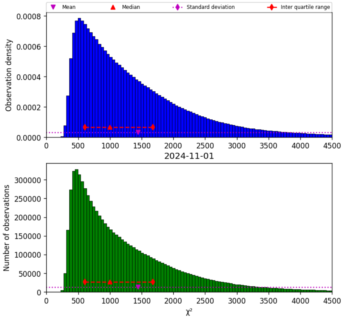
Figure 22: Histogram of “ \chi^2 ” for 2024-10-31 to 2024-11-02
