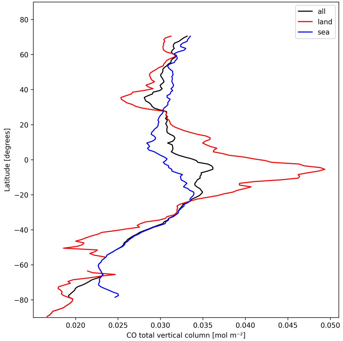
Figure 10: Zonal average of “CO total vertical column” for 2024-10-31 to 2024-11-02.
