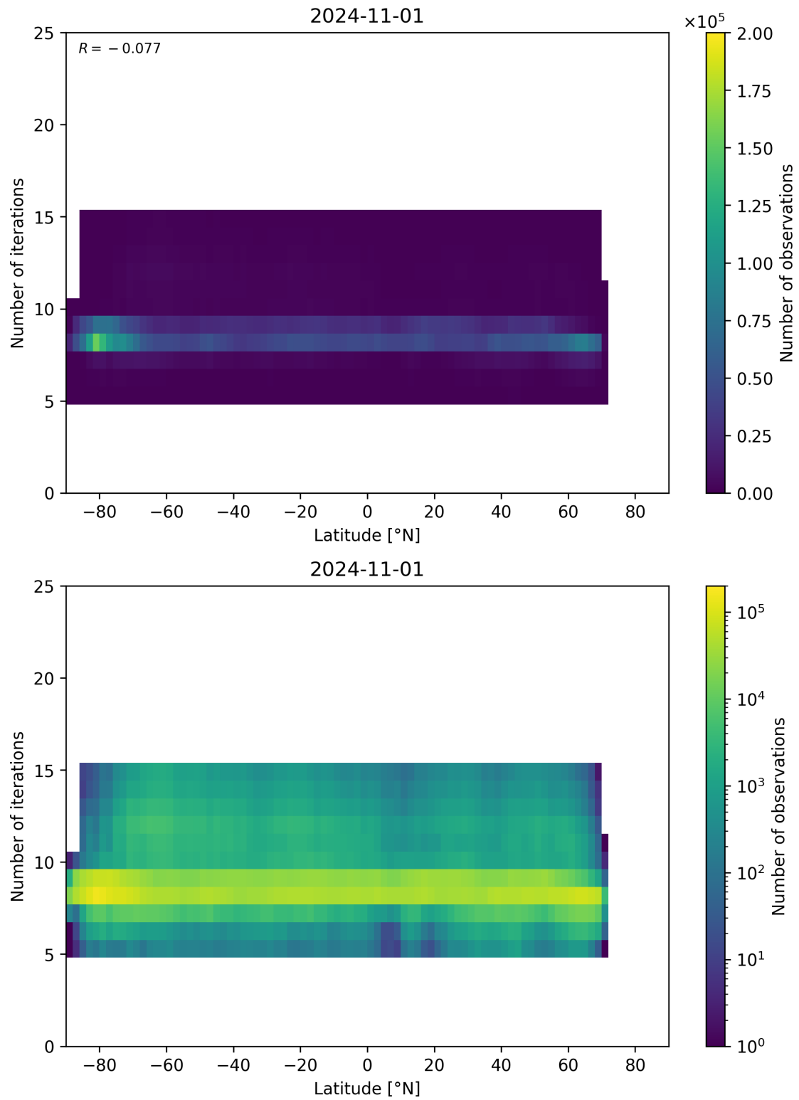
Figure 56: Scatter density plot of “Latitude” against “Number of iterations” for 2024-10-31 to 2024-11-02.
