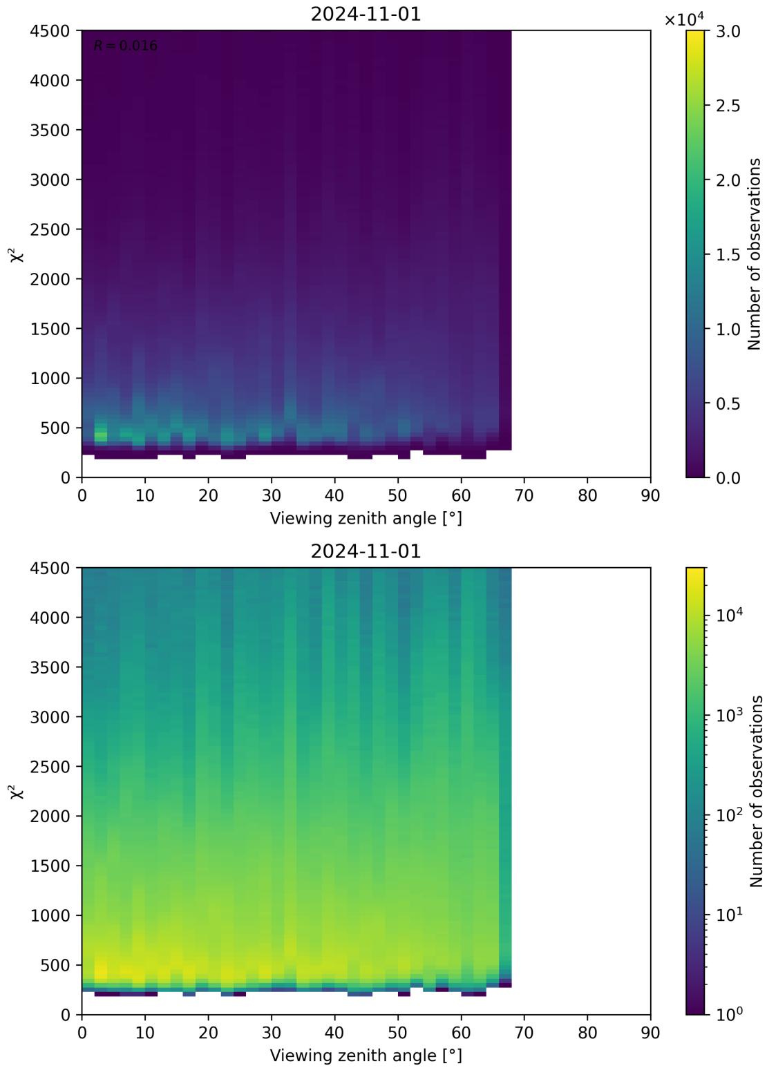
Figure 72: Scatter density plot of “Viewing zenith angle” against “ \chi^2 ” for 2024-10-31 to 2024-11-02.
