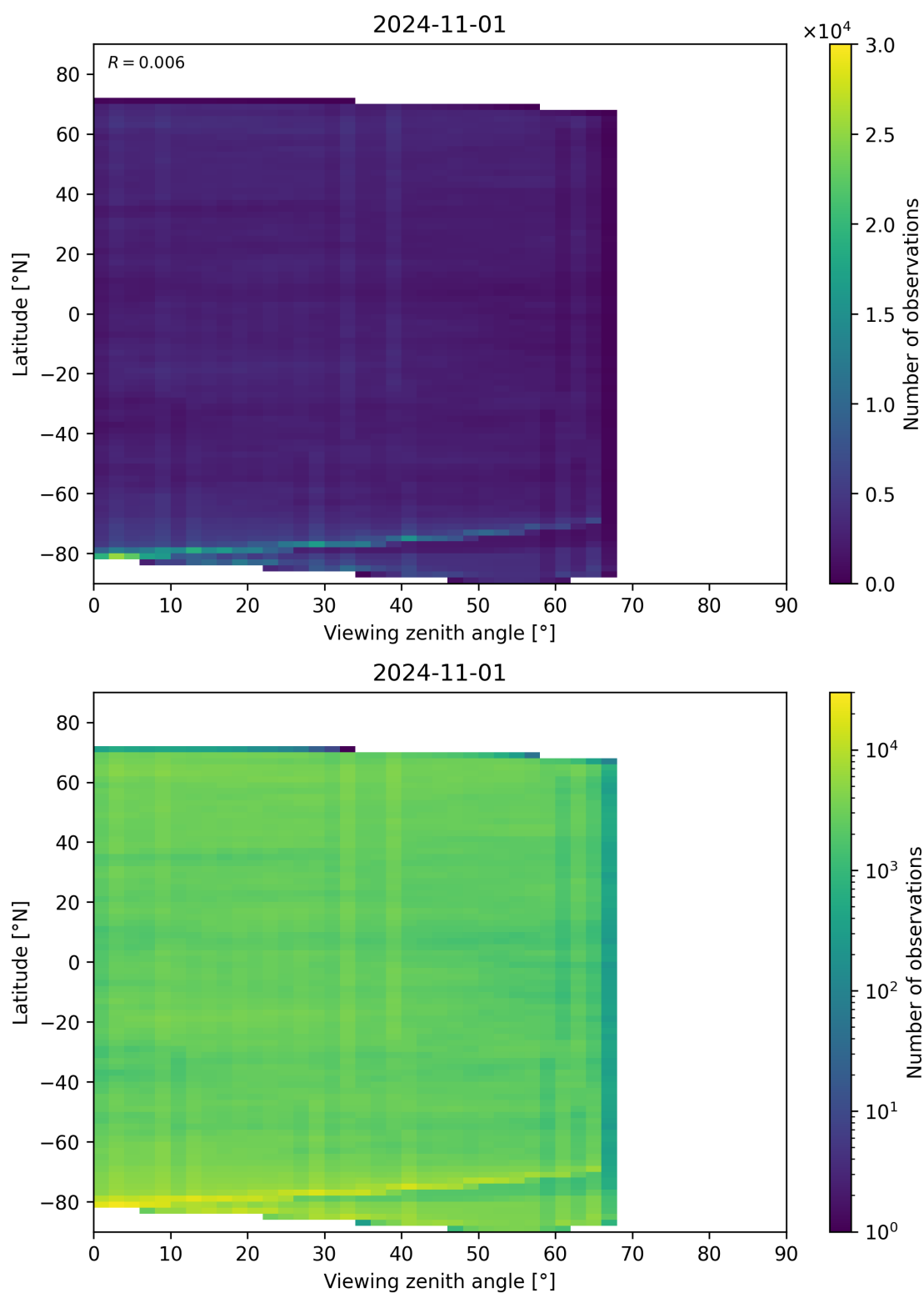
Figure 74: Scatter density plot of “Viewing zenith angle” against “Latitude” for 2024-10-31 to 2024-11-02.
