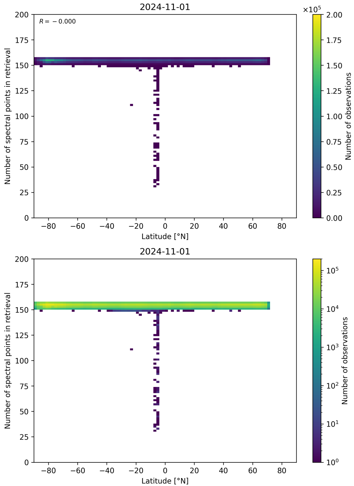
Figure 57: Scatter density plot of “Latitude” against “Number of spectral points in retrieval” for 2024-10-31 to 2024-11-02.
