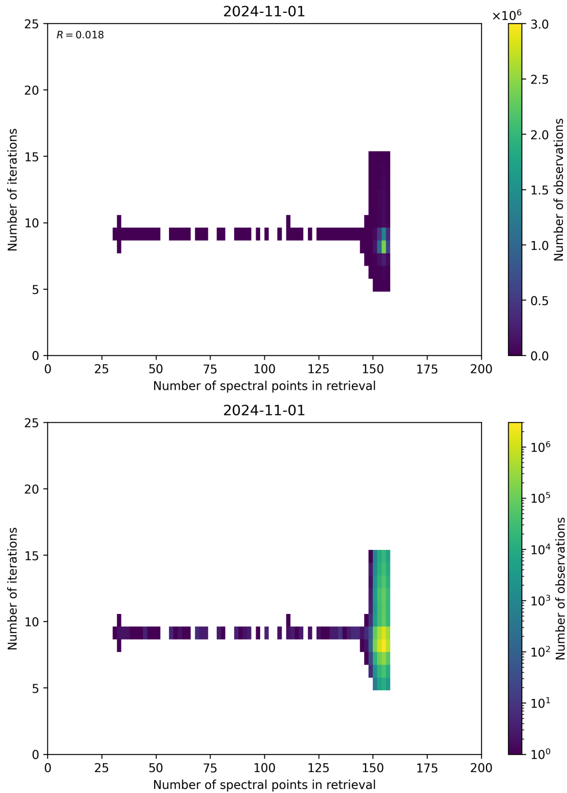
Figure 60: Scatter density plot of “Number of spectral points in retrieval” against “Number of iterations” for 2024-10-31 to 2024-11-02.
