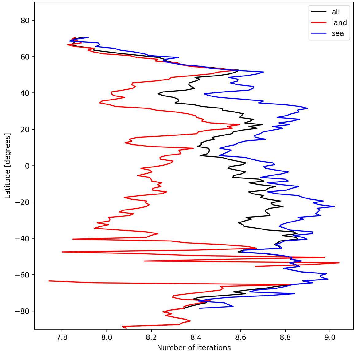
Figure 16: Zonal average of “Number of iterations” for 2024-10-31 to 2024-11-02.
