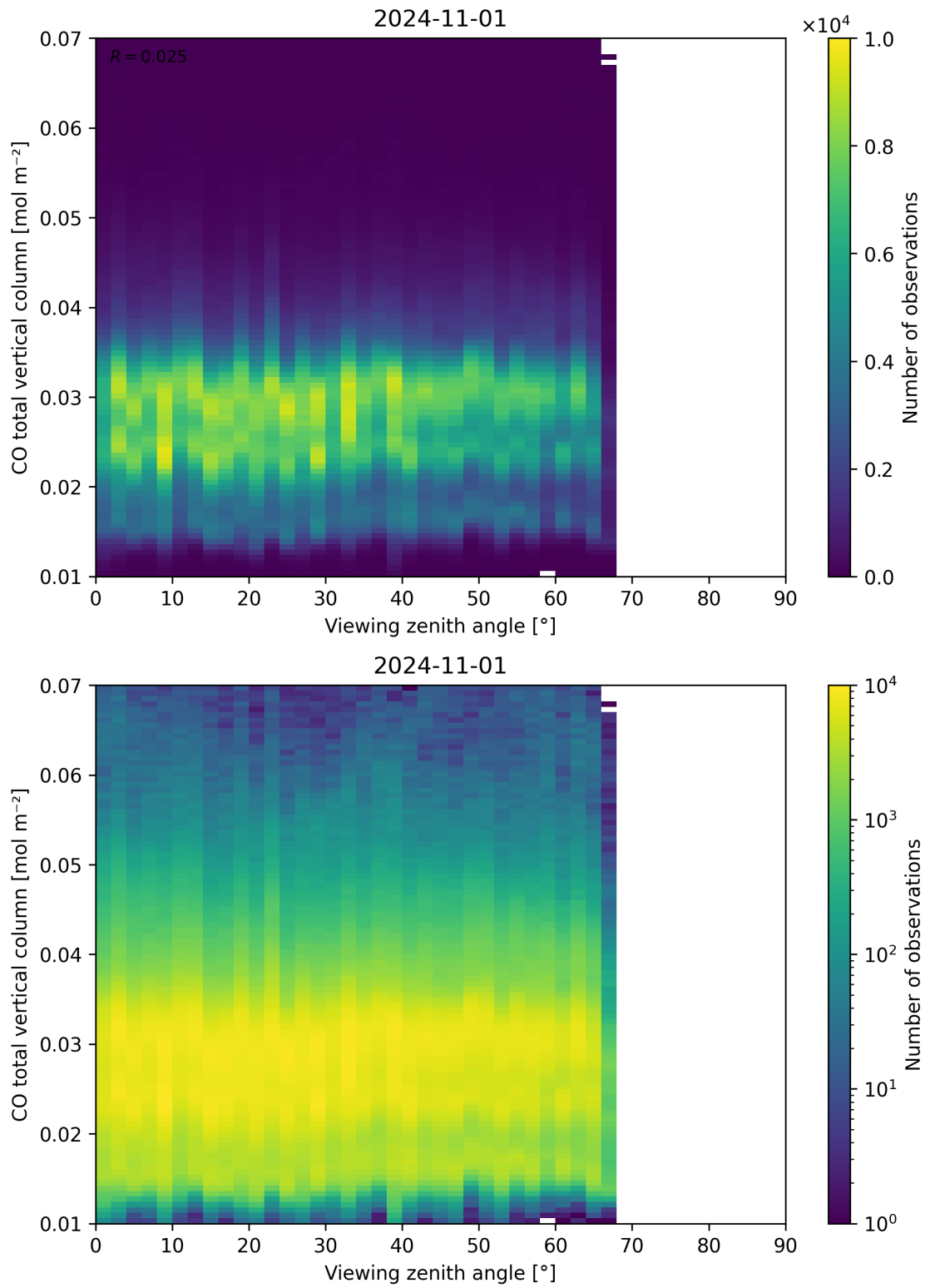
Figure 69: Scatter density plot of “Viewing zenith angle” against “CO total vertical column” for 2024-10-31 to 2024-11-02.
