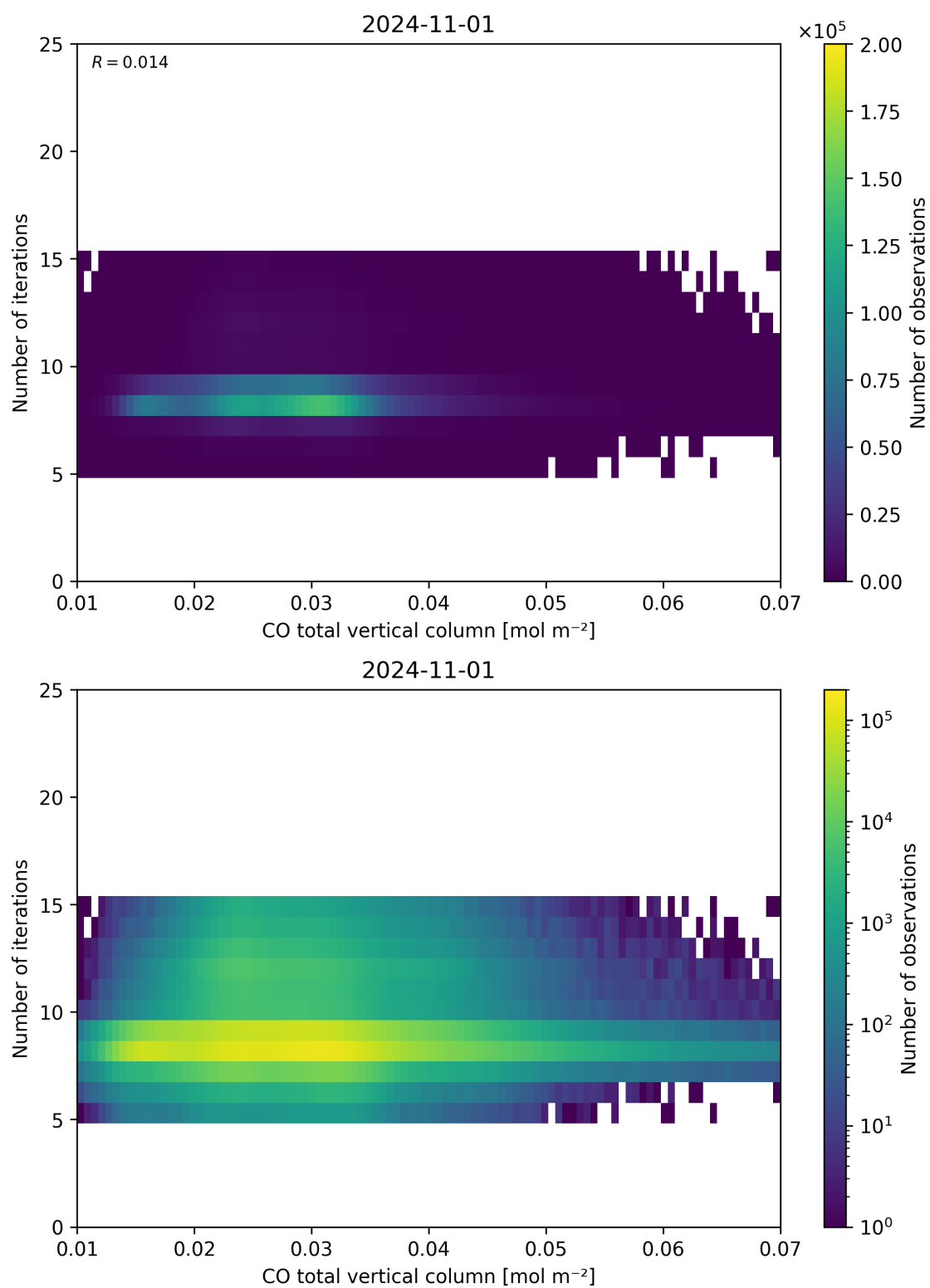
Figure 42: Scatter density plot of “CO total vertical column” against “Number of iterations” for 2024-10-31 to 2024-11-02.
