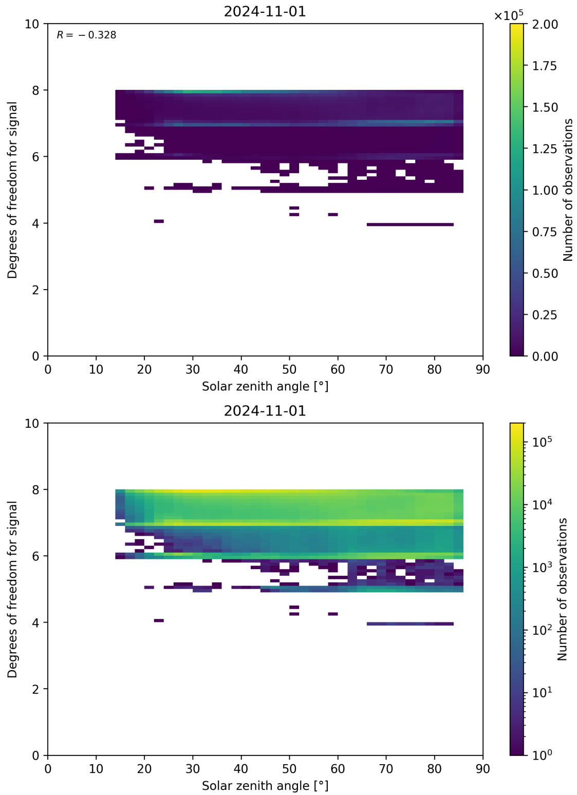
Figure 65: Scatter density plot of “Solar zenith angle” against “Degrees of freedom for signal” for 2024-10-31 to 2024-11-02.
