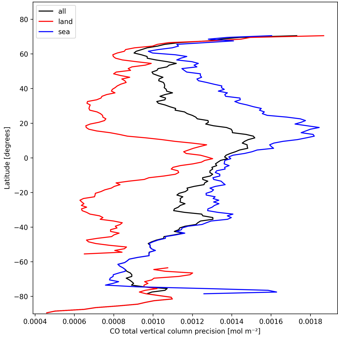
Figure 12: Zonal average of “CO total vertical column precision” for 2024-10-31 to 2024-11-02.
