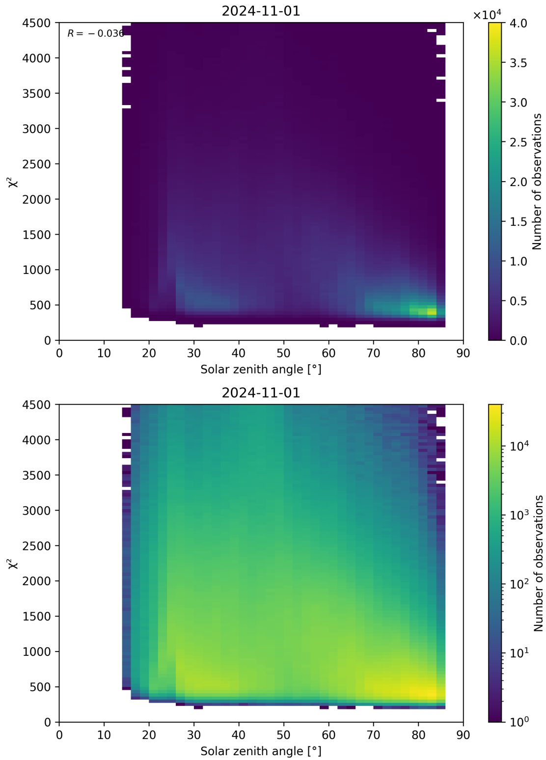
Figure 64: Scatter density plot of “Solar zenith angle” against “ \chi^2 ” for 2024-10-31 to 2024-11-02.
