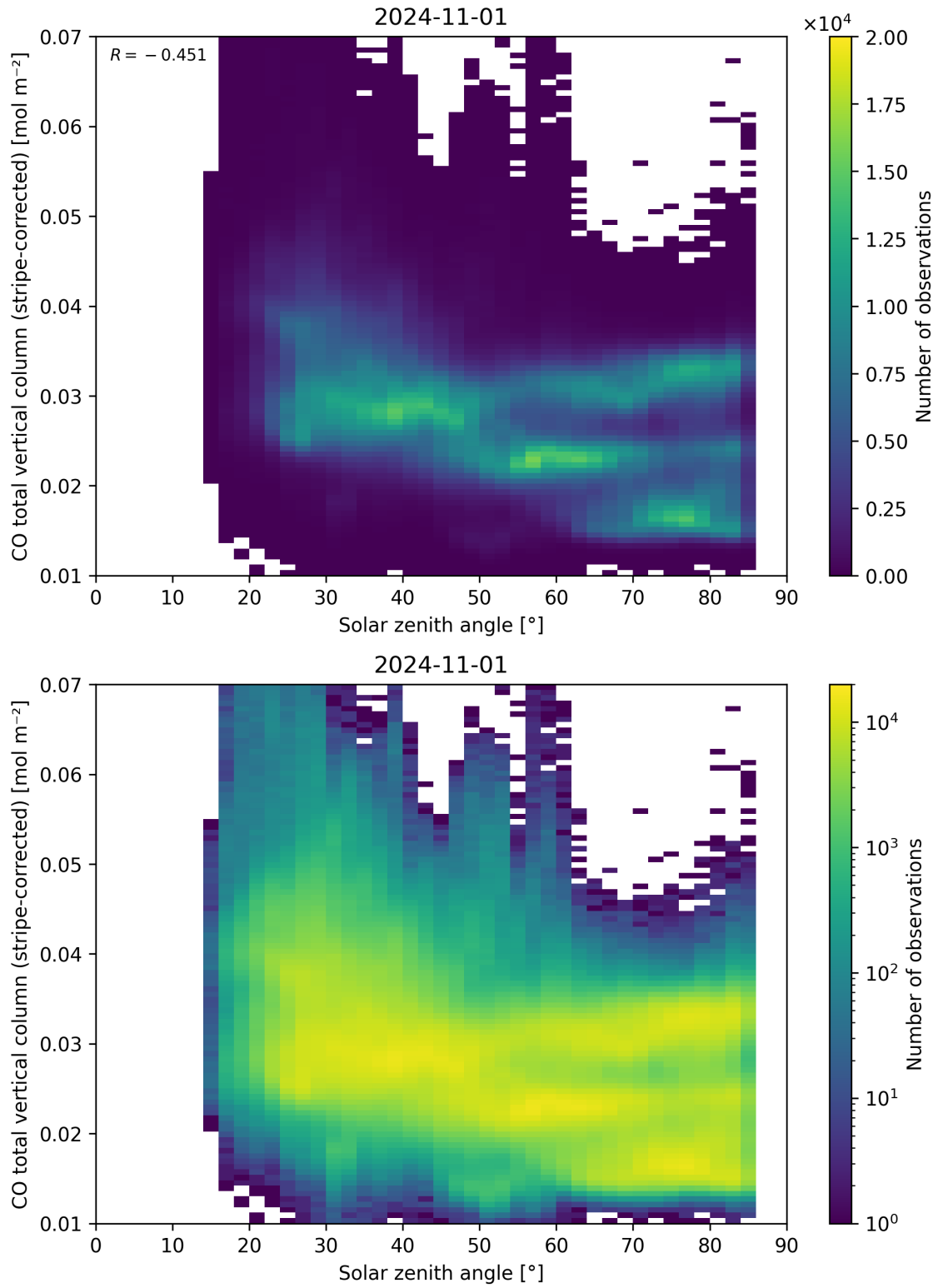
Figure 62: Scatter density plot of “Solar zenith angle” against “CO total vertical column (stripe-corrected)” for 2024-10-31 to 2024-11-02.
