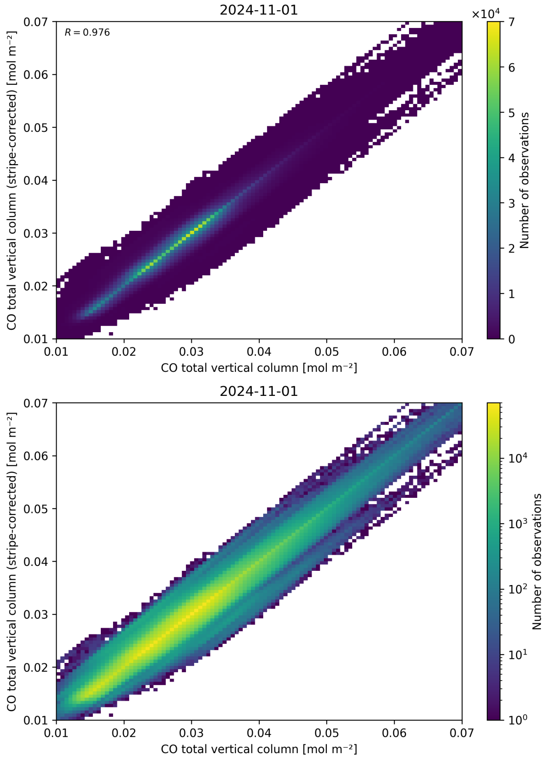
Figure 33: Scatter density plot of “CO total vertical column” against “CO total vertical column (stripe-corrected)” for 2024-10-31 to 2024-11-02.
