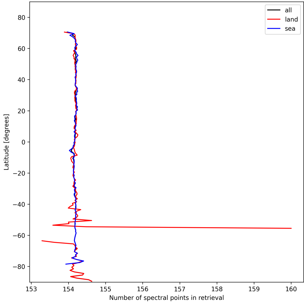
Figure 13: Zonal average of “Number of spectral points in retrieval” for 2024-10-31 to 2024-11-02.
