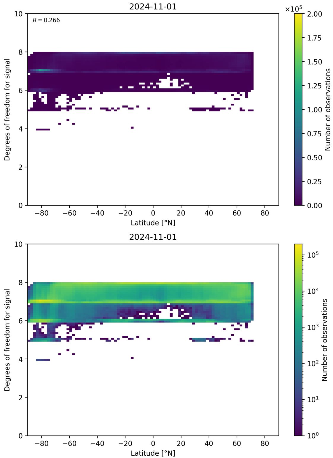
Figure 55: Scatter density plot of “Latitude” against “Degrees of freedom for signal” for 2024-10-31 to 2024-11-02.
