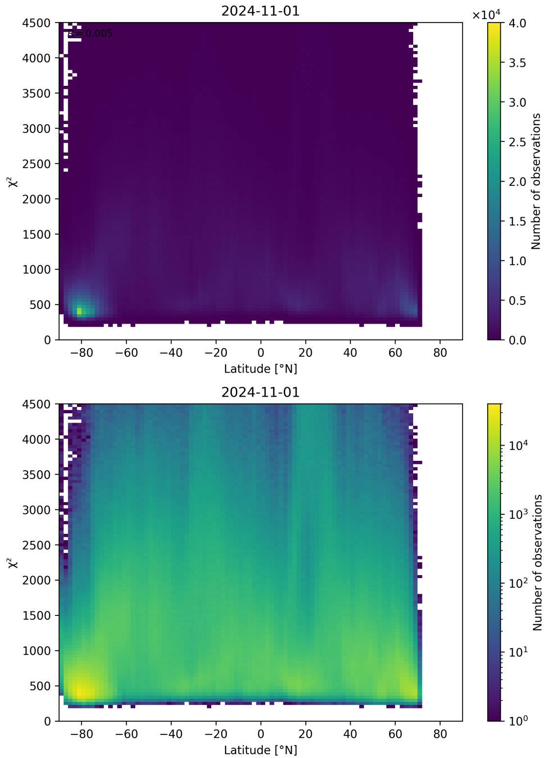
Figure 54: Scatter density plot of “Latitude” against “ \chi^2 ” for 2024-10-31 to 2024-11-02.
