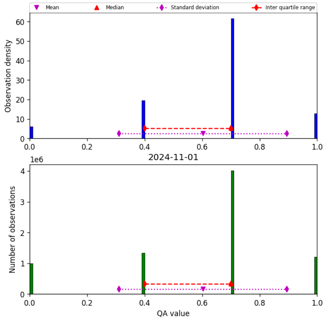
Figure 17: Histogram of “QA value” for 2024-10-31 to 2024-11-02
