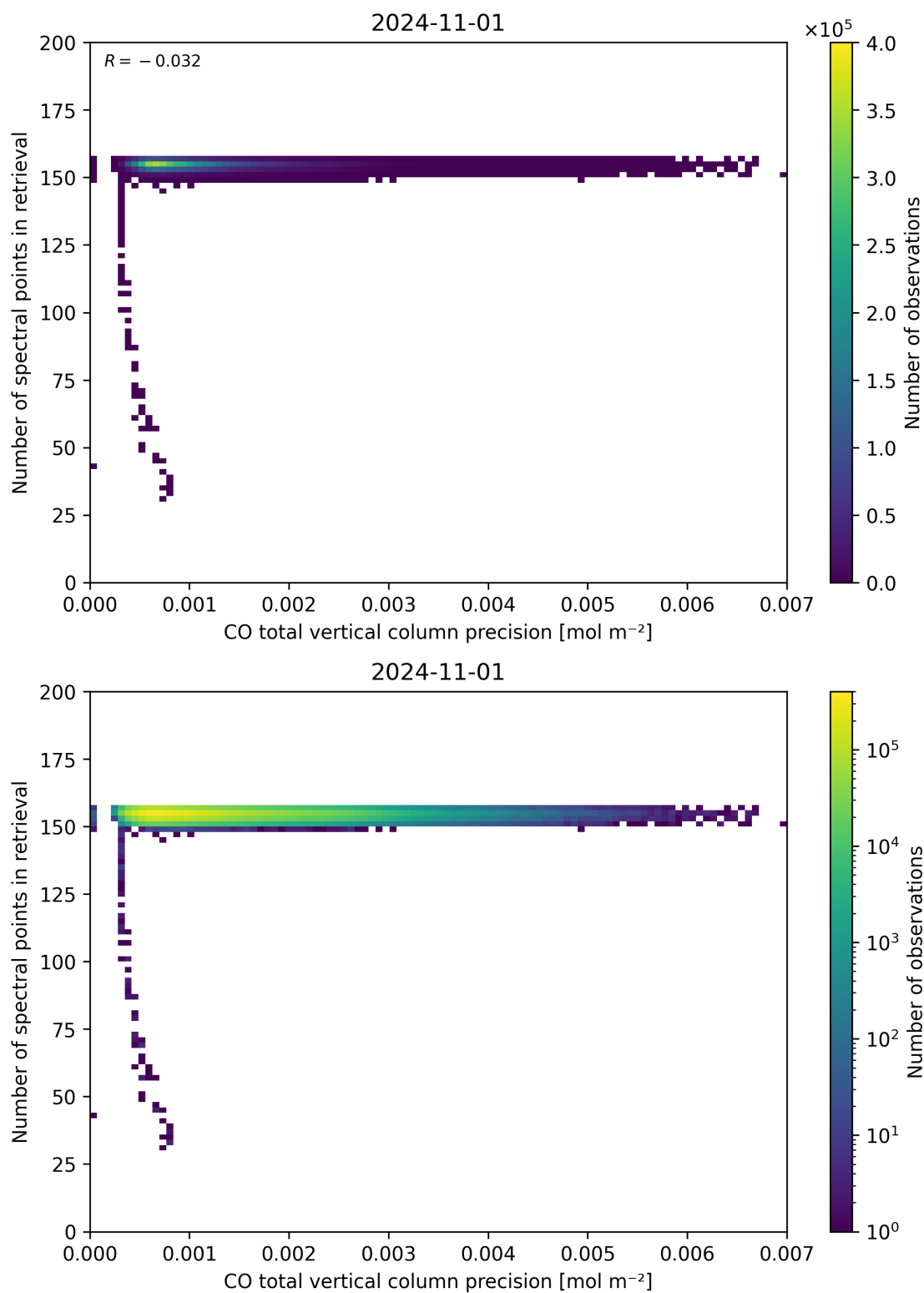
Figure 47: Scatter density plot of “CO total vertical column precision” against “Number of spectral points in retrieval” for 2024-10-31 to 2024-11-02.
