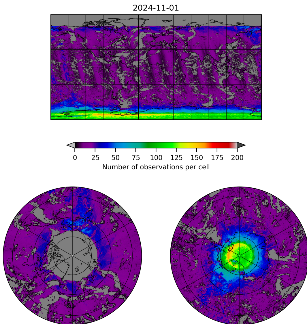
Figure 8: Map of the number of observations for 2024-10-31 to 2024-11-02
