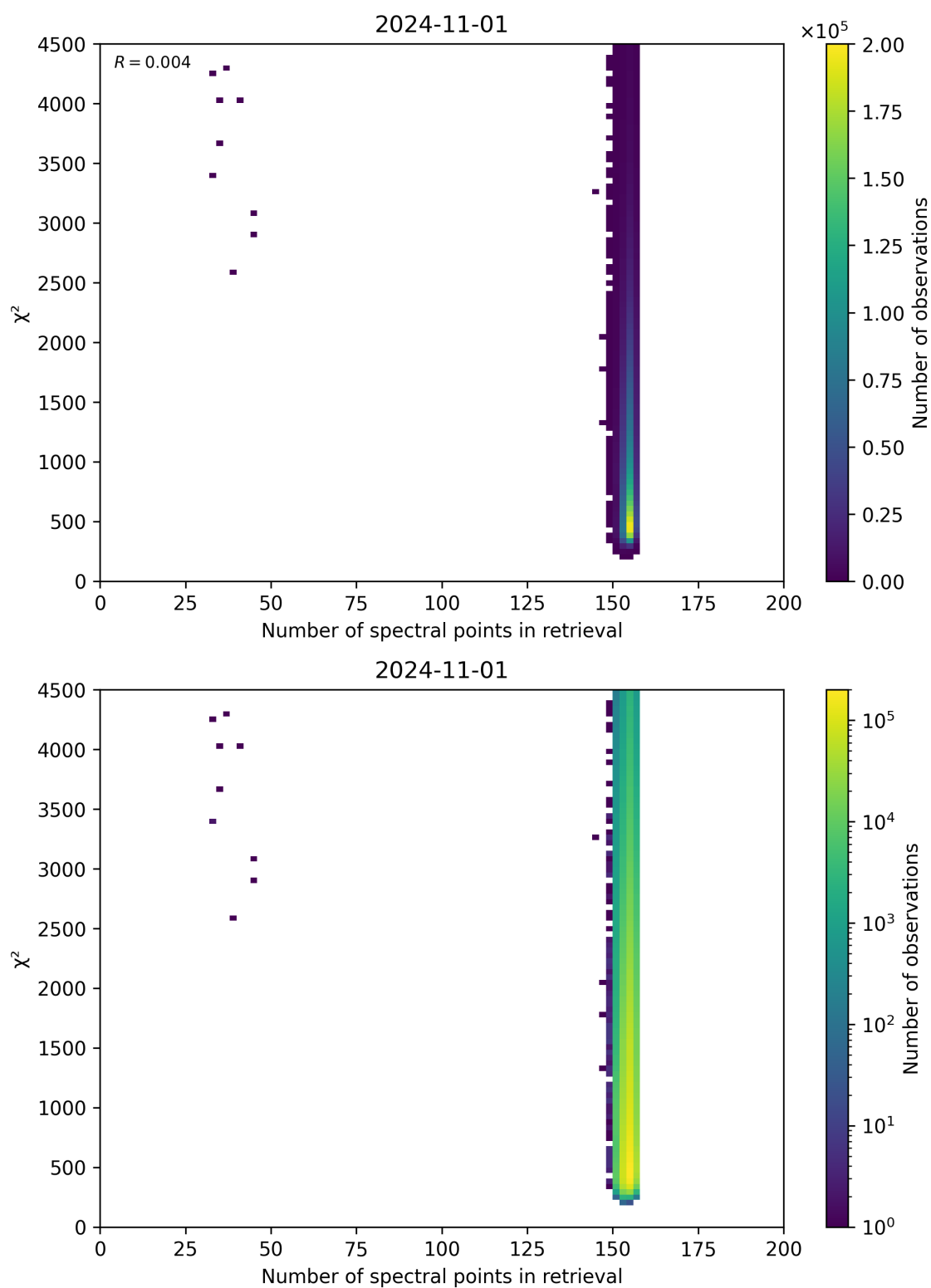
Figure 58: Scatter density plot of “Number of spectral points in retrieval” against “ \chi^2 ” for 2024-10-31 to 2024-11-02.
