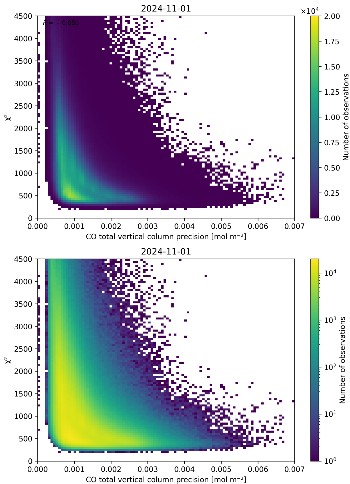
Figure 44: Scatter density plot of “CO total vertical column precision” against “ \chi^2 ” for 2024-10-31 to 2024-11-02.
