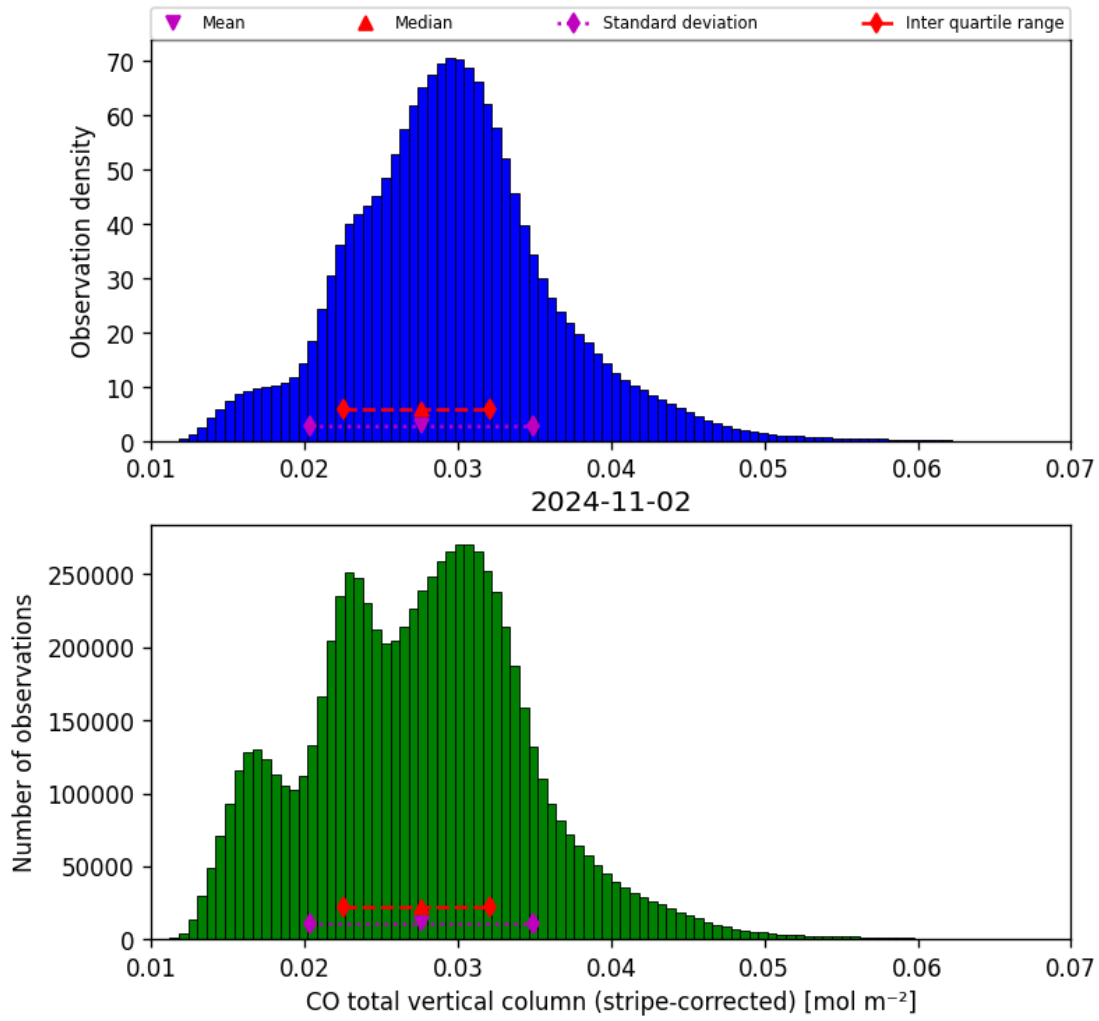
Figure 19: Histogram of “CO total vertical column (stripe-corrected)” for 2024-11-01 to 2024-11-03
