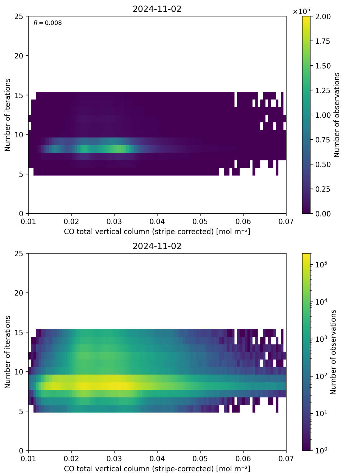
Figure 39: Scatter density plot of “CO total vertical column (stripe-corrected)” against “Number of iterations” for 2024-11-01 to 2024-11-03.
