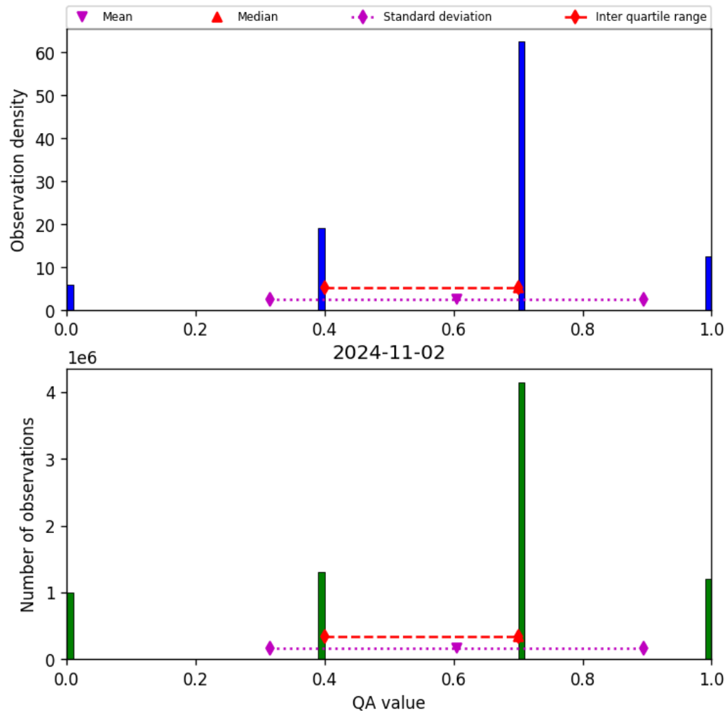
Figure 17: Histogram of “QA value” for 2024-11-01 to 2024-11-03
