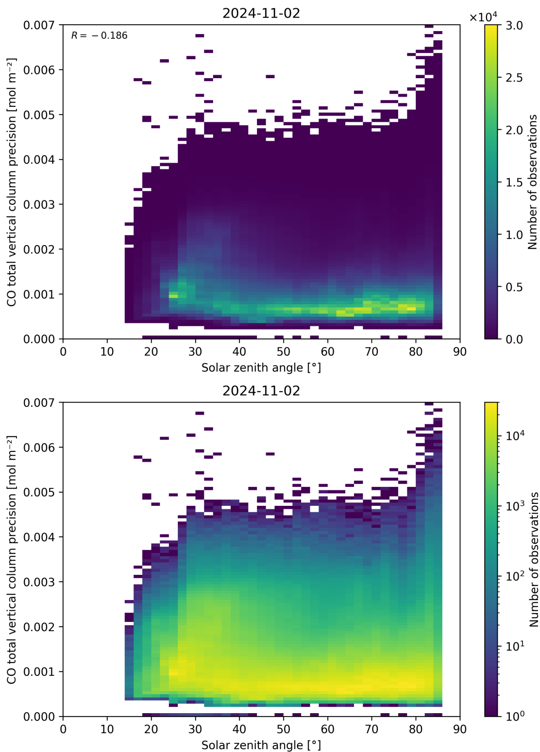
Figure 63: Scatter density plot of “Solar zenith angle” against “CO total vertical column precision” for 2024-11-01 to 2024-11-03.
