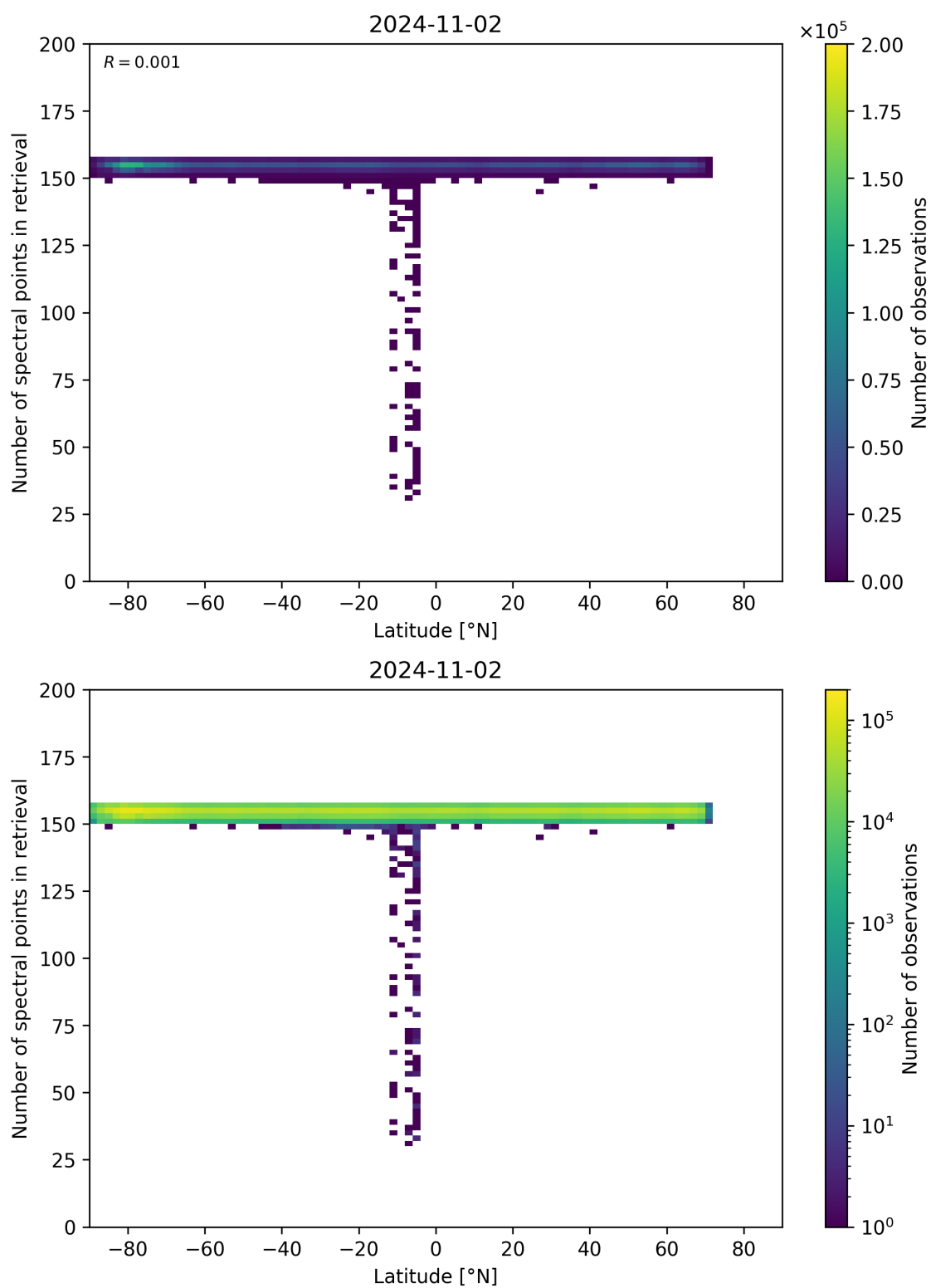
Figure 57: Scatter density plot of “Latitude” against “Number of spectral points in retrieval” for 2024-11-01 to 2024-11-03.
