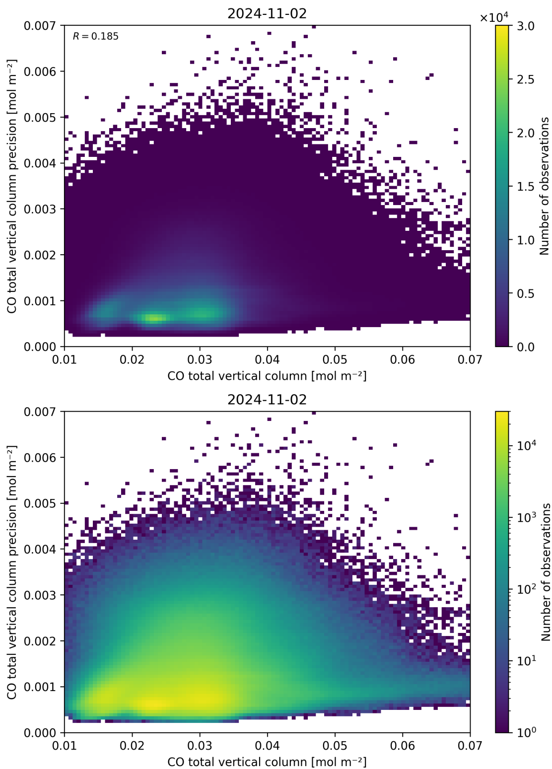
Figure 34: Scatter density plot of “CO total vertical column” against “CO total vertical column precision” for 2024-11-01 to 2024-11-03.
