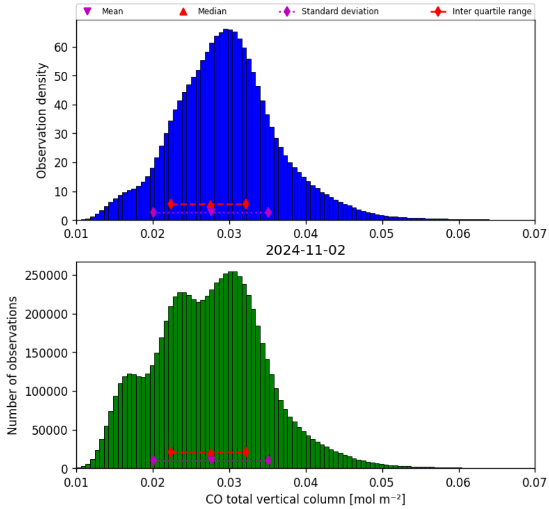
Figure 18: Histogram of “CO total vertical column” for 2024-11-01 to 2024-11-03
