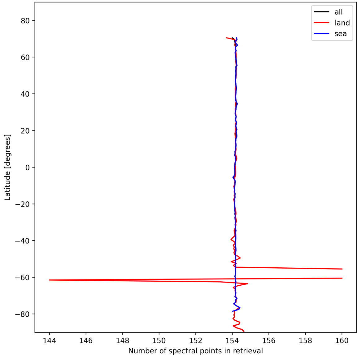
Figure 13: Zonal average of “Number of spectral points in retrieval” for 2024-11-01 to 2024-11-03.
