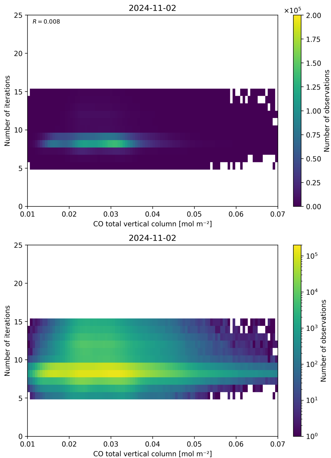
Figure 42: Scatter density plot of “CO total vertical column” against “Number of iterations” for 2024-11-01 to 2024-11-03.
