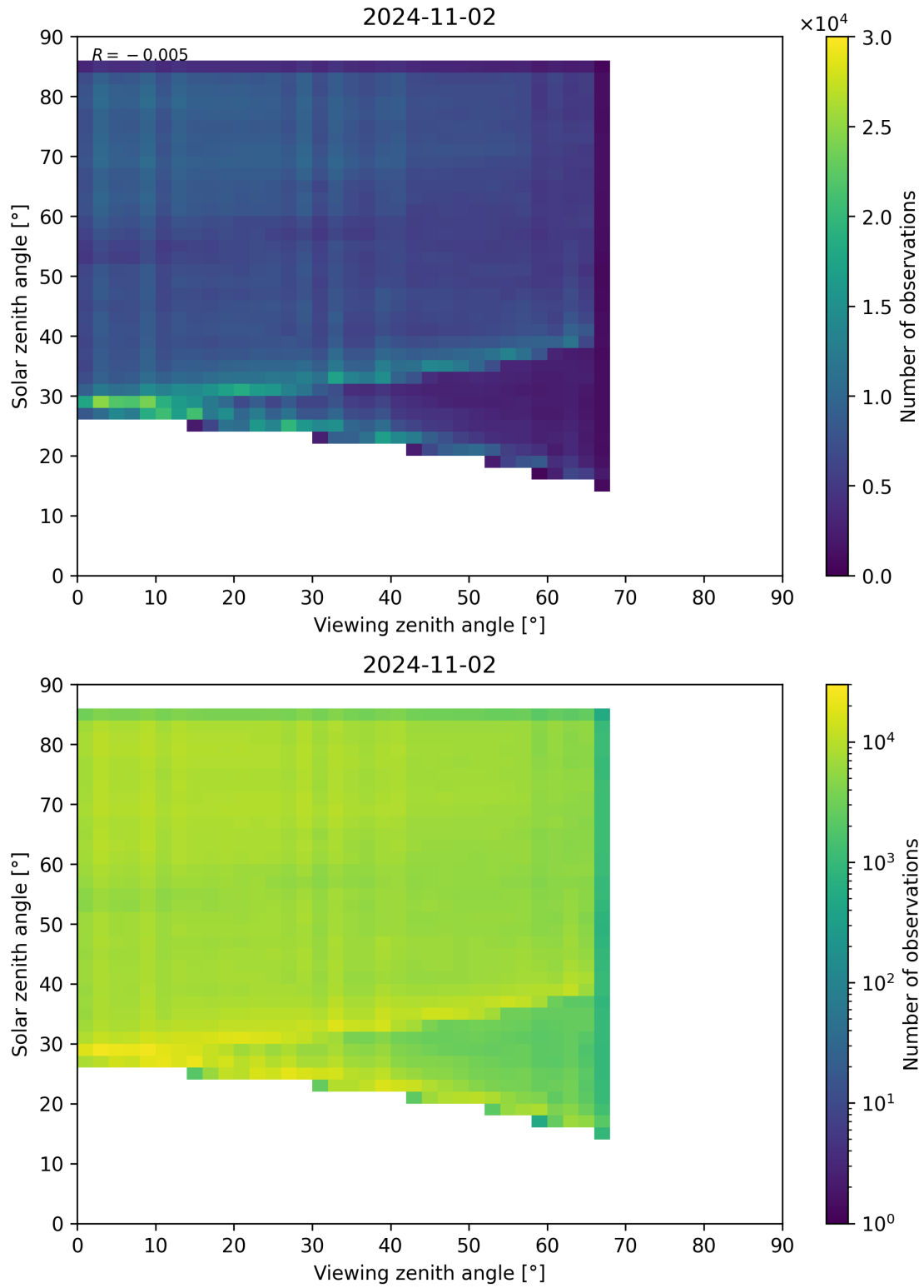
Figure 77: Scatter density plot of “Viewing zenith angle” against “Solar zenith angle” for 2024-11-01 to 2024-11-03.
