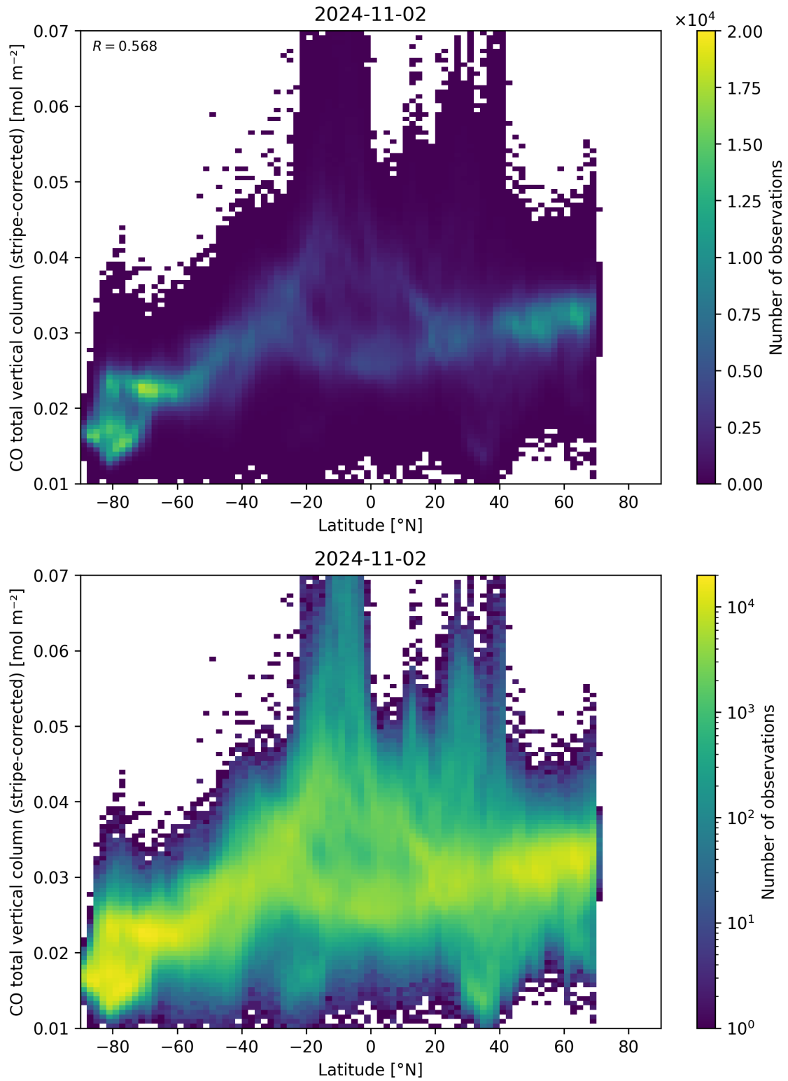
Figure 52: Scatter density plot of “Latitude” against “CO total vertical column (stripe-corrected)” for 2024-11-01 to 2024-11-03.
