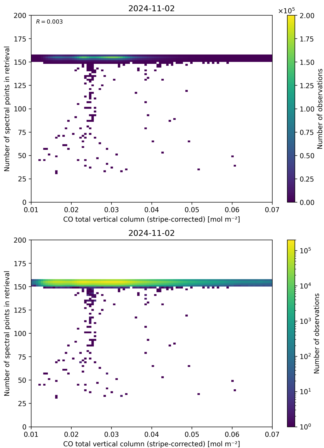
Figure 40: Scatter density plot of “CO total vertical column (stripe-corrected)” against “Number of spectral points in retrieval” for 2024-11-01 to 2024-11-03.
