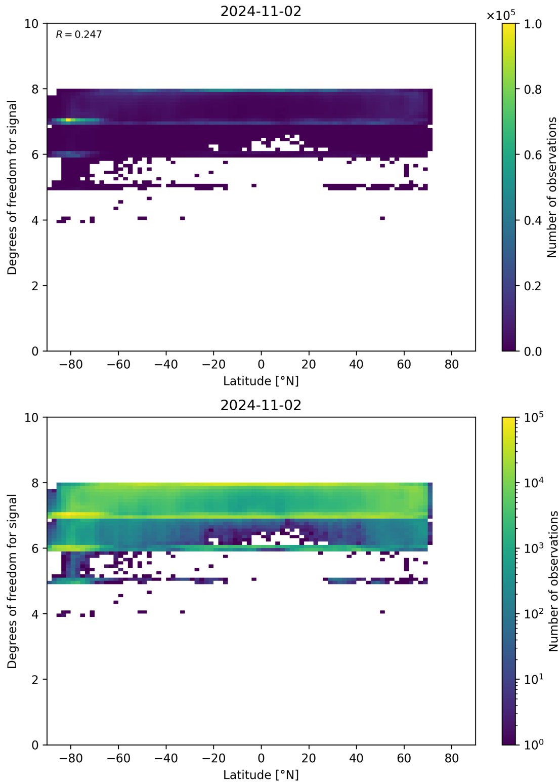
Figure 55: Scatter density plot of “Latitude” against “Degrees of freedom for signal” for 2024-11-01 to 2024-11-03.
