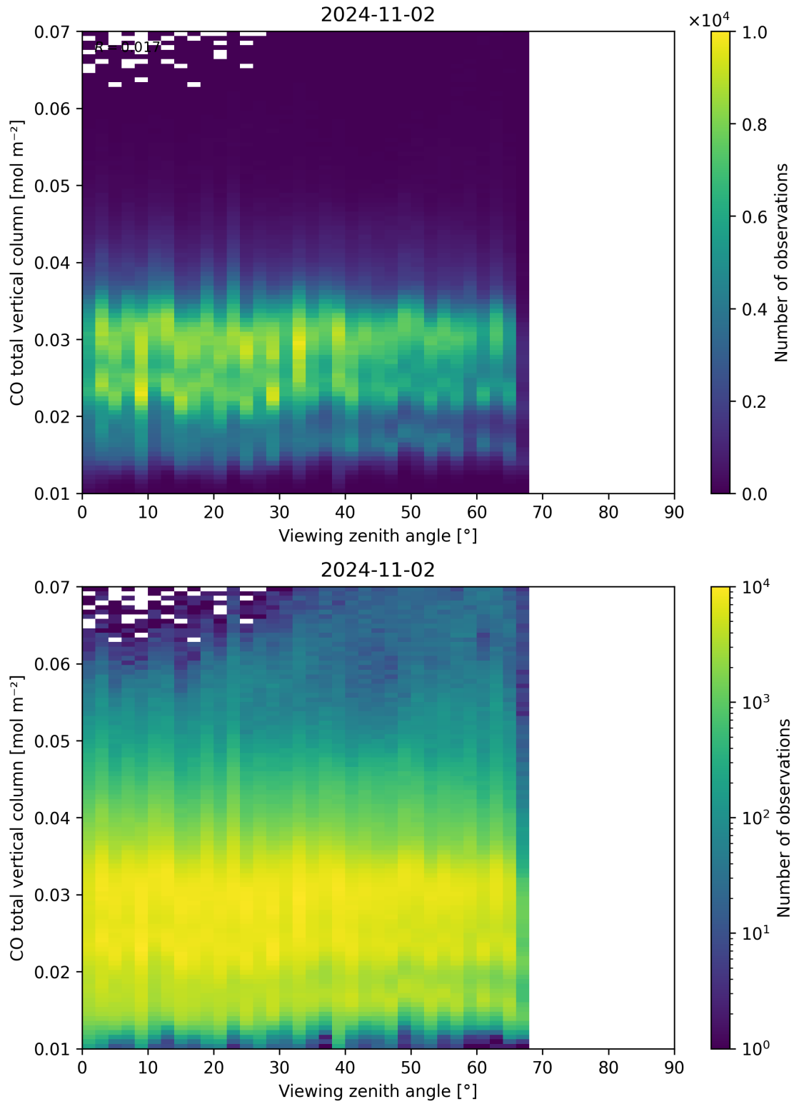
Figure 69: Scatter density plot of “Viewing zenith angle” against “CO total vertical column” for 2024-11-01 to 2024-11-03.
