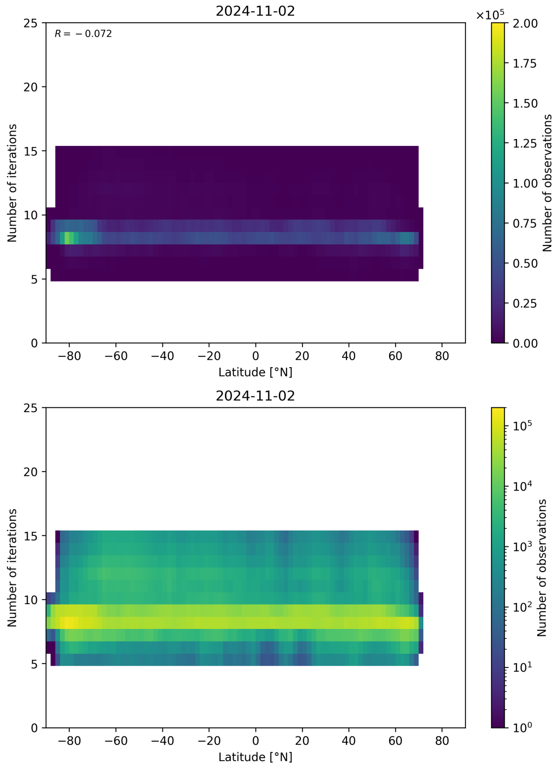
Figure 56: Scatter density plot of “Latitude” against “Number of iterations” for 2024-11-01 to 2024-11-03.
