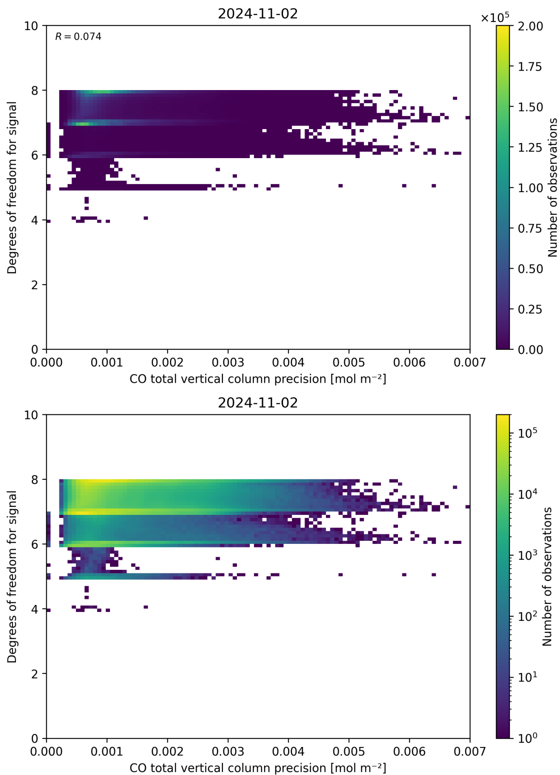
Figure 45: Scatter density plot of “CO total vertical column precision” against “Degrees of freedom for signal” for 2024-11-01 to 2024-11-03.
