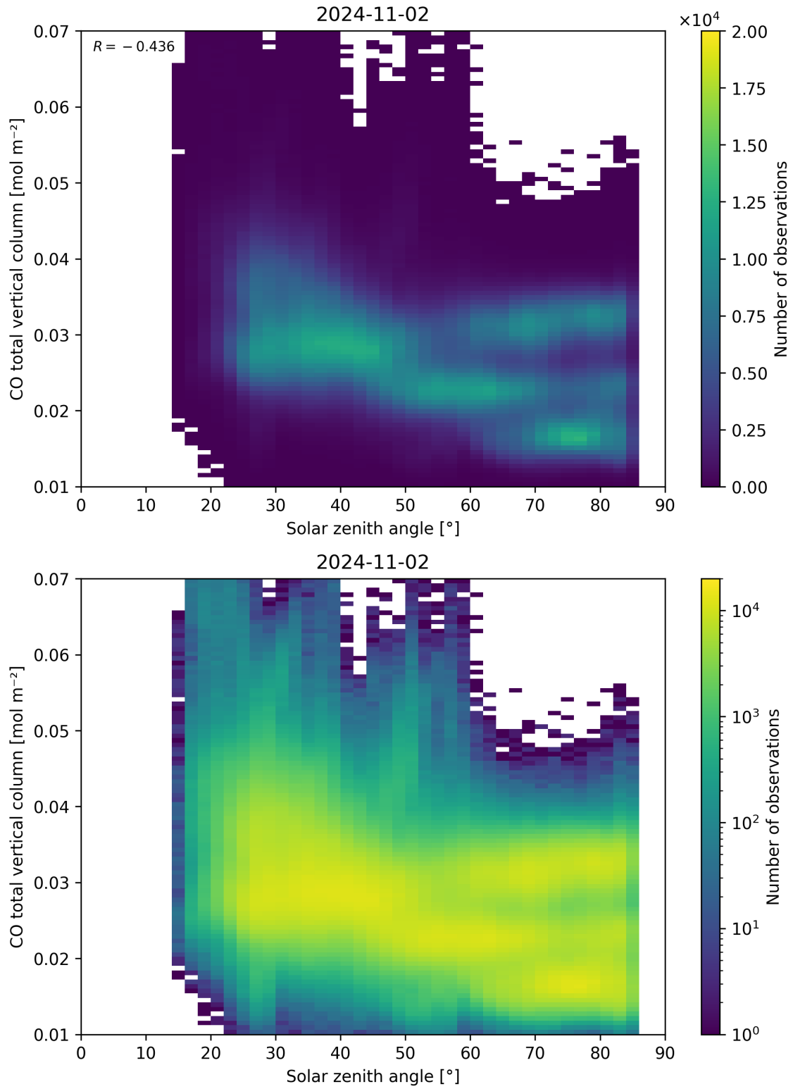
Figure 61: Scatter density plot of “Solar zenith angle” against “CO total vertical column” for 2024-11-01 to 2024-11-03.
