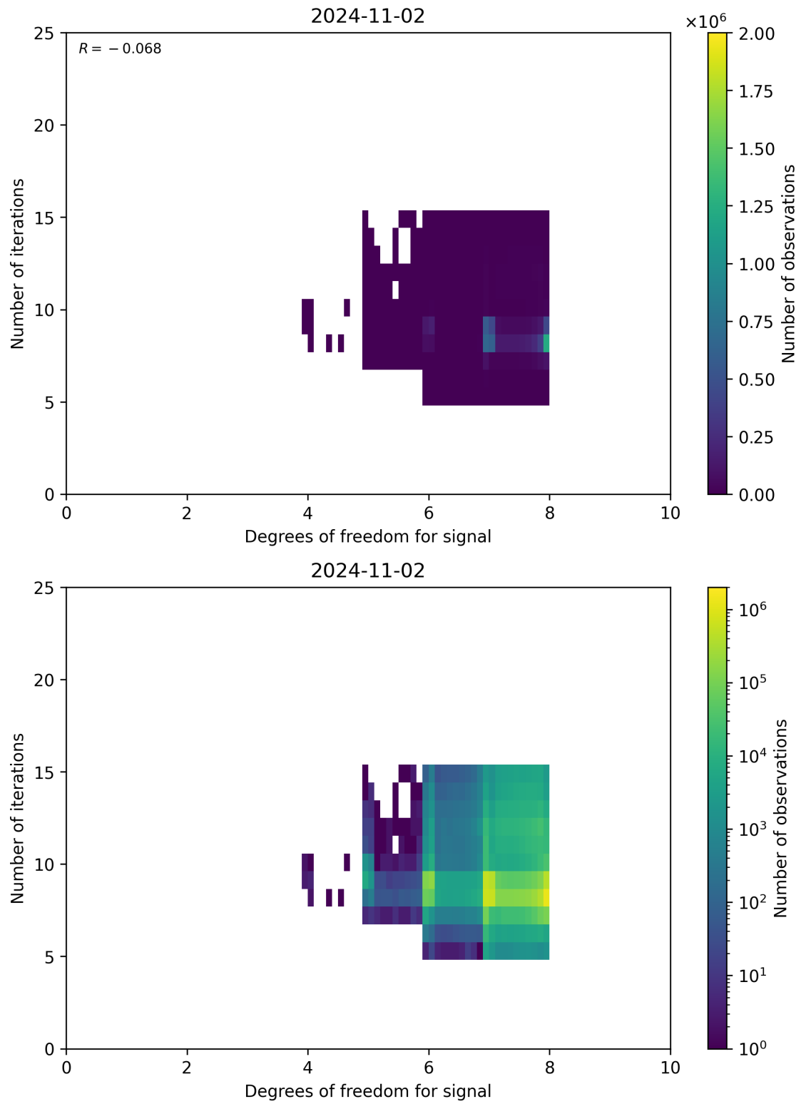
Figure 50: Scatter density plot of “Degrees of freedom for signal” against “Number of iterations” for 2024-11-01 to 2024-11-03.
