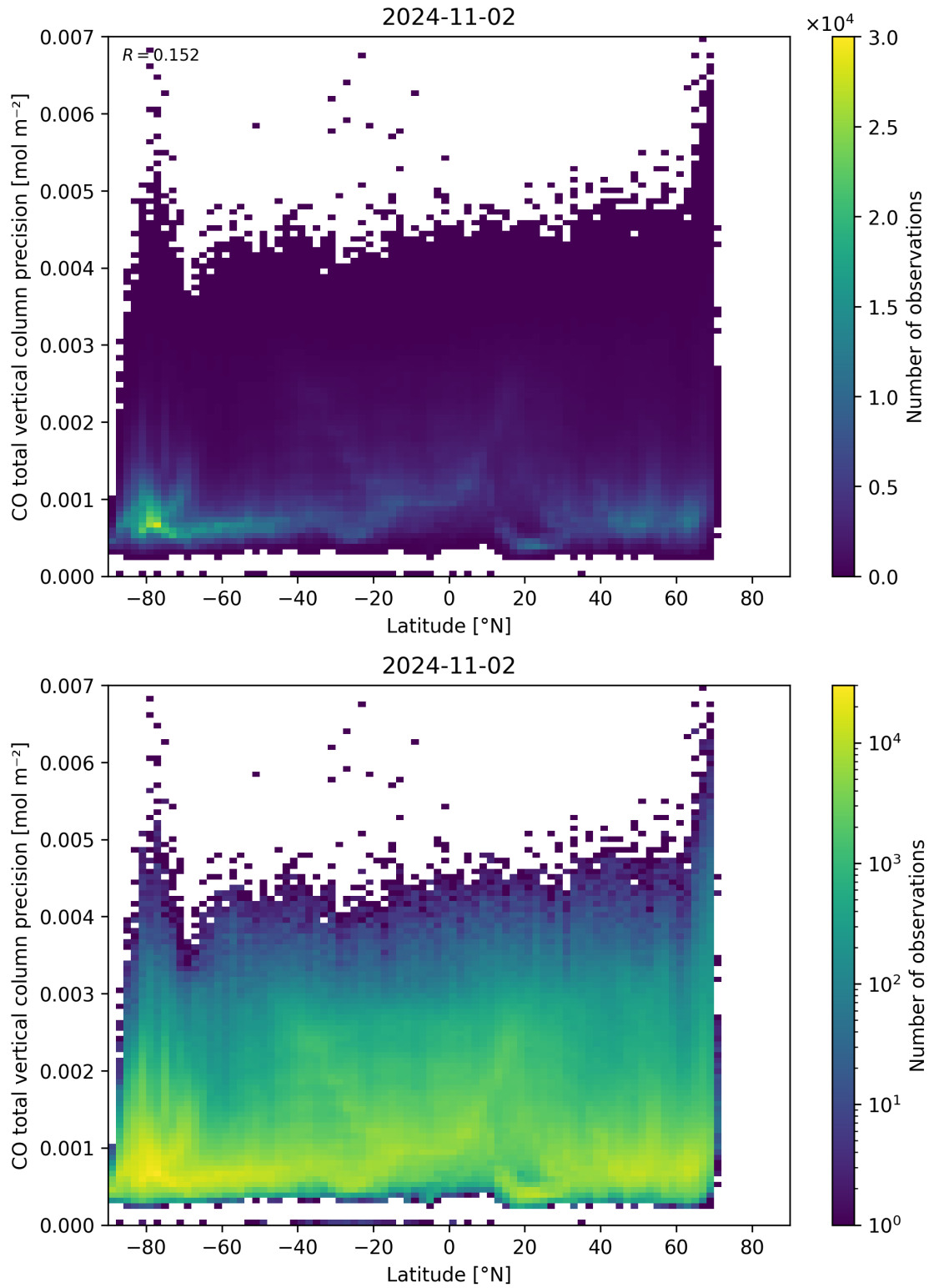
Figure 53: Scatter density plot of “Latitude” against “CO total vertical column precision” for 2024-11-01 to 2024-11-03.
