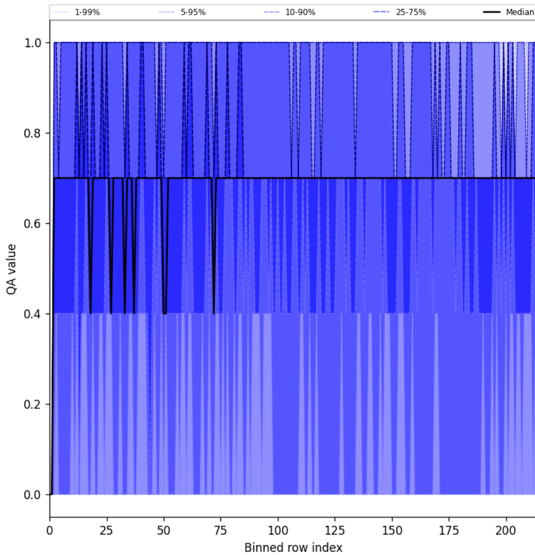
Figure 25: Along track statistics of “QA value” for 2024-11-01 to 2024-11-03
