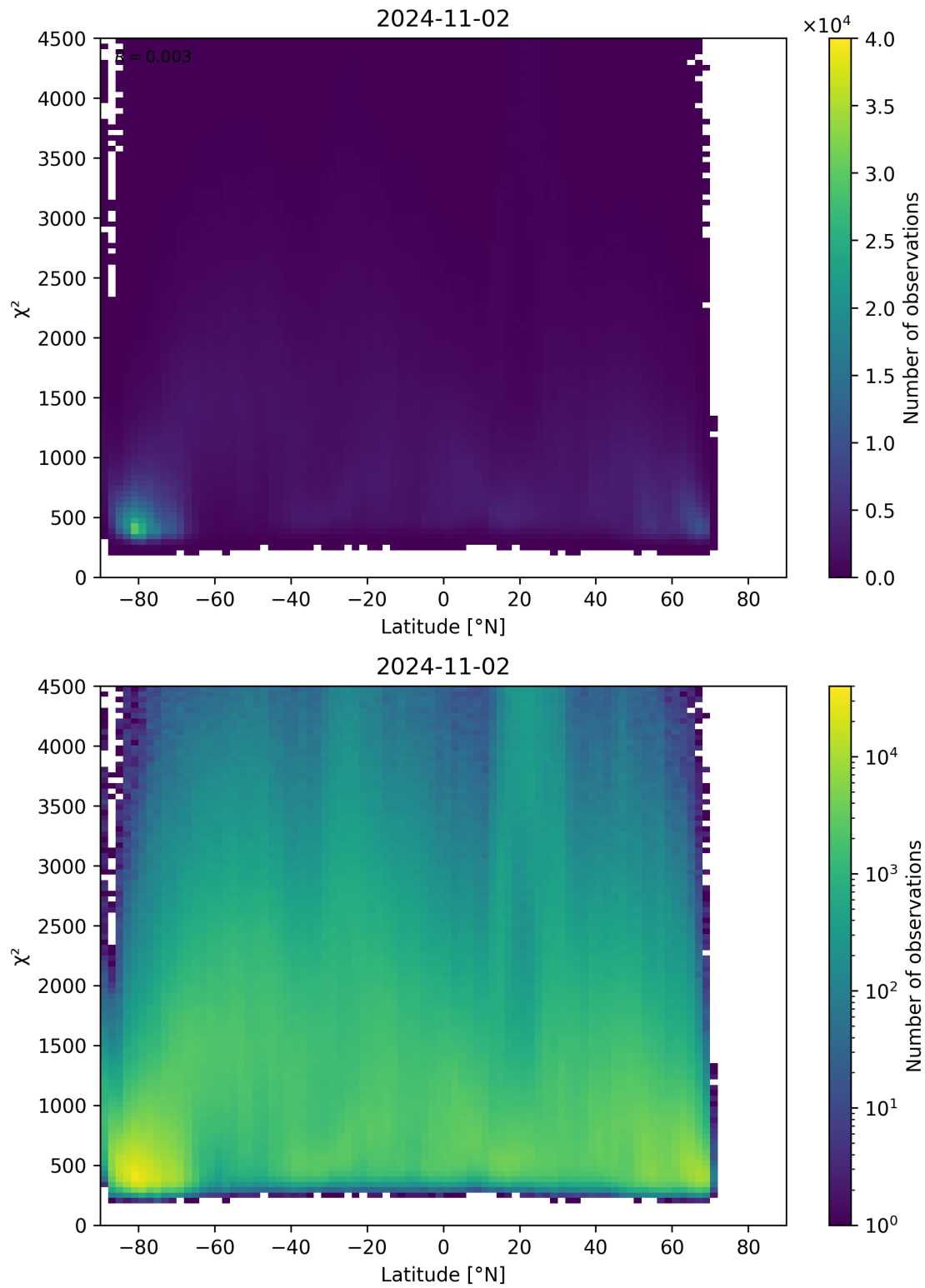
Figure 54: Scatter density plot of “Latitude” against “ \chi^2 ” for 2024-11-01 to 2024-11-03.
