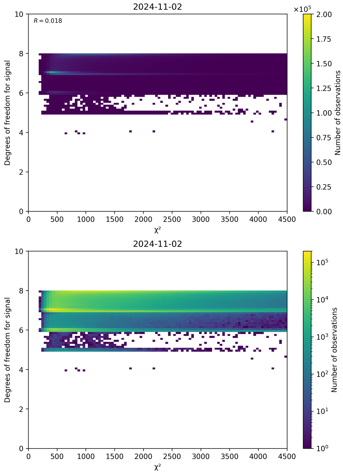
Figure 48: Scatter density plot of “ \chi^2 ” against “Degrees of freedom for signal” for 2024-11-01 to 2024-11-03.
