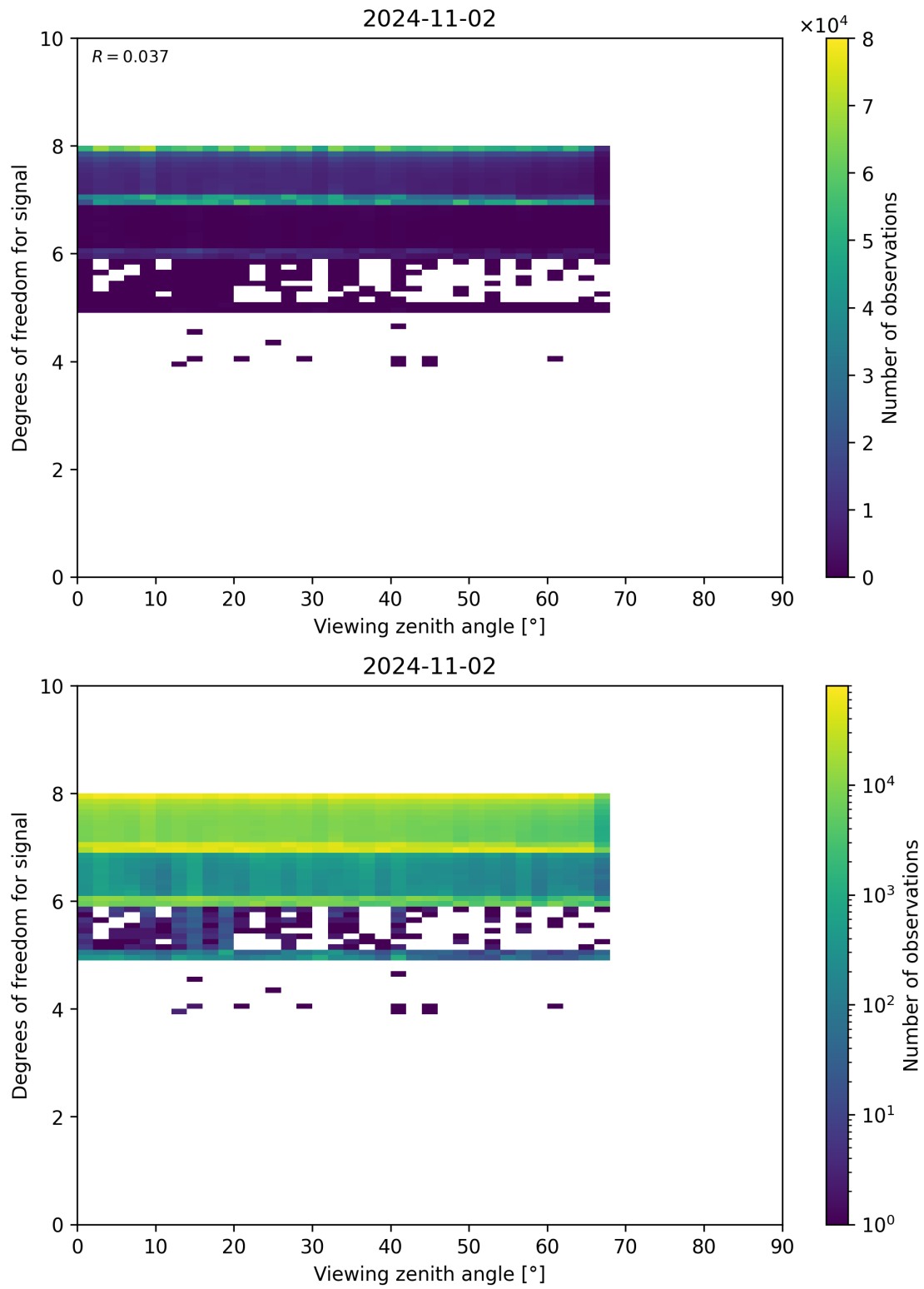
Figure 73: Scatter density plot of “Viewing zenith angle” against “Degrees of freedom for signal” for 2024-11-01 to 2024-11-03.
