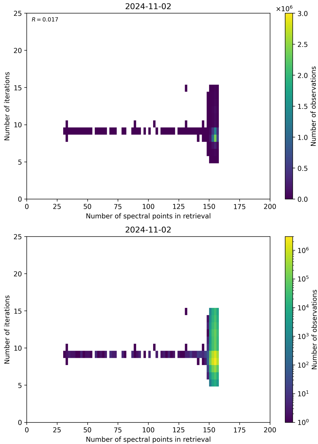
Figure 60: Scatter density plot of “Number of spectral points in retrieval” against “Number of iterations” for 2024-11-01 to 2024-11-03.
