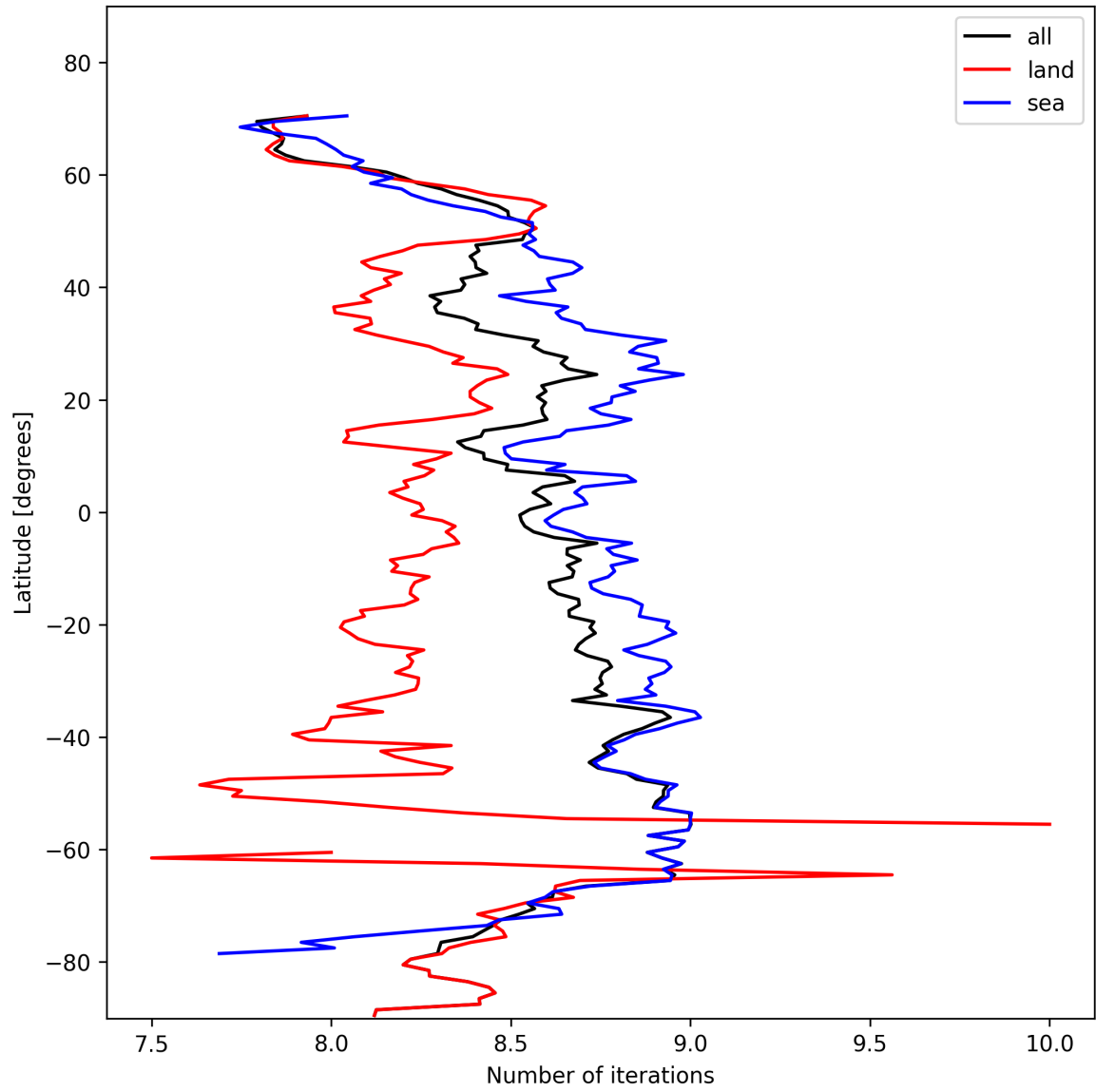
Figure 16: Zonal average of “Number of iterations” for 2024-11-01 to 2024-11-03.
