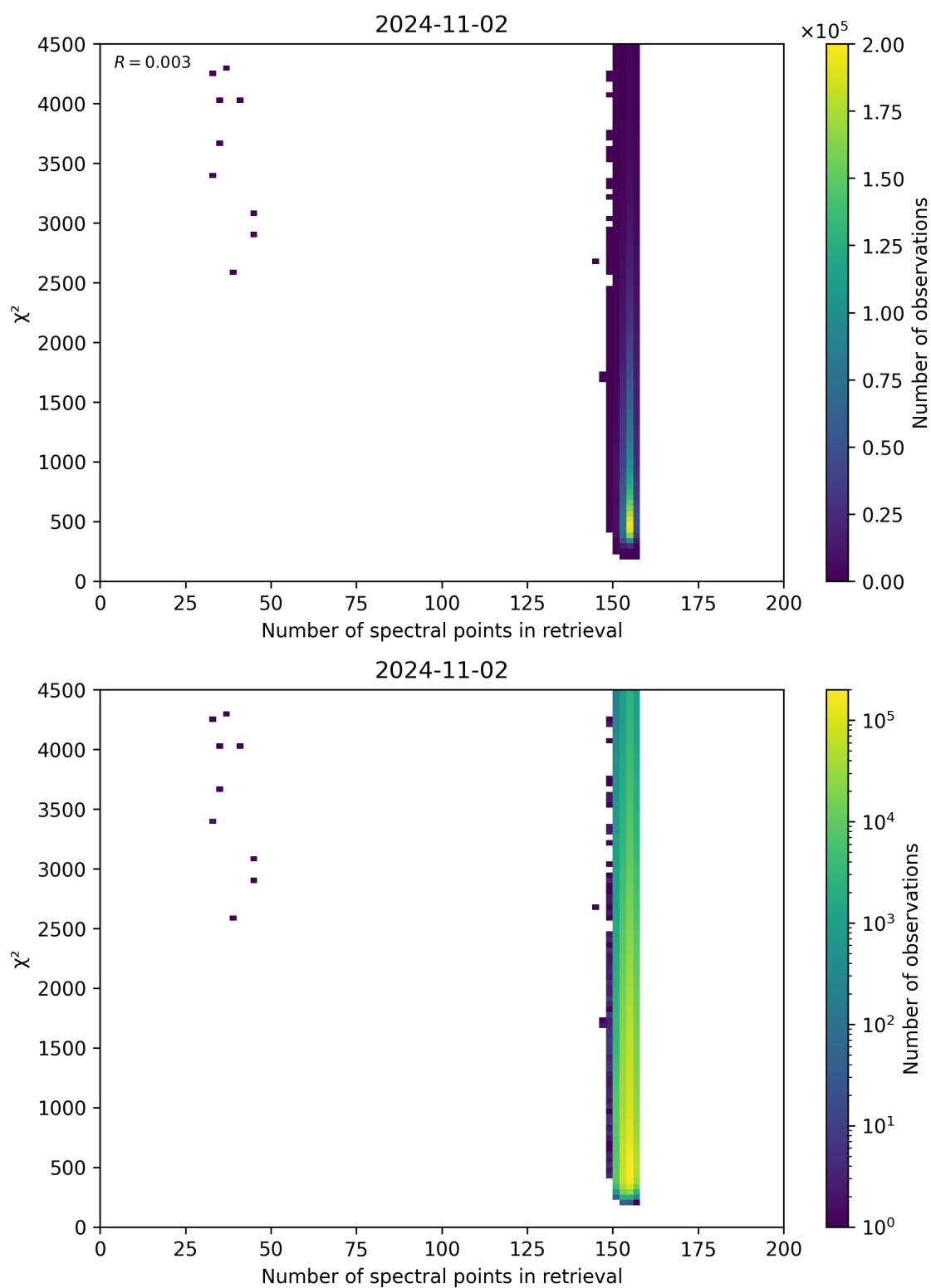
Figure 58: Scatter density plot of “Number of spectral points in retrieval” against “ \chi^2 ” for 2024-11-01 to 2024-11-03.
