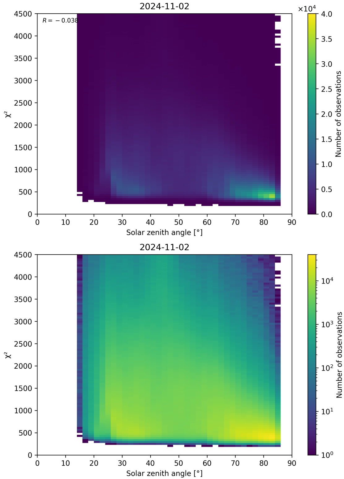
Figure 64: Scatter density plot of “Solar zenith angle” against “ \chi^2 ” for 2024-11-01 to 2024-11-03.
