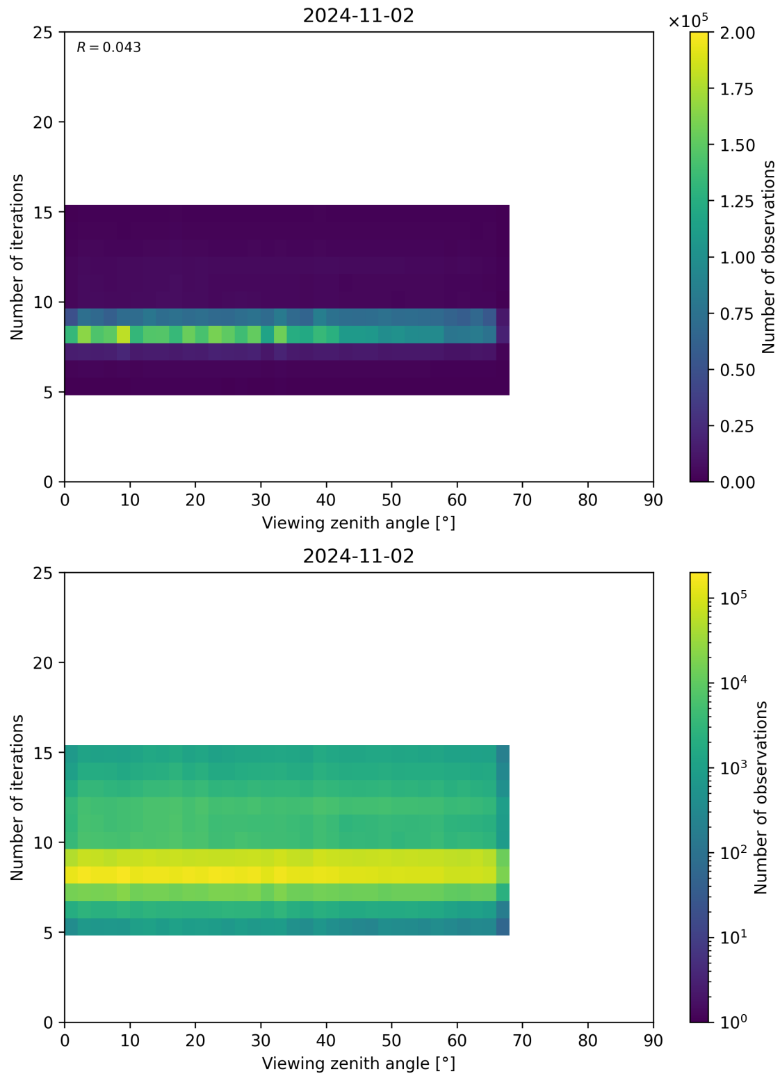
Figure 75: Scatter density plot of “Viewing zenith angle” against “Number of iterations” for 2024-11-01 to 2024-11-03.
