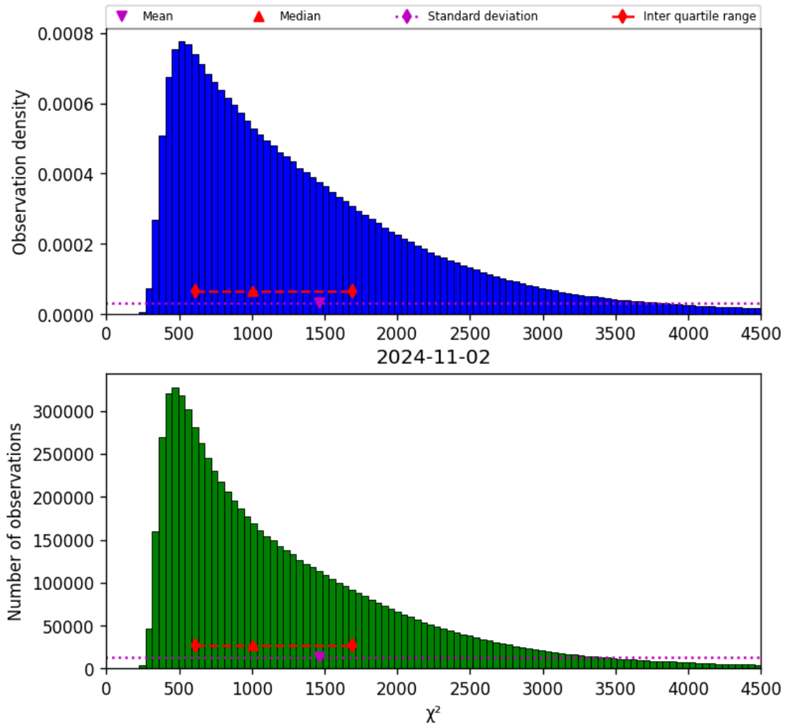
Figure 22: Histogram of “ \chi^2 ” for 2024-11-01 to 2024-11-03
