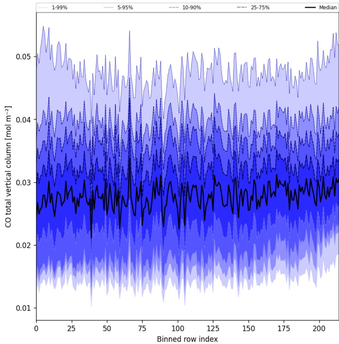
Figure 26: Along track statistics of “CO total vertical column” for 2024-11-01 to 2024-11-03
