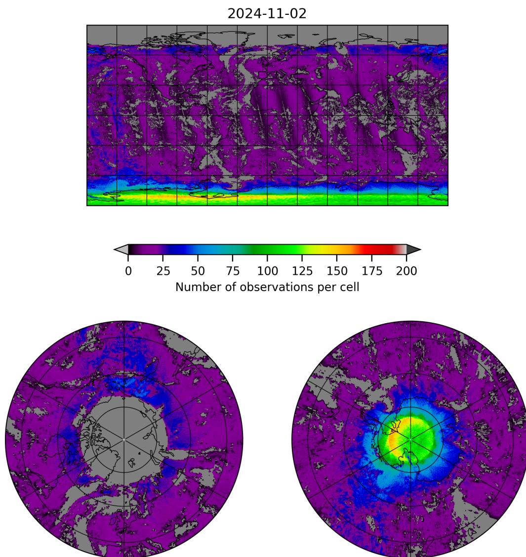
Figure 8: Map of the number of observations for 2024-11-01 to 2024-11-03
