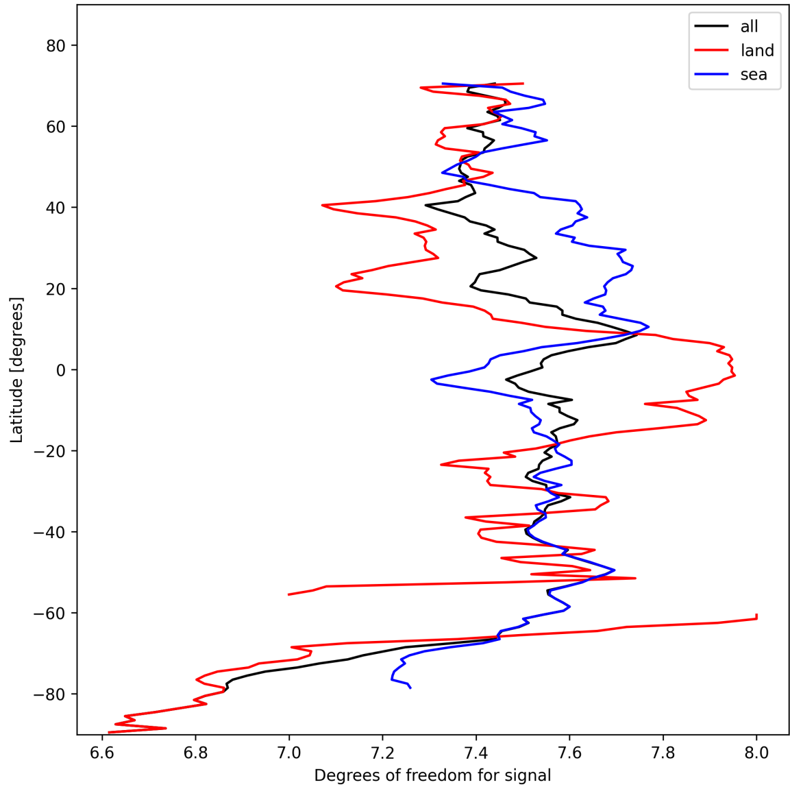
Figure 15: Zonal average of “Degrees of freedom for signal” for 2024-11-01 to 2024-11-03.
