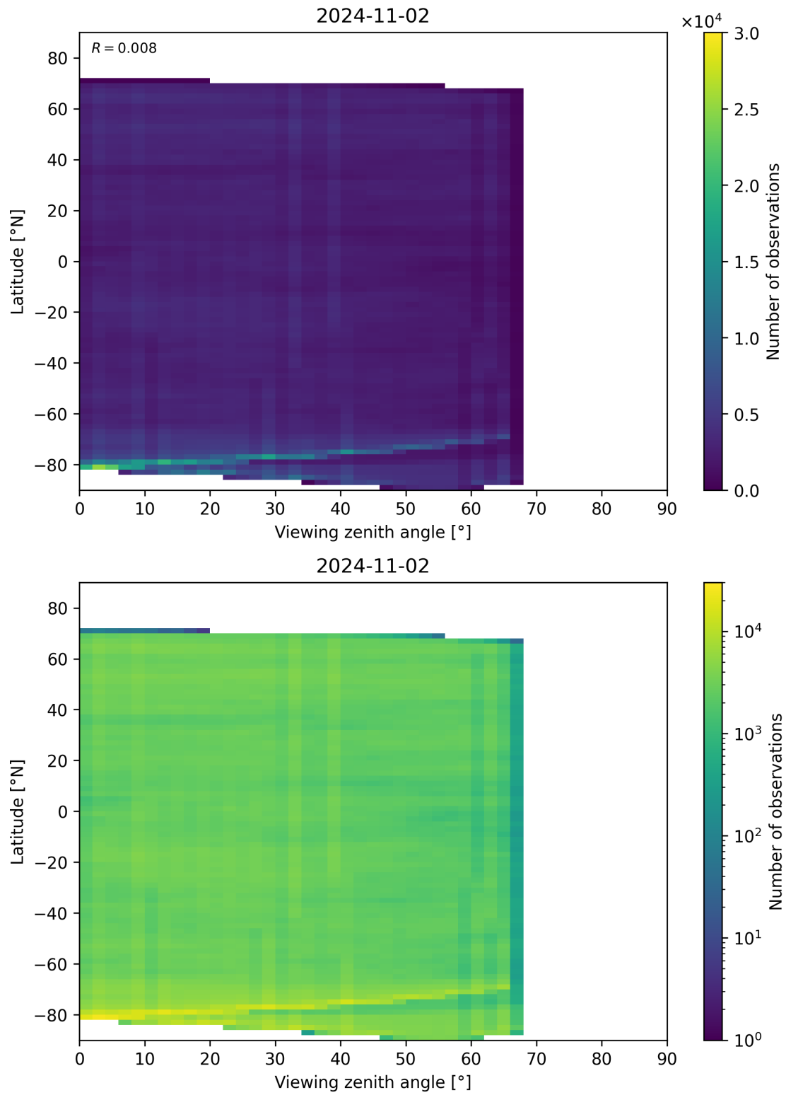
Figure 74: Scatter density plot of “Viewing zenith angle” against “Latitude” for 2024-11-01 to 2024-11-03.
