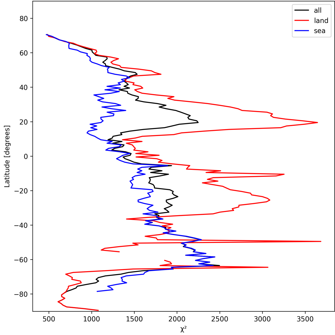
Figure 14: Zonal average of “ \chi^2 ” for 2024-11-01 to 2024-11-03.
