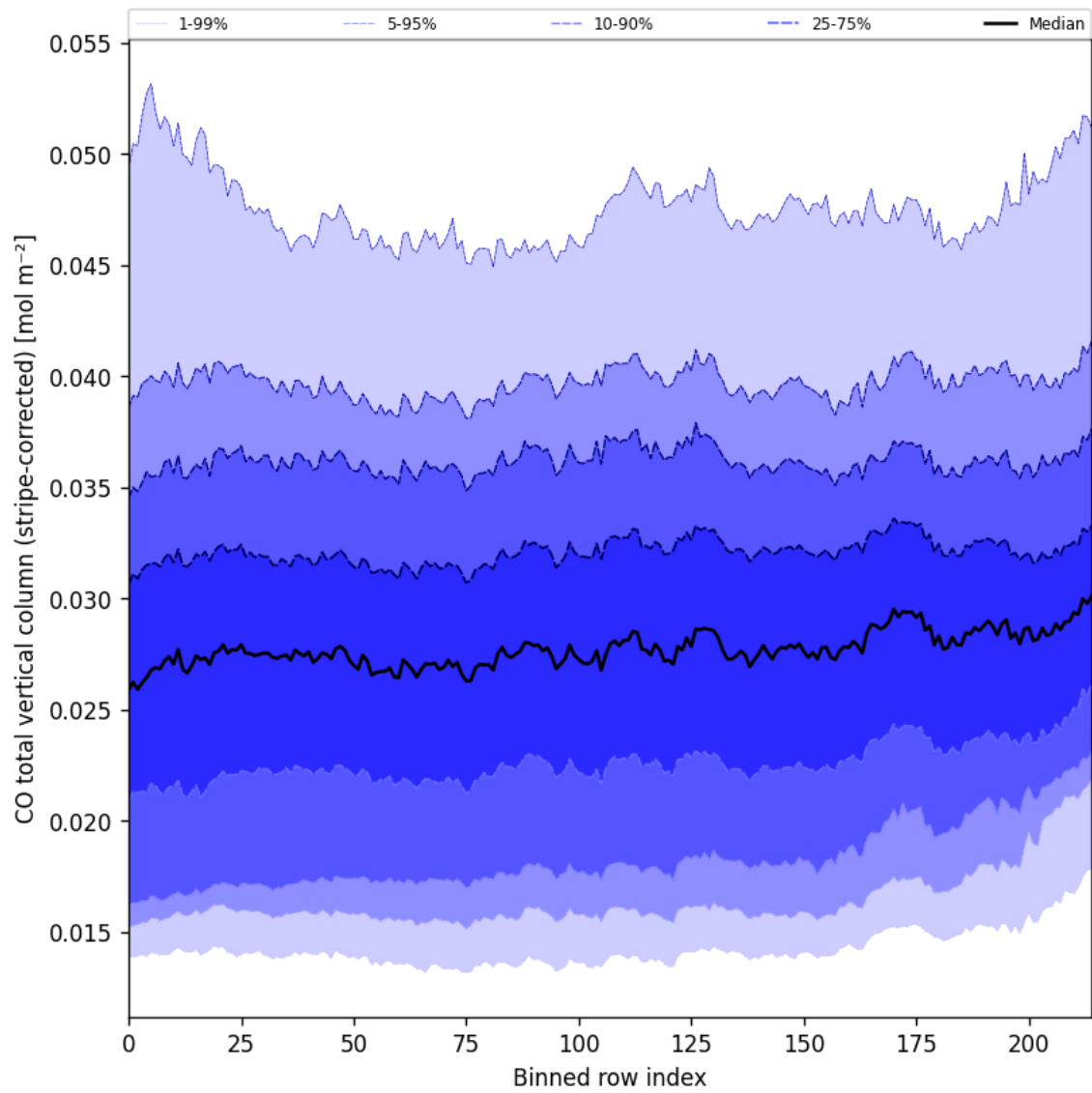
Figure 27: Along track statistics of "CO total vertical column (stripe-corrected)" for 2024-11-01 to 2024-11-03
