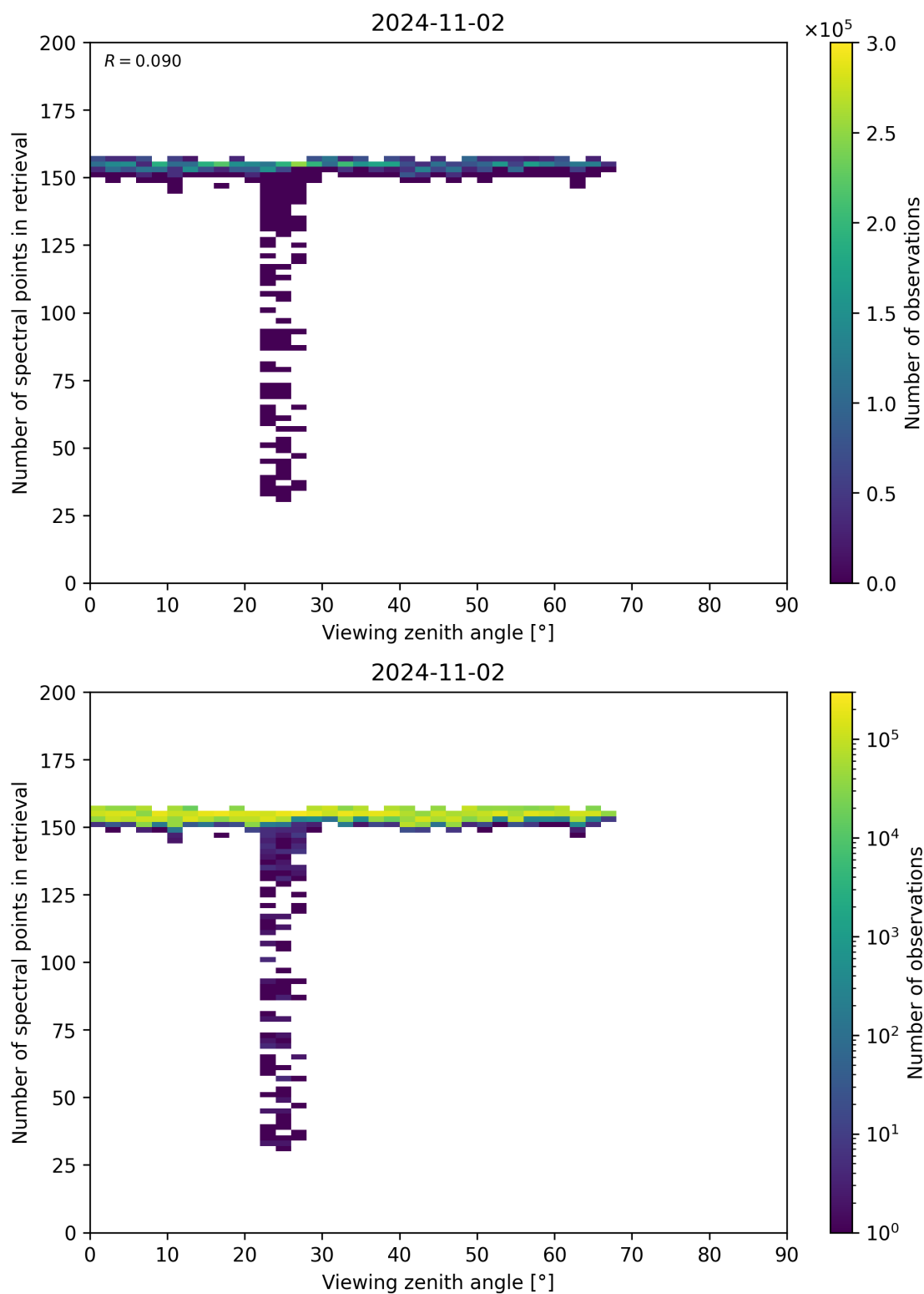
Figure 76: Scatter density plot of “Viewing zenith angle” against “Number of spectral points in retrieval” for 2024-11-01 to 2024-11-03.
