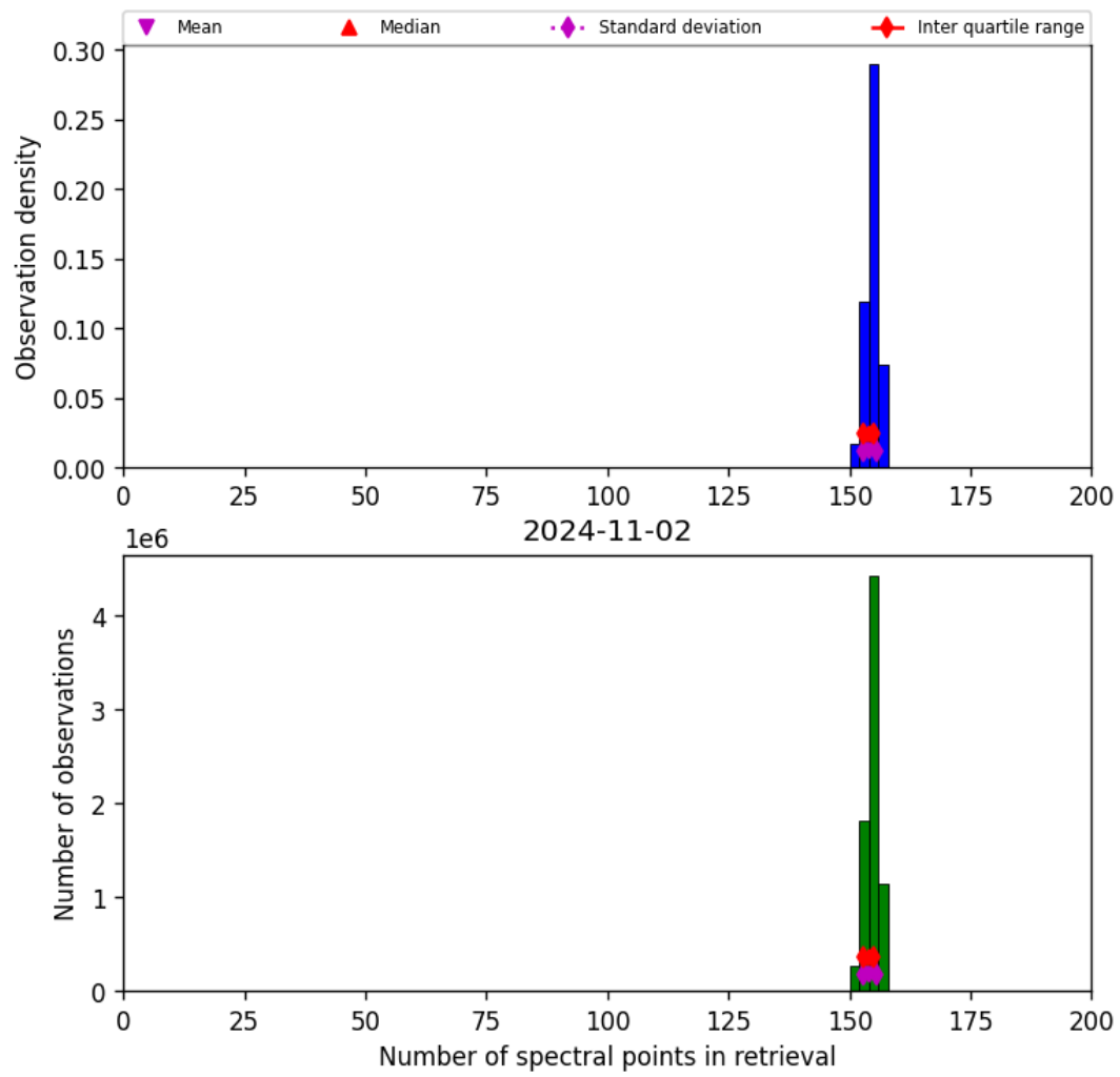
Figure 21: Histogram of “Number of spectral points in retrieval” for 2024-11-01 to 2024-11-03
