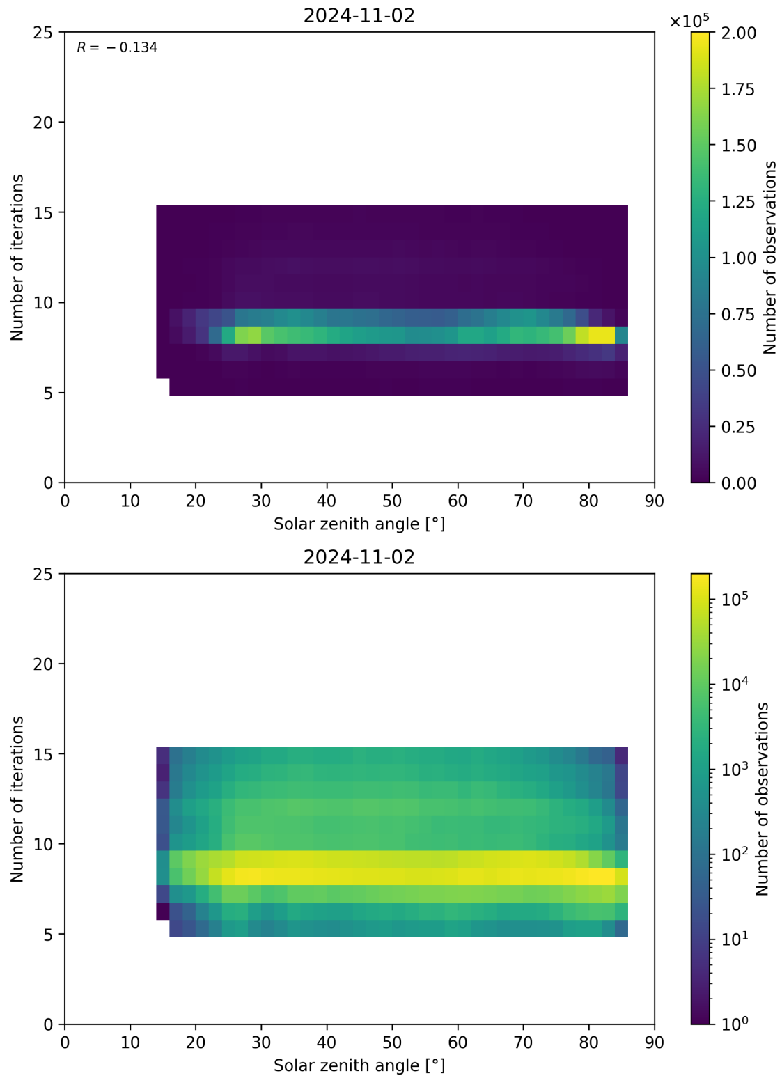
Figure 67: Scatter density plot of “Solar zenith angle” against “Number of iterations” for 2024-11-01 to 2024-11-03.
