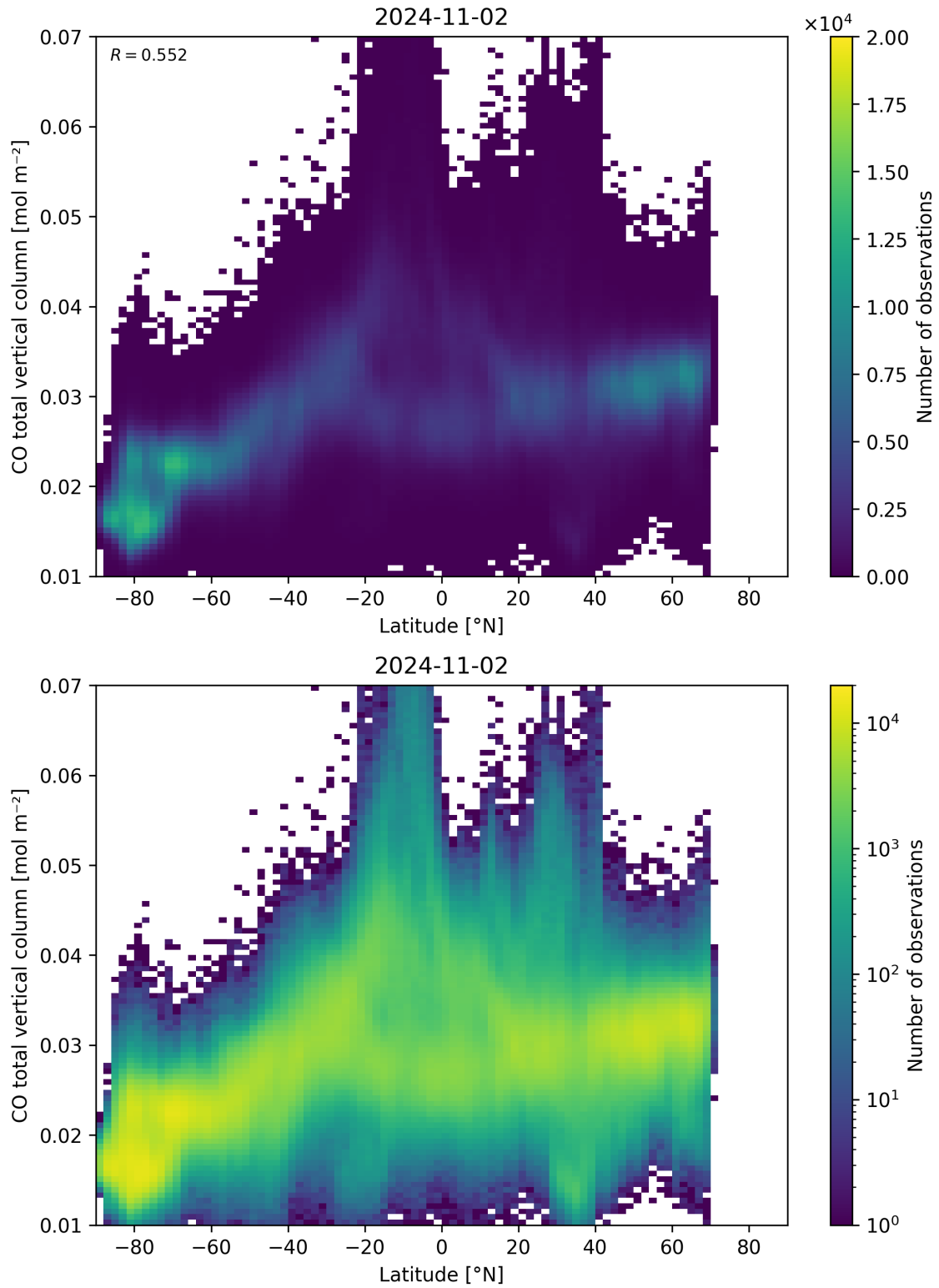
Figure 51: Scatter density plot of “Latitude” against “CO total vertical column” for 2024-11-01 to 2024-11-03.
