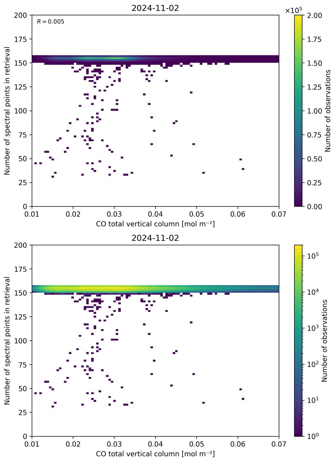
Figure 43: Scatter density plot of “CO total vertical column” against “Number of spectral points in retrieval” for 2024-11-01 to 2024-11-03.
