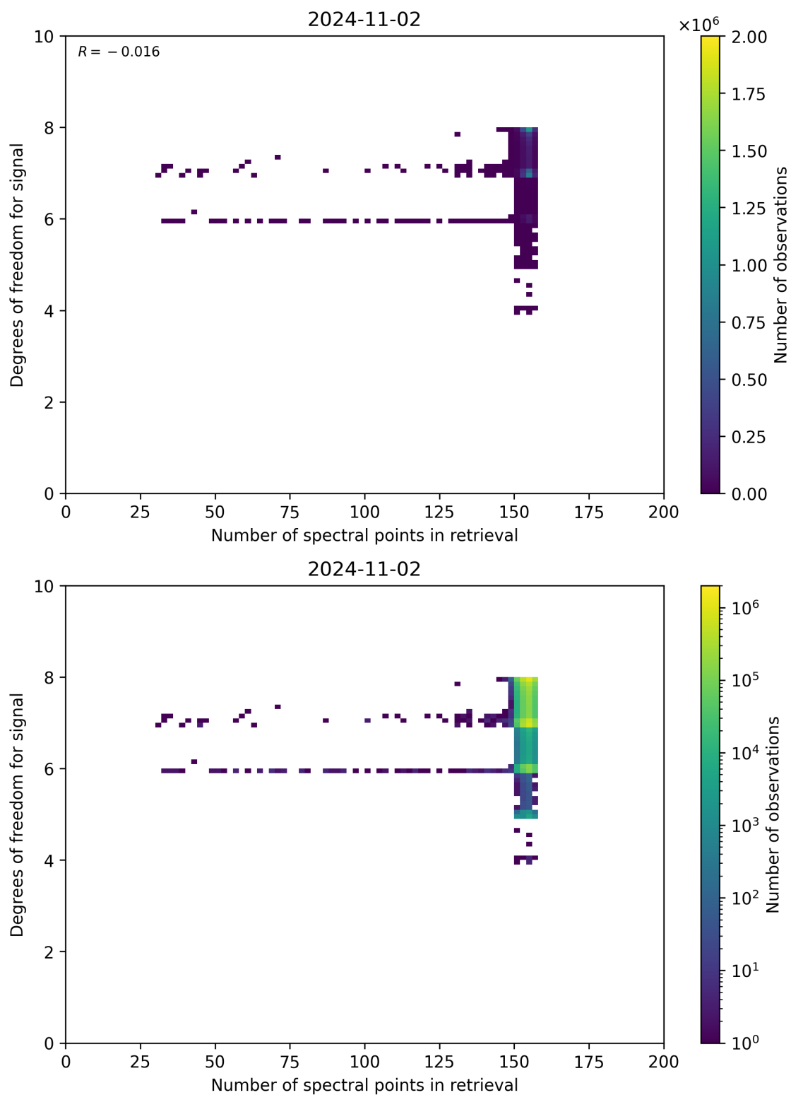
Figure 59: Scatter density plot of “Number of spectral points in retrieval” against “Degrees of freedom for signal” for 2024-11-01 to 2024-11-03.
