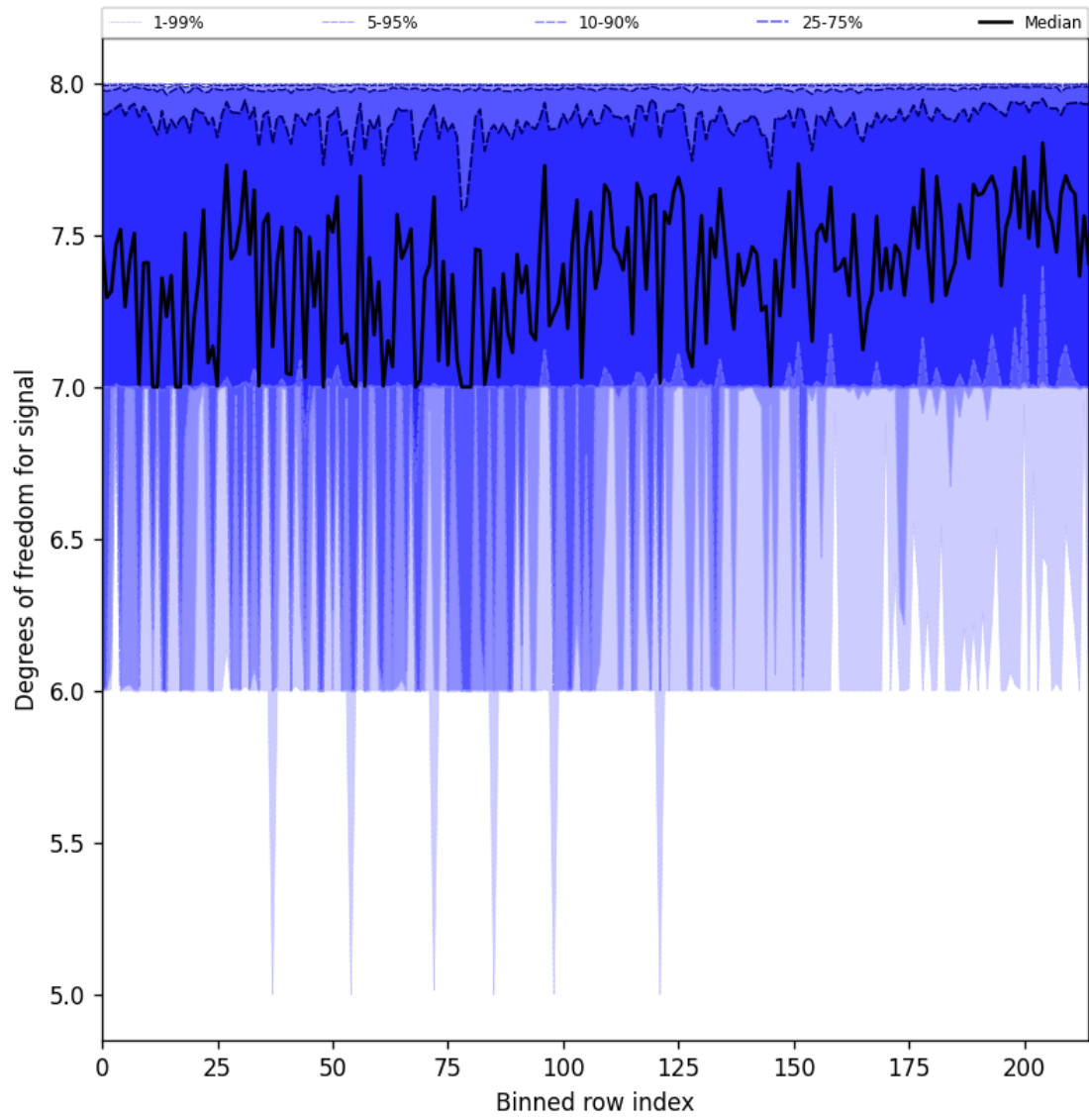
Figure 31: Along track statistics of “Degrees of freedom for signal” for 2024-11-01 to 2024-11-03
