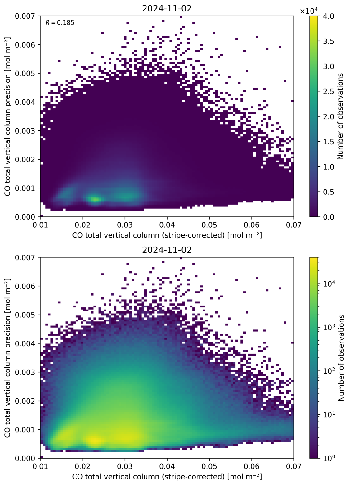
Figure 36: Scatter density plot of “CO total vertical column (stripe-corrected)” against “CO total vertical column precision” for 2024-11-01 to 2024-11-03.
