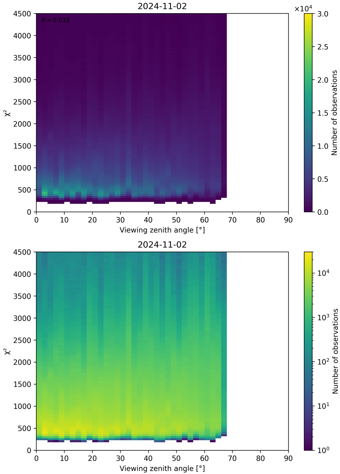
Figure 72: Scatter density plot of “Viewing zenith angle” against “ \chi^2 ” for 2024-11-01 to 2024-11-03.
