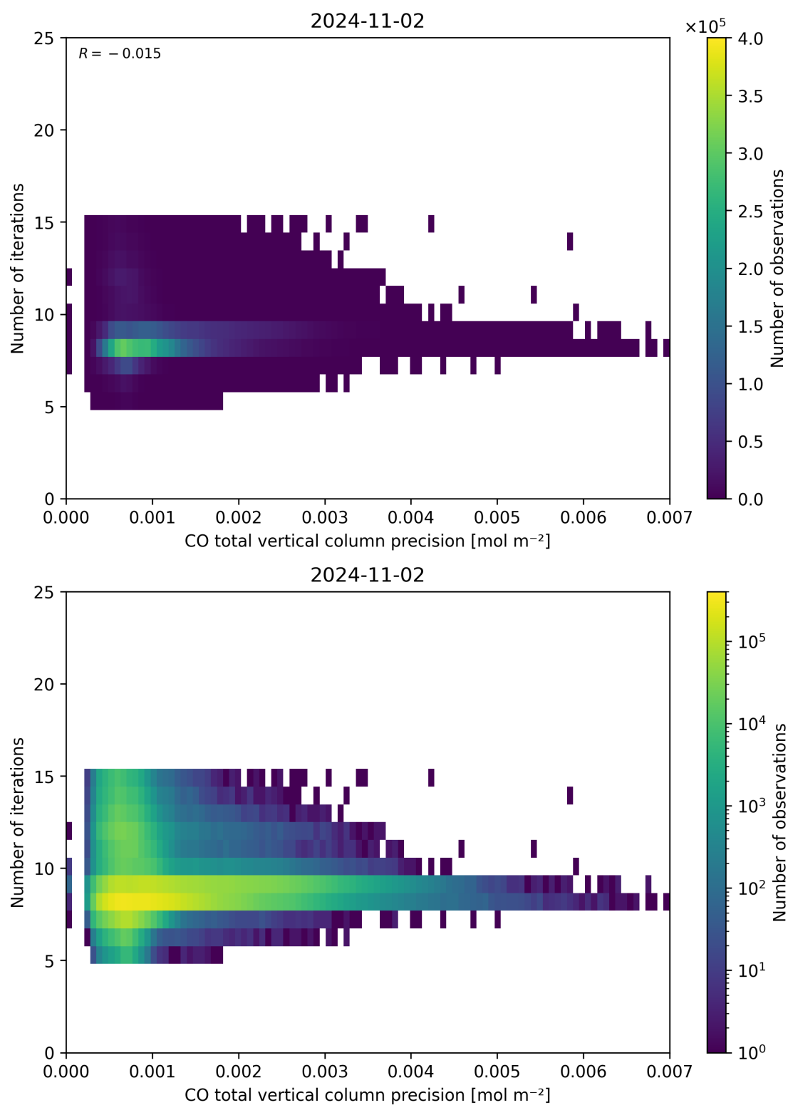
Figure 46: Scatter density plot of “CO total vertical column precision” against “Number of iterations” for 2024-11-01 to 2024-11-03.
