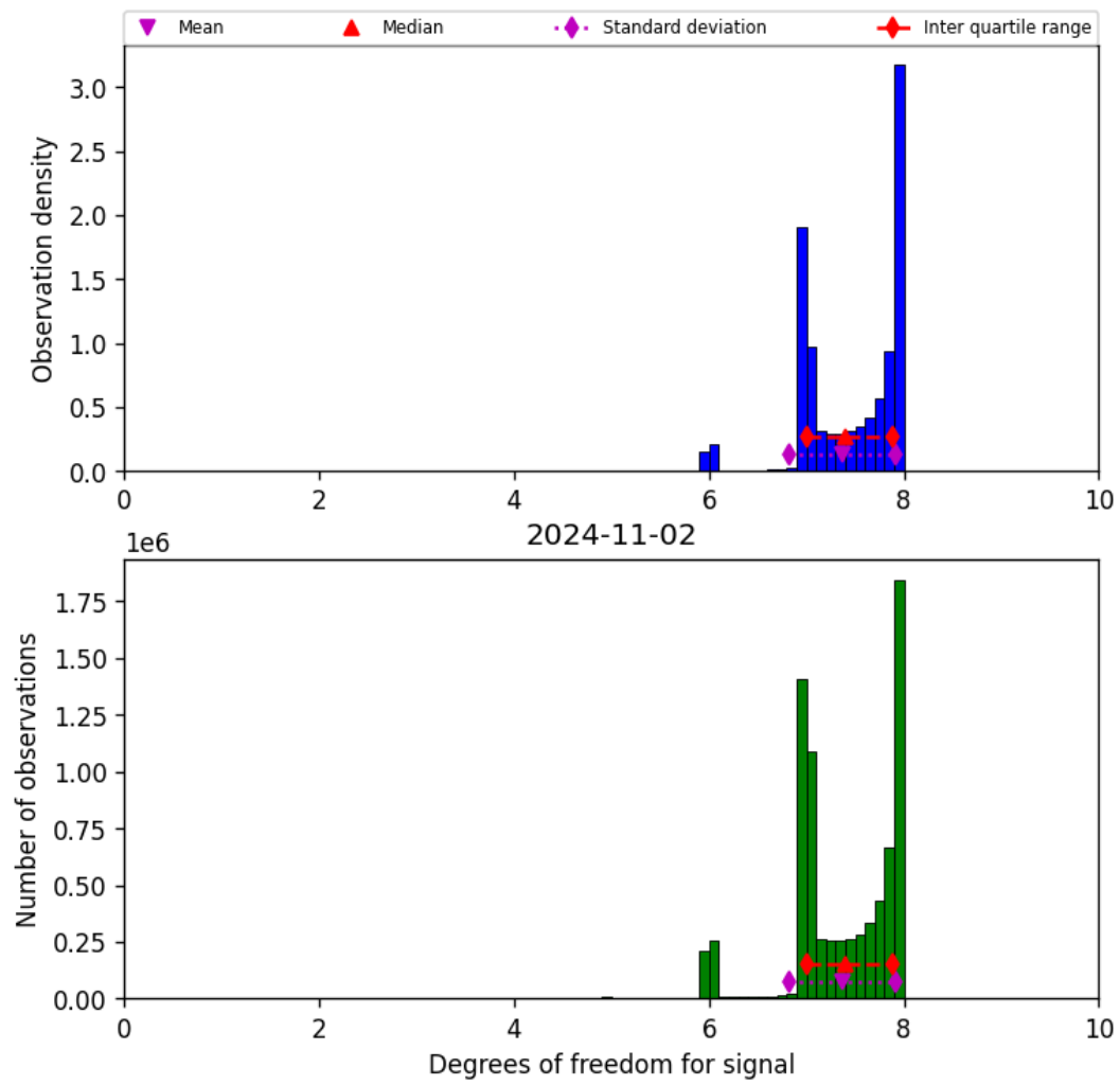
Figure 23: Histogram of “Degrees of freedom for signal” for 2024-11-01 to 2024-11-03
