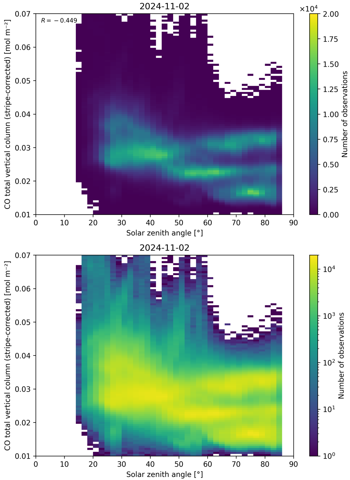
Figure 62: Scatter density plot of “Solar zenith angle” against “CO total vertical column (stripe-corrected)” for 2024-11-01 to 2024-11-03.
