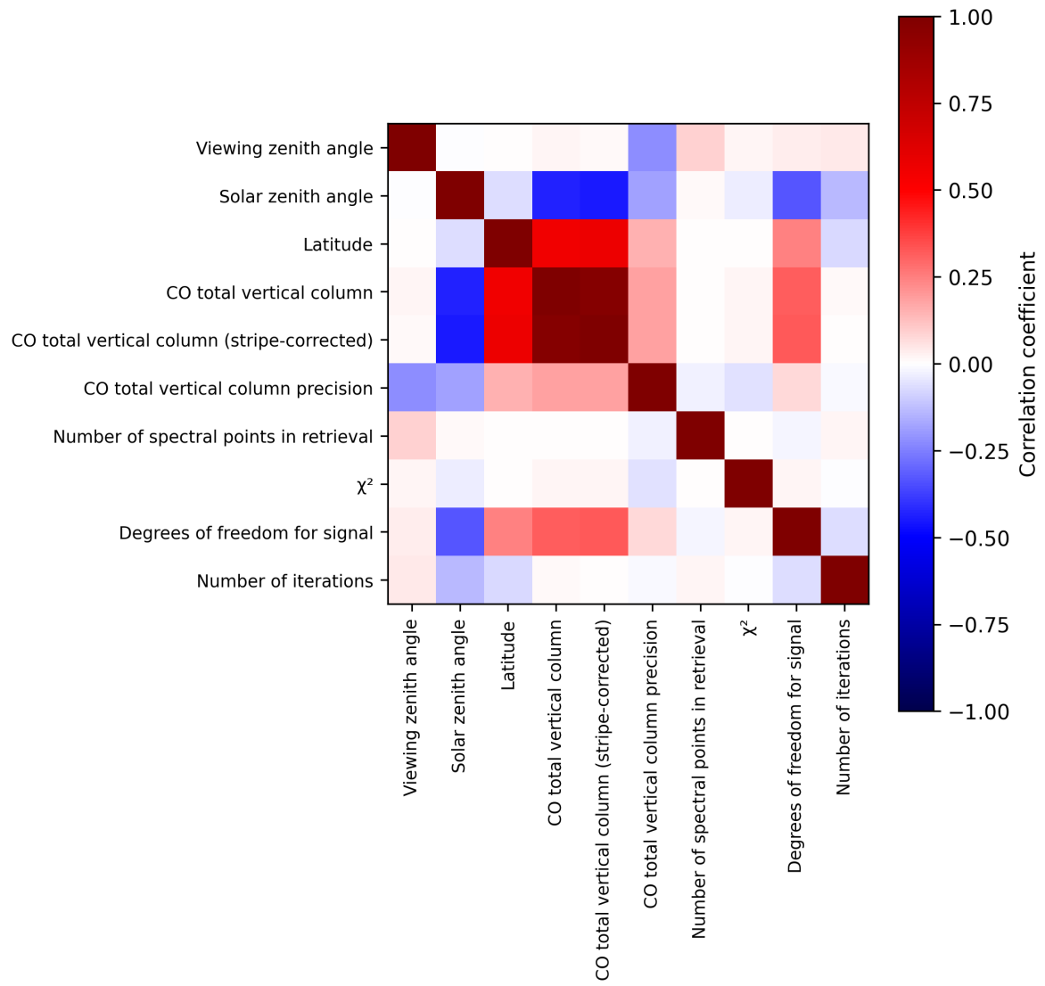
Figure 2: Map of correlation matrix for 2024-11-01 to 2024-11-03.
