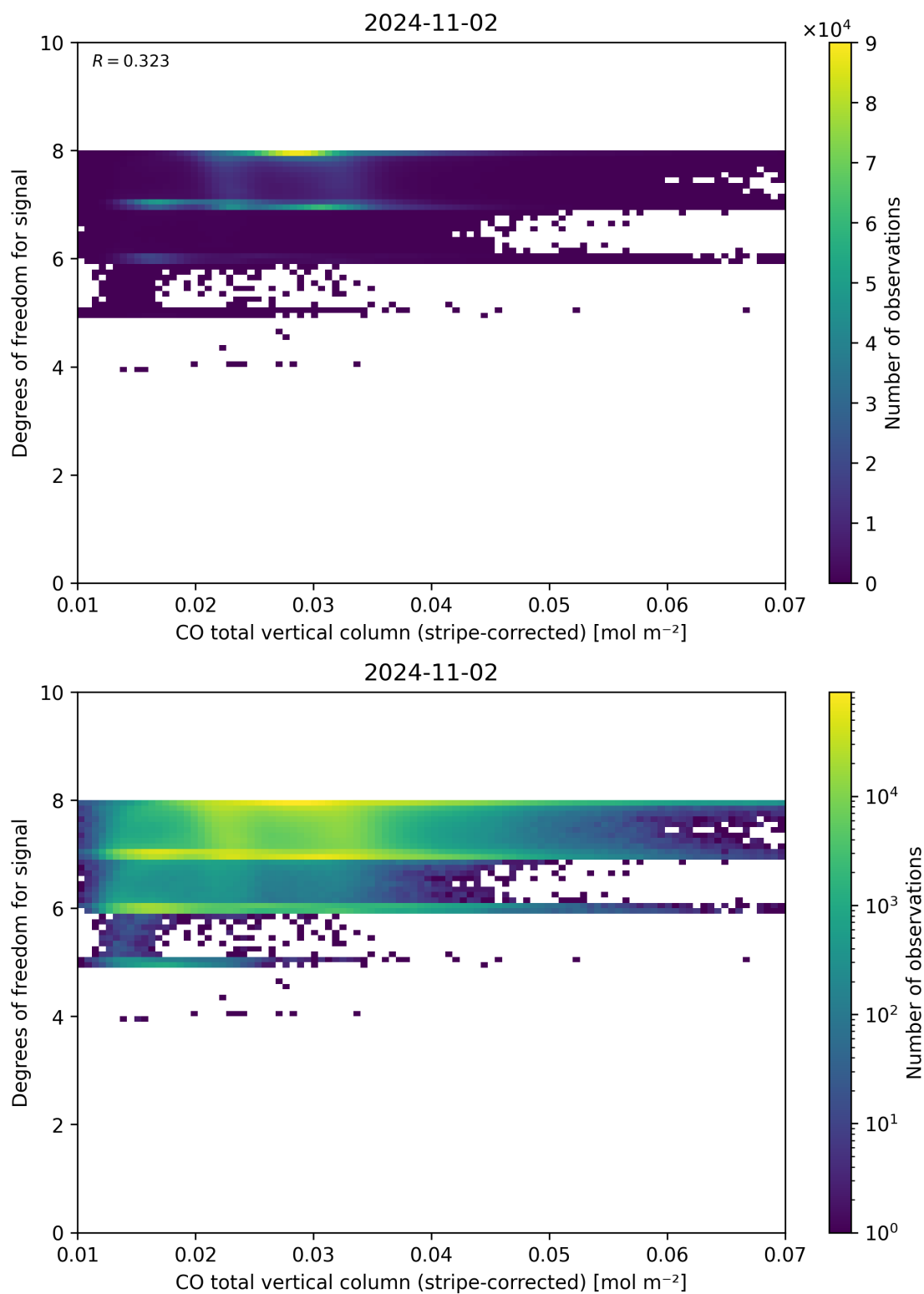
Figure 38: Scatter density plot of “CO total vertical column (stripe-corrected)” against “Degrees of freedom for signal” for 2024-11-01 to 2024-11-03.
