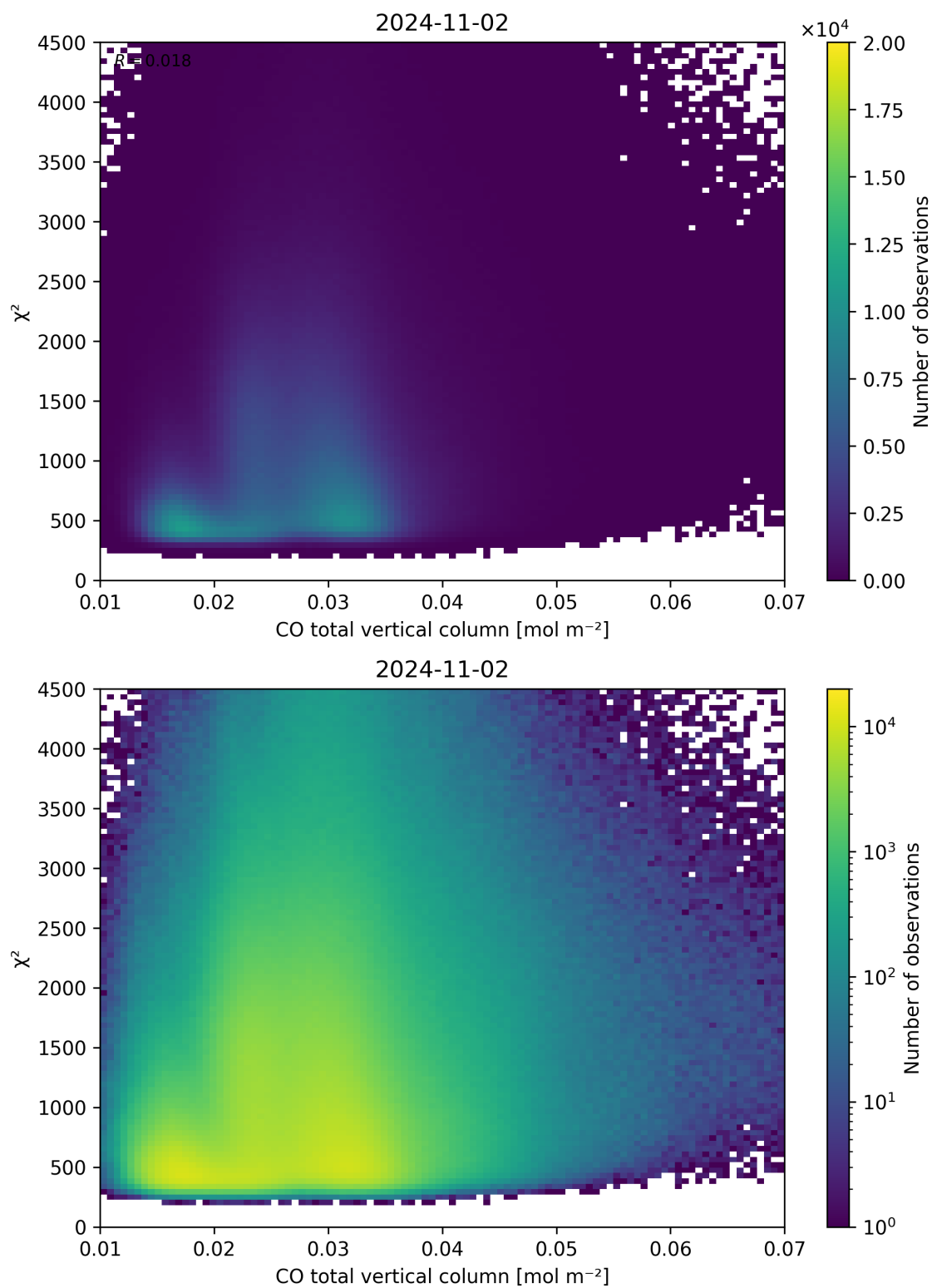
Figure 35: Scatter density plot of “CO total vertical column” against “ \chi^2 ” for 2024-11-01 to 2024-11-03.
