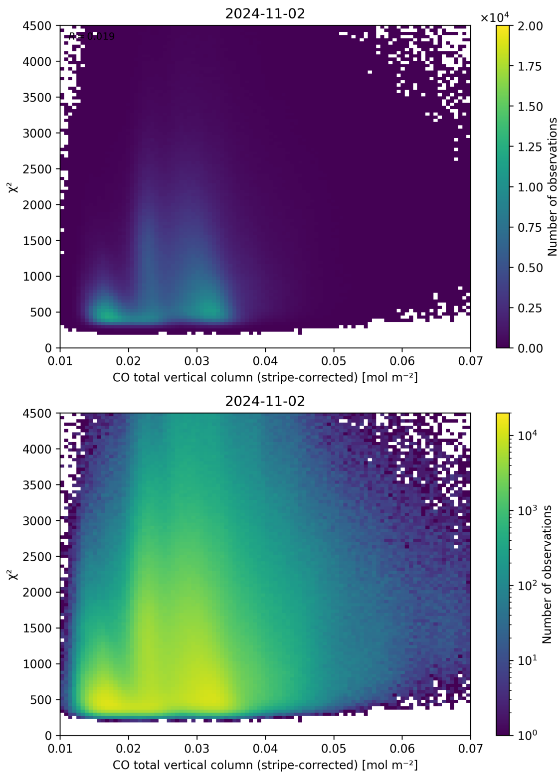
Figure 37: Scatter density plot of “CO total vertical column (stripe-corrected)” against “ \chi^2 ” for 2024-11-01 to 2024-11-03.
