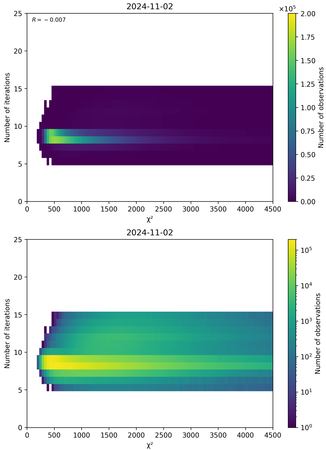
Figure 49: Scatter density plot of “ \chi^2 ” against “Number of iterations” for 2024-11-01 to 2024-11-03.
