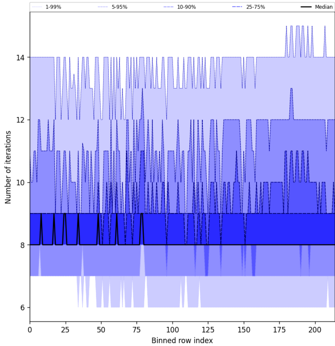
Figure 32: Along track statistics of “Number of iterations” for 2024-11-01 to 2024-11-03
