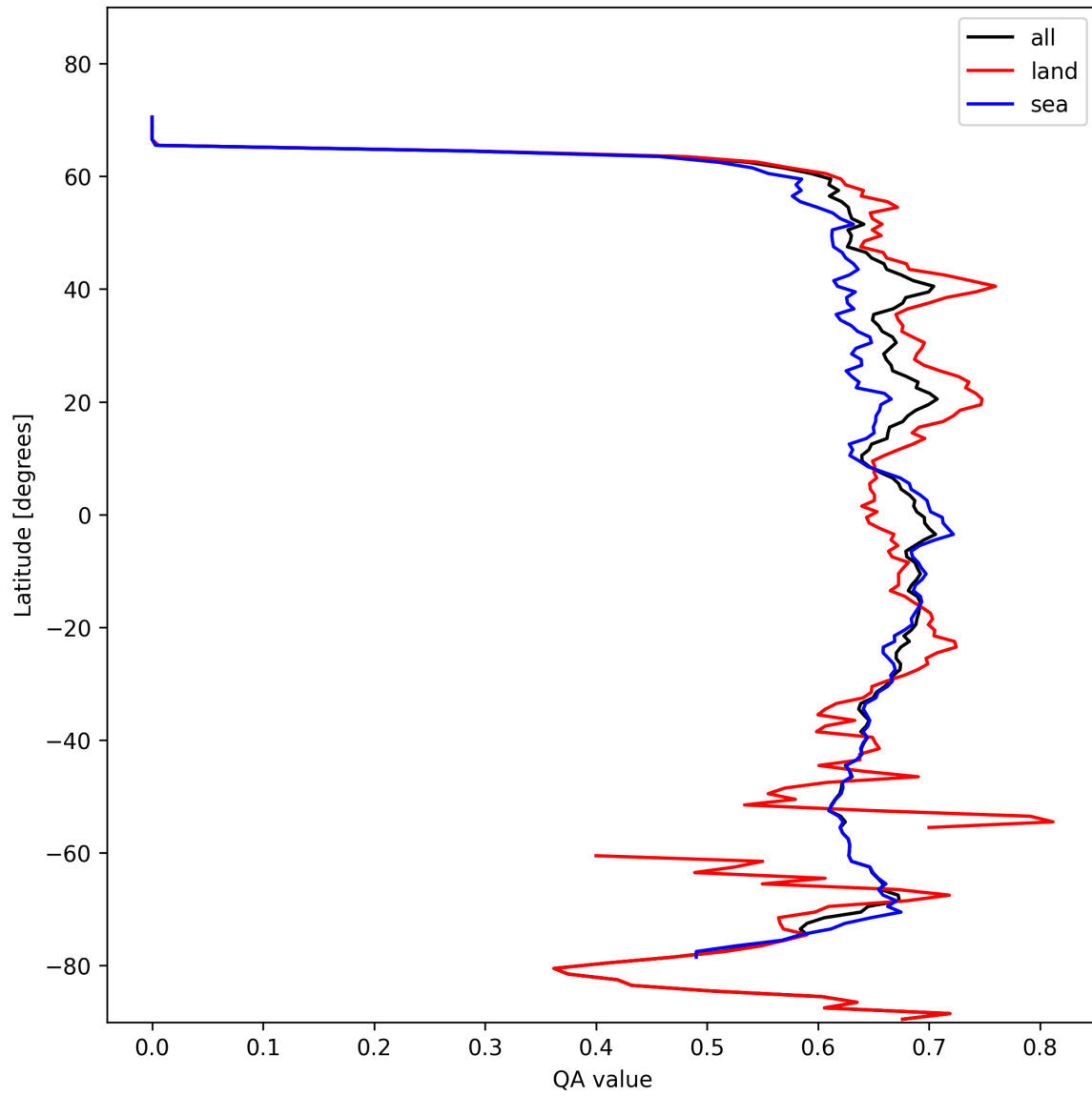
Figure 9: Zonal average of “QA value” for 2024-11-01 to 2024-11-03.
