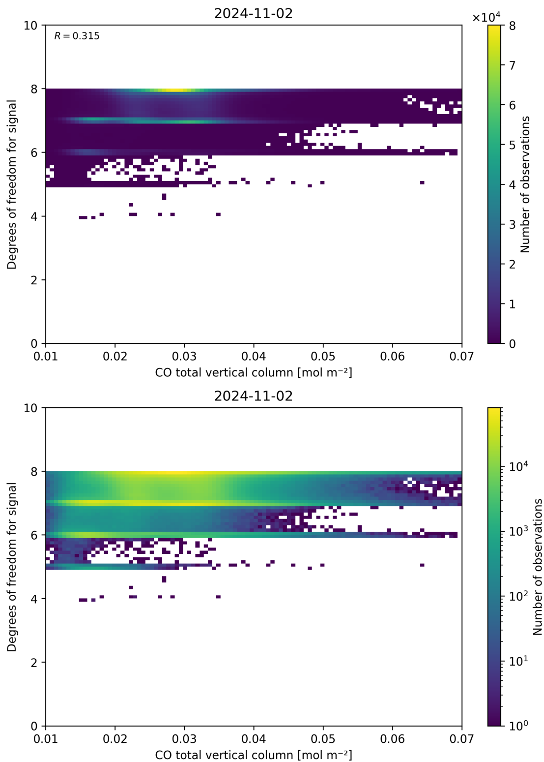
Figure 41: Scatter density plot of “CO total vertical column” against “Degrees of freedom for signal” for 2024-11-01 to 2024-11-03.
