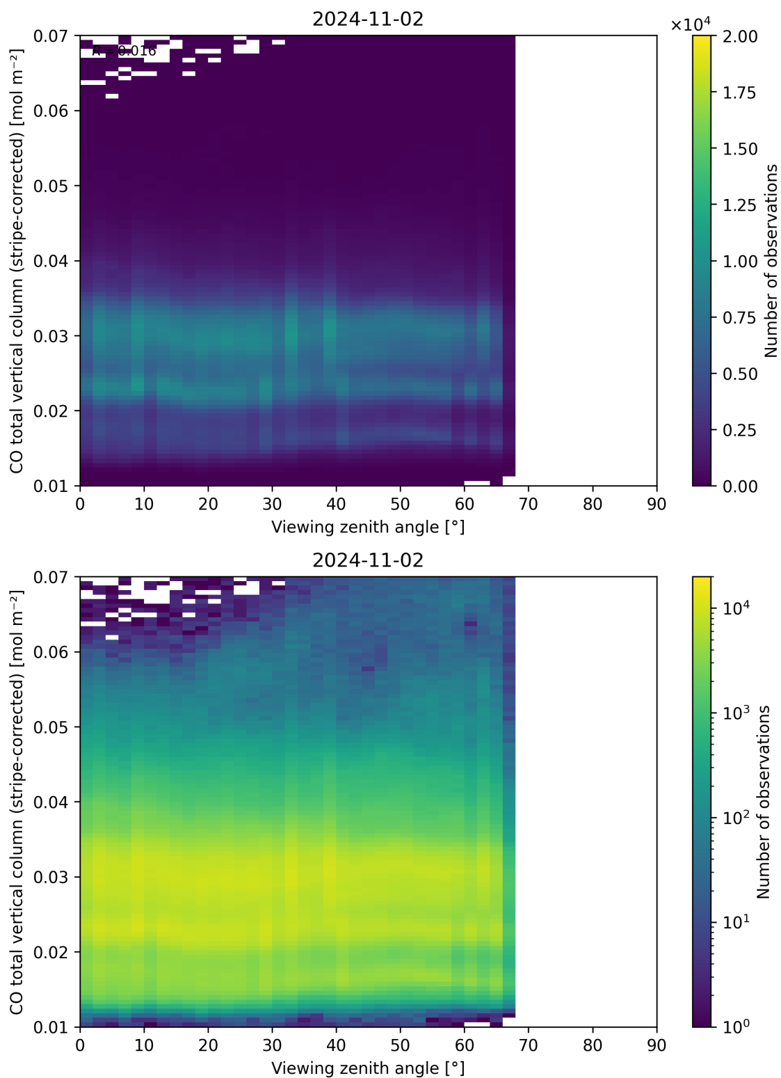
Figure 70: Scatter density plot of “Viewing zenith angle” against “CO total vertical column (stripe-corrected)” for 2024-11-01 to 2024-11-03.
