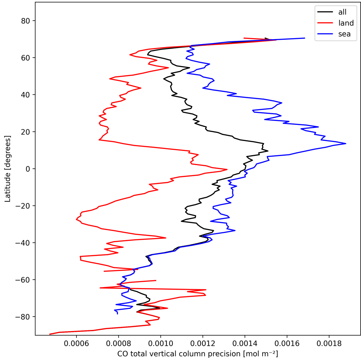
Figure 12: Zonal average of "CO total vertical column precision" for 2024-11-01 to 2024-11-03.
