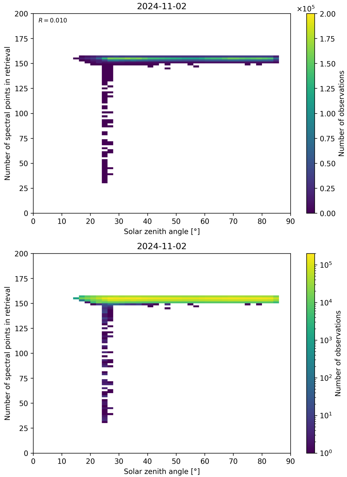
Figure 68: Scatter density plot of “Solar zenith angle” against “Number of spectral points in retrieval” for 2024-11-01 to 2024-11-03.
