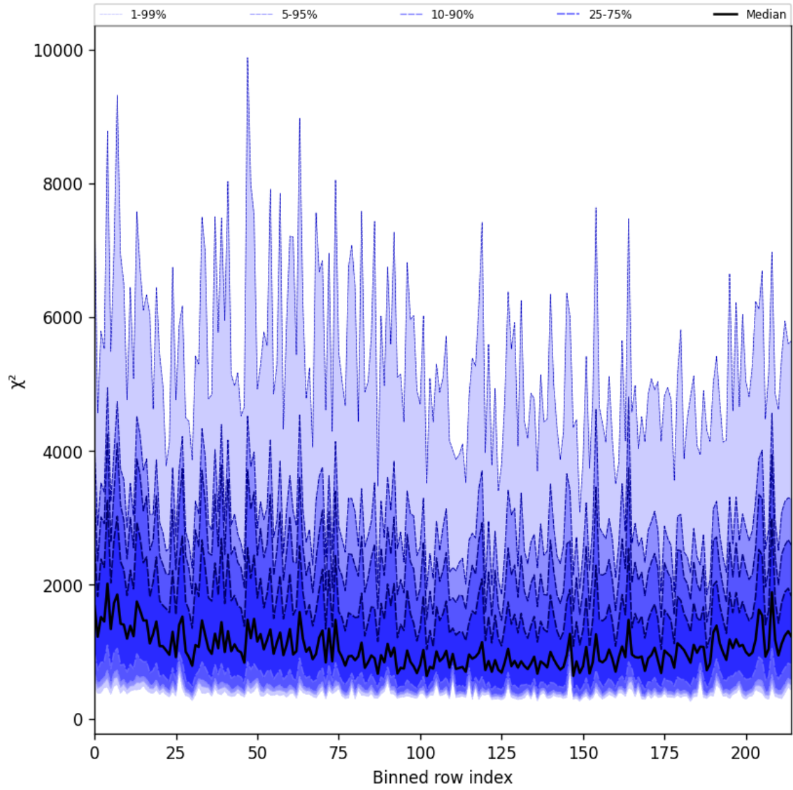
Figure 30: Along track statistics of “ \chi^2 ” for 2024-11-01 to 2024-11-03
