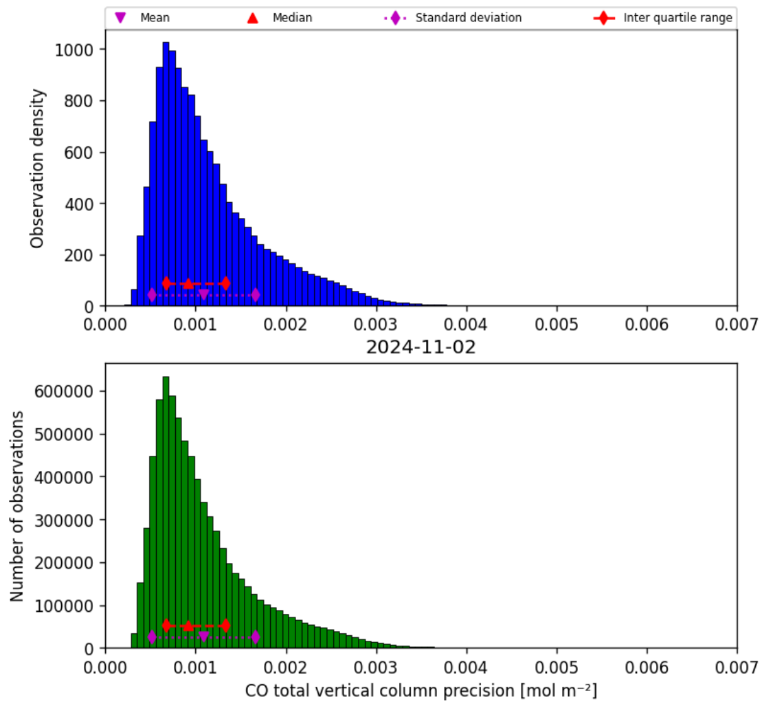
Figure 20: Histogram of “CO total vertical column precision” for 2024-11-01 to 2024-11-03
