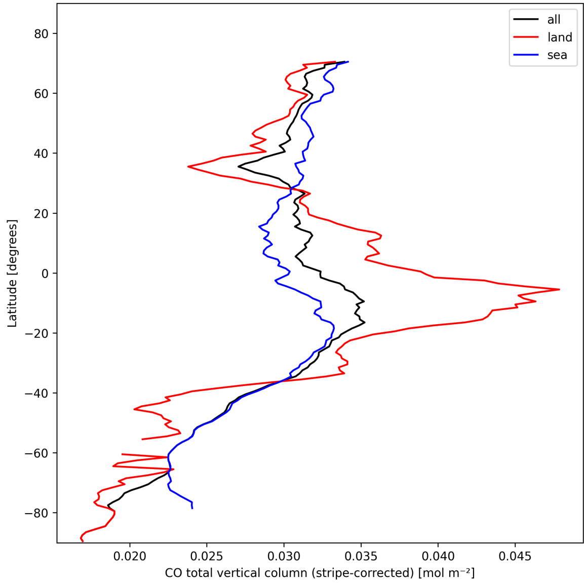
Figure 11: Zonal average of “CO total vertical column (stripe-corrected)” for 2024-11-01 to 2024-11-03.
