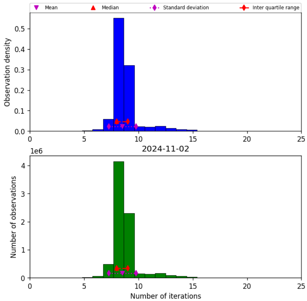
Figure 24: Histogram of “Number of iterations” for 2024-11-01 to 2024-11-03
