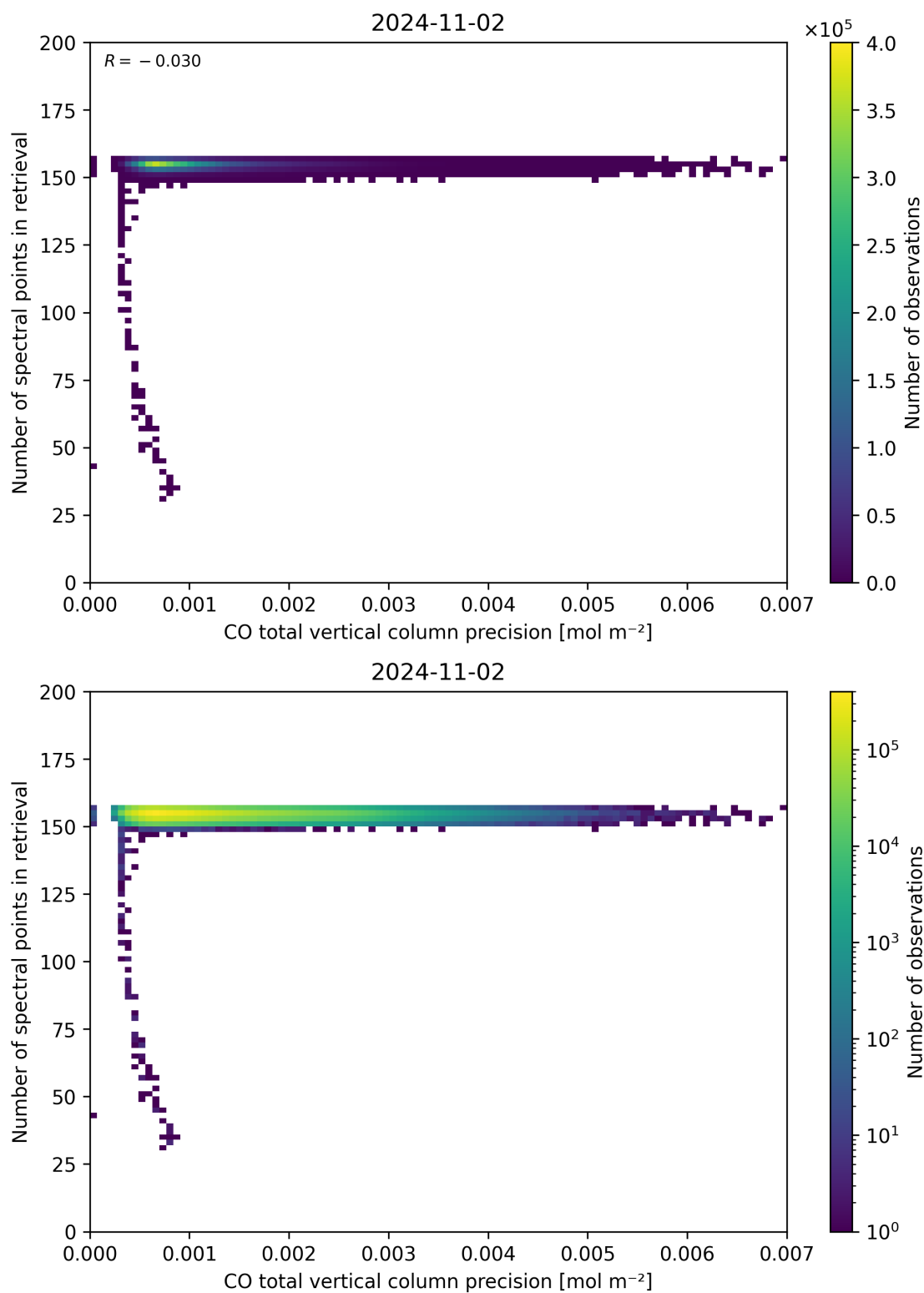
Figure 47: Scatter density plot of “CO total vertical column precision” against “Number of spectral points in retrieval” for 2024-11-01 to 2024-11-03.
