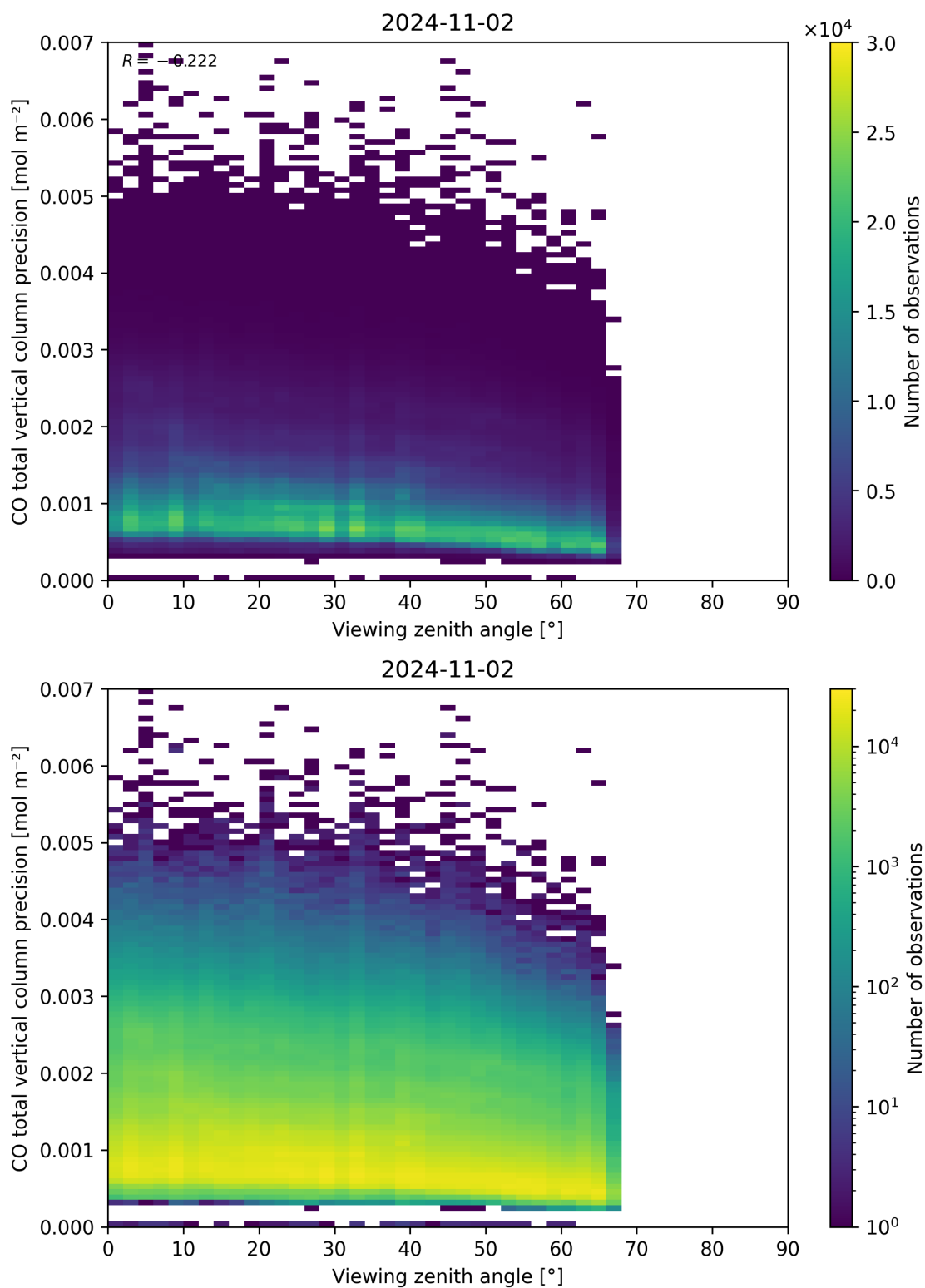
Figure 71: Scatter density plot of “Viewing zenith angle” against “CO total vertical column precision” for 2024-11-01 to 2024-11-03.
