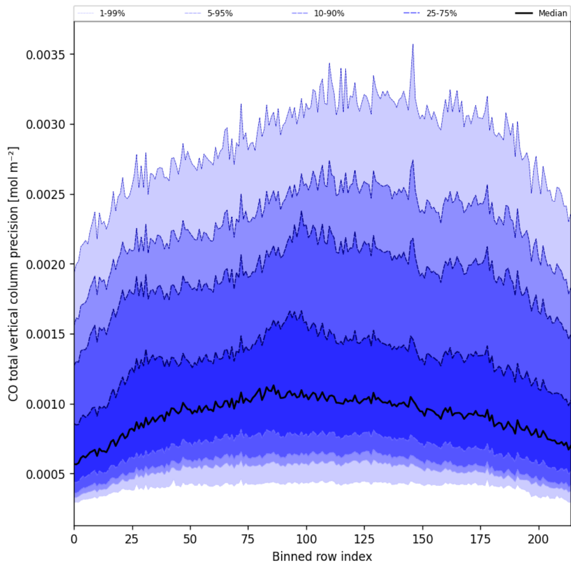
Figure 28: Along track statistics of “CO total vertical column precision” for 2024-11-01 to 2024-11-03
