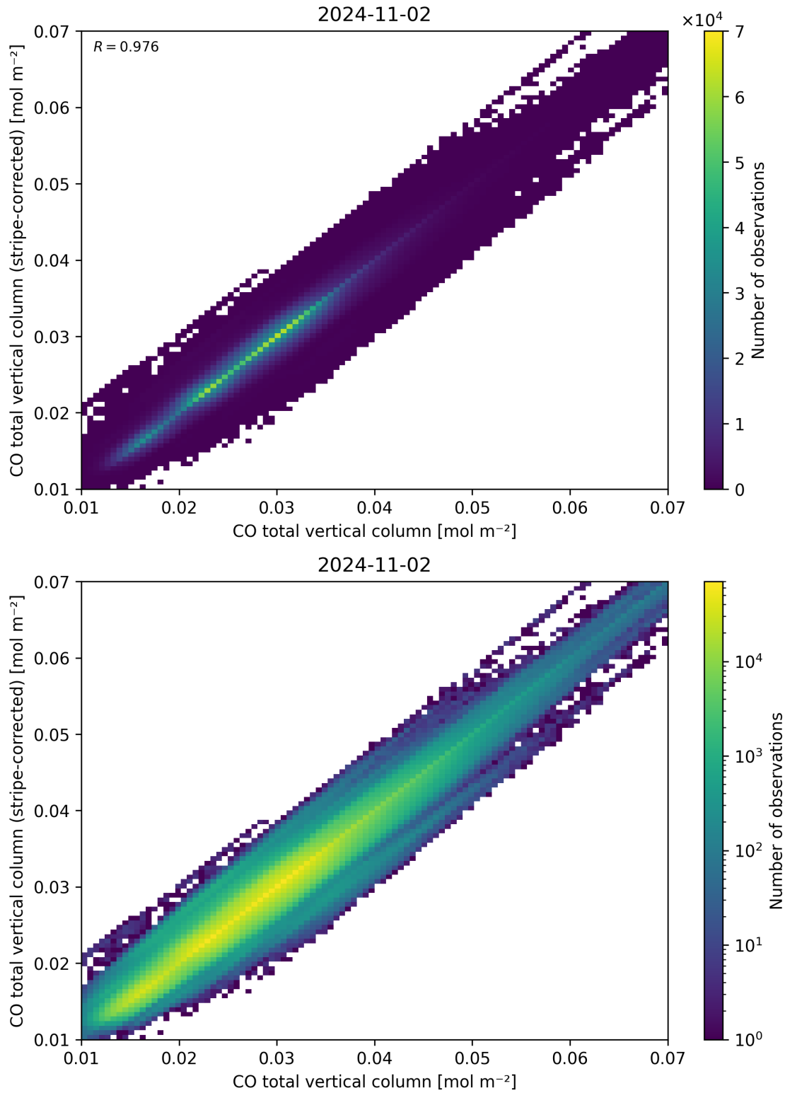
Figure 33: Scatter density plot of “CO total vertical column” against “CO total vertical column (stripe-corrected)” for 2024-11-01 to 2024-11-03.
