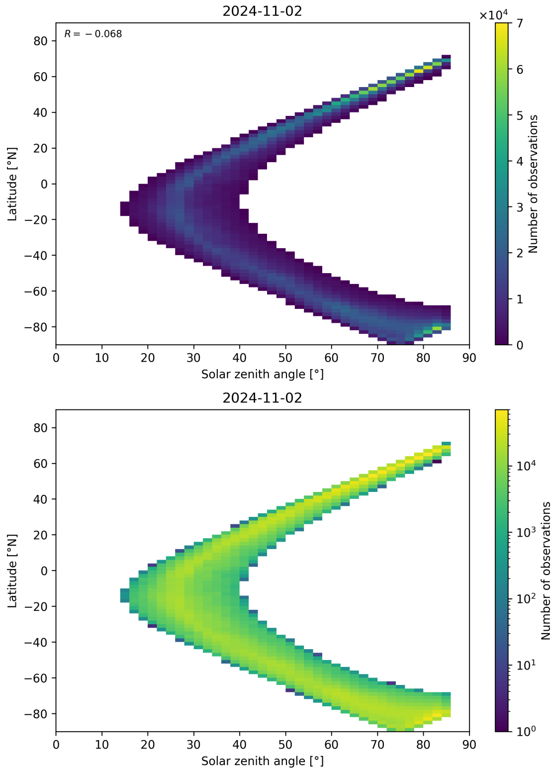
Figure 66: Scatter density plot of “Solar zenith angle” against “Latitude” for 2024-11-01 to 2024-11-03.
