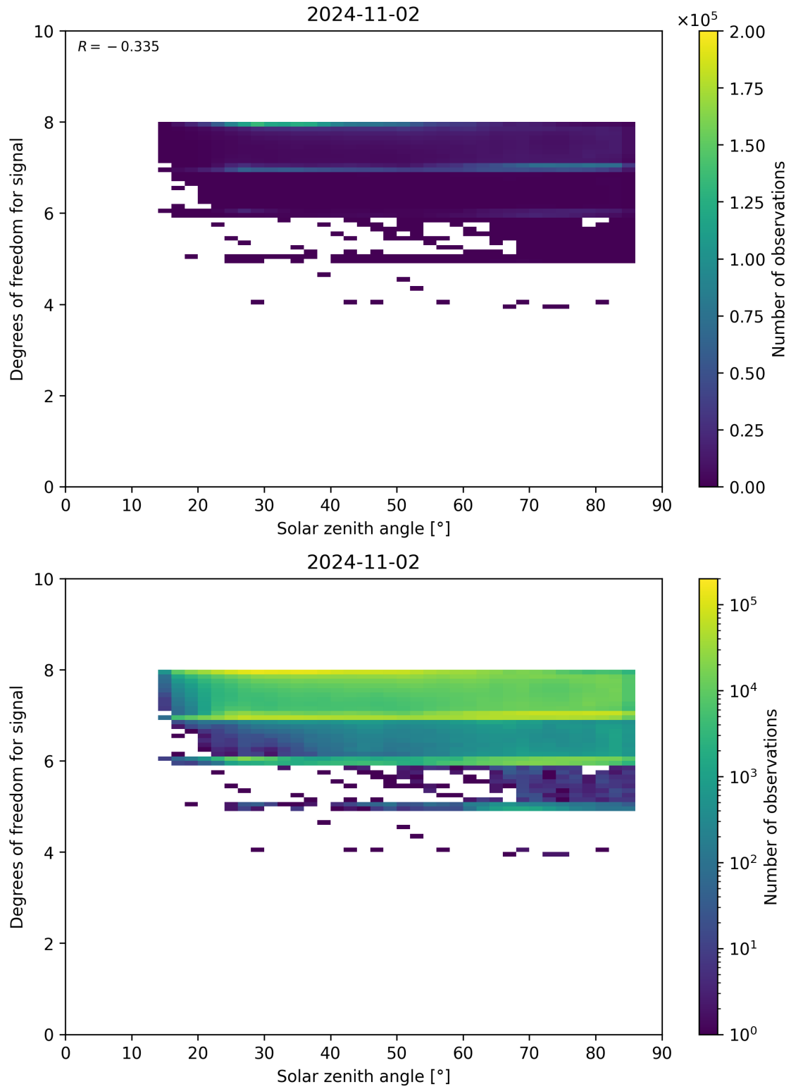
Figure 65: Scatter density plot of “Solar zenith angle” against “Degrees of freedom for signal” for 2024-11-01 to 2024-11-03.
