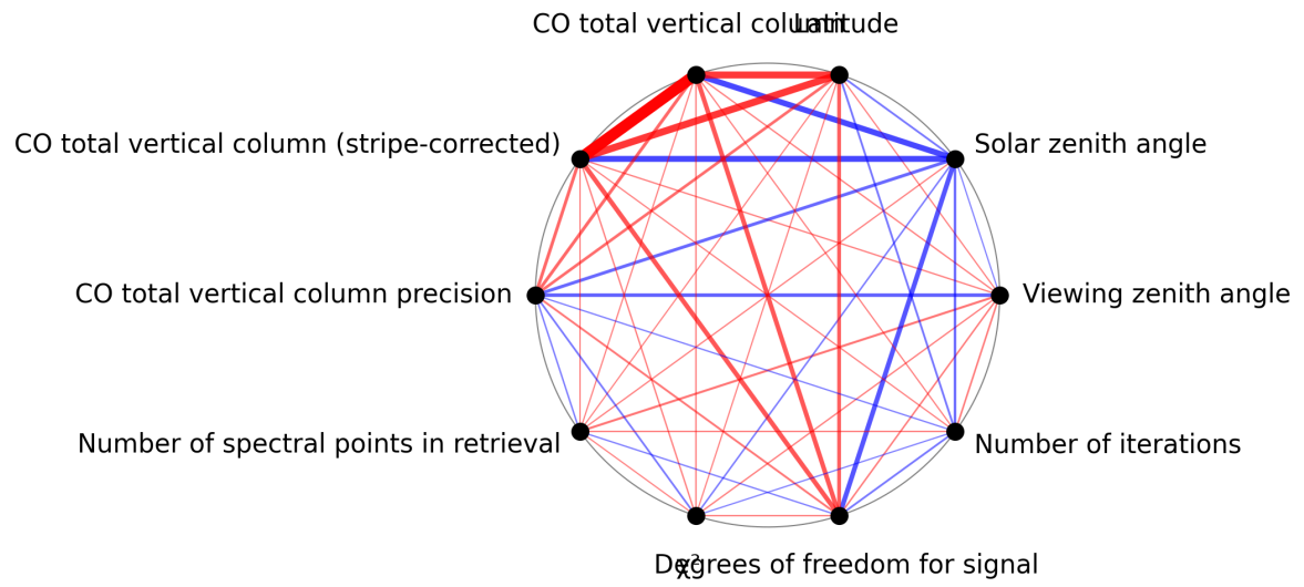
Figure 1: Map of correlation graph for 2024-11-01 to 2024-11-03.
