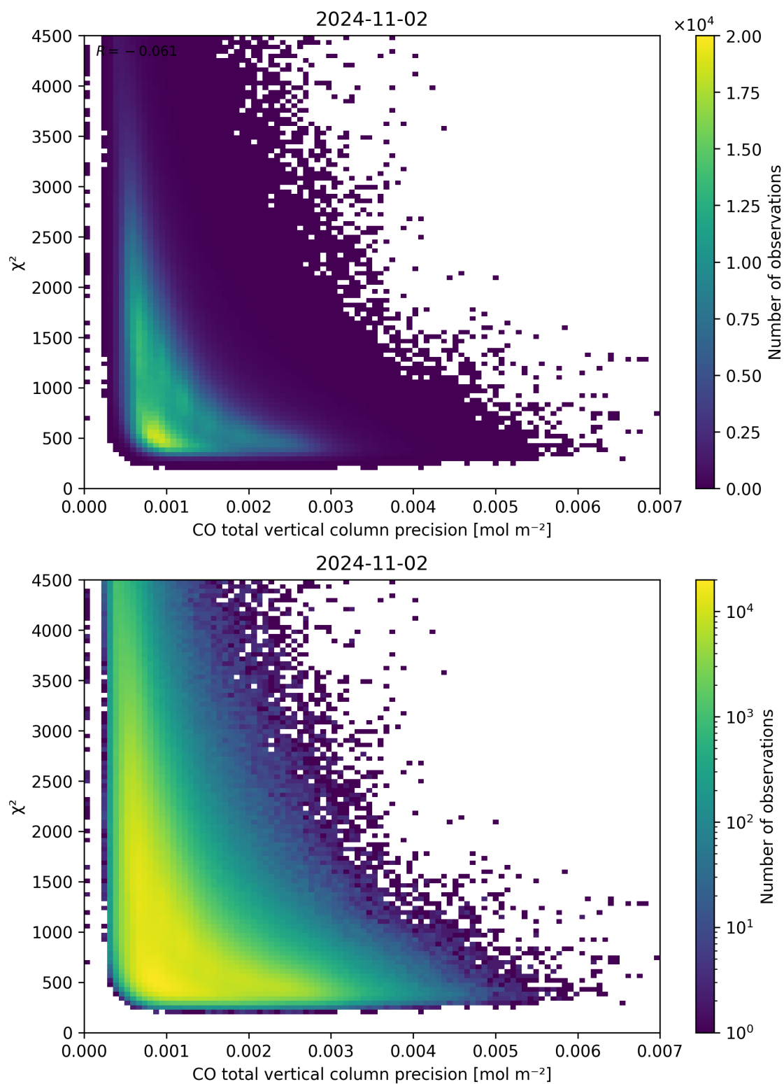
Figure 44: Scatter density plot of “CO total vertical column precision” against “ \chi^2 ” for 2024-11-01 to 2024-11-03.
