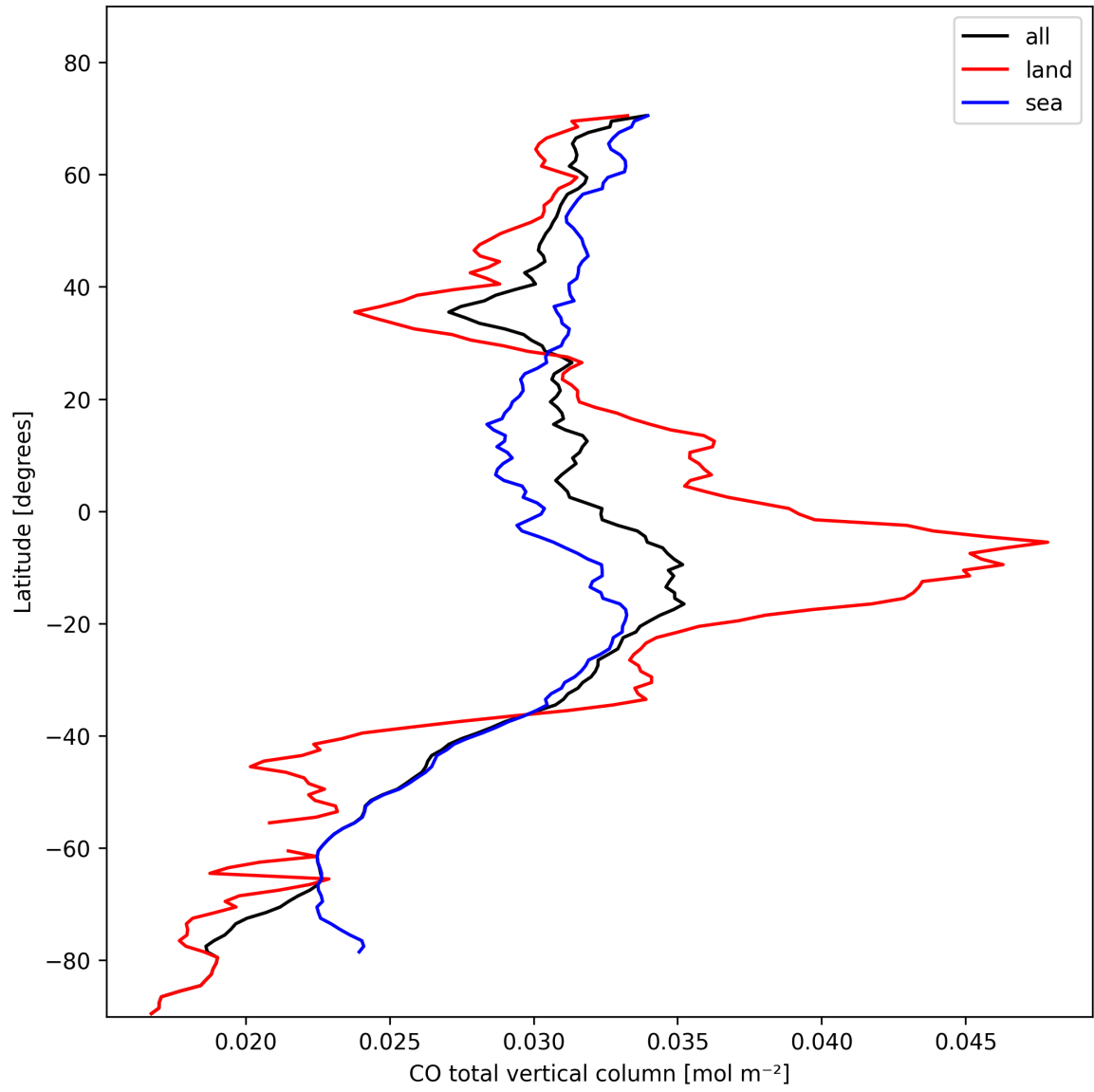
Figure 10: Zonal average of “CO total vertical column” for 2024-11-01 to 2024-11-03.
