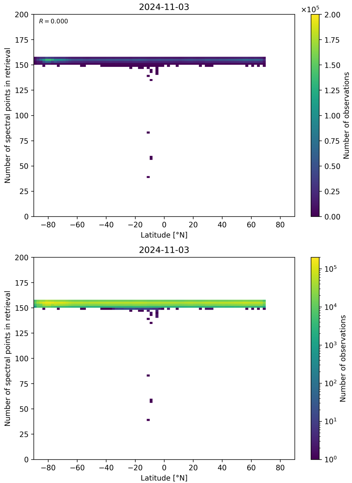
Figure 57: Scatter density plot of “Latitude” against “Number of spectral points in retrieval” for 2024-11-02 to 2024-11-04.
