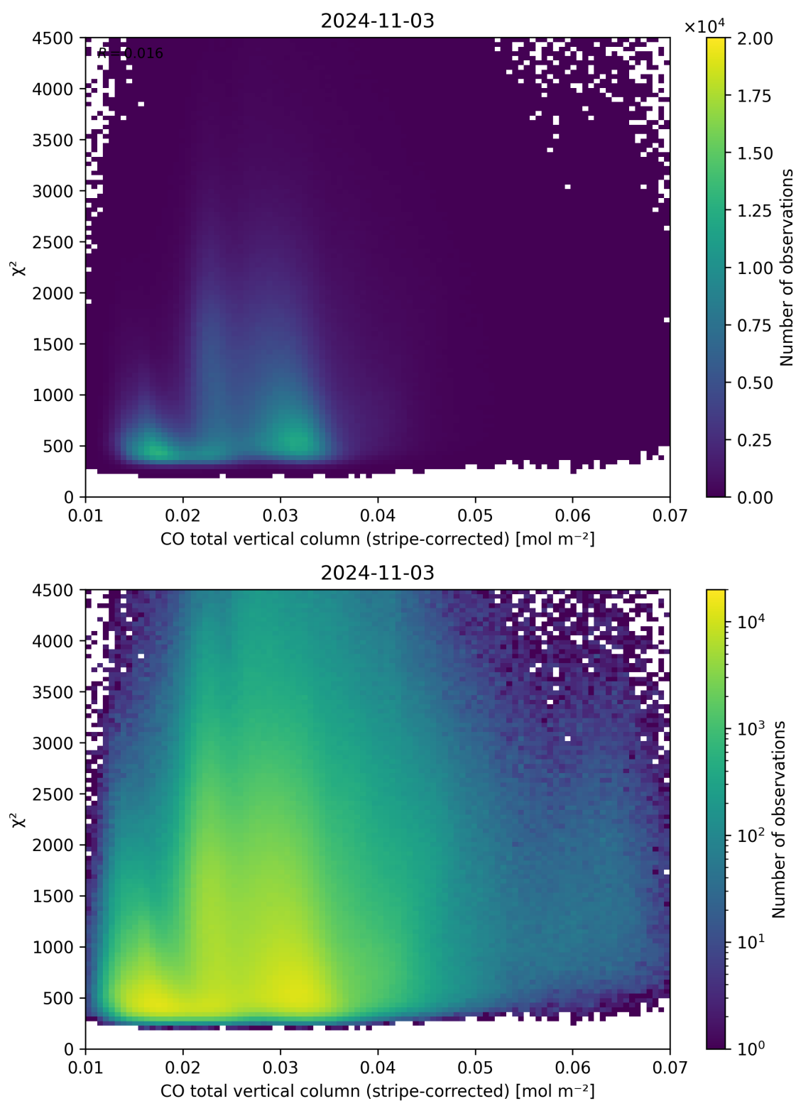
Figure 37: Scatter density plot of “CO total vertical column (stripe-corrected)” against “ \chi^2 ” for 2024-11-02 to 2024-11-04.
