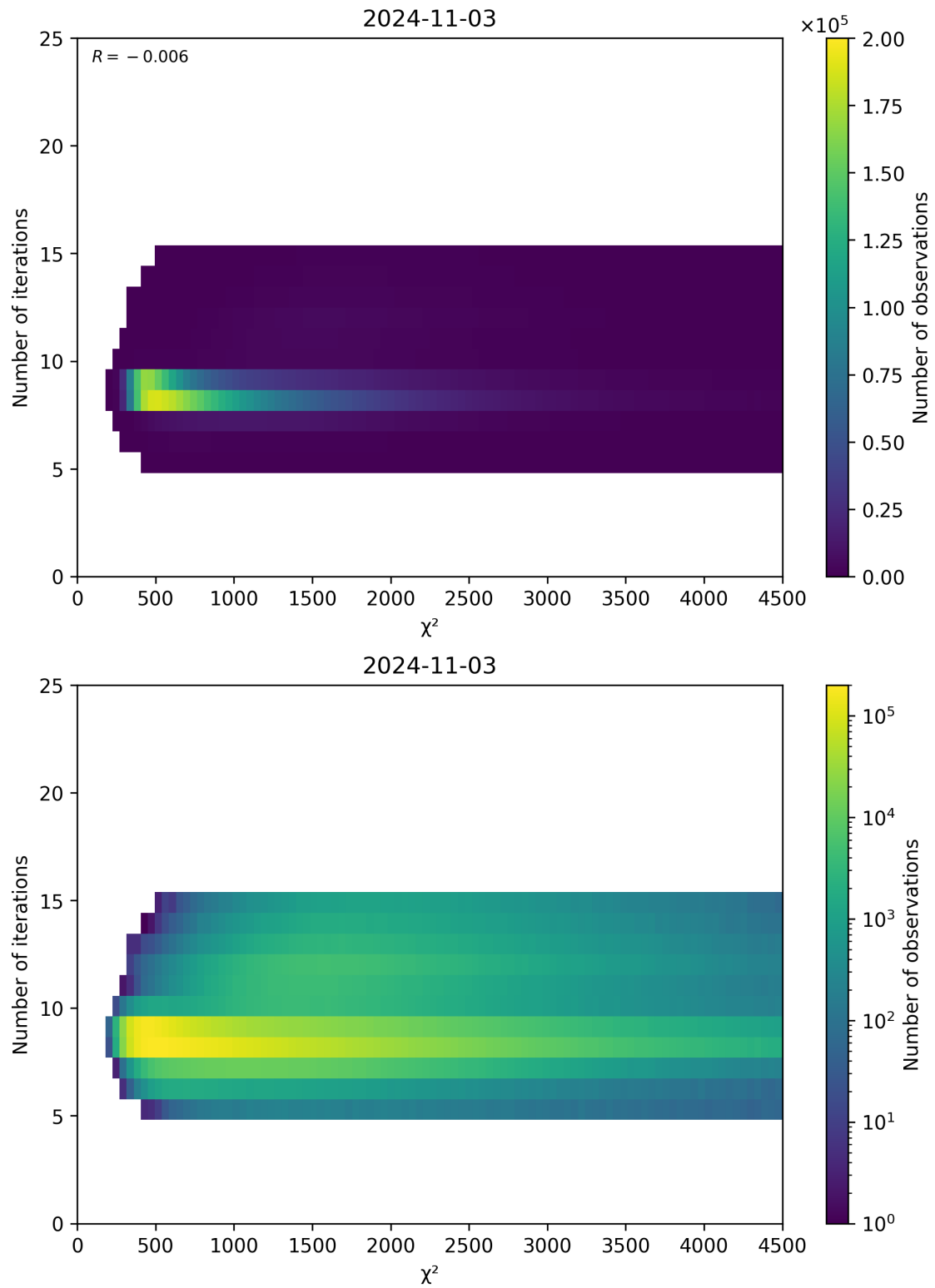
Figure 49: Scatter density plot of “ \chi^2 ” against “Number of iterations” for 2024-11-02 to 2024-11-04.
