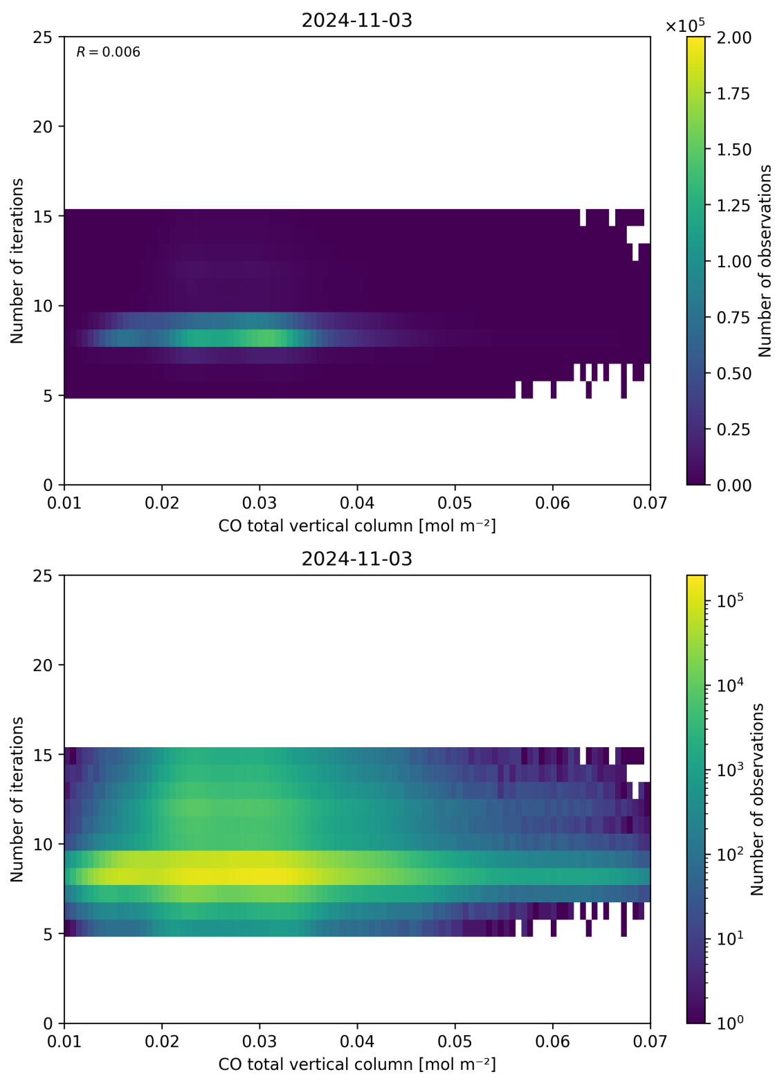
Figure 42: Scatter density plot of “CO total vertical column” against “Number of iterations” for 2024-11-02 to 2024-11-04.
