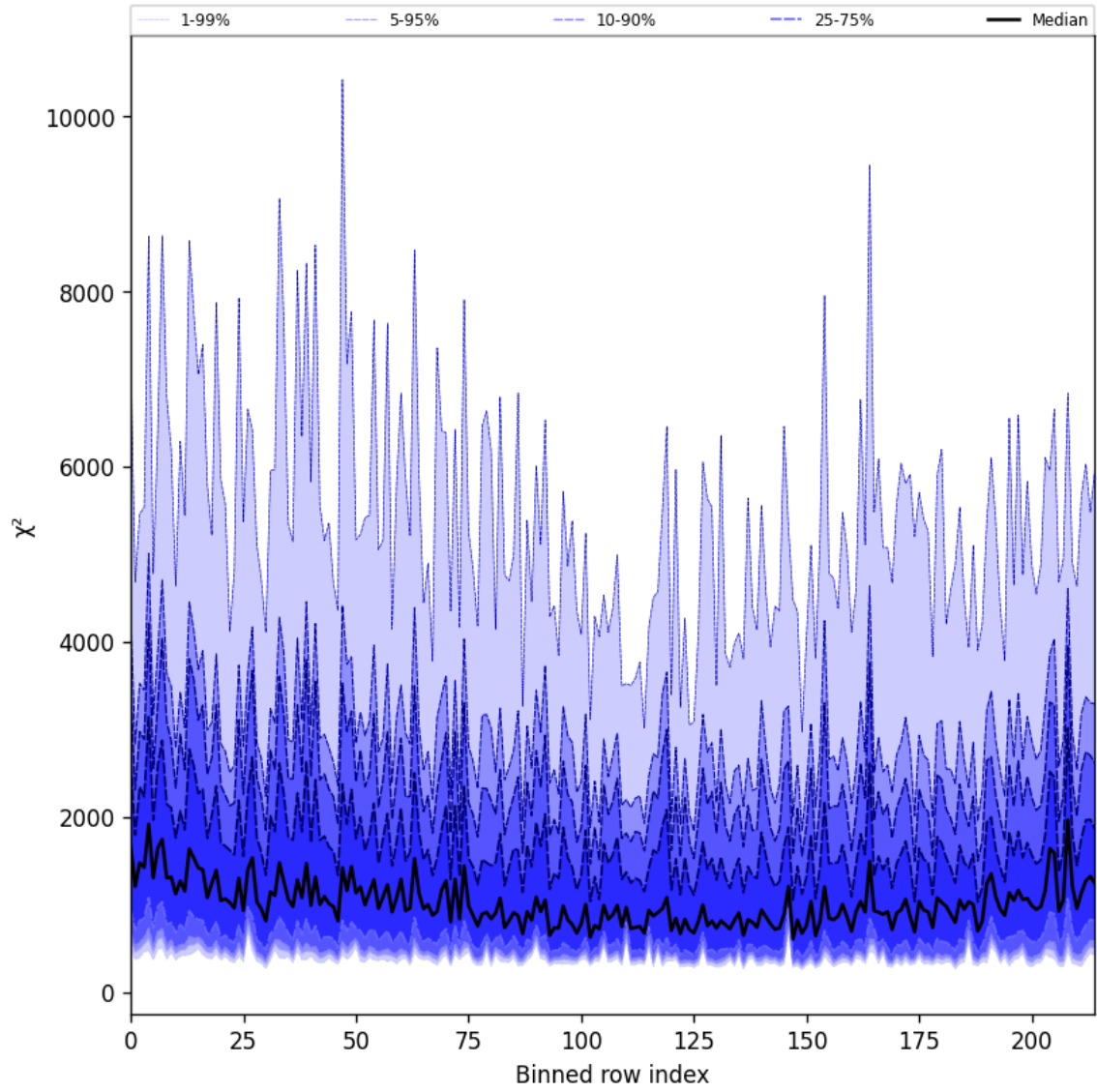
Figure 30: Along track statistics of “ \chi^2 ” for 2024-11-02 to 2024-11-04
