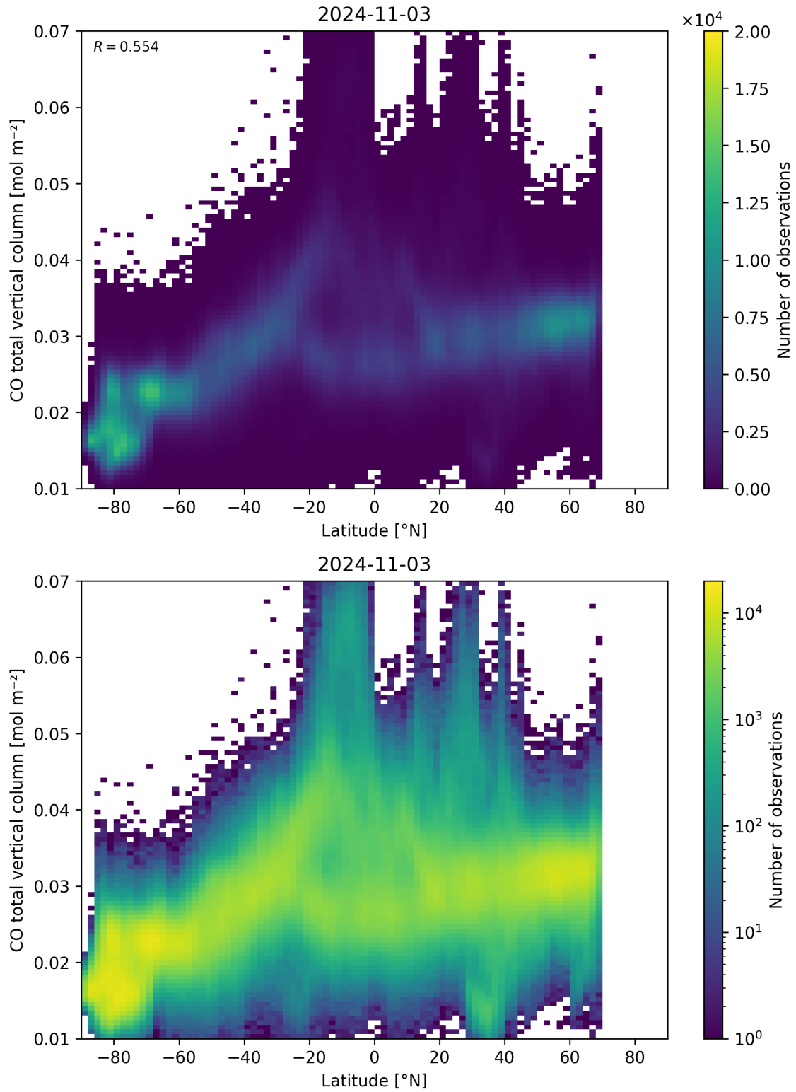
Figure 51: Scatter density plot of “Latitude” against “CO total vertical column” for 2024-11-02 to 2024-11-04.
