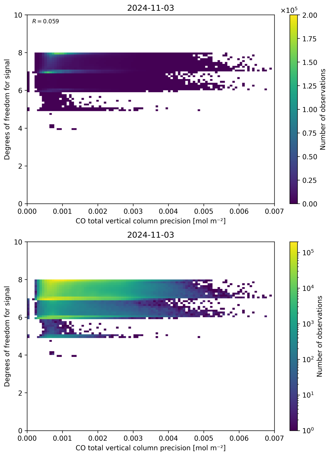
Figure 45: Scatter density plot of “CO total vertical column precision” against “Degrees of freedom for signal” for 2024-11-02 to 2024-11-04.
