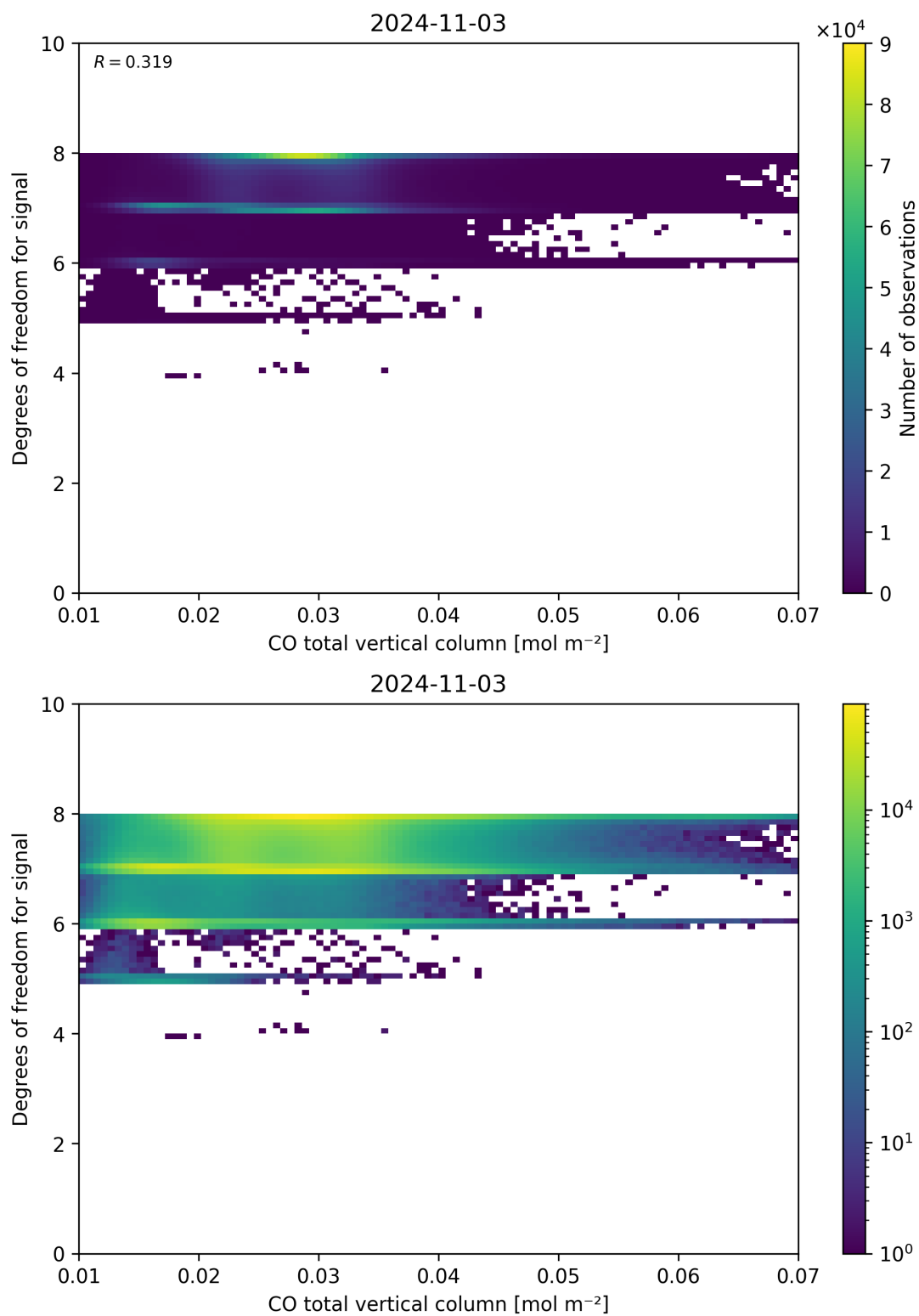
Figure 41: Scatter density plot of “CO total vertical column” against “Degrees of freedom for signal” for 2024-11-02 to 2024-11-04.
