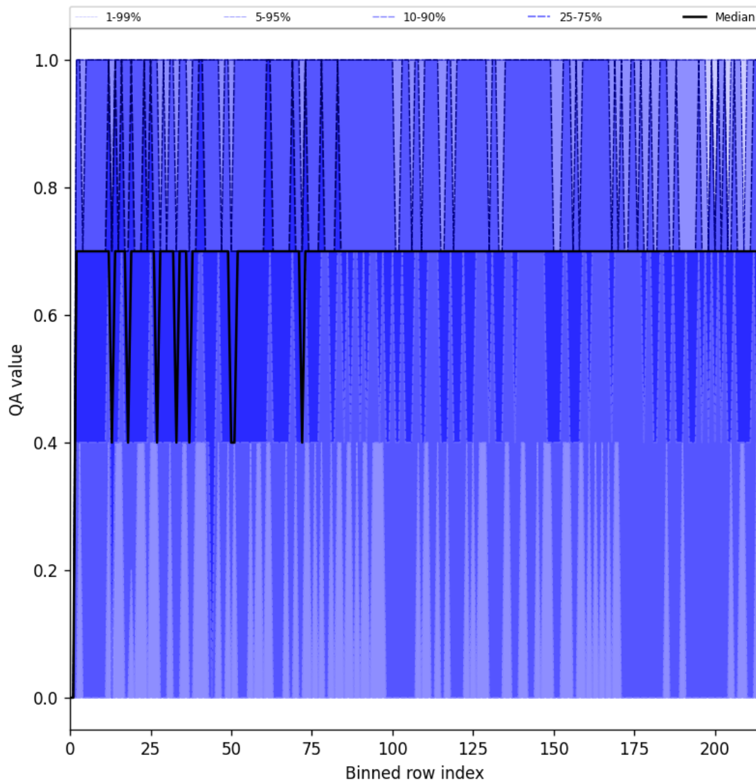
Figure 25: Along track statistics of “QA value” for 2024-11-02 to 2024-11-04
