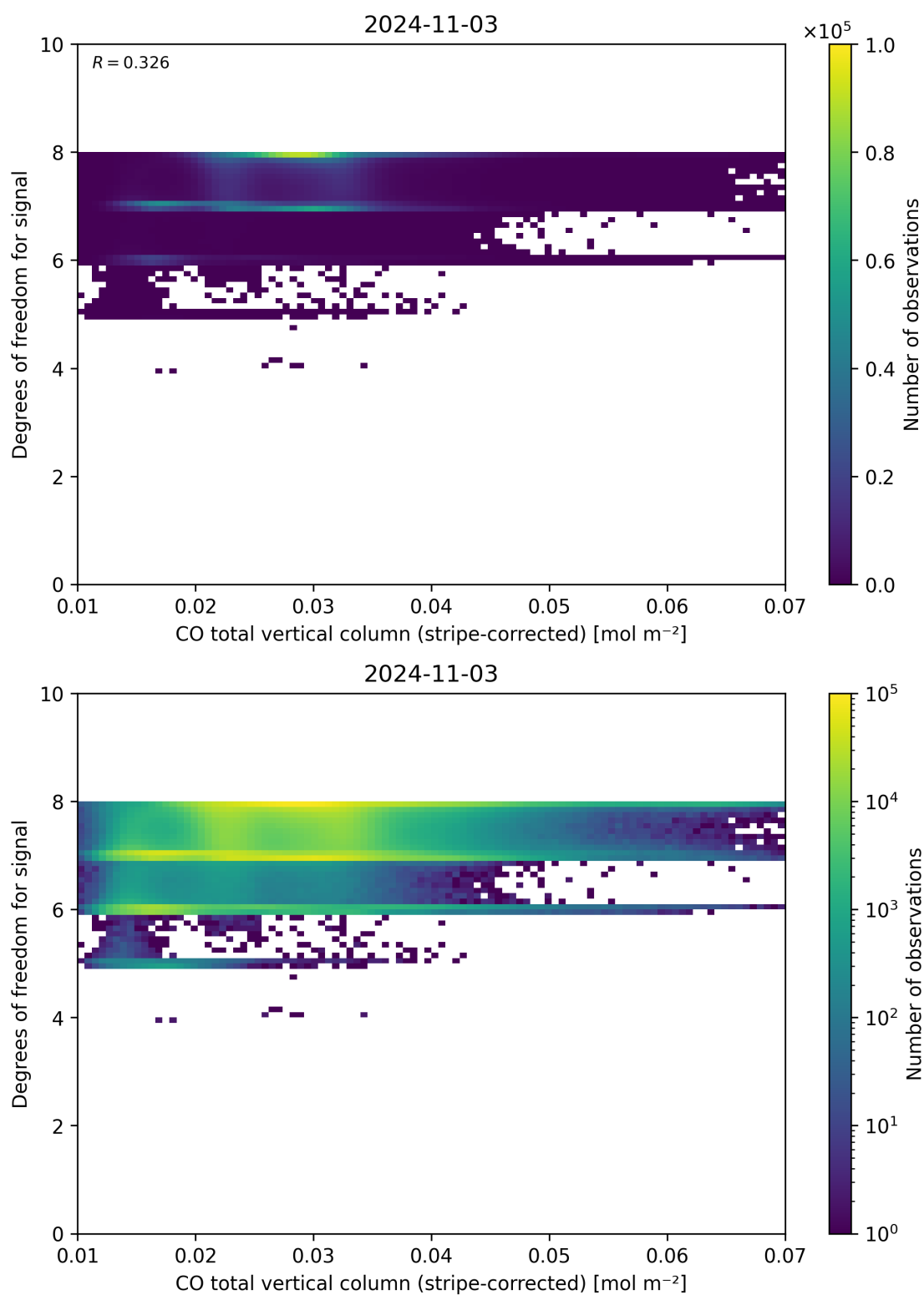
Figure 38: Scatter density plot of “CO total vertical column (stripe-corrected)” against “Degrees of freedom for signal” for 2024-11-02 to 2024-11-04.
