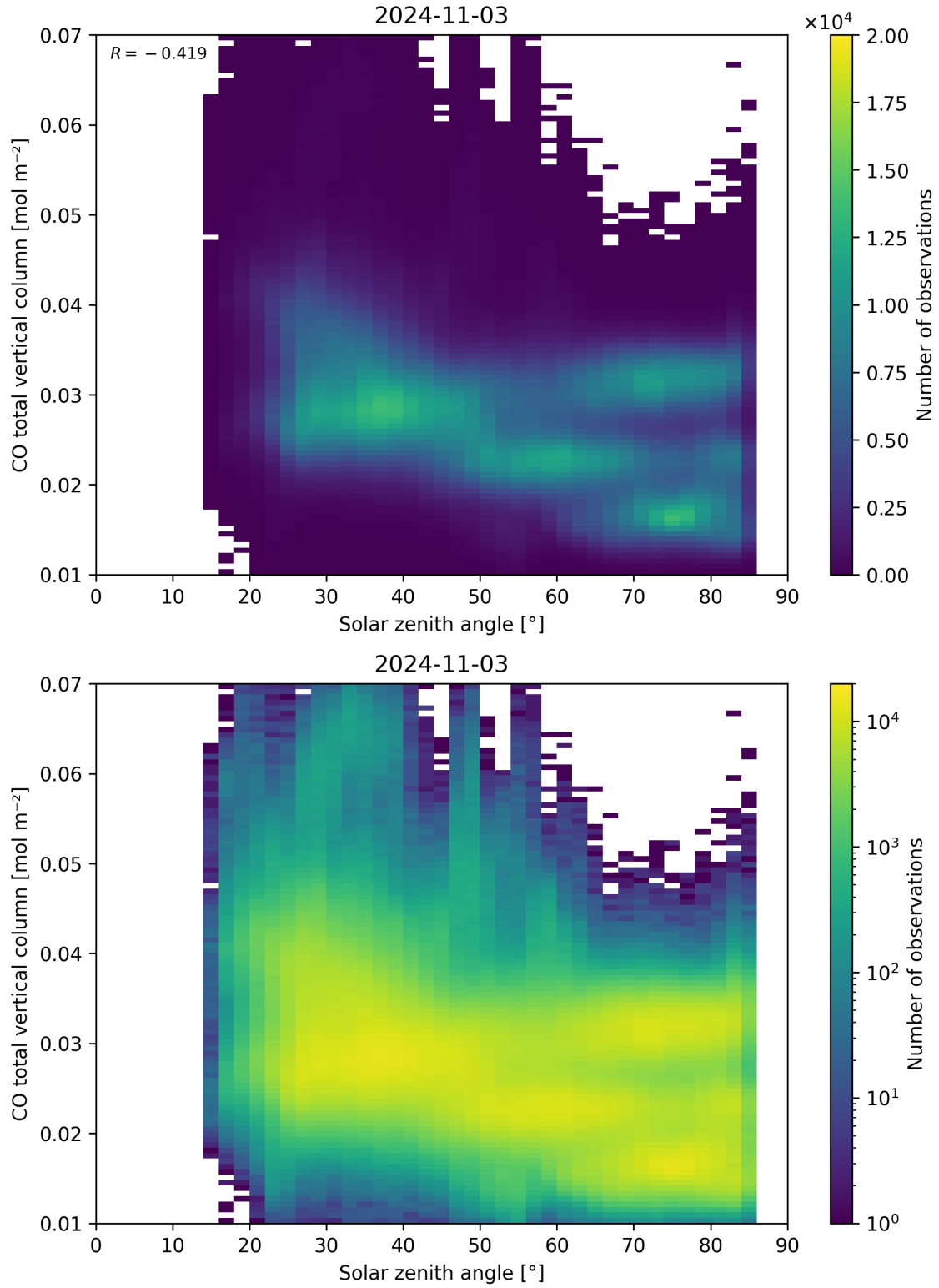
Figure 61: Scatter density plot of “Solar zenith angle” against “CO total vertical column” for 2024-11-02 to 2024-11-04.
