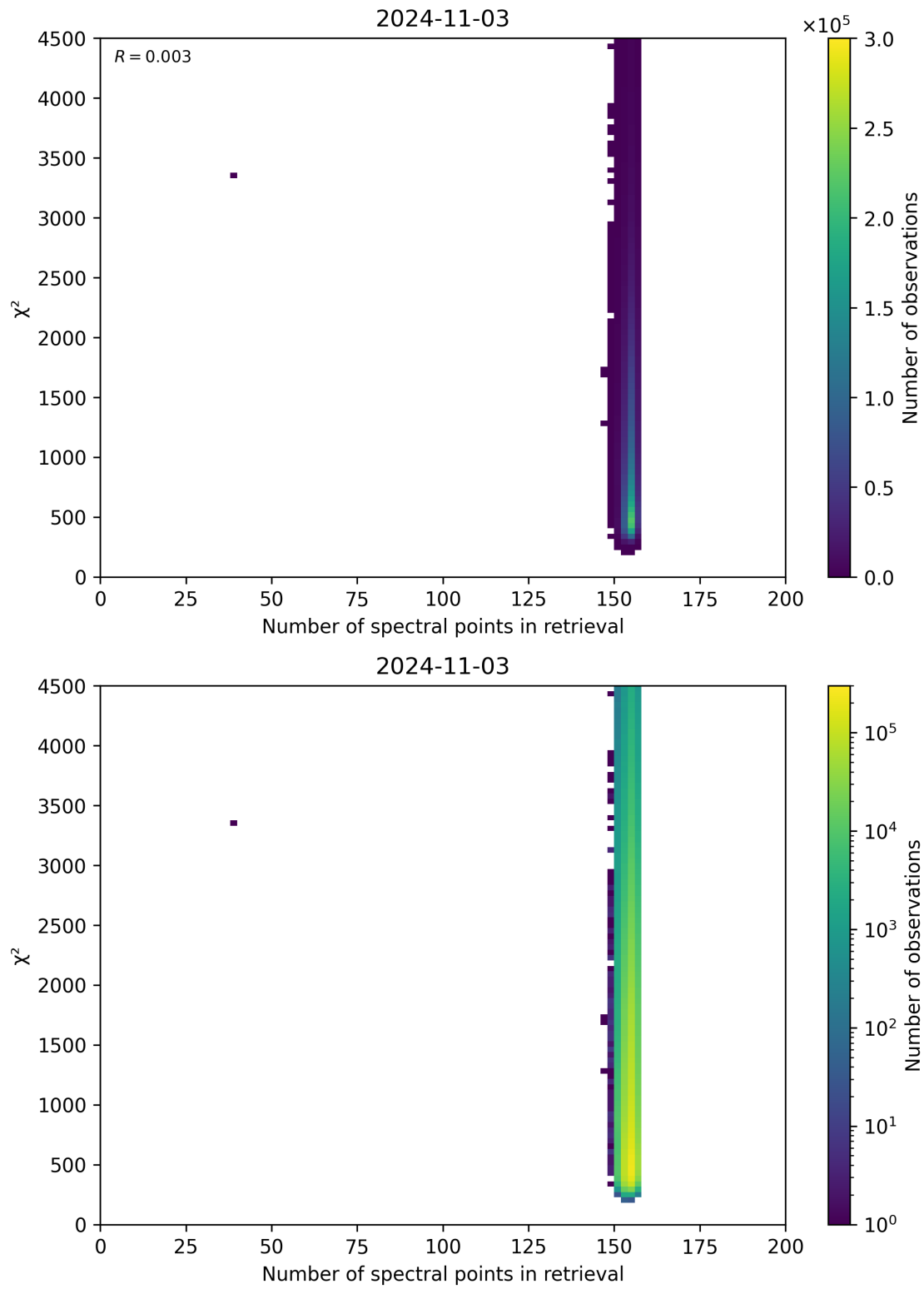
Figure 58: Scatter density plot of “Number of spectral points in retrieval” against “ \chi^2 ” for 2024-11-02 to 2024-11-04.
