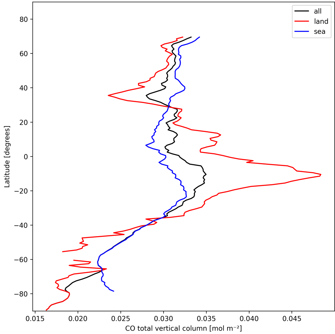
Figure 10: Zonal average of “CO total vertical column” for 2024-11-02 to 2024-11-04.
