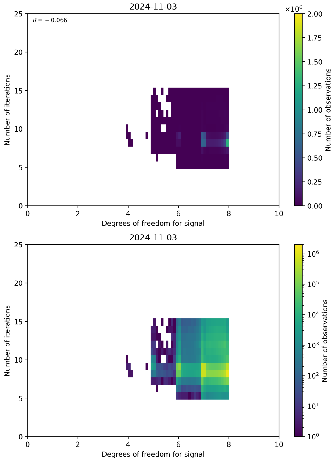
Figure 50: Scatter density plot of “Degrees of freedom for signal” against “Number of iterations” for 2024-11-02 to 2024-11-04.
