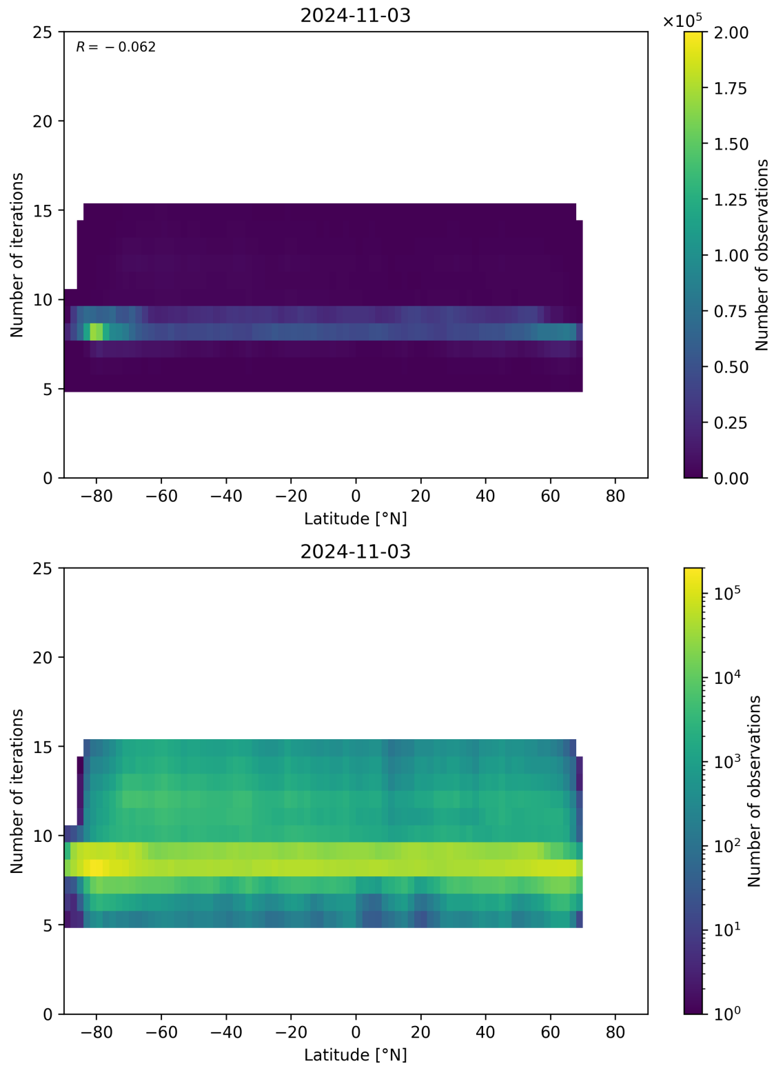
Figure 56: Scatter density plot of “Latitude” against “Number of iterations” for 2024-11-02 to 2024-11-04.
