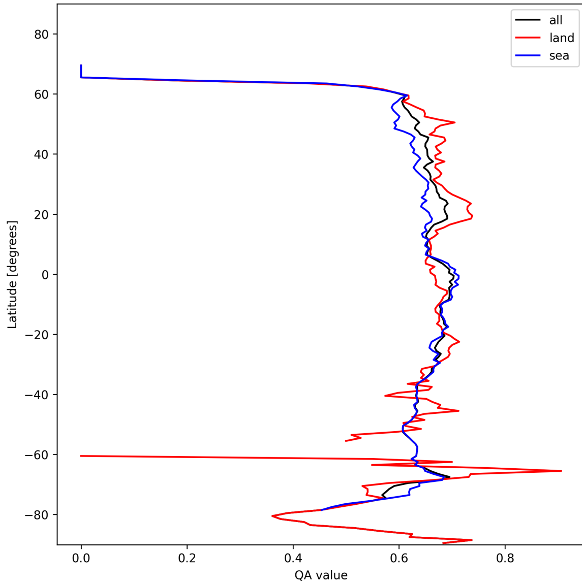
Figure 9: Zonal average of “QA value” for 2024-11-02 to 2024-11-04.
