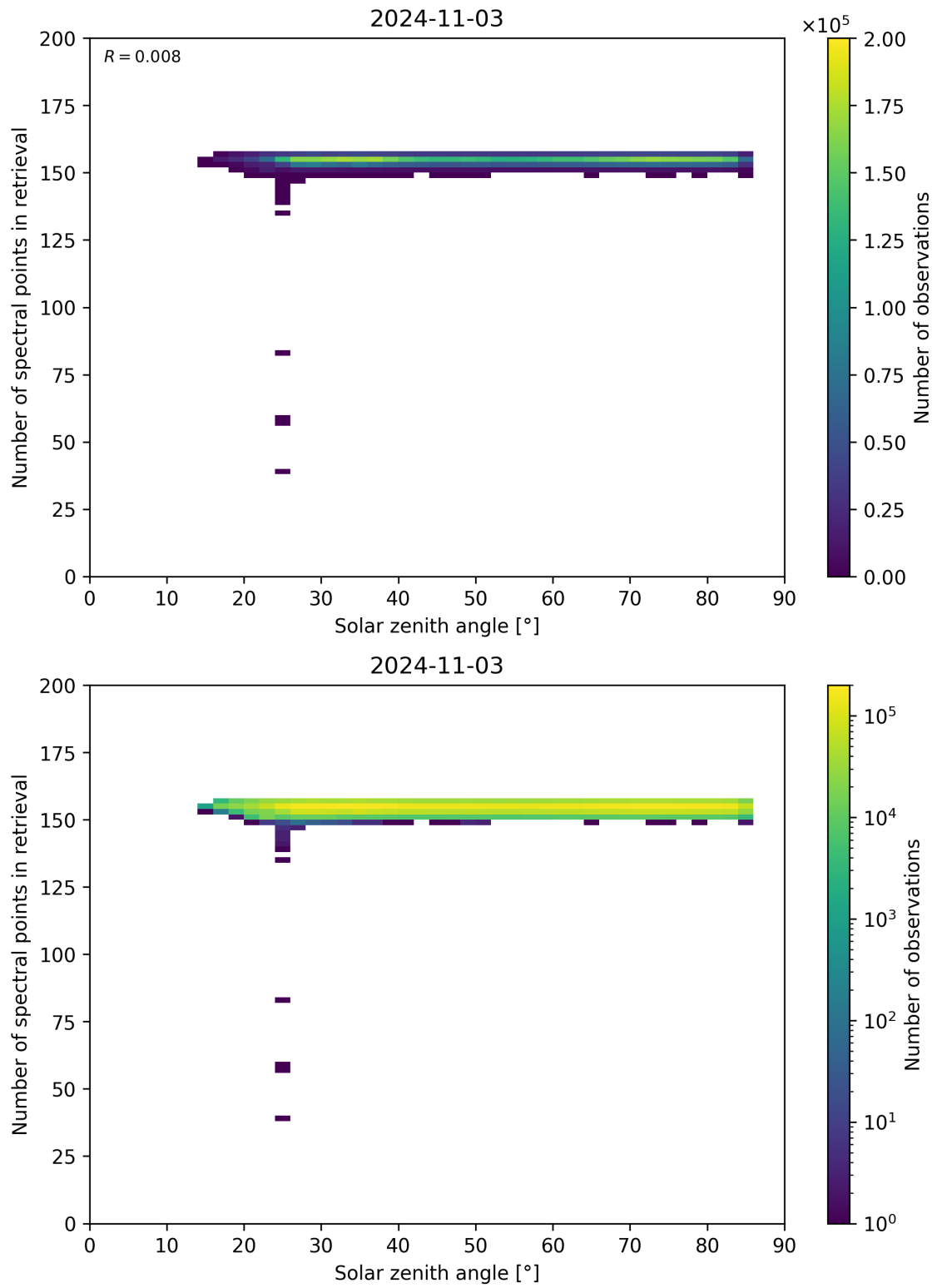
Figure 68: Scatter density plot of “Solar zenith angle” against “Number of spectral points in retrieval” for 2024-11-02 to 2024-11-04.
