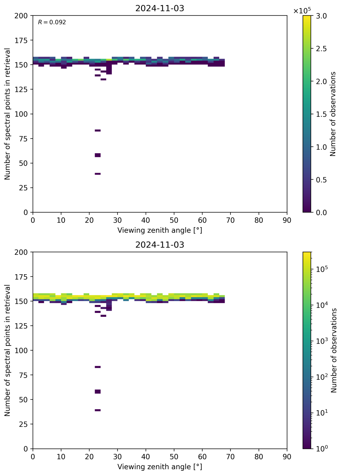
Figure 76: Scatter density plot of “Viewing zenith angle” against “Number of spectral points in retrieval” for 2024-11-02 to 2024-11-04.
