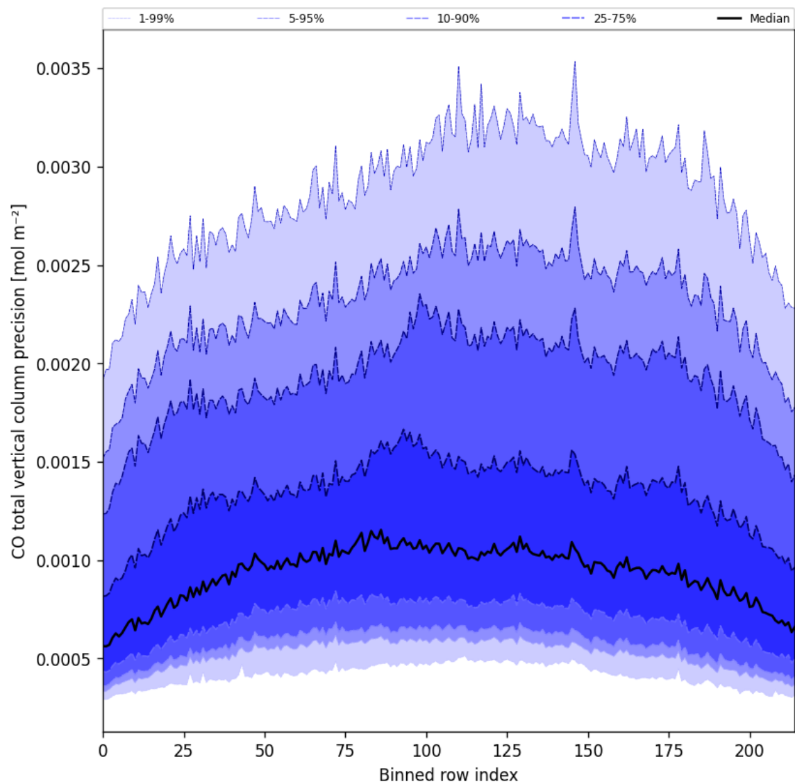
Figure 28: Along track statistics of “CO total vertical column precision” for 2024-11-02 to 2024-11-04
