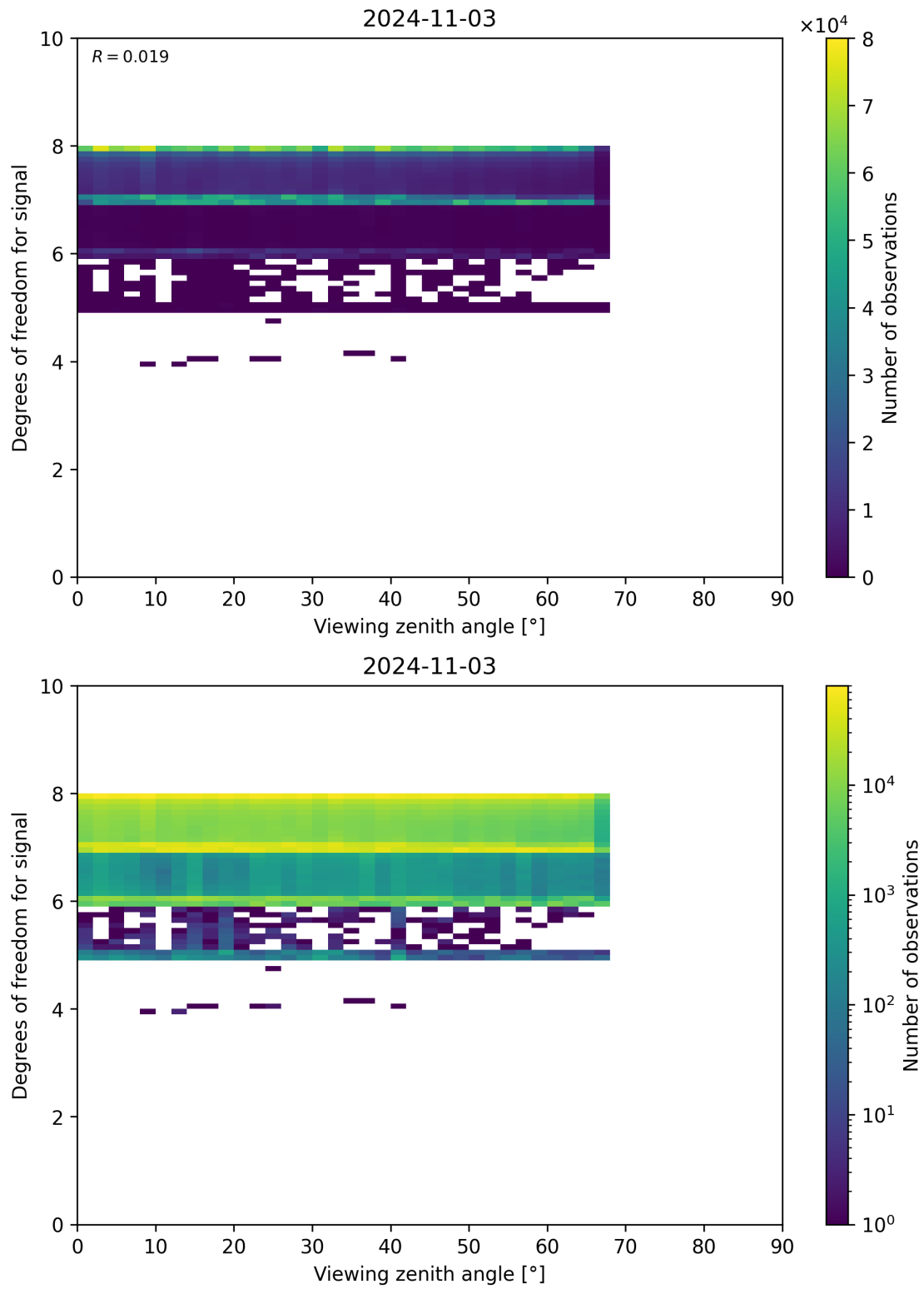
Figure 73: Scatter density plot of “Viewing zenith angle” against “Degrees of freedom for signal” for 2024-11-02 to 2024-11-04.
