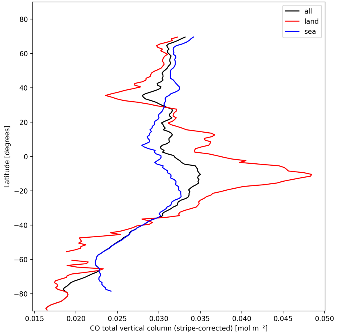
Figure 11: Zonal average of “CO total vertical column (stripe-corrected)” for 2024-11-02 to 2024-11-04.
