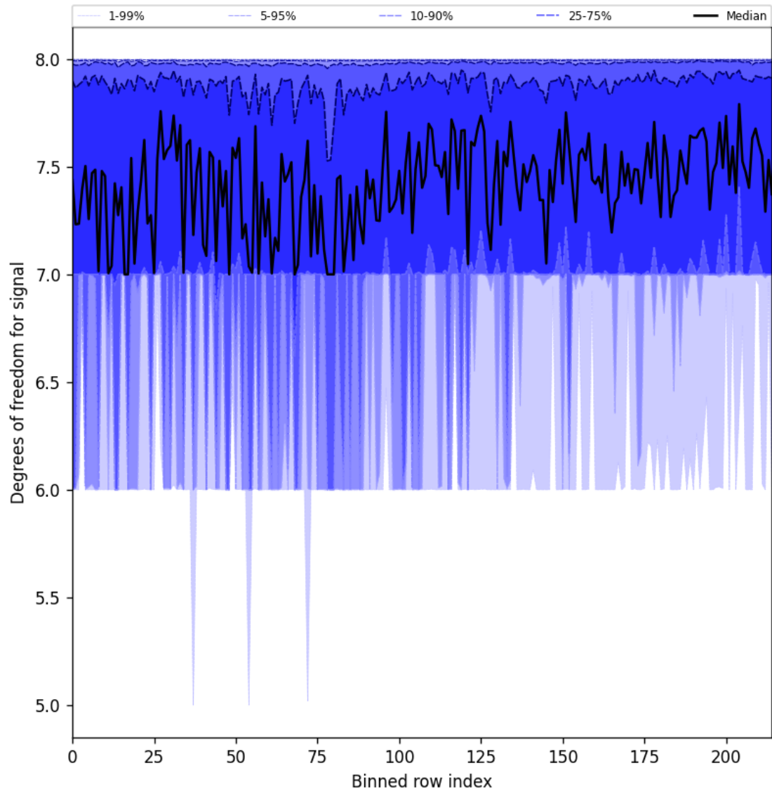
Figure 31: Along track statistics of “Degrees of freedom for signal” for 2024-11-02 to 2024-11-04
