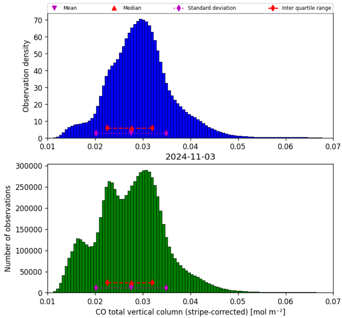
Figure 19: Histogram of “CO total vertical column (stripe-corrected)” for 2024-11-02 to 2024-11-04
