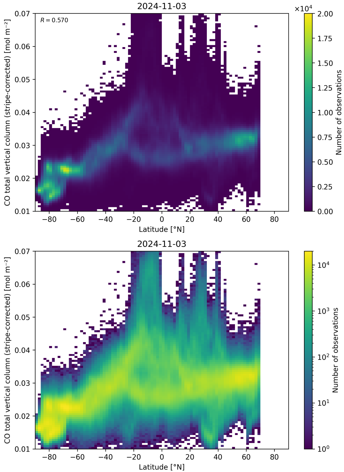
Figure 52: Scatter density plot of “Latitude” against “CO total vertical column (stripe-corrected)” for 2024-11-02 to 2024-11-04.
