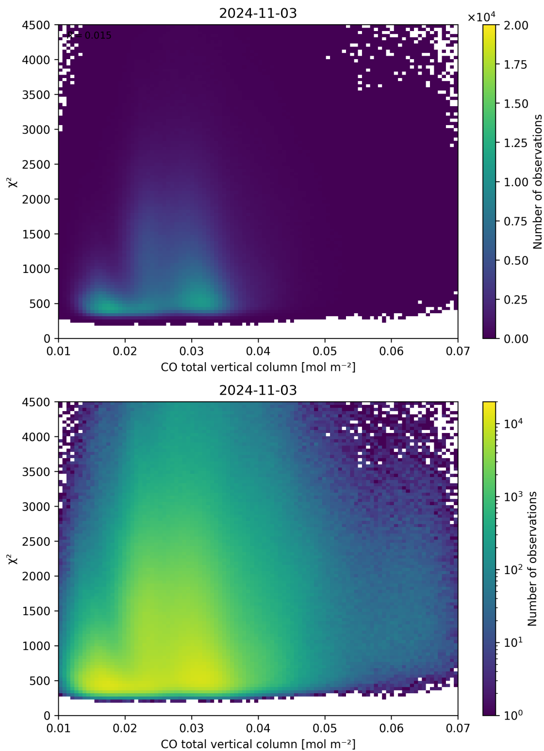
Figure 35: Scatter density plot of “CO total vertical column” against “ \chi^2 ” for 2024-11-02 to 2024-11-04.
