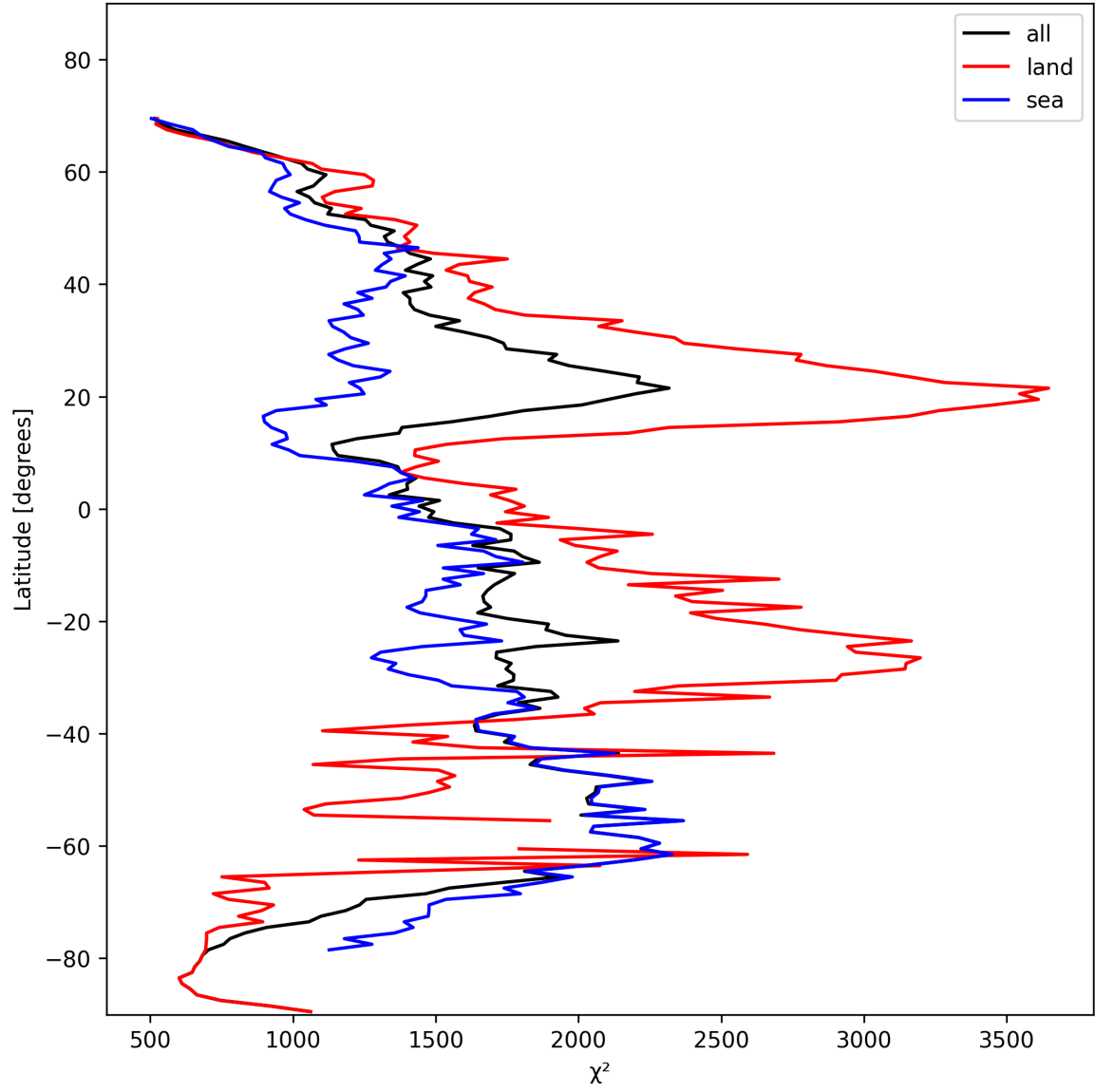
Figure 14: Zonal average of “ \chi^2 ” for 2024-11-02 to 2024-11-04.
