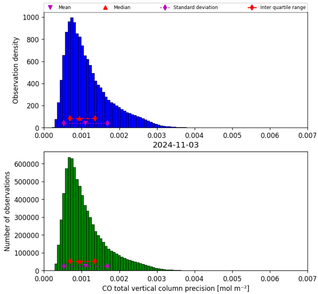
Figure 20: Histogram of “CO total vertical column precision” for 2024-11-02 to 2024-11-04
