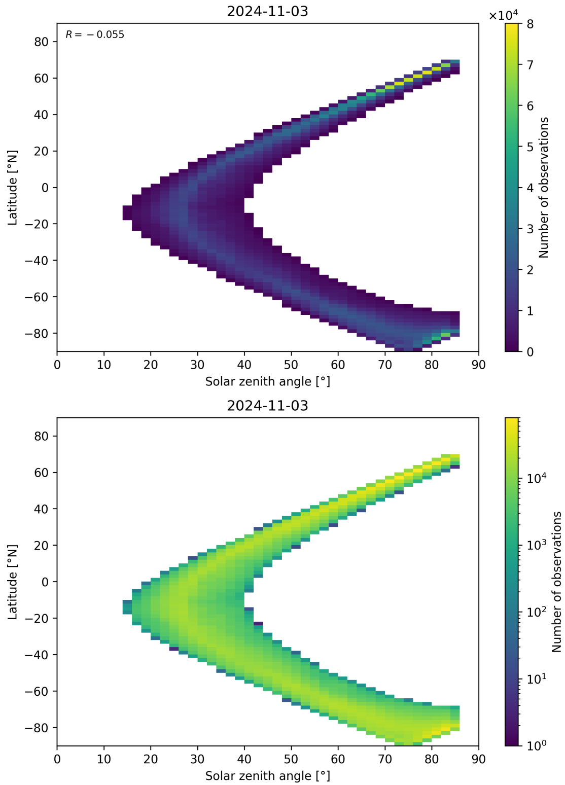
Figure 66: Scatter density plot of “Solar zenith angle” against “Latitude” for 2024-11-02 to 2024-11-04.
