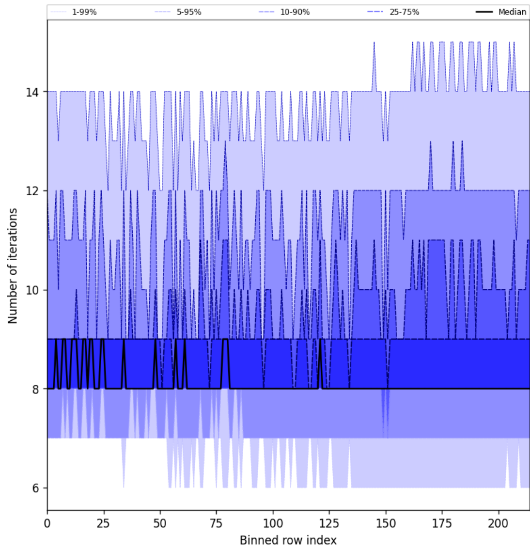
Figure 32: Along track statistics of “Number of iterations” for 2024-11-02 to 2024-11-04
