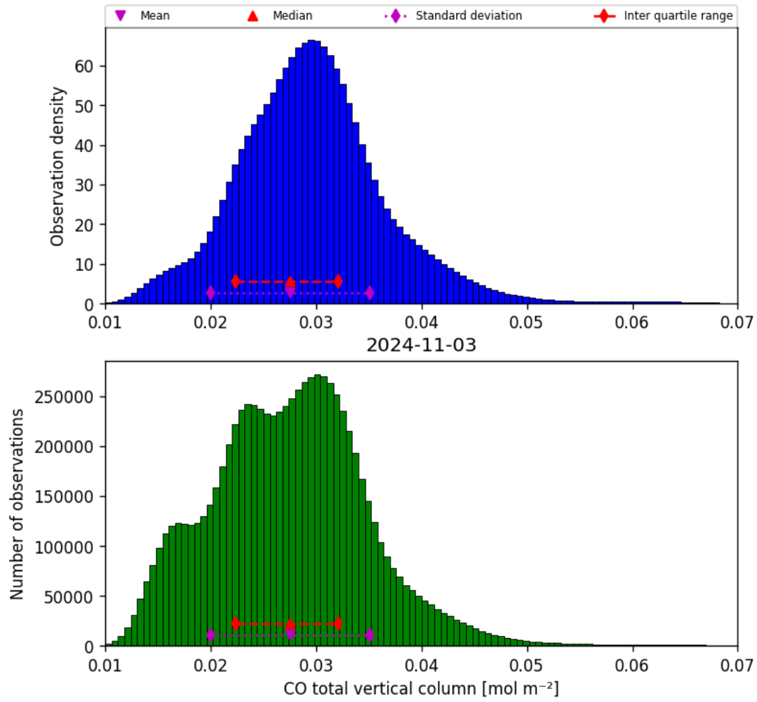
Figure 18: Histogram of “CO total vertical column” for 2024-11-02 to 2024-11-04
