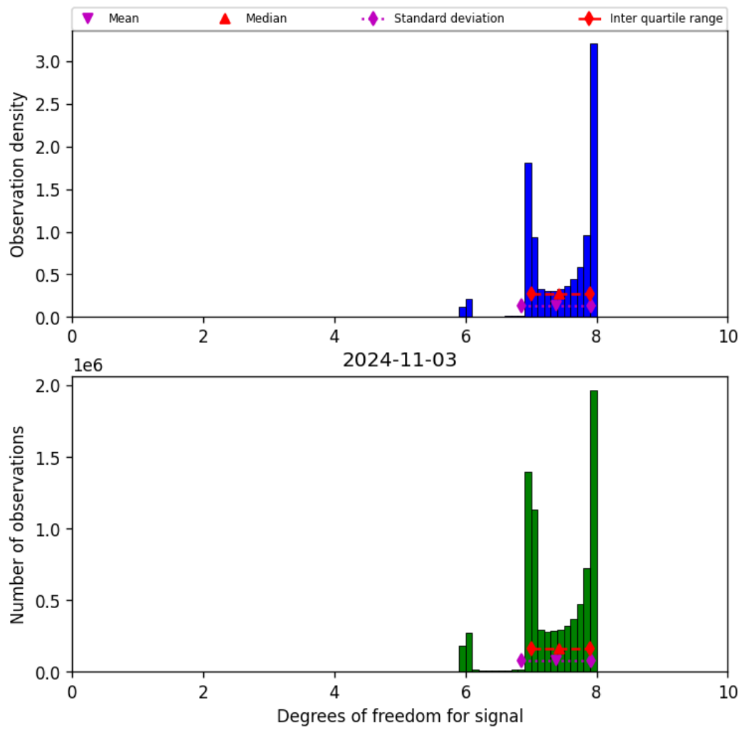
Figure 23: Histogram of “Degrees of freedom for signal” for 2024-11-02 to 2024-11-04
