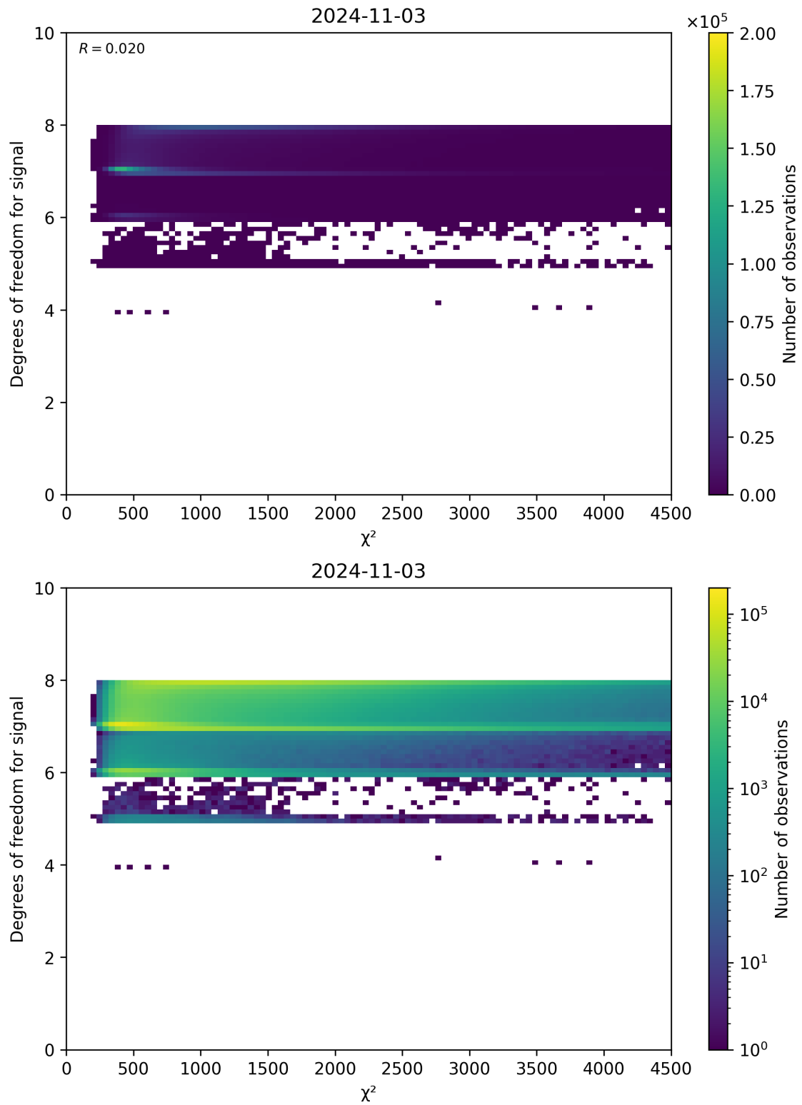
Figure 48: Scatter density plot of “ \chi^2 ” against “Degrees of freedom for signal” for 2024-11-02 to 2024-11-04.
