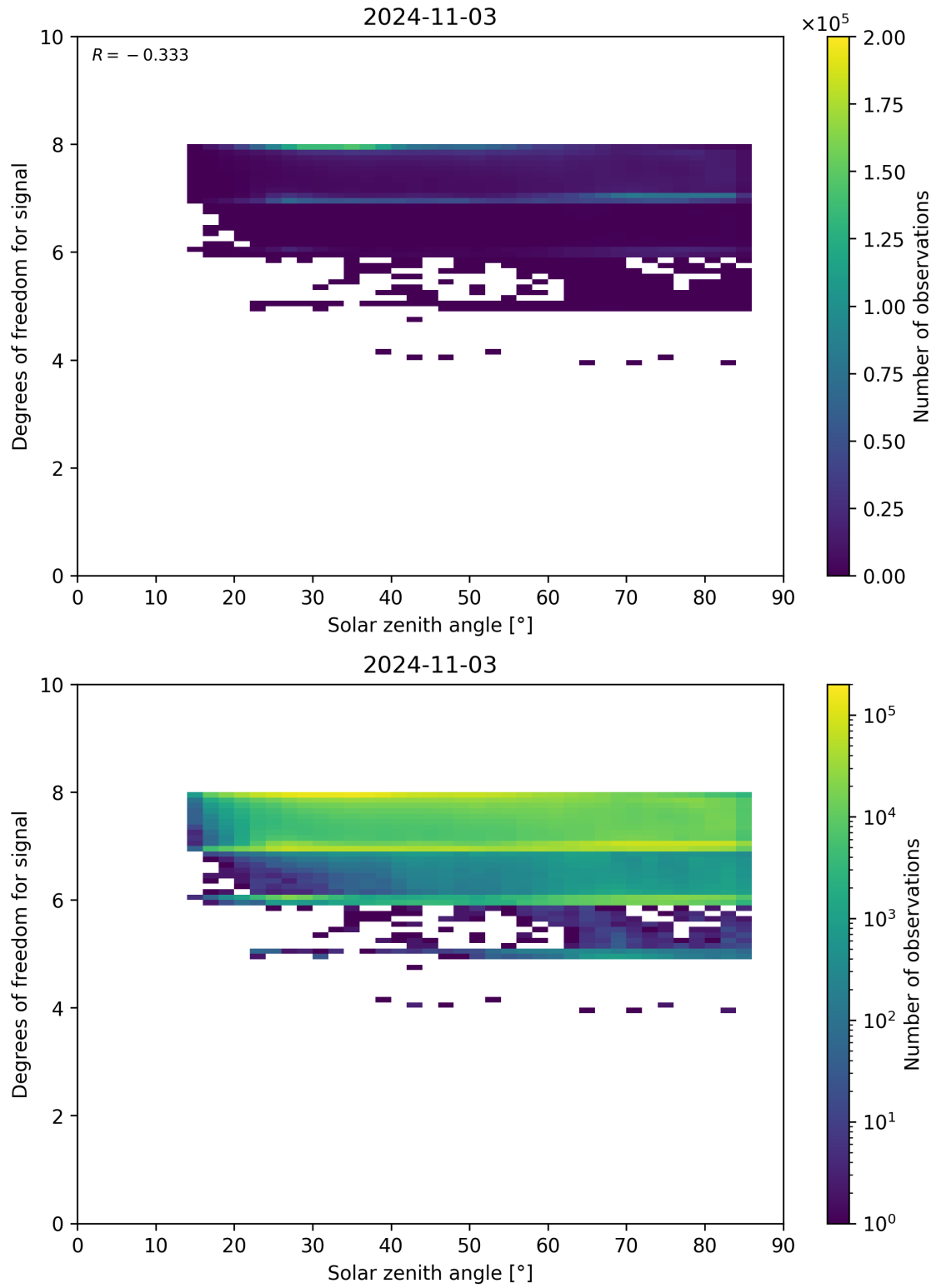
Figure 65: Scatter density plot of “Solar zenith angle” against “Degrees of freedom for signal” for 2024-11-02 to 2024-11-04.
