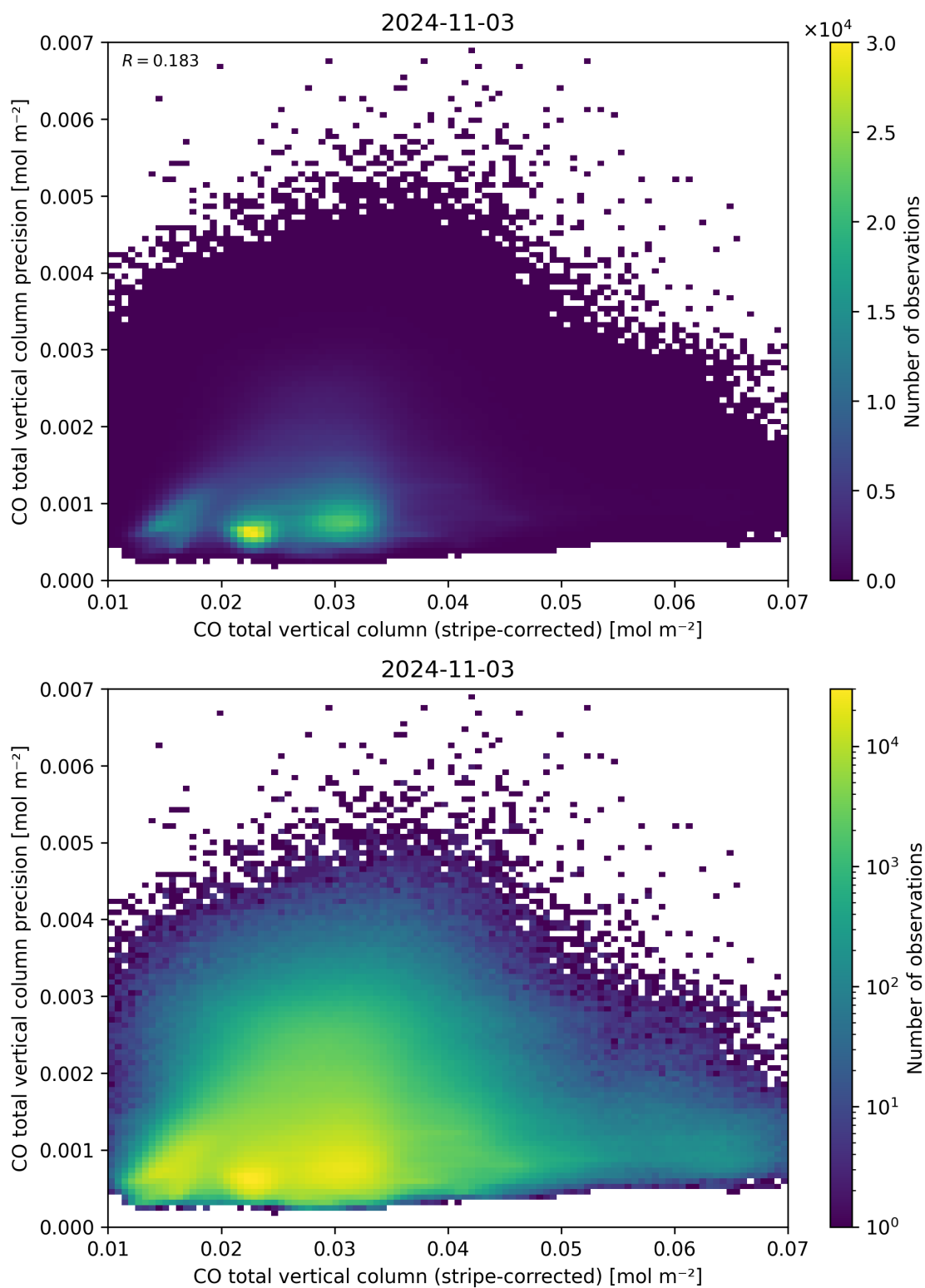
Figure 36: Scatter density plot of “CO total vertical column (stripe-corrected)” against “CO total vertical column precision” for 2024-11-02 to 2024-11-04.
