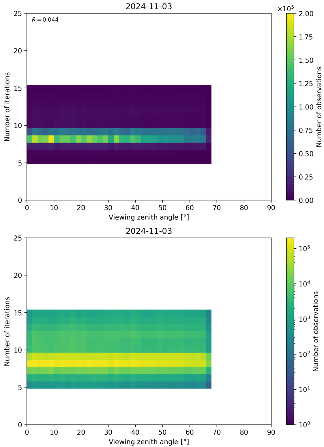
Figure 75: Scatter density plot of “Viewing zenith angle” against “Number of iterations” for 2024-11-02 to 2024-11-04.
