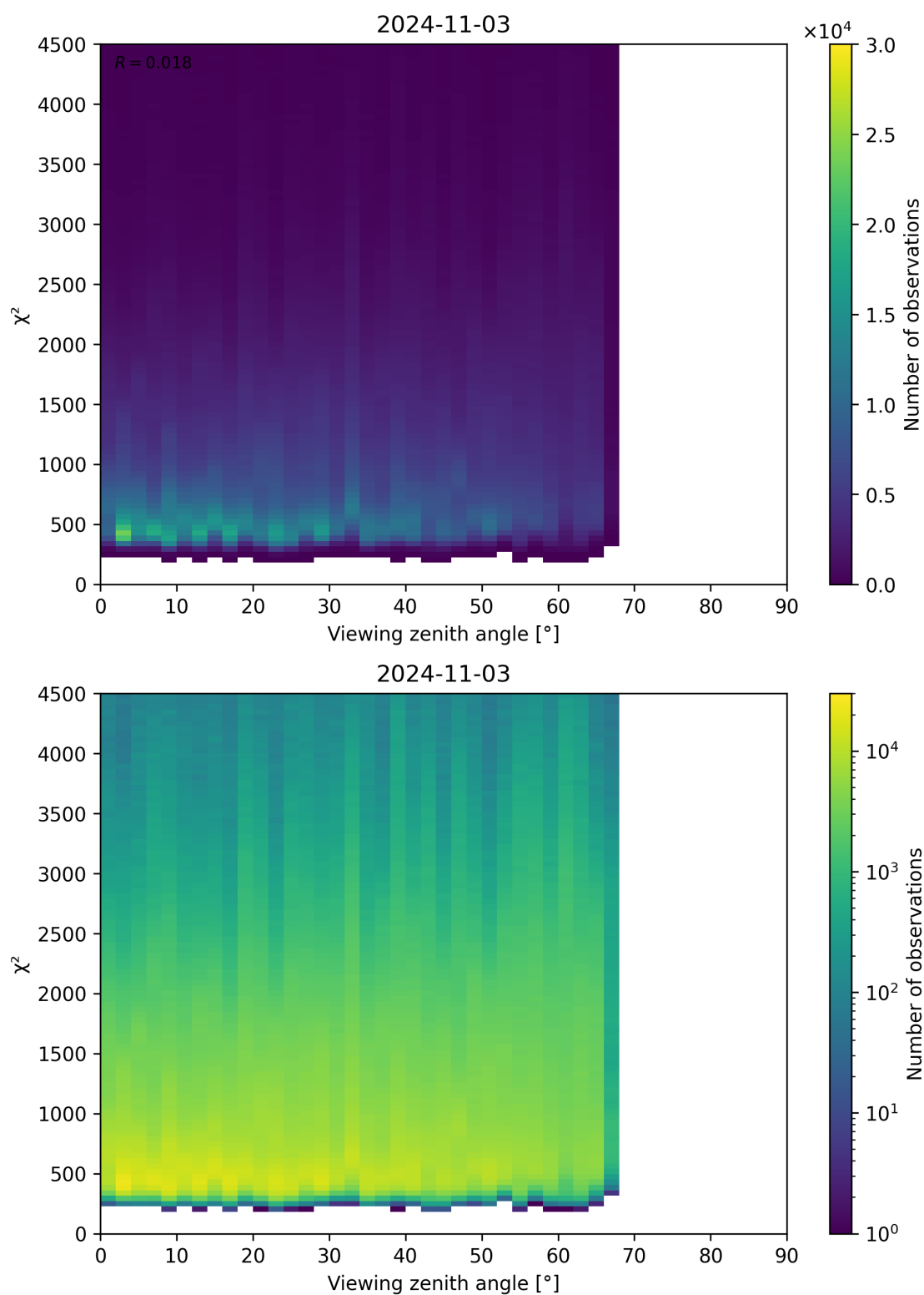
Figure 72: Scatter density plot of “Viewing zenith angle” against “ \chi^2 ” for 2024-11-02 to 2024-11-04.
