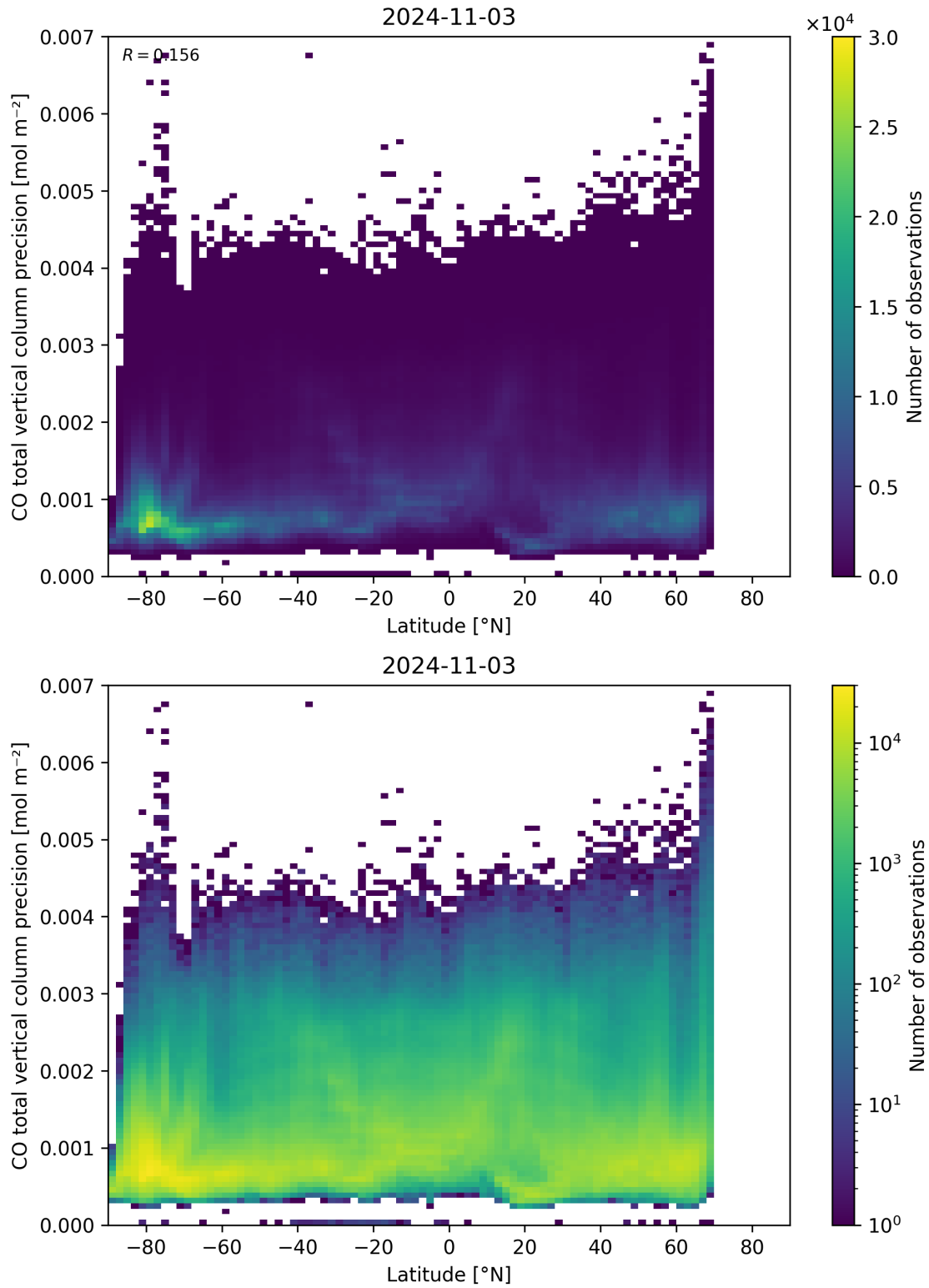
Figure 53: Scatter density plot of “Latitude” against “CO total vertical column precision” for 2024-11-02 to 2024-11-04.
