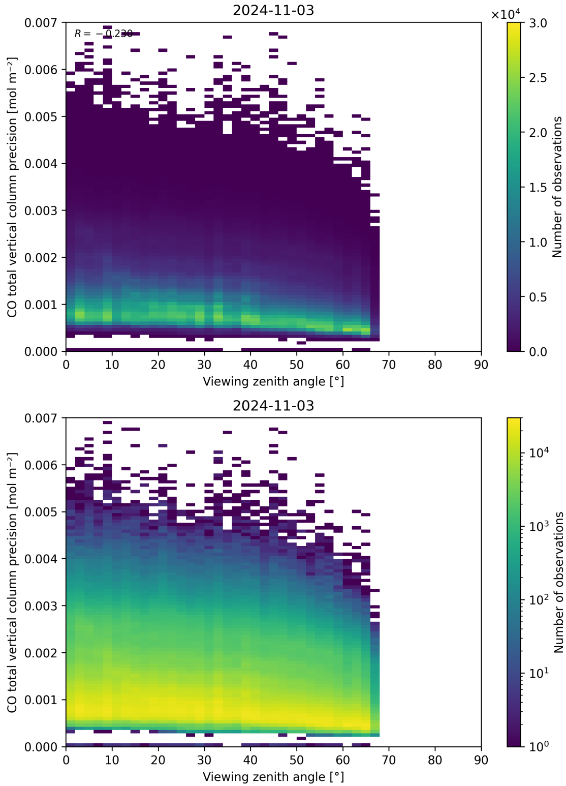
Figure 71: Scatter density plot of “Viewing zenith angle” against “CO total vertical column precision” for 2024-11-02 to 2024-11-04.
