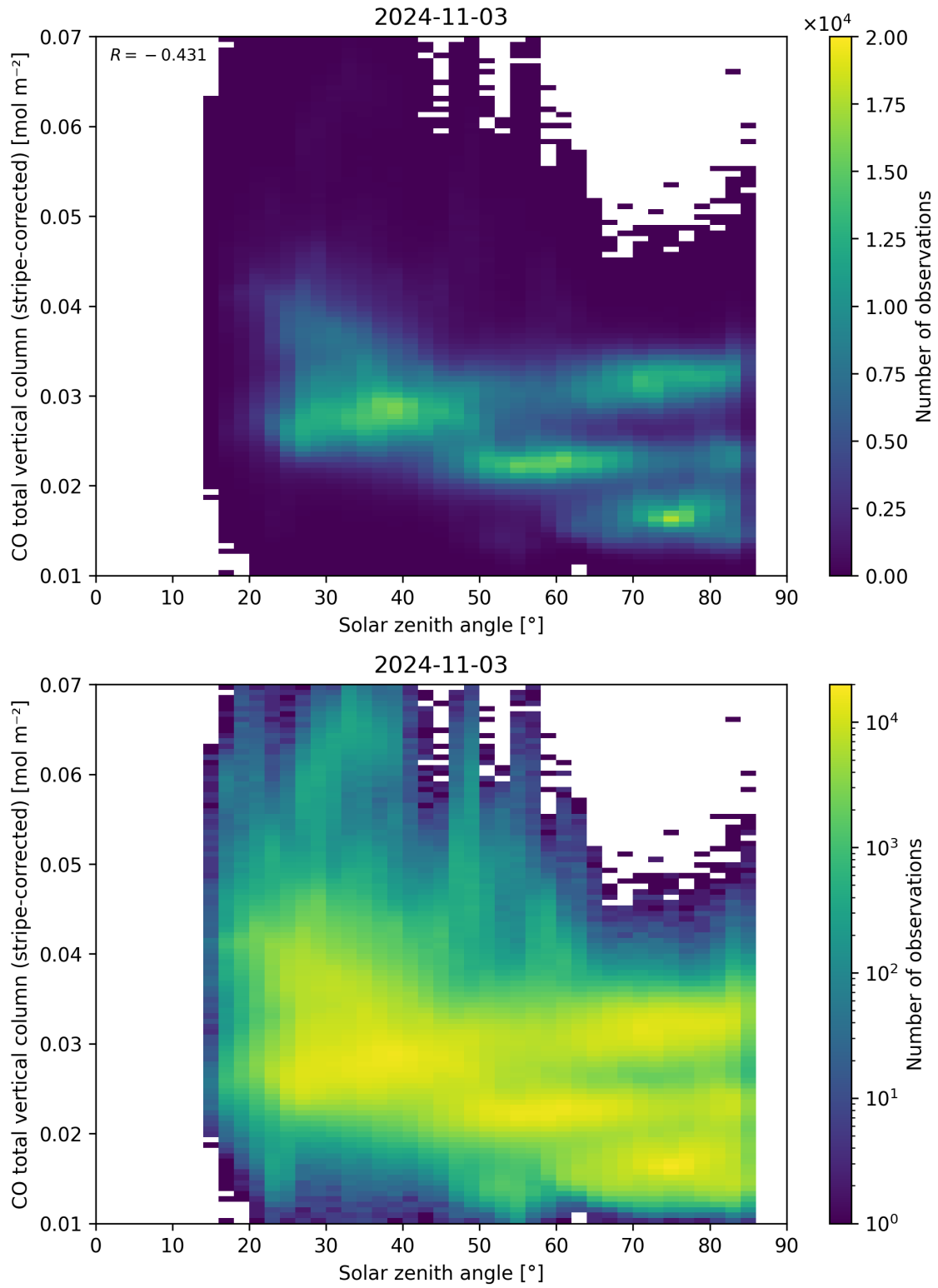
Figure 62: Scatter density plot of “Solar zenith angle” against “CO total vertical column (stripe-corrected)” for 2024-11-02 to 2024-11-04.
