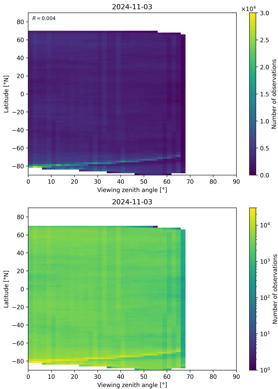
Figure 74: Scatter density plot of “Viewing zenith angle” against “Latitude” for 2024-11-02 to 2024-11-04.
