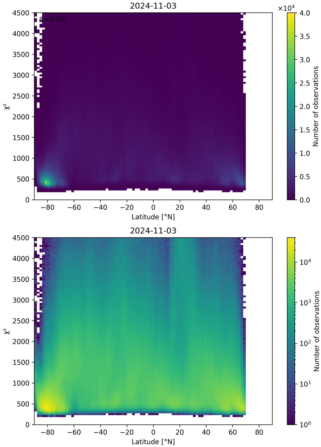
Figure 54: Scatter density plot of “Latitude” against “ \chi^2 ” for 2024-11-02 to 2024-11-04.
