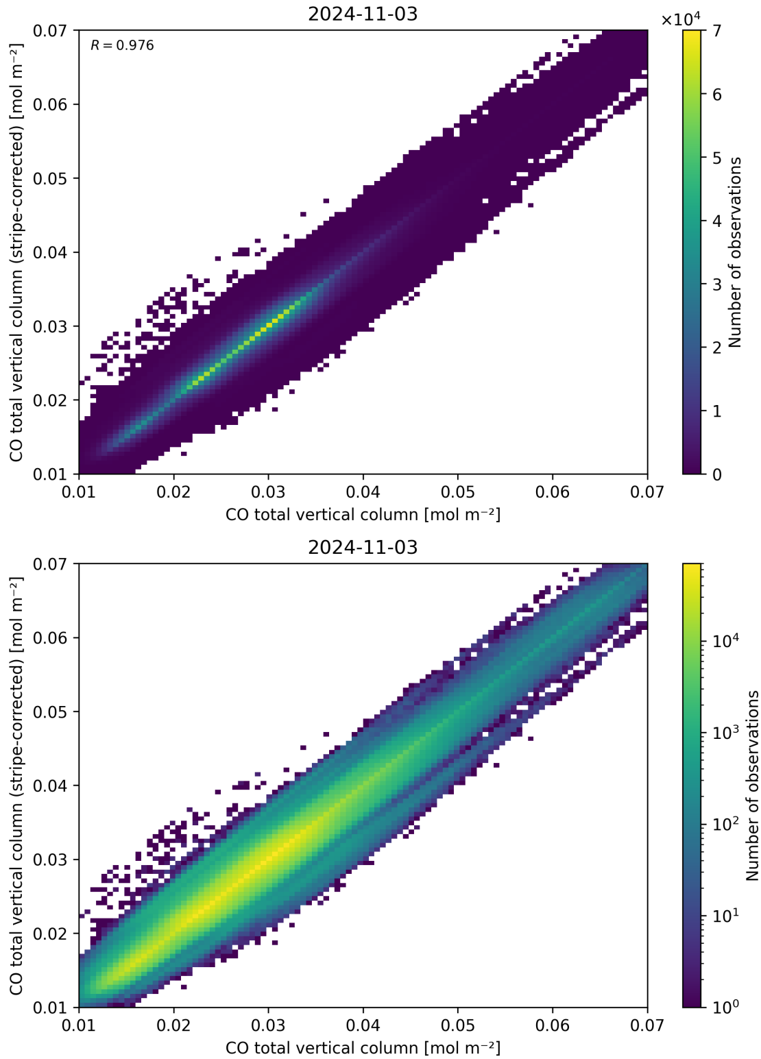
Figure 33: Scatter density plot of “CO total vertical column” against “CO total vertical column (stripe-corrected)” for 2024-11-02 to 2024-11-04.
