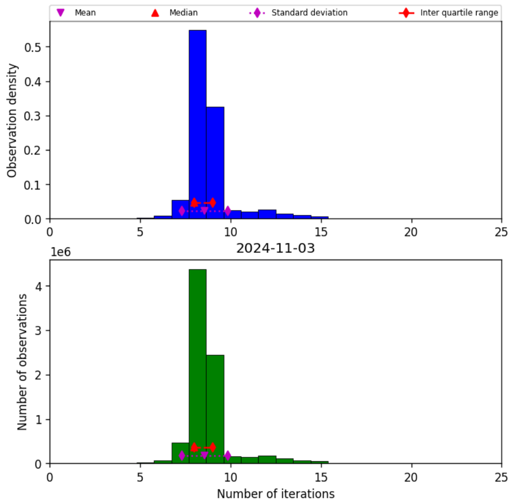
Figure 24: Histogram of “Number of iterations” for 2024-11-02 to 2024-11-04
