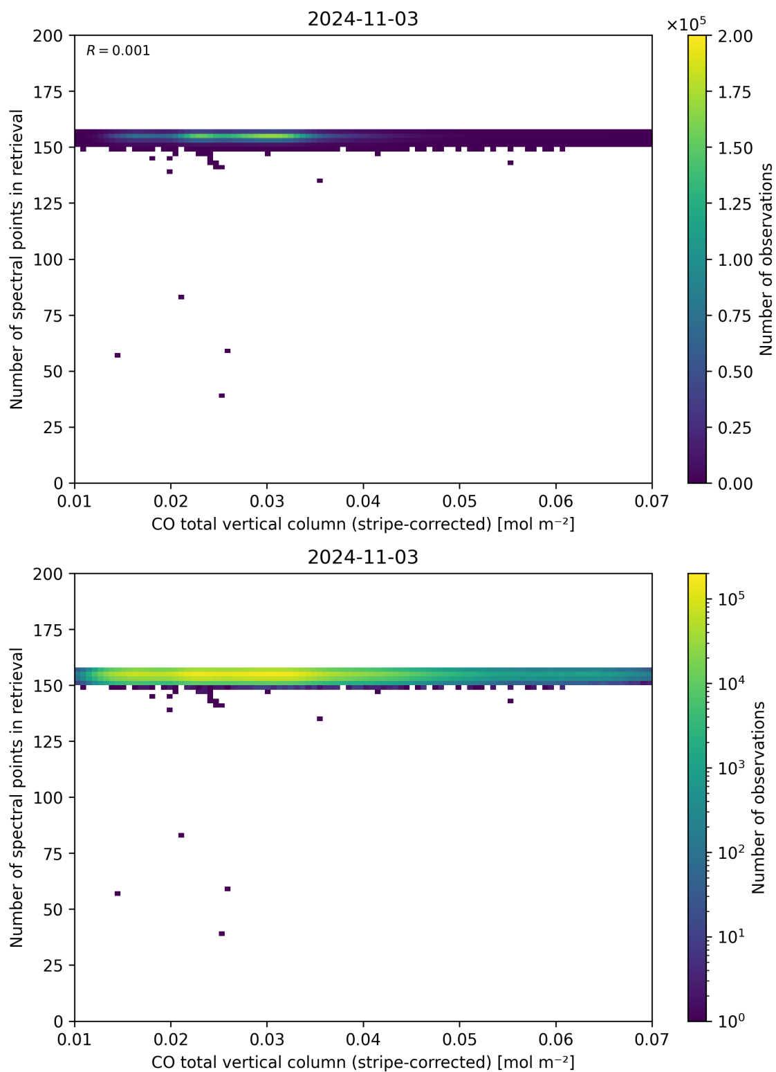
Figure 40: Scatter density plot of “CO total vertical column (stripe-corrected)” against “Number of spectral points in retrieval” for 2024-11-02 to 2024-11-04.
