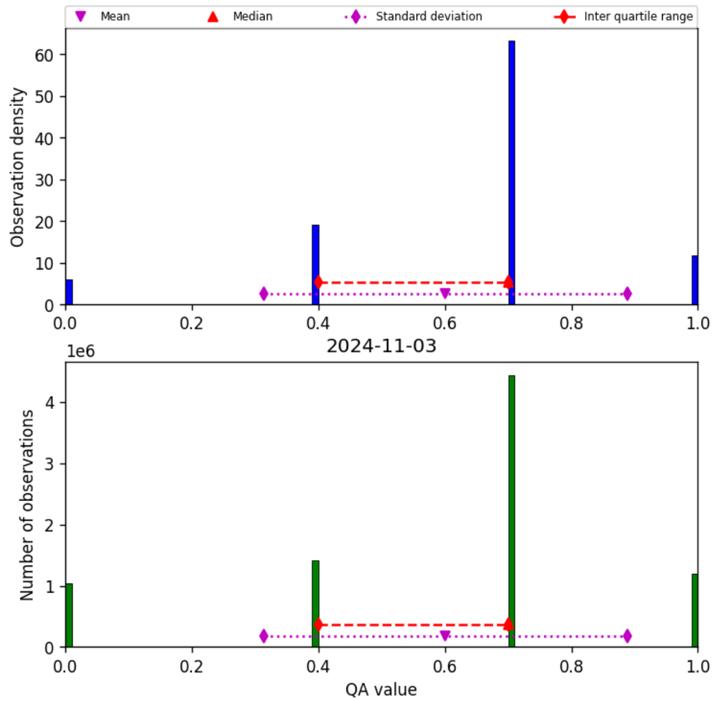
Figure 17: Histogram of “QA value” for 2024-11-02 to 2024-11-04
