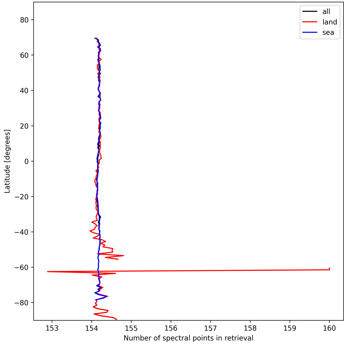
Figure 13: Zonal average of “Number of spectral points in retrieval” for 2024-11-02 to 2024-11-04.
