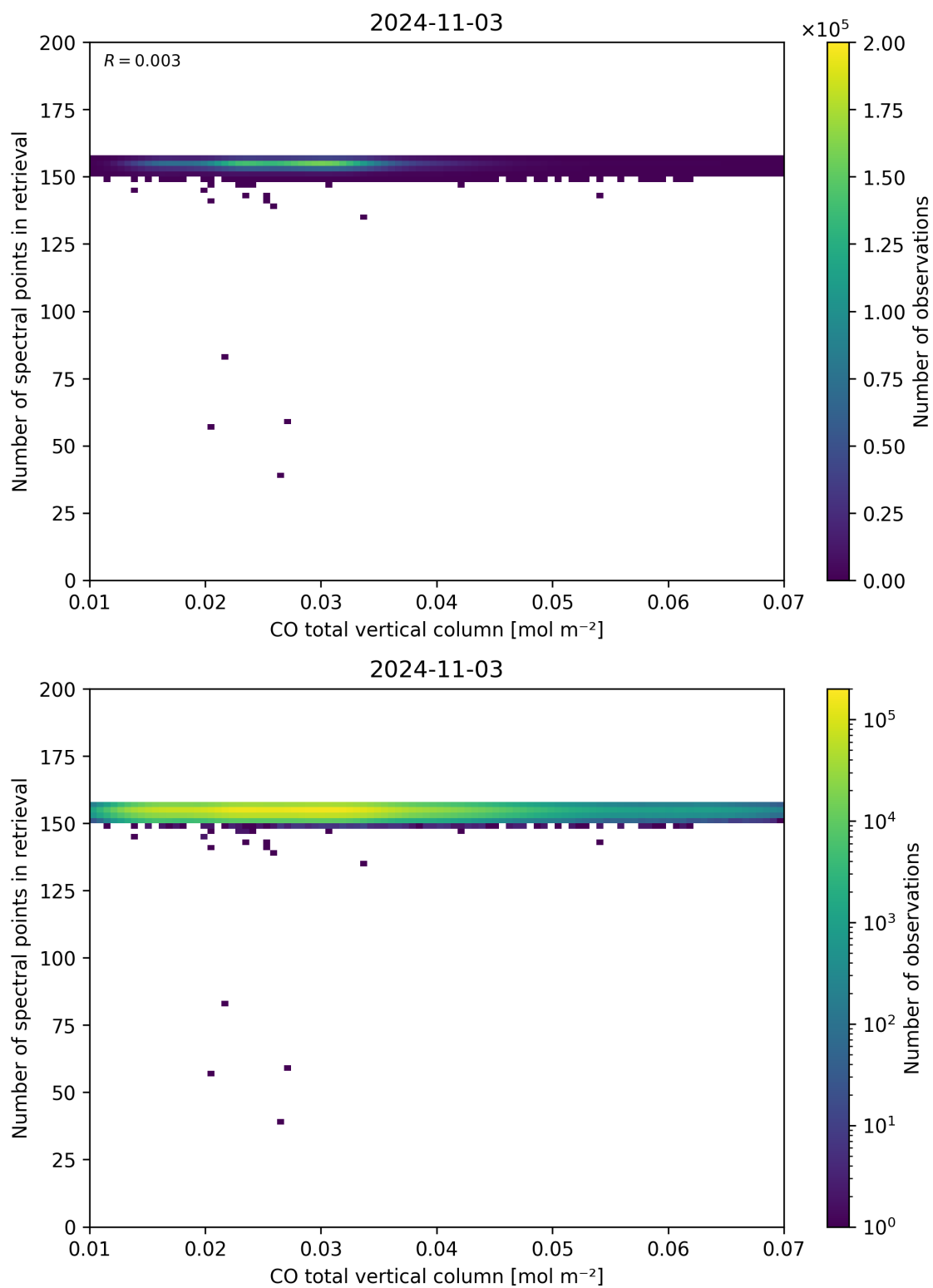
Figure 43: Scatter density plot of “CO total vertical column” against “Number of spectral points in retrieval” for 2024-11-02 to 2024-11-04.
