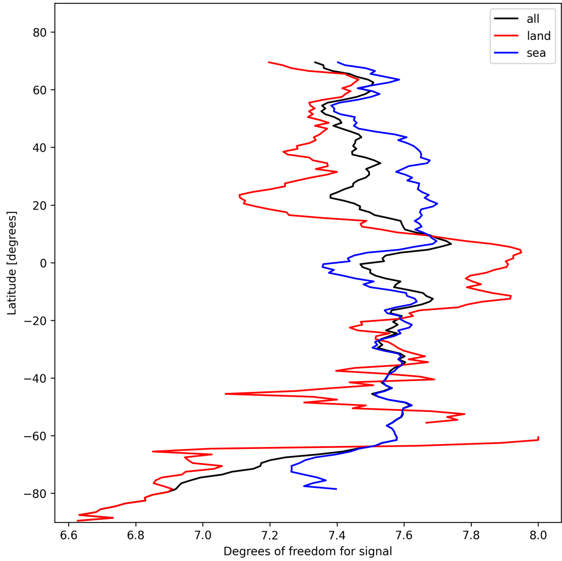
Figure 15: Zonal average of “Degrees of freedom for signal” for 2024-11-02 to 2024-11-04.
