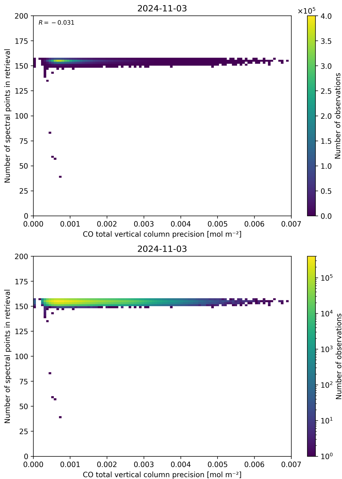
Figure 47: Scatter density plot of “CO total vertical column precision” against “Number of spectral points in retrieval” for 2024-11-02 to 2024-11-04.
