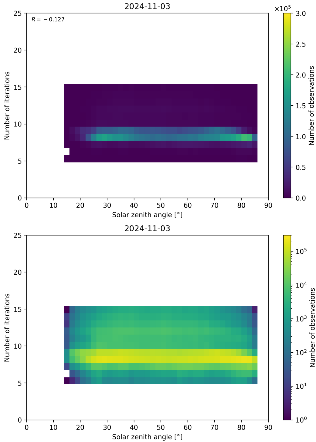
Figure 67: Scatter density plot of “Solar zenith angle” against “Number of iterations” for 2024-11-02 to 2024-11-04.
