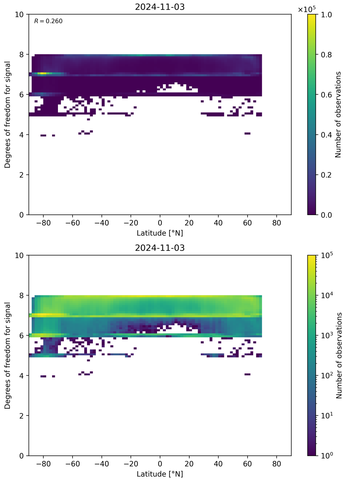
Figure 55: Scatter density plot of “Latitude” against “Degrees of freedom for signal” for 2024-11-02 to 2024-11-04.
