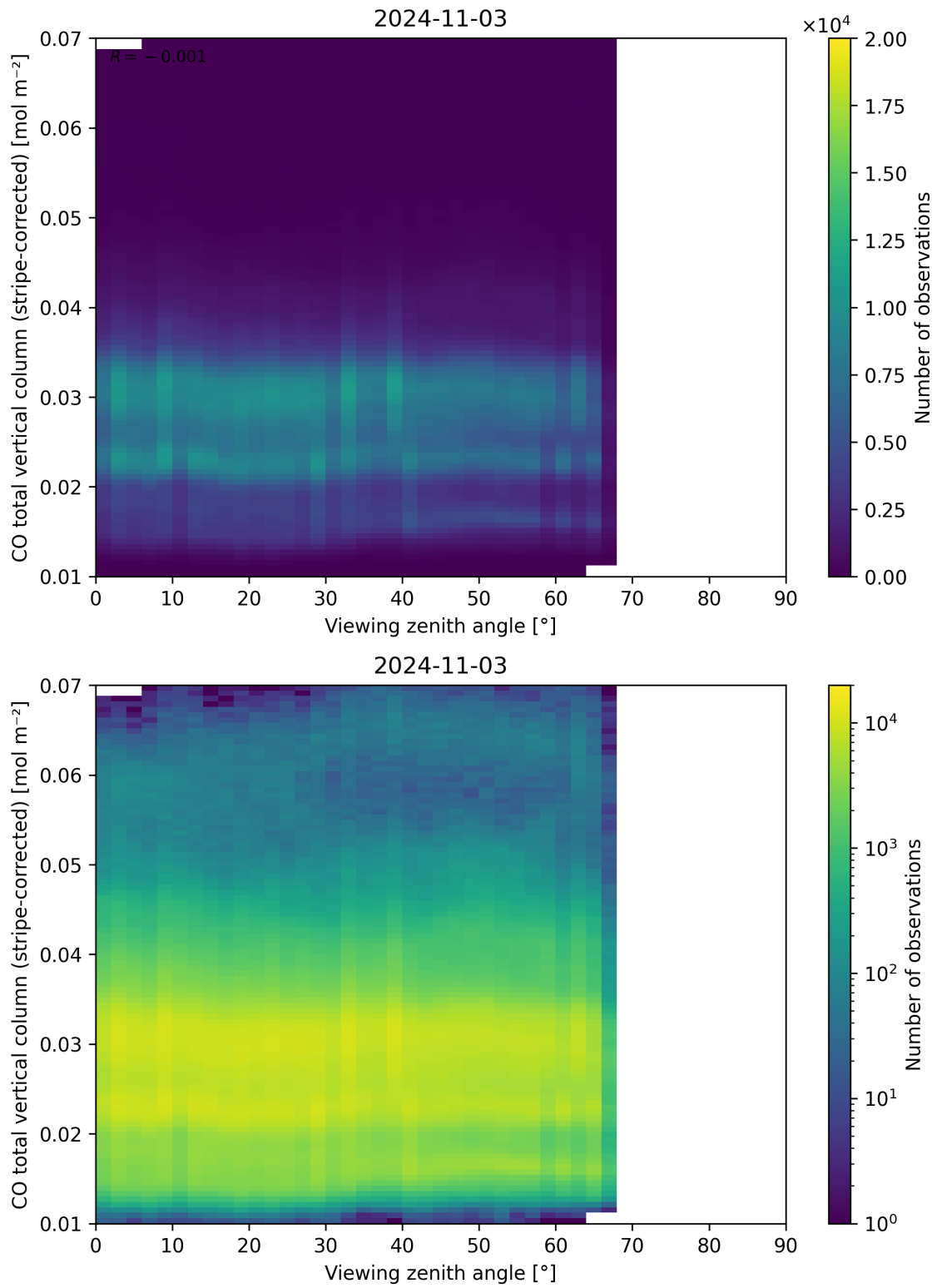
Figure 70: Scatter density plot of “Viewing zenith angle” against “CO total vertical column (stripe-corrected)” for 2024-11-02 to 2024-11-04.
