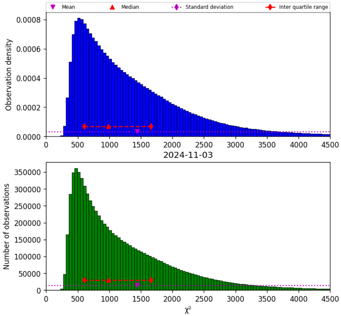
Figure 22: Histogram of " \chi^2 " for 2024-11-02 to 2024-11-04
