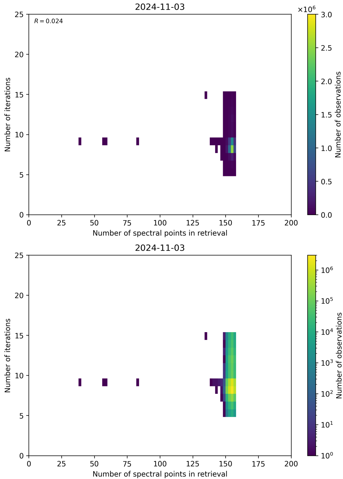
Figure 60: Scatter density plot of “Number of spectral points in retrieval” against “Number of iterations” for 2024-11-02 to 2024-11-04.
