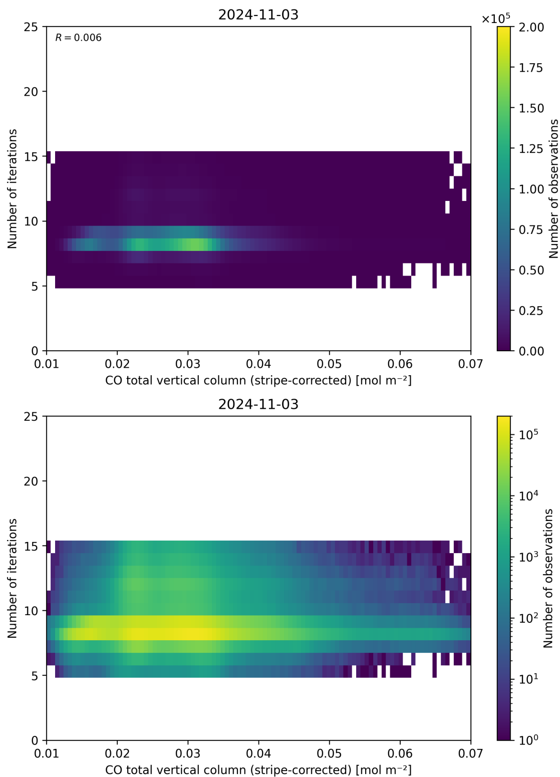
Figure 39: Scatter density plot of “CO total vertical column (stripe-corrected)” against “Number of iterations” for 2024-11-02 to 2024-11-04.
