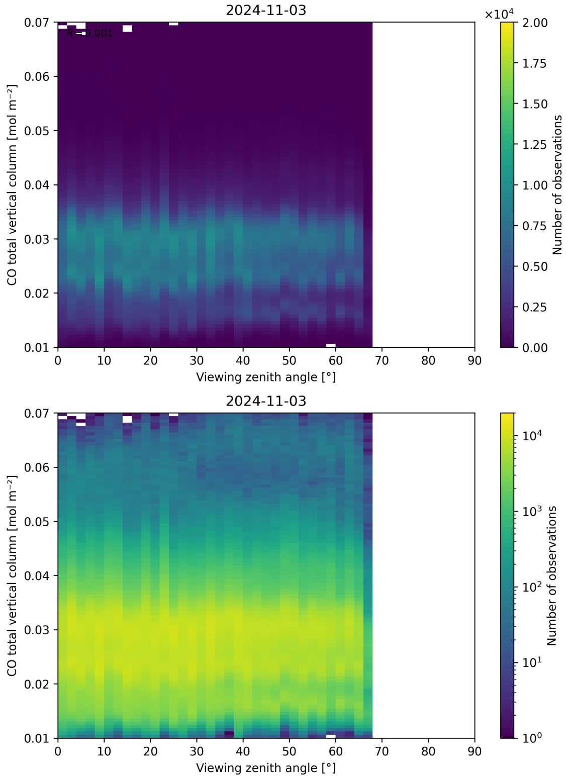
Figure 69: Scatter density plot of “Viewing zenith angle” against “CO total vertical column” for 2024-11-02 to 2024-11-04.
