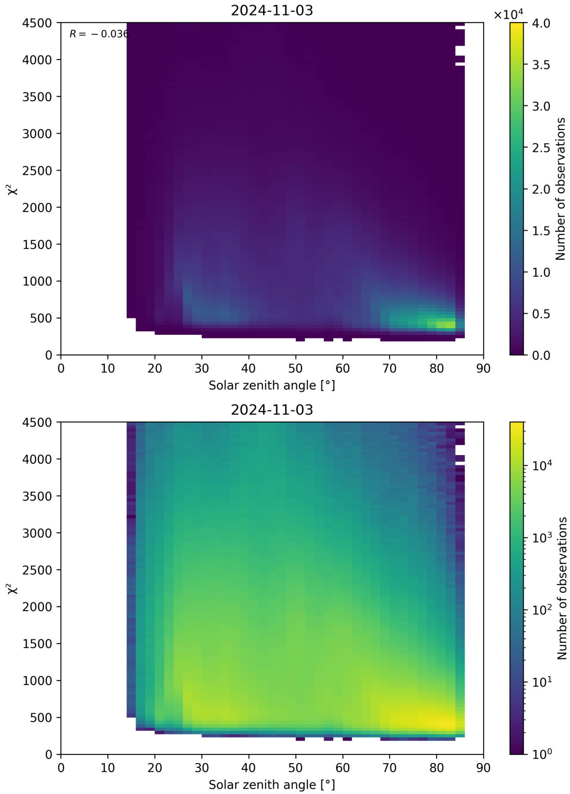
Figure 64: Scatter density plot of “Solar zenith angle” against “ \chi^2 ” for 2024-11-02 to 2024-11-04.
