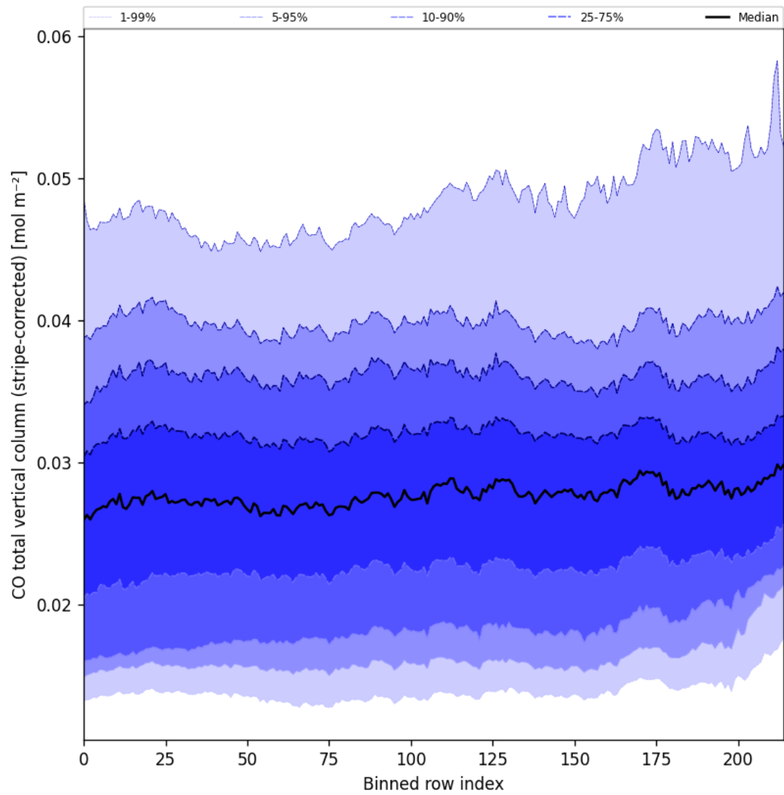
Figure 27: Along track statistics of “CO total vertical column (stripe-corrected)” for 2024-11-02 to 2024-11-04
