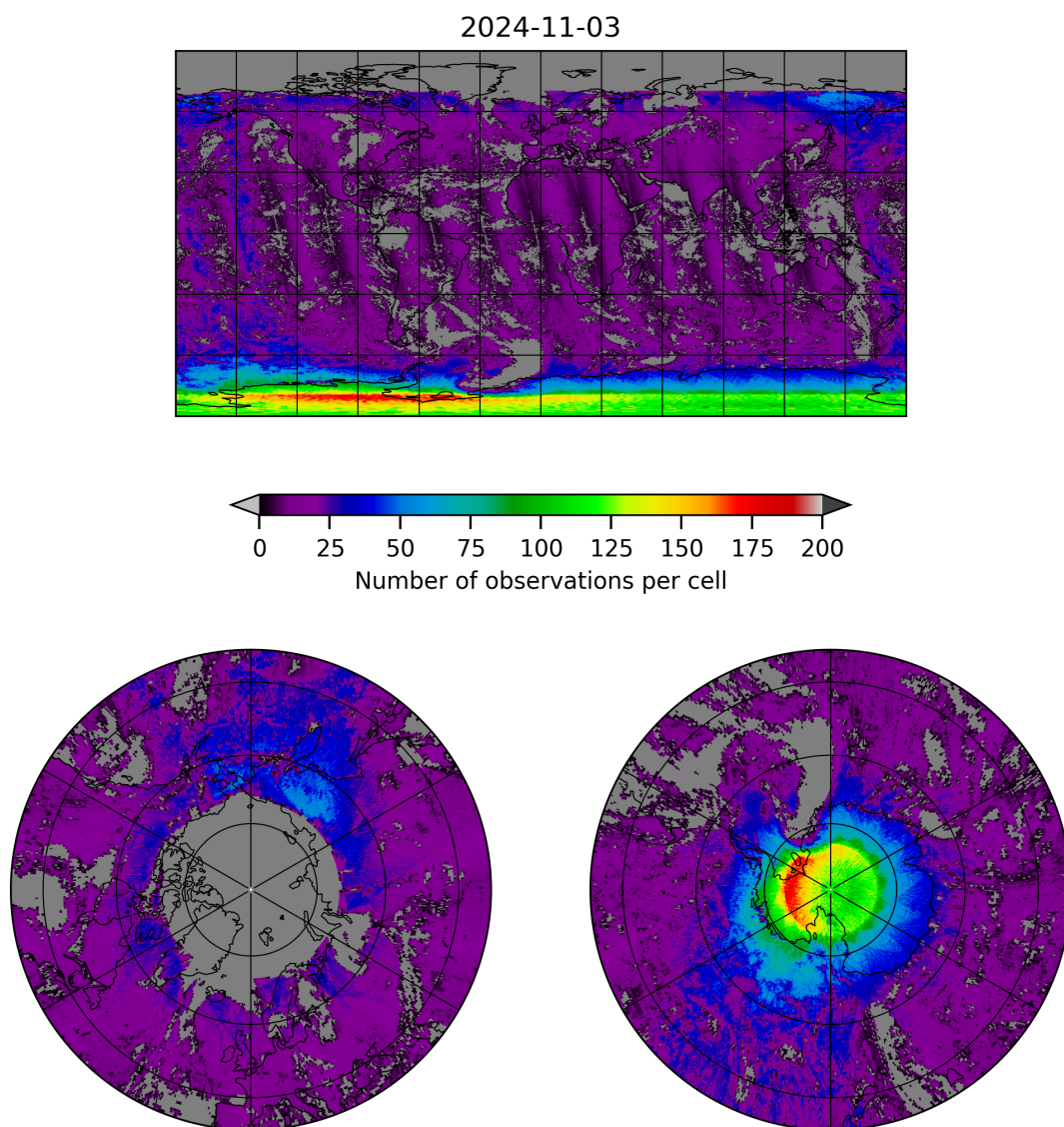
Figure 8: Map of the number of observations for 2024-11-02 to 2024-11-04
