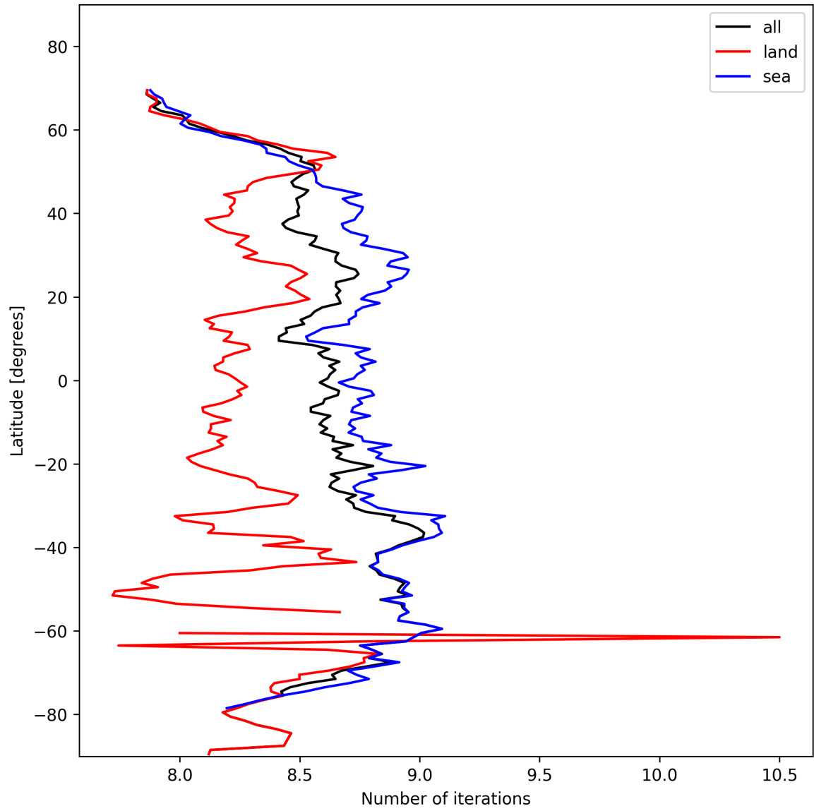
Figure 16: Zonal average of “Number of iterations” for 2024-11-02 to 2024-11-04.
