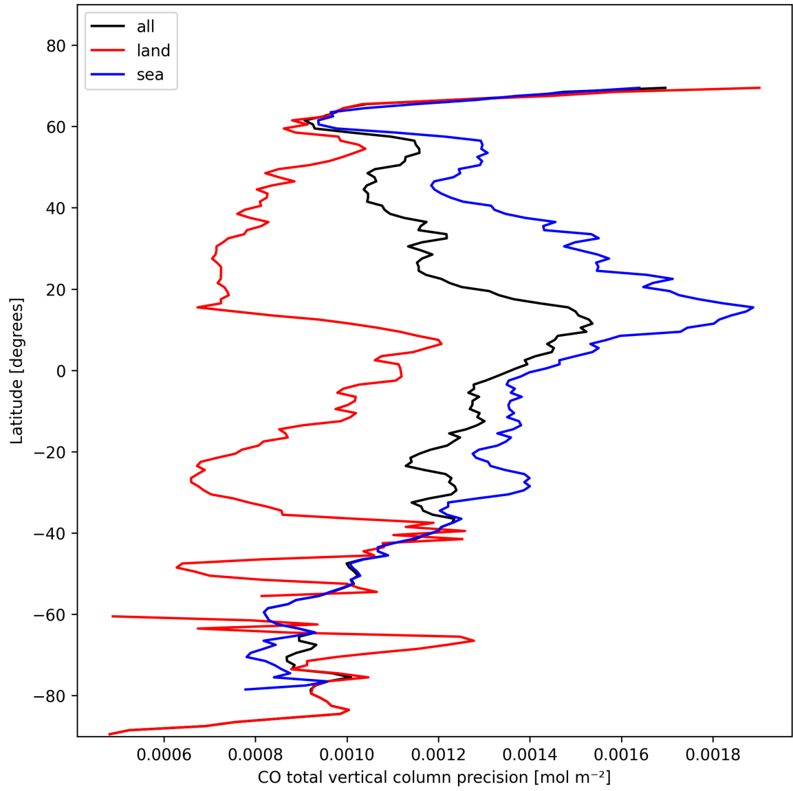
Figure 12: Zonal average of “CO total vertical column precision” for 2024-11-02 to 2024-11-04.
