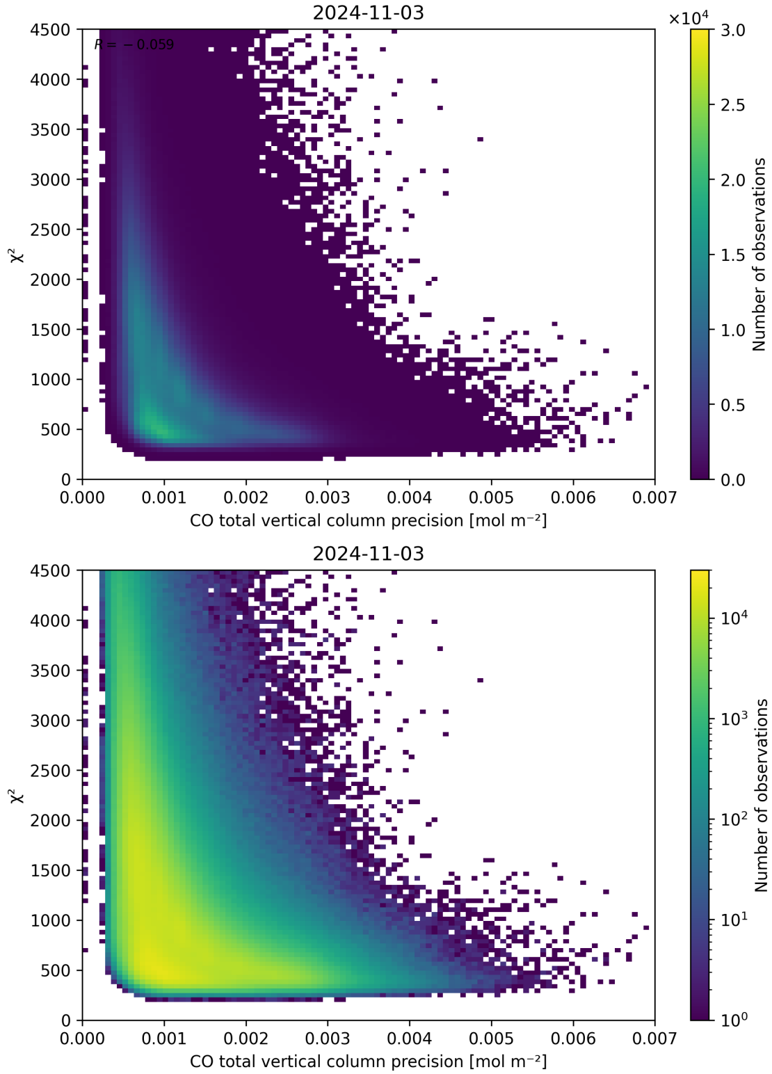
Figure 44: Scatter density plot of “CO total vertical column precision” against “ \chi^2 ” for 2024-11-02 to 2024-11-04.
