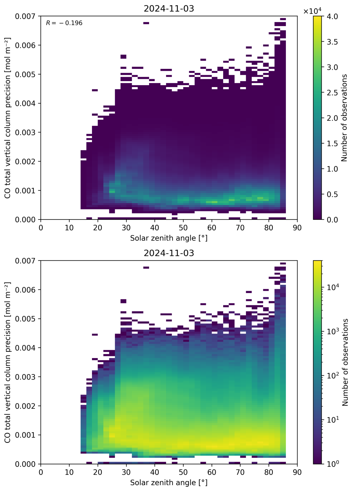
Figure 63: Scatter density plot of “Solar zenith angle” against “CO total vertical column precision” for 2024-11-02 to 2024-11-04.
