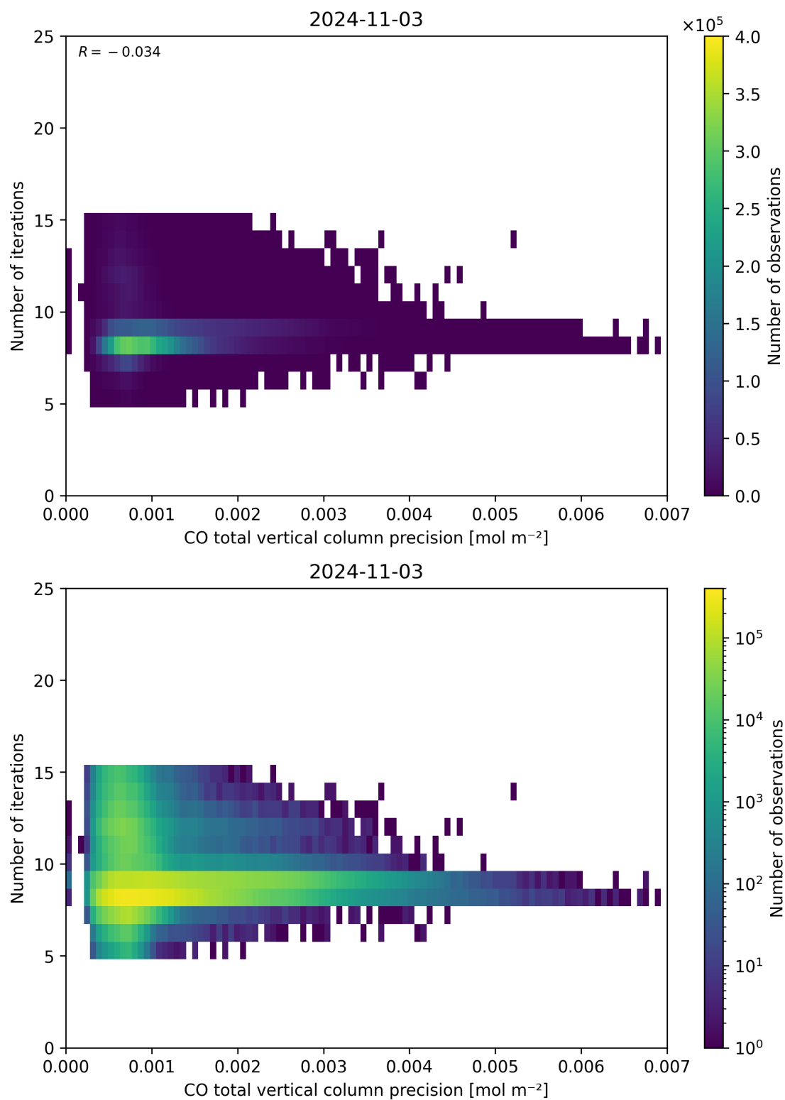
Figure 46: Scatter density plot of “CO total vertical column precision” against “Number of iterations” for 2024-11-02 to 2024-11-04.
