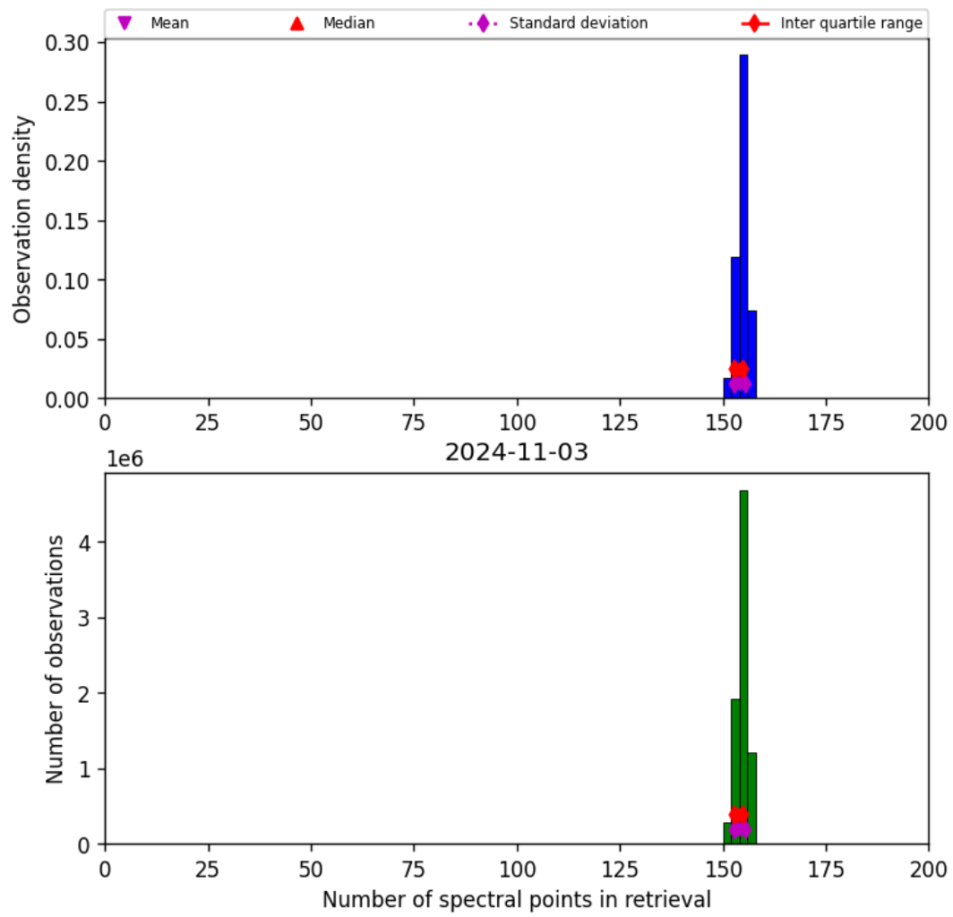
Figure 21: Histogram of “Number of spectral points in retrieval” for 2024-11-02 to 2024-11-04
