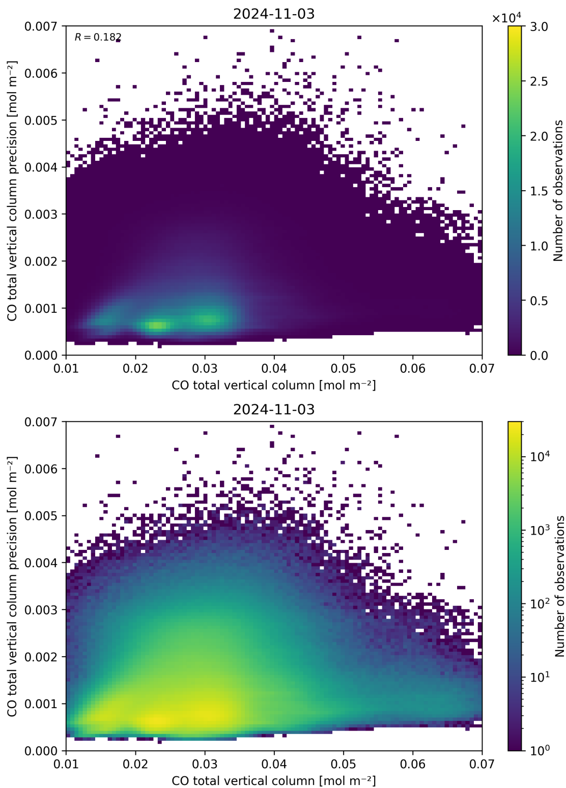
Figure 34: Scatter density plot of “CO total vertical column” against “CO total vertical column precision” for 2024-11-02 to 2024-11-04.
