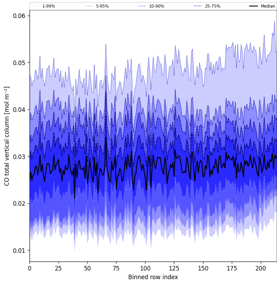
Figure 26: Along track statistics of “CO total vertical column” for 2024-11-02 to 2024-11-04
