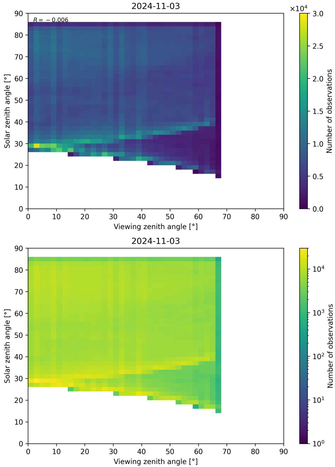
Figure 77: Scatter density plot of “Viewing zenith angle” against “Solar zenith angle” for 2024-11-02 to 2024-11-04.
