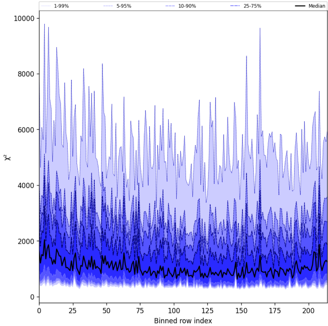
Figure 30: Along track statistics of “ \chi^2 ” for 2024-11-04 to 2024-11-05
