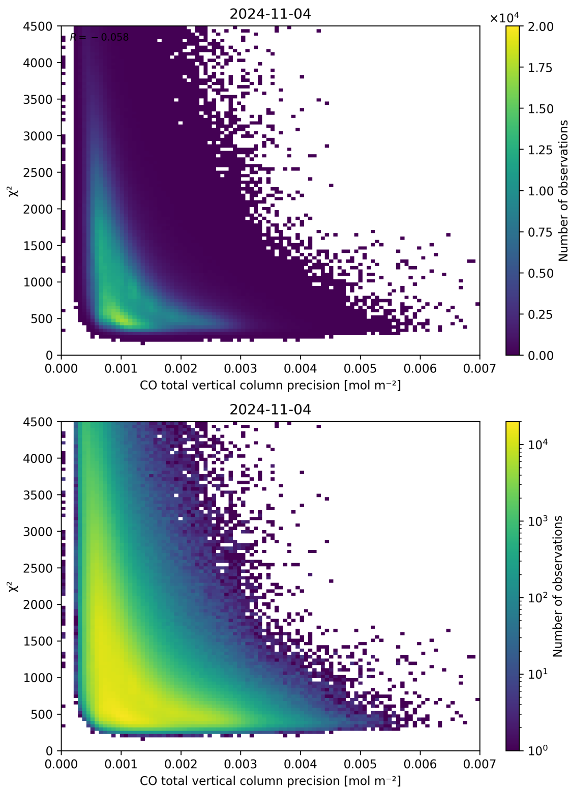
Figure 44: Scatter density plot of “CO total vertical column precision” against “ \chi^2 ” for 2024-11-04 to 2024-11-05.
