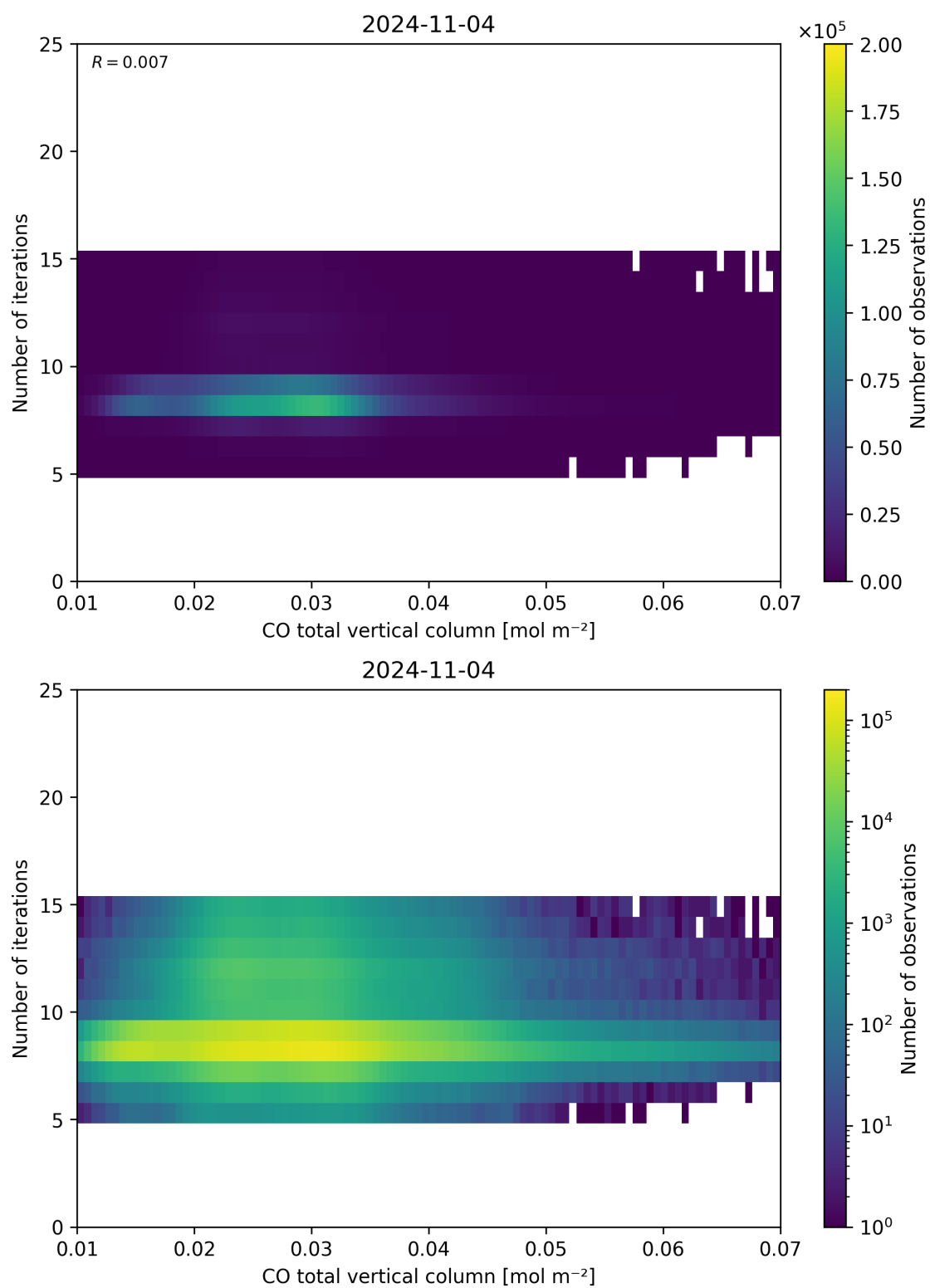
Figure 42: Scatter density plot of “CO total vertical column” against “Number of iterations” for 2024-11-04 to 2024-11-05.
