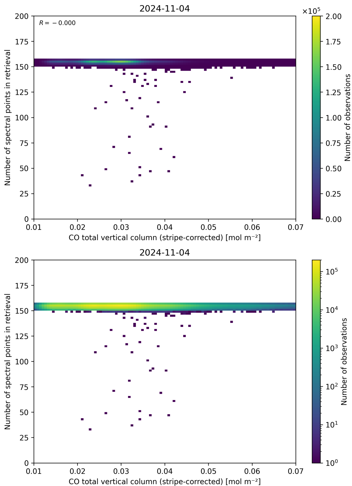
Figure 40: Scatter density plot of “CO total vertical column (stripe-corrected)” against “Number of spectral points in retrieval” for 2024-11-04 to 2024-11-05.
