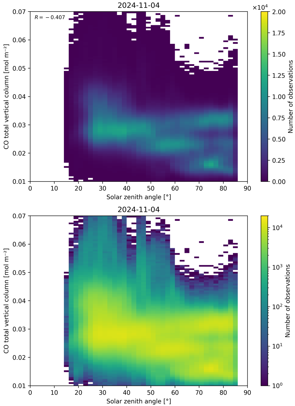
Figure 61: Scatter density plot of “Solar zenith angle” against “CO total vertical column” for 2024-11-04 to 2024-11-05.
