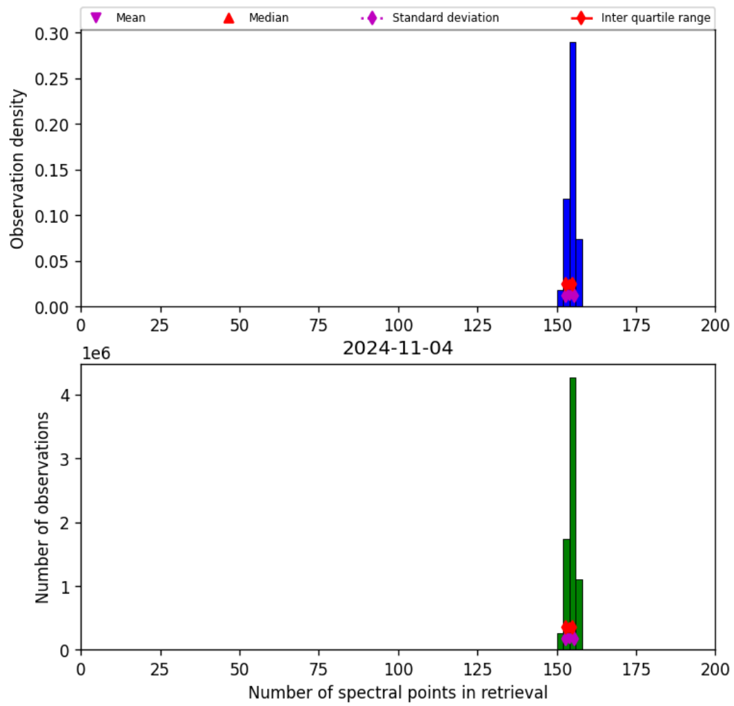
Figure 21: Histogram of “Number of spectral points in retrieval” for 2024-11-04 to 2024-11-05
