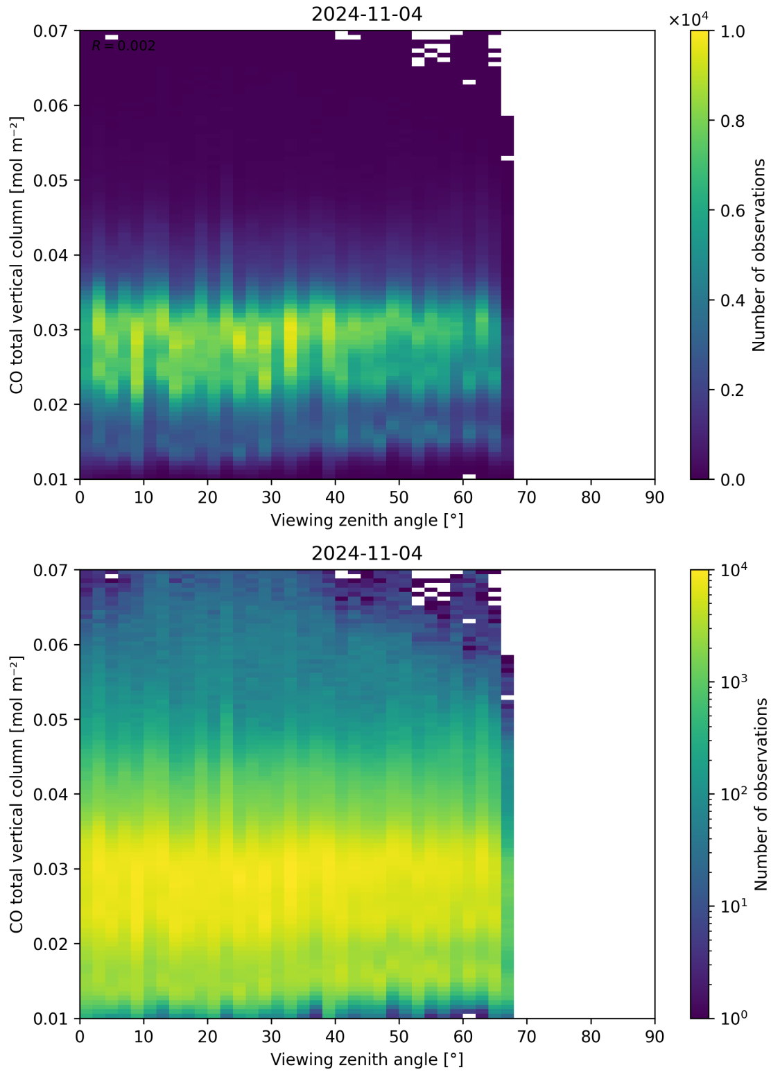
Figure 69: Scatter density plot of “Viewing zenith angle” against “CO total vertical column” for 2024-11-04 to 2024-11-05.
