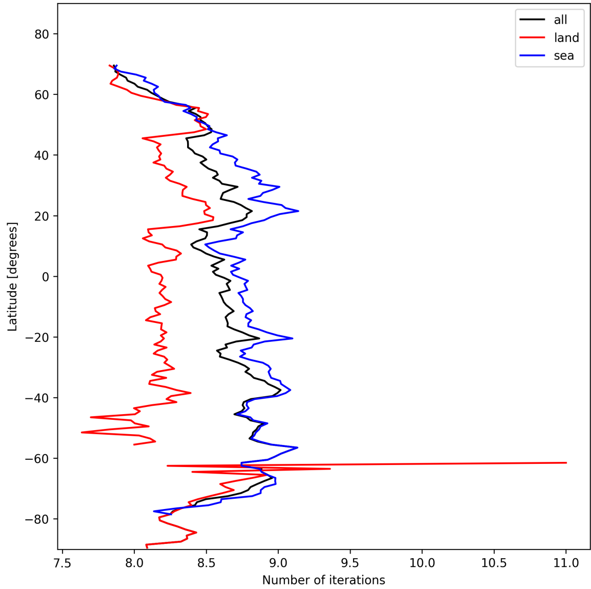
Figure 16: Zonal average of “Number of iterations” for 2024-11-04 to 2024-11-05.
