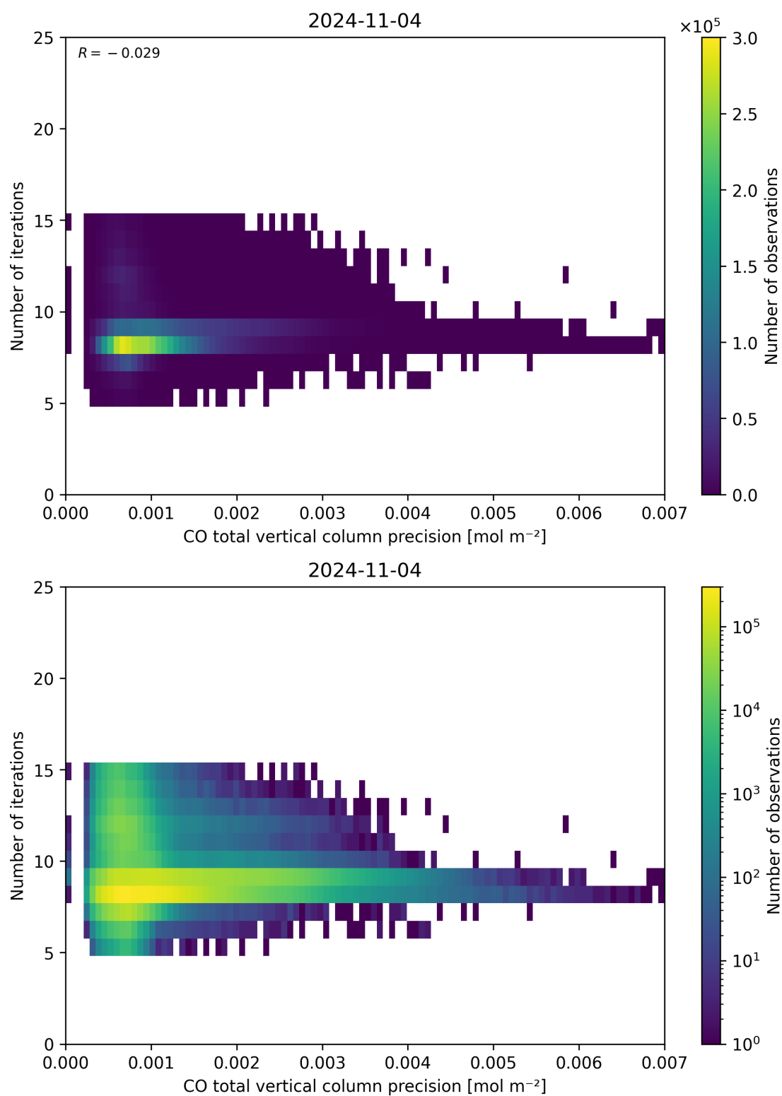
Figure 46: Scatter density plot of “CO total vertical column precision” against “Number of iterations” for 2024-11-04 to 2024-11-05.
