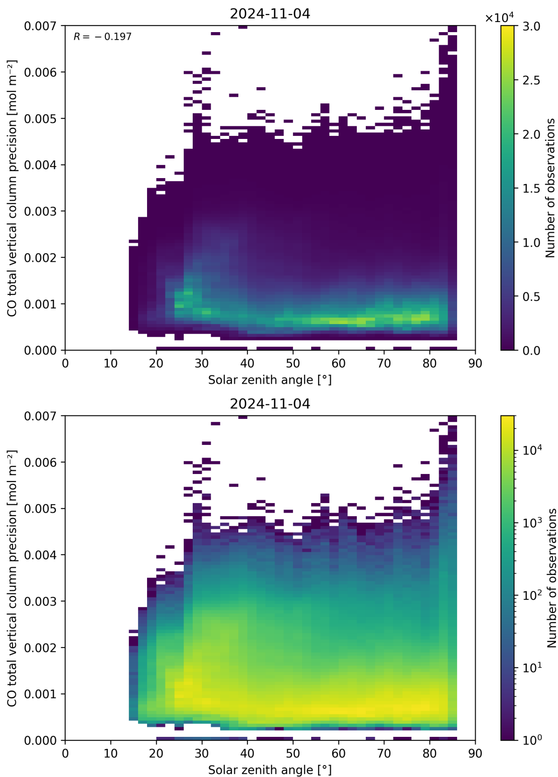
Figure 63: Scatter density plot of “Solar zenith angle” against “CO total vertical column precision” for 2024-11-04 to 2024-11-05.
