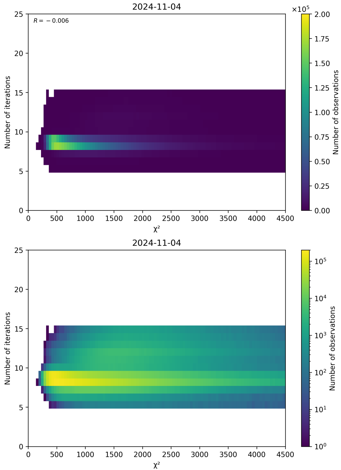
Figure 49: Scatter density plot of “ \chi^2 ” against “Number of iterations” for 2024-11-04 to 2024-11-05.
