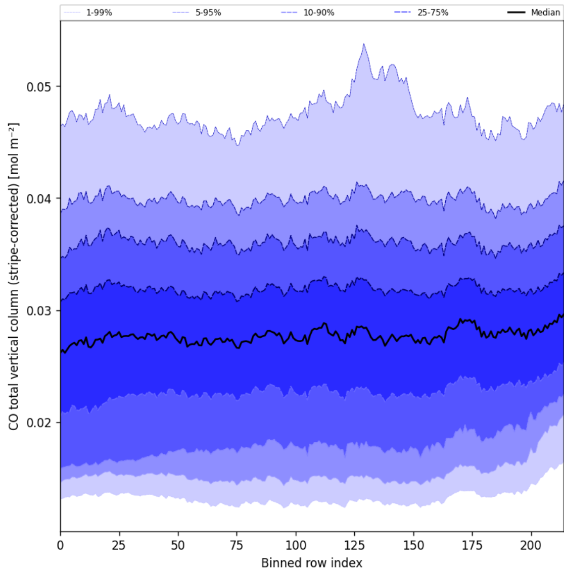
Figure 27: Along track statistics of “CO total vertical column (stripe-corrected)” for 2024-11-04 to 2024-11-05
