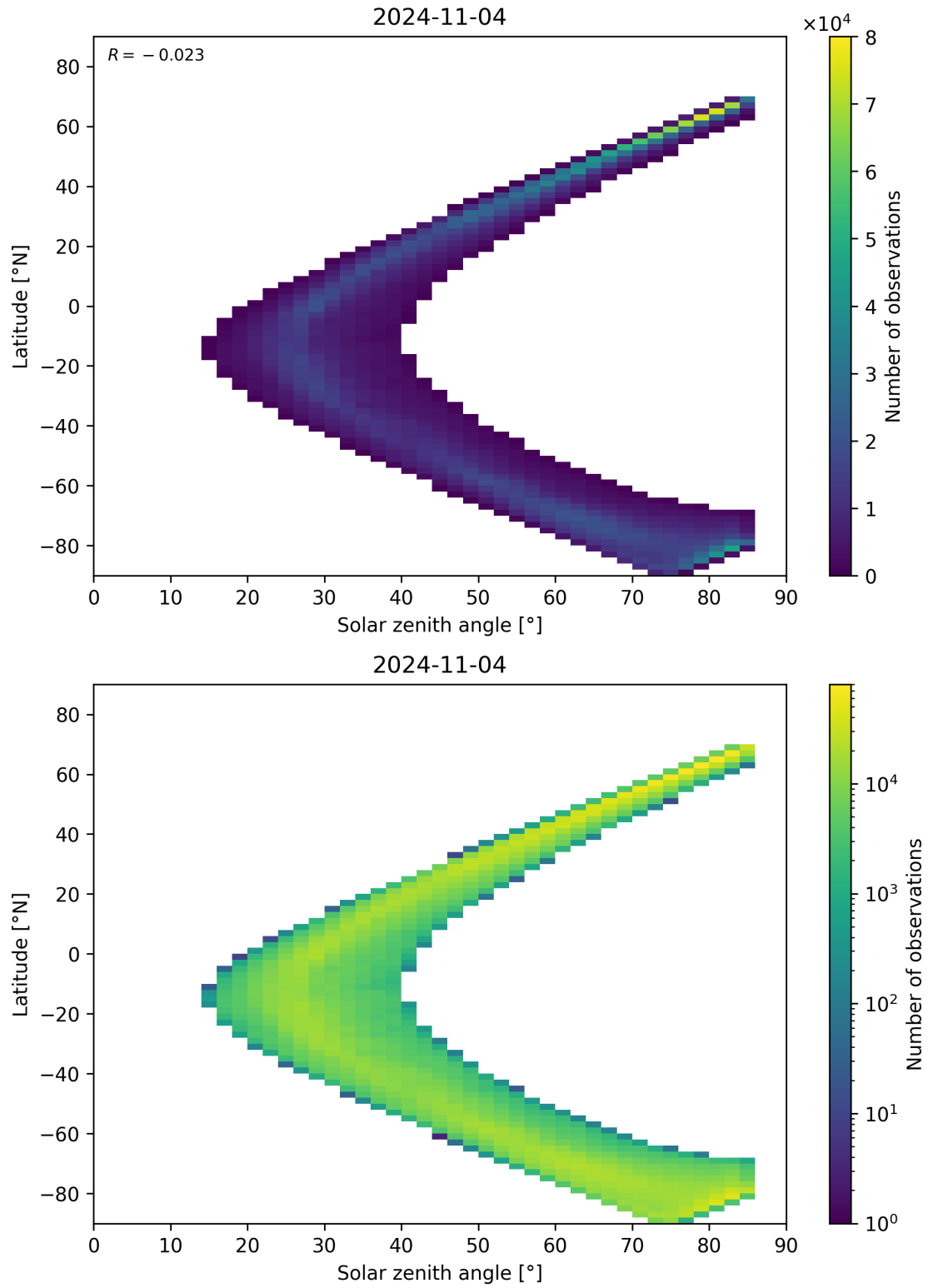
Figure 66: Scatter density plot of “Solar zenith angle” against “Latitude” for 2024-11-04 to 2024-11-05.
