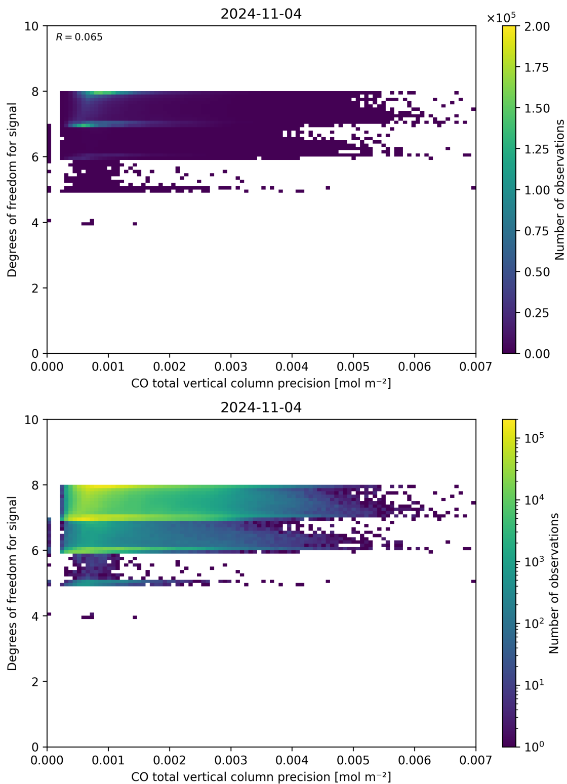
Figure 45: Scatter density plot of “CO total vertical column precision” against “Degrees of freedom for signal” for 2024-11-04 to 2024-11-05.
