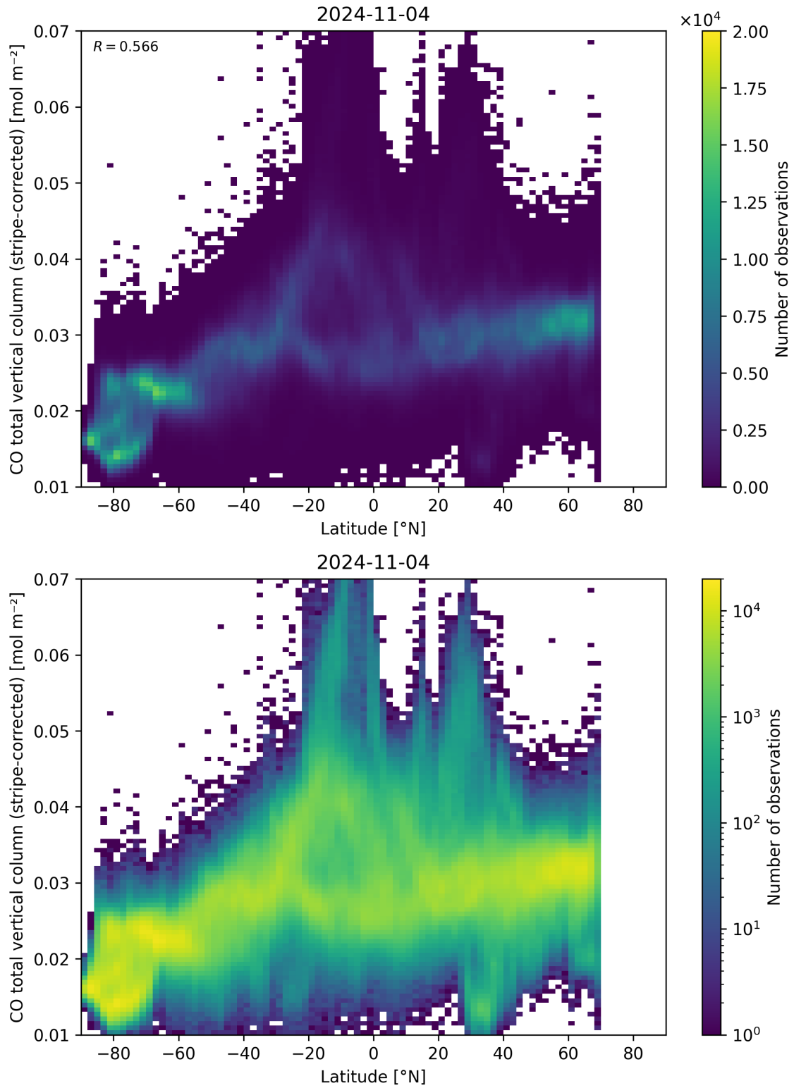
Figure 52: Scatter density plot of “Latitude” against “CO total vertical column (stripe-corrected)” for 2024-11-04 to 2024-11-05.
