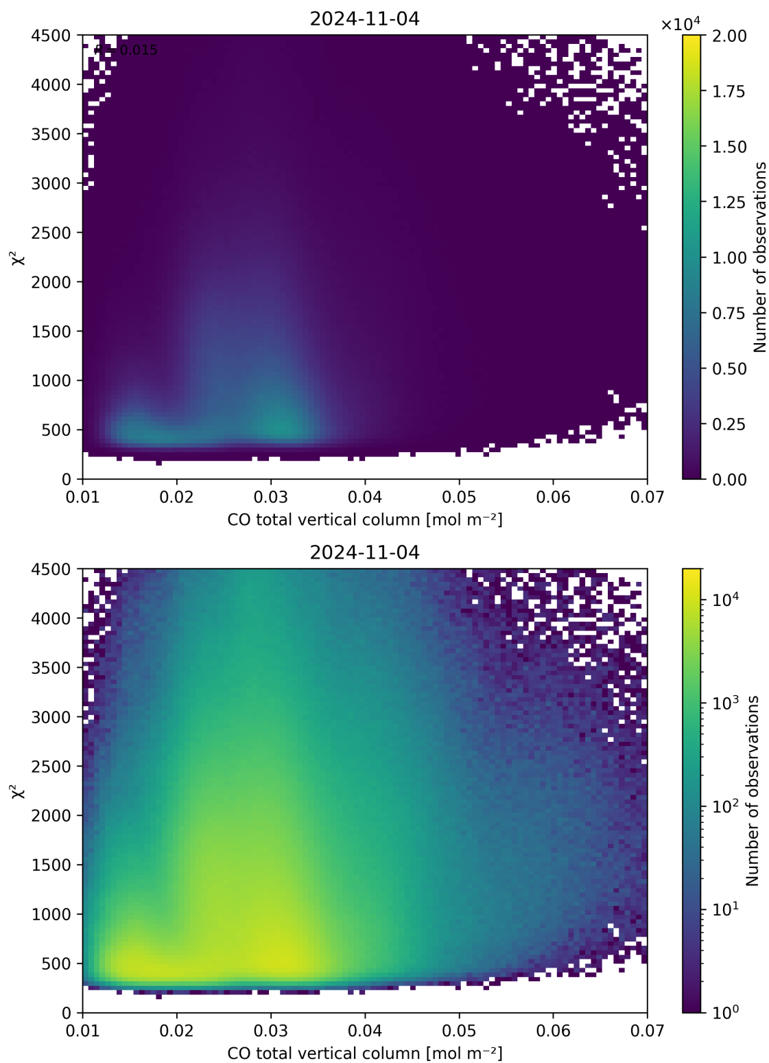
Figure 35: Scatter density plot of “CO total vertical column” against “ \chi^2 ” for 2024-11-04 to 2024-11-05.
