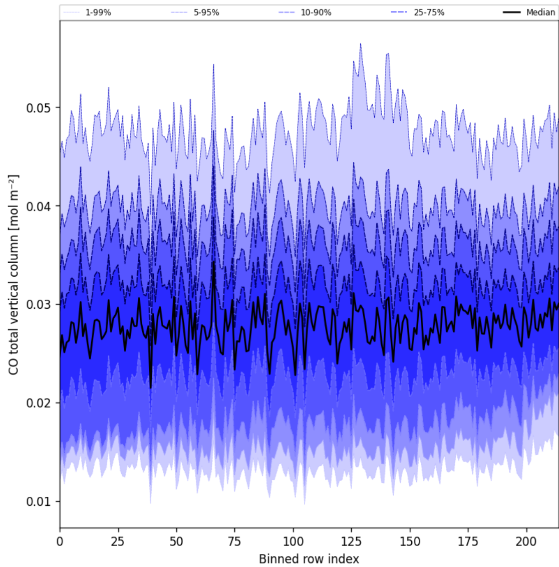
Figure 26: Along track statistics of “CO total vertical column” for 2024-11-04 to 2024-11-05
