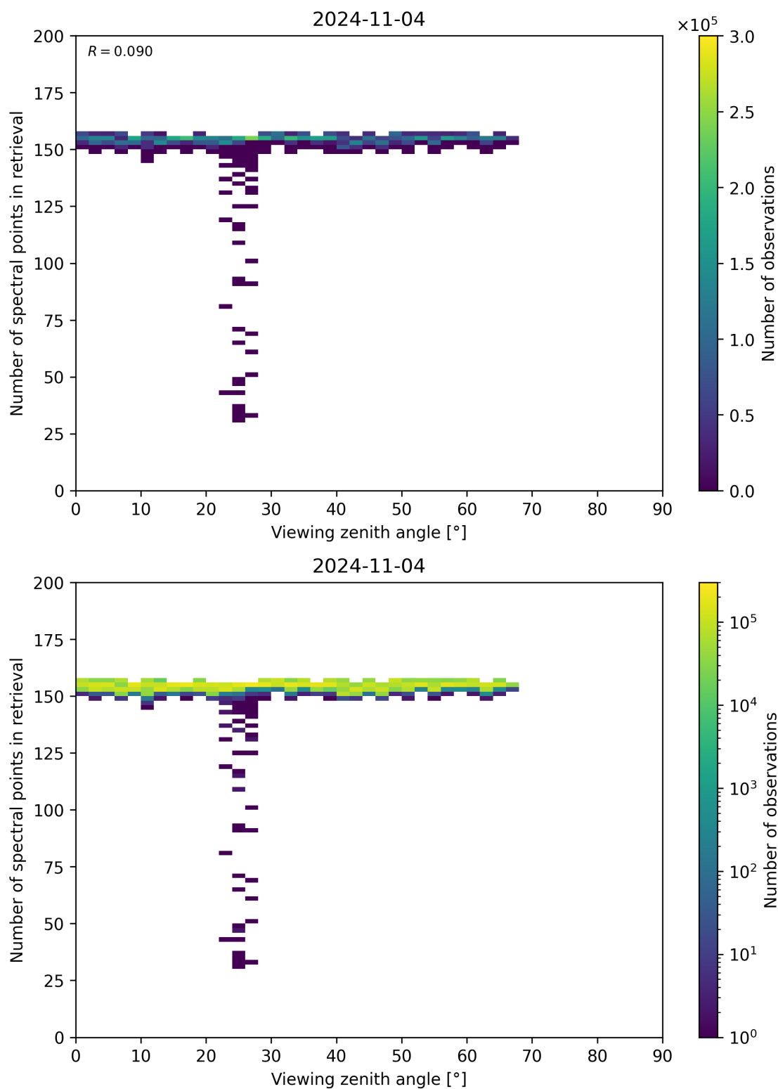
Figure 76: Scatter density plot of “Viewing zenith angle” against “Number of spectral points in retrieval” for 2024-11-04 to 2024-11-05.
