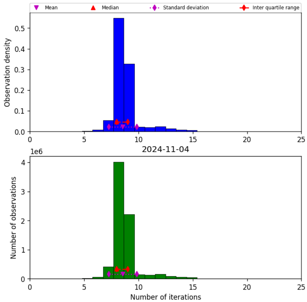
Figure 24: Histogram of “Number of iterations” for 2024-11-04 to 2024-11-05
