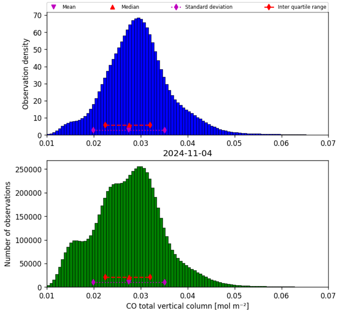
Figure 18: Histogram of “CO total vertical column” for 2024-11-04 to 2024-11-05
