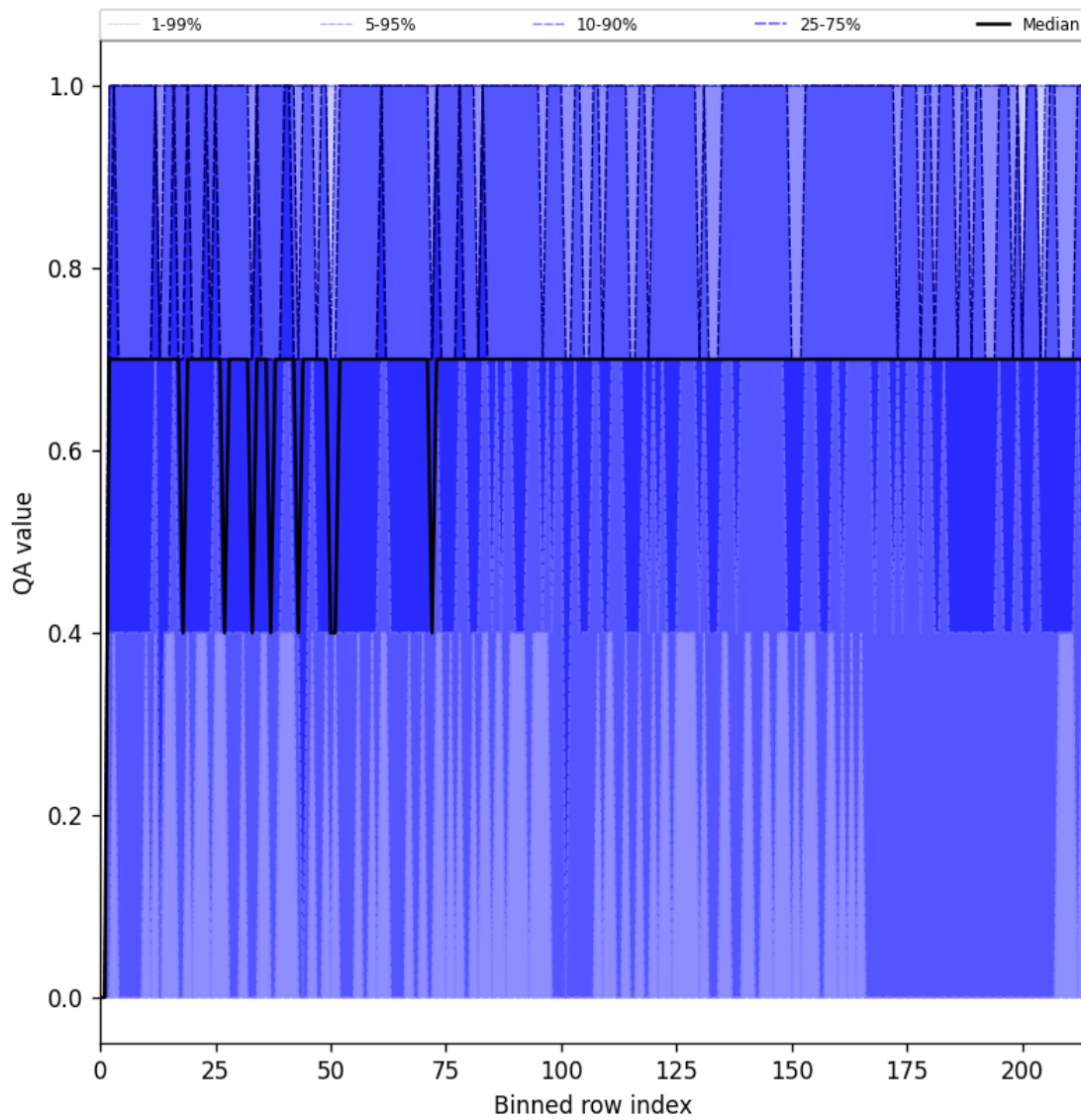
Figure 25: Along track statistics of “QA value” for 2024-11-04 to 2024-11-05
