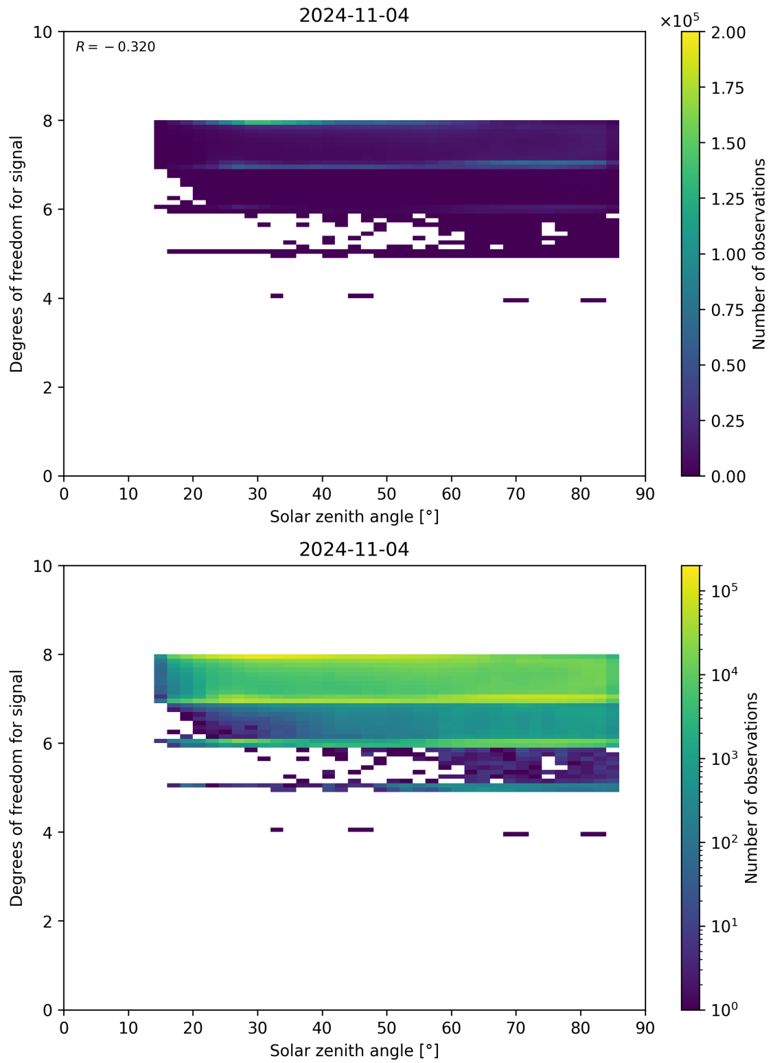
Figure 65: Scatter density plot of “Solar zenith angle” against “Degrees of freedom for signal” for 2024-11-04 to 2024-11-05.
