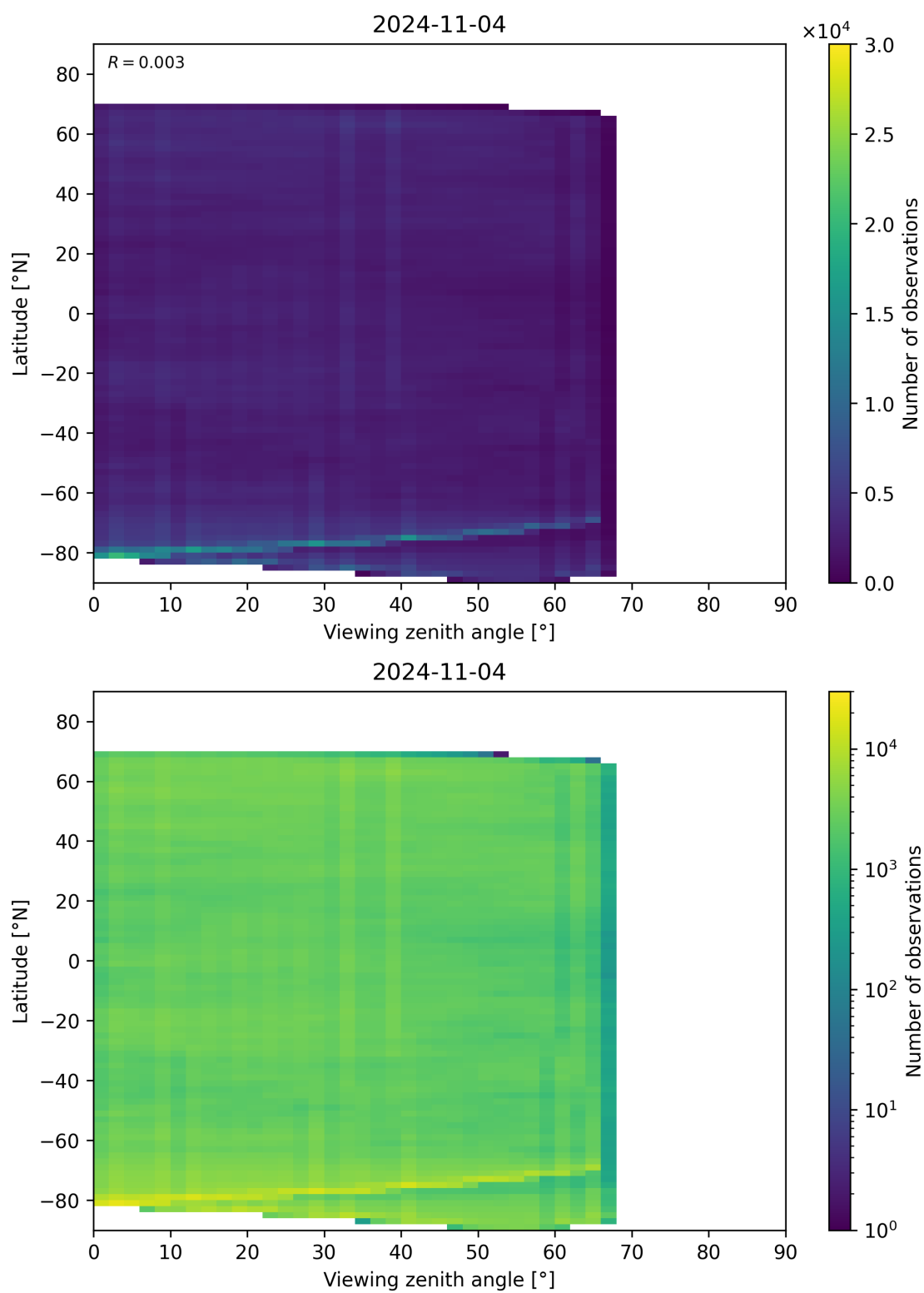
Figure 74: Scatter density plot of “Viewing zenith angle” against “Latitude” for 2024-11-04 to 2024-11-05.
