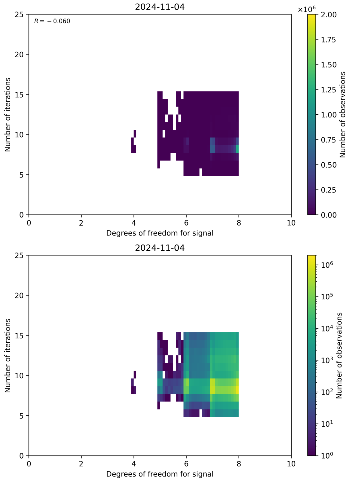
Figure 50: Scatter density plot of “Degrees of freedom for signal” against “Number of iterations” for 2024-11-04 to 2024-11-05.
