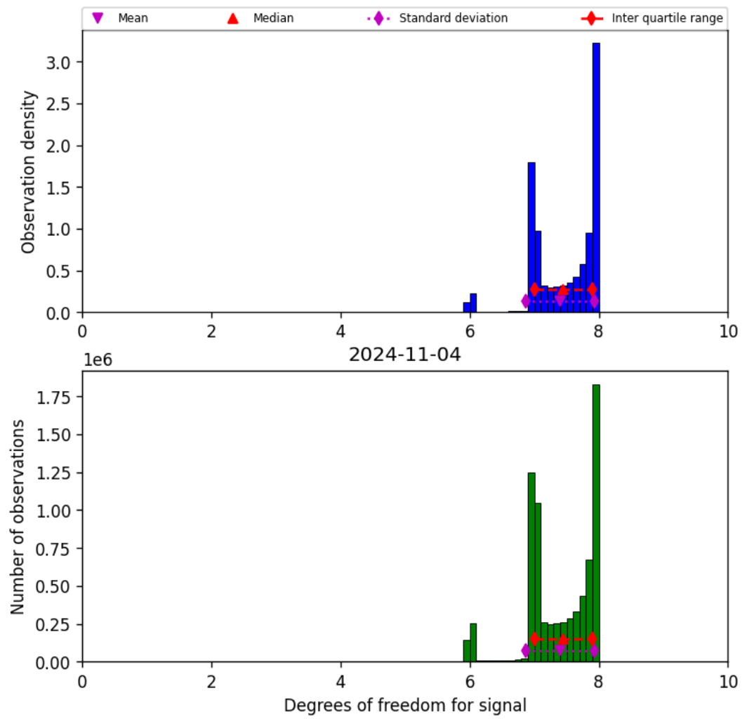
Figure 23: Histogram of “Degrees of freedom for signal” for 2024-11-04 to 2024-11-05
