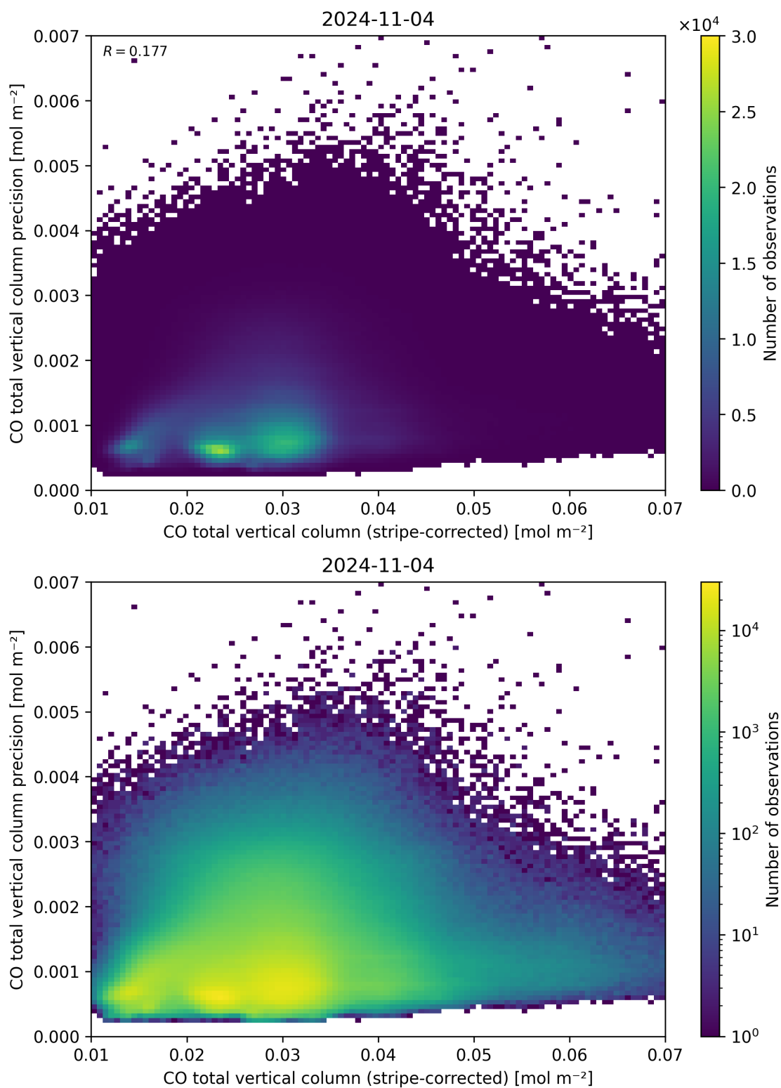
Figure 36: Scatter density plot of “CO total vertical column (stripe-corrected)” against “CO total vertical column precision” for 2024-11-04 to 2024-11-05.
