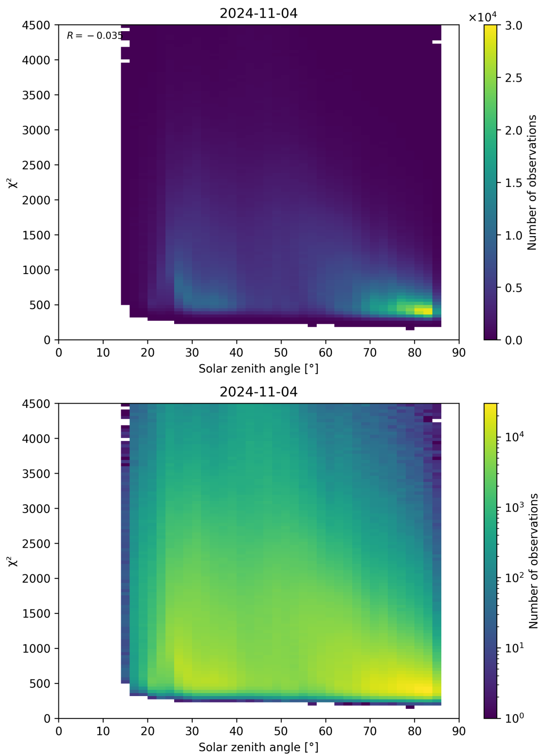
Figure 64: Scatter density plot of “Solar zenith angle” against “ \chi^2 ” for 2024-11-04 to 2024-11-05.
