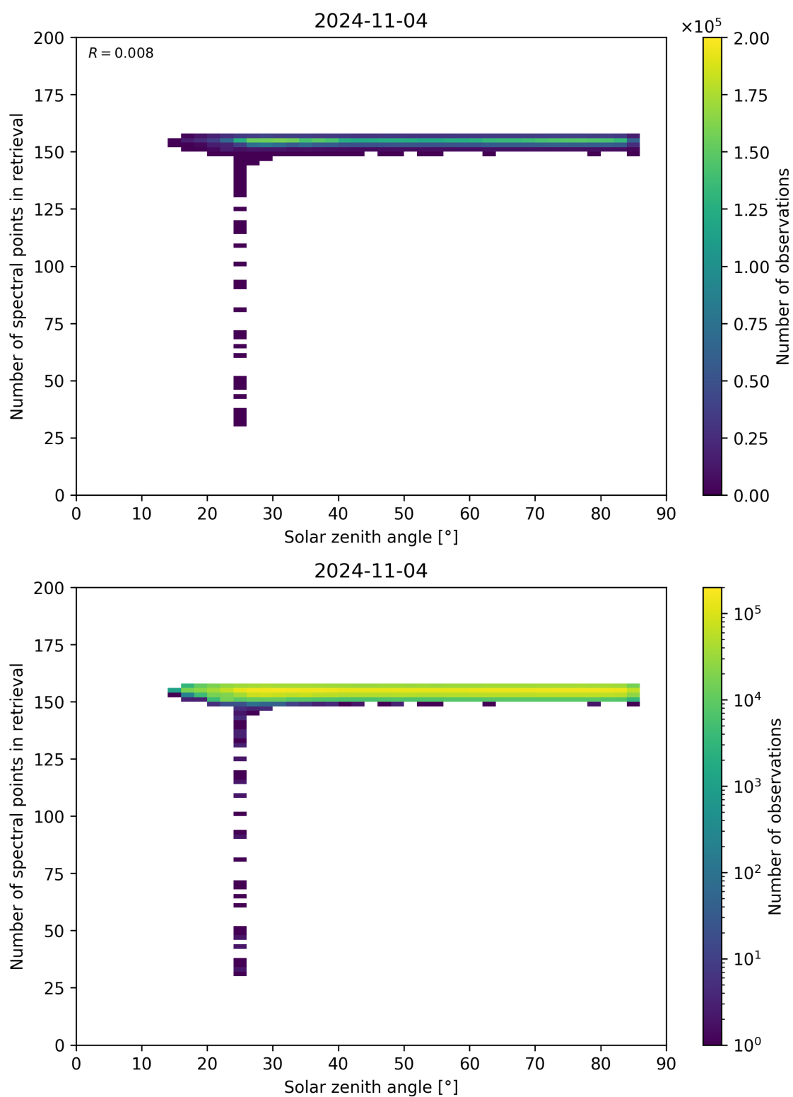
Figure 68: Scatter density plot of “Solar zenith angle” against “Number of spectral points in retrieval” for 2024-11-04 to 2024-11-05.
