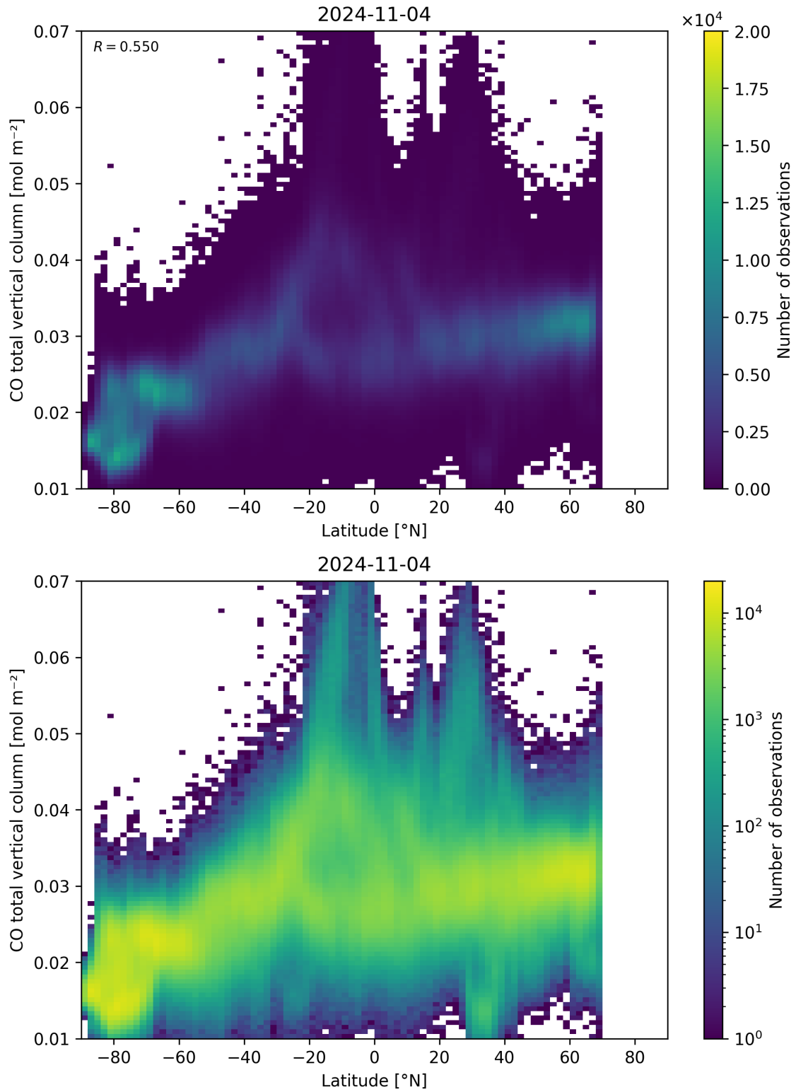
Figure 51: Scatter density plot of “Latitude” against “CO total vertical column” for 2024-11-04 to 2024-11-05.
