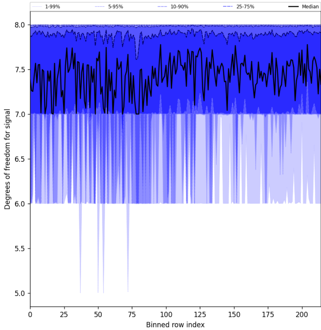
Figure 31: Along track statistics of “Degrees of freedom for signal” for 2024-11-04 to 2024-11-05
