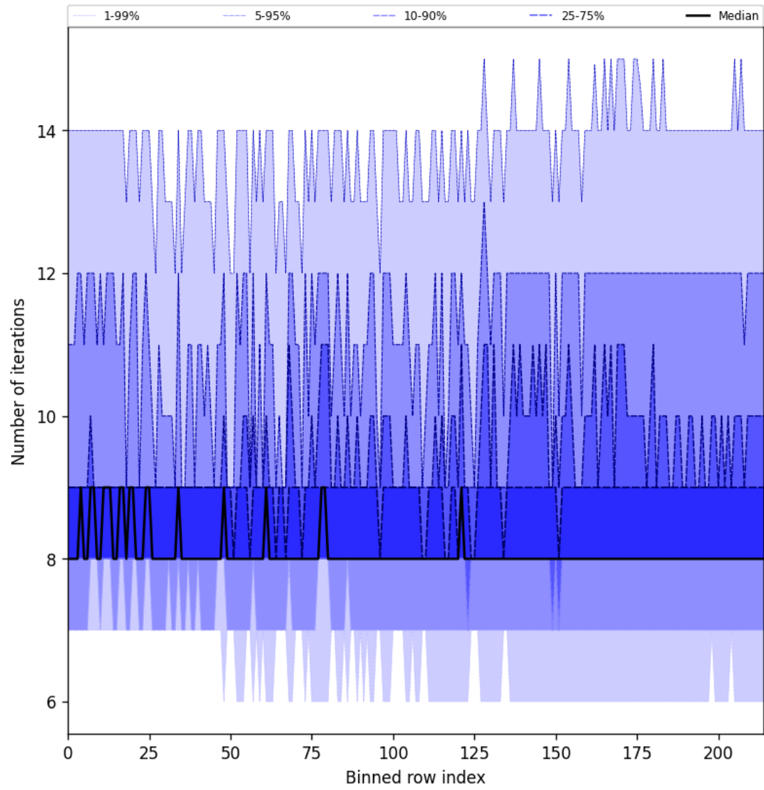
Figure 32: Along track statistics of “Number of iterations” for 2024-11-04 to 2024-11-05
