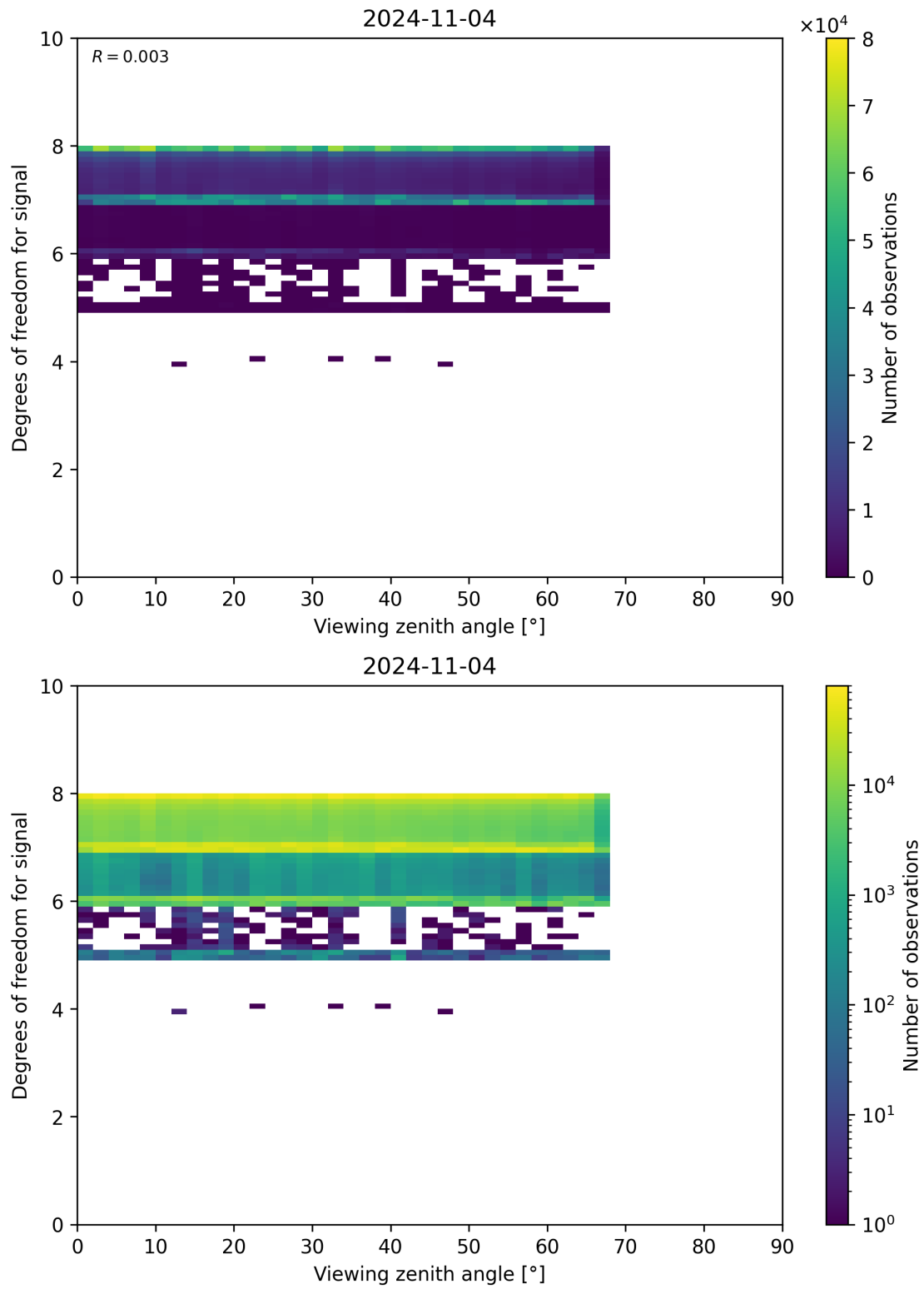
Figure 73: Scatter density plot of “Viewing zenith angle” against “Degrees of freedom for signal” for 2024-11-04 to 2024-11-05.
