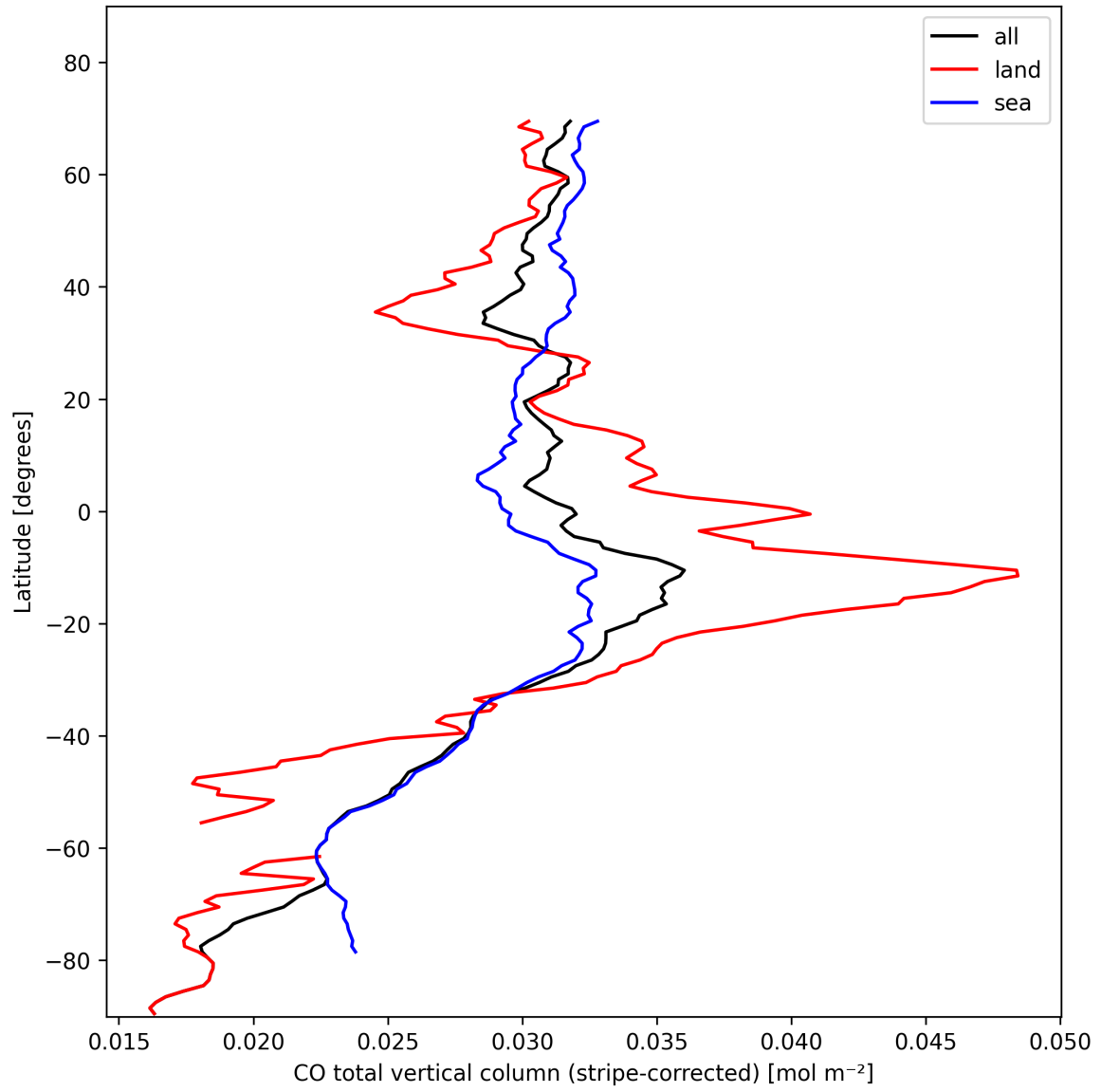
Figure 11: Zonal average of “CO total vertical column (stripe-corrected)” for 2024-11-04 to 2024-11-05.
