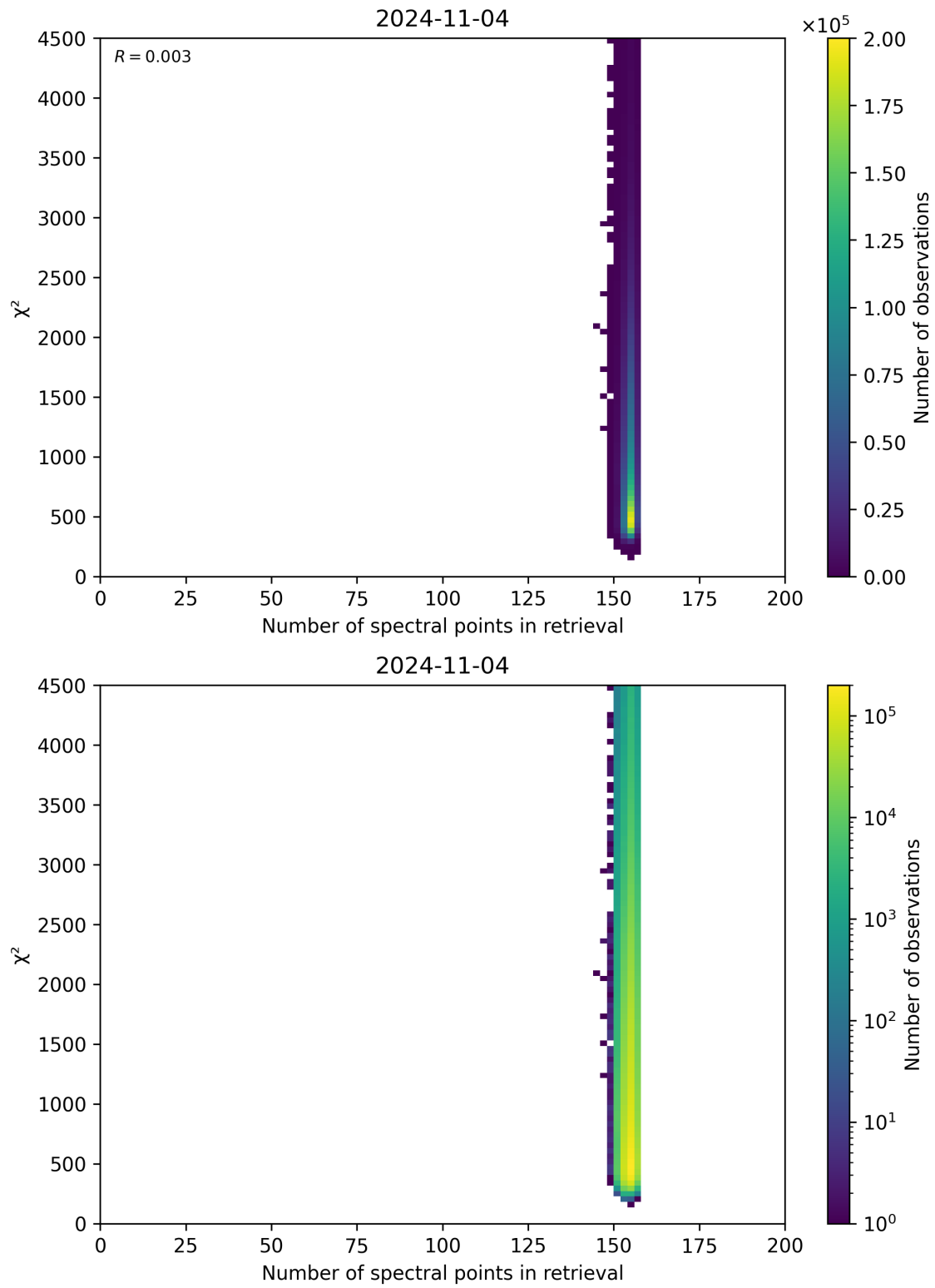
Figure 58: Scatter density plot of “Number of spectral points in retrieval” against “ \chi^2 ” for 2024-11-04 to 2024-11-05.
