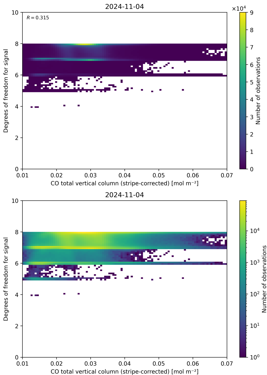
Figure 38: Scatter density plot of “CO total vertical column (stripe-corrected)” against “Degrees of freedom for signal” for 2024-11-04 to 2024-11-05.
