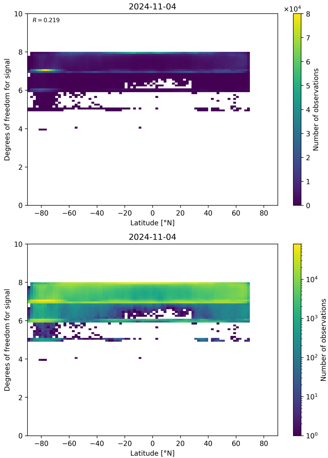
Figure 55: Scatter density plot of “Latitude” against “Degrees of freedom for signal” for 2024-11-04 to 2024-11-05.
