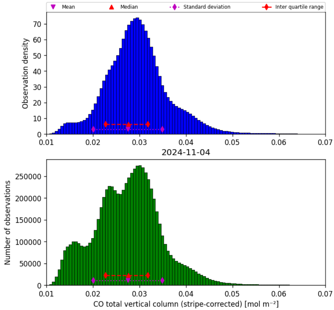
Figure 19: Histogram of “CO total vertical column (stripe-corrected)” for 2024-11-04 to 2024-11-05
