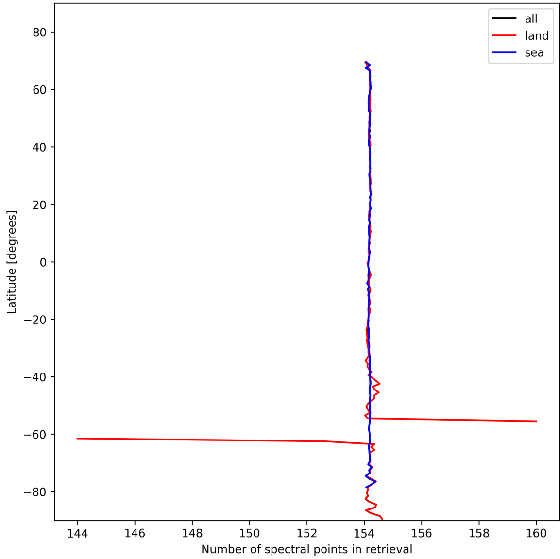
Figure 13: Zonal average of “Number of spectral points in retrieval” for 2024-11-04 to 2024-11-05.
