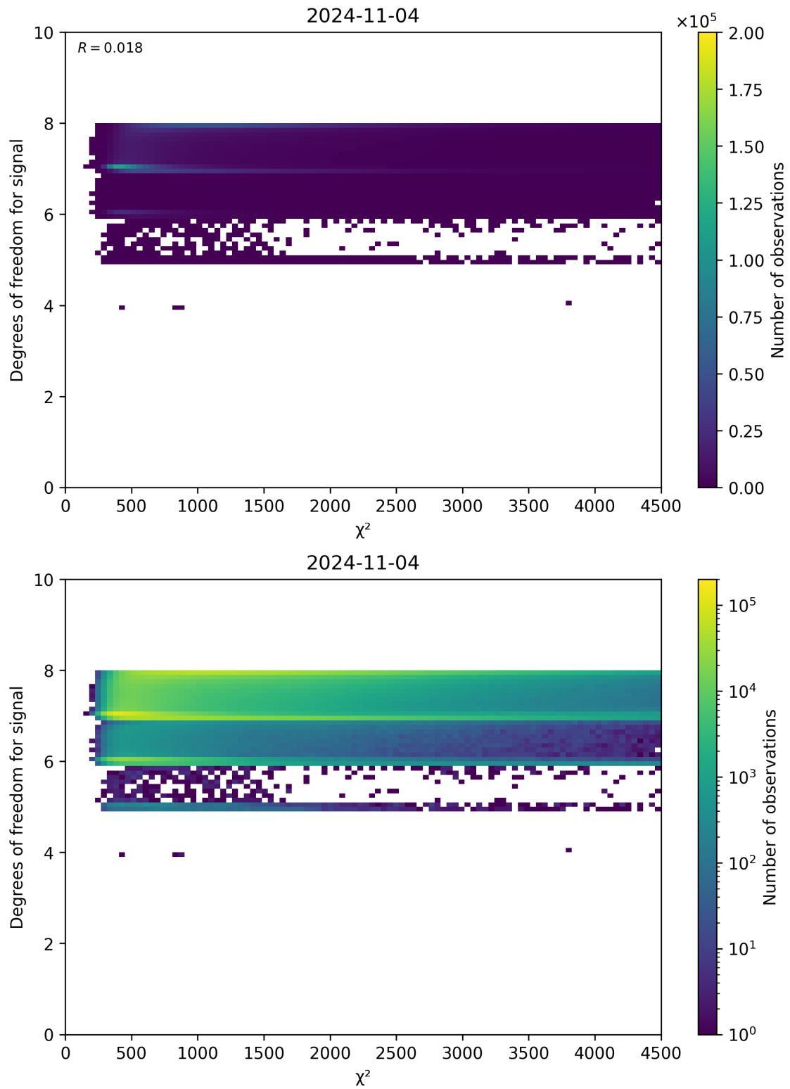
Figure 48: Scatter density plot of “ \chi^2 ” against “Degrees of freedom for signal” for 2024-11-04 to 2024-11-05.
