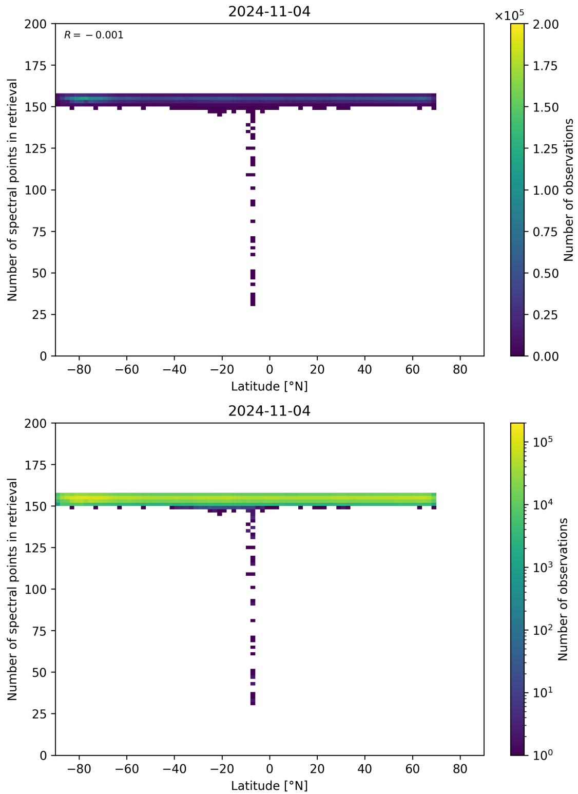
Figure 57: Scatter density plot of “Latitude” against “Number of spectral points in retrieval” for 2024-11-04 to 2024-11-05.
