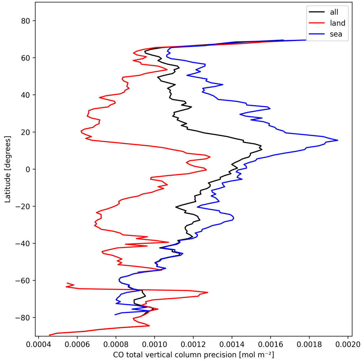
Figure 12: Zonal average of “CO total vertical column precision” for 2024-11-04 to 2024-11-05.
