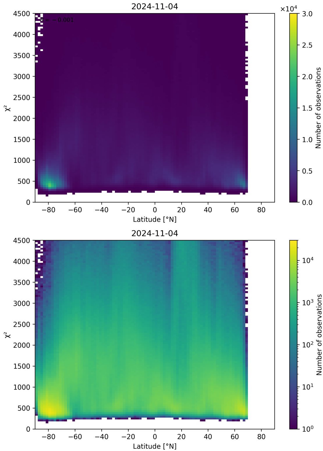
Figure 54: Scatter density plot of “Latitude” against “ \chi^2 ” for 2024-11-04 to 2024-11-05.
