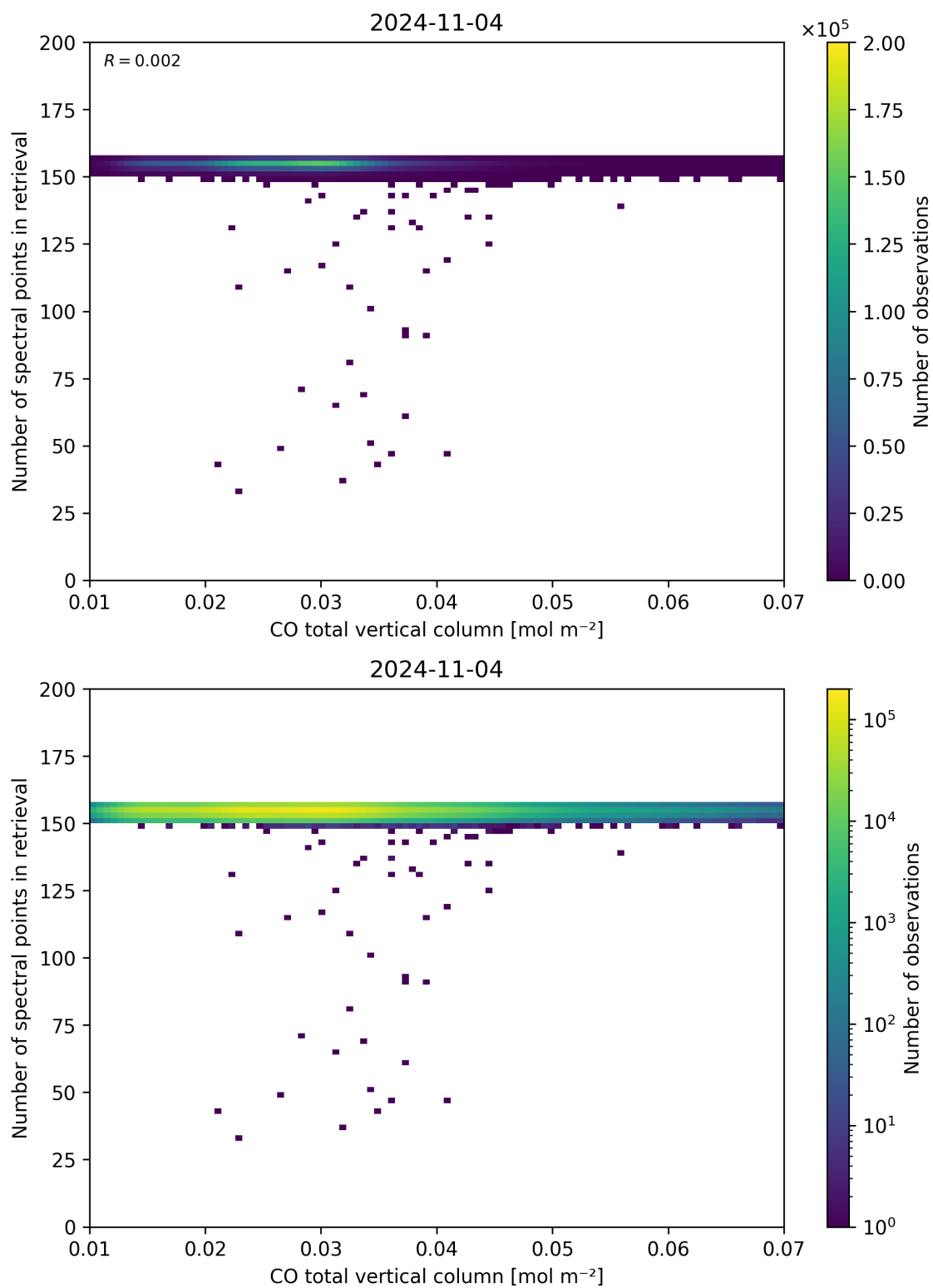
Figure 43: Scatter density plot of “CO total vertical column” against “Number of spectral points in retrieval” for 2024-11-04 to 2024-11-05.
