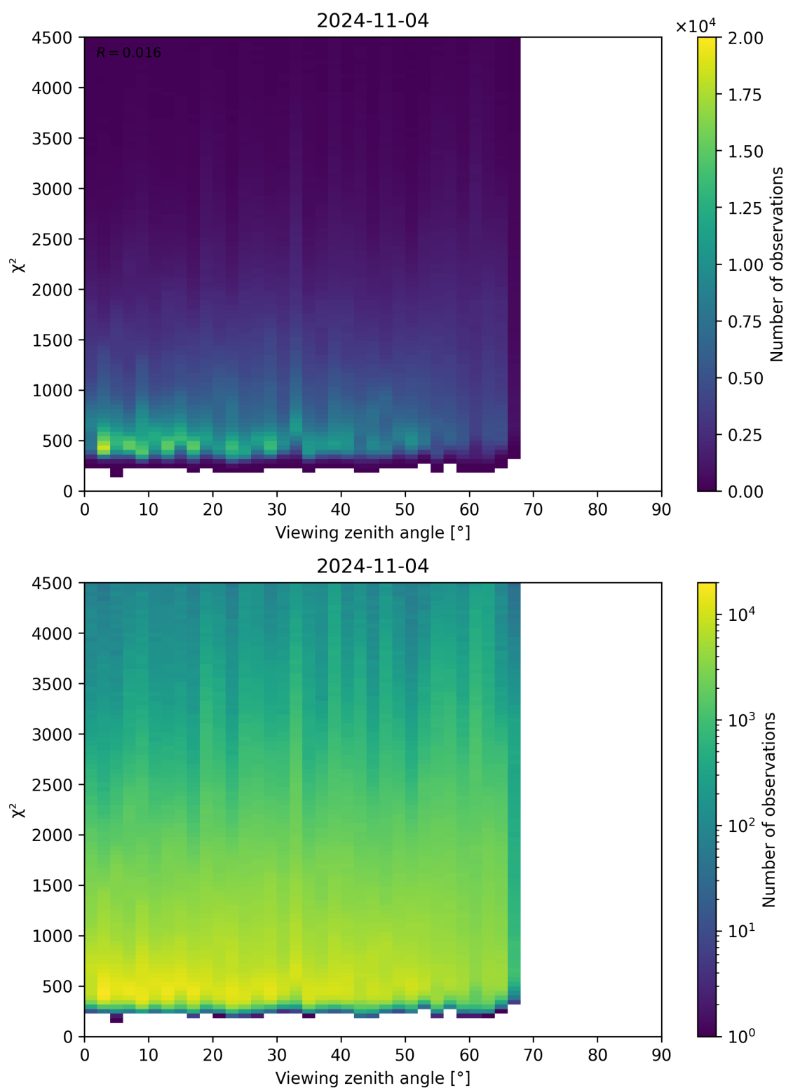
Figure 72: Scatter density plot of “Viewing zenith angle” against “ \chi^2 ” for 2024-11-04 to 2024-11-05.
