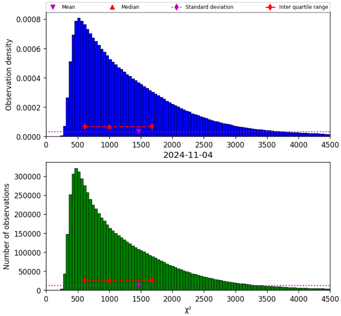
Figure 22: Histogram of " \chi^2 " for 2024-11-04 to 2024-11-05
