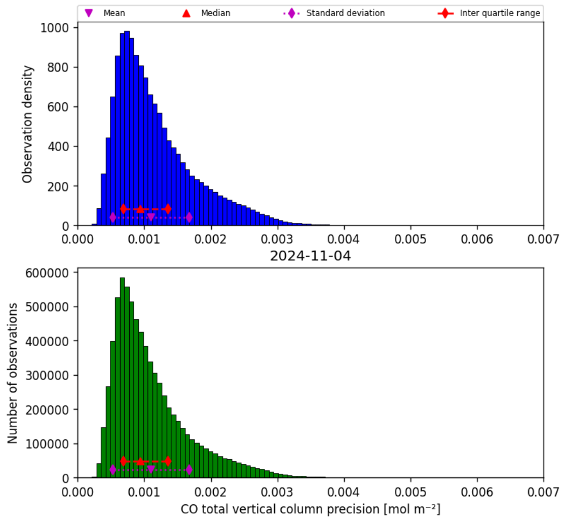
Figure 20: Histogram of “CO total vertical column precision” for 2024-11-04 to 2024-11-05
