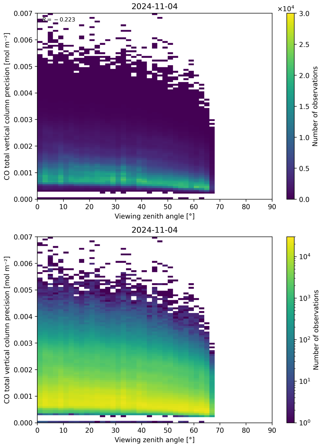
Figure 71: Scatter density plot of “Viewing zenith angle” against “CO total vertical column precision” for 2024-11-04 to 2024-11-05.
