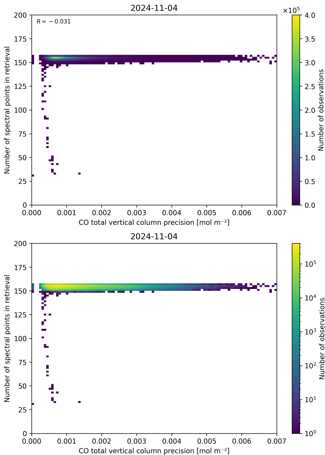
Figure 47: Scatter density plot of “CO total vertical column precision” against “Number of spectral points in retrieval” for 2024-11-04 to 2024-11-05.
