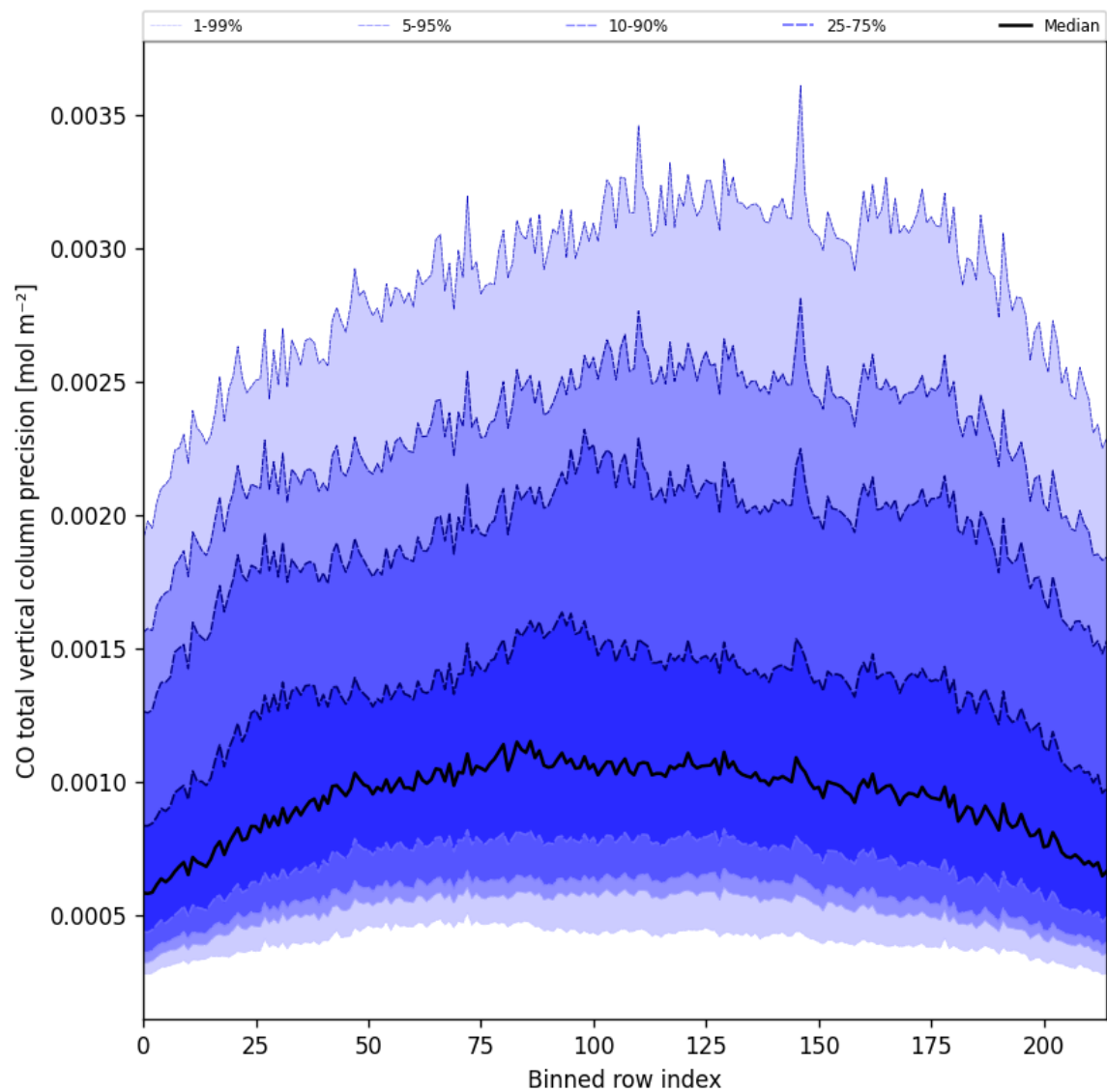
Figure 28: Along track statistics of “CO total vertical column precision” for 2024-11-04 to 2024-11-05
