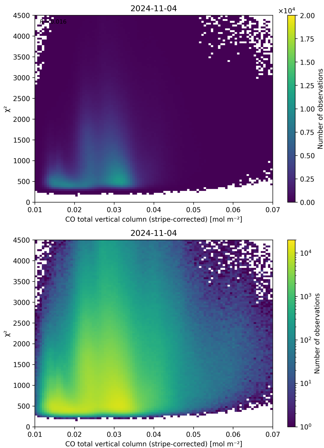
Figure 37: Scatter density plot of “CO total vertical column (stripe-corrected)” against “ \chi^2 ” for 2024-11-04 to 2024-11-05.
