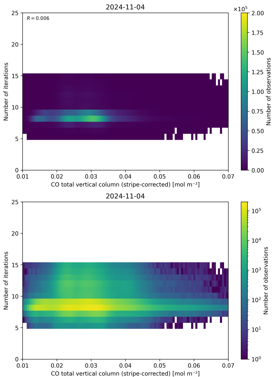
Figure 39: Scatter density plot of “CO total vertical column (stripe-corrected)” against “Number of iterations” for 2024-11-04 to 2024-11-05.
