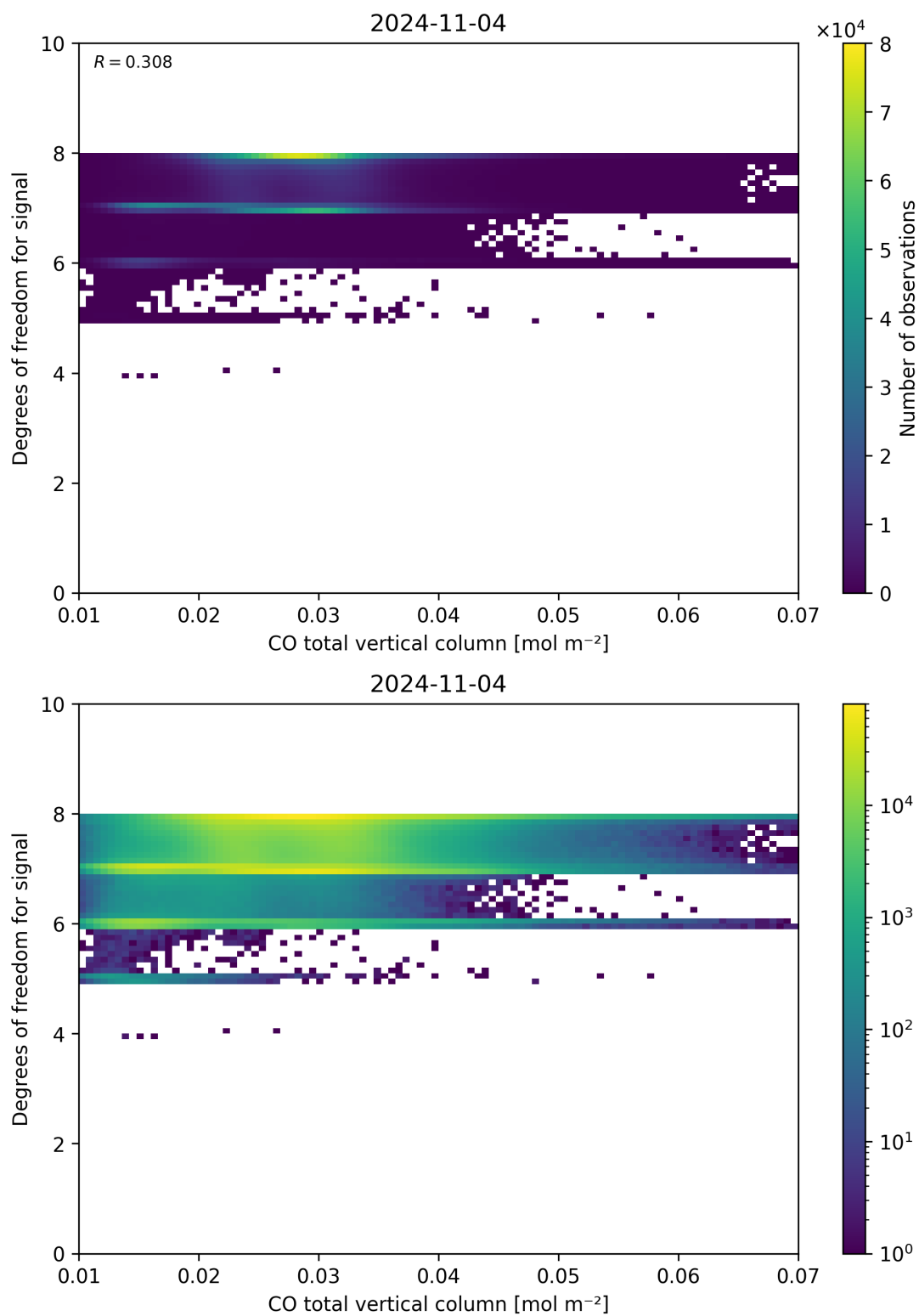
Figure 41: Scatter density plot of “CO total vertical column” against “Degrees of freedom for signal” for 2024-11-04 to 2024-11-05.
