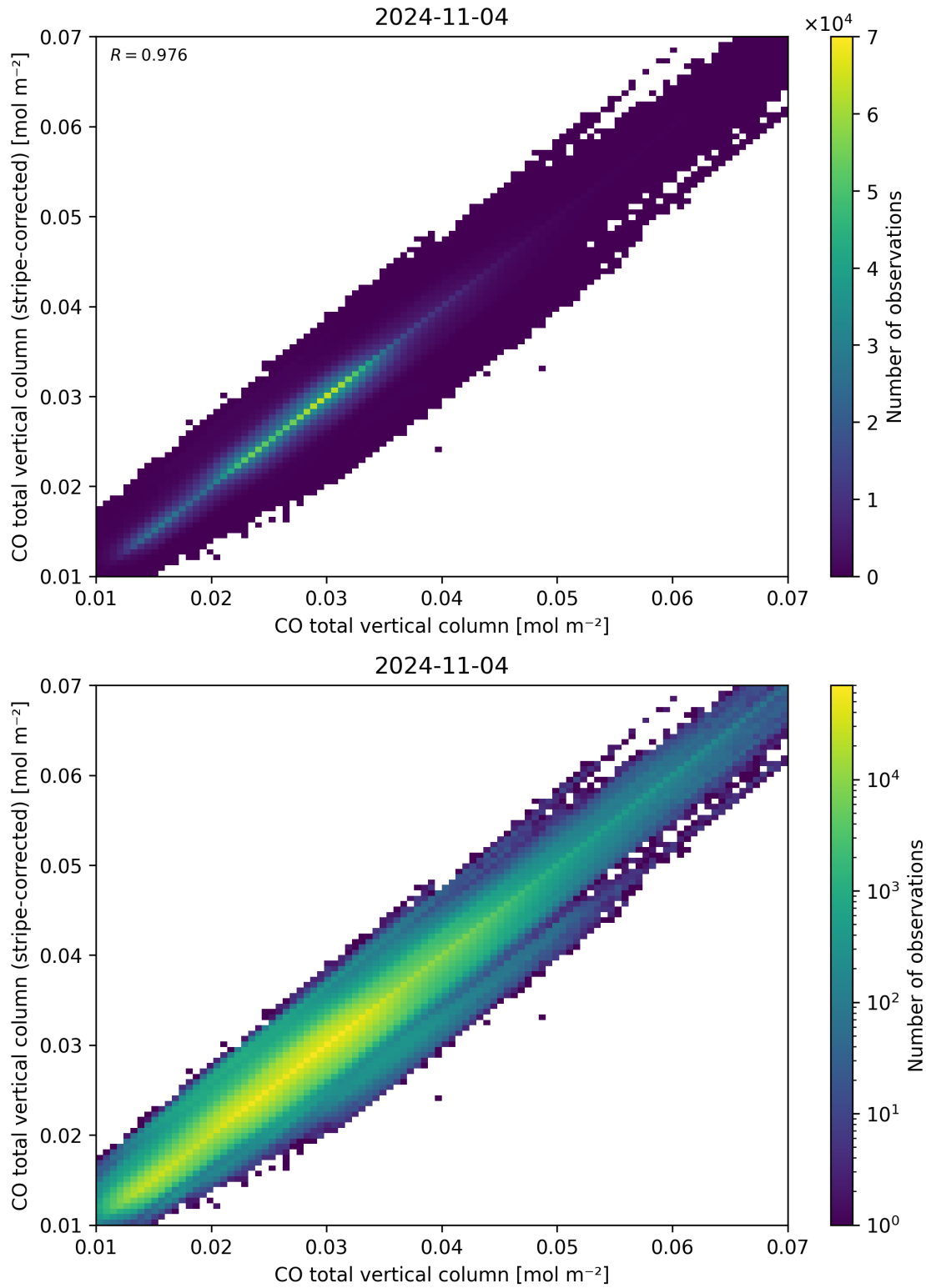
Figure 33: Scatter density plot of “CO total vertical column” against “CO total vertical column (stripe-corrected)” for 2024-11-04 to 2024-11-05.
