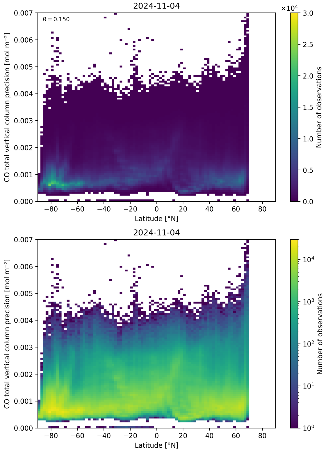
Figure 53: Scatter density plot of “Latitude” against “CO total vertical column precision” for 2024-11-04 to 2024-11-05.
