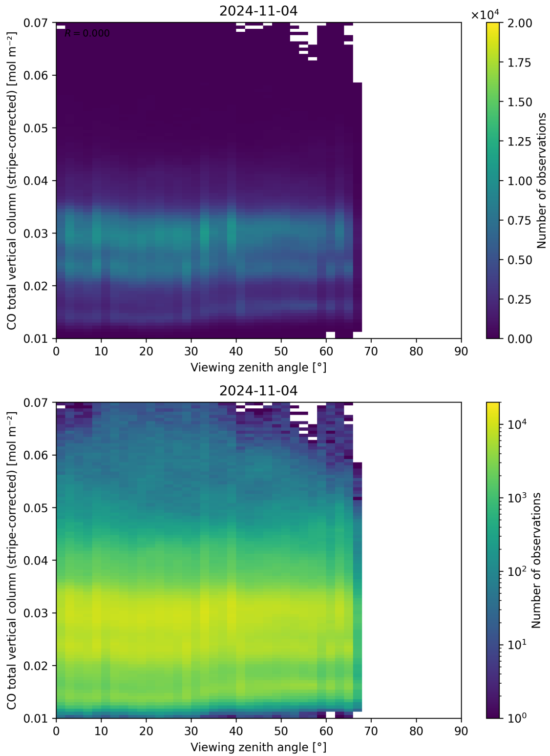
Figure 70: Scatter density plot of “Viewing zenith angle” against “CO total vertical column (stripe-corrected)” for 2024-11-04 to 2024-11-05.
