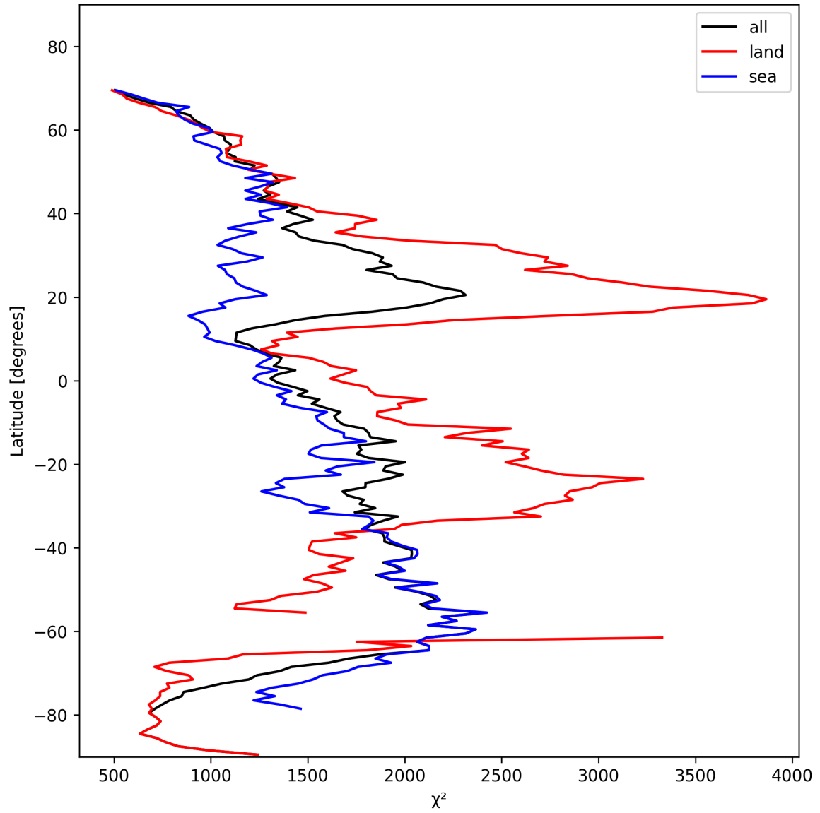
Figure 14: Zonal average of “ \chi^2 ” for 2024-11-04 to 2024-11-05.
