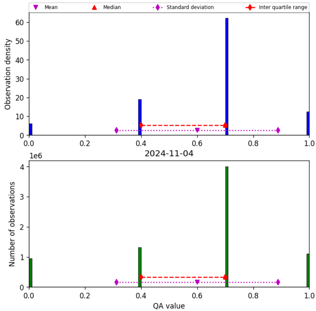
Figure 17: Histogram of “QA value” for 2024-11-04 to 2024-11-05
