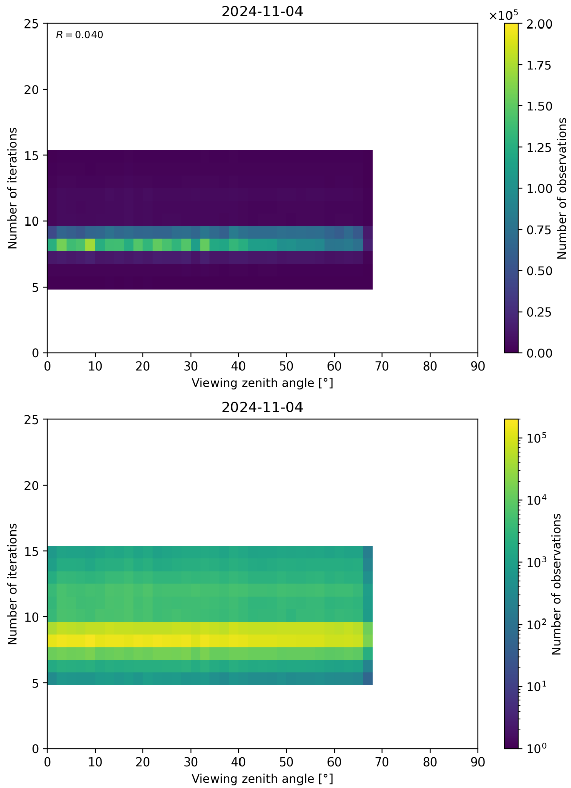
Figure 75: Scatter density plot of “Viewing zenith angle” against “Number of iterations” for 2024-11-04 to 2024-11-05.
