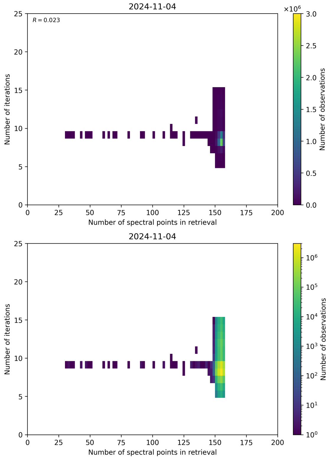
Figure 60: Scatter density plot of “Number of spectral points in retrieval” against “Number of iterations” for 2024-11-04 to 2024-11-05.
