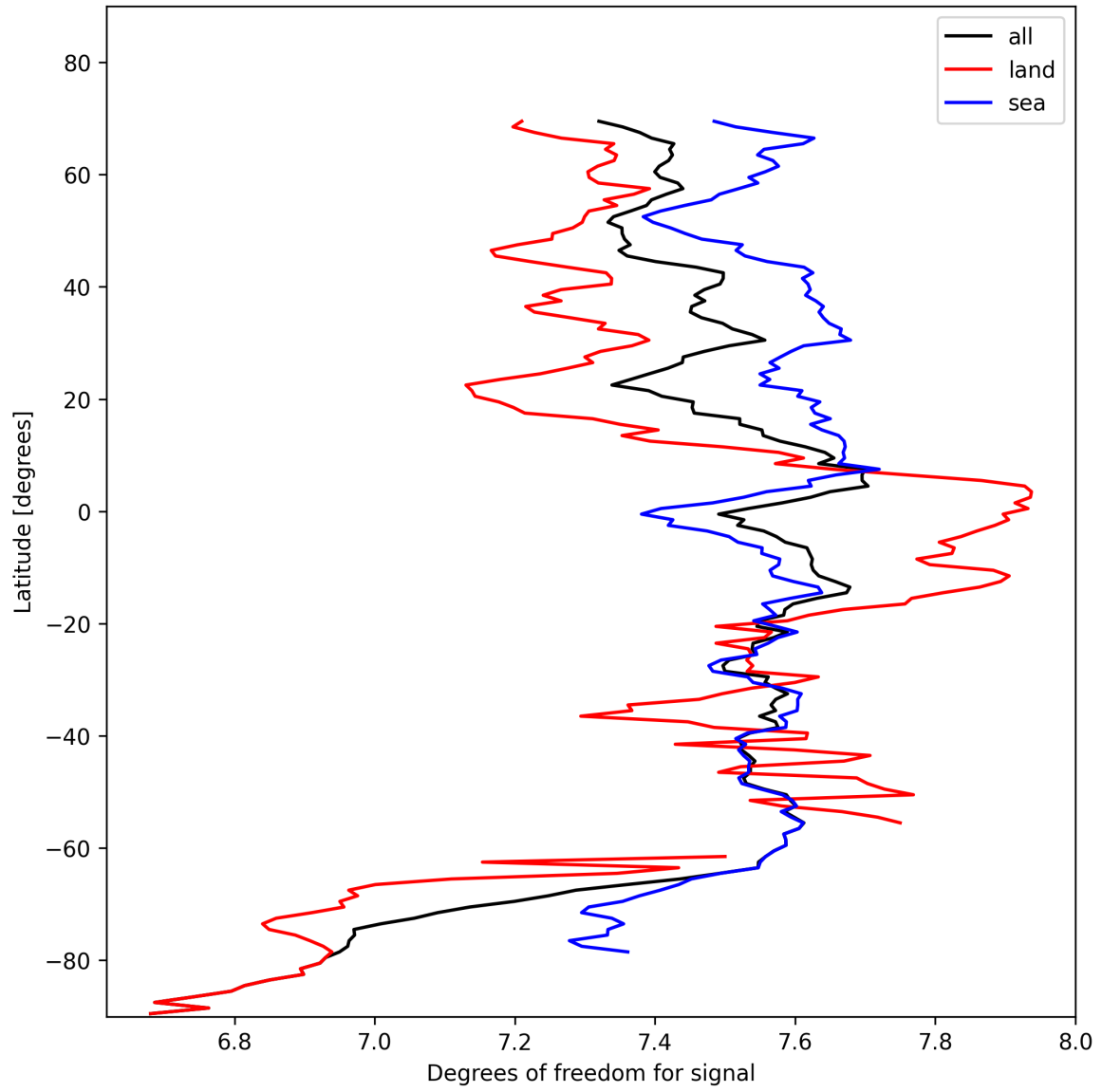
Figure 15: Zonal average of “Degrees of freedom for signal” for 2024-11-04 to 2024-11-05.
