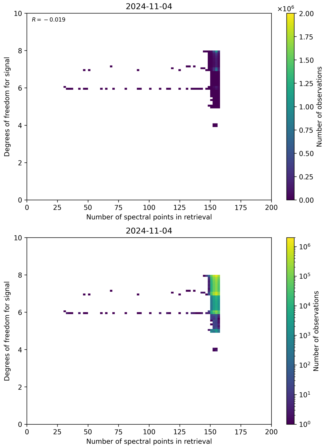
Figure 59: Scatter density plot of “Number of spectral points in retrieval” against “Degrees of freedom for signal” for 2024-11-04 to 2024-11-05.
