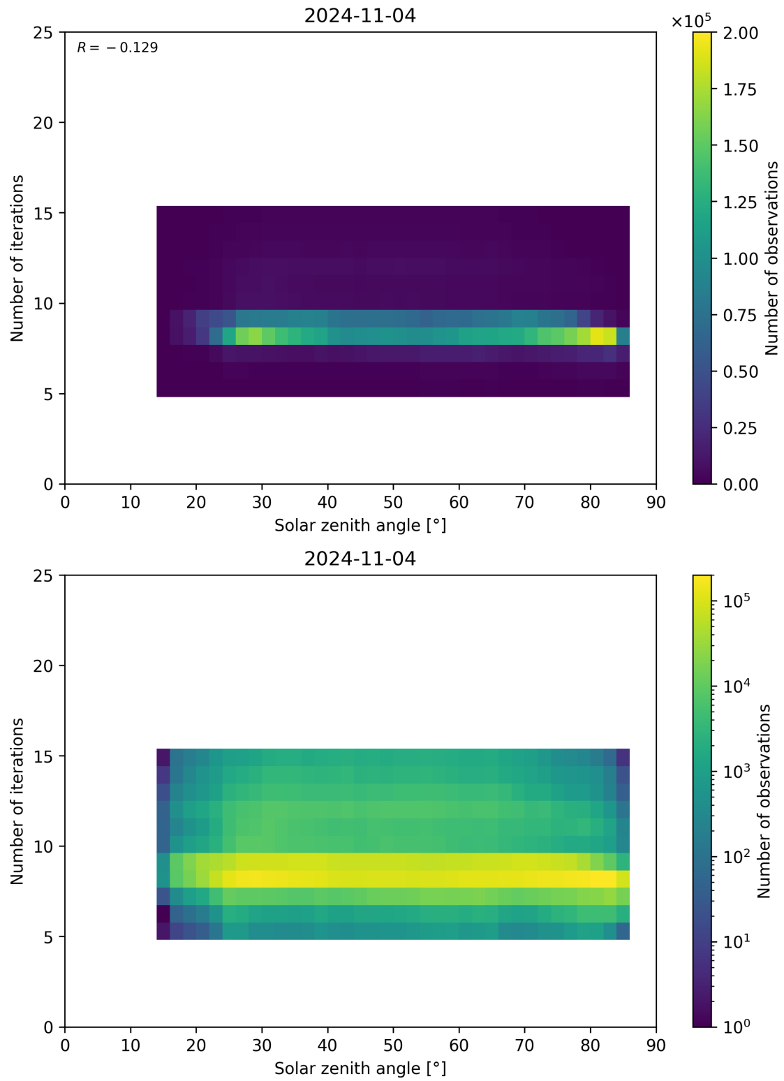
Figure 67: Scatter density plot of “Solar zenith angle” against “Number of iterations” for 2024-11-04 to 2024-11-05.
