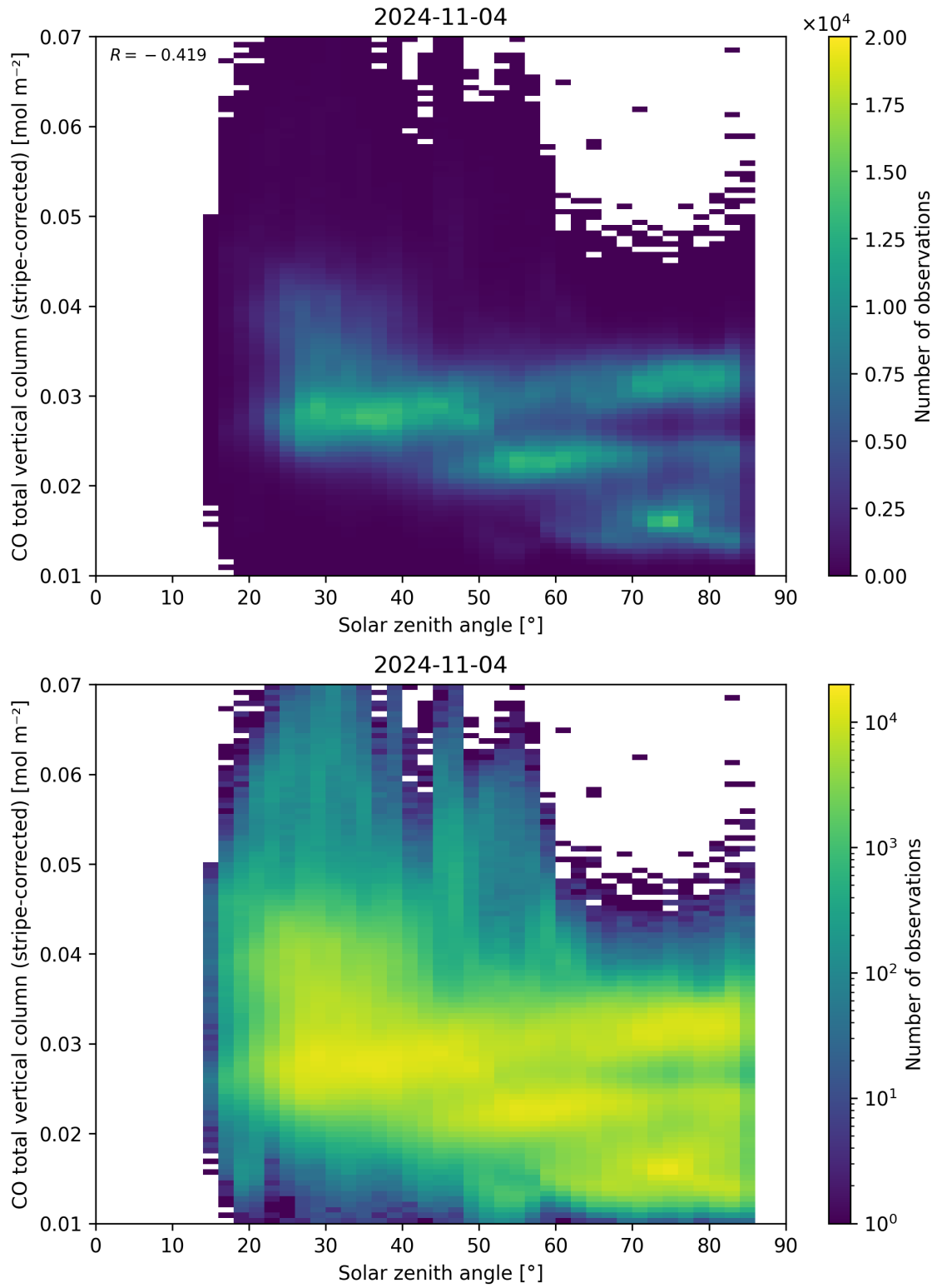
Figure 62: Scatter density plot of “Solar zenith angle” against “CO total vertical column (stripe-corrected)” for 2024-11-04 to 2024-11-05.
