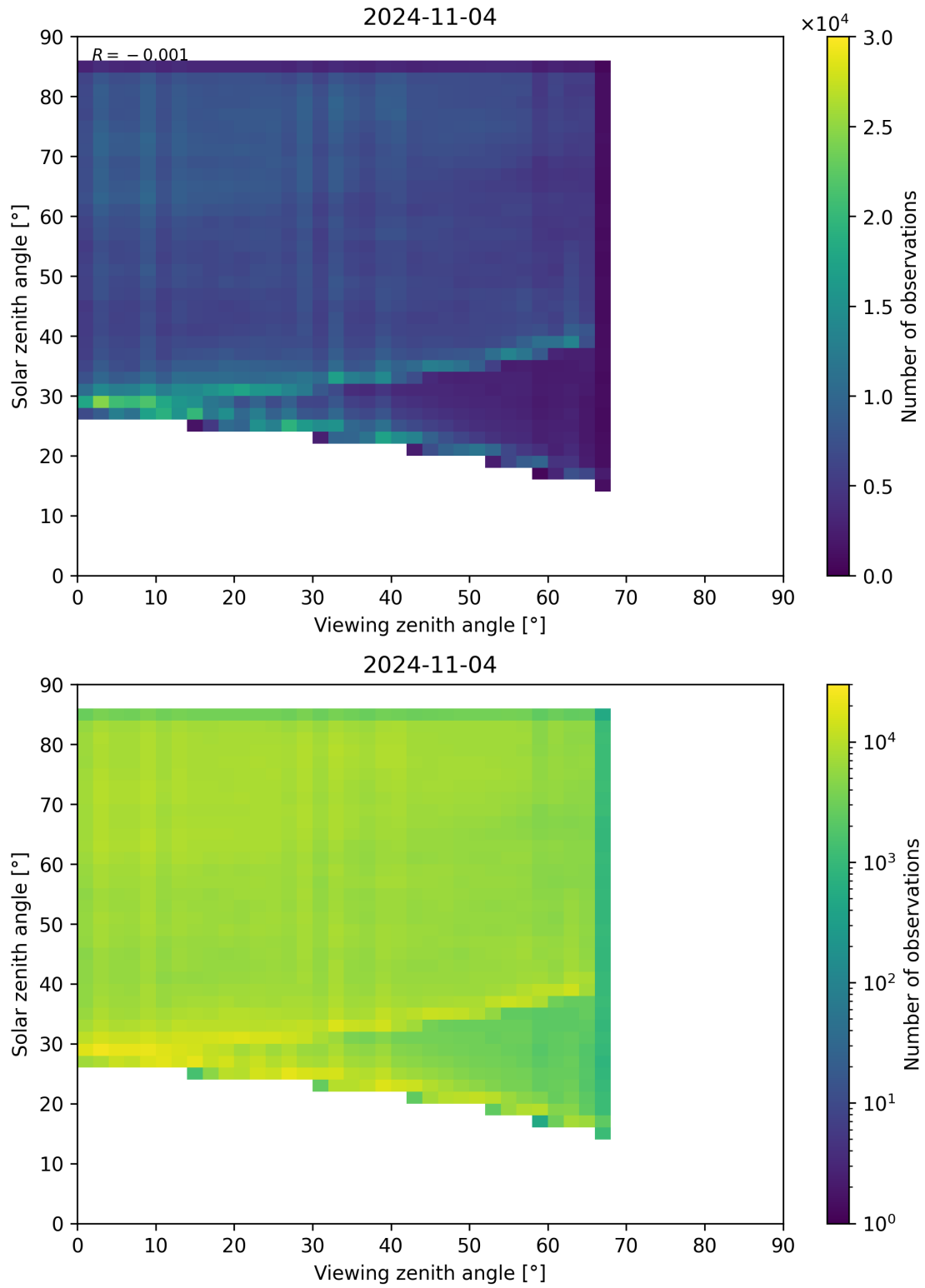
Figure 77: Scatter density plot of “Viewing zenith angle” against “Solar zenith angle” for 2024-11-04 to 2024-11-05.
