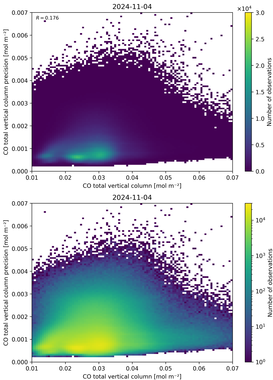
Figure 34: Scatter density plot of “CO total vertical column” against “CO total vertical column precision” for 2024-11-04 to 2024-11-05.
