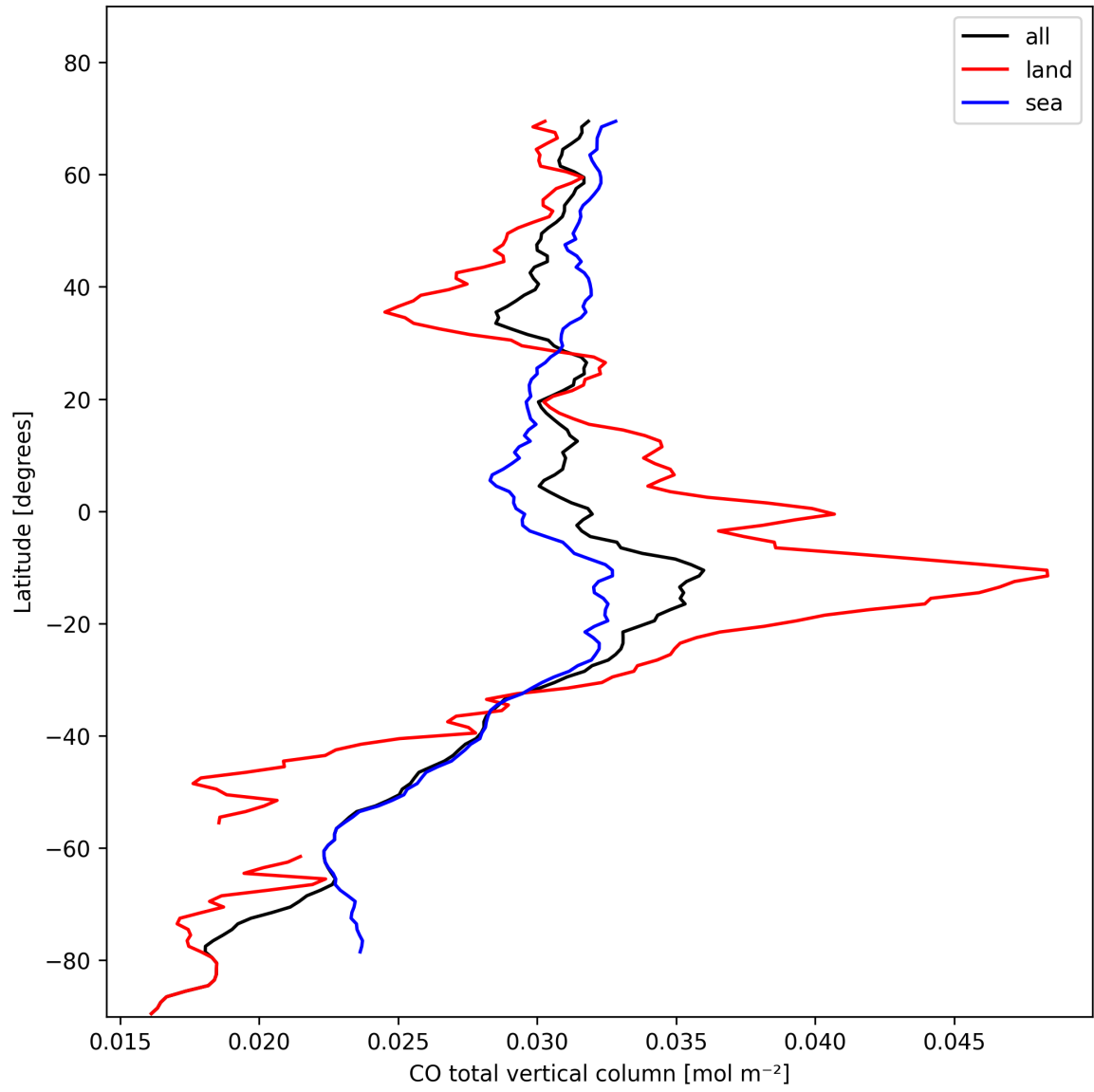
Figure 10: Zonal average of “CO total vertical column” for 2024-11-04 to 2024-11-05.
