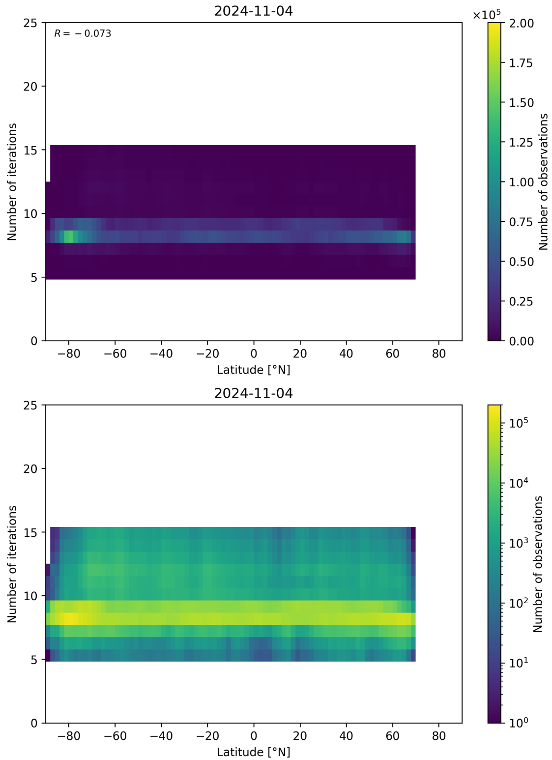
Figure 56: Scatter density plot of “Latitude” against “Number of iterations” for 2024-11-04 to 2024-11-05.
