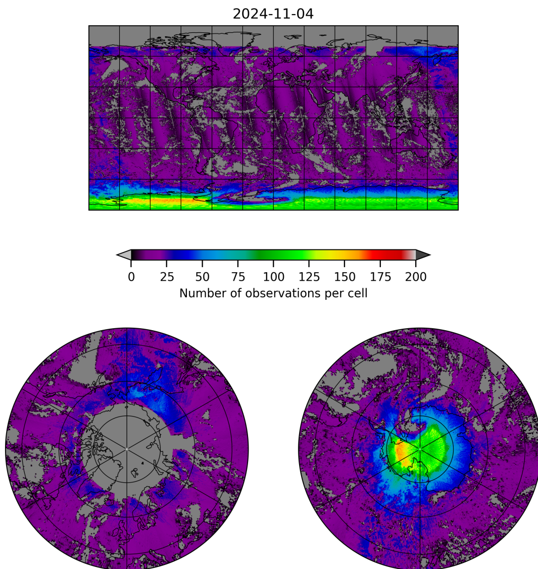
Figure 8: Map of the number of observations for 2024-11-04 to 2024-11-05
