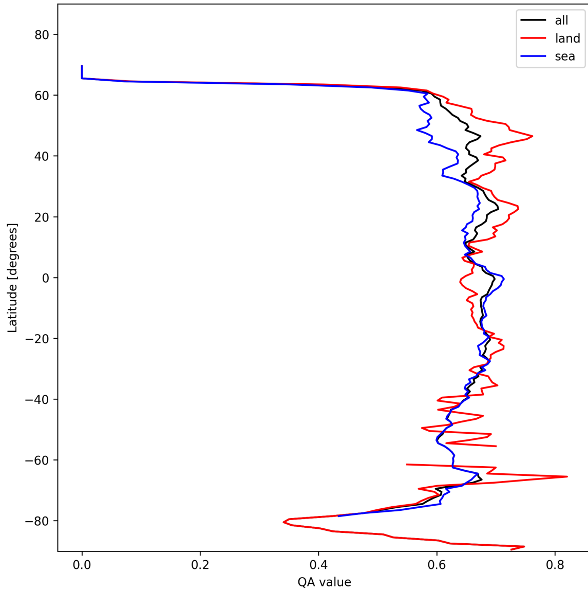
Figure 9: Zonal average of “QA value” for 2024-11-04 to 2024-11-05.
