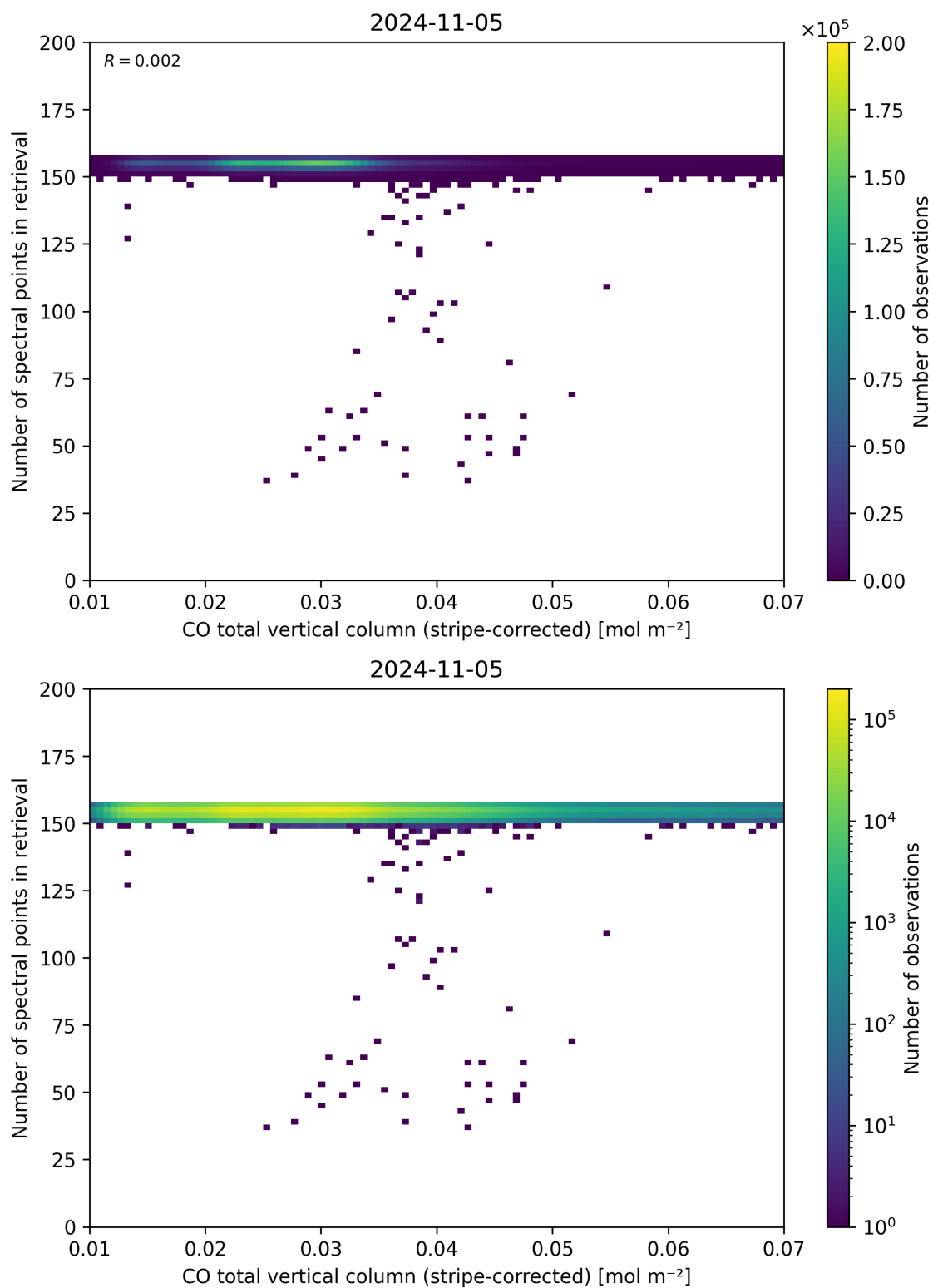
Figure 40: Scatter density plot of “CO total vertical column (stripe-corrected)” against “Number of spectral points in retrieval” for 2024-11-04 to 2024-11-06.
