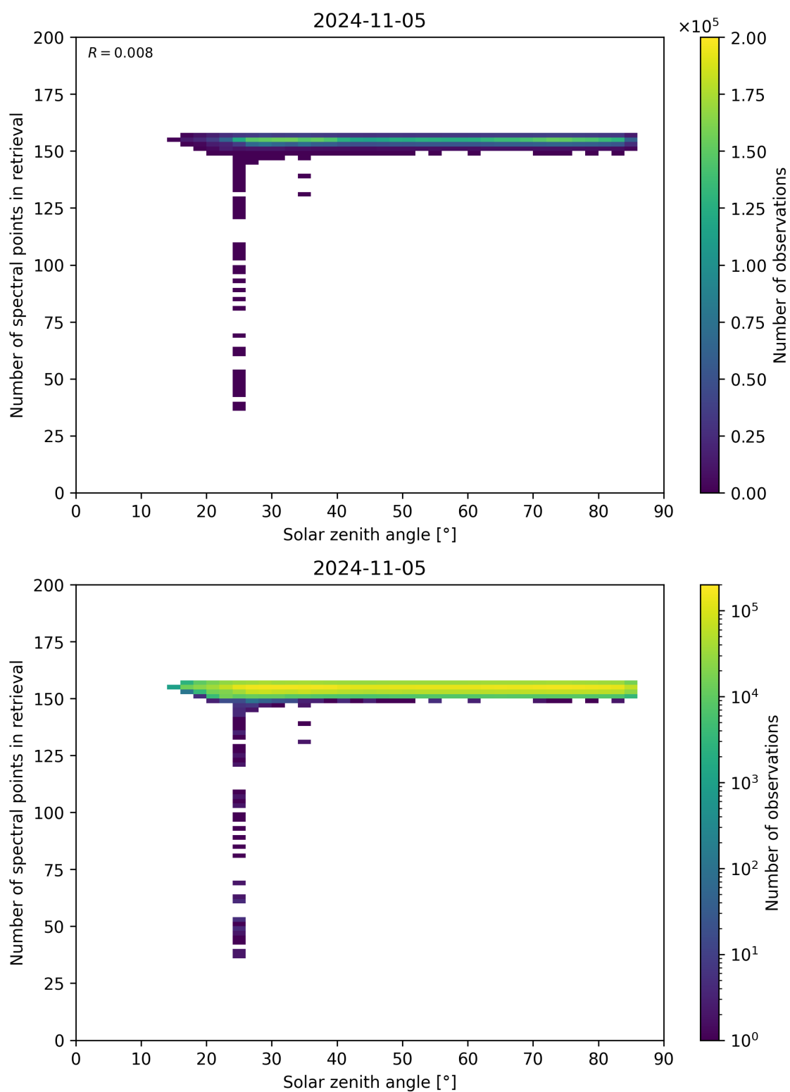
Figure 68: Scatter density plot of “Solar zenith angle” against “Number of spectral points in retrieval” for 2024-11-04 to 2024-11-06.
