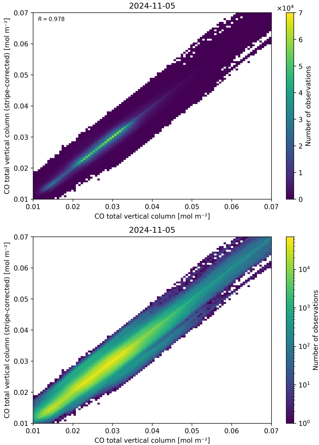
Figure 33: Scatter density plot of “CO total vertical column” against “CO total vertical column (stripe-corrected)” for 2024-11-04 to 2024-11-06.
