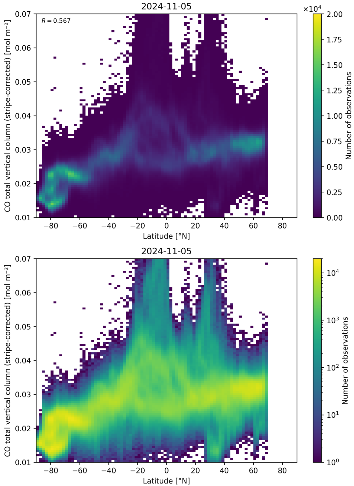
Figure 52: Scatter density plot of “Latitude” against “CO total vertical column (stripe-corrected)” for 2024-11-04 to 2024-11-06.
