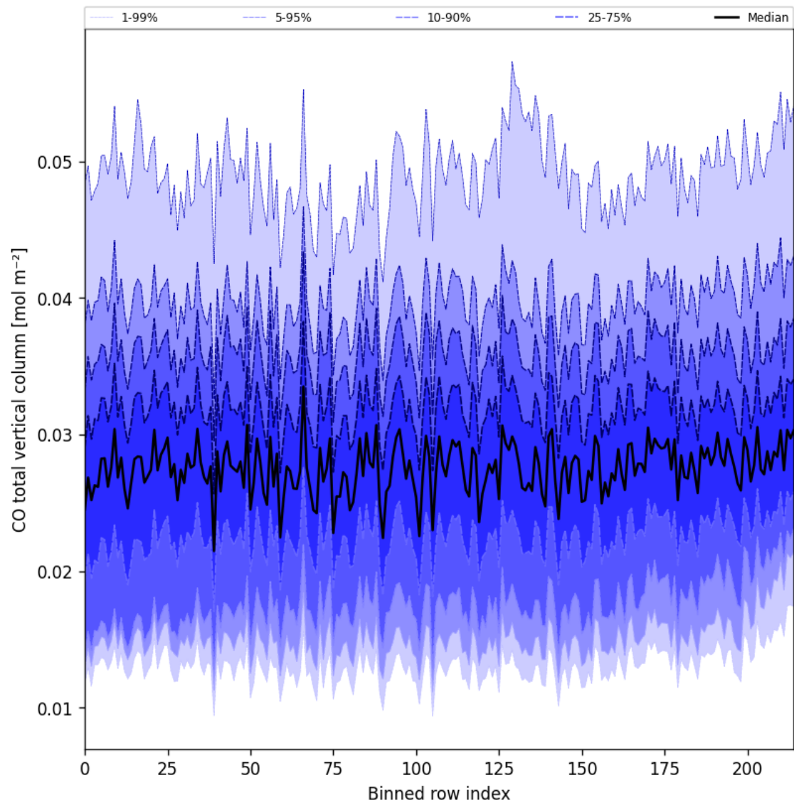
Figure 26: Along track statistics of “CO total vertical column” for 2024-11-04 to 2024-11-06
