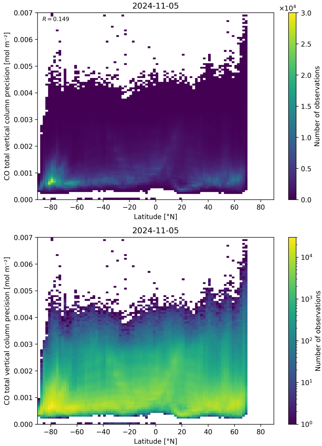
Figure 53: Scatter density plot of “Latitude” against “CO total vertical column precision” for 2024-11-04 to 2024-11-06.
