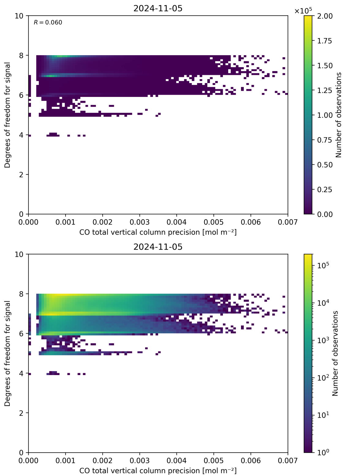
Figure 45: Scatter density plot of “CO total vertical column precision” against “Degrees of freedom for signal” for 2024-11-04 to 2024-11-06.
