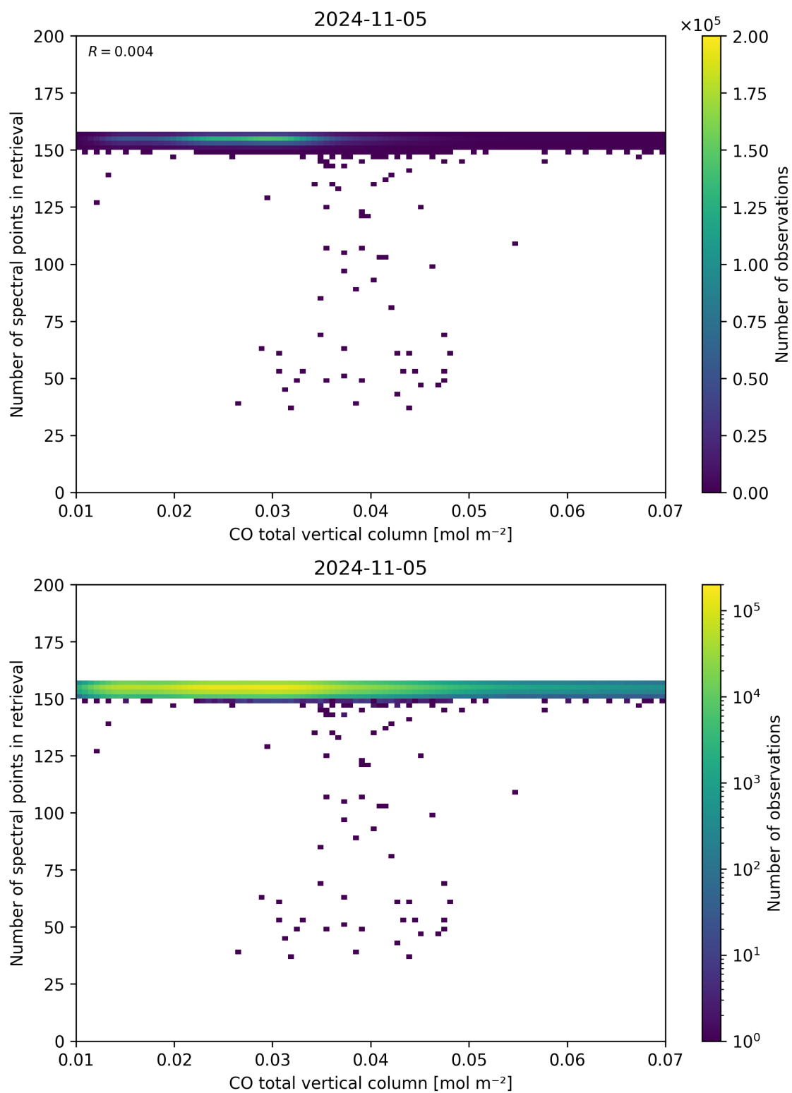
Figure 43: Scatter density plot of “CO total vertical column” against “Number of spectral points in retrieval” for 2024-11-04 to 2024-11-06.
