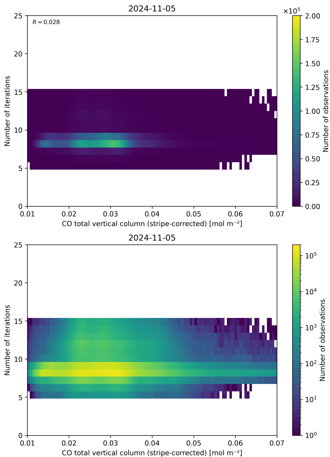
Figure 39: Scatter density plot of “CO total vertical column (stripe-corrected)” against “Number of iterations” for 2024-11-04 to 2024-11-06.
