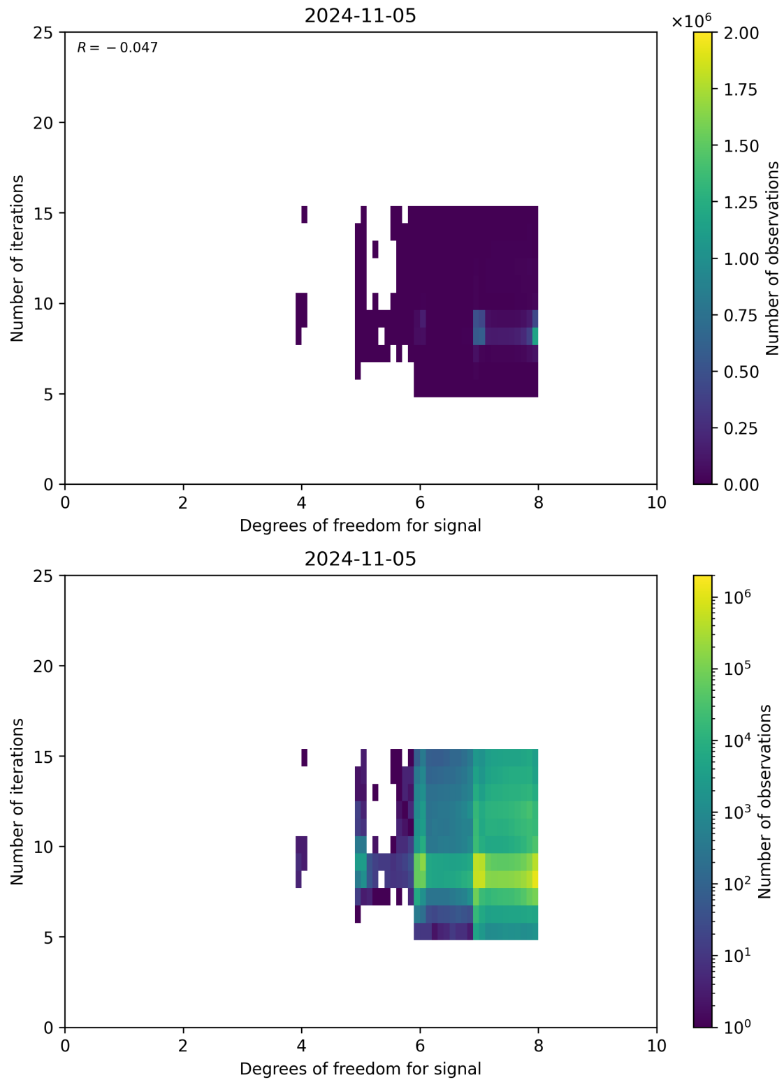
Figure 50: Scatter density plot of “Degrees of freedom for signal” against “Number of iterations” for 2024-11-04 to 2024-11-06.
