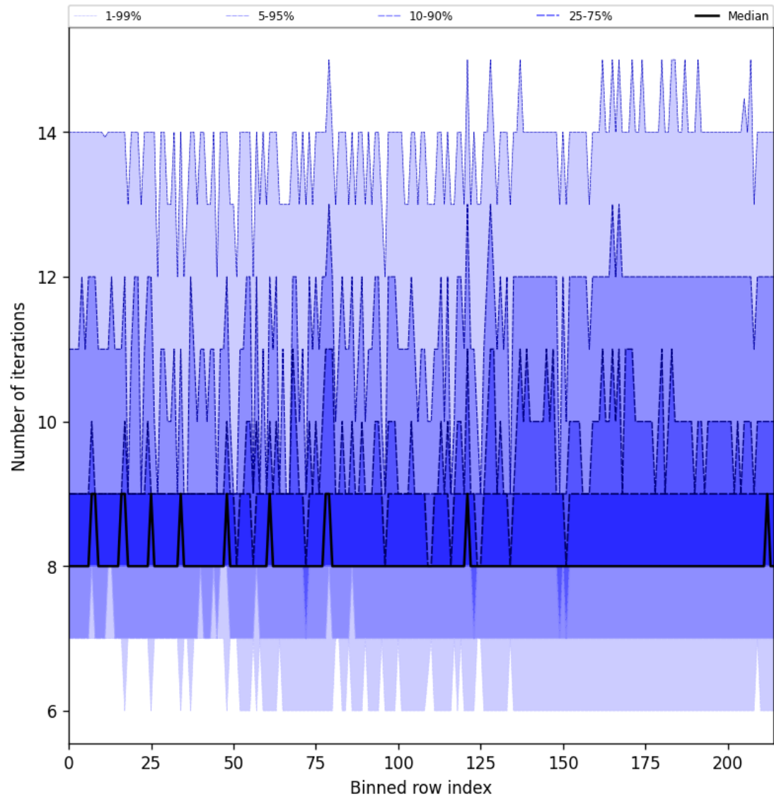
Figure 32: Along track statistics of “Number of iterations” for 2024-11-04 to 2024-11-06
