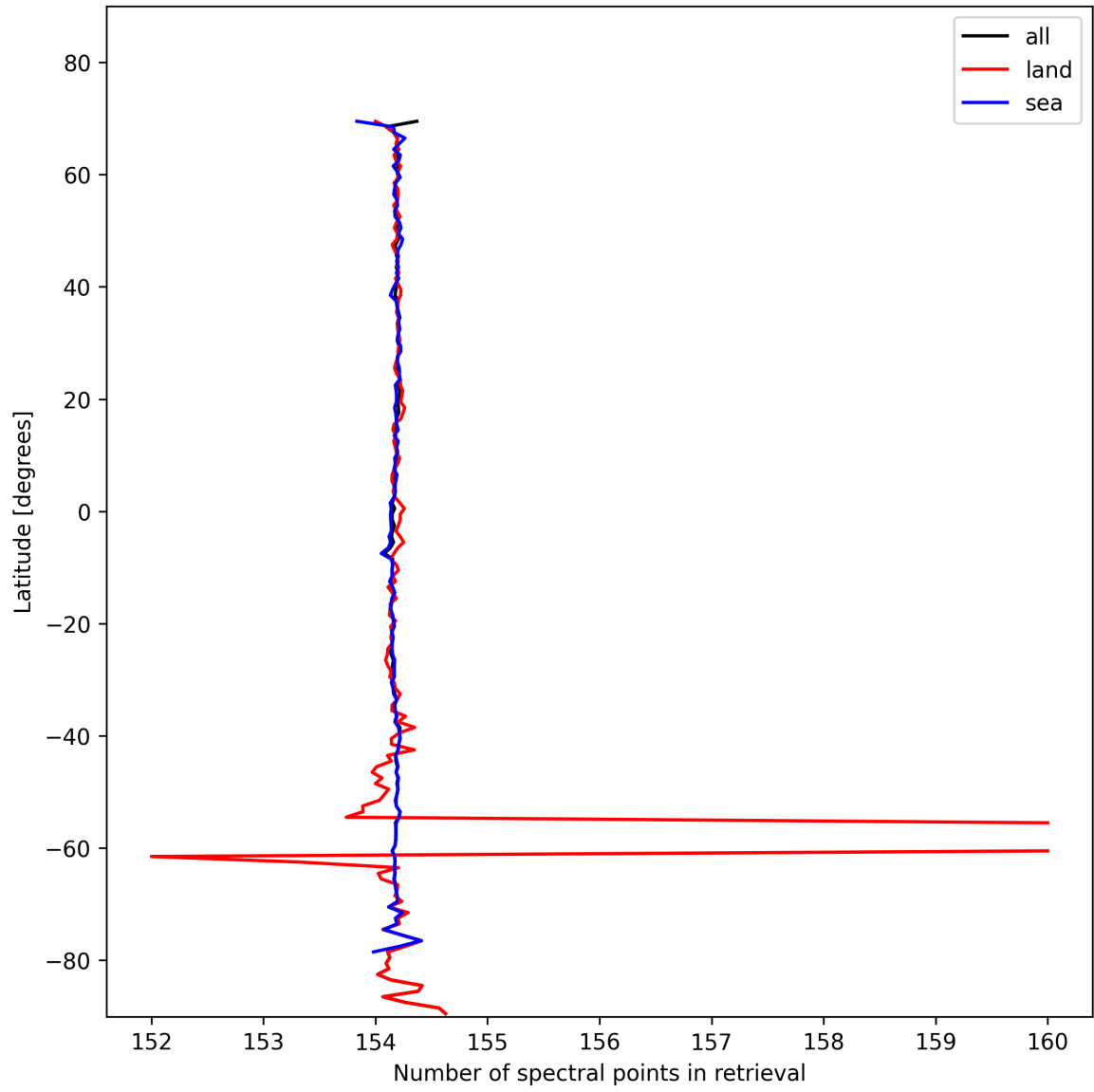
Figure 13: Zonal average of “Number of spectral points in retrieval” for 2024-11-04 to 2024-11-06.
