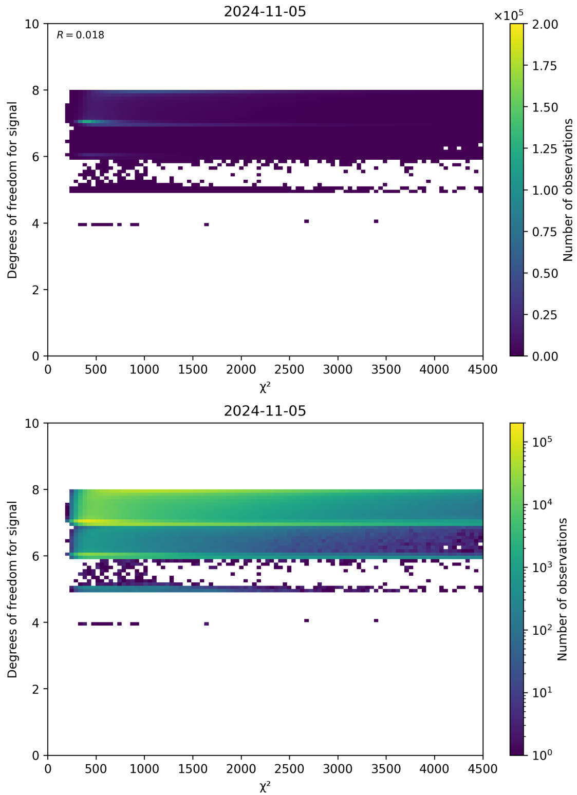
Figure 48: Scatter density plot of “ \chi^2 ” against “Degrees of freedom for signal” for 2024-11-04 to 2024-11-06.
