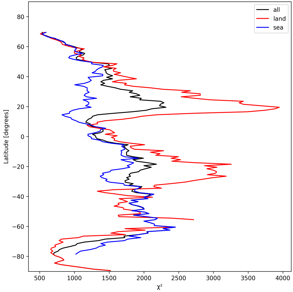
Figure 14: Zonal average of “ \chi^2 ” for 2024-11-04 to 2024-11-06.
