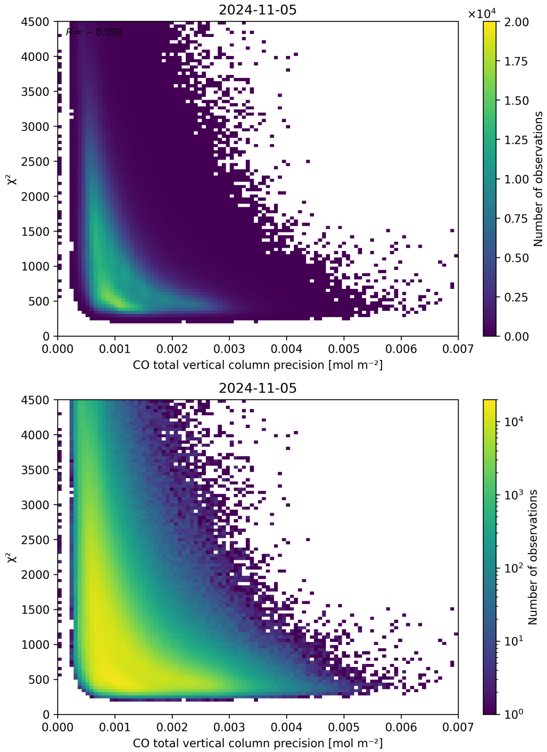
Figure 44: Scatter density plot of “CO total vertical column precision” against “ \chi^2 ” for 2024-11-04 to 2024-11-06.
