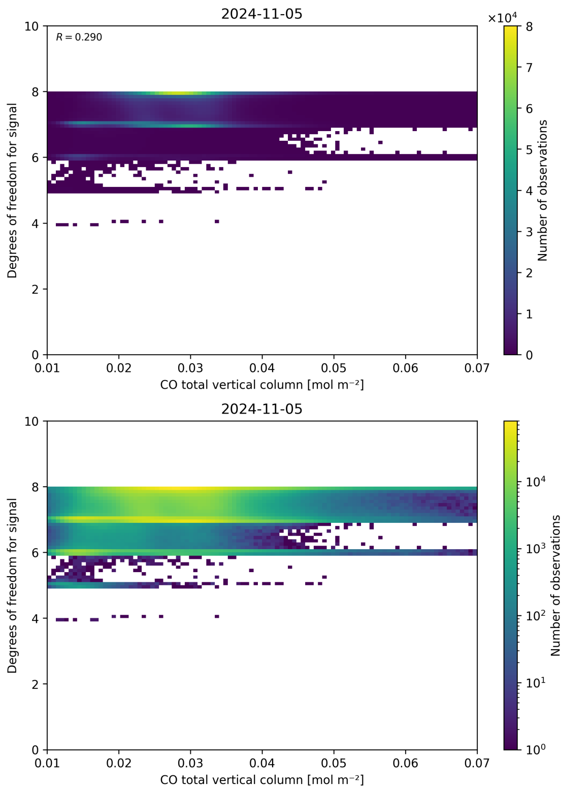
Figure 41: Scatter density plot of “CO total vertical column” against “Degrees of freedom for signal” for 2024-11-04 to 2024-11-06.
