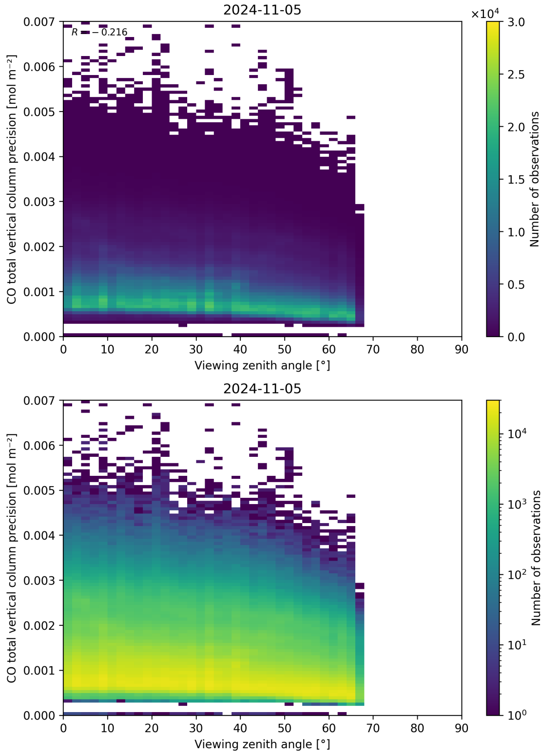
Figure 71: Scatter density plot of “Viewing zenith angle” against “CO total vertical column precision” for 2024-11-04 to 2024-11-06.
