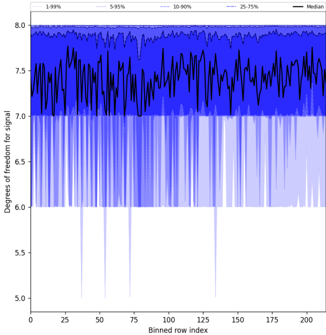
Figure 31: Along track statistics of “Degrees of freedom for signal” for 2024-11-04 to 2024-11-06
