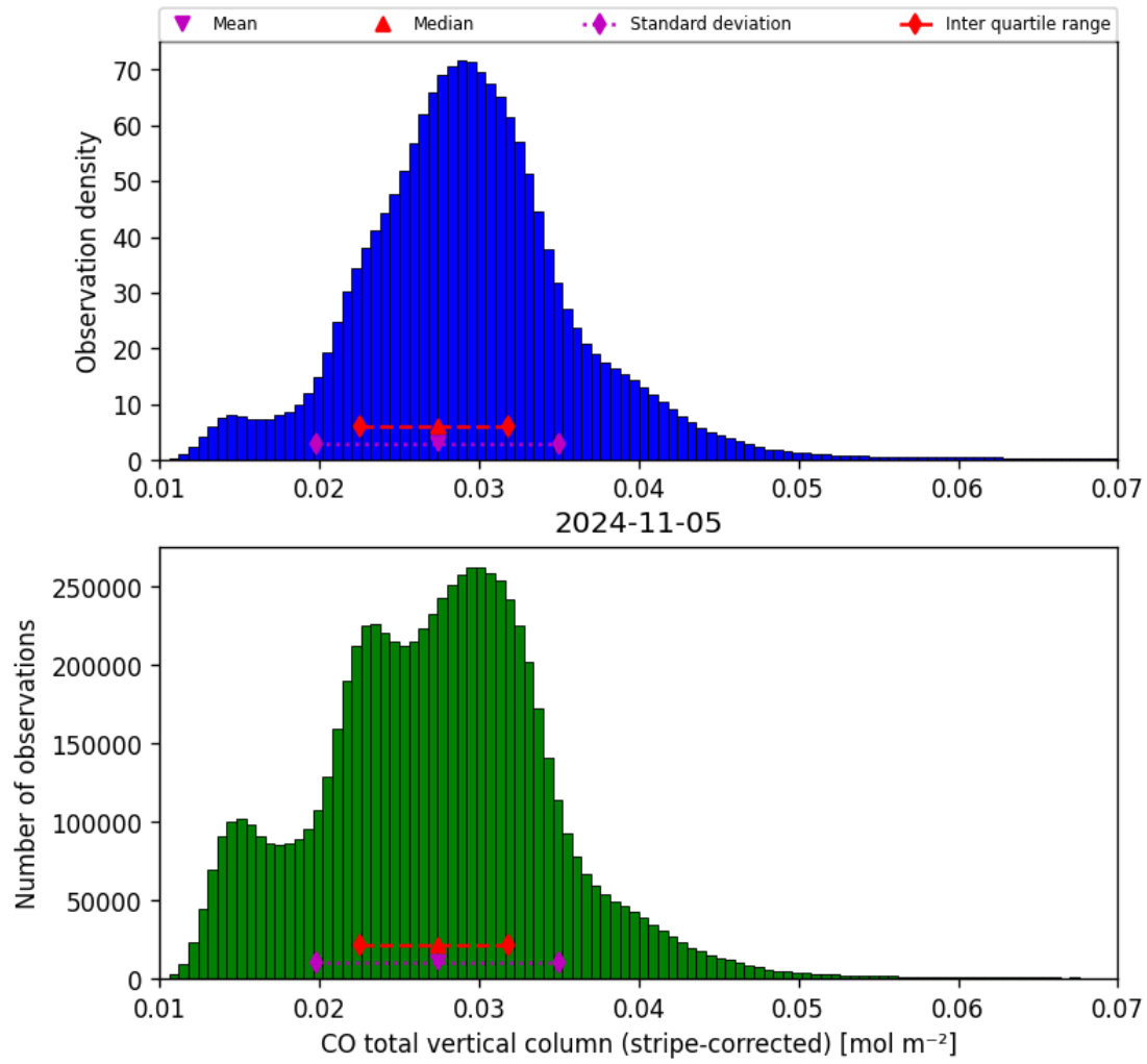
Figure 19: Histogram of “CO total vertical column (stripe-corrected)” for 2024-11-04 to 2024-11-06
