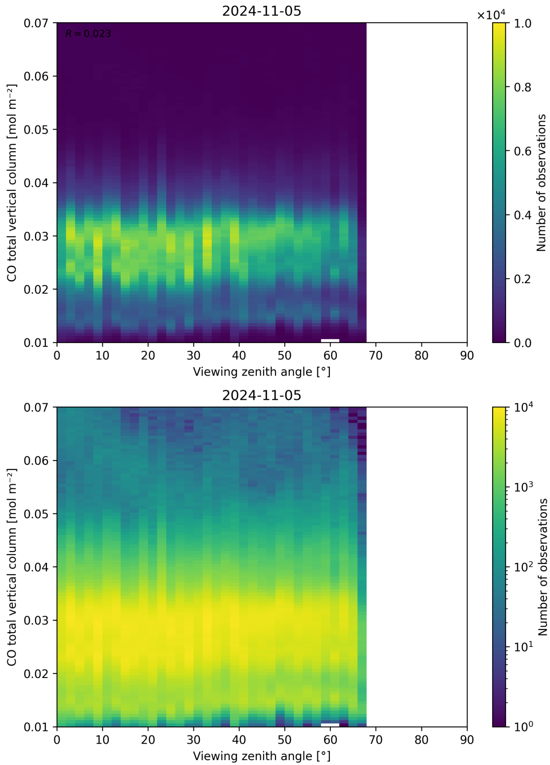
Figure 69: Scatter density plot of “Viewing zenith angle” against “CO total vertical column” for 2024-11-04 to 2024-11-06.
