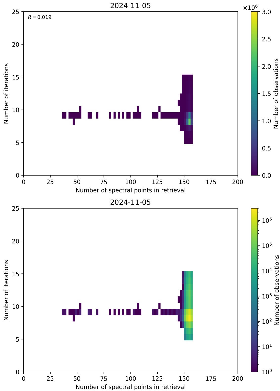
Figure 60: Scatter density plot of “Number of spectral points in retrieval” against “Number of iterations” for 2024-11-04 to 2024-11-06.
