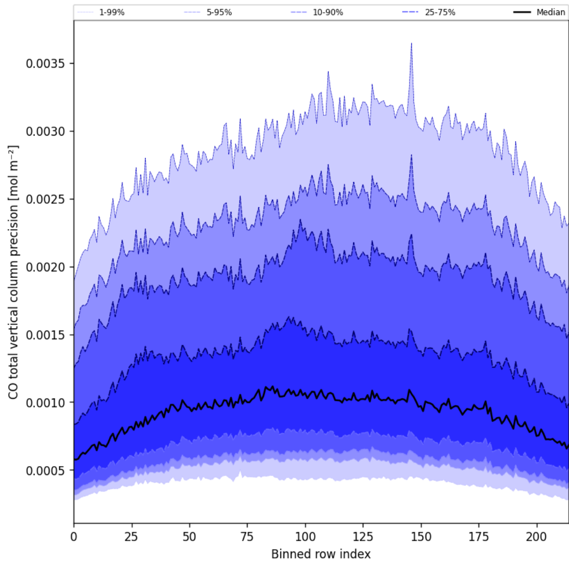
Figure 28: Along track statistics of “CO total vertical column precision” for 2024-11-04 to 2024-11-06
