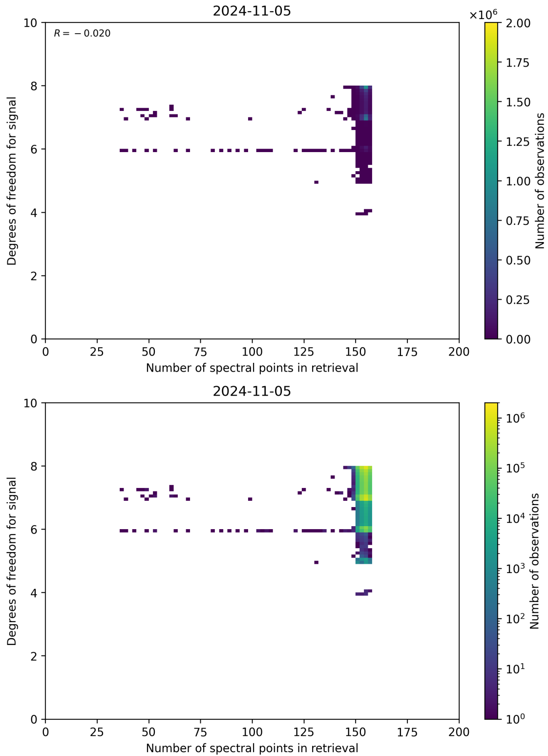
Figure 59: Scatter density plot of “Number of spectral points in retrieval” against “Degrees of freedom for signal” for 2024-11-04 to 2024-11-06.
