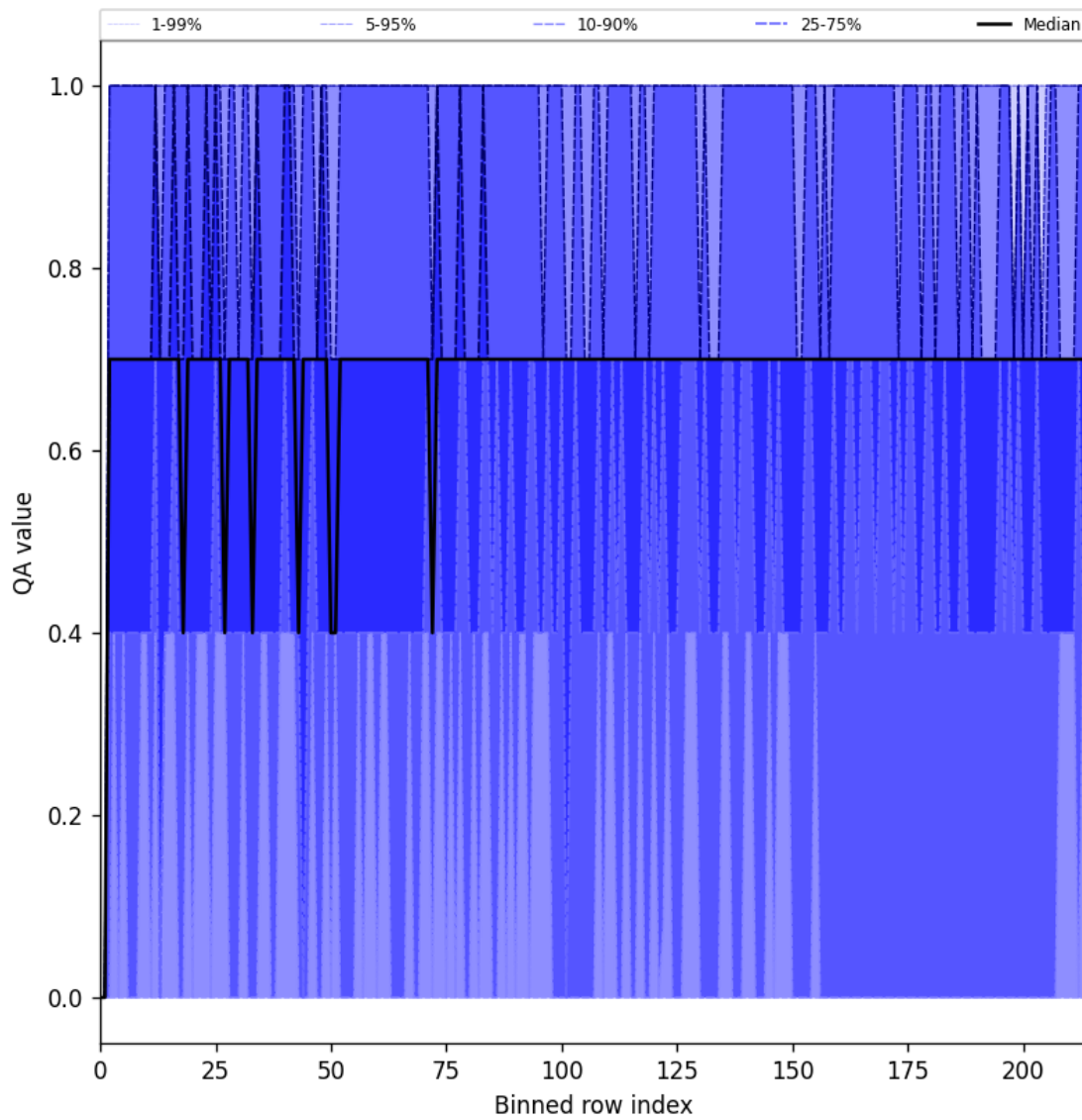
Figure 25: Along track statistics of “QA value” for 2024-11-04 to 2024-11-06
