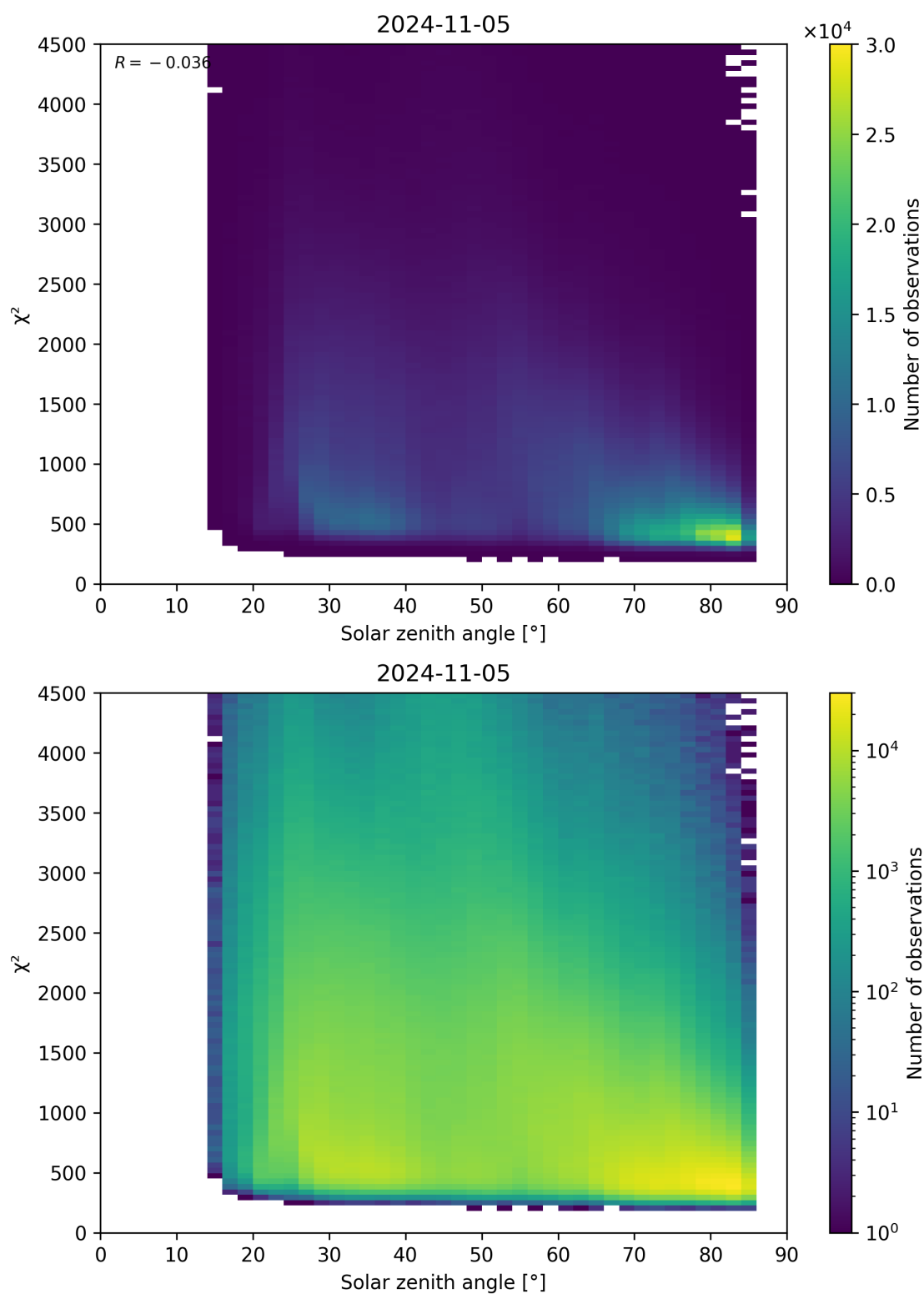
Figure 64: Scatter density plot of “Solar zenith angle” against “ \chi^2 ” for 2024-11-04 to 2024-11-06.
