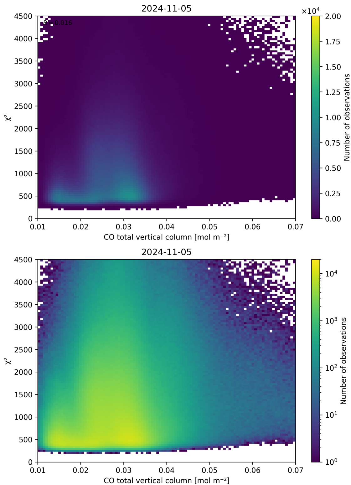
Figure 35: Scatter density plot of “CO total vertical column” against “ \chi^2 ” for 2024-11-04 to 2024-11-06.
