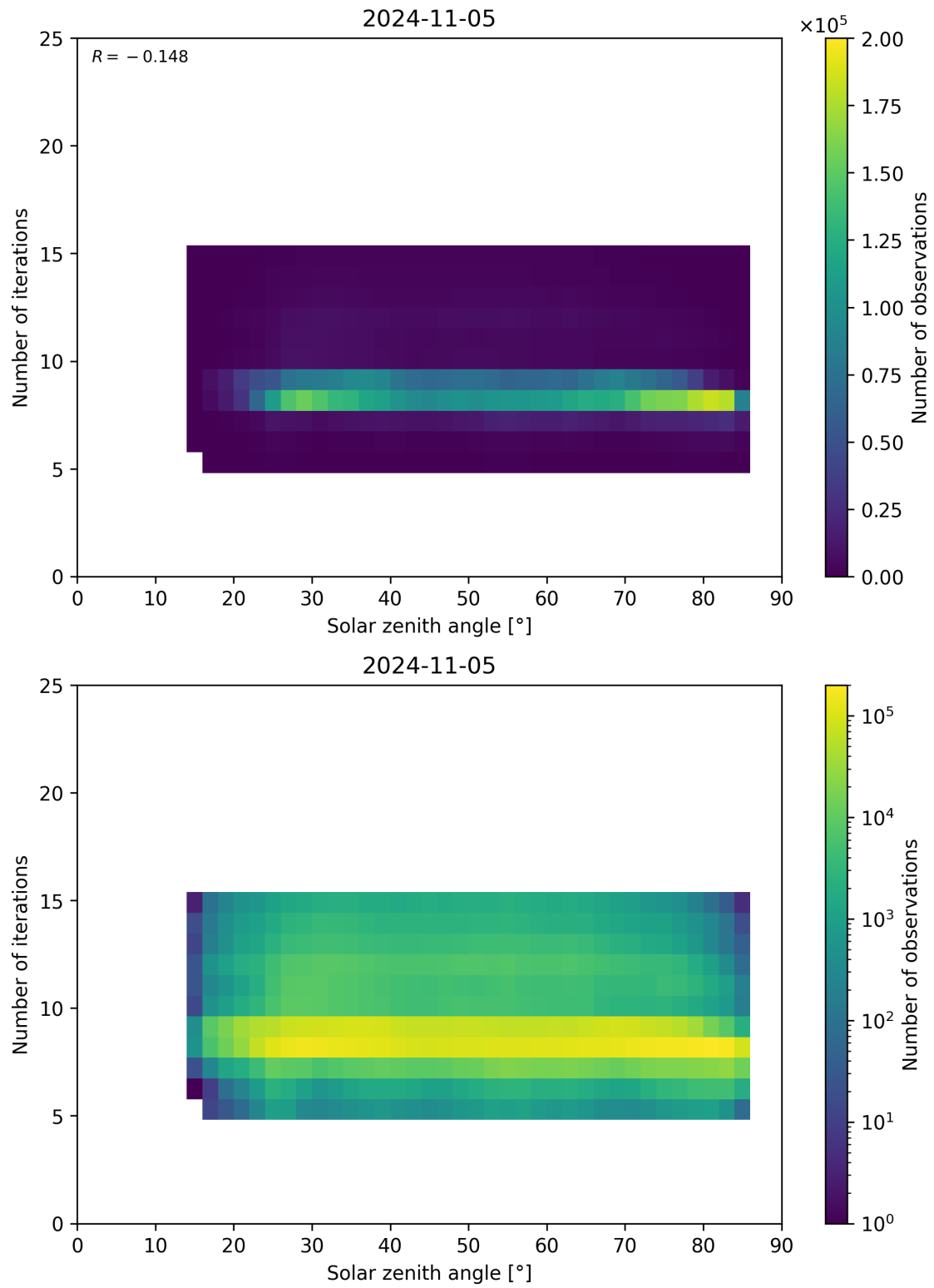
Figure 67: Scatter density plot of “Solar zenith angle” against “Number of iterations” for 2024-11-04 to 2024-11-06.
