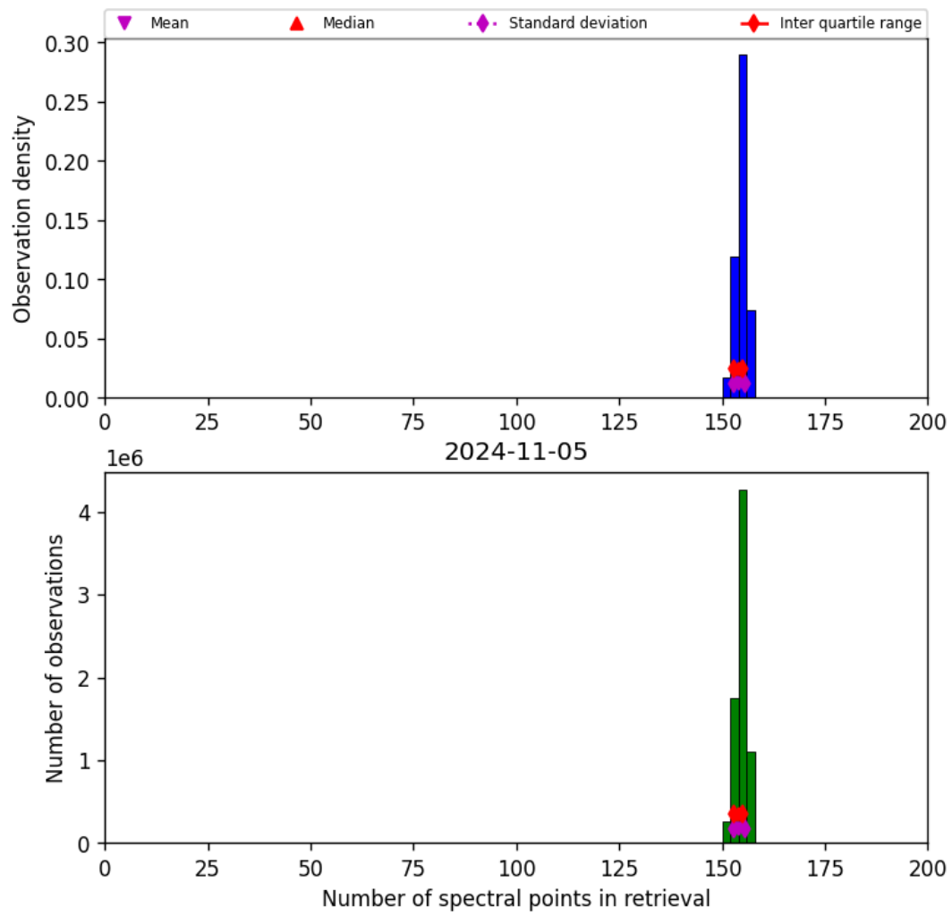
Figure 21: Histogram of “Number of spectral points in retrieval” for 2024-11-04 to 2024-11-06
