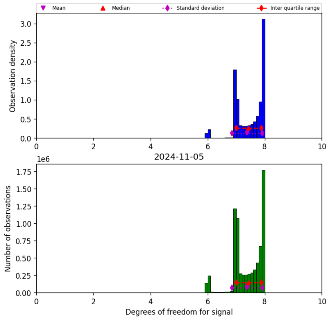
Figure 23: Histogram of “Degrees of freedom for signal” for 2024-11-04 to 2024-11-06
