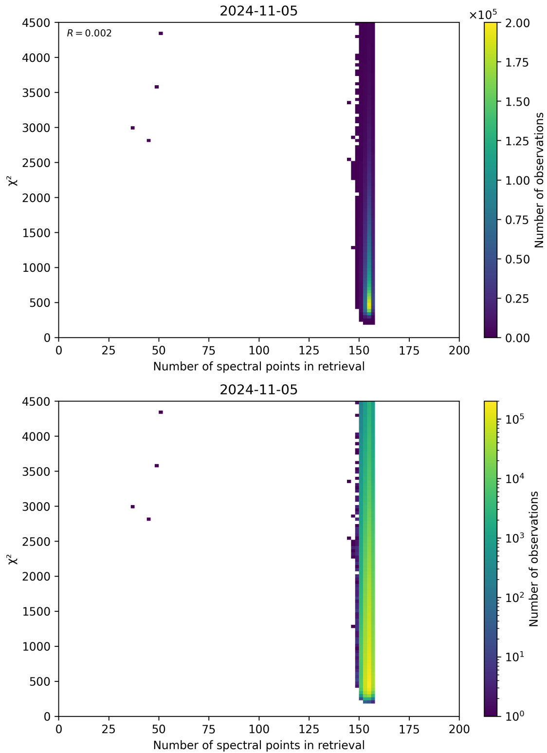
Figure 58: Scatter density plot of “Number of spectral points in retrieval” against “ \chi^2 ” for 2024-11-04 to 2024-11-06.
