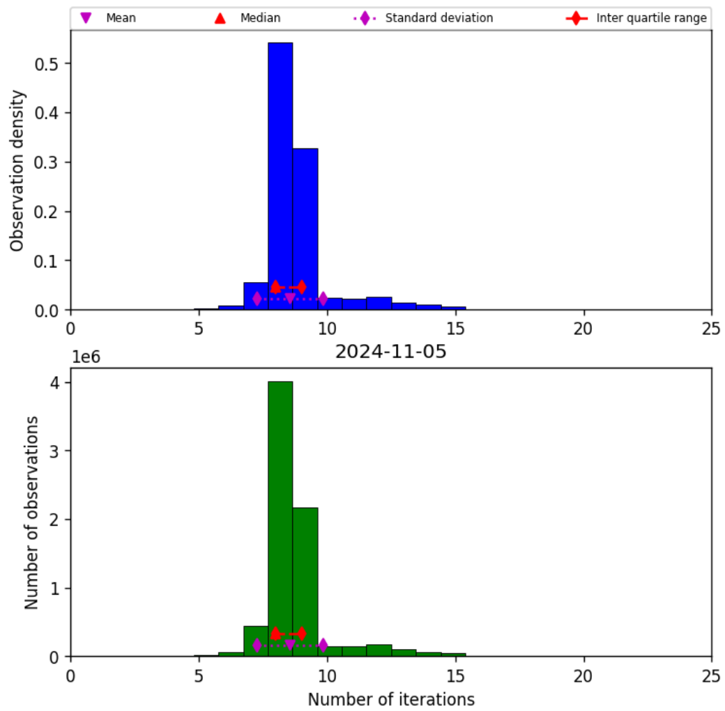
Figure 24: Histogram of “Number of iterations” for 2024-11-04 to 2024-11-06
