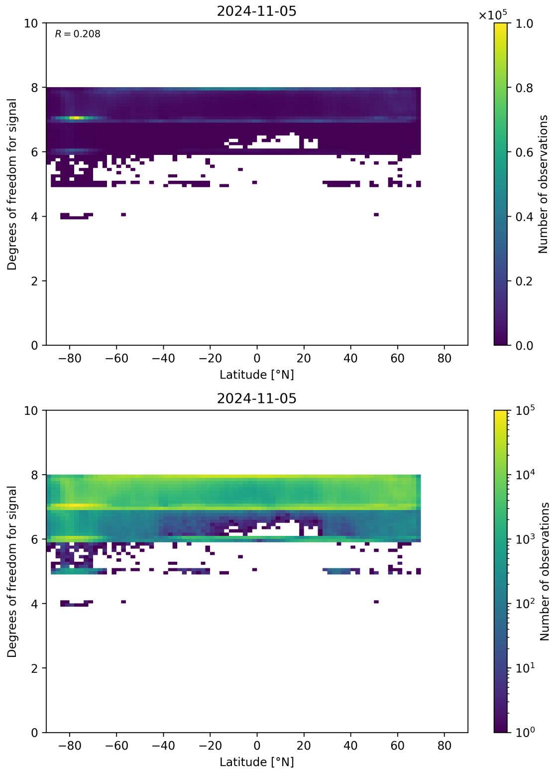
Figure 55: Scatter density plot of “Latitude” against “Degrees of freedom for signal” for 2024-11-04 to 2024-11-06.
