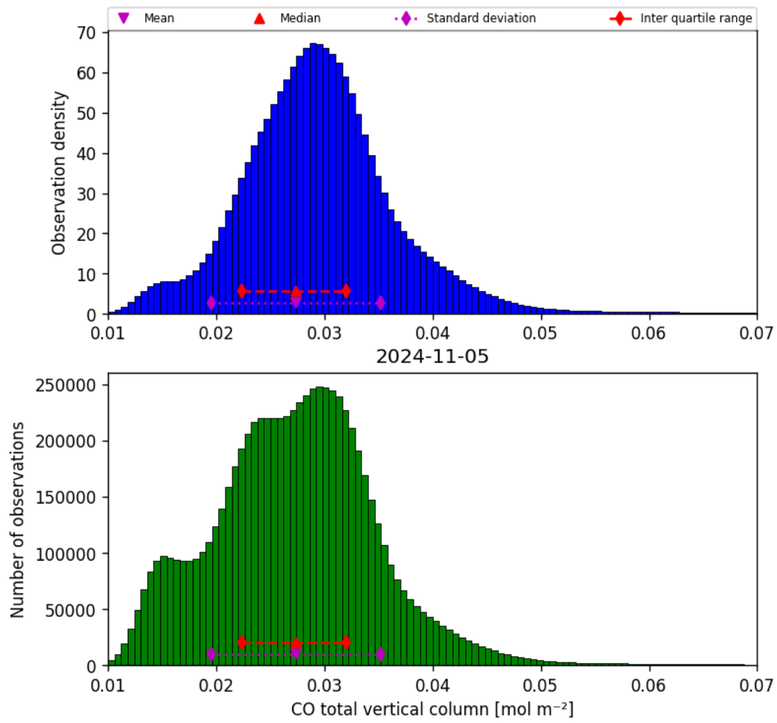
Figure 18: Histogram of “CO total vertical column” for 2024-11-04 to 2024-11-06
