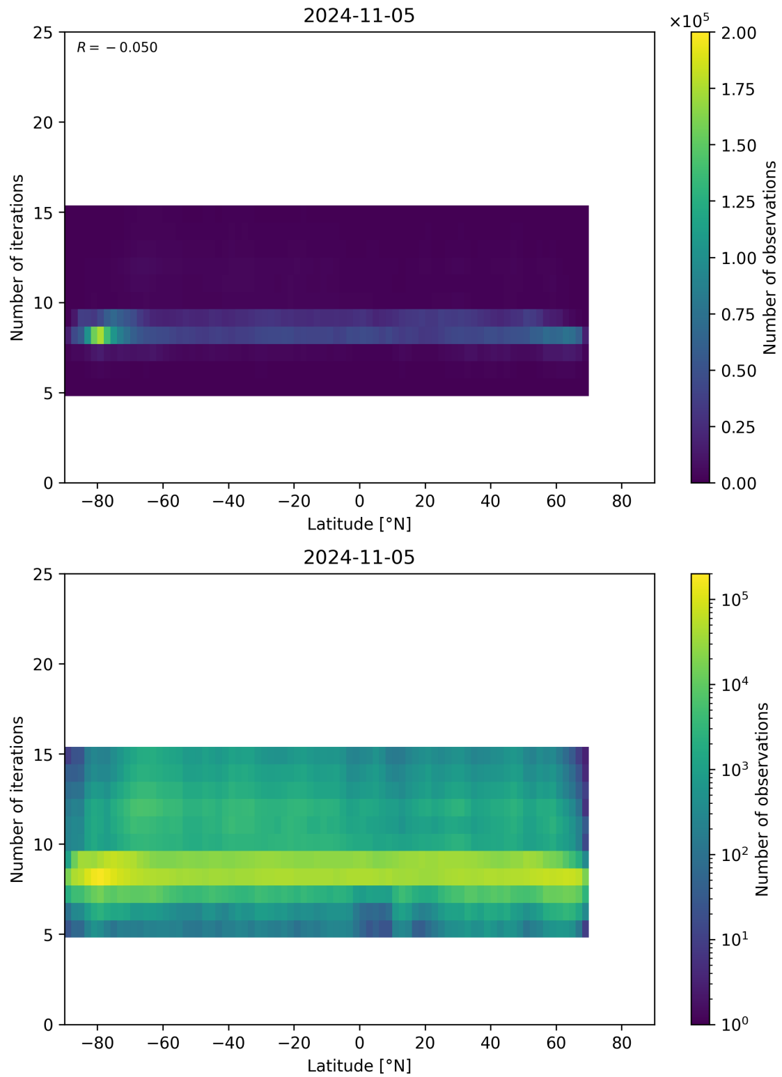
Figure 56: Scatter density plot of “Latitude” against “Number of iterations” for 2024-11-04 to 2024-11-06.
