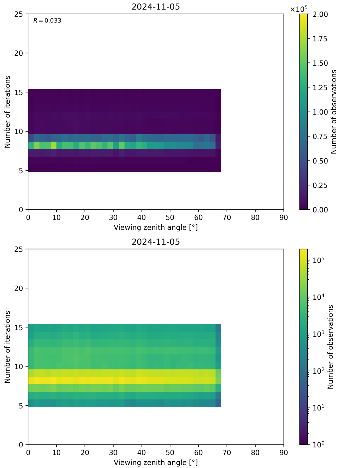
Figure 75: Scatter density plot of “Viewing zenith angle” against “Number of iterations” for 2024-11-04 to 2024-11-06.
