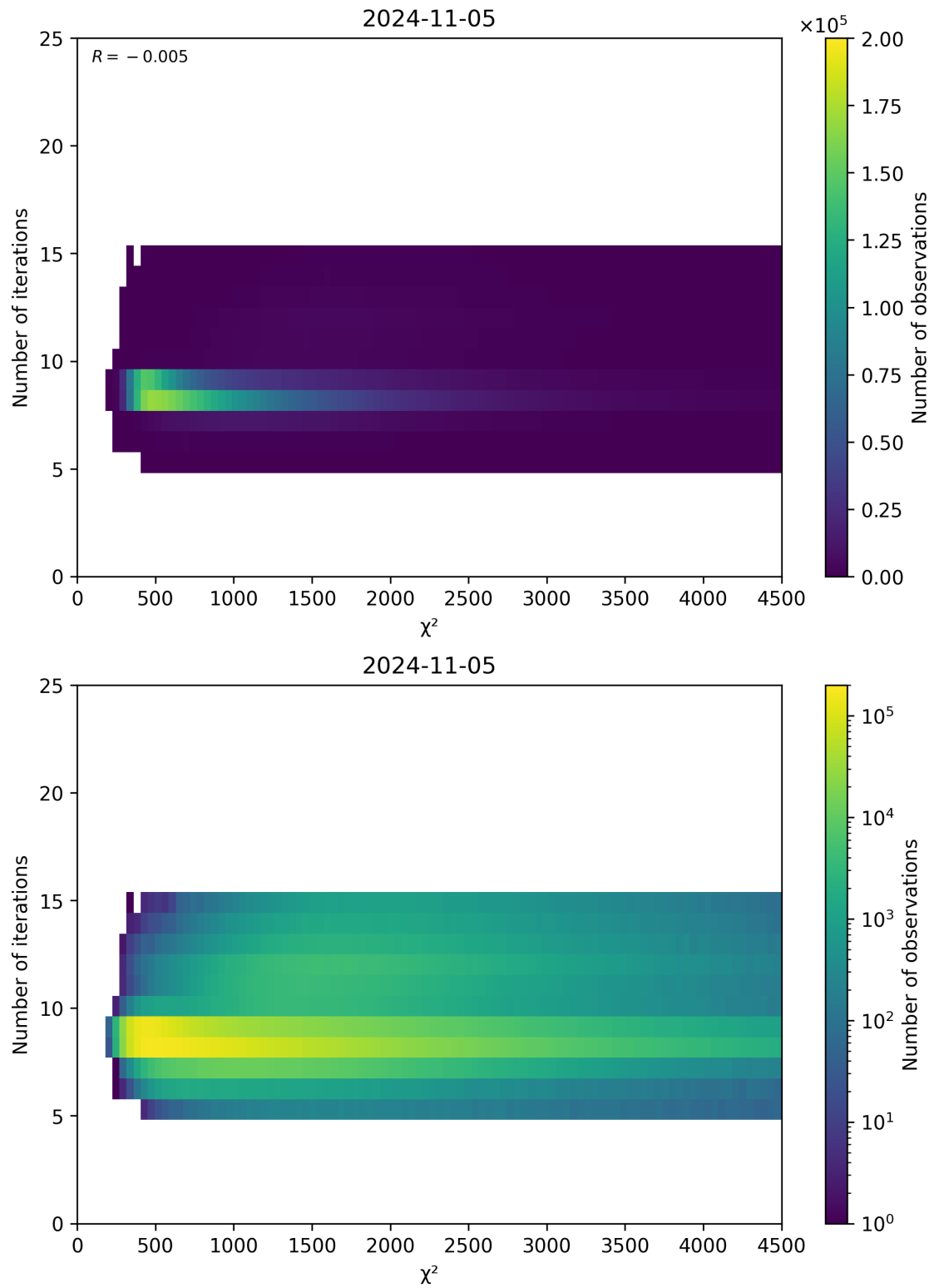
Figure 49: Scatter density plot of “ \chi^2 ” against “Number of iterations” for 2024-11-04 to 2024-11-06.
