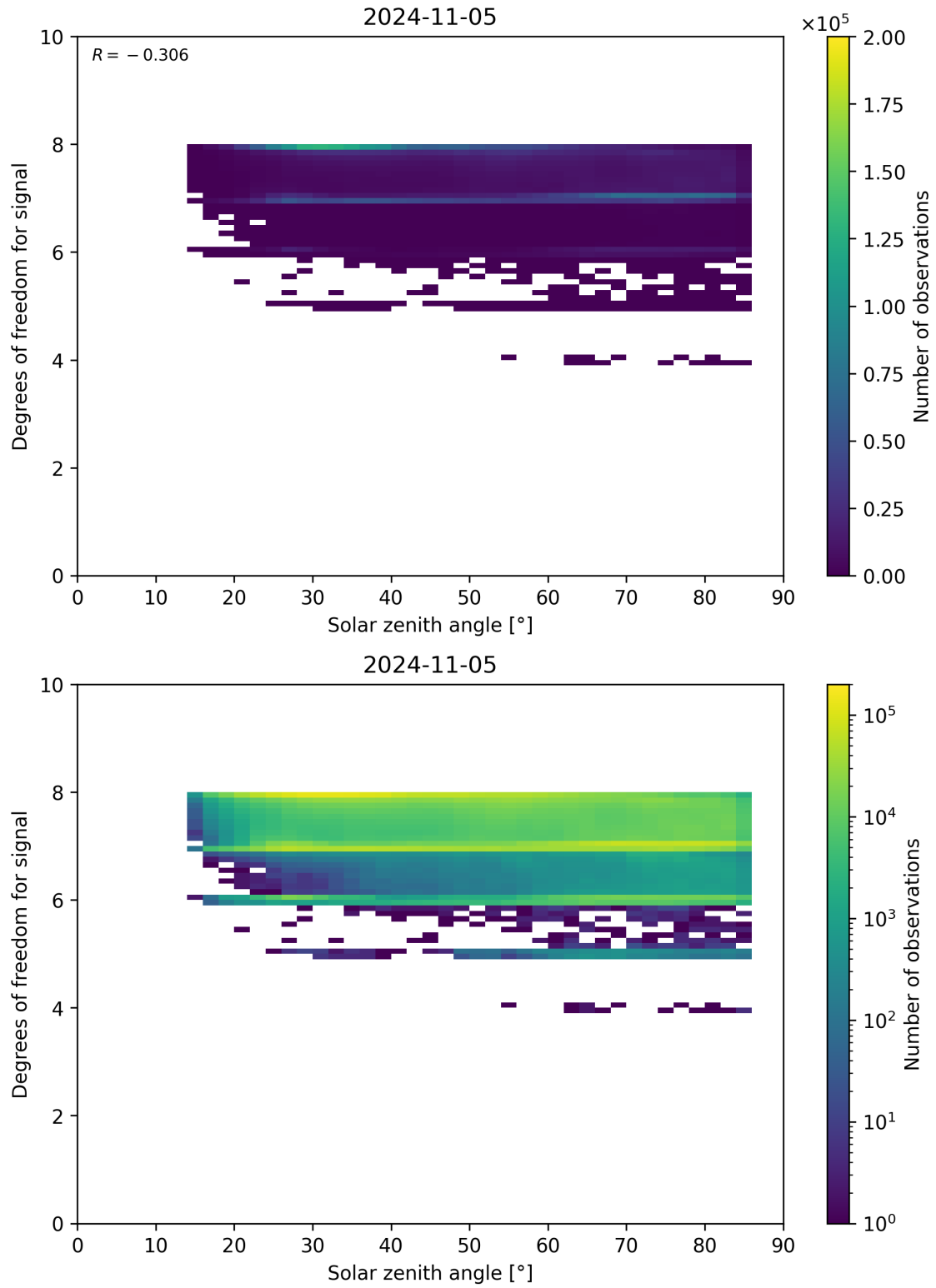
Figure 65: Scatter density plot of “Solar zenith angle” against “Degrees of freedom for signal” for 2024-11-04 to 2024-11-06.
