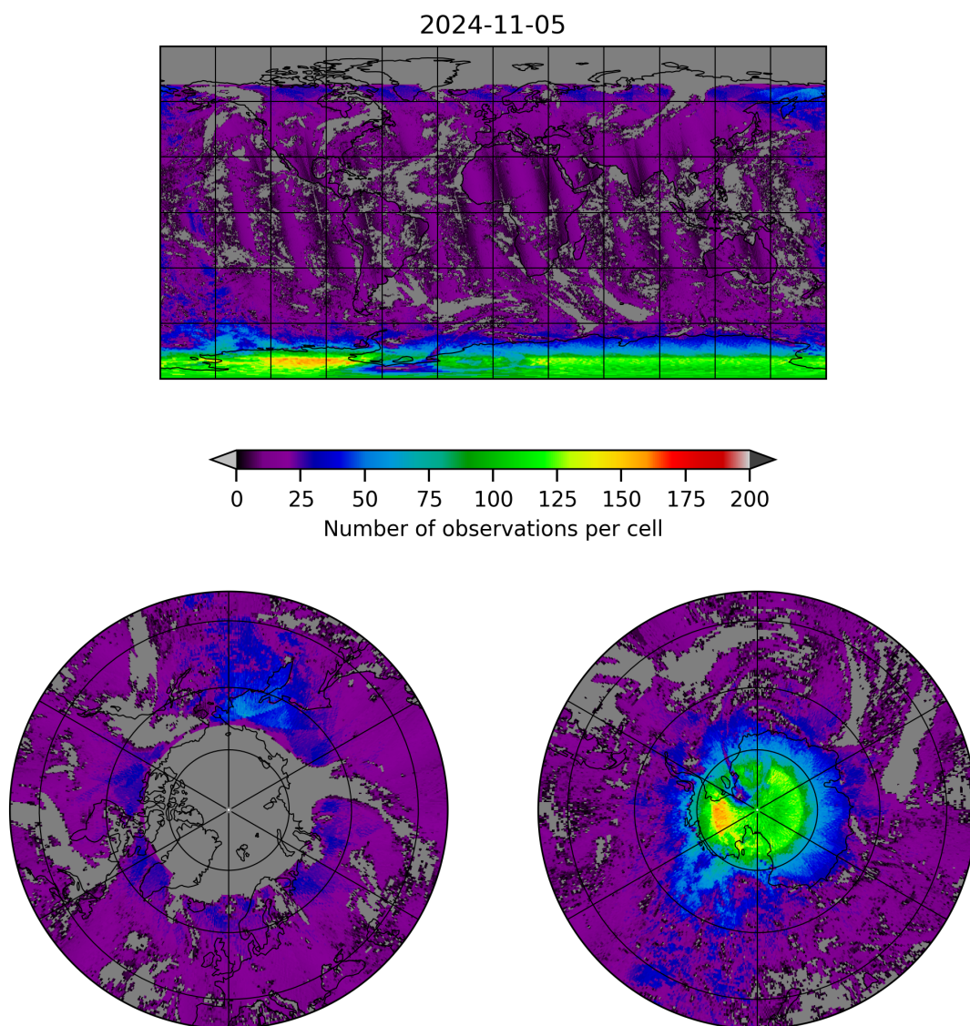
Figure 8: Map of the number of observations for 2024-11-04 to 2024-11-06
