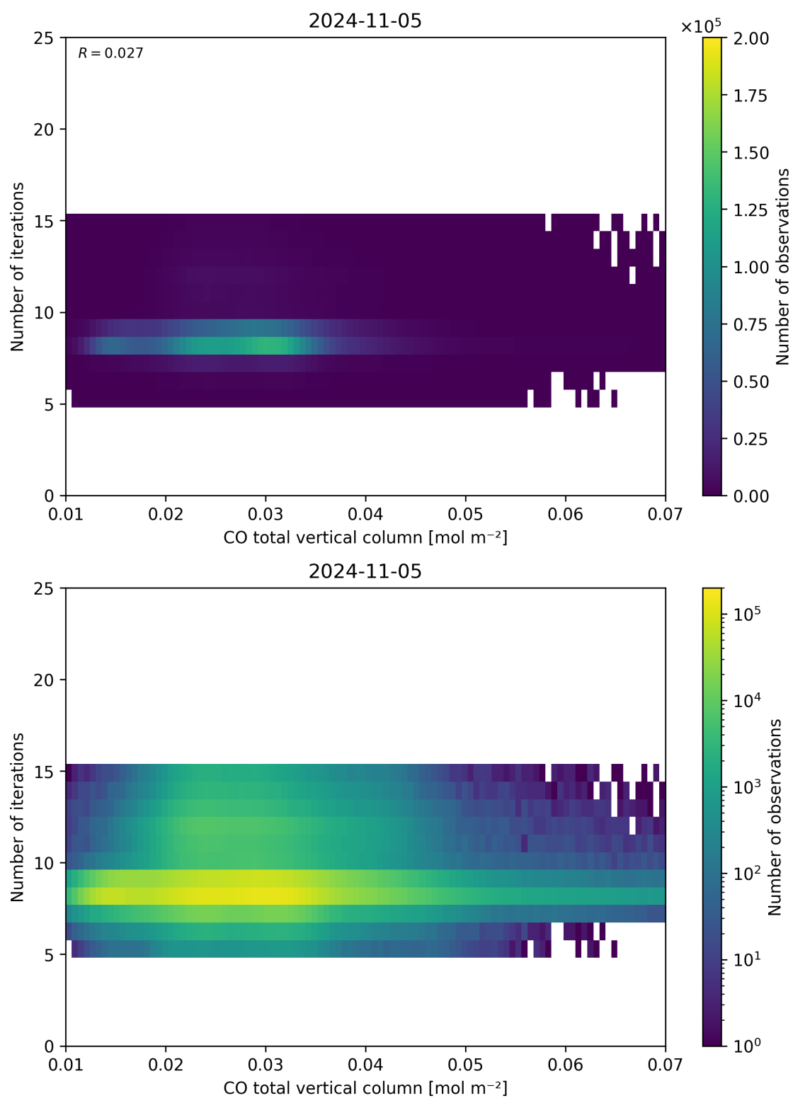
Figure 42: Scatter density plot of “CO total vertical column” against “Number of iterations” for 2024-11-04 to 2024-11-06.
