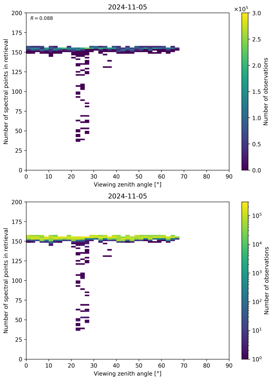
Figure 76: Scatter density plot of “Viewing zenith angle” against “Number of spectral points in retrieval” for 2024-11-04 to 2024-11-06.
