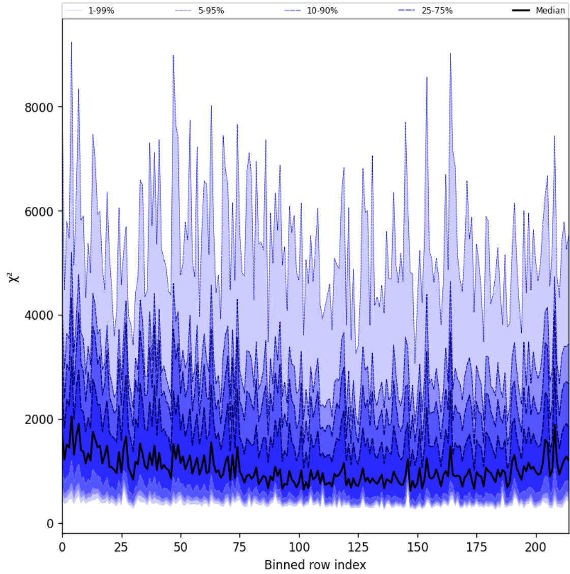
Figure 30: Along track statistics of “ \chi^2 ” for 2024-11-04 to 2024-11-06
