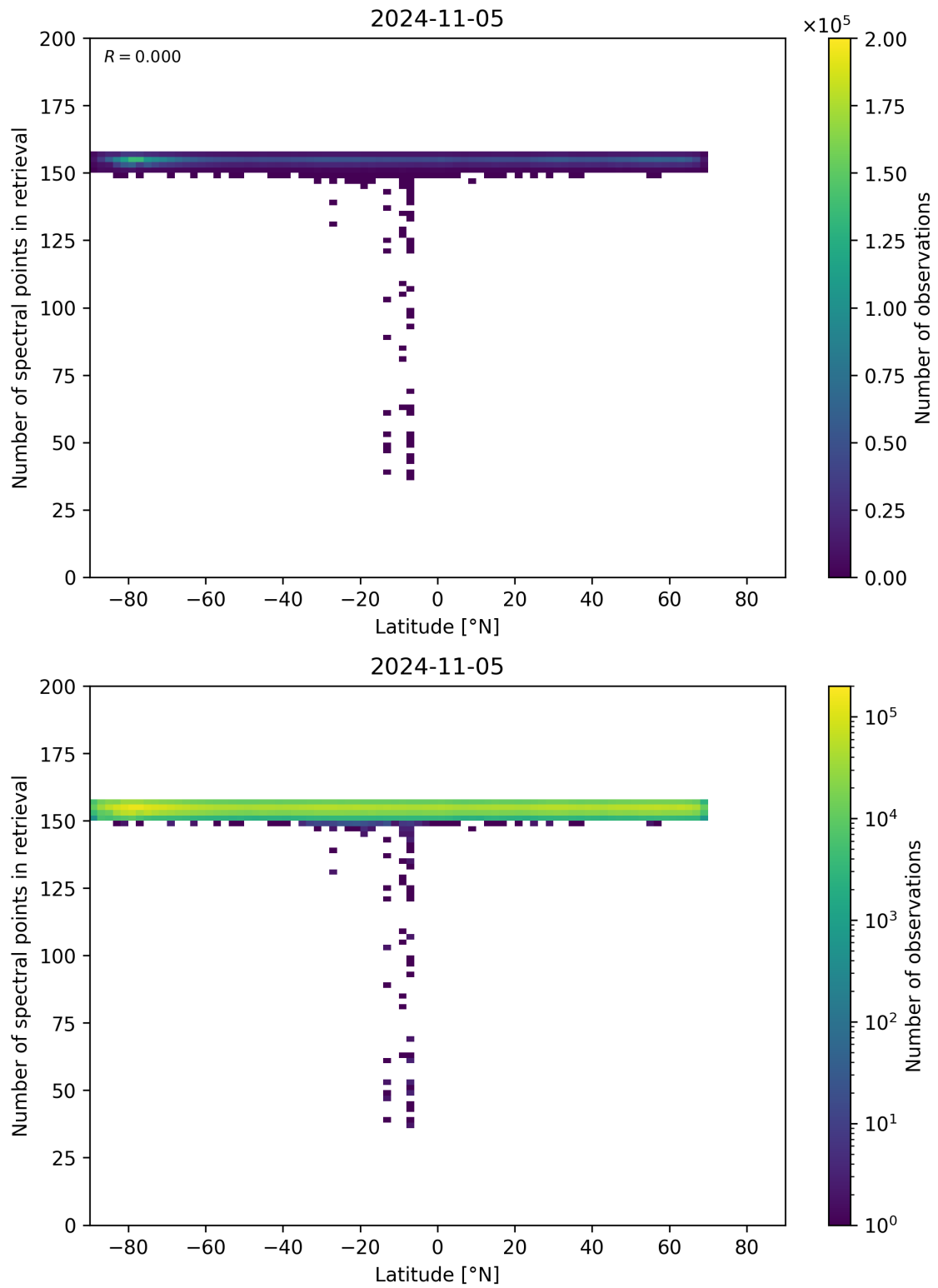
Figure 57: Scatter density plot of “Latitude” against “Number of spectral points in retrieval” for 2024-11-04 to 2024-11-06.
