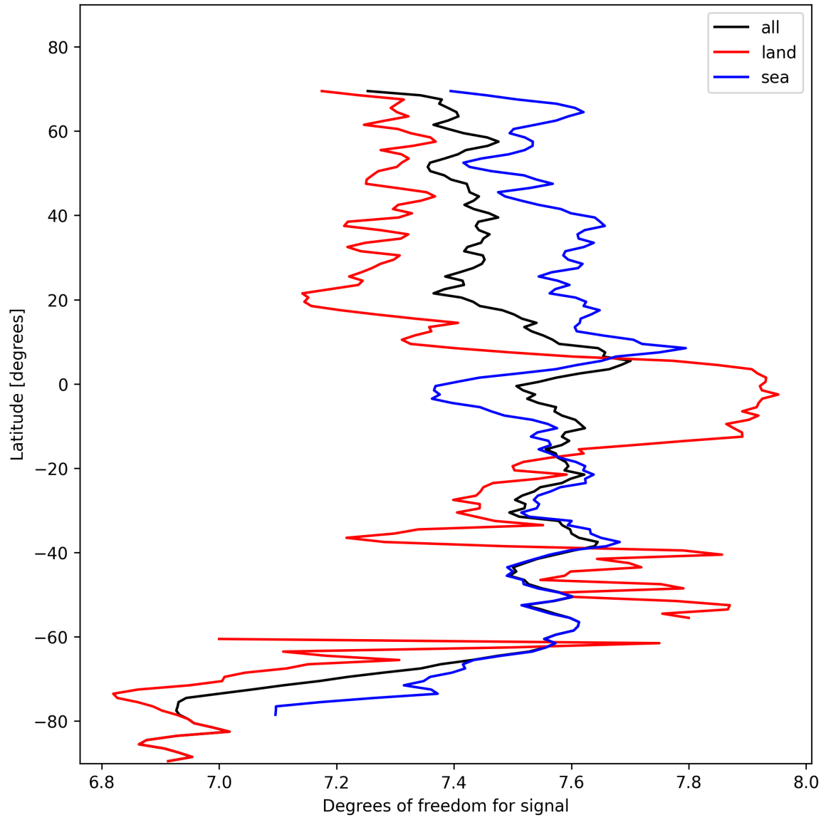
Figure 15: Zonal average of “Degrees of freedom for signal” for 2024-11-04 to 2024-11-06.
