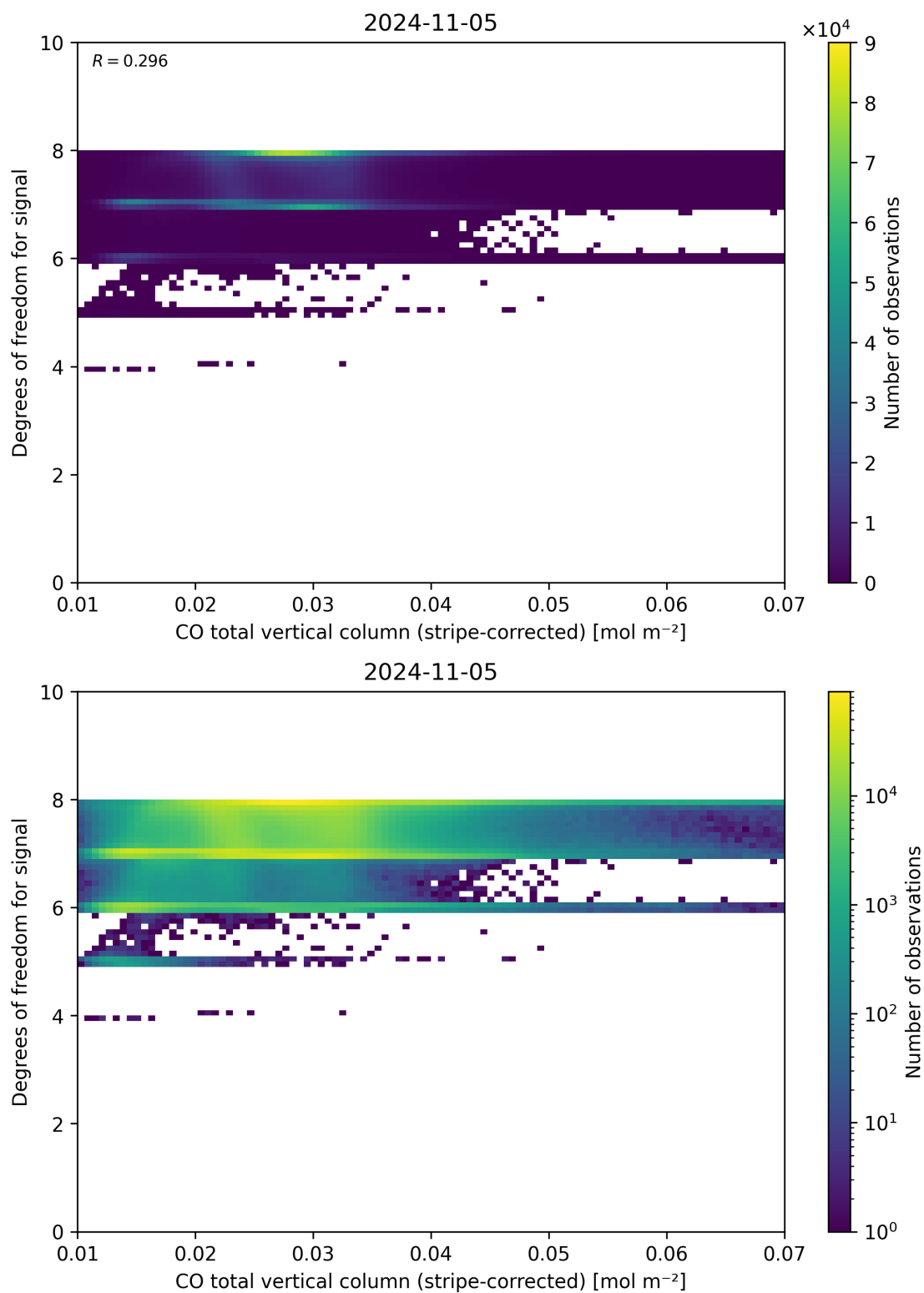
Figure 38: Scatter density plot of “CO total vertical column (stripe-corrected)” against “Degrees of freedom for signal” for 2024-11-04 to 2024-11-06.
