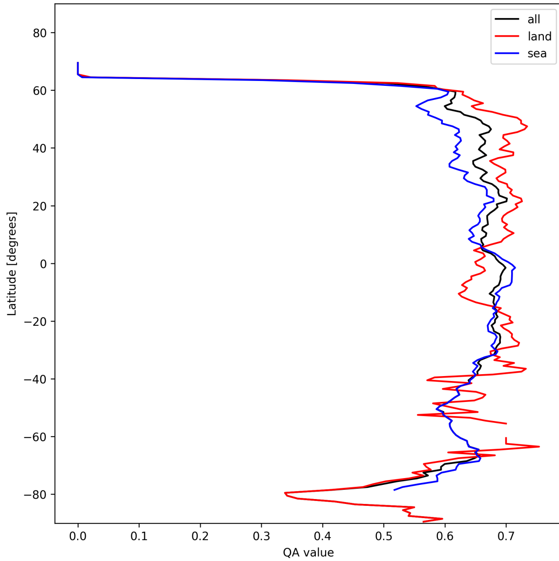
Figure 9: Zonal average of “QA value” for 2024-11-04 to 2024-11-06.
