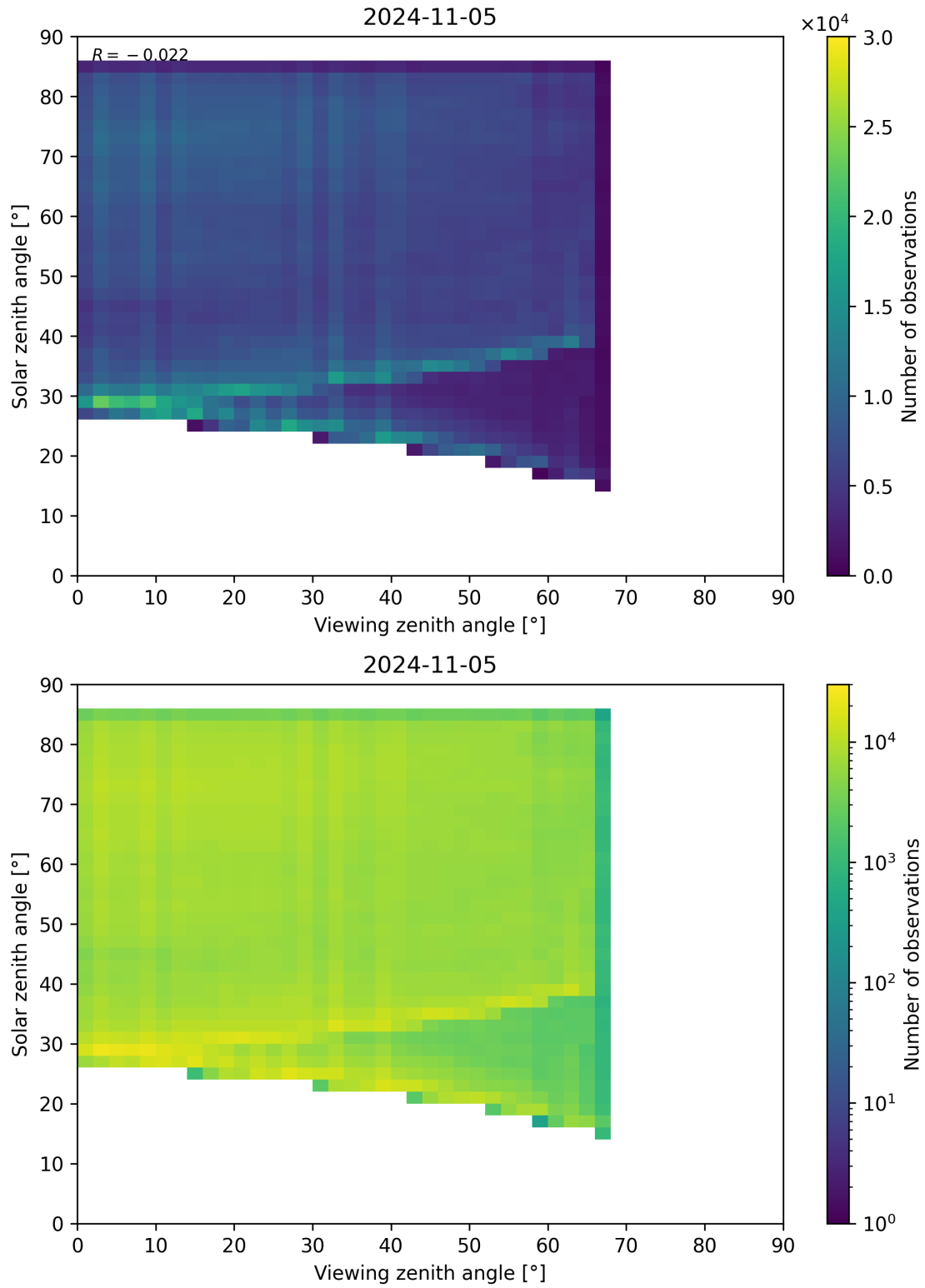
Figure 77: Scatter density plot of “Viewing zenith angle” against “Solar zenith angle” for 2024-11-04 to 2024-11-06.
