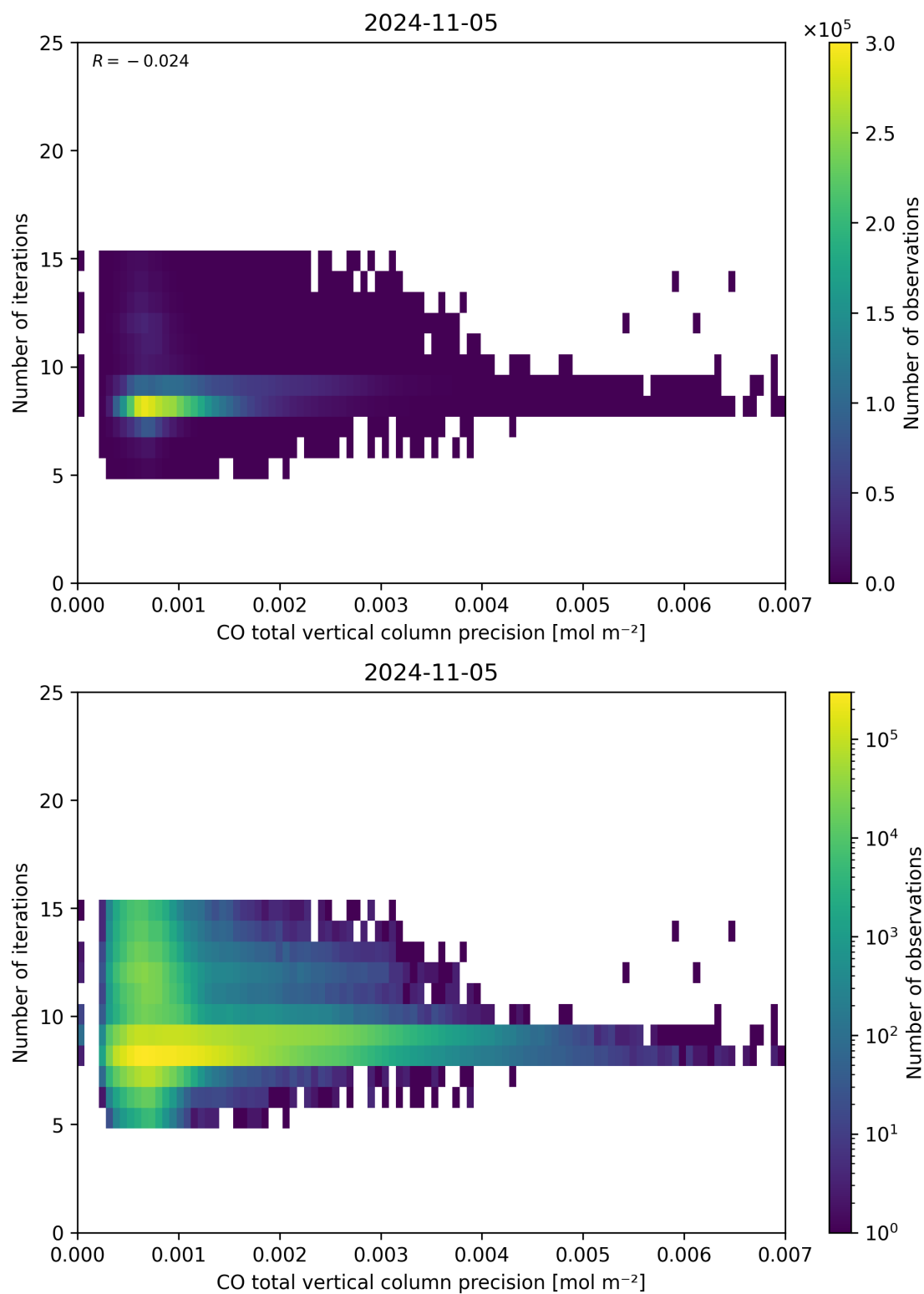
Figure 46: Scatter density plot of “CO total vertical column precision” against “Number of iterations” for 2024-11-04 to 2024-11-06.
