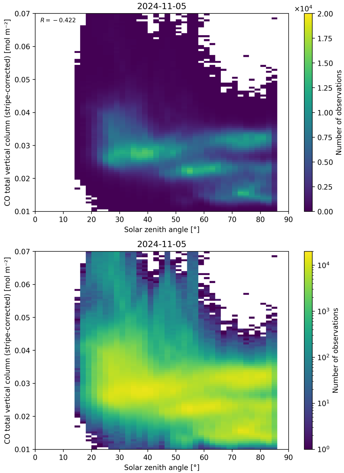
Figure 62: Scatter density plot of “Solar zenith angle” against “CO total vertical column (stripe-corrected)” for 2024-11-04 to 2024-11-06.
