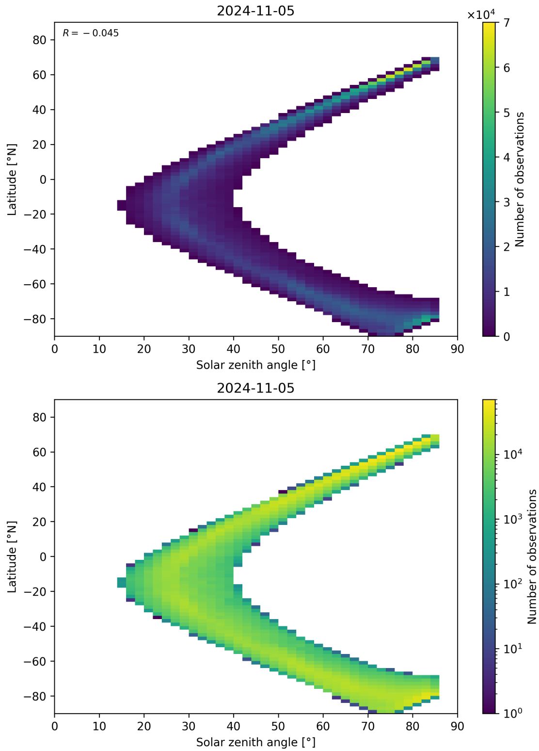
Figure 66: Scatter density plot of “Solar zenith angle” against “Latitude” for 2024-11-04 to 2024-11-06.
