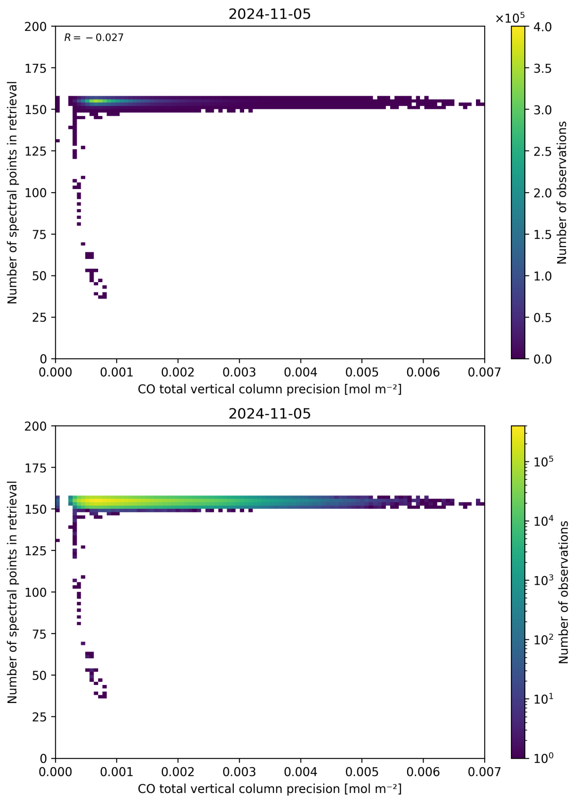
Figure 47: Scatter density plot of “CO total vertical column precision” against “Number of spectral points in retrieval” for 2024-11-04 to 2024-11-06.
