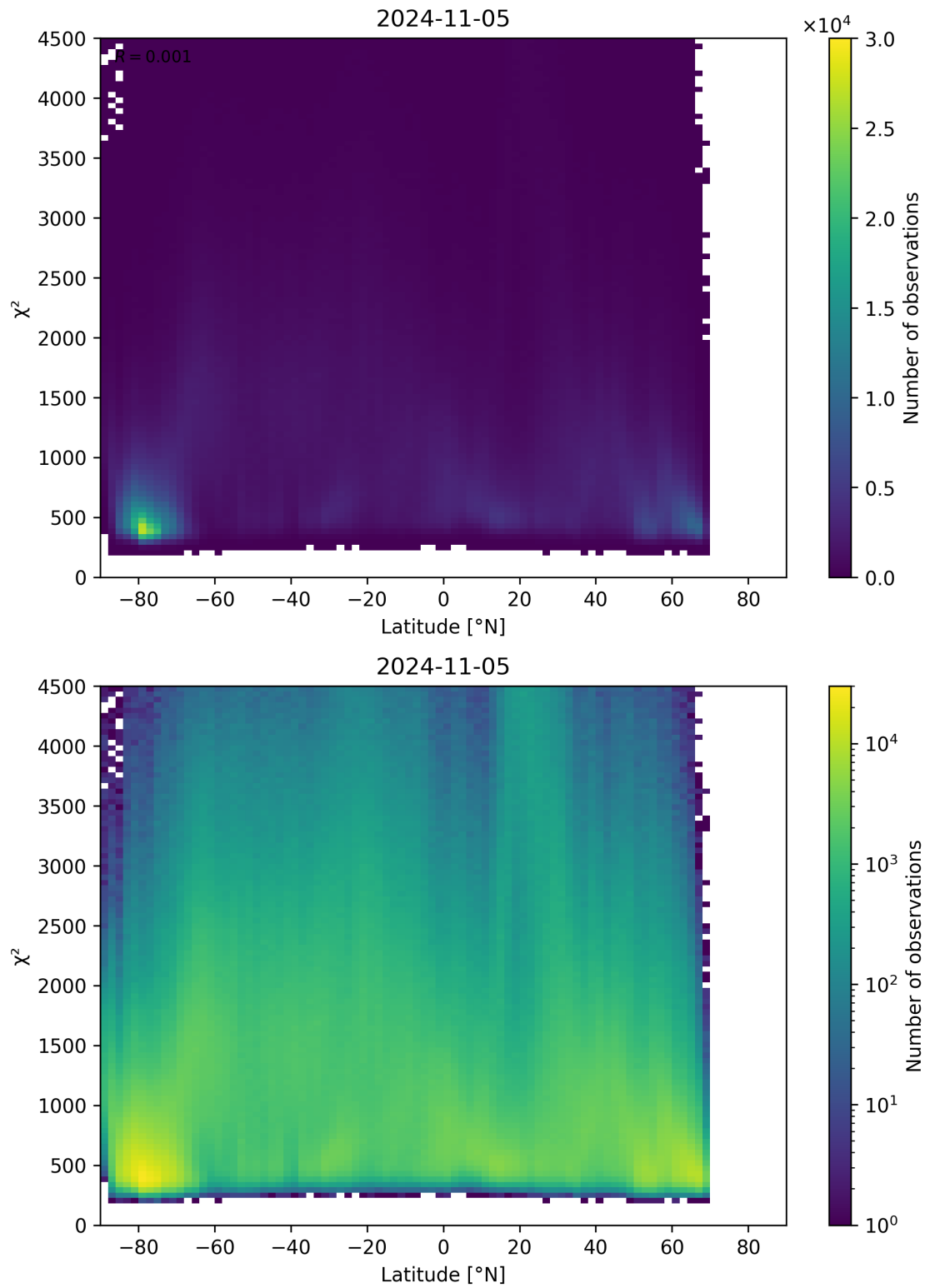
Figure 54: Scatter density plot of “Latitude” against “ \chi^2 ” for 2024-11-04 to 2024-11-06.
