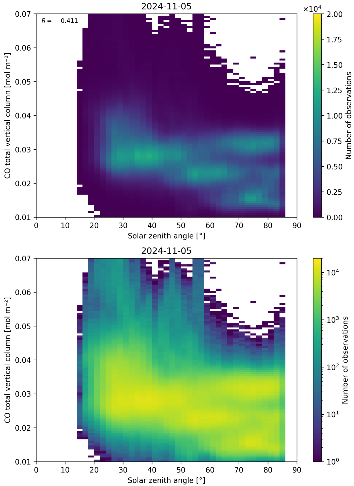
Figure 61: Scatter density plot of “Solar zenith angle” against “CO total vertical column” for 2024-11-04 to 2024-11-06.
