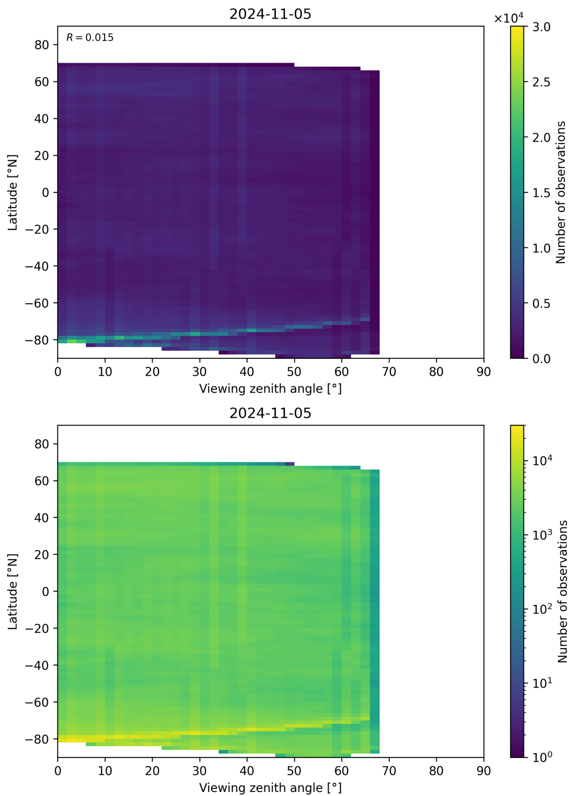
Figure 74: Scatter density plot of “Viewing zenith angle” against “Latitude” for 2024-11-04 to 2024-11-06.
