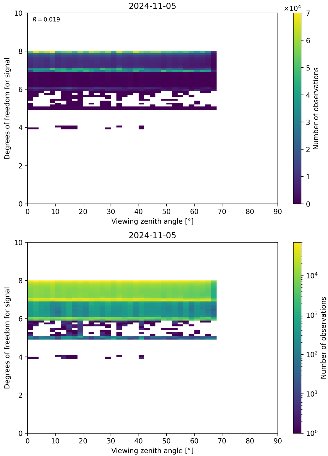
Figure 73: Scatter density plot of “Viewing zenith angle” against “Degrees of freedom for signal” for 2024-11-04 to 2024-11-06.
