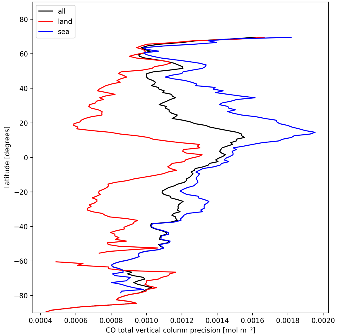
Figure 12: Zonal average of “CO total vertical column precision” for 2024-11-04 to 2024-11-06.
