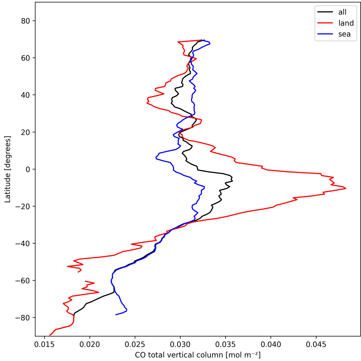
Figure 10: Zonal average of “CO total vertical column” for 2024-11-04 to 2024-11-06.
