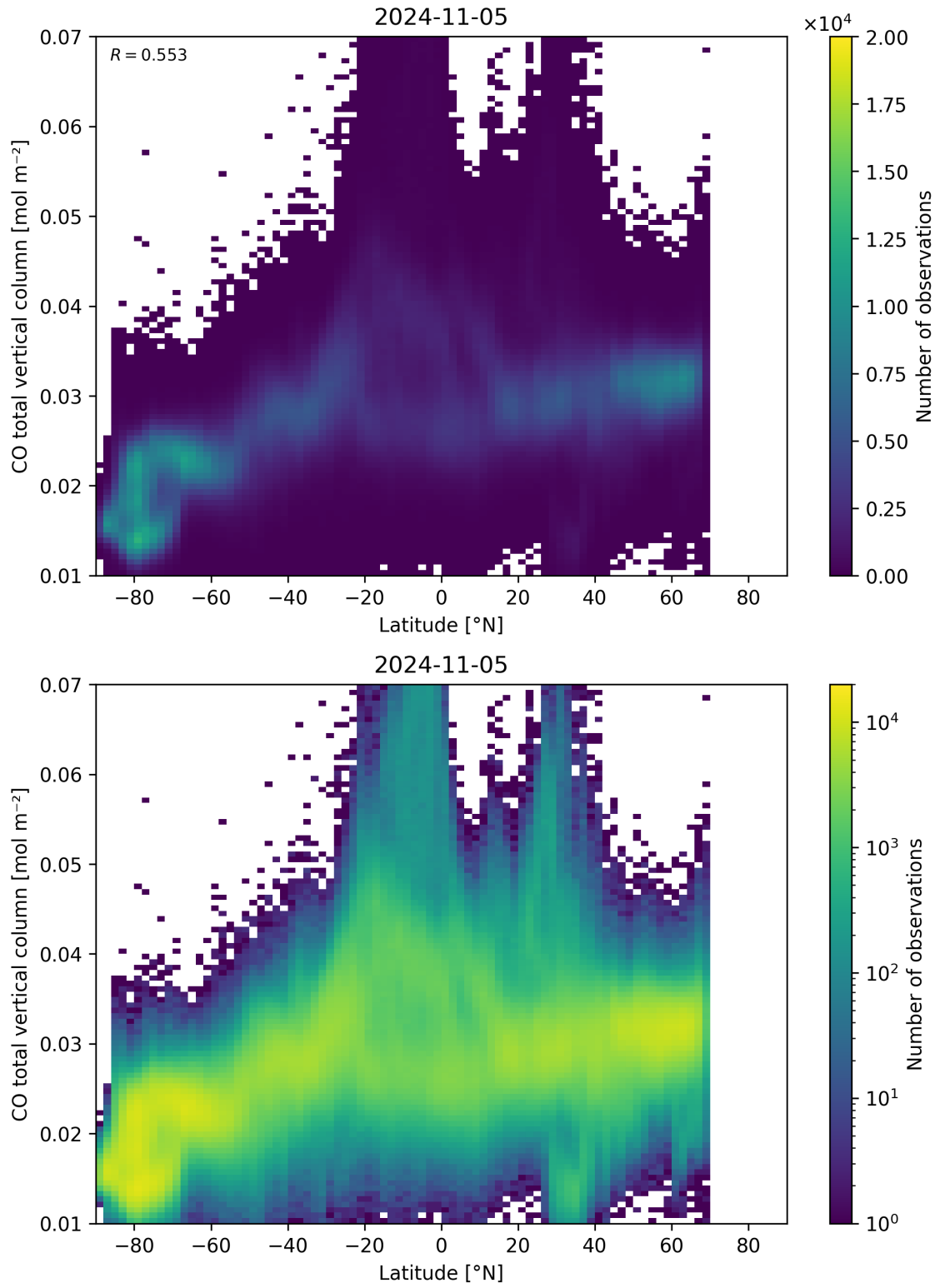
Figure 51: Scatter density plot of “Latitude” against “CO total vertical column” for 2024-11-04 to 2024-11-06.
