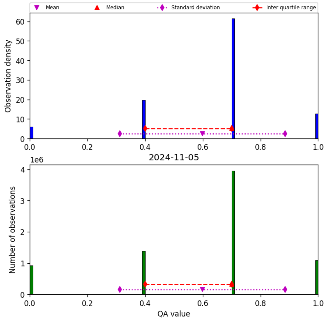
Figure 17: Histogram of “QA value” for 2024-11-04 to 2024-11-06
