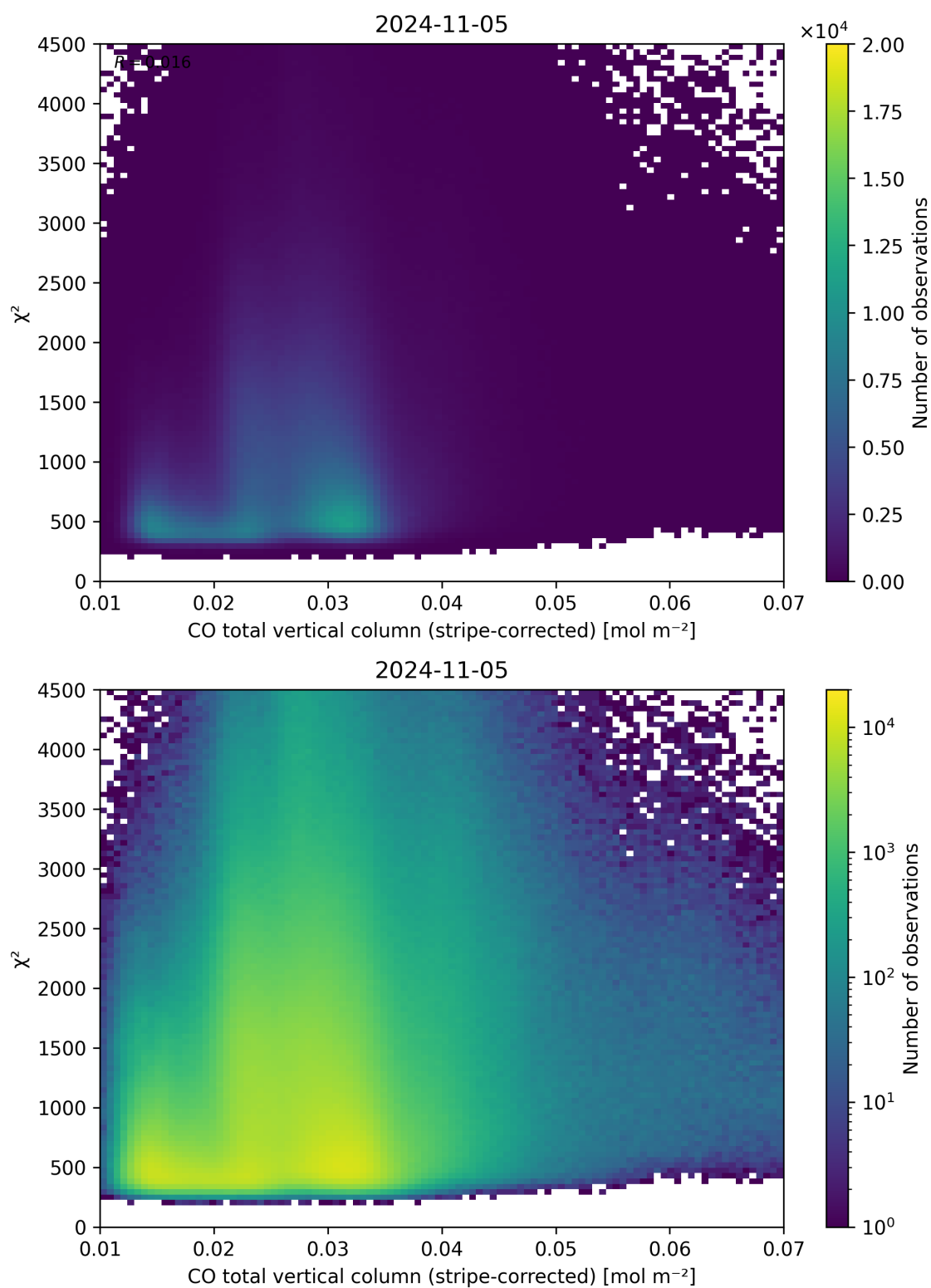
Figure 37: Scatter density plot of “CO total vertical column (stripe-corrected)” against “ \chi^2 ” for 2024-11-04 to 2024-11-06.
