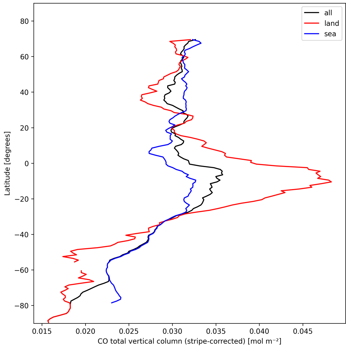
Figure 11: Zonal average of “CO total vertical column (stripe-corrected)” for 2024-11-04 to 2024-11-06.
