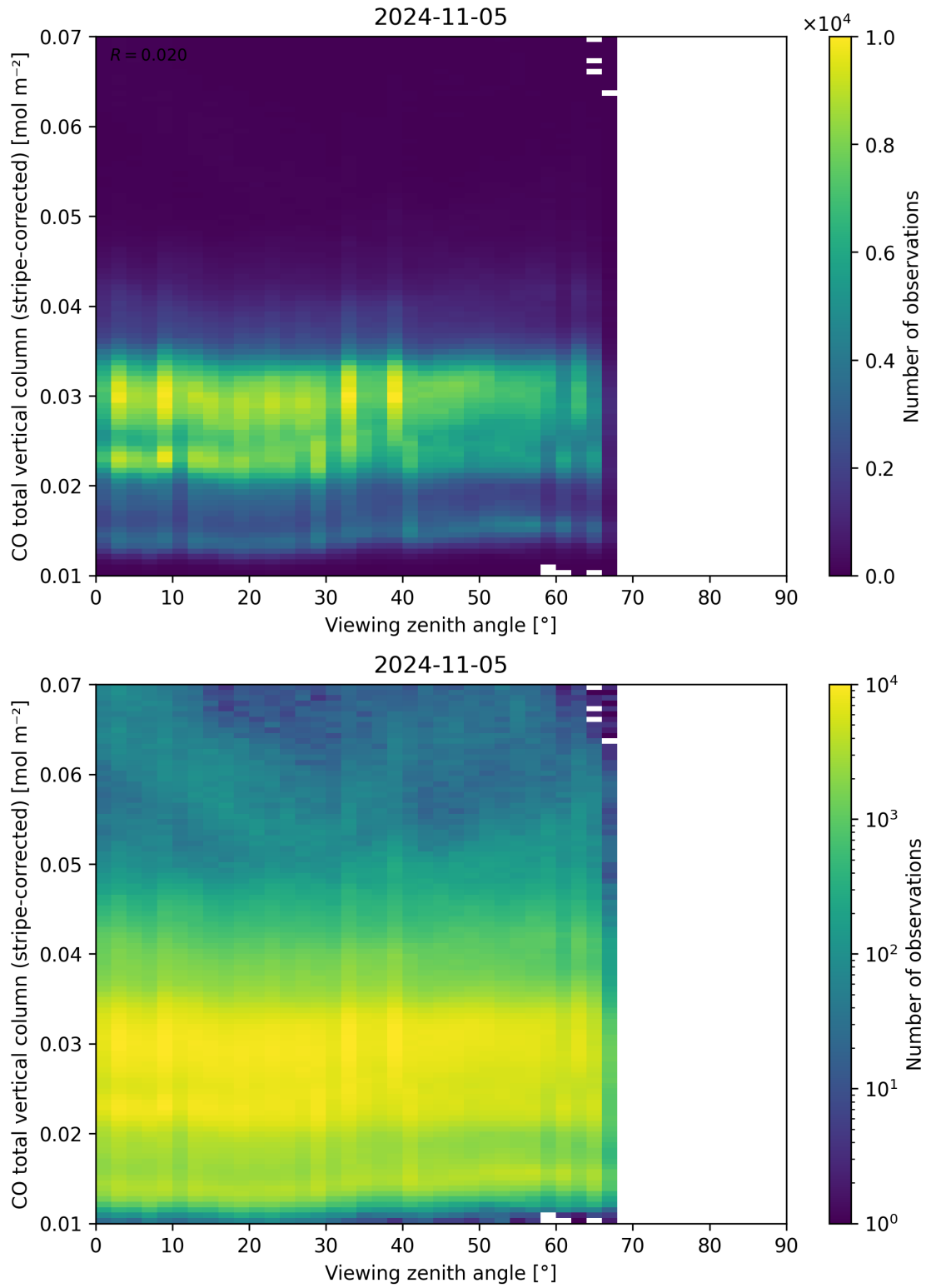
Figure 70: Scatter density plot of “Viewing zenith angle” against “CO total vertical column (stripe-corrected)” for 2024-11-04 to 2024-11-06.
