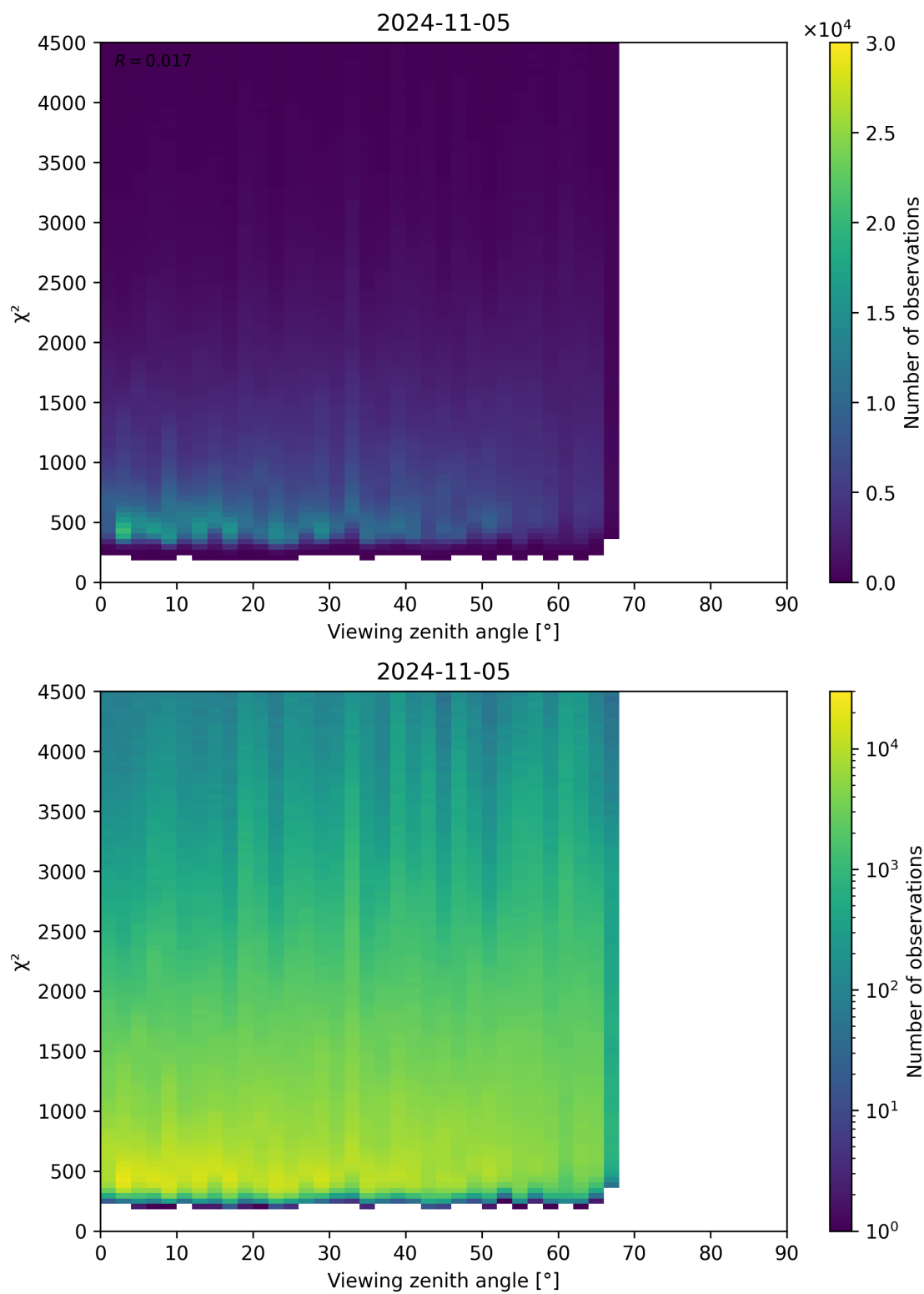
Figure 72: Scatter density plot of “Viewing zenith angle” against “ \chi^2 ” for 2024-11-04 to 2024-11-06.
