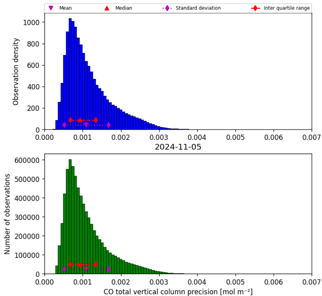
Figure 20: Histogram of “CO total vertical column precision” for 2024-11-04 to 2024-11-06
