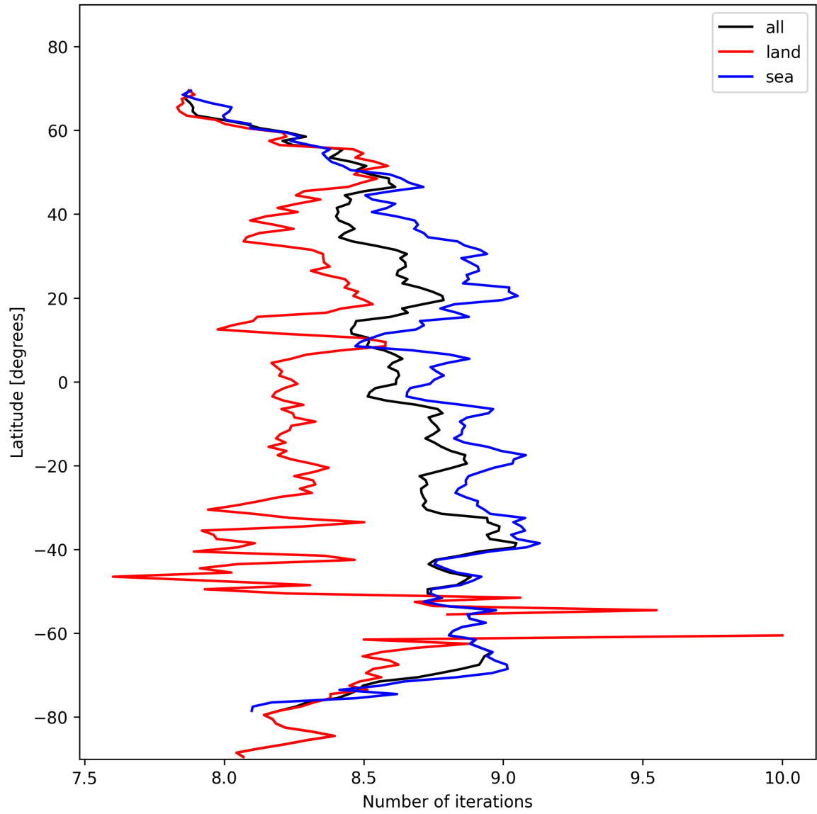
Figure 16: Zonal average of “Number of iterations” for 2024-11-04 to 2024-11-06.
