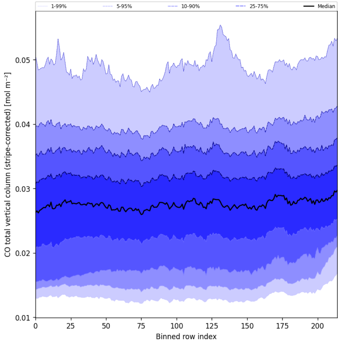
Figure 27: Along track statistics of “CO total vertical column (stripe-corrected)” for 2024-11-04 to 2024-11-06
