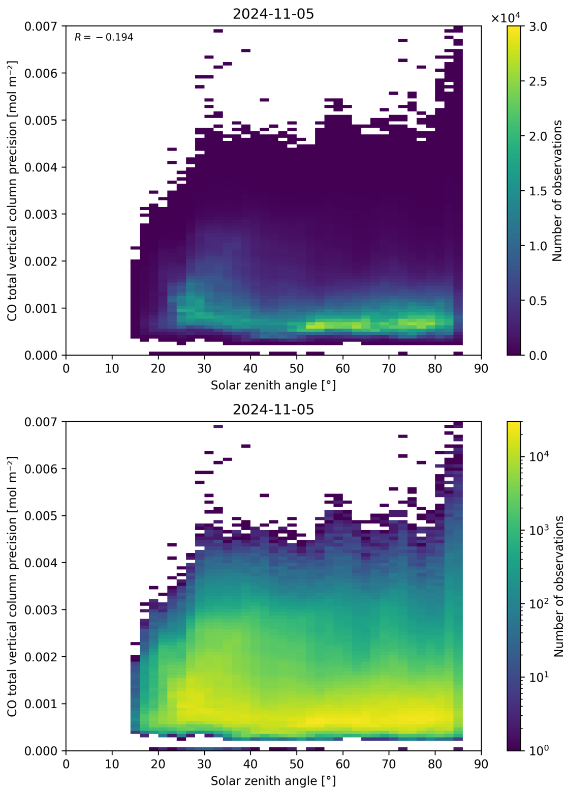
Figure 63: Scatter density plot of “Solar zenith angle” against “CO total vertical column precision” for 2024-11-04 to 2024-11-06.
