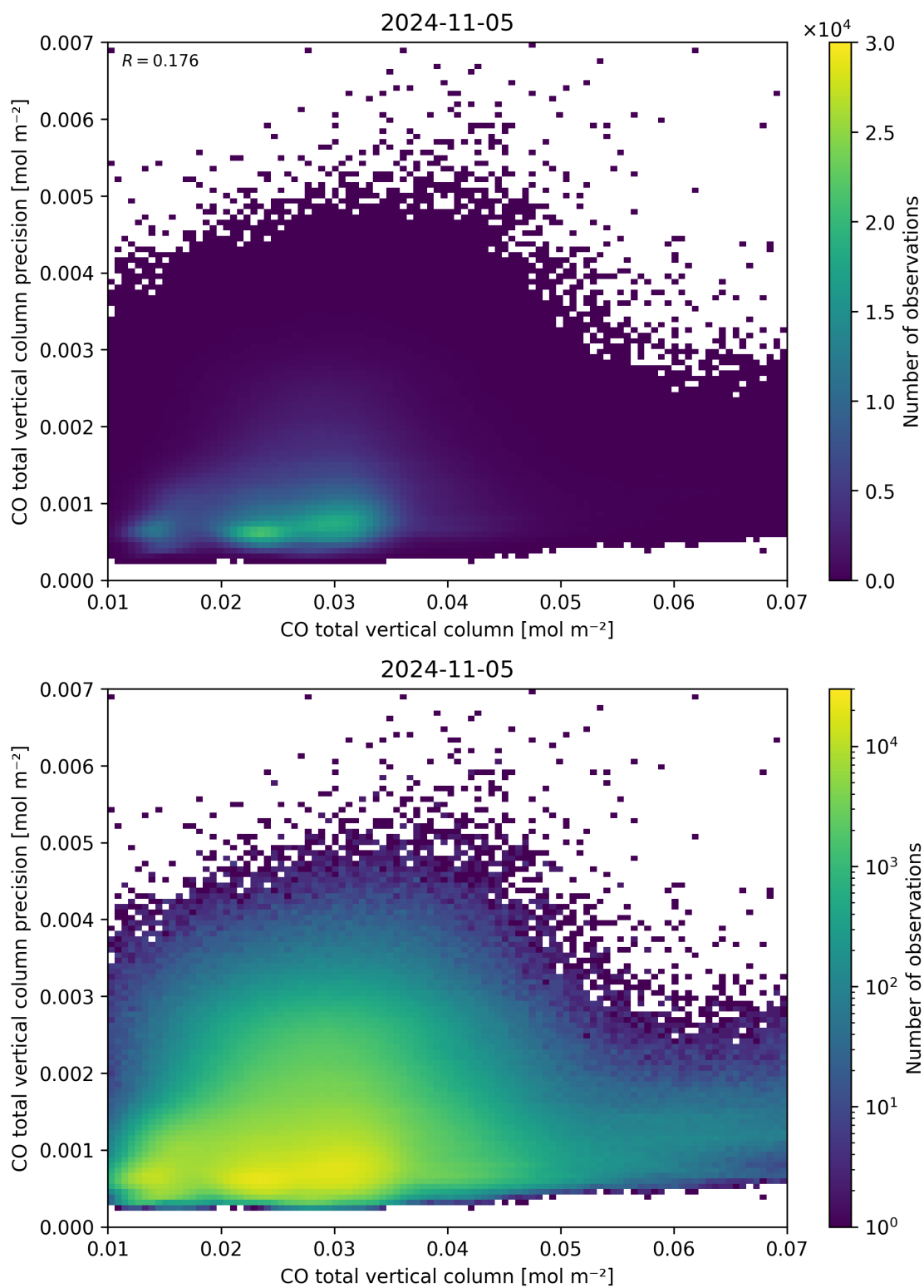
Figure 34: Scatter density plot of “CO total vertical column” against “CO total vertical column precision” for 2024-11-04 to 2024-11-06.
