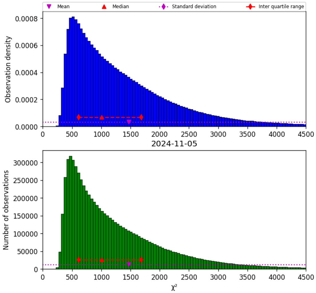
Figure 22: Histogram of “ \chi^2 ” for 2024-11-04 to 2024-11-06
