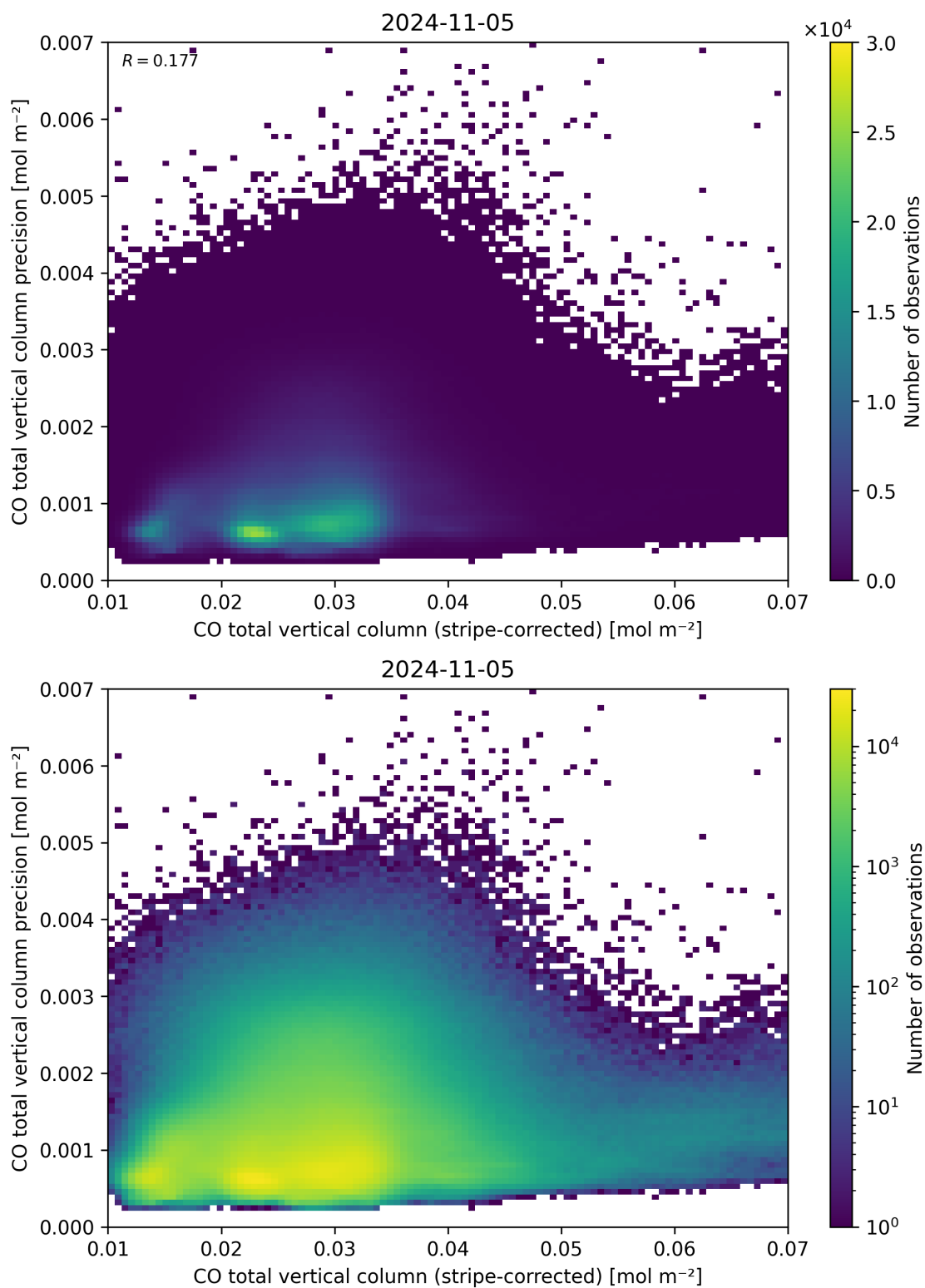
Figure 36: Scatter density plot of “CO total vertical column (stripe-corrected)” against “CO total vertical column precision” for 2024-11-04 to 2024-11-06.
