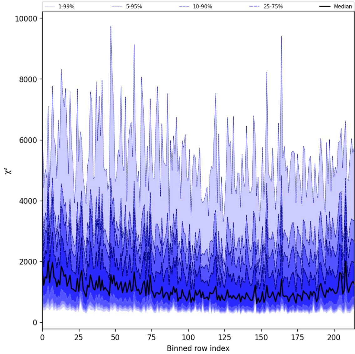
Figure 30: Along track statistics of “ \chi^2 ” for 2024-11-05 to 2024-11-07
