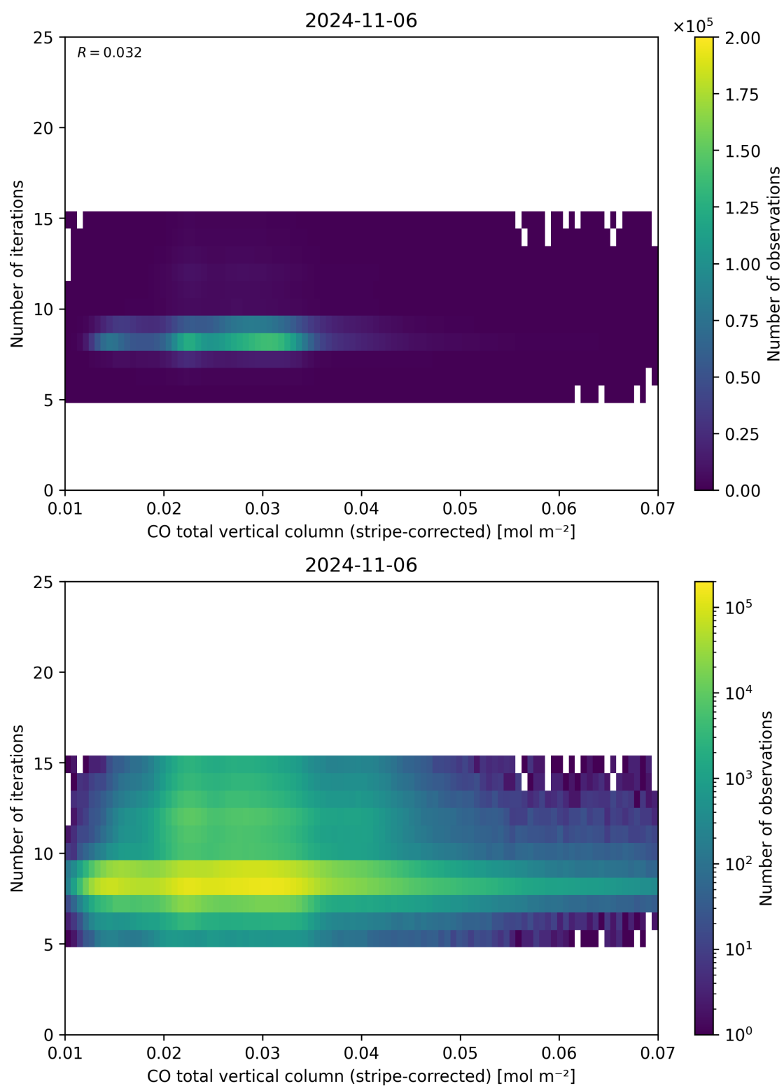
Figure 39: Scatter density plot of “CO total vertical column (stripe-corrected)” against “Number of iterations” for 2024-11-05 to 2024-11-07.
