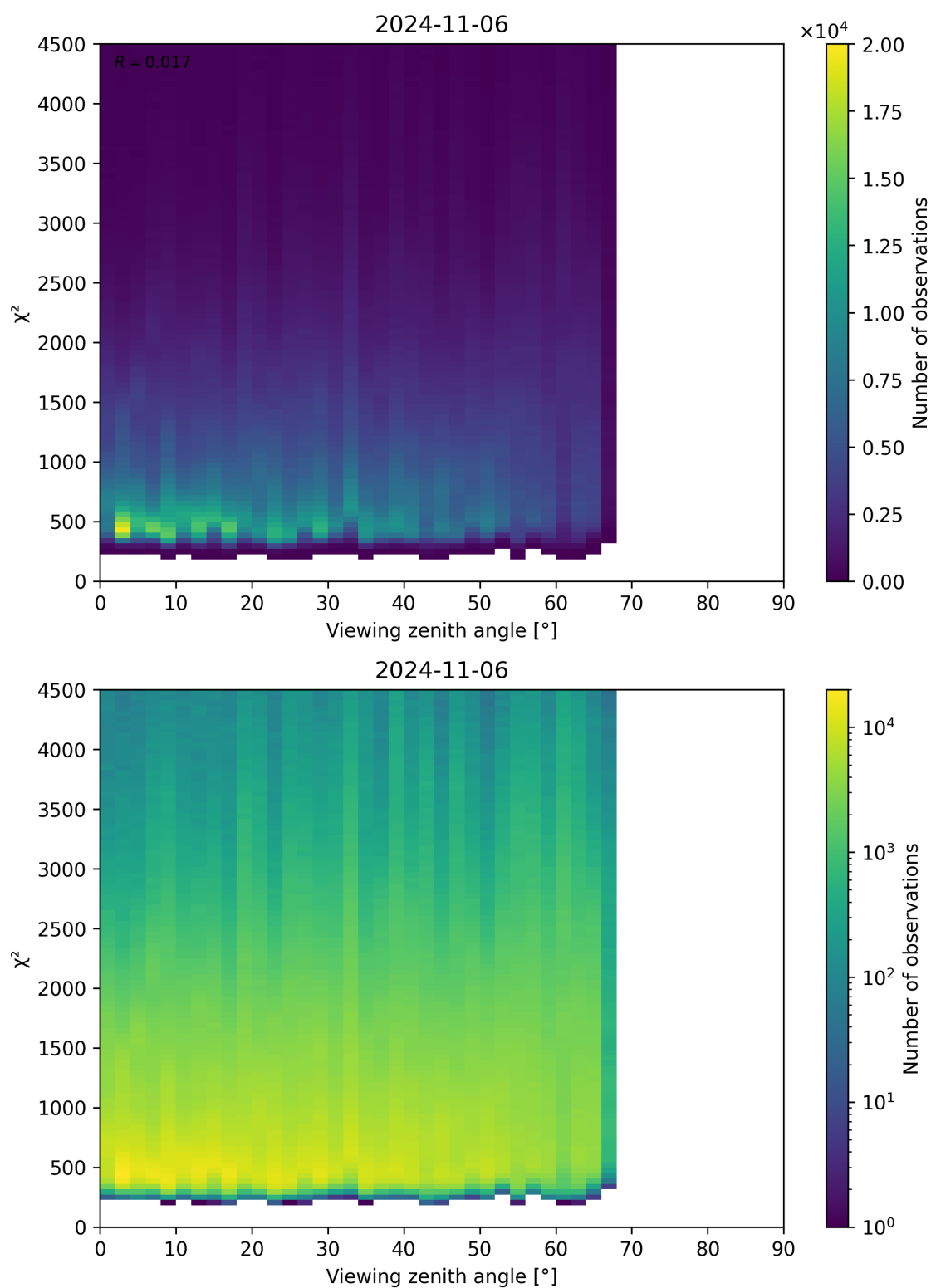
Figure 72: Scatter density plot of “Viewing zenith angle” against “ \chi^2 ” for 2024-11-05 to 2024-11-07.
