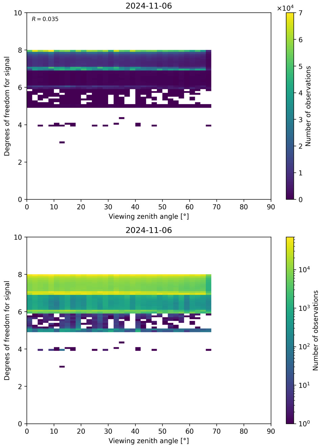
Figure 73: Scatter density plot of “Viewing zenith angle” against “Degrees of freedom for signal” for 2024-11-05 to 2024-11-07.
