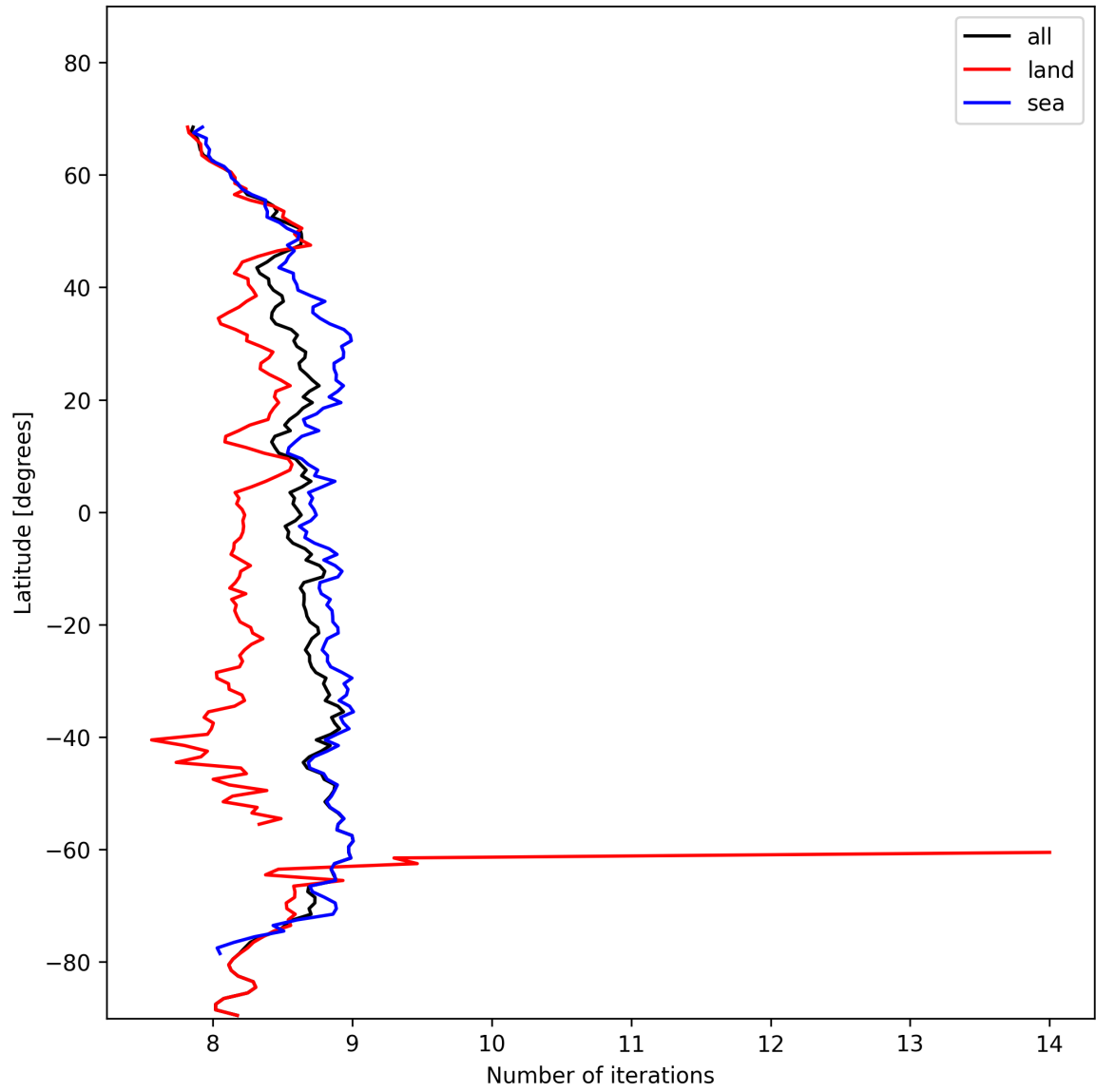
Figure 16: Zonal average of “Number of iterations” for 2024-11-05 to 2024-11-07.
