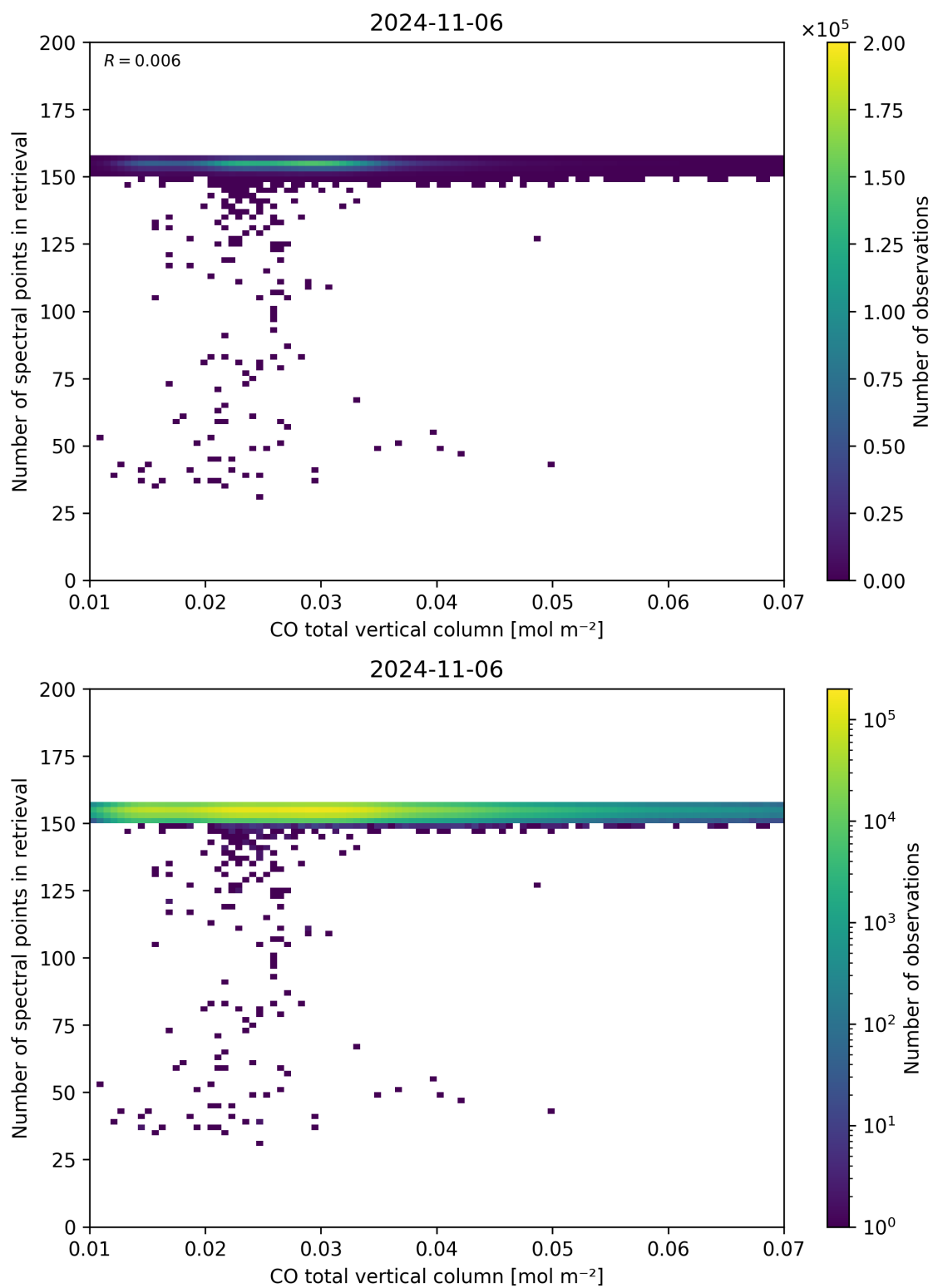
Figure 43: Scatter density plot of “CO total vertical column” against “Number of spectral points in retrieval” for 2024-11-05 to 2024-11-07.
