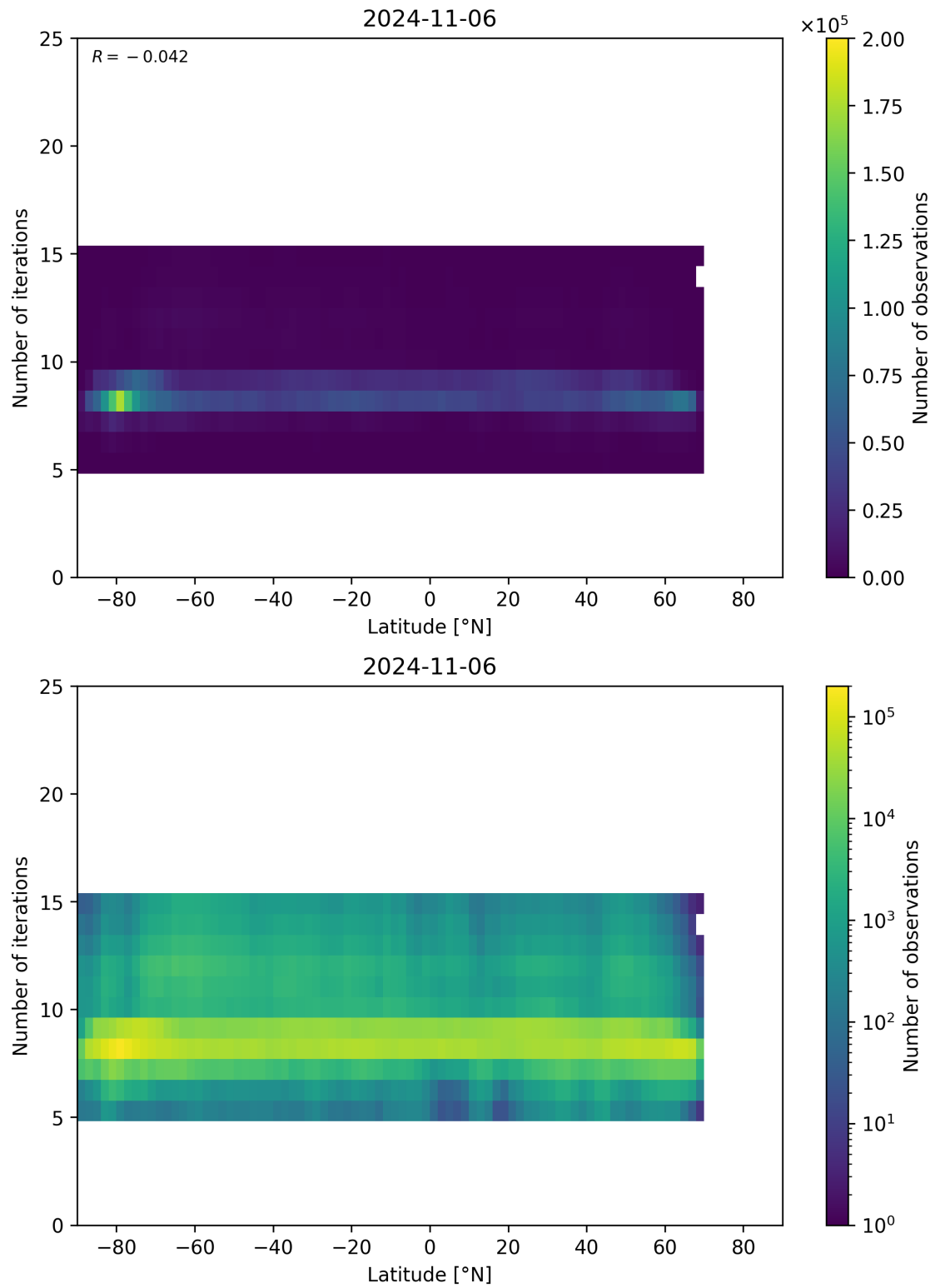
Figure 56: Scatter density plot of “Latitude” against “Number of iterations” for 2024-11-05 to 2024-11-07.
