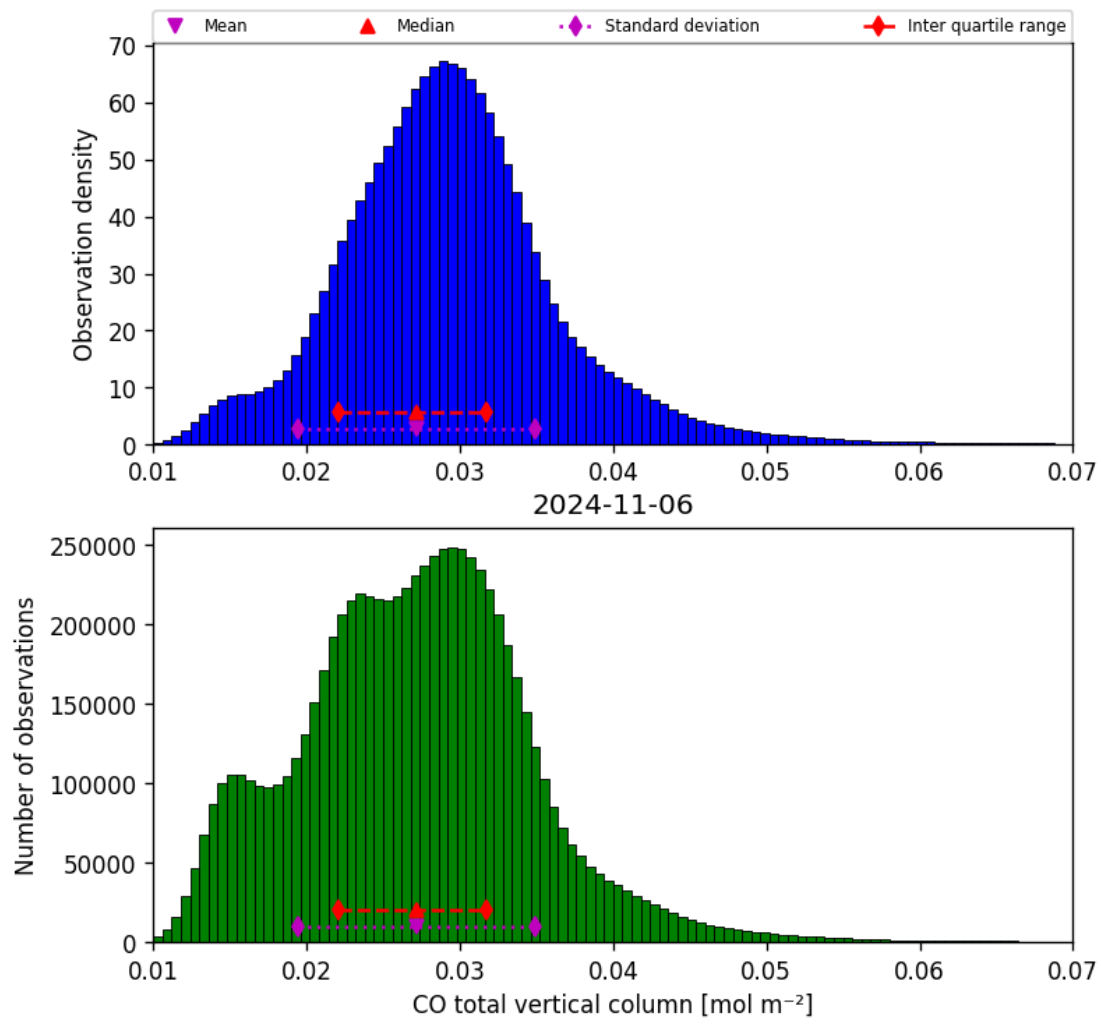
Figure 18: Histogram of “CO total vertical column” for 2024-11-05 to 2024-11-07
