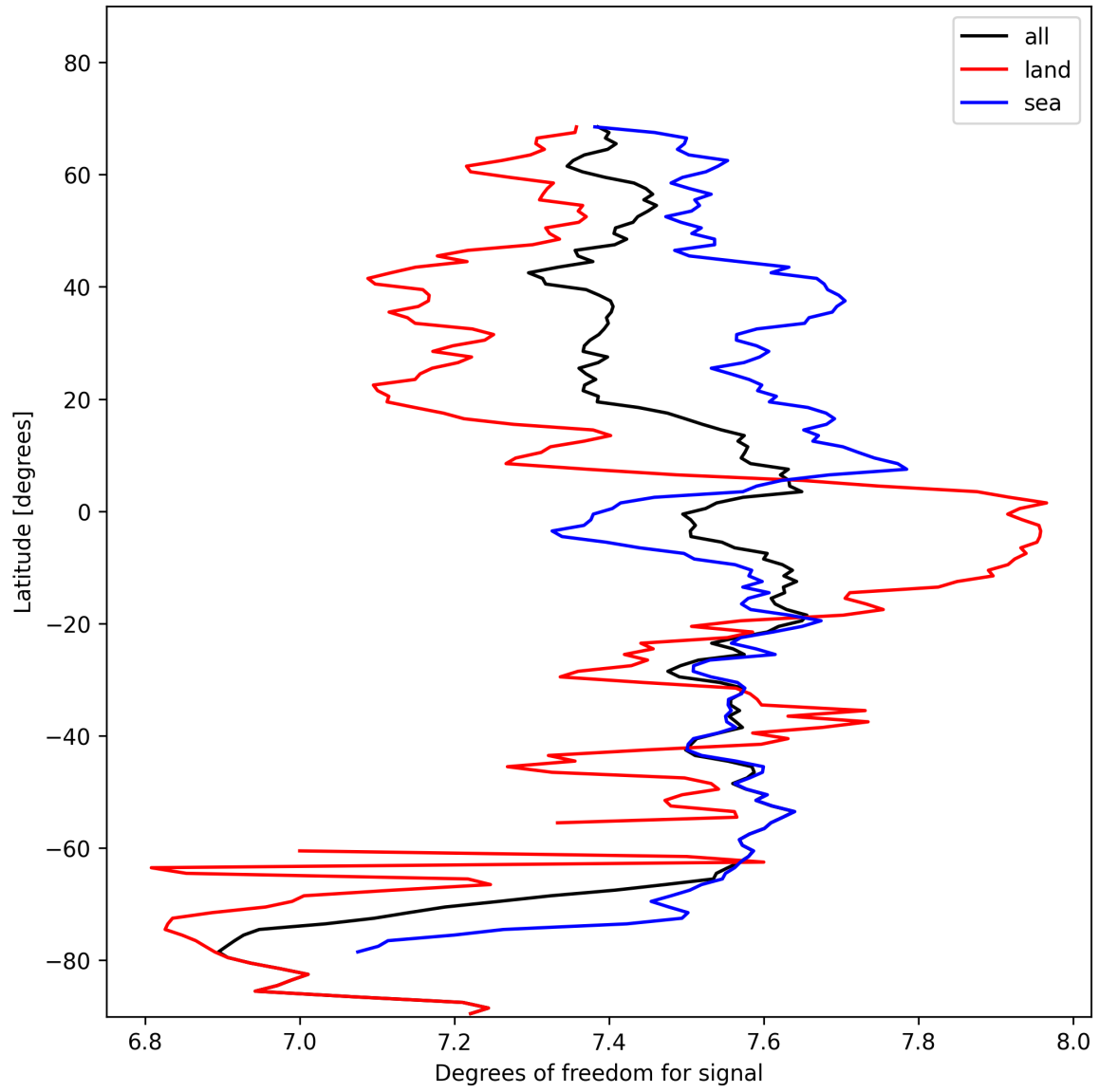
Figure 15: Zonal average of “Degrees of freedom for signal” for 2024-11-05 to 2024-11-07.
