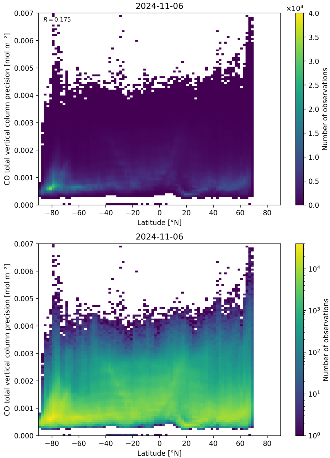
Figure 53: Scatter density plot of “Latitude” against “CO total vertical column precision” for 2024-11-05 to 2024-11-07.
