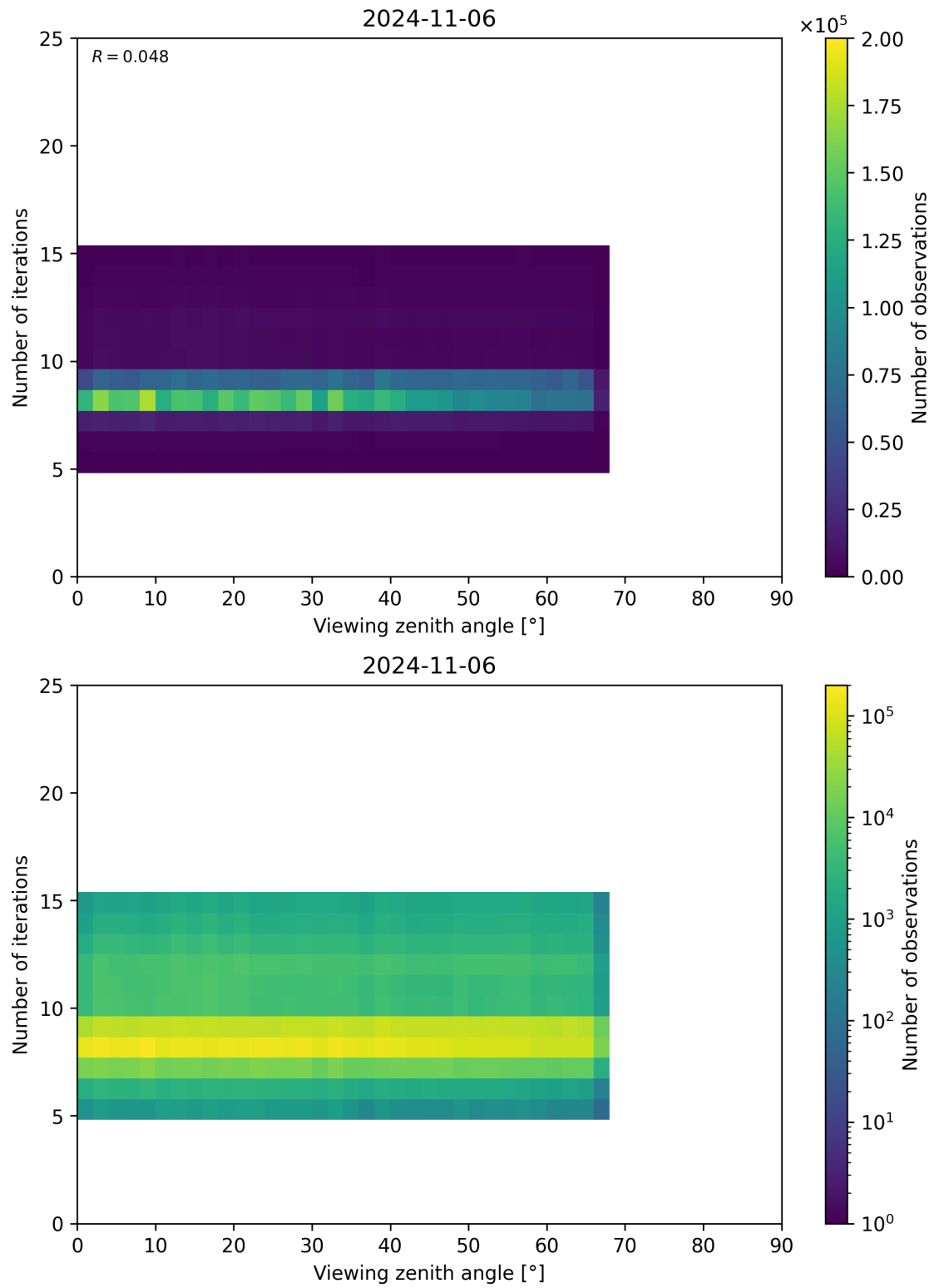
Figure 75: Scatter density plot of “Viewing zenith angle” against “Number of iterations” for 2024-11-05 to 2024-11-07.
