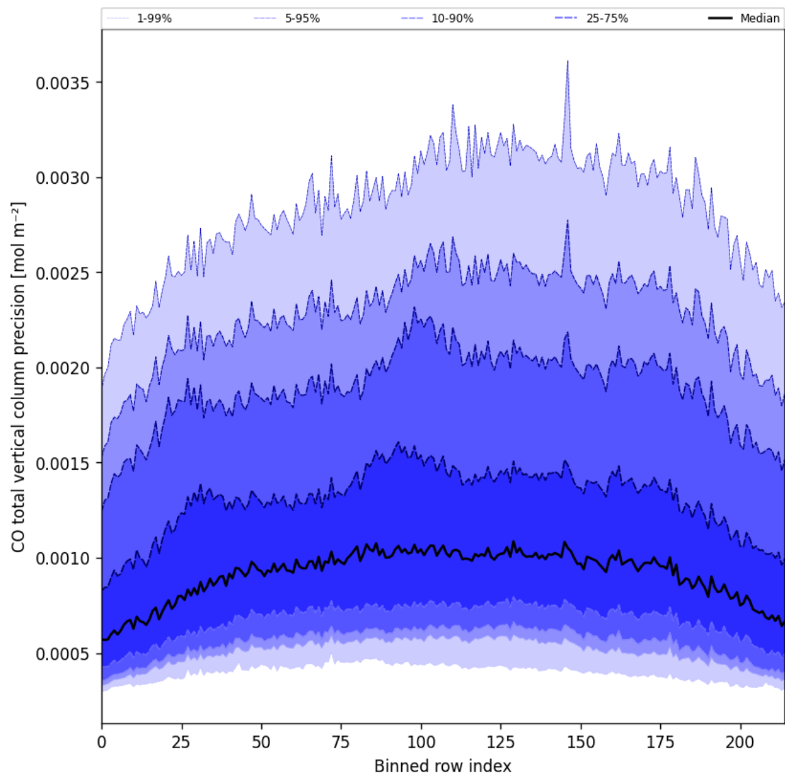
Figure 28: Along track statistics of “CO total vertical column precision” for 2024-11-05 to 2024-11-07
