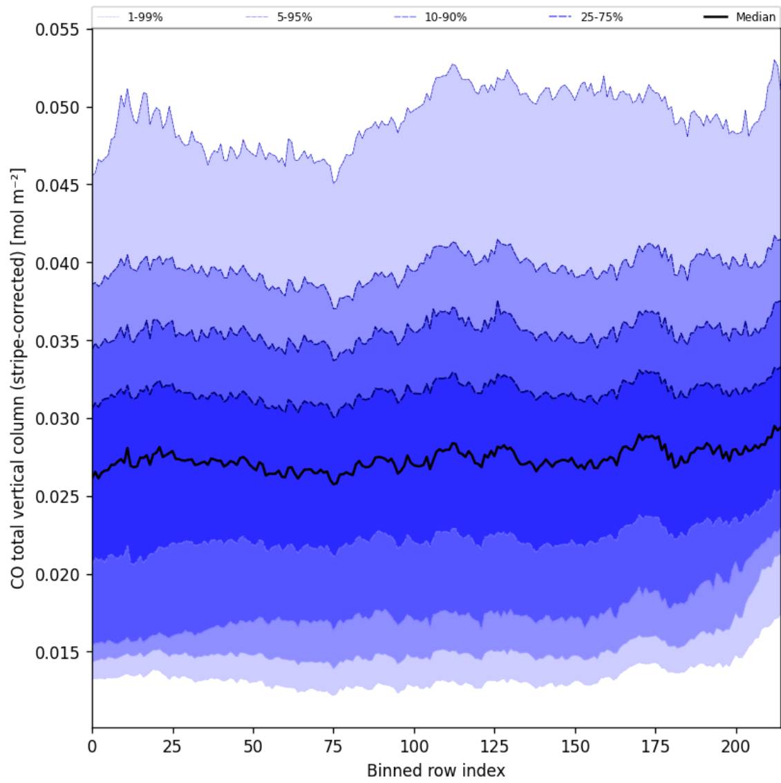
Figure 27: Along track statistics of "CO total vertical column (stripe-corrected)" for 2024-11-05 to 2024-11-07
