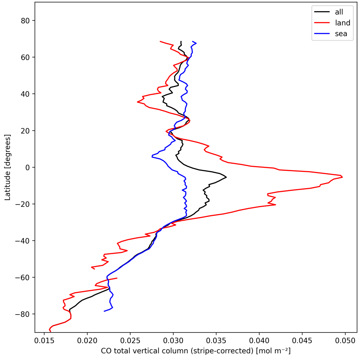
Figure 11: Zonal average of “CO total vertical column (stripe-corrected)” for 2024-11-05 to 2024-11-07.
