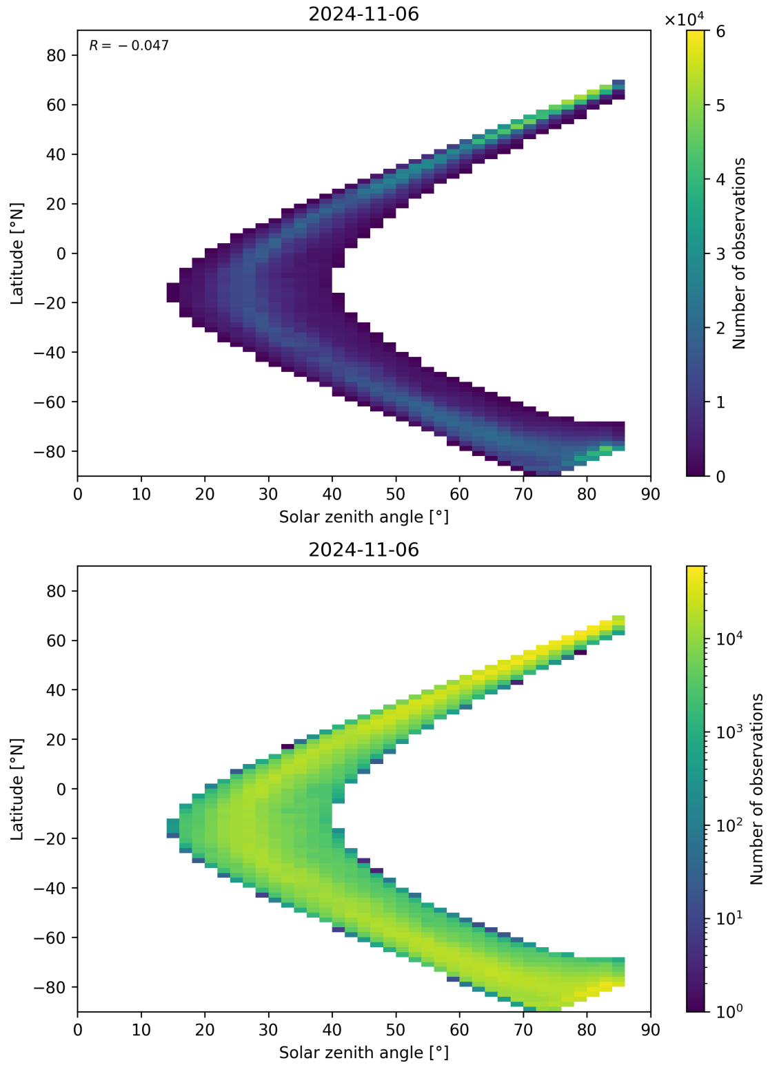
Figure 66: Scatter density plot of “Solar zenith angle” against “Latitude” for 2024-11-05 to 2024-11-07.
