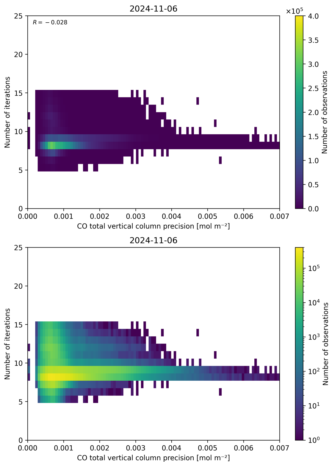
Figure 46: Scatter density plot of “CO total vertical column precision” against “Number of iterations” for 2024-11-05 to 2024-11-07.
