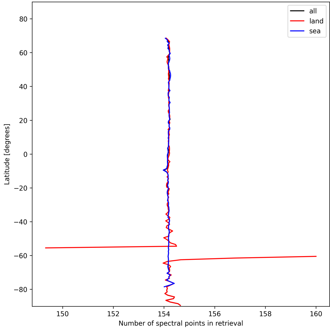
Figure 13: Zonal average of “Number of spectral points in retrieval” for 2024-11-05 to 2024-11-07.
