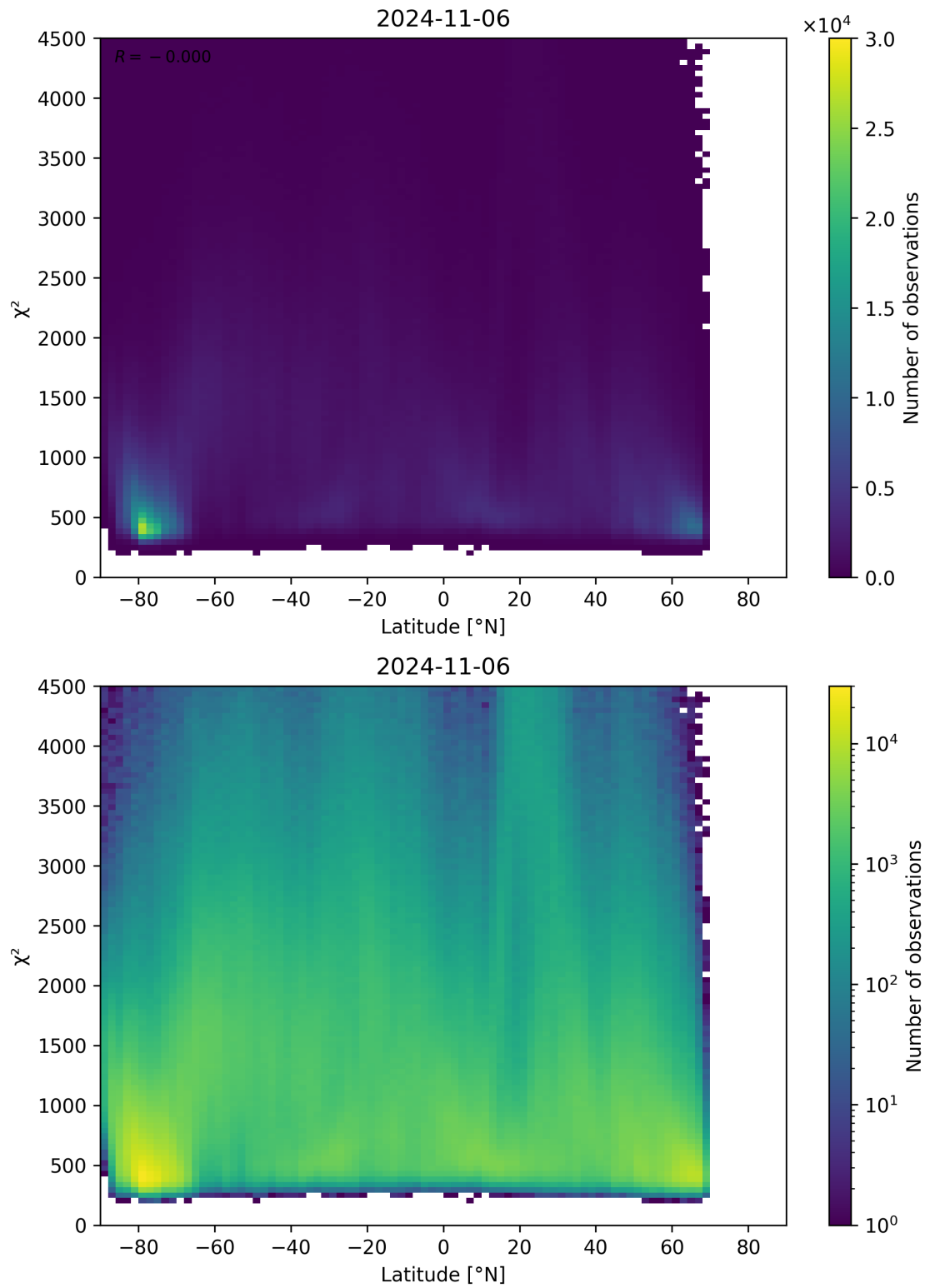
Figure 54: Scatter density plot of “Latitude” against “ \chi^2 ” for 2024-11-05 to 2024-11-07.
