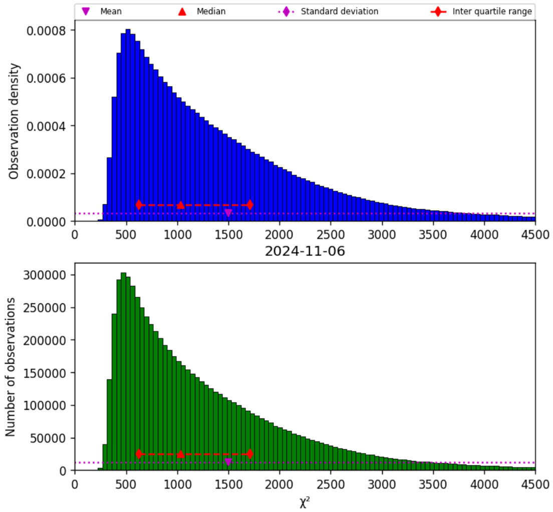
Figure 22: Histogram of “ \chi^2 ” for 2024-11-05 to 2024-11-07
