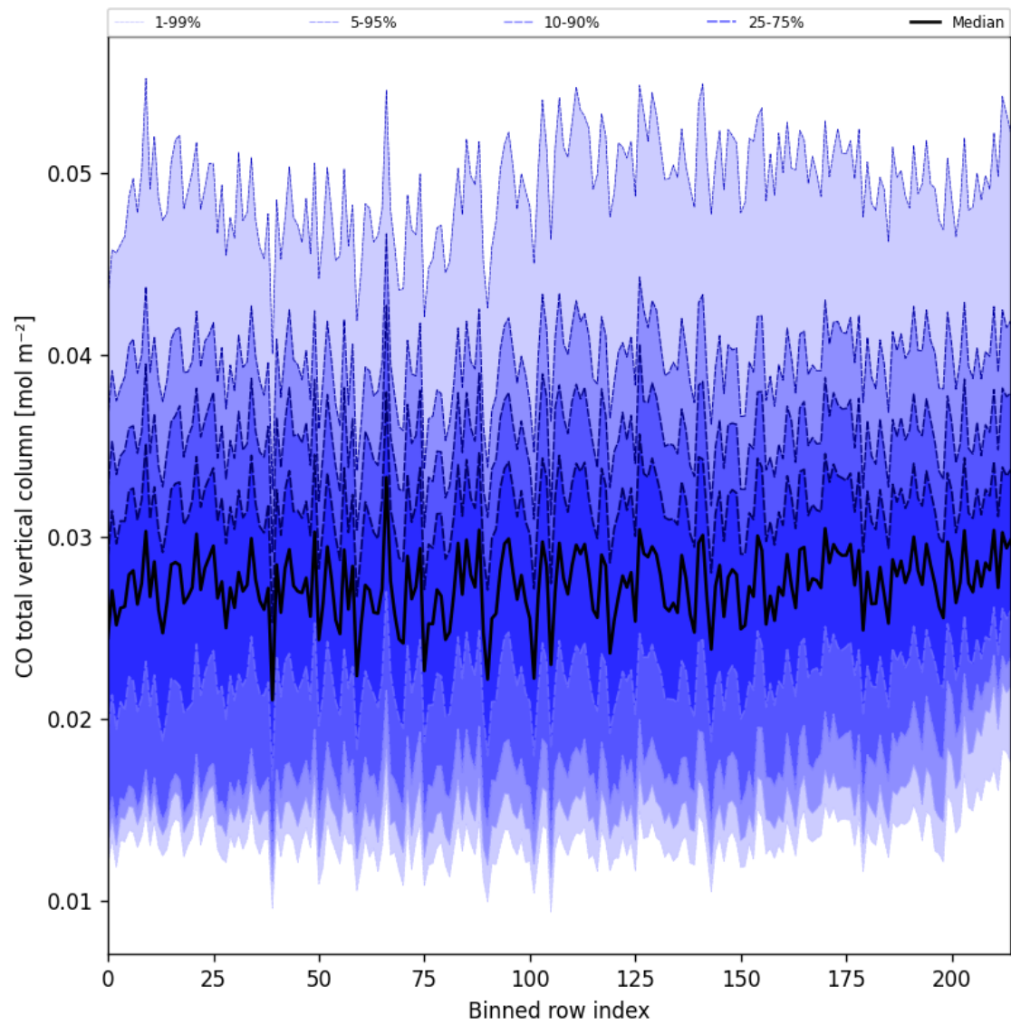
Figure 26: Along track statistics of “CO total vertical column” for 2024-11-05 to 2024-11-07
