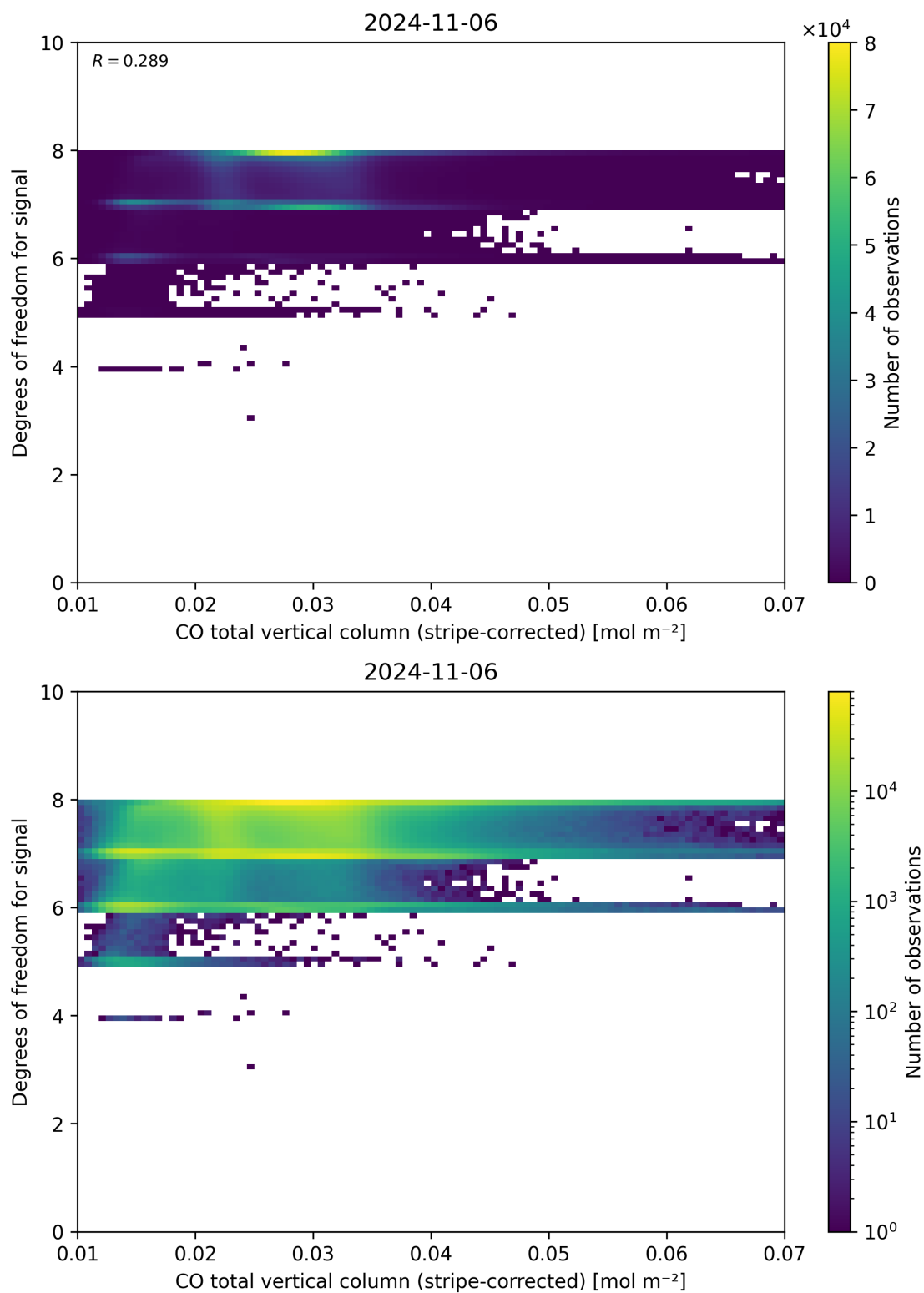
Figure 38: Scatter density plot of “CO total vertical column (stripe-corrected)” against “Degrees of freedom for signal” for 2024-11-05 to 2024-11-07.
