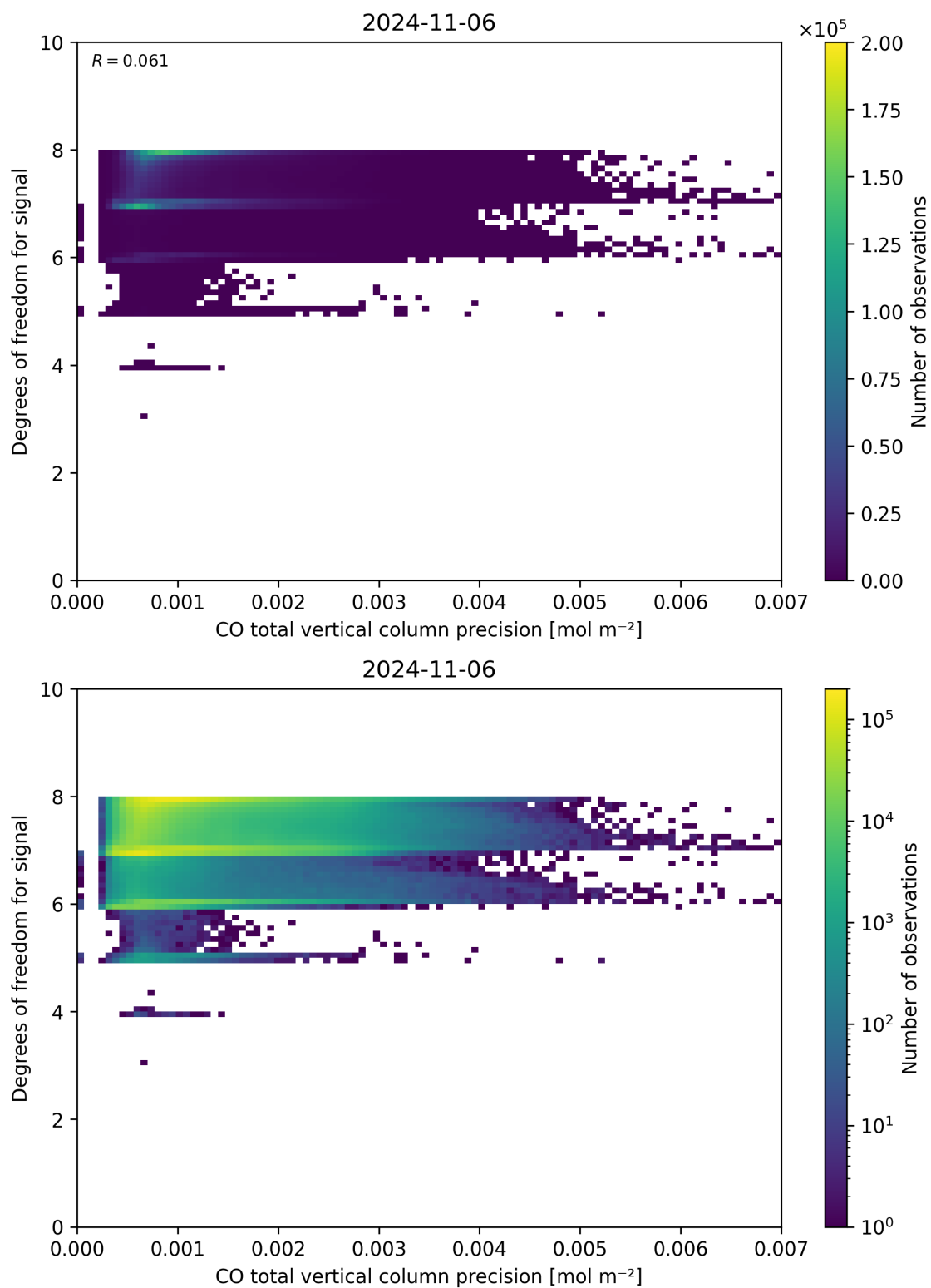
Figure 45: Scatter density plot of “CO total vertical column precision” against “Degrees of freedom for signal” for 2024-11-05 to 2024-11-07.
