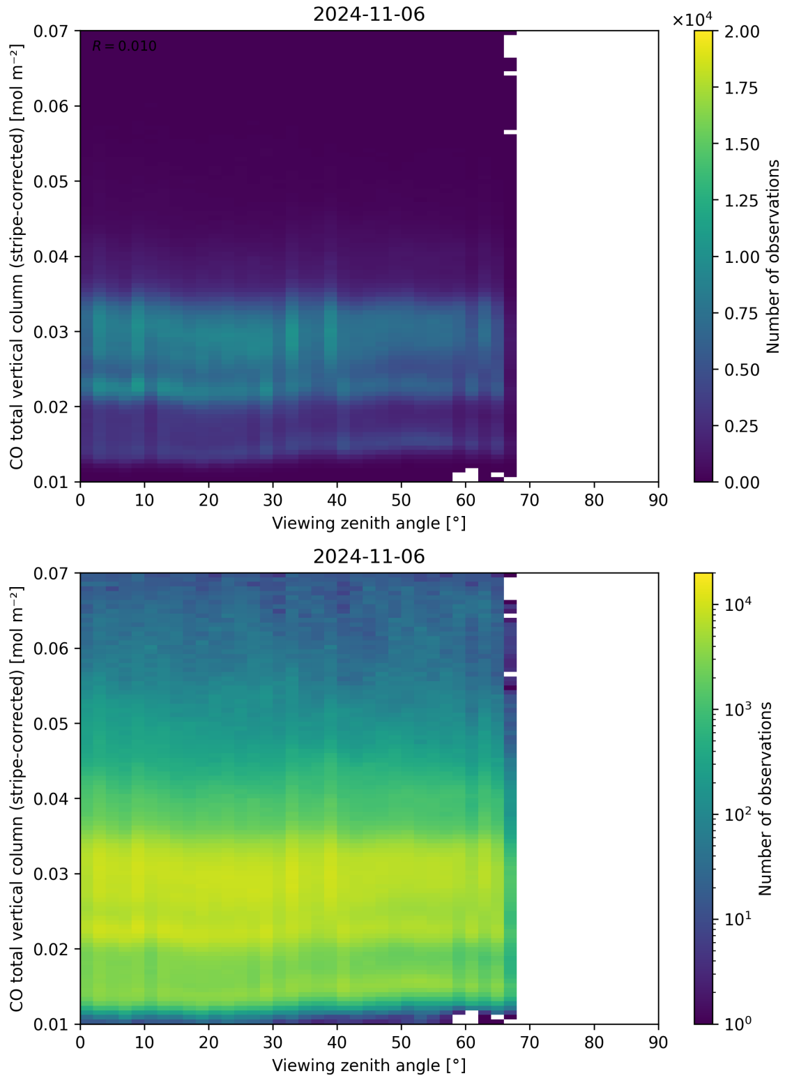
Figure 70: Scatter density plot of “Viewing zenith angle” against “CO total vertical column (stripe-corrected)” for 2024-11-05 to 2024-11-07.
