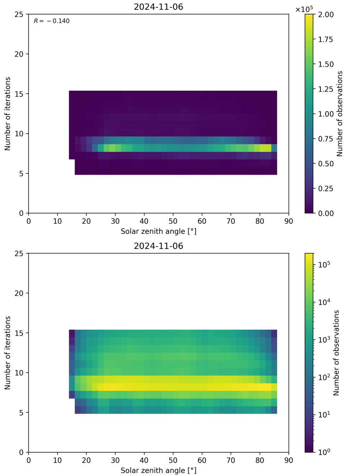
Figure 67: Scatter density plot of “Solar zenith angle” against “Number of iterations” for 2024-11-05 to 2024-11-07.
