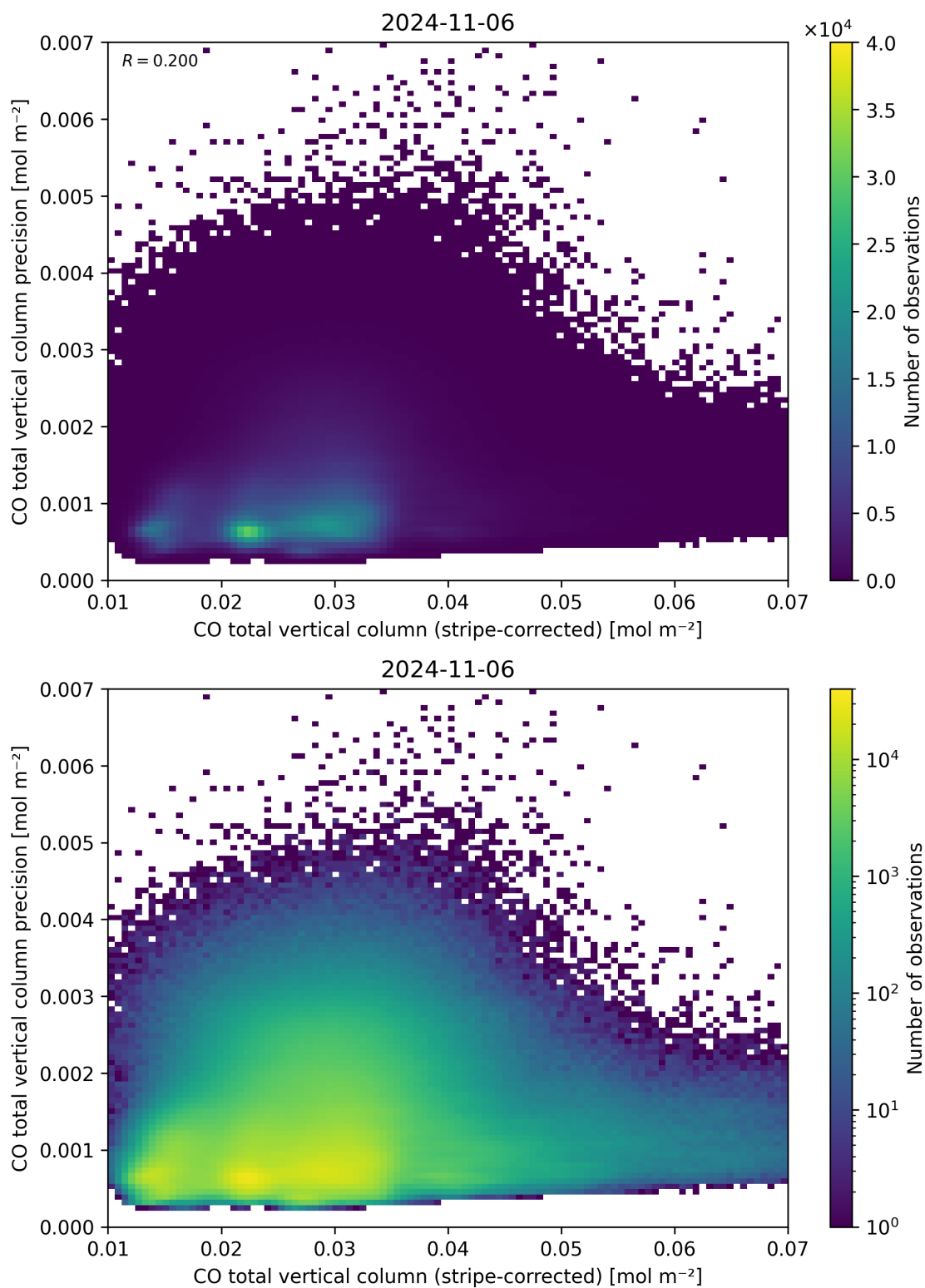
Figure 36: Scatter density plot of “CO total vertical column (stripe-corrected)” against “CO total vertical column precision” for 2024-11-05 to 2024-11-07.
