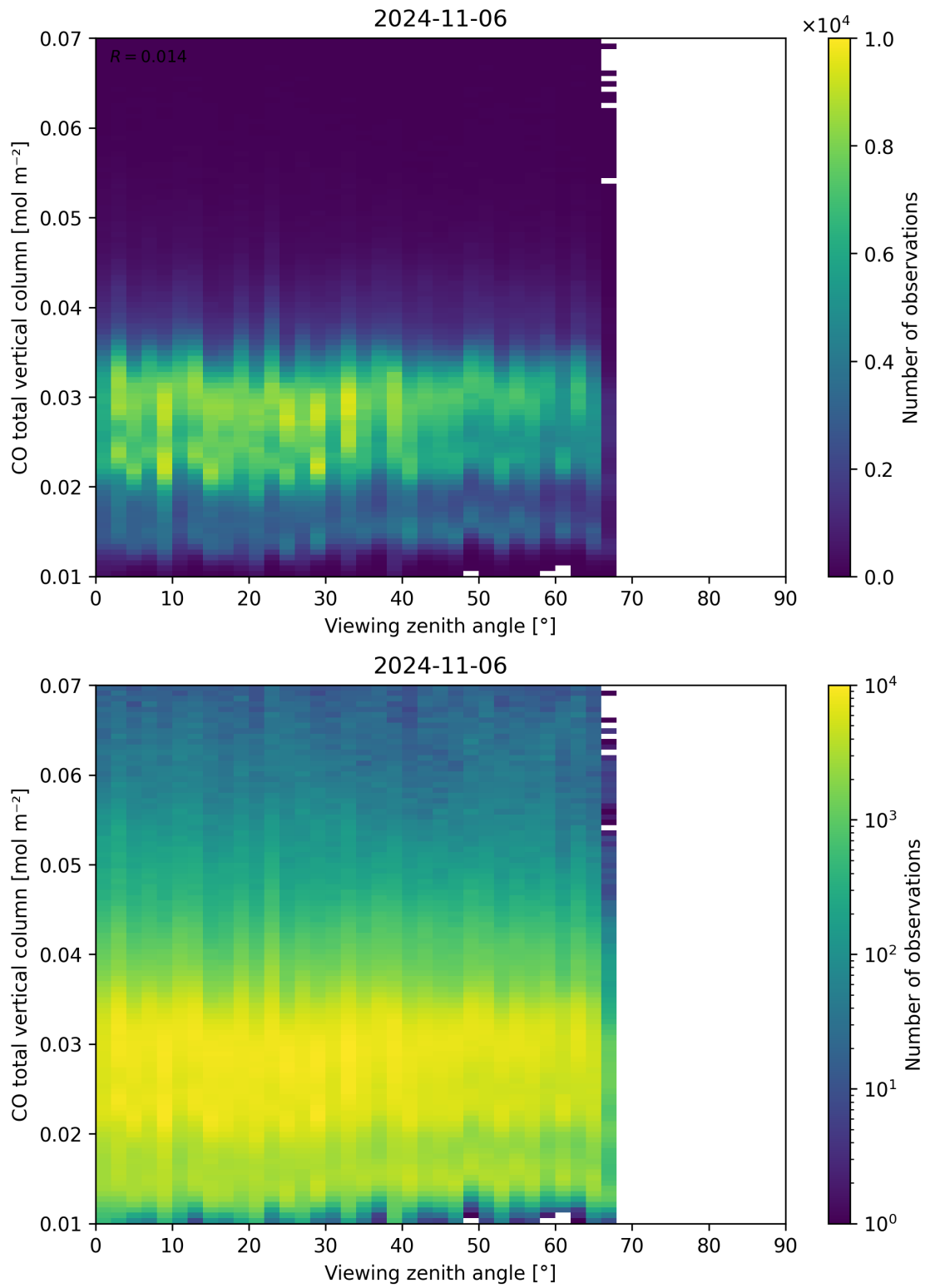
Figure 69: Scatter density plot of “Viewing zenith angle” against “CO total vertical column” for 2024-11-05 to 2024-11-07.
