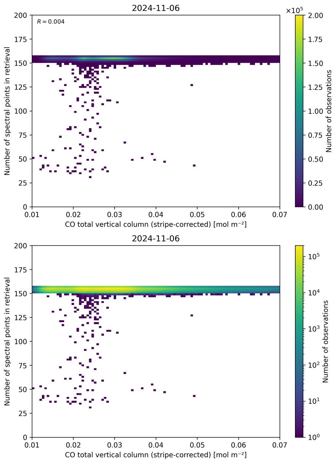
Figure 40: Scatter density plot of “CO total vertical column (stripe-corrected)” against “Number of spectral points in retrieval” for 2024-11-05 to 2024-11-07.
