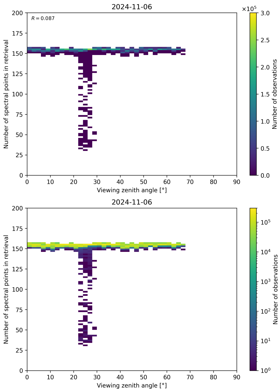
Figure 76: Scatter density plot of “Viewing zenith angle” against “Number of spectral points in retrieval” for 2024-11-05 to 2024-11-07.
