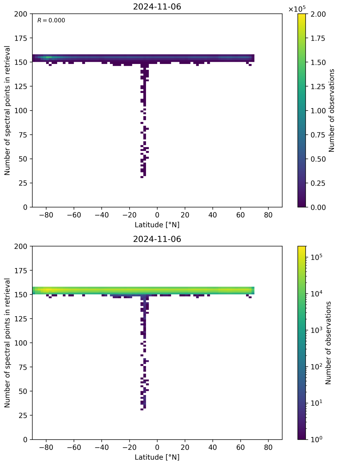
Figure 57: Scatter density plot of “Latitude” against “Number of spectral points in retrieval” for 2024-11-05 to 2024-11-07.
