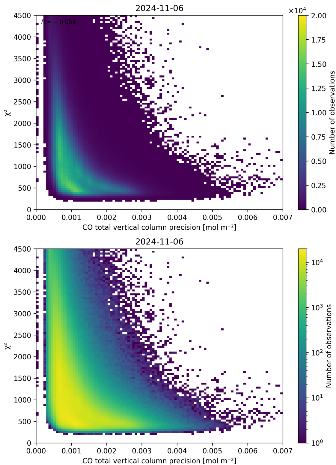
Figure 44: Scatter density plot of “CO total vertical column precision” against “ \chi^2 ” for 2024-11-05 to 2024-11-07.
