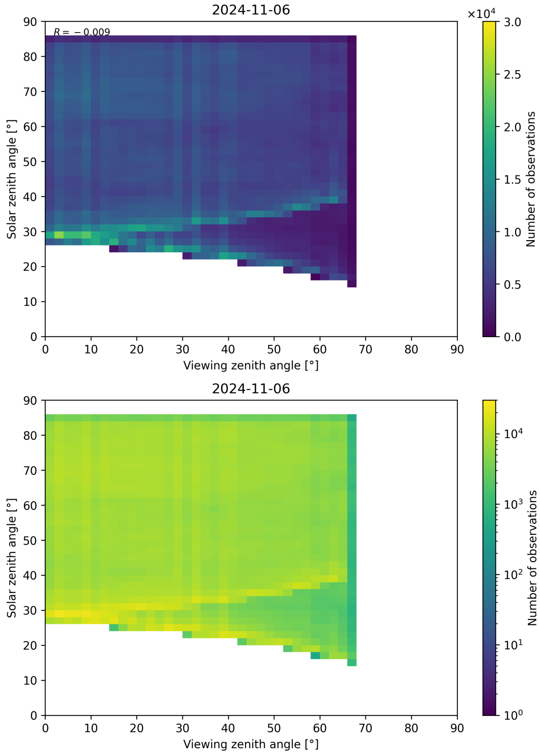
Figure 77: Scatter density plot of “Viewing zenith angle” against “Solar zenith angle” for 2024-11-05 to 2024-11-07.
