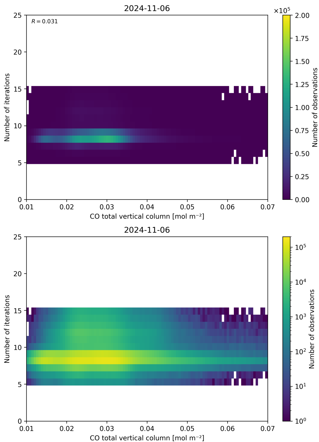
Figure 42: Scatter density plot of “CO total vertical column” against “Number of iterations” for 2024-11-05 to 2024-11-07.
