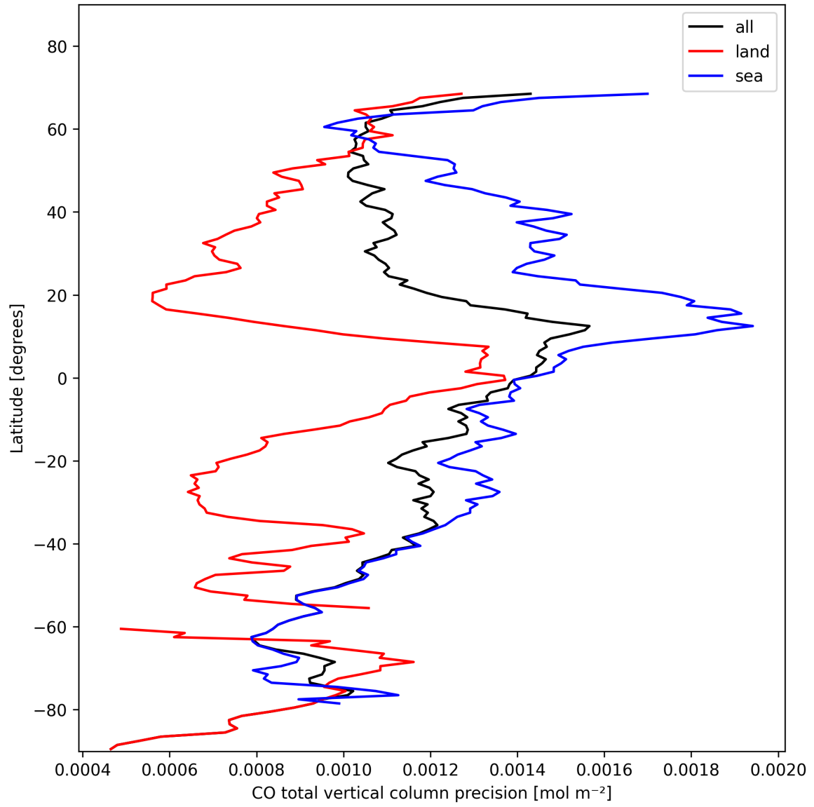
Figure 12: Zonal average of “CO total vertical column precision” for 2024-11-05 to 2024-11-07.
