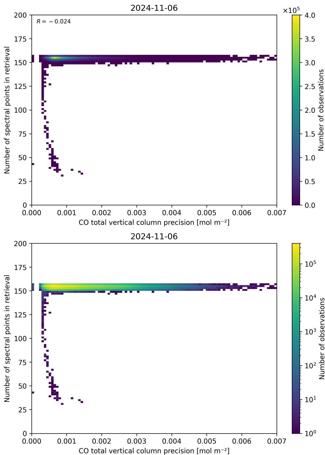
Figure 47: Scatter density plot of “CO total vertical column precision” against “Number of spectral points in retrieval” for 2024-11-05 to 2024-11-07.
