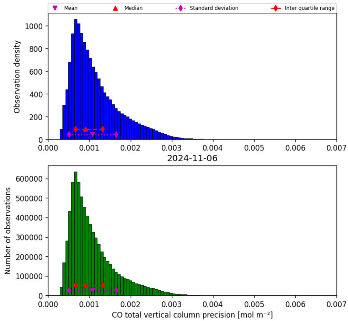
Figure 20: Histogram of “CO total vertical column precision” for 2024-11-05 to 2024-11-07
