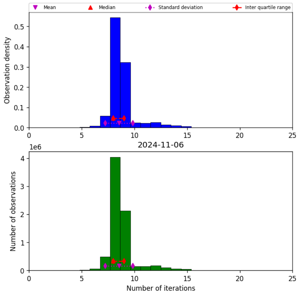
Figure 24: Histogram of “Number of iterations” for 2024-11-05 to 2024-11-07
