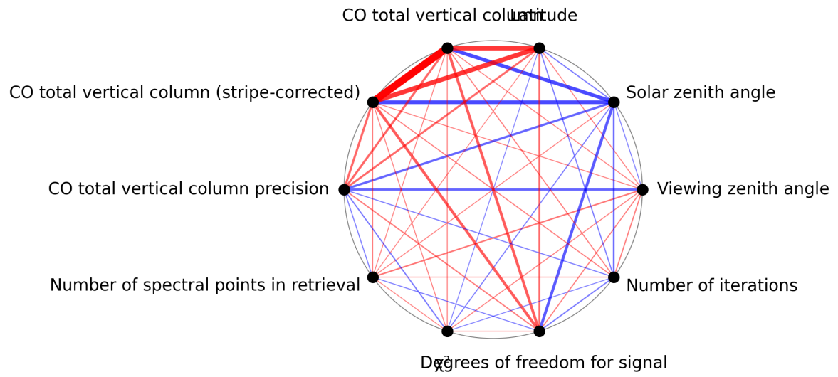
Figure 1: Map of correlation graph for 2024-11-05 to 2024-11-07.
