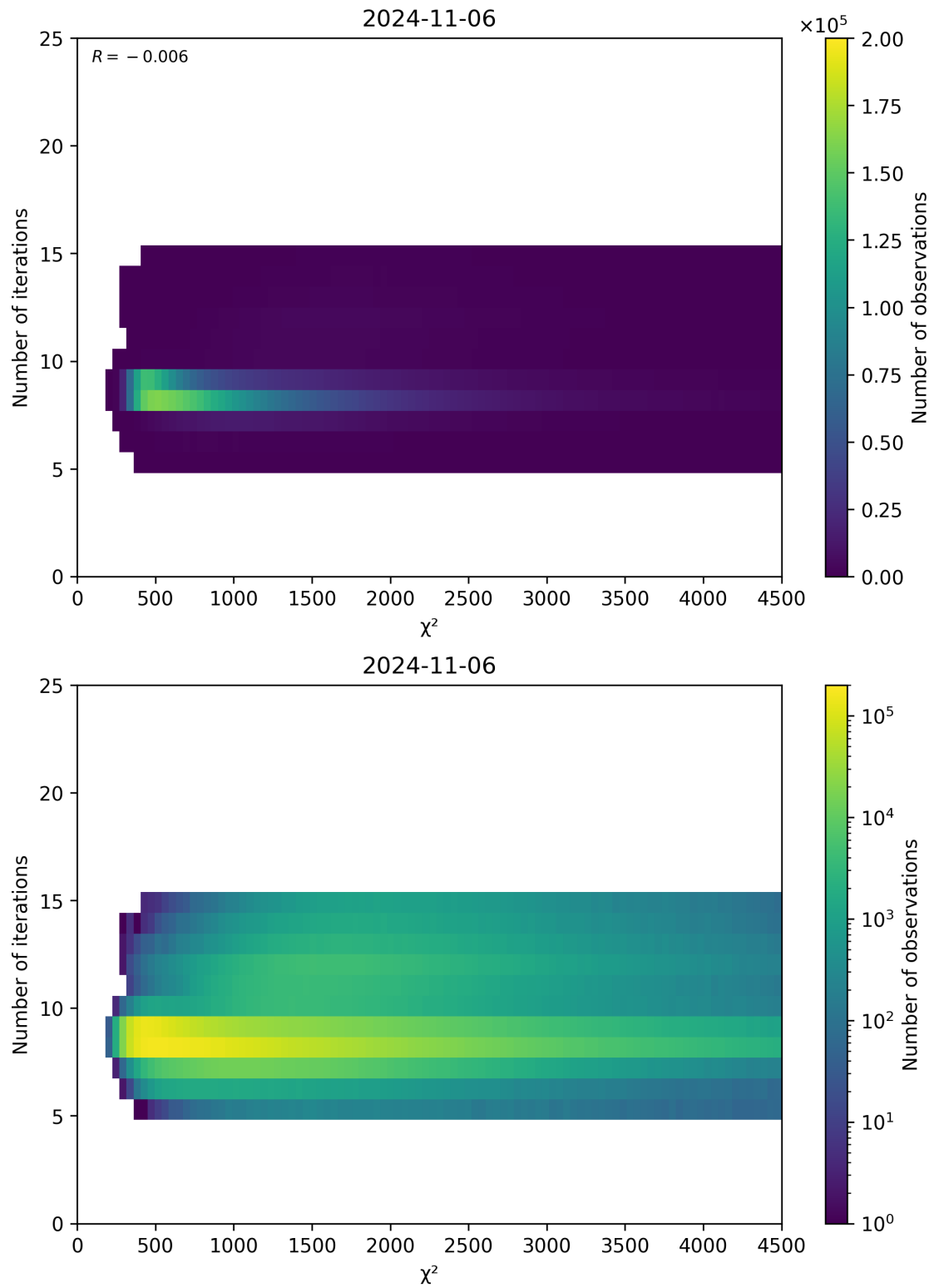
Figure 49: Scatter density plot of “ \chi^2 ” against “Number of iterations” for 2024-11-05 to 2024-11-07.
