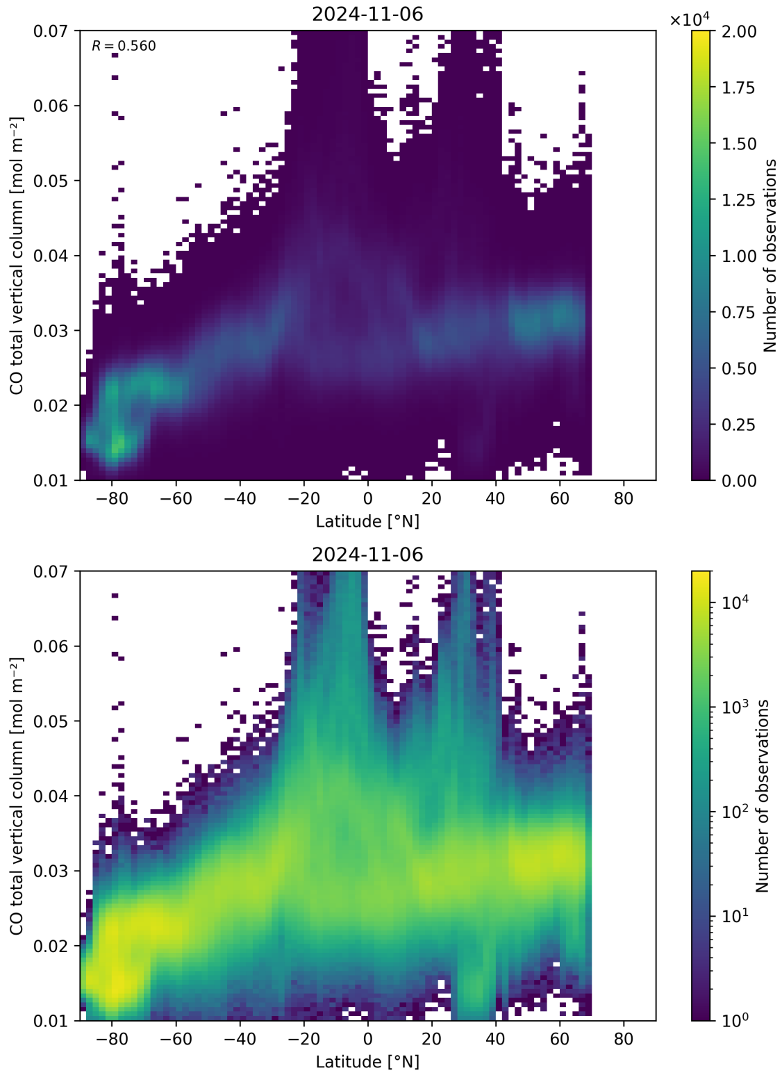
Figure 51: Scatter density plot of “Latitude” against “CO total vertical column” for 2024-11-05 to 2024-11-07.
