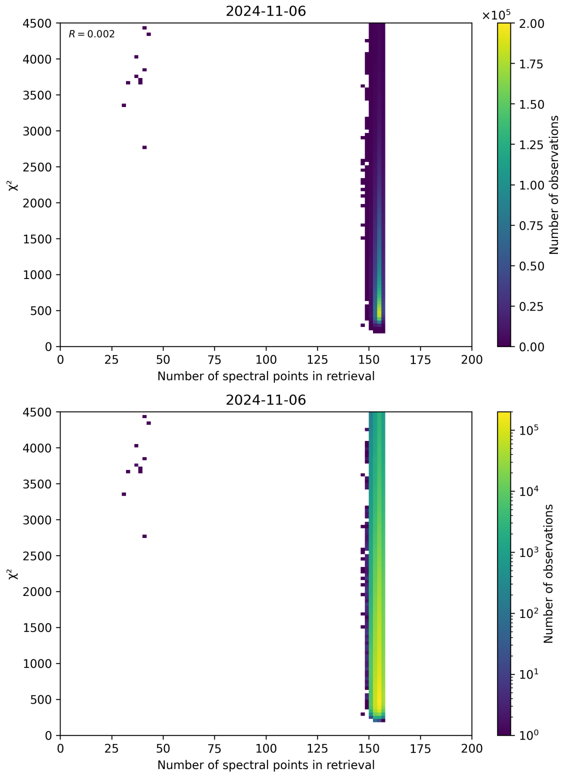
Figure 58: Scatter density plot of “Number of spectral points in retrieval” against “ \chi^2 ” for 2024-11-05 to 2024-11-07.
