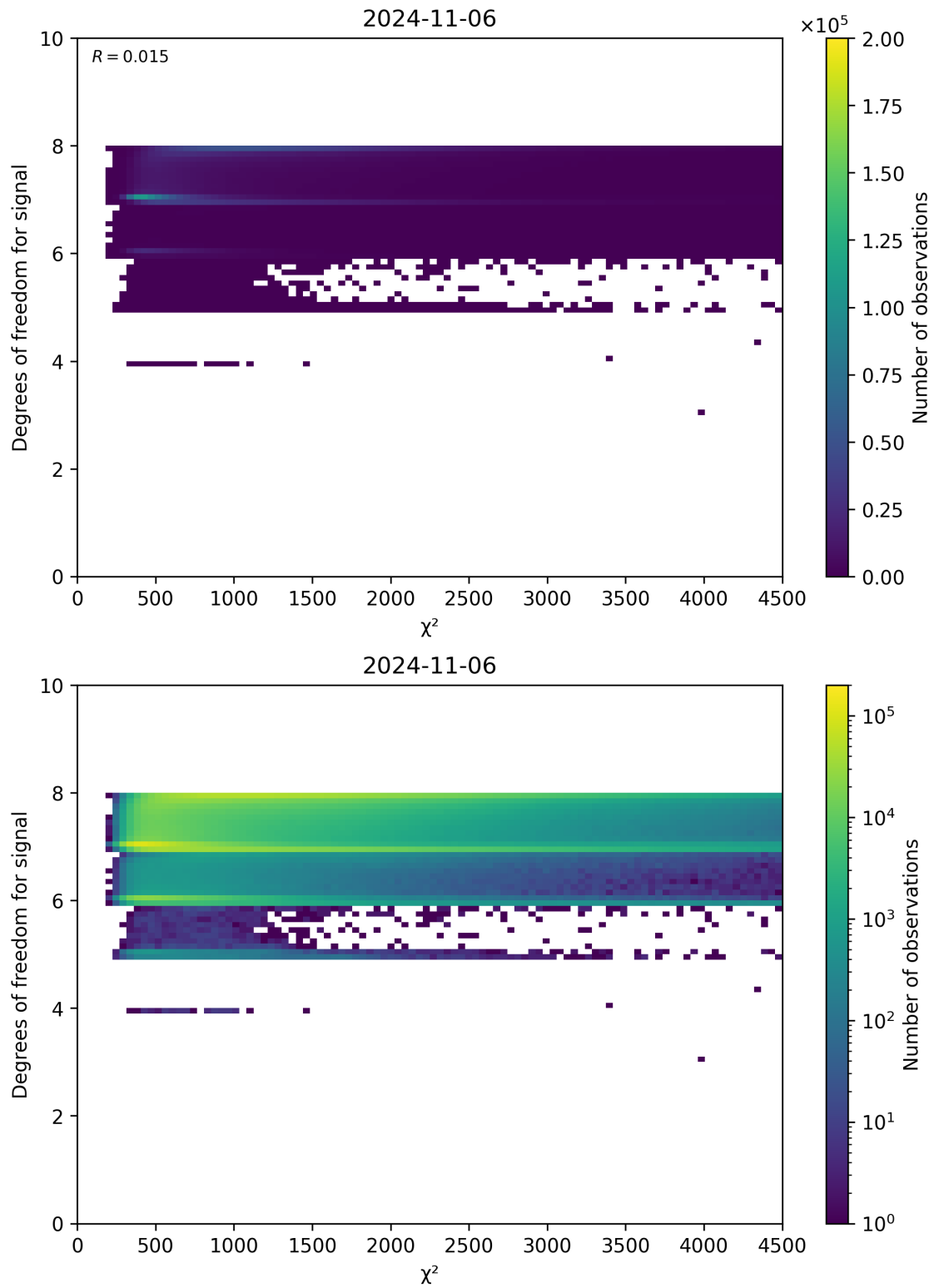
Figure 48: Scatter density plot of “ \chi^2 ” against “Degrees of freedom for signal” for 2024-11-05 to 2024-11-07.
