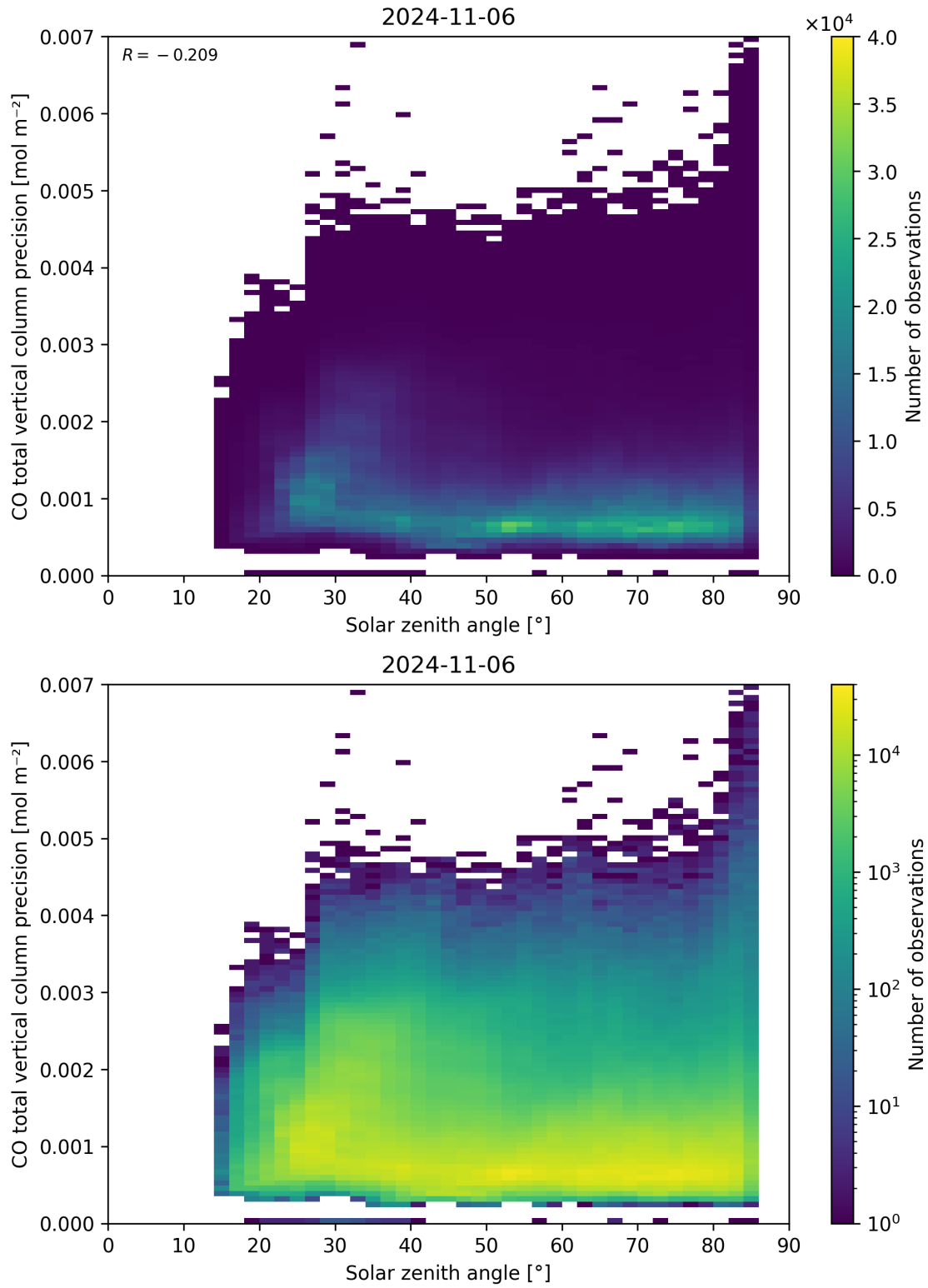
Figure 63: Scatter density plot of “Solar zenith angle” against “CO total vertical column precision” for 2024-11-05 to 2024-11-07.
