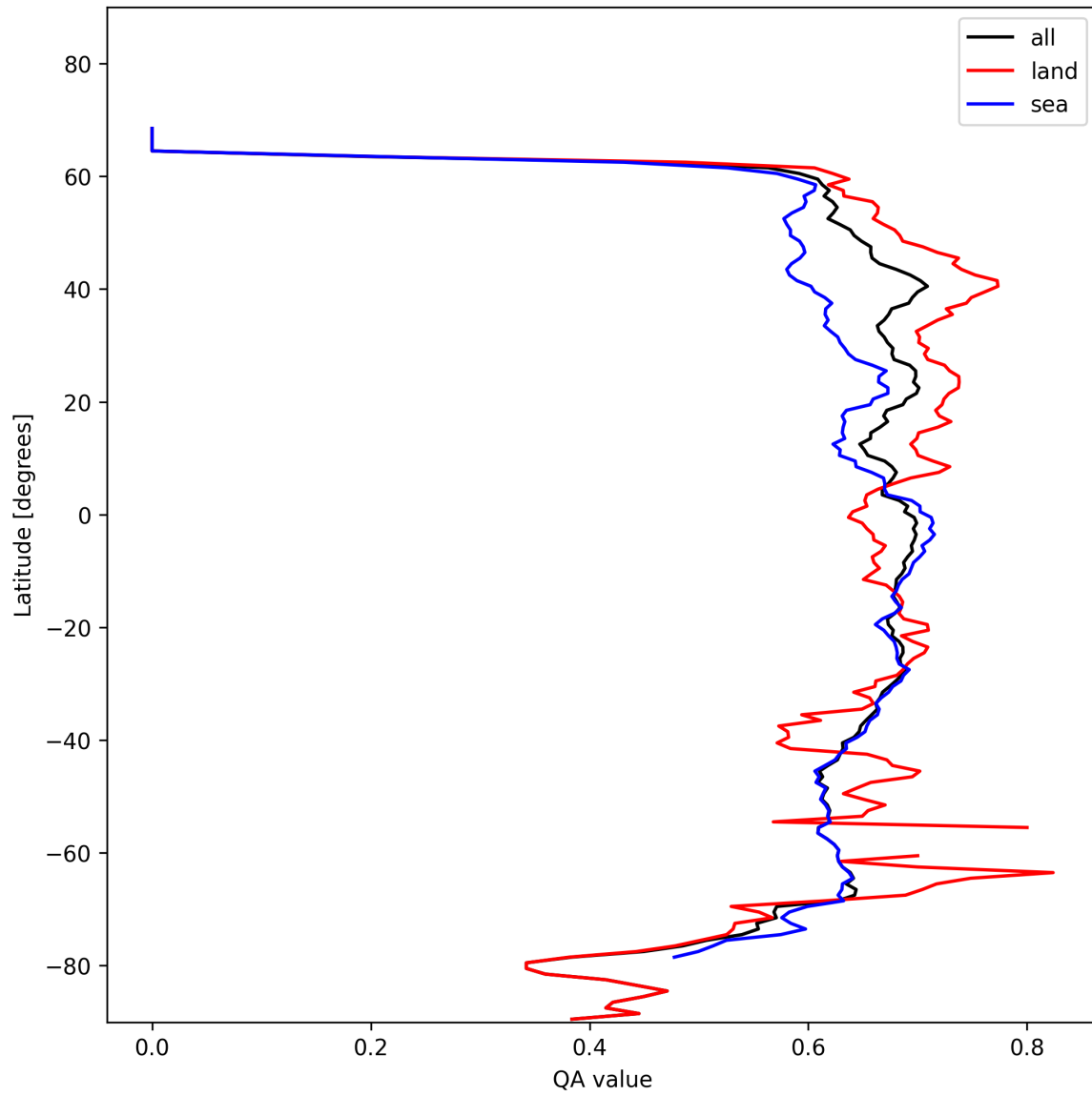
Figure 9: Zonal average of “QA value” for 2024-11-05 to 2024-11-07.
