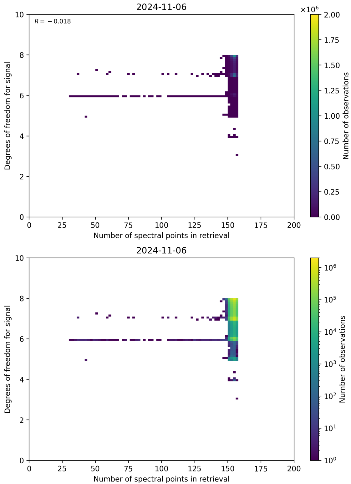
Figure 59: Scatter density plot of “Number of spectral points in retrieval” against “Degrees of freedom for signal” for 2024-11-05 to 2024-11-07.
