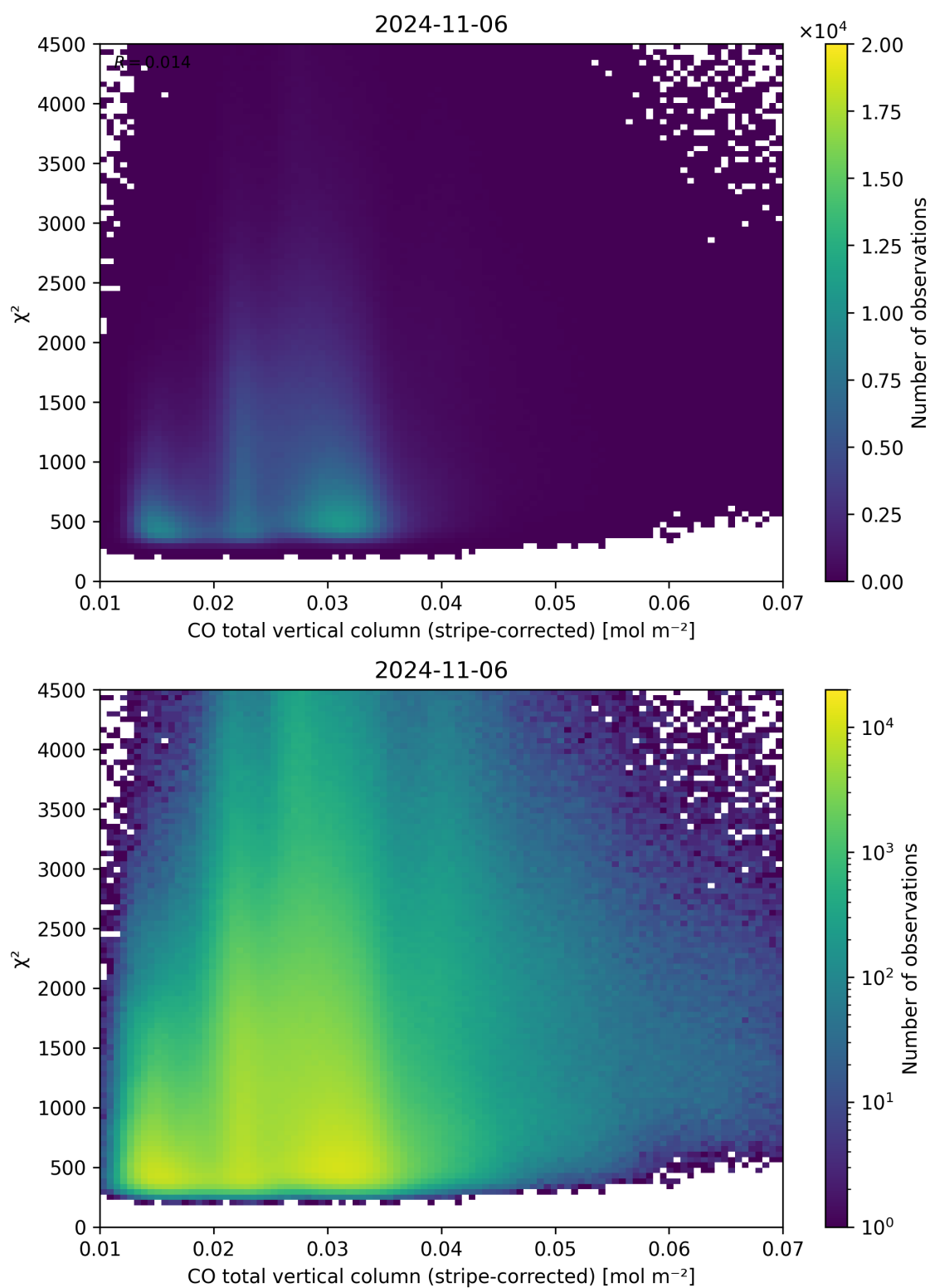
Figure 37: Scatter density plot of “CO total vertical column (stripe-corrected)” against “ \chi^2 ” for 2024-11-05 to 2024-11-07.
