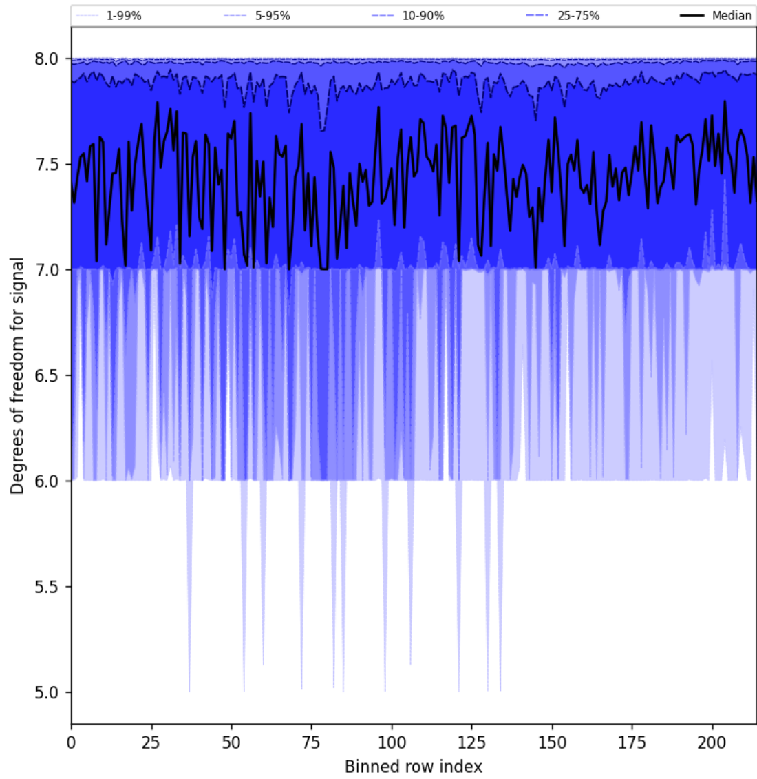
Figure 31: Along track statistics of “Degrees of freedom for signal” for 2024-11-05 to 2024-11-07
