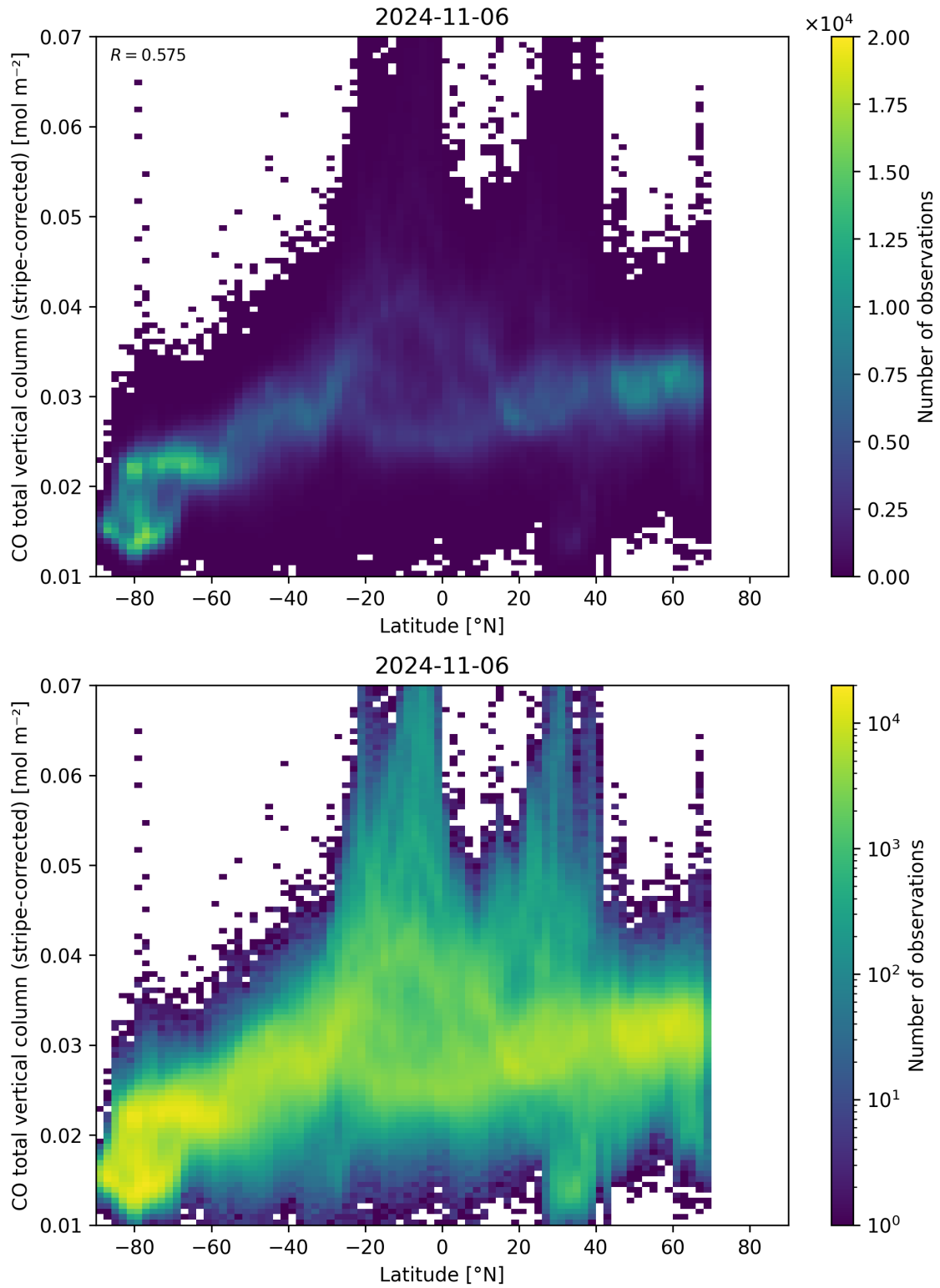
Figure 52: Scatter density plot of “Latitude” against “CO total vertical column (stripe-corrected)” for 2024-11-05 to 2024-11-07.
