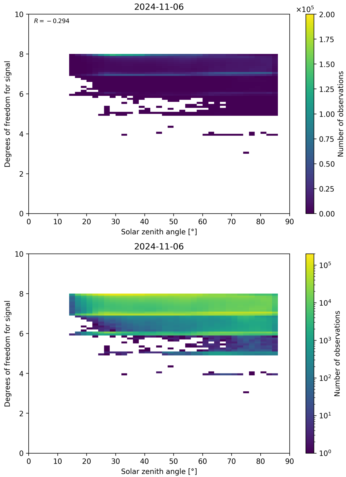
Figure 65: Scatter density plot of “Solar zenith angle” against “Degrees of freedom for signal” for 2024-11-05 to 2024-11-07.
