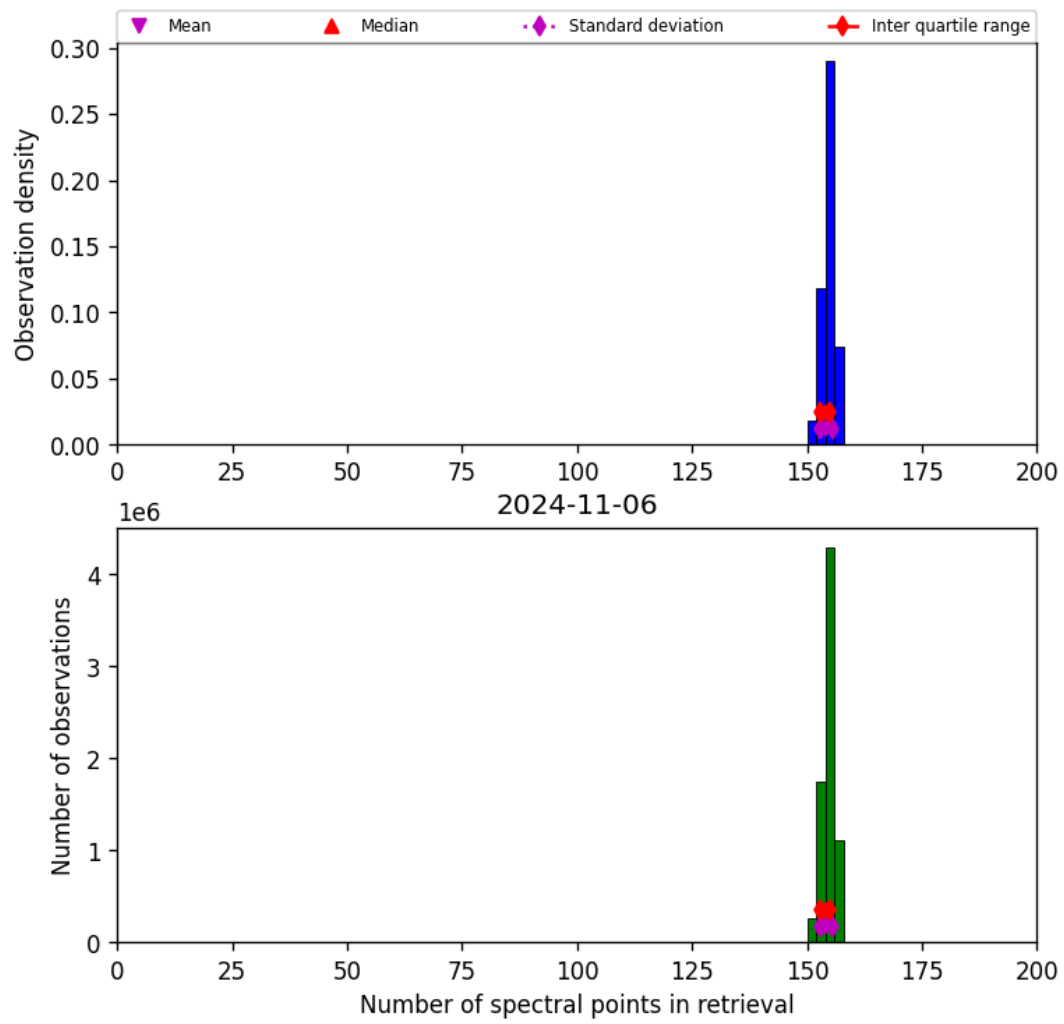
Figure 21: Histogram of “Number of spectral points in retrieval” for 2024-11-05 to 2024-11-07
