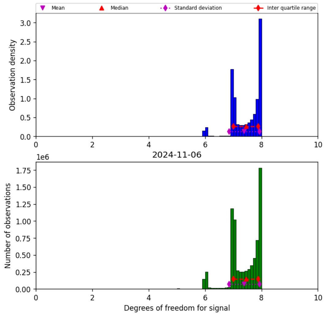
Figure 23: Histogram of “Degrees of freedom for signal” for 2024-11-05 to 2024-11-07
