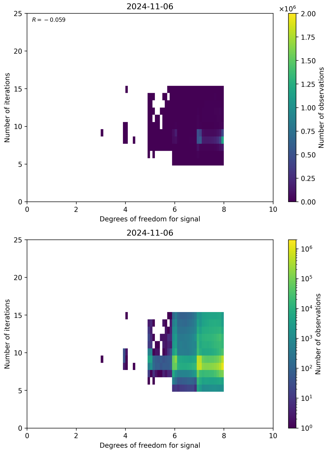
Figure 50: Scatter density plot of “Degrees of freedom for signal” against “Number of iterations” for 2024-11-05 to 2024-11-07.
