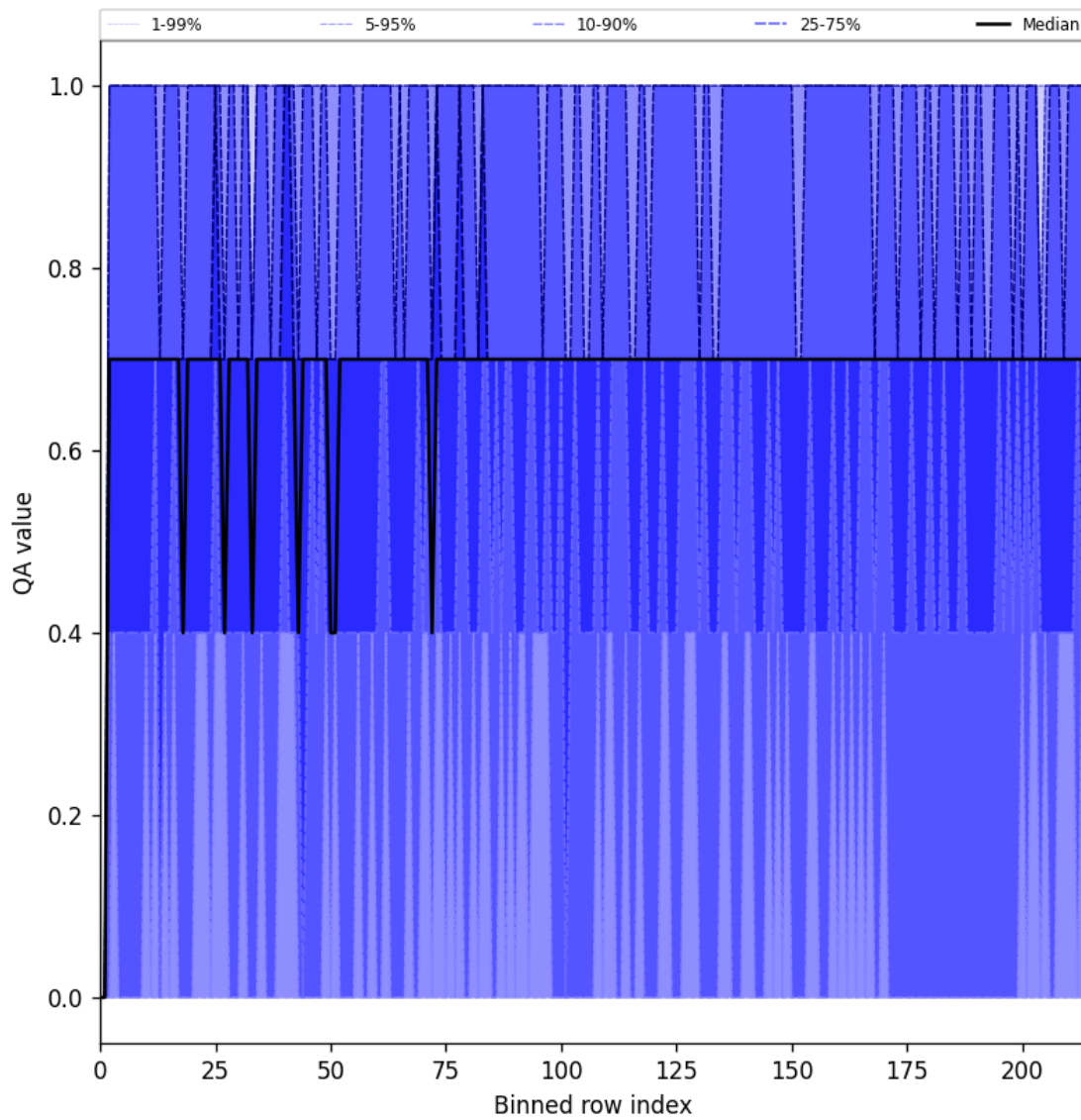
Figure 25: Along track statistics of “QA value” for 2024-11-05 to 2024-11-07
