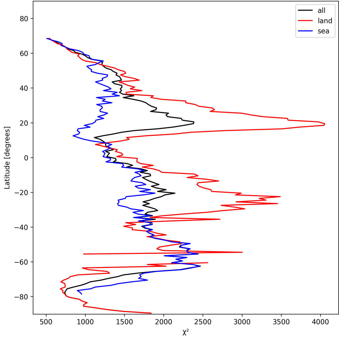
Figure 14: Zonal average of “ \chi^2 ” for 2024-11-05 to 2024-11-07.
