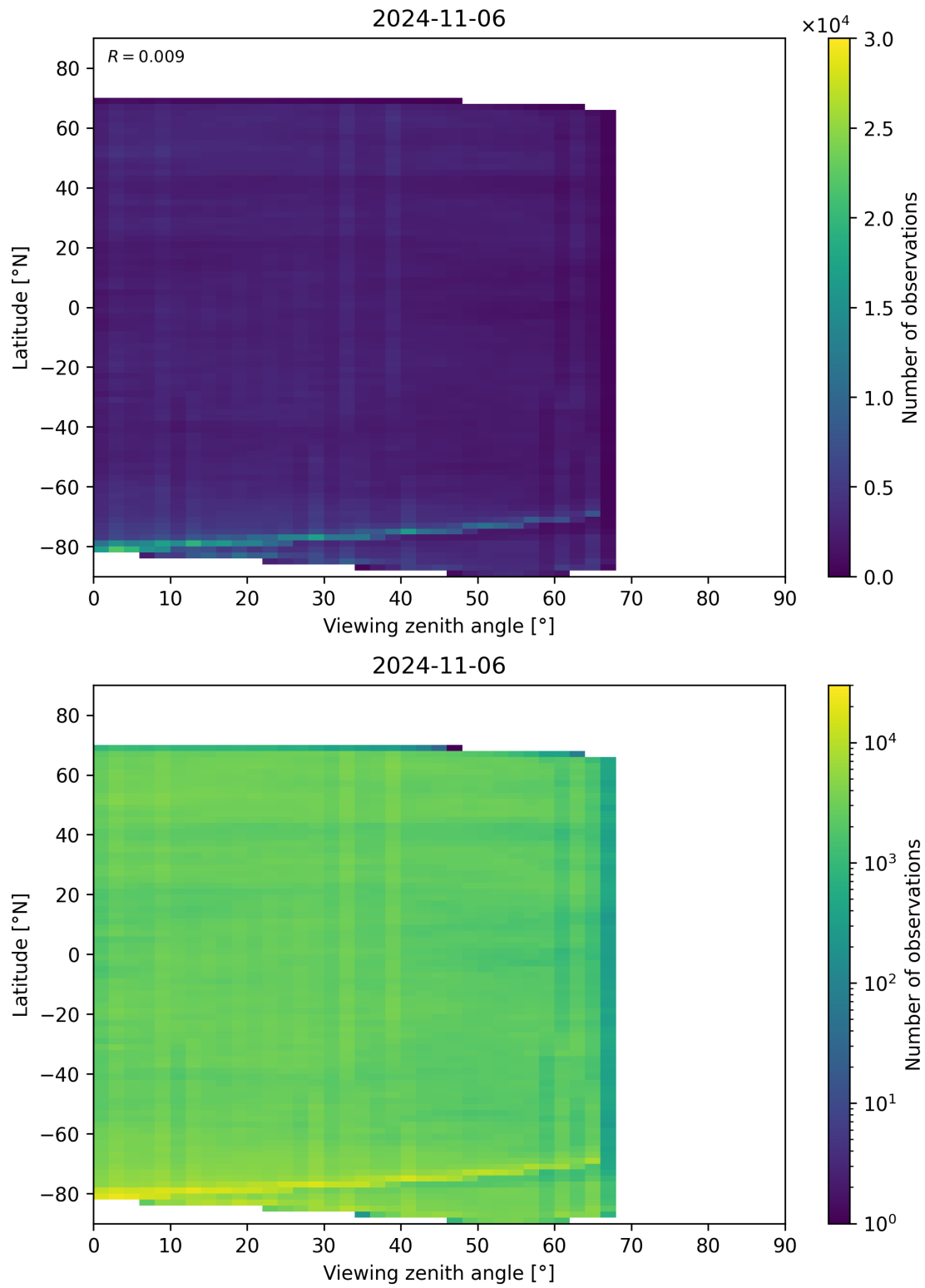
Figure 74: Scatter density plot of “Viewing zenith angle” against “Latitude” for 2024-11-05 to 2024-11-07.
