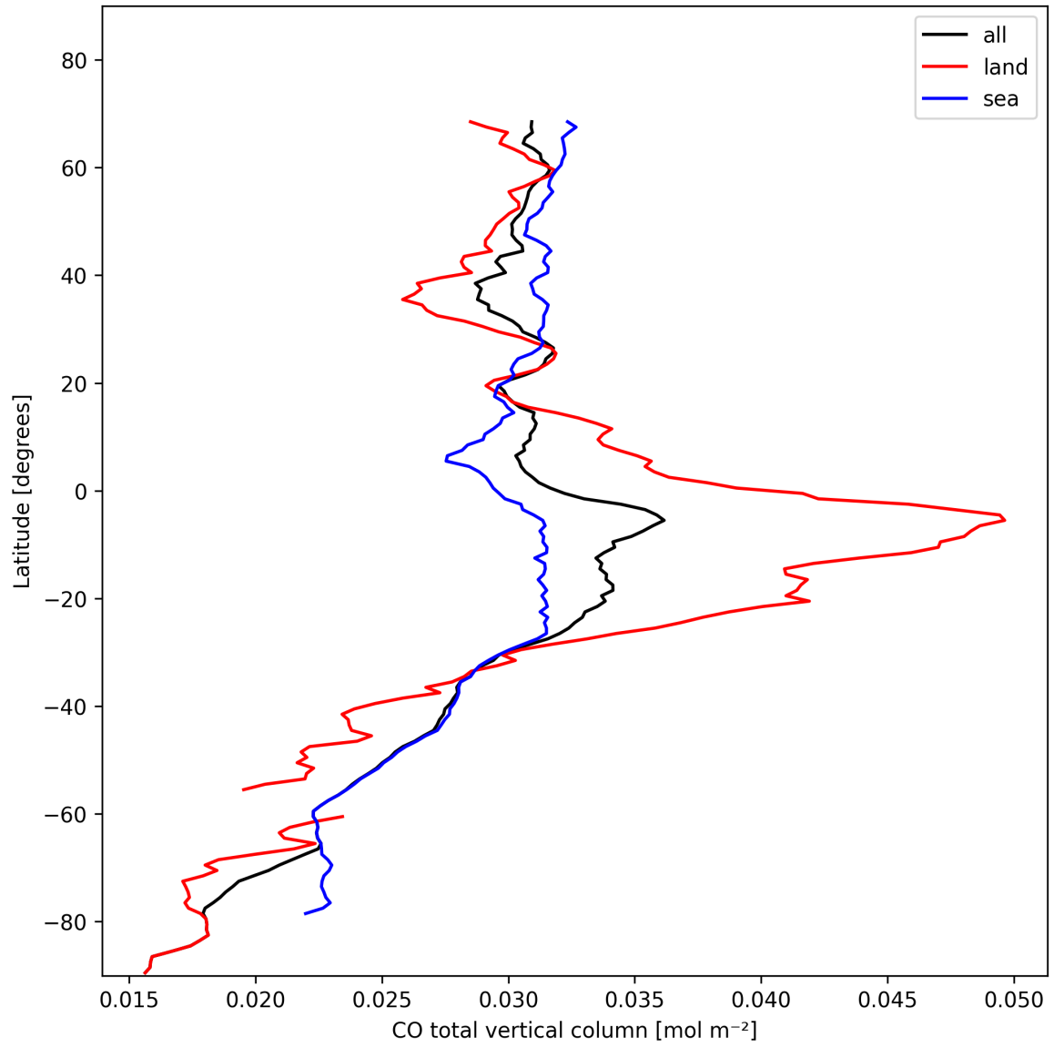
Figure 10: Zonal average of “CO total vertical column” for 2024-11-05 to 2024-11-07.
