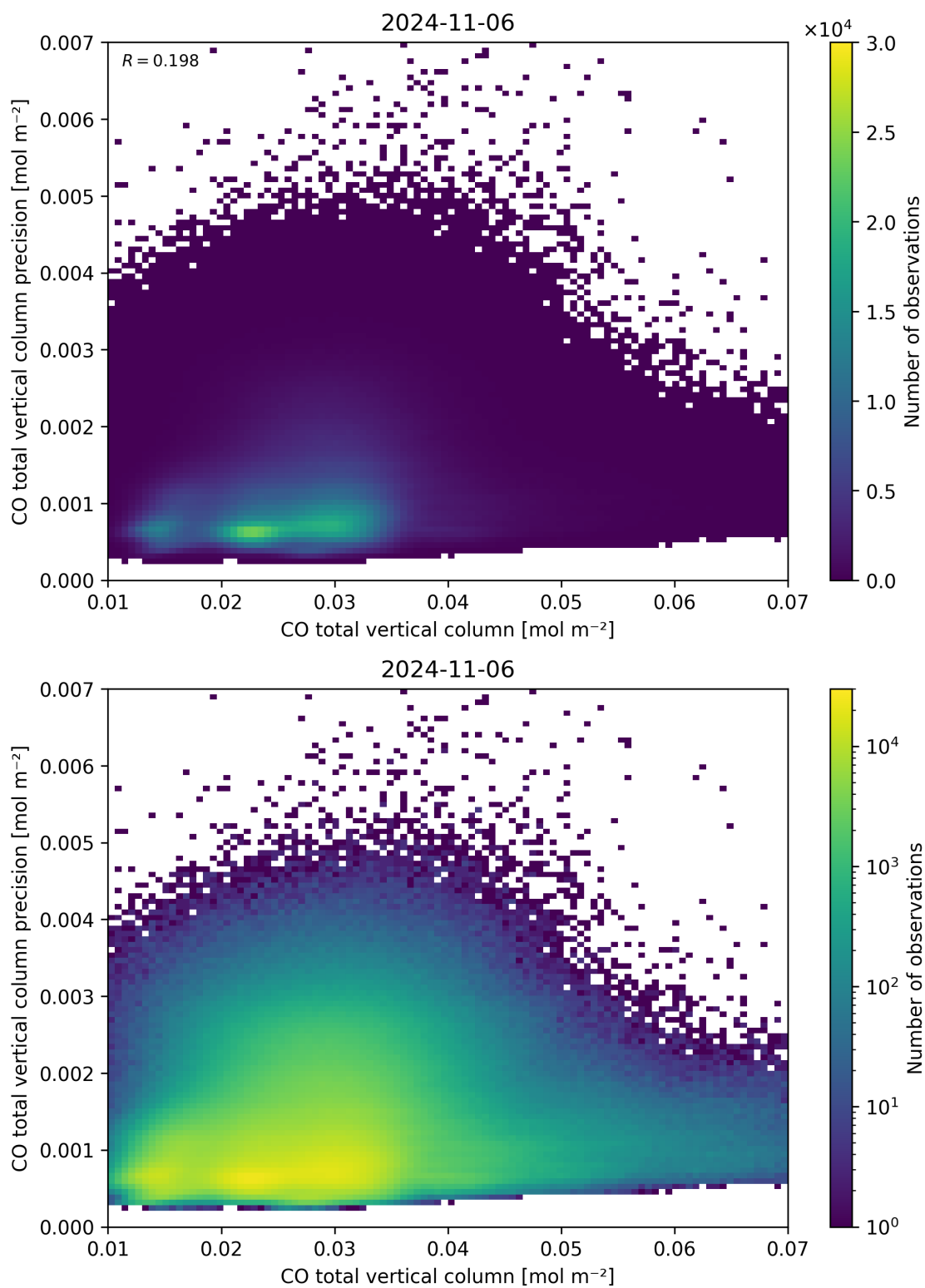
Figure 34: Scatter density plot of “CO total vertical column” against “CO total vertical column precision” for 2024-11-05 to 2024-11-07.
