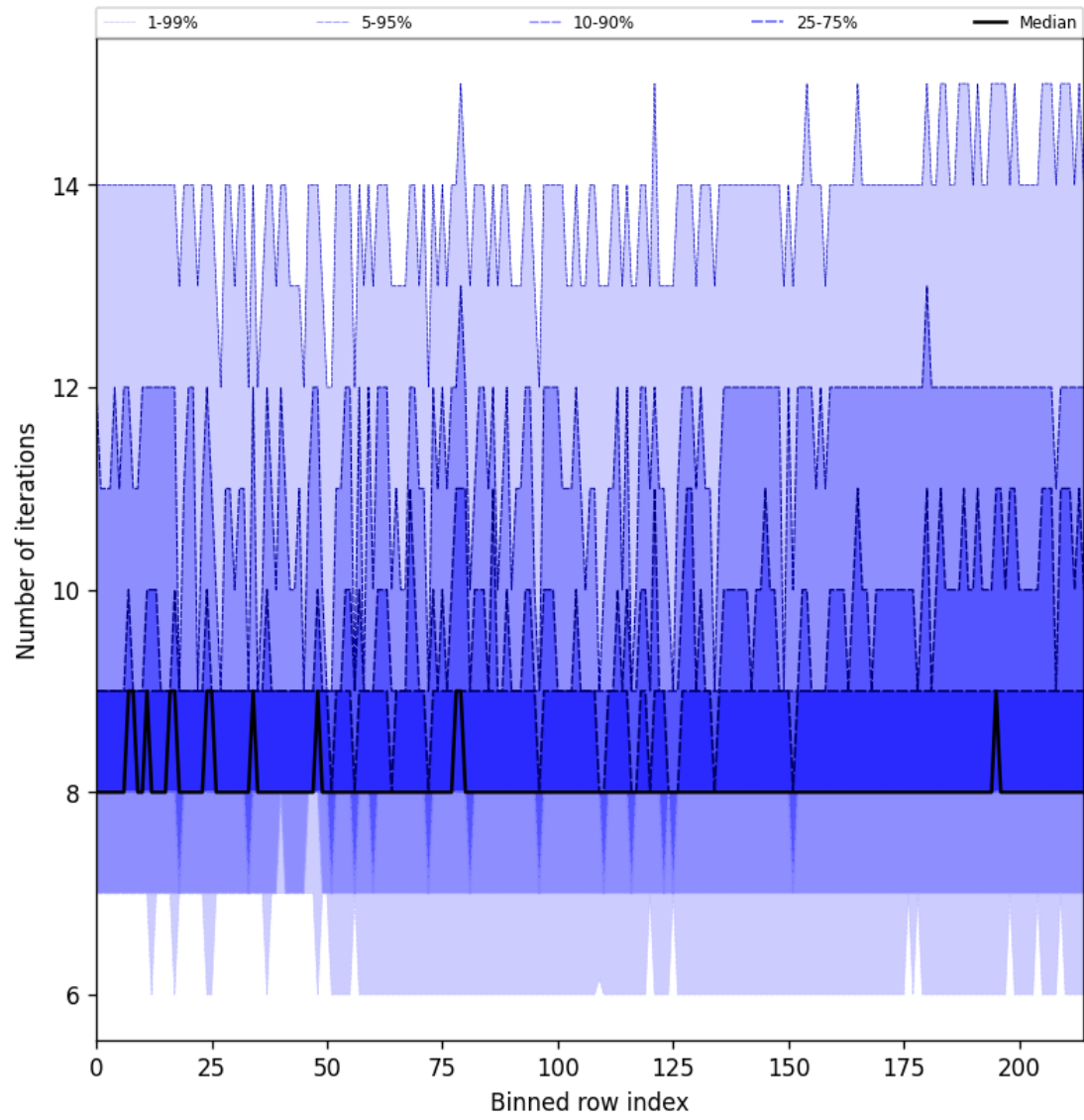
Figure 32: Along track statistics of “Number of iterations” for 2024-11-05 to 2024-11-07
