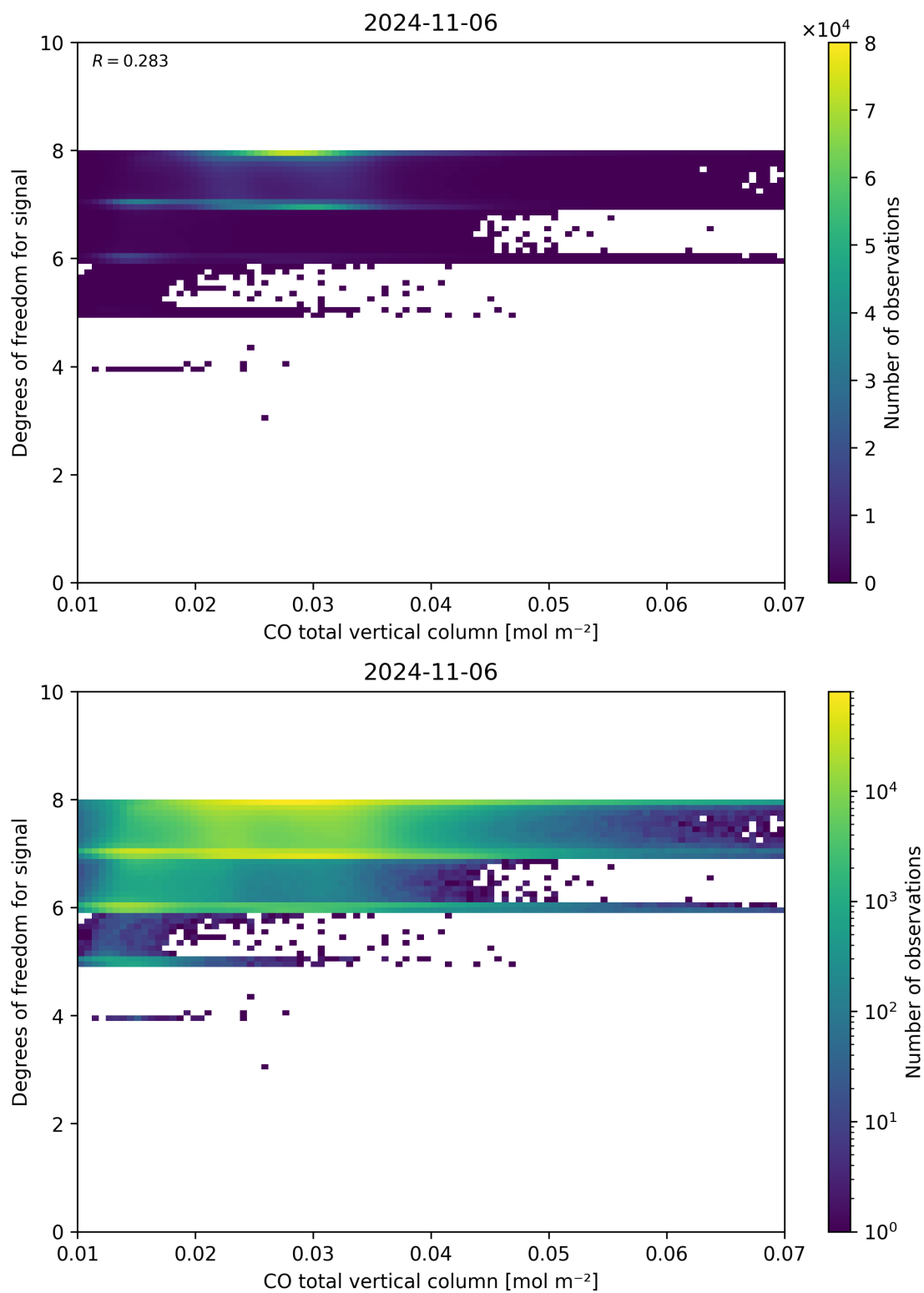
Figure 41: Scatter density plot of “CO total vertical column” against “Degrees of freedom for signal” for 2024-11-05 to 2024-11-07.
