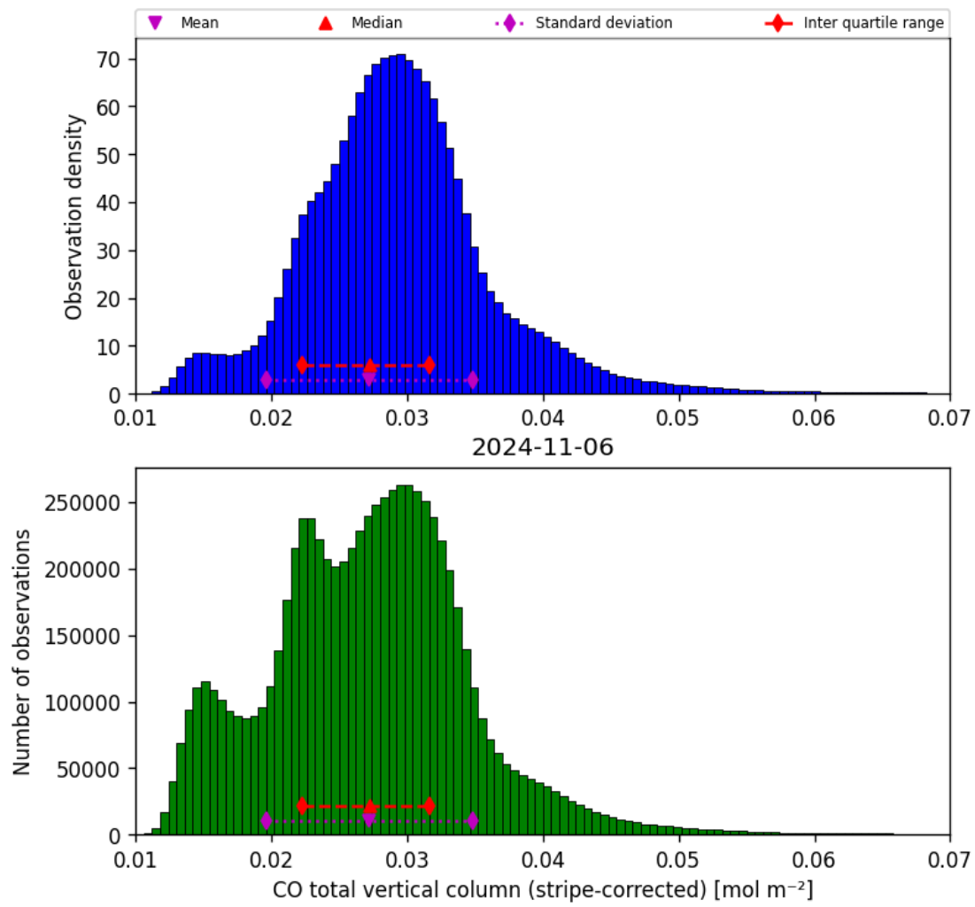
Figure 19: Histogram of “CO total vertical column (stripe-corrected)” for 2024-11-05 to 2024-11-07
