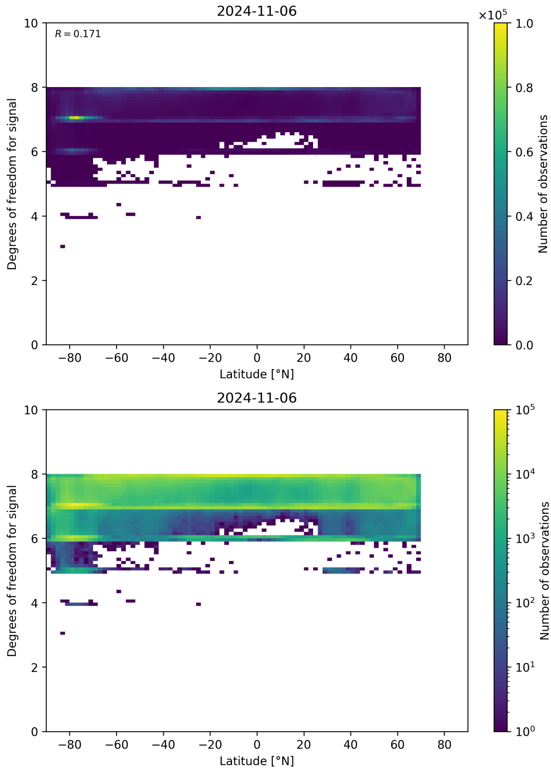
Figure 55: Scatter density plot of “Latitude” against “Degrees of freedom for signal” for 2024-11-05 to 2024-11-07.
