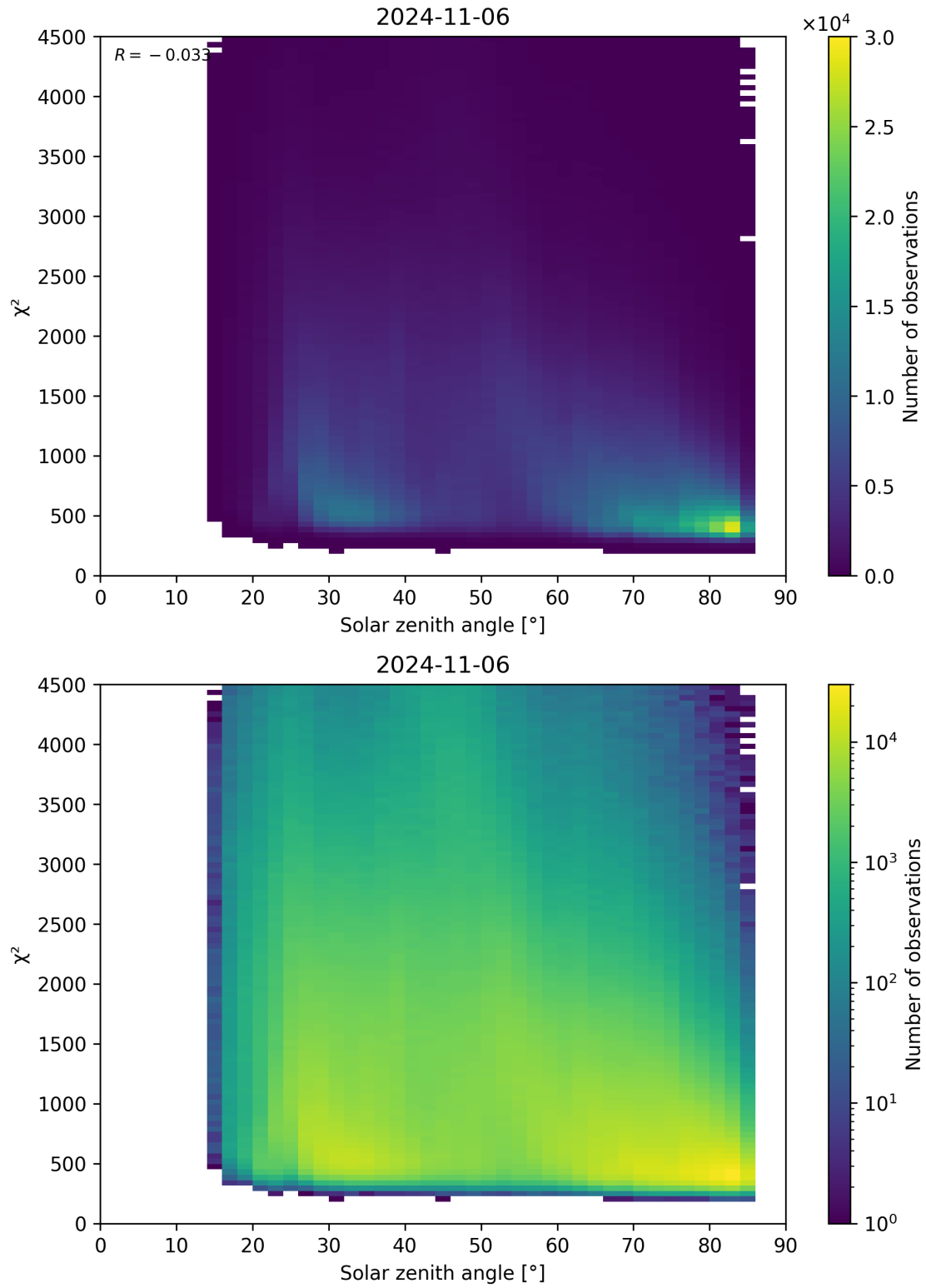
Figure 64: Scatter density plot of “Solar zenith angle” against “ \chi^2 ” for 2024-11-05 to 2024-11-07.
