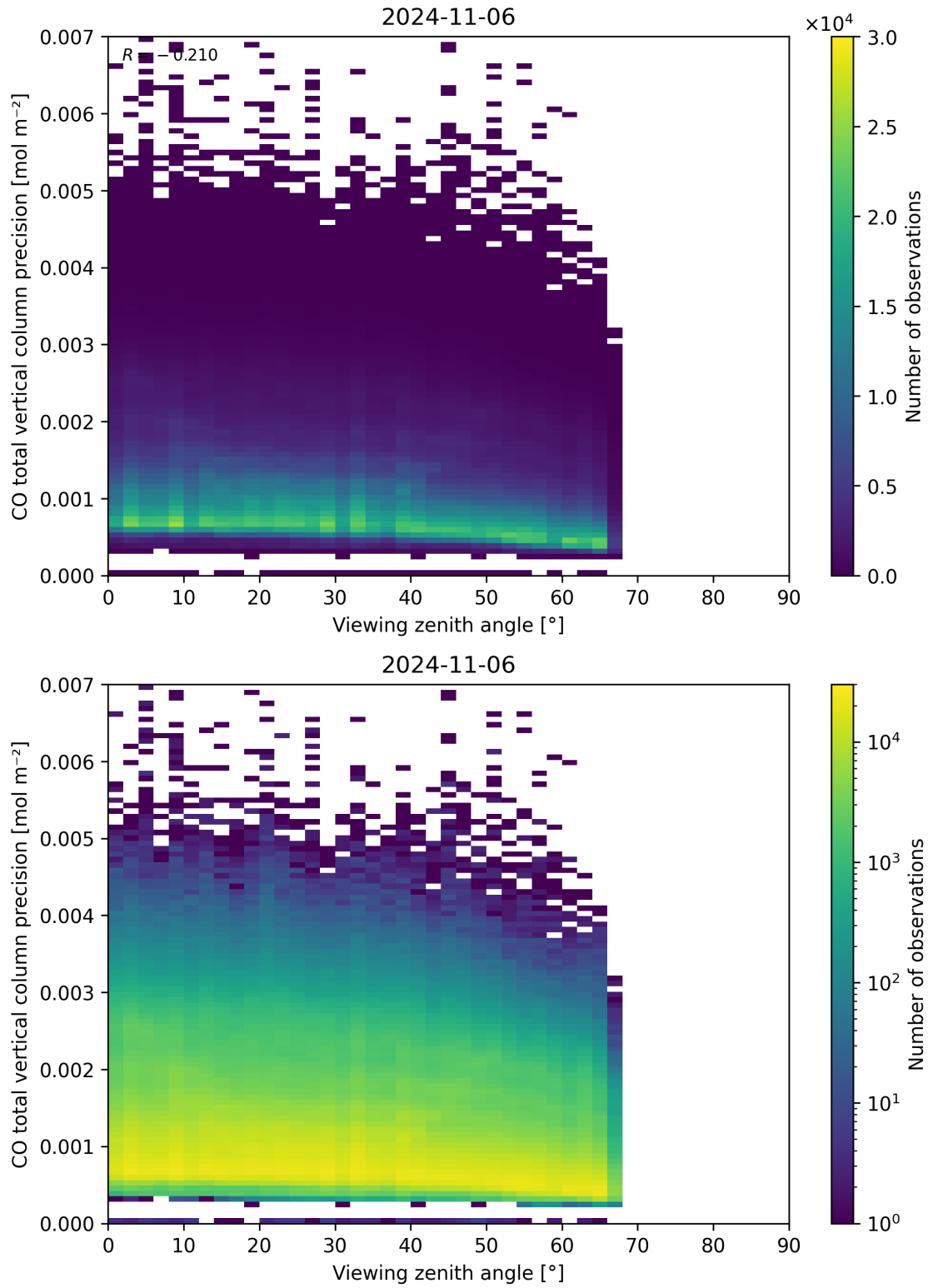
Figure 71: Scatter density plot of “Viewing zenith angle” against “CO total vertical column precision” for 2024-11-05 to 2024-11-07.
