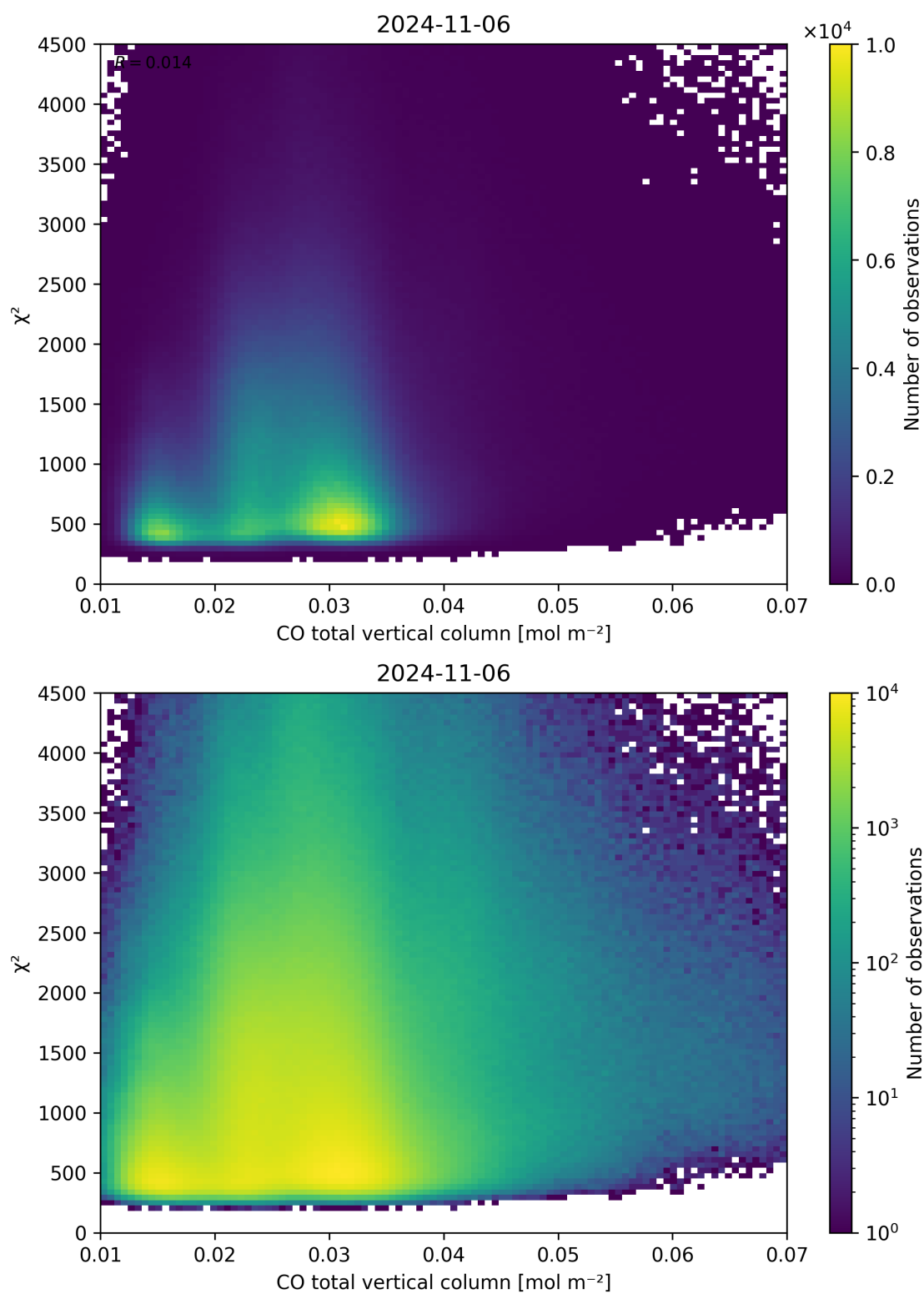
Figure 35: Scatter density plot of “CO total vertical column” against “ \chi^2 ” for 2024-11-05 to 2024-11-07.
