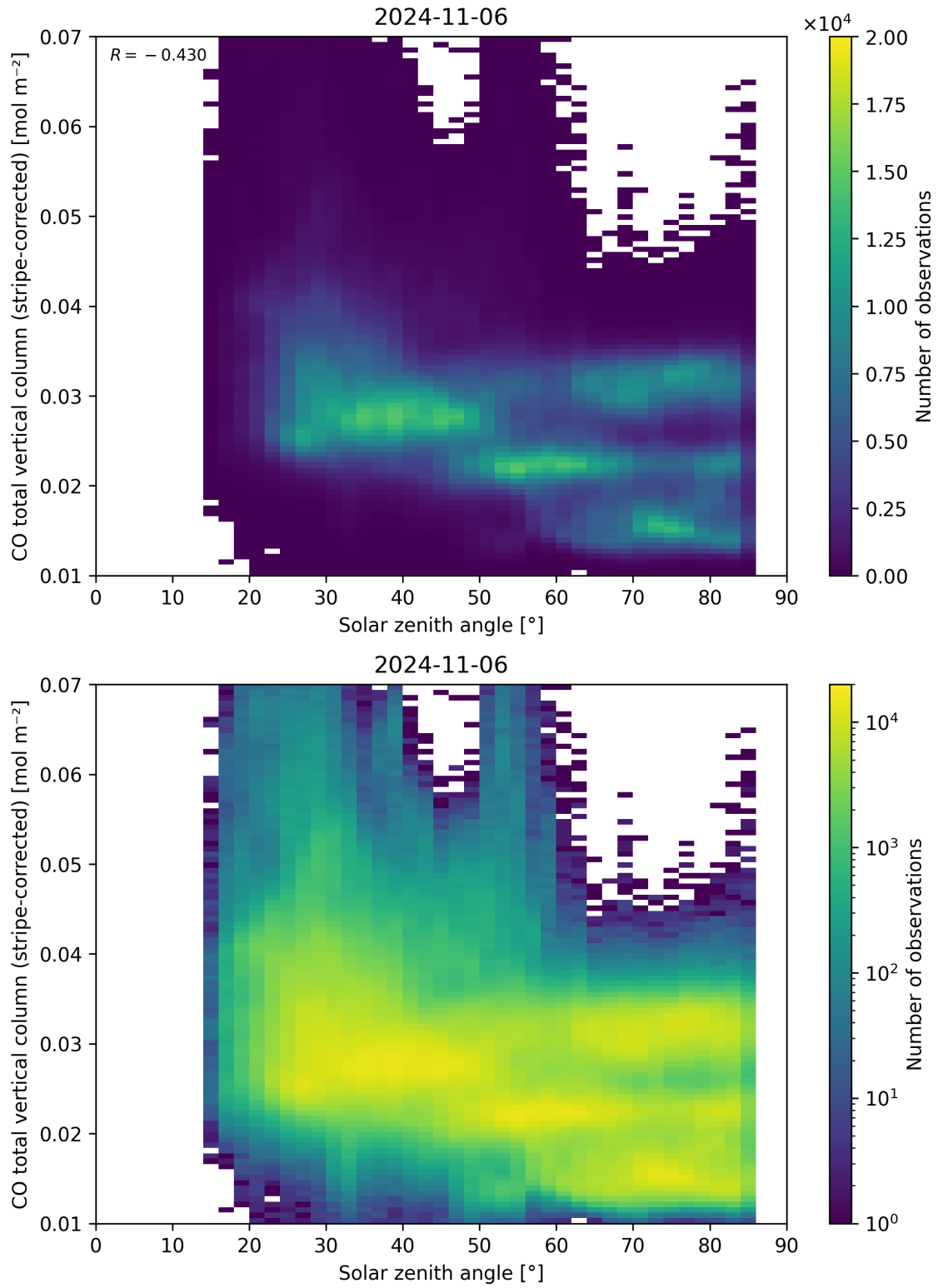
Figure 62: Scatter density plot of “Solar zenith angle” against “CO total vertical column (stripe-corrected)” for 2024-11-05 to 2024-11-07.
