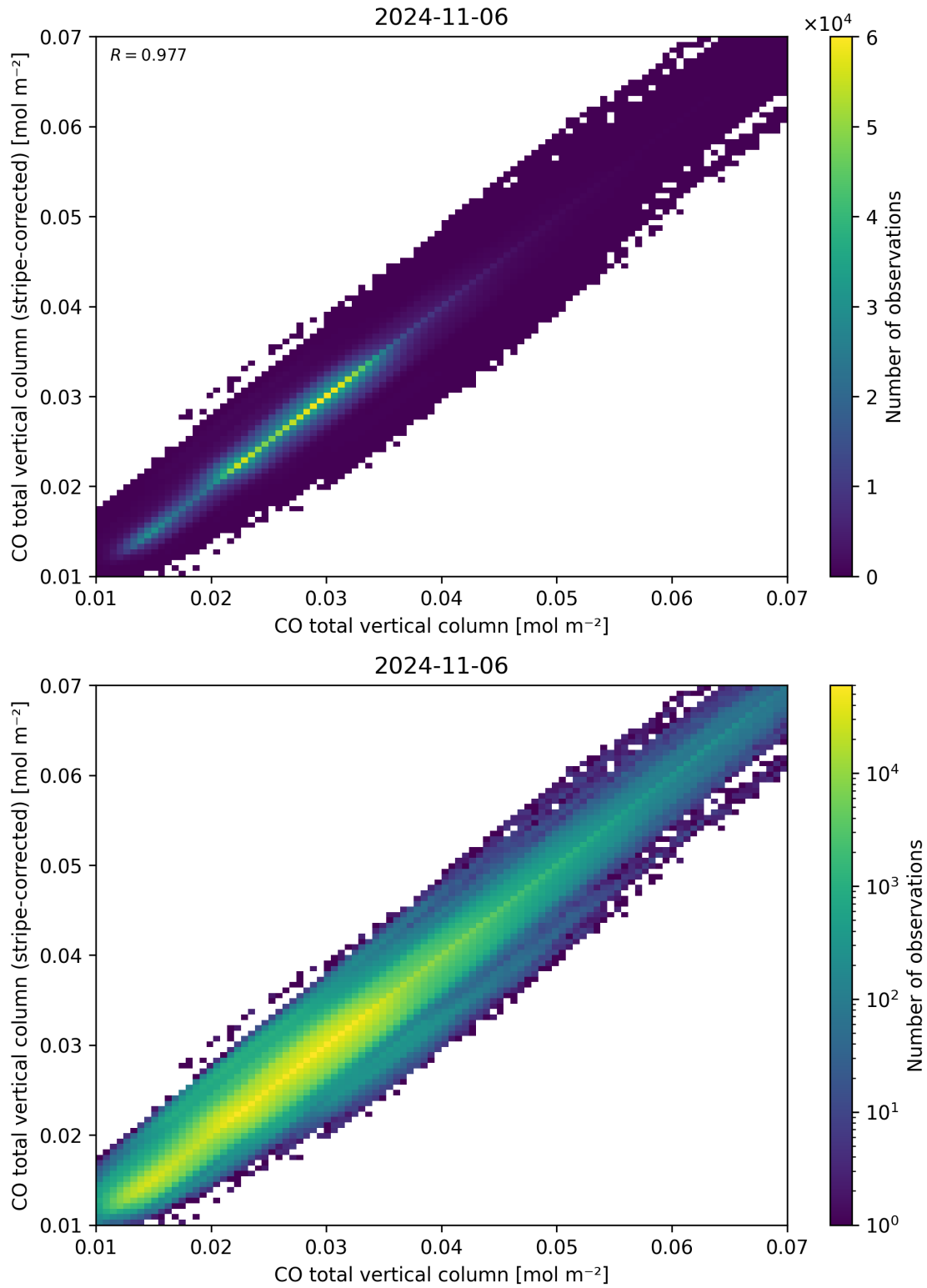
Figure 33: Scatter density plot of “CO total vertical column” against “CO total vertical column (stripe-corrected)” for 2024-11-05 to 2024-11-07.
