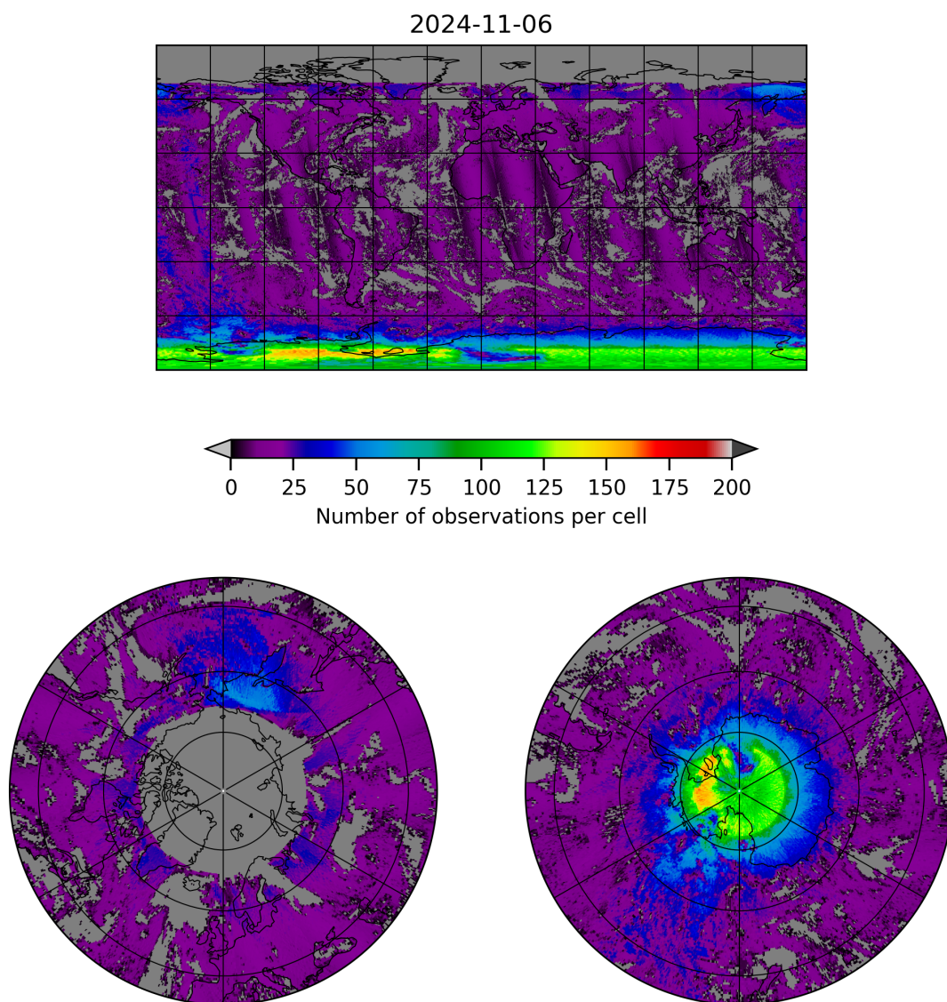
Figure 8: Map of the number of observations for 2024-11-05 to 2024-11-07
