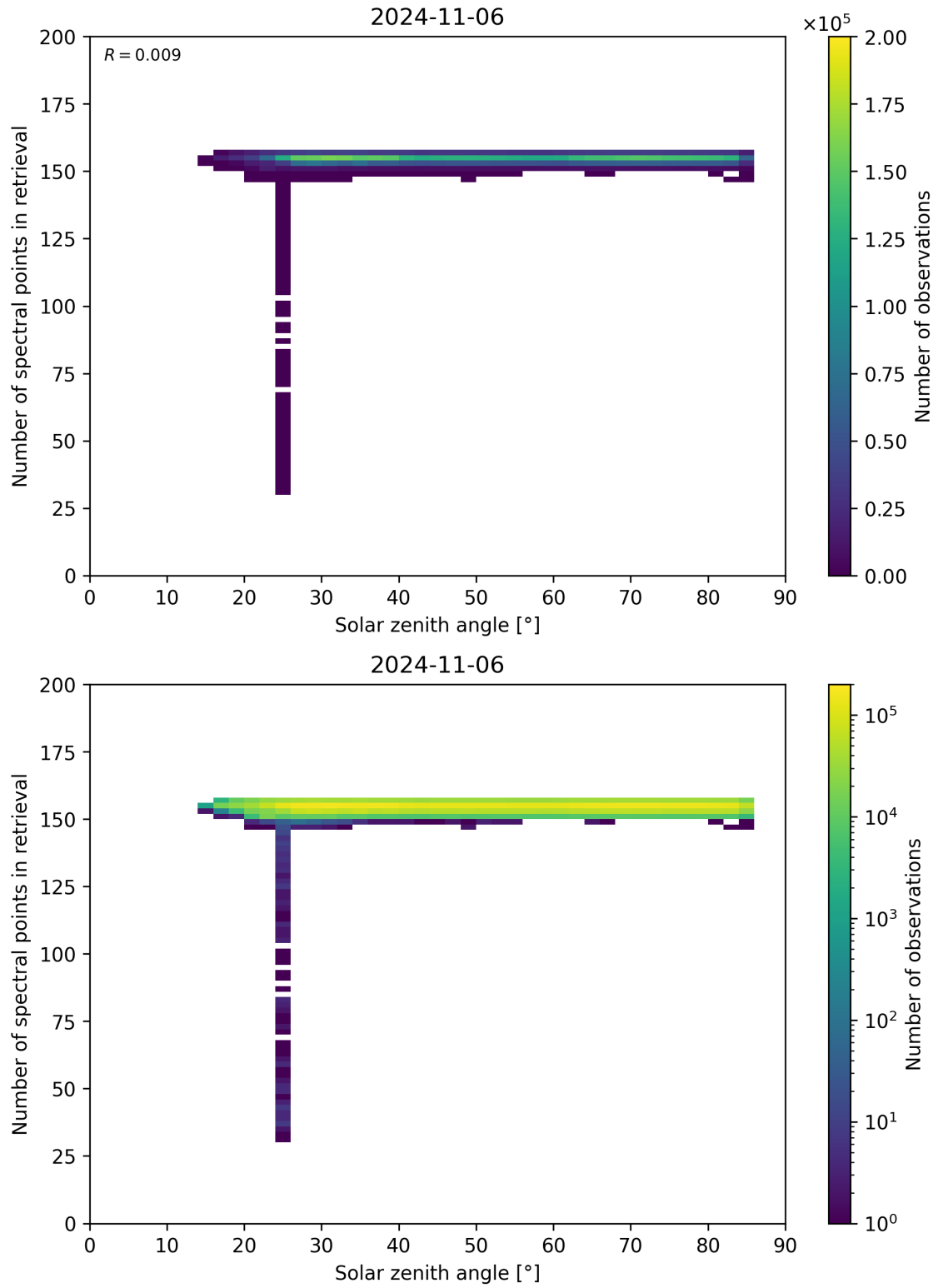
Figure 68: Scatter density plot of “Solar zenith angle” against “Number of spectral points in retrieval” for 2024-11-05 to 2024-11-07.
