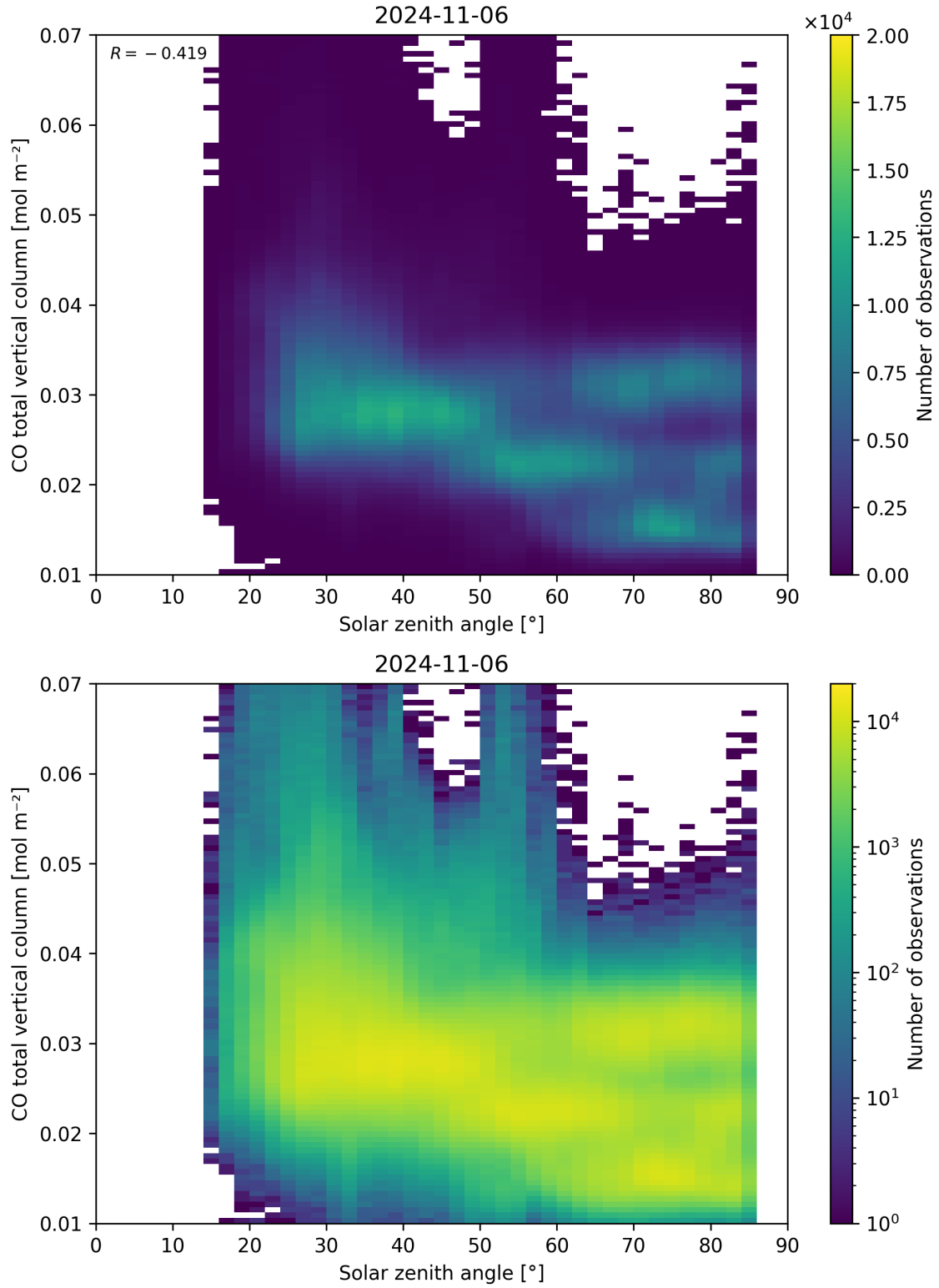
Figure 61: Scatter density plot of “Solar zenith angle” against “CO total vertical column” for 2024-11-05 to 2024-11-07.
