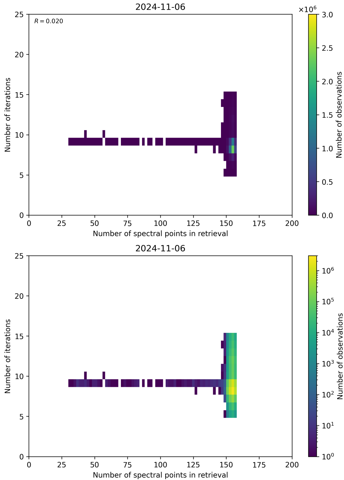
Figure 60: Scatter density plot of “Number of spectral points in retrieval” against “Number of iterations” for 2024-11-05 to 2024-11-07.
