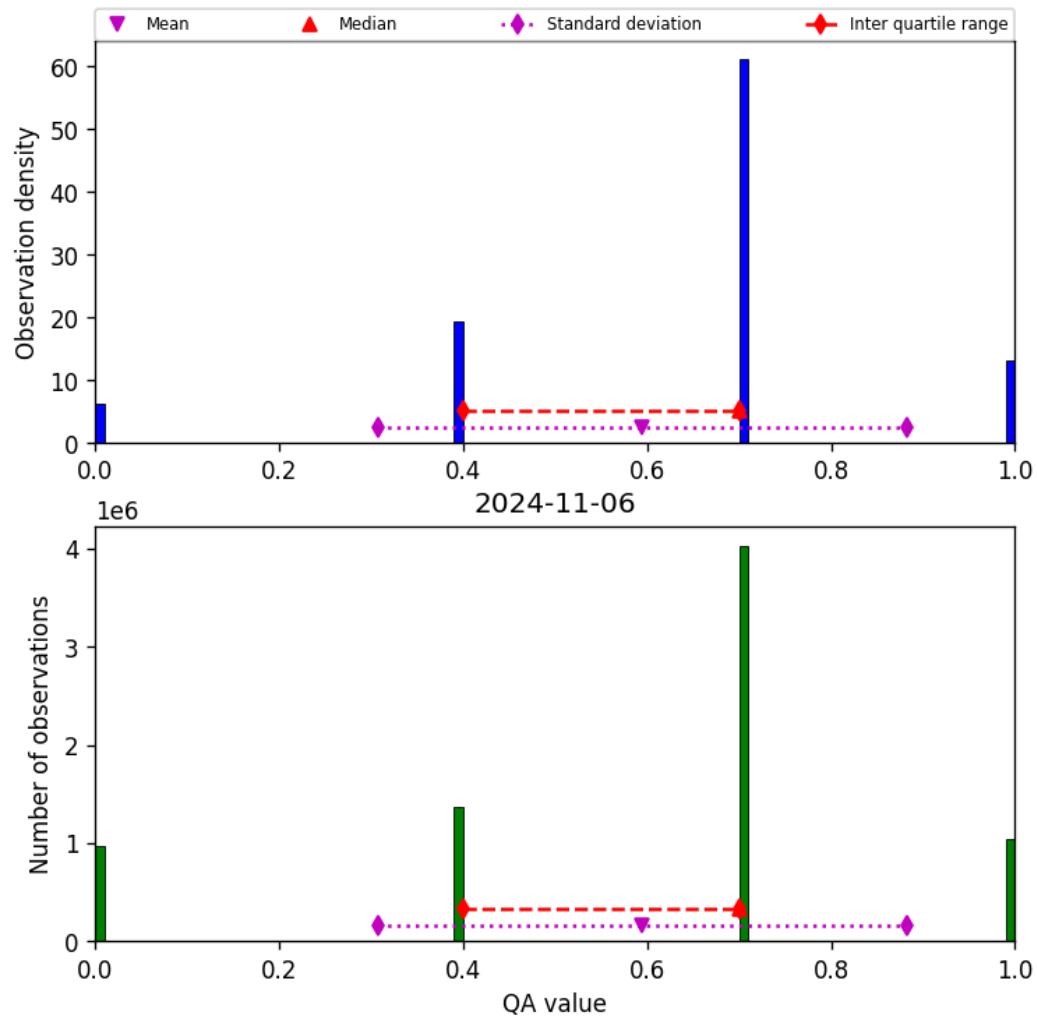
Figure 17: Histogram of “QA value” for 2024-11-05 to 2024-11-07
