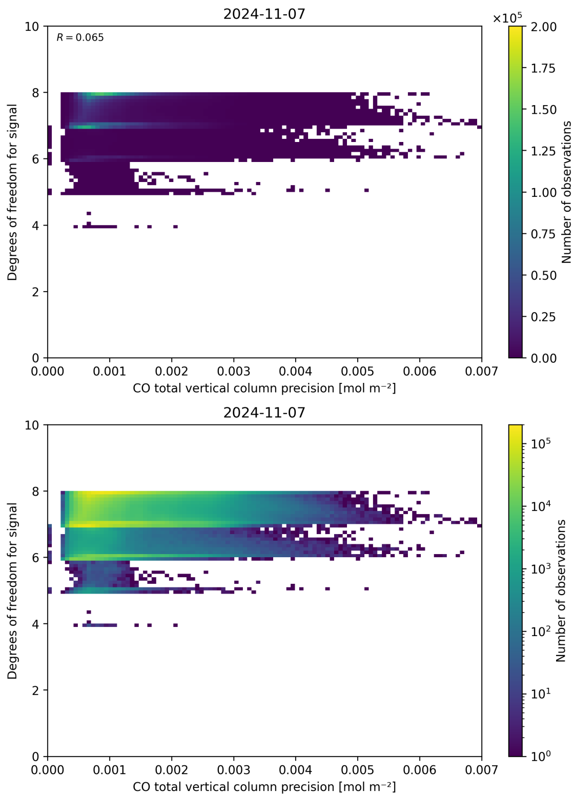
Figure 45: Scatter density plot of “CO total vertical column precision” against “Degrees of freedom for signal” for 2024-11-06 to 2024-11-08.
