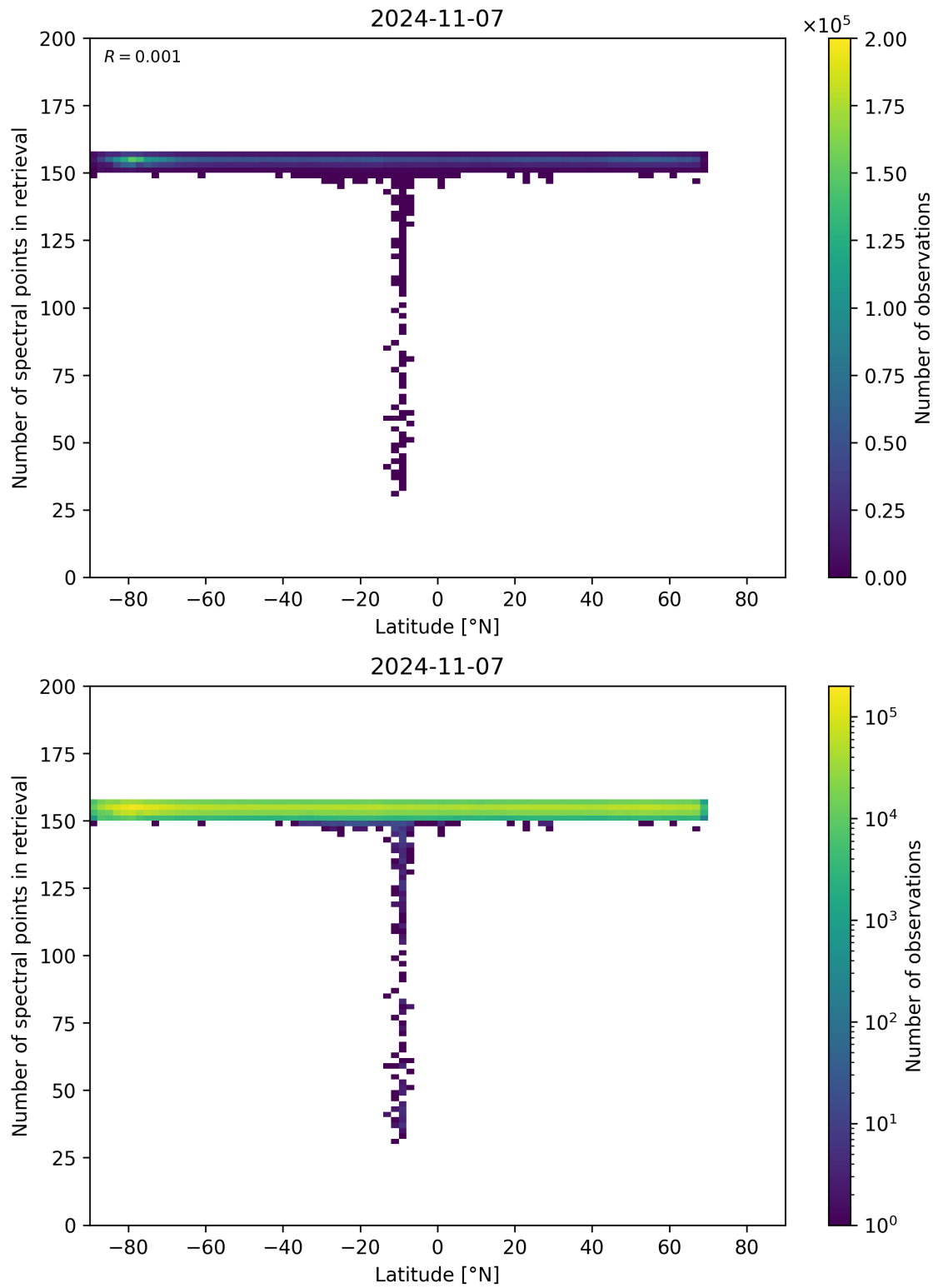
Figure 57: Scatter density plot of “Latitude” against “Number of spectral points in retrieval” for 2024-11-06 to 2024-11-08.
