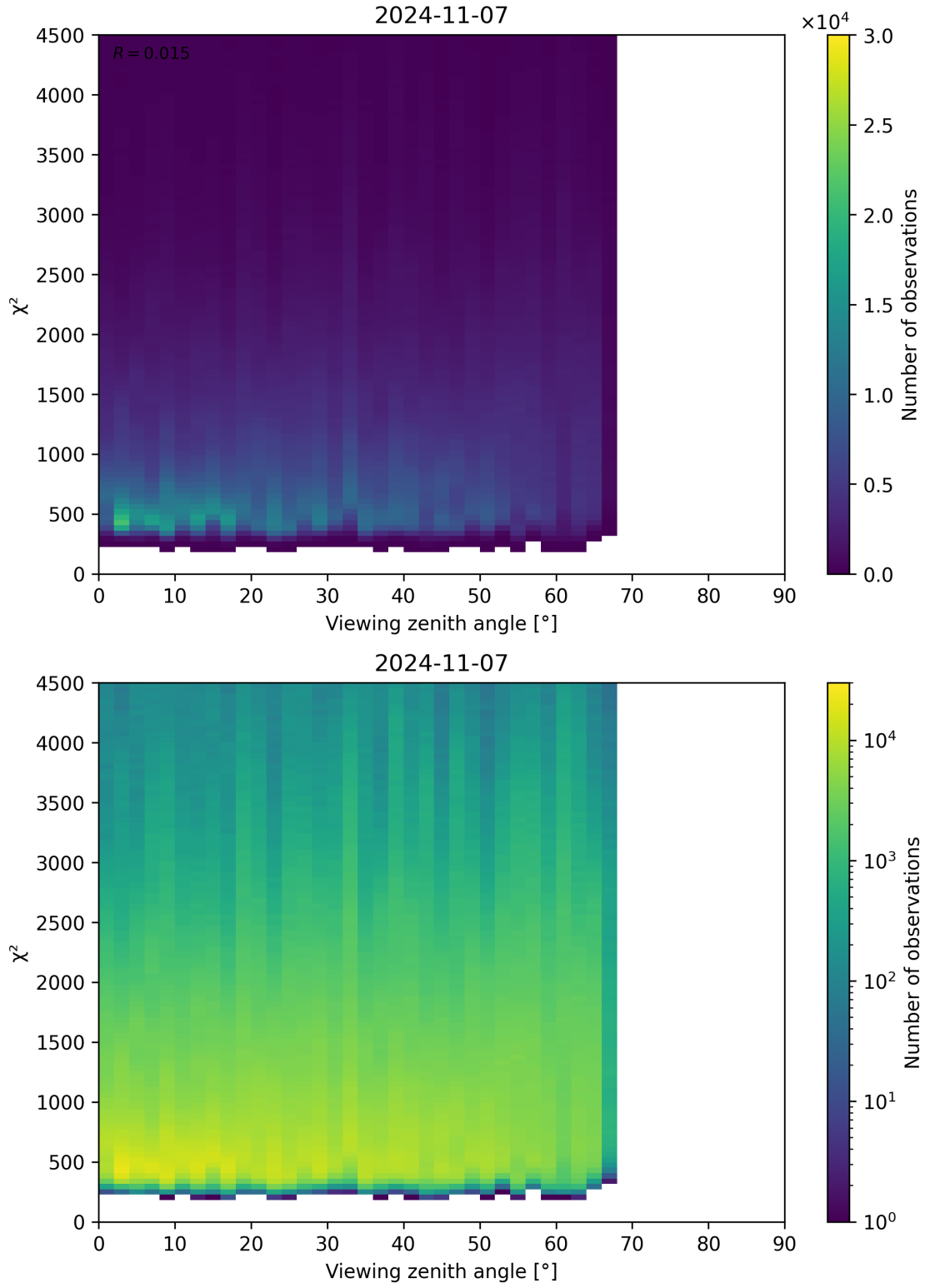
Figure 72: Scatter density plot of “Viewing zenith angle” against “ \chi^2 ” for 2024-11-06 to 2024-11-08.
