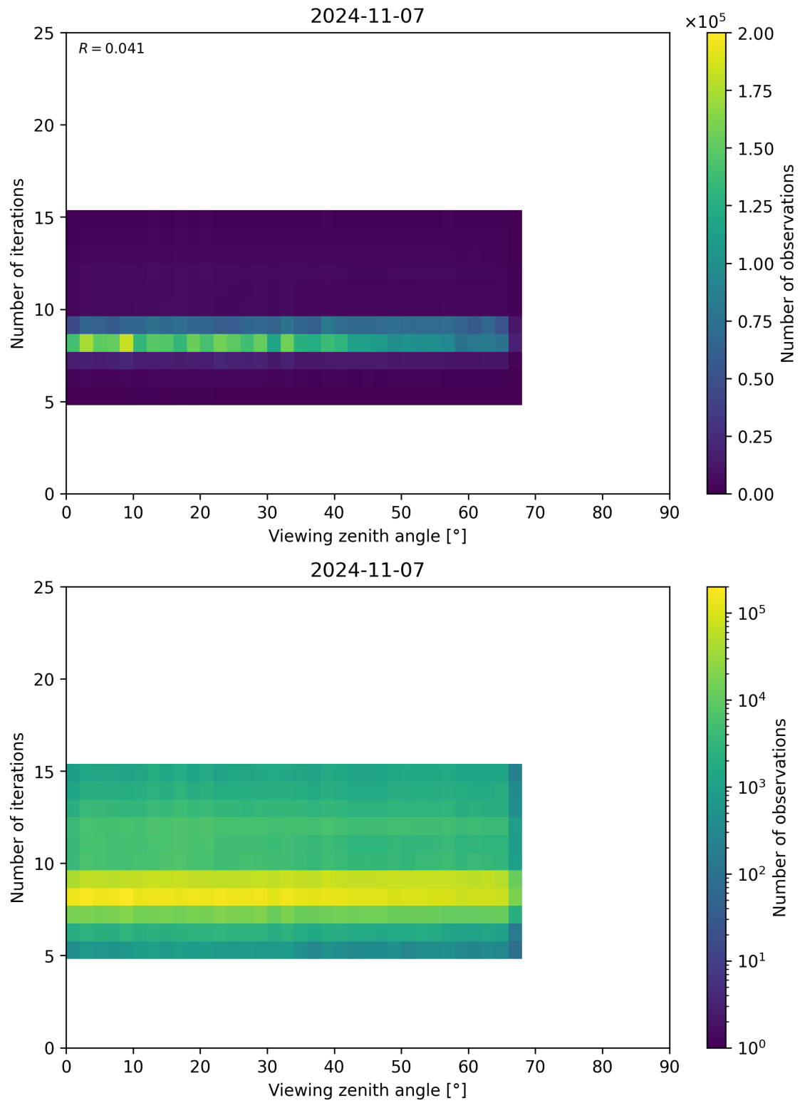
Figure 75: Scatter density plot of “Viewing zenith angle” against “Number of iterations” for 2024-11-06 to 2024-11-08.
