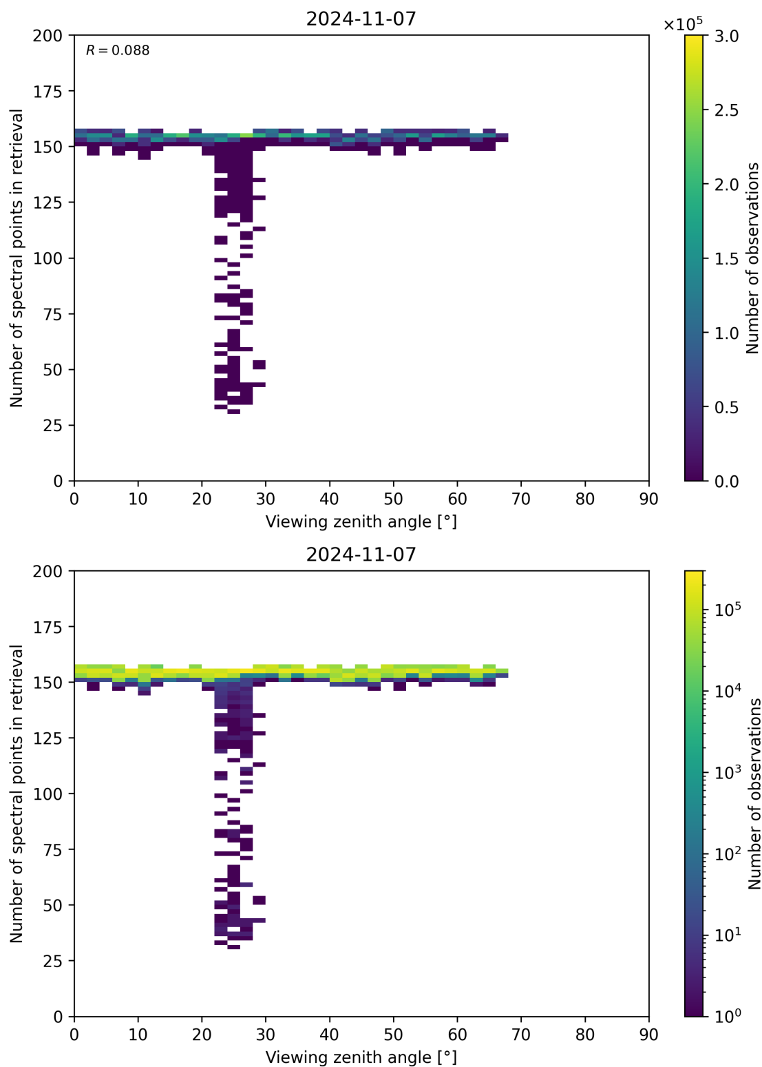
Figure 76: Scatter density plot of “Viewing zenith angle” against “Number of spectral points in retrieval” for 2024-11-06 to 2024-11-08.
