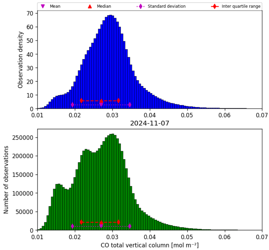
Figure 18: Histogram of “CO total vertical column” for 2024-11-06 to 2024-11-08
