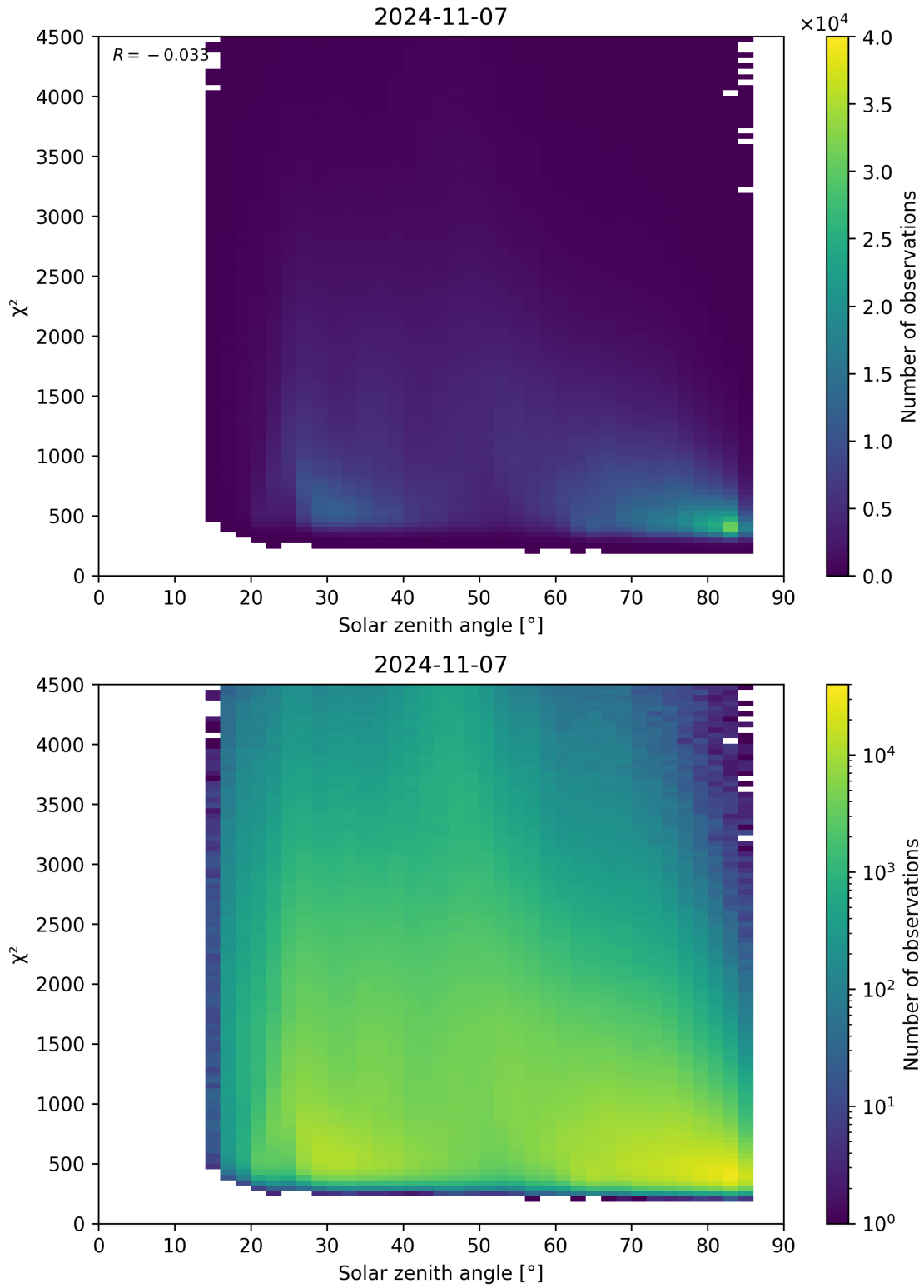
Figure 64: Scatter density plot of “Solar zenith angle” against “ \chi^2 ” for 2024-11-06 to 2024-11-08.
