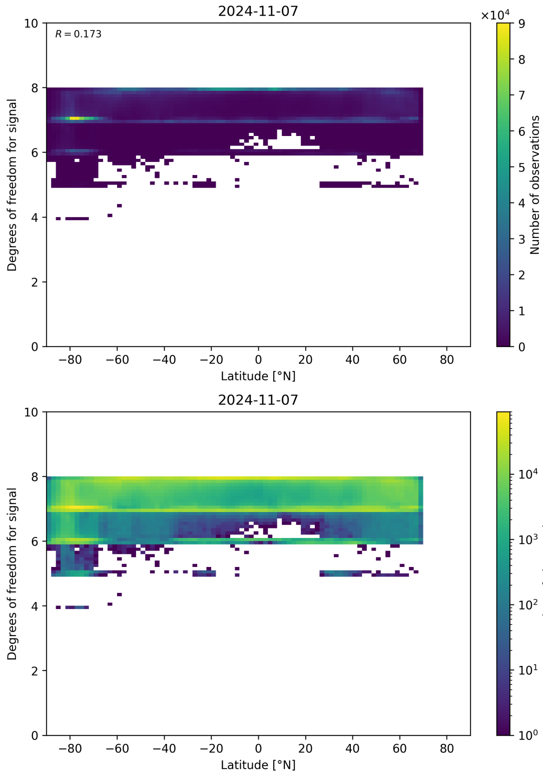
Figure 55: Scatter density plot of “Latitude” against “Degrees of freedom for signal” for 2024-11-06 to 2024-11-08.
