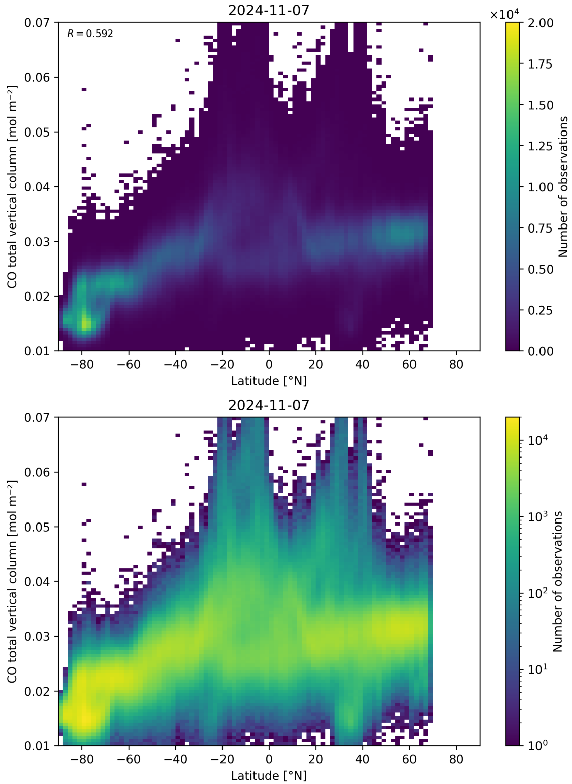
Figure 51: Scatter density plot of “Latitude” against “CO total vertical column” for 2024-11-06 to 2024-11-08.
