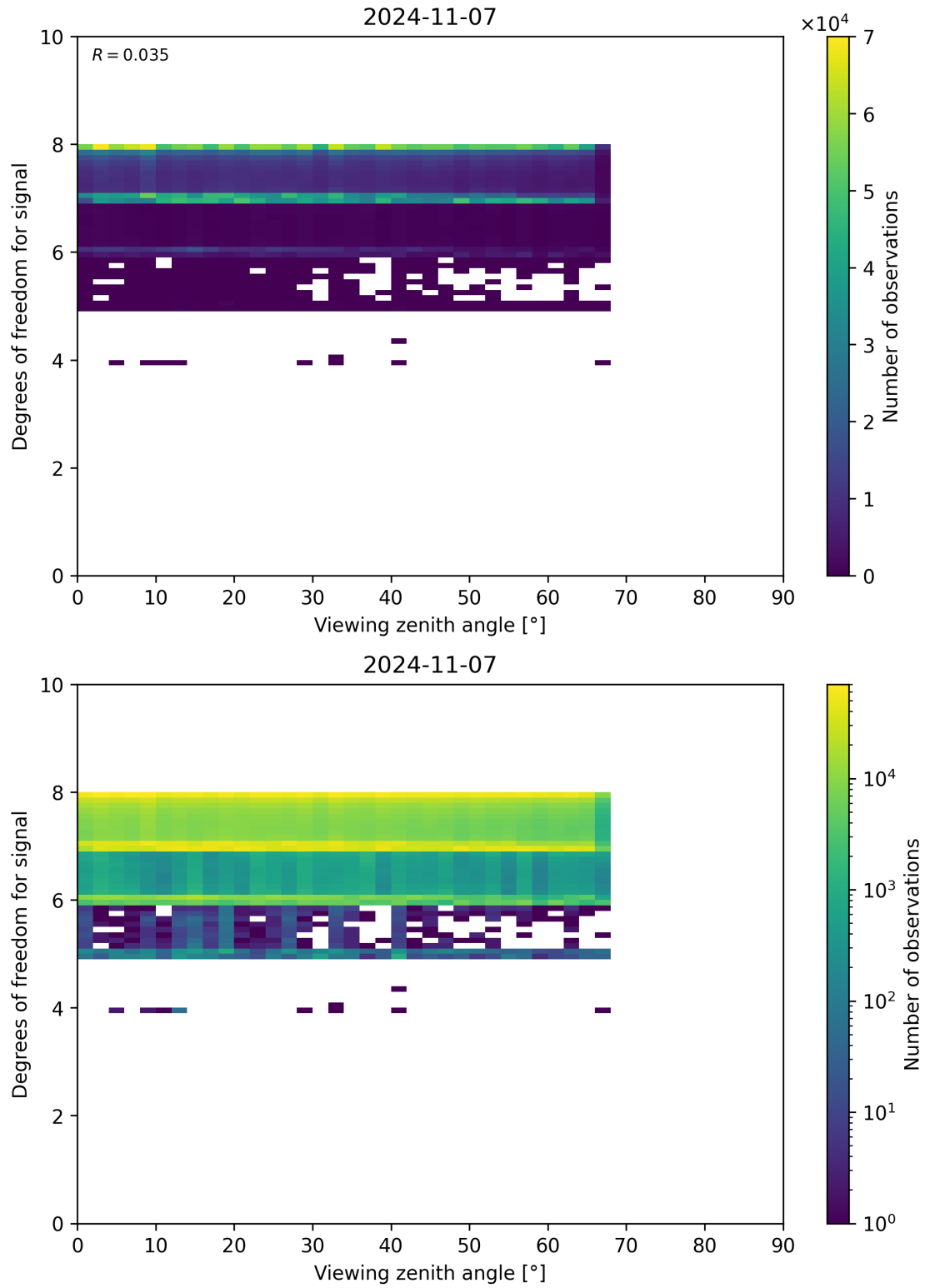
Figure 73: Scatter density plot of “Viewing zenith angle” against “Degrees of freedom for signal” for 2024-11-06 to 2024-11-08.
