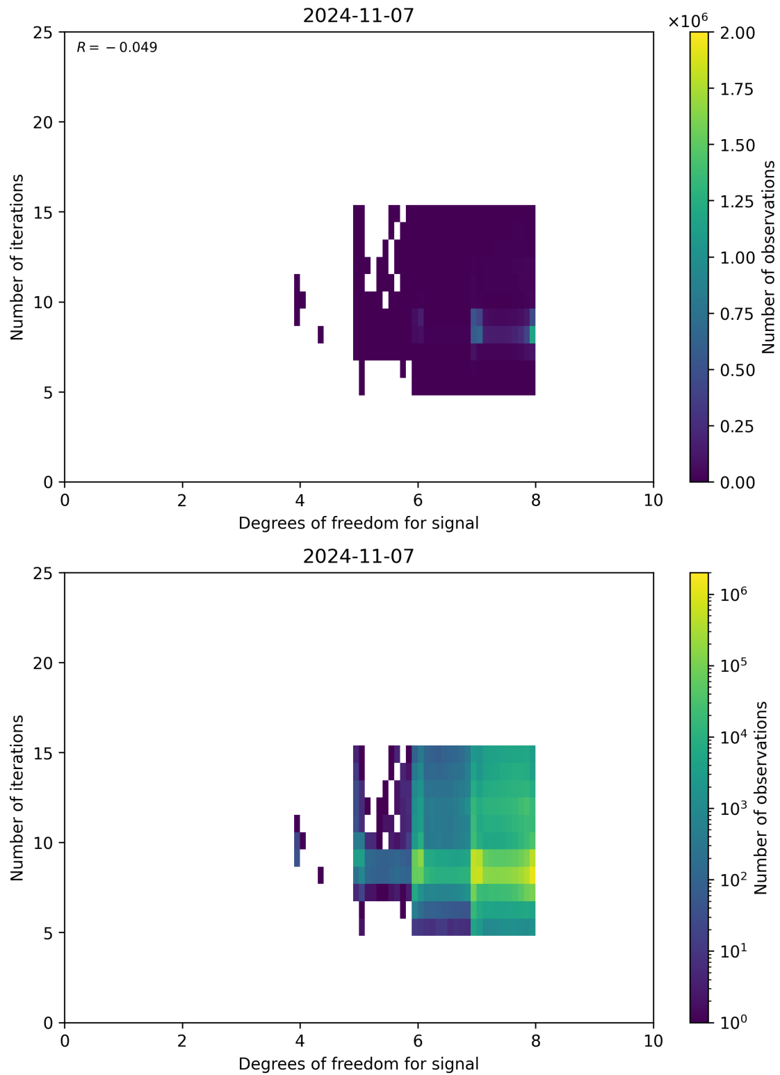
Figure 50: Scatter density plot of “Degrees of freedom for signal” against “Number of iterations” for 2024-11-06 to 2024-11-08.
