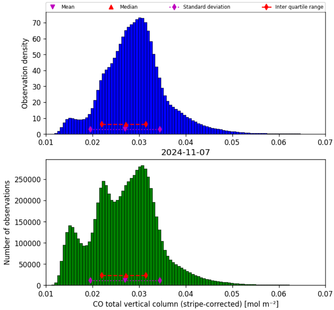
Figure 19: Histogram of “CO total vertical column (stripe-corrected)” for 2024-11-06 to 2024-11-08
