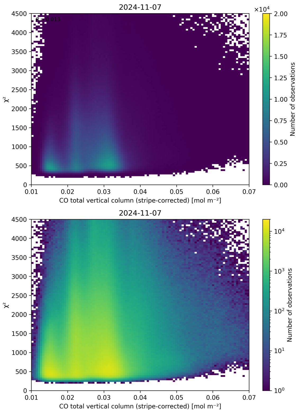
Figure 37: Scatter density plot of “CO total vertical column (stripe-corrected)” against “ \chi^2 ” for 2024-11-06 to 2024-11-08.
