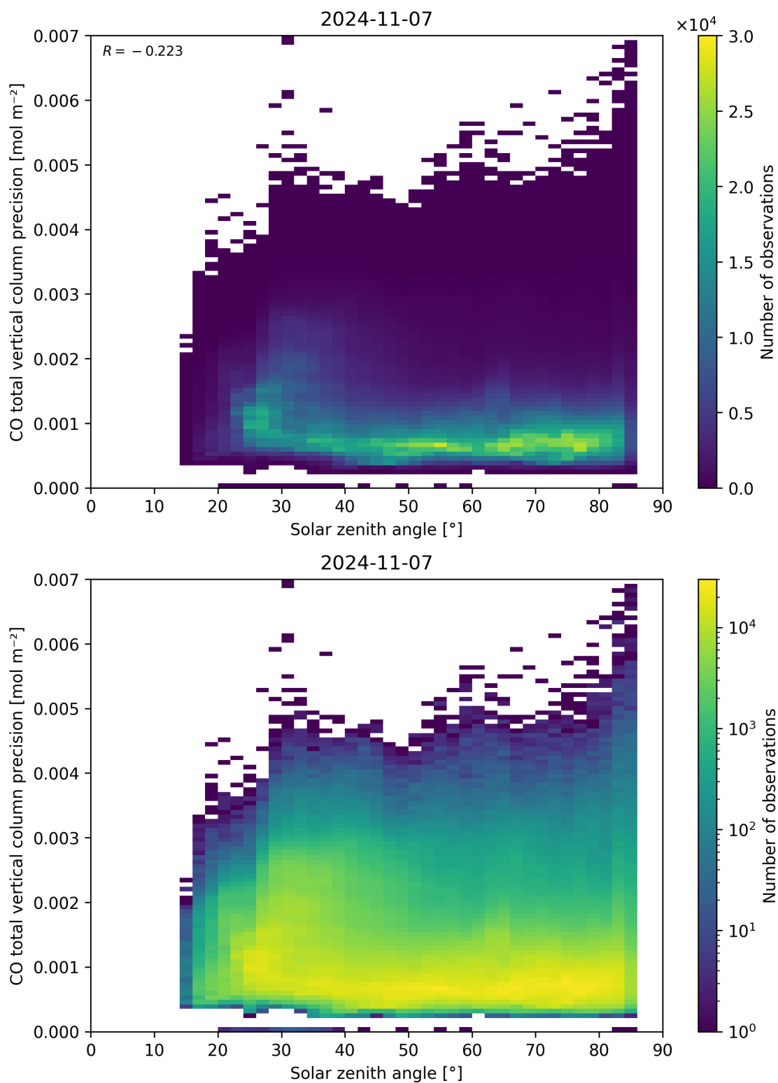
Figure 63: Scatter density plot of “Solar zenith angle” against “CO total vertical column precision” for 2024-11-06 to 2024-11-08.
