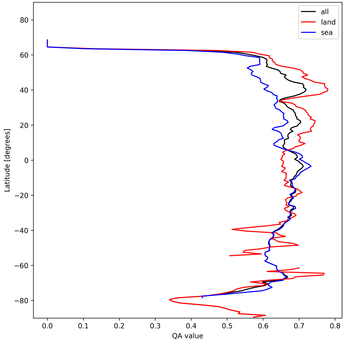
Figure 9: Zonal average of “QA value” for 2024-11-06 to 2024-11-08.
