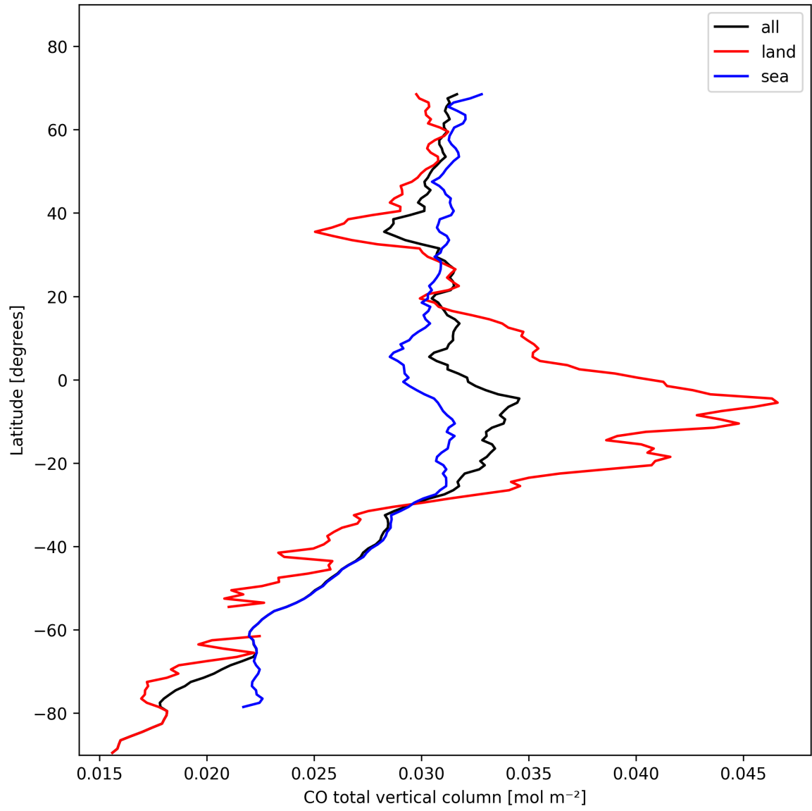
Figure 10: Zonal average of “CO total vertical column” for 2024-11-06 to 2024-11-08.
