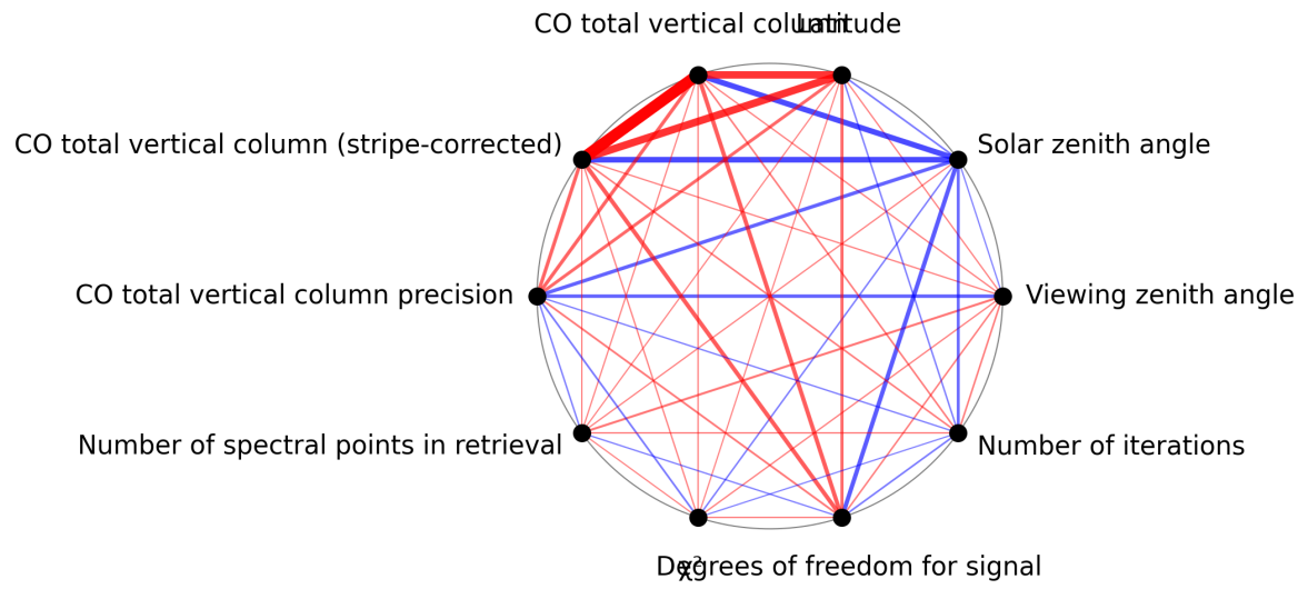
Figure 1: Map of correlation graph for 2024-11-06 to 2024-11-08.
