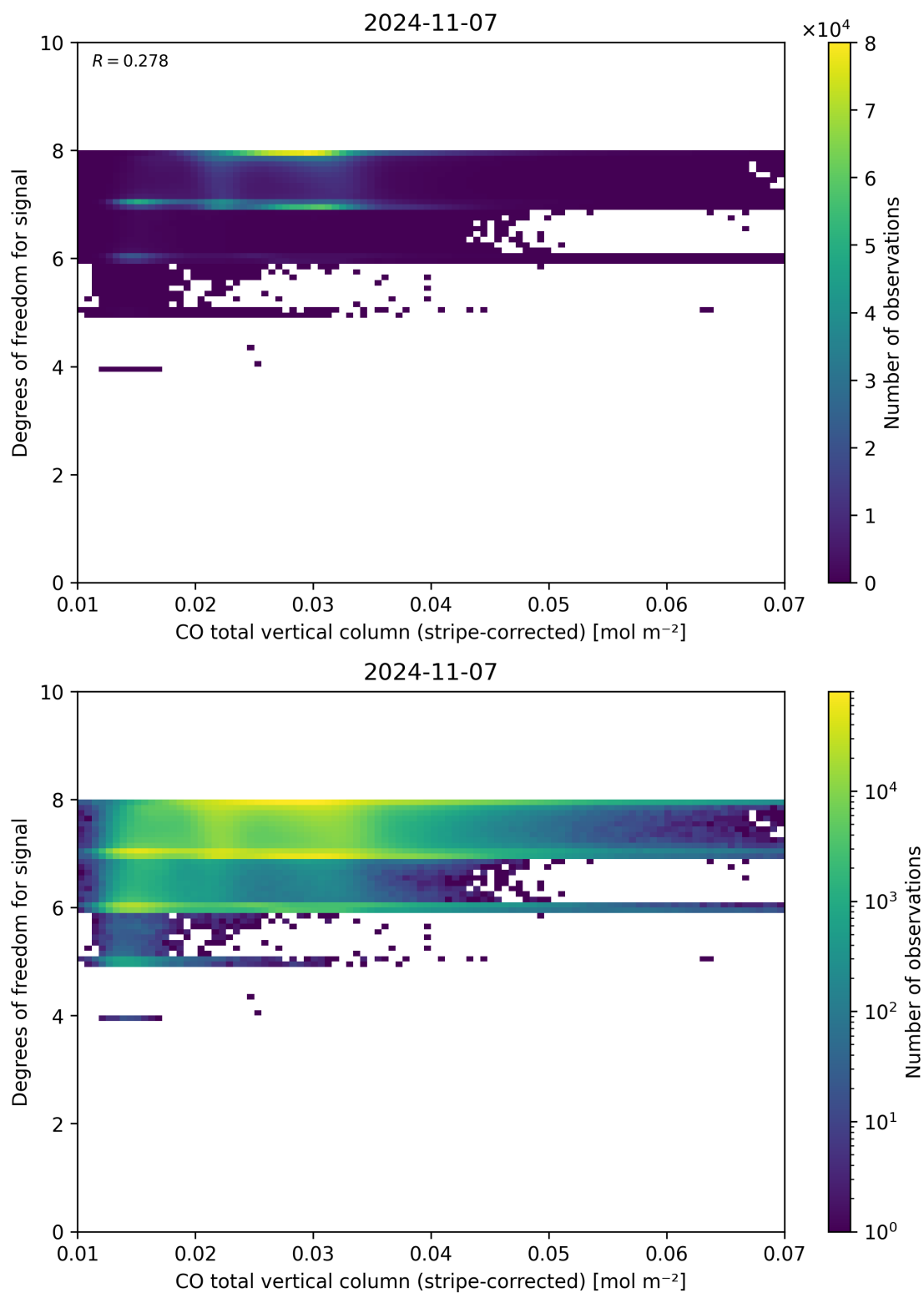
Figure 38: Scatter density plot of “CO total vertical column (stripe-corrected)” against “Degrees of freedom for signal” for 2024-11-06 to 2024-11-08.
