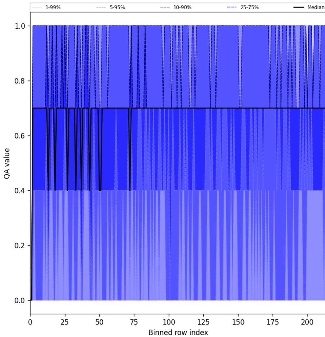
Figure 25: Along track statistics of “QA value” for 2024-11-06 to 2024-11-08
