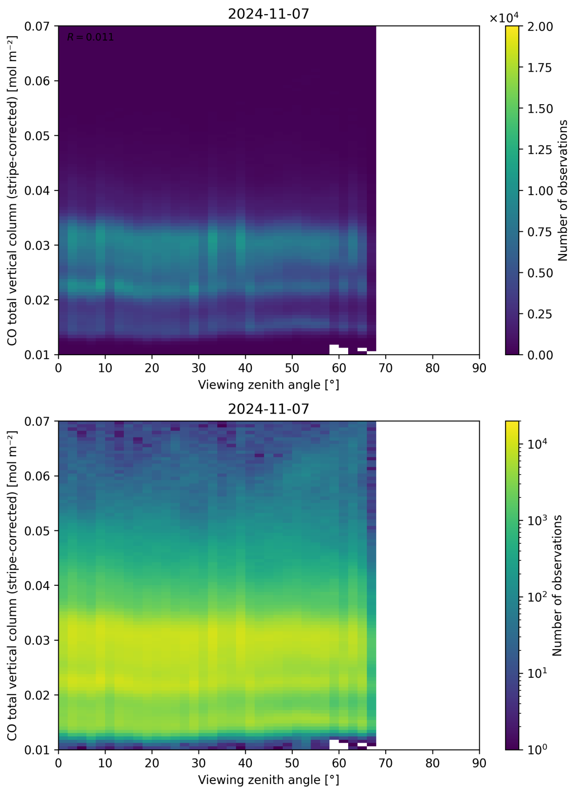
Figure 70: Scatter density plot of “Viewing zenith angle” against “CO total vertical column (stripe-corrected)” for 2024-11-06 to 2024-11-08.
