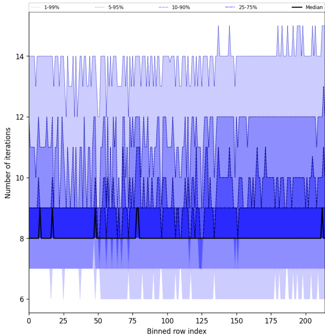
Figure 32: Along track statistics of “Number of iterations” for 2024-11-06 to 2024-11-08
