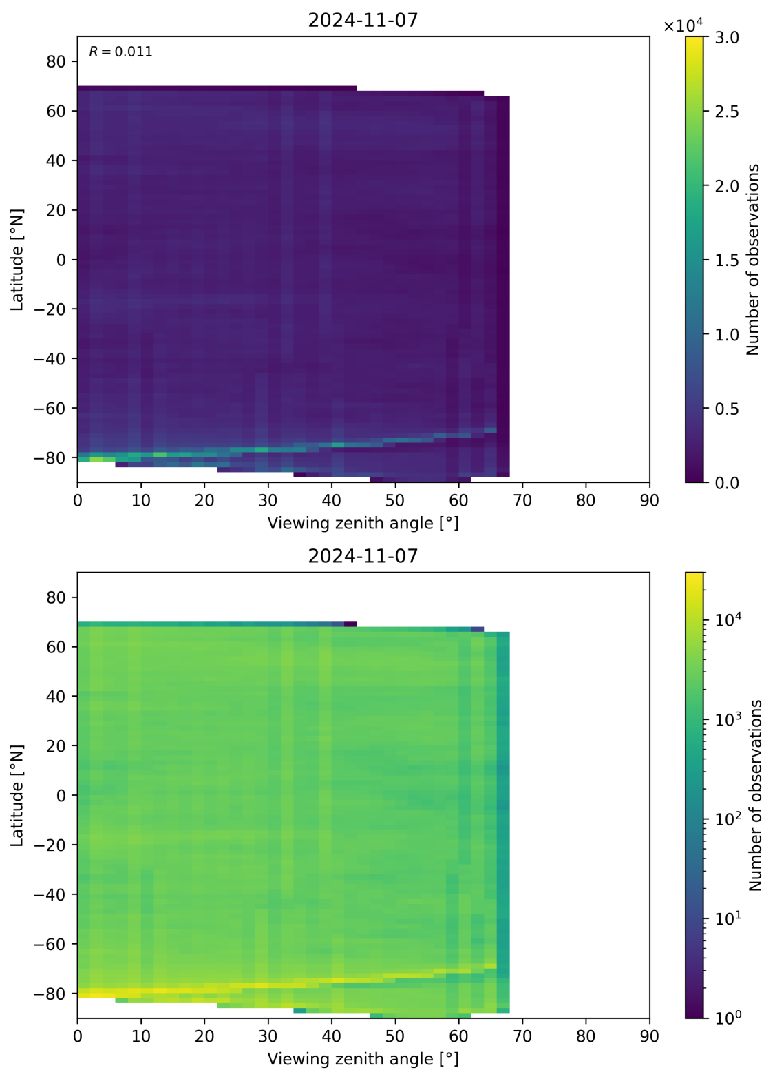
Figure 74: Scatter density plot of “Viewing zenith angle” against “Latitude” for 2024-11-06 to 2024-11-08.
