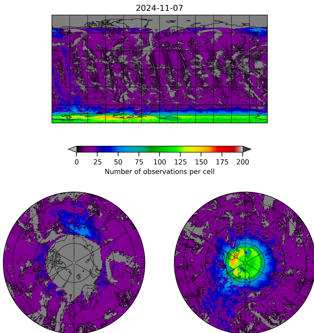
Figure 8: Map of the number of observations for 2024-11-06 to 2024-11-08
