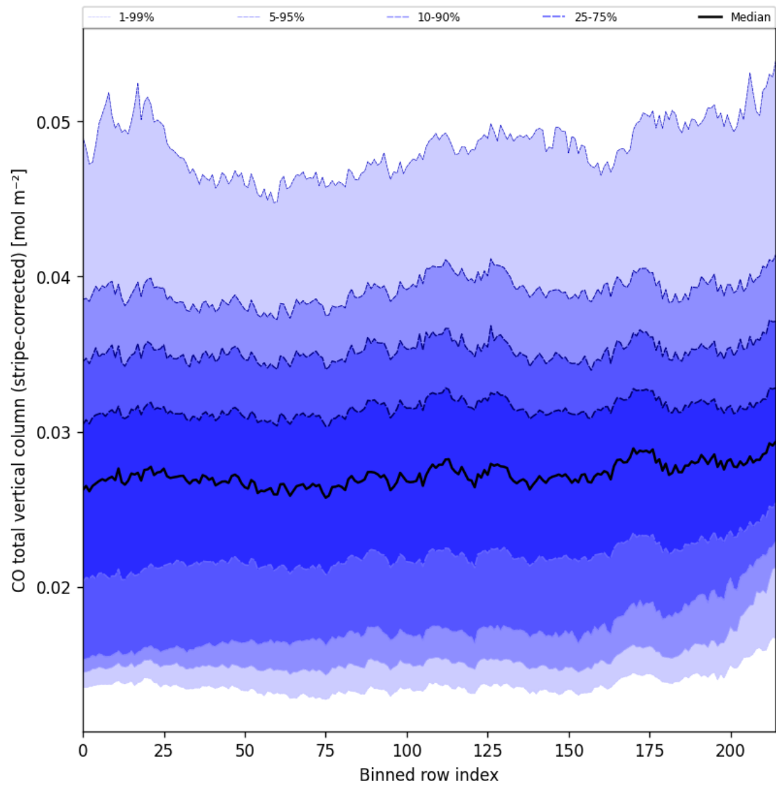
Figure 27: Along track statistics of “CO total vertical column (stripe-corrected)” for 2024-11-06 to 2024-11-08
