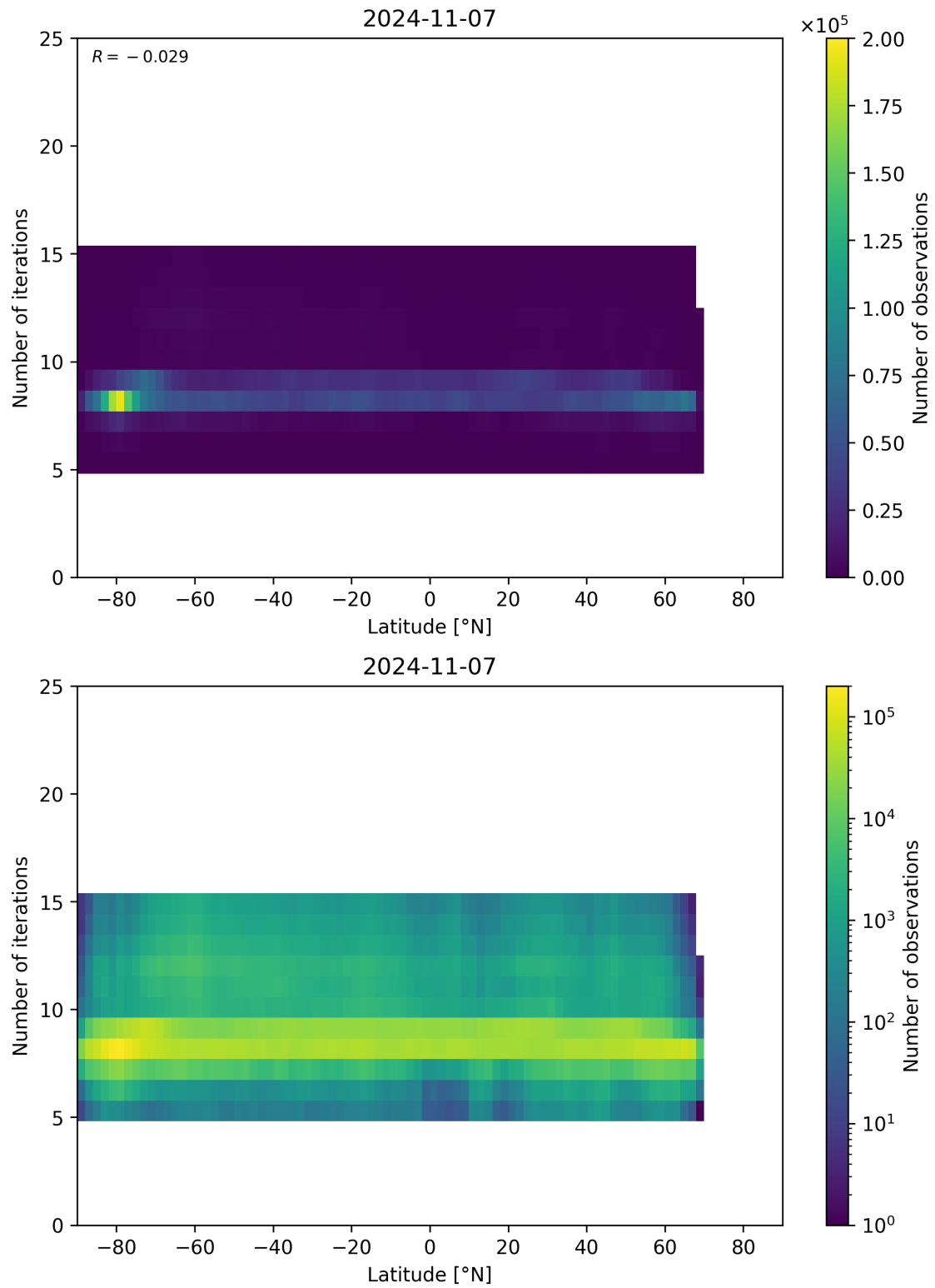
Figure 56: Scatter density plot of “Latitude” against “Number of iterations” for 2024-11-06 to 2024-11-08.
