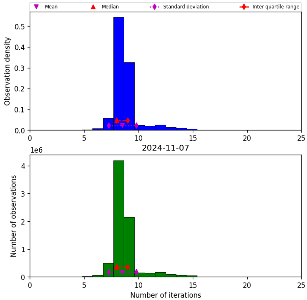
Figure 24: Histogram of “Number of iterations” for 2024-11-06 to 2024-11-08
