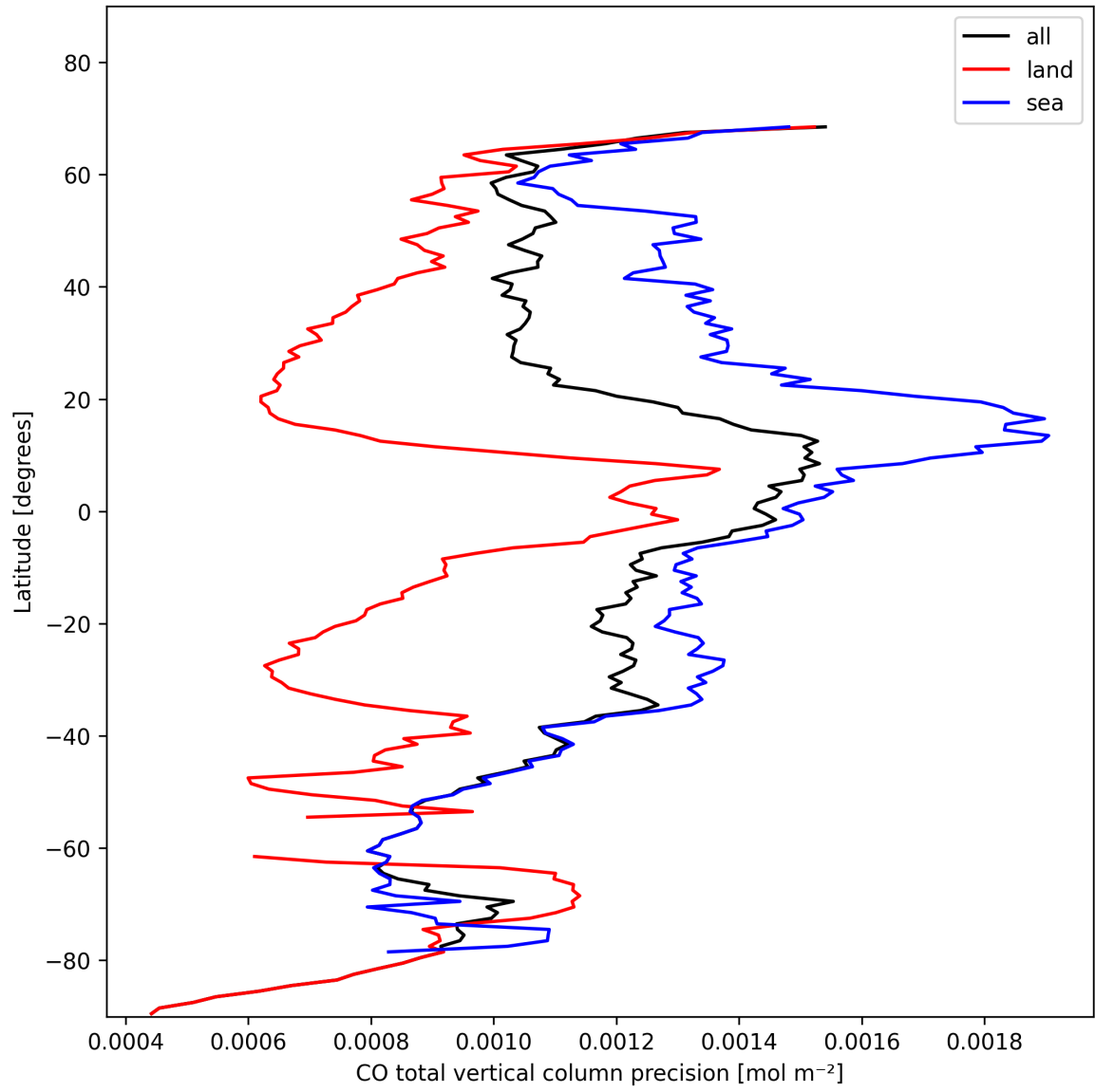
Figure 12: Zonal average of “CO total vertical column precision” for 2024-11-06 to 2024-11-08.
