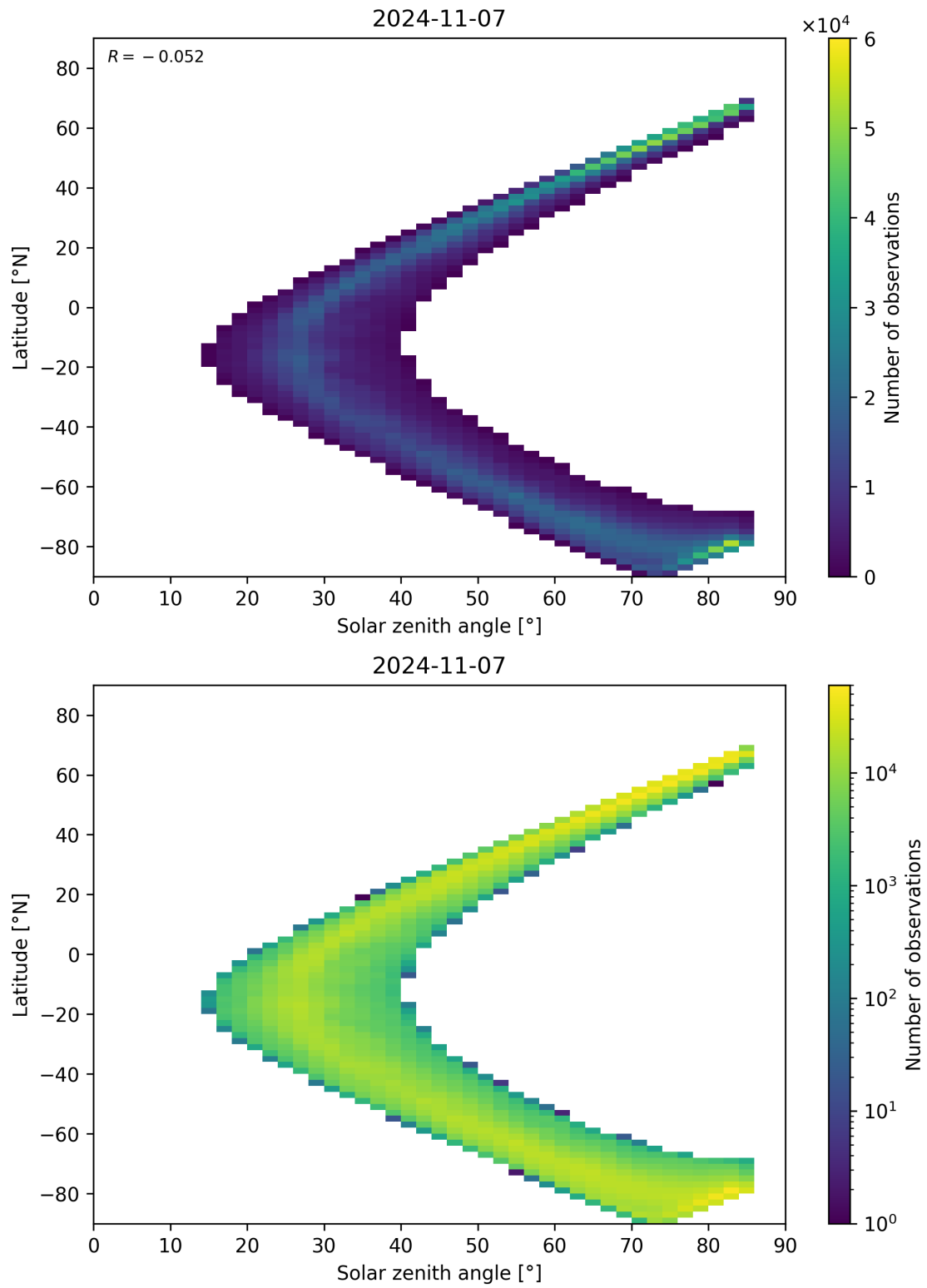
Figure 66: Scatter density plot of “Solar zenith angle” against “Latitude” for 2024-11-06 to 2024-11-08.
