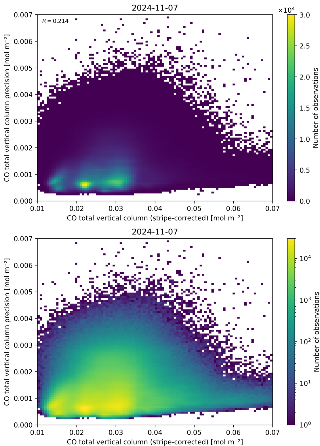
Figure 36: Scatter density plot of “CO total vertical column (stripe-corrected)” against “CO total vertical column precision” for 2024-11-06 to 2024-11-08.
