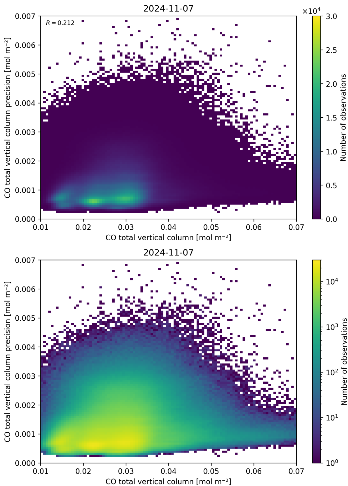
Figure 34: Scatter density plot of “CO total vertical column” against “CO total vertical column precision” for 2024-11-06 to 2024-11-08.
