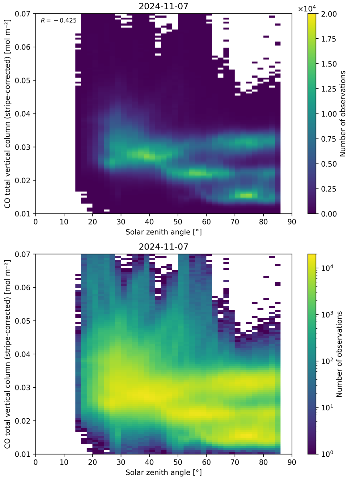
Figure 62: Scatter density plot of “Solar zenith angle” against “CO total vertical column (stripe-corrected)” for 2024-11-06 to 2024-11-08.
