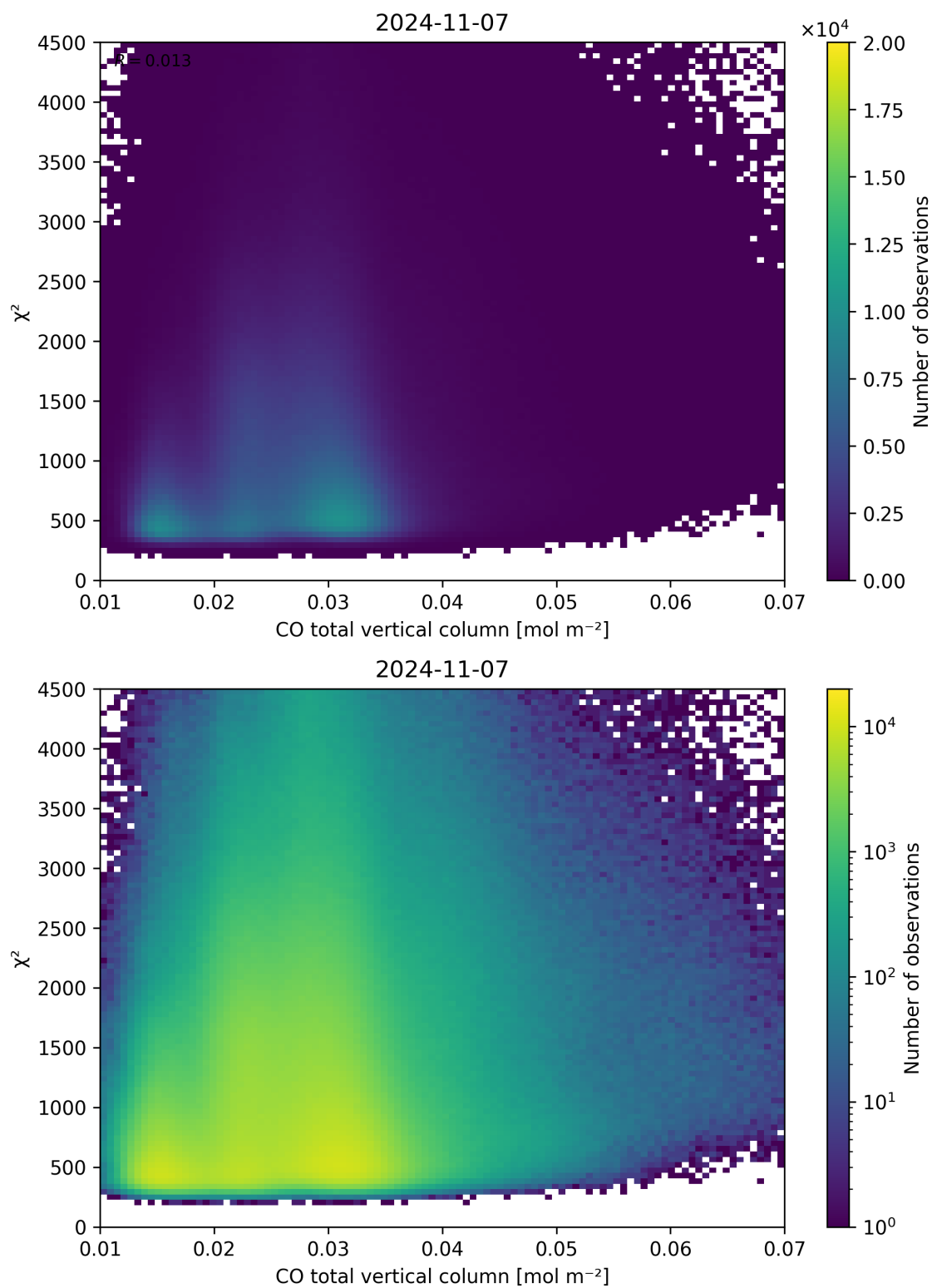
Figure 35: Scatter density plot of “CO total vertical column” against “ \chi^2 ” for 2024-11-06 to 2024-11-08.
