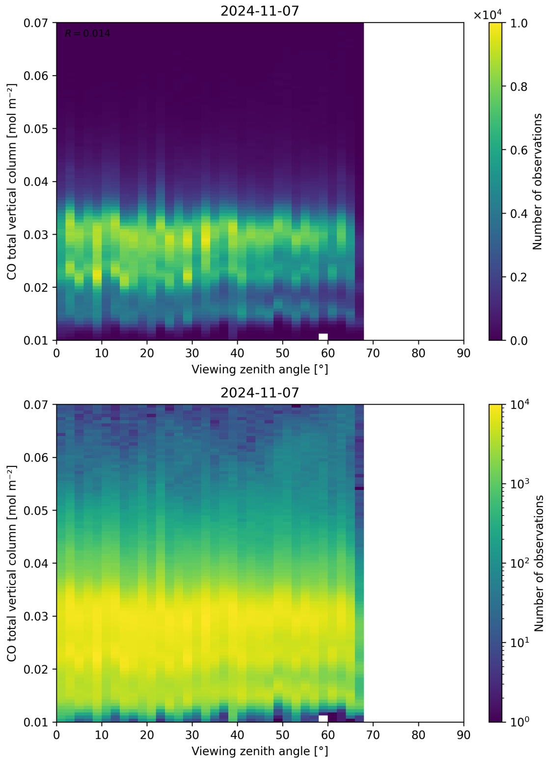
Figure 69: Scatter density plot of “Viewing zenith angle” against “CO total vertical column” for 2024-11-06 to 2024-11-08.
