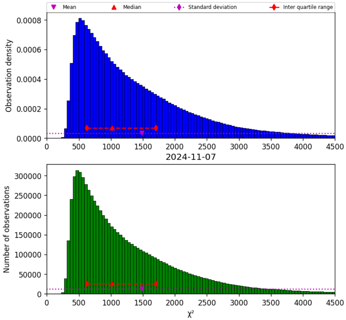
Figure 22: Histogram of " \chi^2 " for 2024-11-06 to 2024-11-08
