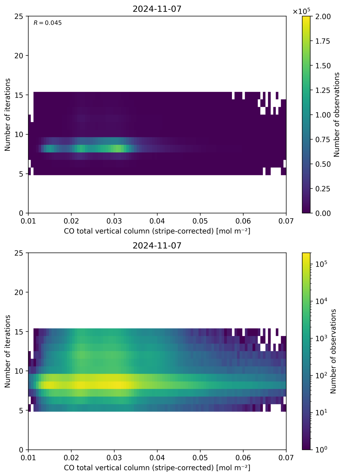
Figure 39: Scatter density plot of “CO total vertical column (stripe-corrected)” against “Number of iterations” for 2024-11-06 to 2024-11-08.
