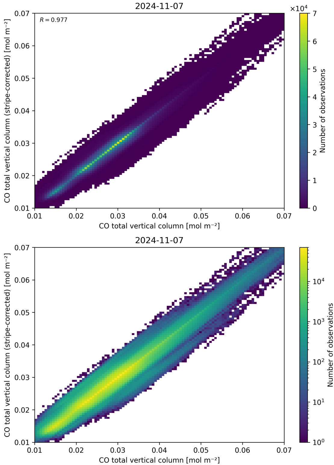
Figure 33: Scatter density plot of “CO total vertical column” against “CO total vertical column (stripe-corrected)” for 2024-11-06 to 2024-11-08.
