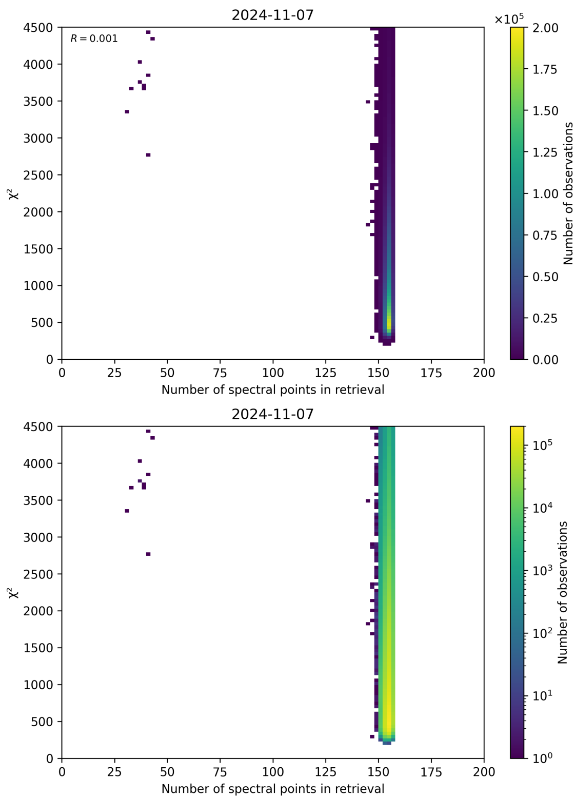
Figure 58: Scatter density plot of “Number of spectral points in retrieval” against “ \chi^2 ” for 2024-11-06 to 2024-11-08.
