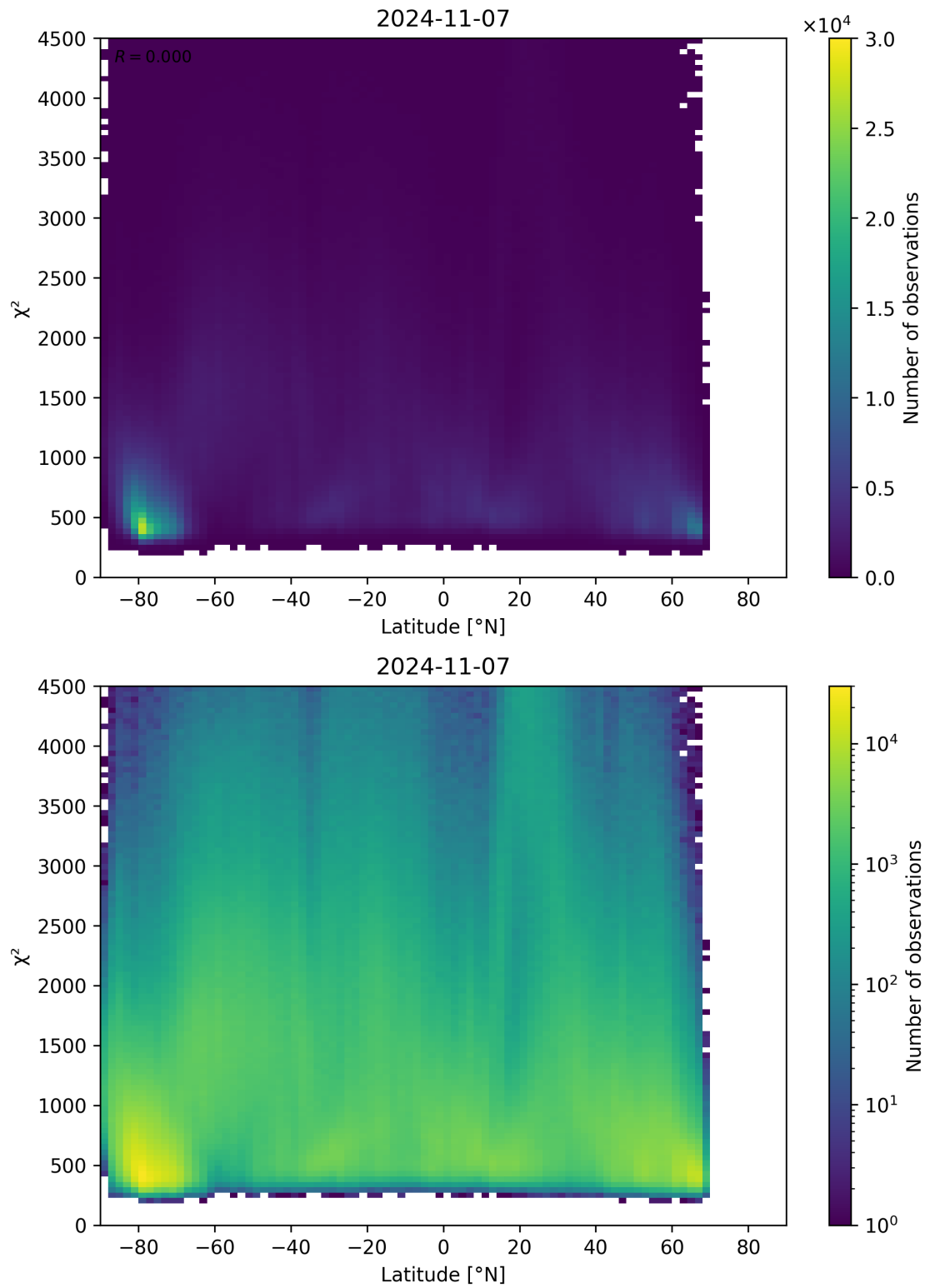
Figure 54: Scatter density plot of “Latitude” against “ \chi^2 ” for 2024-11-06 to 2024-11-08.
