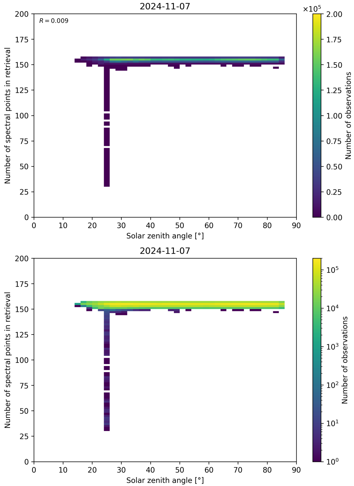
Figure 68: Scatter density plot of “Solar zenith angle” against “Number of spectral points in retrieval” for 2024-11-06 to 2024-11-08.
