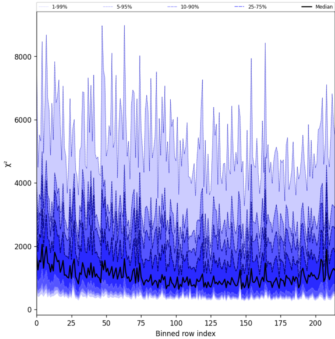
Figure 30: Along track statistics of “ \chi^2 ” for 2024-11-06 to 2024-11-08
