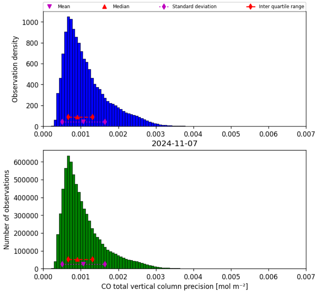
Figure 20: Histogram of “CO total vertical column precision” for 2024-11-06 to 2024-11-08
