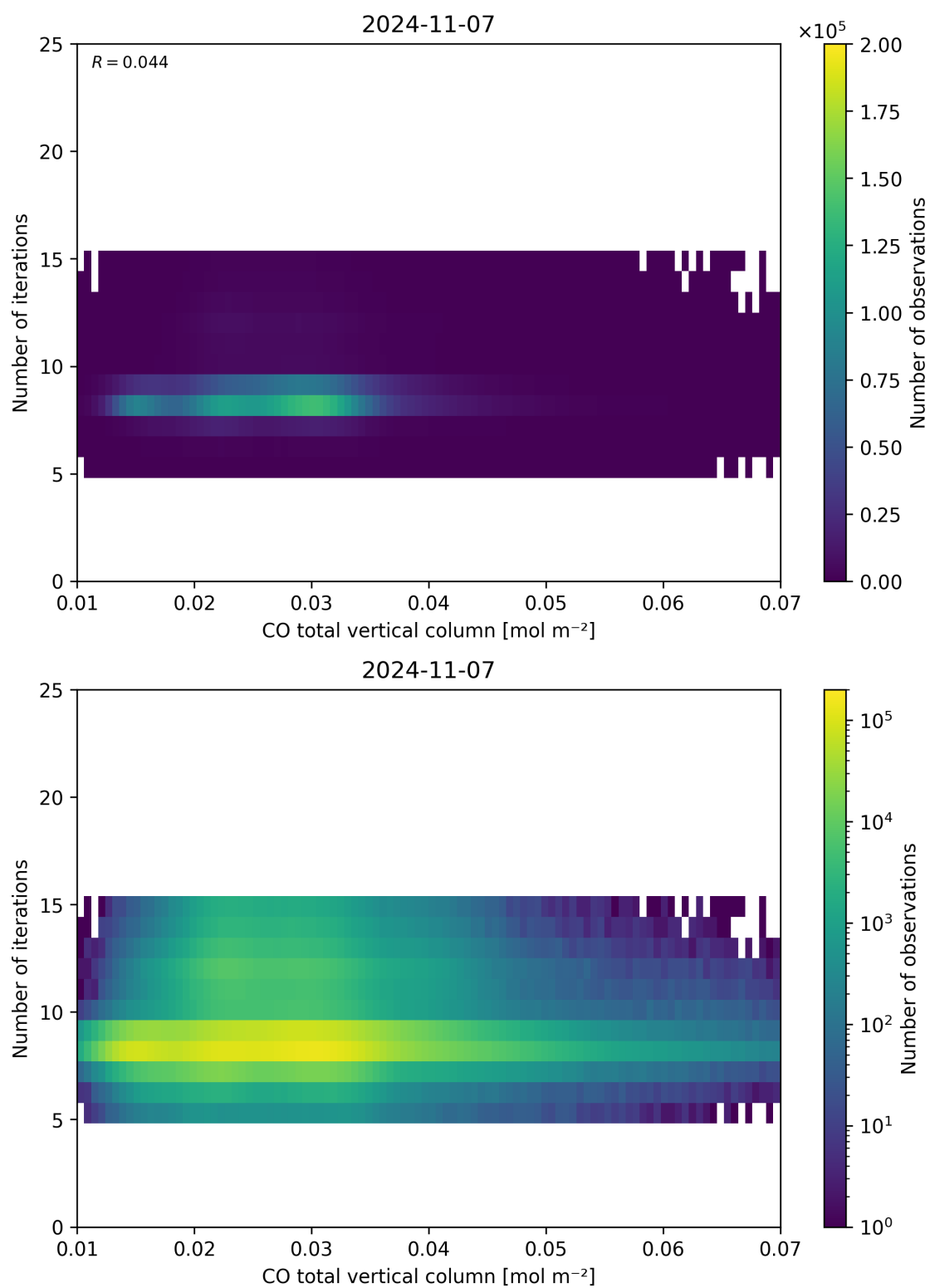
Figure 42: Scatter density plot of “CO total vertical column” against “Number of iterations” for 2024-11-06 to 2024-11-08.
