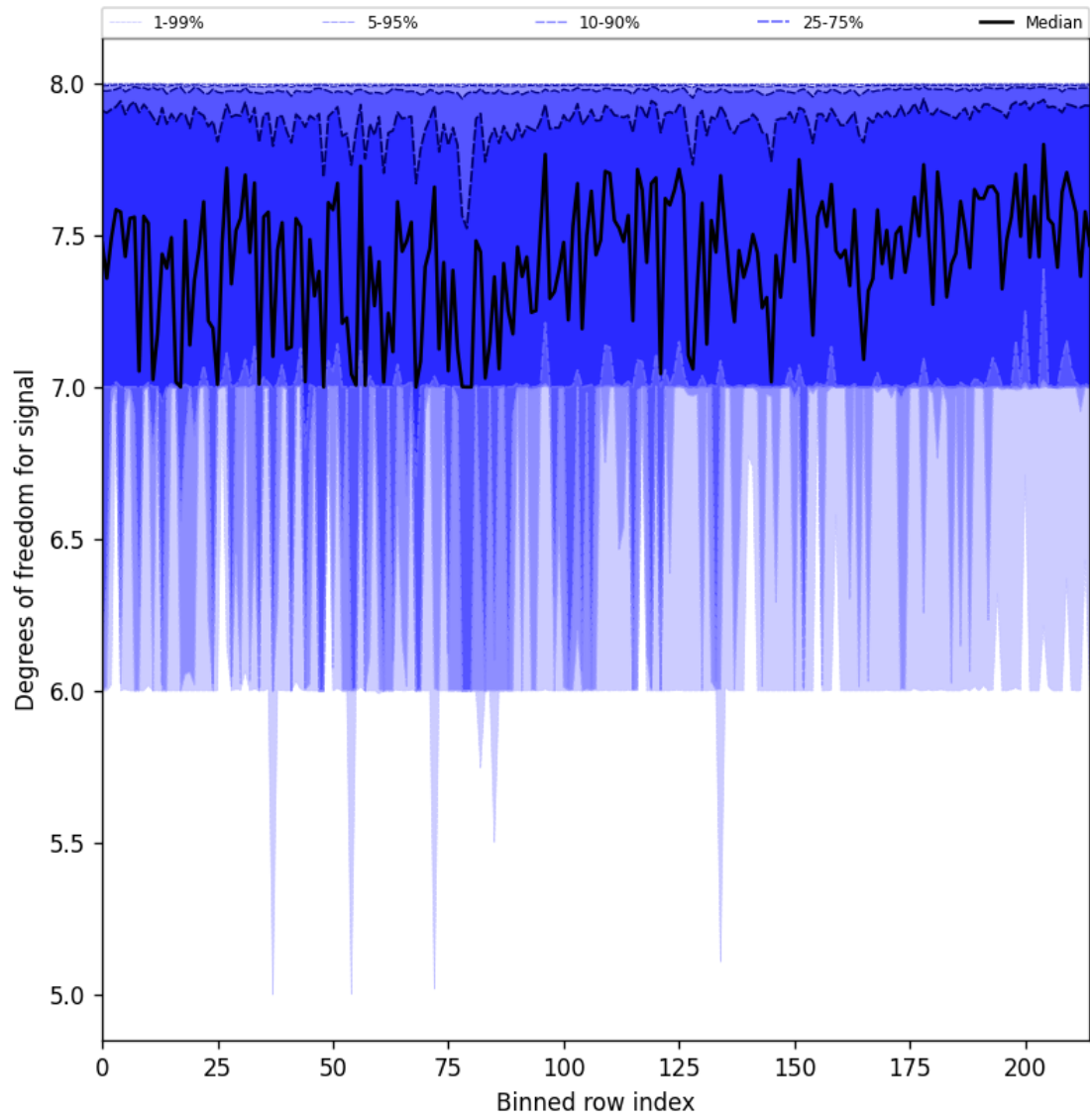
Figure 31: Along track statistics of “Degrees of freedom for signal” for 2024-11-06 to 2024-11-08
