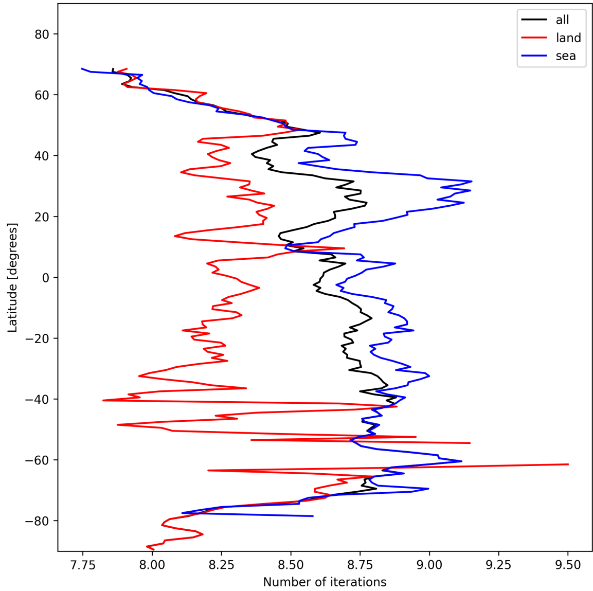
Figure 16: Zonal average of “Number of iterations” for 2024-11-06 to 2024-11-08.
