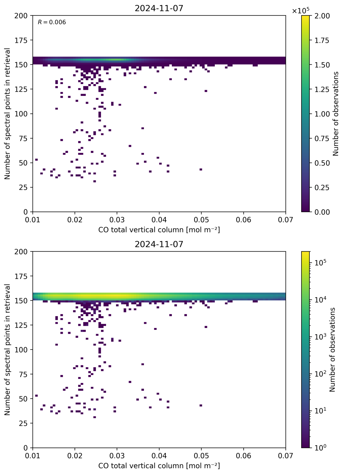
Figure 43: Scatter density plot of “CO total vertical column” against “Number of spectral points in retrieval” for 2024-11-06 to 2024-11-08.
