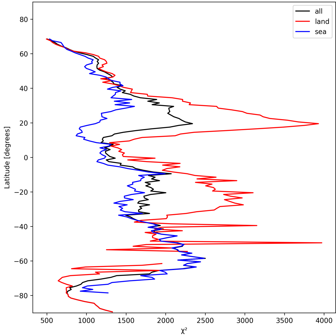
Figure 14: Zonal average of “ \chi^2 ” for 2024-11-06 to 2024-11-08.
