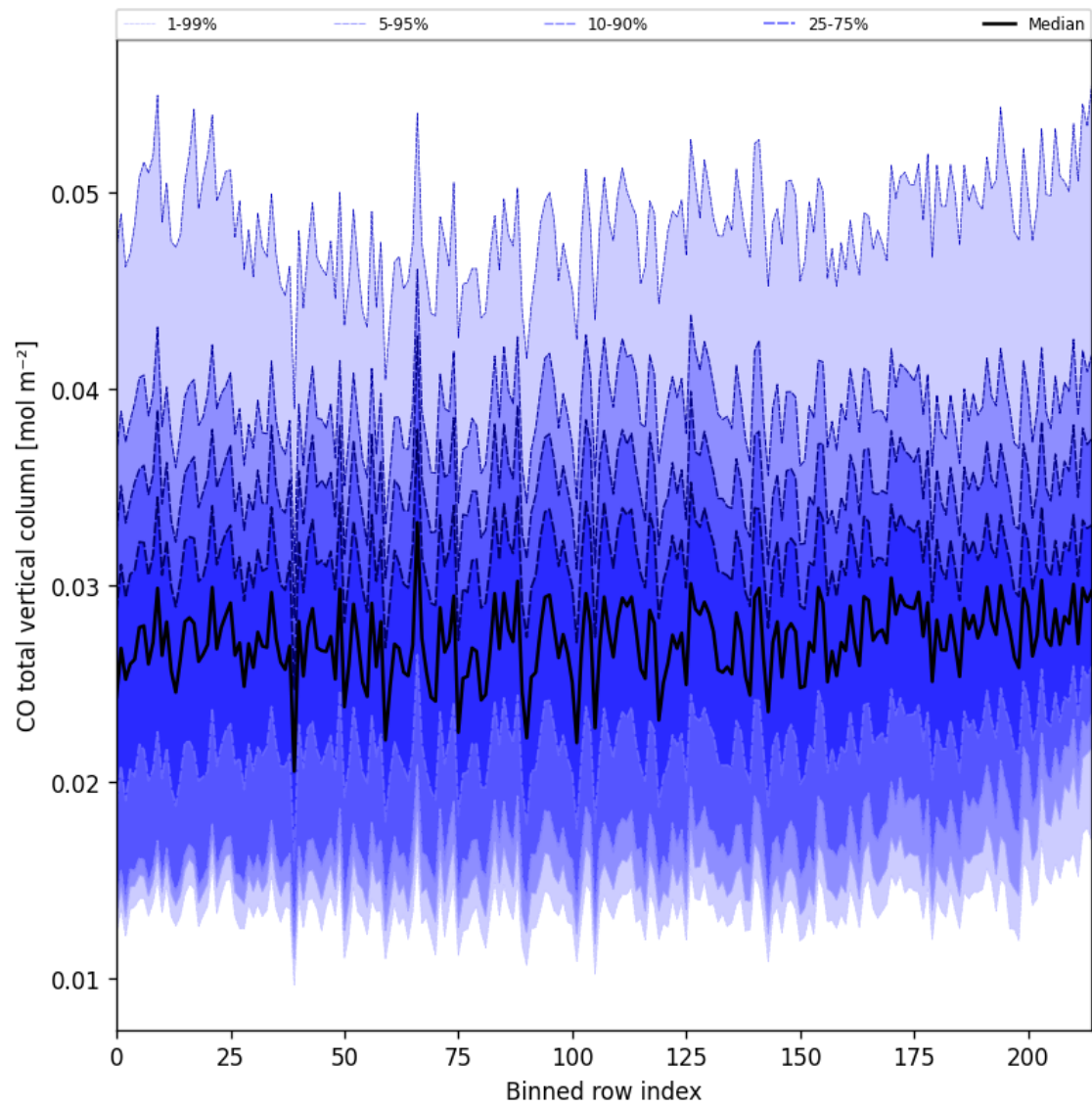
Figure 26: Along track statistics of “CO total vertical column” for 2024-11-06 to 2024-11-08
