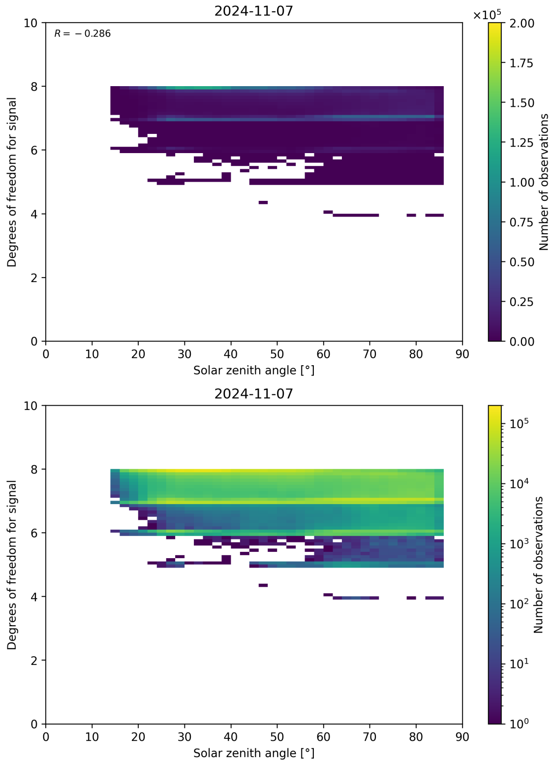
Figure 65: Scatter density plot of “Solar zenith angle” against “Degrees of freedom for signal” for 2024-11-06 to 2024-11-08.
