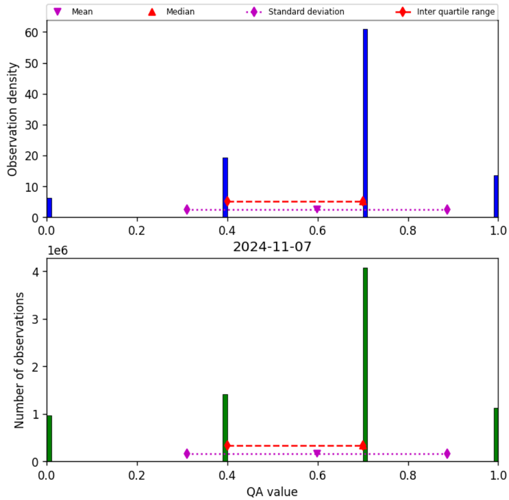
Figure 17: Histogram of “QA value” for 2024-11-06 to 2024-11-08
