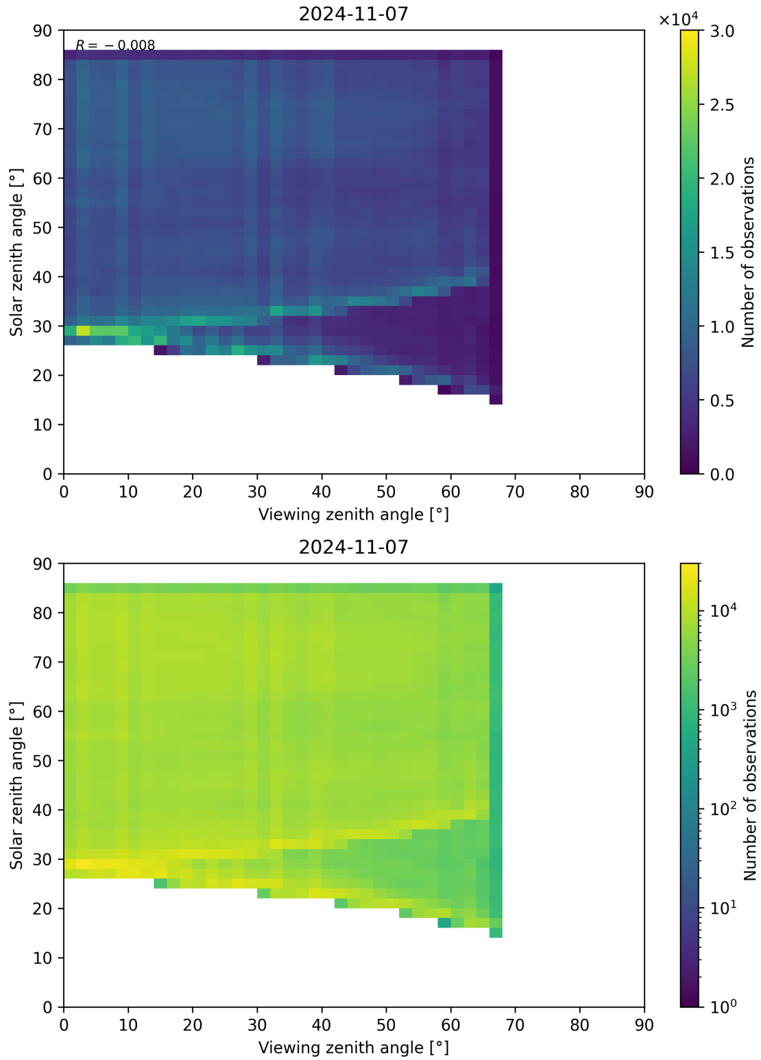
Figure 77: Scatter density plot of “Viewing zenith angle” against “Solar zenith angle” for 2024-11-06 to 2024-11-08.
