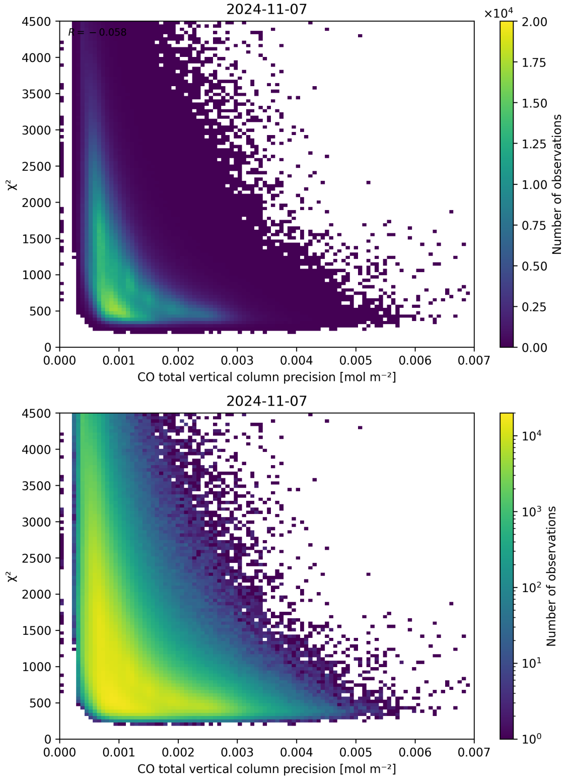
Figure 44: Scatter density plot of “CO total vertical column precision” against “ \chi^2 ” for 2024-11-06 to 2024-11-08.
