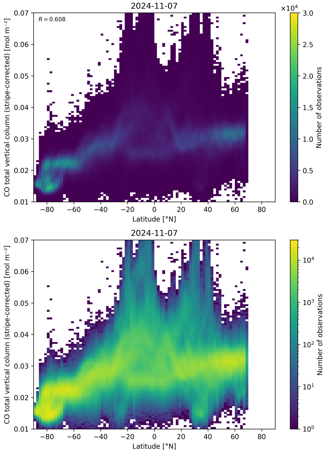
Figure 52: Scatter density plot of “Latitude” against “CO total vertical column (stripe-corrected)” for 2024-11-06 to 2024-11-08.
