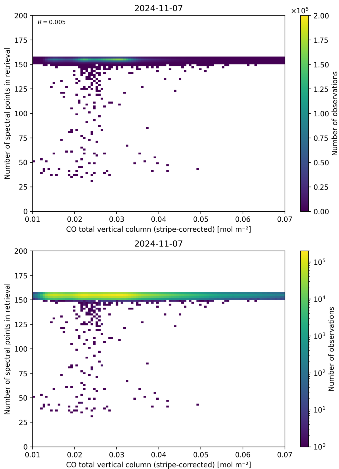
Figure 40: Scatter density plot of “CO total vertical column (stripe-corrected)” against “Number of spectral points in retrieval” for 2024-11-06 to 2024-11-08.
