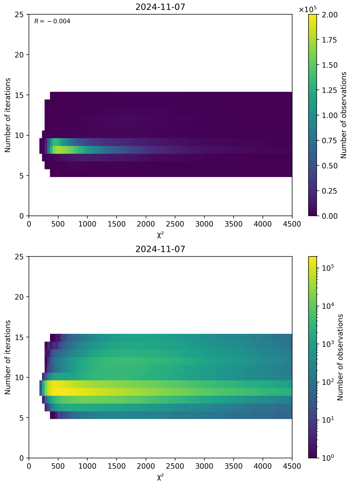
Figure 49: Scatter density plot of “ \chi^2 ” against “Number of iterations” for 2024-11-06 to 2024-11-08.
