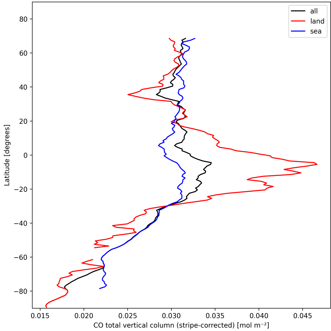
Figure 11: Zonal average of “CO total vertical column (stripe-corrected)” for 2024-11-06 to 2024-11-08.
