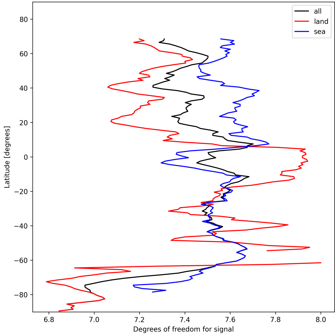
Figure 15: Zonal average of “Degrees of freedom for signal” for 2024-11-06 to 2024-11-08.
