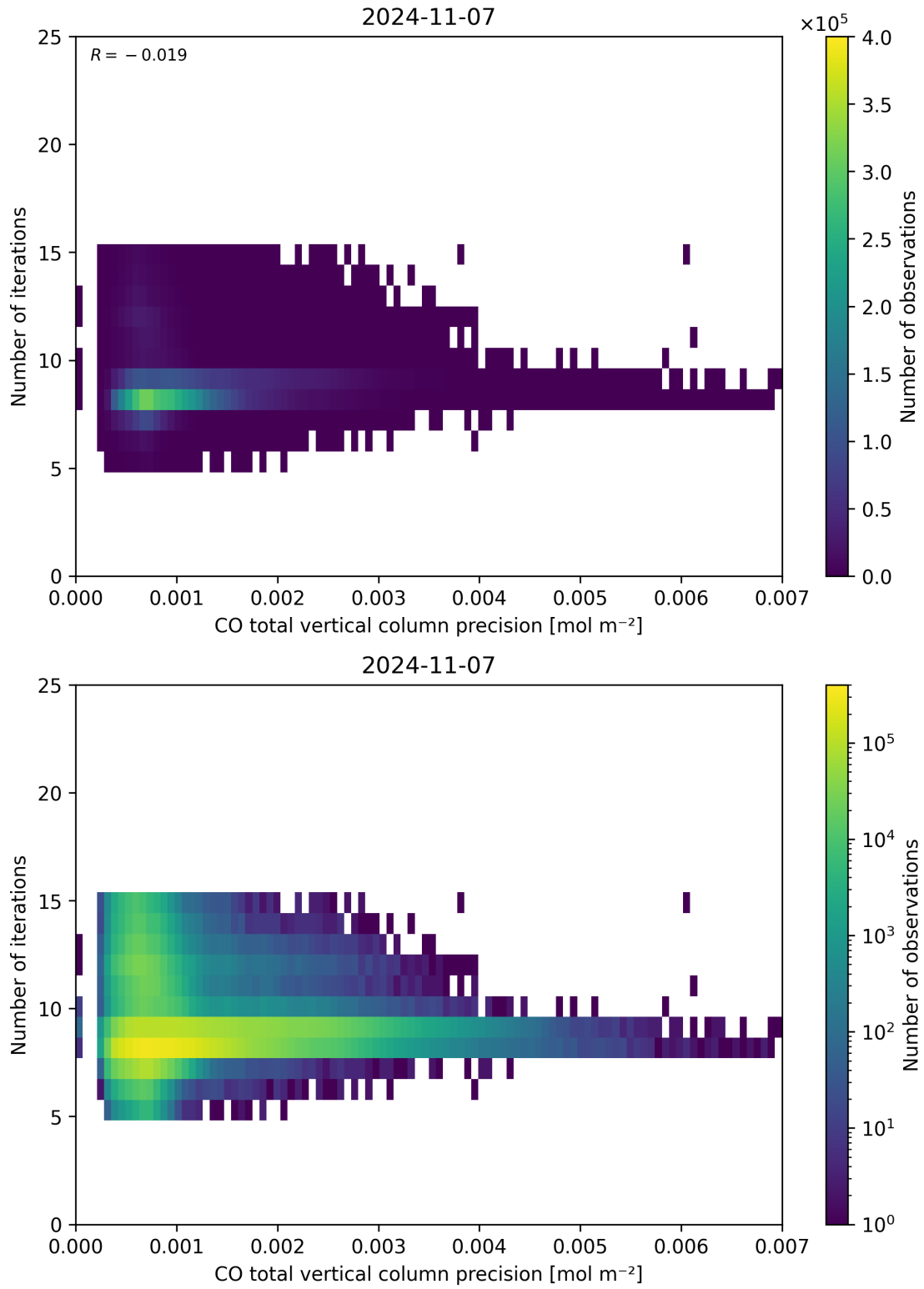
Figure 46: Scatter density plot of “CO total vertical column precision” against “Number of iterations” for 2024-11-06 to 2024-11-08.
