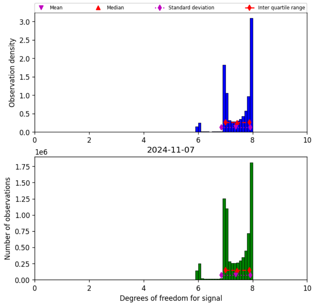
Figure 23: Histogram of “Degrees of freedom for signal” for 2024-11-06 to 2024-11-08
