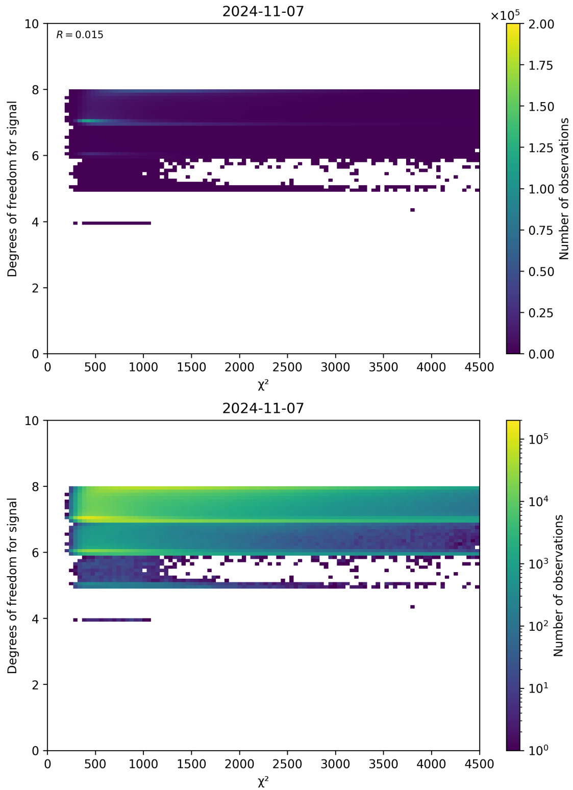
Figure 48: Scatter density plot of “ \chi^2 ” against “Degrees of freedom for signal” for 2024-11-06 to 2024-11-08.
