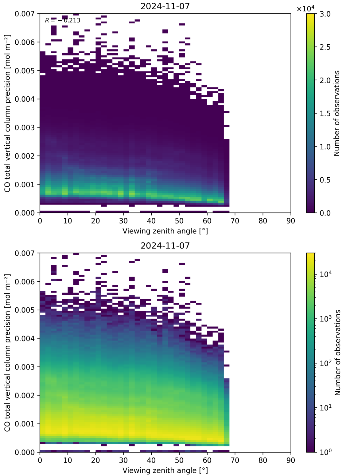
Figure 71: Scatter density plot of “Viewing zenith angle” against “CO total vertical column precision” for 2024-11-06 to 2024-11-08.
