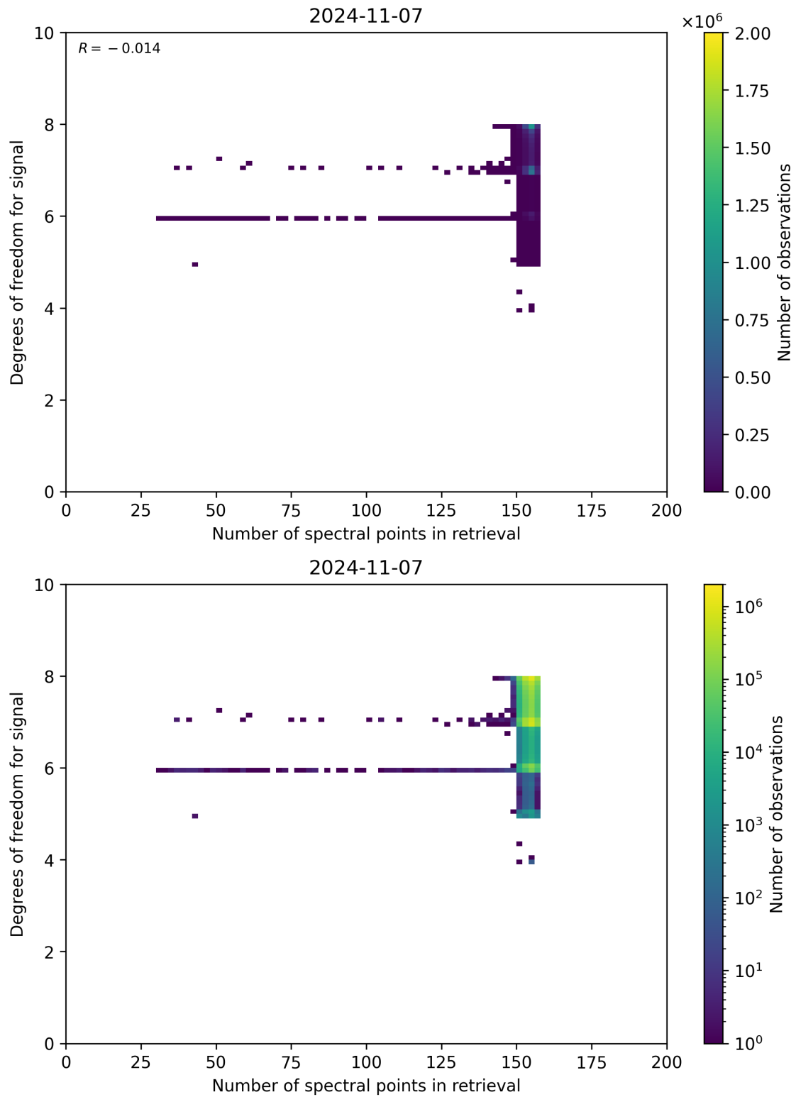
Figure 59: Scatter density plot of “Number of spectral points in retrieval” against “Degrees of freedom for signal” for 2024-11-06 to 2024-11-08.
