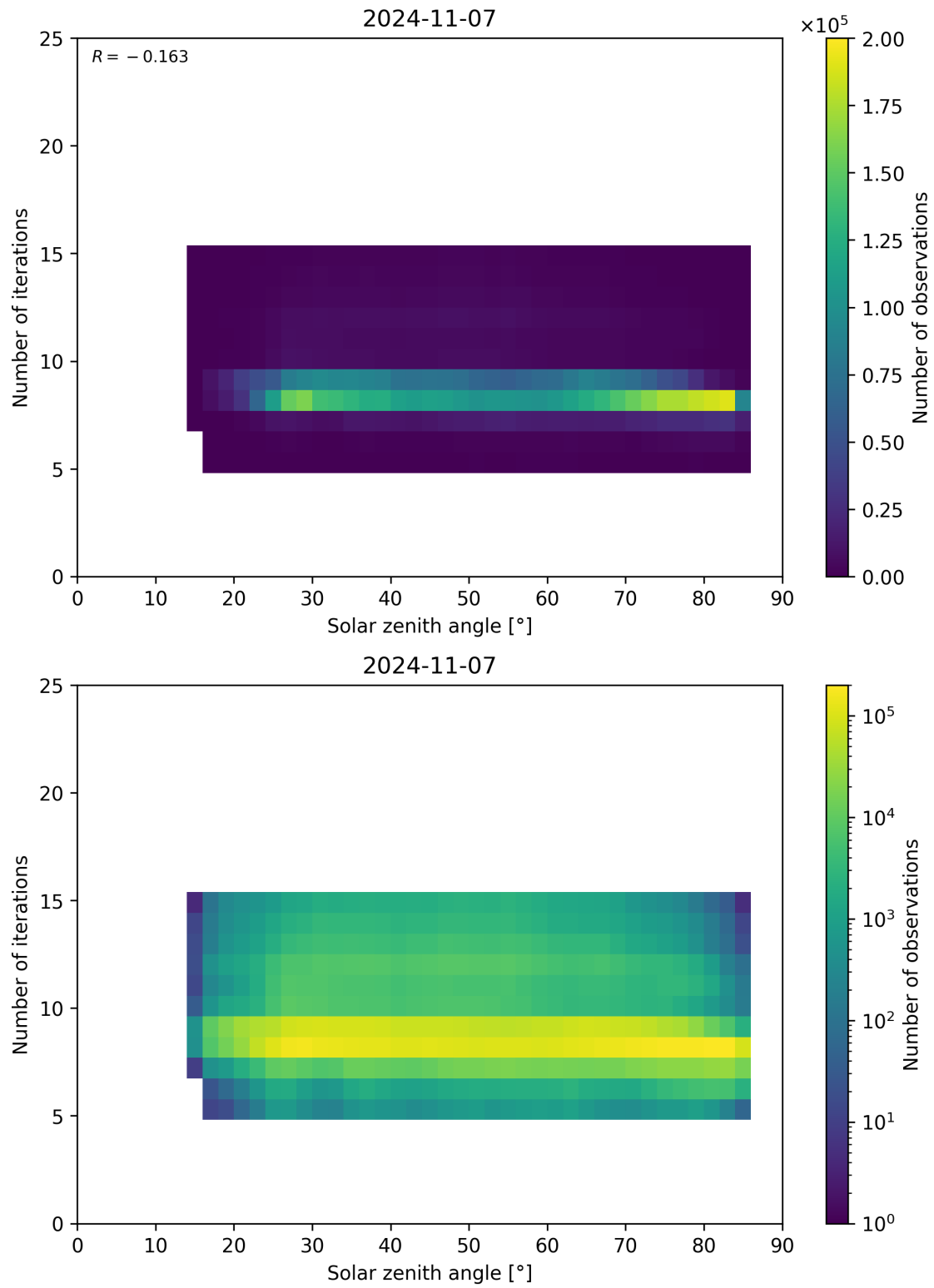
Figure 67: Scatter density plot of “Solar zenith angle” against “Number of iterations” for 2024-11-06 to 2024-11-08.
