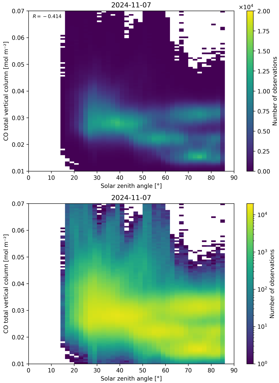
Figure 61: Scatter density plot of “Solar zenith angle” against “CO total vertical column” for 2024-11-06 to 2024-11-08.
