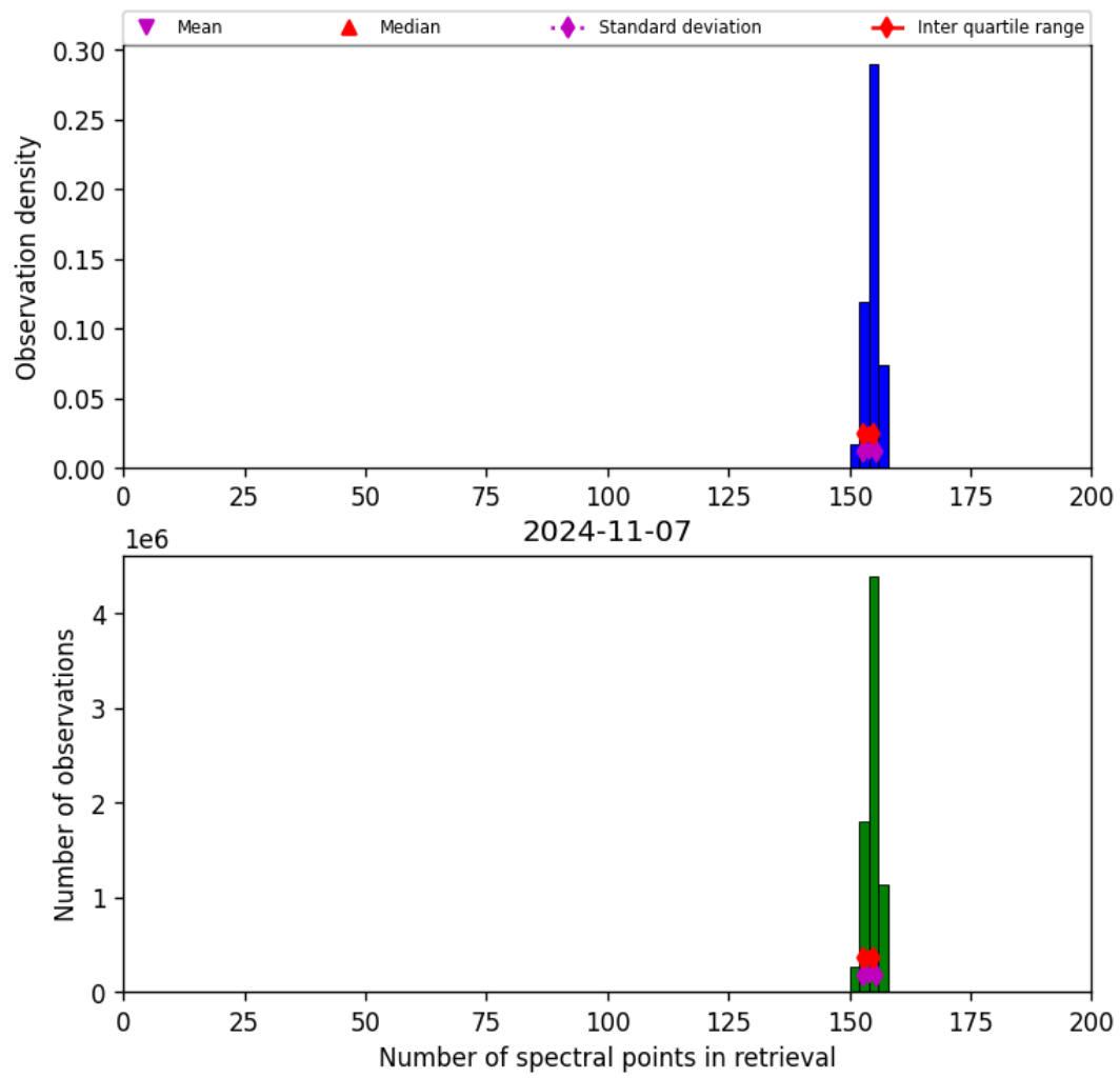
Figure 21: Histogram of “Number of spectral points in retrieval” for 2024-11-06 to 2024-11-08
