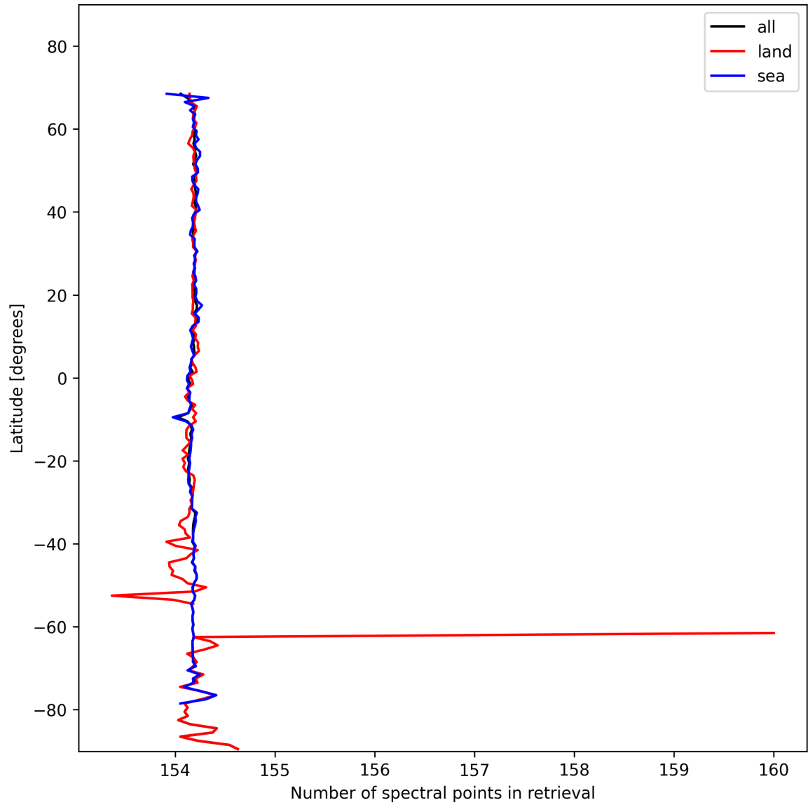
Figure 13: Zonal average of “Number of spectral points in retrieval” for 2024-11-06 to 2024-11-08.
