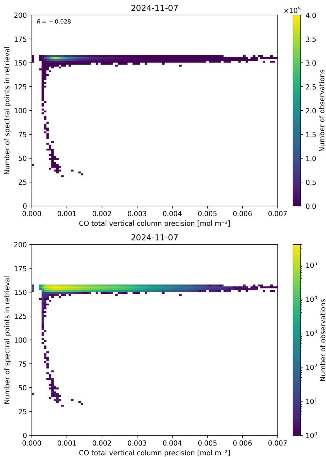
Figure 47: Scatter density plot of “CO total vertical column precision” against “Number of spectral points in retrieval” for 2024-11-06 to 2024-11-08.
