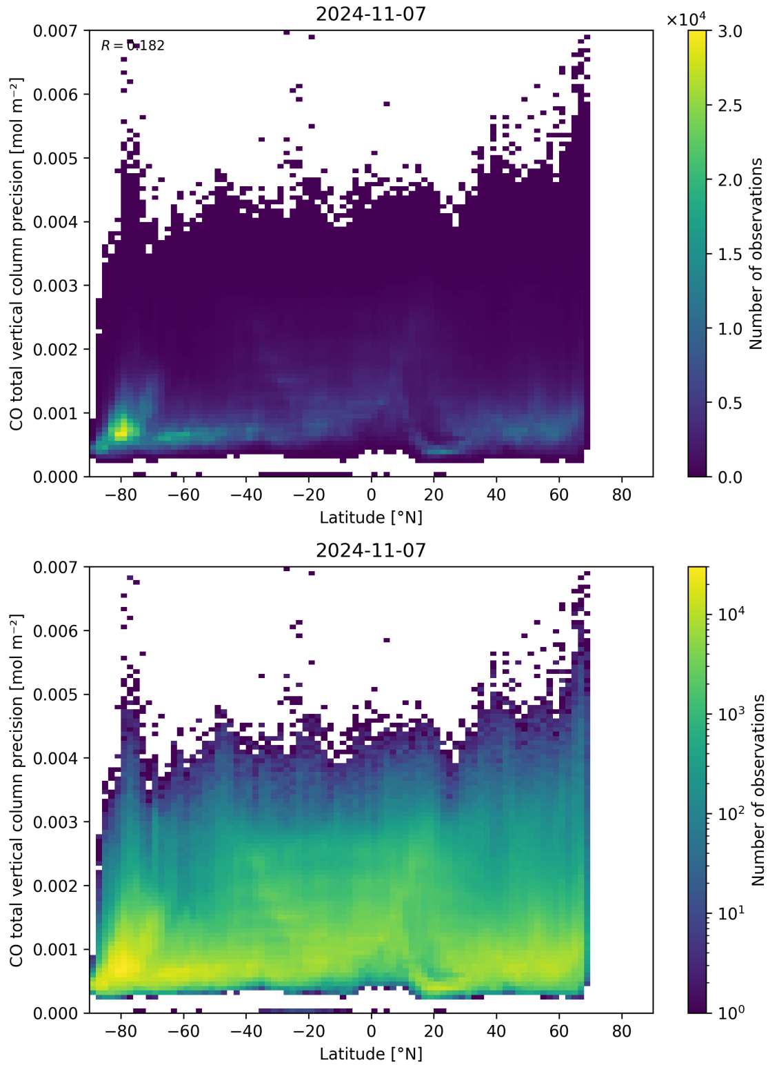
Figure 53: Scatter density plot of “Latitude” against “CO total vertical column precision” for 2024-11-06 to 2024-11-08.
