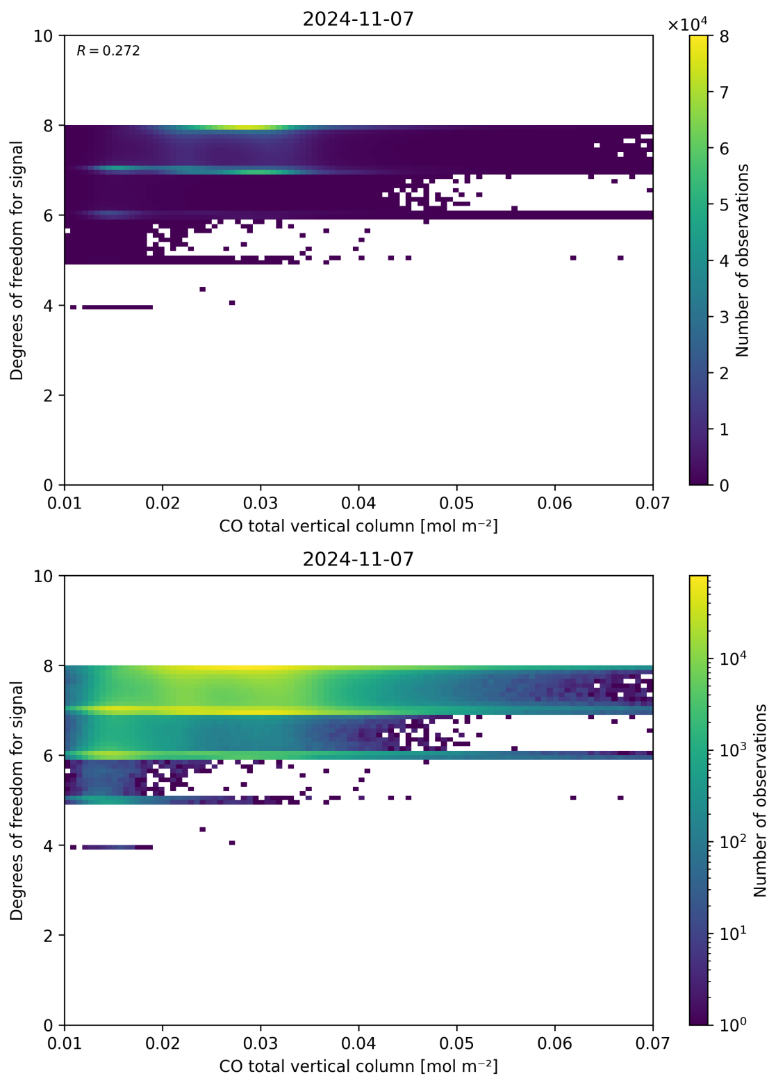
Figure 41: Scatter density plot of “CO total vertical column” against “Degrees of freedom for signal” for 2024-11-06 to 2024-11-08.
