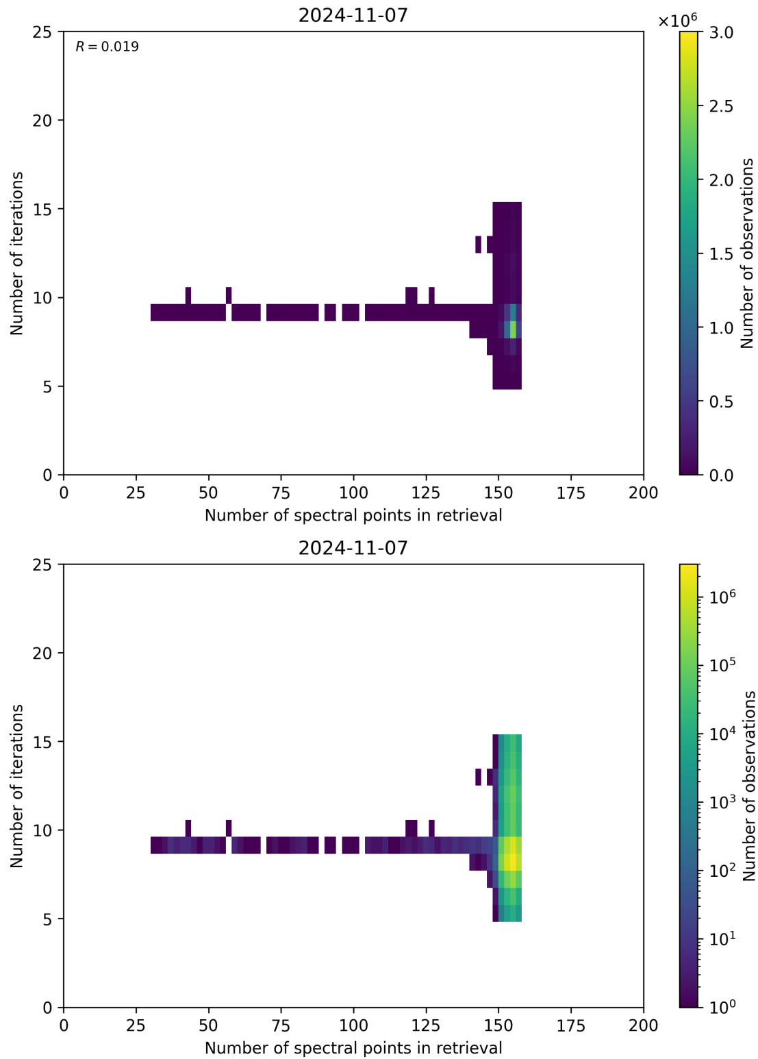
Figure 60: Scatter density plot of “Number of spectral points in retrieval” against “Number of iterations” for 2024-11-06 to 2024-11-08.
