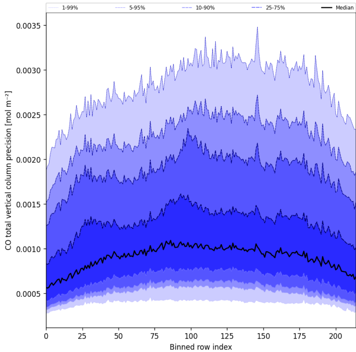
Figure 28: Along track statistics of “CO total vertical column precision” for 2024-11-06 to 2024-11-08
