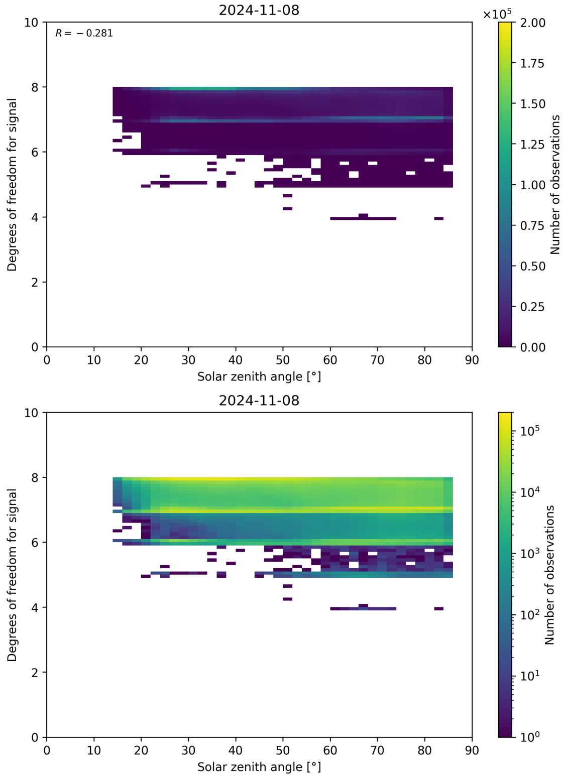
Figure 65: Scatter density plot of “Solar zenith angle” against “Degrees of freedom for signal” for 2024-11-07 to 2024-11-09.
