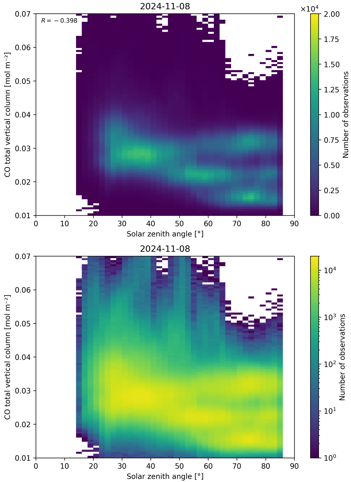
Figure 61: Scatter density plot of “Solar zenith angle” against “CO total vertical column” for 2024-11-07 to 2024-11-09.
