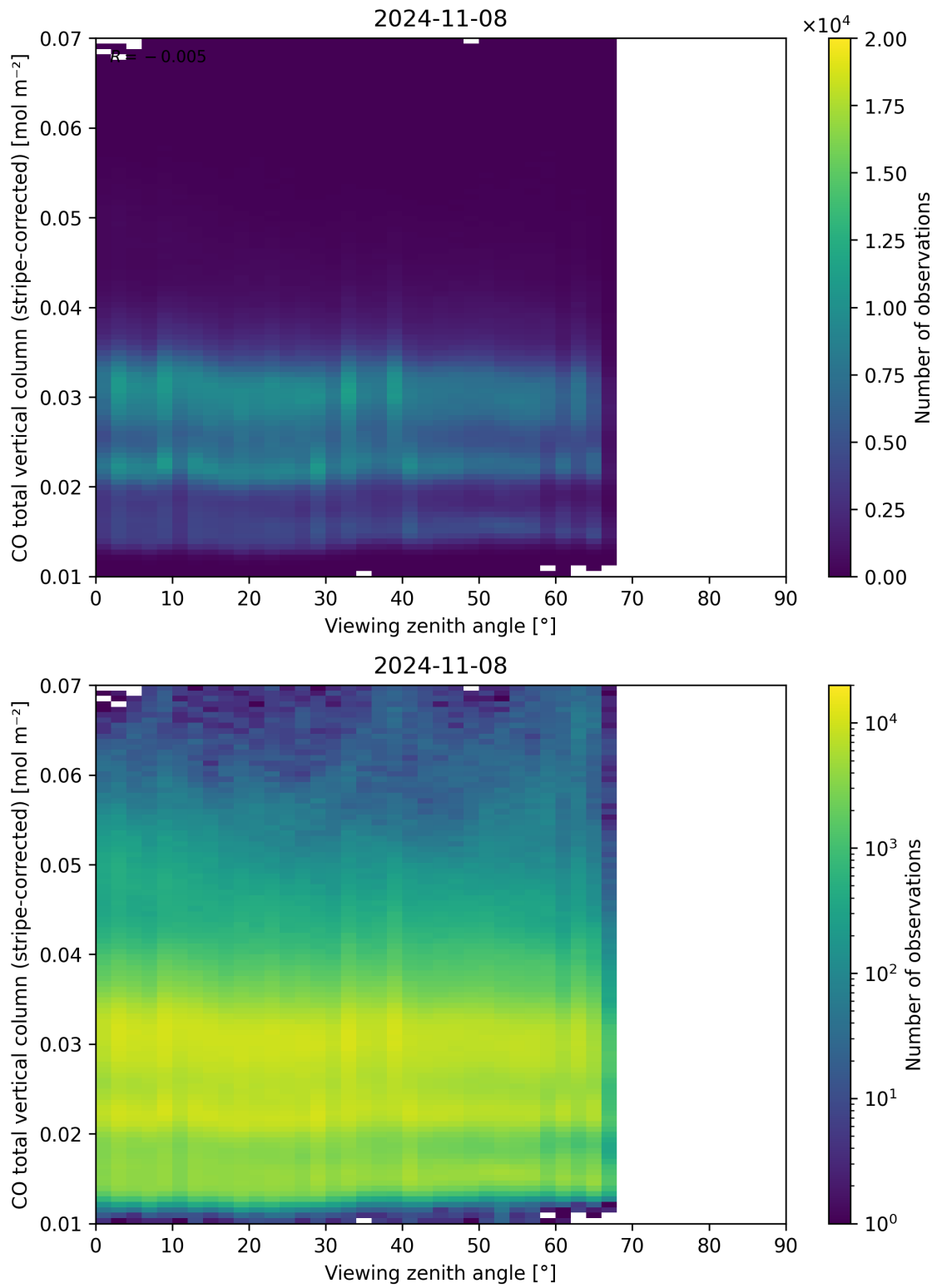
Figure 70: Scatter density plot of “Viewing zenith angle” against “CO total vertical column (stripe-corrected)” for 2024-11-07 to 2024-11-09.
