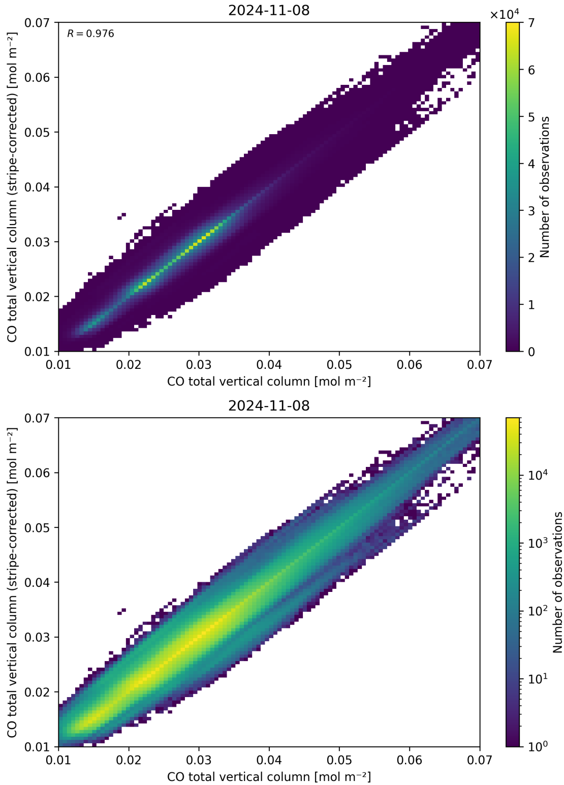
Figure 33: Scatter density plot of “CO total vertical column” against “CO total vertical column (stripe-corrected)” for 2024-11-07 to 2024-11-09.
