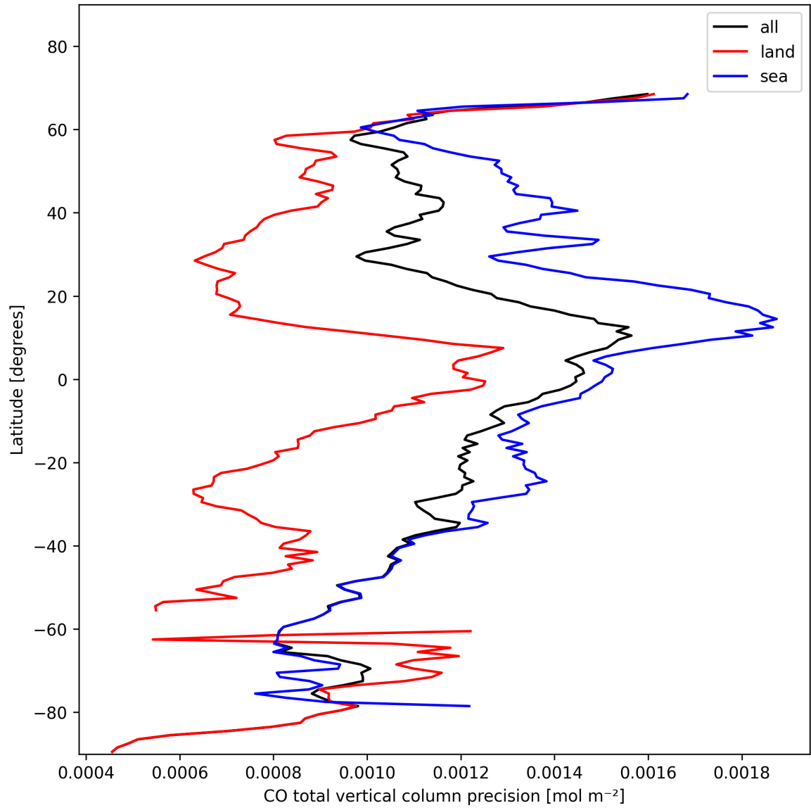
Figure 12: Zonal average of “CO total vertical column precision” for 2024-11-07 to 2024-11-09.
