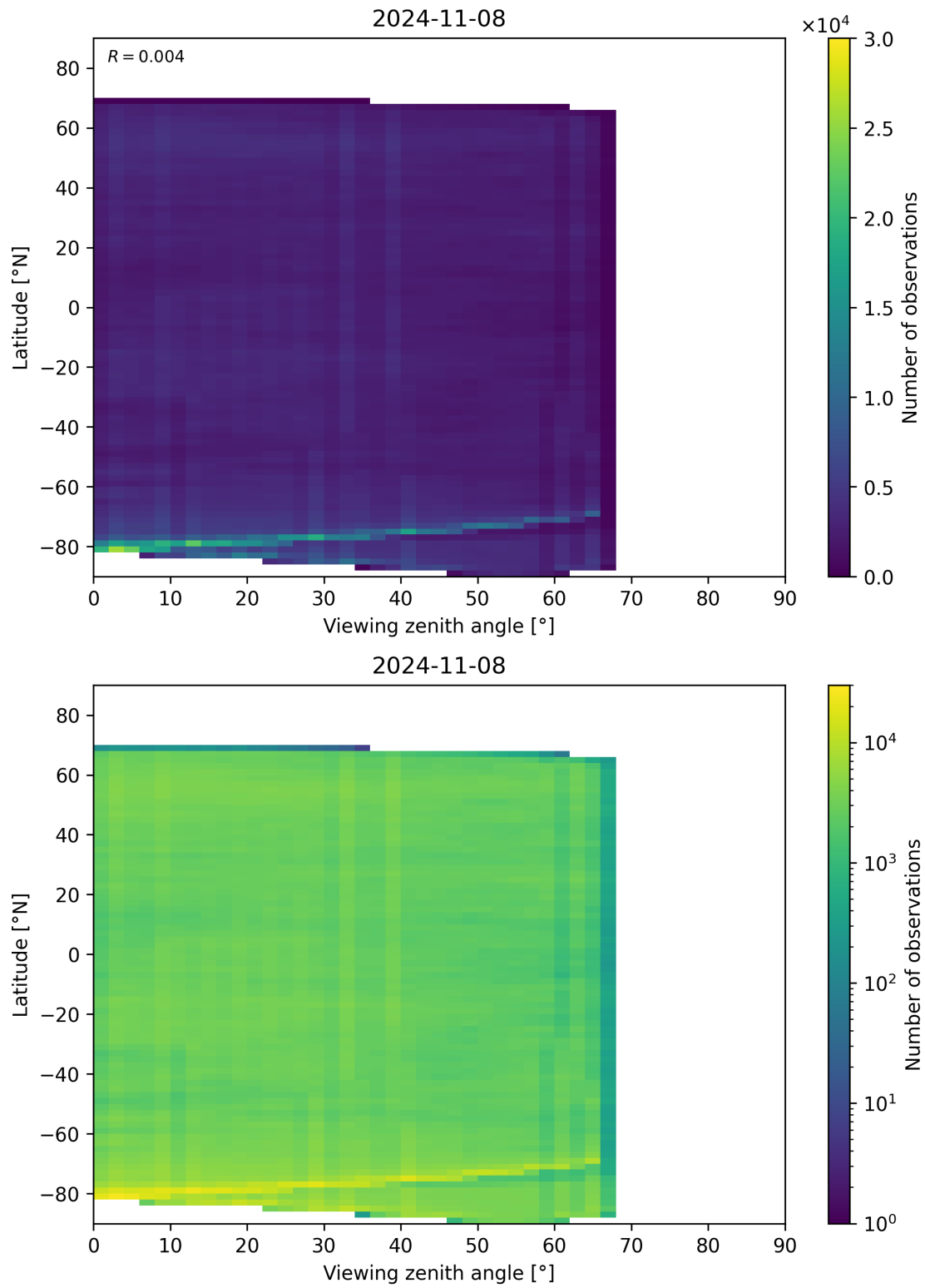
Figure 74: Scatter density plot of “Viewing zenith angle” against “Latitude” for 2024-11-07 to 2024-11-09.
