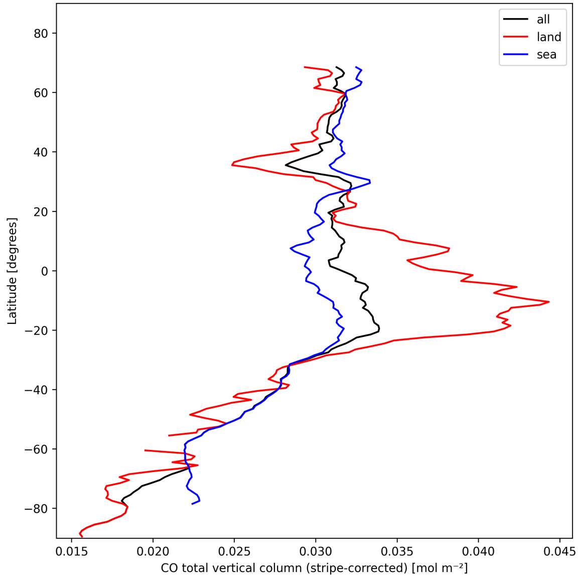
Figure 11: Zonal average of “CO total vertical column (stripe-corrected)” for 2024-11-07 to 2024-11-09.
