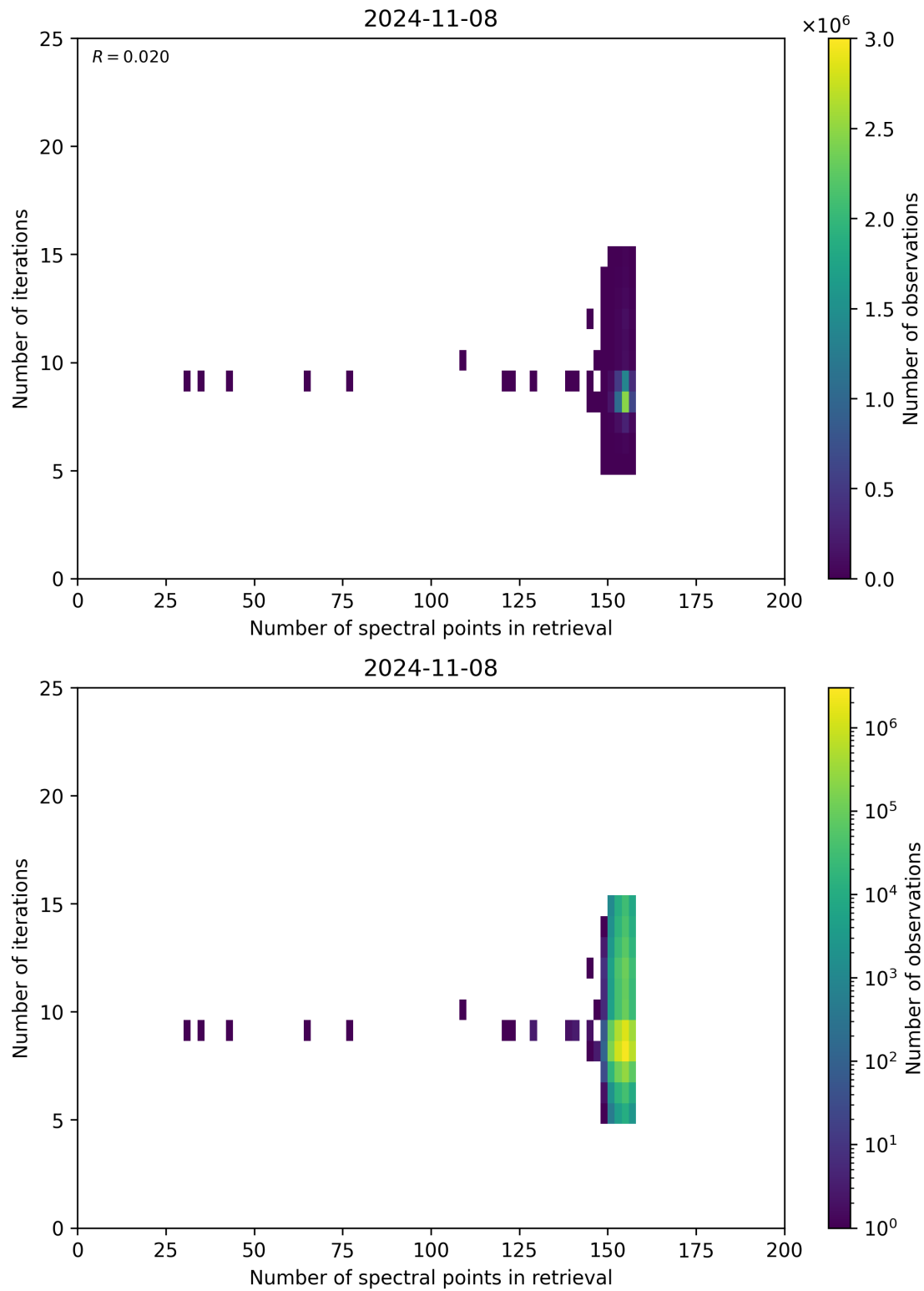
Figure 60: Scatter density plot of “Number of spectral points in retrieval” against “Number of iterations” for 2024-11-07 to 2024-11-09.
