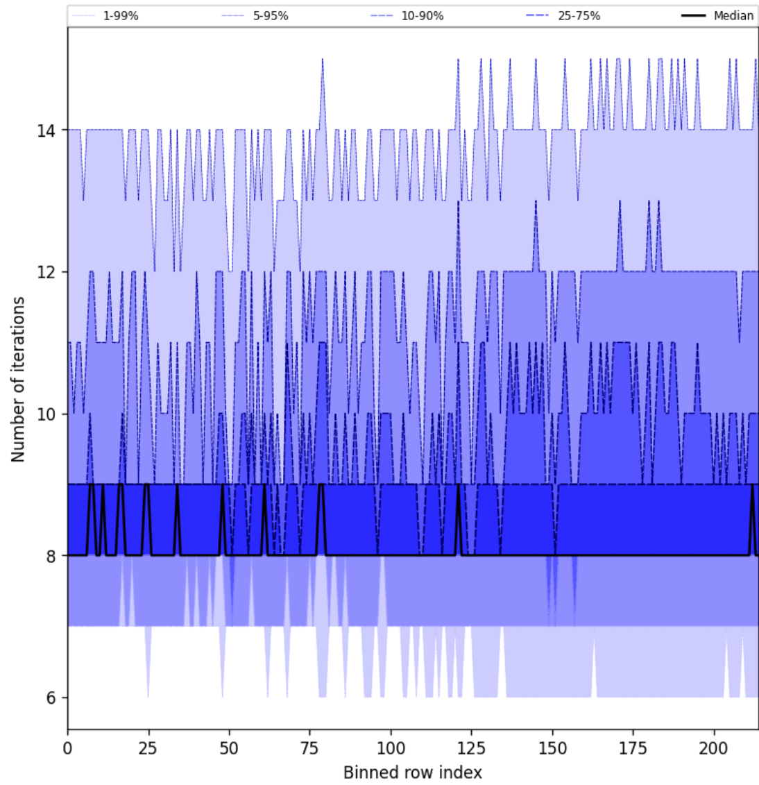
Figure 32: Along track statistics of “Number of iterations” for 2024-11-07 to 2024-11-09
