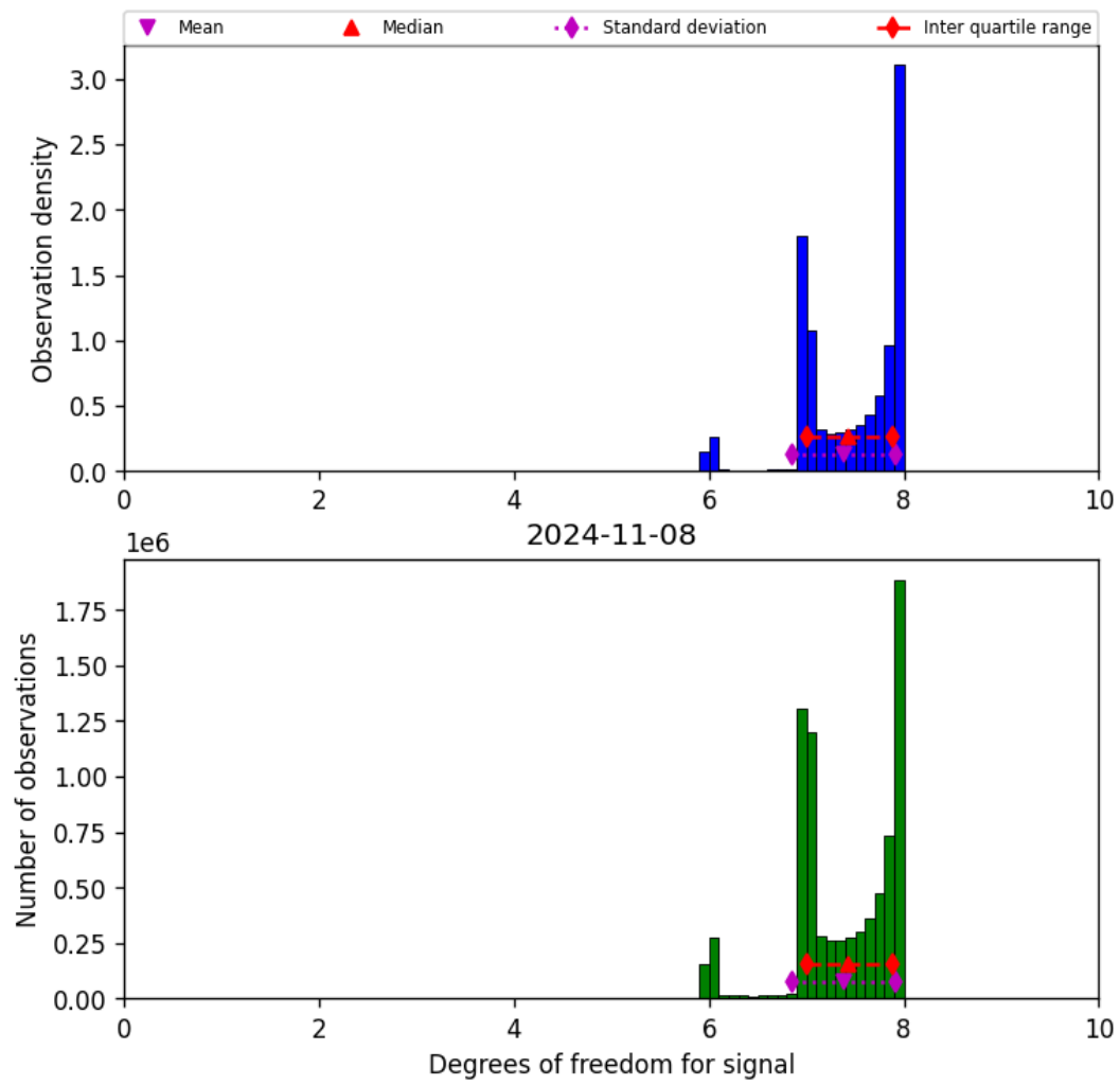
Figure 23: Histogram of “Degrees of freedom for signal” for 2024-11-07 to 2024-11-09
