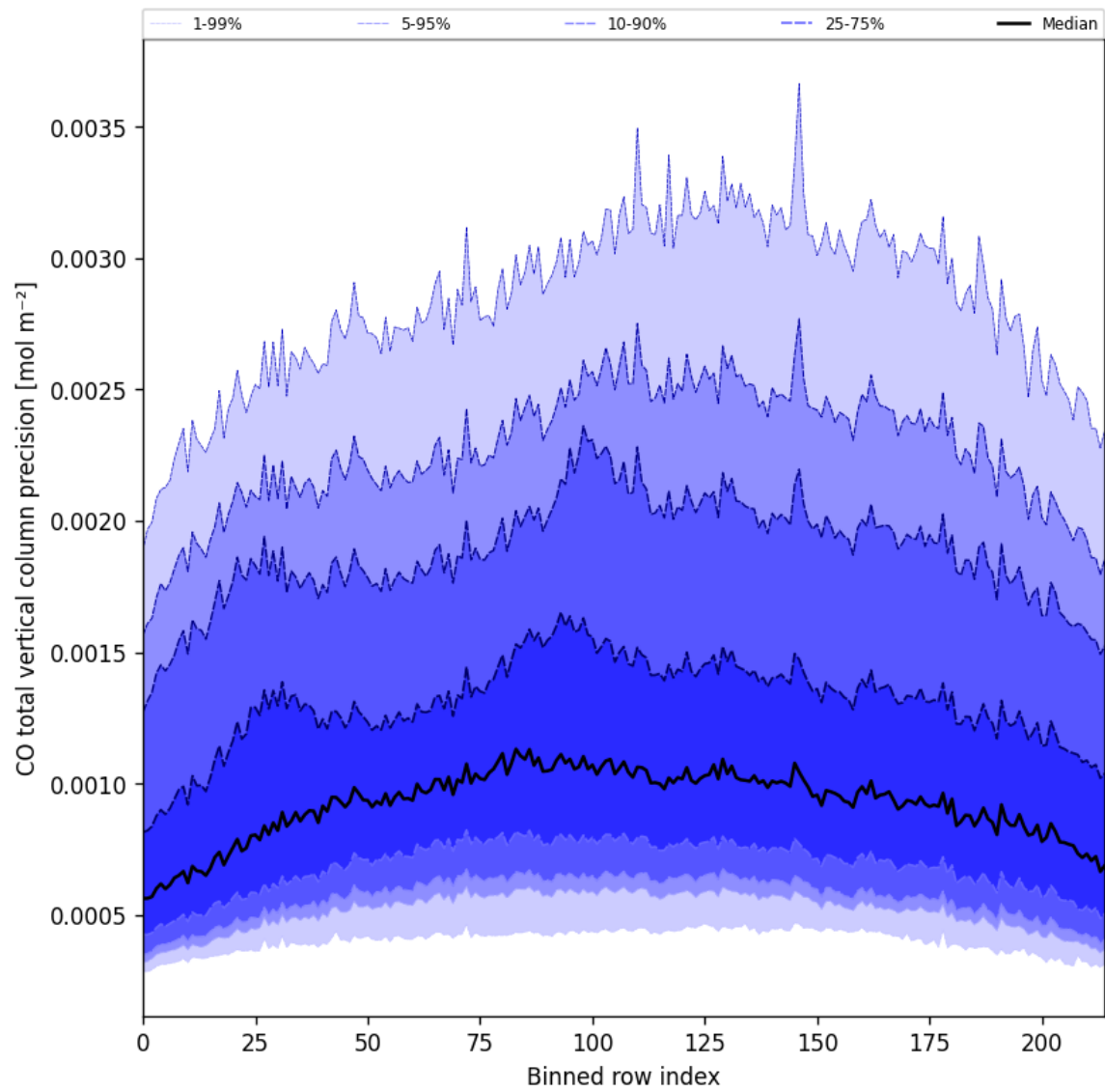
Figure 28: Along track statistics of “CO total vertical column precision” for 2024-11-07 to 2024-11-09
