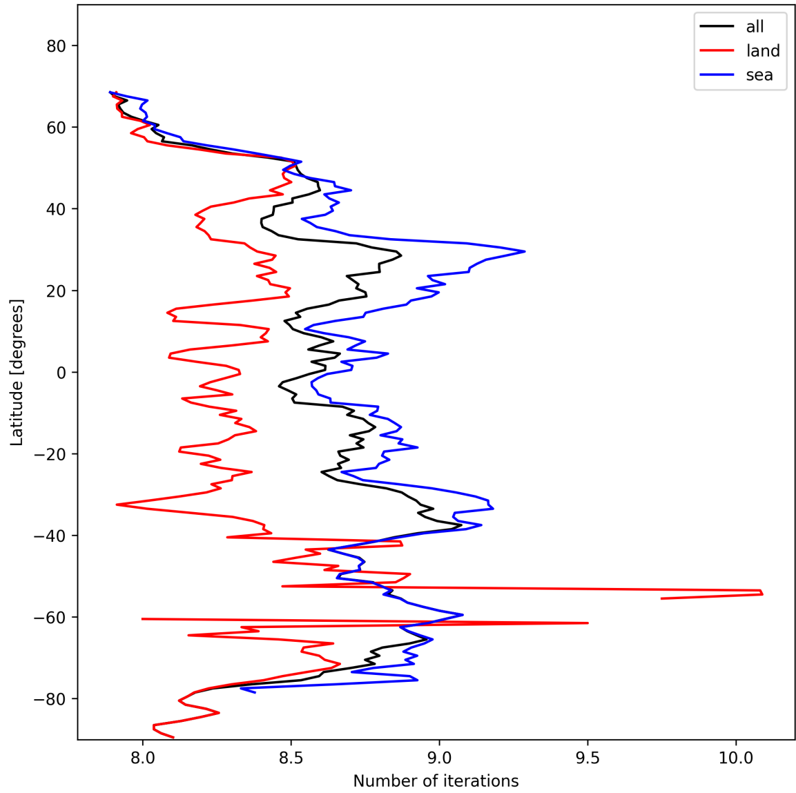
Figure 16: Zonal average of “Number of iterations” for 2024-11-07 to 2024-11-09.
