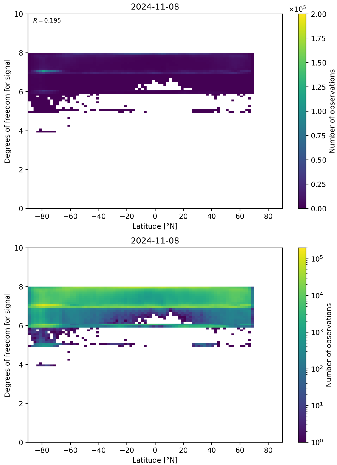
Figure 55: Scatter density plot of “Latitude” against “Degrees of freedom for signal” for 2024-11-07 to 2024-11-09.
