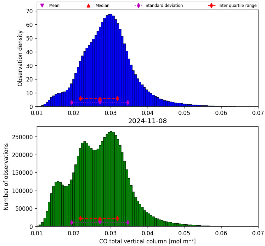
Figure 18: Histogram of “CO total vertical column” for 2024-11-07 to 2024-11-09
