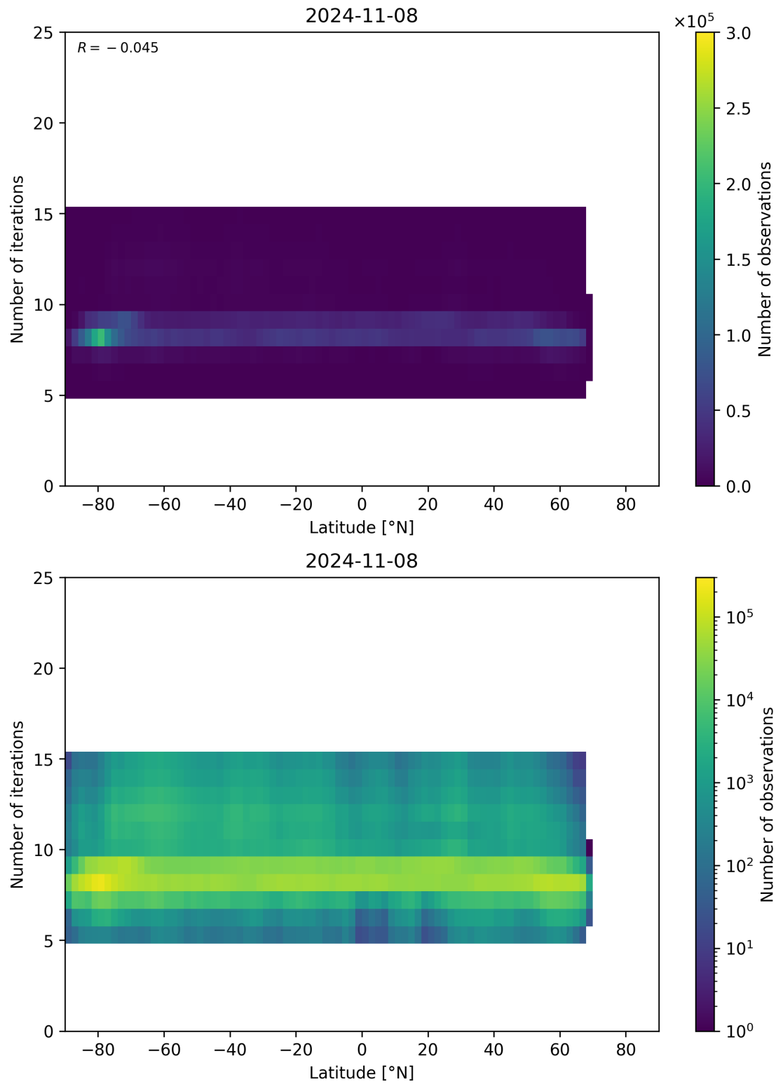
Figure 56: Scatter density plot of “Latitude” against “Number of iterations” for 2024-11-07 to 2024-11-09.
