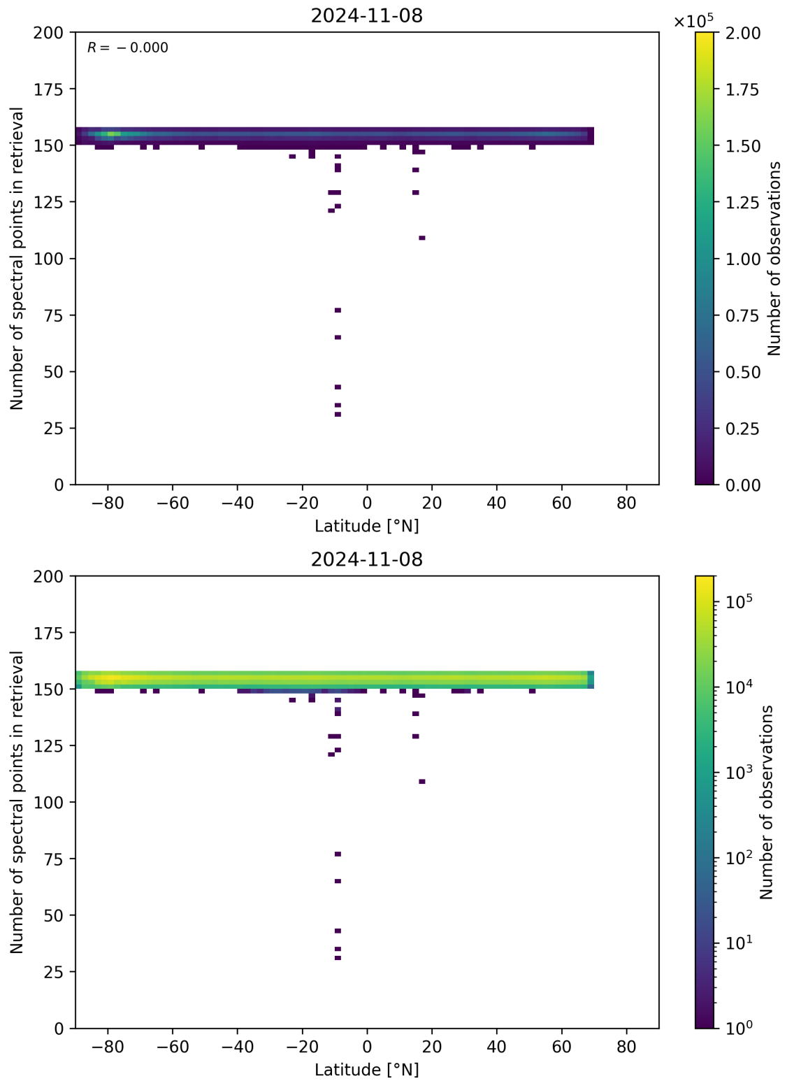
Figure 57: Scatter density plot of “Latitude” against “Number of spectral points in retrieval” for 2024-11-07 to 2024-11-09.
