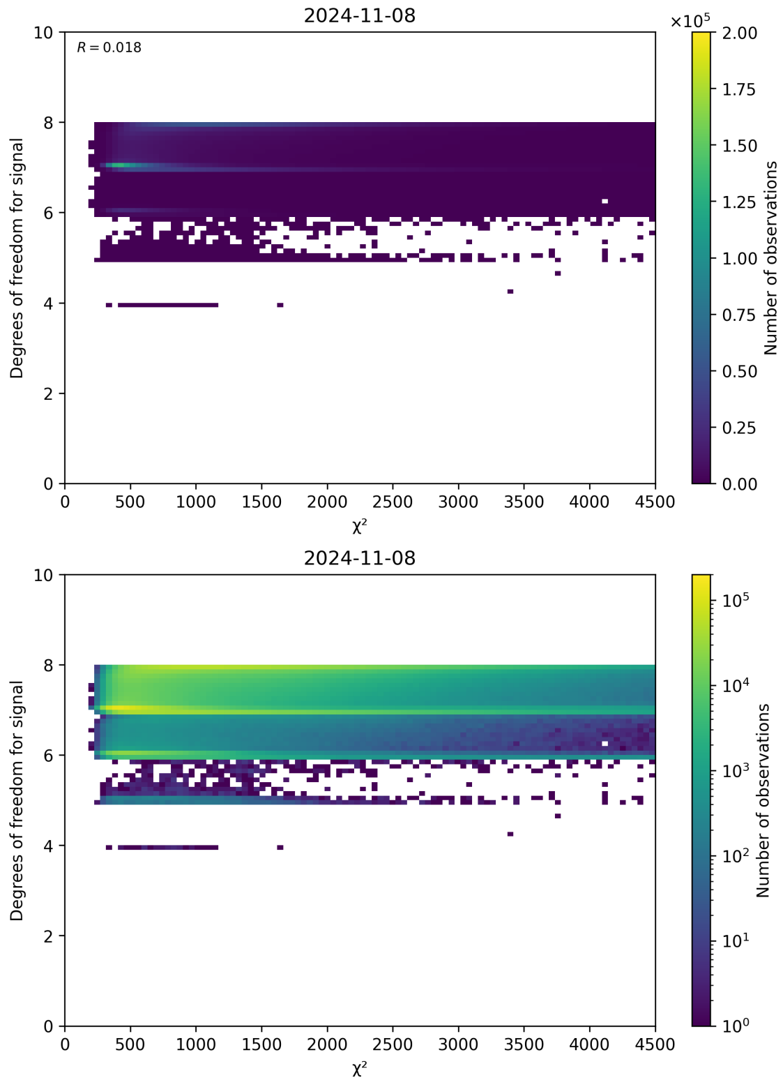
Figure 48: Scatter density plot of “ \chi^2 ” against “Degrees of freedom for signal” for 2024-11-07 to 2024-11-09.
