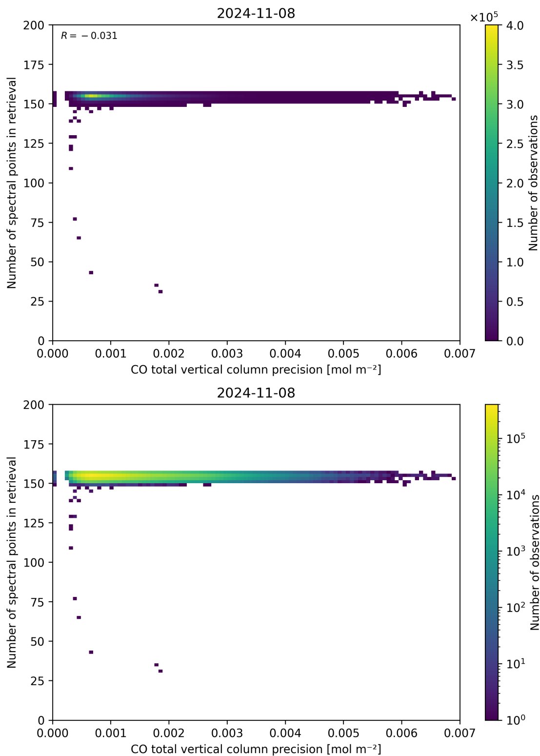
Figure 47: Scatter density plot of “CO total vertical column precision” against “Number of spectral points in retrieval” for 2024-11-07 to 2024-11-09.
