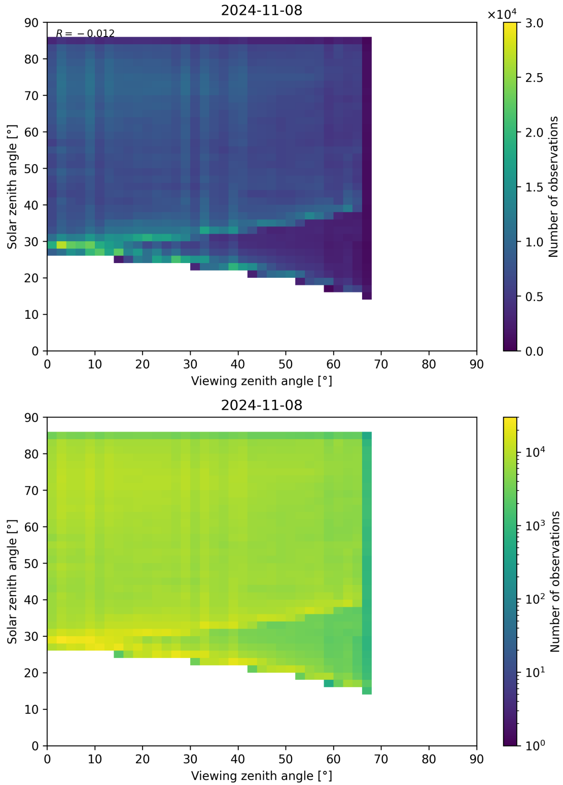
Figure 77: Scatter density plot of “Viewing zenith angle” against “Solar zenith angle” for 2024-11-07 to 2024-11-09.
