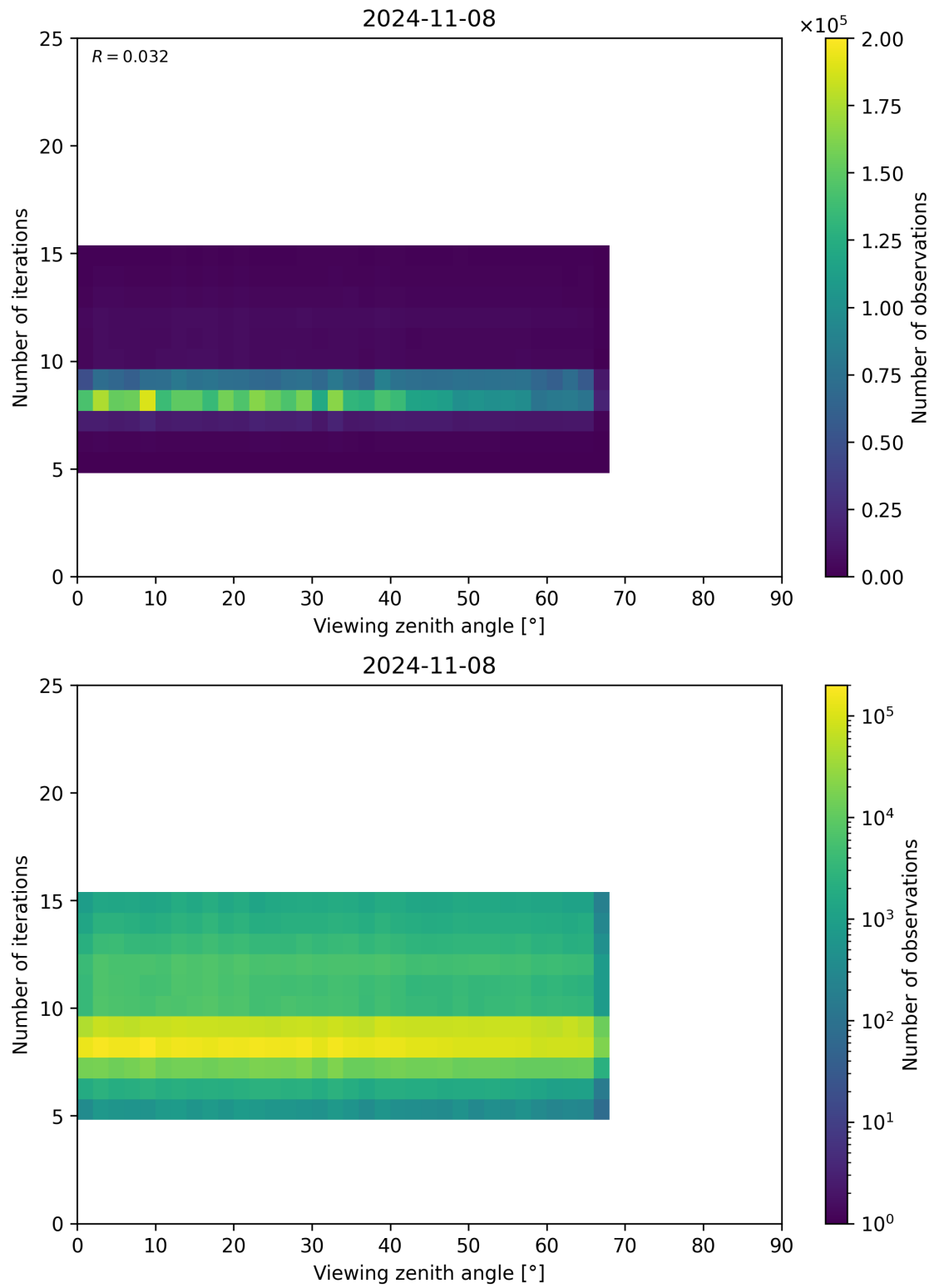
Figure 75: Scatter density plot of “Viewing zenith angle” against “Number of iterations” for 2024-11-07 to 2024-11-09.
