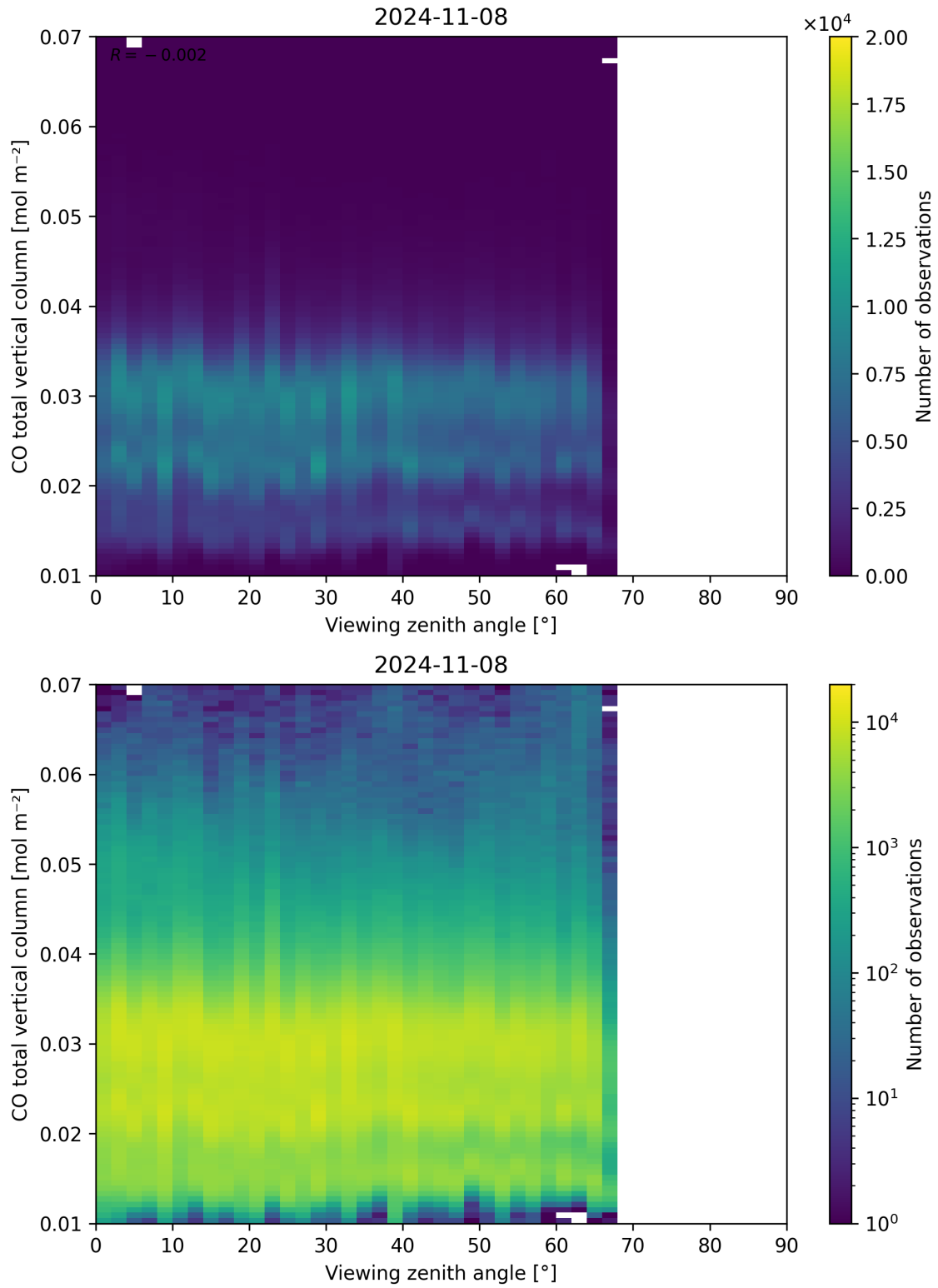
Figure 69: Scatter density plot of “Viewing zenith angle” against “CO total vertical column” for 2024-11-07 to 2024-11-09.
