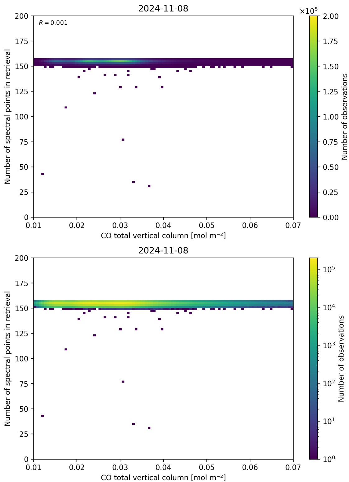
Figure 43: Scatter density plot of “CO total vertical column” against “Number of spectral points in retrieval” for 2024-11-07 to 2024-11-09.
