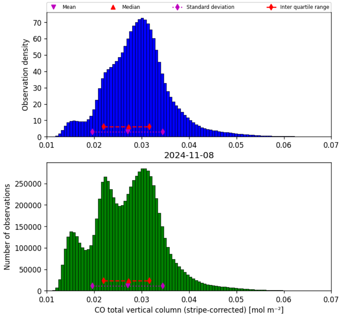
Figure 19: Histogram of “CO total vertical column (stripe-corrected)” for 2024-11-07 to 2024-11-09
