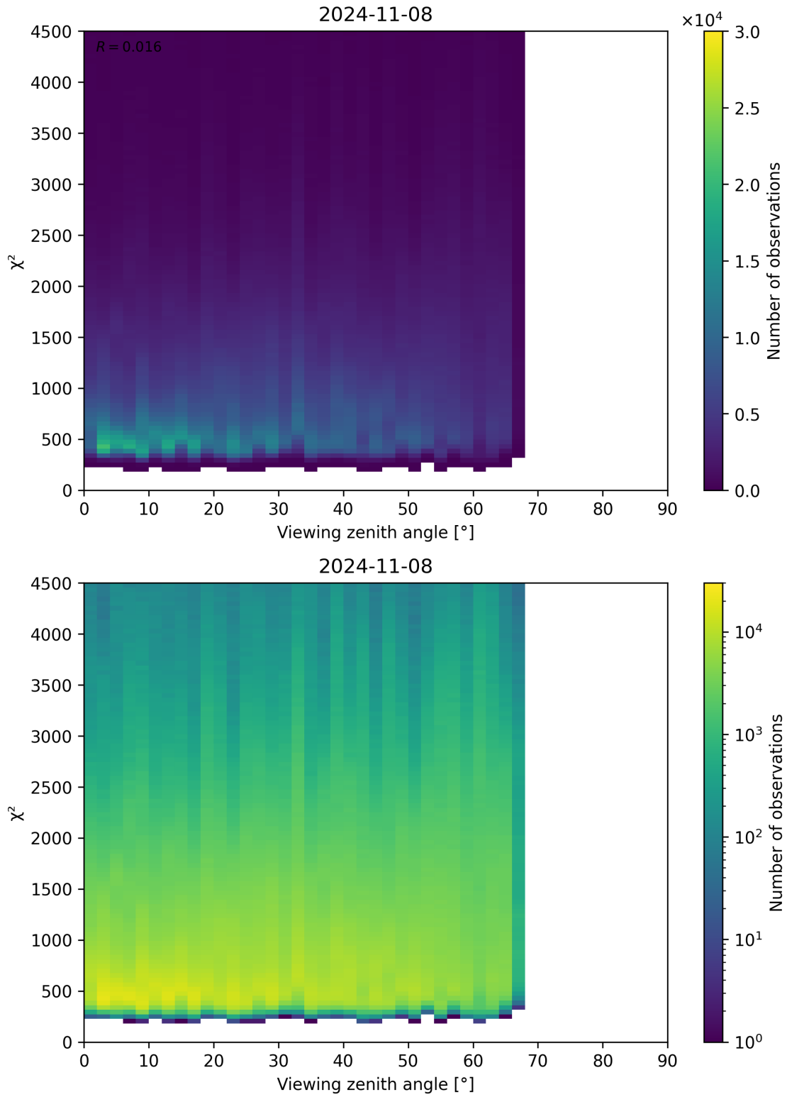
Figure 72: Scatter density plot of “Viewing zenith angle” against “ \chi^2 ” for 2024-11-07 to 2024-11-09.
