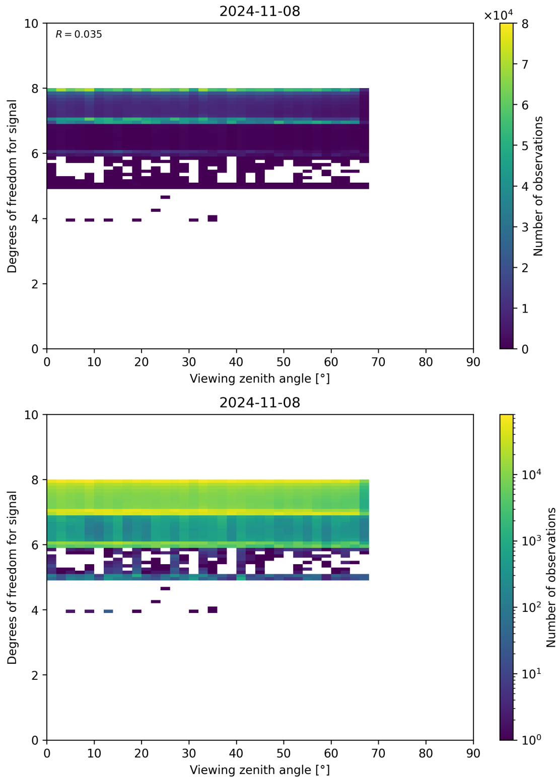
Figure 73: Scatter density plot of “Viewing zenith angle” against “Degrees of freedom for signal” for 2024-11-07 to 2024-11-09.
