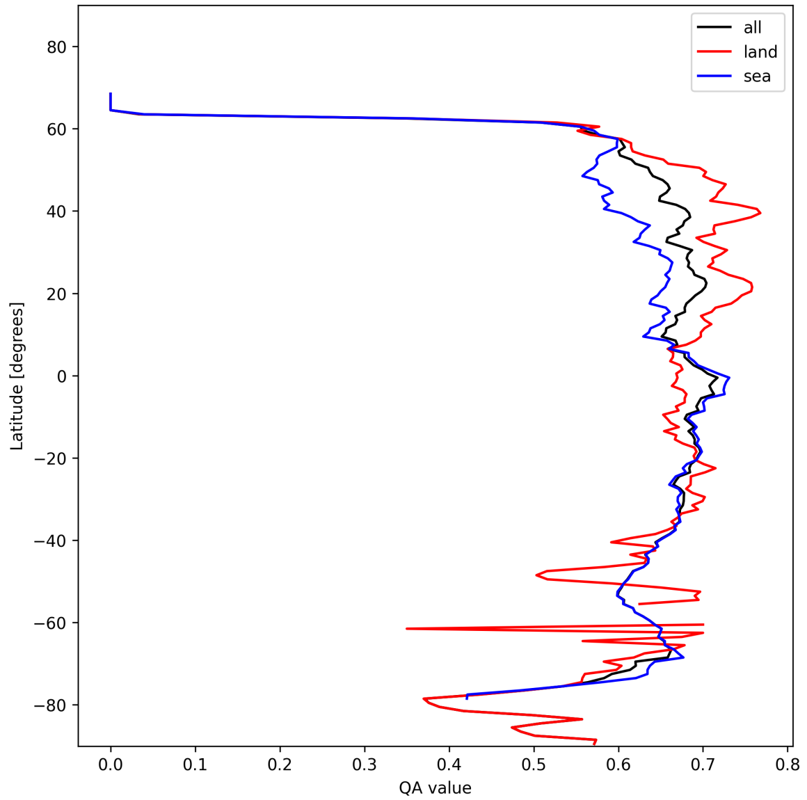
Figure 9: Zonal average of “QA value” for 2024-11-07 to 2024-11-09.
