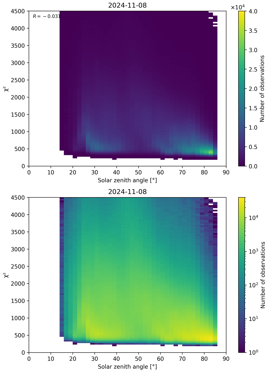
Figure 64: Scatter density plot of “Solar zenith angle” against “ \chi^2 ” for 2024-11-07 to 2024-11-09.
