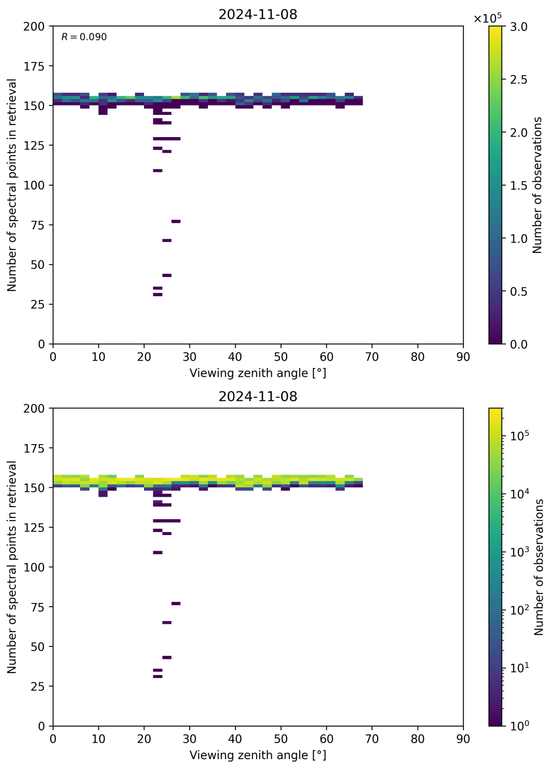
Figure 76: Scatter density plot of “Viewing zenith angle” against “Number of spectral points in retrieval” for 2024-11-07 to 2024-11-09.
