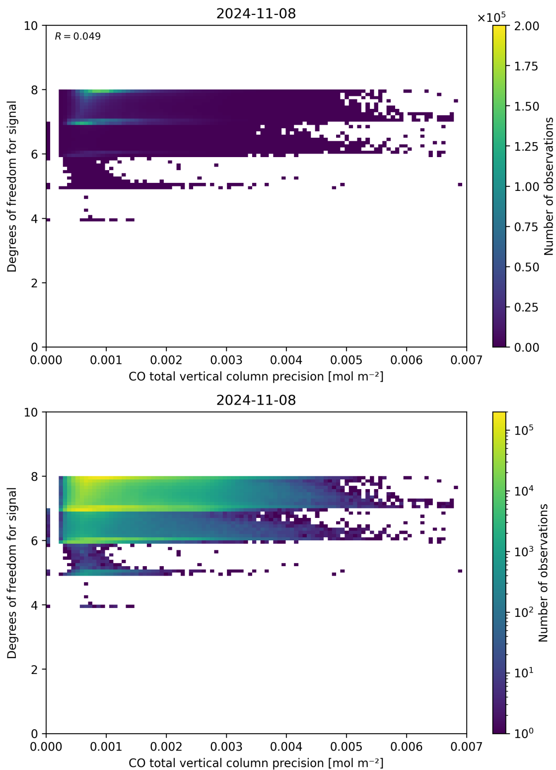
Figure 45: Scatter density plot of “CO total vertical column precision” against “Degrees of freedom for signal” for 2024-11-07 to 2024-11-09.
