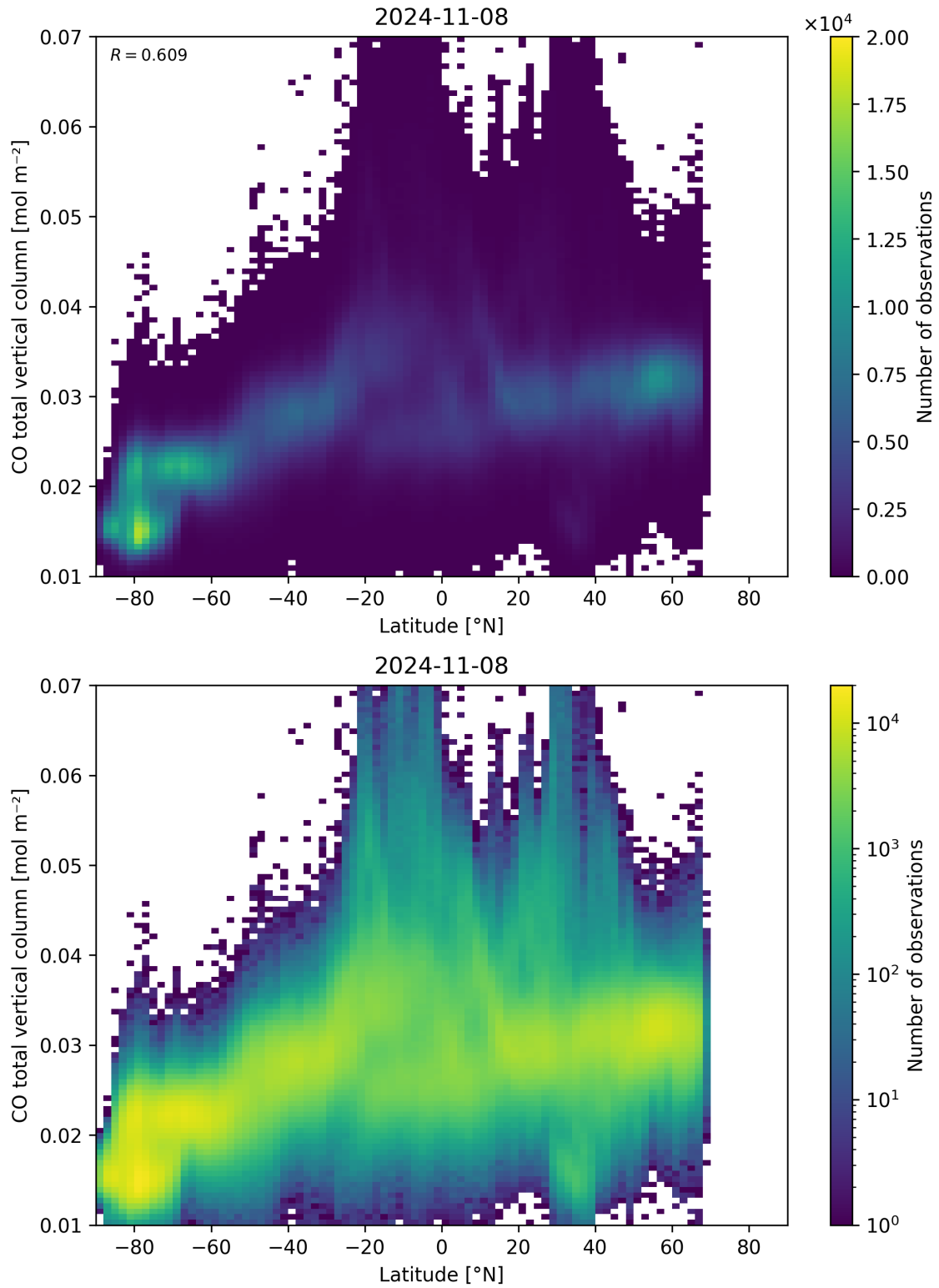
Figure 51: Scatter density plot of “Latitude” against “CO total vertical column” for 2024-11-07 to 2024-11-09.
