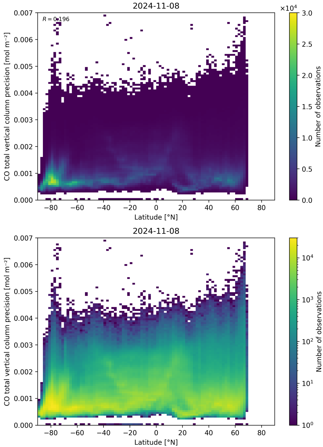
Figure 53: Scatter density plot of “Latitude” against “CO total vertical column precision” for 2024-11-07 to 2024-11-09.
