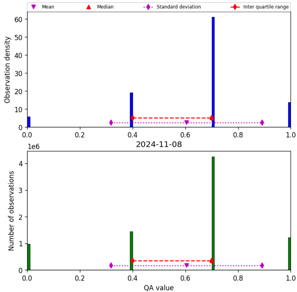
Figure 17: Histogram of “QA value” for 2024-11-07 to 2024-11-09
