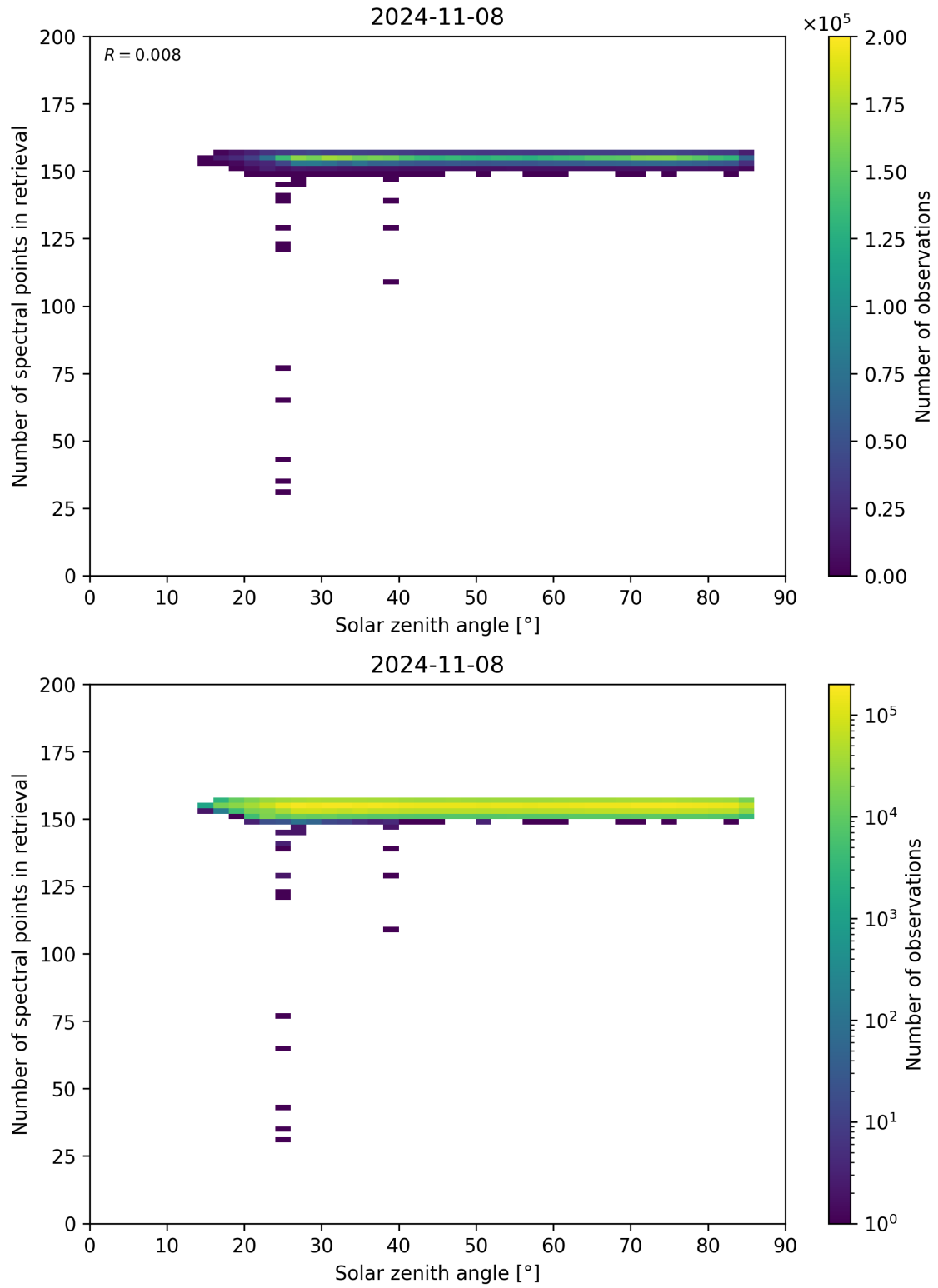
Figure 68: Scatter density plot of “Solar zenith angle” against “Number of spectral points in retrieval” for 2024-11-07 to 2024-11-09.
