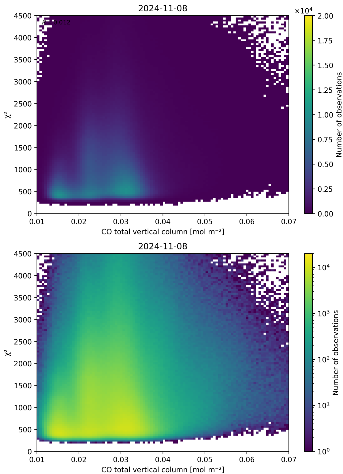
Figure 35: Scatter density plot of “CO total vertical column” against “ \chi^2 ” for 2024-11-07 to 2024-11-09.
