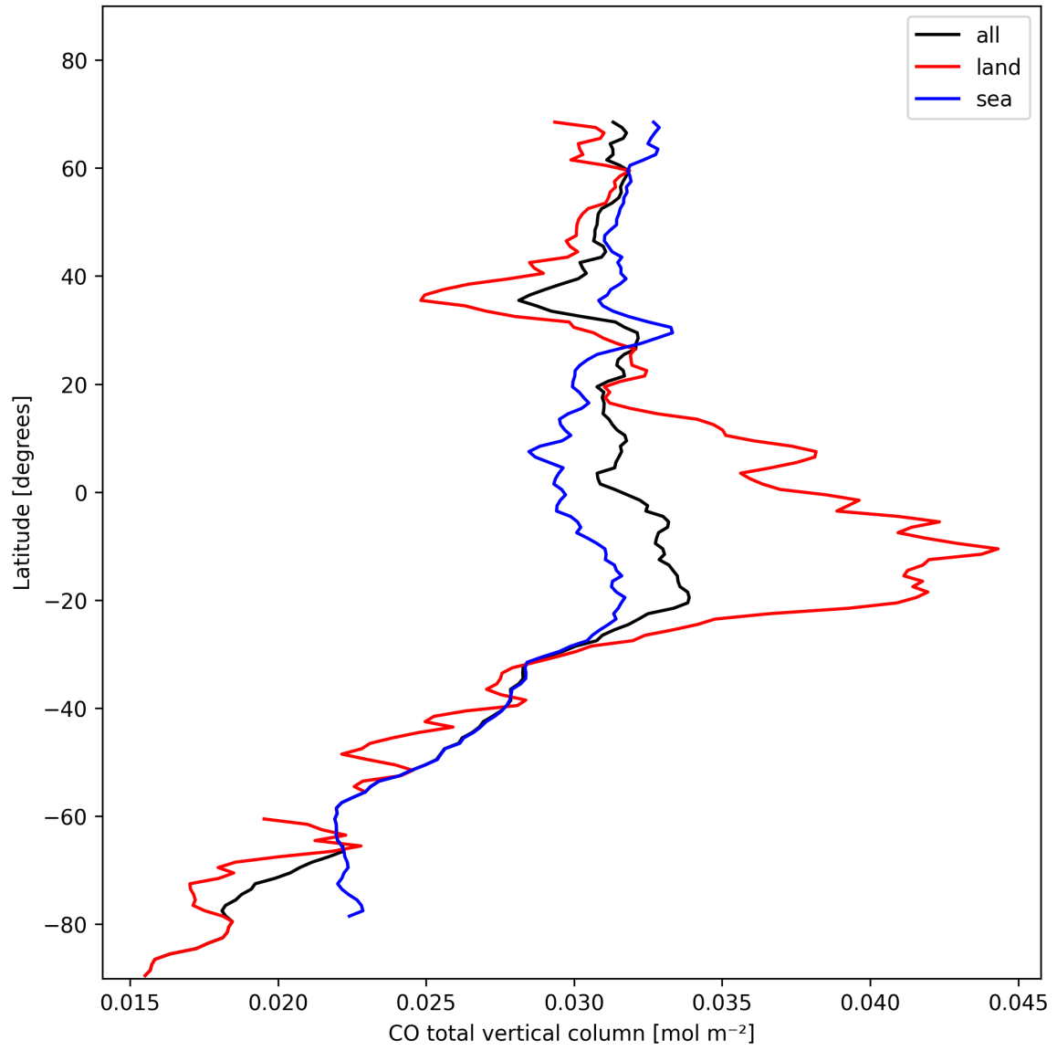
Figure 10: Zonal average of “CO total vertical column” for 2024-11-07 to 2024-11-09.
