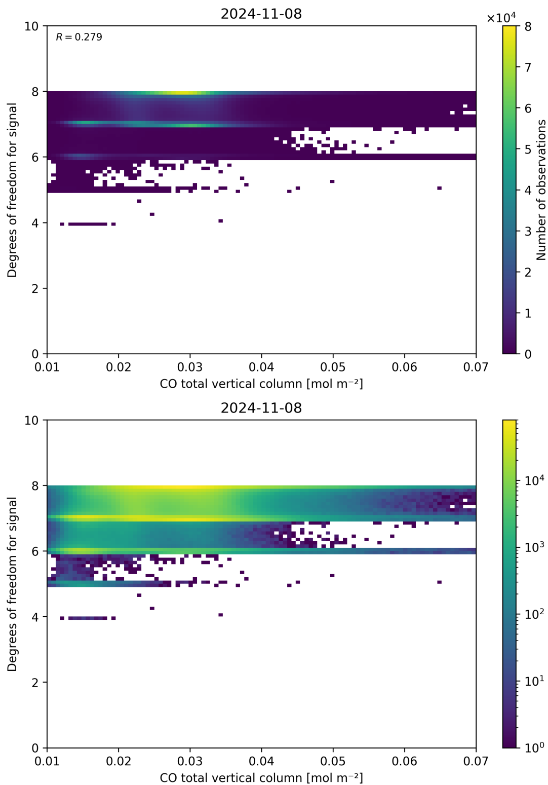
Figure 41: Scatter density plot of “CO total vertical column” against “Degrees of freedom for signal” for 2024-11-07 to 2024-11-09.
