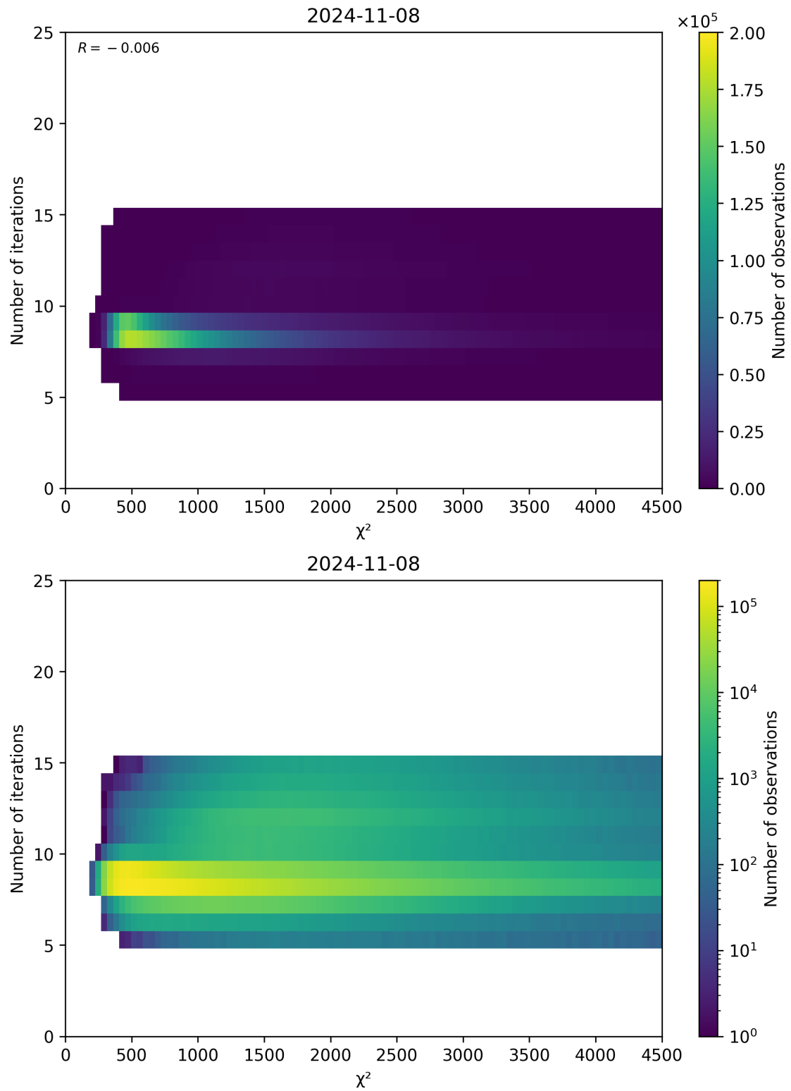
Figure 49: Scatter density plot of “ \chi^2 ” against “Number of iterations” for 2024-11-07 to 2024-11-09.
