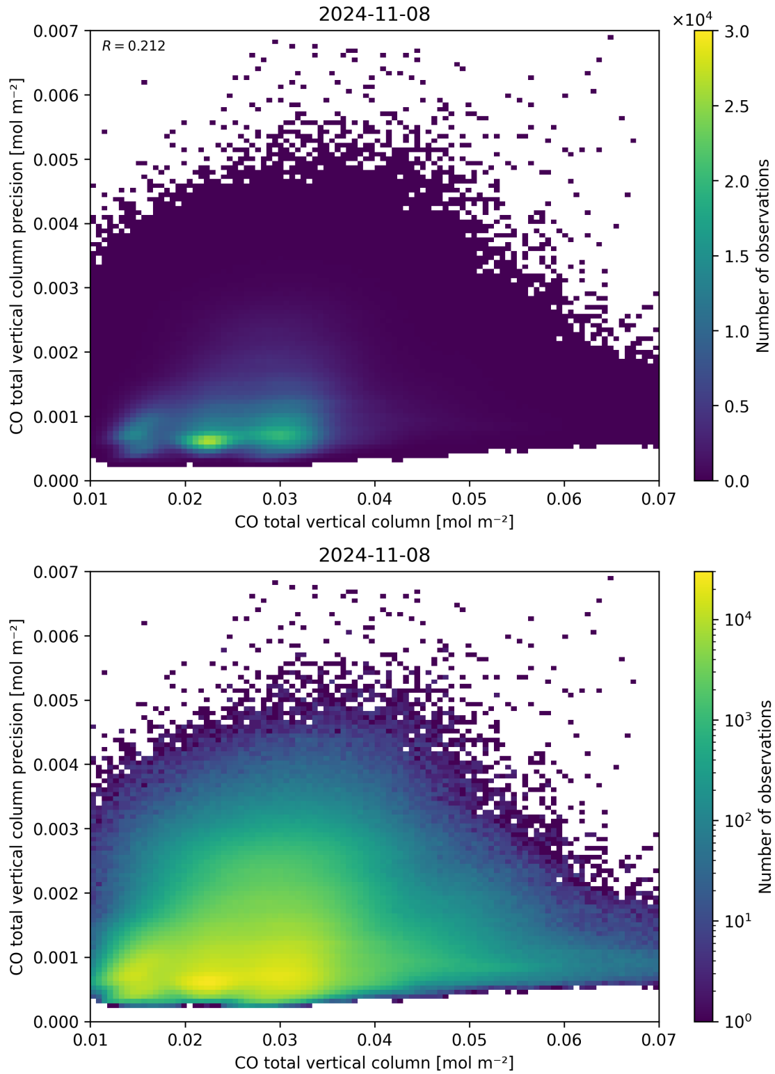
Figure 34: Scatter density plot of “CO total vertical column” against “CO total vertical column precision” for 2024-11-07 to 2024-11-09.
