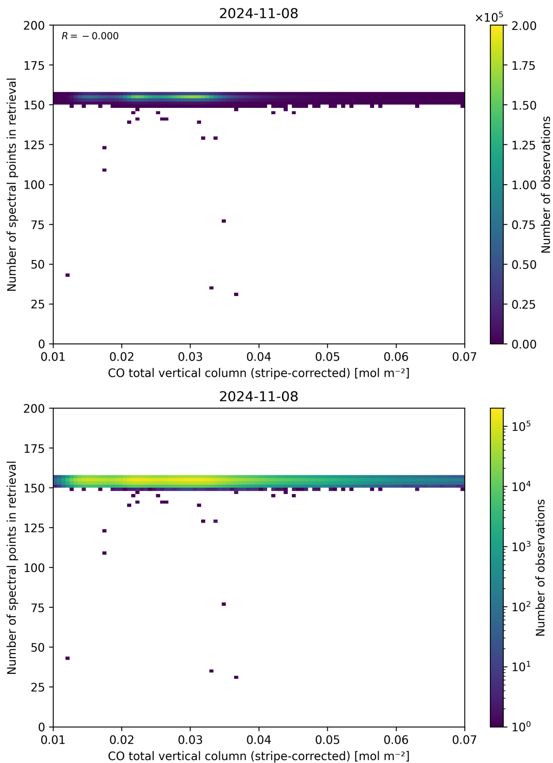
Figure 40: Scatter density plot of “CO total vertical column (stripe-corrected)” against “Number of spectral points in retrieval” for 2024-11-07 to 2024-11-09.
