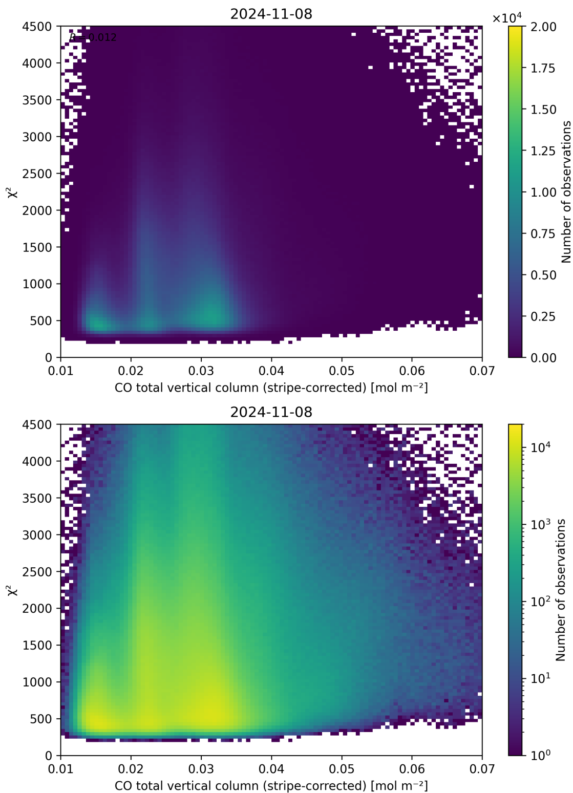
Figure 37: Scatter density plot of “CO total vertical column (stripe-corrected)” against “ \chi^2 ” for 2024-11-07 to 2024-11-09.
