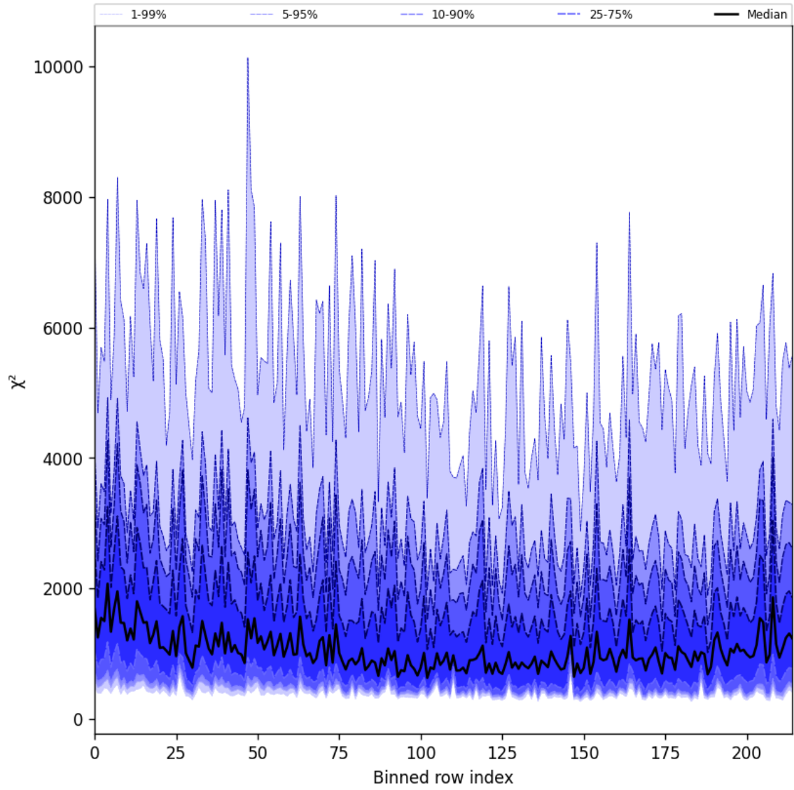
Figure 30: Along track statistics of “ \chi^2 ” for 2024-11-07 to 2024-11-09
