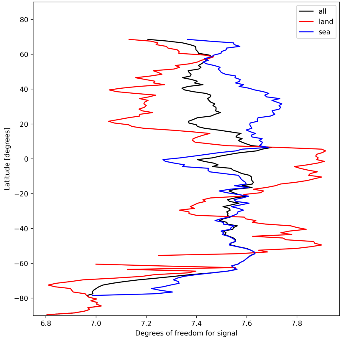
Figure 15: Zonal average of “Degrees of freedom for signal” for 2024-11-07 to 2024-11-09.
