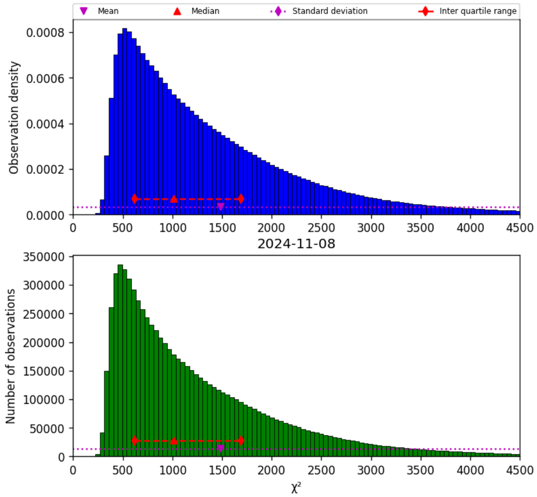
Figure 22: Histogram of “ \chi^2 ” for 2024-11-07 to 2024-11-09
