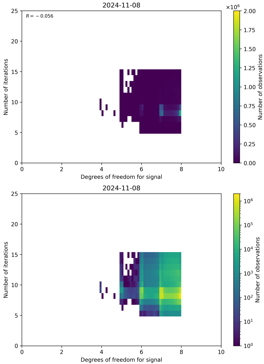
Figure 50: Scatter density plot of “Degrees of freedom for signal” against “Number of iterations” for 2024-11-07 to 2024-11-09.
