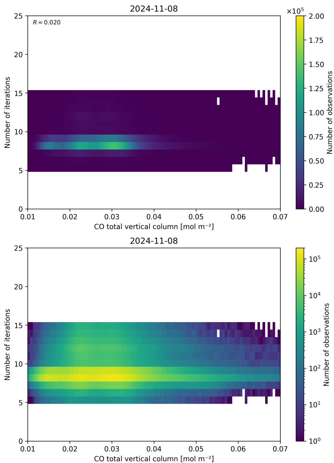
Figure 42: Scatter density plot of “CO total vertical column” against “Number of iterations” for 2024-11-07 to 2024-11-09.
