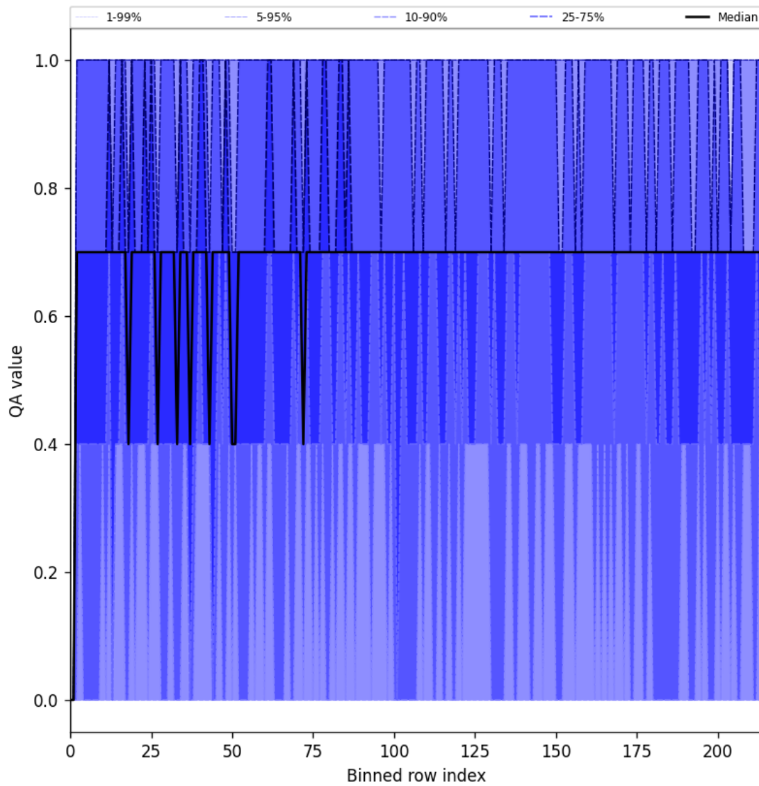
Figure 25: Along track statistics of “QA value” for 2024-11-07 to 2024-11-09
