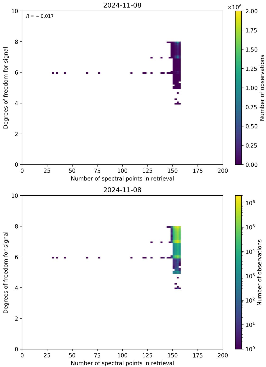
Figure 59: Scatter density plot of “Number of spectral points in retrieval” against “Degrees of freedom for signal” for 2024-11-07 to 2024-11-09.
