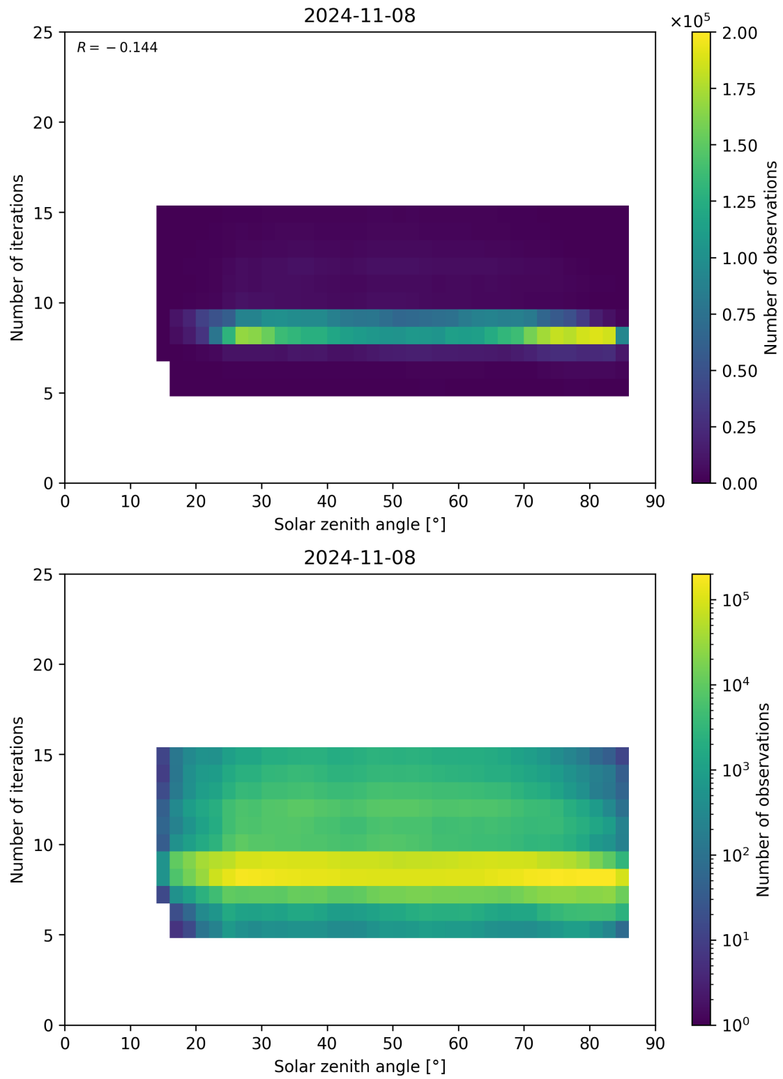
Figure 67: Scatter density plot of “Solar zenith angle” against “Number of iterations” for 2024-11-07 to 2024-11-09.
