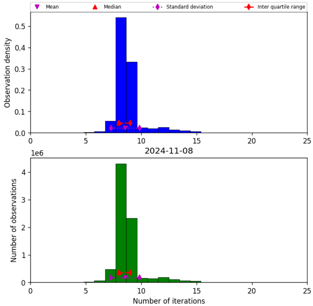
Figure 24: Histogram of “Number of iterations” for 2024-11-07 to 2024-11-09
