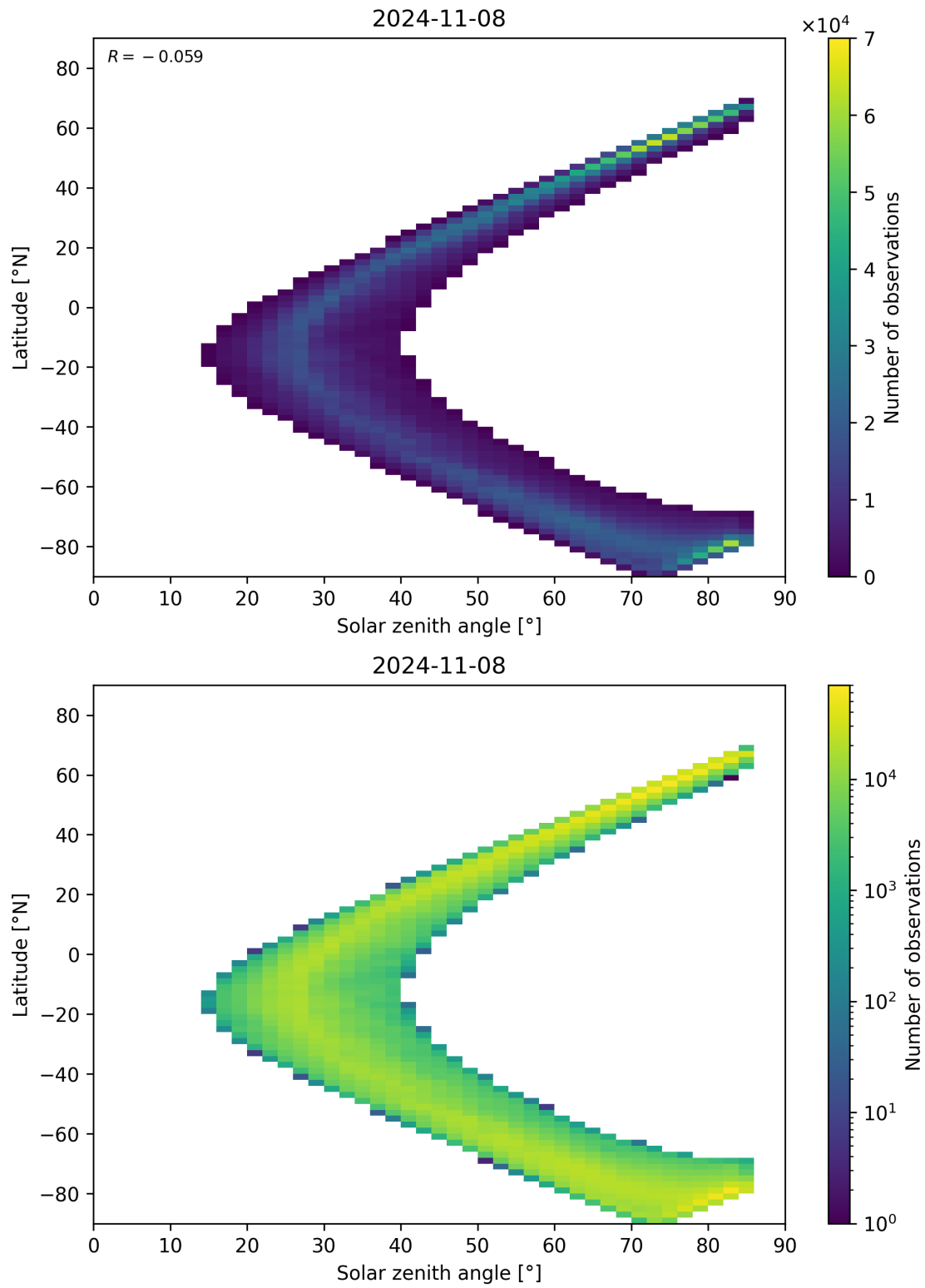
Figure 66: Scatter density plot of “Solar zenith angle” against “Latitude” for 2024-11-07 to 2024-11-09.
