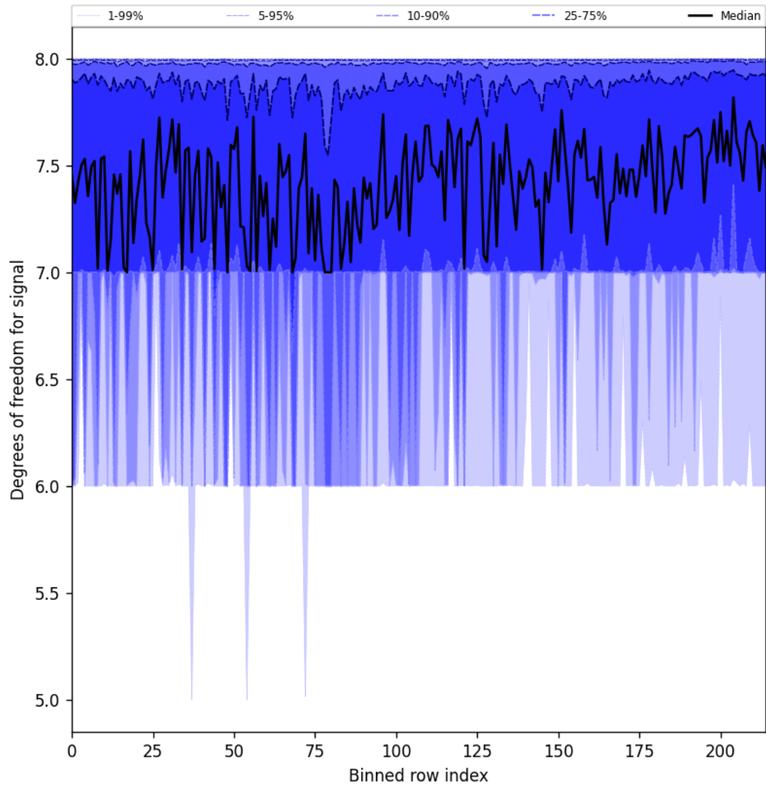
Figure 31: Along track statistics of “Degrees of freedom for signal” for 2024-11-07 to 2024-11-09
