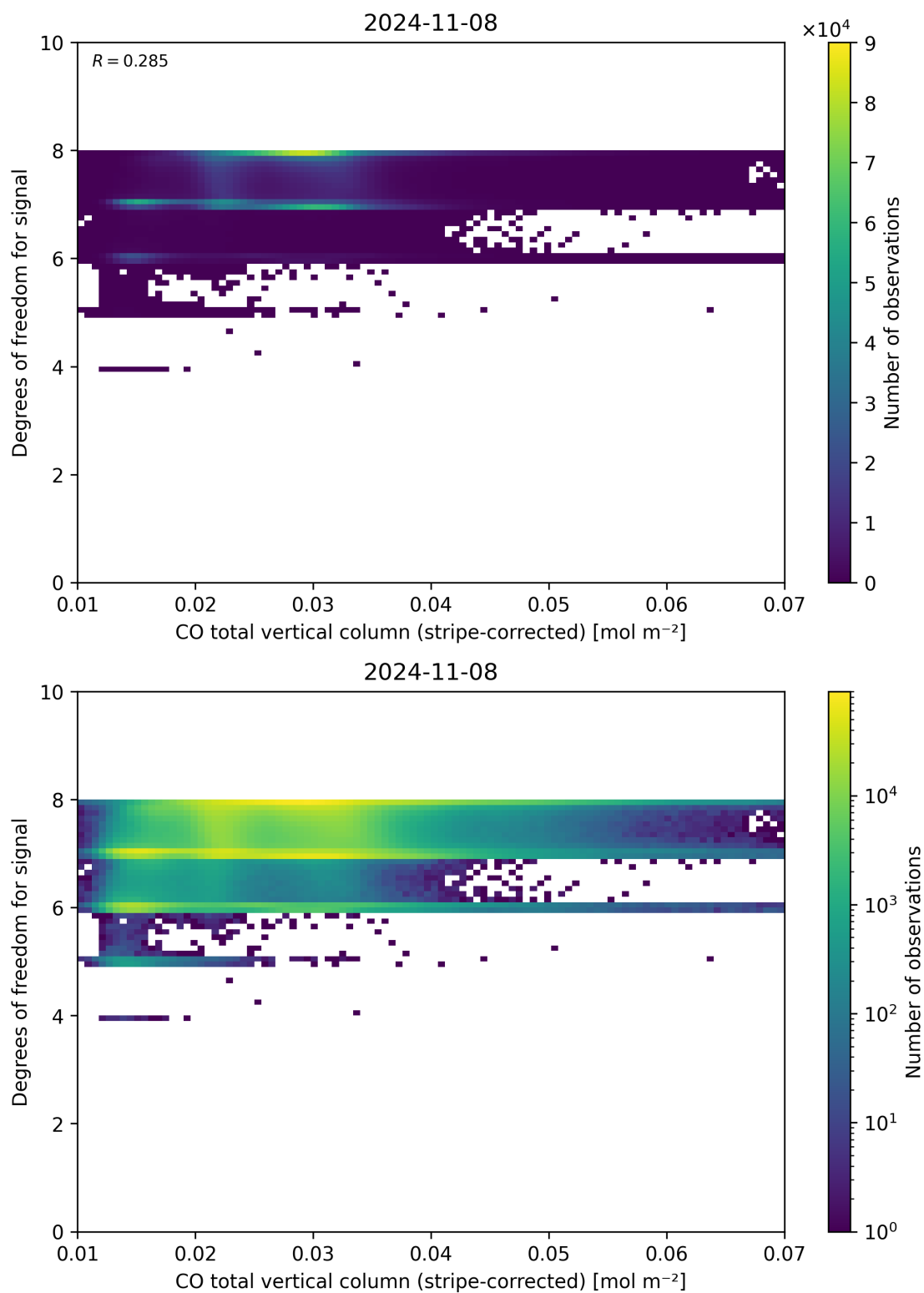
Figure 38: Scatter density plot of “CO total vertical column (stripe-corrected)” against “Degrees of freedom for signal” for 2024-11-07 to 2024-11-09.
