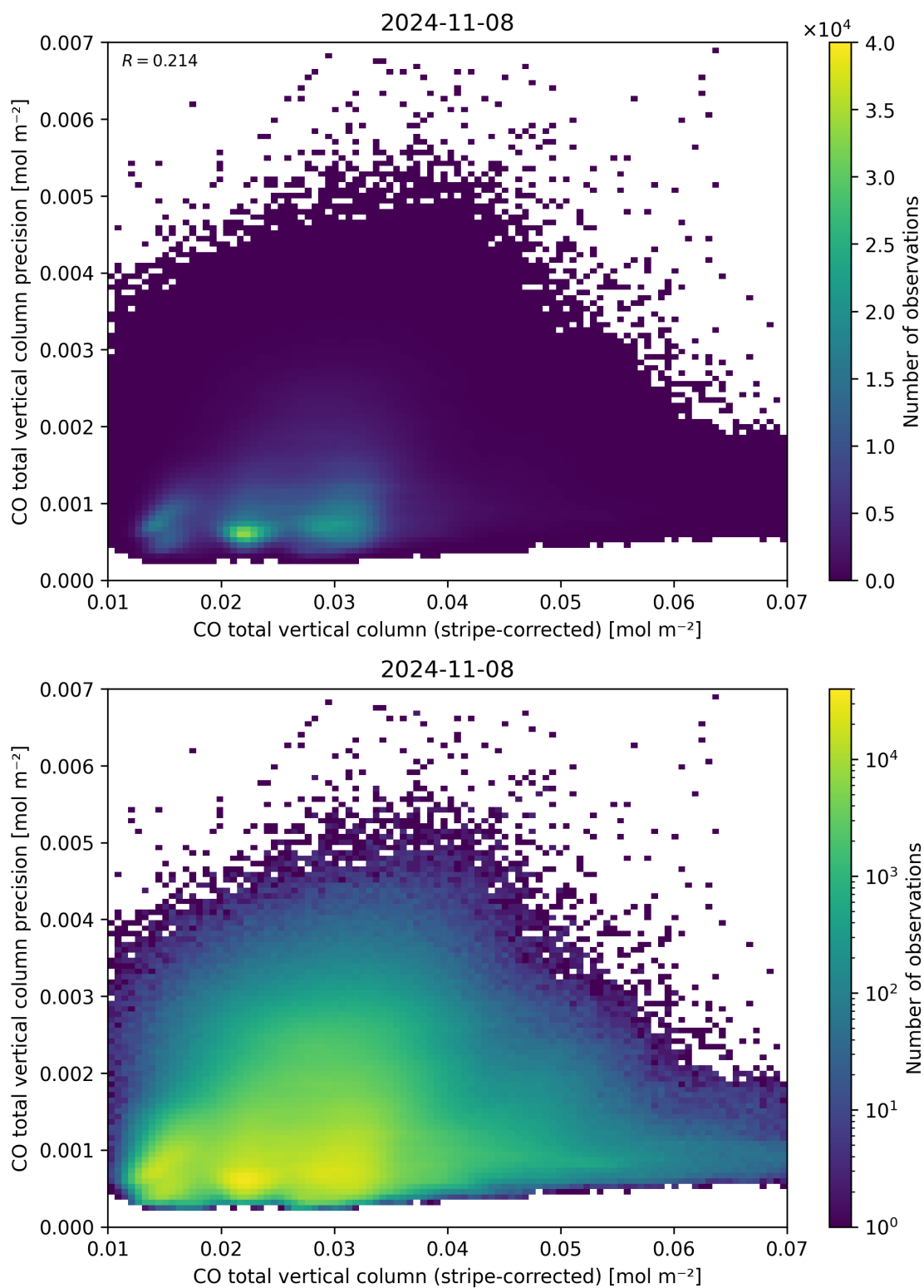
Figure 36: Scatter density plot of “CO total vertical column (stripe-corrected)” against “CO total vertical column precision” for 2024-11-07 to 2024-11-09.
