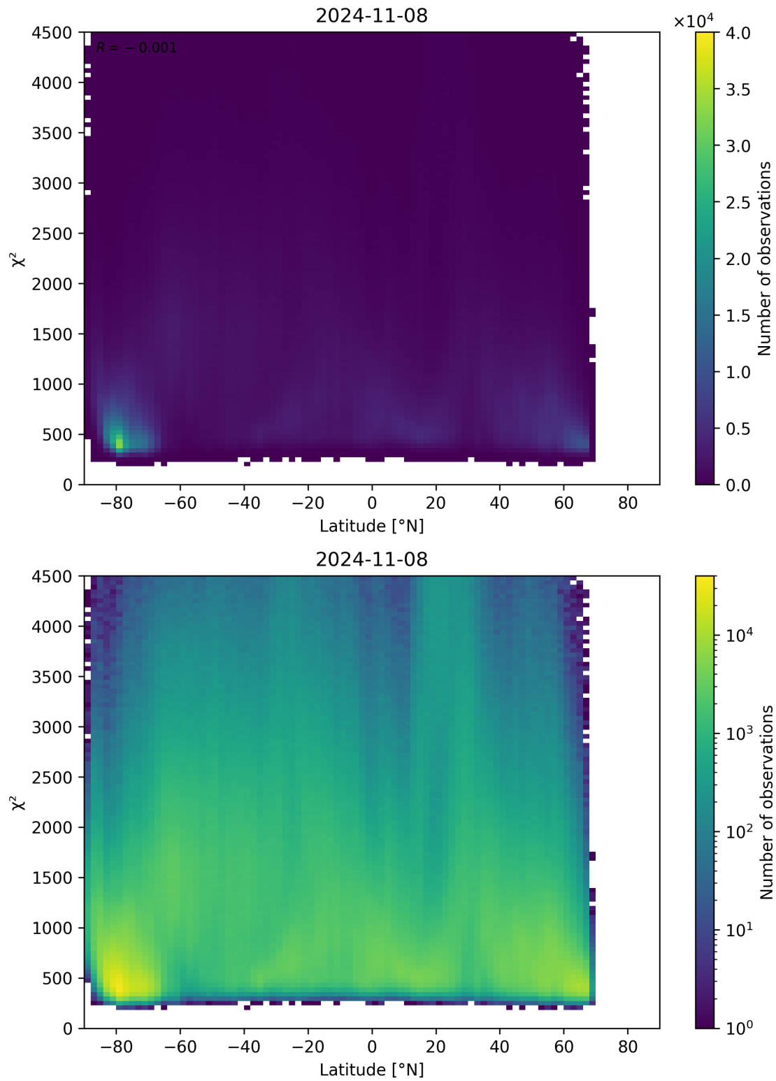
Figure 54: Scatter density plot of “Latitude” against “ \chi^2 ” for 2024-11-07 to 2024-11-09.
