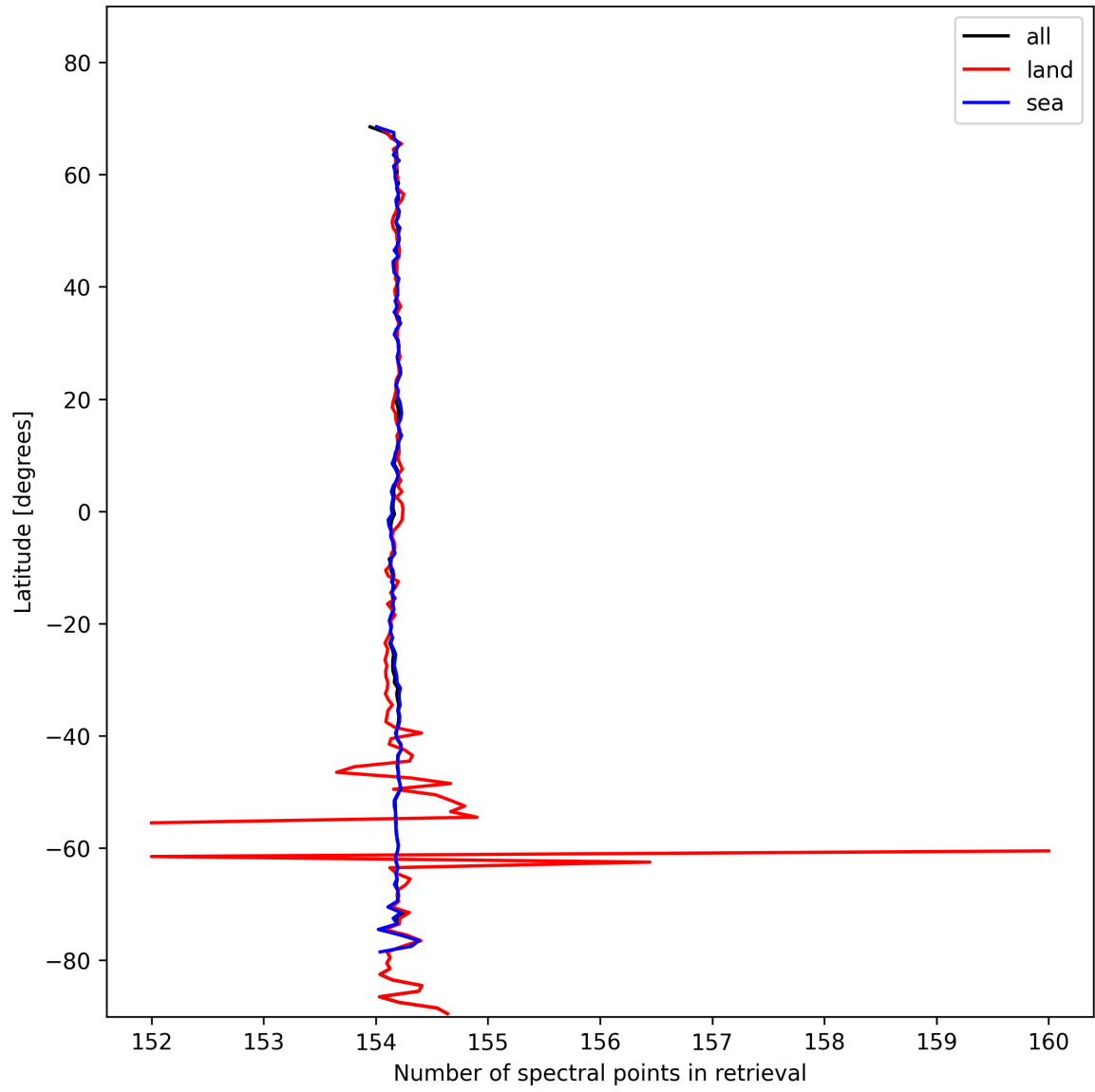
Figure 13: Zonal average of “Number of spectral points in retrieval” for 2024-11-07 to 2024-11-09.
