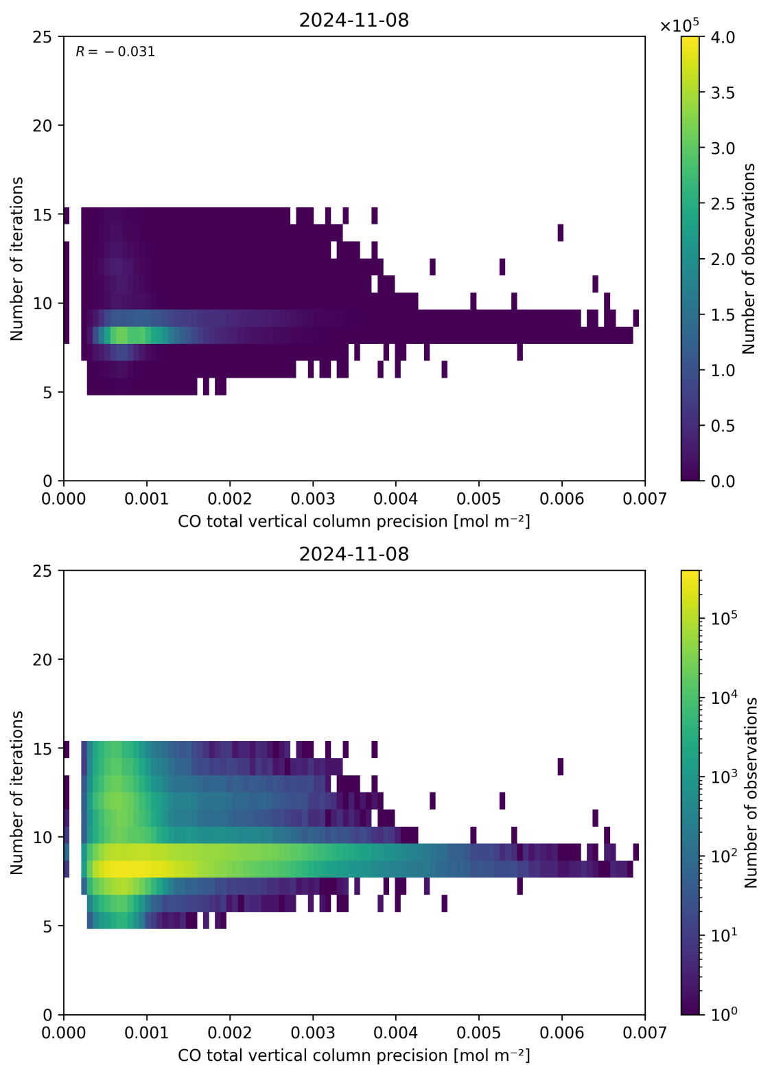
Figure 46: Scatter density plot of “CO total vertical column precision” against “Number of iterations” for 2024-11-07 to 2024-11-09.
