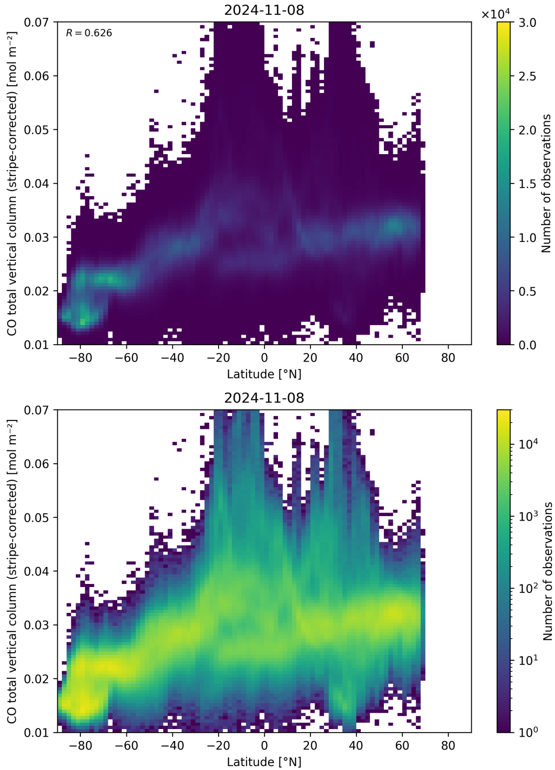
Figure 52: Scatter density plot of “Latitude” against “CO total vertical column (stripe-corrected)” for 2024-11-07 to 2024-11-09.
