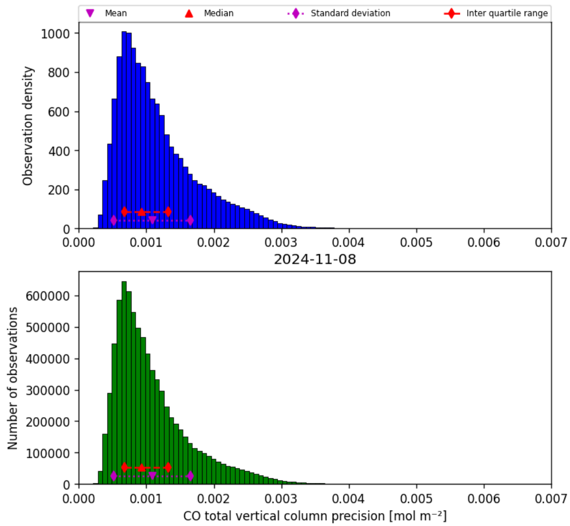
Figure 20: Histogram of “CO total vertical column precision” for 2024-11-07 to 2024-11-09
