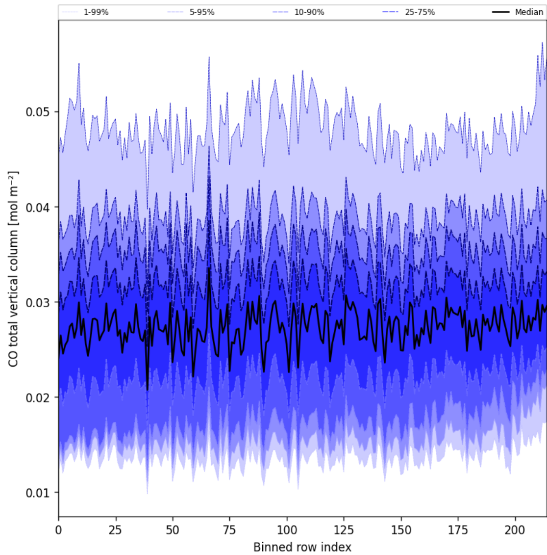
Figure 26: Along track statistics of “CO total vertical column” for 2024-11-07 to 2024-11-09
