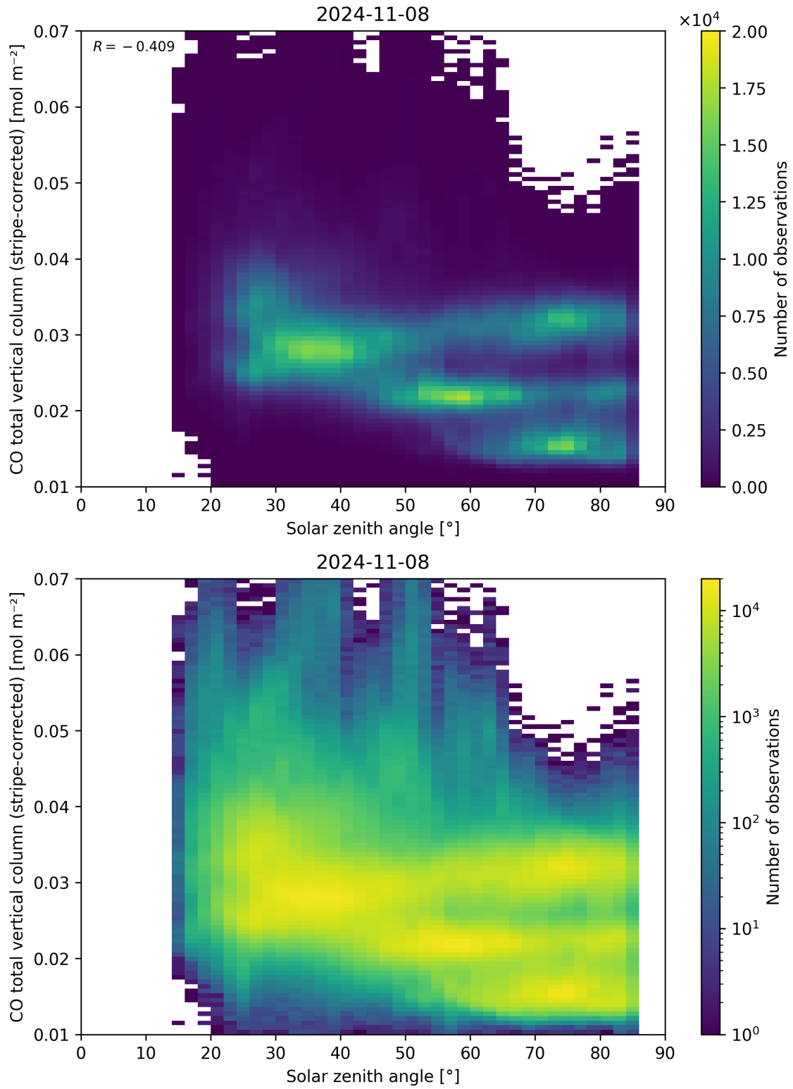
Figure 62: Scatter density plot of “Solar zenith angle” against “CO total vertical column (stripe-corrected)” for 2024-11-07 to 2024-11-09.
