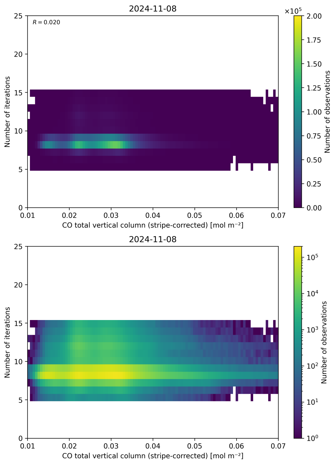
Figure 39: Scatter density plot of “CO total vertical column (stripe-corrected)” against “Number of iterations” for 2024-11-07 to 2024-11-09.
