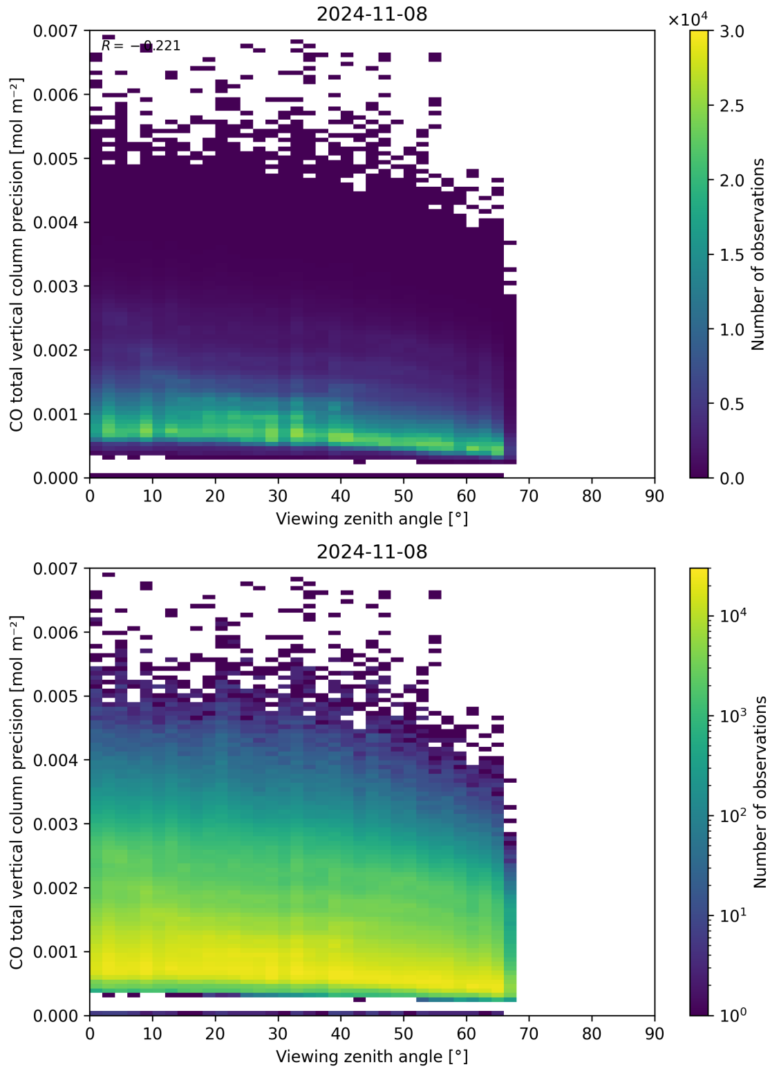
Figure 71: Scatter density plot of “Viewing zenith angle” against “CO total vertical column precision” for 2024-11-07 to 2024-11-09.
