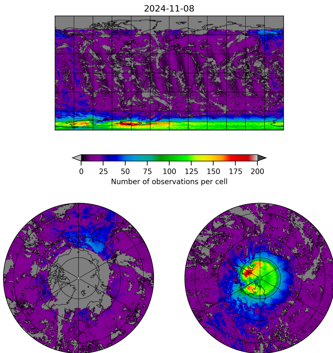
Figure 8: Map of the number of observations for 2024-11-07 to 2024-11-09
