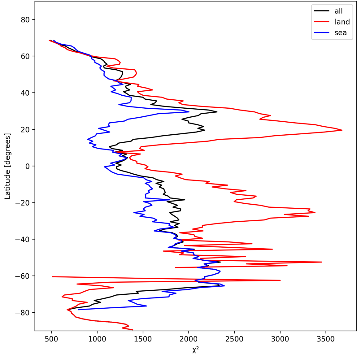
Figure 14: Zonal average of “ \chi^2 ” for 2024-11-07 to 2024-11-09.
