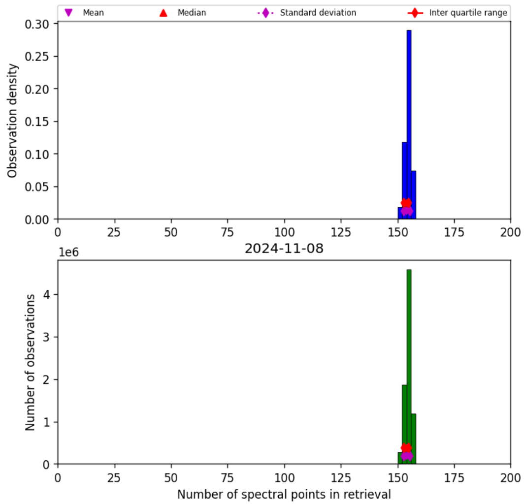
Figure 21: Histogram of “Number of spectral points in retrieval” for 2024-11-07 to 2024-11-09
