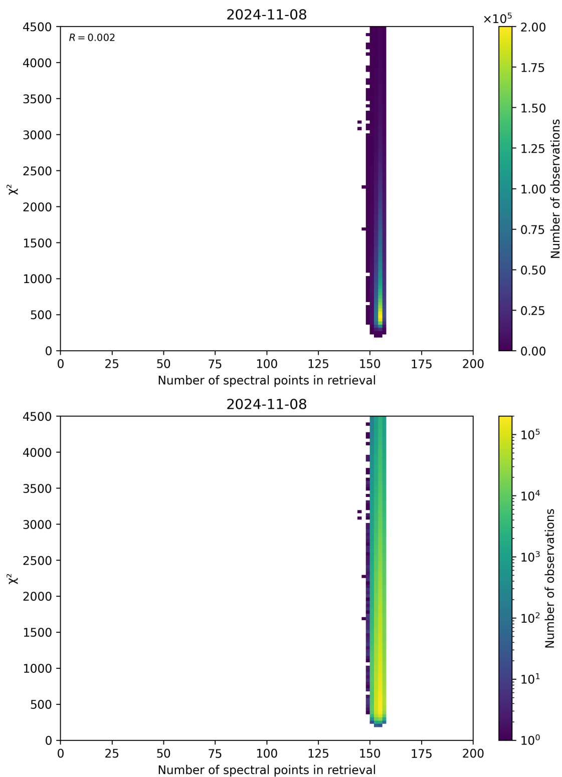
Figure 58: Scatter density plot of “Number of spectral points in retrieval” against “ \chi^2 ” for 2024-11-07 to 2024-11-09.
