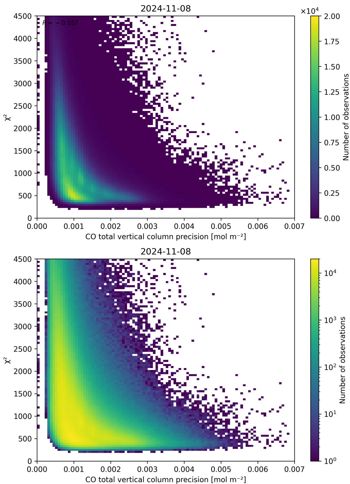
Figure 44: Scatter density plot of “CO total vertical column precision” against “ \chi^2 ” for 2024-11-07 to 2024-11-09.
