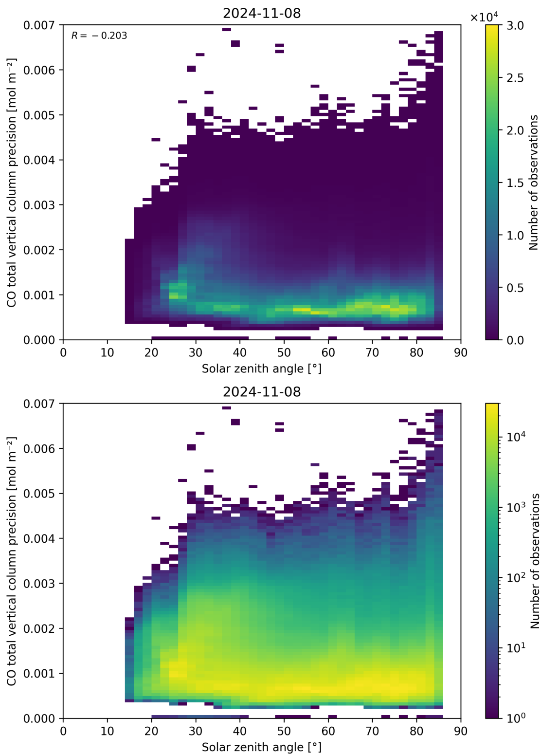
Figure 63: Scatter density plot of “Solar zenith angle” against “CO total vertical column precision” for 2024-11-07 to 2024-11-09.
