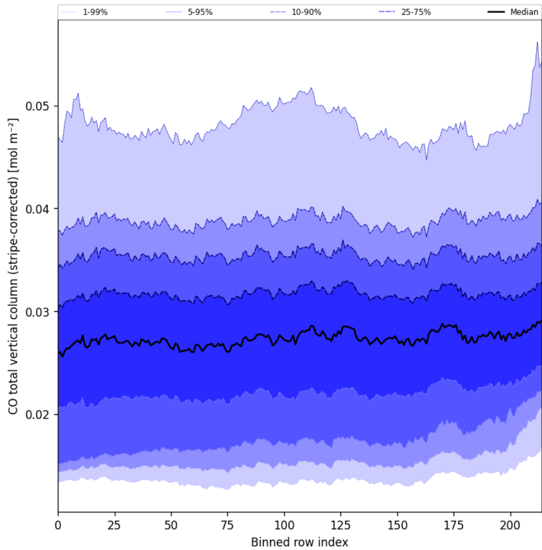
Figure 27: Along track statistics of “CO total vertical column (stripe-corrected)” for 2024-11-07 to 2024-11-09
