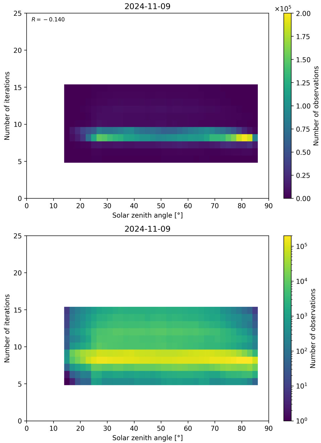
Figure 67: Scatter density plot of “Solar zenith angle” against “Number of iterations” for 2024-11-09 to 2024-11-10.
