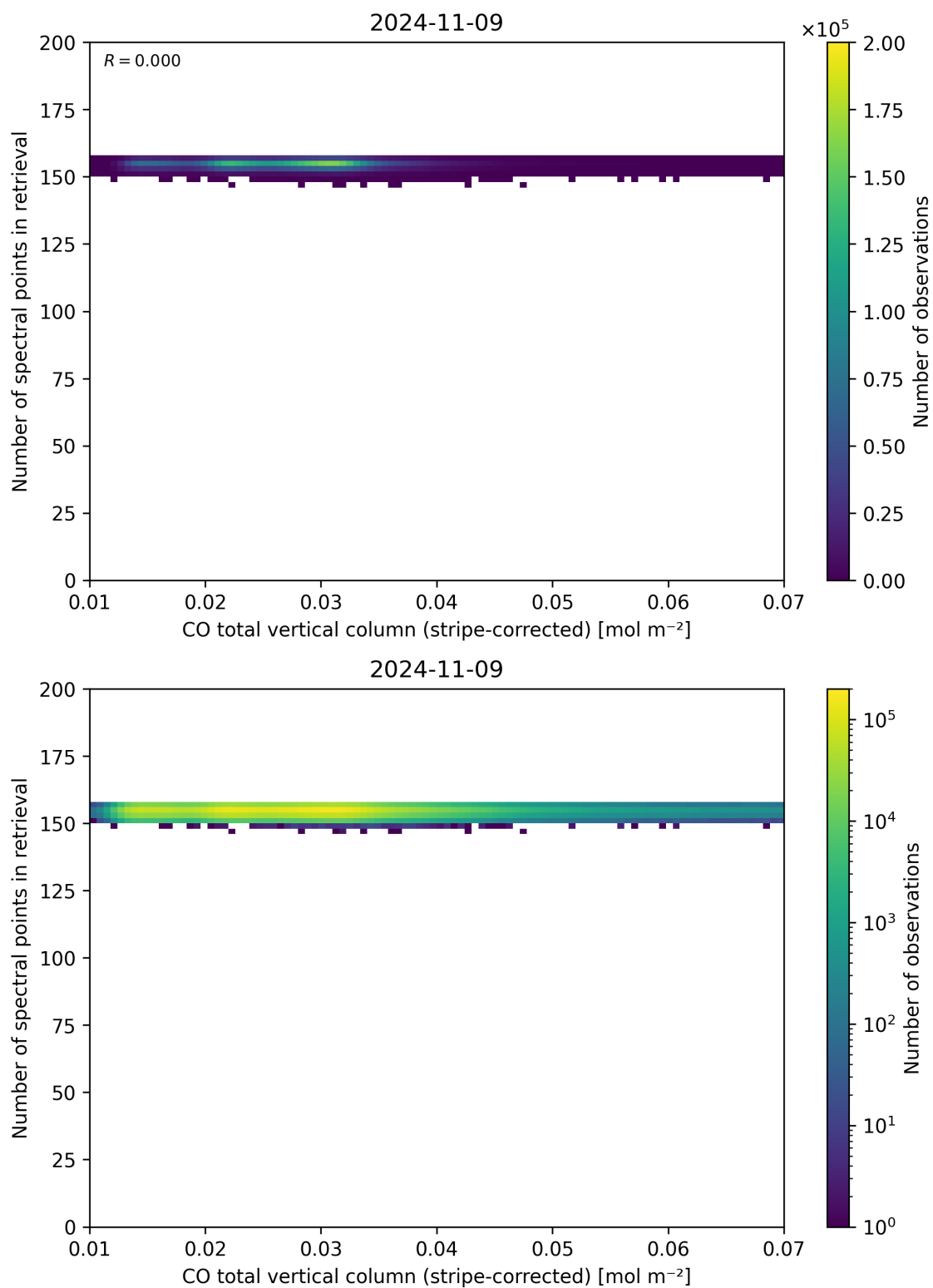
Figure 40: Scatter density plot of “CO total vertical column (stripe-corrected)” against “Number of spectral points in retrieval” for 2024-11-09 to 2024-11-10.
