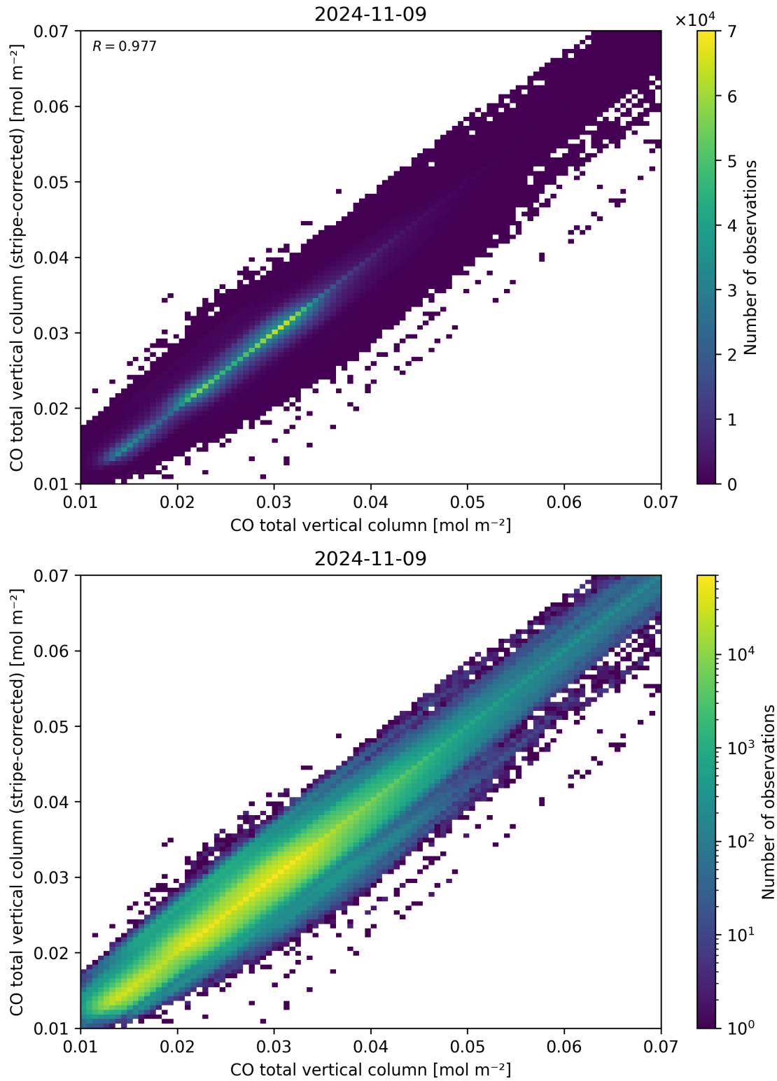
Figure 33: Scatter density plot of “CO total vertical column” against “CO total vertical column (stripe-corrected)” for 2024-11-09 to 2024-11-10.
