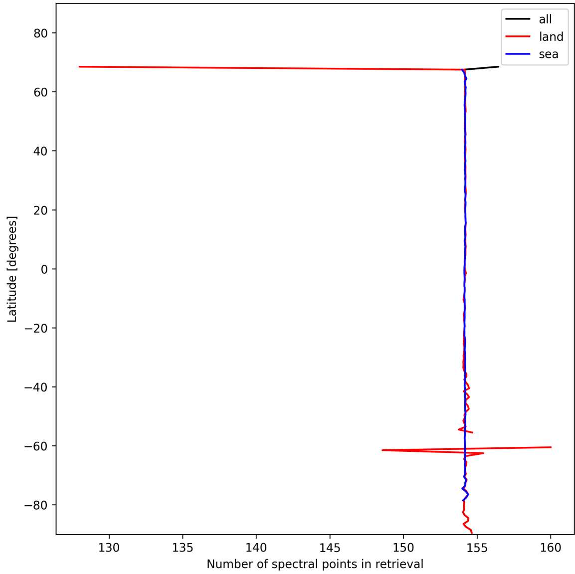
Figure 13: Zonal average of “Number of spectral points in retrieval” for 2024-11-09 to 2024-11-10.
