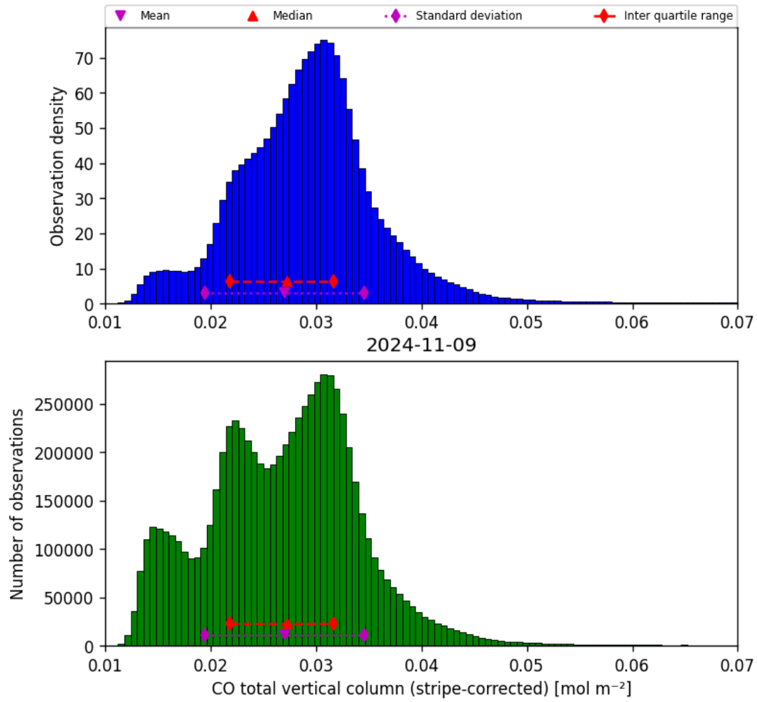
Figure 19: Histogram of “CO total vertical column (stripe-corrected)” for 2024-11-09 to 2024-11-10
