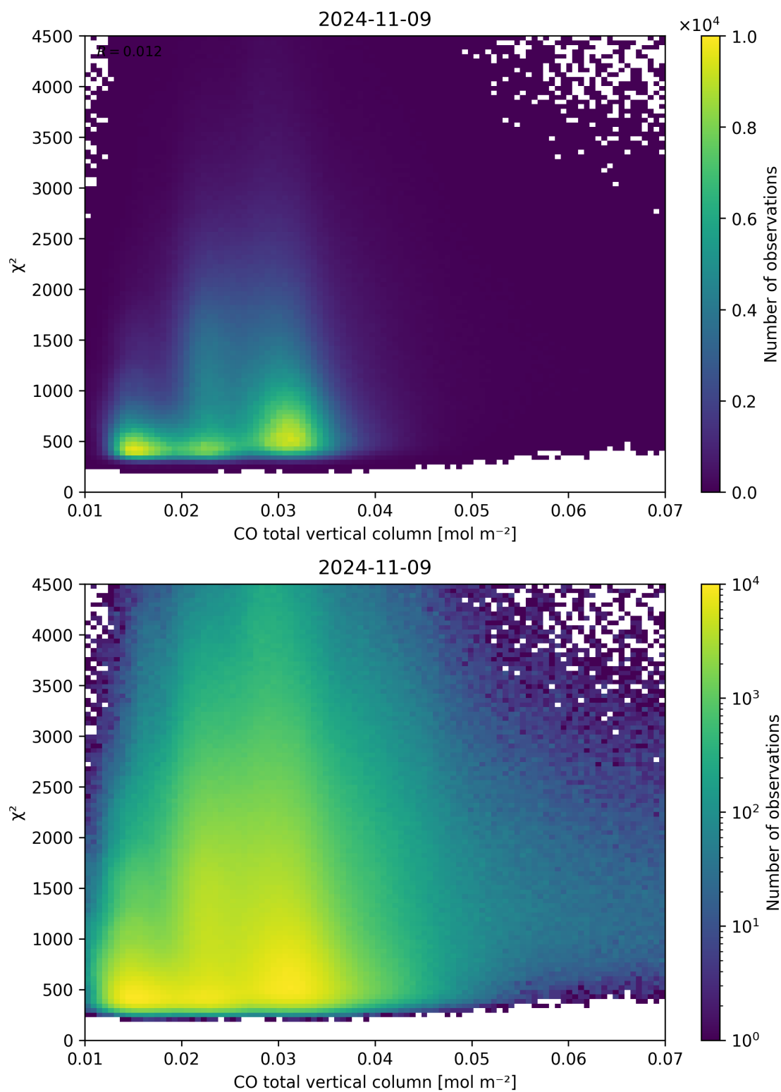
Figure 35: Scatter density plot of “CO total vertical column” against “ \chi^2 ” for 2024-11-09 to 2024-11-10.
