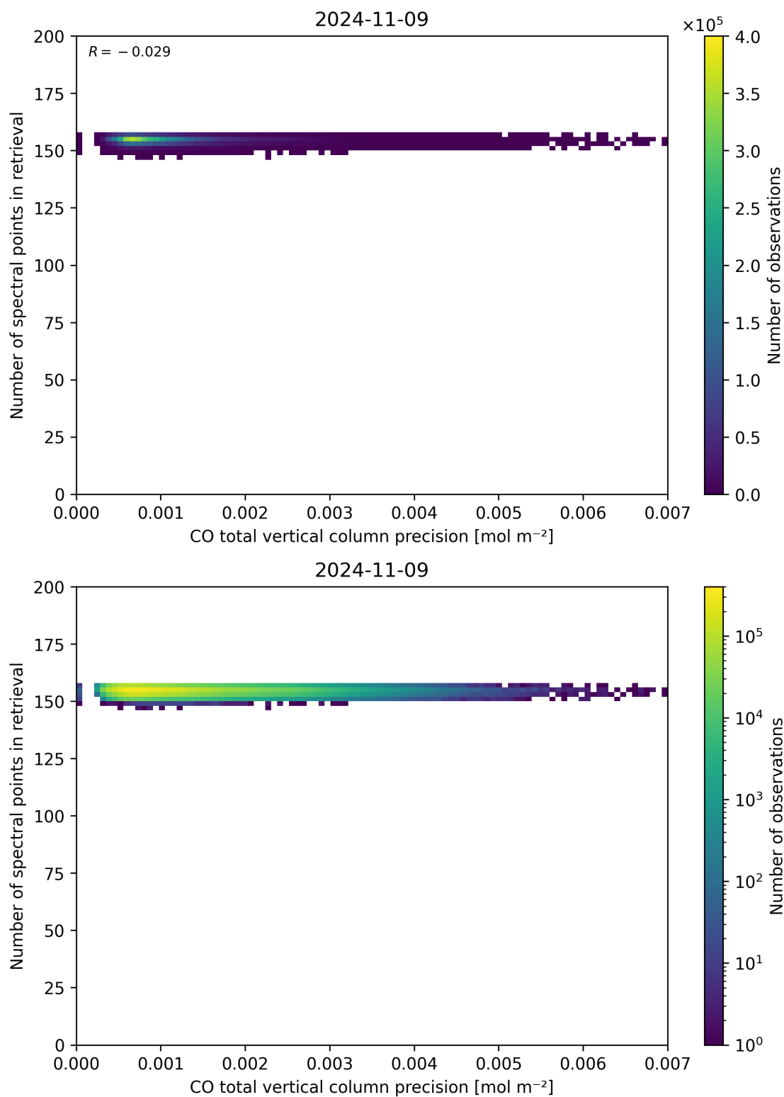
Figure 47: Scatter density plot of “CO total vertical column precision” against “Number of spectral points in retrieval” for 2024-11-09 to 2024-11-10.
