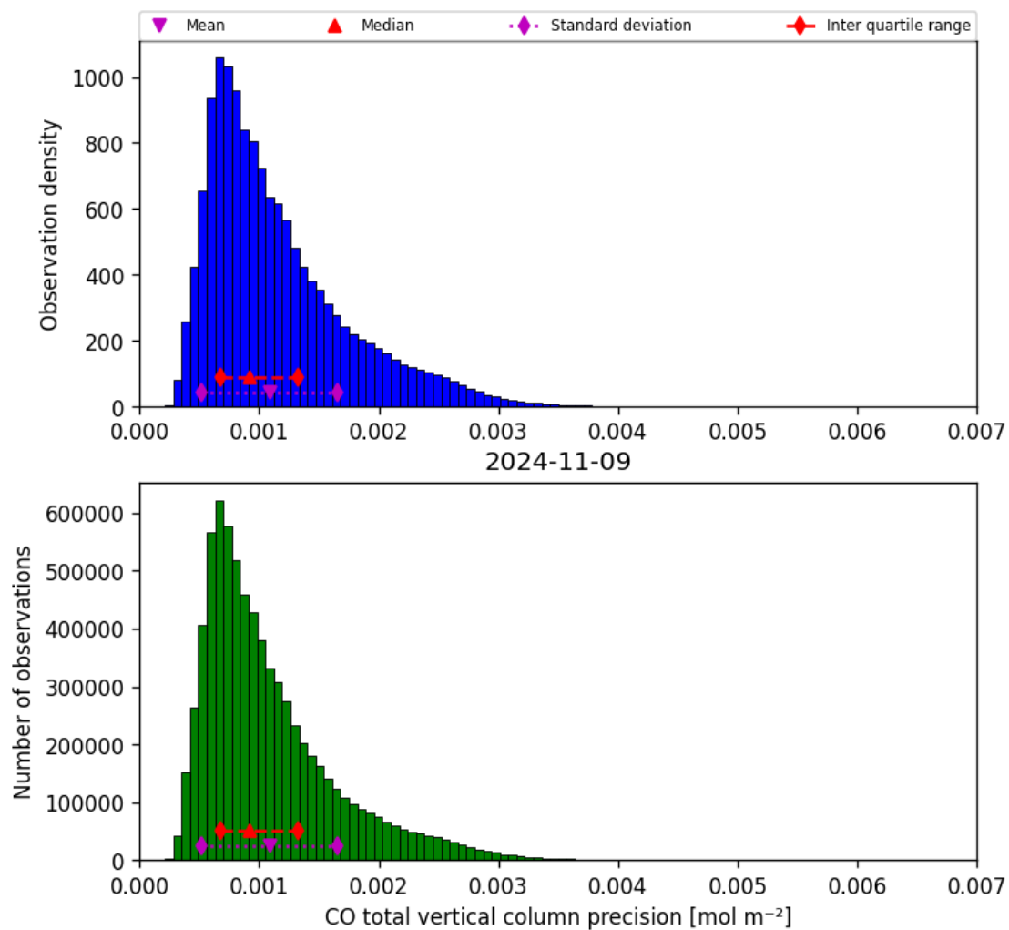
Figure 20: Histogram of “CO total vertical column precision” for 2024-11-09 to 2024-11-10
