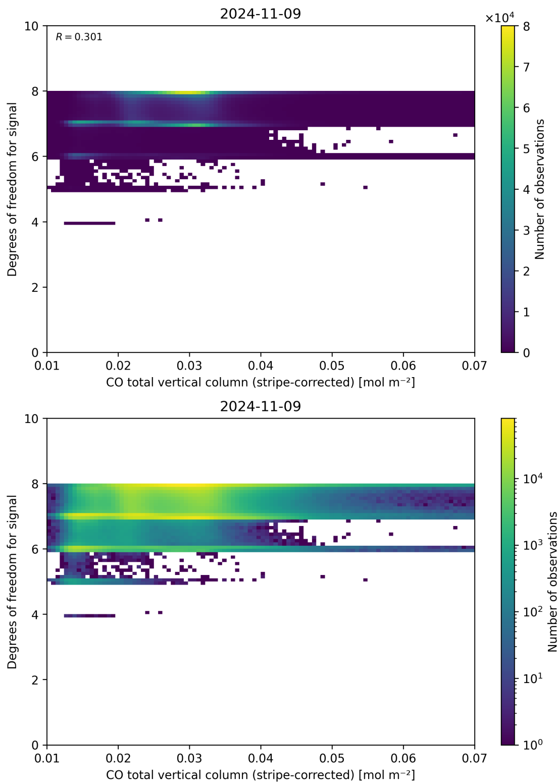
Figure 38: Scatter density plot of “CO total vertical column (stripe-corrected)” against “Degrees of freedom for signal” for 2024-11-09 to 2024-11-10.
