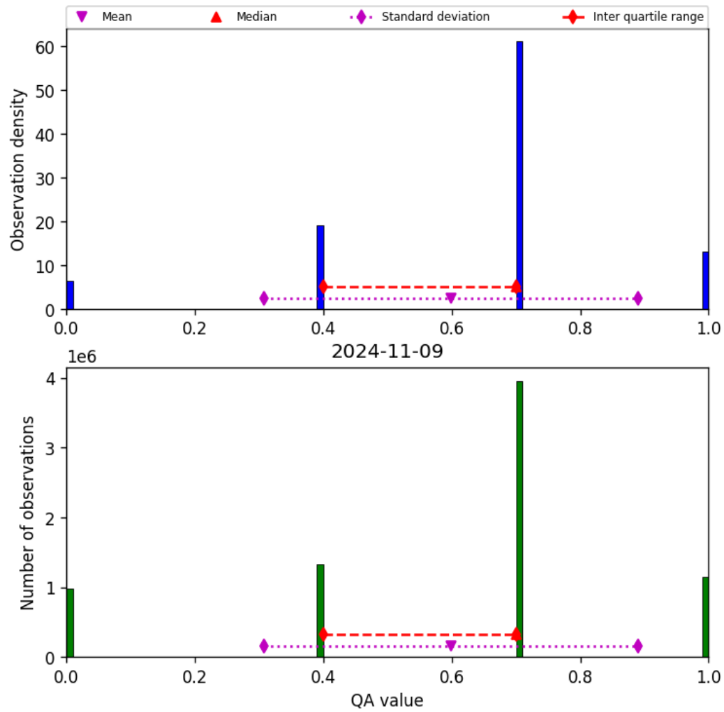
Figure 17: Histogram of "QA value" for 2024-11-09 to 2024-11-10
