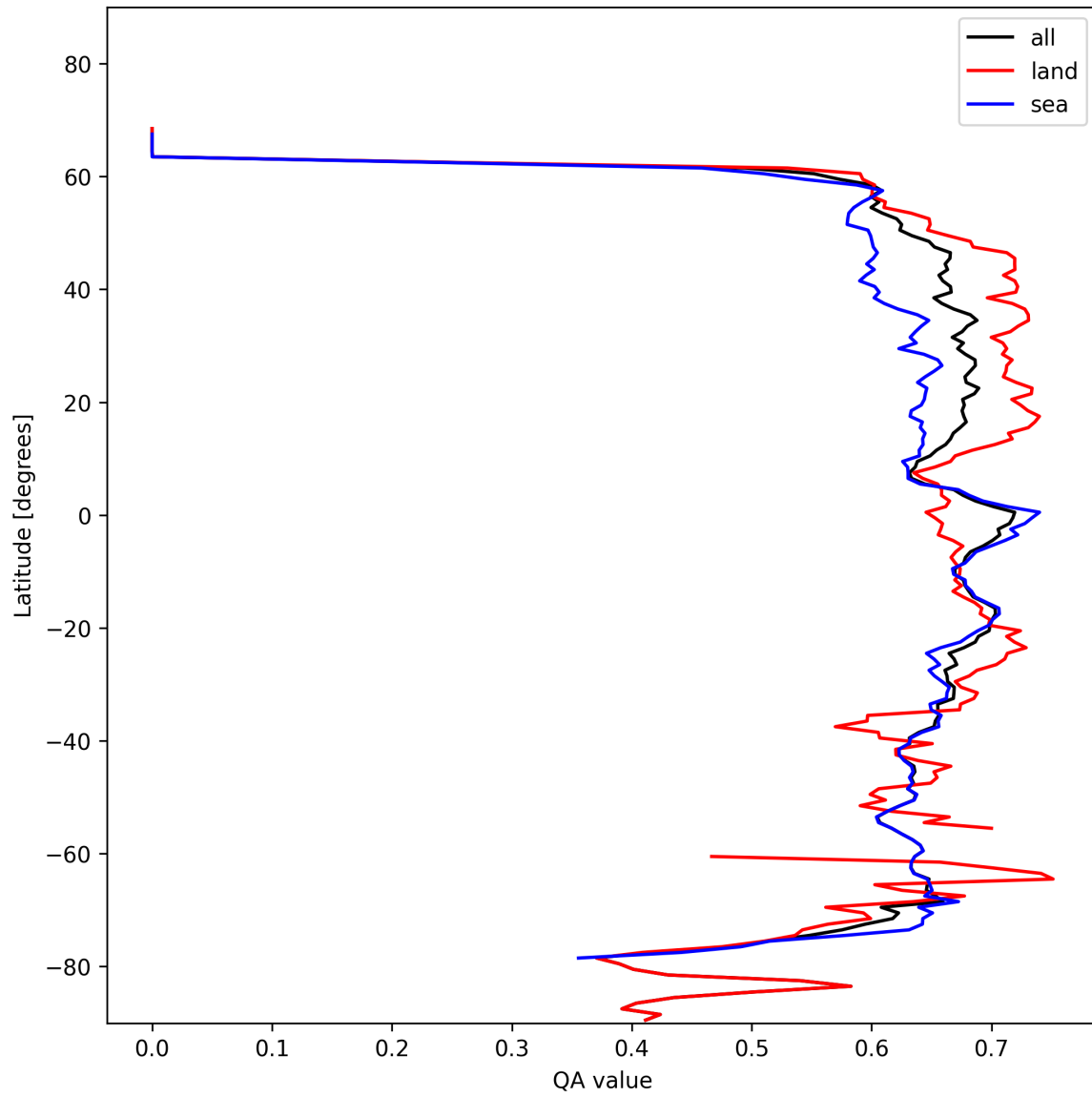
Figure 9: Zonal average of “QA value” for 2024-11-09 to 2024-11-10.
