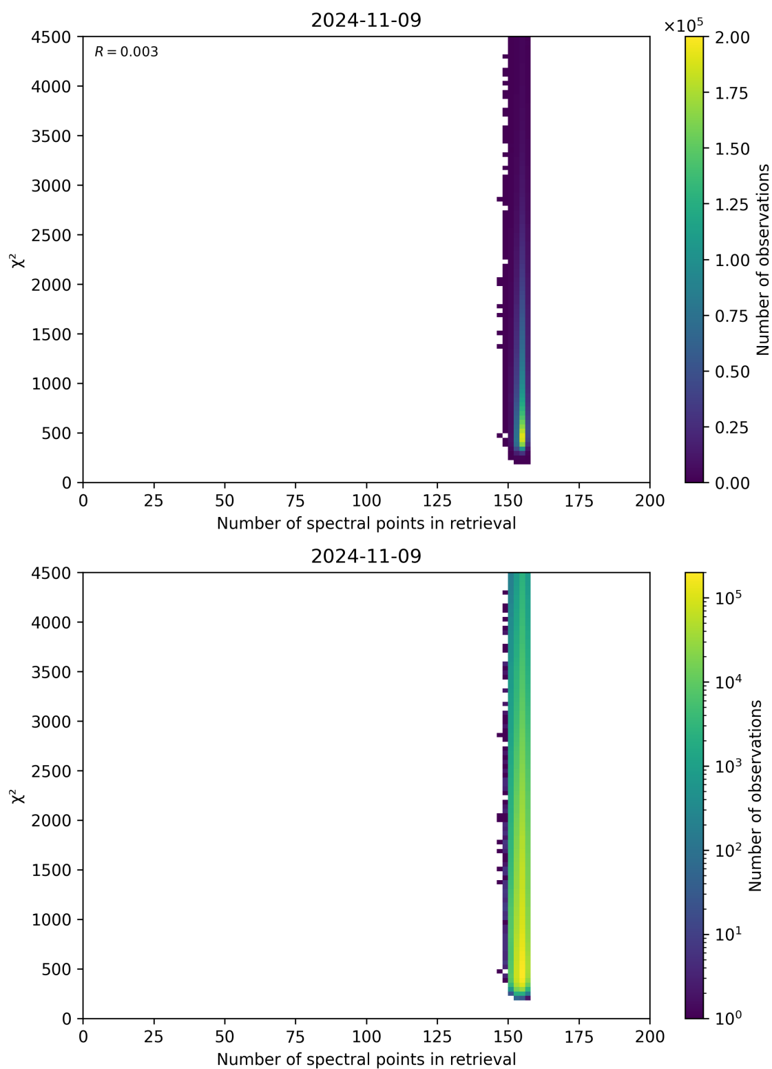
Figure 58: Scatter density plot of “Number of spectral points in retrieval” against “ \chi^2 ” for 2024-11-09 to 2024-11-10.
