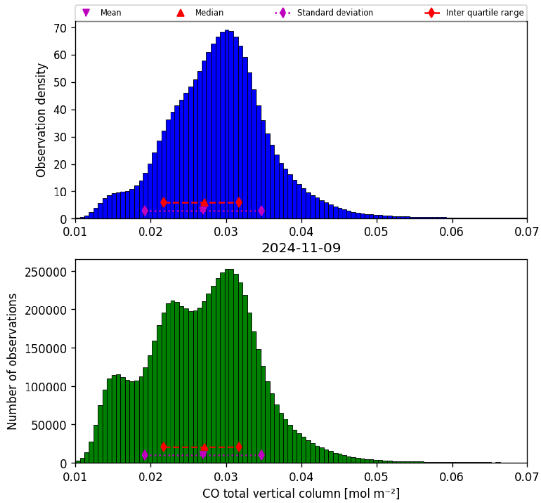
Figure 18: Histogram of “CO total vertical column” for 2024-11-09 to 2024-11-10
