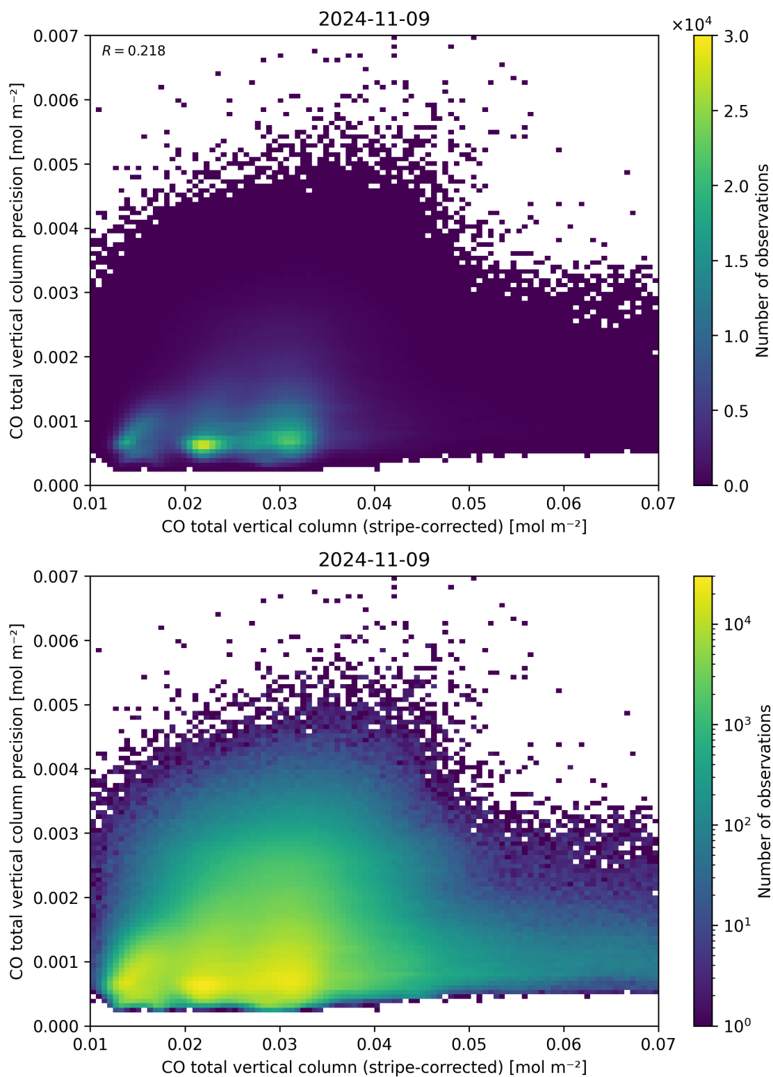
Figure 36: Scatter density plot of “CO total vertical column (stripe-corrected)” against “CO total vertical column precision” for 2024-11-09 to 2024-11-10.
