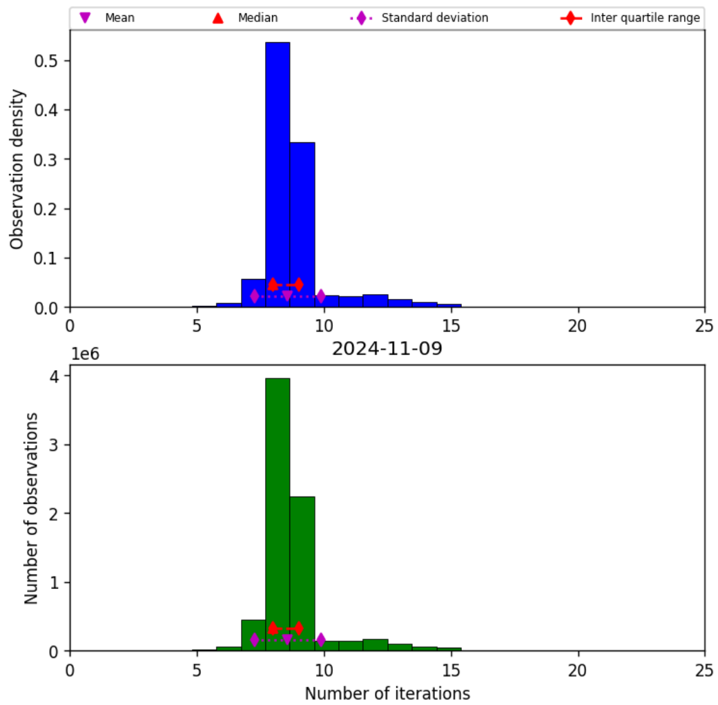
Figure 24: Histogram of “Number of iterations” for 2024-11-09 to 2024-11-10
