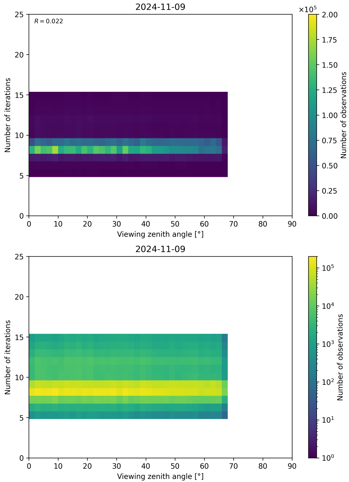
Figure 75: Scatter density plot of “Viewing zenith angle” against “Number of iterations” for 2024-11-09 to 2024-11-10.
