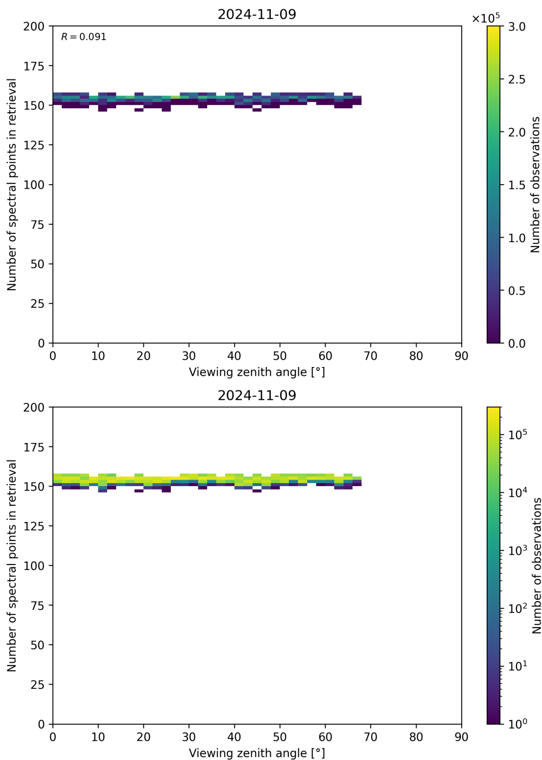
Figure 76: Scatter density plot of “Viewing zenith angle” against “Number of spectral points in retrieval” for 2024-11-09 to 2024-11-10.
