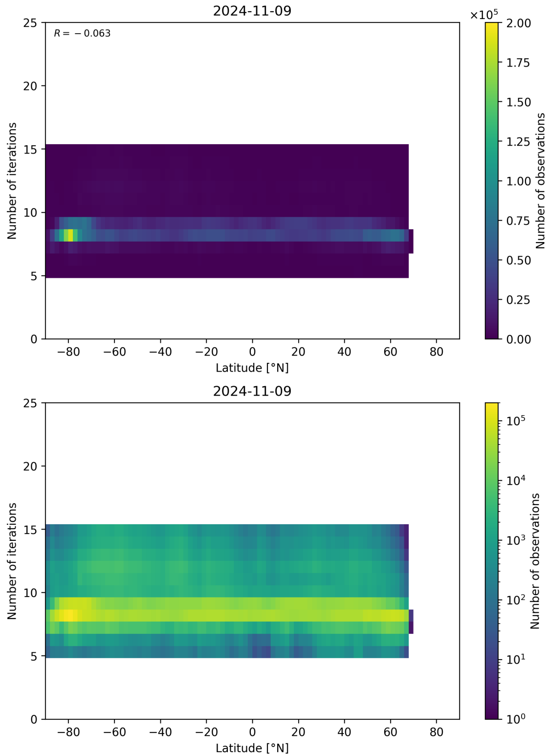
Figure 56: Scatter density plot of “Latitude” against “Number of iterations” for 2024-11-09 to 2024-11-10.
