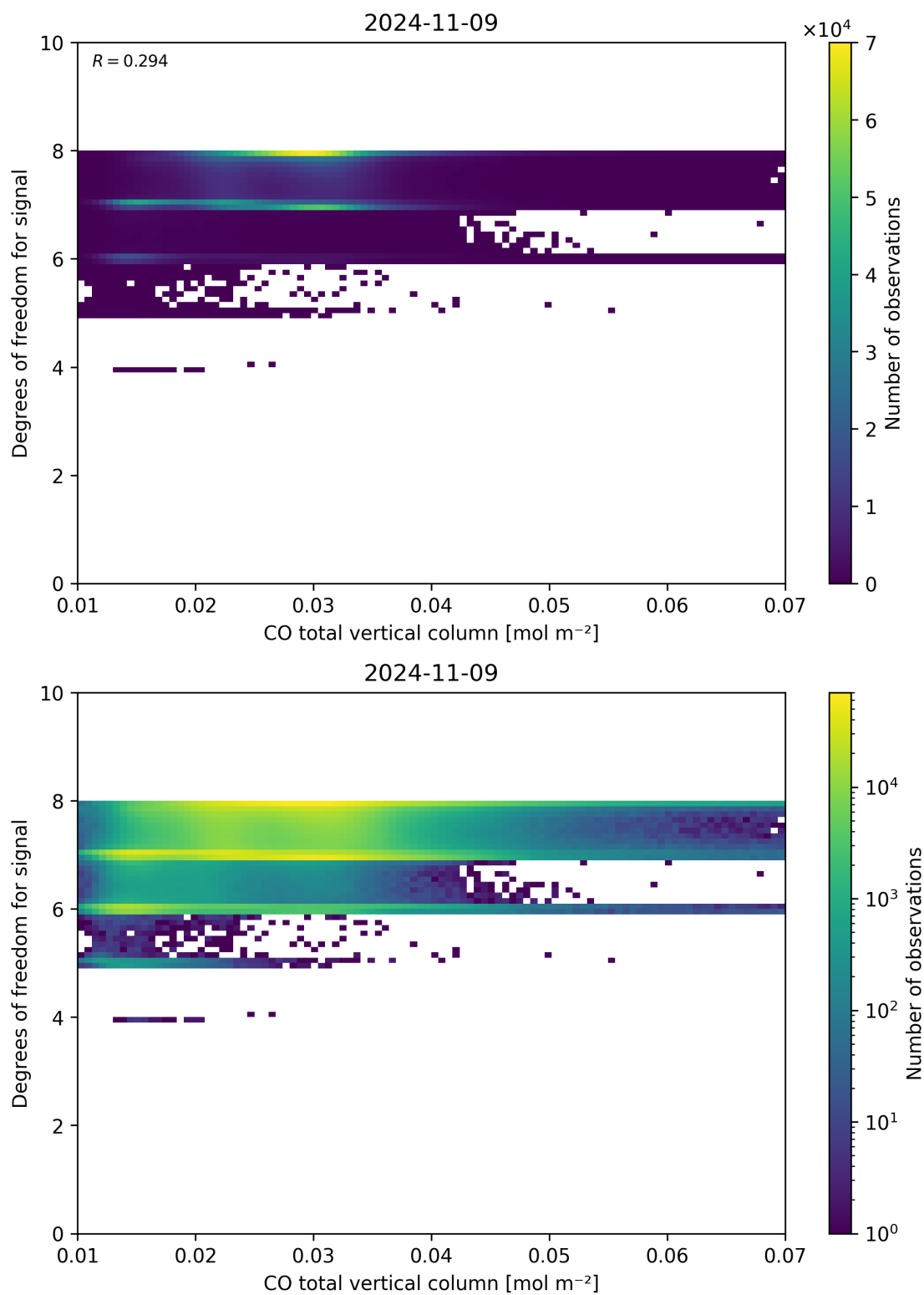
Figure 41: Scatter density plot of “CO total vertical column” against “Degrees of freedom for signal” for 2024-11-09 to 2024-11-10.
