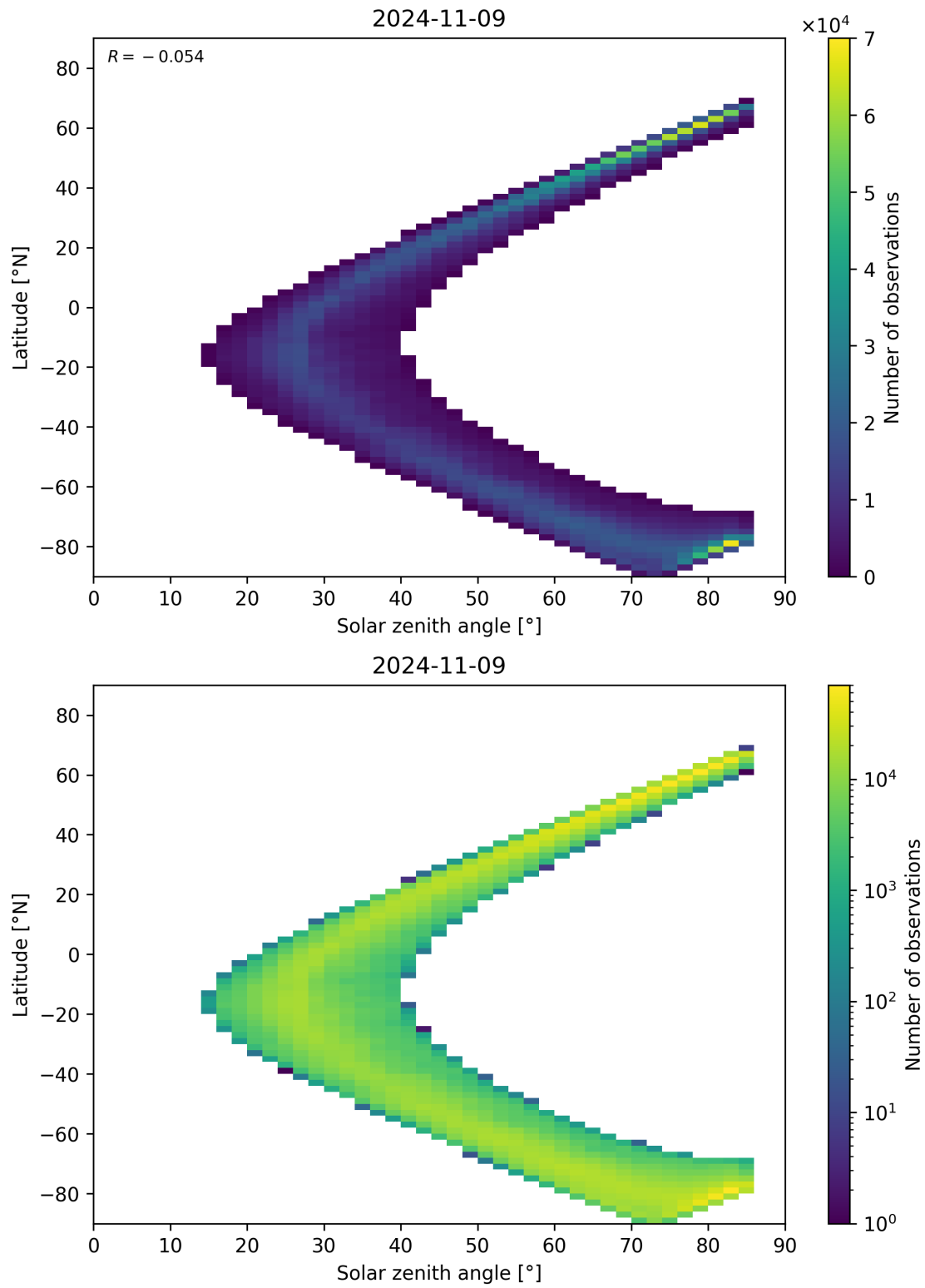
Figure 66: Scatter density plot of “Solar zenith angle” against “Latitude” for 2024-11-09 to 2024-11-10.
