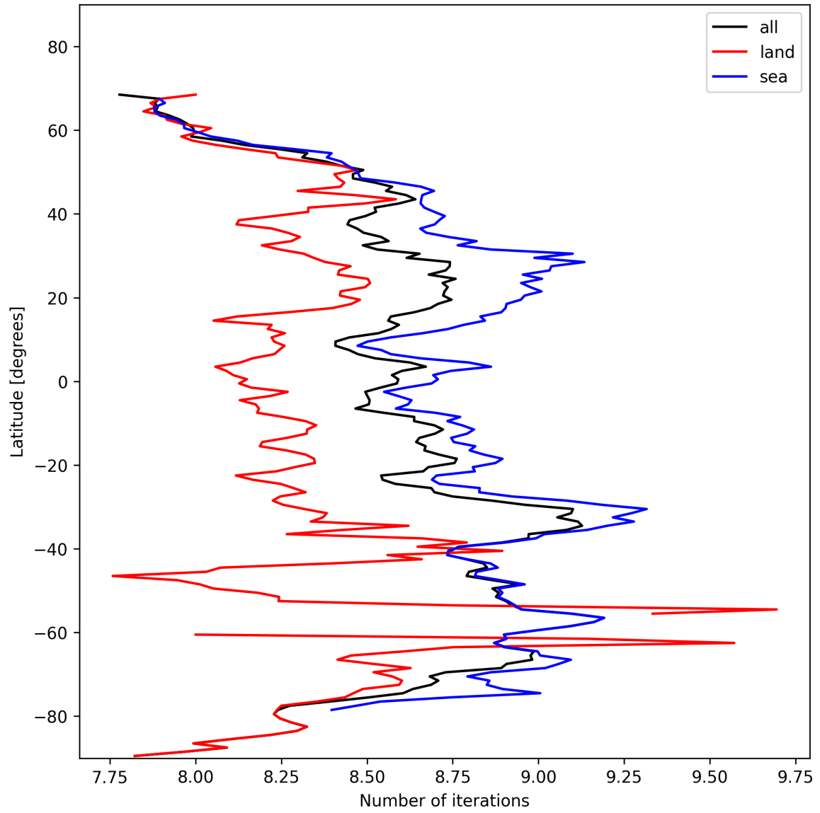
Figure 16: Zonal average of “Number of iterations” for 2024-11-09 to 2024-11-10.
