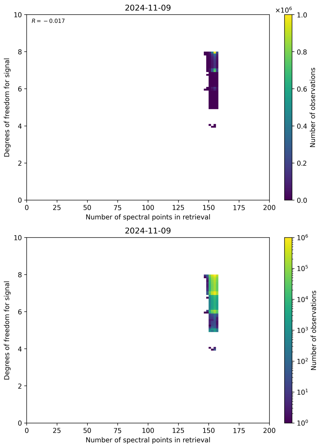
Figure 59: Scatter density plot of “Number of spectral points in retrieval” against “Degrees of freedom for signal” for 2024-11-09 to 2024-11-10.
