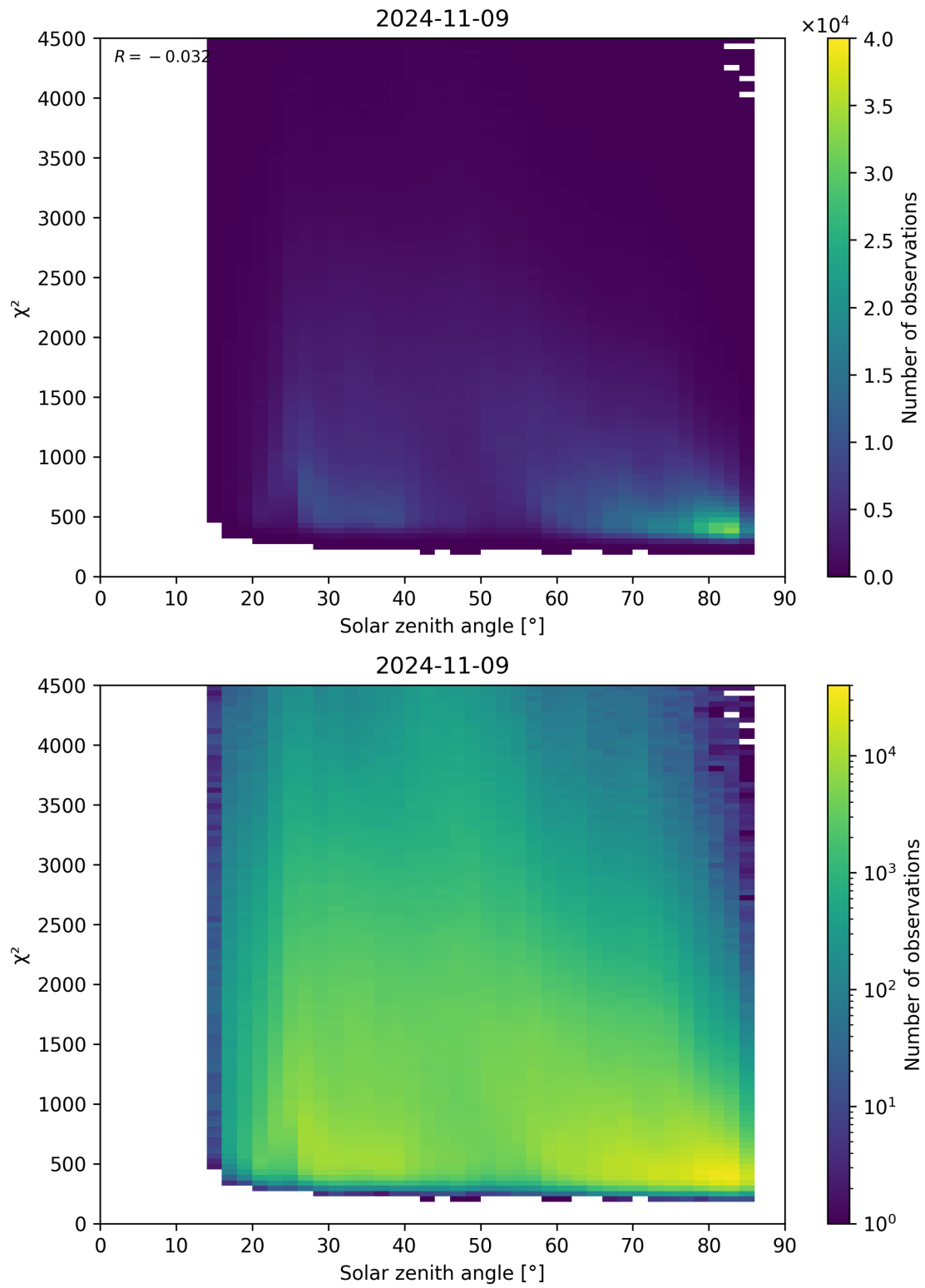
Figure 64: Scatter density plot of “Solar zenith angle” against “ \chi^2 ” for 2024-11-09 to 2024-11-10.
