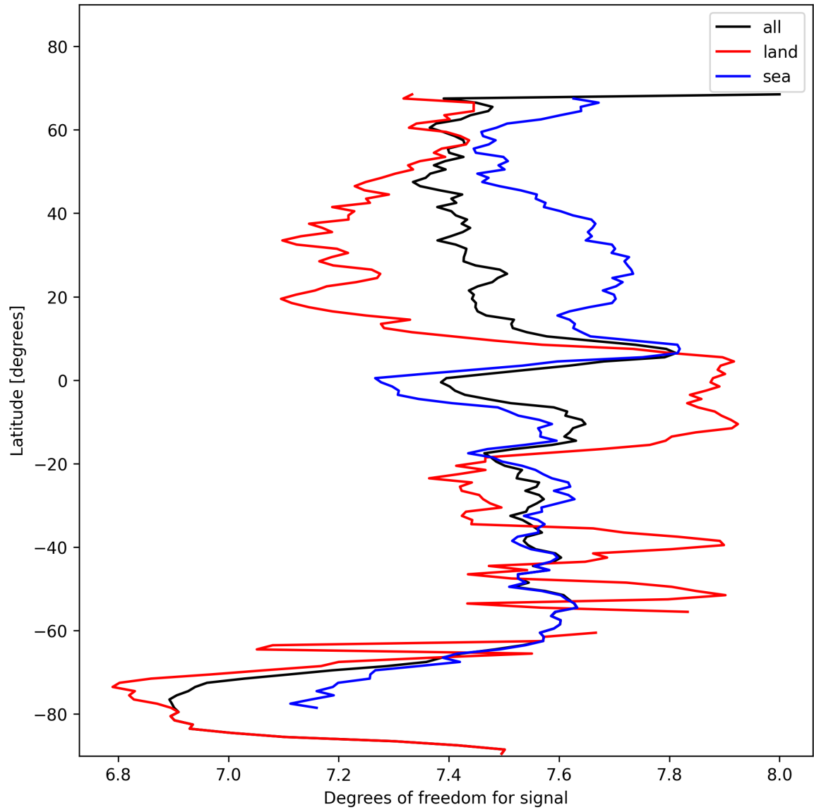
Figure 15: Zonal average of “Degrees of freedom for signal” for 2024-11-09 to 2024-11-10.
