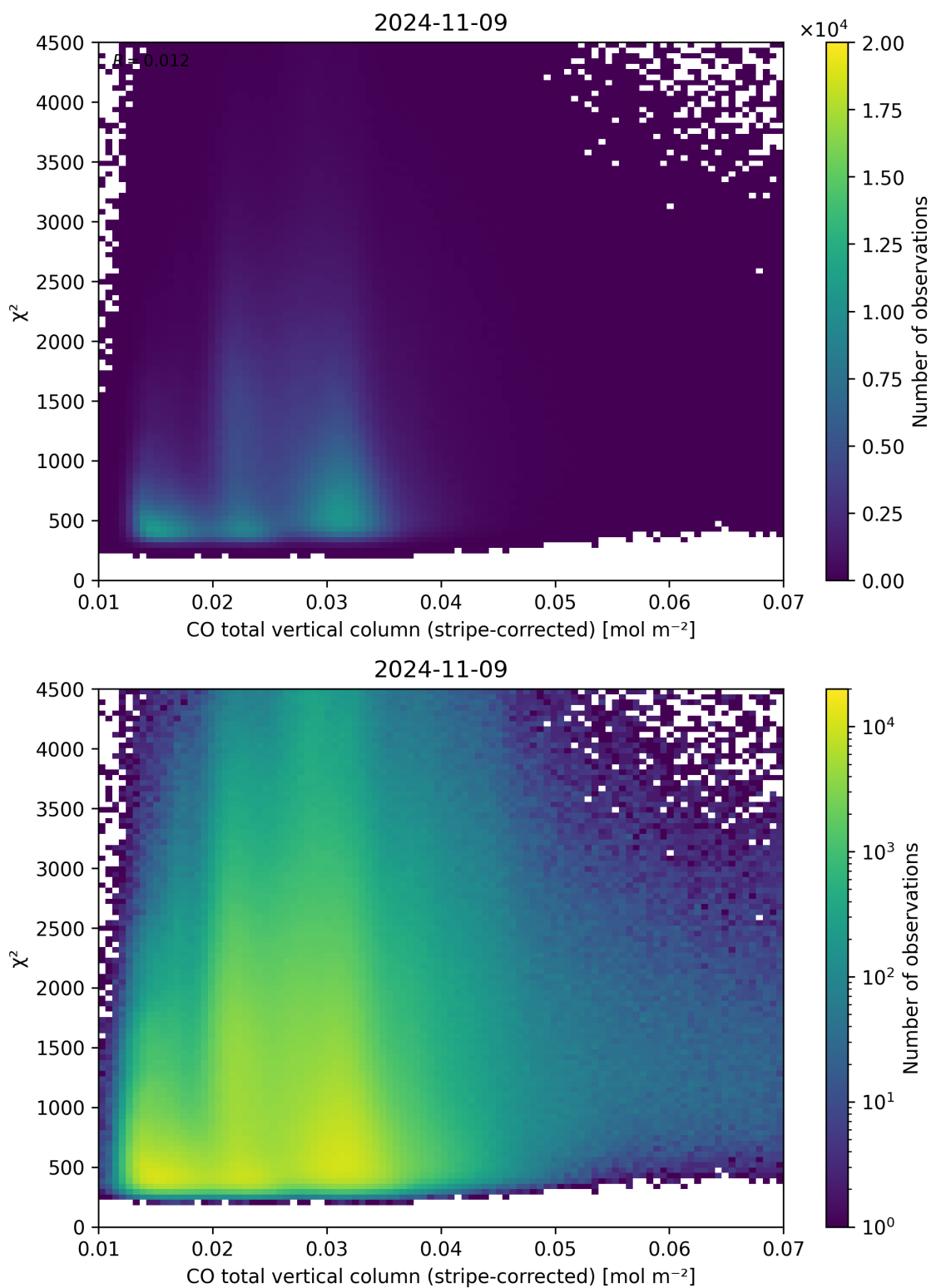
Figure 37: Scatter density plot of “CO total vertical column (stripe-corrected)” against “ \chi^2 ” for 2024-11-09 to 2024-11-10.
