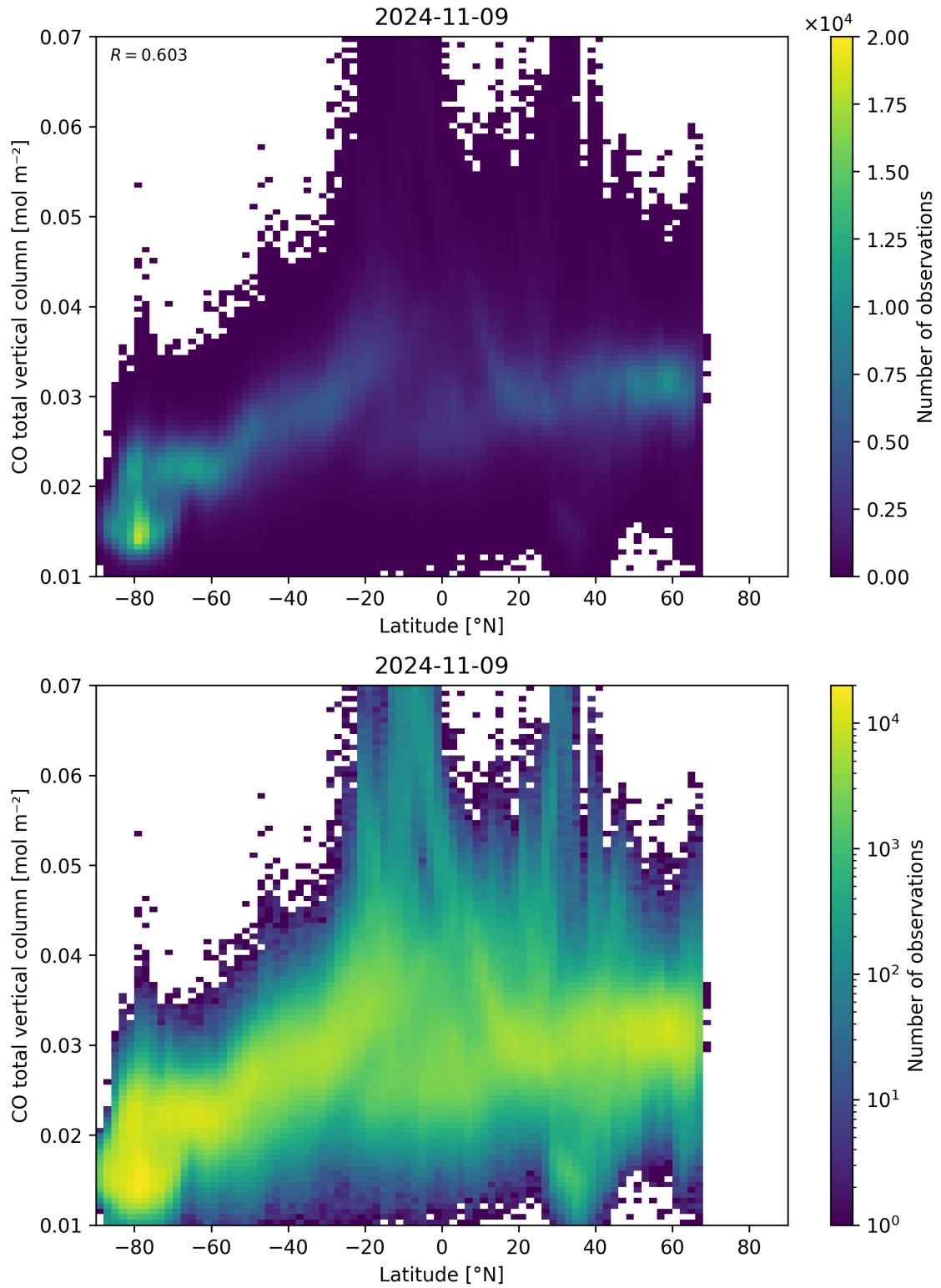
Figure 51: Scatter density plot of “Latitude” against “CO total vertical column” for 2024-11-09 to 2024-11-10.
