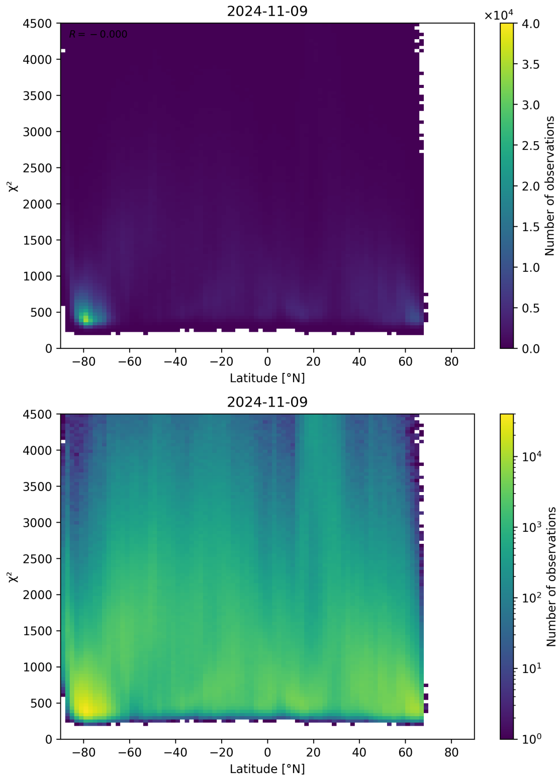
Figure 54: Scatter density plot of “Latitude” against “ \chi^2 ” for 2024-11-09 to 2024-11-10.
