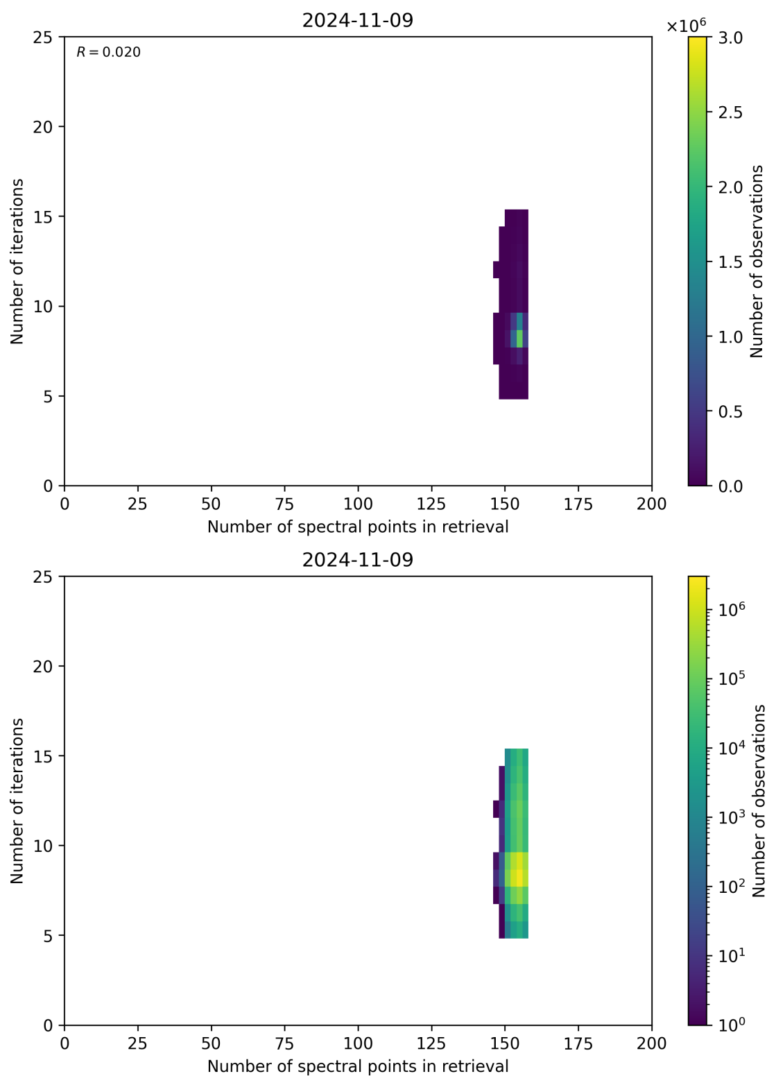
Figure 60: Scatter density plot of “Number of spectral points in retrieval” against “Number of iterations” for 2024-11-09 to 2024-11-10.
