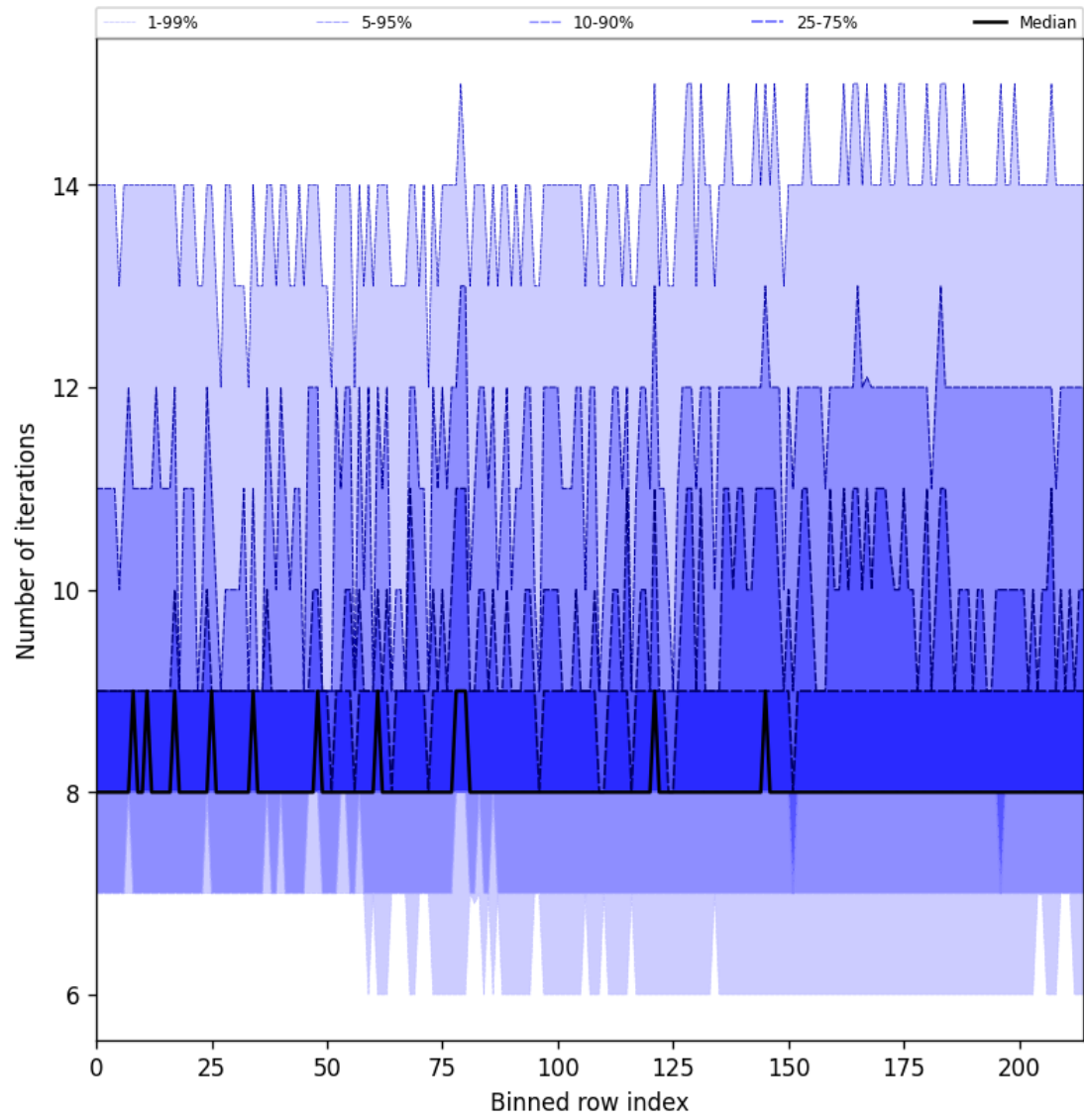
Figure 32: Along track statistics of “Number of iterations” for 2024-11-09 to 2024-11-10
