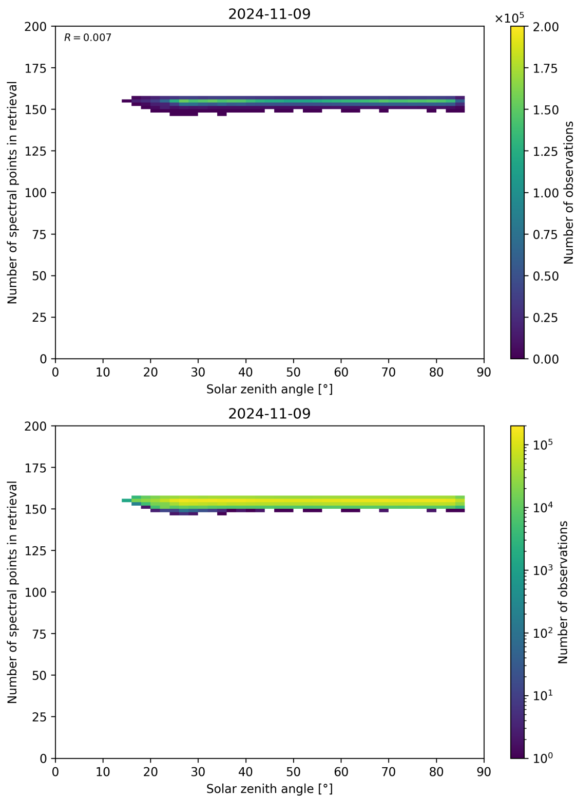
Figure 68: Scatter density plot of “Solar zenith angle” against “Number of spectral points in retrieval” for 2024-11-09 to 2024-11-10.
