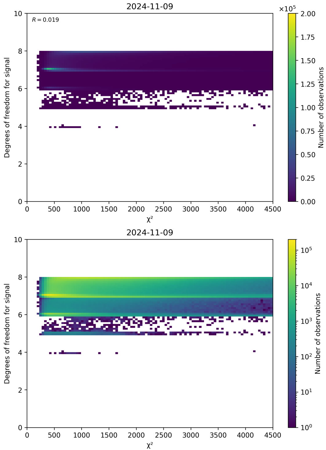
Figure 48: Scatter density plot of “ \chi^2 ” against “Degrees of freedom for signal” for 2024-11-09 to 2024-11-10.
