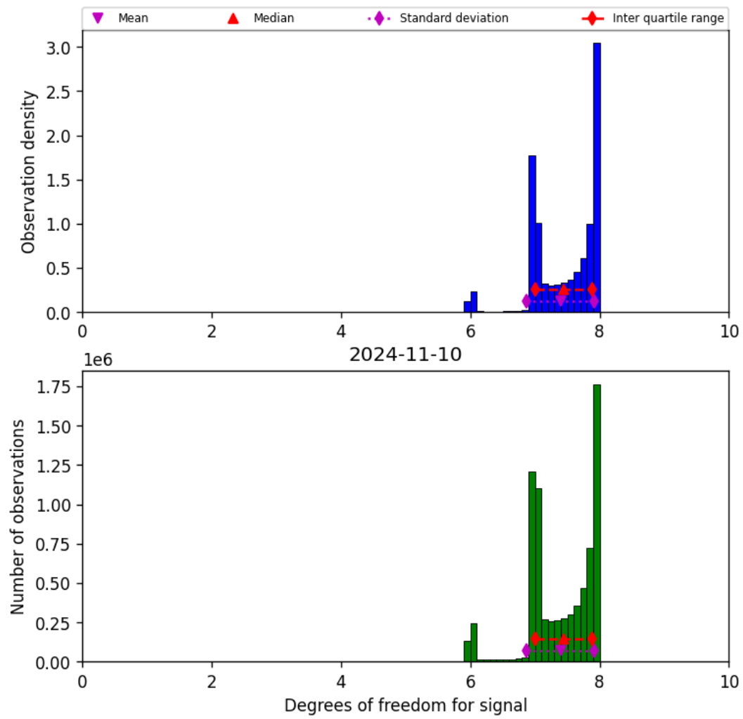
Figure 23: Histogram of “Degrees of freedom for signal” for 2024-11-09 to 2024-11-11
