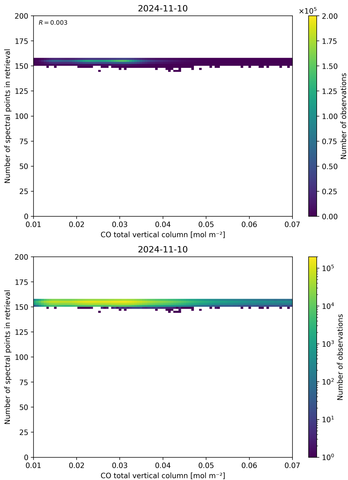
Figure 43: Scatter density plot of “CO total vertical column” against “Number of spectral points in retrieval” for 2024-11-09 to 2024-11-11.
