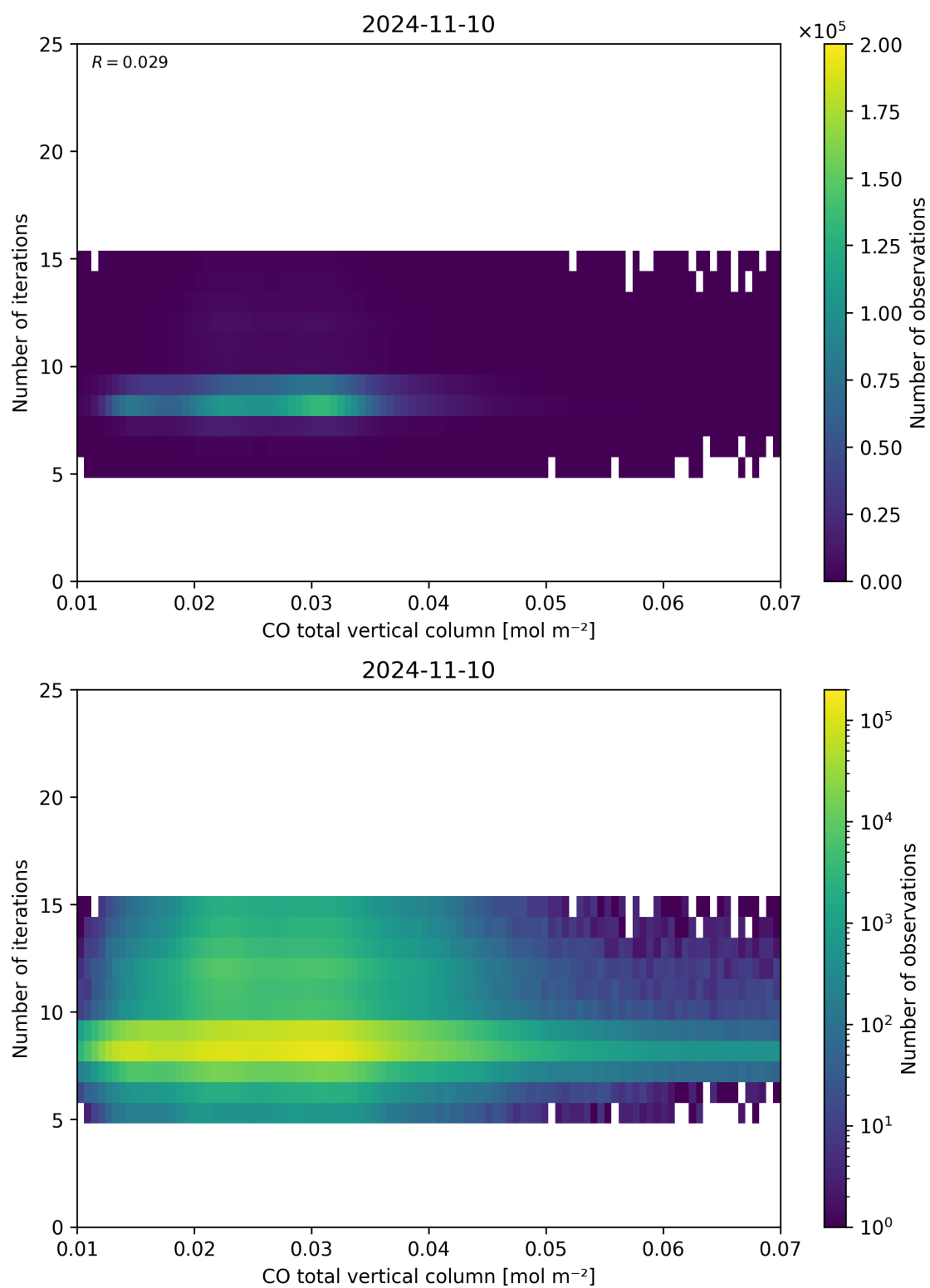
Figure 42: Scatter density plot of “CO total vertical column” against “Number of iterations” for 2024-11-09 to 2024-11-11.
