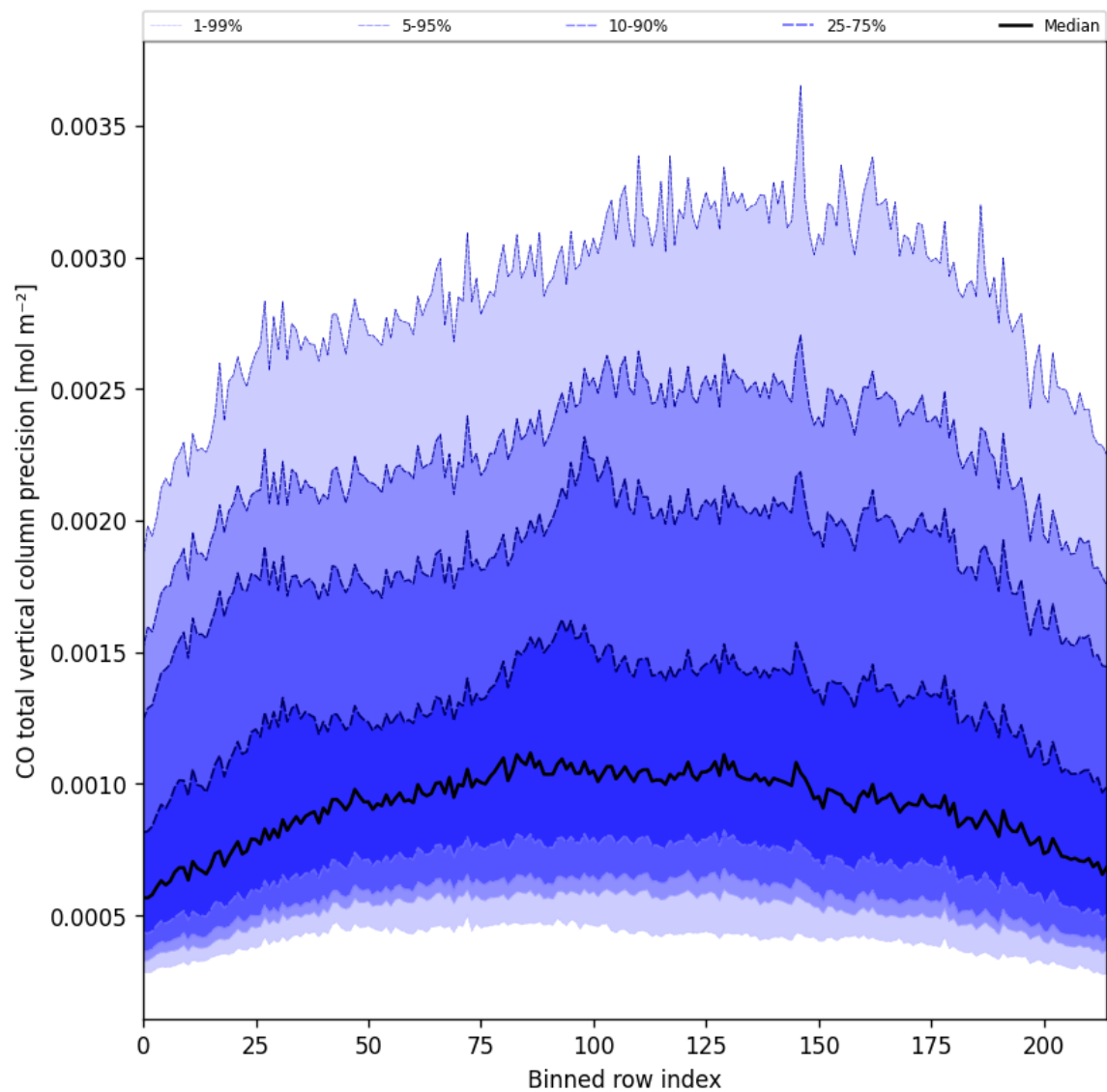
Figure 28: Along track statistics of “CO total vertical column precision” for 2024-11-09 to 2024-11-11
