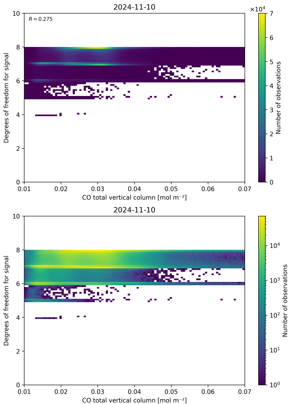
Figure 41: Scatter density plot of “CO total vertical column” against “Degrees of freedom for signal” for 2024-11-09 to 2024-11-11.
