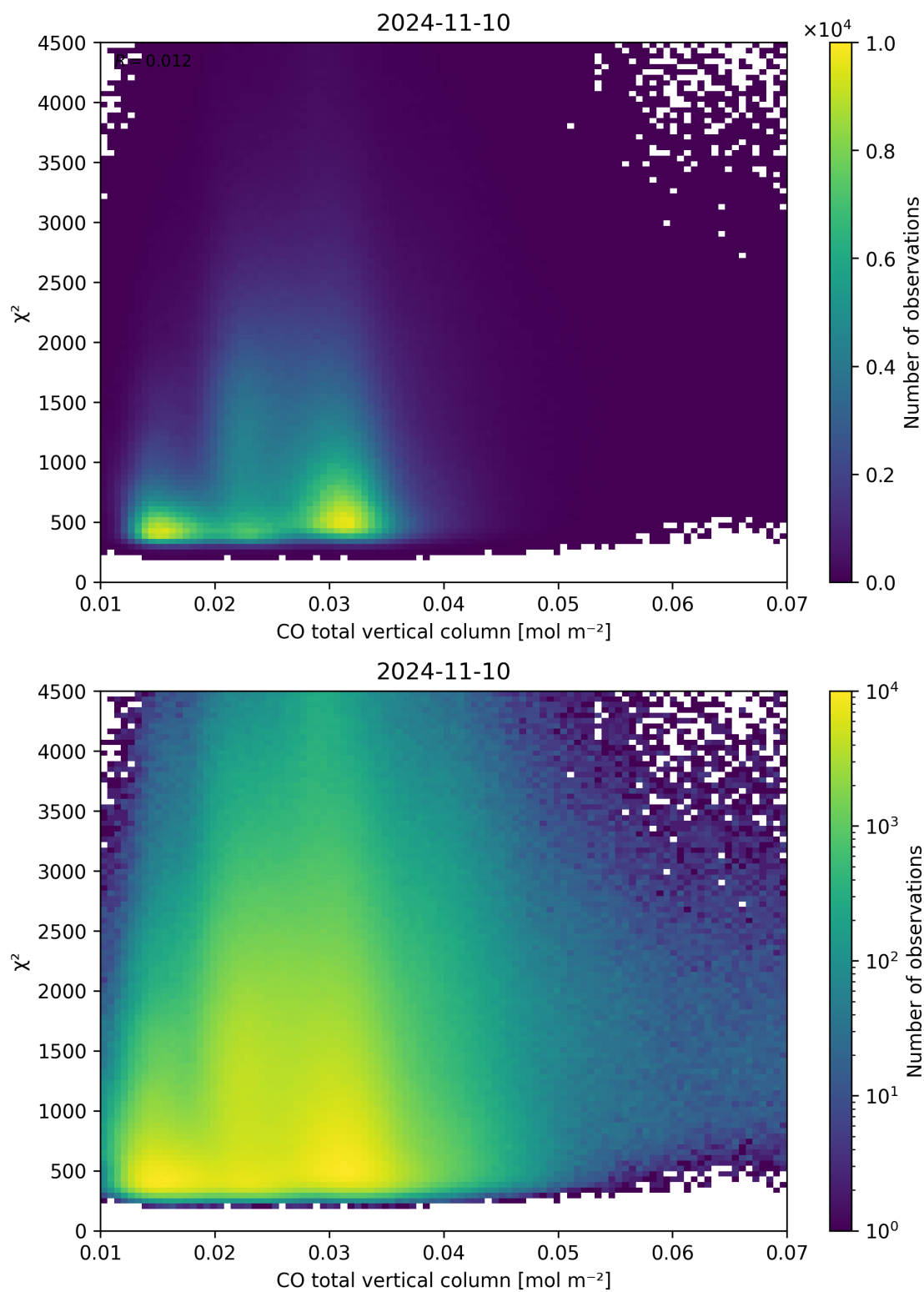
Figure 35: Scatter density plot of “CO total vertical column” against “ \chi^2 ” for 2024-11-09 to 2024-11-11.
