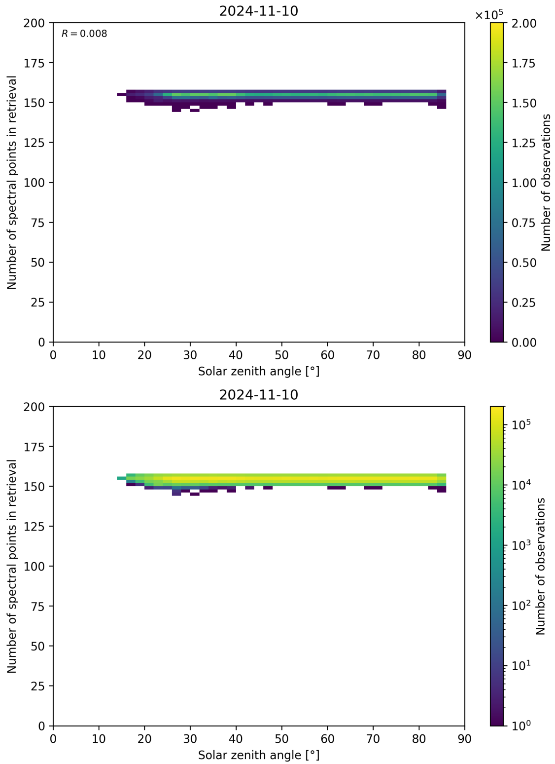
Figure 68: Scatter density plot of “Solar zenith angle” against “Number of spectral points in retrieval” for 2024-11-09 to 2024-11-11.
