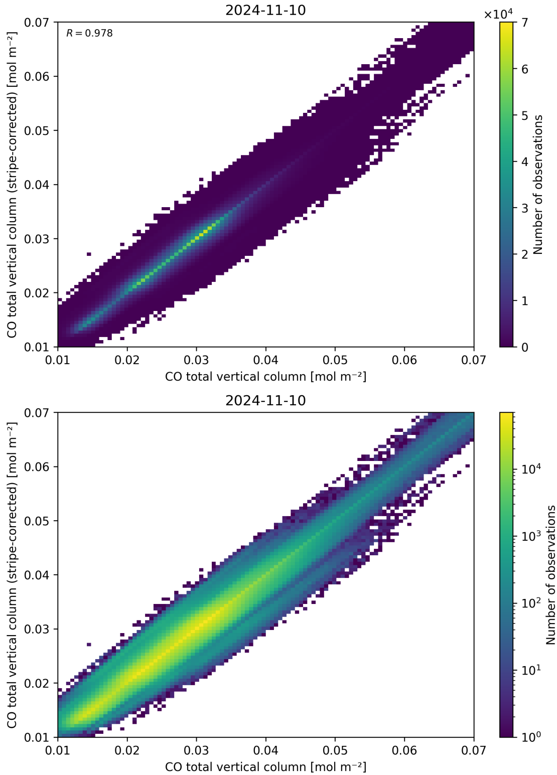
Figure 33: Scatter density plot of “CO total vertical column” against “CO total vertical column (stripe-corrected)” for 2024-11-09 to 2024-11-11.
