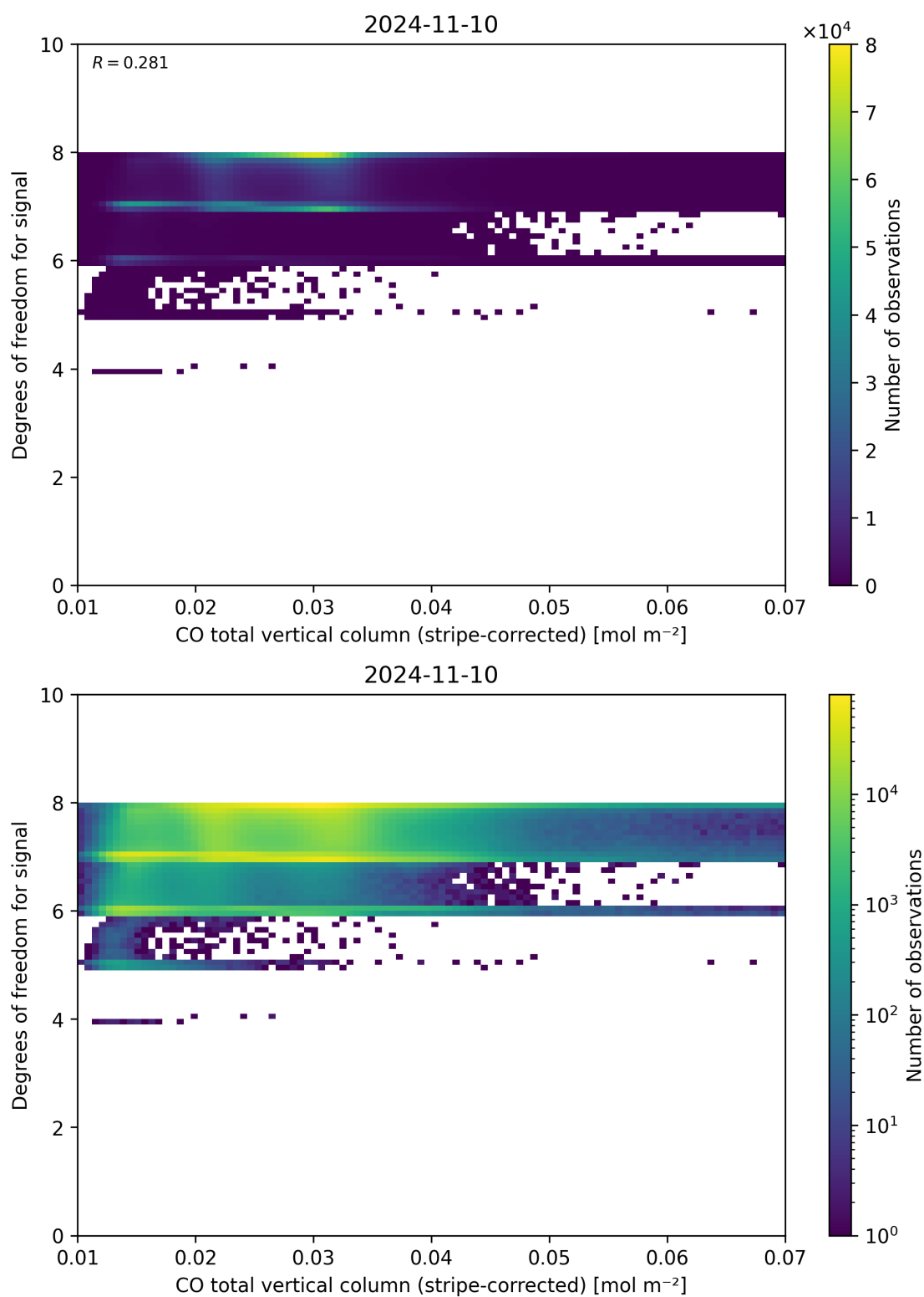
Figure 38: Scatter density plot of “CO total vertical column (stripe-corrected)” against “Degrees of freedom for signal” for 2024-11-09 to 2024-11-11.
