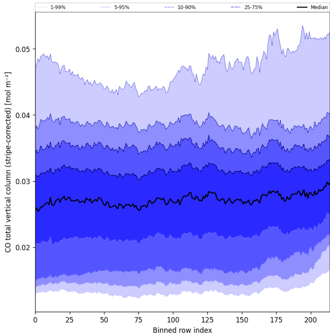
Figure 27: Along track statistics of “CO total vertical column (stripe-corrected)” for 2024-11-09 to 2024-11-11
