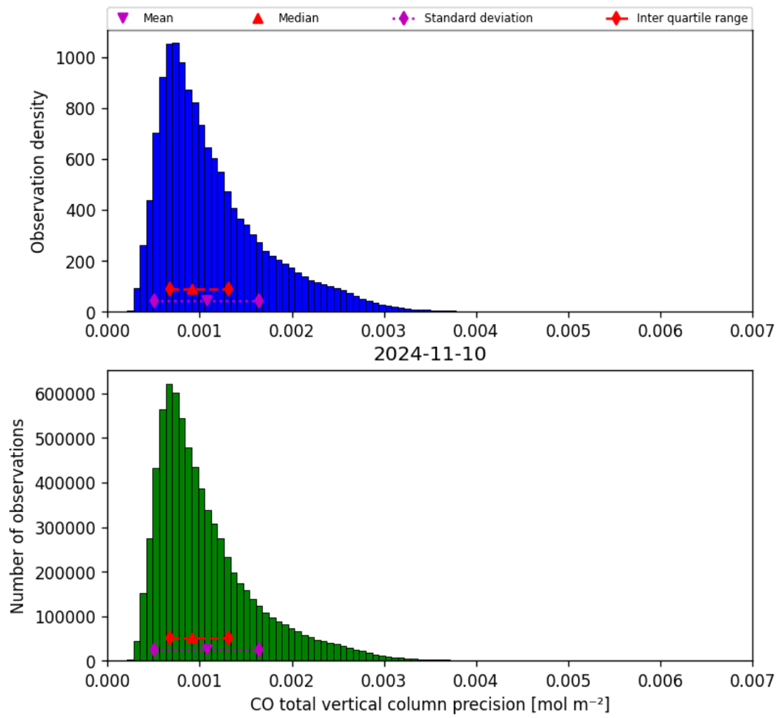
Figure 20: Histogram of “CO total vertical column precision” for 2024-11-09 to 2024-11-11
