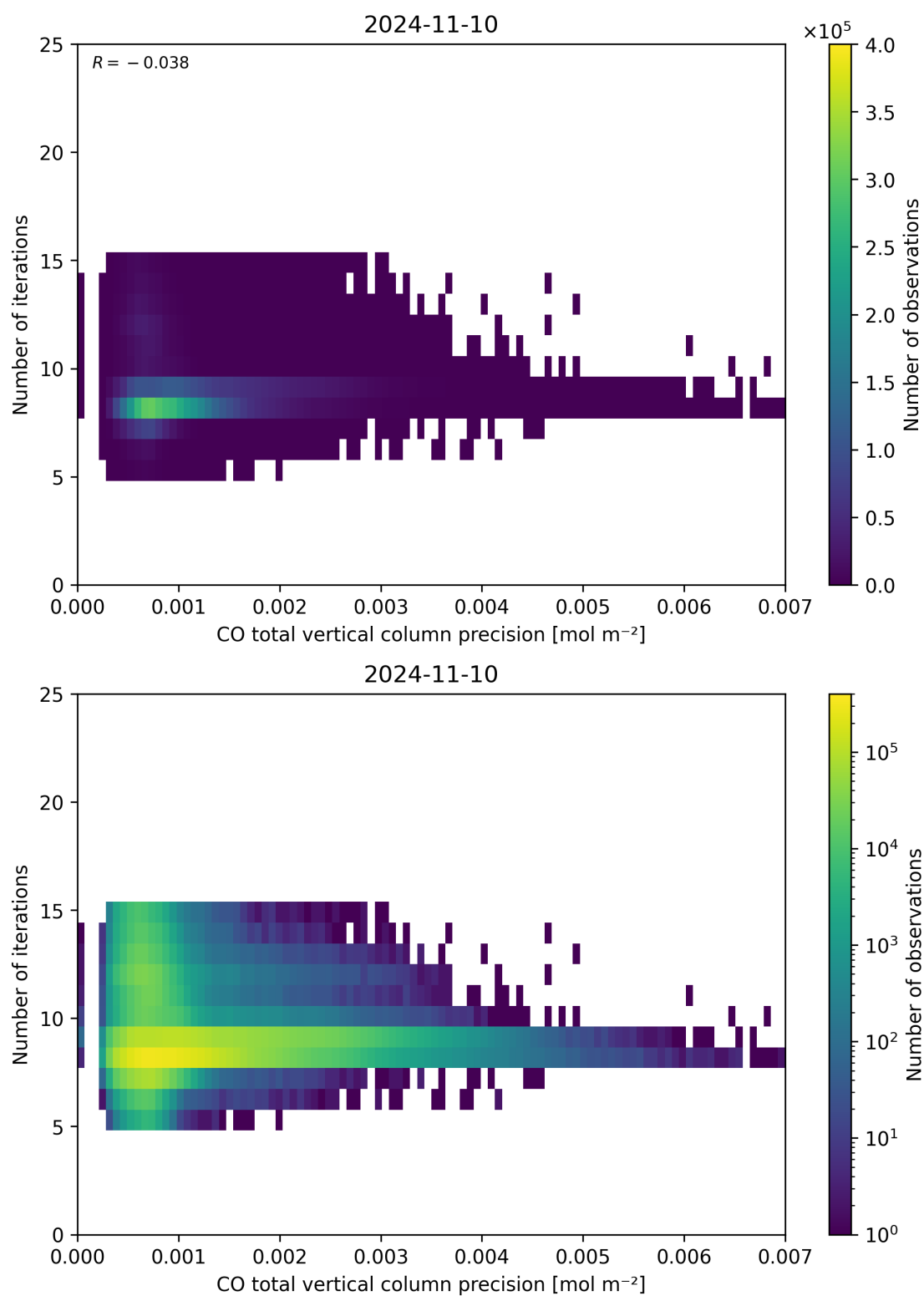
Figure 46: Scatter density plot of “CO total vertical column precision” against “Number of iterations” for 2024-11-09 to 2024-11-11.
