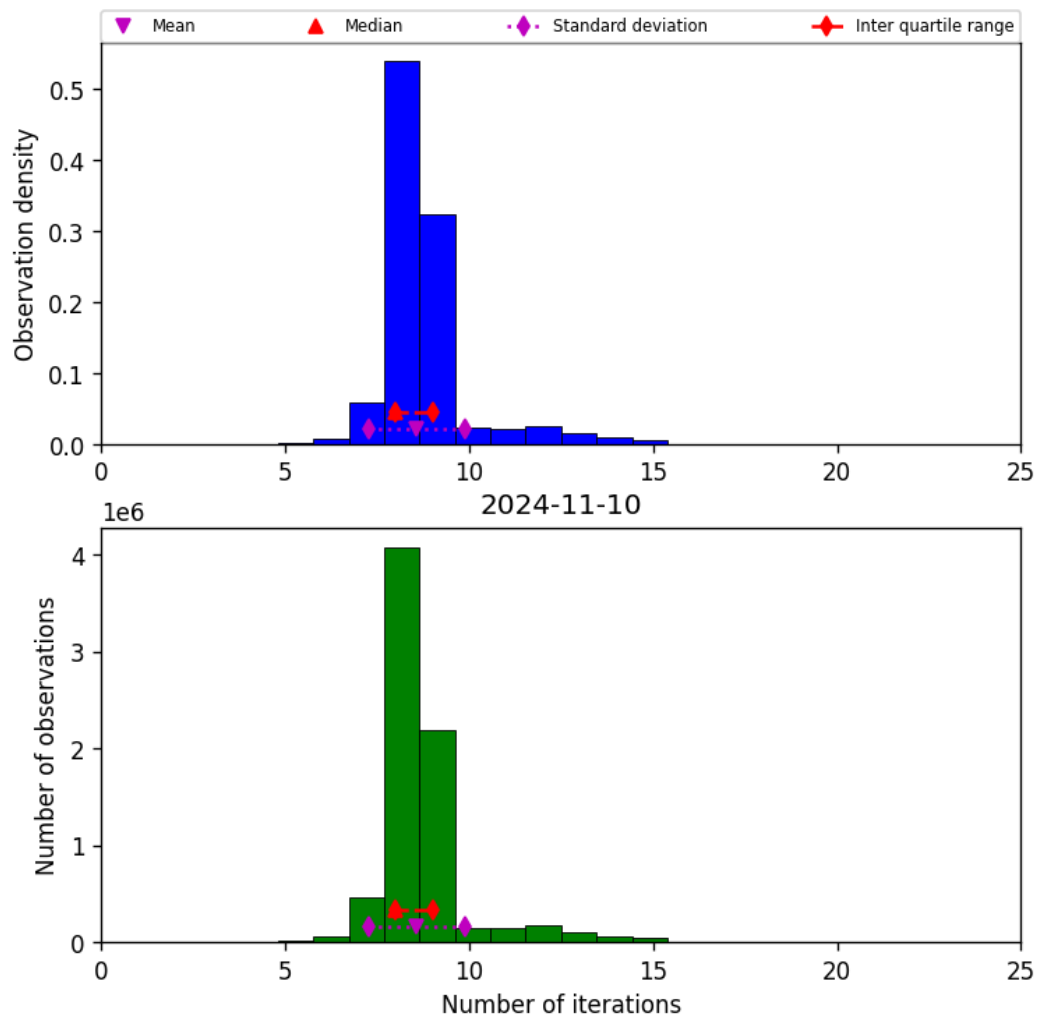
Figure 24: Histogram of “Number of iterations” for 2024-11-09 to 2024-11-11
