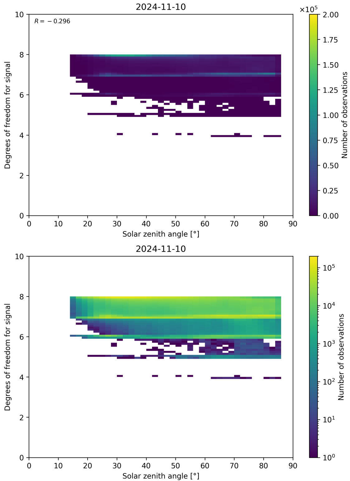
Figure 65: Scatter density plot of “Solar zenith angle” against “Degrees of freedom for signal” for 2024-11-09 to 2024-11-11.
