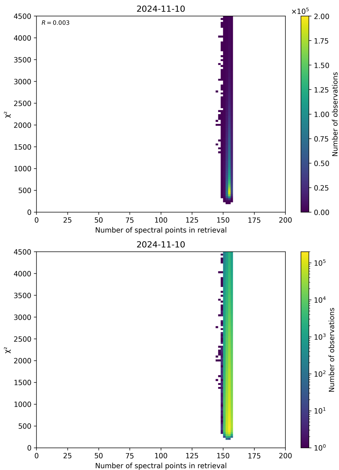
Figure 58: Scatter density plot of “Number of spectral points in retrieval” against “ \chi^2 ” for 2024-11-09 to 2024-11-11.
