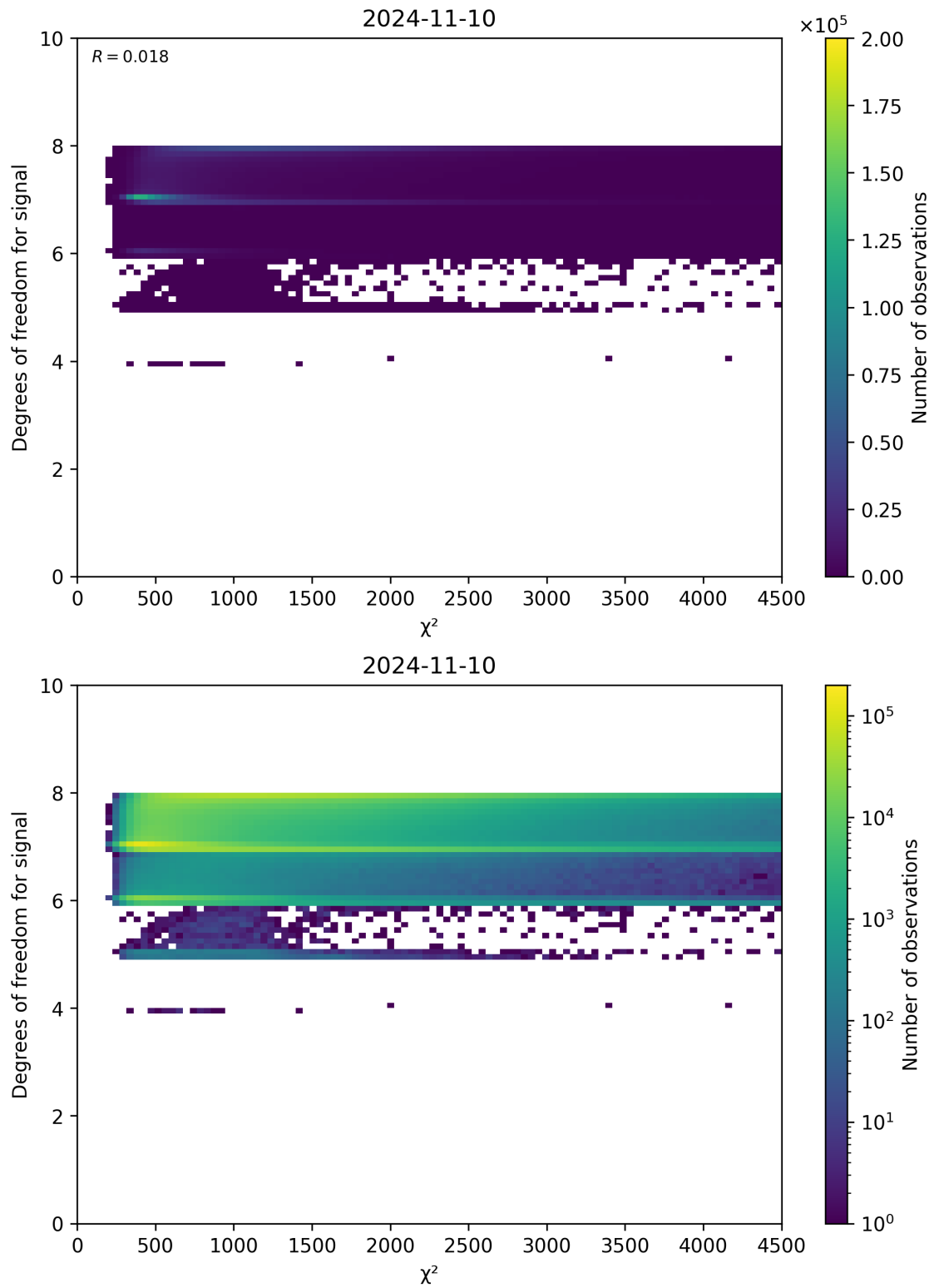
Figure 48: Scatter density plot of “ \chi^2 ” against “Degrees of freedom for signal” for 2024-11-09 to 2024-11-11.
