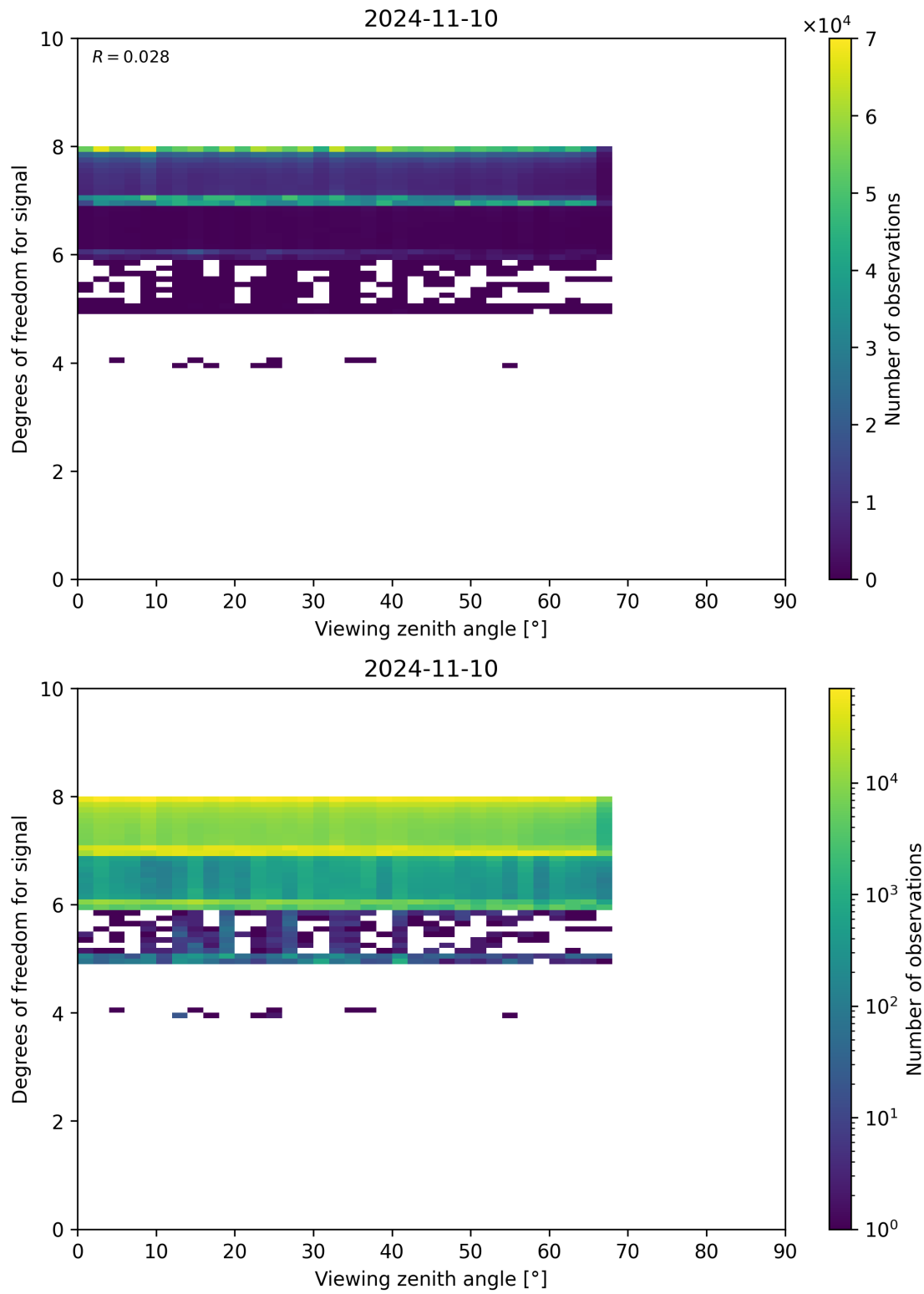
Figure 73: Scatter density plot of “Viewing zenith angle” against “Degrees of freedom for signal” for 2024-11-09 to 2024-11-11.
