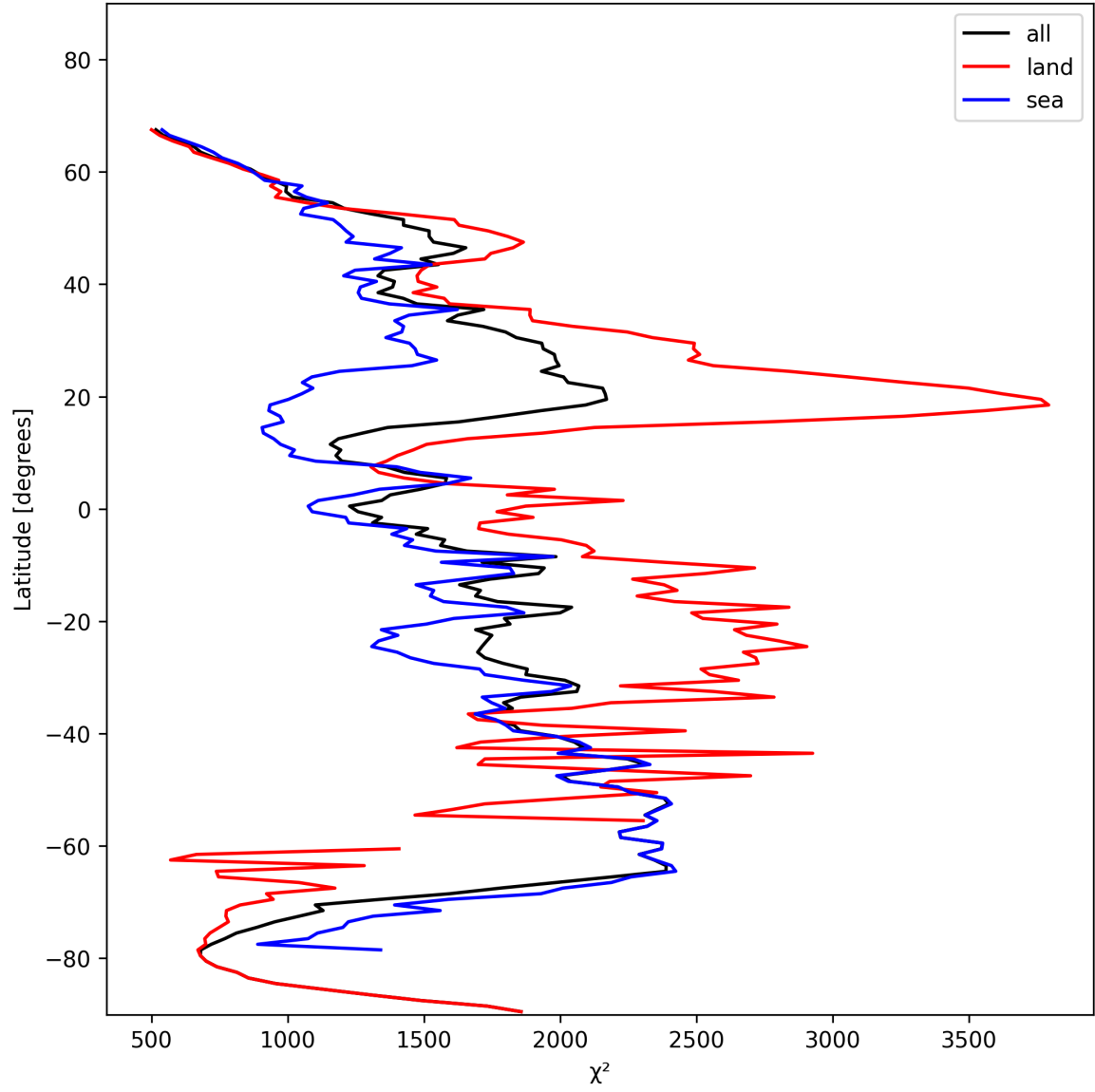
Figure 14: Zonal average of “ \chi^2 ” for 2024-11-09 to 2024-11-11.
