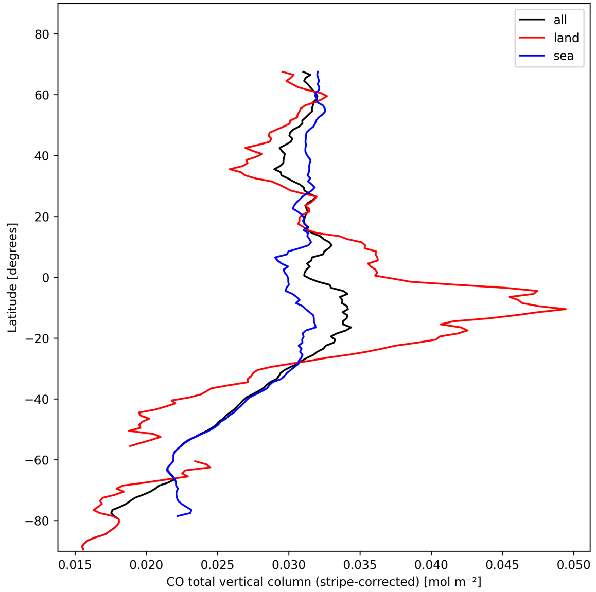
Figure 11: Zonal average of “CO total vertical column (stripe-corrected)” for 2024-11-09 to 2024-11-11.
