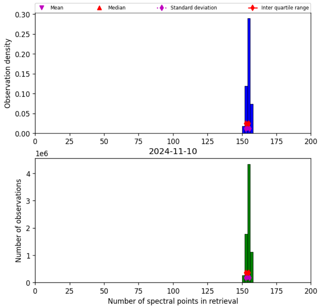
Figure 21: Histogram of “Number of spectral points in retrieval” for 2024-11-09 to 2024-11-11
