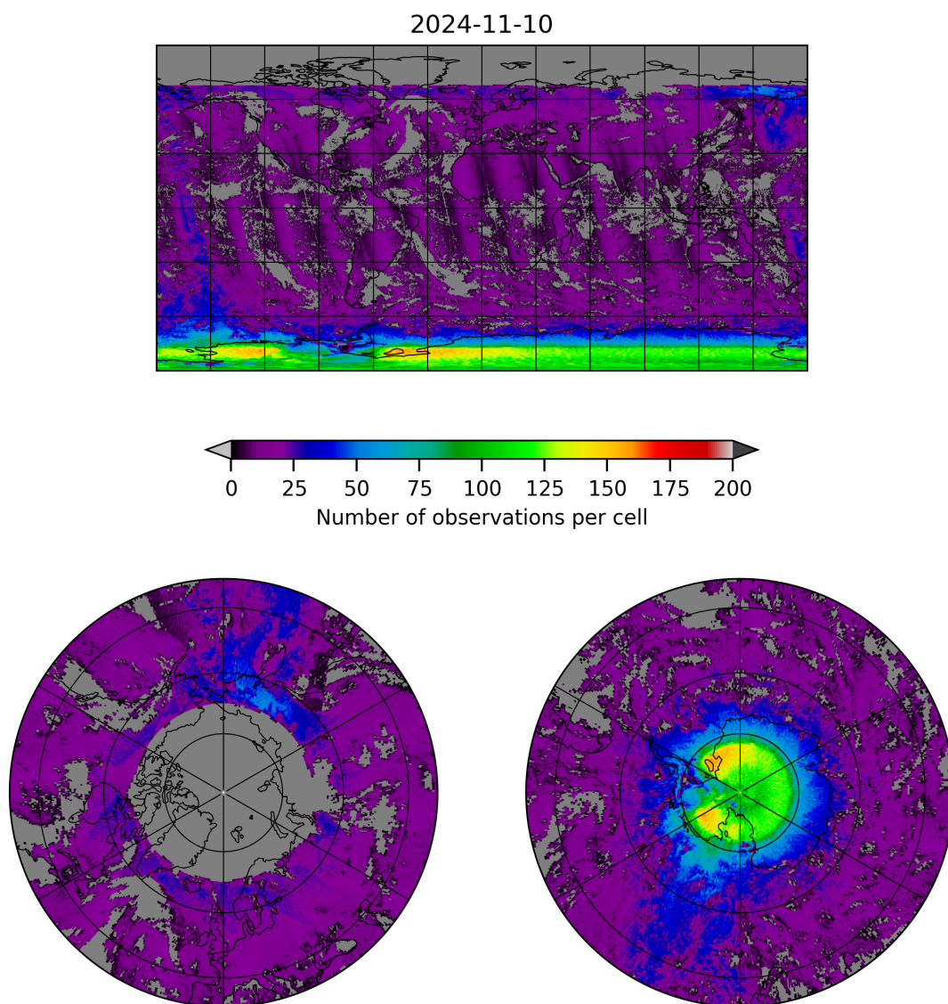
Figure 8: Map of the number of observations for 2024-11-09 to 2024-11-11
