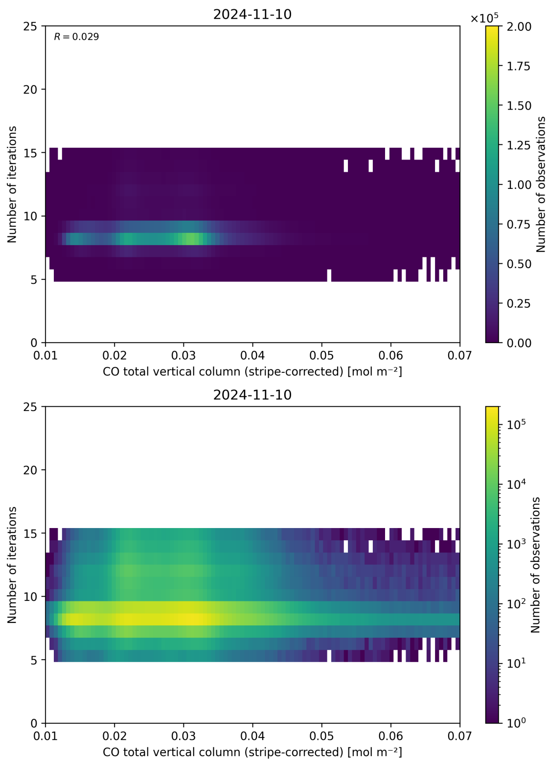
Figure 39: Scatter density plot of “CO total vertical column (stripe-corrected)” against “Number of iterations” for 2024-11-09 to 2024-11-11.
