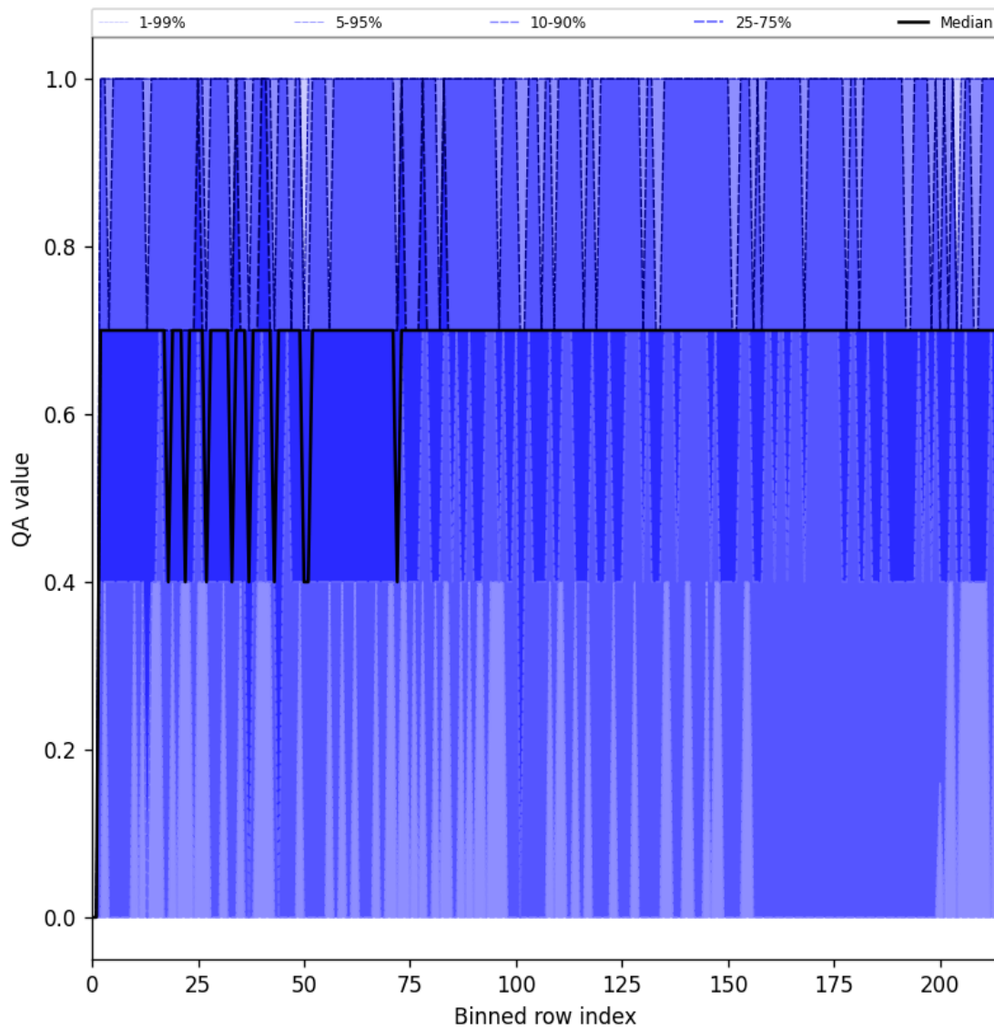
Figure 25: Along track statistics of “QA value” for 2024-11-09 to 2024-11-11
