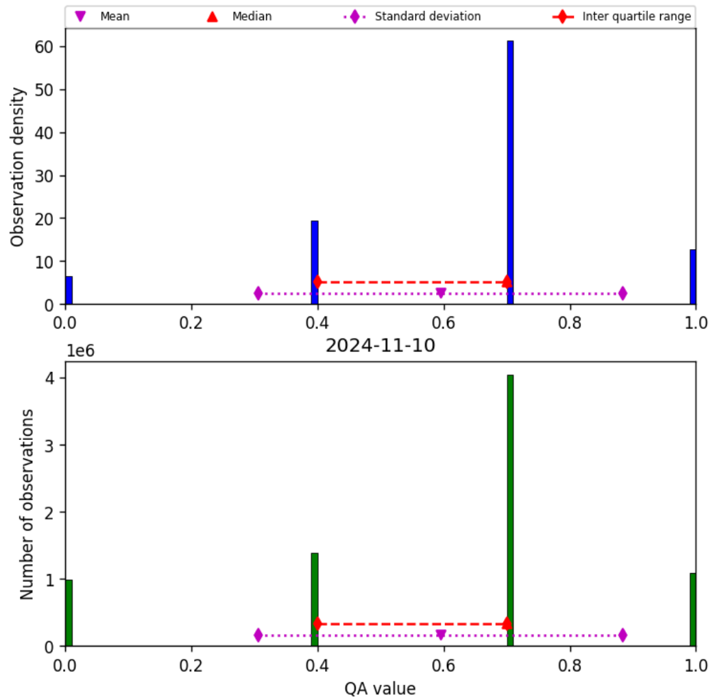
Figure 17: Histogram of “QA value” for 2024-11-09 to 2024-11-11
