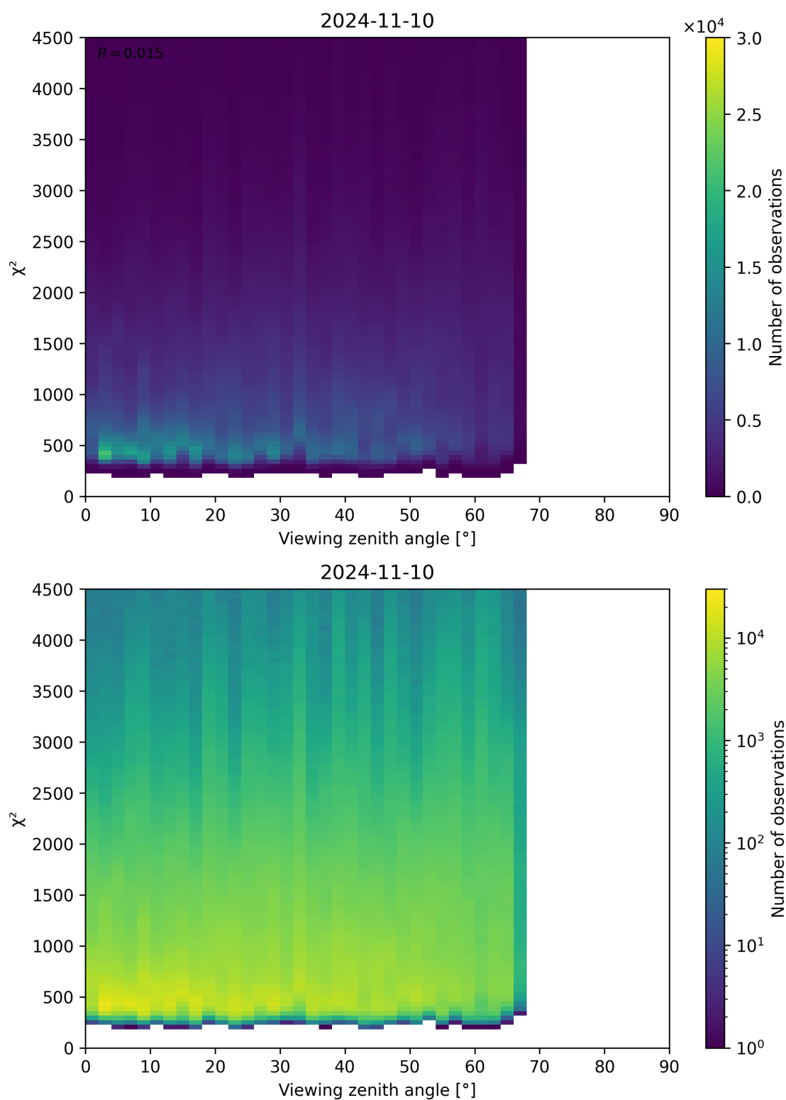
Figure 72: Scatter density plot of “Viewing zenith angle” against “ \chi^2 ” for 2024-11-09 to 2024-11-11.
