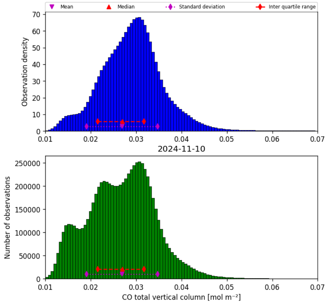
Figure 18: Histogram of “CO total vertical column” for 2024-11-09 to 2024-11-11
