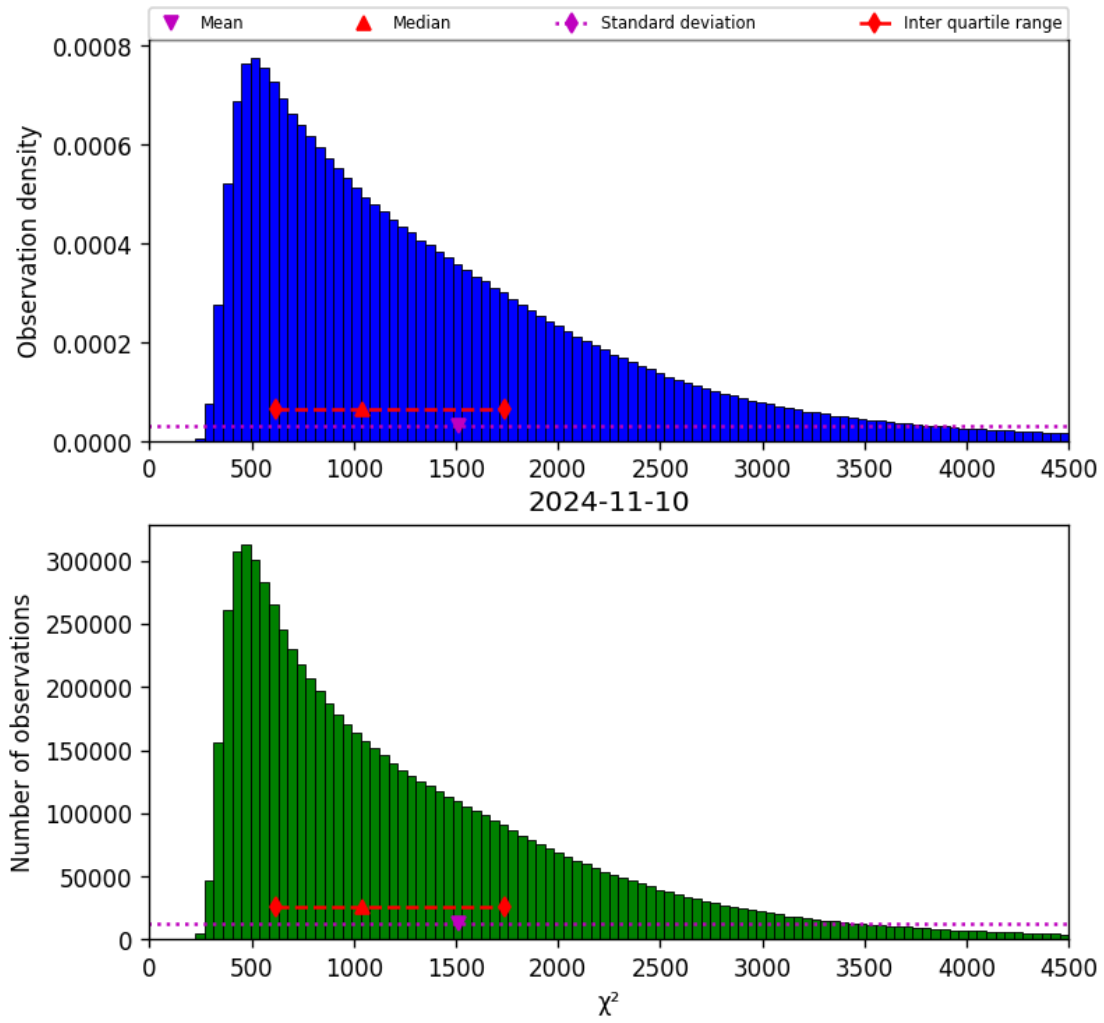
Figure 22: Histogram of “ \chi^2 ” for 2024-11-09 to 2024-11-11
