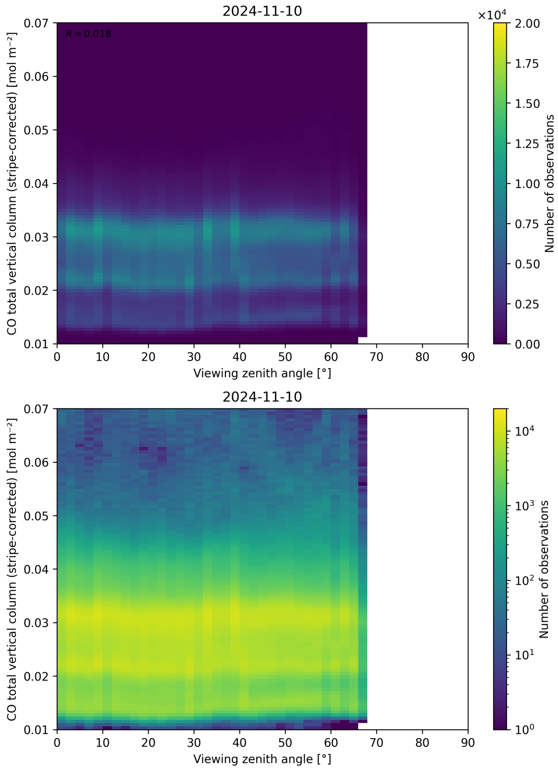
Figure 70: Scatter density plot of “Viewing zenith angle” against “CO total vertical column (stripe-corrected)” for 2024-11-09 to 2024-11-11.
