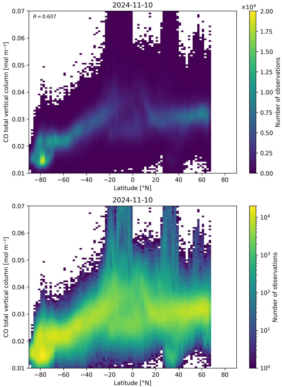
Figure 51: Scatter density plot of “Latitude” against “CO total vertical column” for 2024-11-09 to 2024-11-11.
