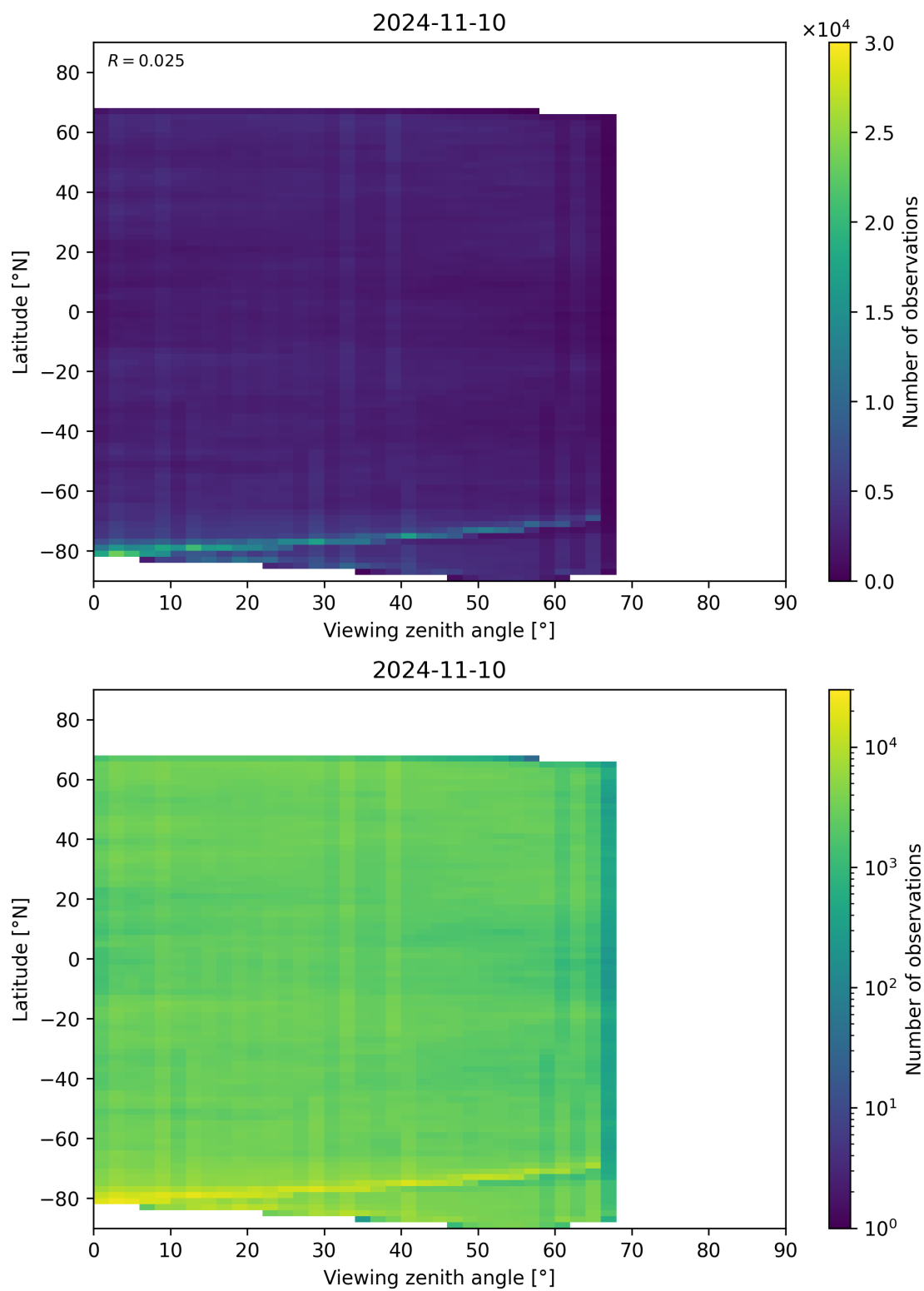
Figure 74: Scatter density plot of “Viewing zenith angle” against “Latitude” for 2024-11-09 to 2024-11-11.
