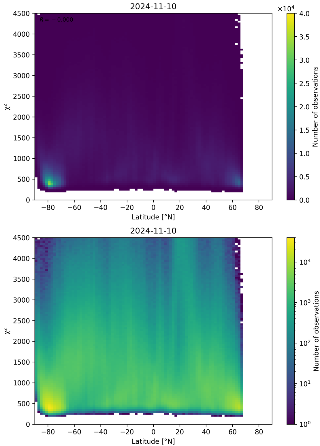
Figure 54: Scatter density plot of “Latitude” against “ \chi^2 ” for 2024-11-09 to 2024-11-11.
