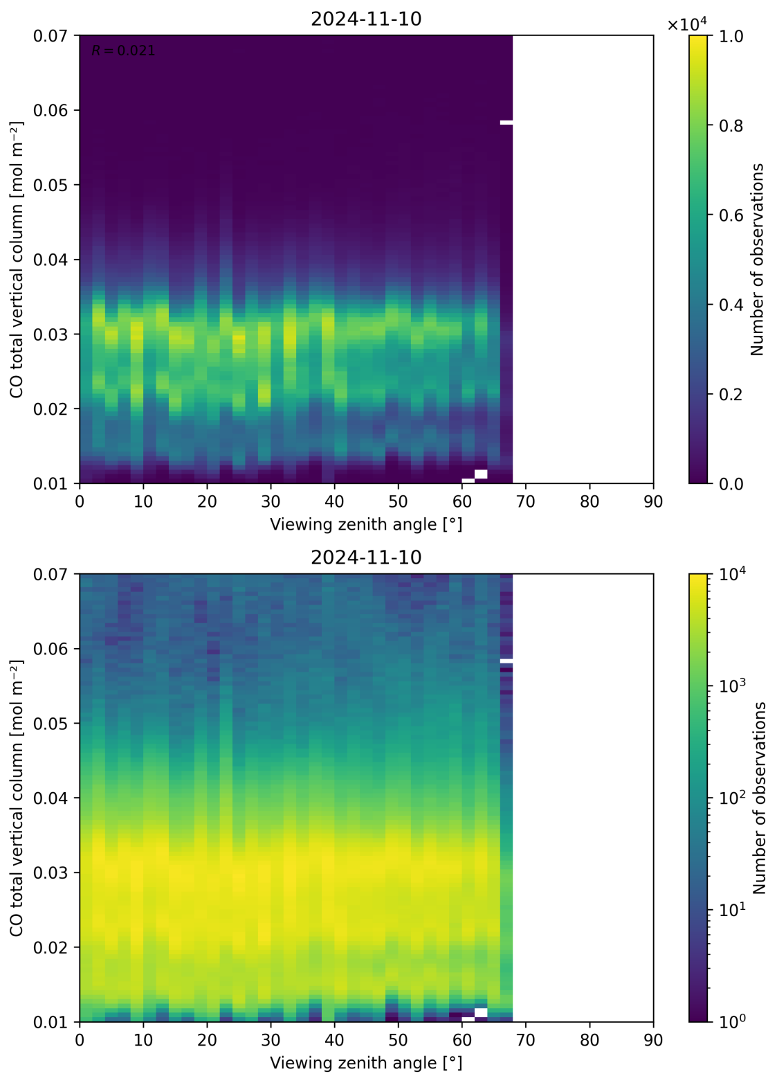
Figure 69: Scatter density plot of “Viewing zenith angle” against “CO total vertical column” for 2024-11-09 to 2024-11-11.
