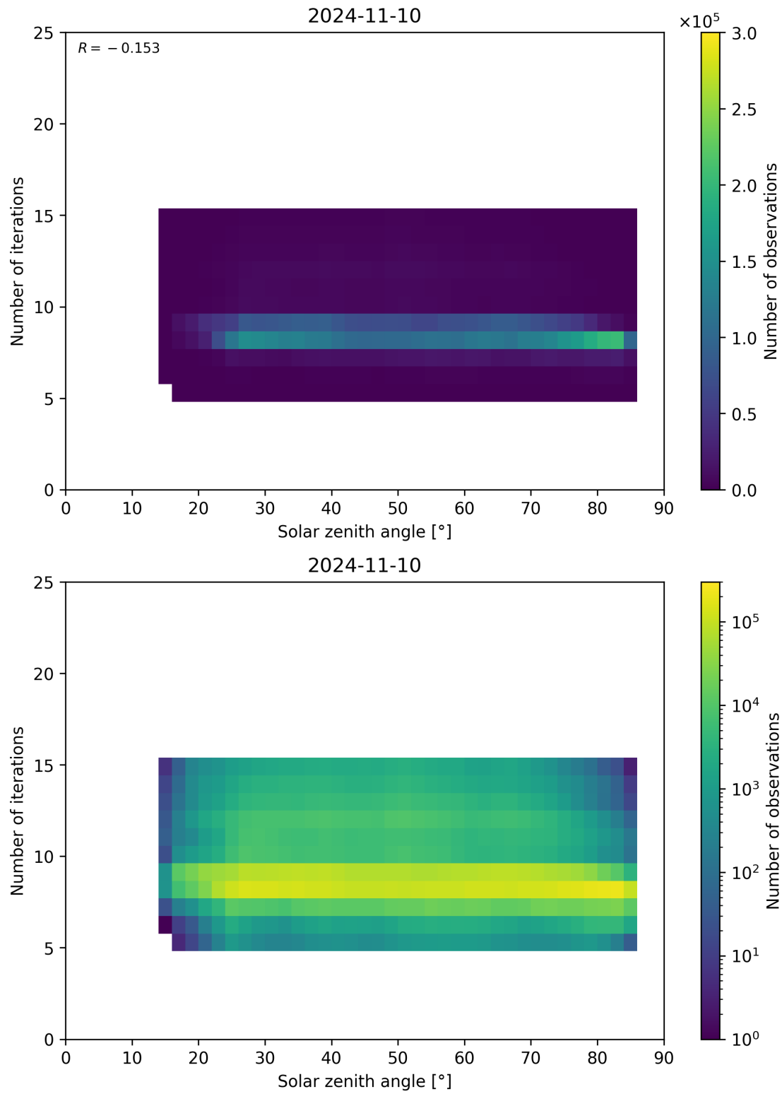
Figure 67: Scatter density plot of “Solar zenith angle” against “Number of iterations” for 2024-11-09 to 2024-11-11.
