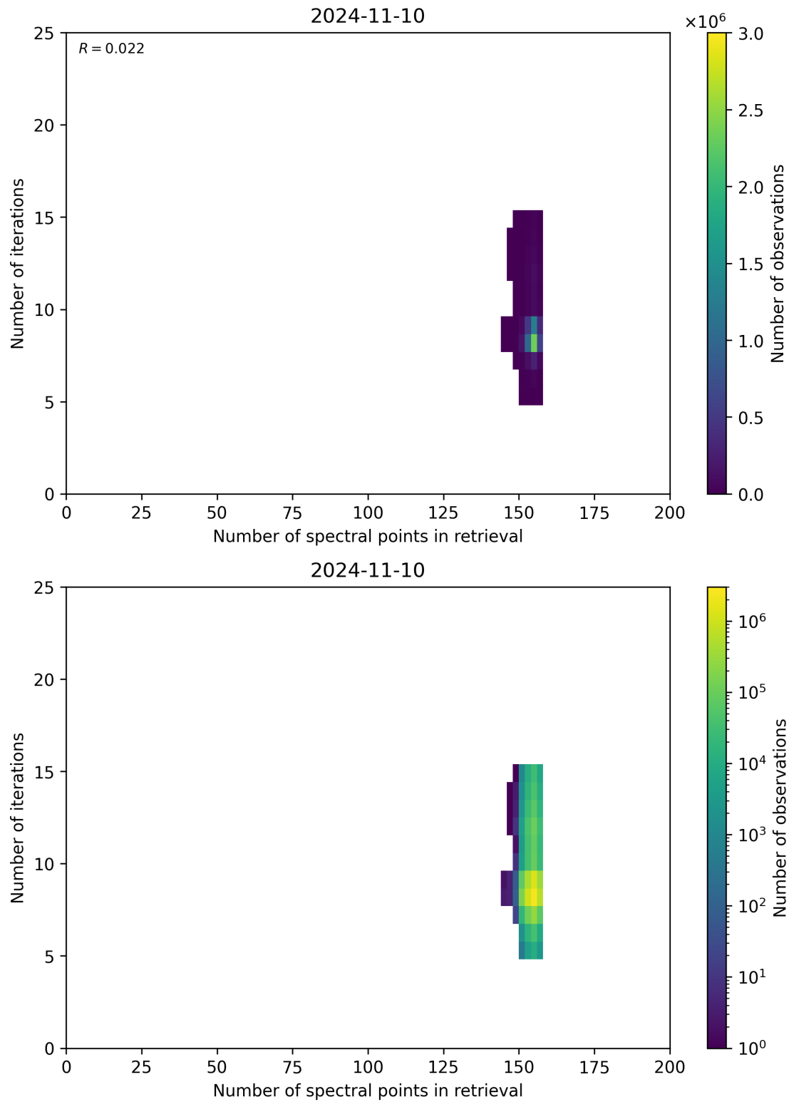
Figure 60: Scatter density plot of “Number of spectral points in retrieval” against “Number of iterations” for 2024-11-09 to 2024-11-11.
