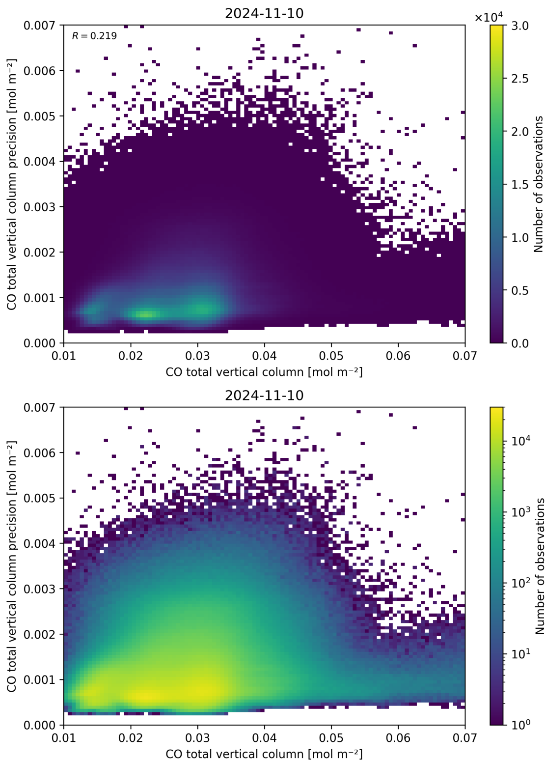
Figure 34: Scatter density plot of “CO total vertical column” against “CO total vertical column precision” for 2024-11-09 to 2024-11-11.
