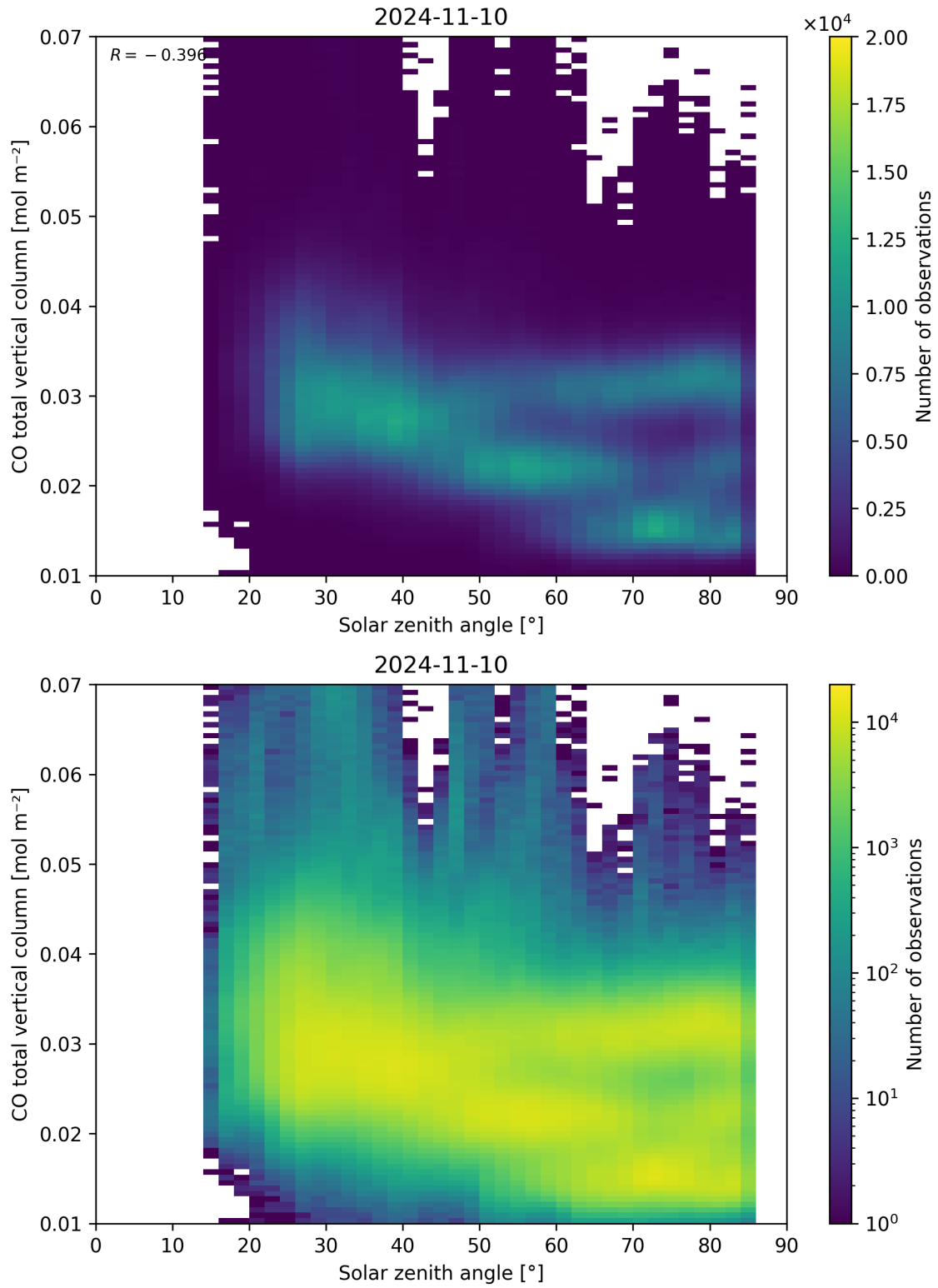
Figure 61: Scatter density plot of “Solar zenith angle” against “CO total vertical column” for 2024-11-09 to 2024-11-11.
