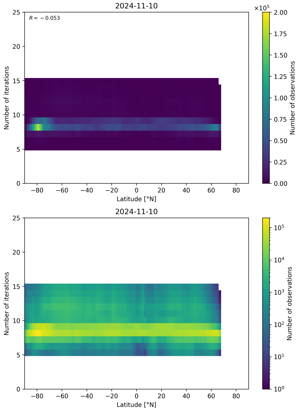
Figure 56: Scatter density plot of “Latitude” against “Number of iterations” for 2024-11-09 to 2024-11-11.
