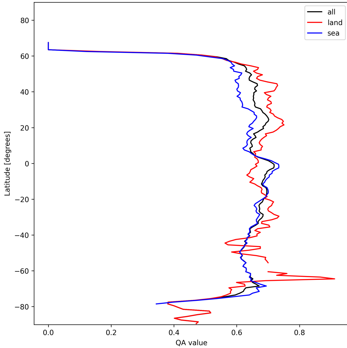
Figure 9: Zonal average of “QA value” for 2024-11-09 to 2024-11-11.
