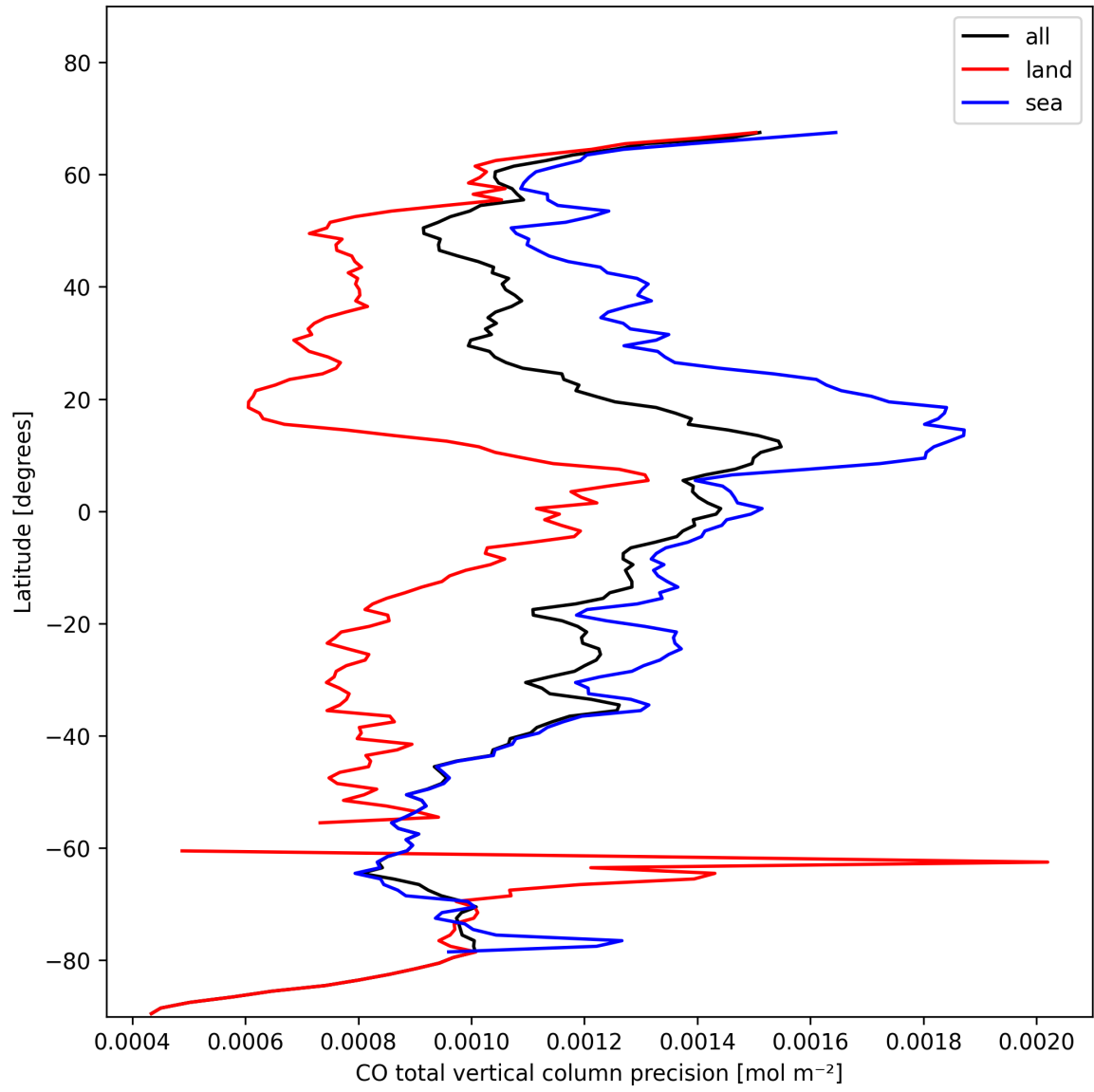
Figure 12: Zonal average of “CO total vertical column precision” for 2024-11-09 to 2024-11-11.
