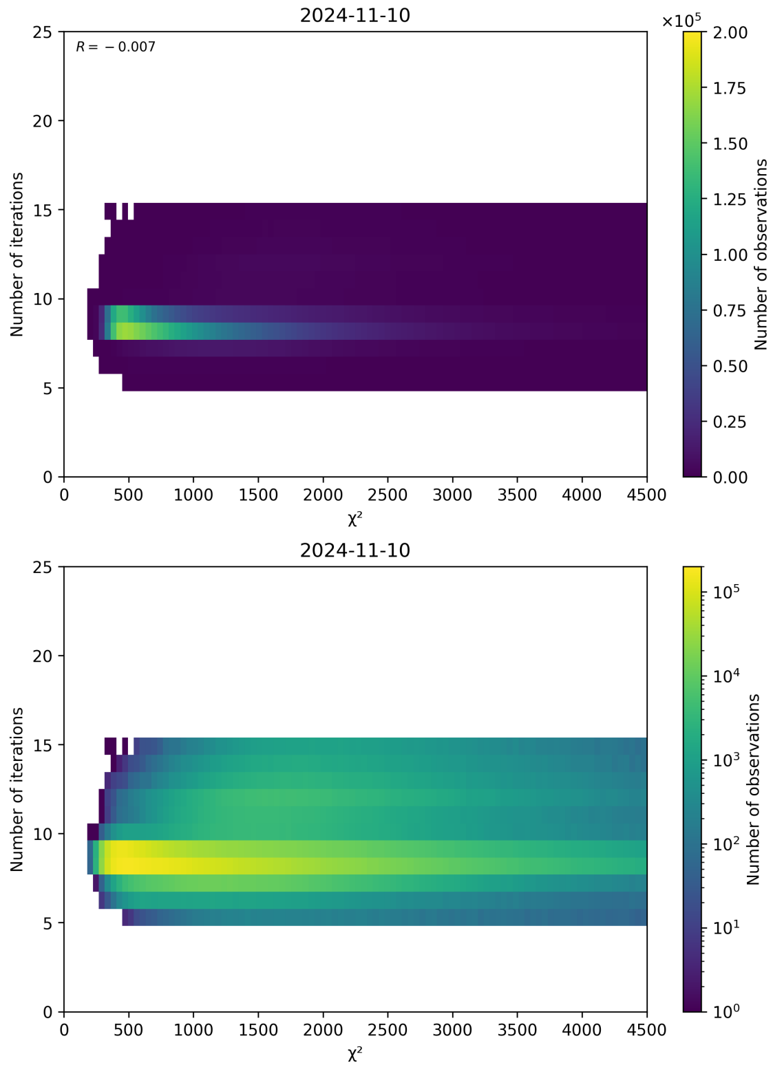
Figure 49: Scatter density plot of “ \chi^2 ” against “Number of iterations” for 2024-11-09 to 2024-11-11.
