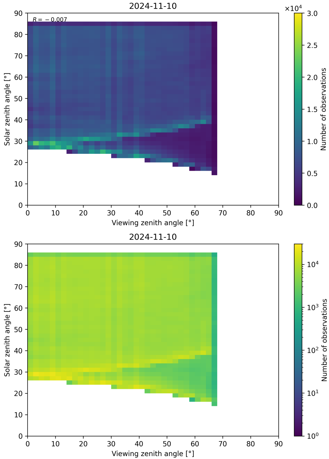
Figure 77: Scatter density plot of “Viewing zenith angle” against “Solar zenith angle” for 2024-11-09 to 2024-11-11.
