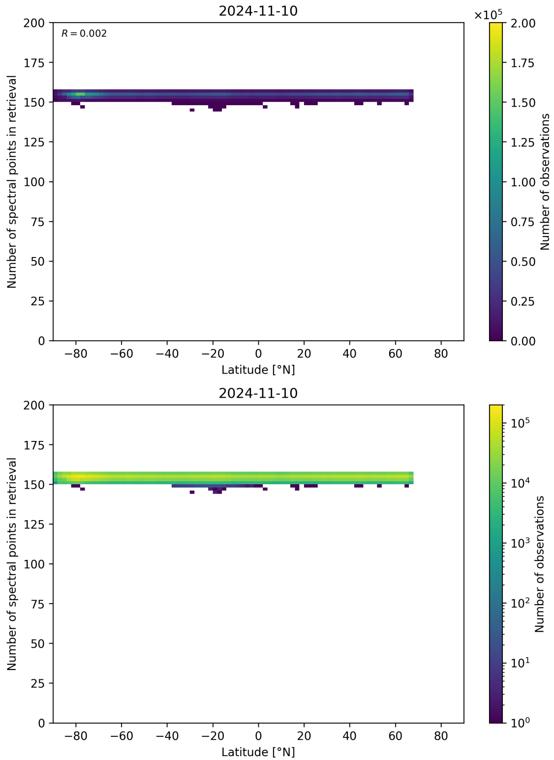
Figure 57: Scatter density plot of “Latitude” against “Number of spectral points in retrieval” for 2024-11-09 to 2024-11-11.
