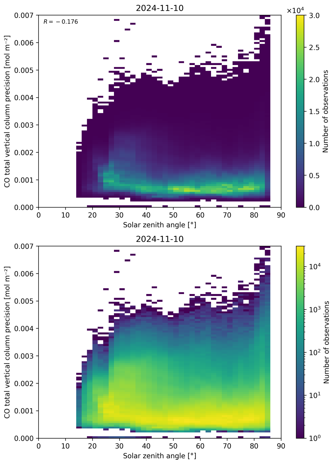
Figure 63: Scatter density plot of “Solar zenith angle” against “CO total vertical column precision” for 2024-11-09 to 2024-11-11.
