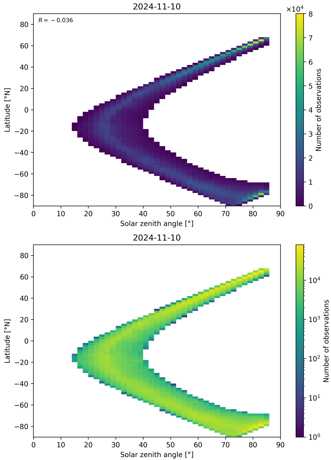
Figure 66: Scatter density plot of “Solar zenith angle” against “Latitude” for 2024-11-09 to 2024-11-11.
