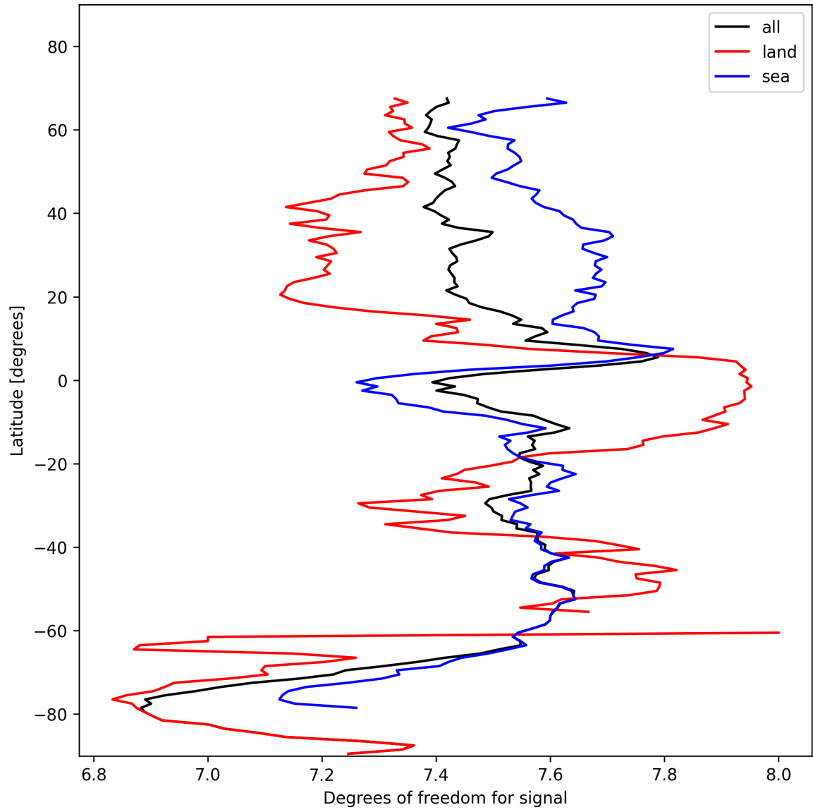
Figure 15: Zonal average of “Degrees of freedom for signal” for 2024-11-09 to 2024-11-11.
