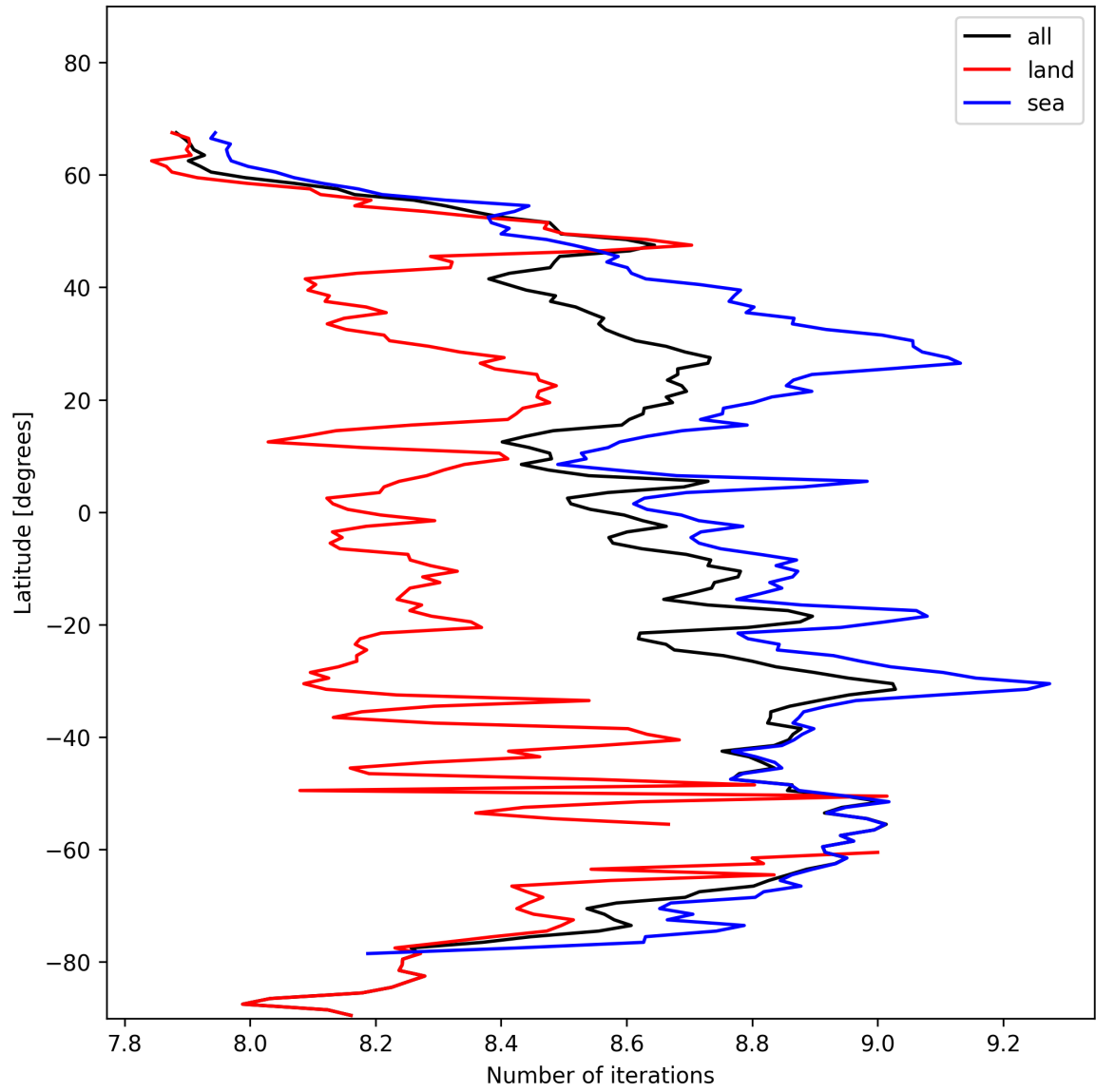
Figure 16: Zonal average of “Number of iterations” for 2024-11-09 to 2024-11-11.
