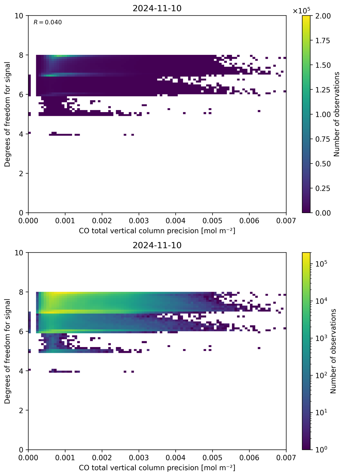
Figure 45: Scatter density plot of “CO total vertical column precision” against “Degrees of freedom for signal” for 2024-11-09 to 2024-11-11.
