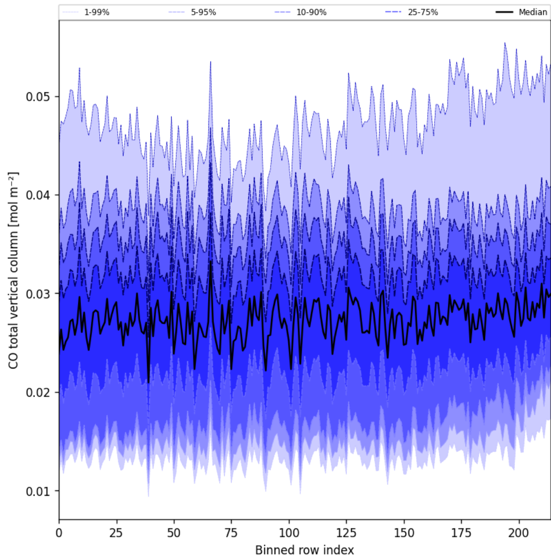
Figure 26: Along track statistics of “CO total vertical column” for 2024-11-09 to 2024-11-11
