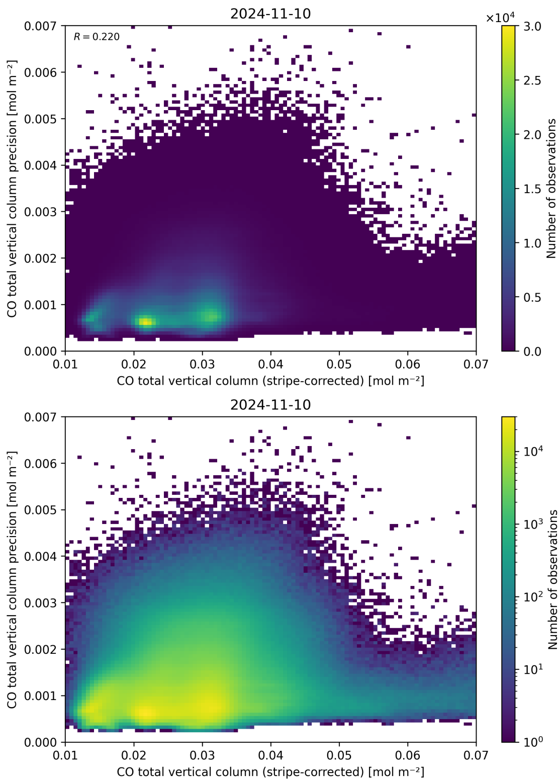
Figure 36: Scatter density plot of “CO total vertical column (stripe-corrected)” against “CO total vertical column precision” for 2024-11-09 to 2024-11-11.
