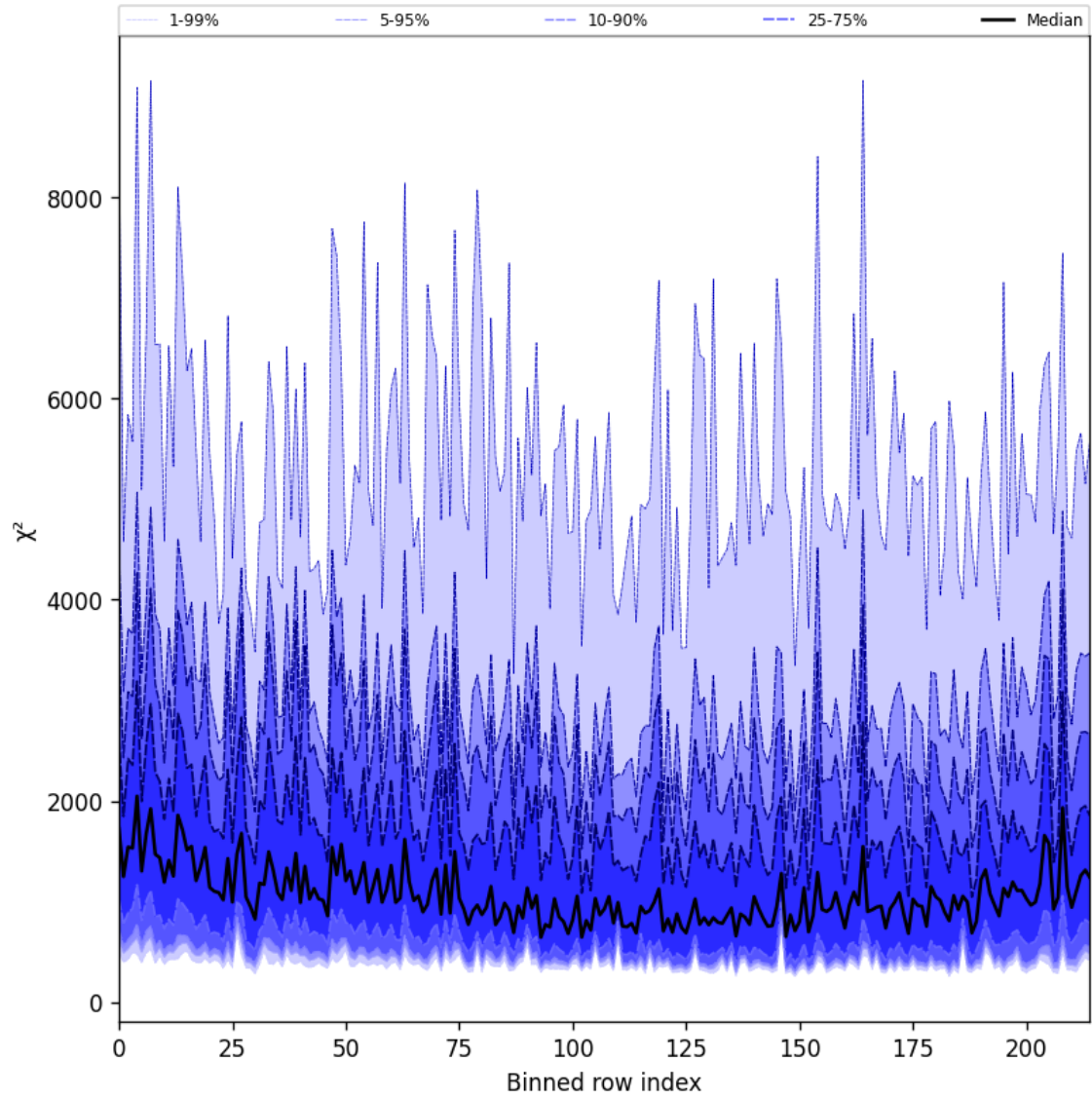
Figure 30: Along track statistics of “ \chi^2 ” for 2024-11-09 to 2024-11-11
