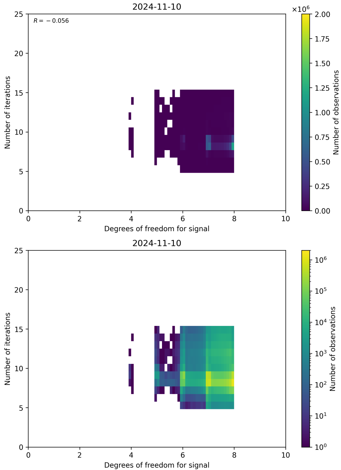
Figure 50: Scatter density plot of “Degrees of freedom for signal” against “Number of iterations” for 2024-11-09 to 2024-11-11.
