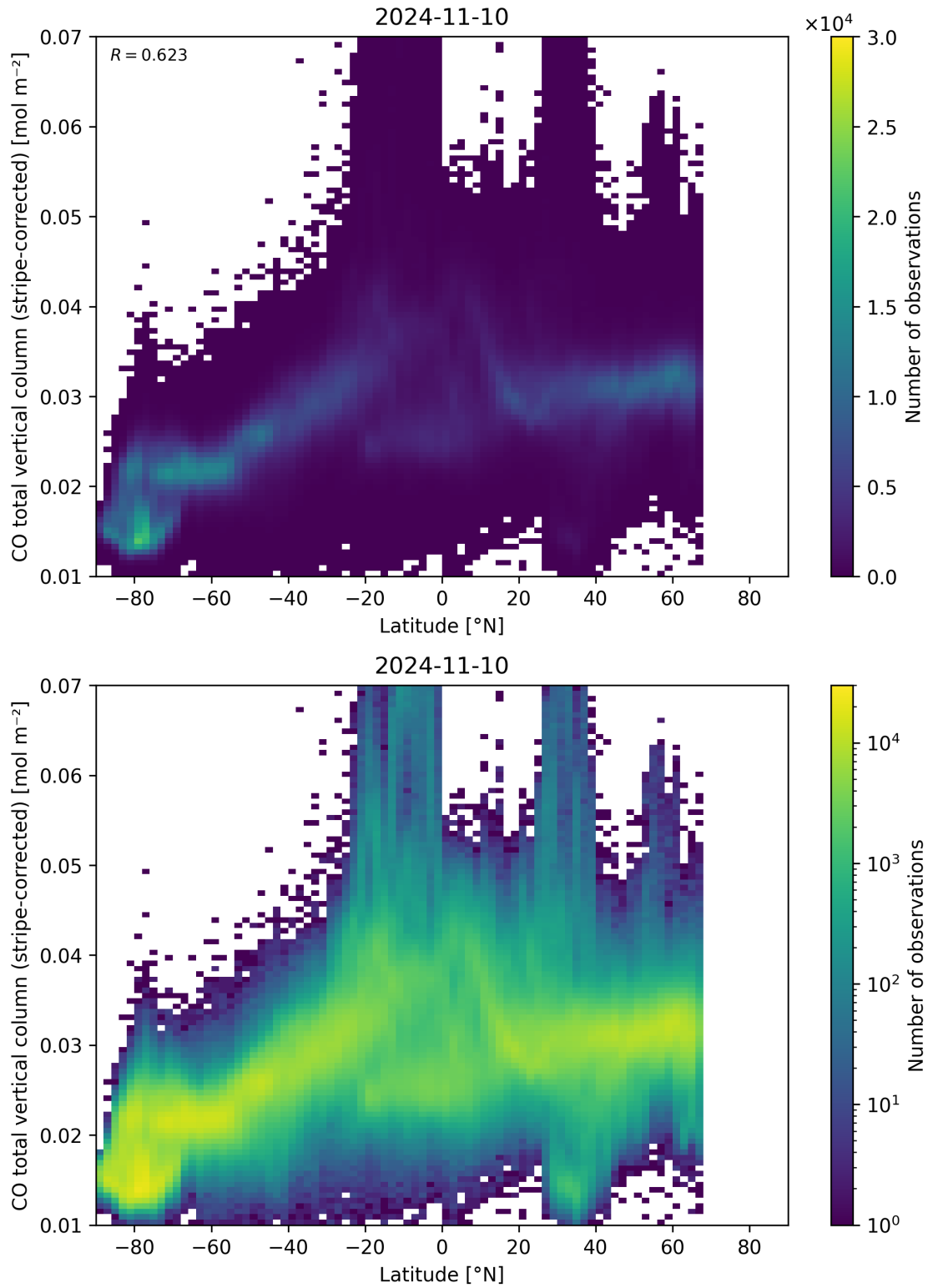
Figure 52: Scatter density plot of “Latitude” against “CO total vertical column (stripe-corrected)” for 2024-11-09 to 2024-11-11.
