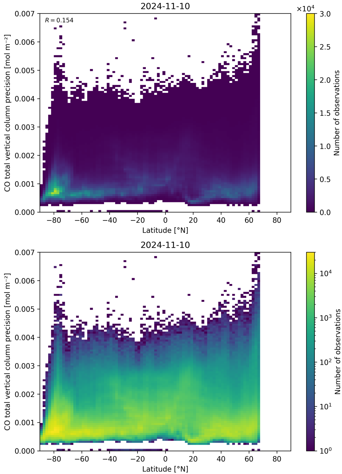
Figure 53: Scatter density plot of “Latitude” against “CO total vertical column precision” for 2024-11-09 to 2024-11-11.
