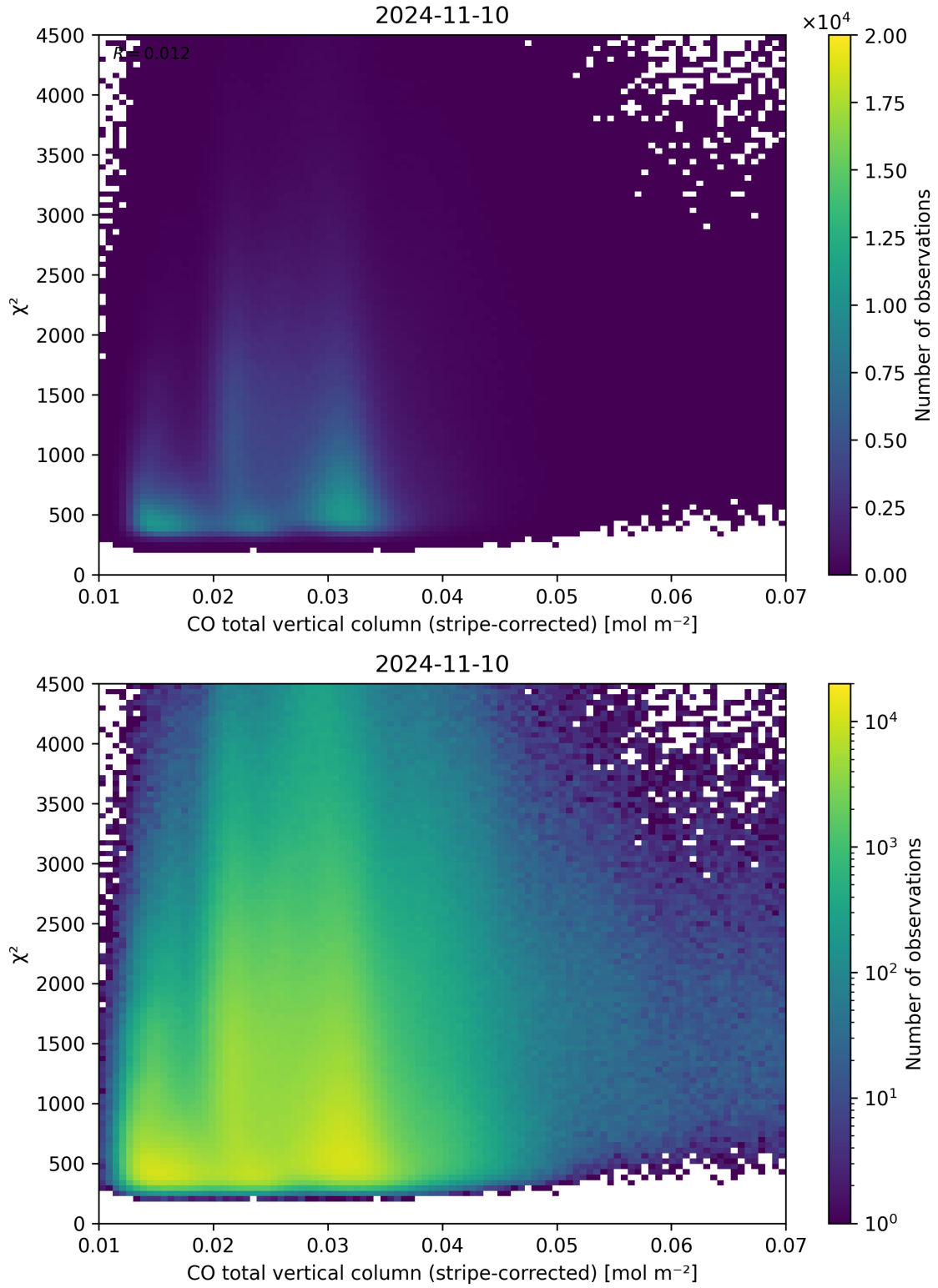
Figure 37: Scatter density plot of “CO total vertical column (stripe-corrected)” against “ \chi^2 ” for 2024-11-09 to 2024-11-11.
