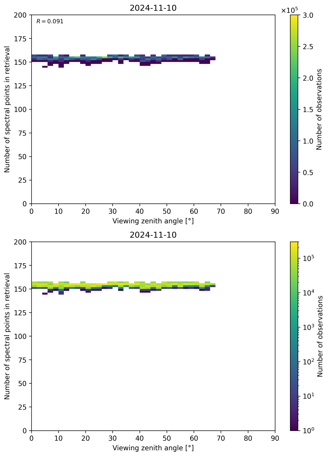
Figure 76: Scatter density plot of “Viewing zenith angle” against “Number of spectral points in retrieval” for 2024-11-09 to 2024-11-11.
