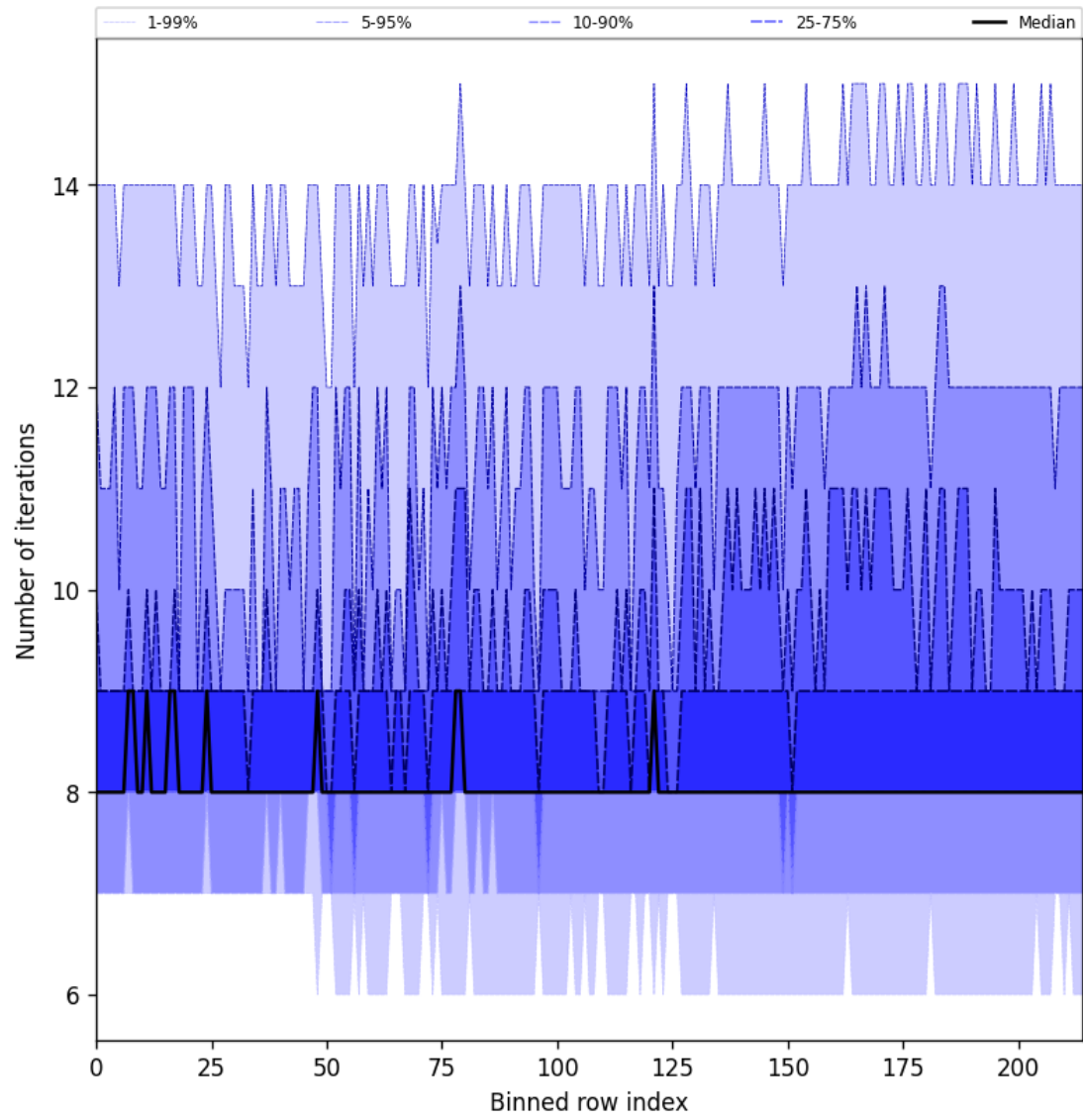
Figure 32: Along track statistics of “Number of iterations” for 2024-11-09 to 2024-11-11
