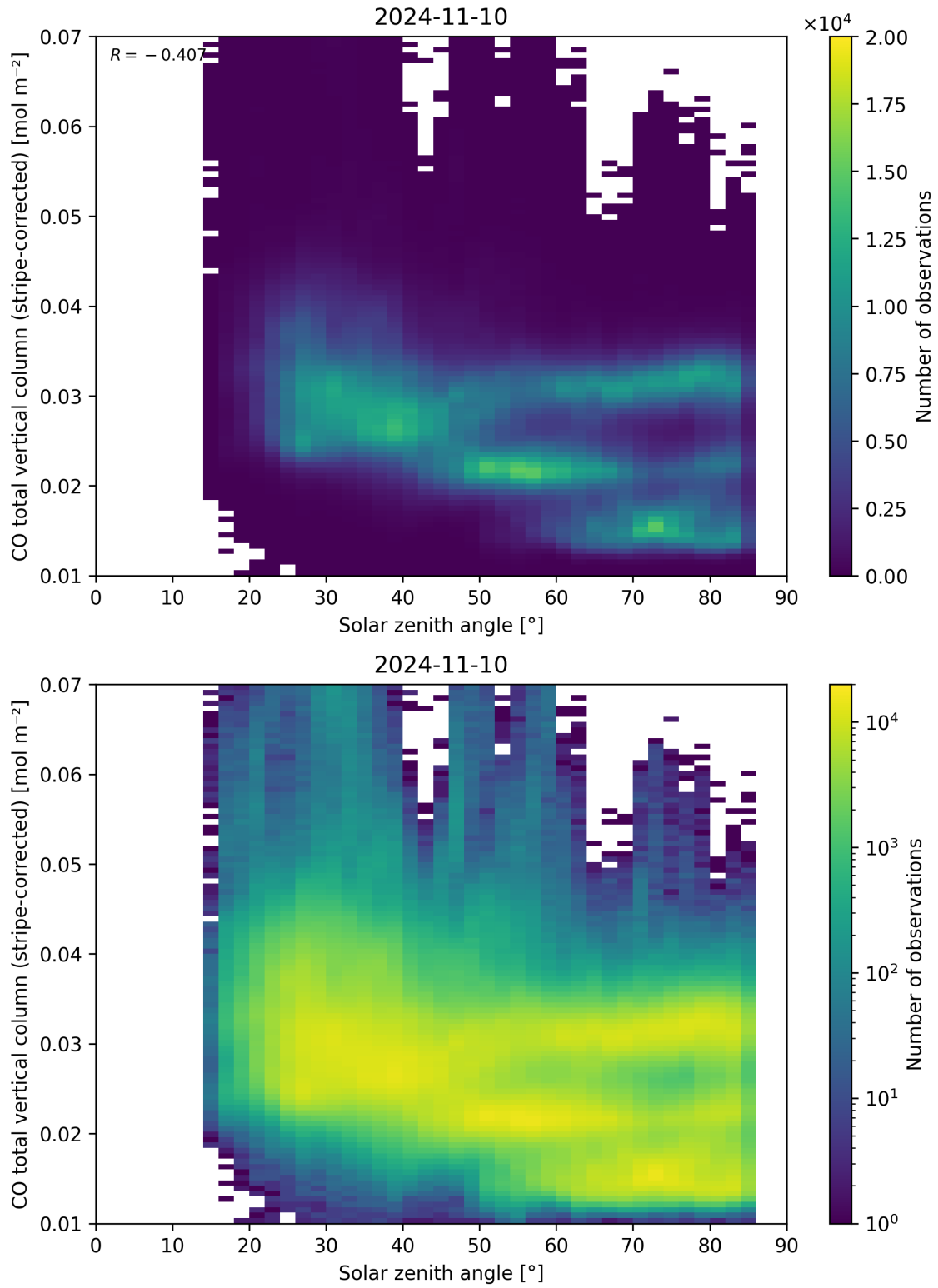
Figure 62: Scatter density plot of “Solar zenith angle” against “CO total vertical column (stripe-corrected)” for 2024-11-09 to 2024-11-11.
