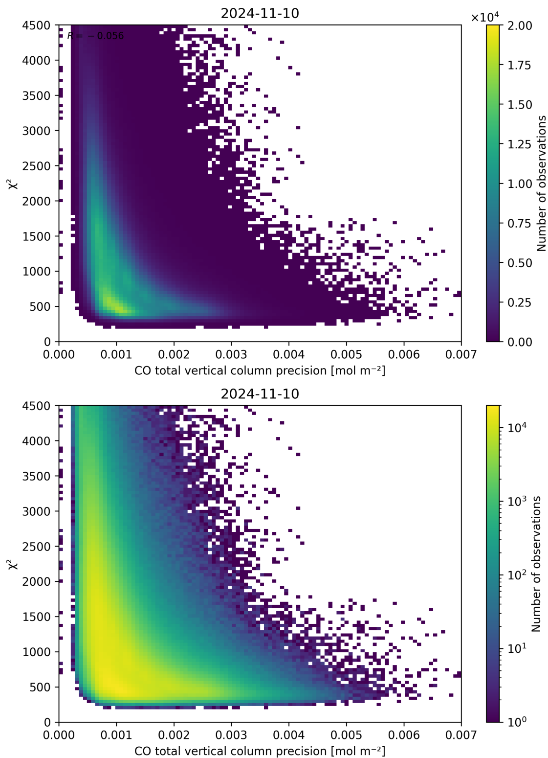
Figure 44: Scatter density plot of “CO total vertical column precision” against “ \chi^2 ” for 2024-11-09 to 2024-11-11.
