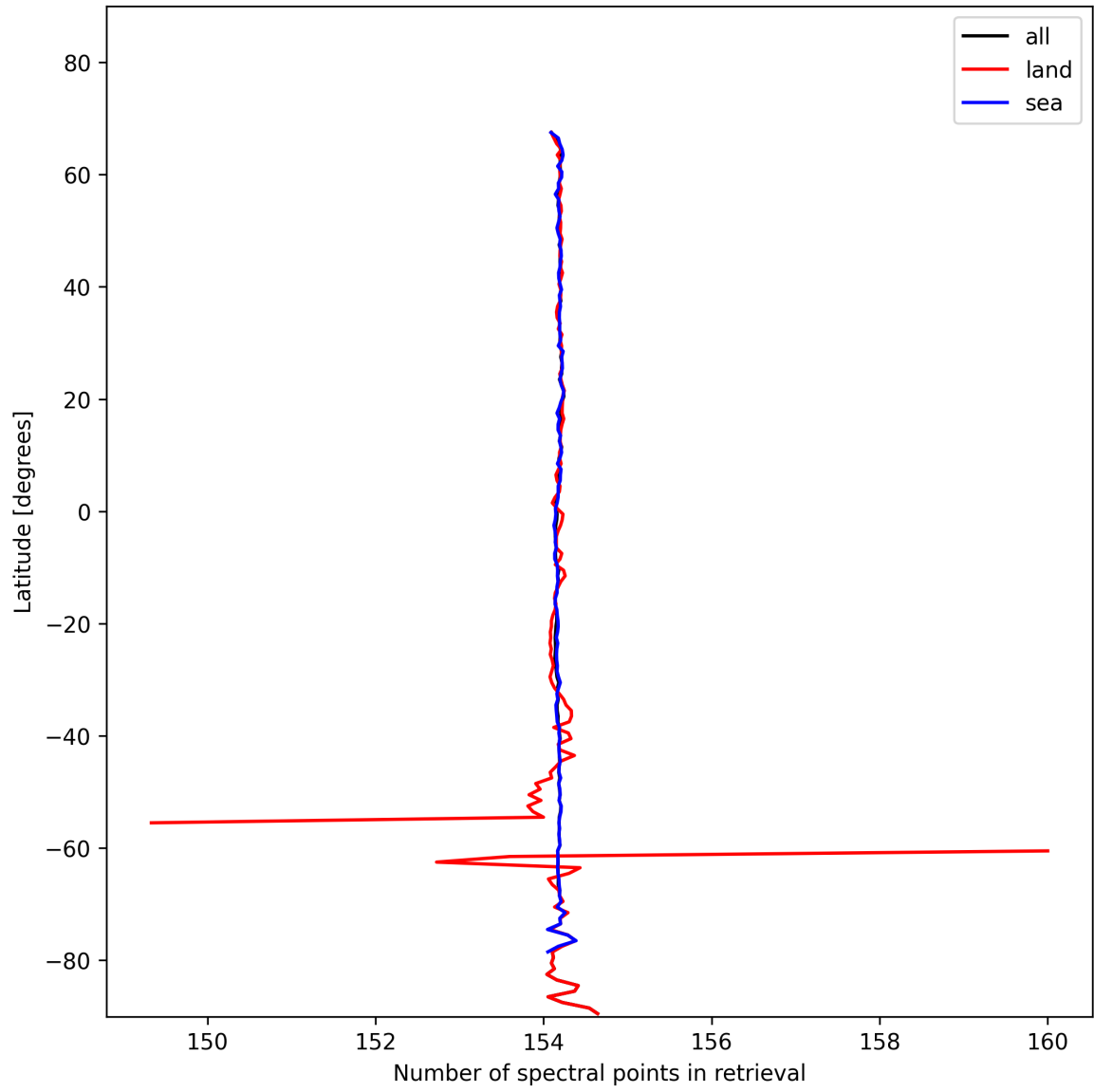
Figure 13: Zonal average of “Number of spectral points in retrieval” for 2024-11-09 to 2024-11-11.
