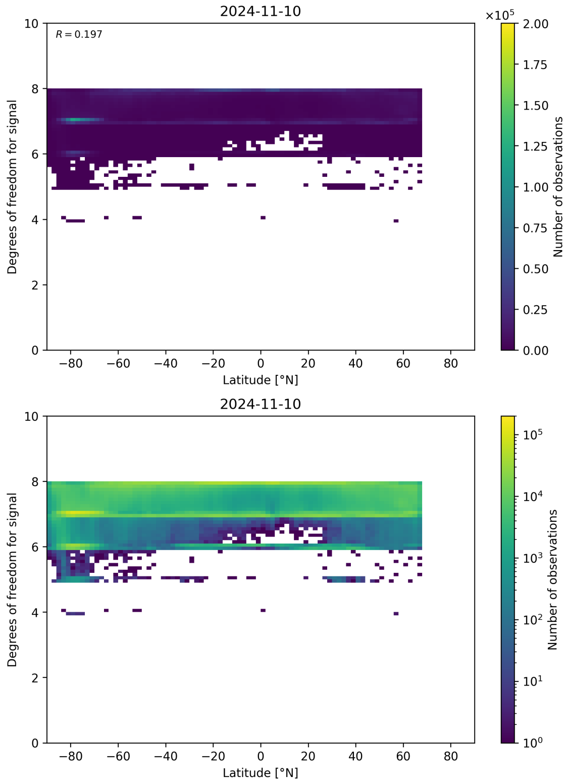
Figure 55: Scatter density plot of “Latitude” against “Degrees of freedom for signal” for 2024-11-09 to 2024-11-11.
