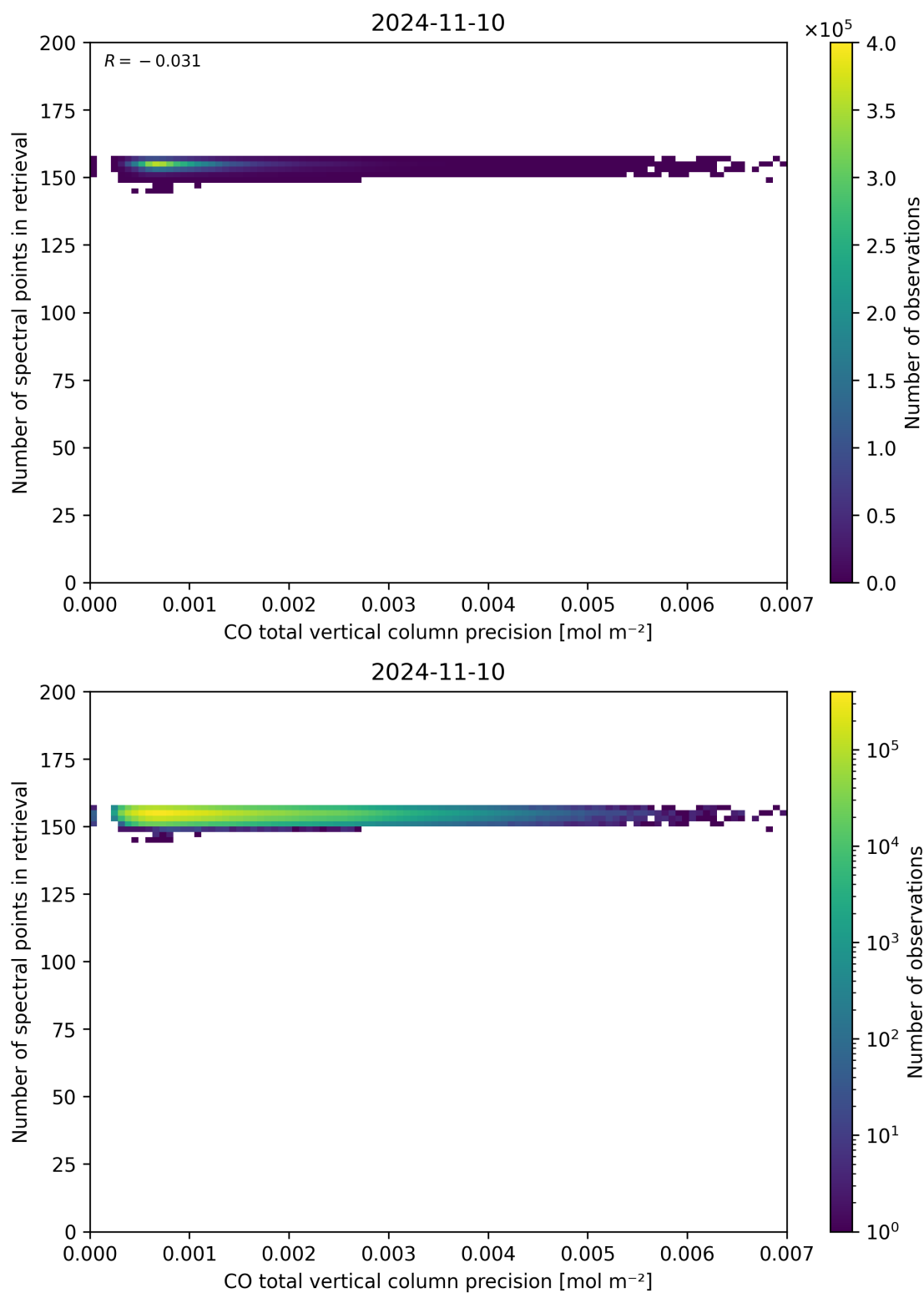
Figure 47: Scatter density plot of “CO total vertical column precision” against “Number of spectral points in retrieval” for 2024-11-09 to 2024-11-11.
