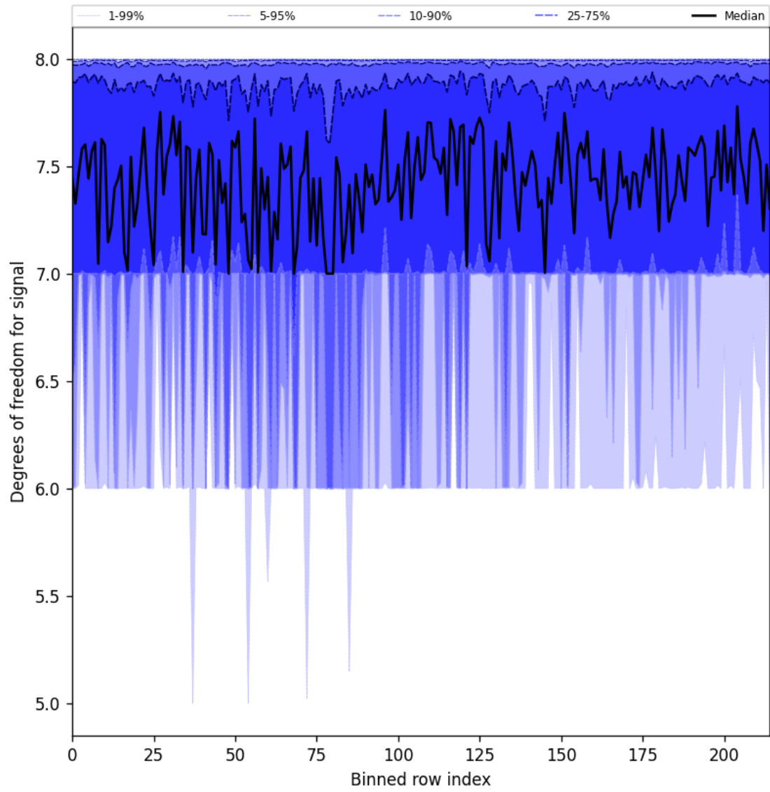
Figure 31: Along track statistics of “Degrees of freedom for signal” for 2024-11-09 to 2024-11-11
