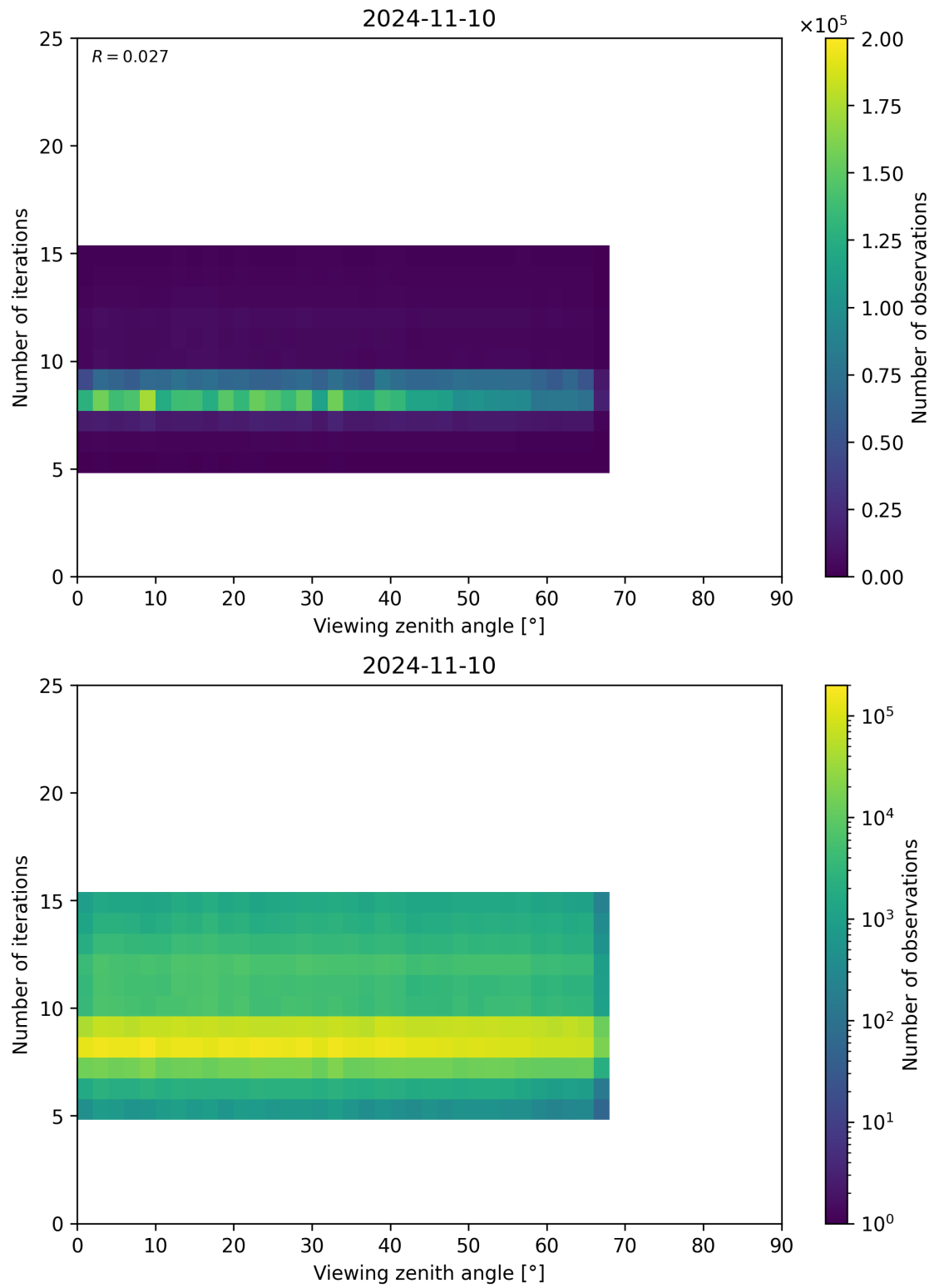
Figure 75: Scatter density plot of “Viewing zenith angle” against “Number of iterations” for 2024-11-09 to 2024-11-11.
