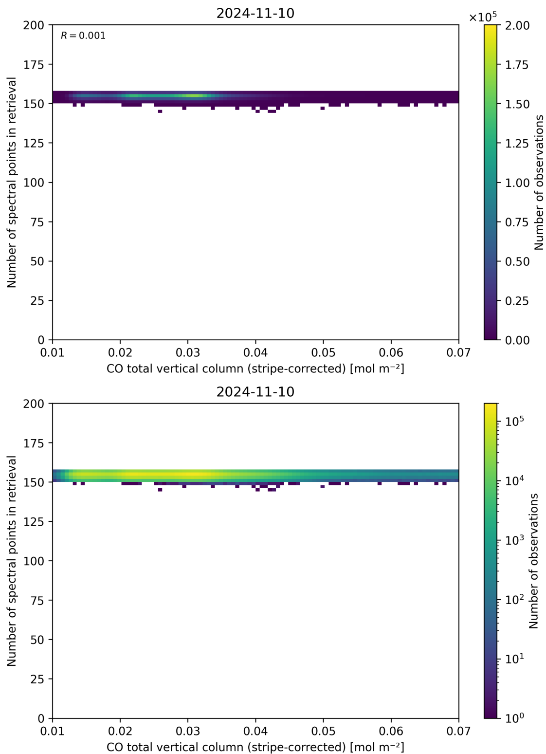
Figure 40: Scatter density plot of “CO total vertical column (stripe-corrected)” against “Number of spectral points in retrieval” for 2024-11-09 to 2024-11-11.
