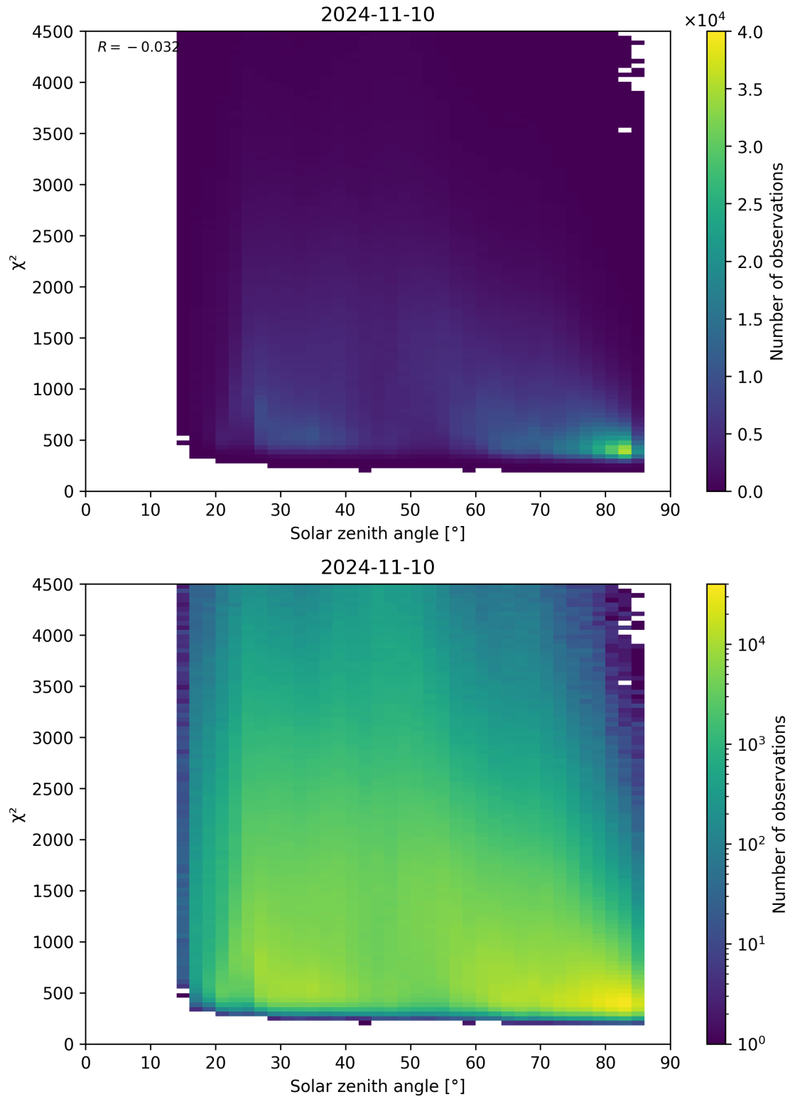
Figure 64: Scatter density plot of “Solar zenith angle” against “ \chi^2 ” for 2024-11-09 to 2024-11-11.
