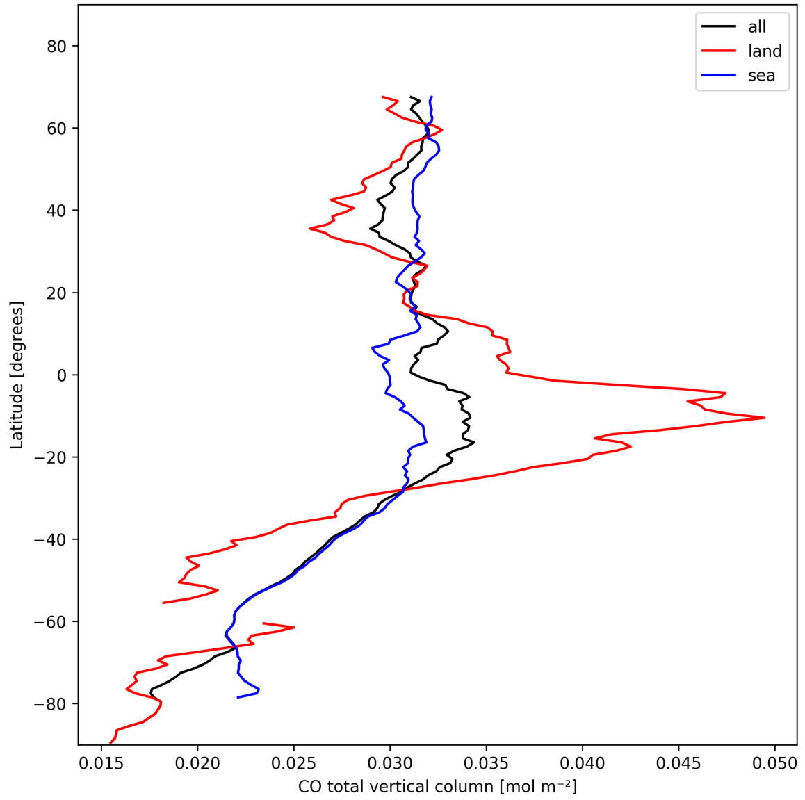
Figure 10: Zonal average of “CO total vertical column” for 2024-11-09 to 2024-11-11.
