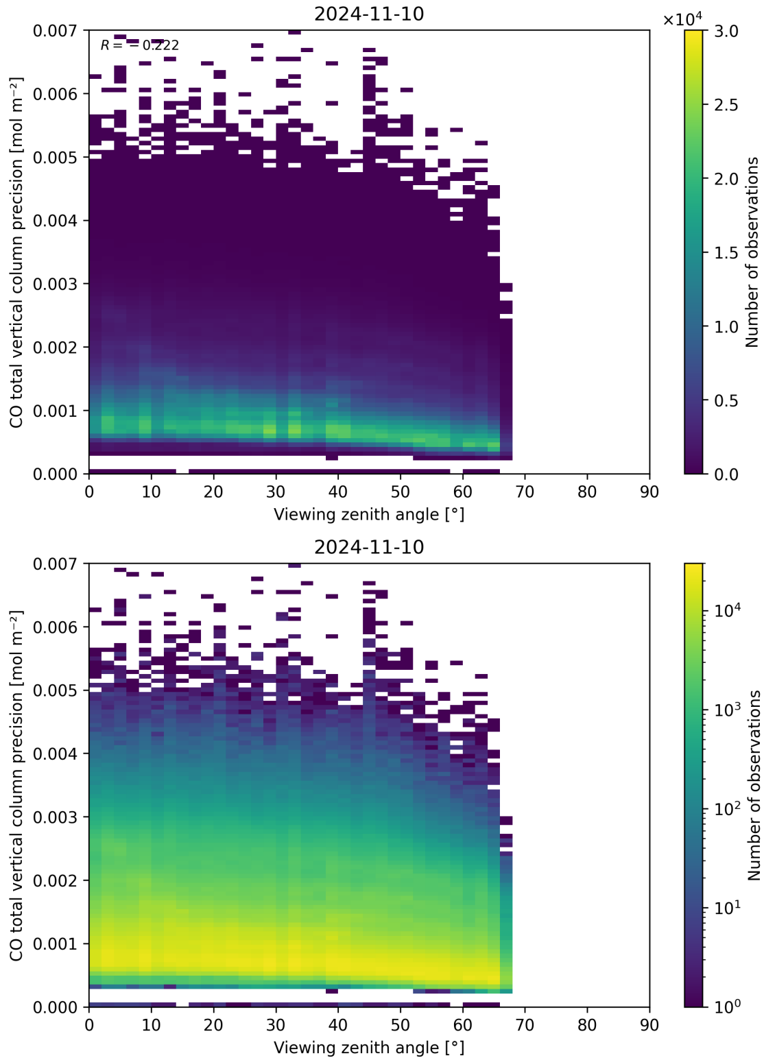
Figure 71: Scatter density plot of “Viewing zenith angle” against “CO total vertical column precision” for 2024-11-09 to 2024-11-11.
