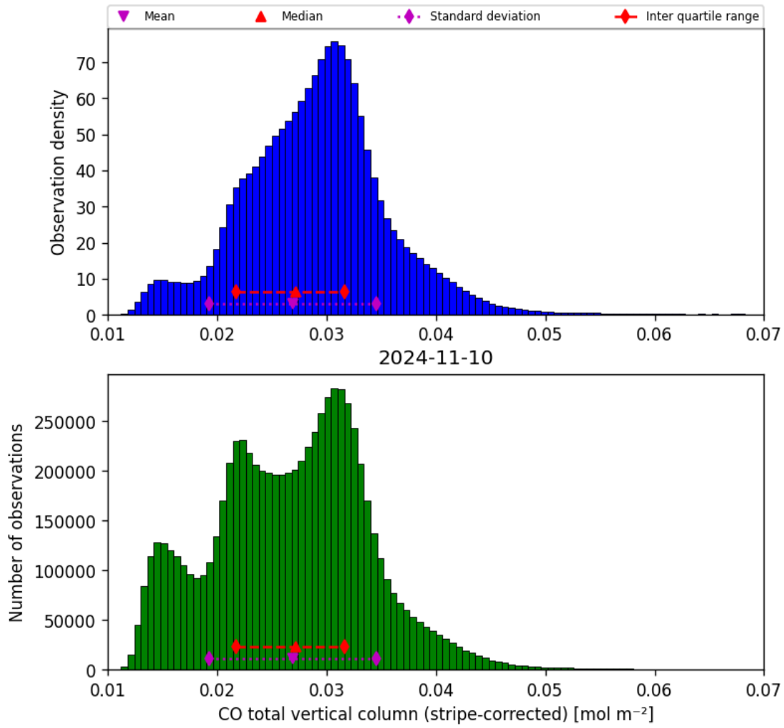
Figure 19: Histogram of “CO total vertical column (stripe-corrected)” for 2024-11-09 to 2024-11-11
