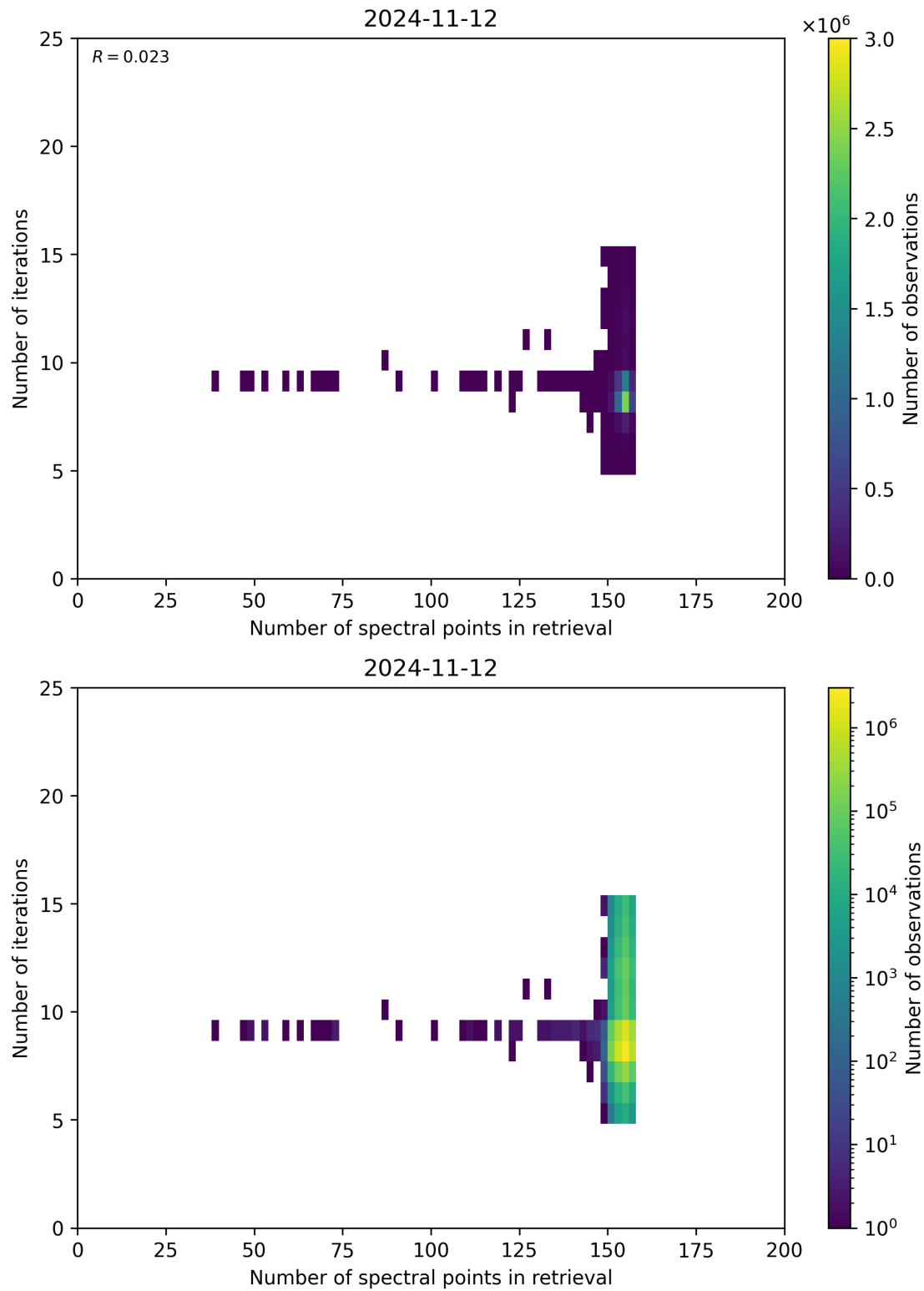
Figure 60: Scatter density plot of “Number of spectral points in retrieval” against “Number of iterations” for 2024-11-11 to 2024-11-13.
