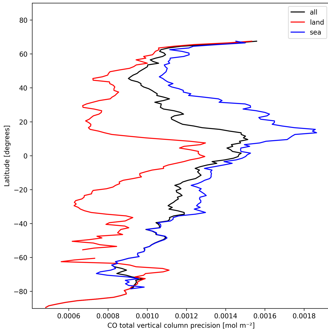
Figure 12: Zonal average of “CO total vertical column precision” for 2024-11-11 to 2024-11-13.
