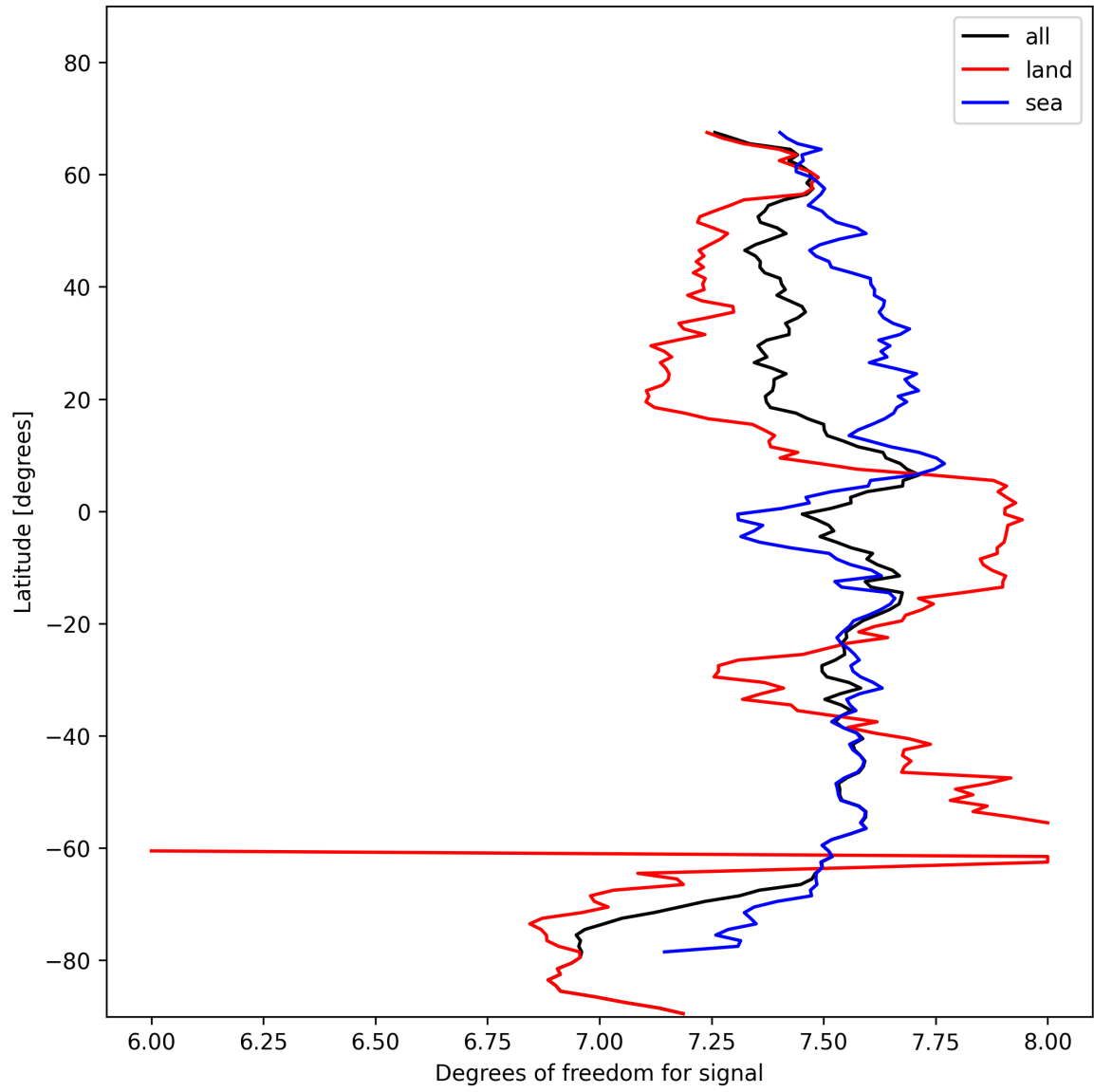
Figure 15: Zonal average of “Degrees of freedom for signal” for 2024-11-11 to 2024-11-13.
