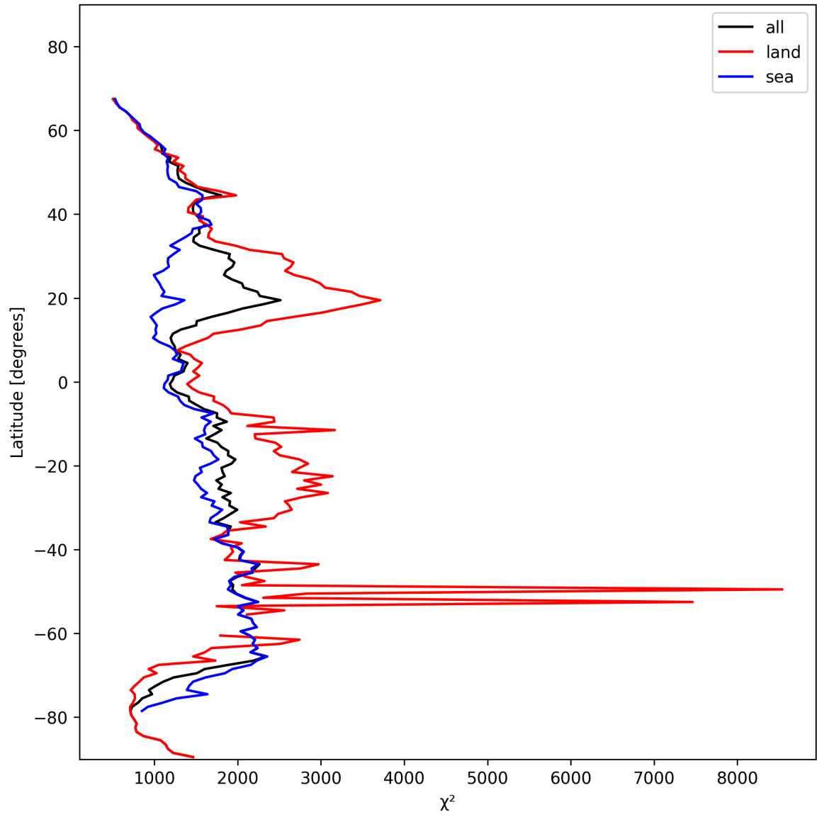
Figure 14: Zonal average of “ \chi^2 ” for 2024-11-11 to 2024-11-13.
