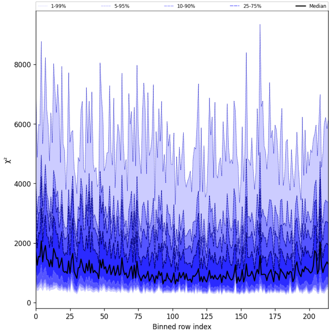
Figure 30: Along track statistics of “ \chi^2 ” for 2024-11-11 to 2024-11-13
