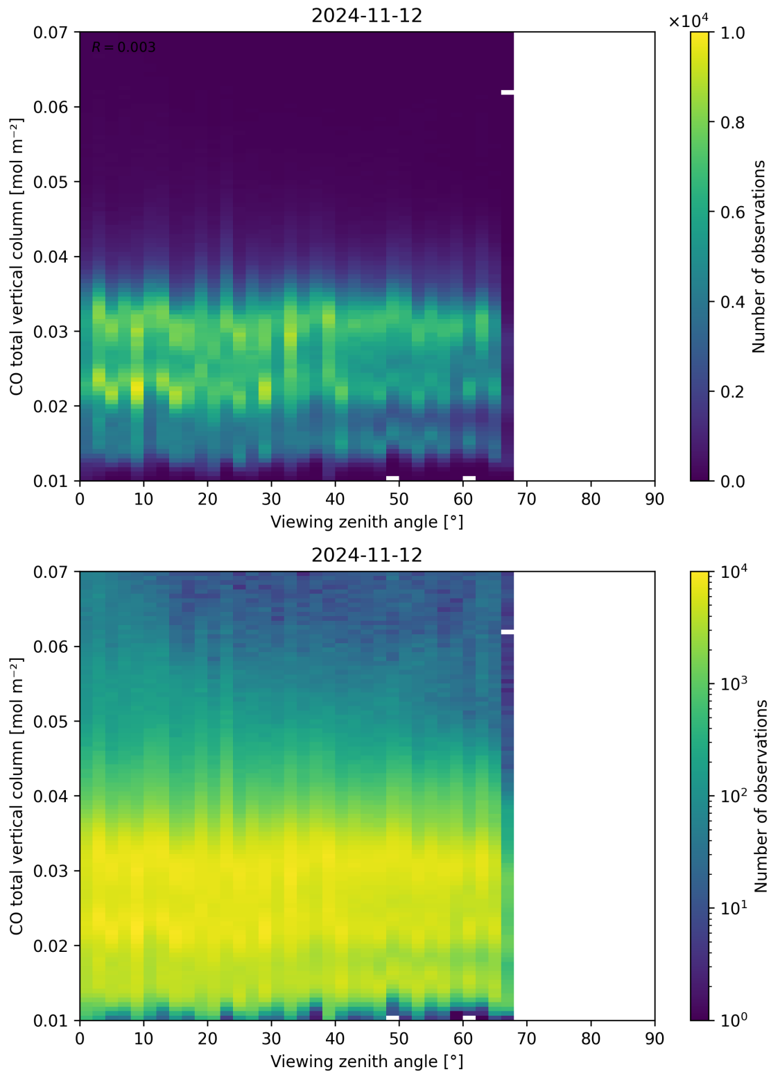
Figure 69: Scatter density plot of “Viewing zenith angle” against “CO total vertical column” for 2024-11-11 to 2024-11-13.
