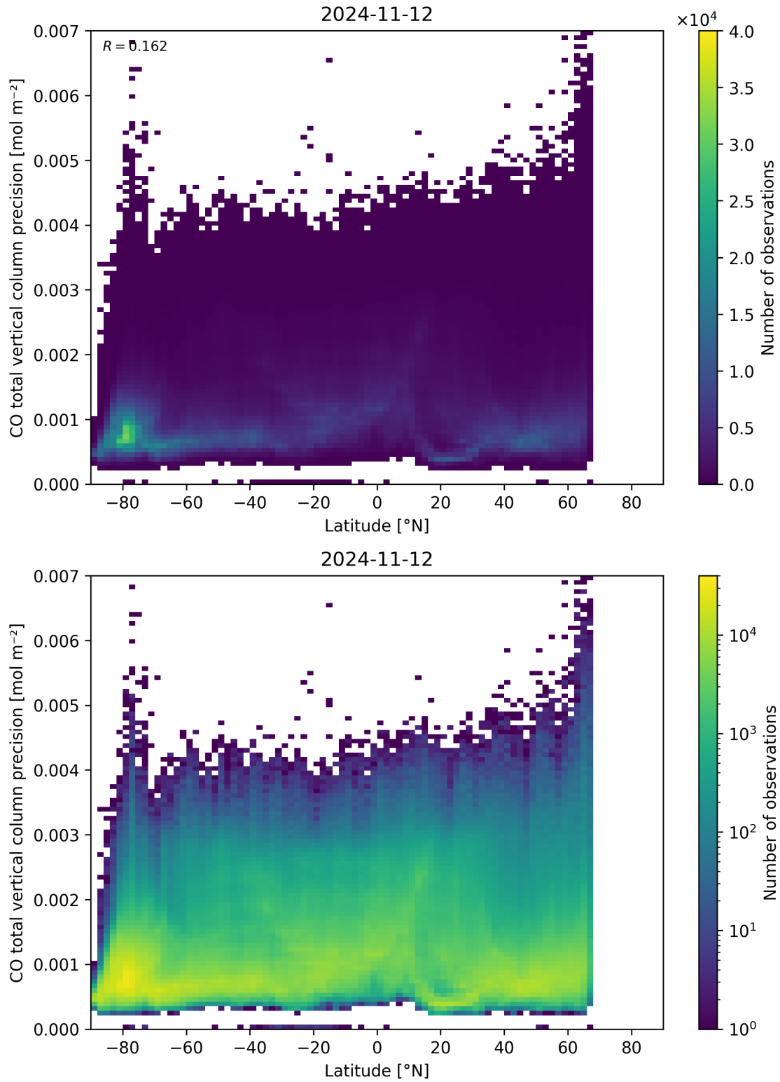
Figure 53: Scatter density plot of “Latitude” against “CO total vertical column precision” for 2024-11-11 to 2024-11-13.
