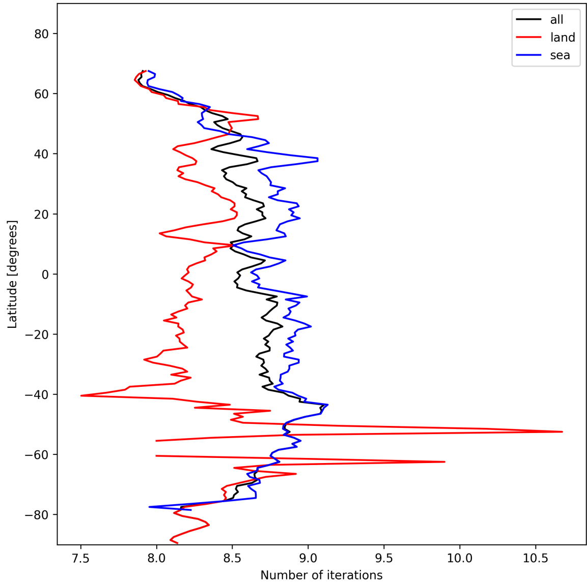
Figure 16: Zonal average of “Number of iterations” for 2024-11-11 to 2024-11-13.
