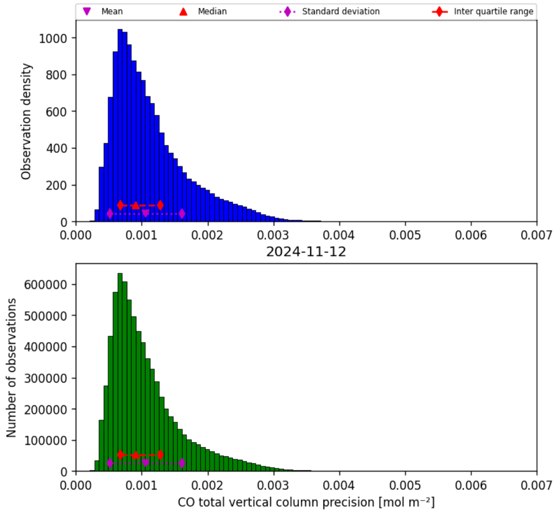
Figure 20: Histogram of “CO total vertical column precision” for 2024-11-11 to 2024-11-13
