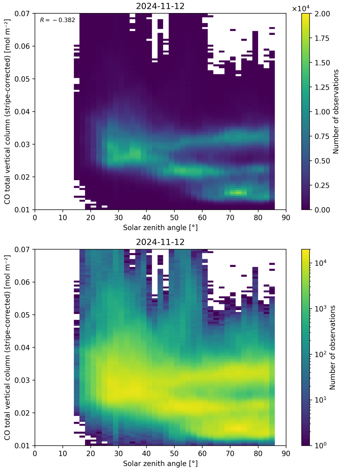
Figure 62: Scatter density plot of “Solar zenith angle” against “CO total vertical column (stripe-corrected)” for 2024-11-11 to 2024-11-13.
