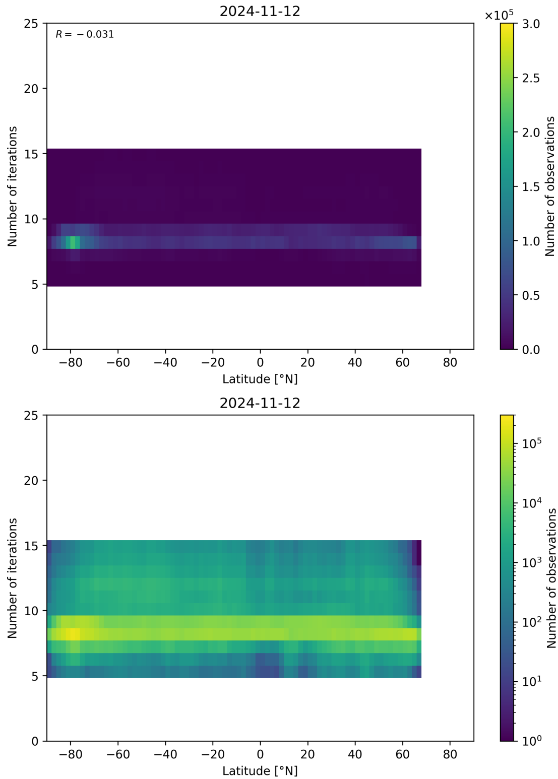
Figure 56: Scatter density plot of “Latitude” against “Number of iterations” for 2024-11-11 to 2024-11-13.
