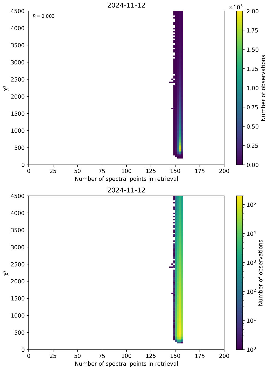
Figure 58: Scatter density plot of “Number of spectral points in retrieval” against “ \chi^2 ” for 2024-11-11 to 2024-11-13.
