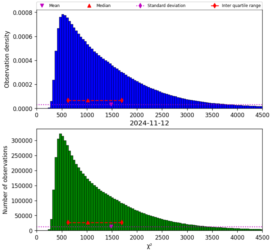
Figure 22: Histogram of “ \chi^2 ” for 2024-11-11 to 2024-11-13
