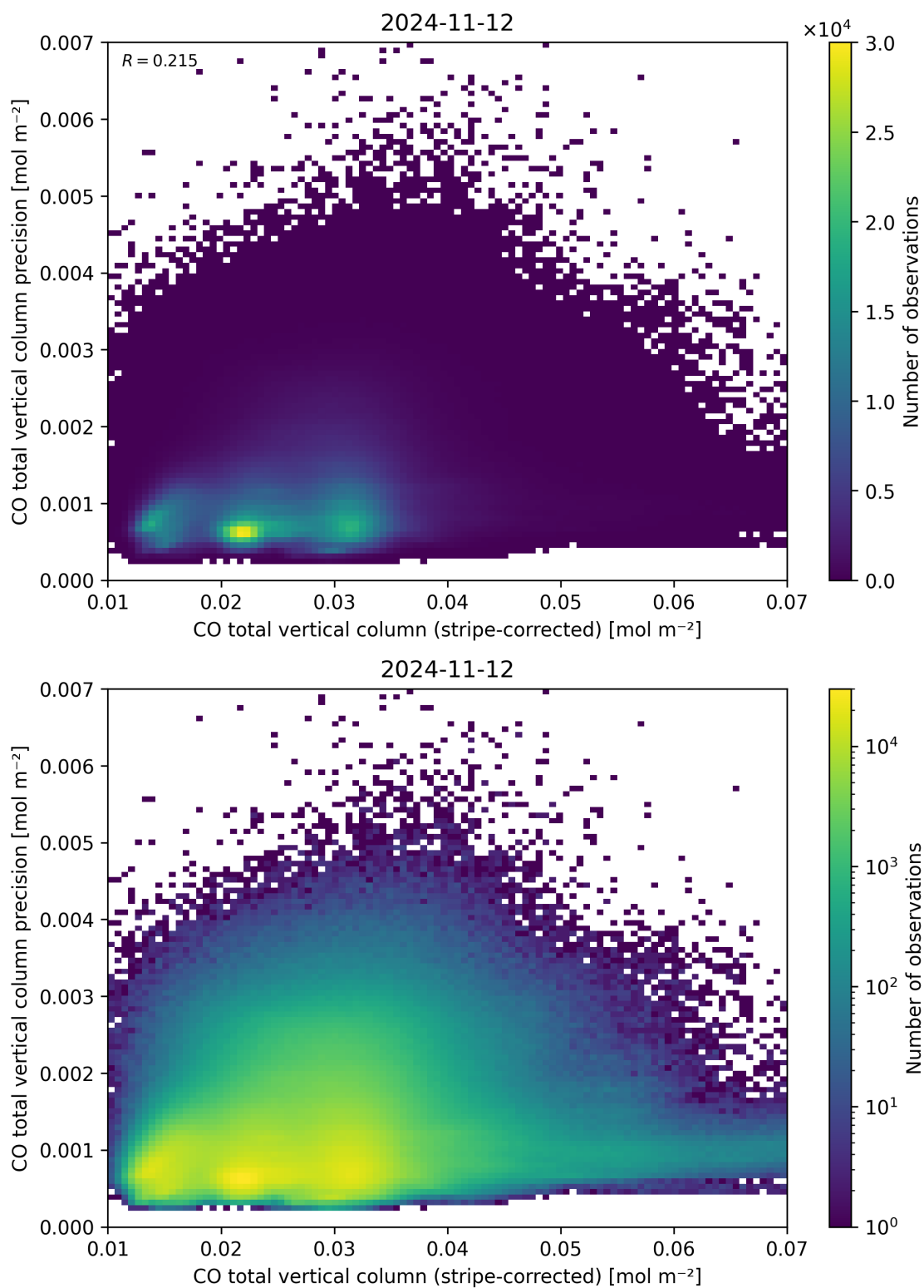
Figure 36: Scatter density plot of “CO total vertical column (stripe-corrected)” against “CO total vertical column precision” for 2024-11-11 to 2024-11-13.
