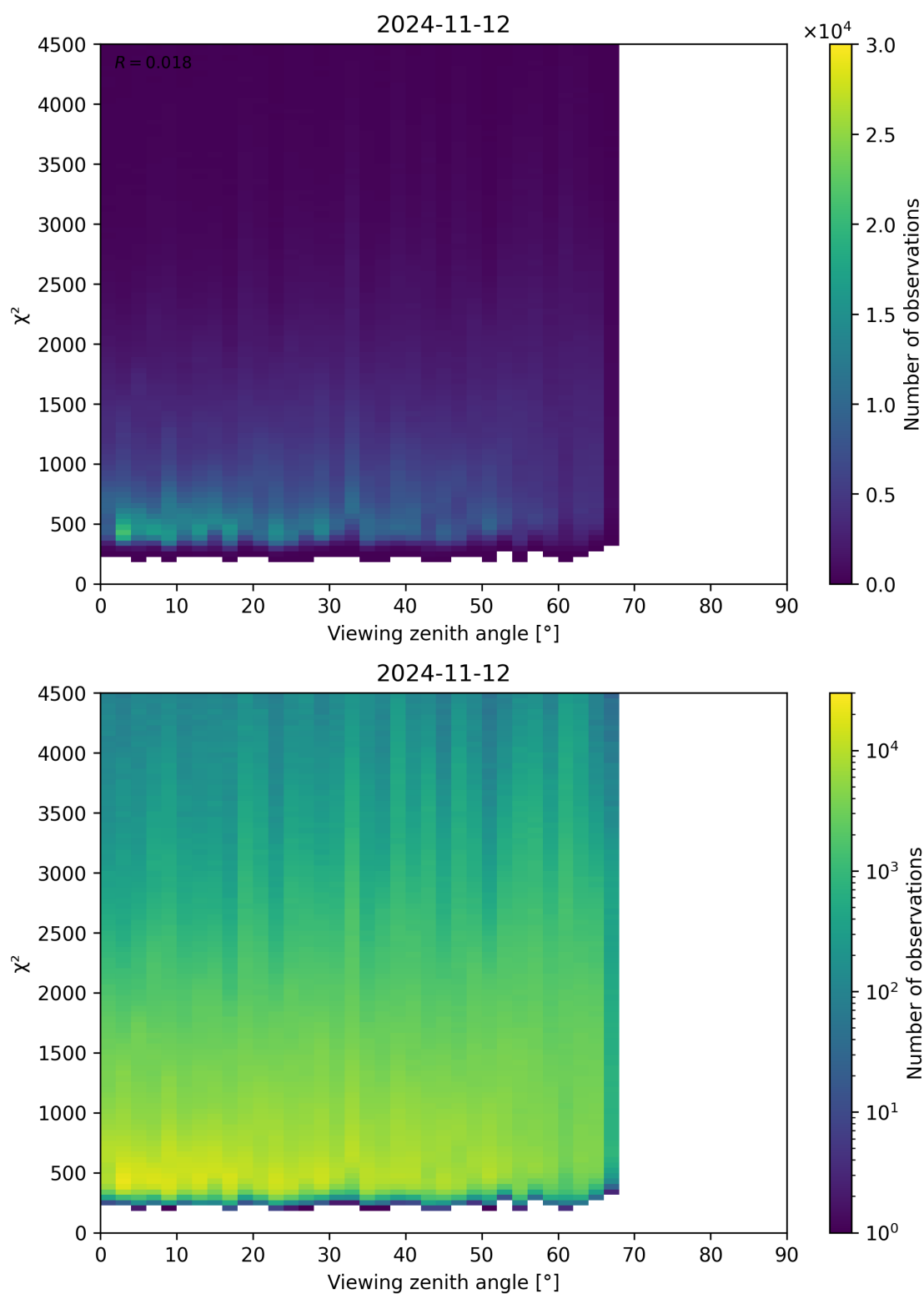
Figure 72: Scatter density plot of “Viewing zenith angle” against “ \chi^2 ” for 2024-11-11 to 2024-11-13.
