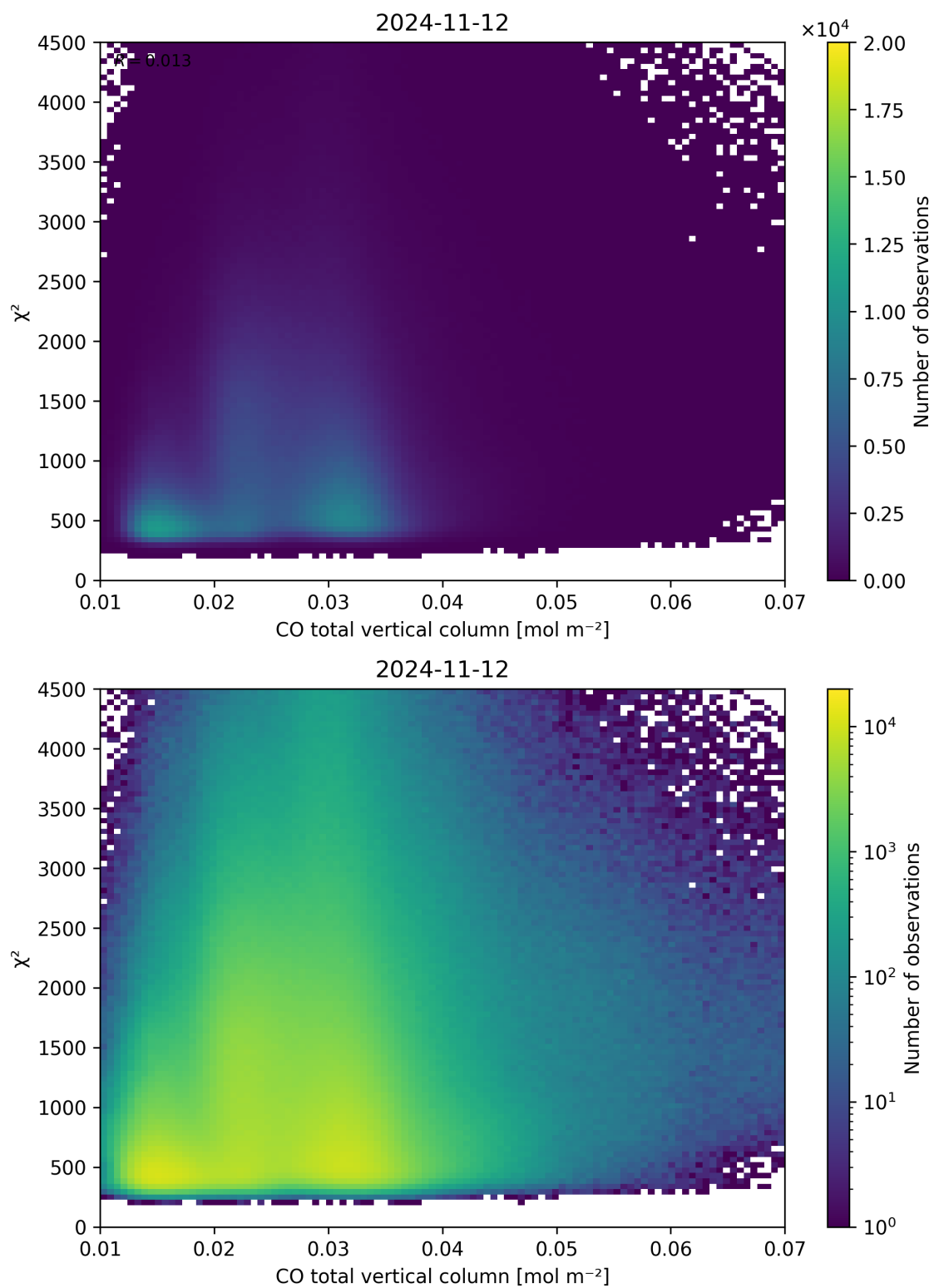
Figure 35: Scatter density plot of “CO total vertical column” against “ \chi^2 ” for 2024-11-11 to 2024-11-13.
