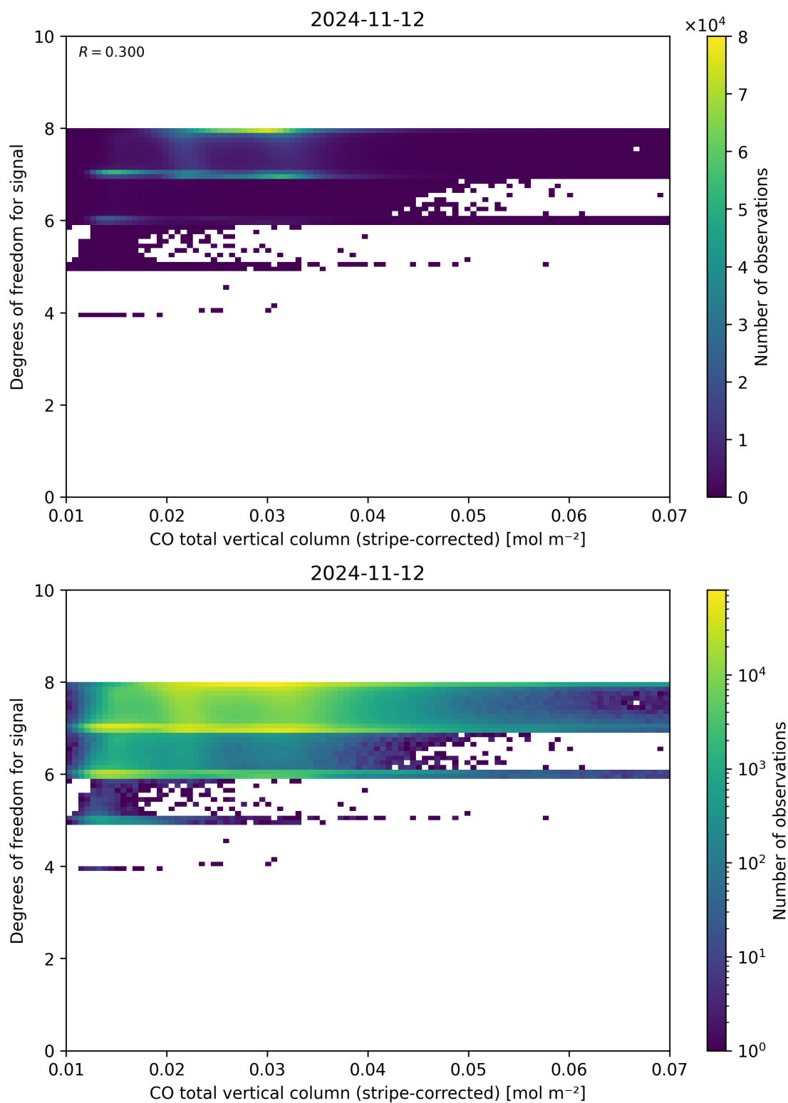
Figure 38: Scatter density plot of “CO total vertical column (stripe-corrected)” against “Degrees of freedom for signal” for 2024-11-11 to 2024-11-13.
