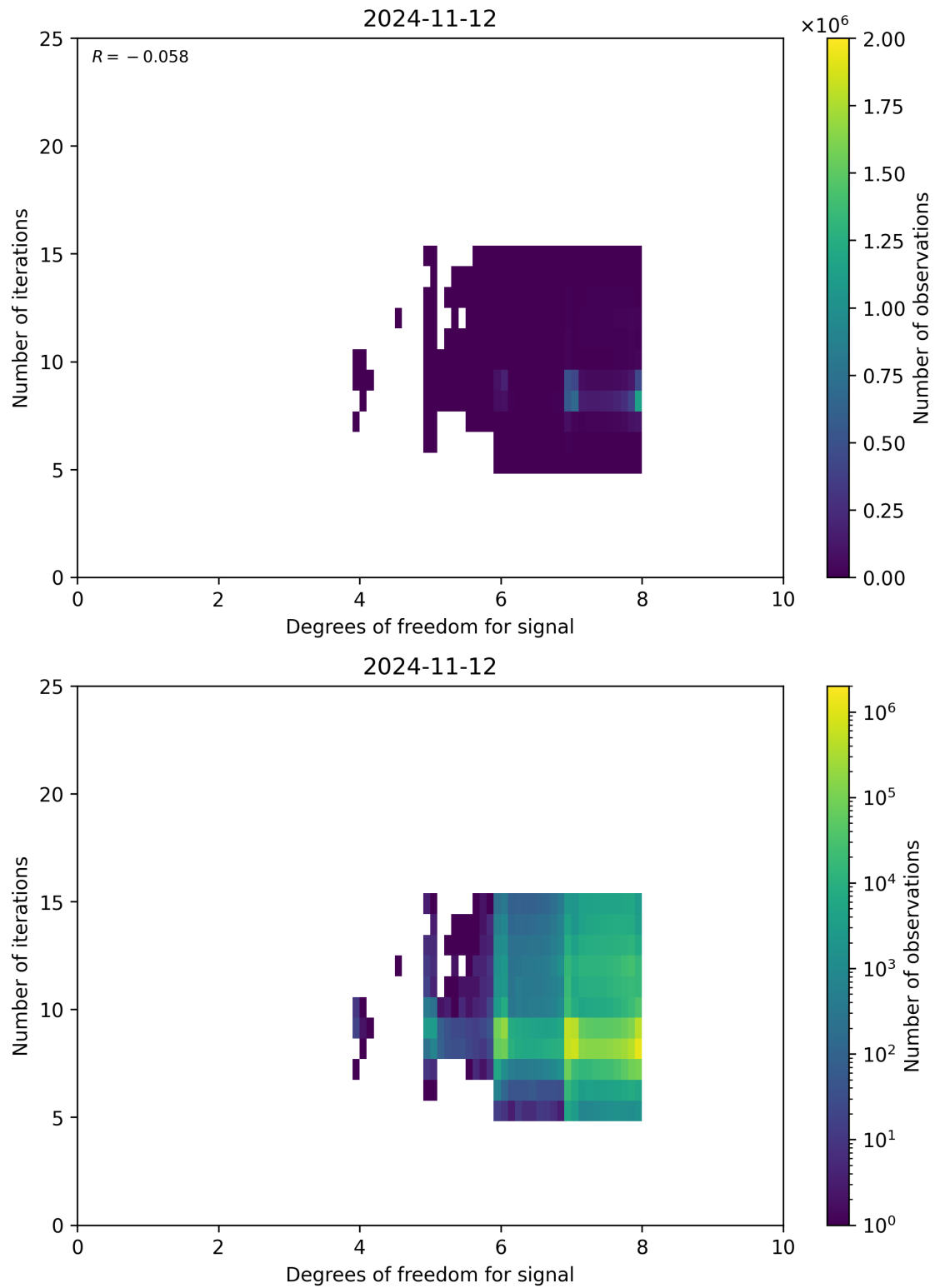
Figure 50: Scatter density plot of “Degrees of freedom for signal” against “Number of iterations” for 2024-11-11 to 2024-11-13.
