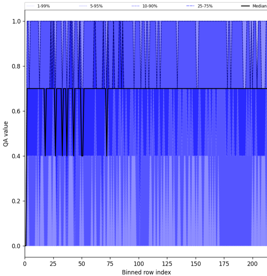
Figure 25: Along track statistics of “QA value” for 2024-11-11 to 2024-11-13
