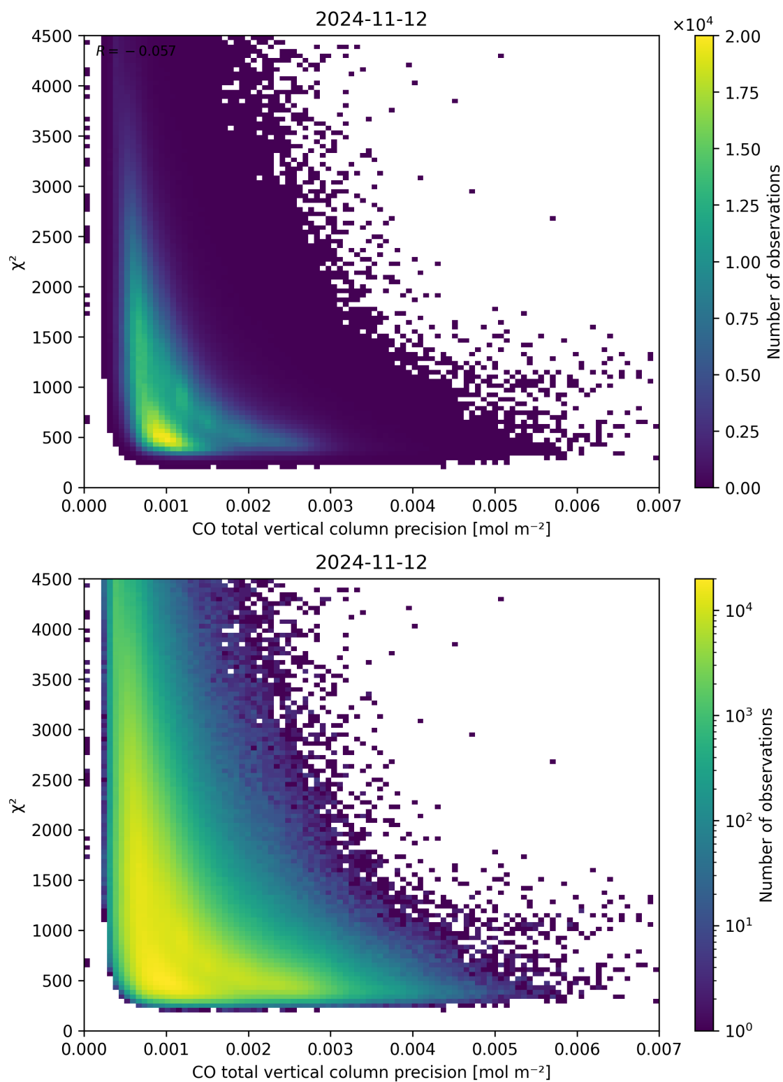
Figure 44: Scatter density plot of “CO total vertical column precision” against “ \chi^2 ” for 2024-11-11 to 2024-11-13.
