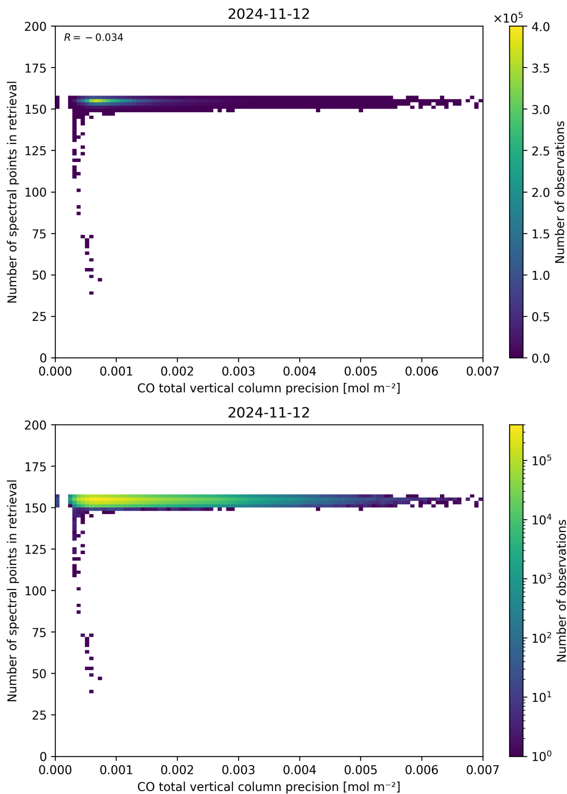
Figure 47: Scatter density plot of “CO total vertical column precision” against “Number of spectral points in retrieval” for 2024-11-11 to 2024-11-13.
