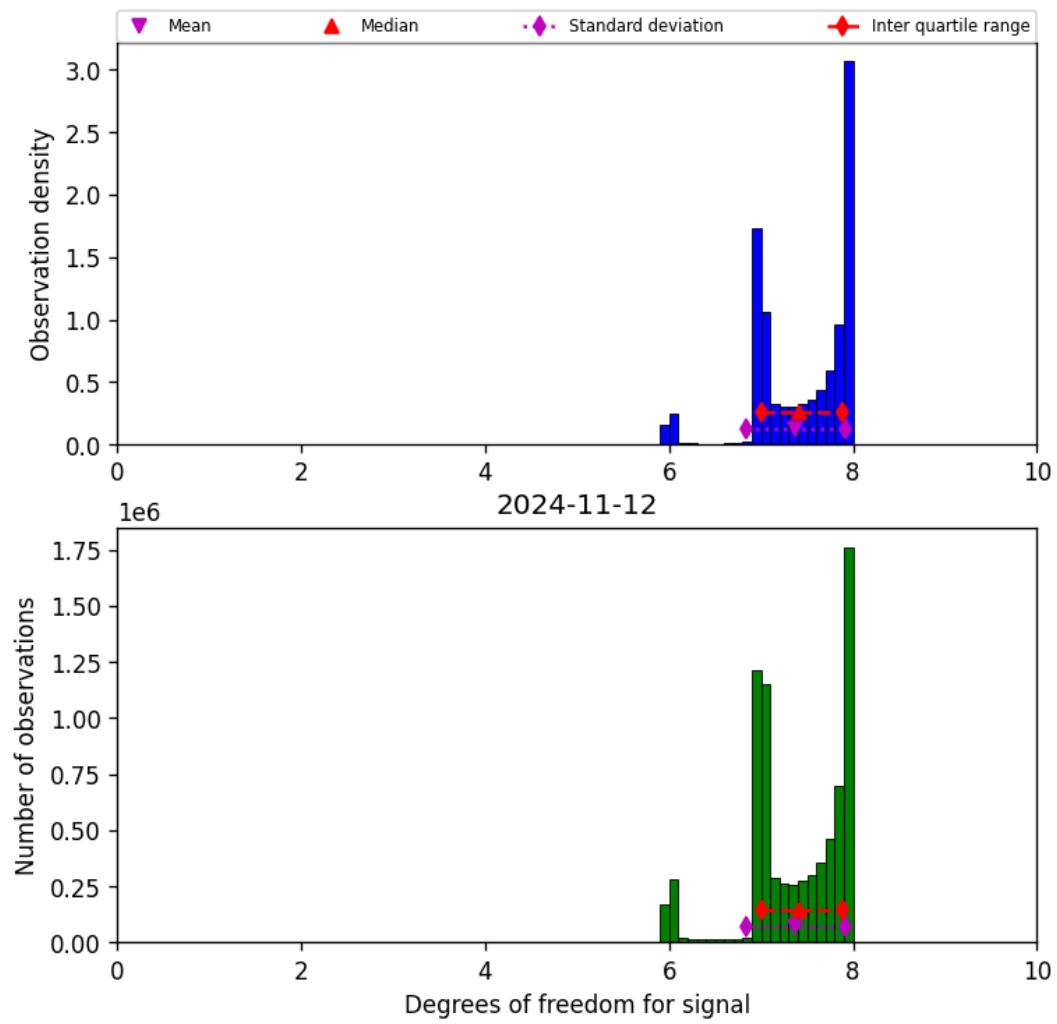
Figure 23: Histogram of “Degrees of freedom for signal” for 2024-11-11 to 2024-11-13
