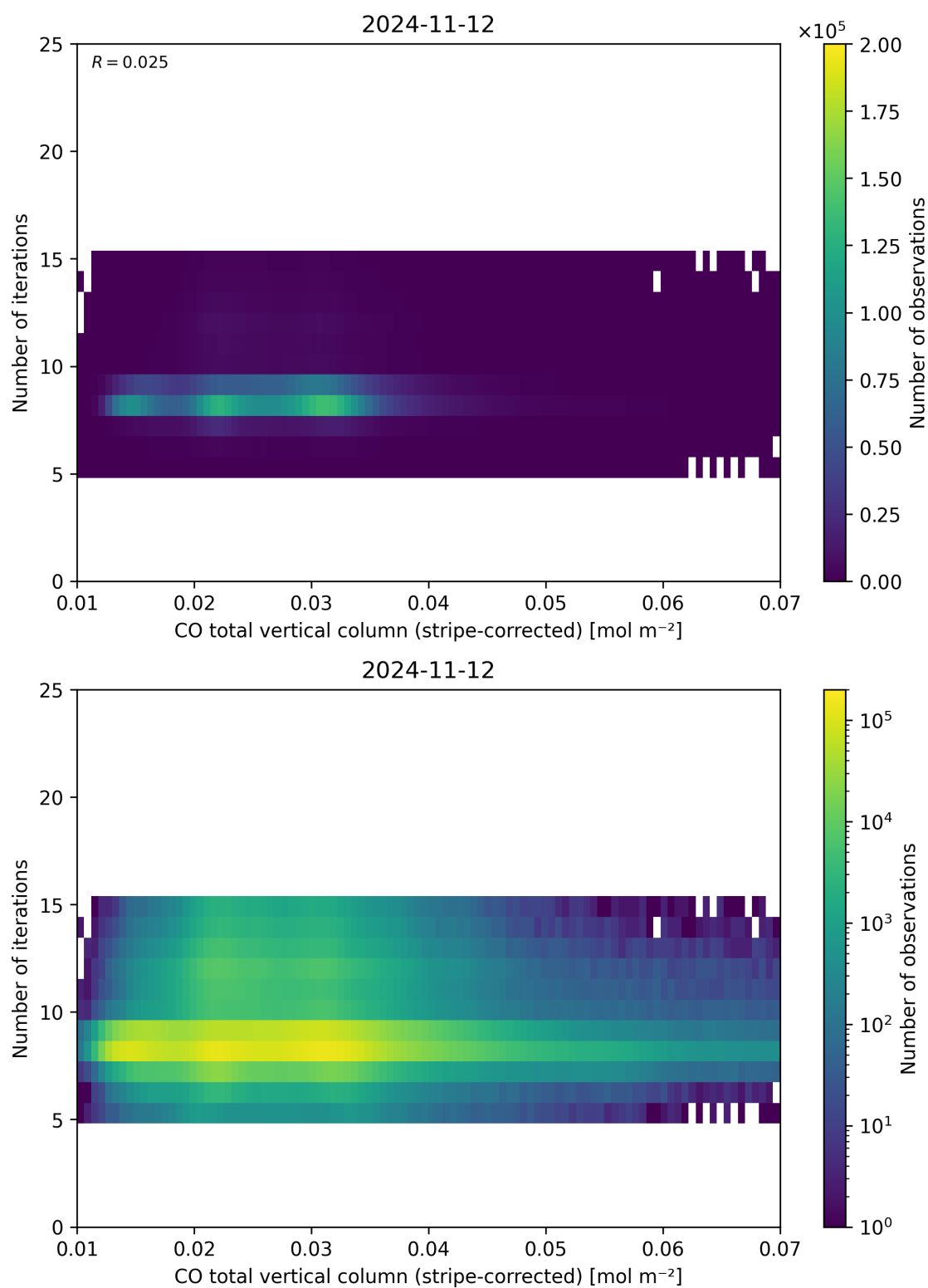
Figure 39: Scatter density plot of “CO total vertical column (stripe-corrected)” against “Number of iterations” for 2024-11-11 to 2024-11-13.
