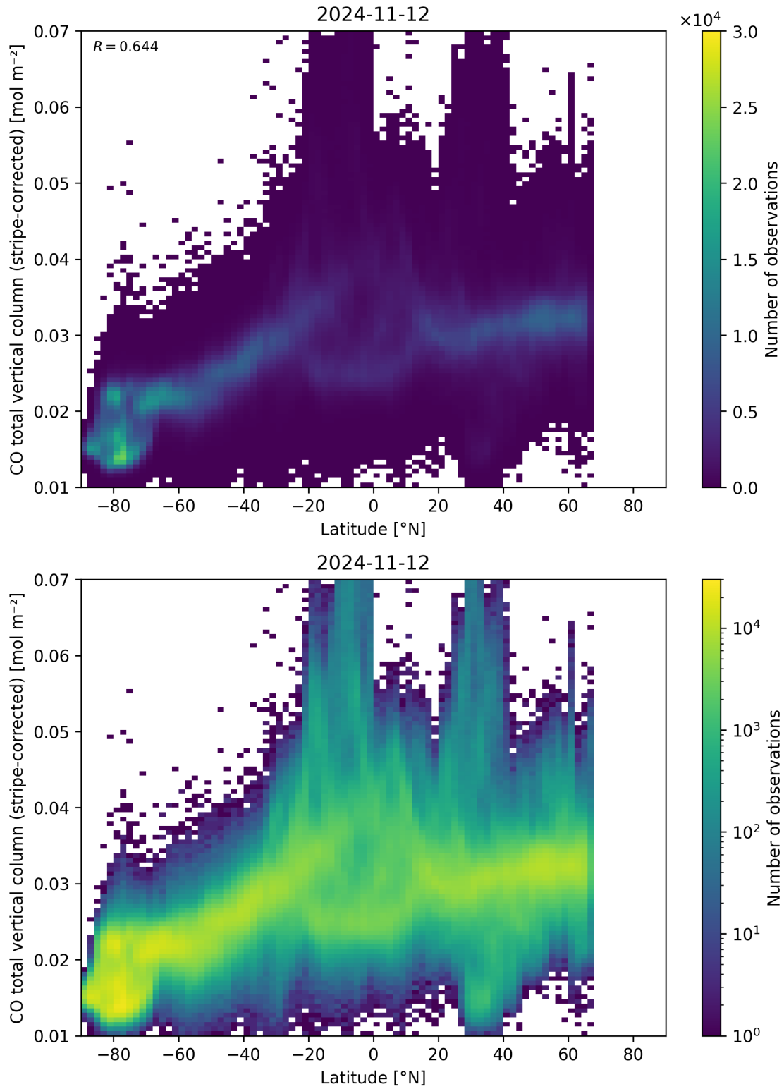
Figure 52: Scatter density plot of “Latitude” against “CO total vertical column (stripe-corrected)” for 2024-11-11 to 2024-11-13.
