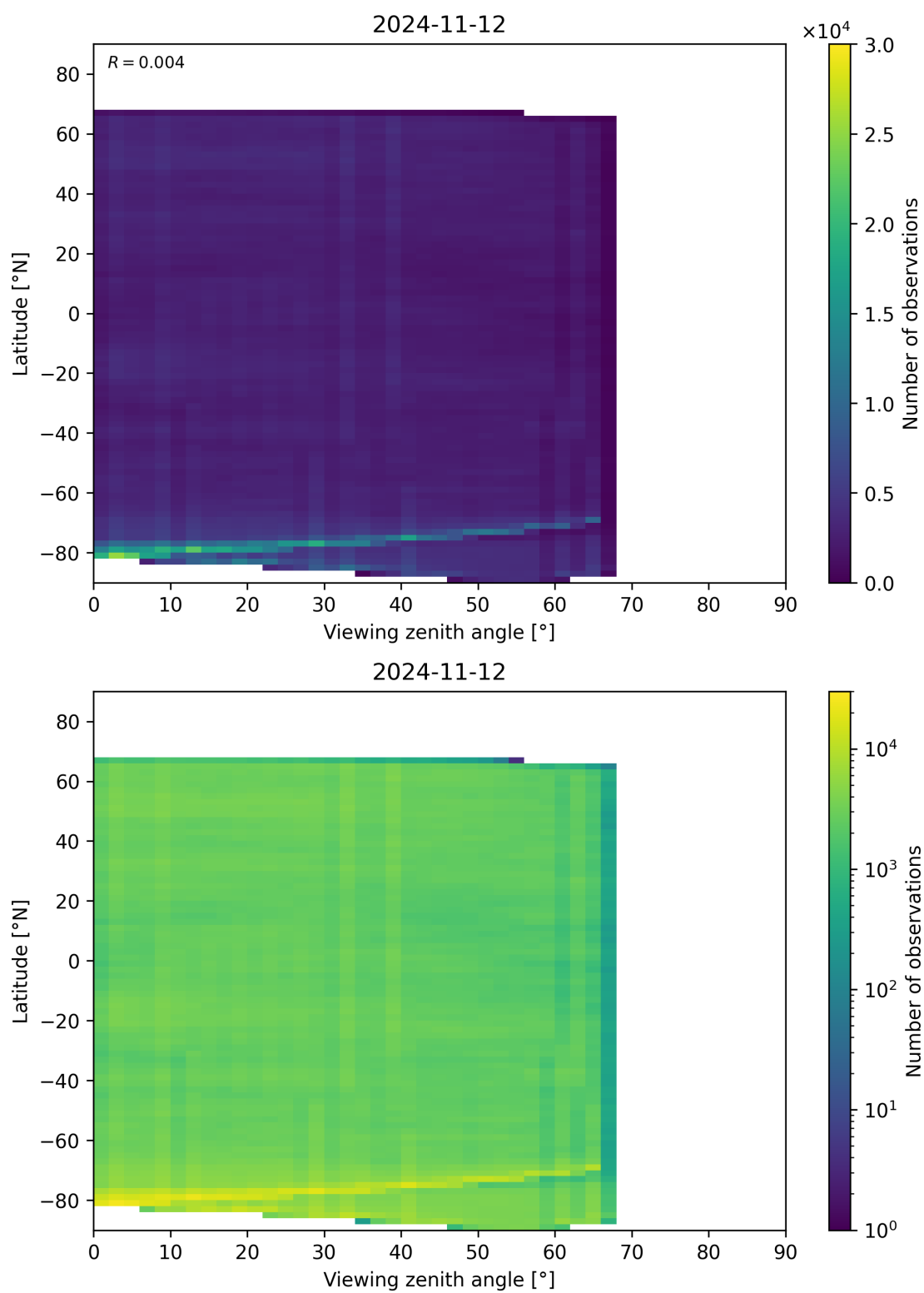
Figure 74: Scatter density plot of “Viewing zenith angle” against “Latitude” for 2024-11-11 to 2024-11-13.
