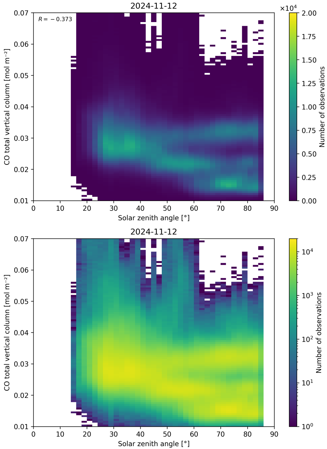
Figure 61: Scatter density plot of “Solar zenith angle” against “CO total vertical column” for 2024-11-11 to 2024-11-13.
