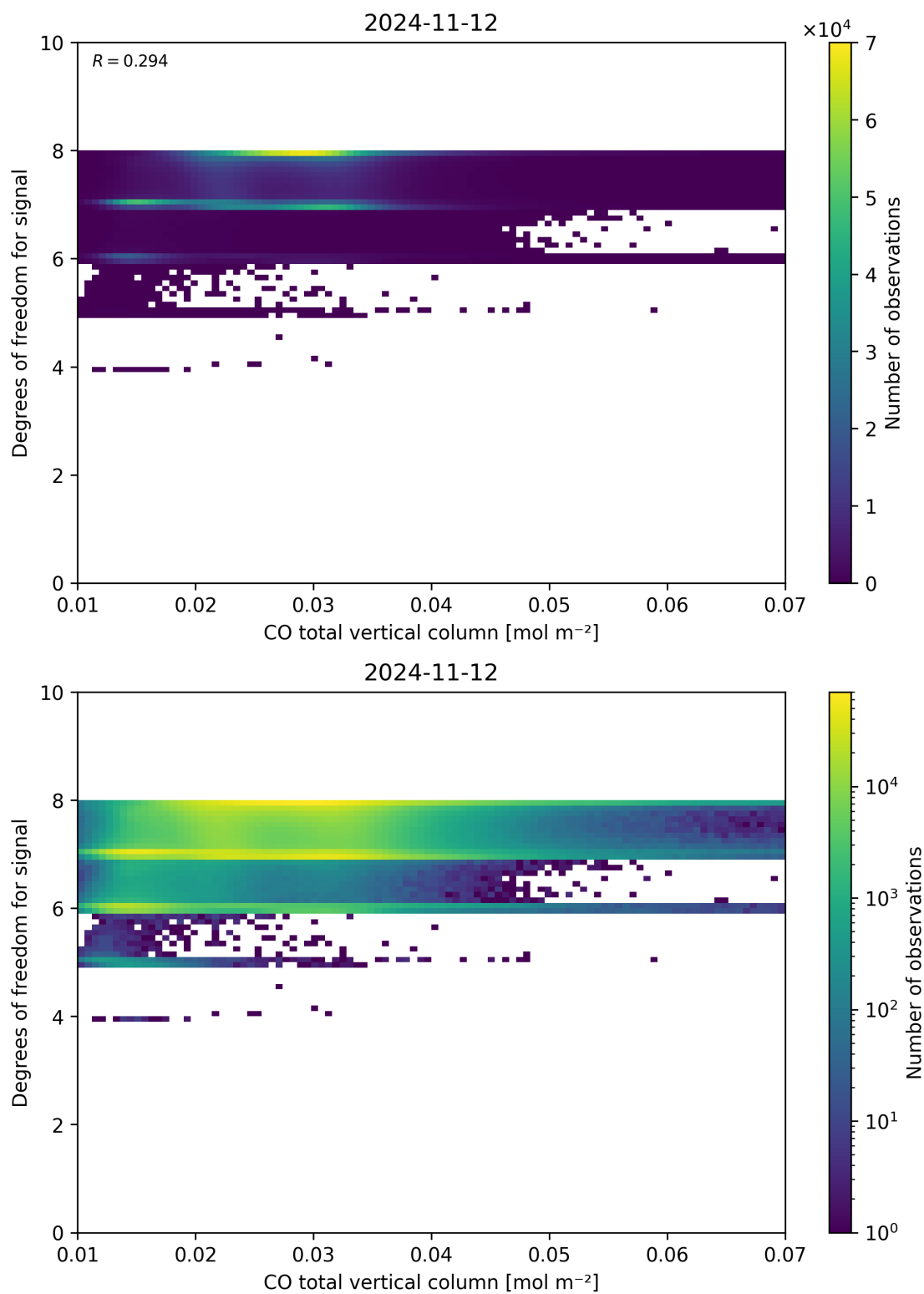
Figure 41: Scatter density plot of “CO total vertical column” against “Degrees of freedom for signal” for 2024-11-11 to 2024-11-13.
