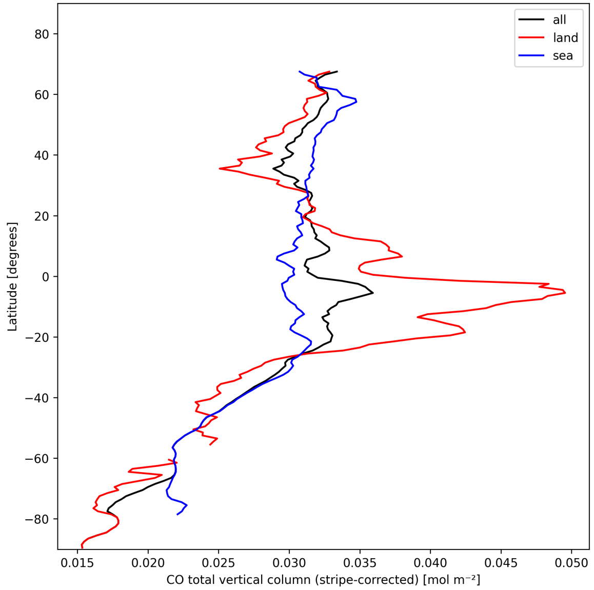
Figure 11: Zonal average of “CO total vertical column (stripe-corrected)” for 2024-11-11 to 2024-11-13.
