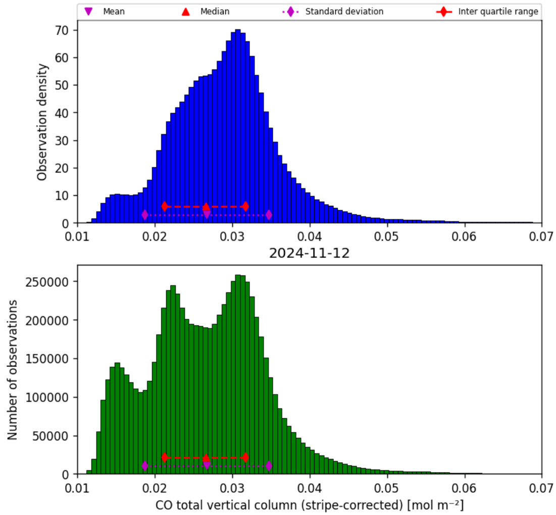
Figure 19: Histogram of “CO total vertical column (stripe-corrected)” for 2024-11-11 to 2024-11-13
