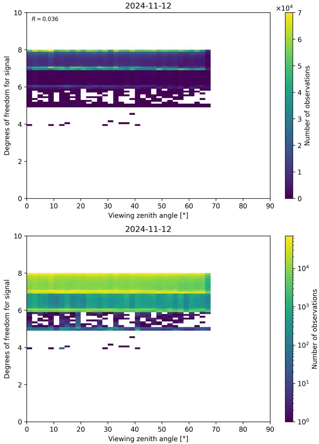
Figure 73: Scatter density plot of “Viewing zenith angle” against “Degrees of freedom for signal” for 2024-11-11 to 2024-11-13.
