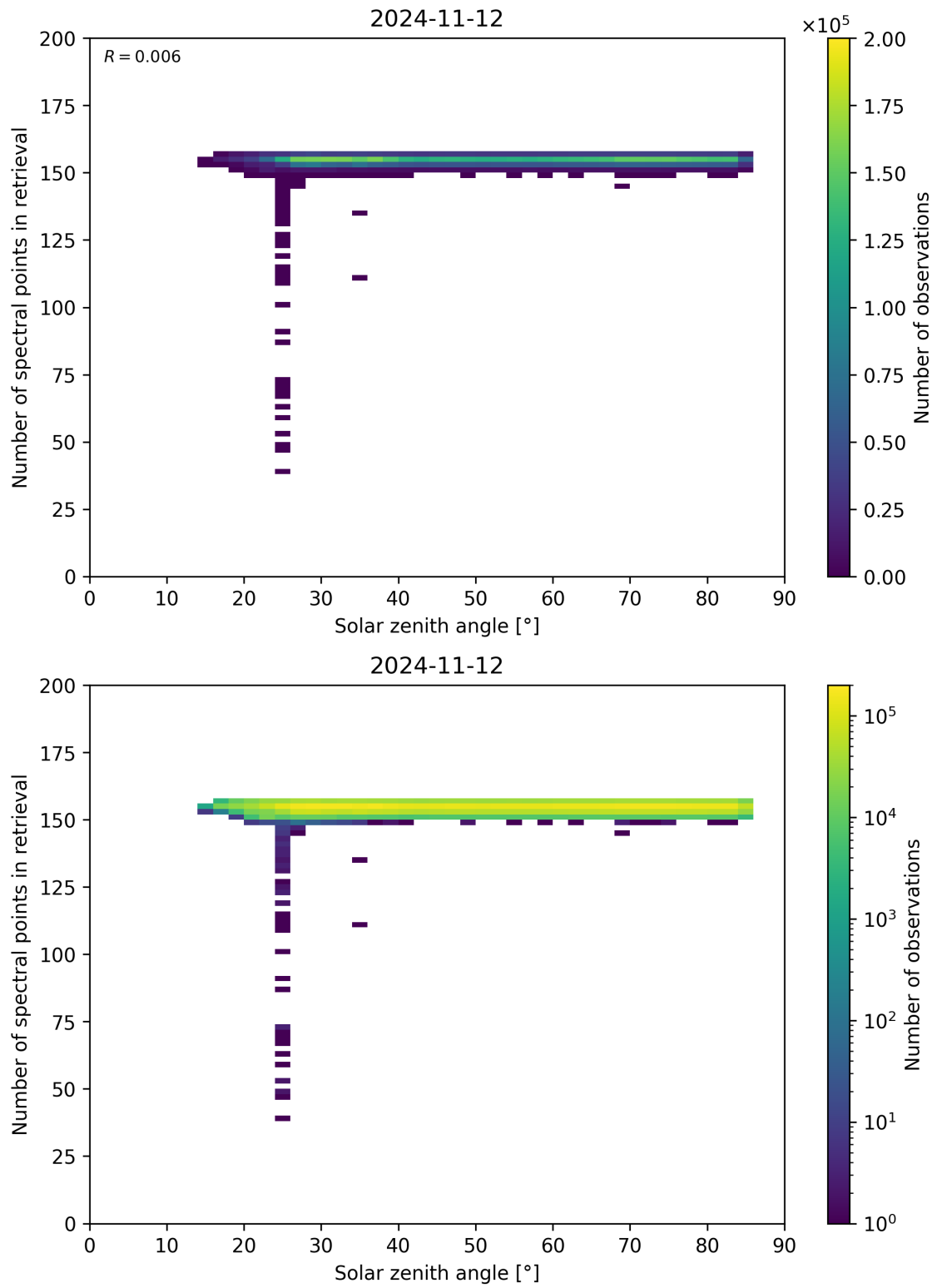
Figure 68: Scatter density plot of “Solar zenith angle” against “Number of spectral points in retrieval” for 2024-11-11 to 2024-11-13.
