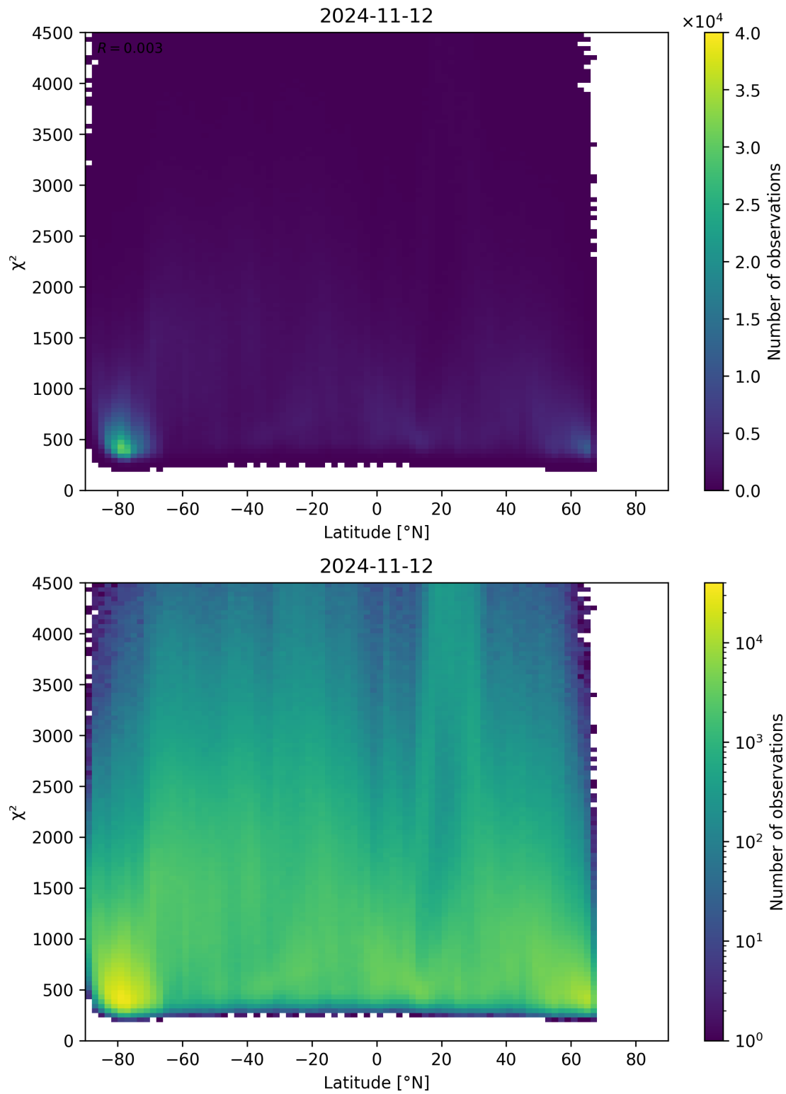
Figure 54: Scatter density plot of “Latitude” against “ \chi^2 ” for 2024-11-11 to 2024-11-13.
