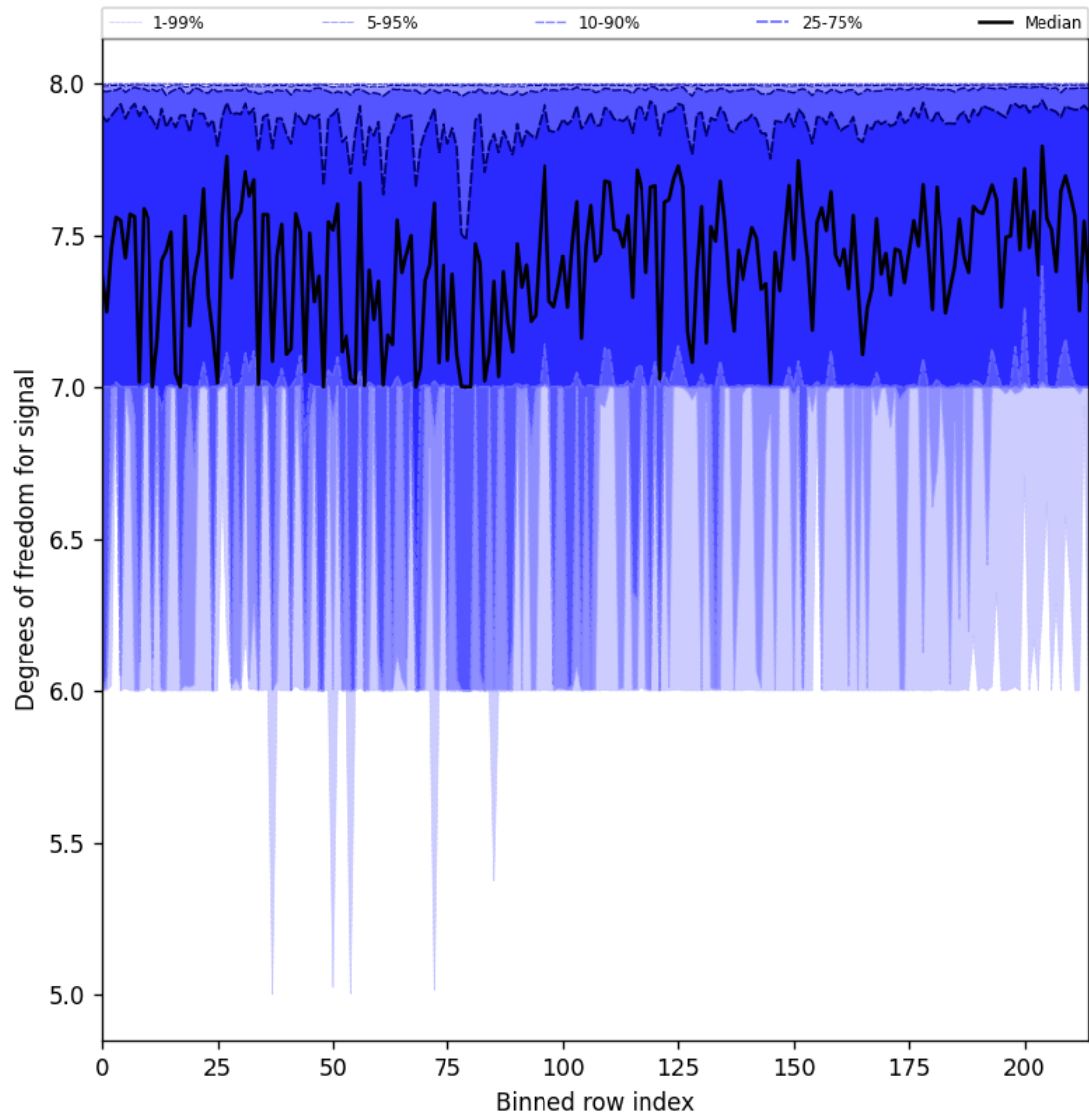
Figure 31: Along track statistics of “Degrees of freedom for signal” for 2024-11-11 to 2024-11-13
