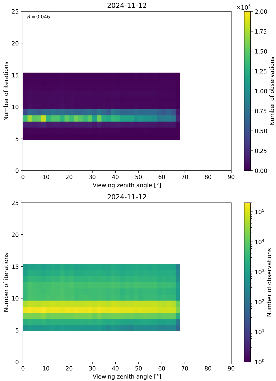
Figure 75: Scatter density plot of “Viewing zenith angle” against “Number of iterations” for 2024-11-11 to 2024-11-13.
