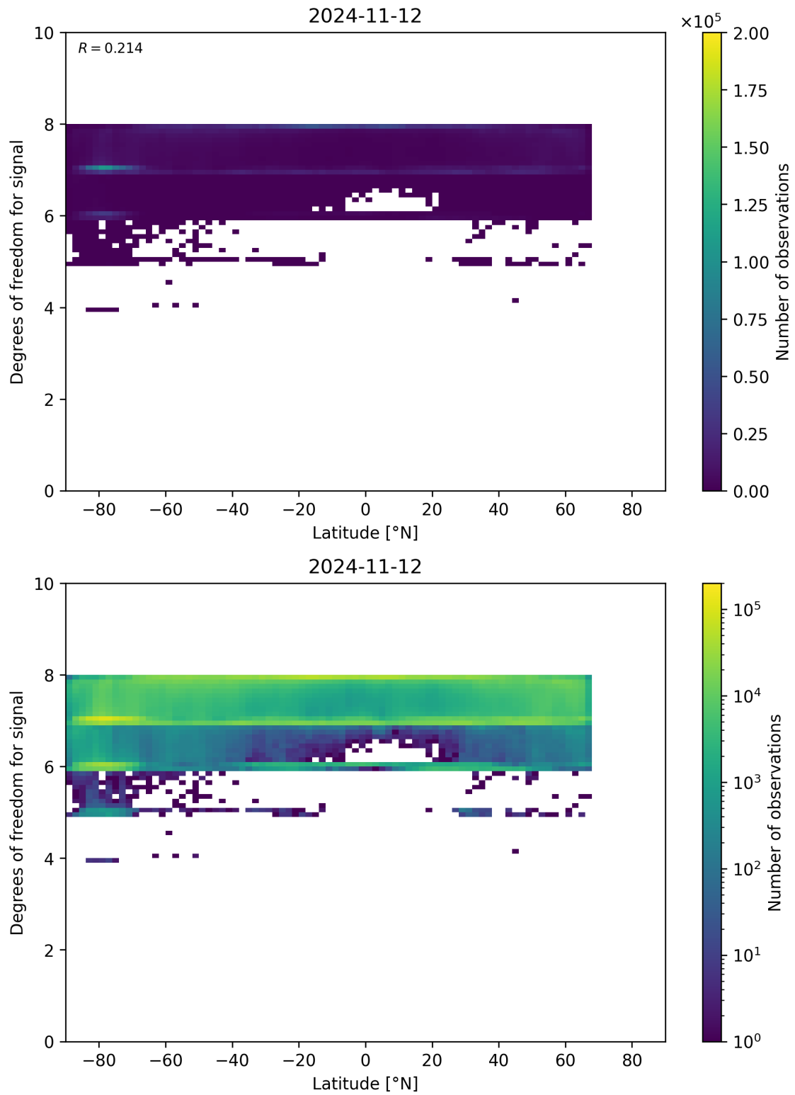
Figure 55: Scatter density plot of “Latitude” against “Degrees of freedom for signal” for 2024-11-11 to 2024-11-13.
