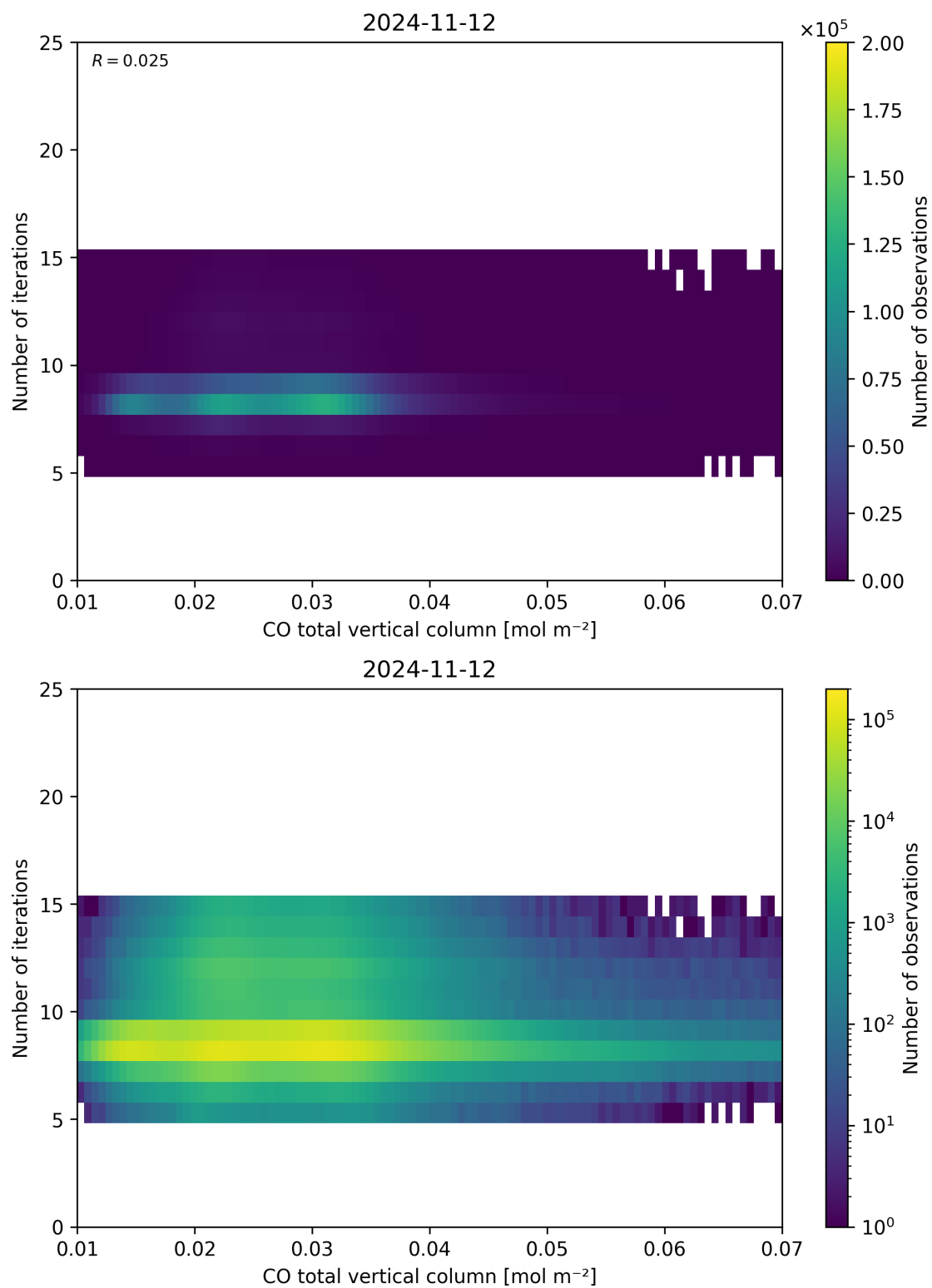
Figure 42: Scatter density plot of “CO total vertical column” against “Number of iterations” for 2024-11-11 to 2024-11-13.
