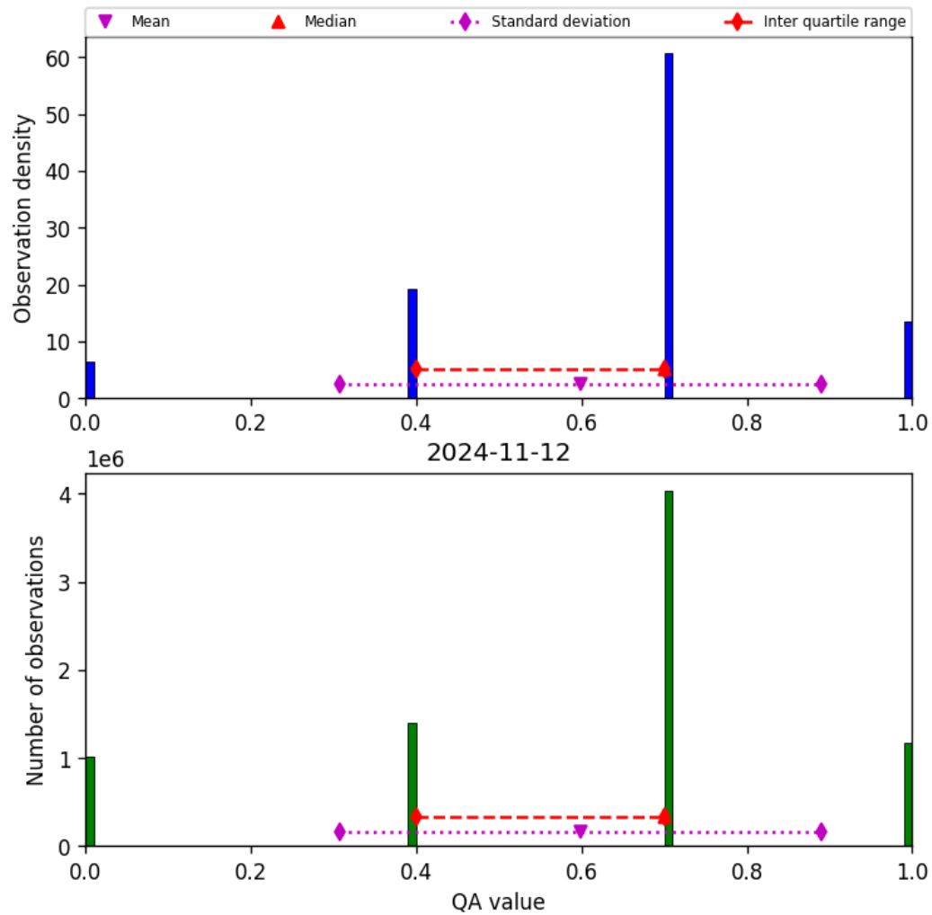
Figure 17: Histogram of “QA value” for 2024-11-11 to 2024-11-13
