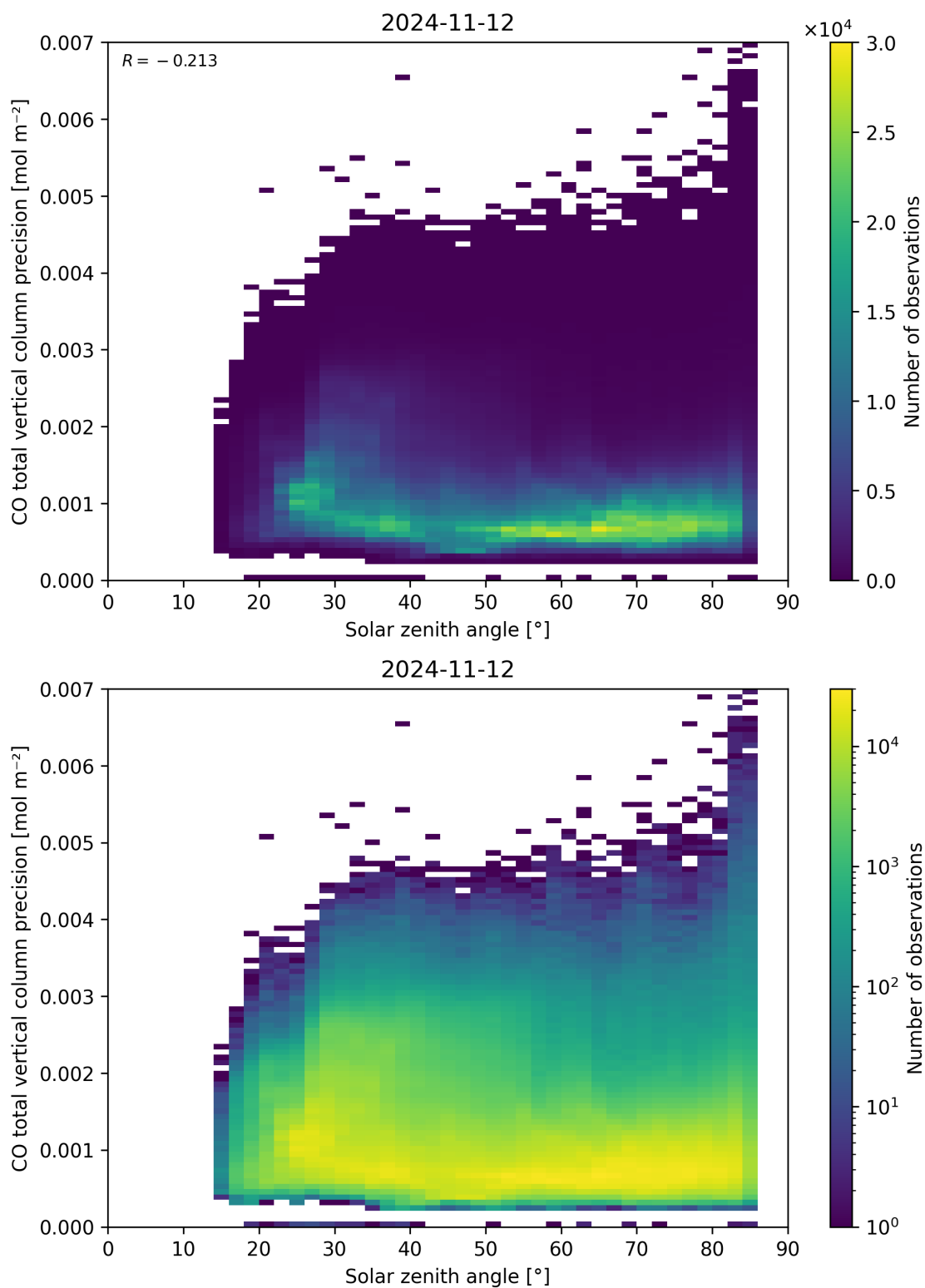
Figure 63: Scatter density plot of “Solar zenith angle” against “CO total vertical column precision” for 2024-11-11 to 2024-11-13.
