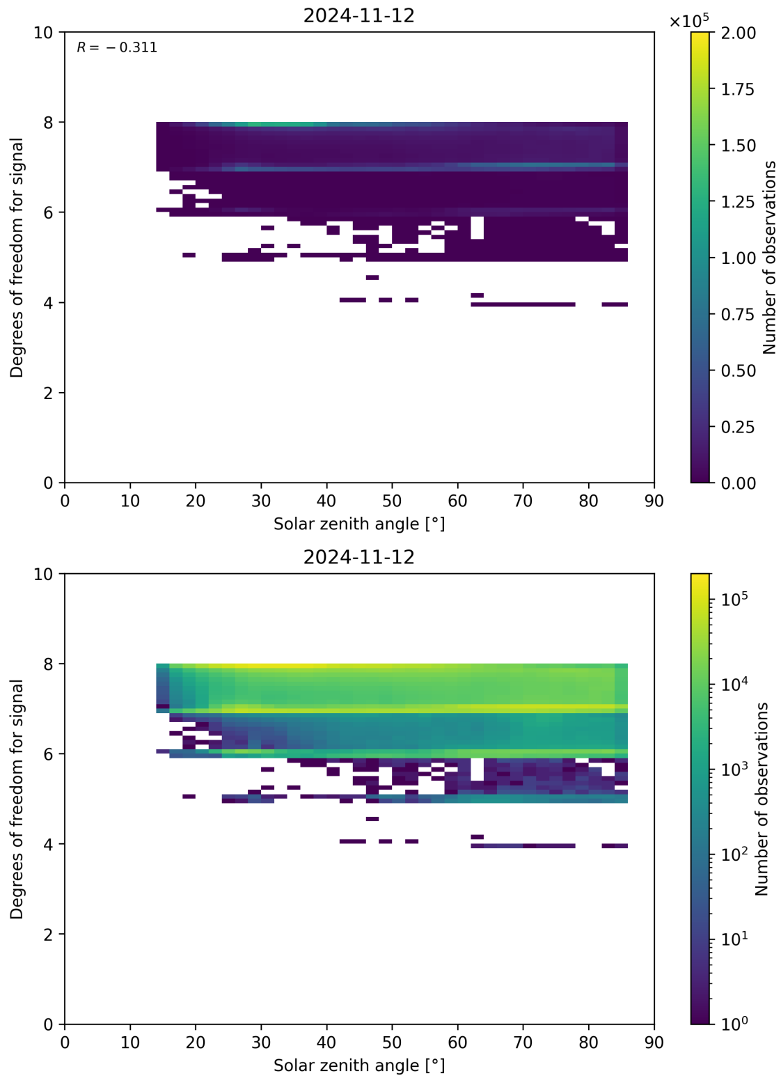
Figure 65: Scatter density plot of “Solar zenith angle” against “Degrees of freedom for signal” for 2024-11-11 to 2024-11-13.
