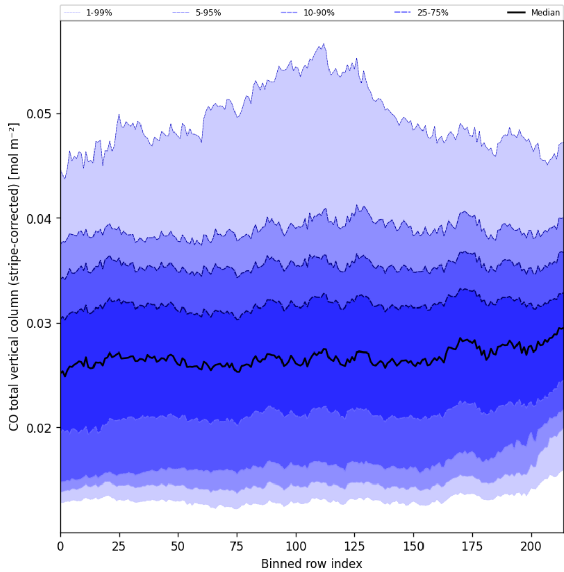
Figure 27: Along track statistics of “CO total vertical column (stripe-corrected)” for 2024-11-11 to 2024-11-13
