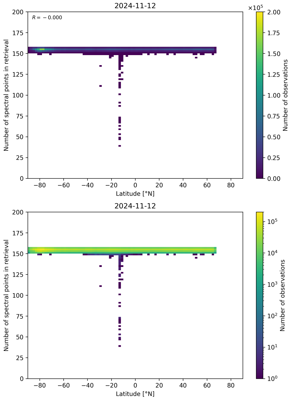
Figure 57: Scatter density plot of “Latitude” against “Number of spectral points in retrieval” for 2024-11-11 to 2024-11-13.
