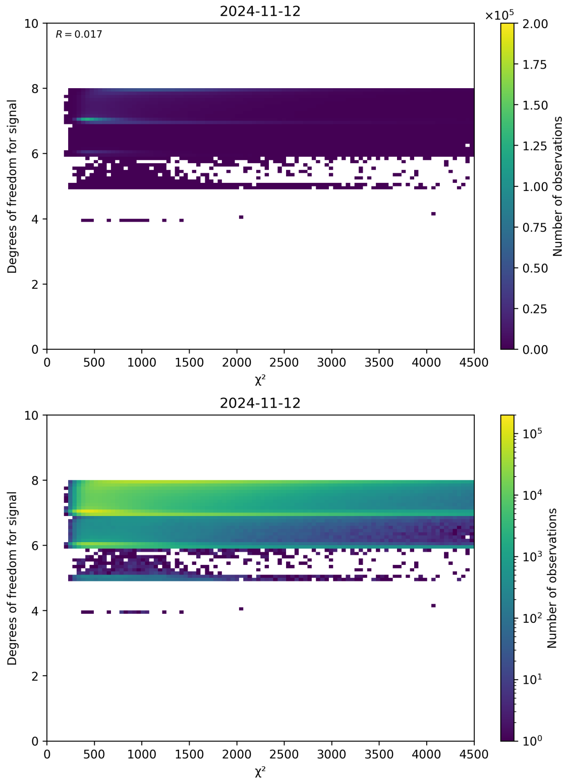
Figure 48: Scatter density plot of “ \chi^2 ” against “Degrees of freedom for signal” for 2024-11-11 to 2024-11-13.
