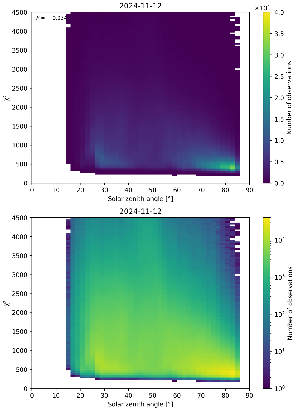
Figure 64: Scatter density plot of “Solar zenith angle” against “ \chi^2 ” for 2024-11-11 to 2024-11-13.
