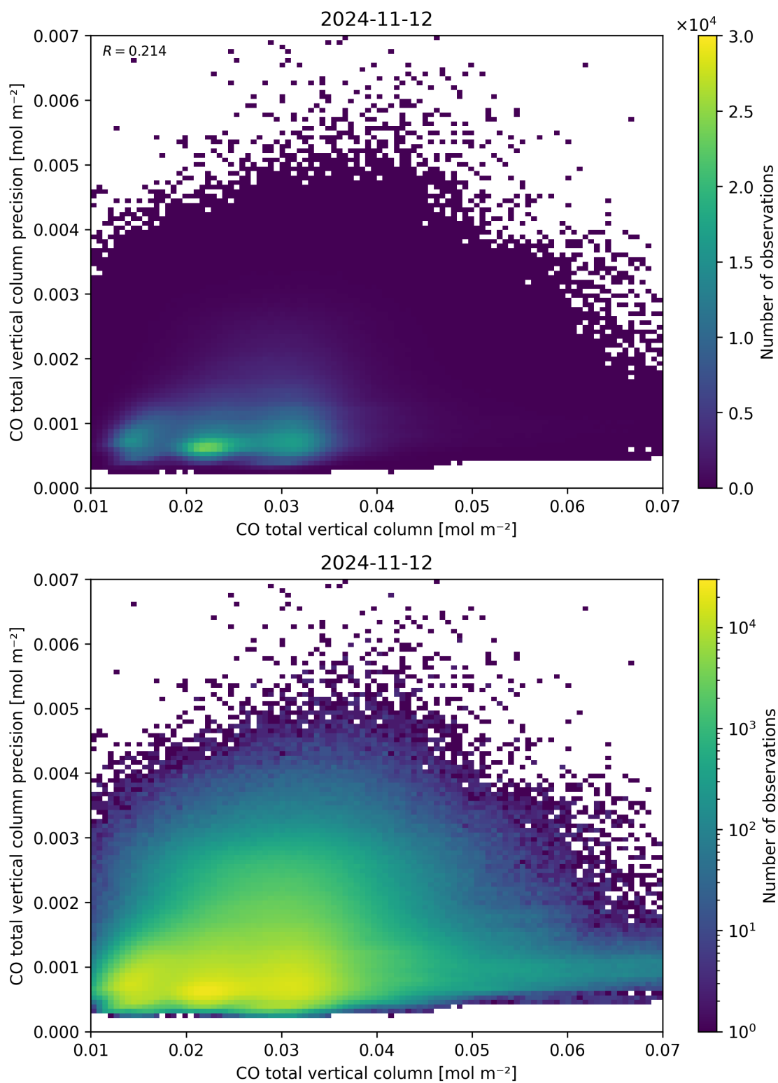
Figure 34: Scatter density plot of “CO total vertical column” against “CO total vertical column precision” for 2024-11-11 to 2024-11-13.
