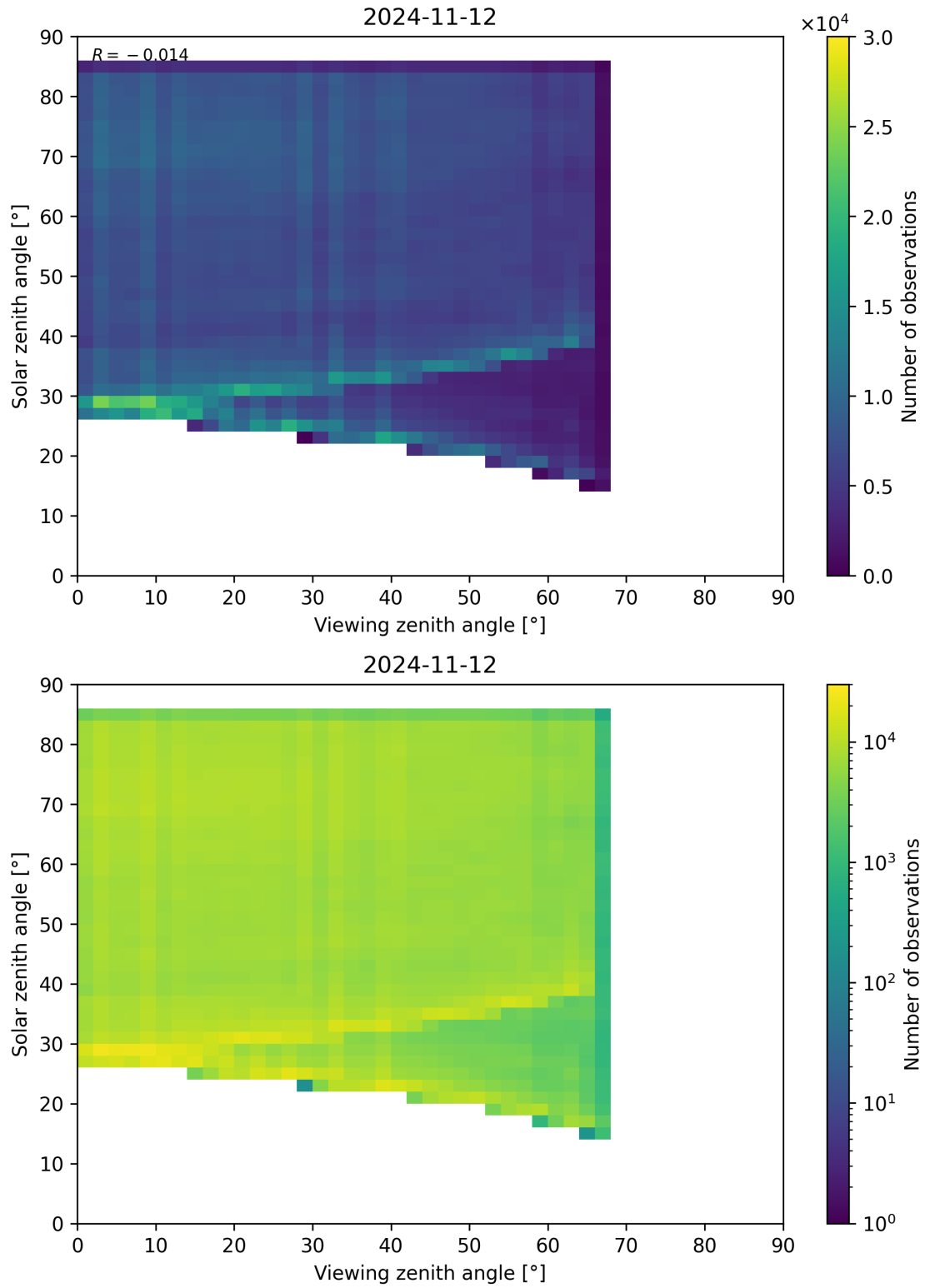
Figure 77: Scatter density plot of “Viewing zenith angle” against “Solar zenith angle” for 2024-11-11 to 2024-11-13.
