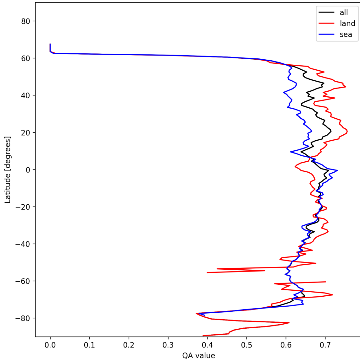
Figure 9: Zonal average of “QA value” for 2024-11-11 to 2024-11-13.
