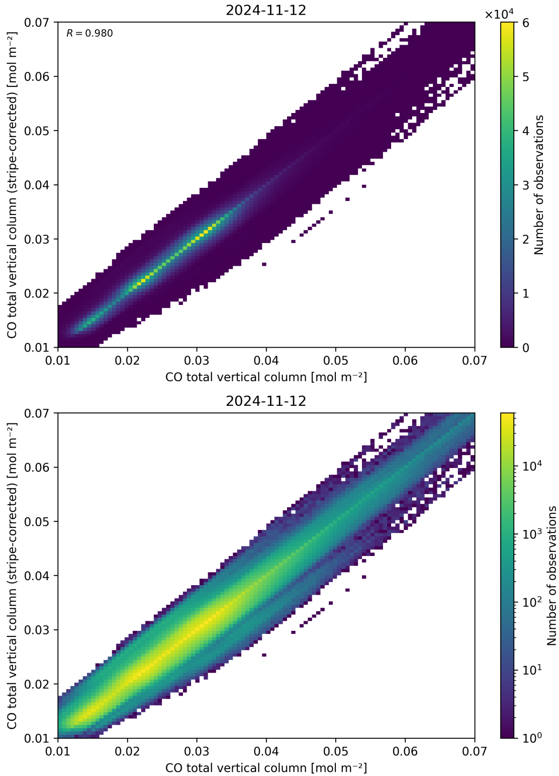
Figure 33: Scatter density plot of “CO total vertical column” against “CO total vertical column (stripe-corrected)” for 2024-11-11 to 2024-11-13.
