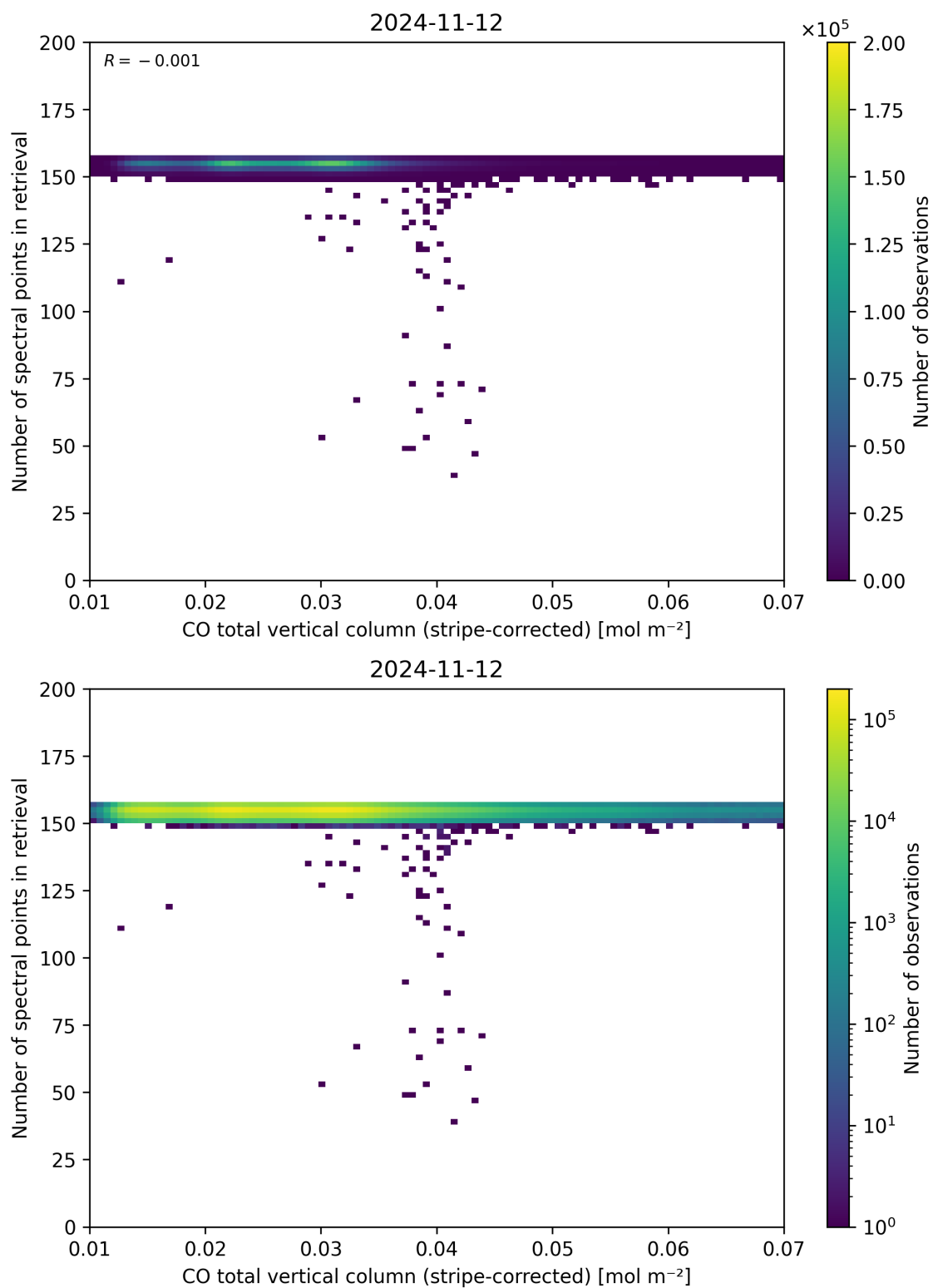
Figure 40: Scatter density plot of “CO total vertical column (stripe-corrected)” against “Number of spectral points in retrieval” for 2024-11-11 to 2024-11-13.
