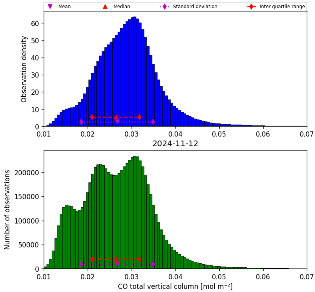
Figure 18: Histogram of “CO total vertical column” for 2024-11-11 to 2024-11-13
