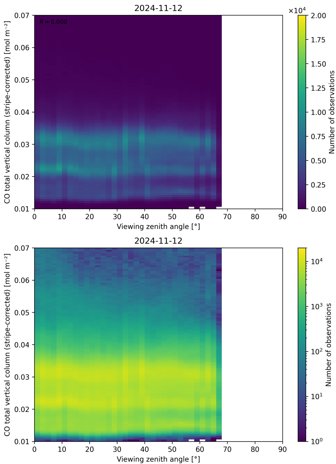
Figure 70: Scatter density plot of “Viewing zenith angle” against “CO total vertical column (stripe-corrected)” for 2024-11-11 to 2024-11-13.
