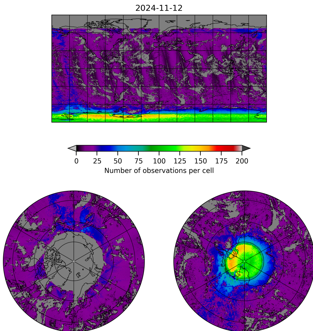
Figure 8: Map of the number of observations for 2024-11-11 to 2024-11-13
