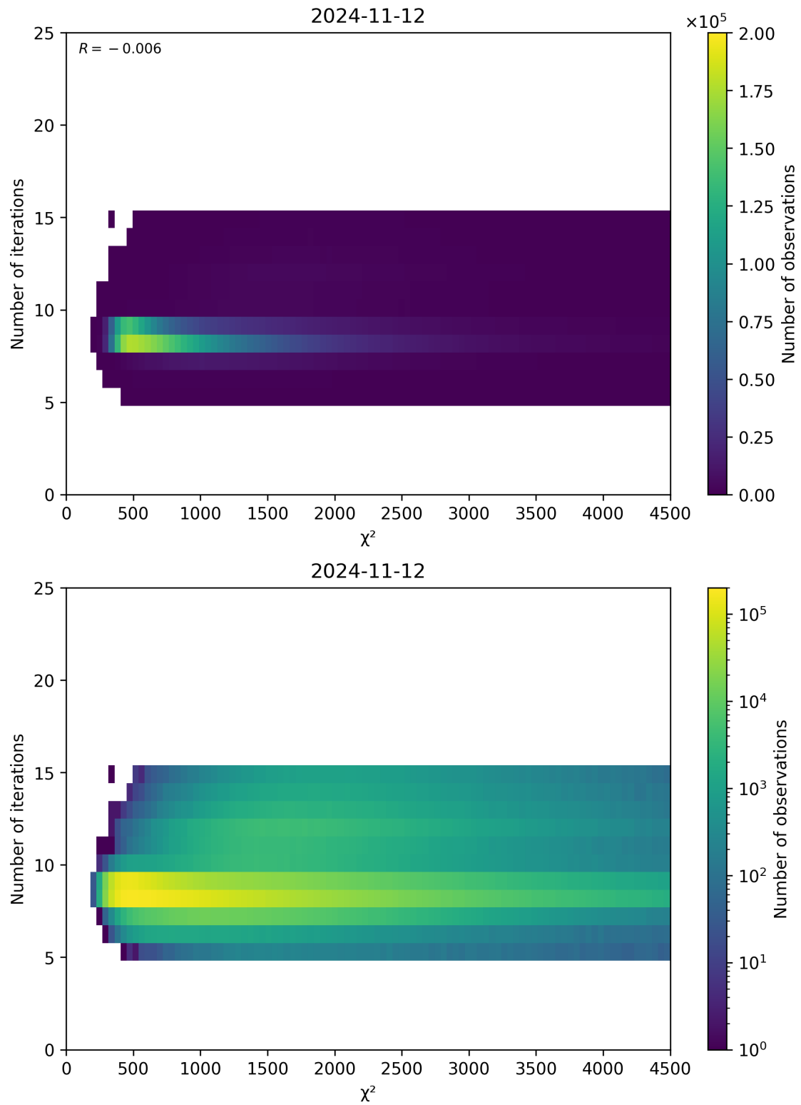
Figure 49: Scatter density plot of “ \chi^2 ” against “Number of iterations” for 2024-11-11 to 2024-11-13.
