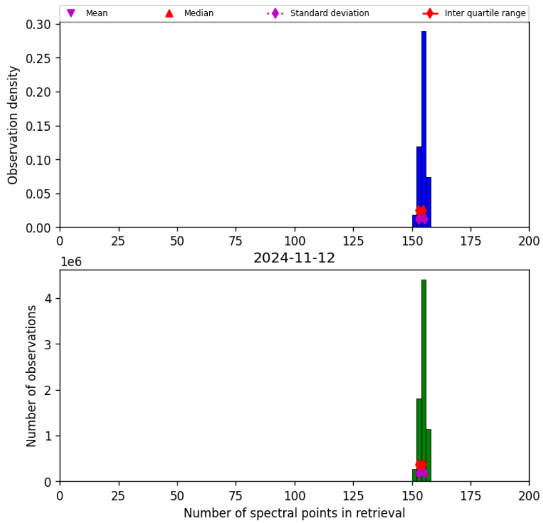
Figure 21: Histogram of “Number of spectral points in retrieval” for 2024-11-11 to 2024-11-13
