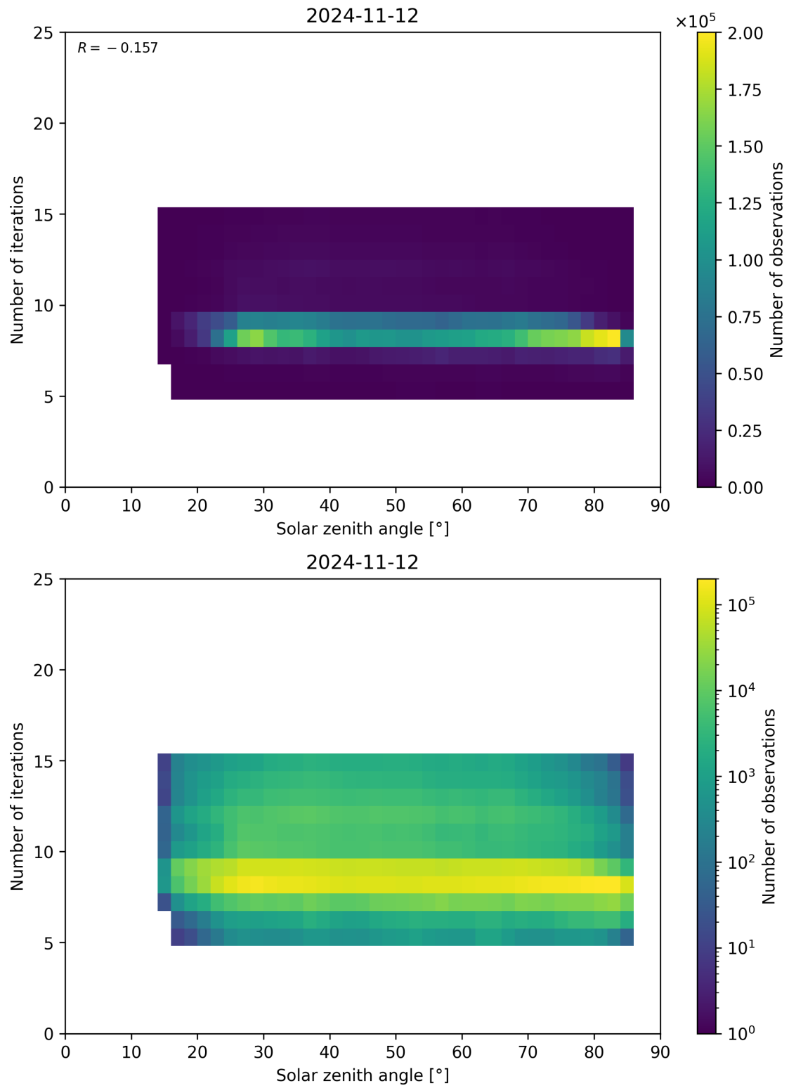
Figure 67: Scatter density plot of “Solar zenith angle” against “Number of iterations” for 2024-11-11 to 2024-11-13.
