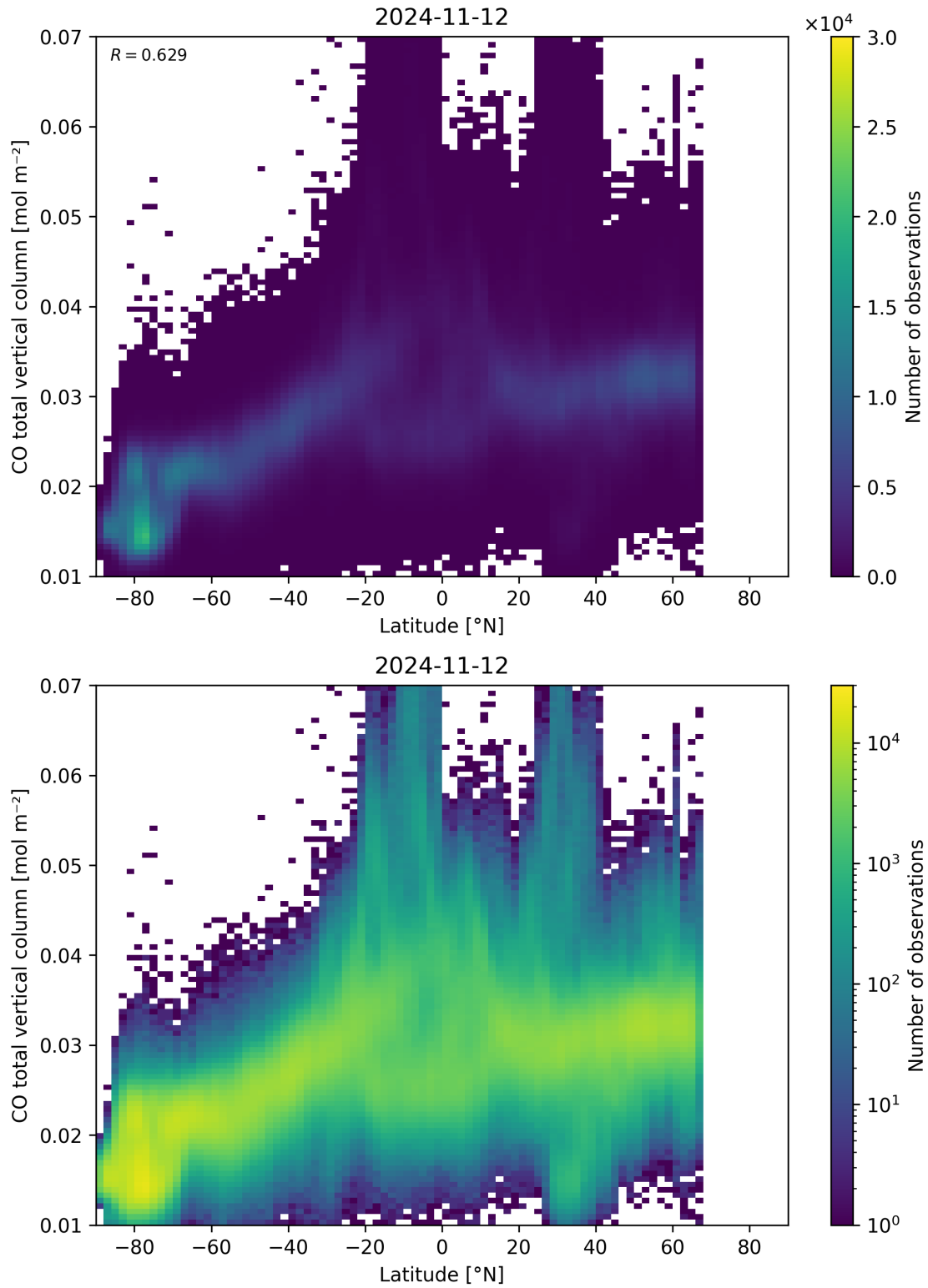
Figure 51: Scatter density plot of “Latitude” against “CO total vertical column” for 2024-11-11 to 2024-11-13.
