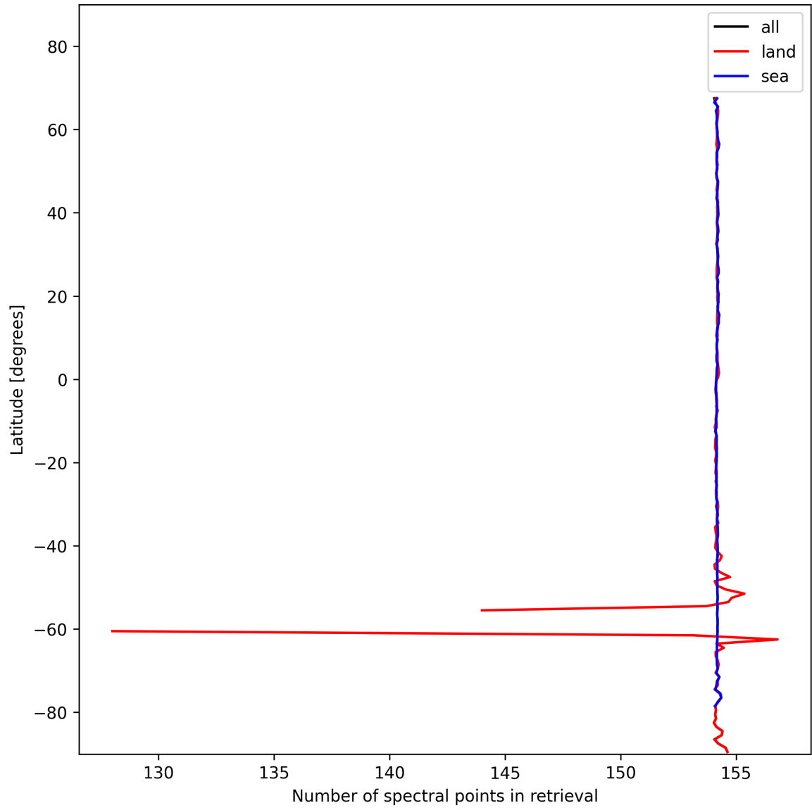
Figure 13: Zonal average of “Number of spectral points in retrieval” for 2024-11-11 to 2024-11-13.
