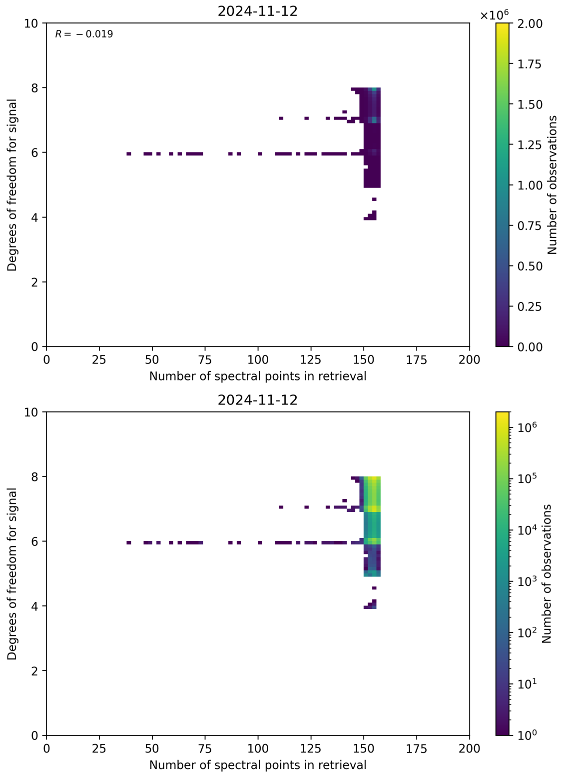
Figure 59: Scatter density plot of “Number of spectral points in retrieval” against “Degrees of freedom for signal” for 2024-11-11 to 2024-11-13.
