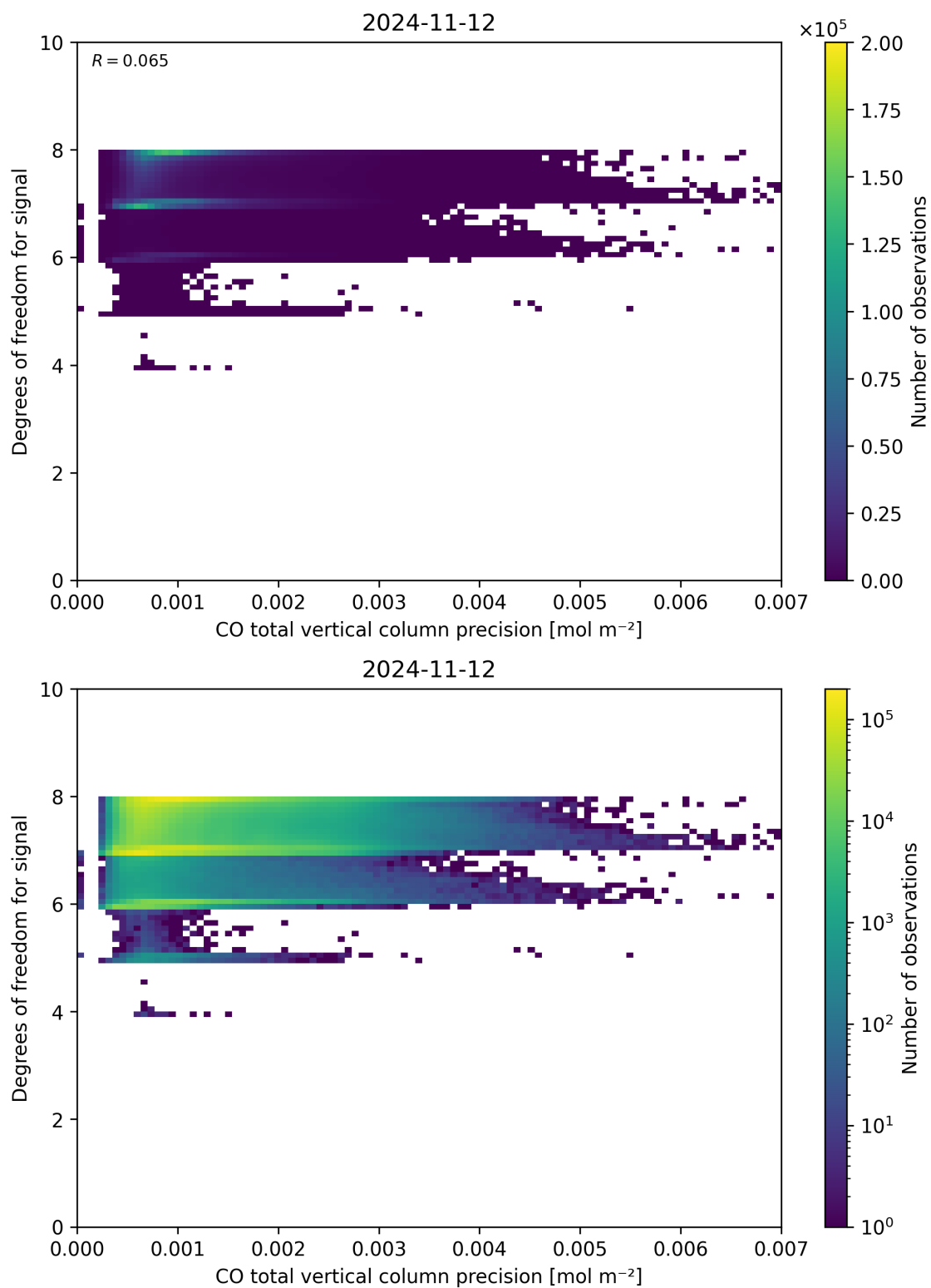
Figure 45: Scatter density plot of “CO total vertical column precision” against “Degrees of freedom for signal” for 2024-11-11 to 2024-11-13.
