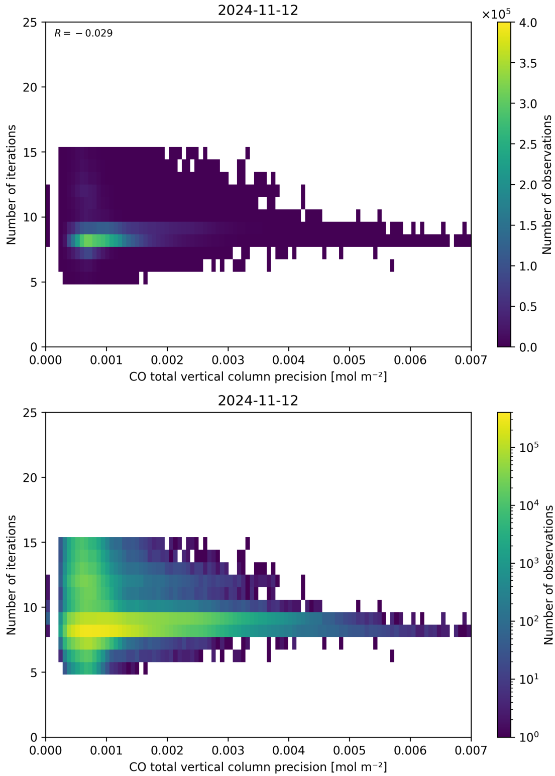
Figure 46: Scatter density plot of “CO total vertical column precision” against “Number of iterations” for 2024-11-11 to 2024-11-13.
