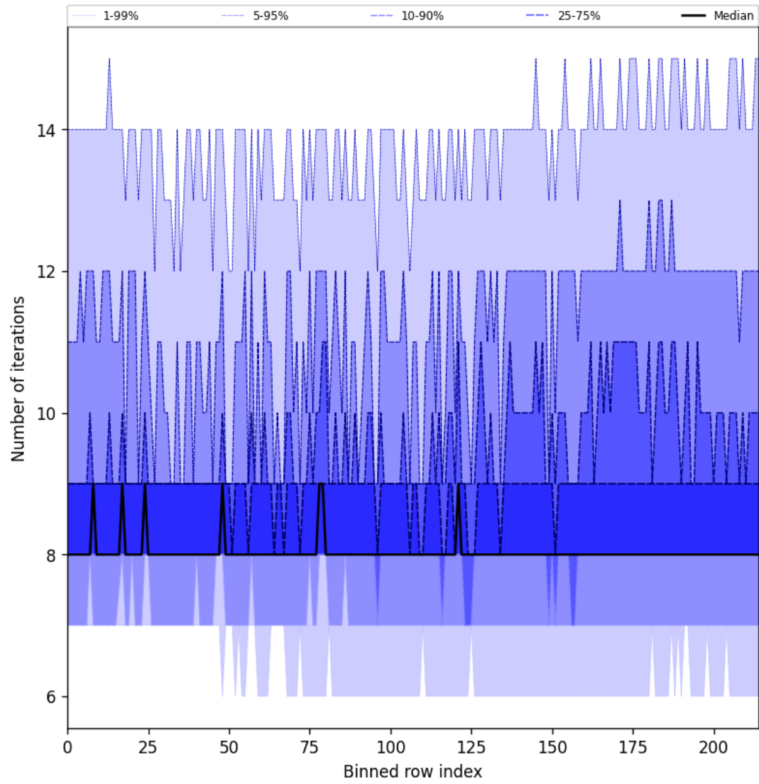
Figure 32: Along track statistics of “Number of iterations” for 2024-11-11 to 2024-11-13
