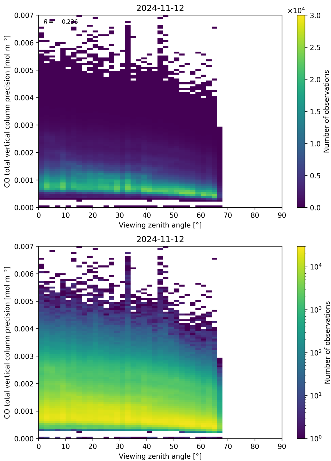
Figure 71: Scatter density plot of “Viewing zenith angle” against “CO total vertical column precision” for 2024-11-11 to 2024-11-13.
