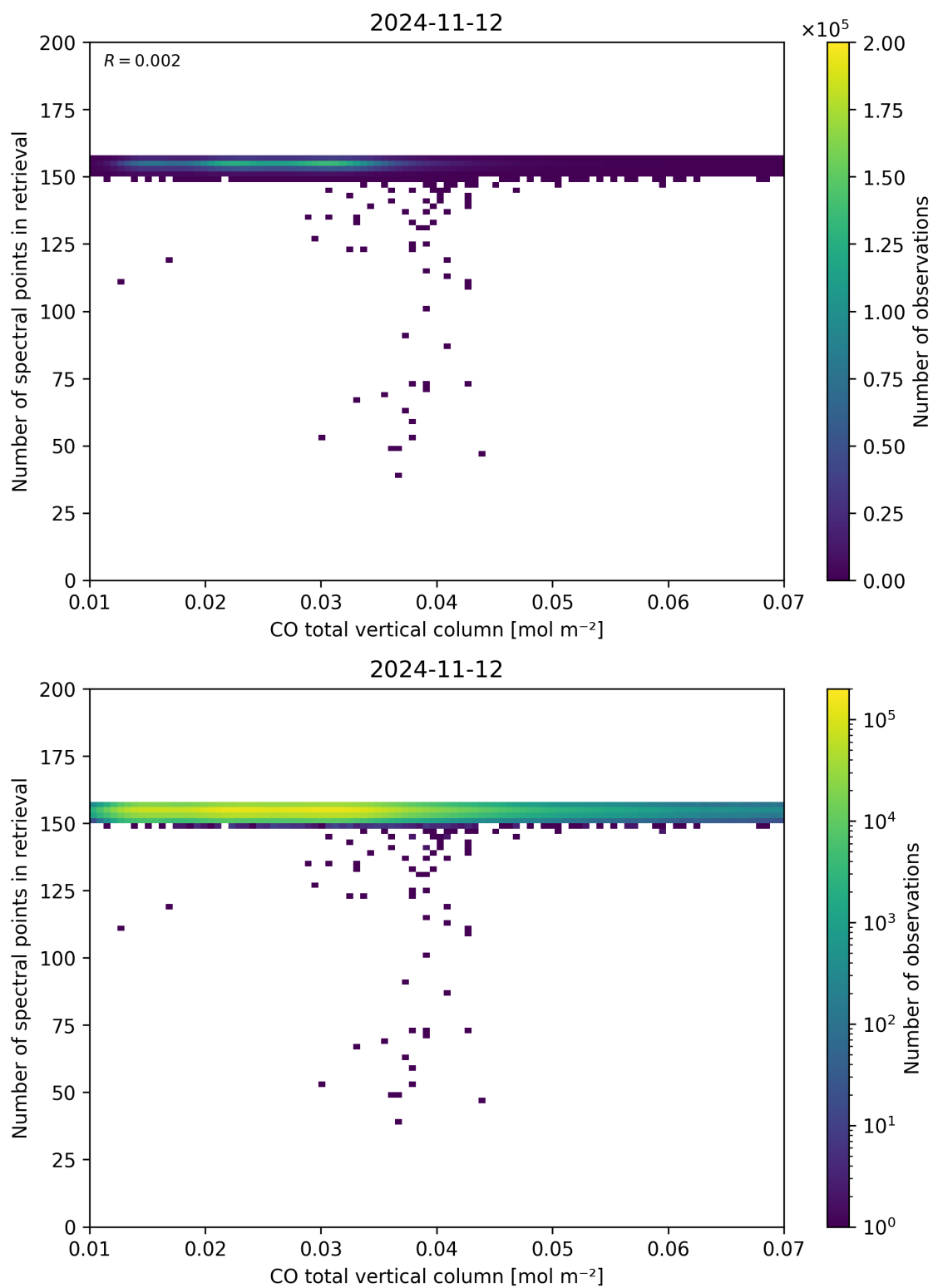
Figure 43: Scatter density plot of “CO total vertical column” against “Number of spectral points in retrieval” for 2024-11-11 to 2024-11-13.
