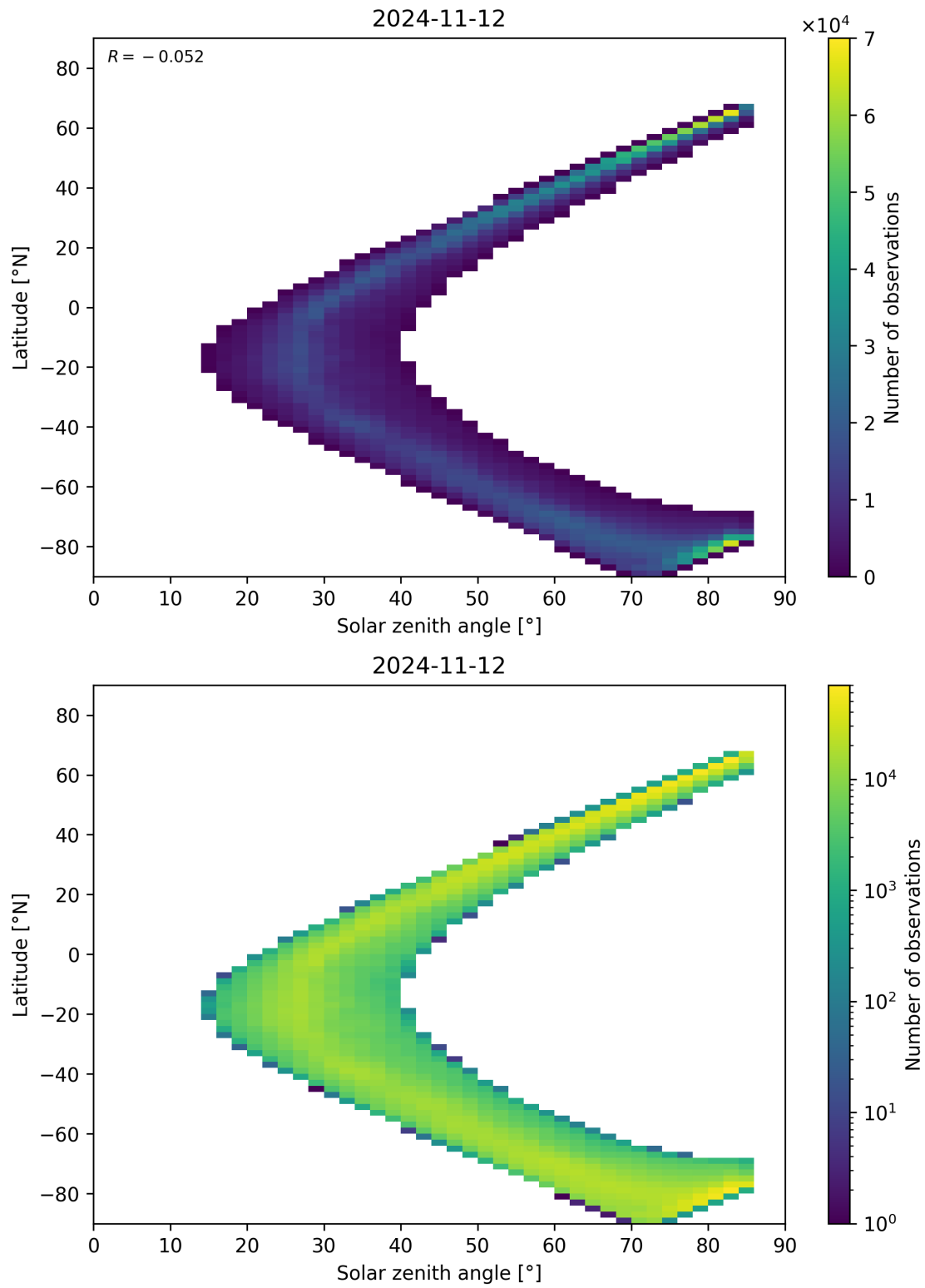
Figure 66: Scatter density plot of “Solar zenith angle” against “Latitude” for 2024-11-11 to 2024-11-13.
