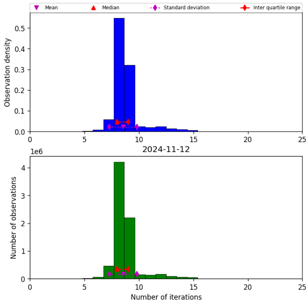
Figure 24: Histogram of “Number of iterations” for 2024-11-11 to 2024-11-13
