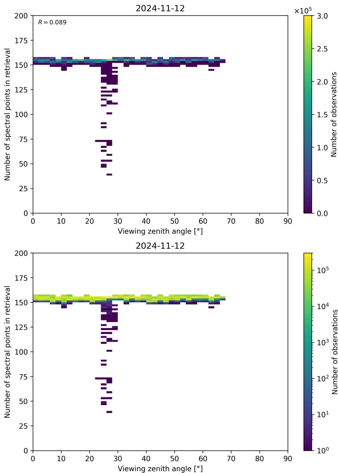
Figure 76: Scatter density plot of “Viewing zenith angle” against “Number of spectral points in retrieval” for 2024-11-11 to 2024-11-13.
