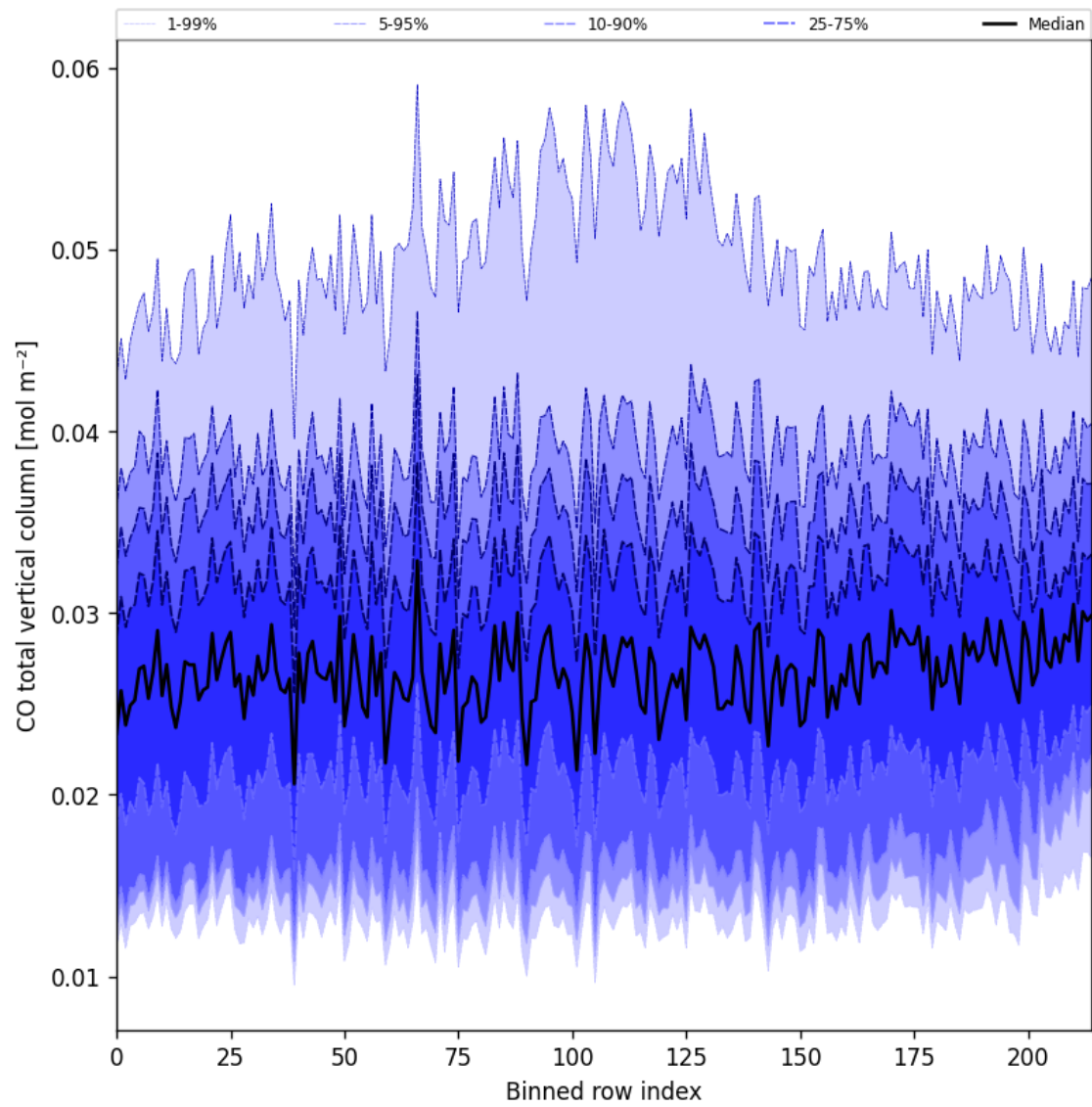
Figure 26: Along track statistics of “CO total vertical column” for 2024-11-11 to 2024-11-13
