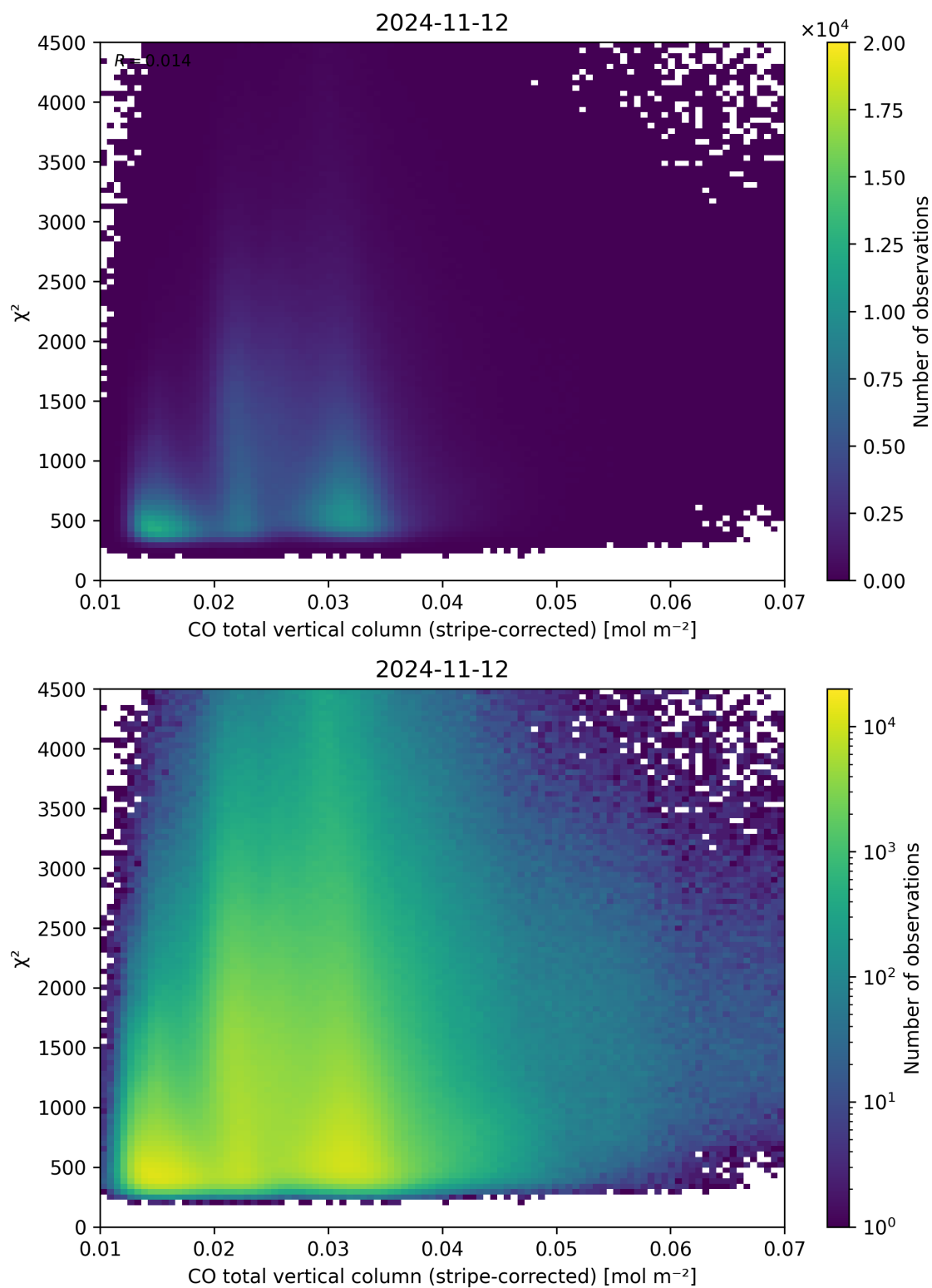
Figure 37: Scatter density plot of “CO total vertical column (stripe-corrected)” against “ \chi^2 ” for 2024-11-11 to 2024-11-13.
