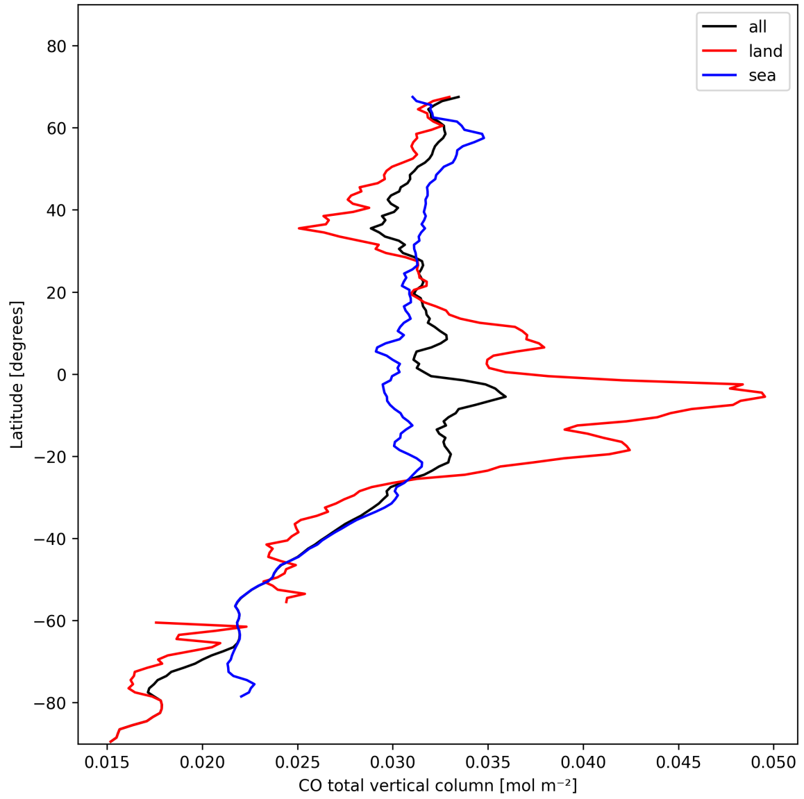
Figure 10: Zonal average of “CO total vertical column” for 2024-11-11 to 2024-11-13.
