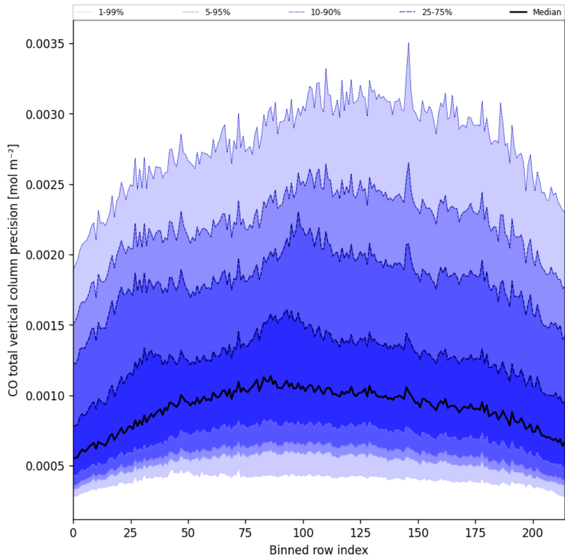
Figure 28: Along track statistics of “CO total vertical column precision” for 2024-11-11 to 2024-11-13
