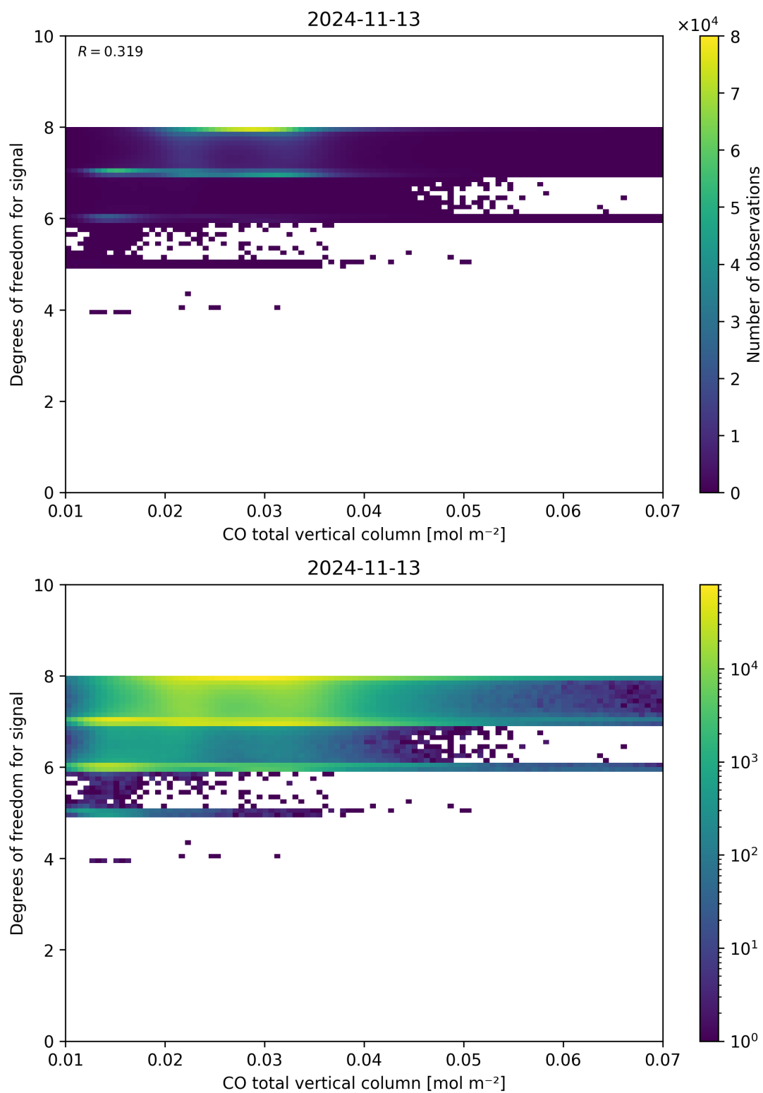
Figure 41: Scatter density plot of “CO total vertical column” against “Degrees of freedom for signal” for 2024-11-12 to 2024-11-14.
