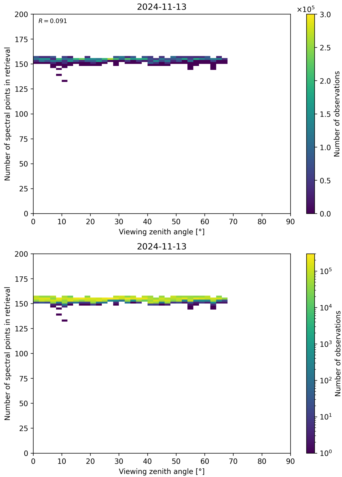
Figure 76: Scatter density plot of “Viewing zenith angle” against “Number of spectral points in retrieval” for 2024-11-12 to 2024-11-14.
