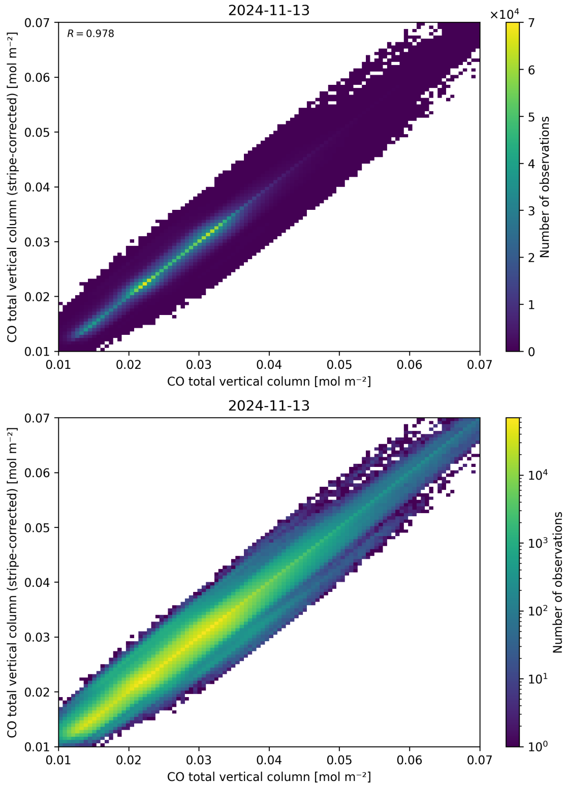
Figure 33: Scatter density plot of “CO total vertical column” against “CO total vertical column (stripe-corrected)” for 2024-11-12 to 2024-11-14.
