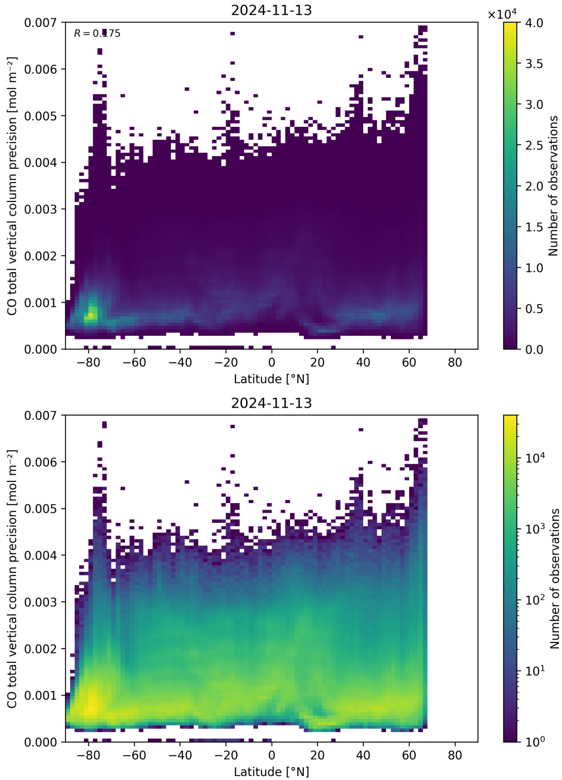
Figure 53: Scatter density plot of “Latitude” against “CO total vertical column precision” for 2024-11-12 to 2024-11-14.
