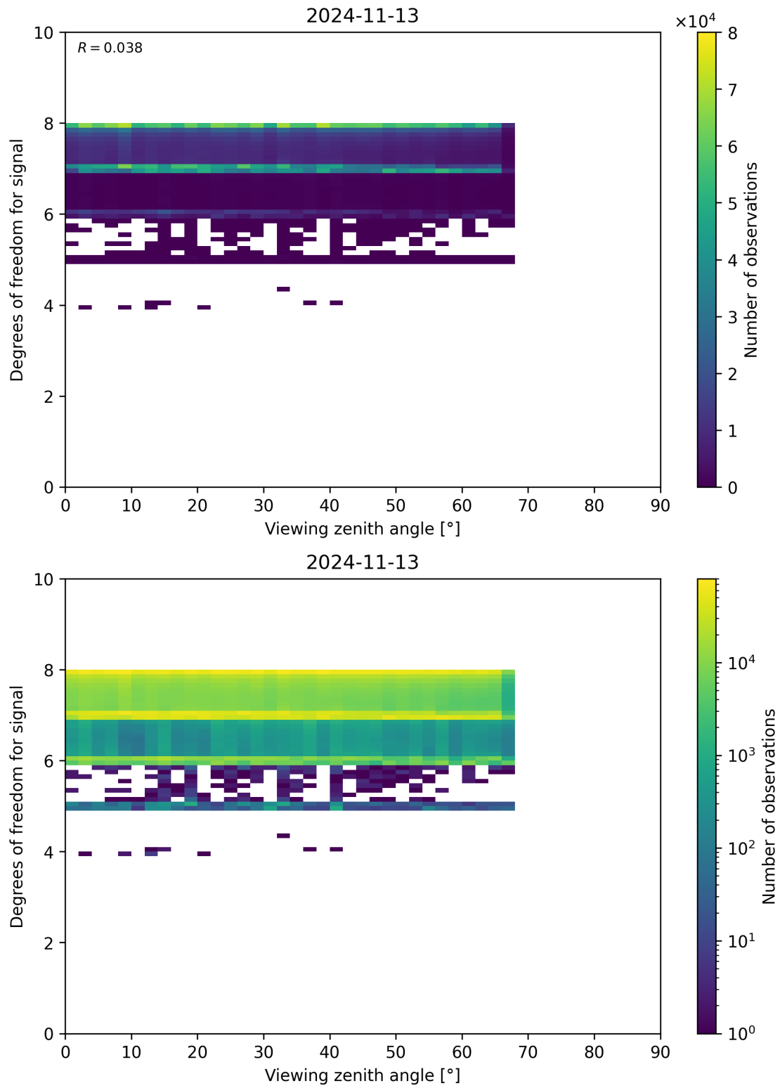
Figure 73: Scatter density plot of “Viewing zenith angle” against “Degrees of freedom for signal” for 2024-11-12 to 2024-11-14.
