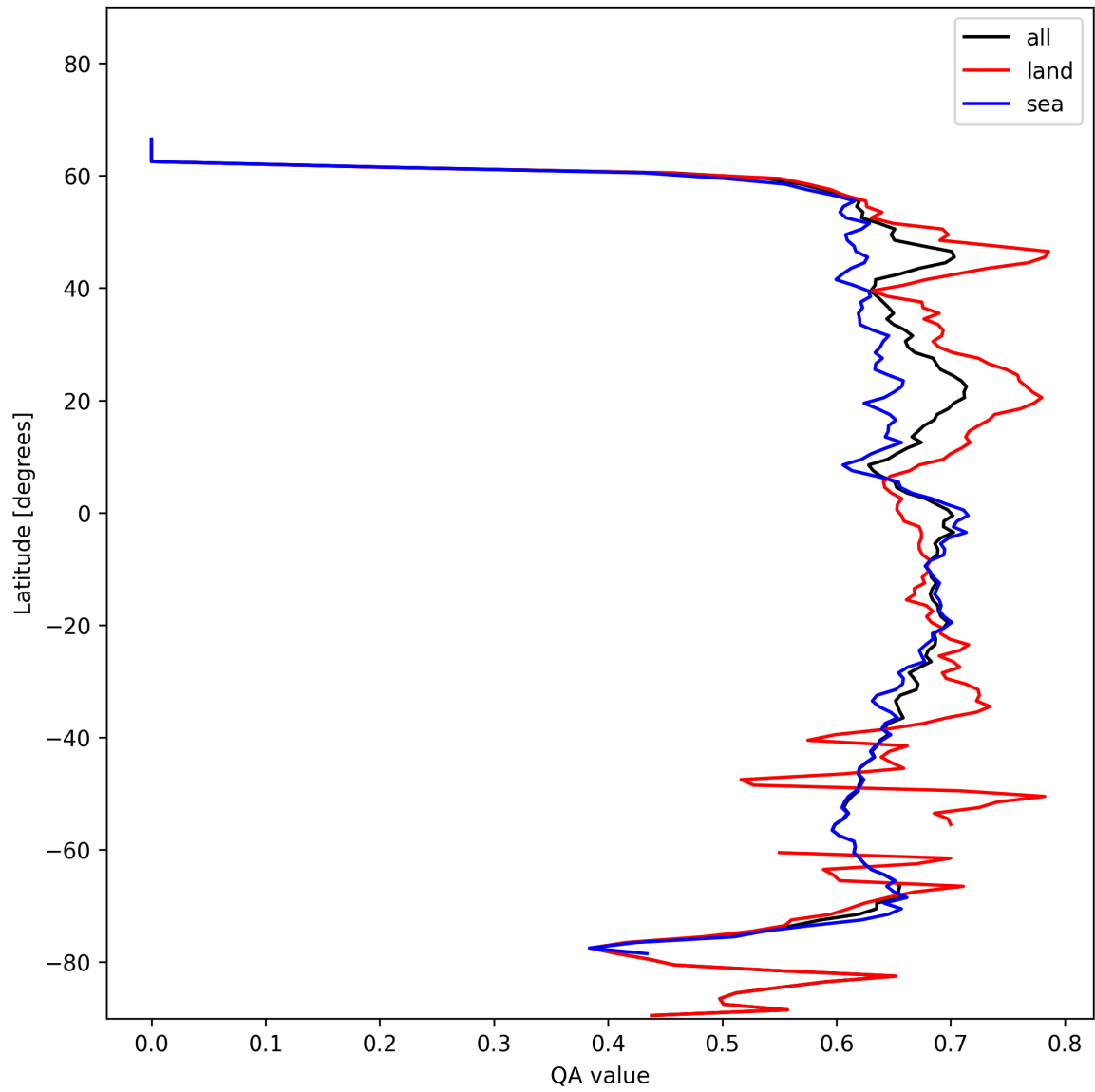
Figure 9: Zonal average of “QA value” for 2024-11-12 to 2024-11-14.
