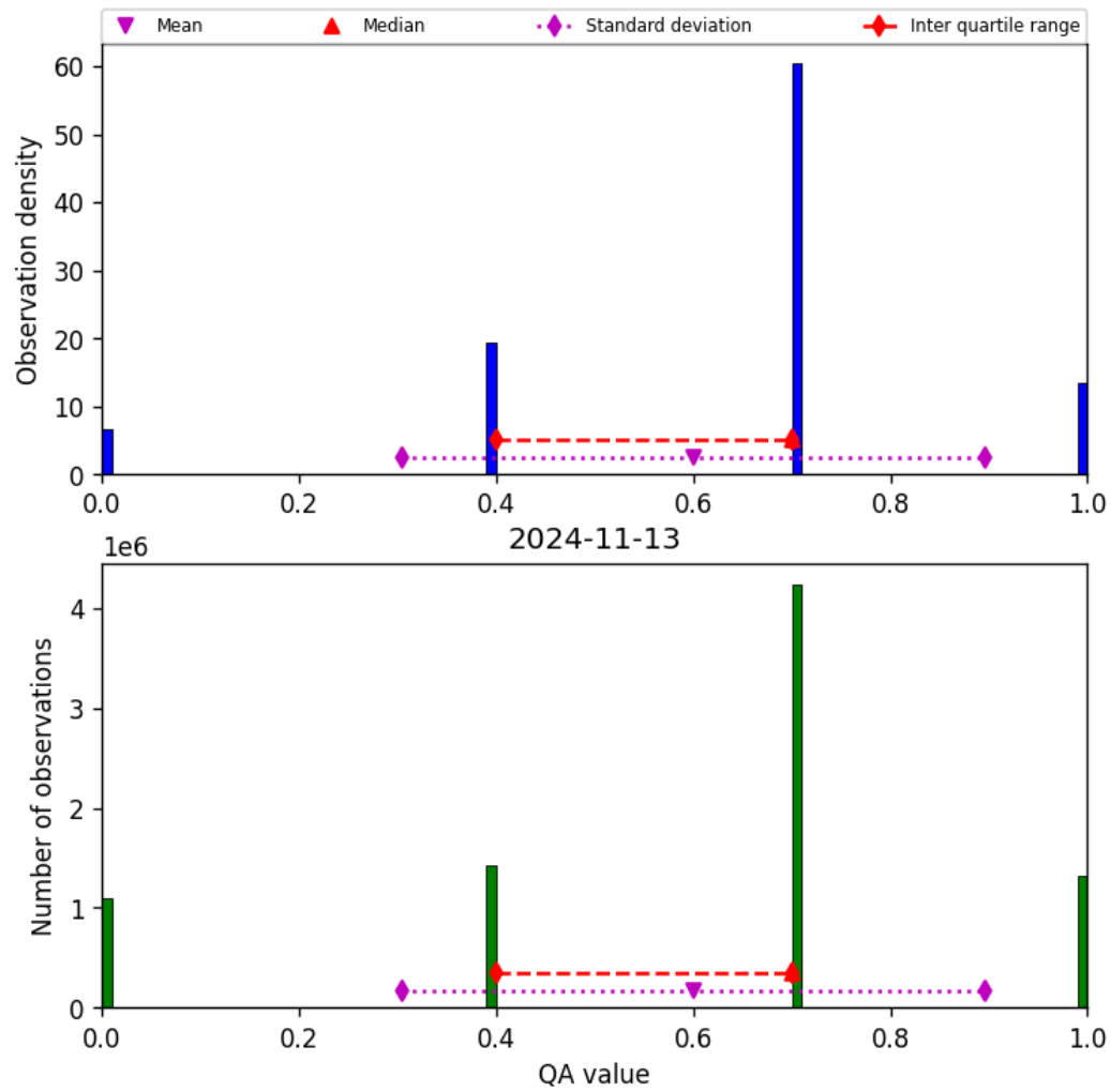
Figure 17: Histogram of “QA value” for 2024-11-12 to 2024-11-14
