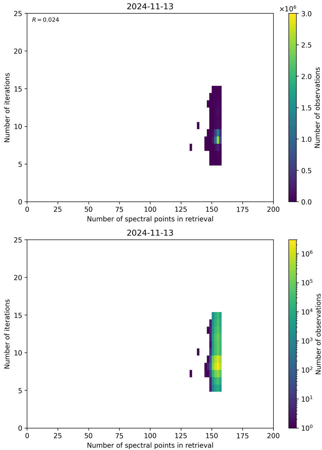
Figure 60: Scatter density plot of “Number of spectral points in retrieval” against “Number of iterations” for 2024-11-12 to 2024-11-14.
