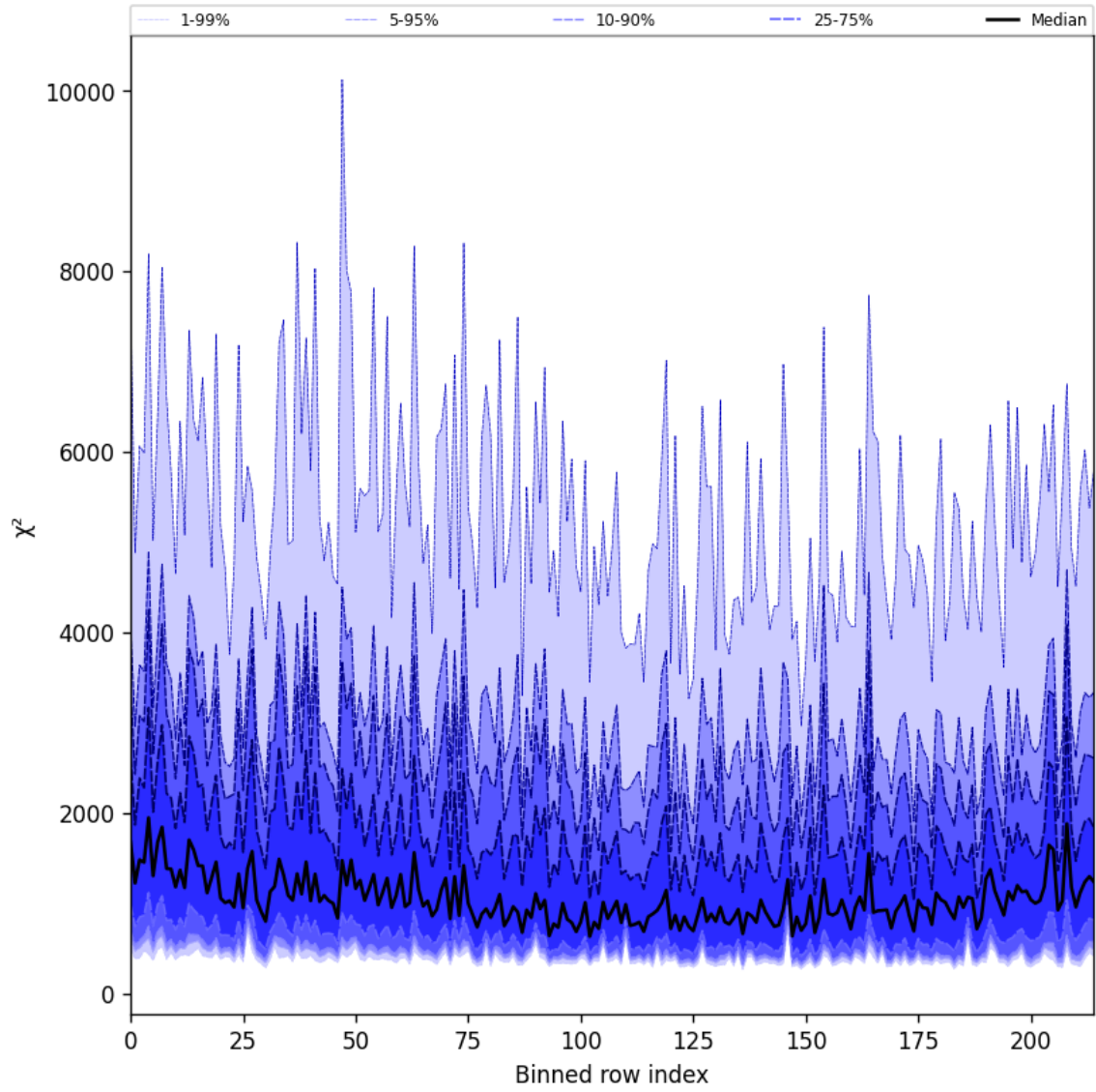
Figure 30: Along track statistics of “ \chi^2 ” for 2024-11-12 to 2024-11-14
