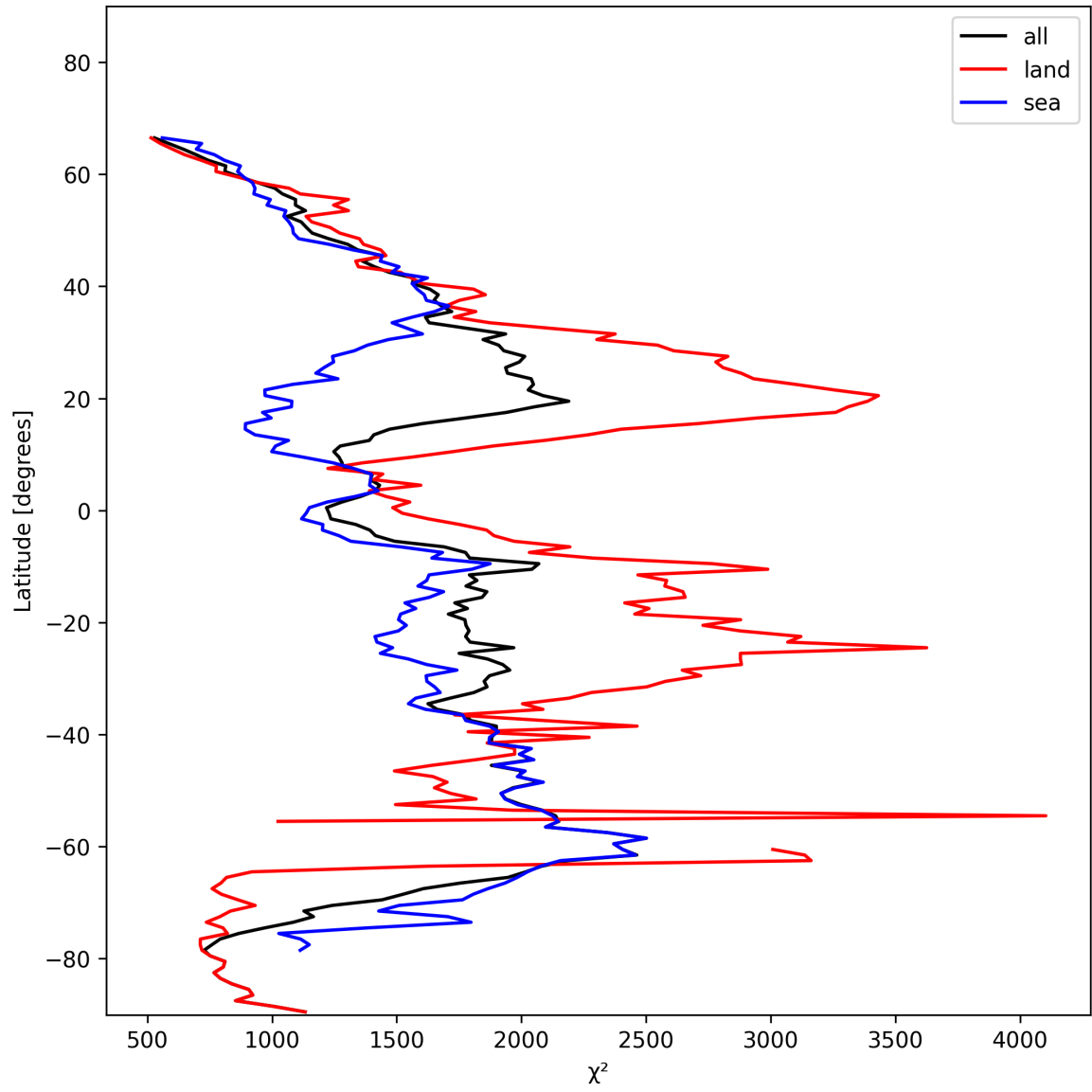
Figure 14: Zonal average of “ \chi^2 ” for 2024-11-12 to 2024-11-14.
