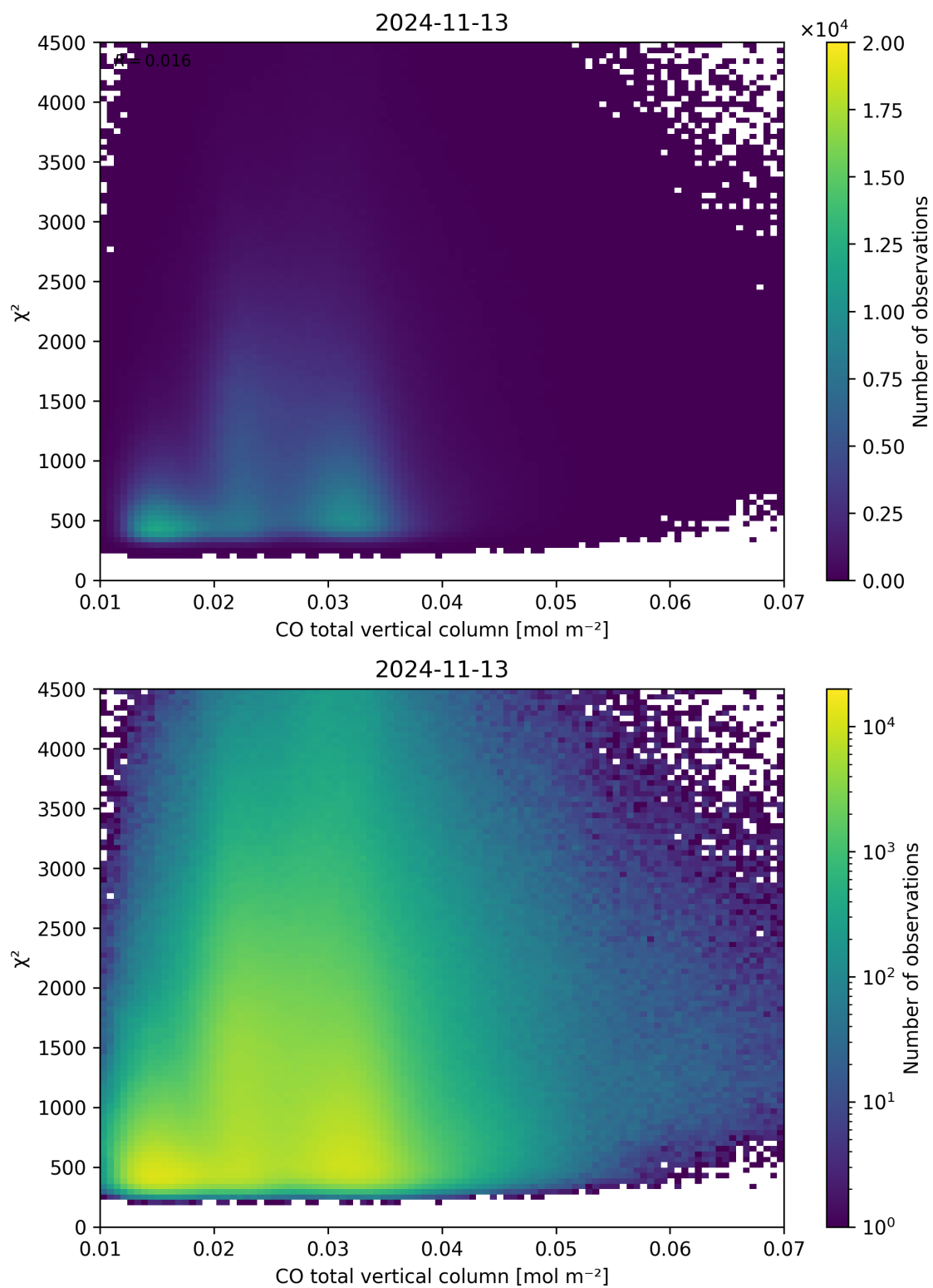
Figure 35: Scatter density plot of “CO total vertical column” against “ \chi^2 ” for 2024-11-12 to 2024-11-14.
