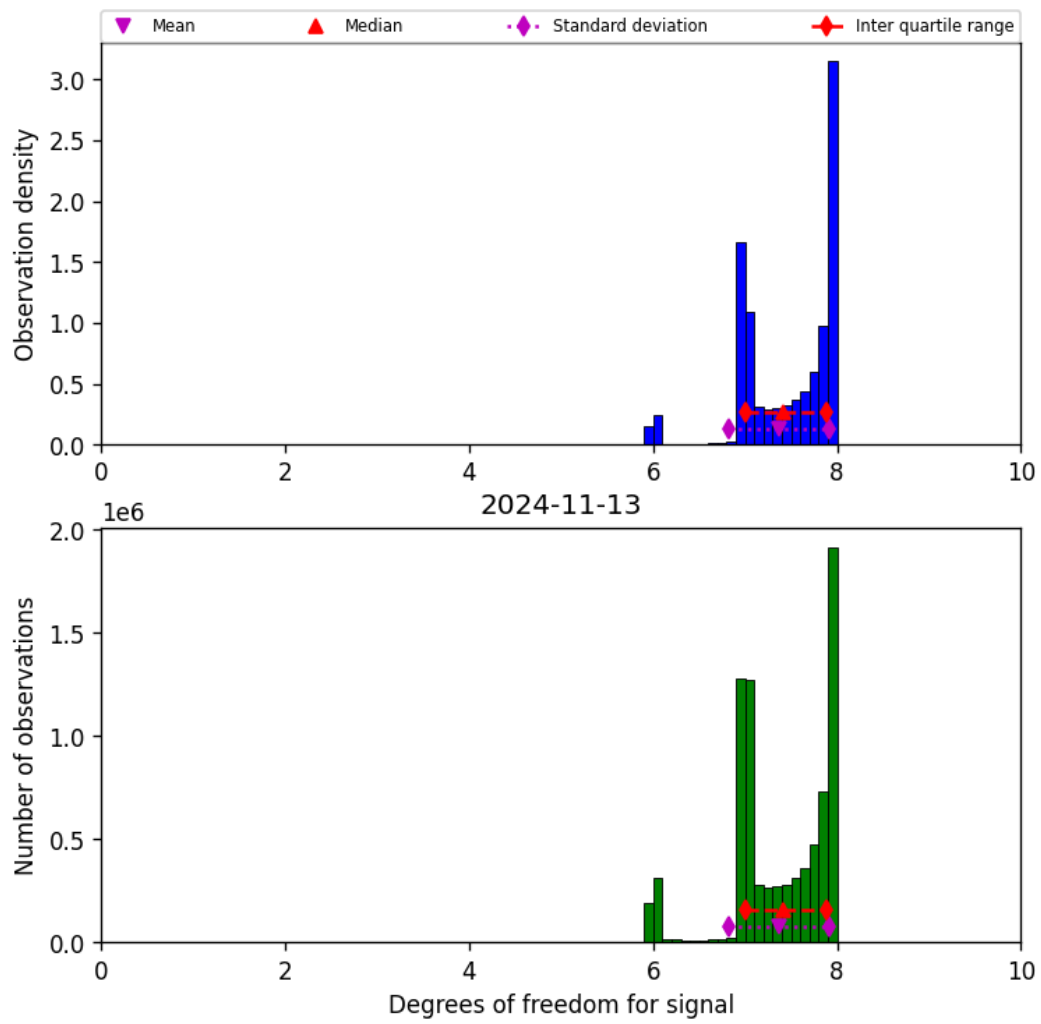
Figure 23: Histogram of “Degrees of freedom for signal” for 2024-11-12 to 2024-11-14
