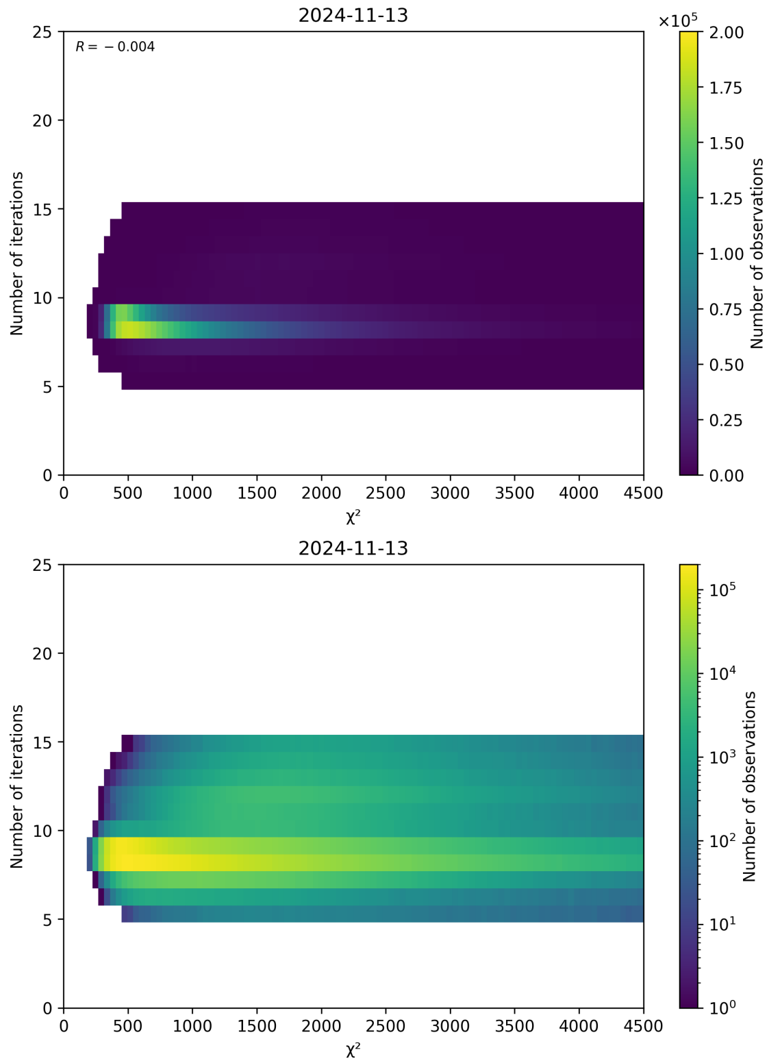
Figure 49: Scatter density plot of “ \chi^2 ” against “Number of iterations” for 2024-11-12 to 2024-11-14.
