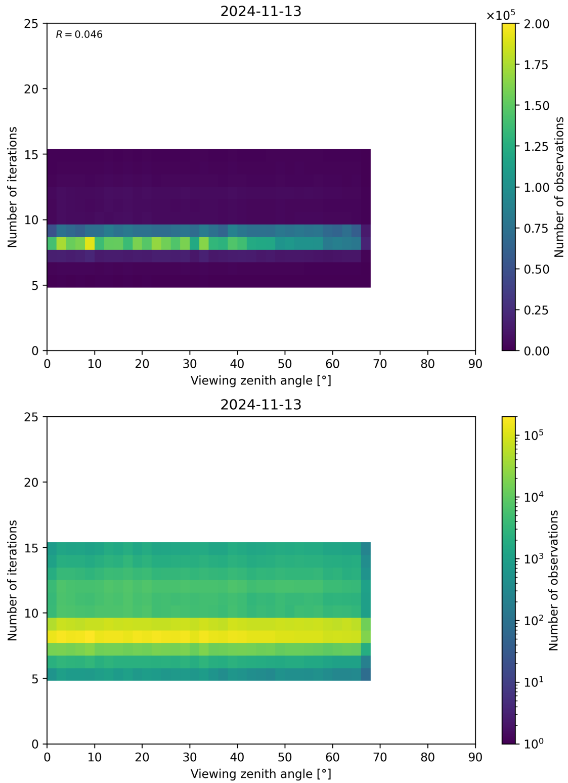
Figure 75: Scatter density plot of “Viewing zenith angle” against “Number of iterations” for 2024-11-12 to 2024-11-14.
