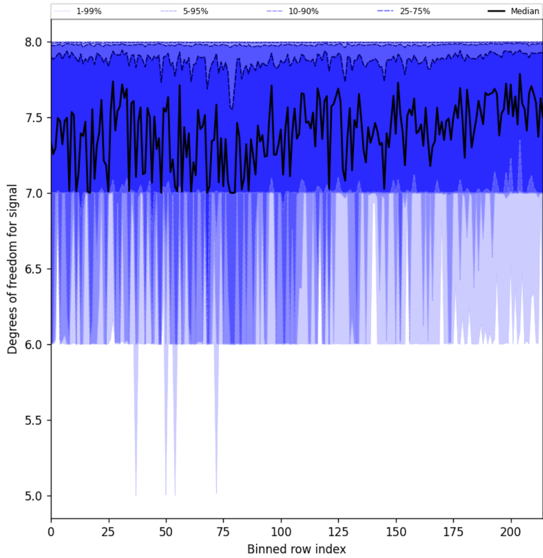
Figure 31: Along track statistics of “Degrees of freedom for signal” for 2024-11-12 to 2024-11-14
