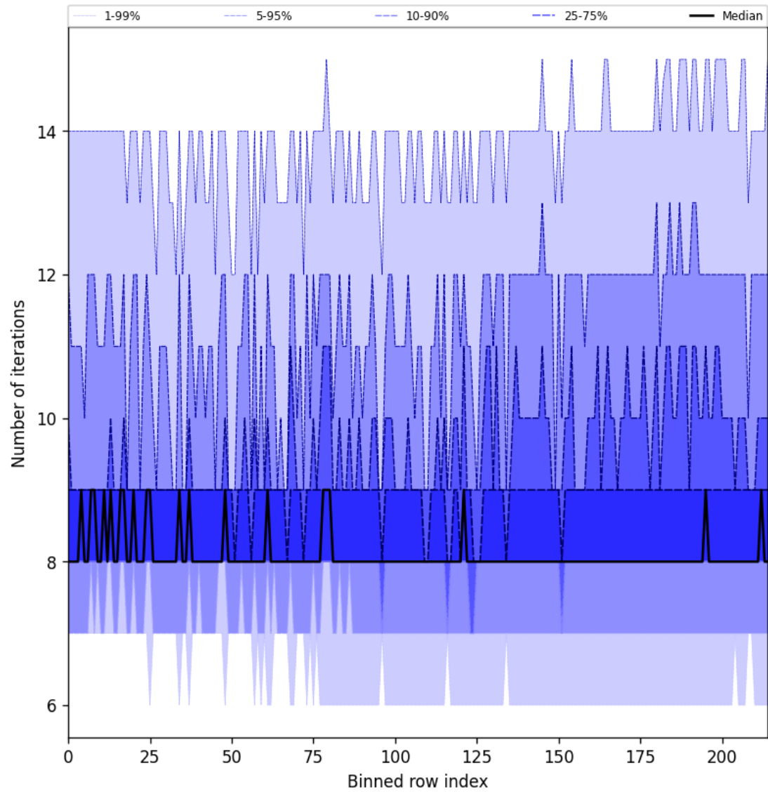
Figure 32: Along track statistics of “Number of iterations” for 2024-11-12 to 2024-11-14
