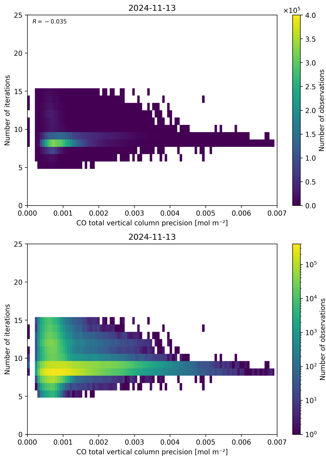
Figure 46: Scatter density plot of “CO total vertical column precision” against “Number of iterations” for 2024-11-12 to 2024-11-14.
