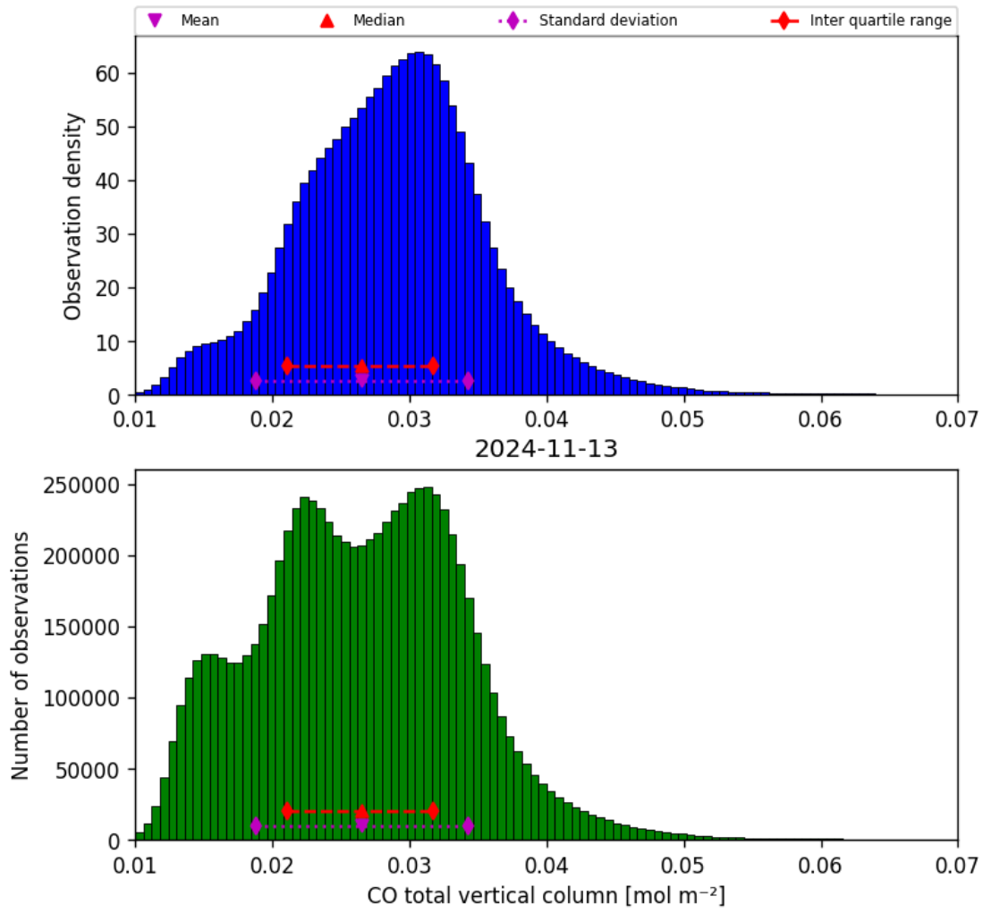
Figure 18: Histogram of “CO total vertical column” for 2024-11-12 to 2024-11-14
