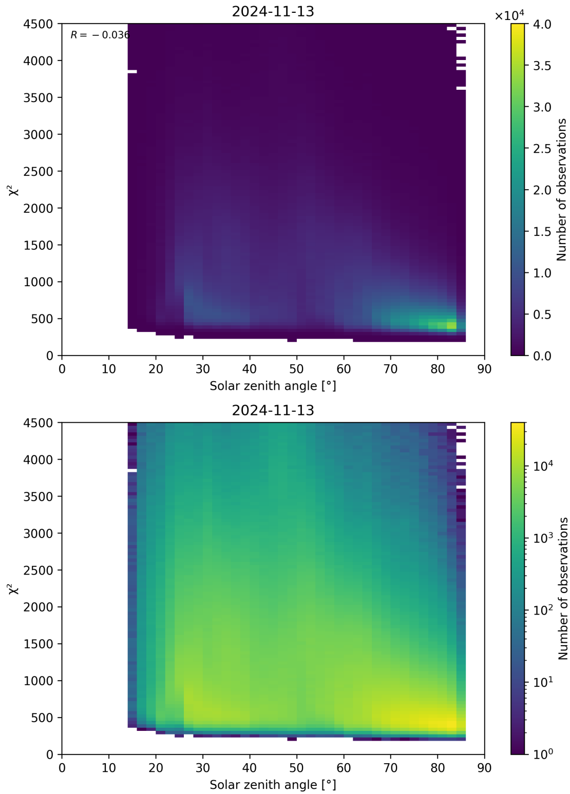
Figure 64: Scatter density plot of “Solar zenith angle” against “ \chi^2 ” for 2024-11-12 to 2024-11-14.
