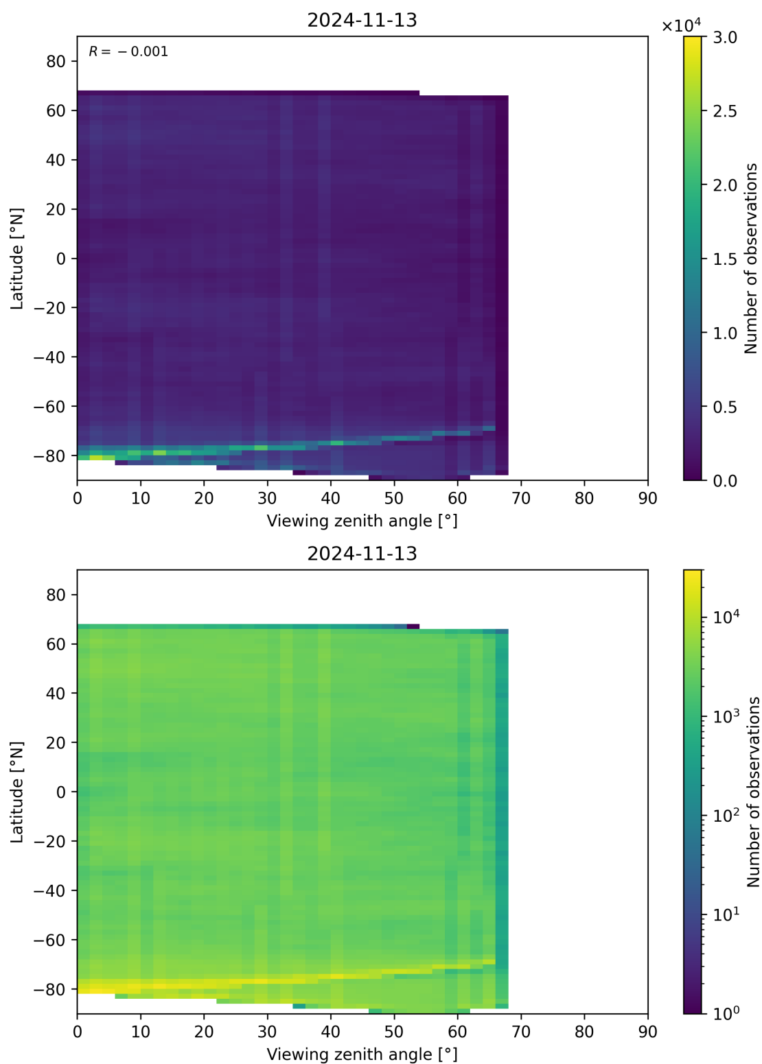
Figure 74: Scatter density plot of “Viewing zenith angle” against “Latitude” for 2024-11-12 to 2024-11-14.
