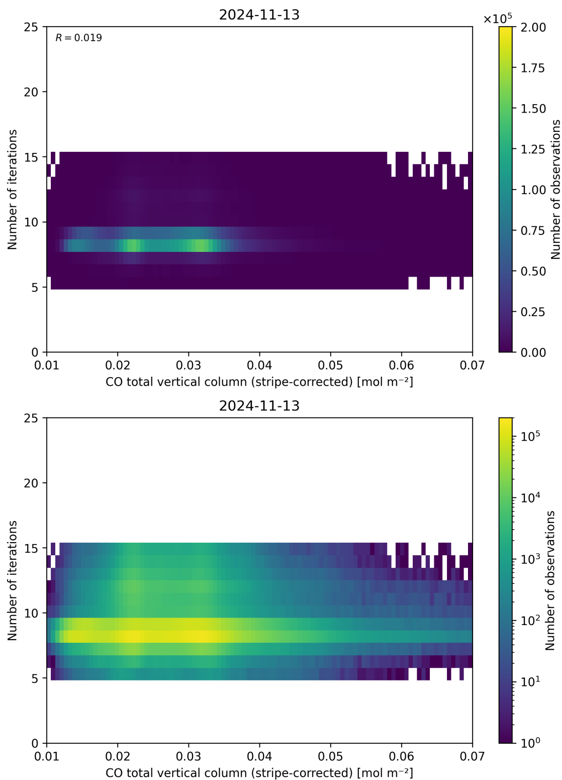
Figure 39: Scatter density plot of “CO total vertical column (stripe-corrected)” against “Number of iterations” for 2024-11-12 to 2024-11-14.
