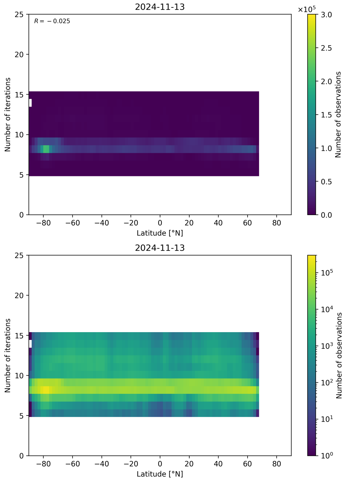
Figure 56: Scatter density plot of “Latitude” against “Number of iterations” for 2024-11-12 to 2024-11-14.
