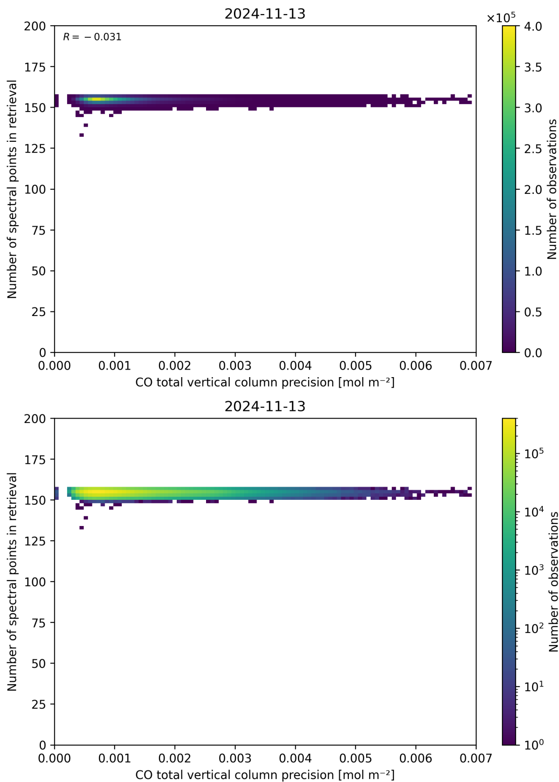
Figure 47: Scatter density plot of “CO total vertical column precision” against “Number of spectral points in retrieval” for 2024-11-12 to 2024-11-14.
