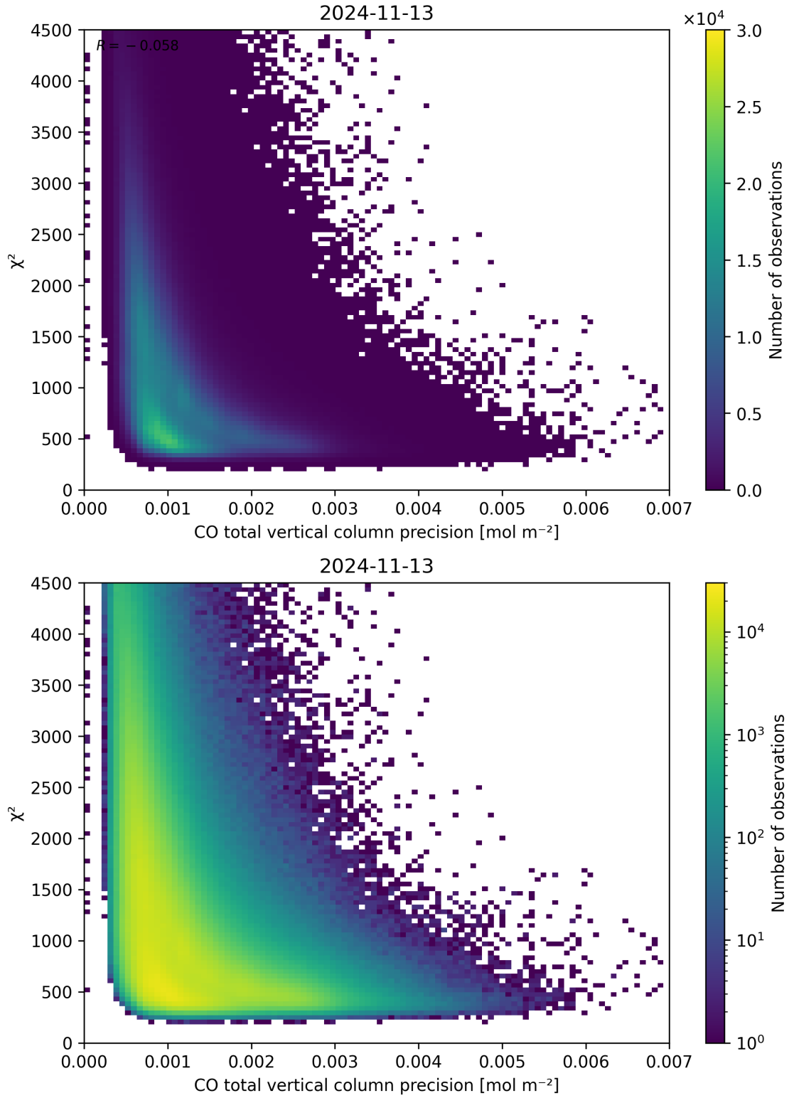
Figure 44: Scatter density plot of “CO total vertical column precision” against “ \chi^2 ” for 2024-11-12 to 2024-11-14.
