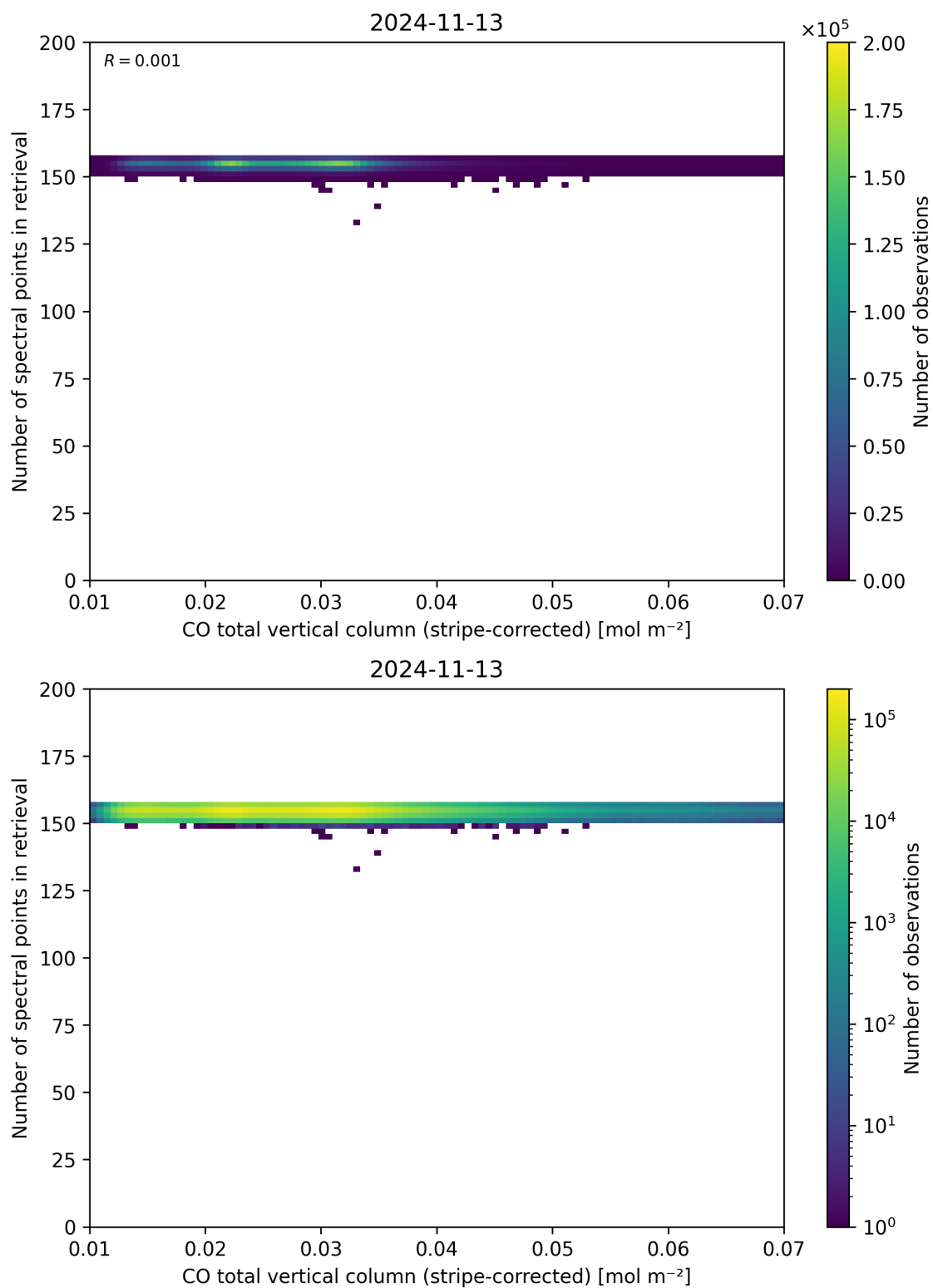
Figure 40: Scatter density plot of “CO total vertical column (stripe-corrected)” against “Number of spectral points in retrieval” for 2024-11-12 to 2024-11-14.
