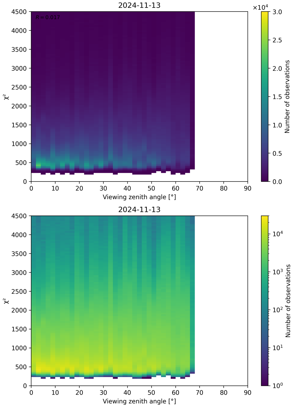
Figure 72: Scatter density plot of “Viewing zenith angle” against “ \chi^2 ” for 2024-11-12 to 2024-11-14.
