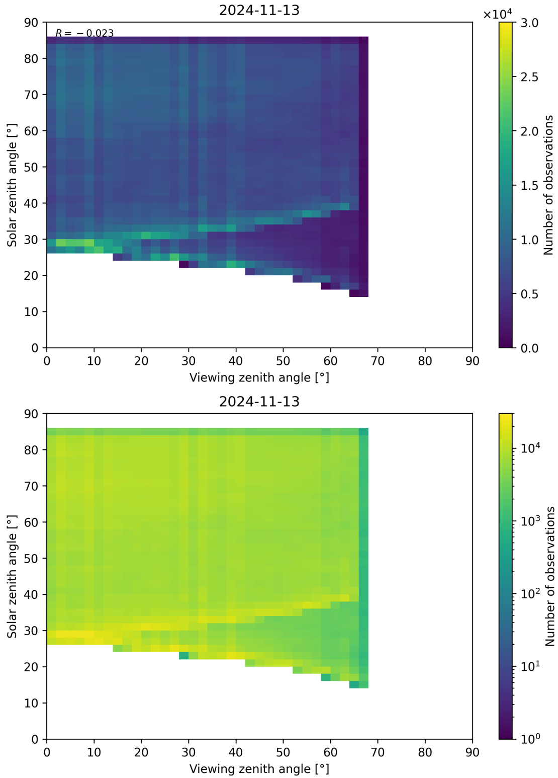
Figure 77: Scatter density plot of “Viewing zenith angle” against “Solar zenith angle” for 2024-11-12 to 2024-11-14.
