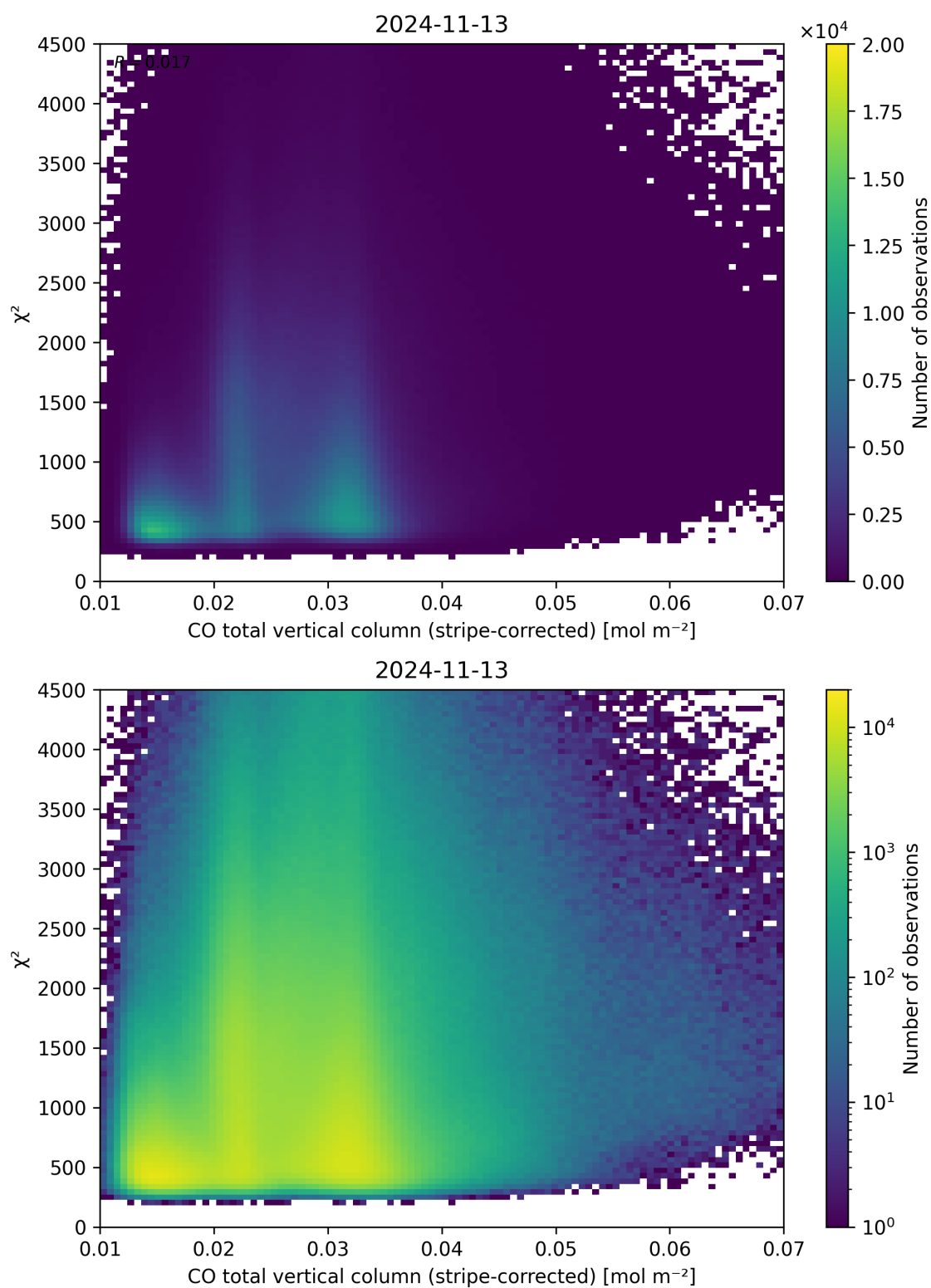
Figure 37: Scatter density plot of “CO total vertical column (stripe-corrected)” against “ \chi^2 ” for 2024-11-12 to 2024-11-14.
