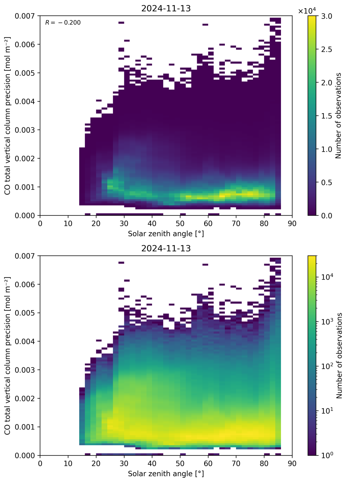
Figure 63: Scatter density plot of “Solar zenith angle” against “CO total vertical column precision” for 2024-11-12 to 2024-11-14.
