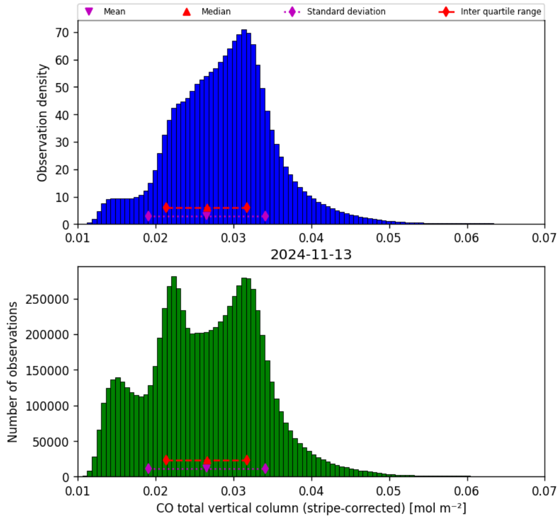
Figure 19: Histogram of “CO total vertical column (stripe-corrected)” for 2024-11-12 to 2024-11-14
