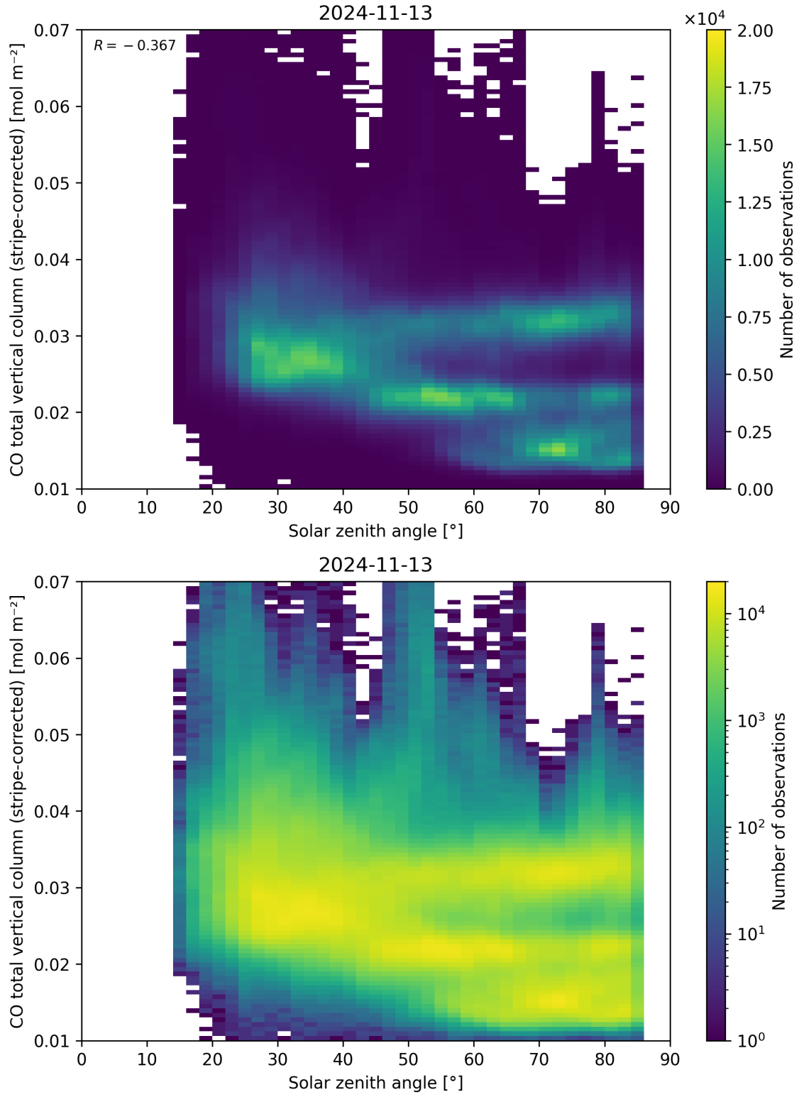
Figure 62: Scatter density plot of “Solar zenith angle” against “CO total vertical column (stripe-corrected)” for 2024-11-12 to 2024-11-14.
