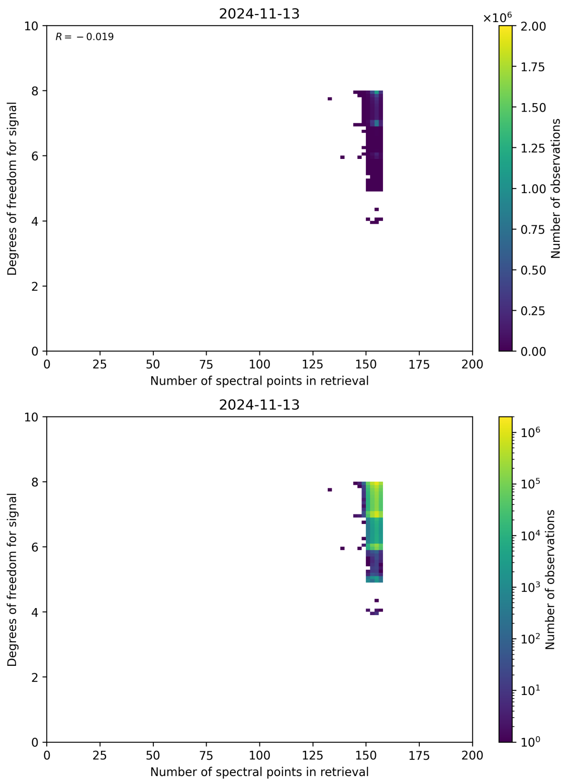
Figure 59: Scatter density plot of “Number of spectral points in retrieval” against “Degrees of freedom for signal” for 2024-11-12 to 2024-11-14.
