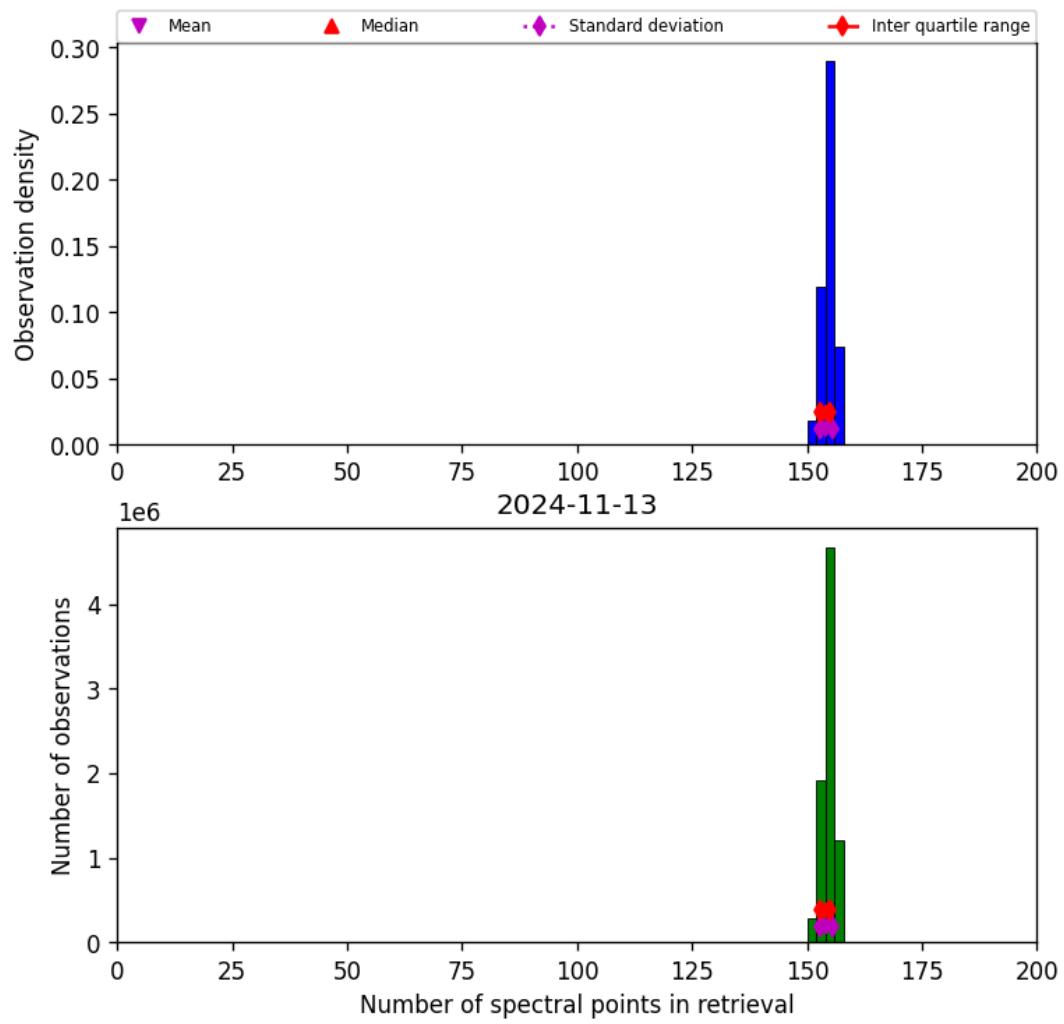
Figure 21: Histogram of “Number of spectral points in retrieval” for 2024-11-12 to 2024-11-14
