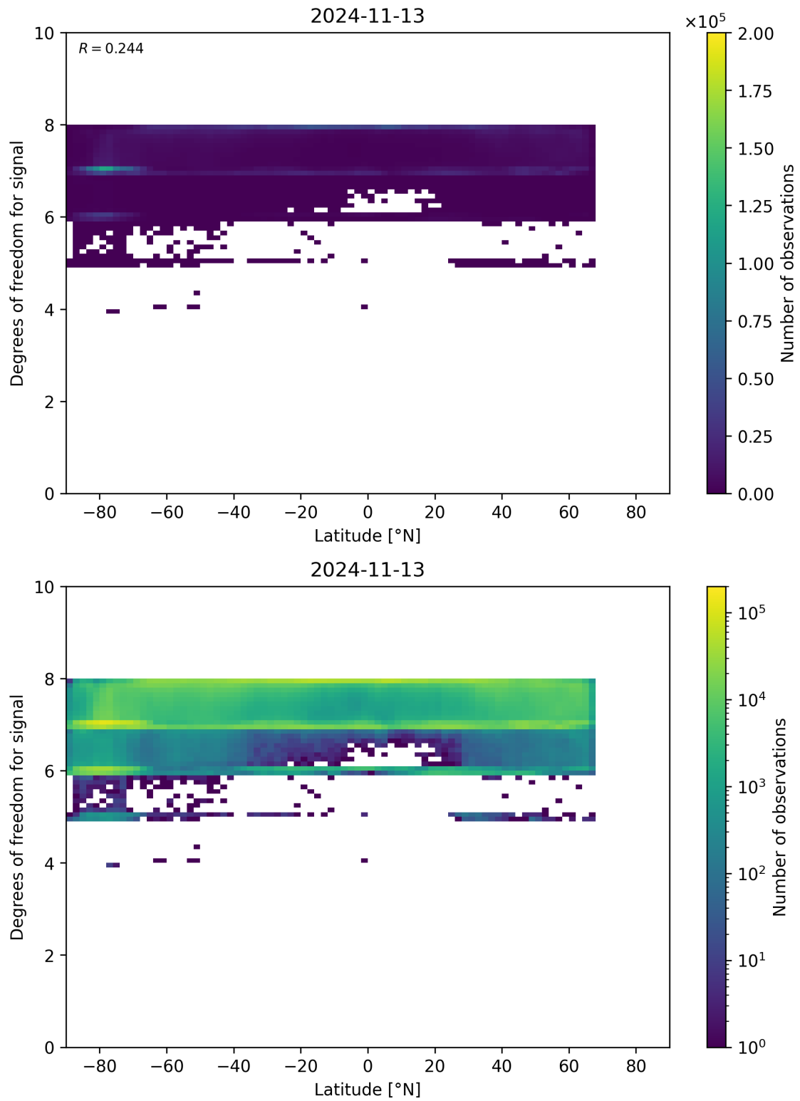
Figure 55: Scatter density plot of “Latitude” against “Degrees of freedom for signal” for 2024-11-12 to 2024-11-14.
