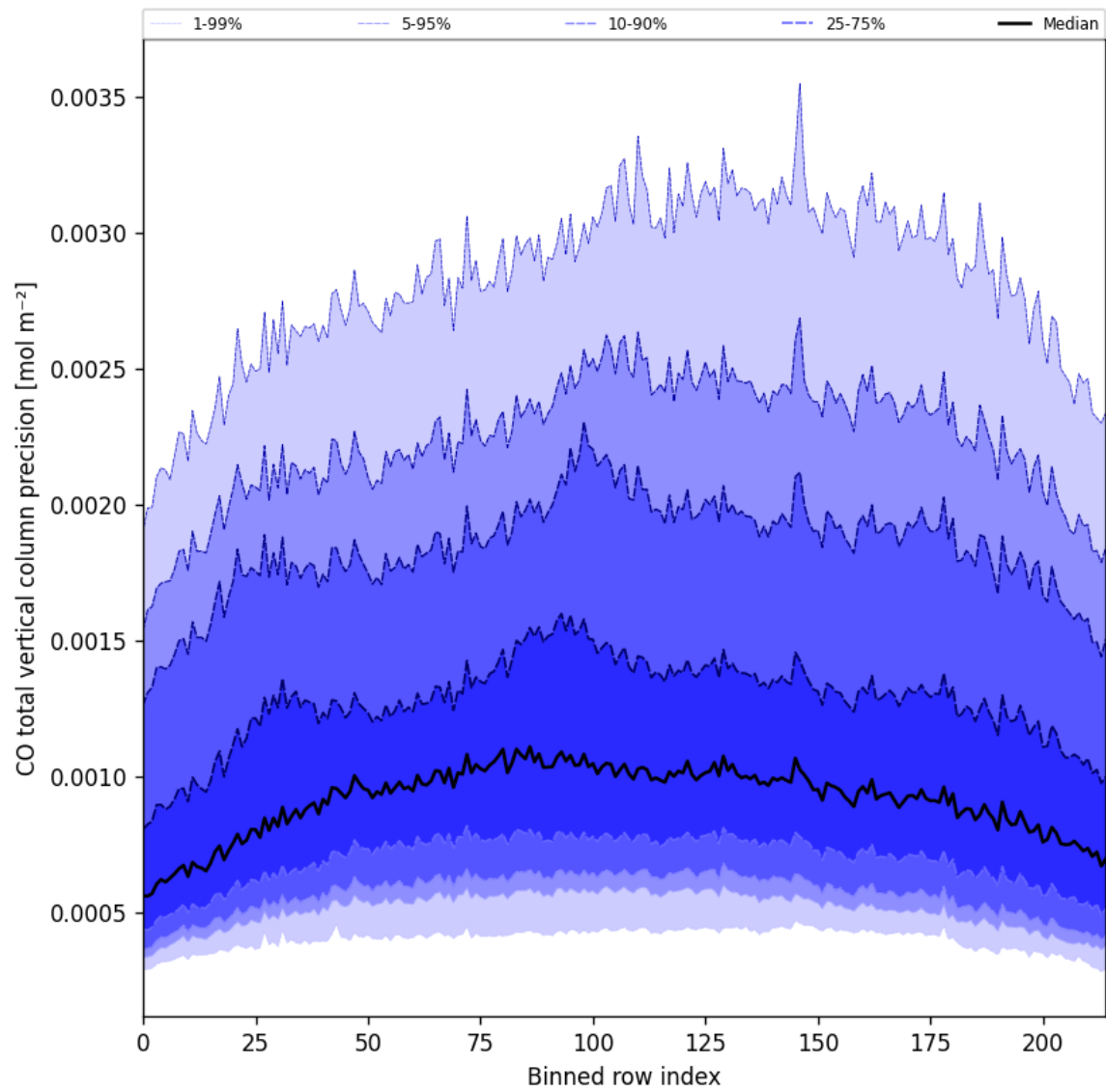
Figure 28: Along track statistics of “CO total vertical column precision” for 2024-11-12 to 2024-11-14
