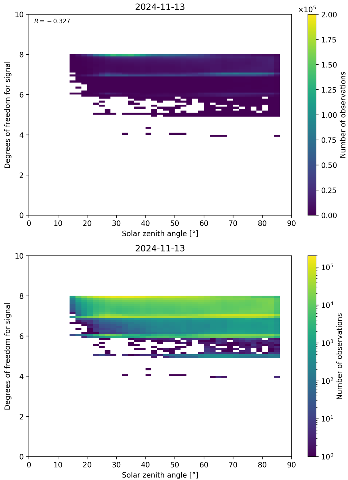
Figure 65: Scatter density plot of “Solar zenith angle” against “Degrees of freedom for signal” for 2024-11-12 to 2024-11-14.
