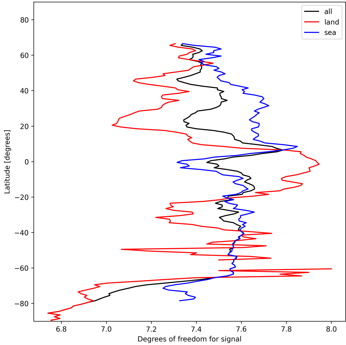
Figure 15: Zonal average of “Degrees of freedom for signal” for 2024-11-12 to 2024-11-14.
