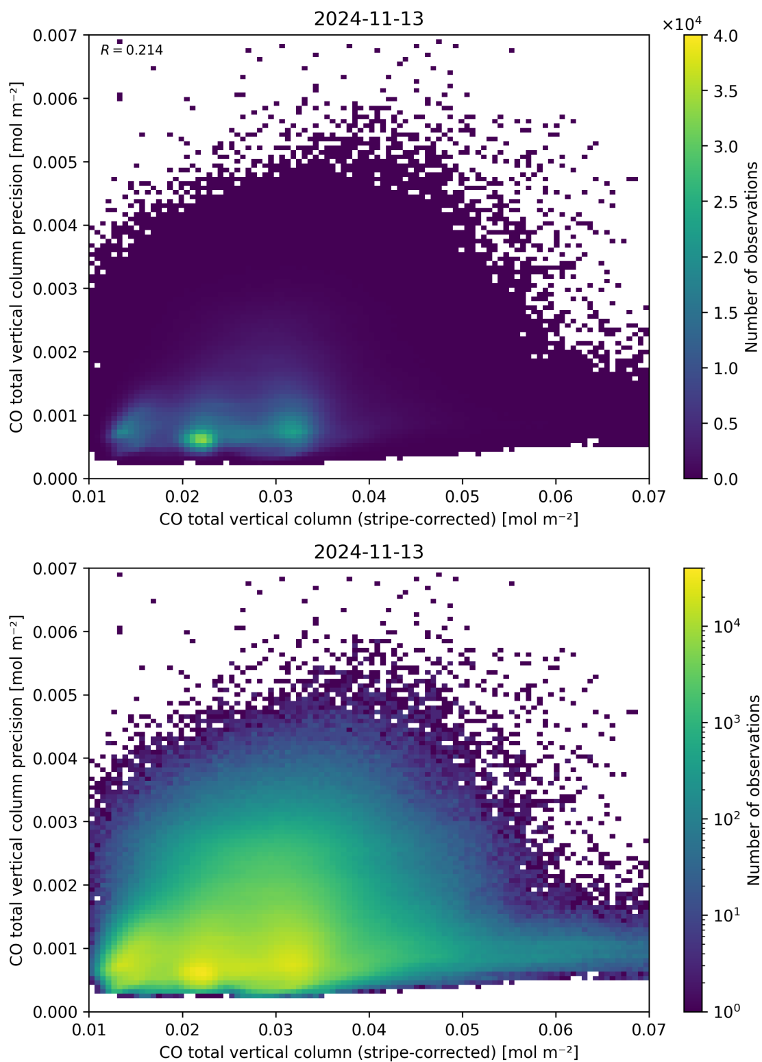
Figure 36: Scatter density plot of “CO total vertical column (stripe-corrected)” against “CO total vertical column precision” for 2024-11-12 to 2024-11-14.
