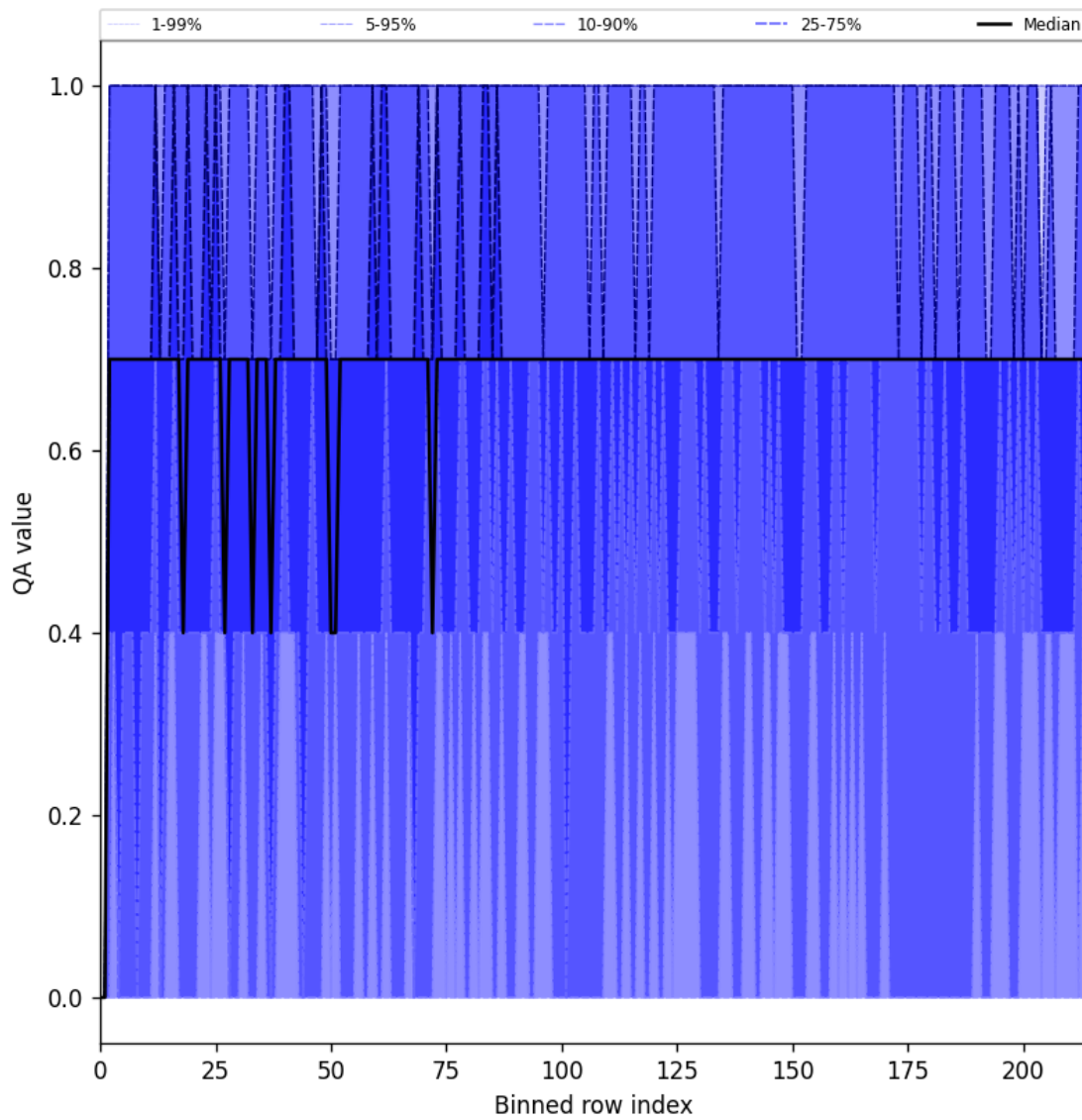
Figure 25: Along track statistics of “QA value” for 2024-11-12 to 2024-11-14
