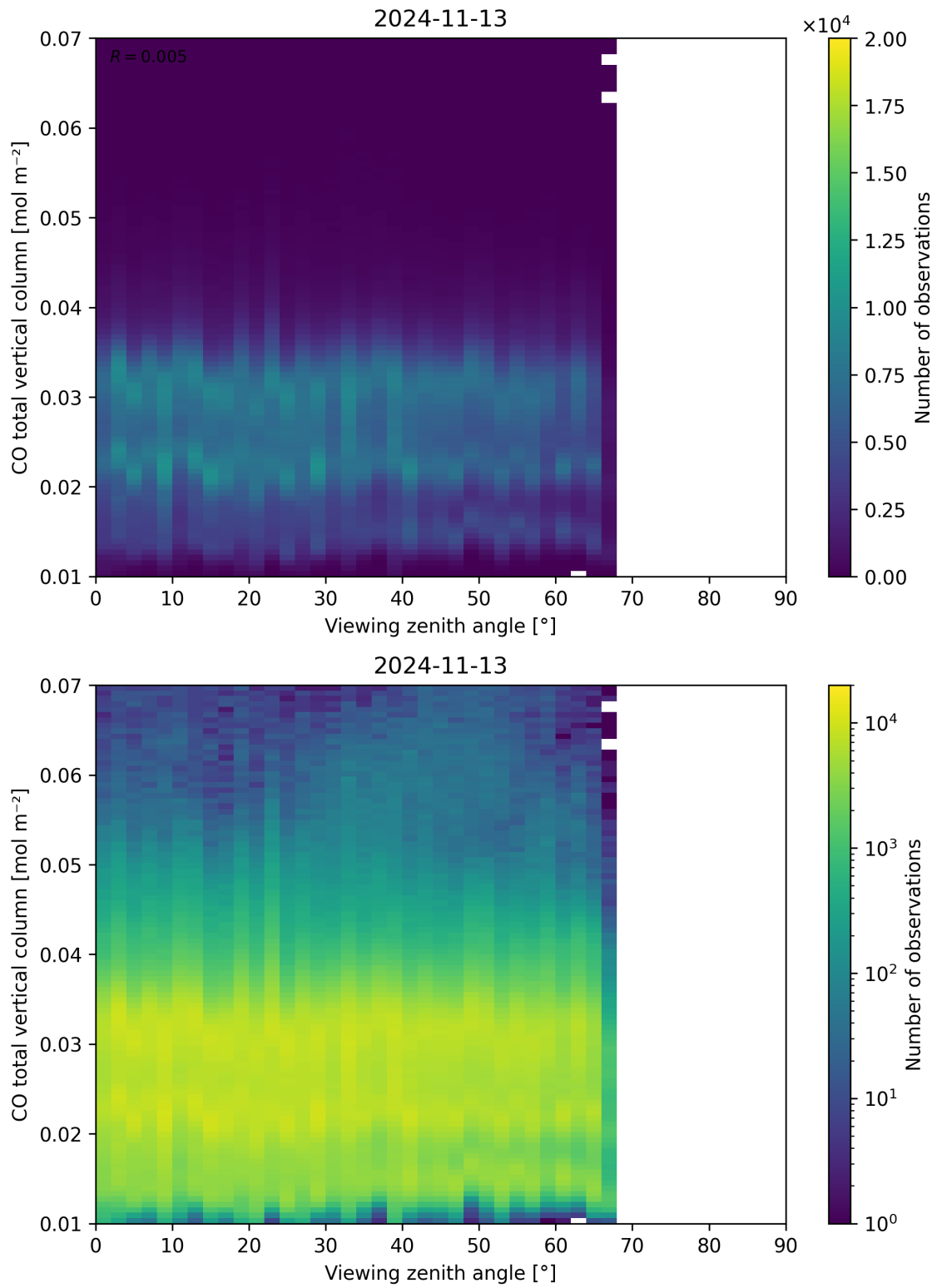
Figure 69: Scatter density plot of “Viewing zenith angle” against “CO total vertical column” for 2024-11-12 to 2024-11-14.
