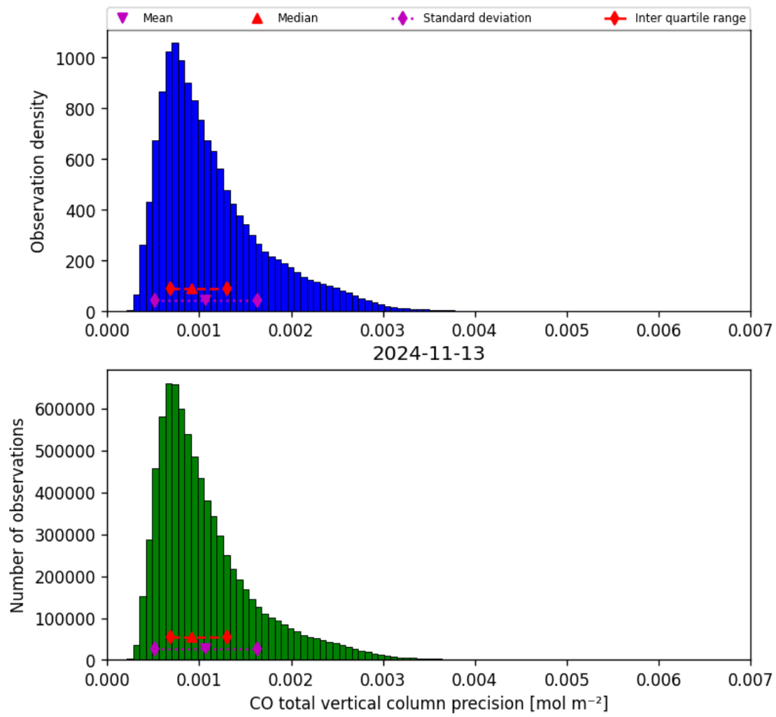
Figure 20: Histogram of “CO total vertical column precision” for 2024-11-12 to 2024-11-14
