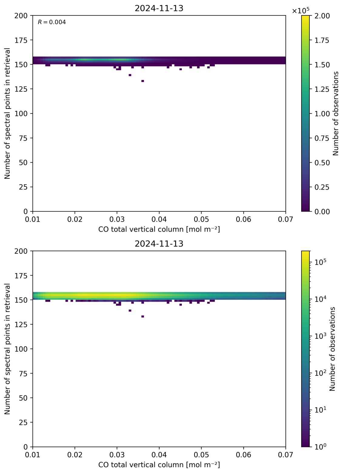
Figure 43: Scatter density plot of “CO total vertical column” against “Number of spectral points in retrieval” for 2024-11-12 to 2024-11-14.
