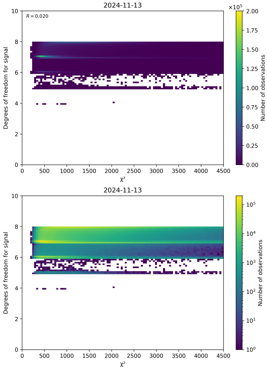
Figure 48: Scatter density plot of “ \chi^2 ” against “Degrees of freedom for signal” for 2024-11-12 to 2024-11-14.
