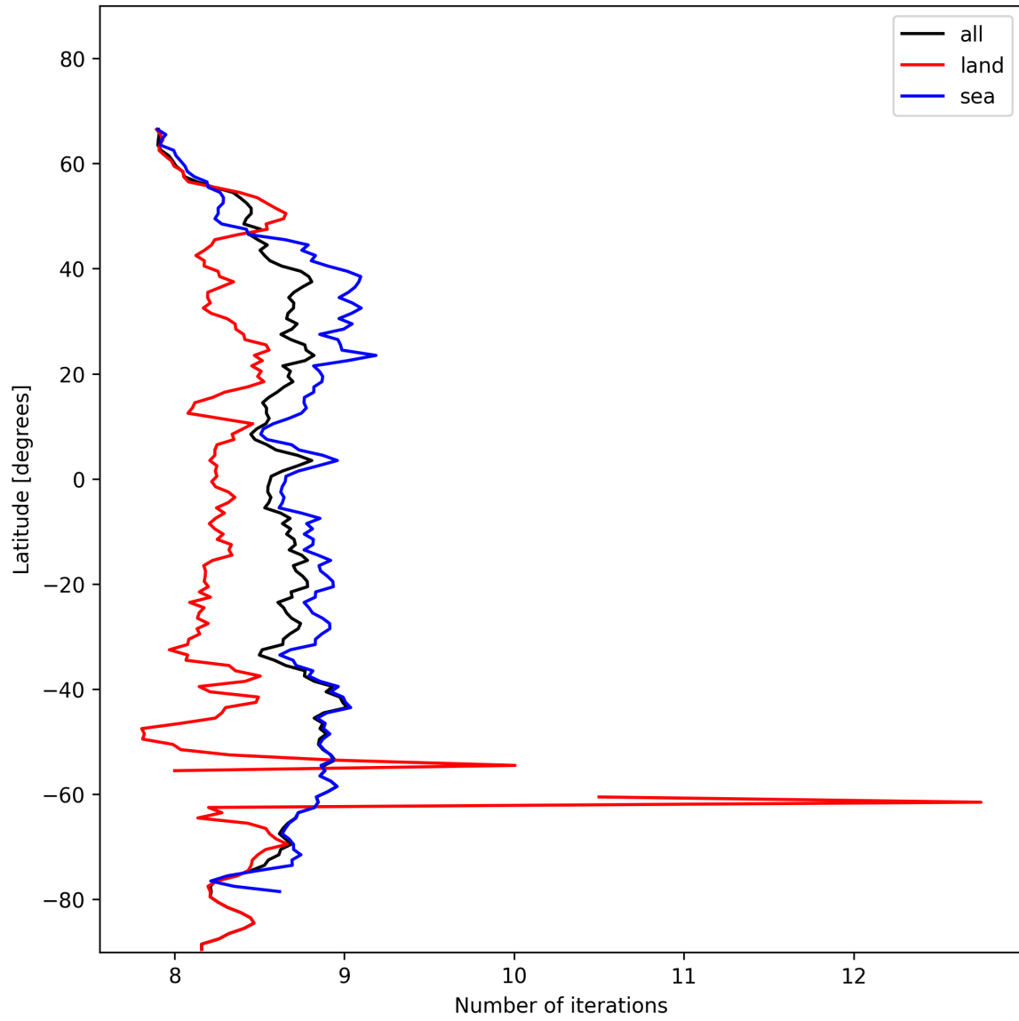
Figure 16: Zonal average of “Number of iterations” for 2024-11-12 to 2024-11-14.
