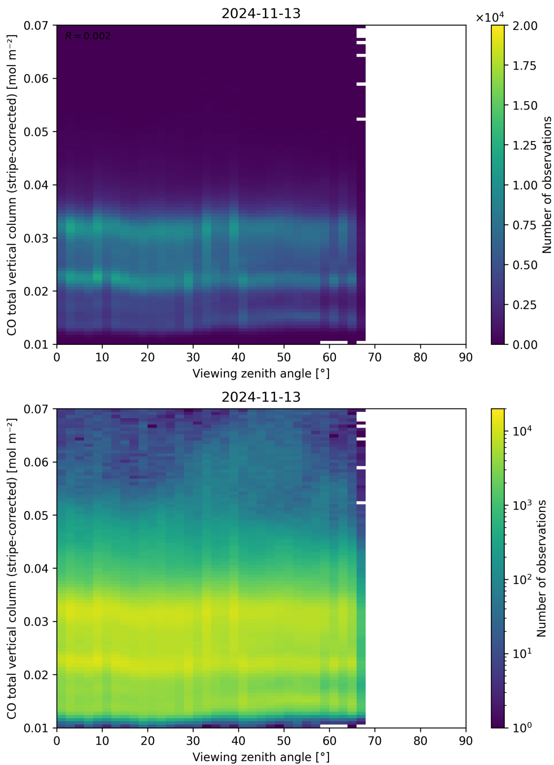
Figure 70: Scatter density plot of “Viewing zenith angle” against “CO total vertical column (stripe-corrected)” for 2024-11-12 to 2024-11-14.
