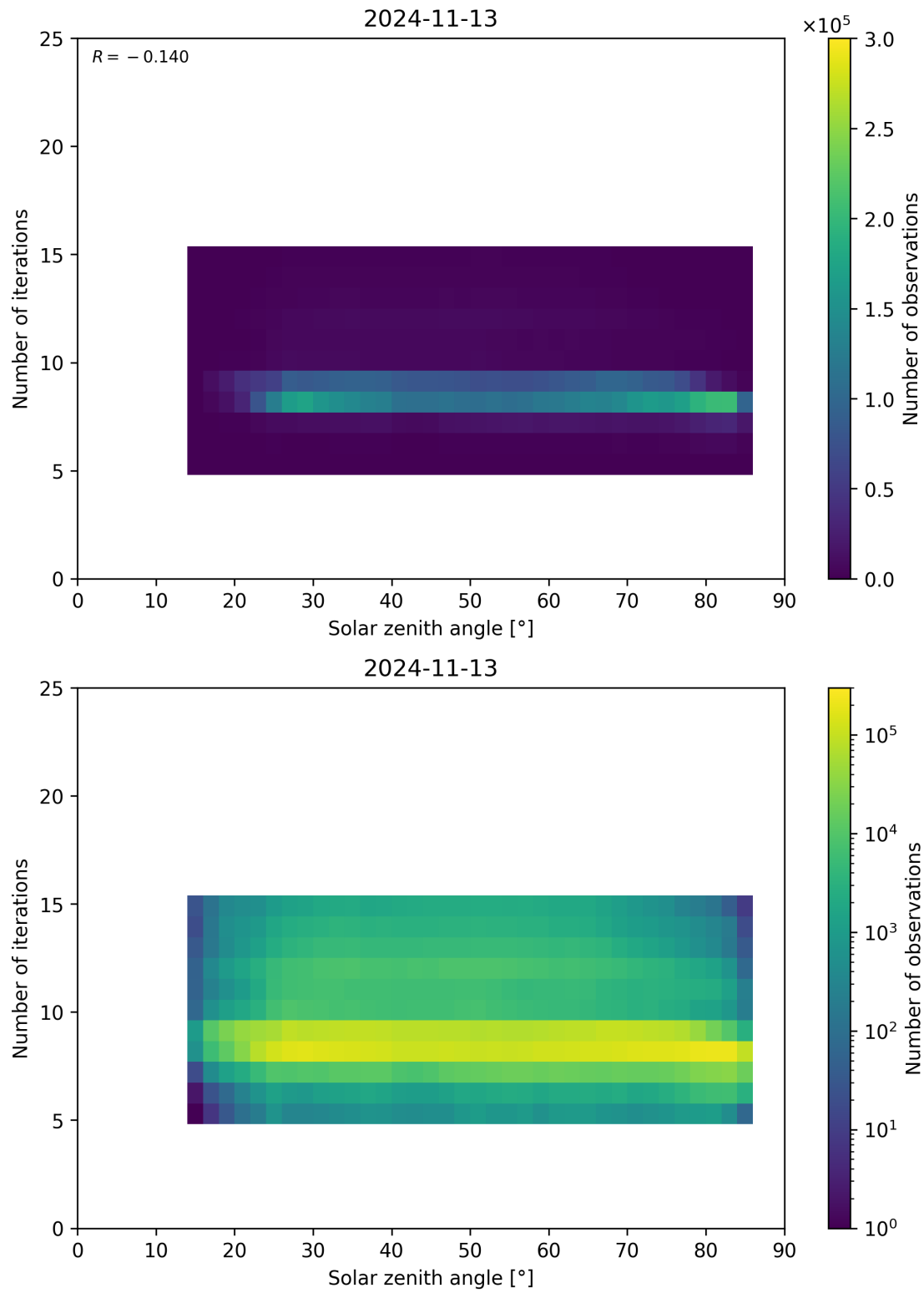
Figure 67: Scatter density plot of “Solar zenith angle” against “Number of iterations” for 2024-11-12 to 2024-11-14.
