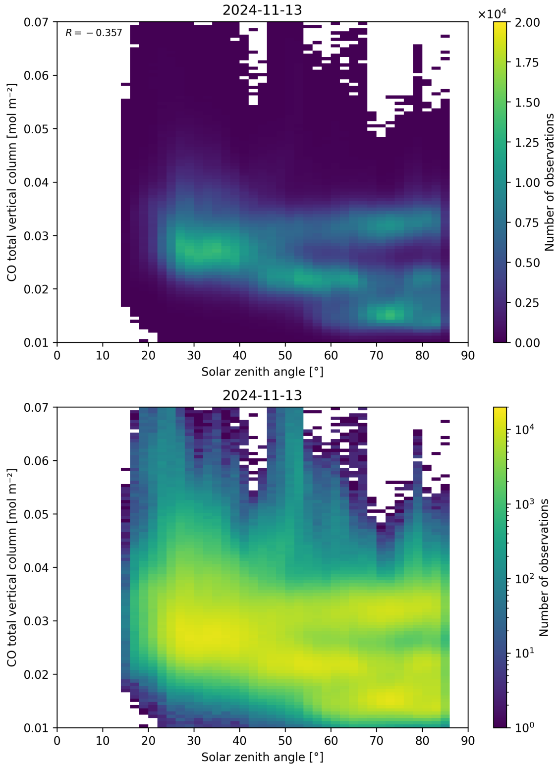
Figure 61: Scatter density plot of “Solar zenith angle” against “CO total vertical column” for 2024-11-12 to 2024-11-14.
