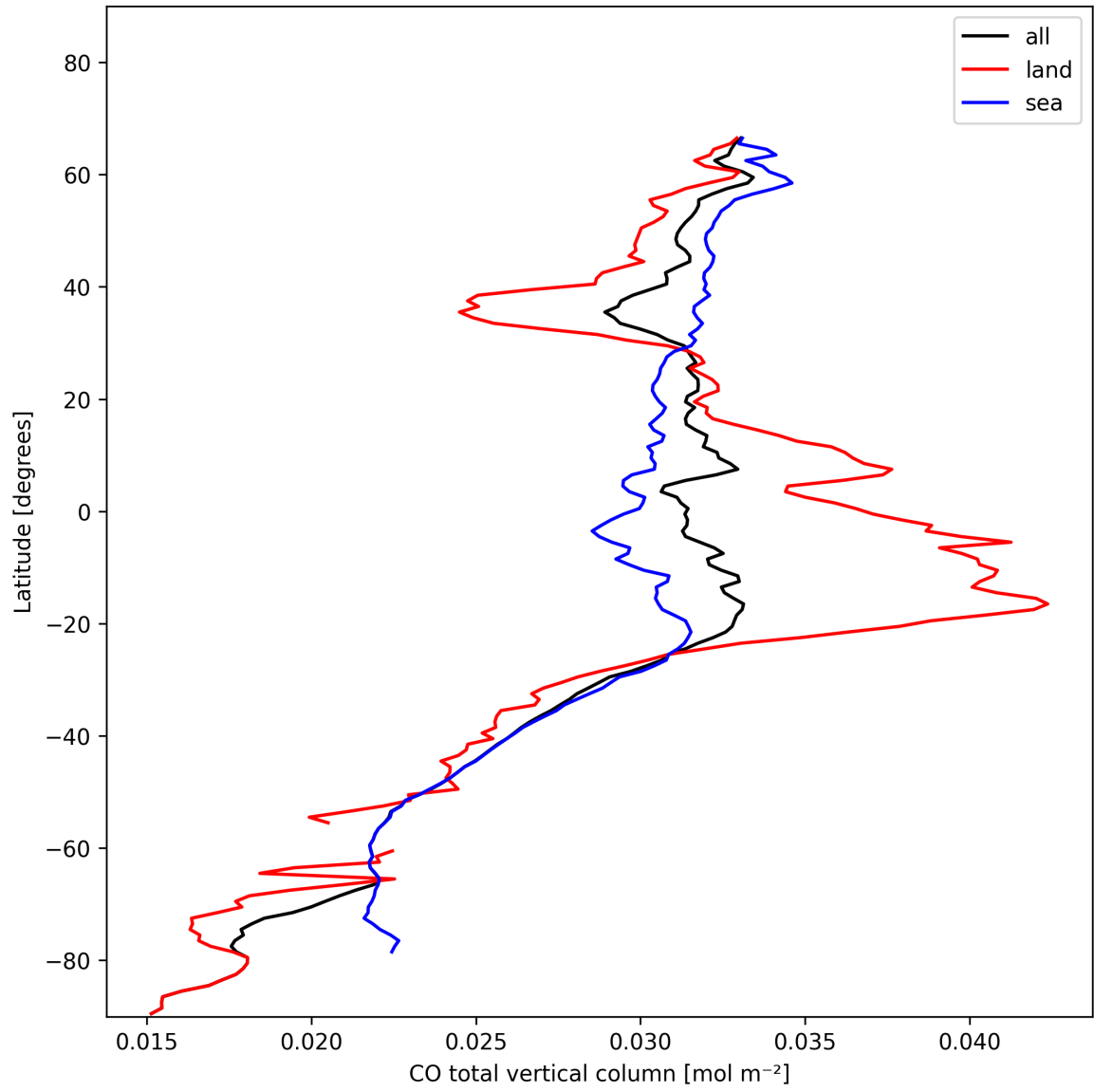
Figure 10: Zonal average of “CO total vertical column” for 2024-11-12 to 2024-11-14.
