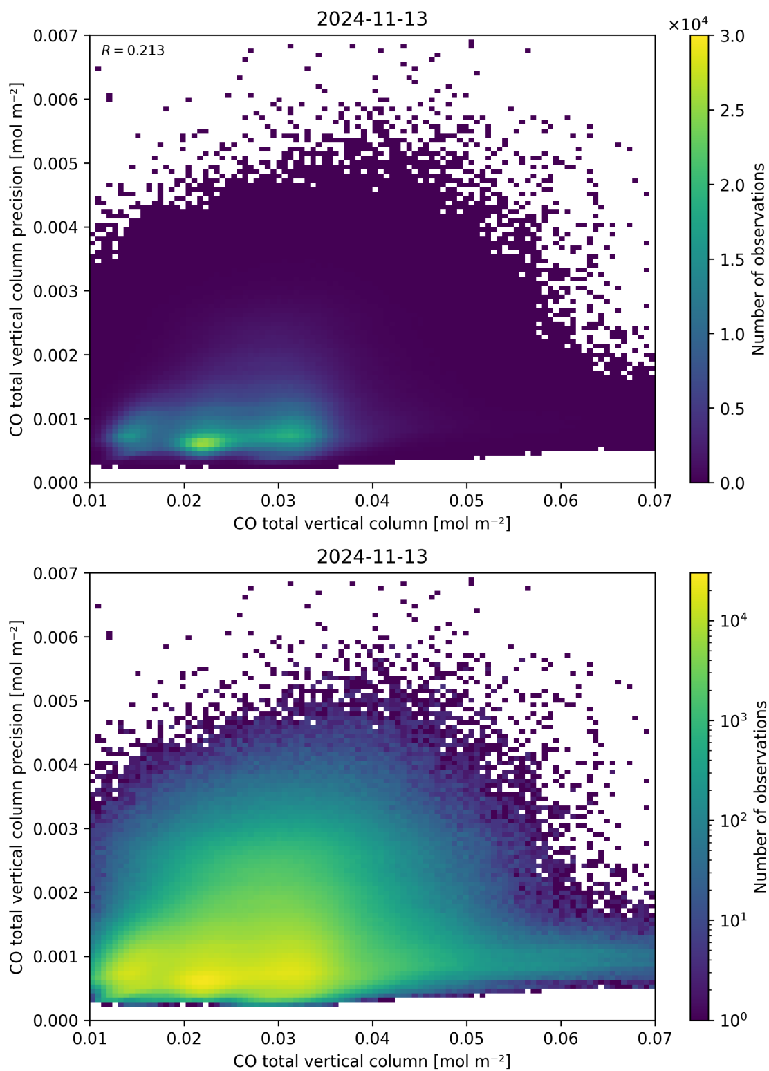
Figure 34: Scatter density plot of “CO total vertical column” against “CO total vertical column precision” for 2024-11-12 to 2024-11-14.
