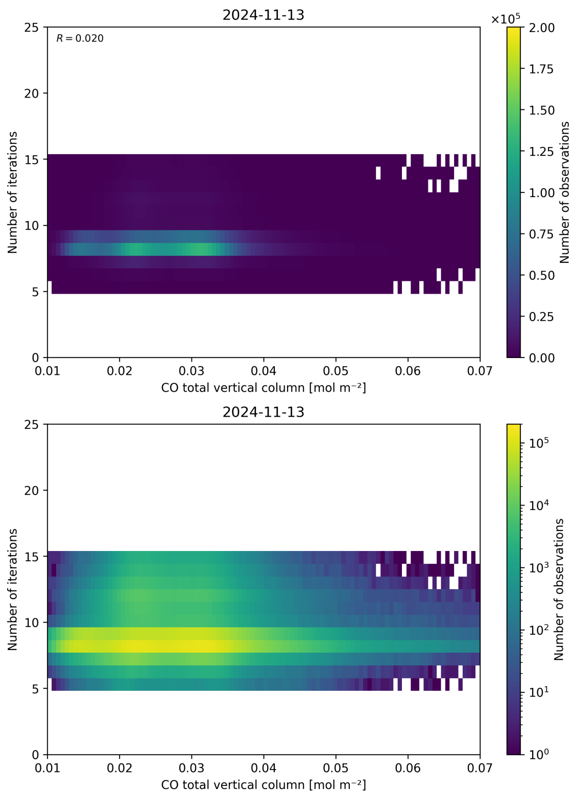
Figure 42: Scatter density plot of “CO total vertical column” against “Number of iterations” for 2024-11-12 to 2024-11-14.
