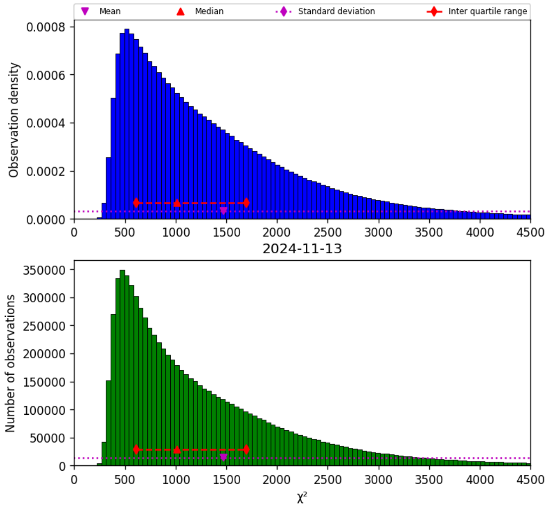
Figure 22: Histogram of “ \chi^2 ” for 2024-11-12 to 2024-11-14
