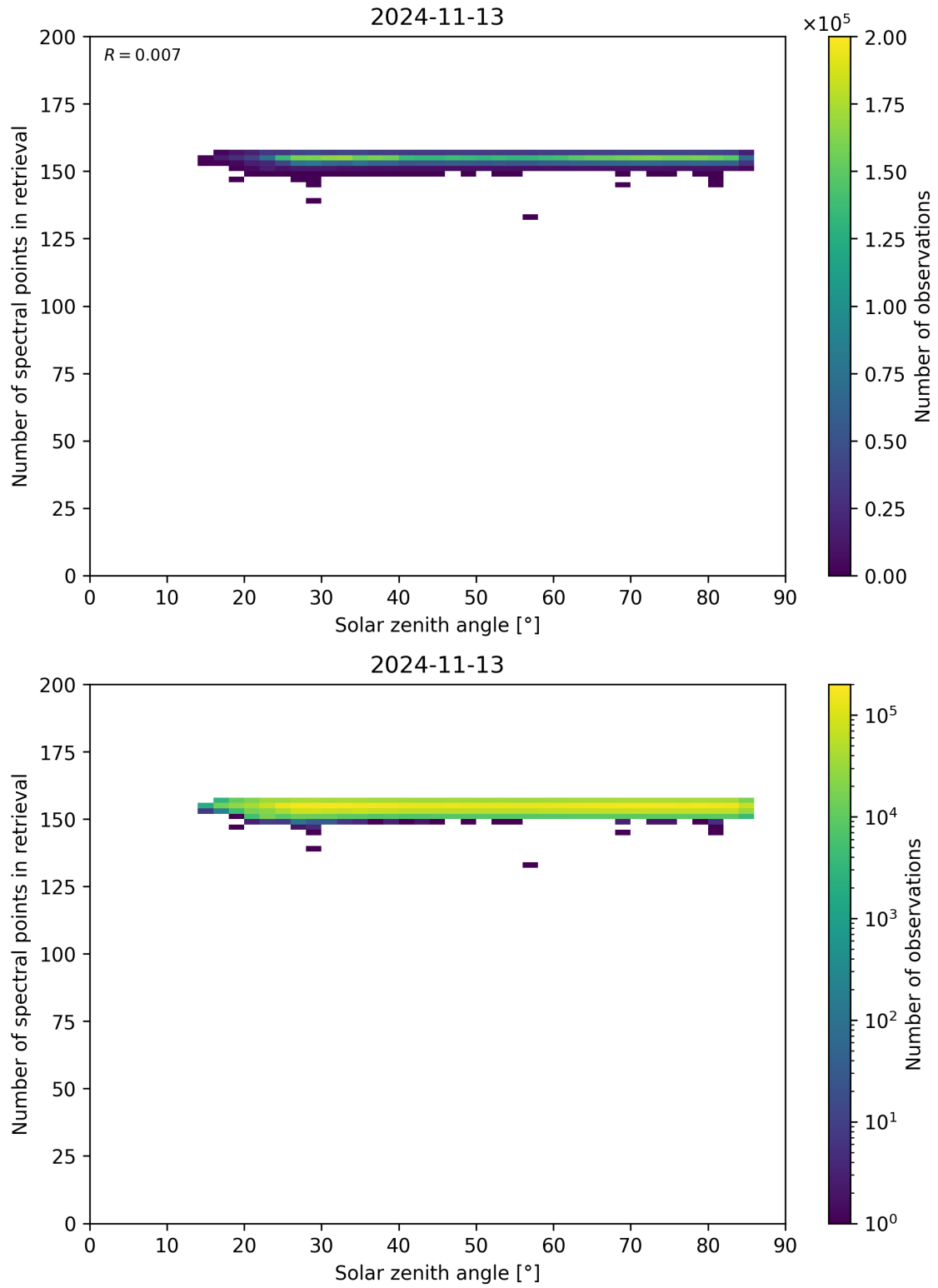
Figure 68: Scatter density plot of “Solar zenith angle” against “Number of spectral points in retrieval” for 2024-11-12 to 2024-11-14.
