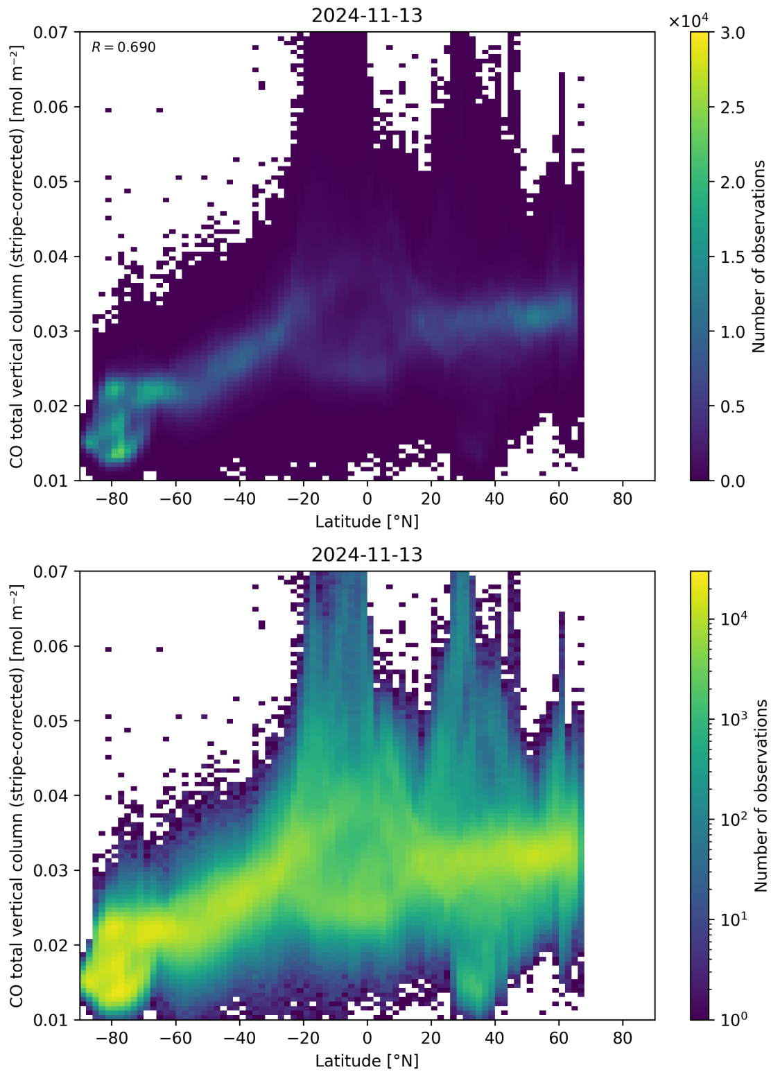
Figure 52: Scatter density plot of “Latitude” against “CO total vertical column (stripe-corrected)” for 2024-11-12 to 2024-11-14.
