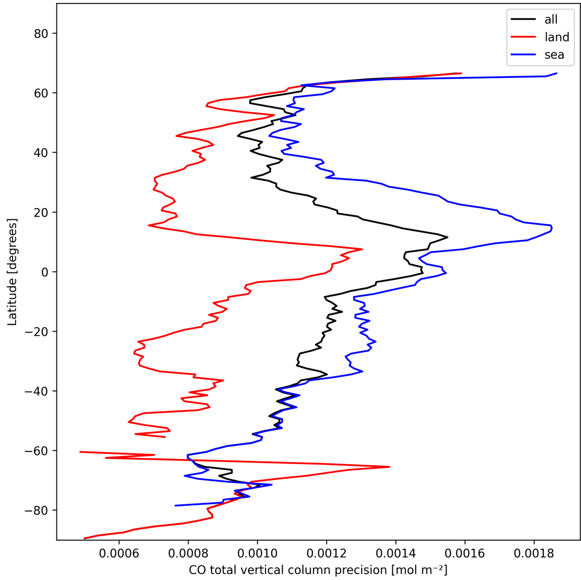
Figure 12: Zonal average of “CO total vertical column precision” for 2024-11-12 to 2024-11-14.
