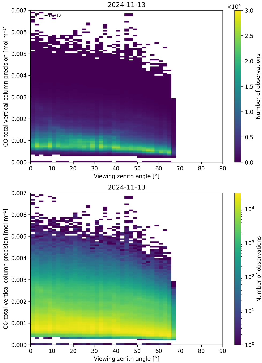
Figure 71: Scatter density plot of “Viewing zenith angle” against “CO total vertical column precision” for 2024-11-12 to 2024-11-14.
