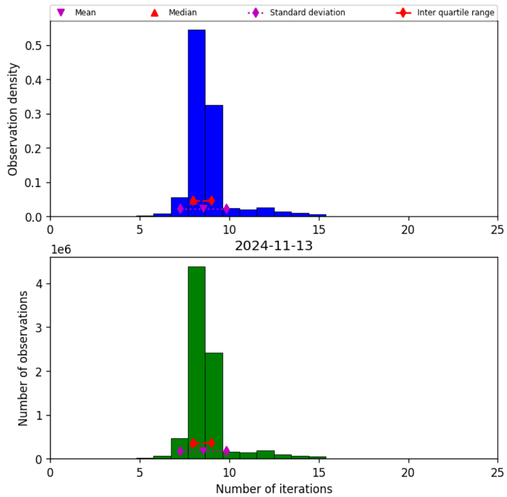
Figure 24: Histogram of “Number of iterations” for 2024-11-12 to 2024-11-14
