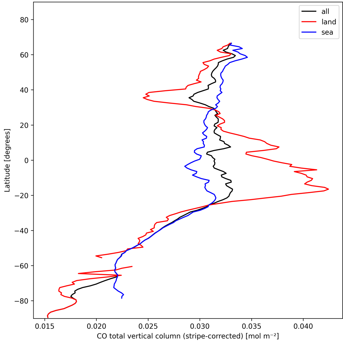
Figure 11: Zonal average of “CO total vertical column (stripe-corrected)” for 2024-11-12 to 2024-11-14.
