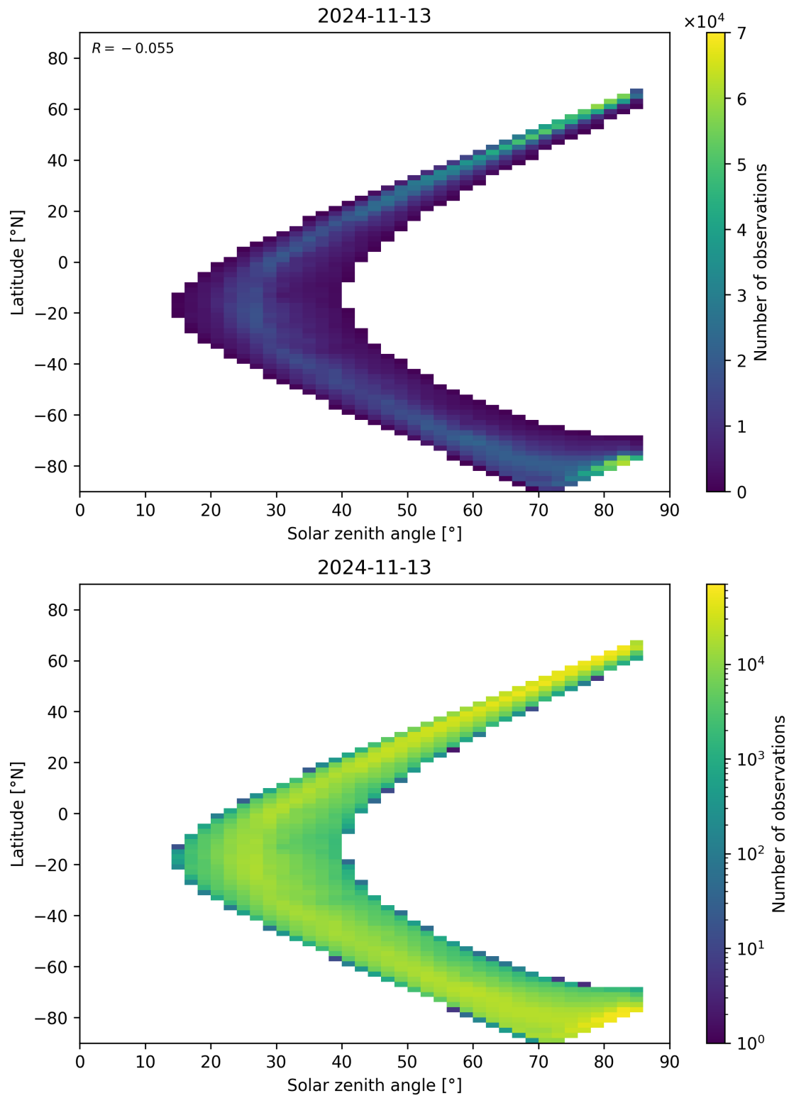
Figure 66: Scatter density plot of “Solar zenith angle” against “Latitude” for 2024-11-12 to 2024-11-14.
