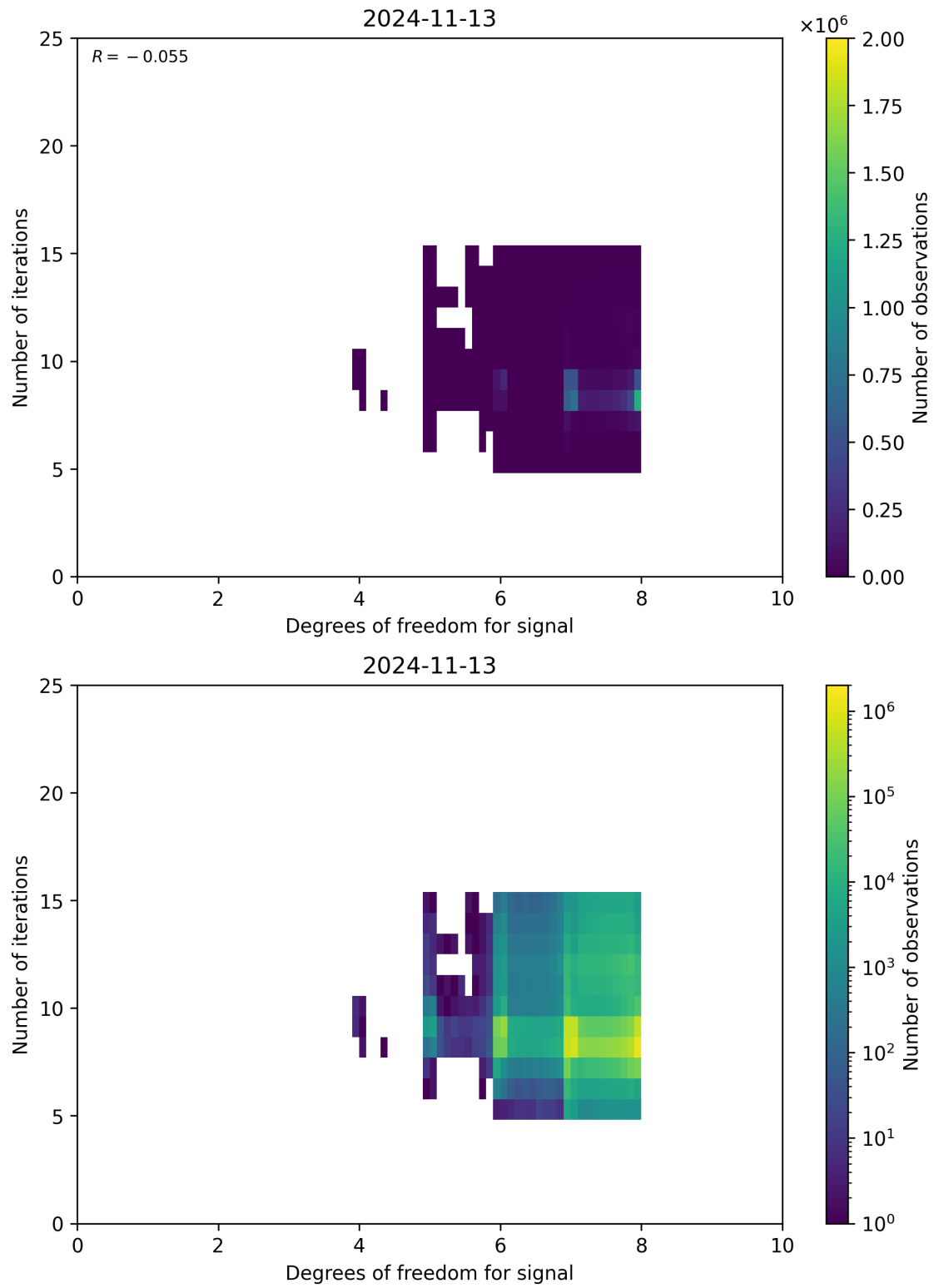
Figure 50: Scatter density plot of “Degrees of freedom for signal” against “Number of iterations” for 2024-11-12 to 2024-11-14.
