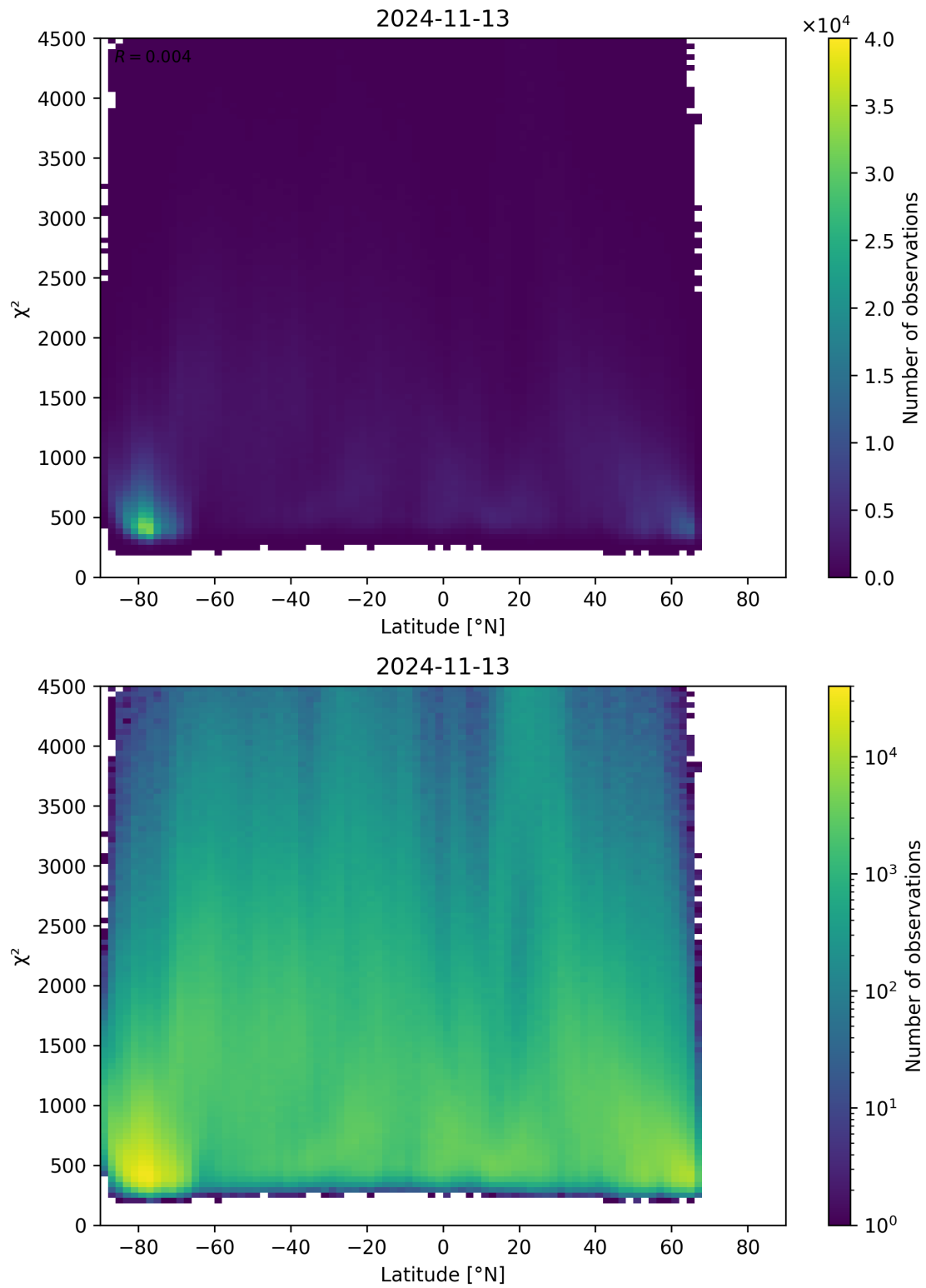
Figure 54: Scatter density plot of “Latitude” against “ \chi^2 ” for 2024-11-12 to 2024-11-14.
