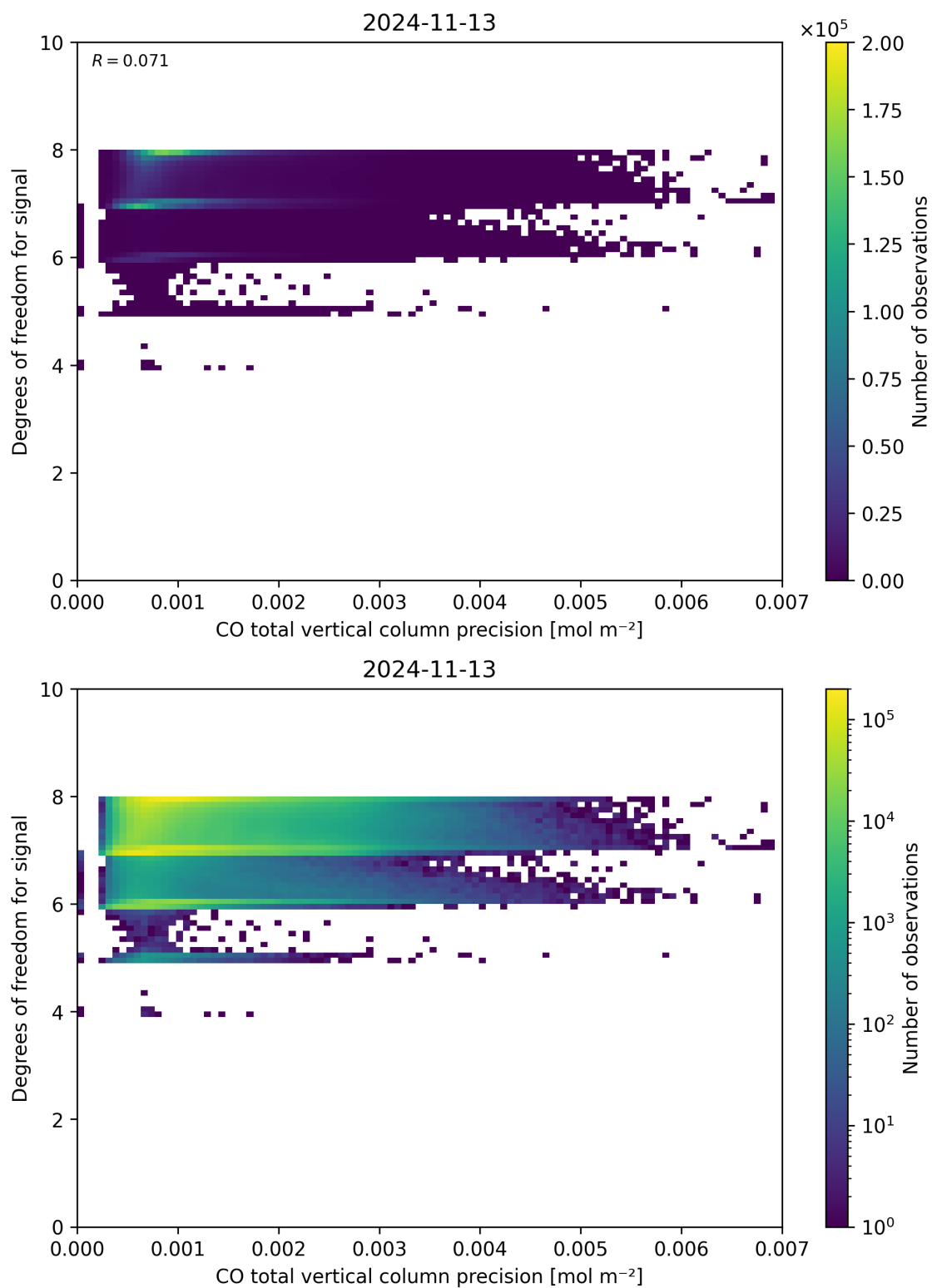
Figure 45: Scatter density plot of “CO total vertical column precision” against “Degrees of freedom for signal” for 2024-11-12 to 2024-11-14.
