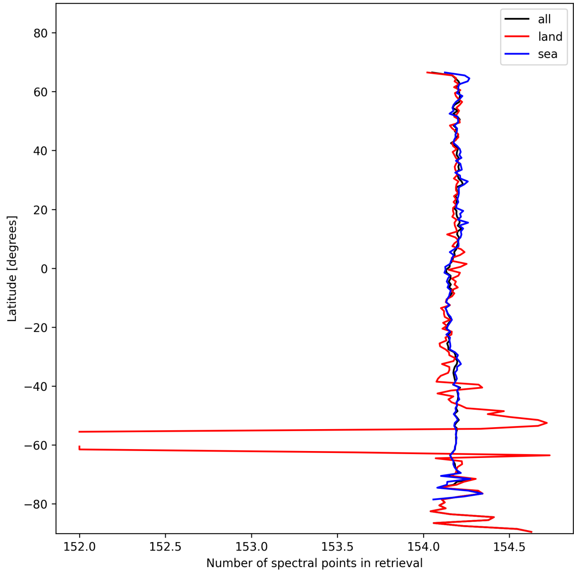
Figure 13: Zonal average of “Number of spectral points in retrieval” for 2024-11-12 to 2024-11-14.
