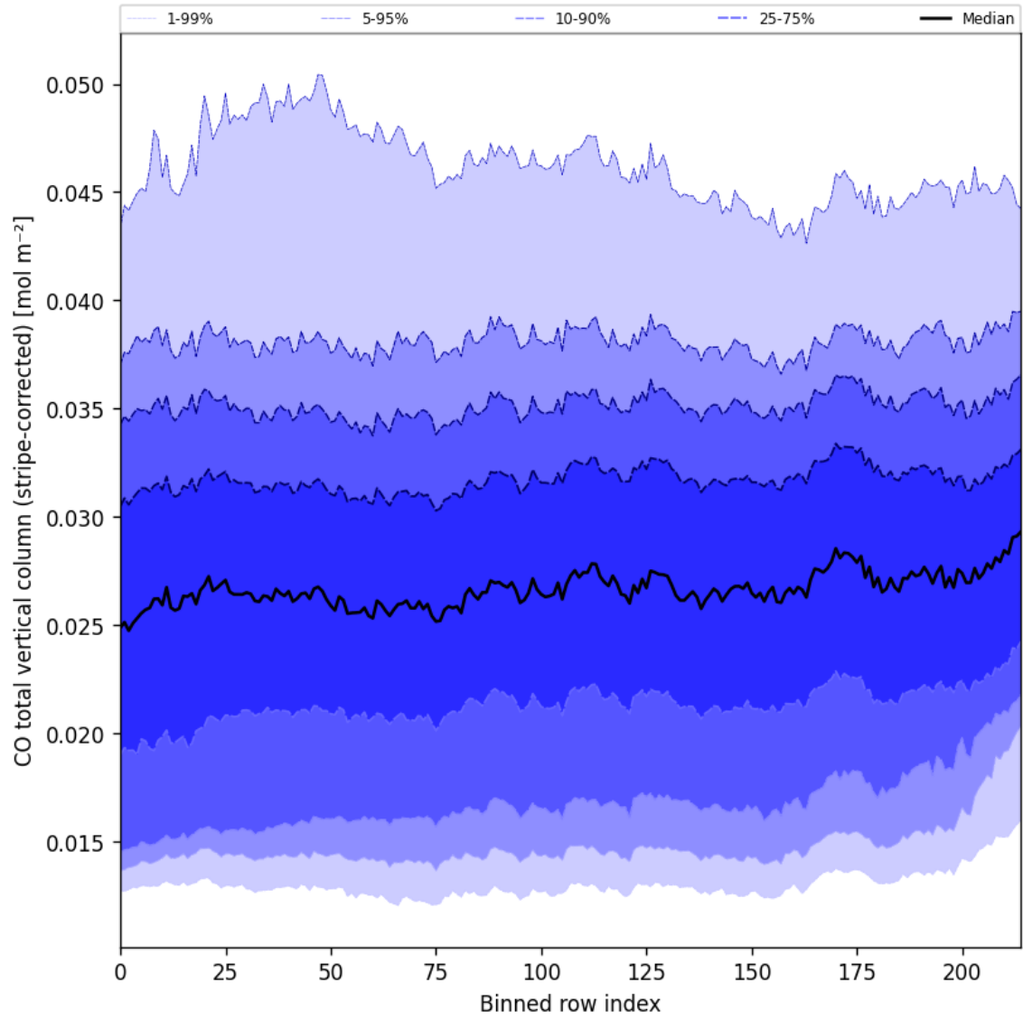
Figure 27: Along track statistics of “CO total vertical column (stripe-corrected)” for 2024-11-12 to 2024-11-14
