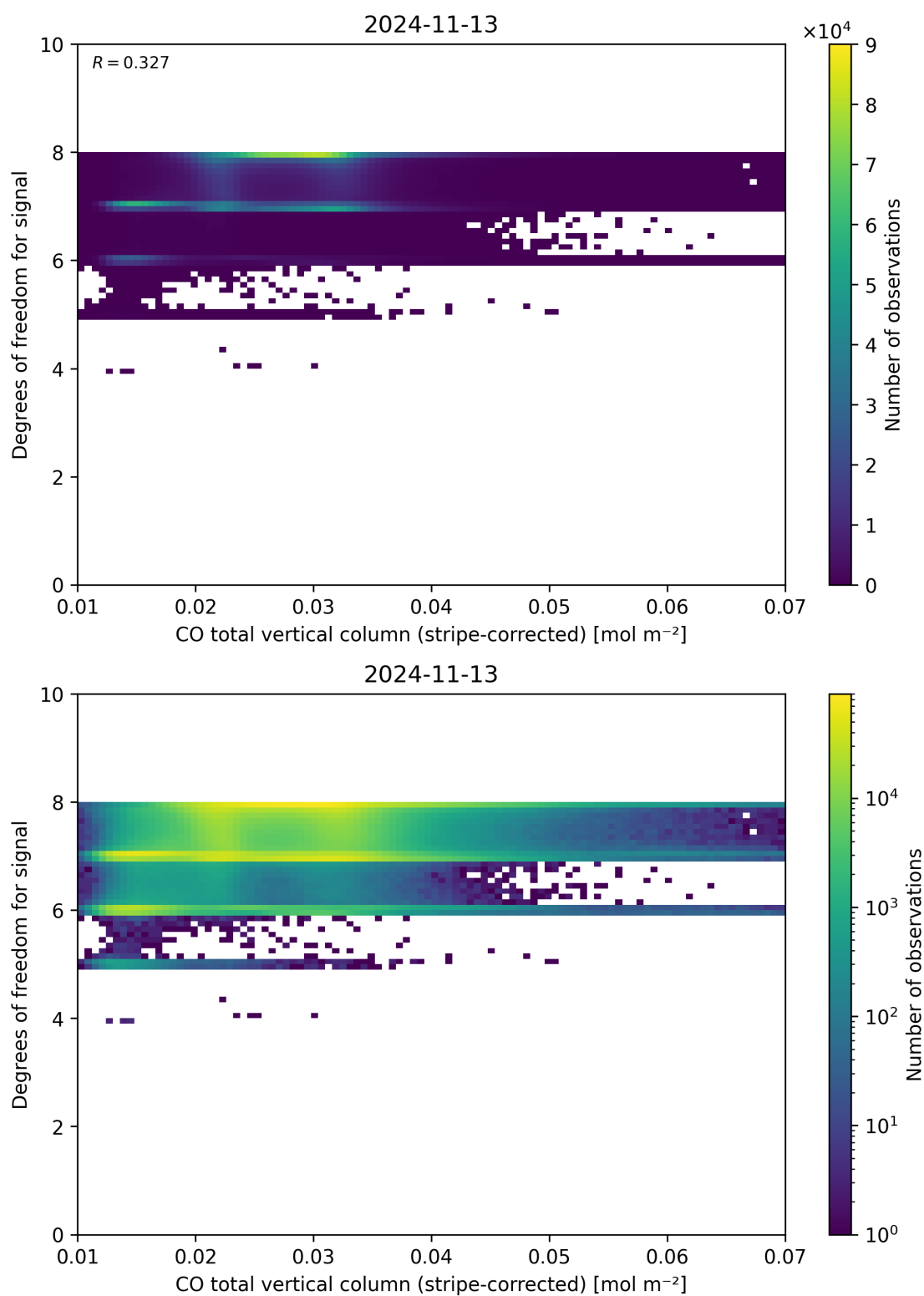
Figure 38: Scatter density plot of “CO total vertical column (stripe-corrected)” against “Degrees of freedom for signal” for 2024-11-12 to 2024-11-14.
