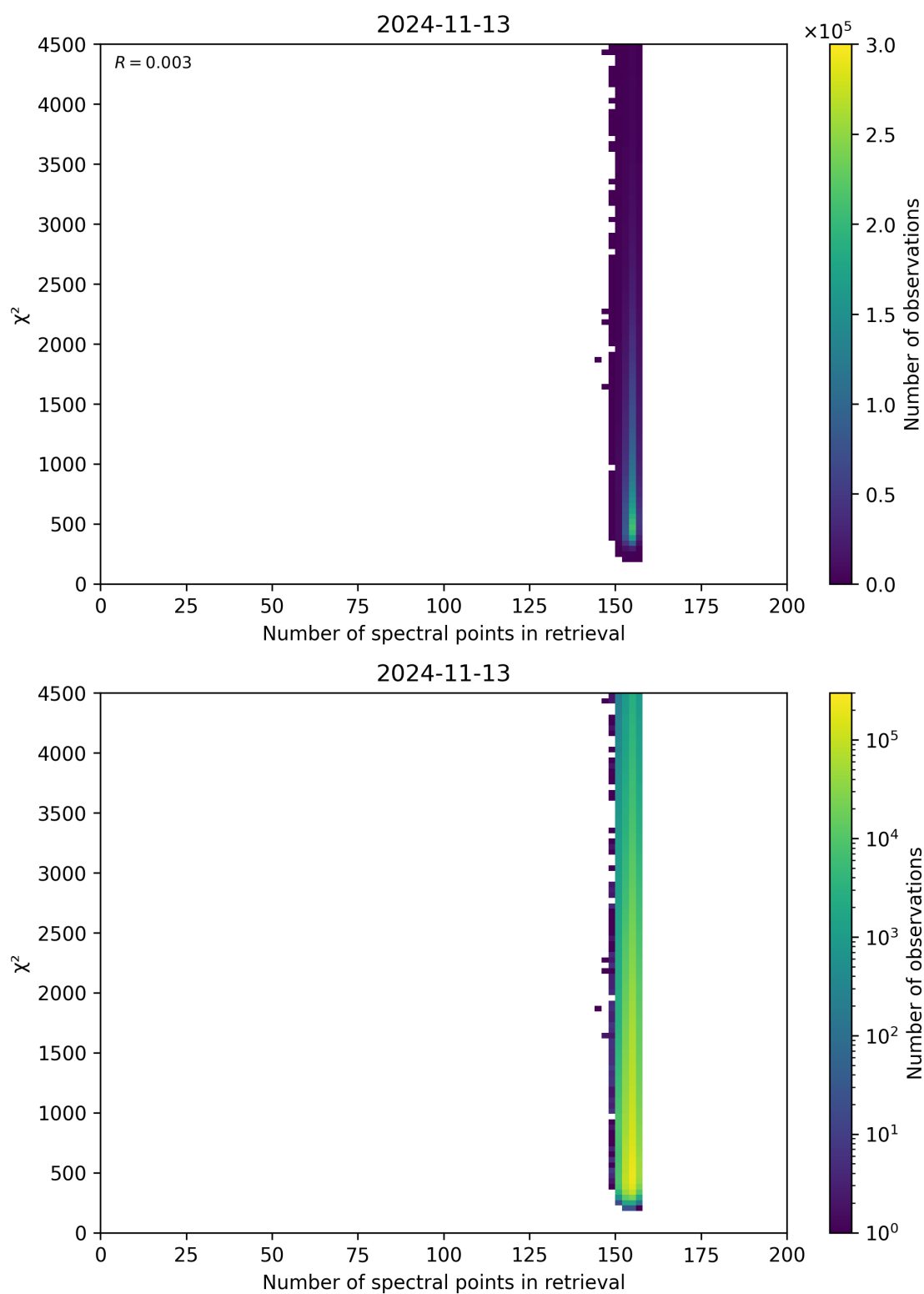
Figure 58: Scatter density plot of “Number of spectral points in retrieval” against “ \chi^2 ” for 2024-11-12 to 2024-11-14.
