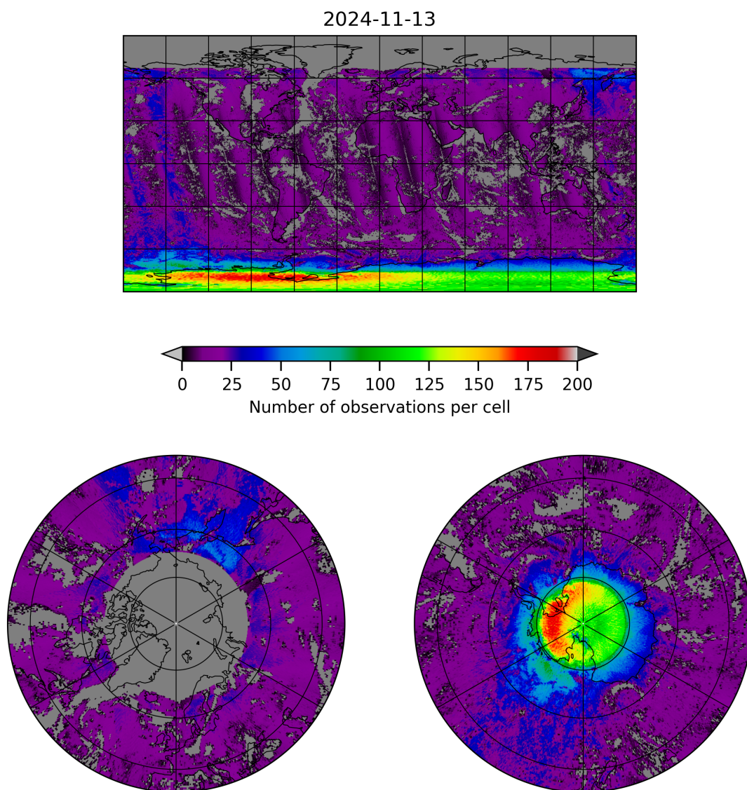
Figure 8: Map of the number of observations for 2024-11-12 to 2024-11-14
