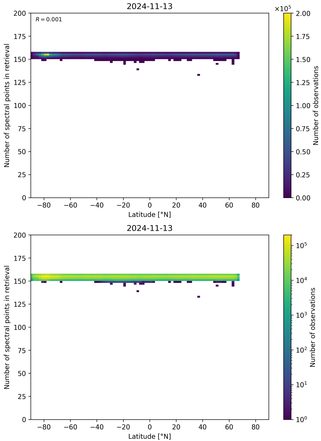
Figure 57: Scatter density plot of “Latitude” against “Number of spectral points in retrieval” for 2024-11-12 to 2024-11-14.
