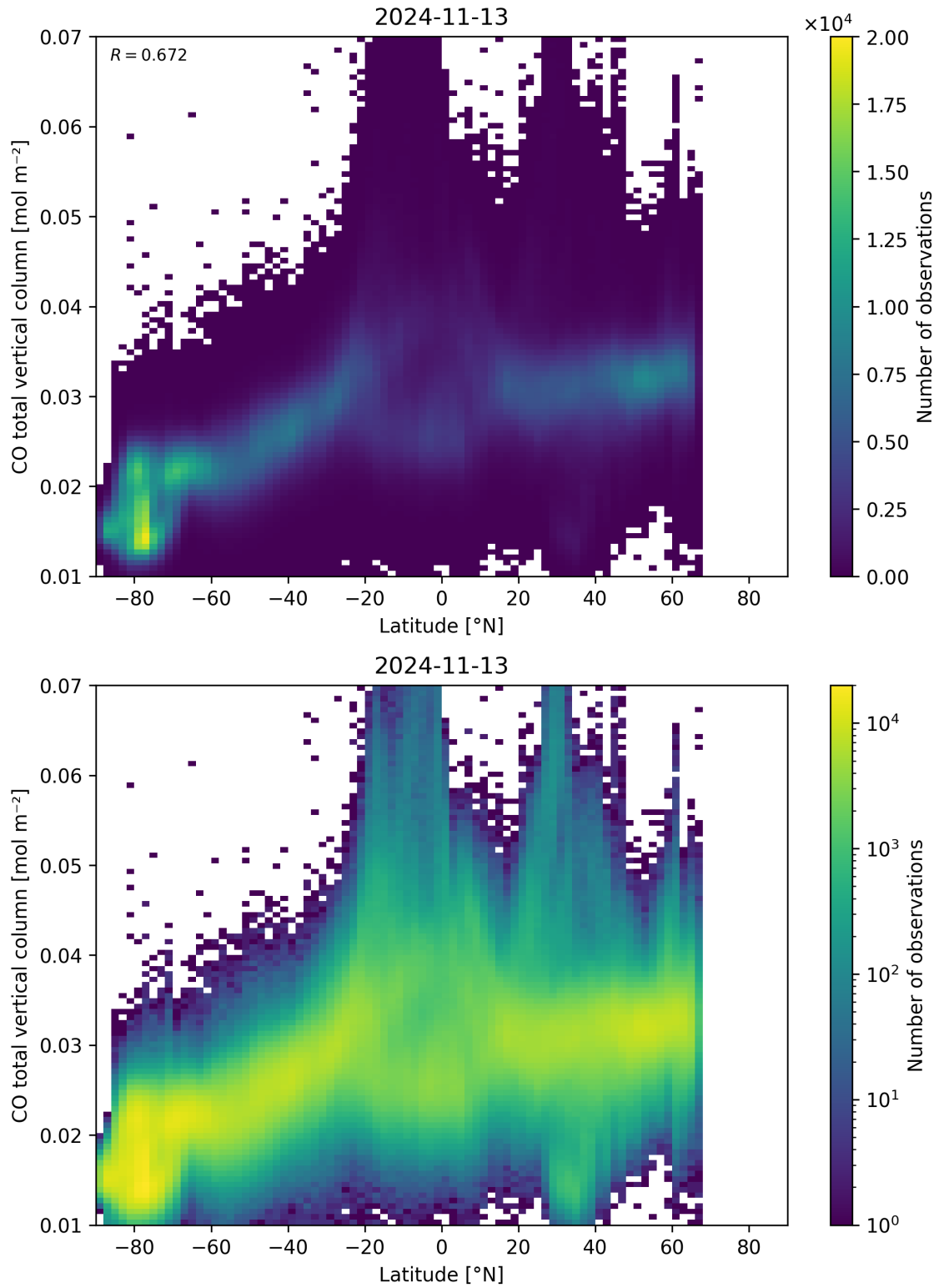
Figure 51: Scatter density plot of “Latitude” against “CO total vertical column” for 2024-11-12 to 2024-11-14.
