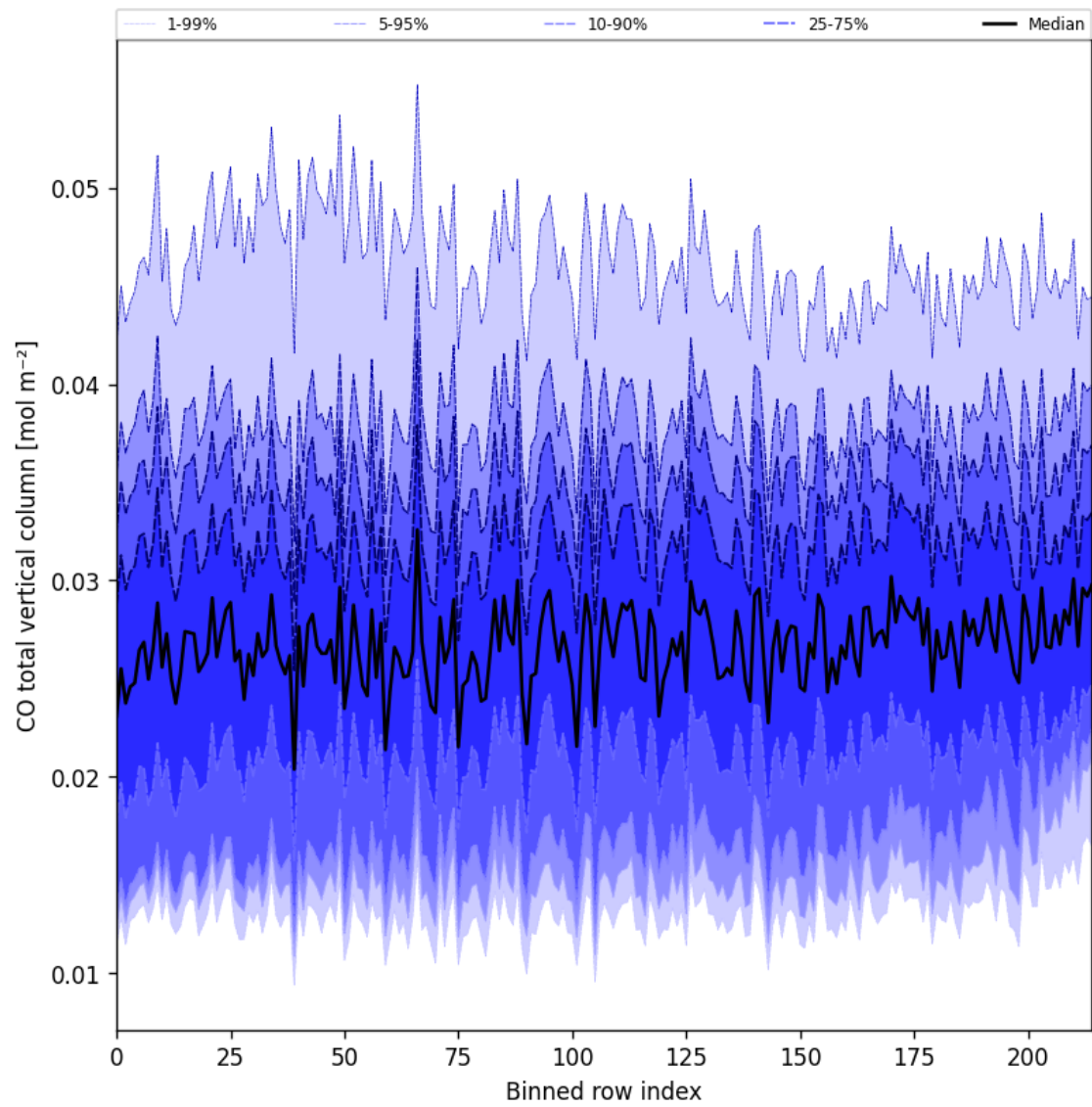
Figure 26: Along track statistics of "CO total vertical column" for 2024-11-12 to 2024-11-14
