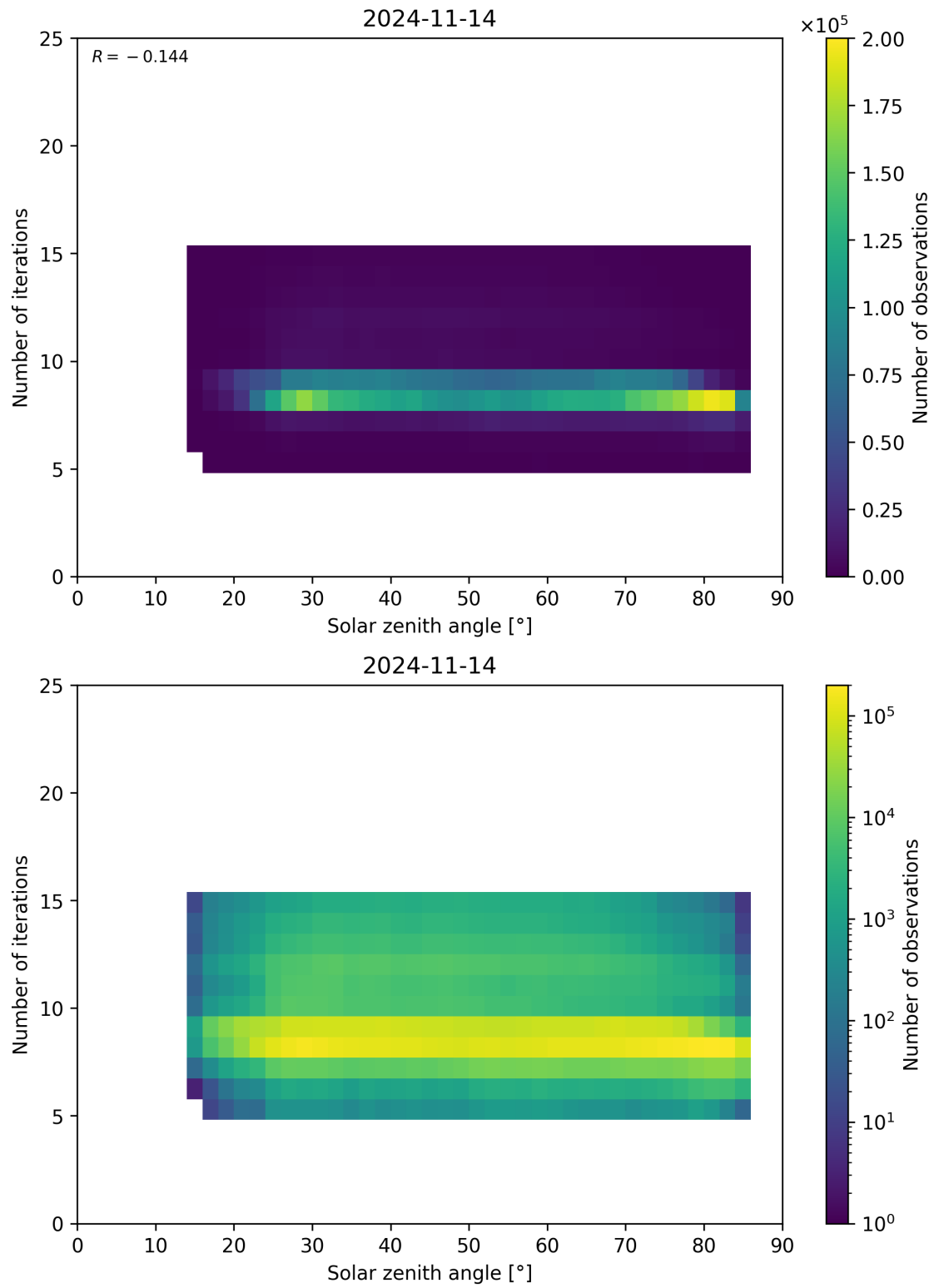
Figure 67: Scatter density plot of “Solar zenith angle” against “Number of iterations” for 2024-11-14 to 2024-11-15.
