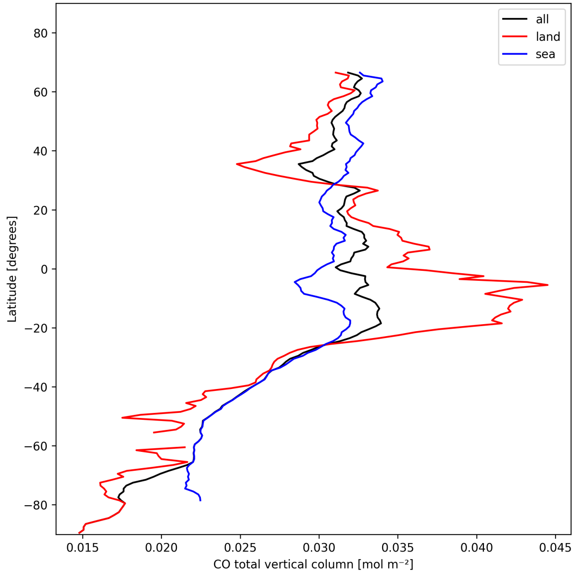
Figure 10: Zonal average of “CO total vertical column” for 2024-11-14 to 2024-11-15.
