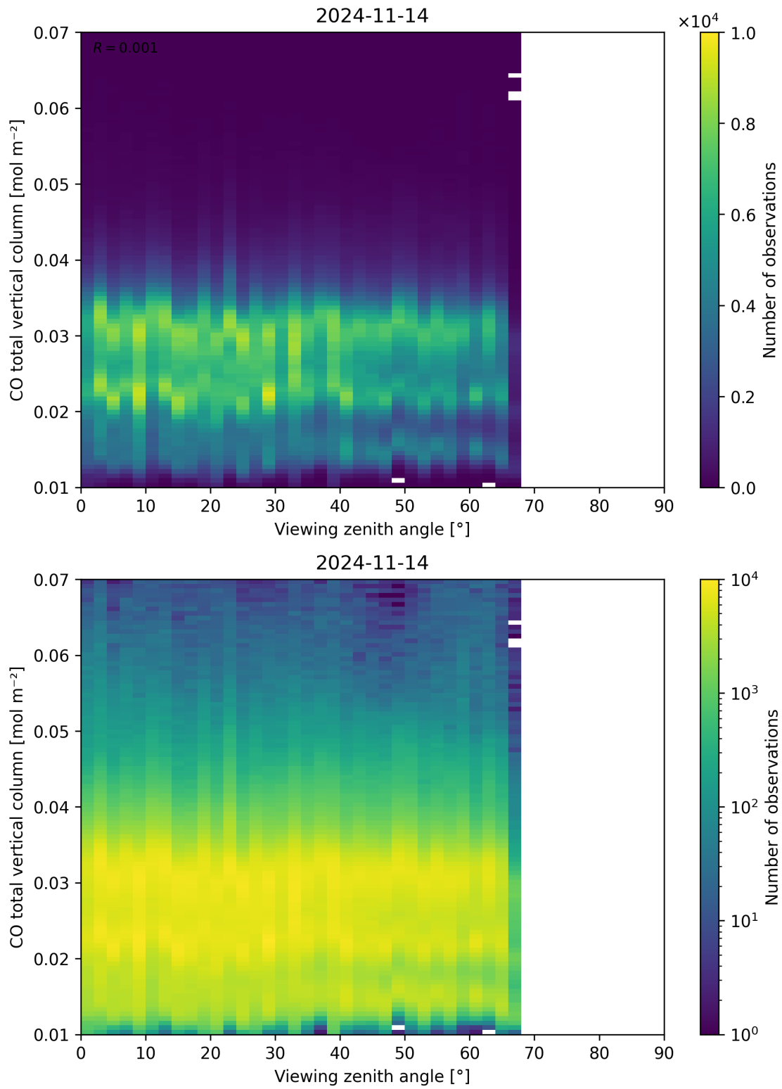
Figure 69: Scatter density plot of “Viewing zenith angle” against “CO total vertical column” for 2024-11-14 to 2024-11-15.
