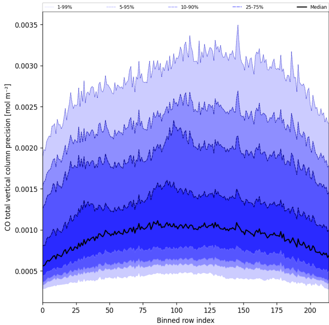
Figure 28: Along track statistics of “CO total vertical column precision” for 2024-11-14 to 2024-11-15
