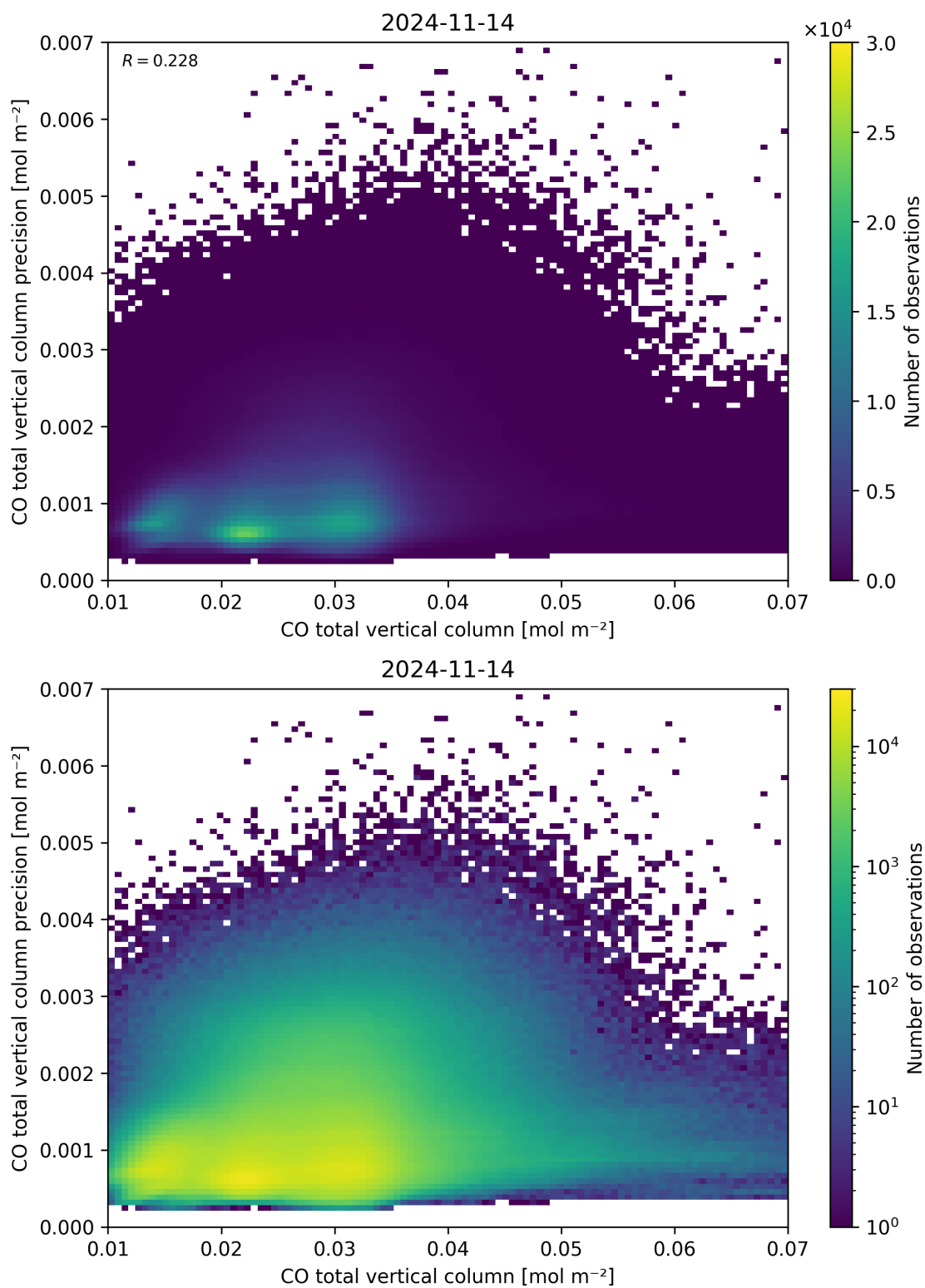
Figure 34: Scatter density plot of “CO total vertical column” against “CO total vertical column precision” for 2024-11-14 to 2024-11-15.
