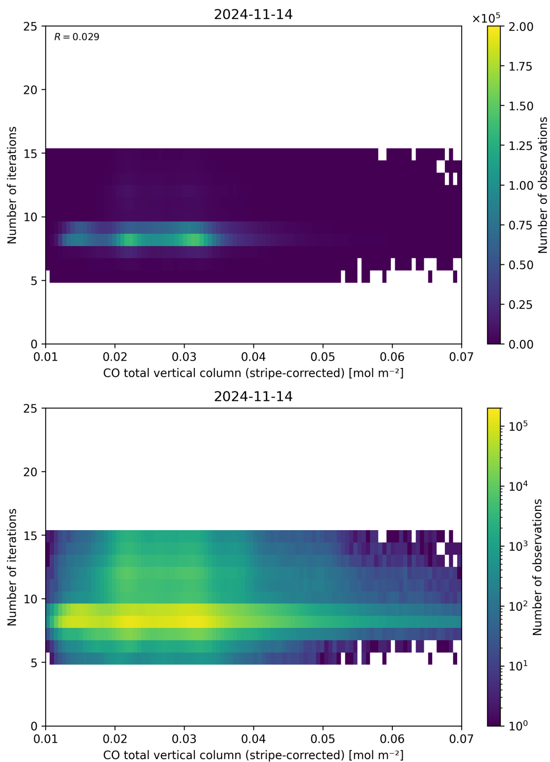
Figure 39: Scatter density plot of “CO total vertical column (stripe-corrected)” against “Number of iterations” for 2024-11-14 to 2024-11-15.
