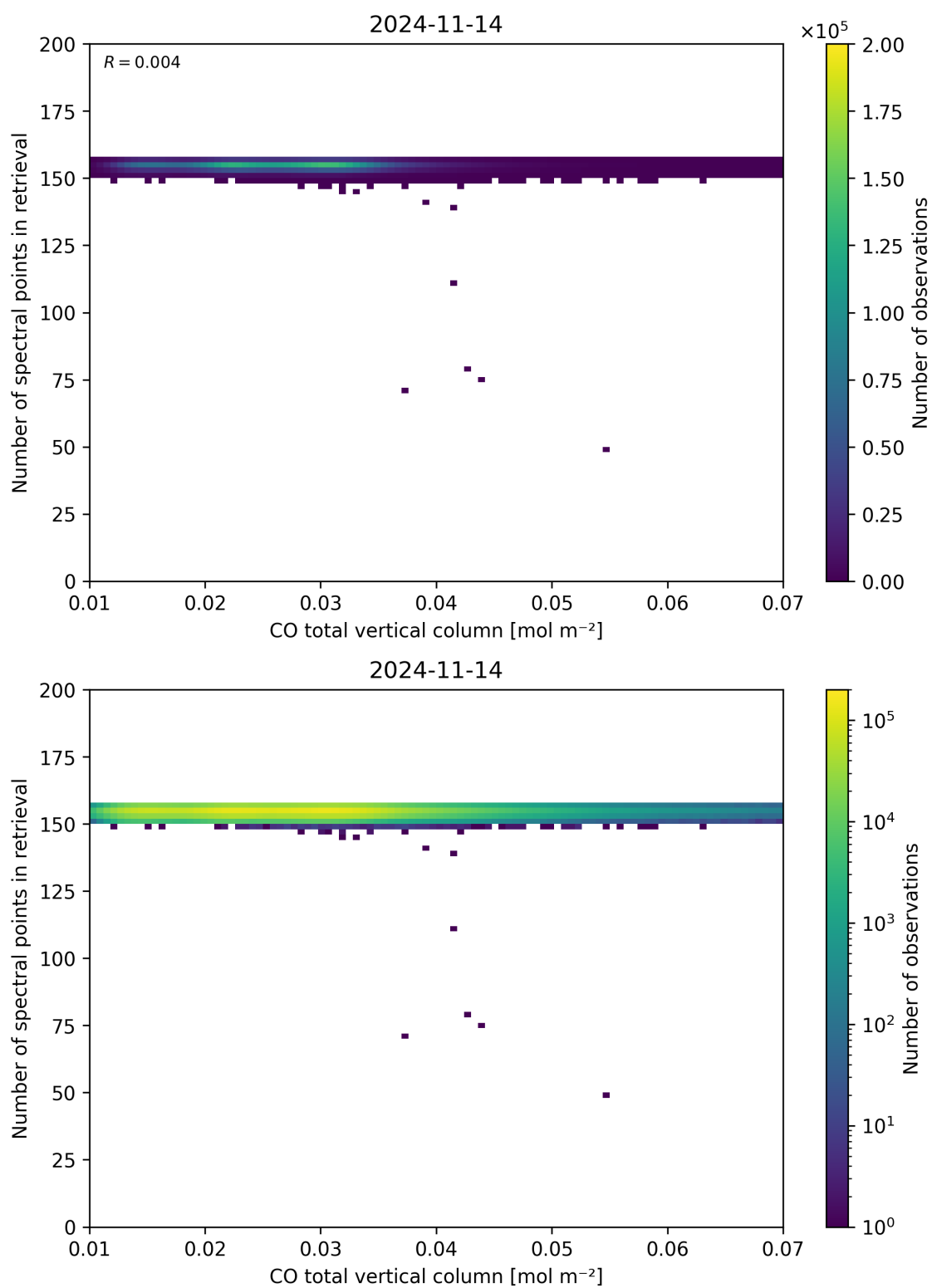
Figure 43: Scatter density plot of “CO total vertical column” against “Number of spectral points in retrieval” for 2024-11-14 to 2024-11-15.
