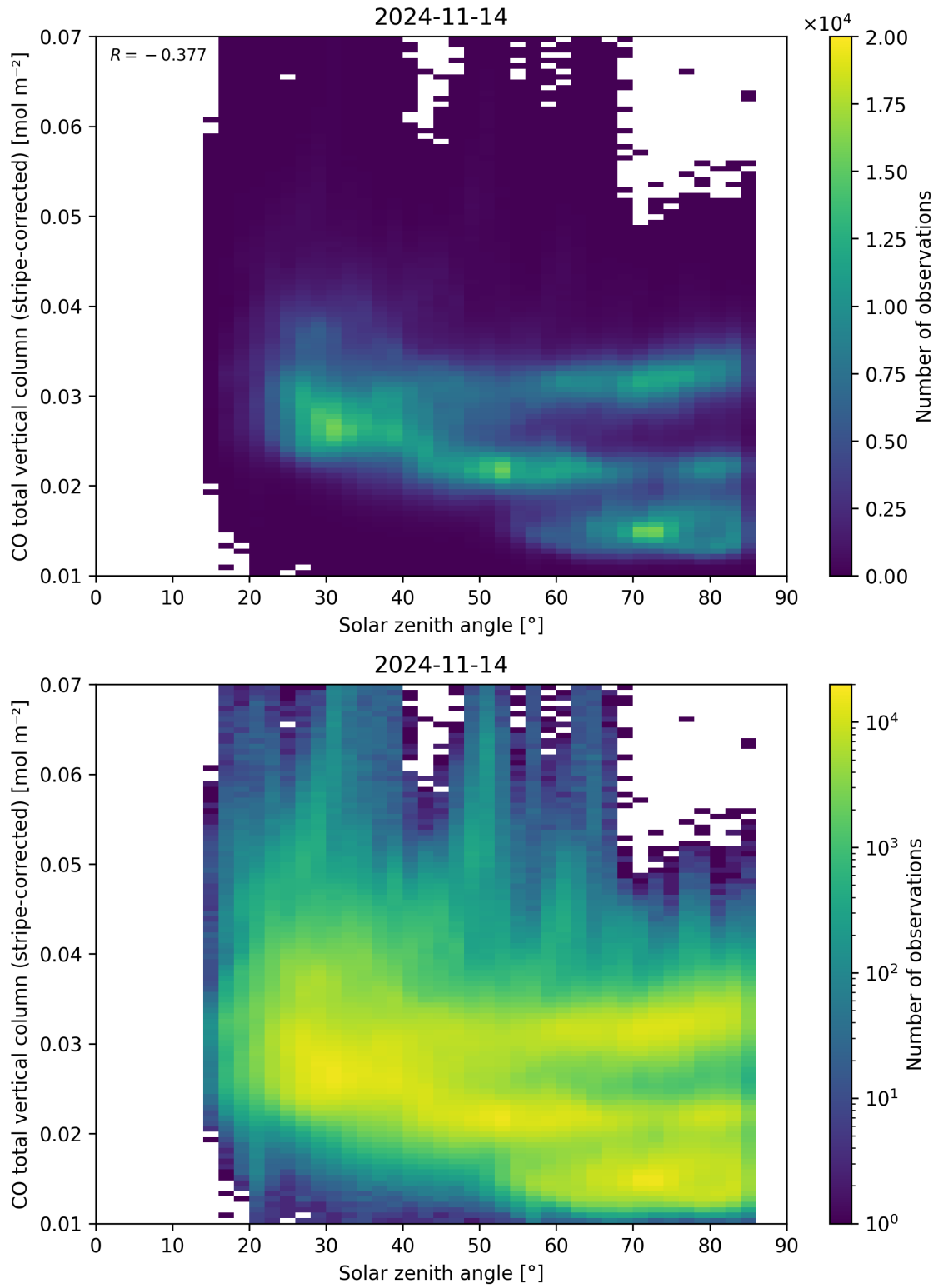
Figure 62: Scatter density plot of “Solar zenith angle” against “CO total vertical column (stripe-corrected)” for 2024-11-14 to 2024-11-15.
