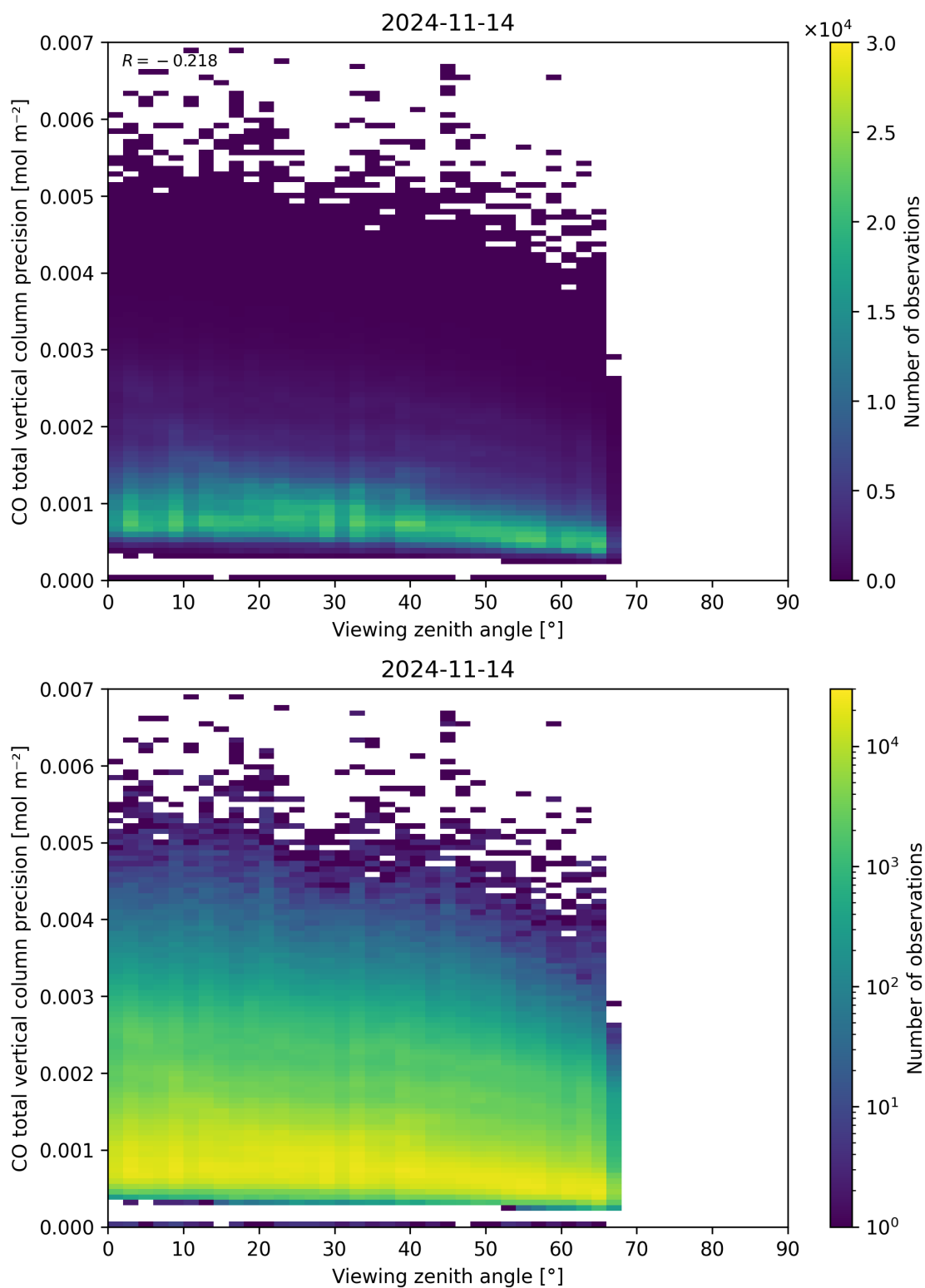
Figure 71: Scatter density plot of “Viewing zenith angle” against “CO total vertical column precision” for 2024-11-14 to 2024-11-15.
