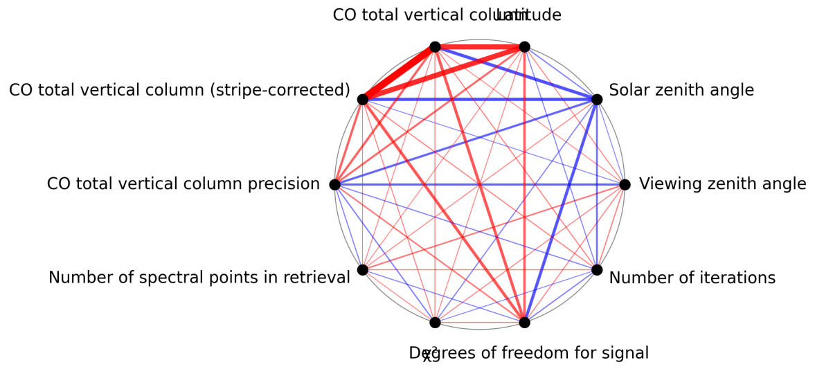
Figure 1: Map of correlation graph for 2024-11-14 to 2024-11-15.
