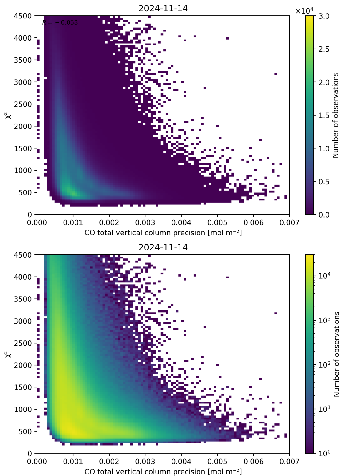
Figure 44: Scatter density plot of “CO total vertical column precision” against “ \chi^2 ” for 2024-11-14 to 2024-11-15.
