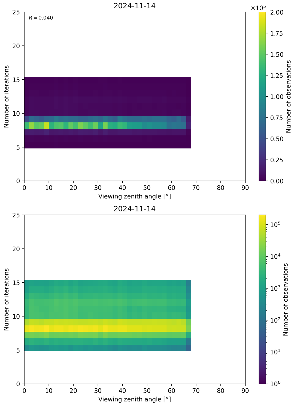
Figure 75: Scatter density plot of “Viewing zenith angle” against “Number of iterations” for 2024-11-14 to 2024-11-15.
