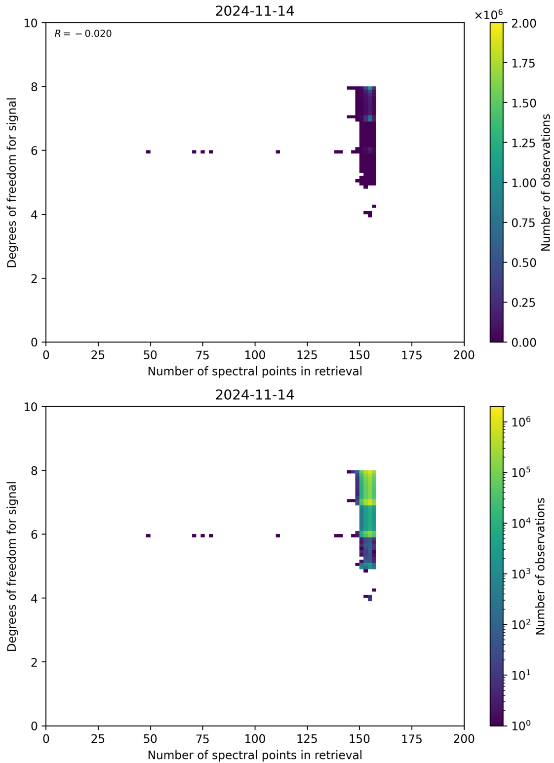
Figure 59: Scatter density plot of “Number of spectral points in retrieval” against “Degrees of freedom for signal” for 2024-11-14 to 2024-11-15.
