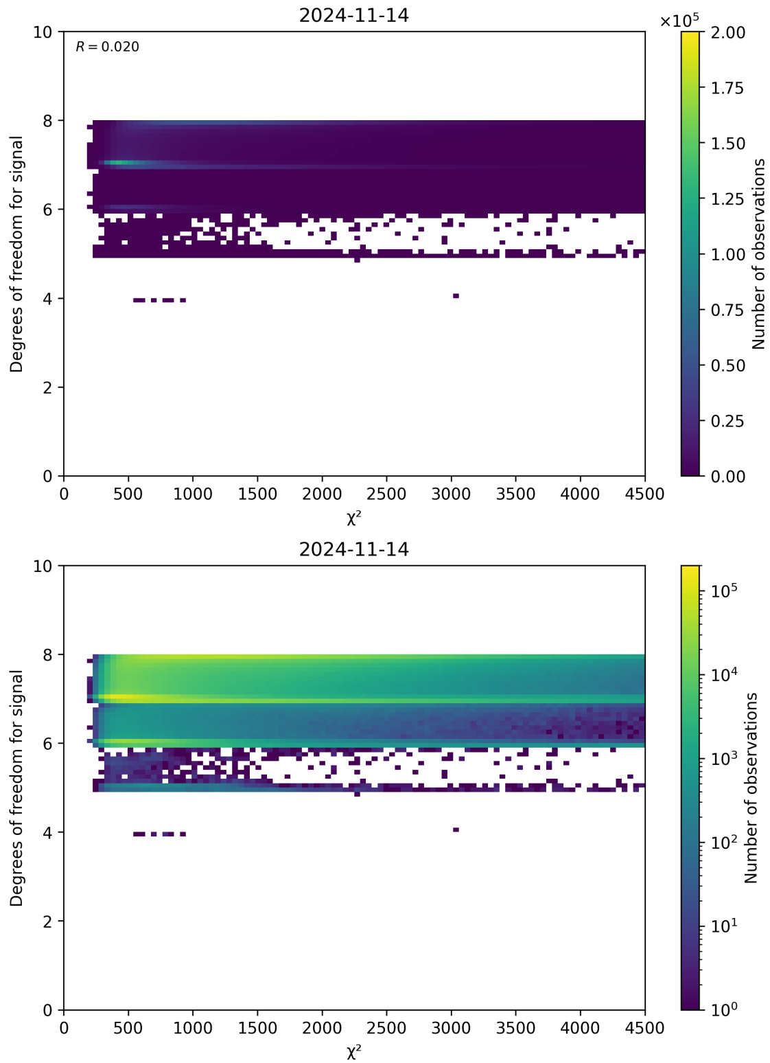
Figure 48: Scatter density plot of “ \chi^2 ” against “Degrees of freedom for signal” for 2024-11-14 to 2024-11-15.
