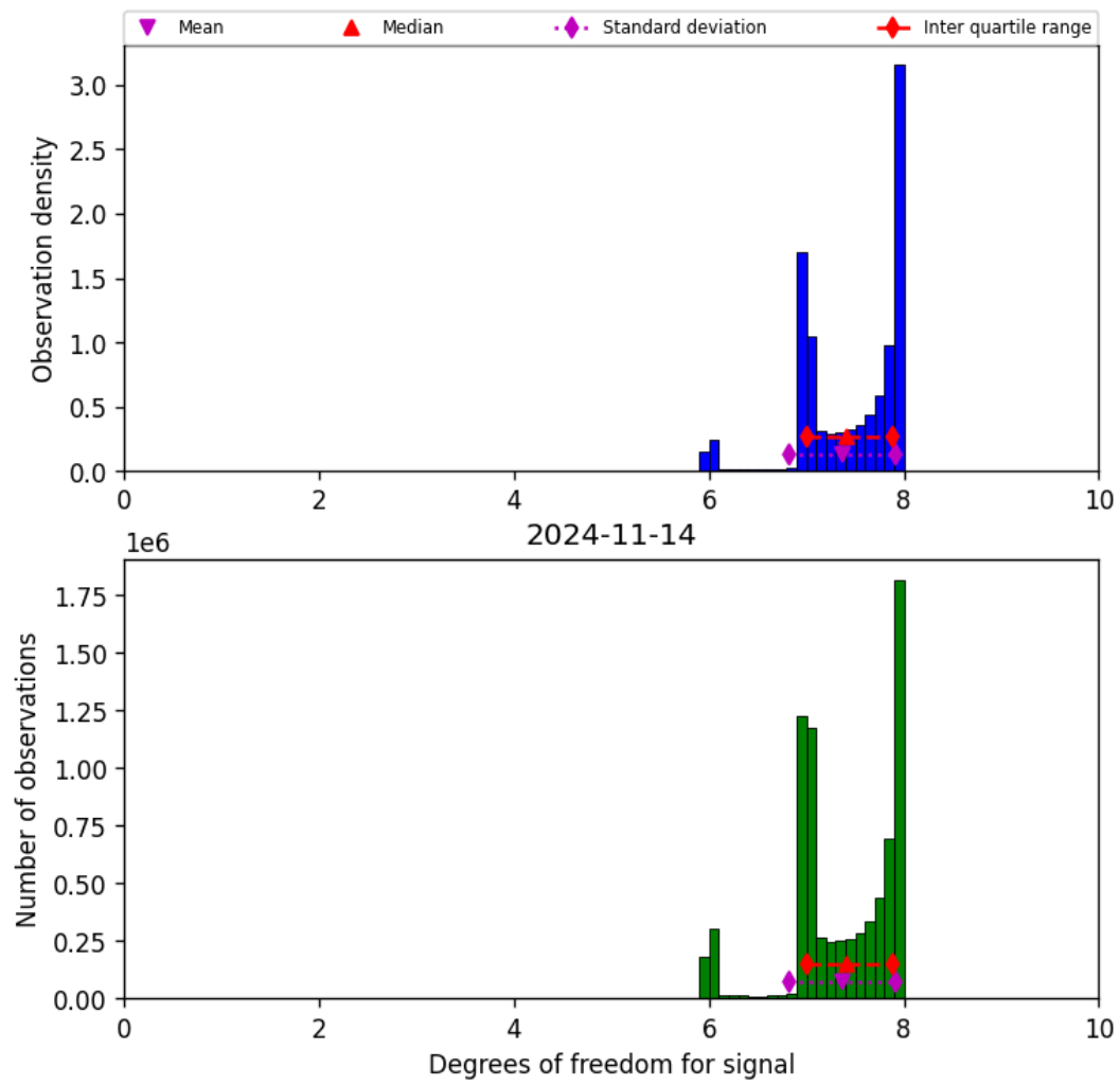
Figure 23: Histogram of “Degrees of freedom for signal” for 2024-11-14 to 2024-11-15
