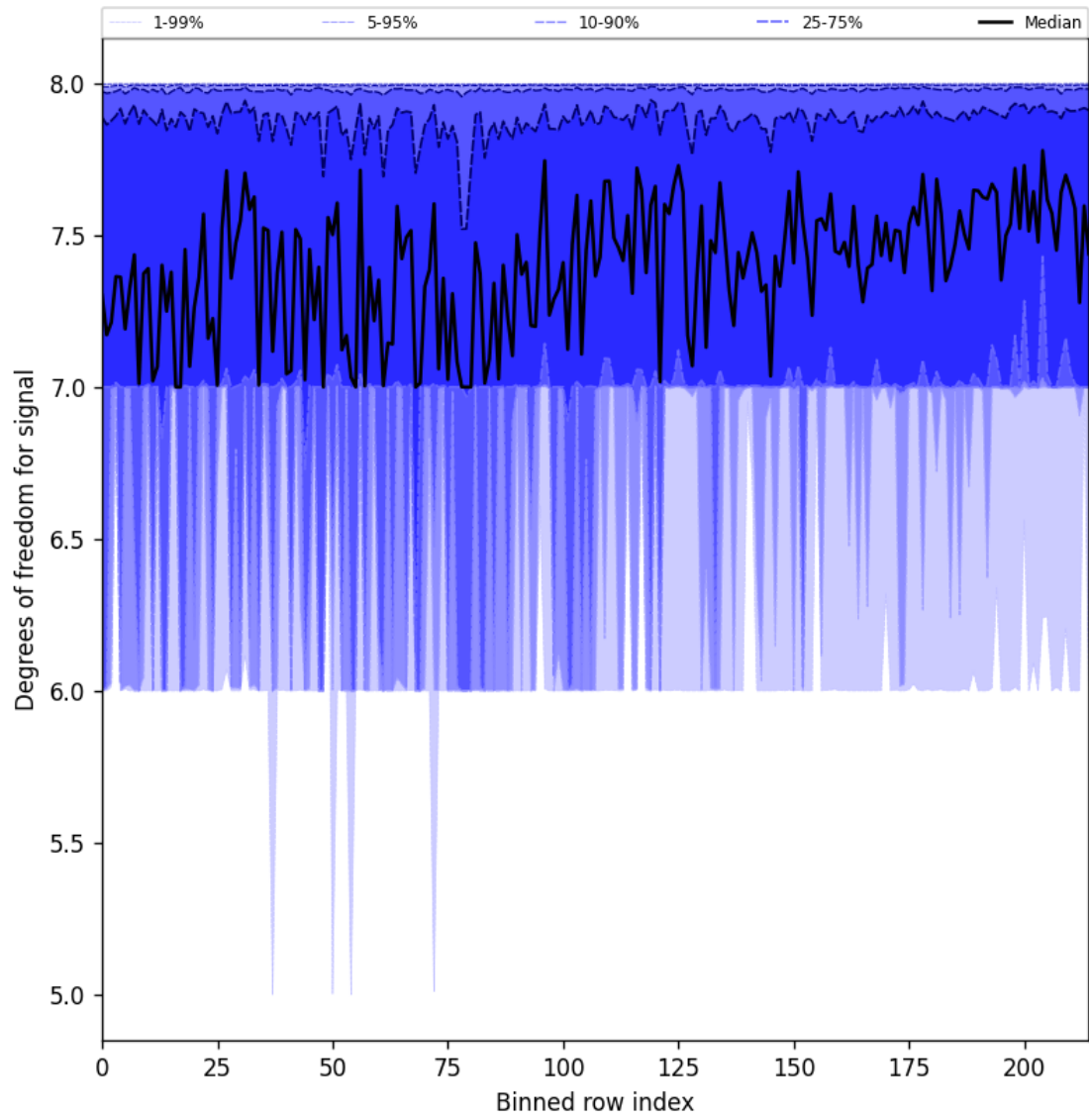
Figure 31: Along track statistics of “Degrees of freedom for signal” for 2024-11-14 to 2024-11-15
