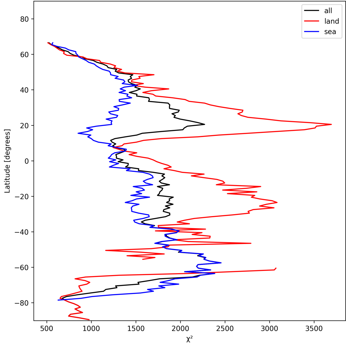
Figure 14: Zonal average of “ \chi^2 ” for 2024-11-14 to 2024-11-15.
