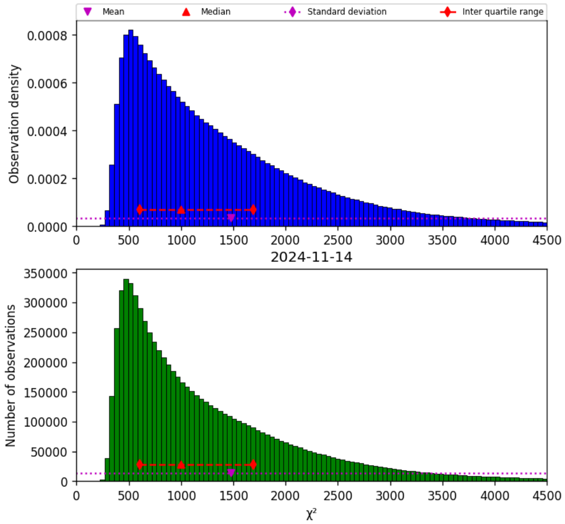
Figure 22: Histogram of “ \chi^2 ” for 2024-11-14 to 2024-11-15
