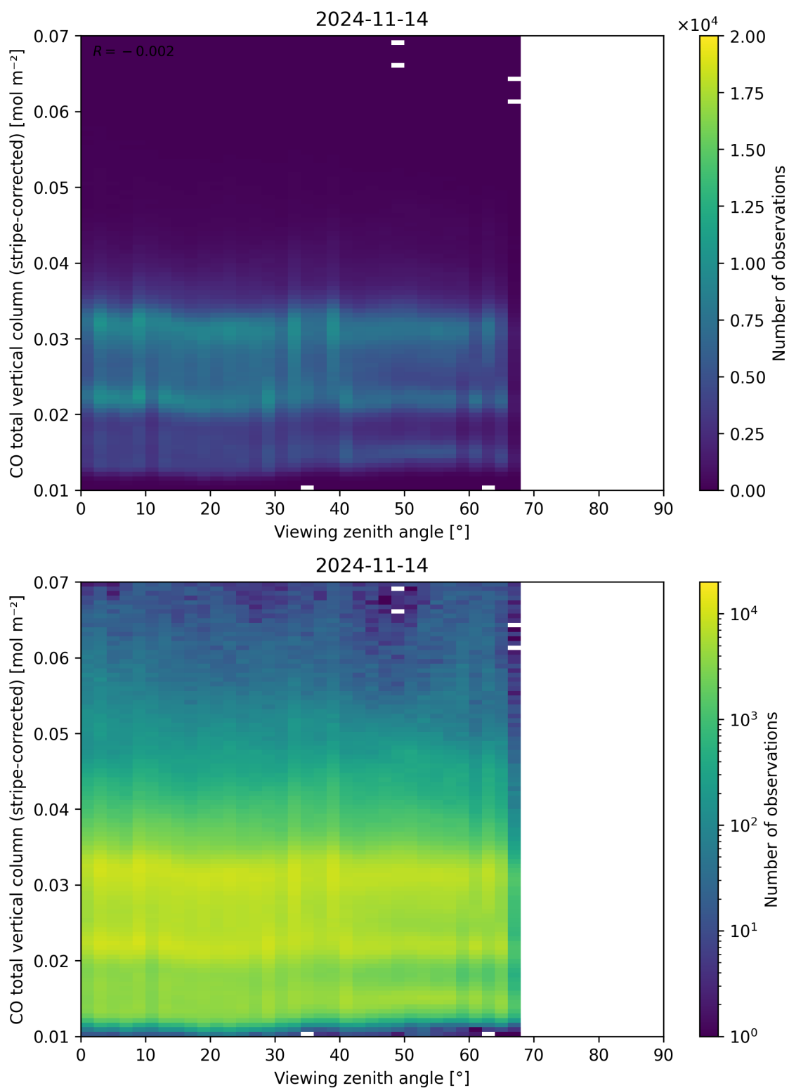
Figure 70: Scatter density plot of “Viewing zenith angle” against “CO total vertical column (stripe-corrected)” for 2024-11-14 to 2024-11-15.
