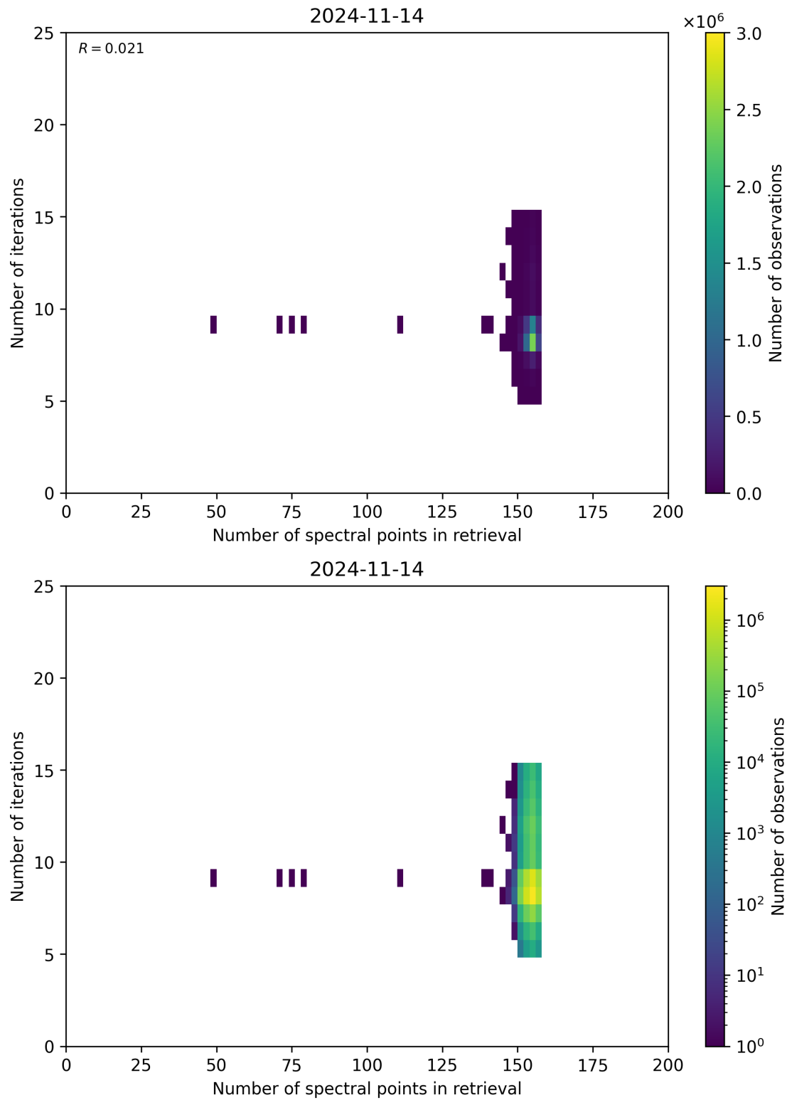
Figure 60: Scatter density plot of “Number of spectral points in retrieval” against “Number of iterations” for 2024-11-14 to 2024-11-15.
