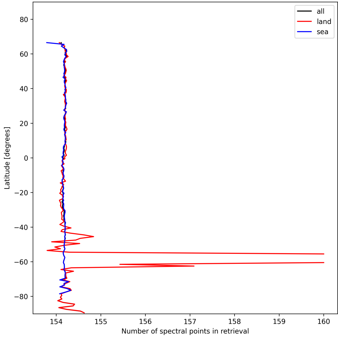
Figure 13: Zonal average of “Number of spectral points in retrieval” for 2024-11-14 to 2024-11-15.
