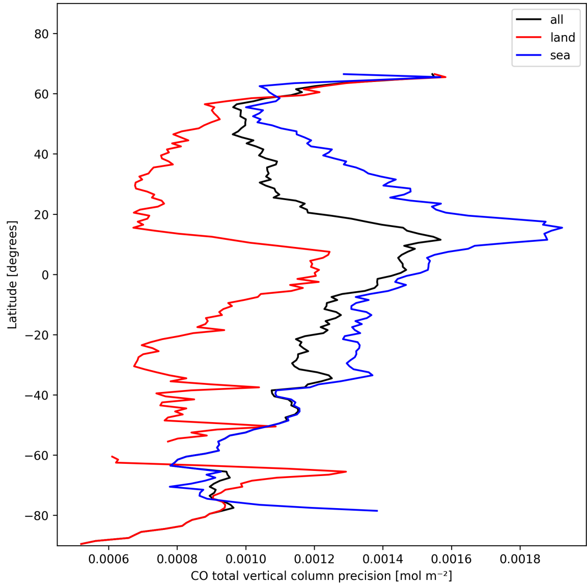
Figure 12: Zonal average of “CO total vertical column precision” for 2024-11-14 to 2024-11-15.
