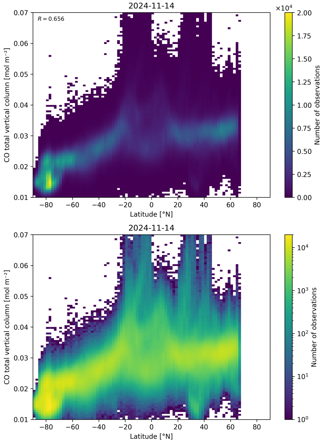
Figure 51: Scatter density plot of “Latitude” against “CO total vertical column” for 2024-11-14 to 2024-11-15.
