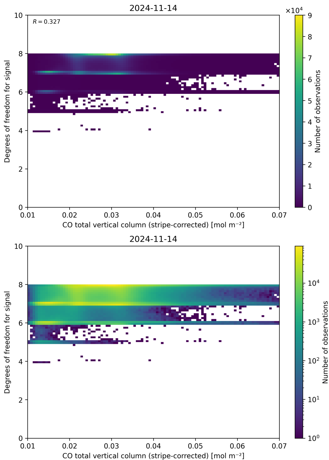
Figure 38: Scatter density plot of “CO total vertical column (stripe-corrected)” against “Degrees of freedom for signal” for 2024-11-14 to 2024-11-15.
