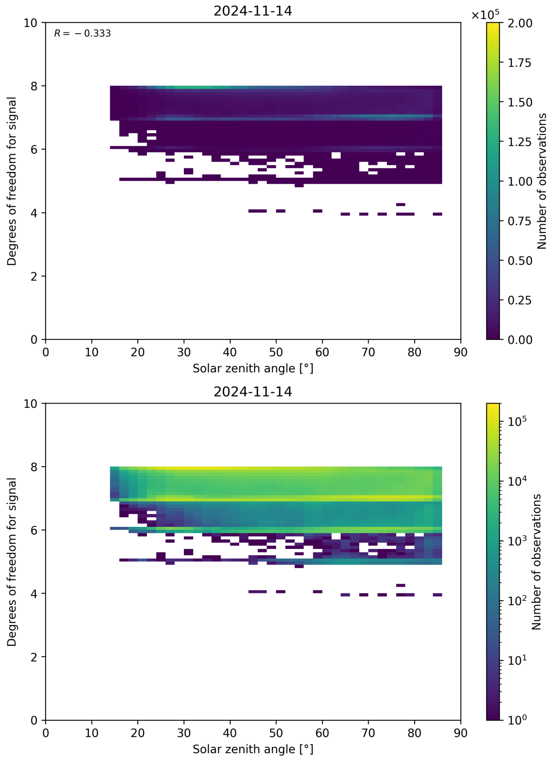
Figure 65: Scatter density plot of “Solar zenith angle” against “Degrees of freedom for signal” for 2024-11-14 to 2024-11-15.
