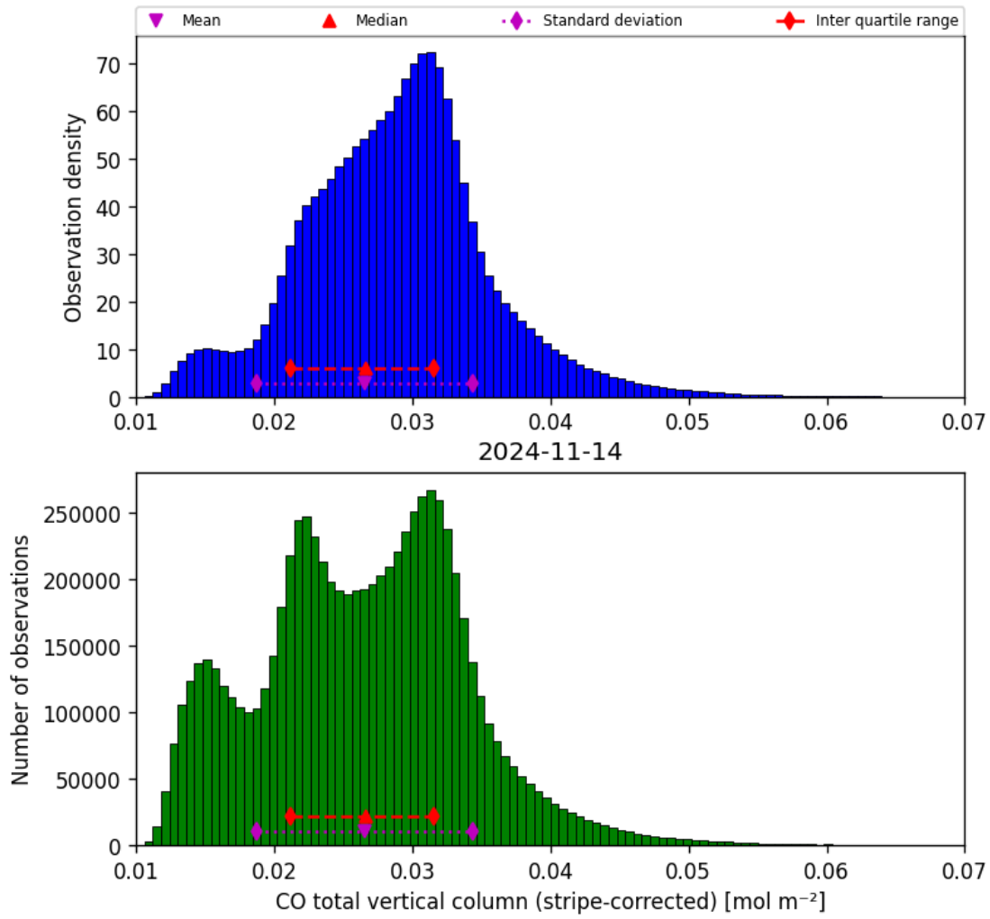
Figure 19: Histogram of “CO total vertical column (stripe-corrected)” for 2024-11-14 to 2024-11-15
