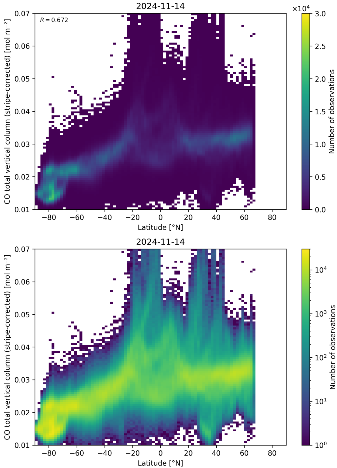
Figure 52: Scatter density plot of “Latitude” against “CO total vertical column (stripe-corrected)” for 2024-11-14 to 2024-11-15.
