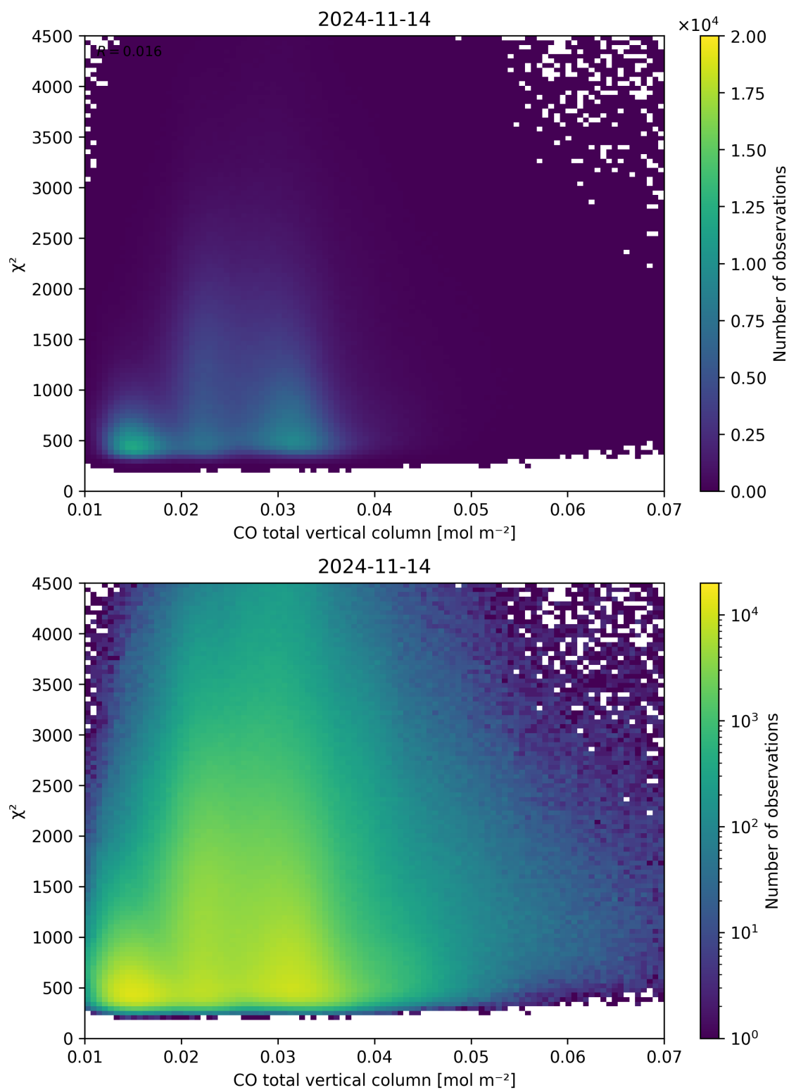
Figure 35: Scatter density plot of “CO total vertical column” against “ \chi^2 ” for 2024-11-14 to 2024-11-15.
