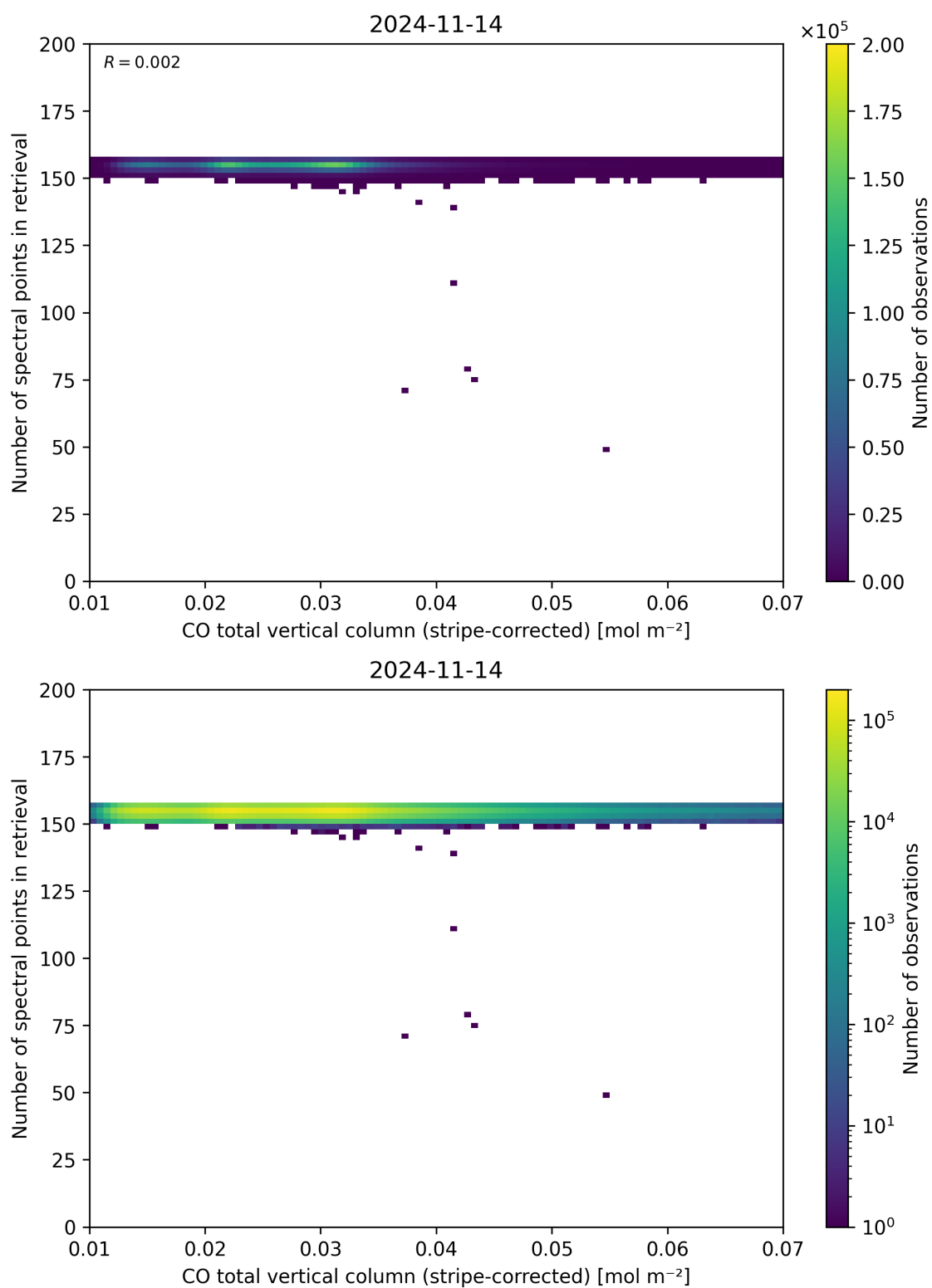
Figure 40: Scatter density plot of “CO total vertical column (stripe-corrected)” against “Number of spectral points in retrieval” for 2024-11-14 to 2024-11-15.
