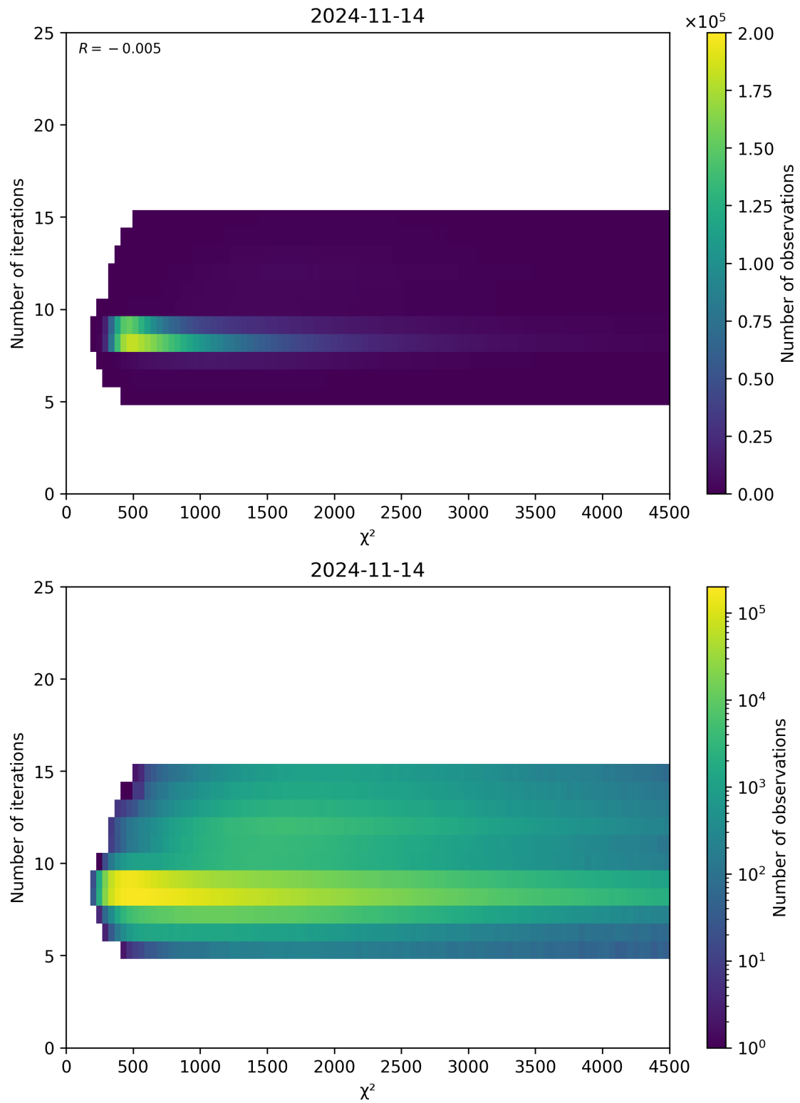
Figure 49: Scatter density plot of “ \chi^2 ” against “Number of iterations” for 2024-11-14 to 2024-11-15.
