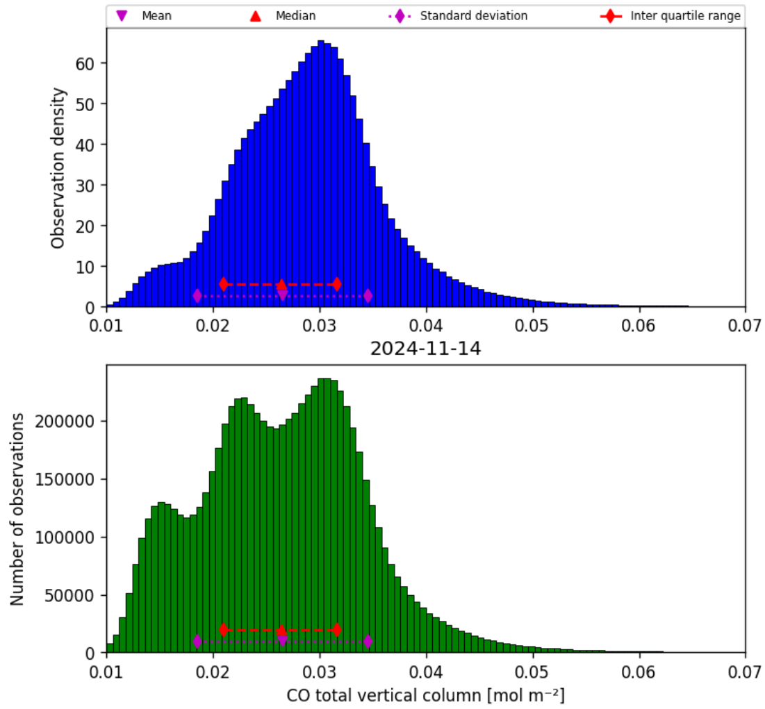
Figure 18: Histogram of “CO total vertical column” for 2024-11-14 to 2024-11-15
