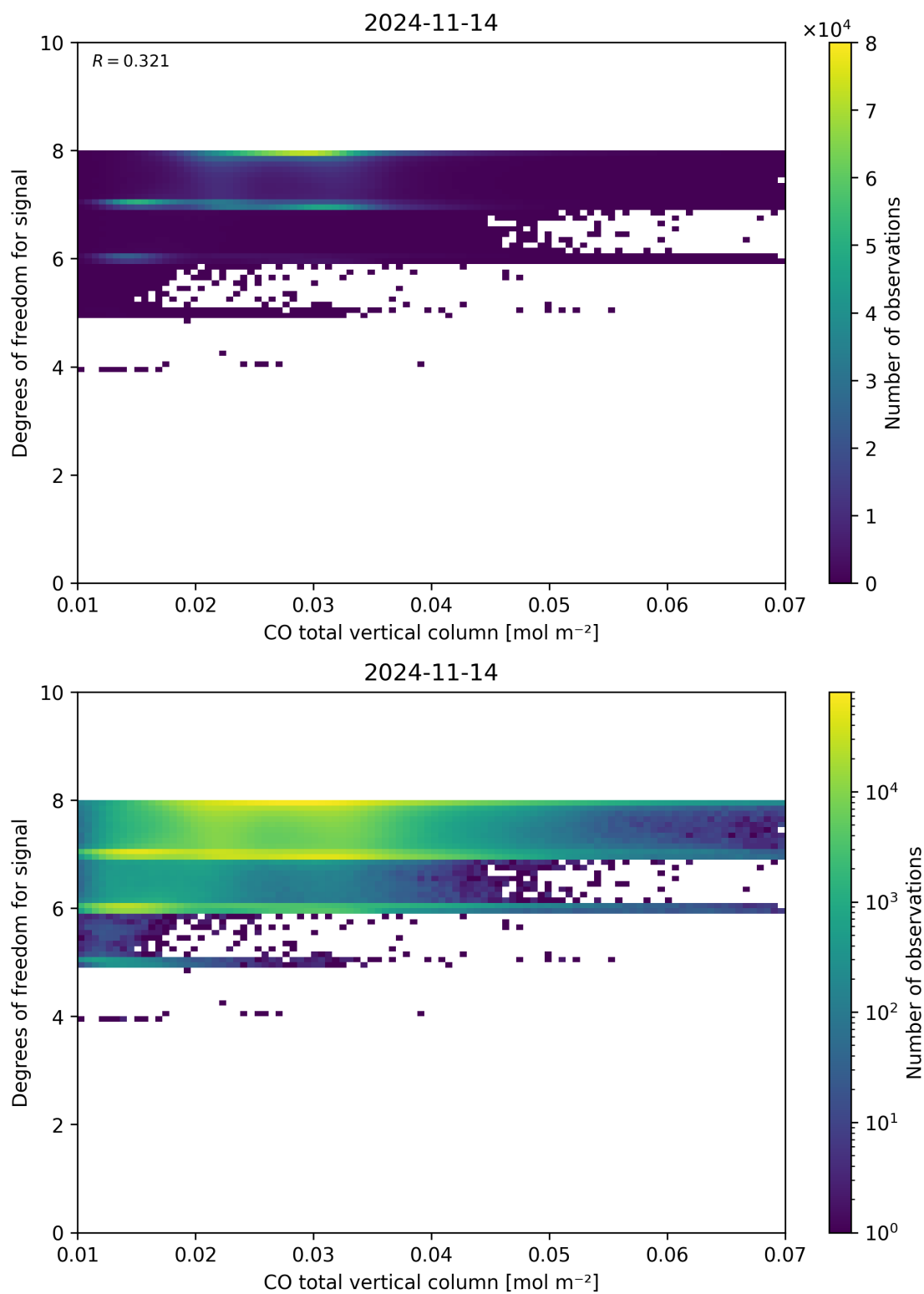
Figure 41: Scatter density plot of “CO total vertical column” against “Degrees of freedom for signal” for 2024-11-14 to 2024-11-15.
