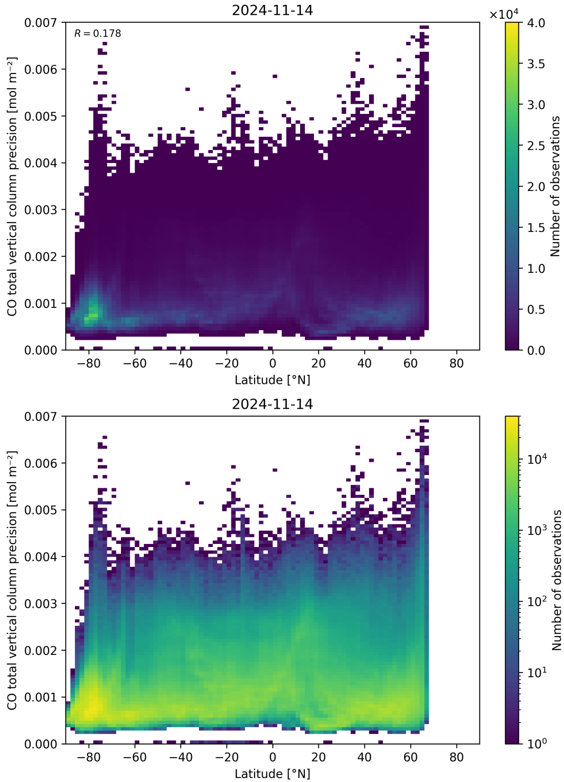
Figure 53: Scatter density plot of “Latitude” against “CO total vertical column precision” for 2024-11-14 to 2024-11-15.
