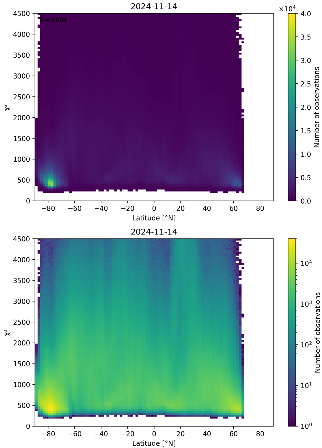
Figure 54: Scatter density plot of “Latitude” against “ \chi^2 ” for 2024-11-14 to 2024-11-15.
