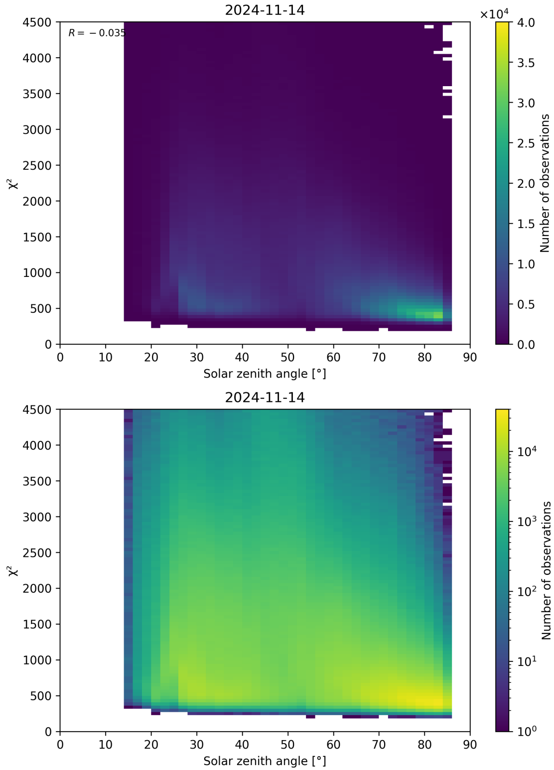
Figure 64: Scatter density plot of “Solar zenith angle” against “ \chi^2 ” for 2024-11-14 to 2024-11-15.
