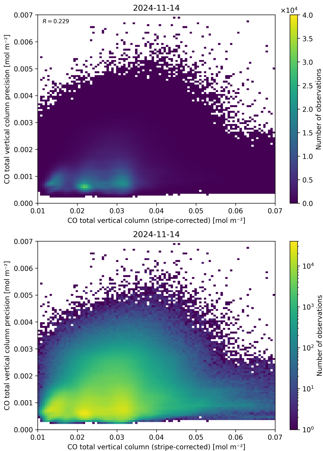
Figure 36: Scatter density plot of “CO total vertical column (stripe-corrected)” against “CO total vertical column precision” for 2024-11-14 to 2024-11-15.
