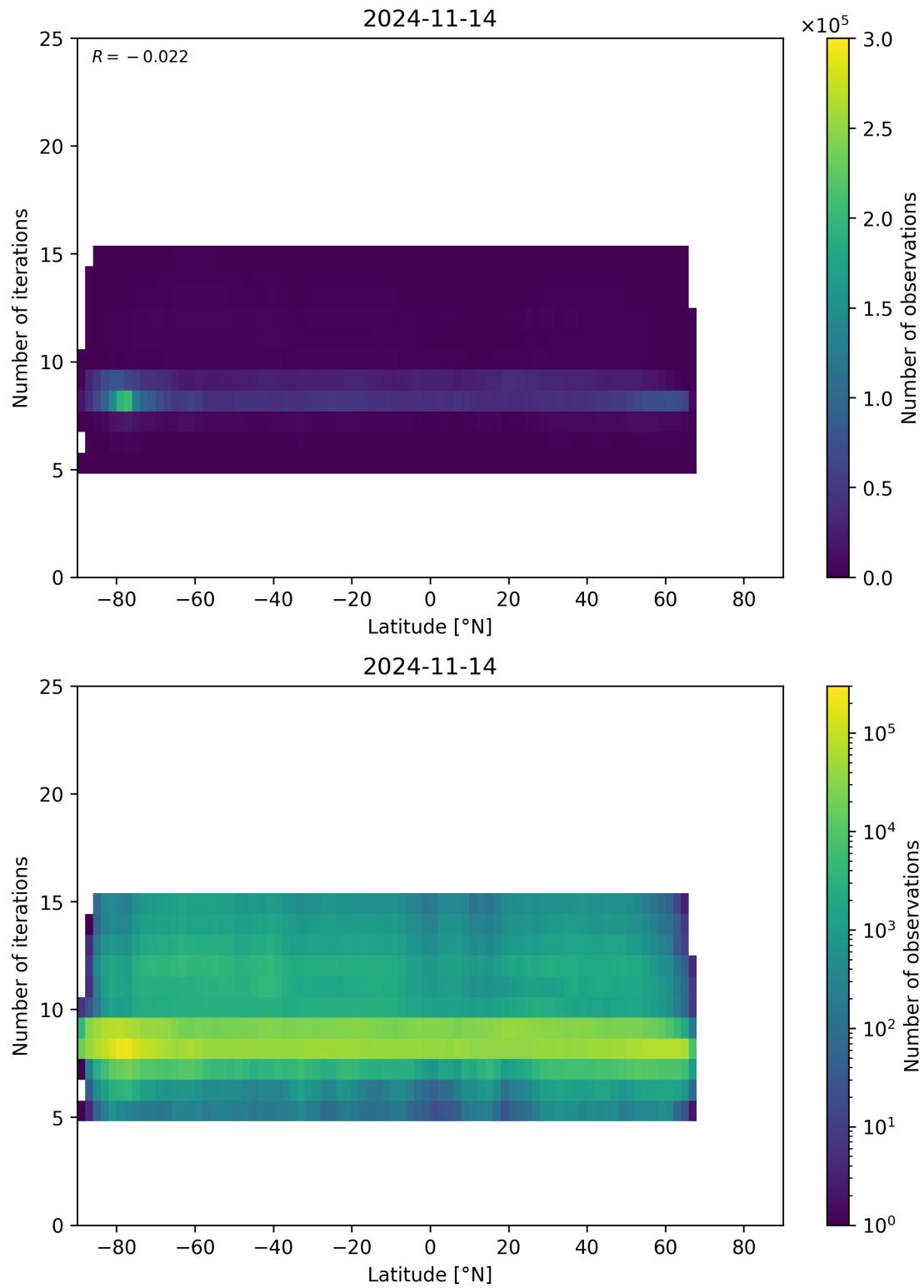
Figure 56: Scatter density plot of “Latitude” against “Number of iterations” for 2024-11-14 to 2024-11-15.
