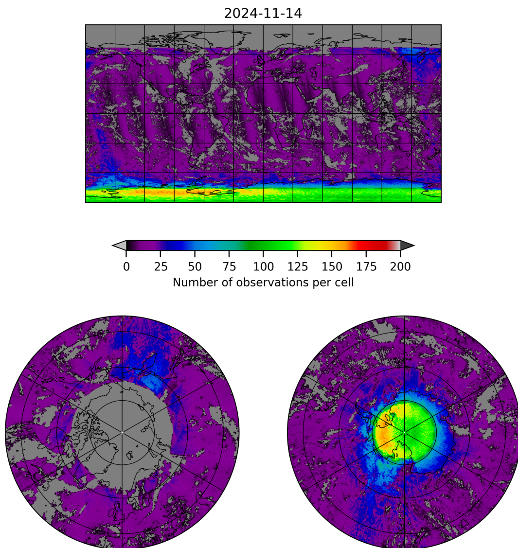
Figure 8: Map of the number of observations for 2024-11-14 to 2024-11-15
