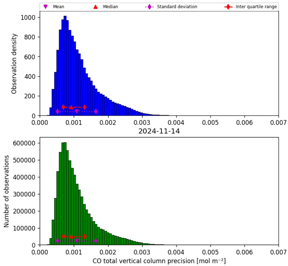
Figure 20: Histogram of “CO total vertical column precision” for 2024-11-14 to 2024-11-15
