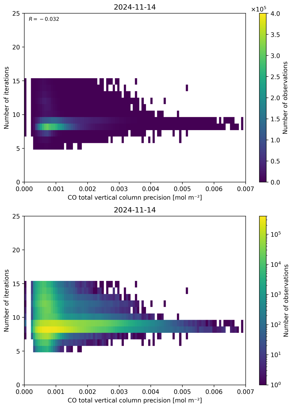
Figure 46: Scatter density plot of “CO total vertical column precision” against “Number of iterations” for 2024-11-14 to 2024-11-15.
