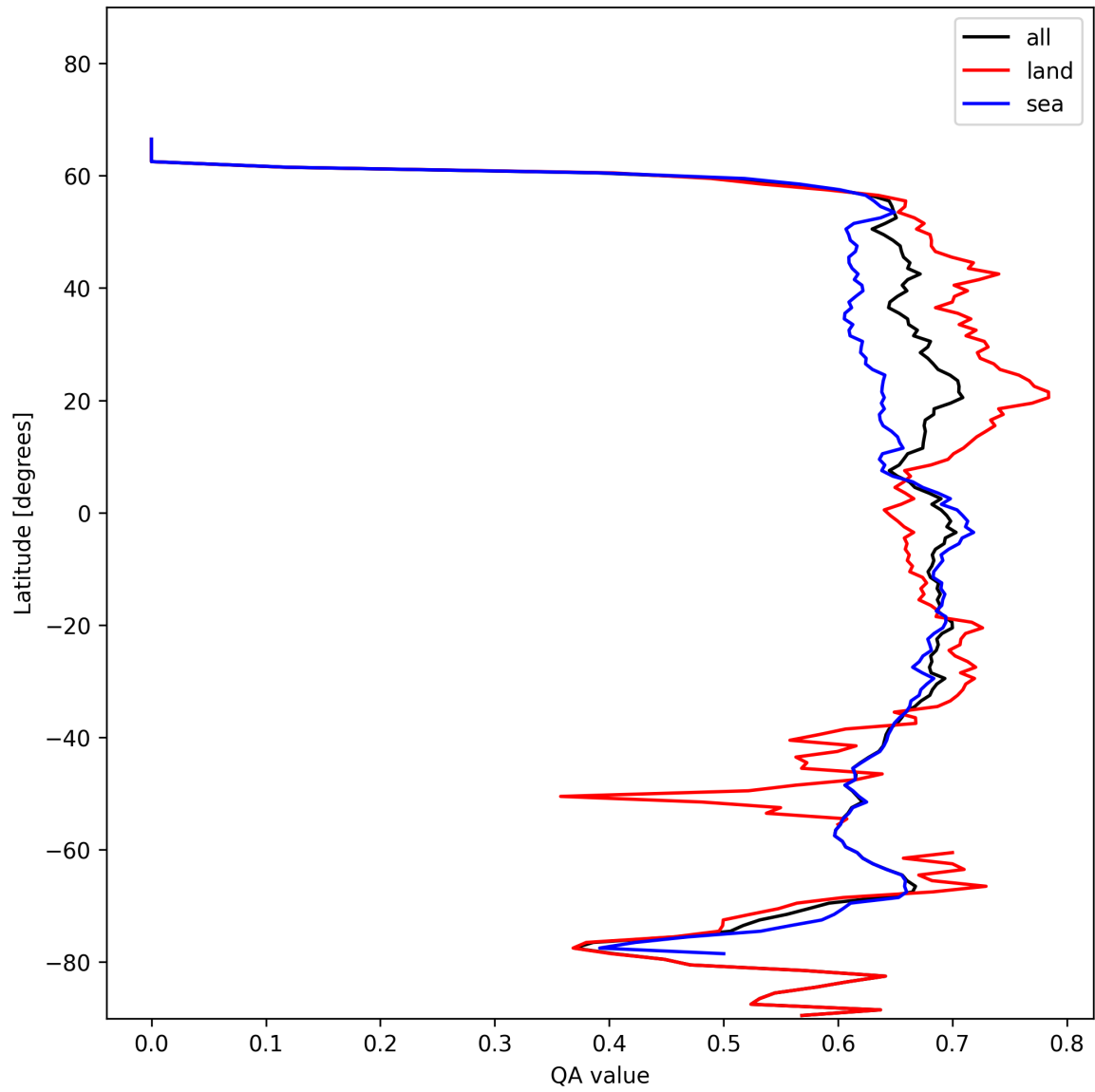
Figure 9: Zonal average of “QA value” for 2024-11-14 to 2024-11-15.
