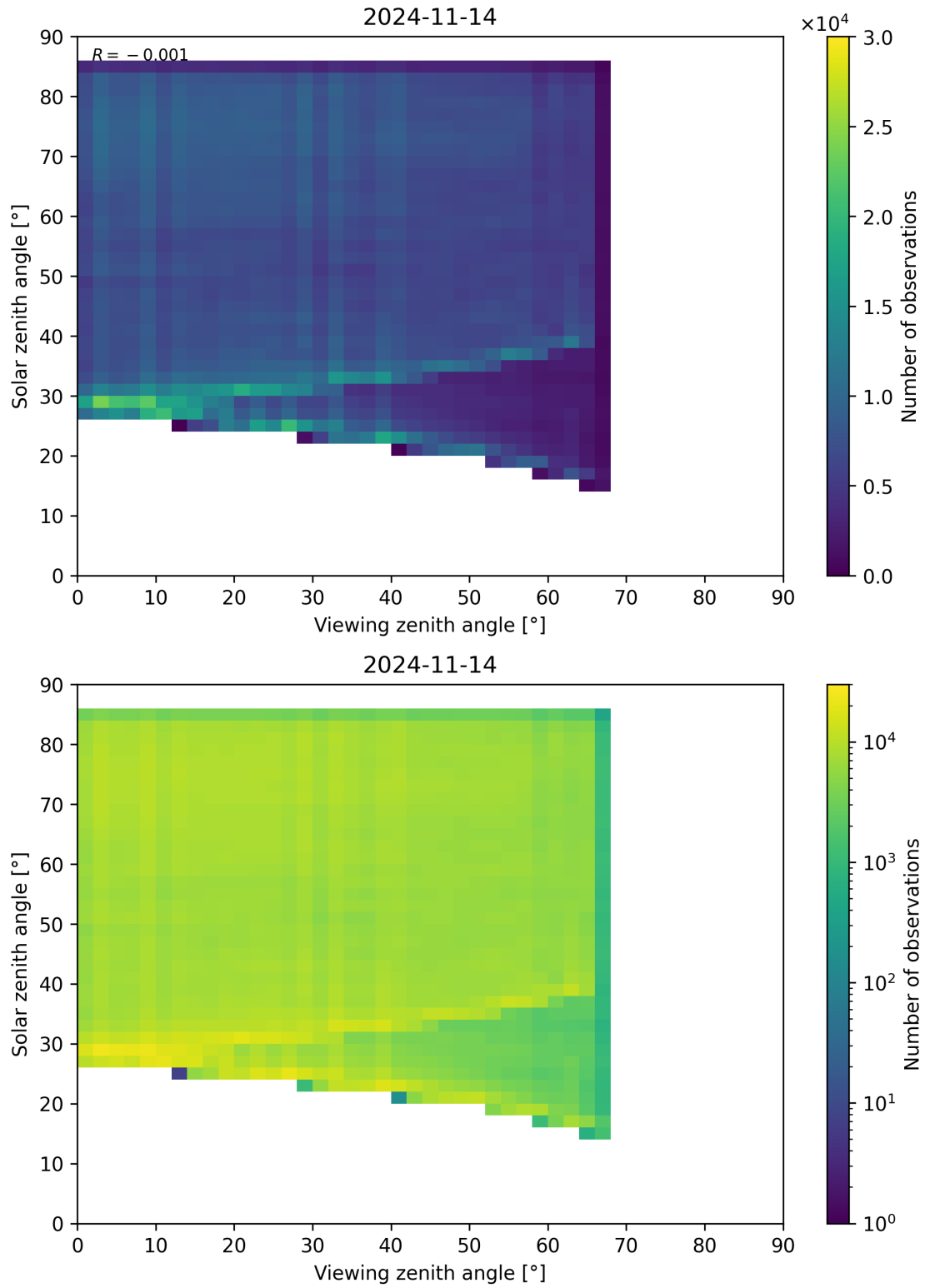
Figure 77: Scatter density plot of “Viewing zenith angle” against “Solar zenith angle” for 2024-11-14 to 2024-11-15.
