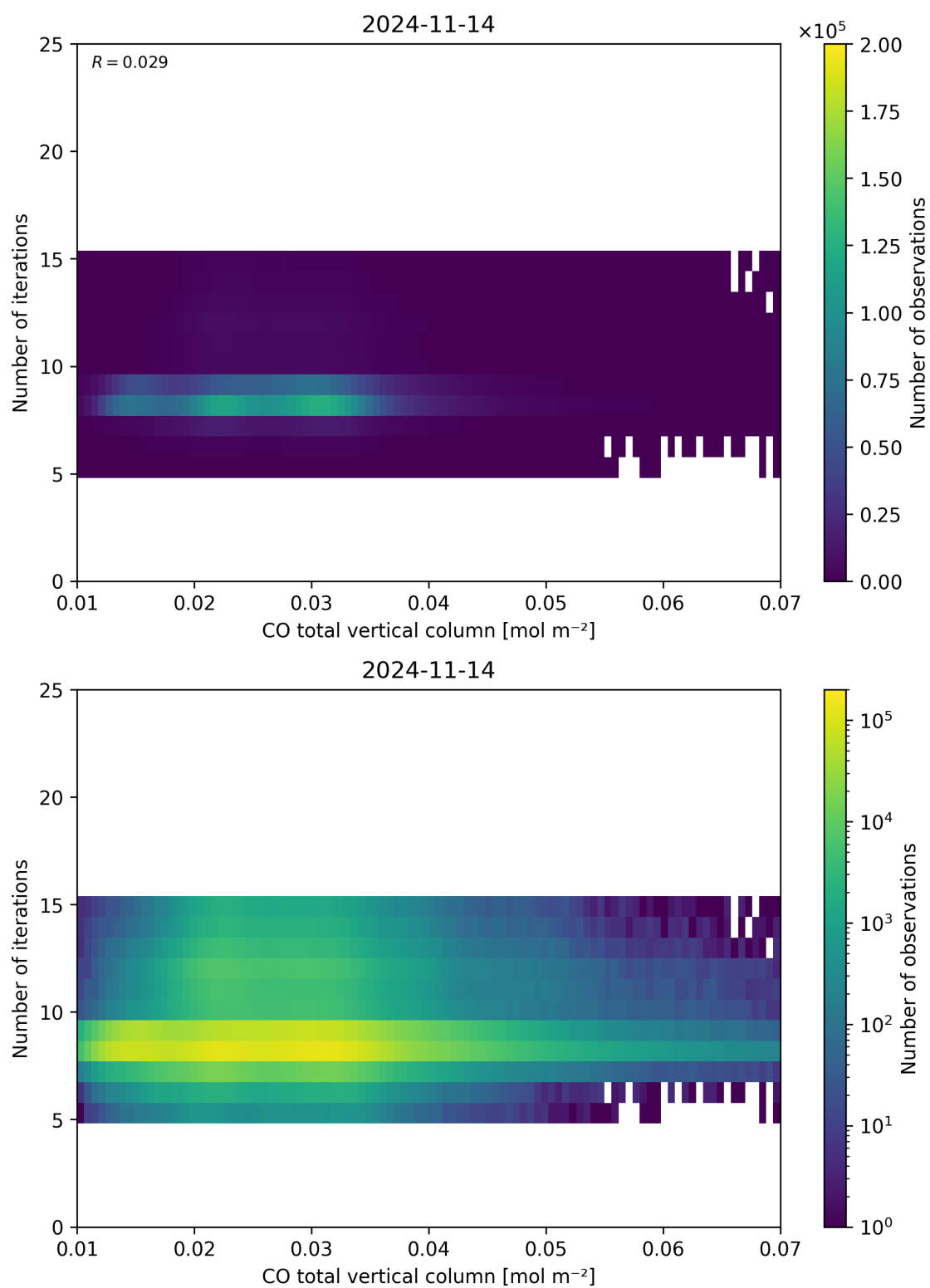
Figure 42: Scatter density plot of “CO total vertical column” against “Number of iterations” for 2024-11-14 to 2024-11-15.
