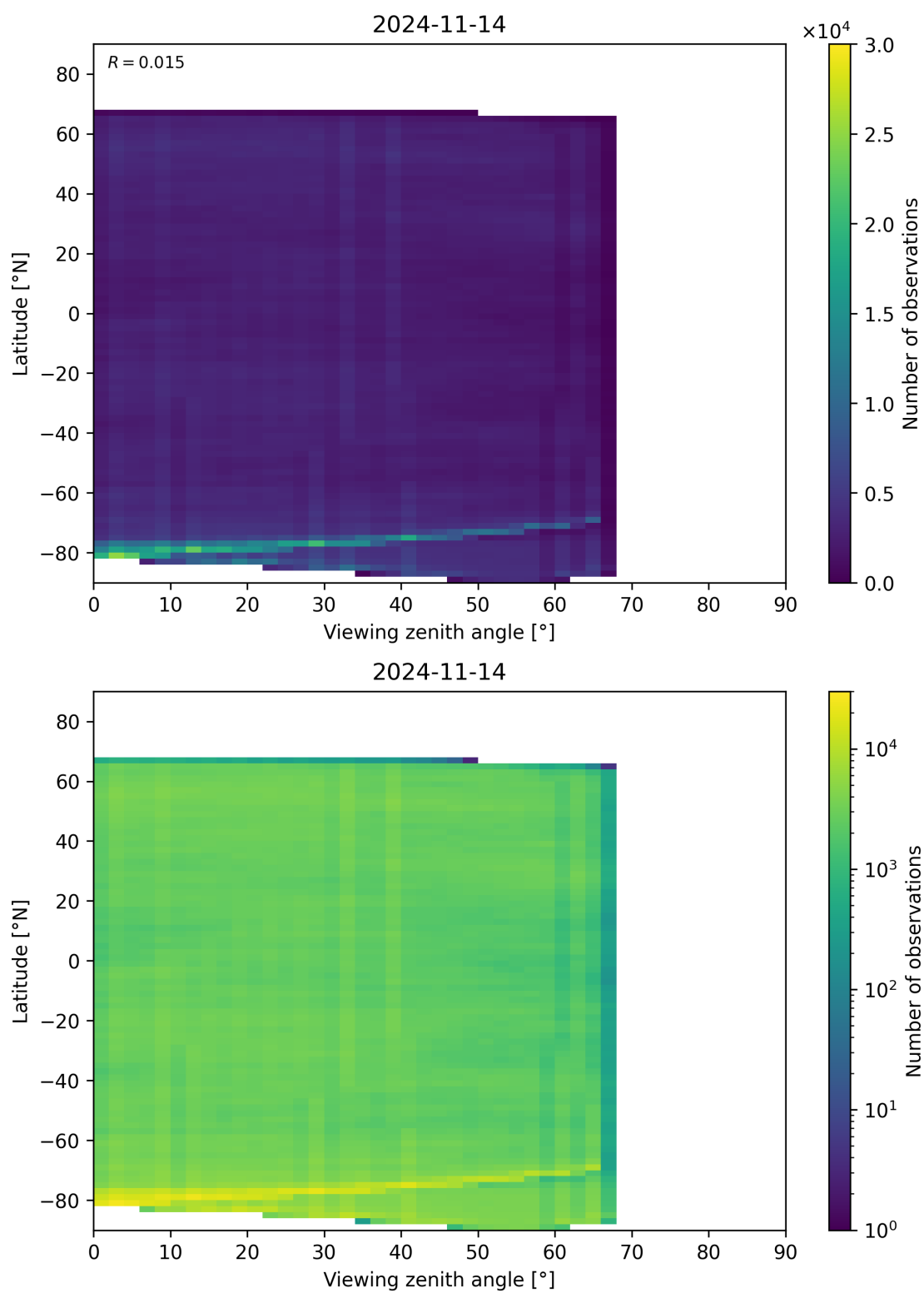
Figure 74: Scatter density plot of “Viewing zenith angle” against “Latitude” for 2024-11-14 to 2024-11-15.
