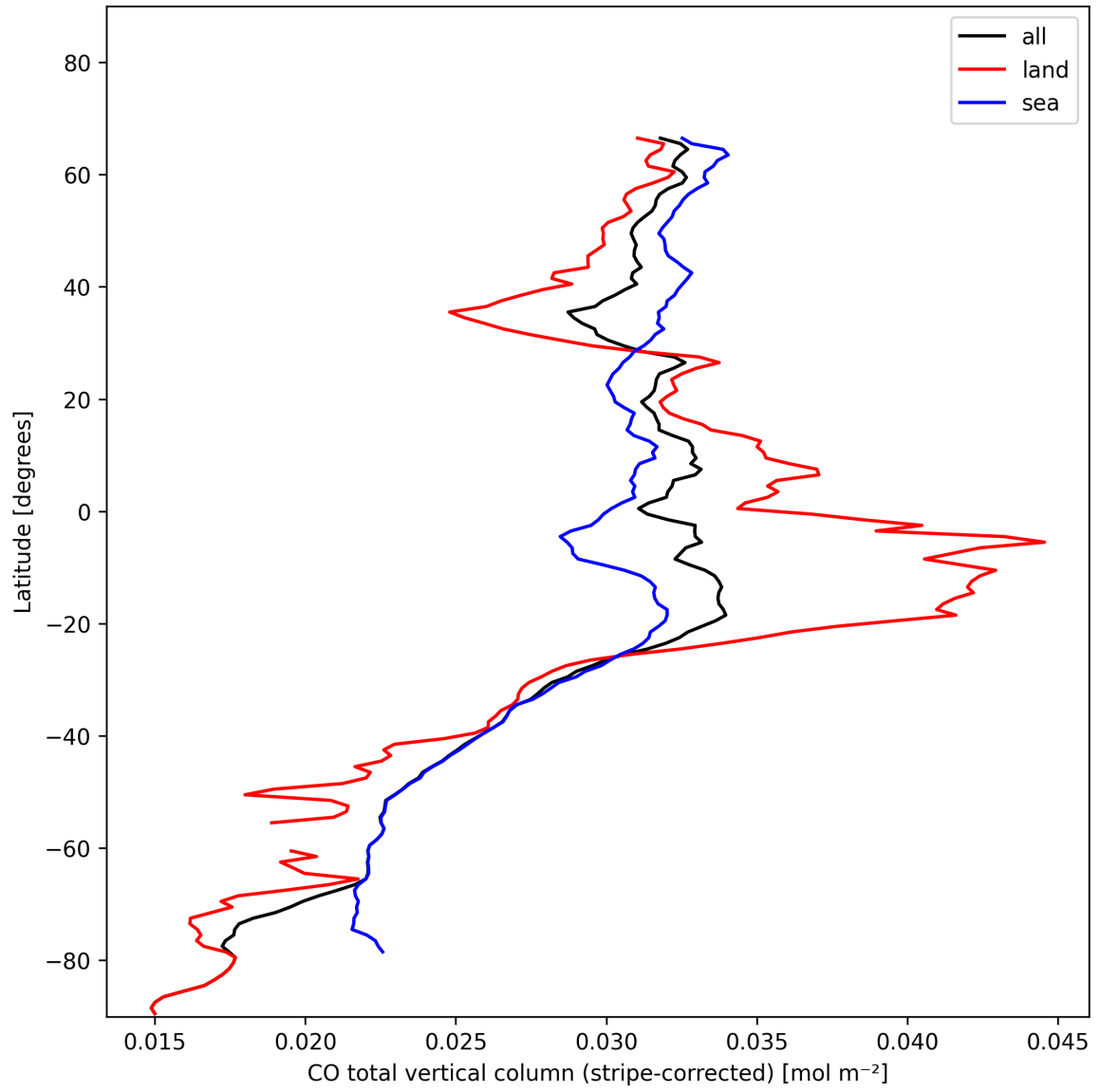
Figure 11: Zonal average of “CO total vertical column (stripe-corrected)” for 2024-11-14 to 2024-11-15.
