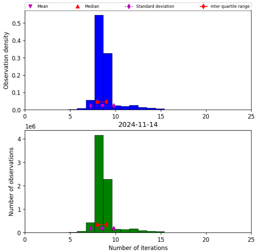
Figure 24: Histogram of “Number of iterations” for 2024-11-14 to 2024-11-15
