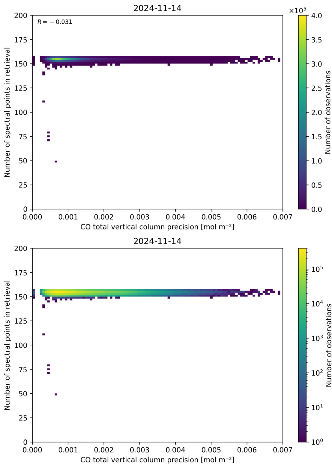
Figure 47: Scatter density plot of “CO total vertical column precision” against “Number of spectral points in retrieval” for 2024-11-14 to 2024-11-15.
