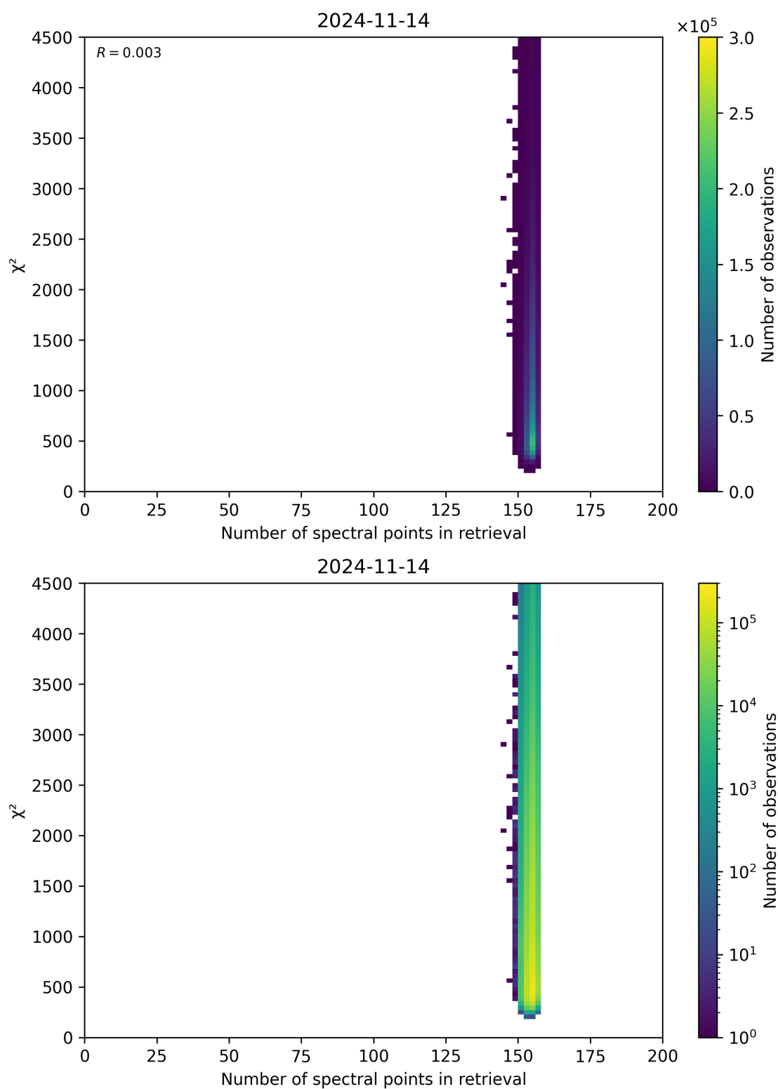
Figure 58: Scatter density plot of “Number of spectral points in retrieval” against “ \chi^2 ” for 2024-11-14 to 2024-11-15.
