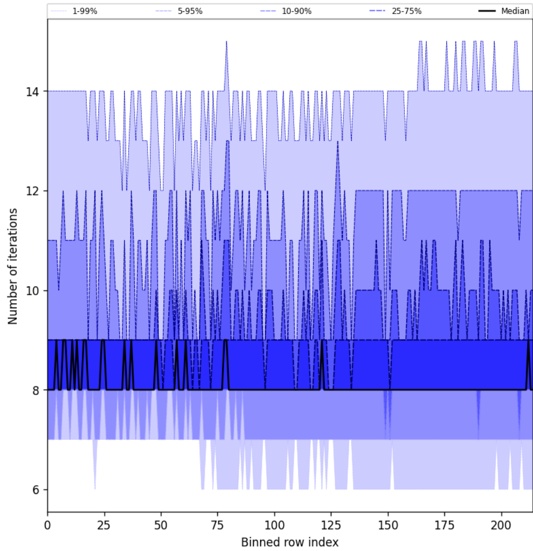
Figure 32: Along track statistics of “Number of iterations” for 2024-11-14 to 2024-11-15
