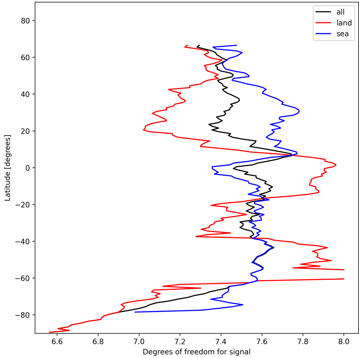
Figure 15: Zonal average of “Degrees of freedom for signal” for 2024-11-14 to 2024-11-15.
