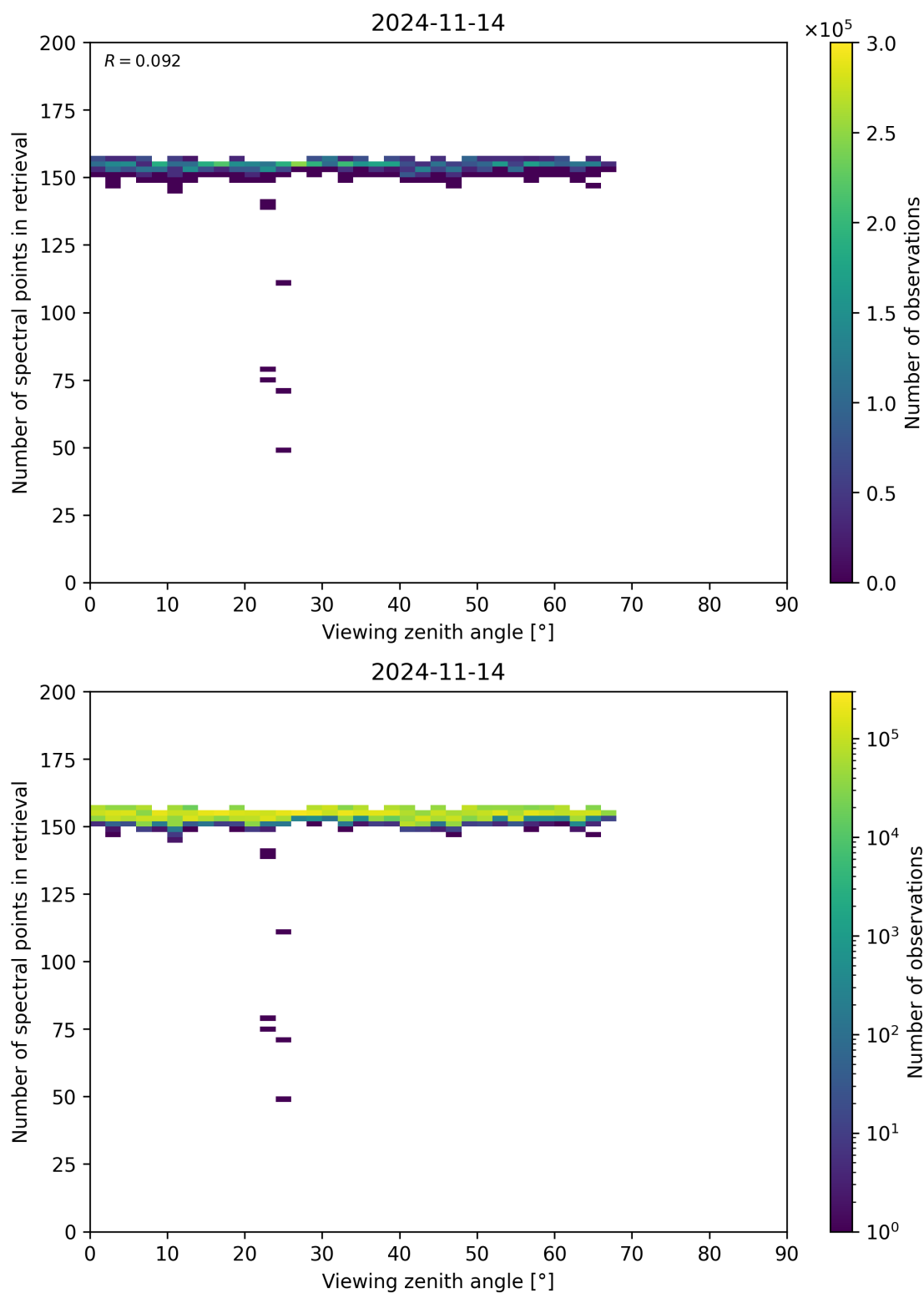
Figure 76: Scatter density plot of “Viewing zenith angle” against “Number of spectral points in retrieval” for 2024-11-14 to 2024-11-15.
