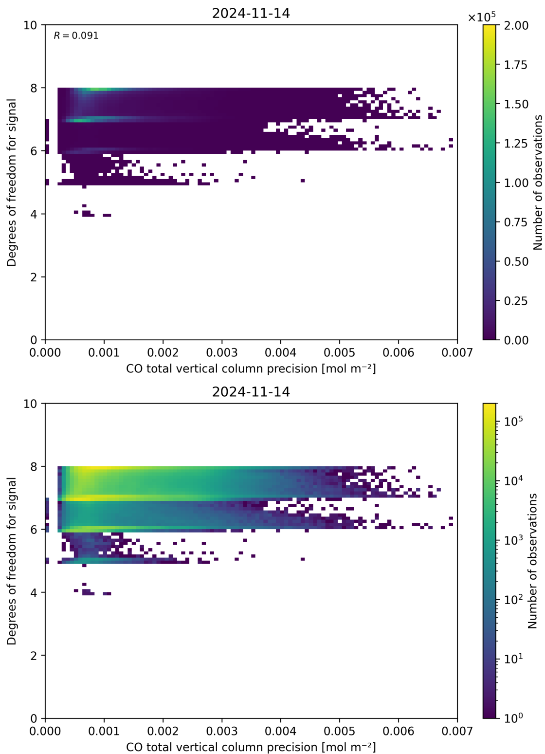
Figure 45: Scatter density plot of “CO total vertical column precision” against “Degrees of freedom for signal” for 2024-11-14 to 2024-11-15.
