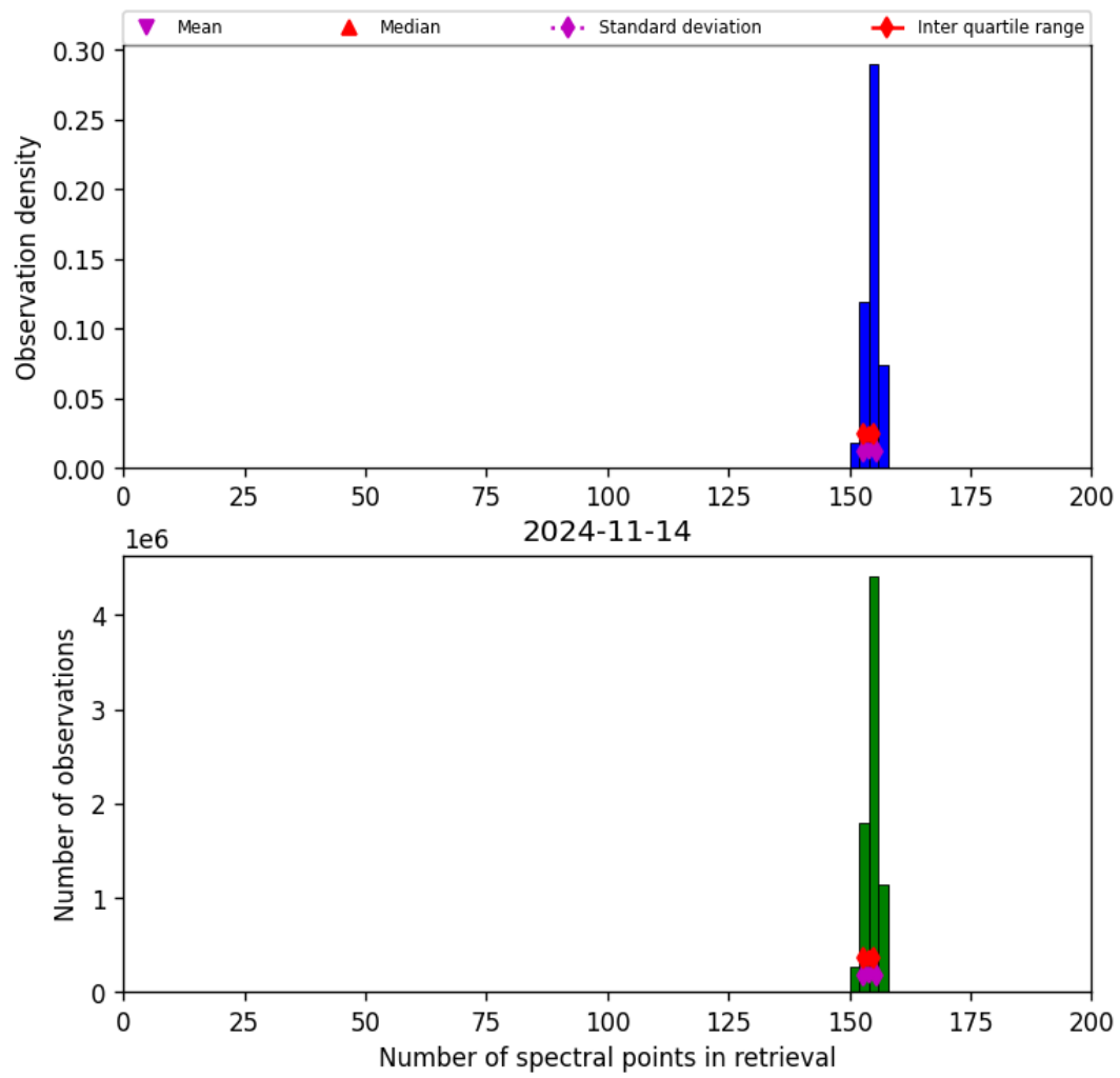
Figure 21: Histogram of “Number of spectral points in retrieval” for 2024-11-14 to 2024-11-15
