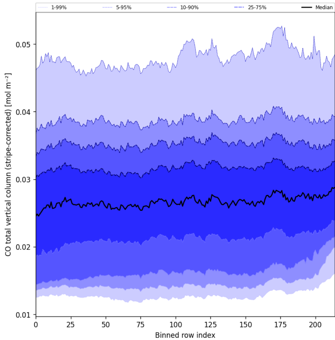
Figure 27: Along track statistics of “CO total vertical column (stripe-corrected)” for 2024-11-14 to 2024-11-15
