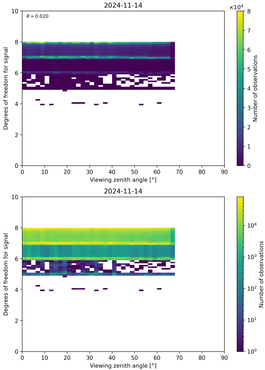
Figure 73: Scatter density plot of “Viewing zenith angle” against “Degrees of freedom for signal” for 2024-11-14 to 2024-11-15.
