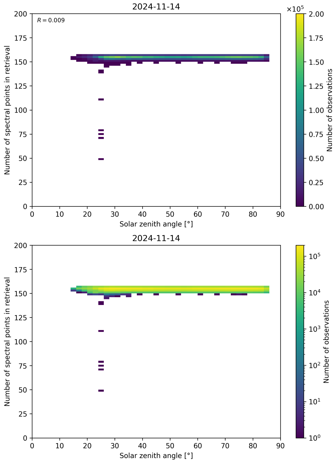
Figure 68: Scatter density plot of “Solar zenith angle” against “Number of spectral points in retrieval” for 2024-11-14 to 2024-11-15.
