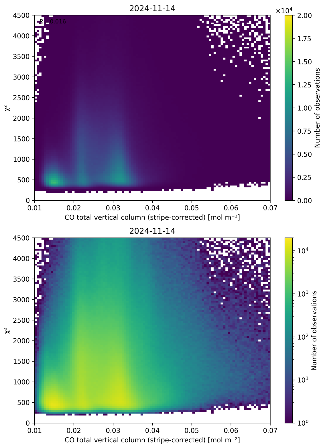
Figure 37: Scatter density plot of “CO total vertical column (stripe-corrected)” against “ \chi^2 ” for 2024-11-14 to 2024-11-15.
