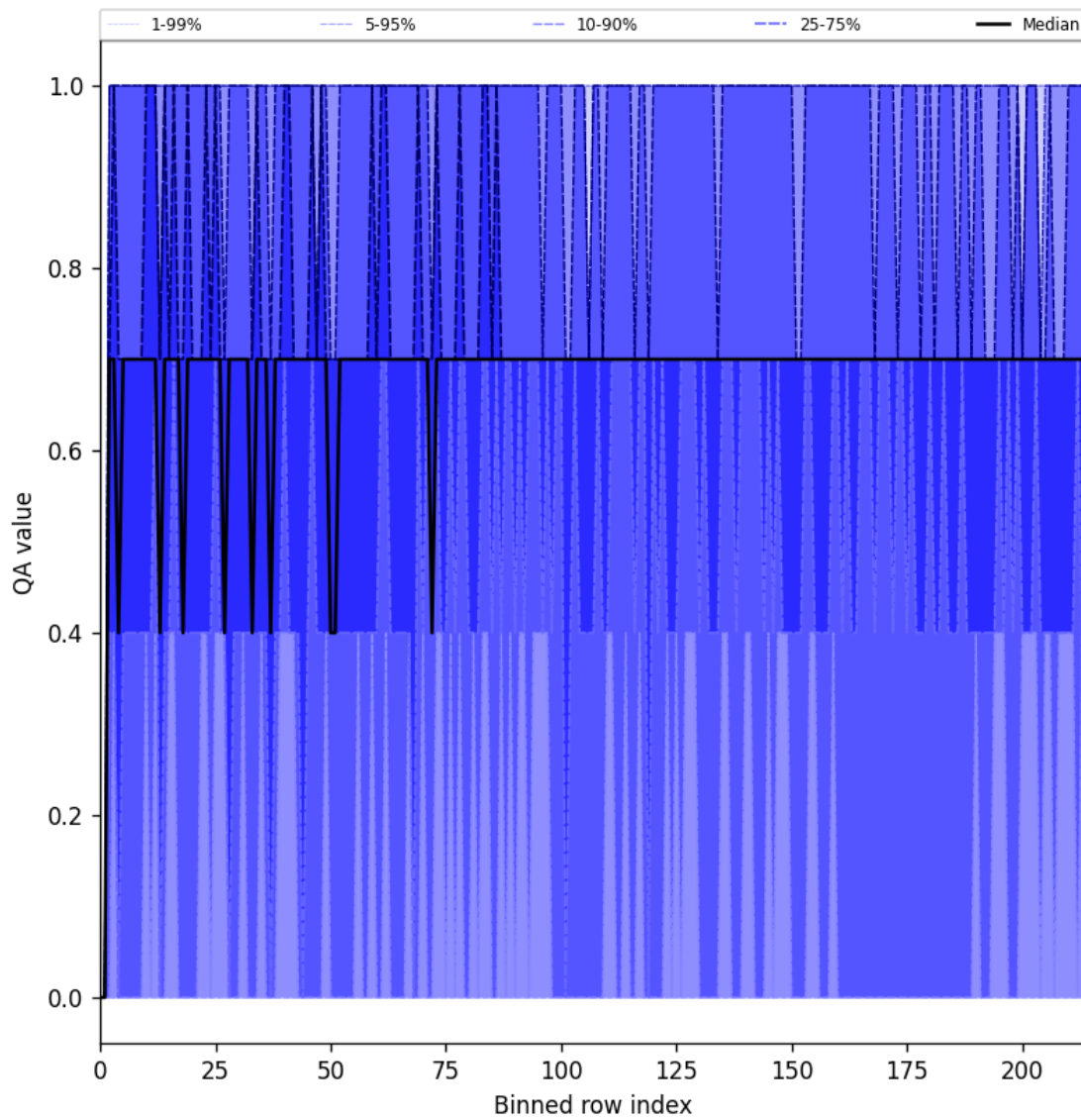
Figure 25: Along track statistics of “QA value” for 2024-11-14 to 2024-11-15
