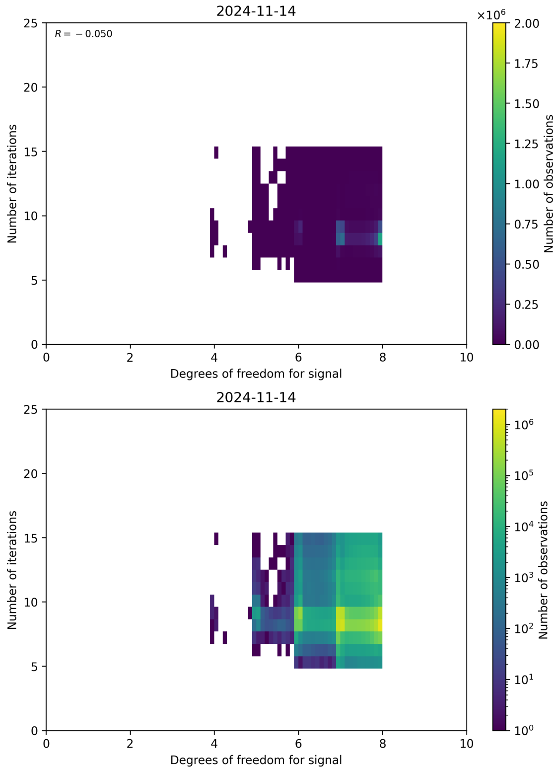
Figure 50: Scatter density plot of “Degrees of freedom for signal” against “Number of iterations” for 2024-11-14 to 2024-11-15.
