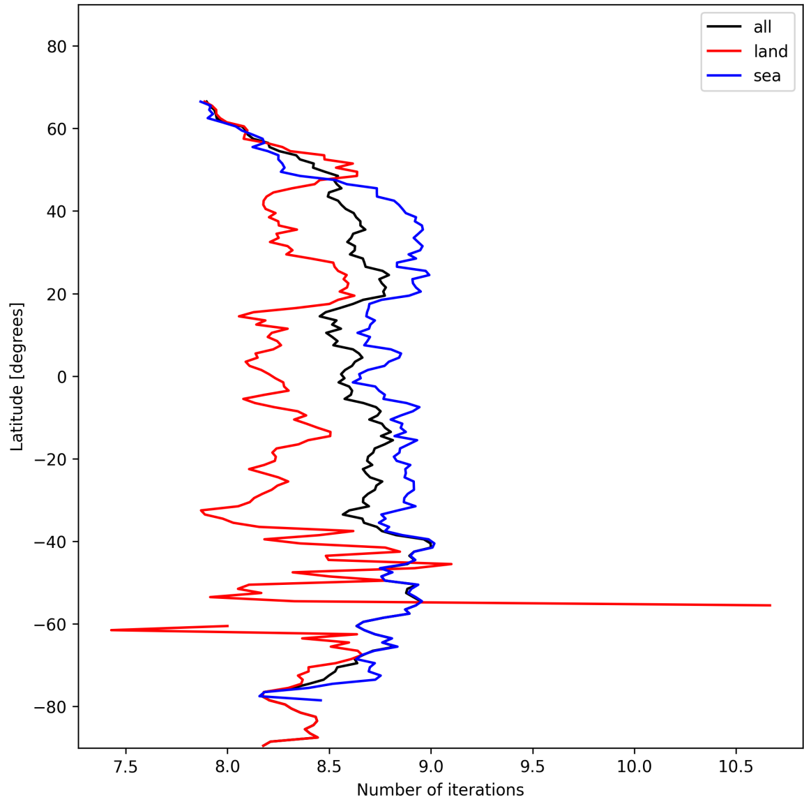
Figure 16: Zonal average of “Number of iterations” for 2024-11-14 to 2024-11-15.
