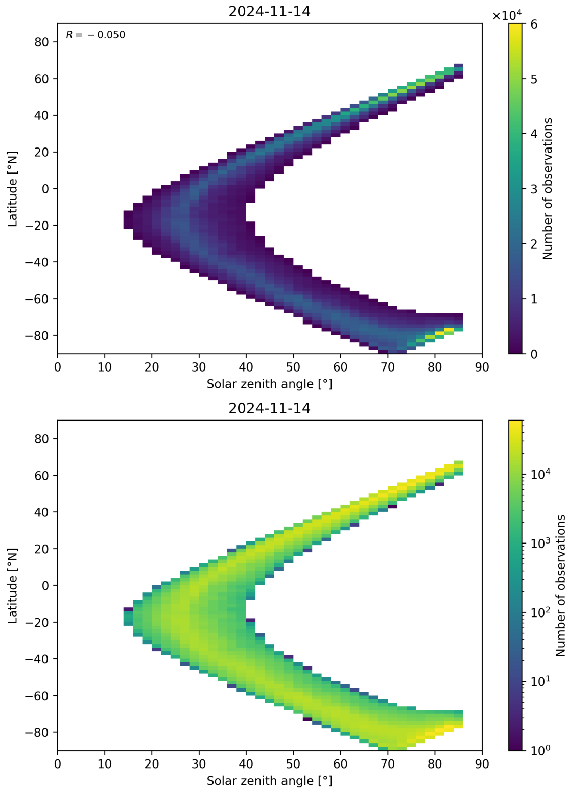
Figure 66: Scatter density plot of “Solar zenith angle” against “Latitude” for 2024-11-14 to 2024-11-15.
