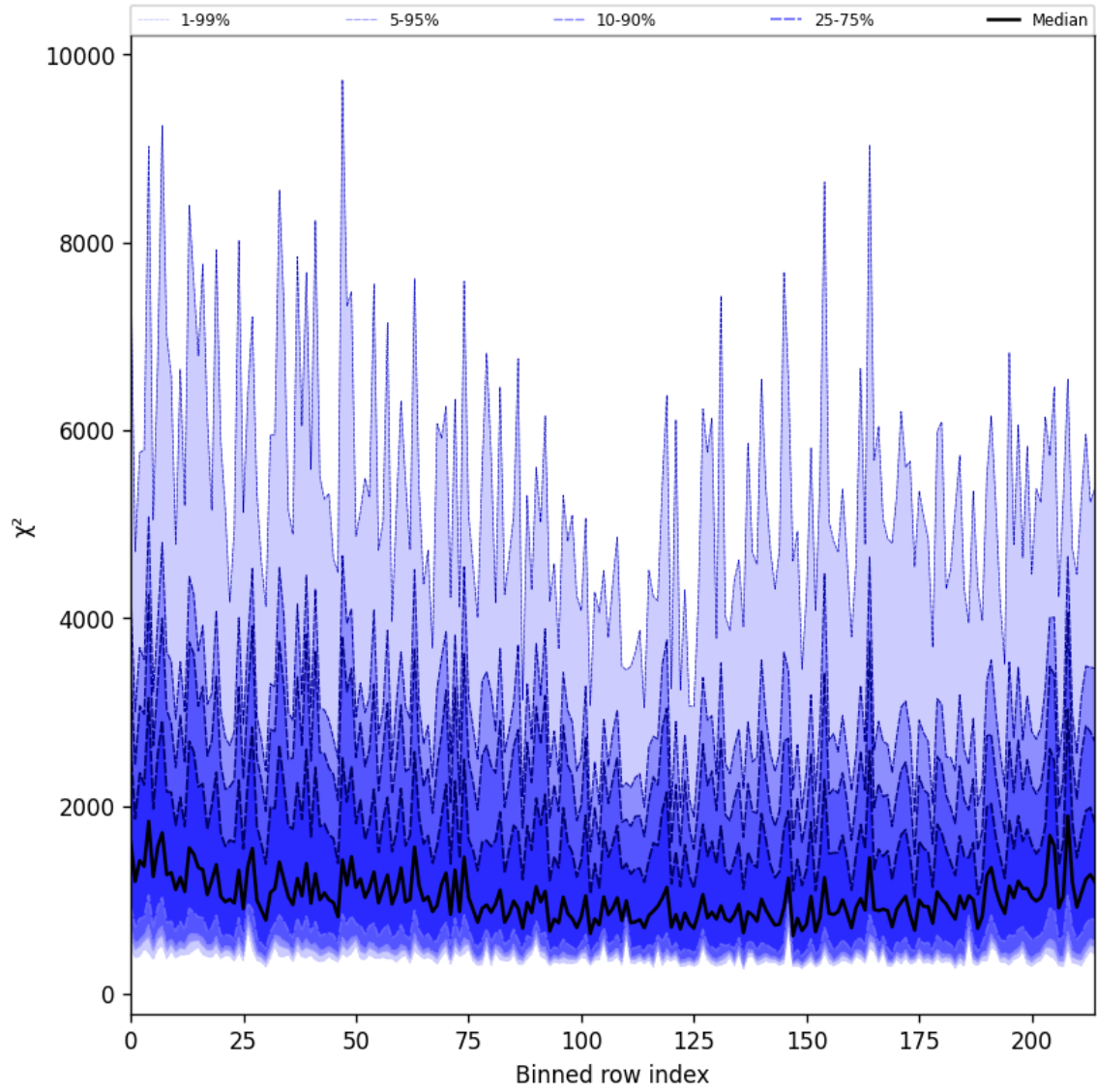
Figure 30: Along track statistics of “ \chi^2 ” for 2024-11-14 to 2024-11-15
