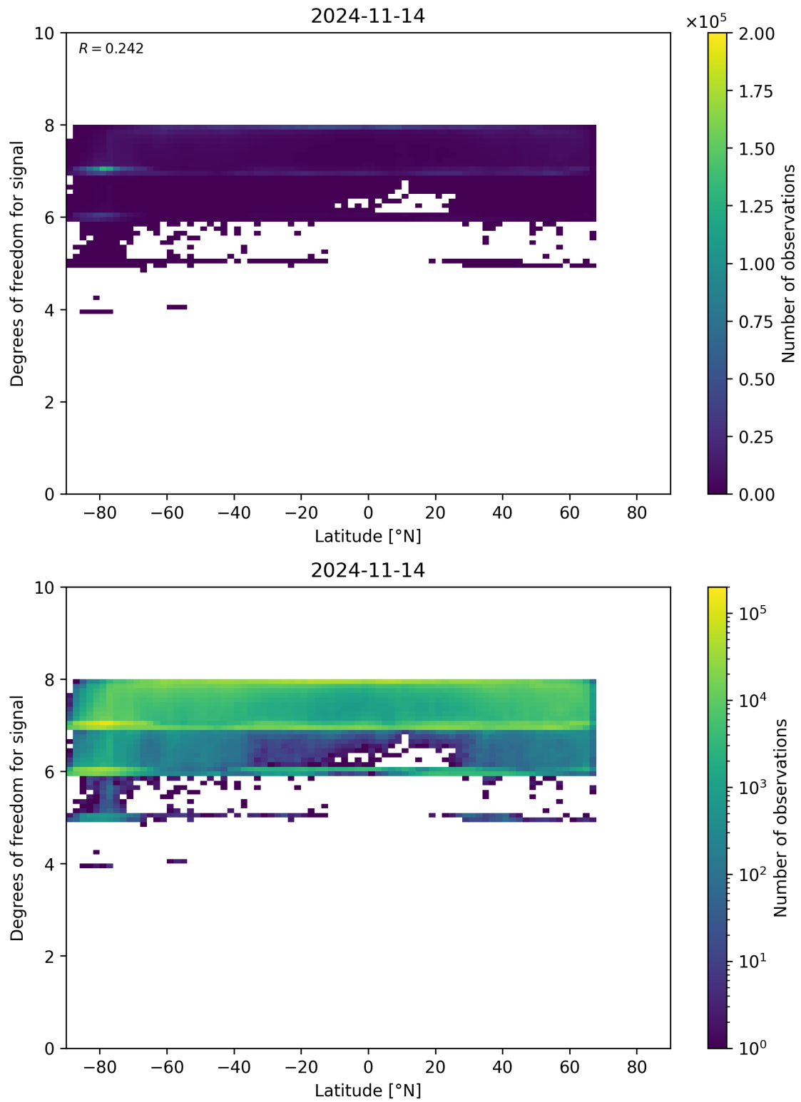
Figure 55: Scatter density plot of “Latitude” against “Degrees of freedom for signal” for 2024-11-14 to 2024-11-15.
