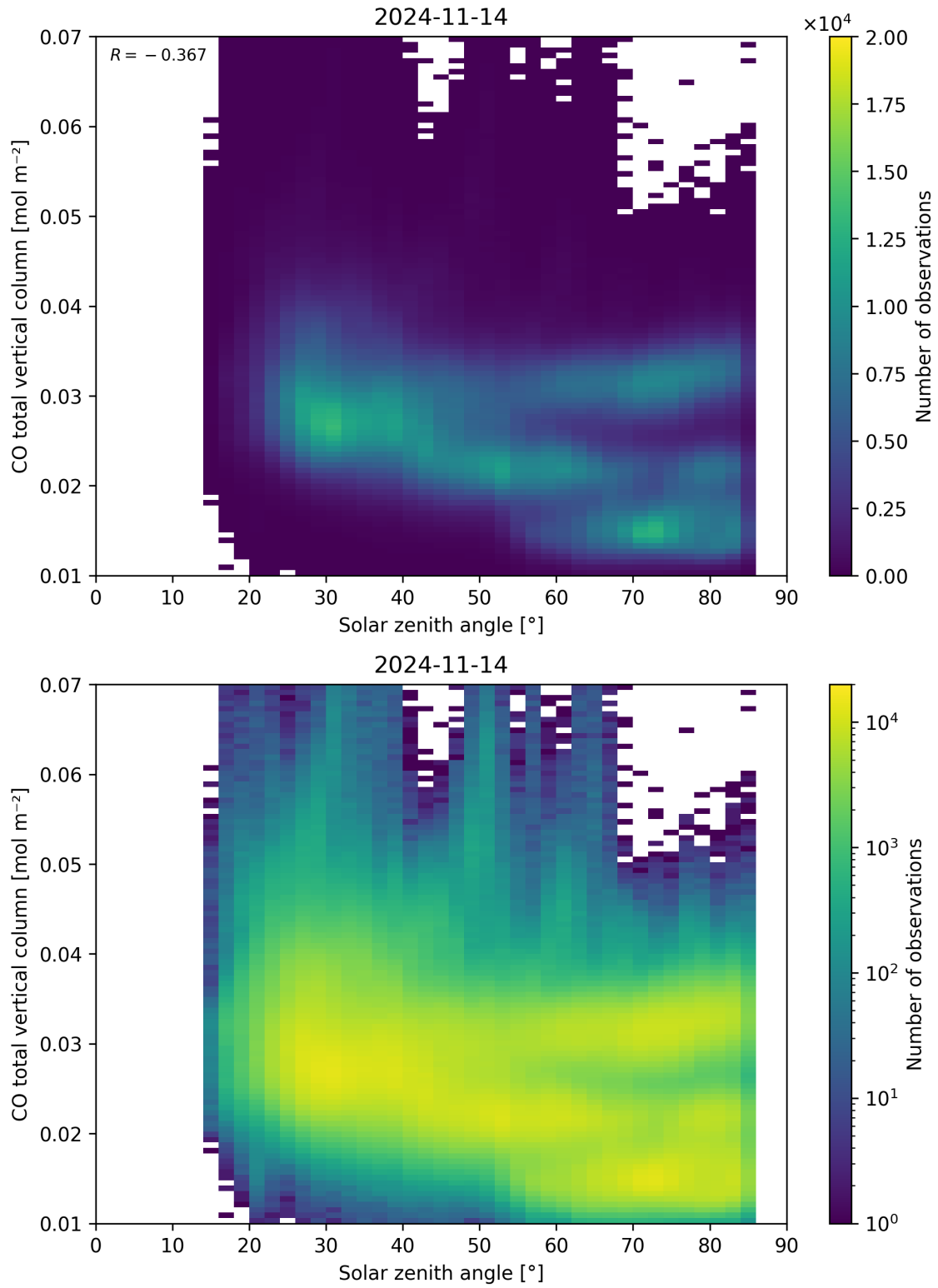
Figure 61: Scatter density plot of “Solar zenith angle” against “CO total vertical column” for 2024-11-14 to 2024-11-15.
