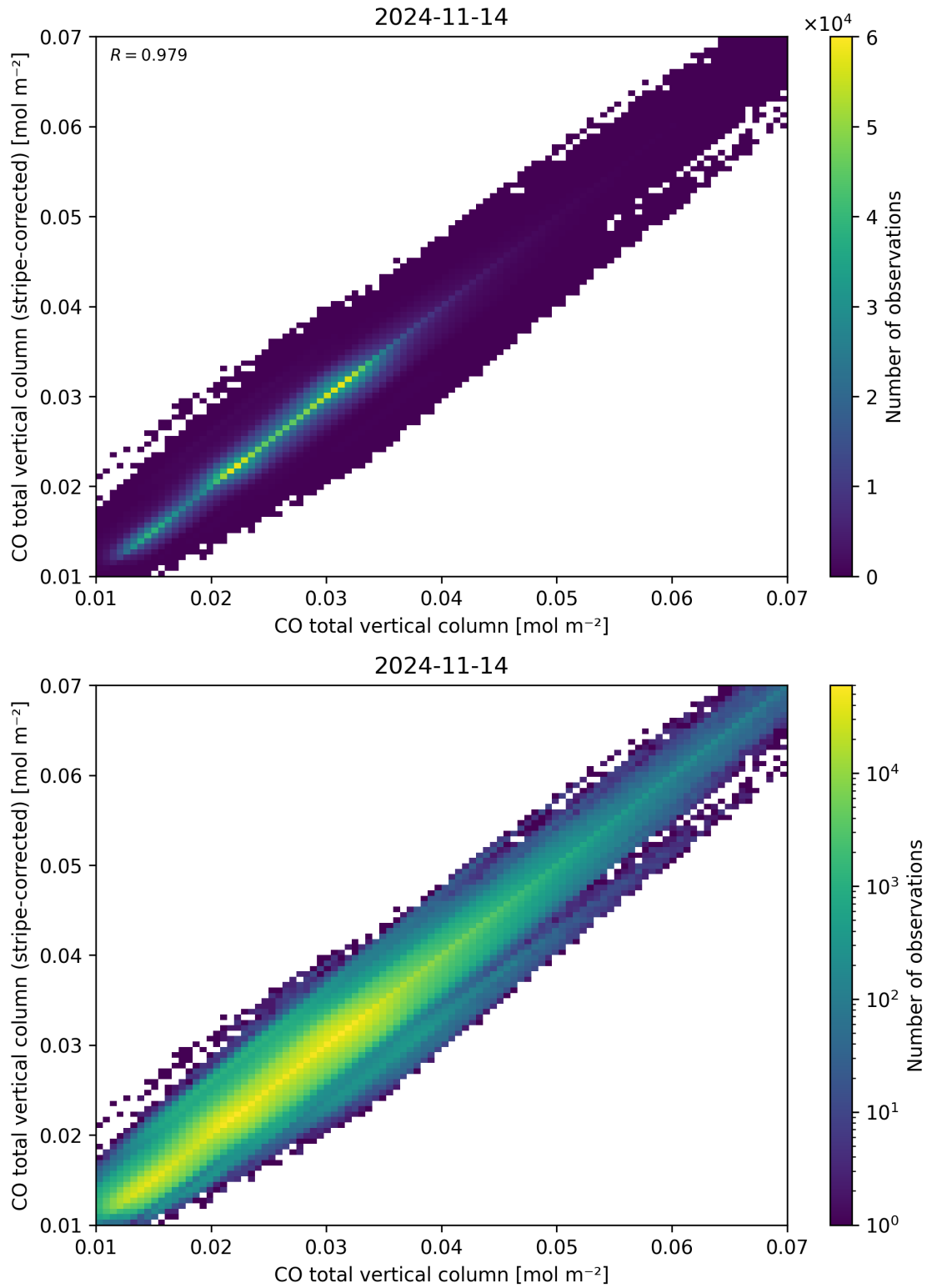
Figure 33: Scatter density plot of “CO total vertical column” against “CO total vertical column (stripe-corrected)” for 2024-11-14 to 2024-11-15.
