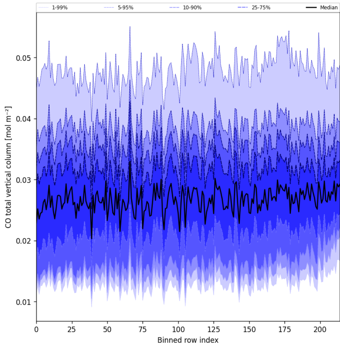
Figure 26: Along track statistics of “CO total vertical column” for 2024-11-14 to 2024-11-15
