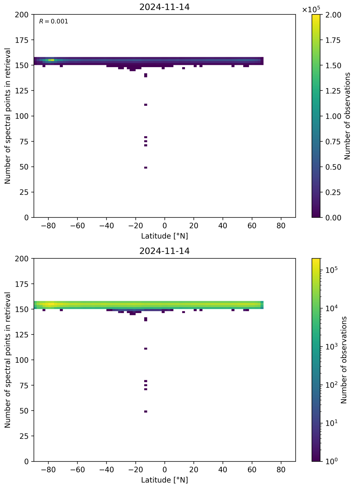
Figure 57: Scatter density plot of “Latitude” against “Number of spectral points in retrieval” for 2024-11-14 to 2024-11-15.
