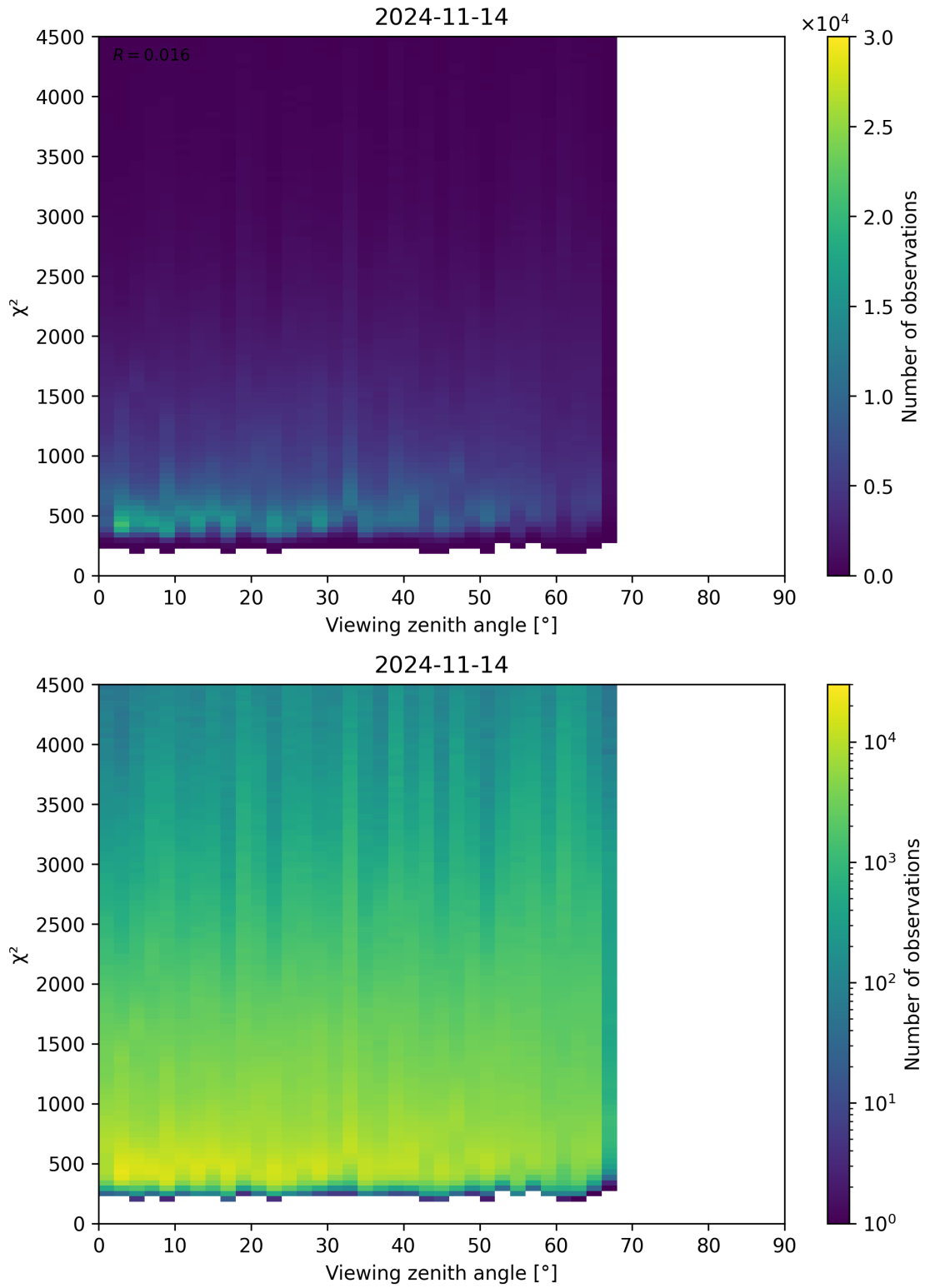
Figure 72: Scatter density plot of “Viewing zenith angle” against “ \chi^2 ” for 2024-11-14 to 2024-11-15.
