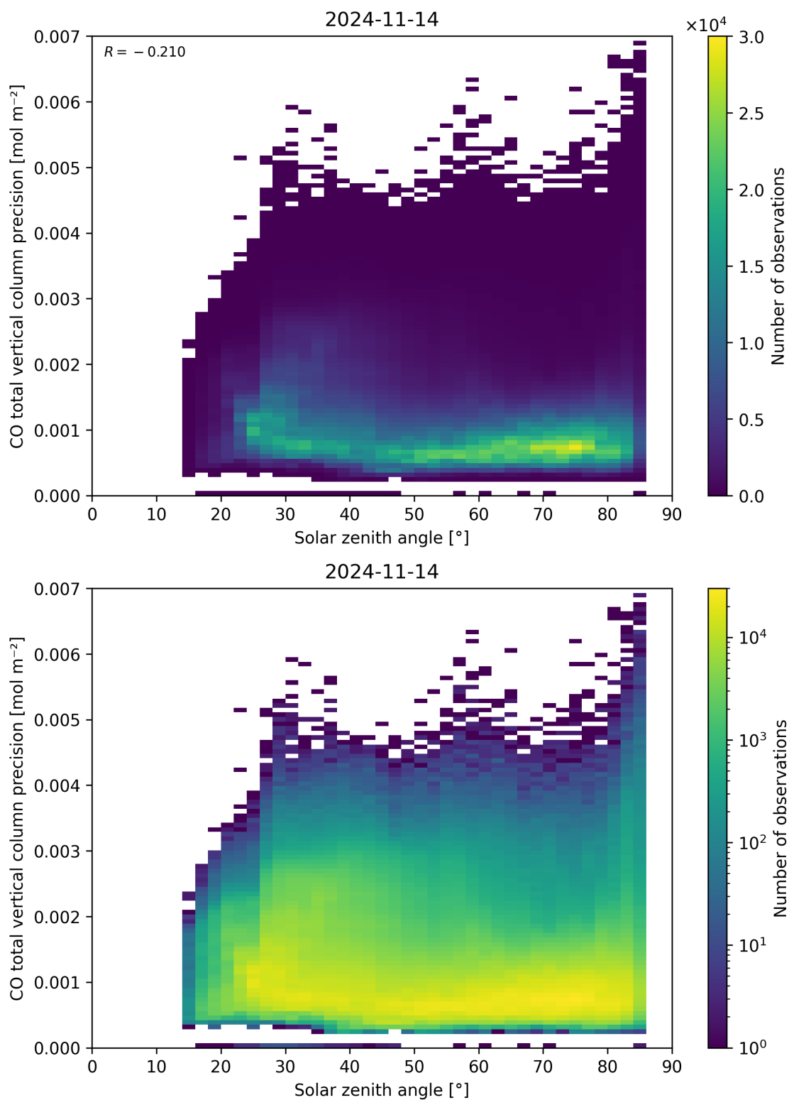
Figure 63: Scatter density plot of “Solar zenith angle” against “CO total vertical column precision” for 2024-11-14 to 2024-11-15.
