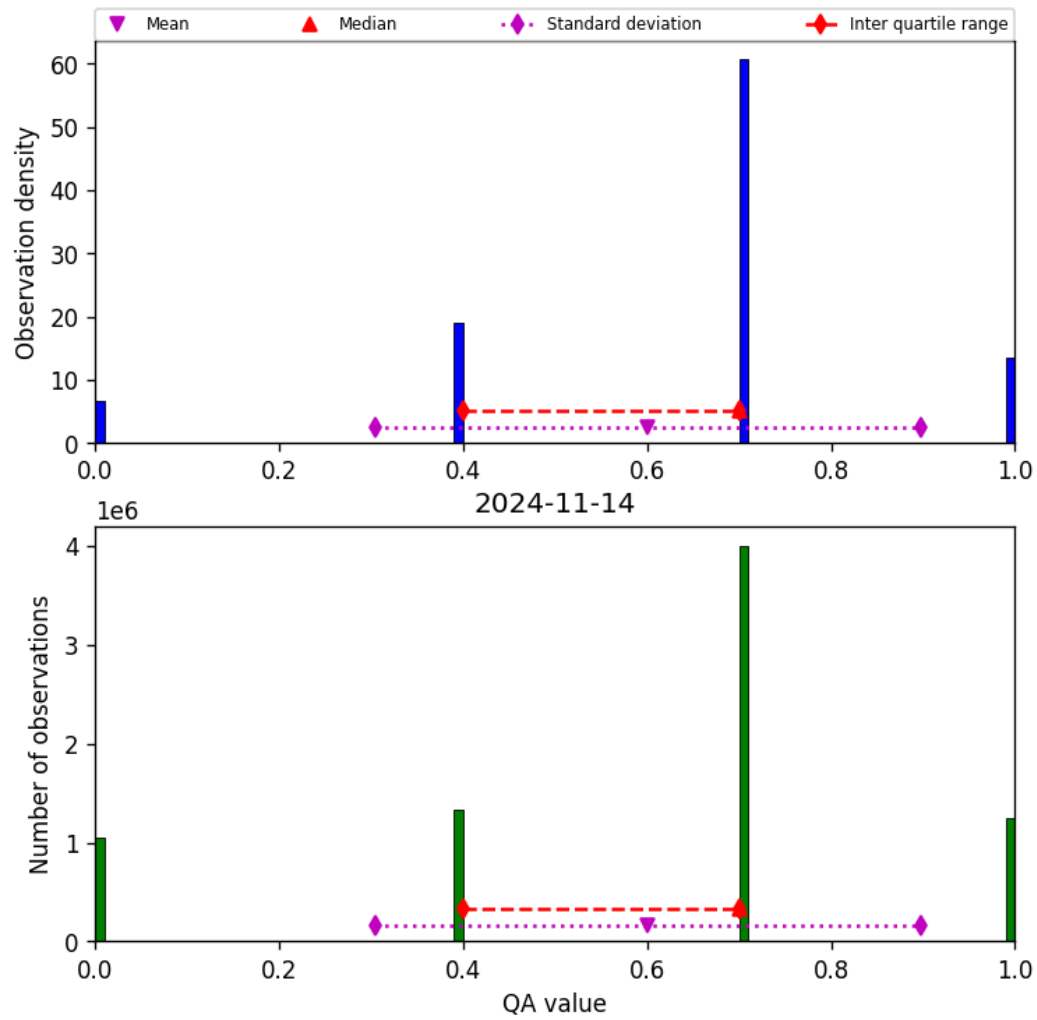
Figure 17: Histogram of “QA value” for 2024-11-14 to 2024-11-15
