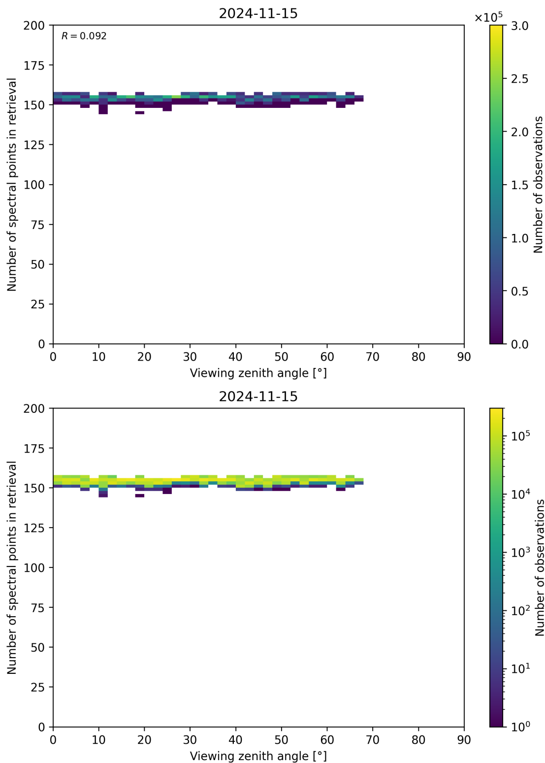
Figure 76: Scatter density plot of “Viewing zenith angle” against “Number of spectral points in retrieval” for 2024-11-14 to 2024-11-16.
