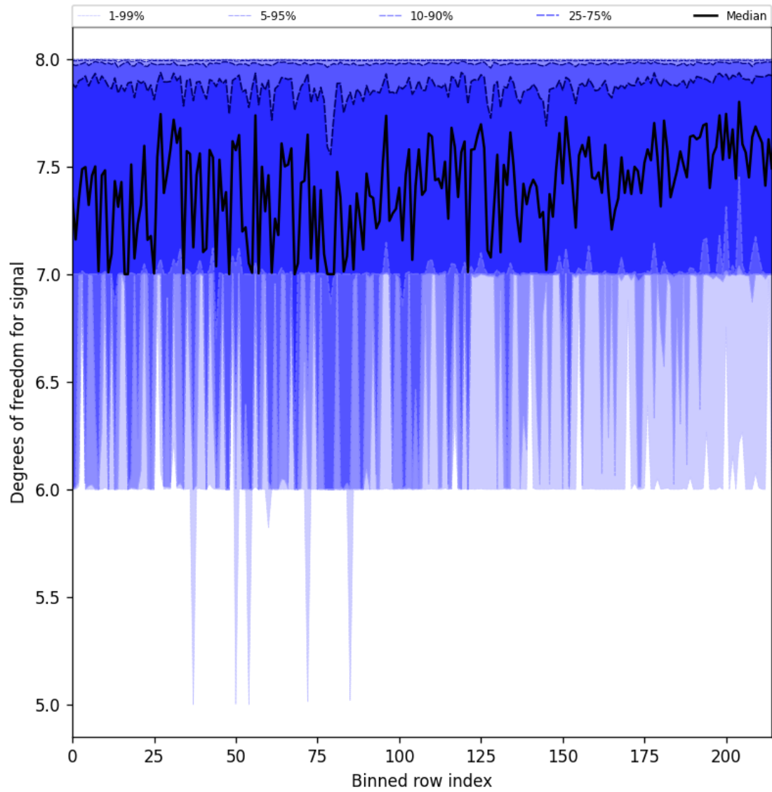
Figure 31: Along track statistics of “Degrees of freedom for signal” for 2024-11-14 to 2024-11-16
