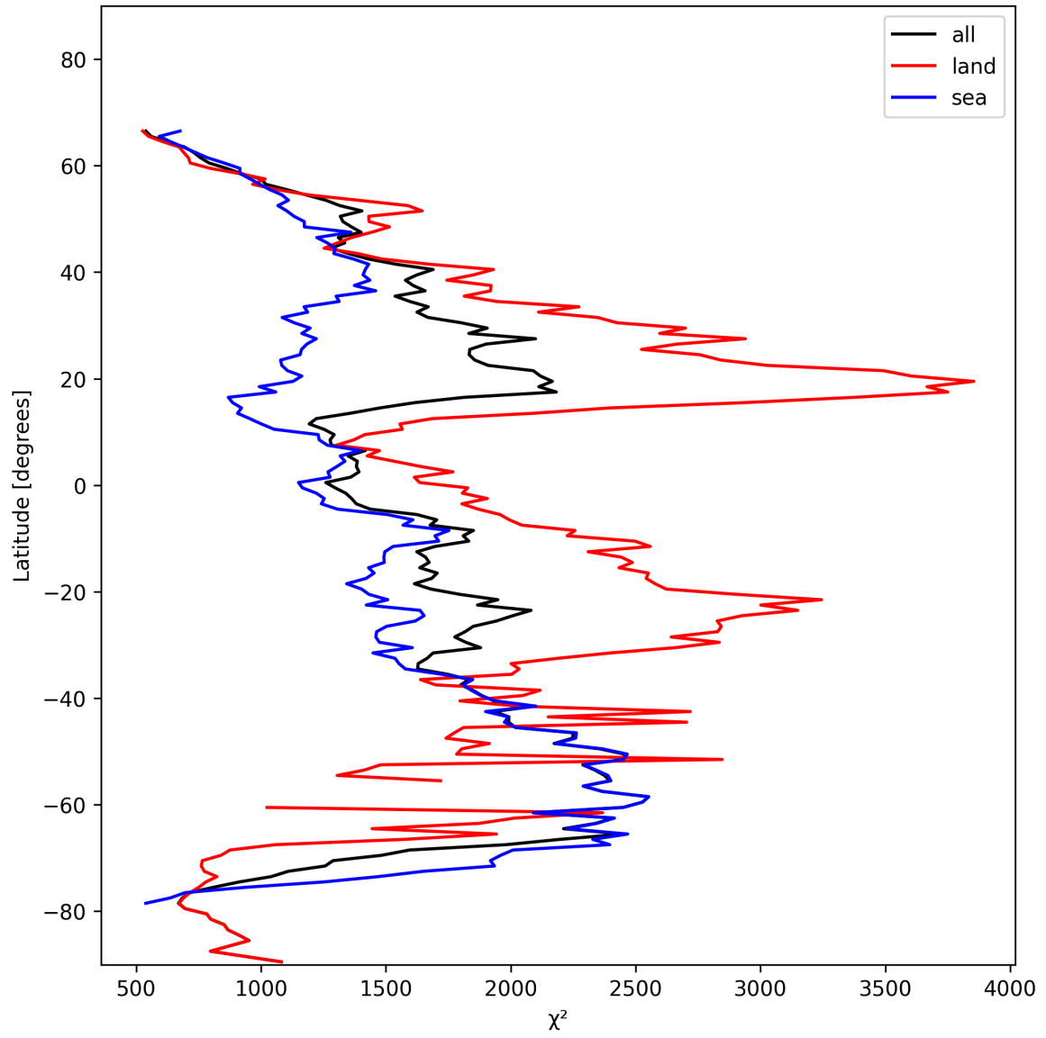
Figure 14: Zonal average of “ \chi^2 ” for 2024-11-14 to 2024-11-16.
