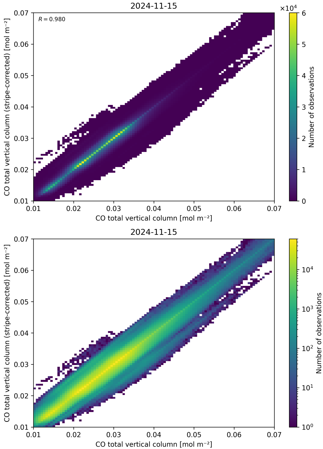
Figure 33: Scatter density plot of “CO total vertical column” against “CO total vertical column (stripe-corrected)” for 2024-11-14 to 2024-11-16.
