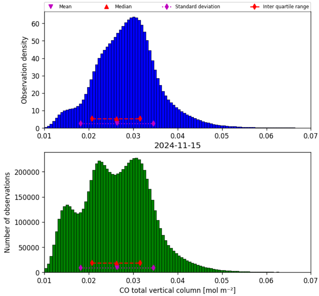
Figure 18: Histogram of “CO total vertical column” for 2024-11-14 to 2024-11-16
