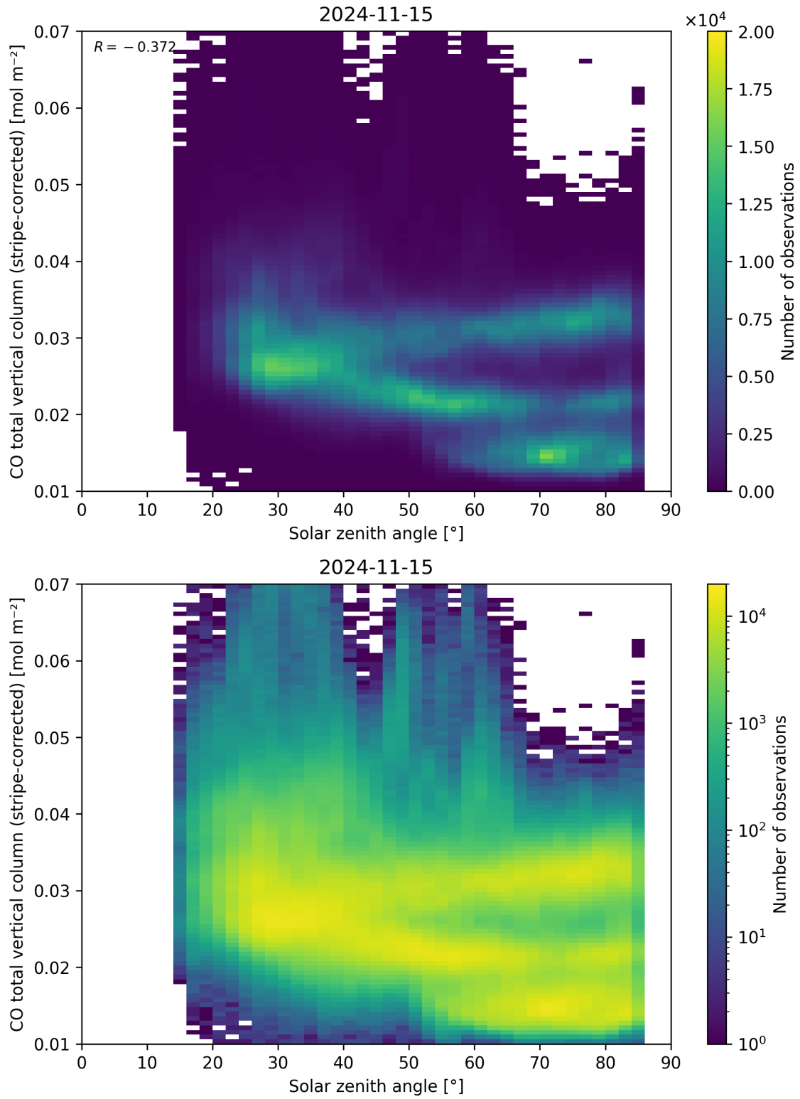
Figure 62: Scatter density plot of “Solar zenith angle” against “CO total vertical column (stripe-corrected)” for 2024-11-14 to 2024-11-16.
