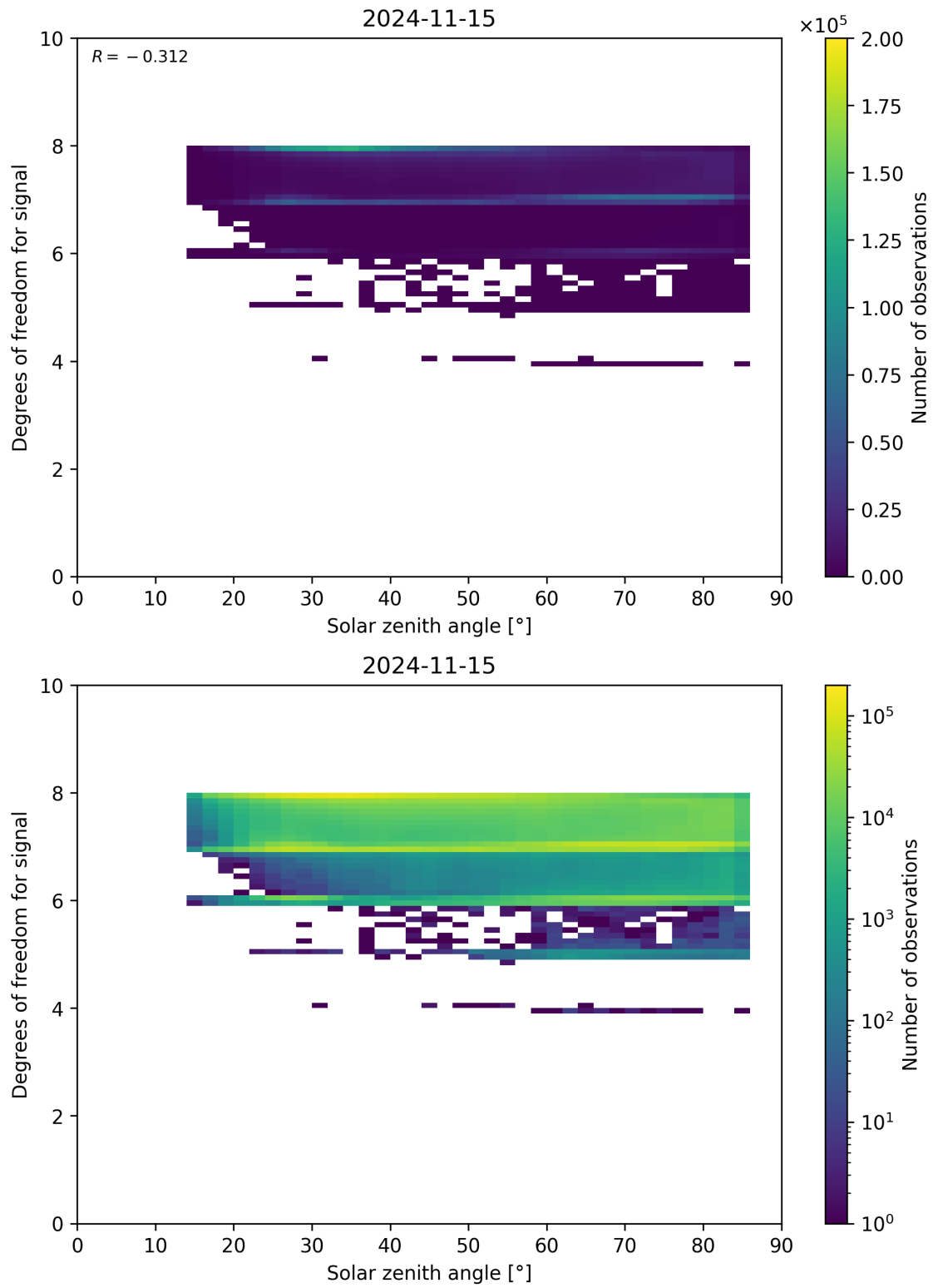
Figure 65: Scatter density plot of “Solar zenith angle” against “Degrees of freedom for signal” for 2024-11-14 to 2024-11-16.
