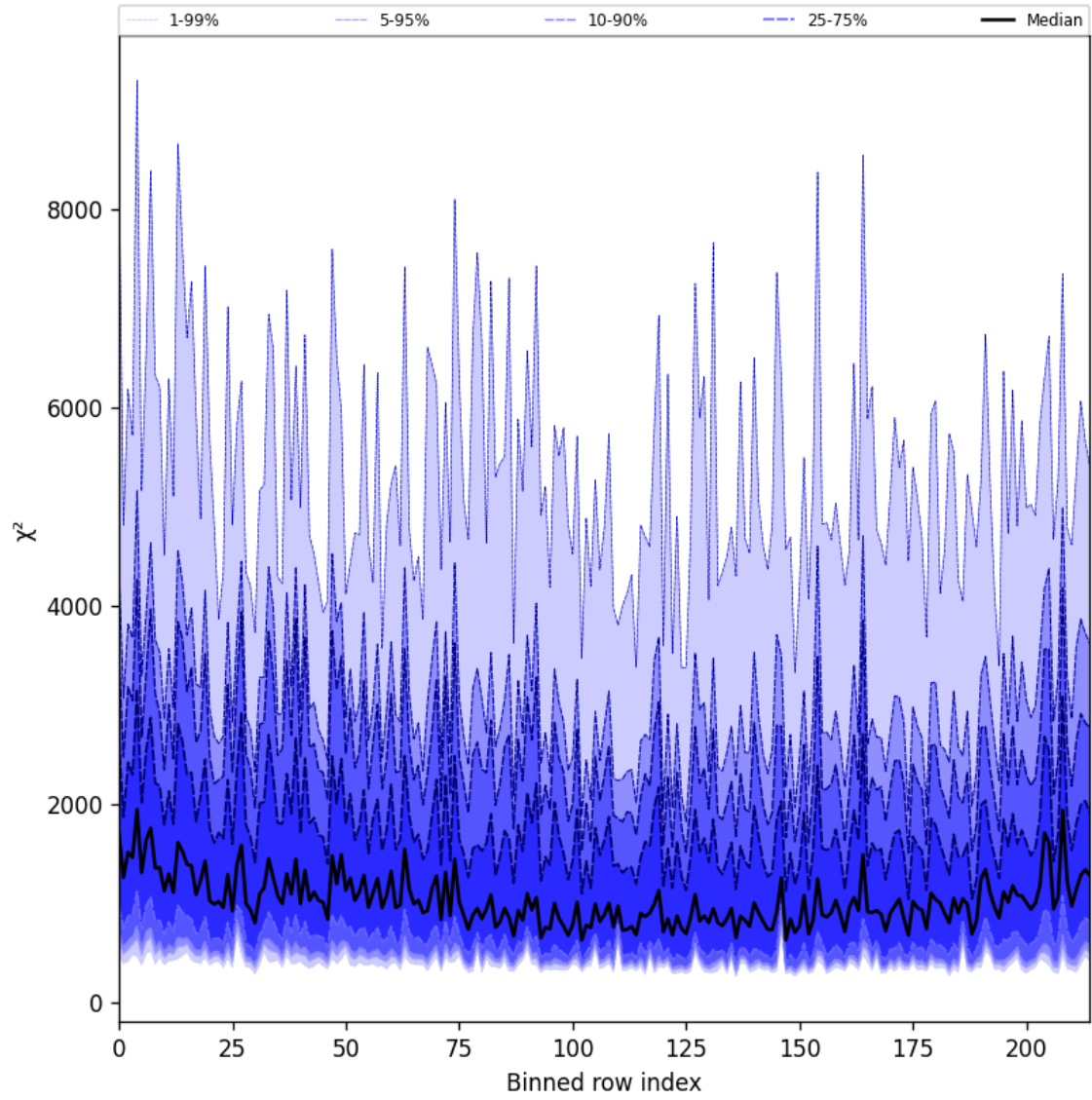
Figure 30: Along track statistics of “ \chi^2 ” for 2024-11-14 to 2024-11-16
