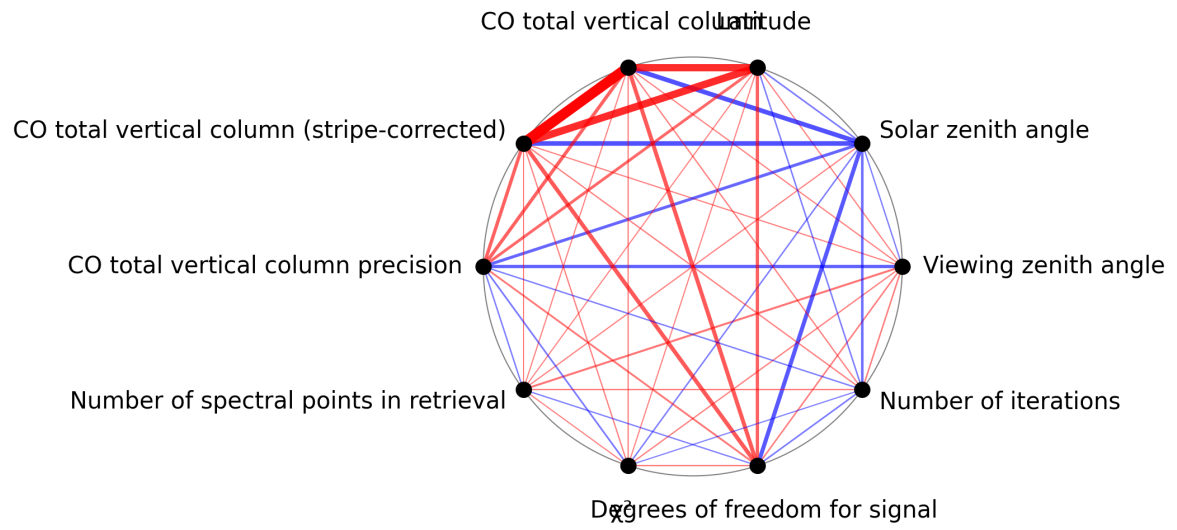
Figure 1: Map of correlation graph for 2024-11-14 to 2024-11-16.
