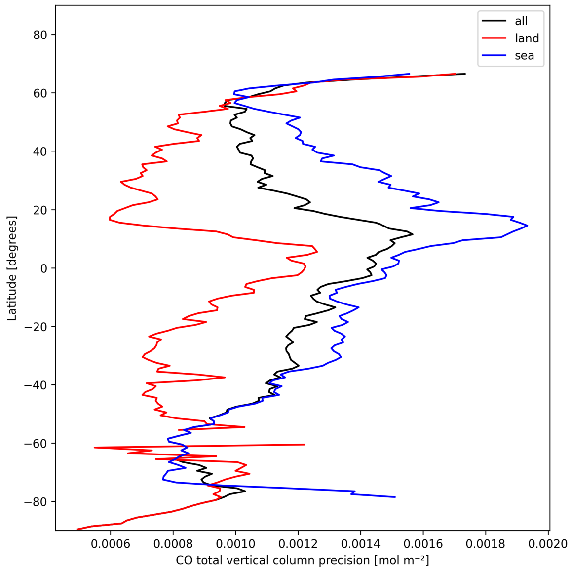
Figure 12: Zonal average of “CO total vertical column precision” for 2024-11-14 to 2024-11-16.
