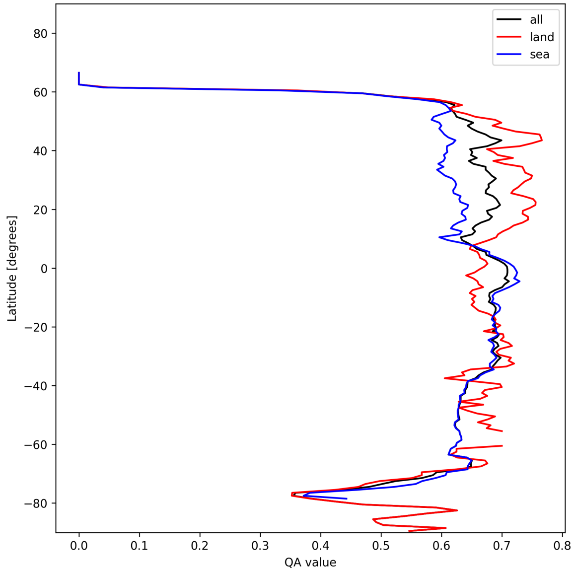
Figure 9: Zonal average of “QA value” for 2024-11-14 to 2024-11-16.
