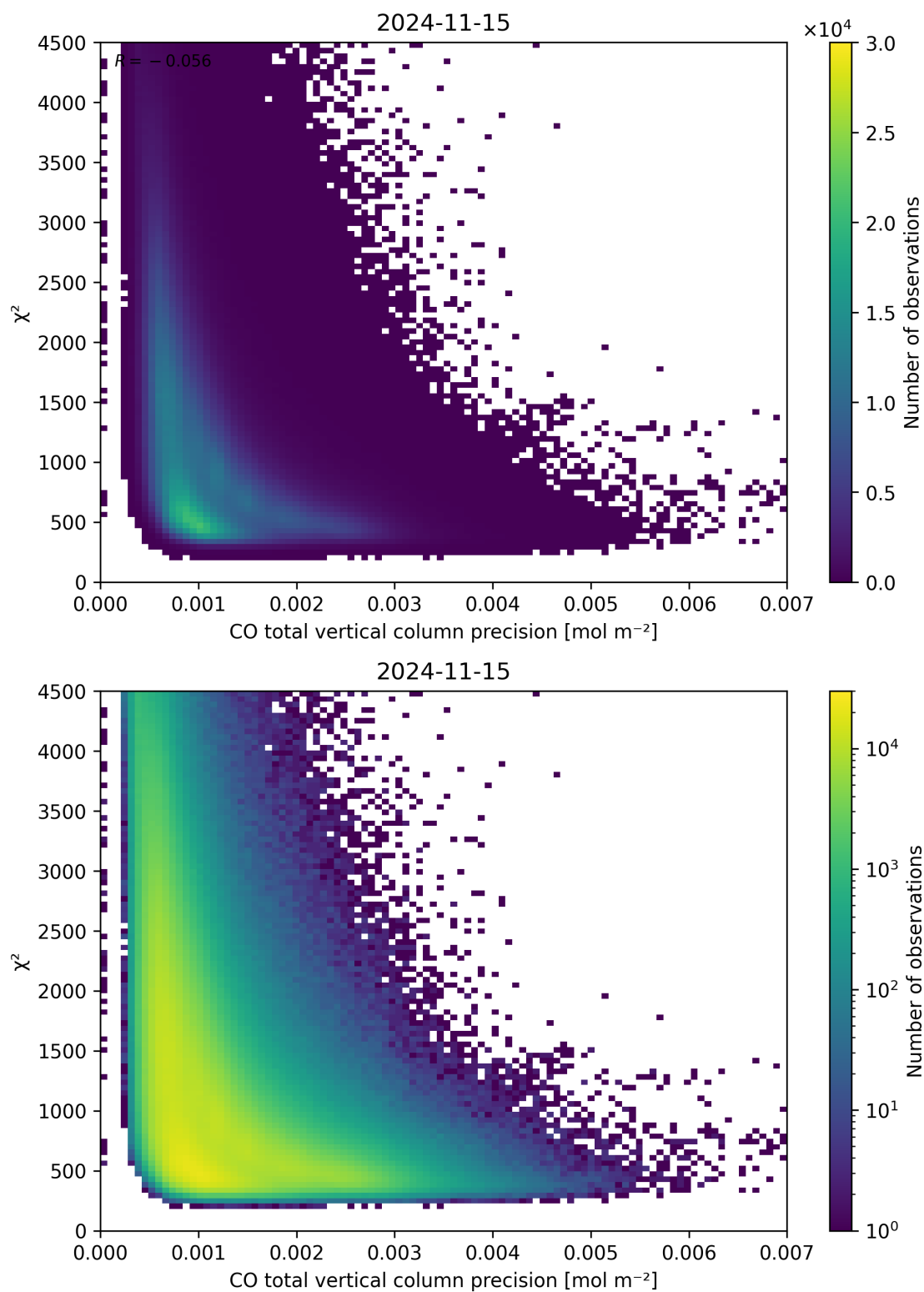
Figure 44: Scatter density plot of “CO total vertical column precision” against “ \chi^2 ” for 2024-11-14 to 2024-11-16.
