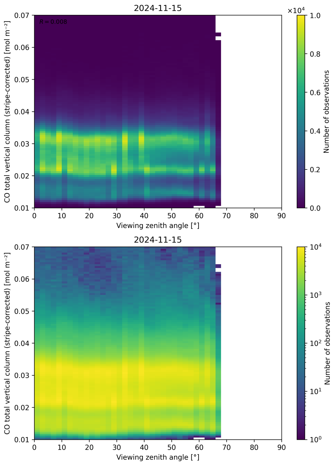
Figure 70: Scatter density plot of “Viewing zenith angle” against “CO total vertical column (stripe-corrected)” for 2024-11-14 to 2024-11-16.
