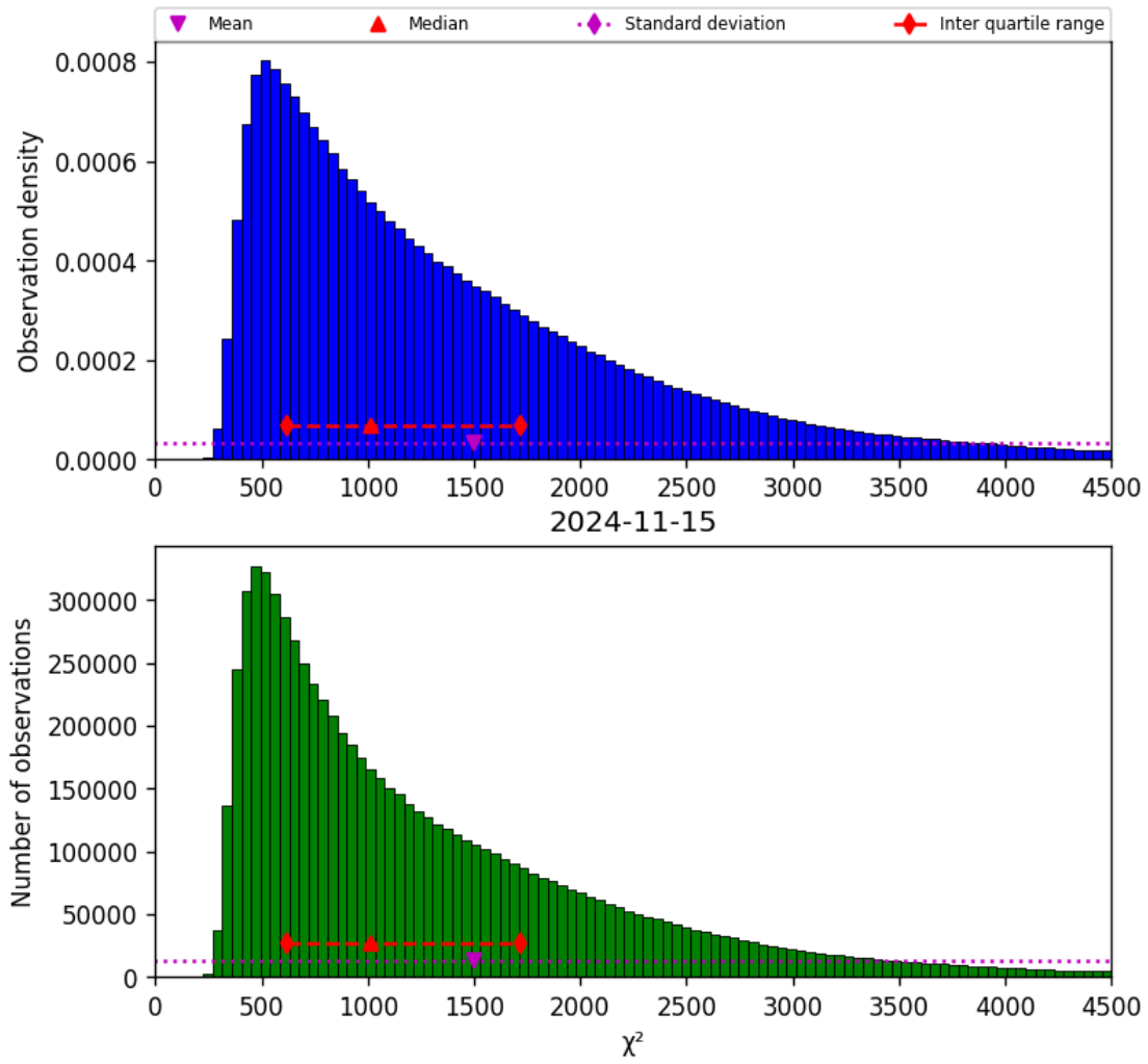
Figure 22: Histogram of “ \chi^2 ” for 2024-11-14 to 2024-11-16
