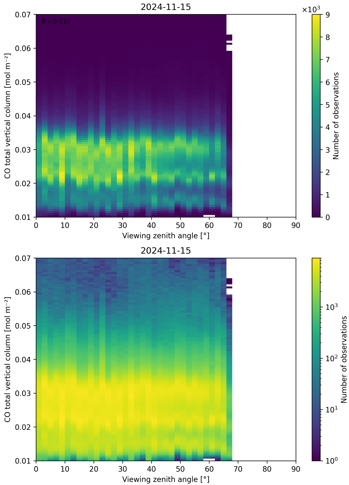
Figure 69: Scatter density plot of “Viewing zenith angle” against “CO total vertical column” for 2024-11-14 to 2024-11-16.
