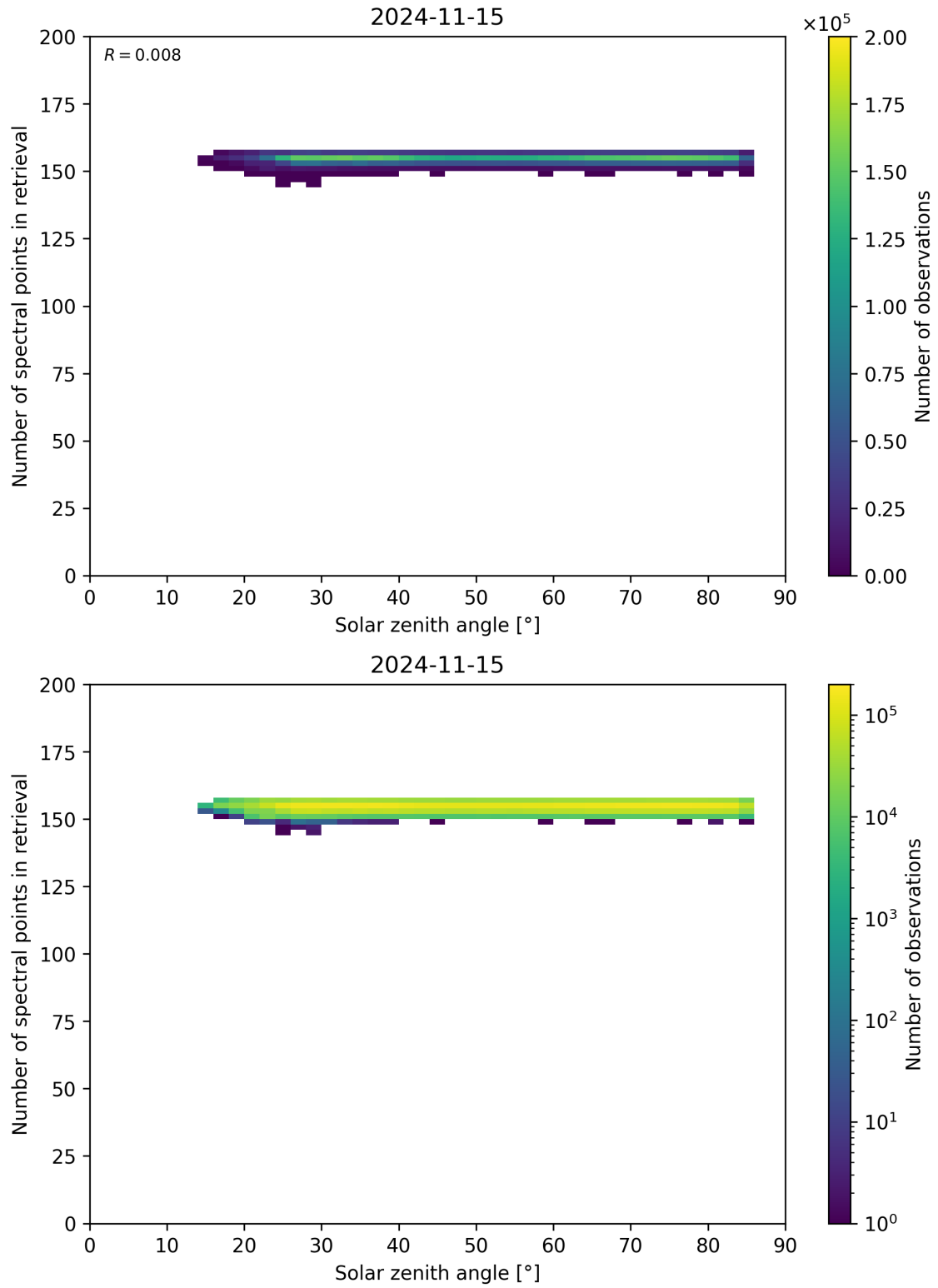
Figure 68: Scatter density plot of “Solar zenith angle” against “Number of spectral points in retrieval” for 2024-11-14 to 2024-11-16.
