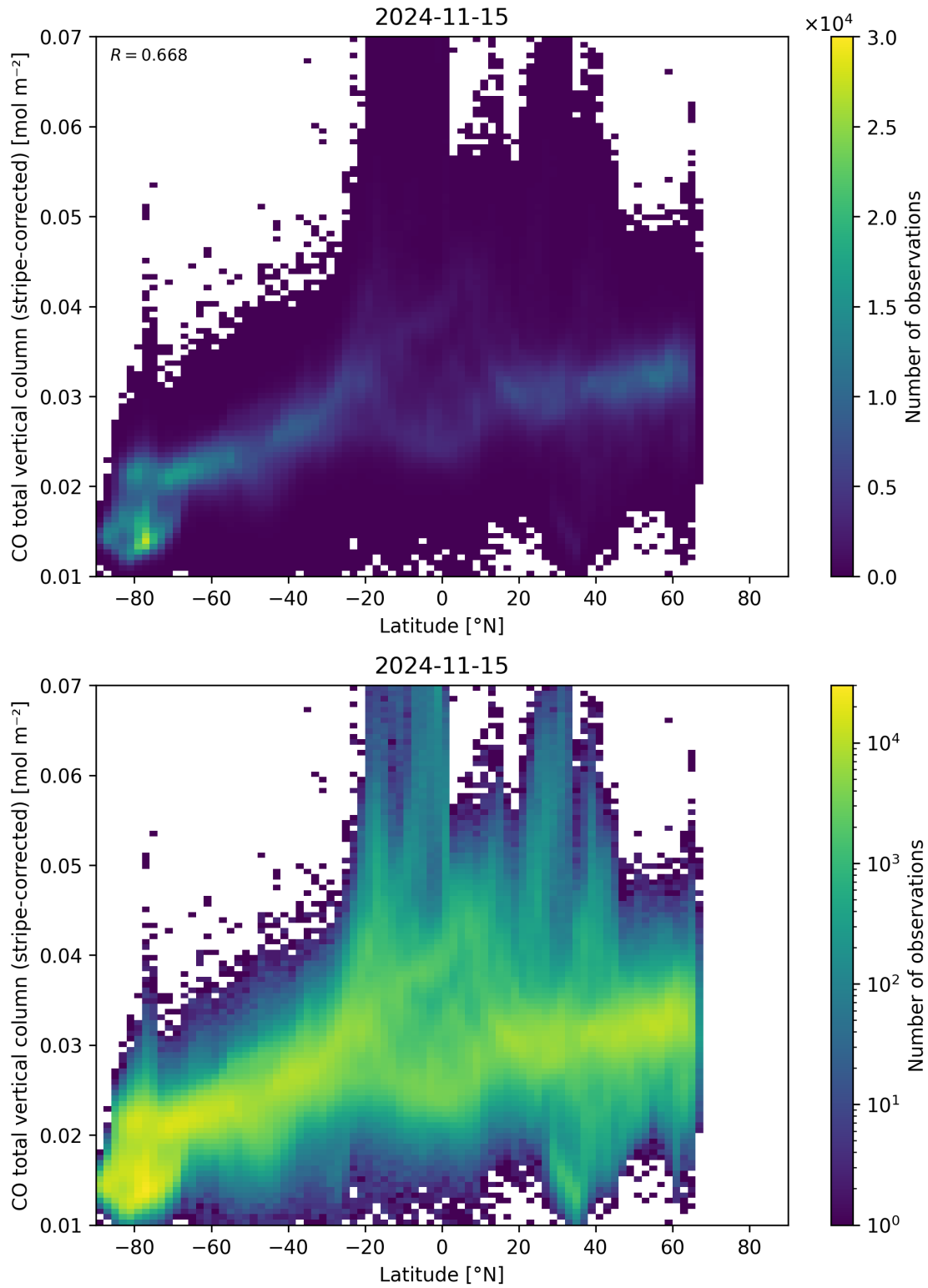
Figure 52: Scatter density plot of “Latitude” against “CO total vertical column (stripe-corrected)” for 2024-11-14 to 2024-11-16.
