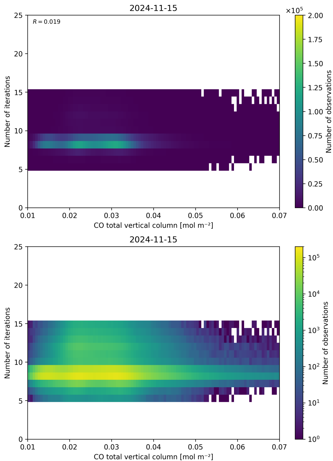
Figure 42: Scatter density plot of “CO total vertical column” against “Number of iterations” for 2024-11-14 to 2024-11-16.
