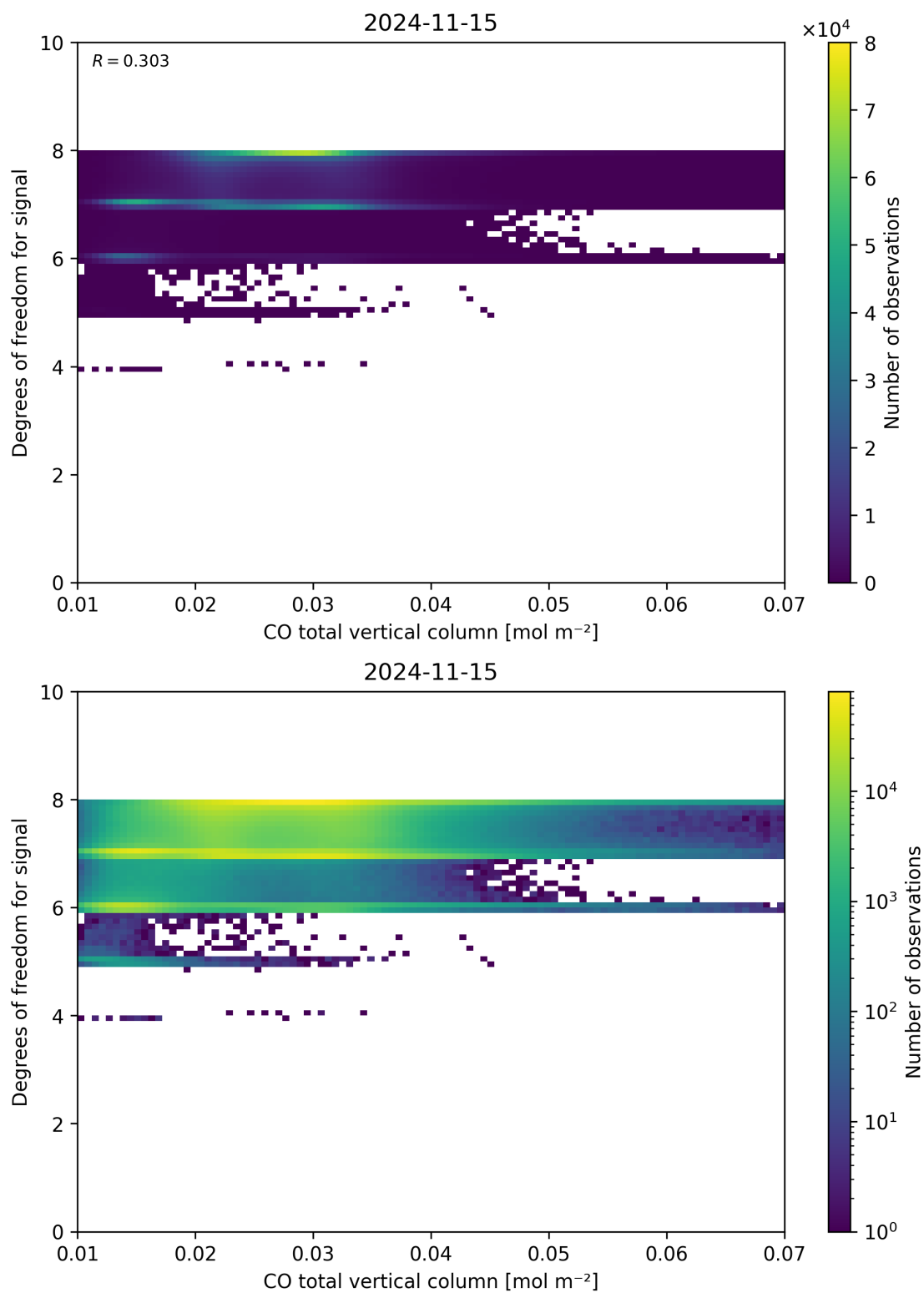
Figure 41: Scatter density plot of “CO total vertical column” against “Degrees of freedom for signal” for 2024-11-14 to 2024-11-16.
