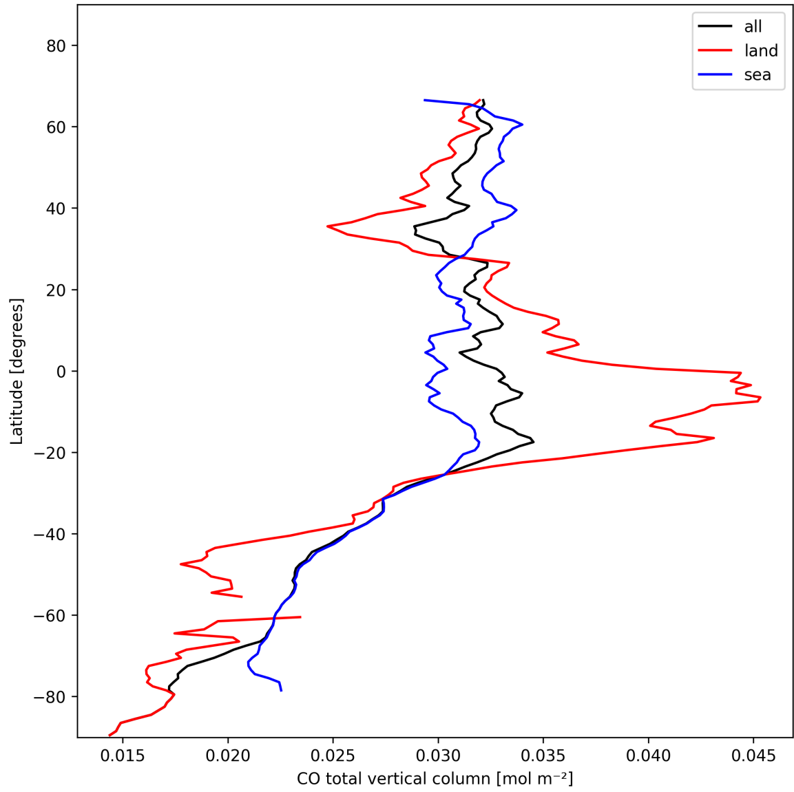
Figure 10: Zonal average of “CO total vertical column” for 2024-11-14 to 2024-11-16.
