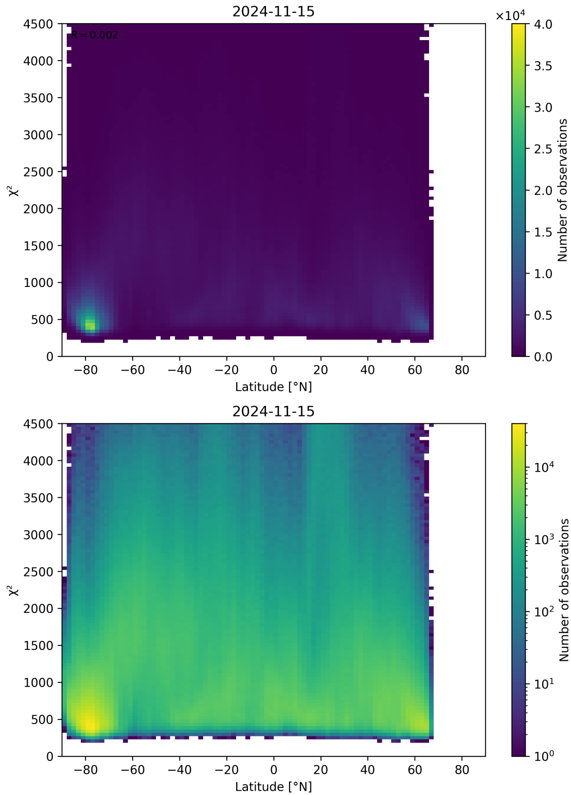
Figure 54: Scatter density plot of “Latitude” against “ \chi^2 ” for 2024-11-14 to 2024-11-16.
