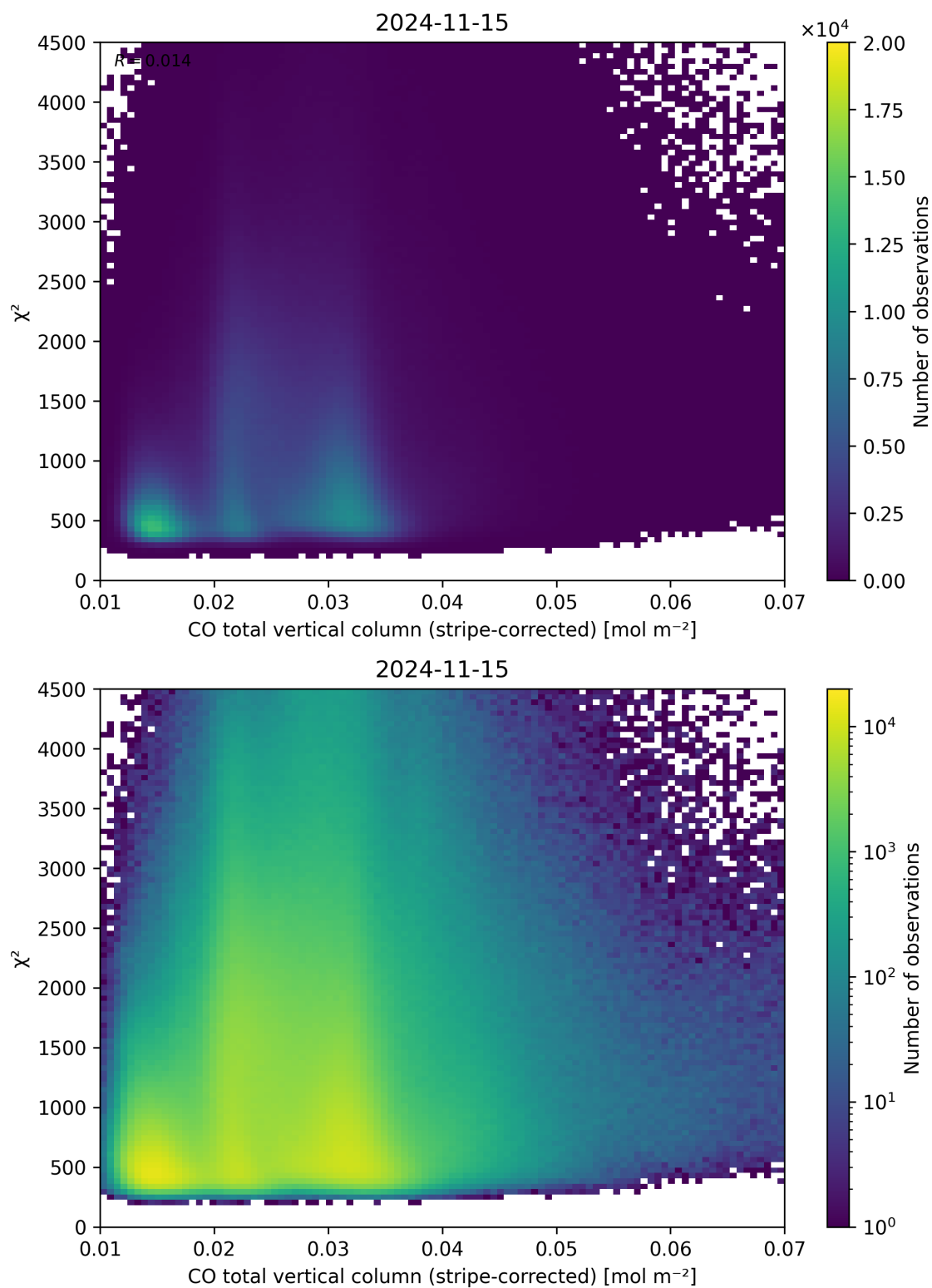
Figure 37: Scatter density plot of “CO total vertical column (stripe-corrected)” against “ \chi^2 ” for 2024-11-14 to 2024-11-16.
