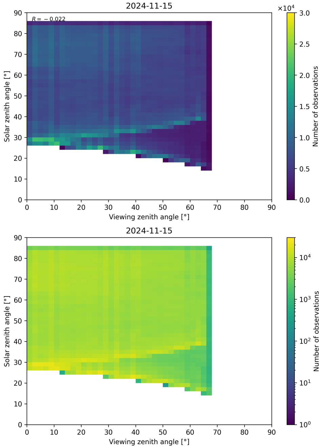
Figure 77: Scatter density plot of “Viewing zenith angle” against “Solar zenith angle” for 2024-11-14 to 2024-11-16.
