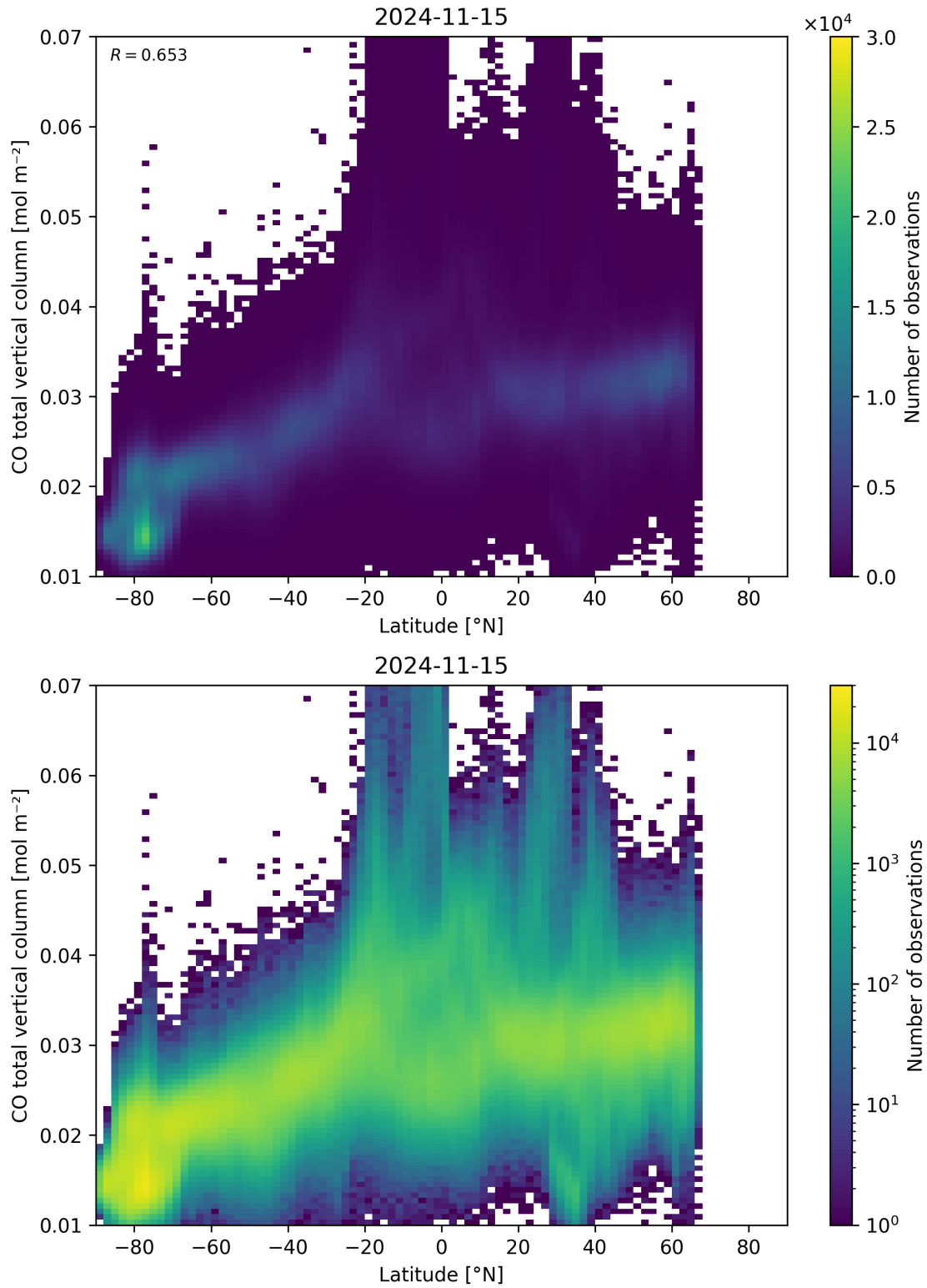
Figure 51: Scatter density plot of “Latitude” against “CO total vertical column” for 2024-11-14 to 2024-11-16.
