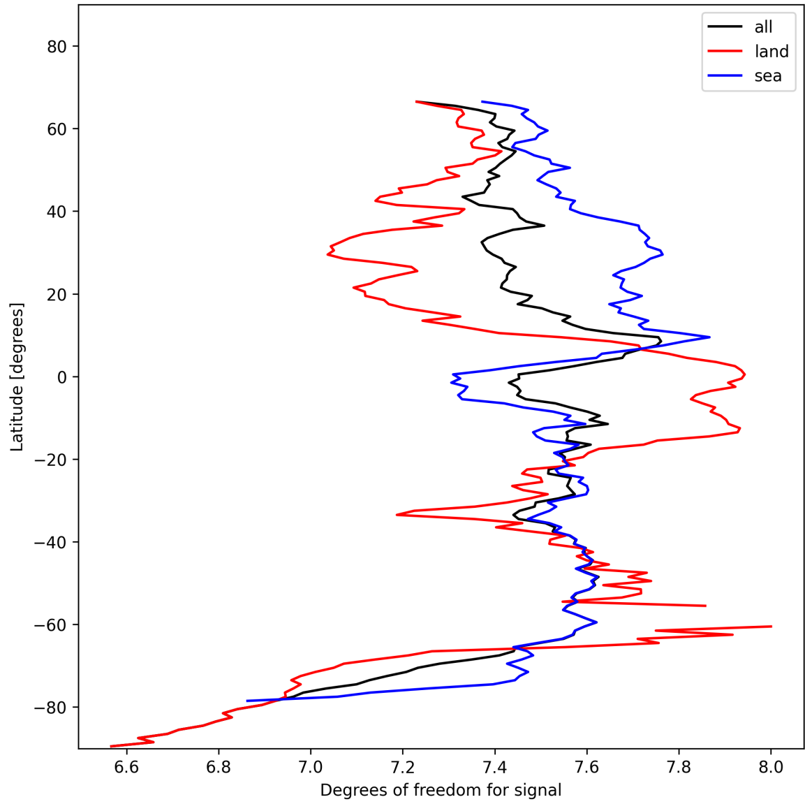
Figure 15: Zonal average of “Degrees of freedom for signal” for 2024-11-14 to 2024-11-16.
