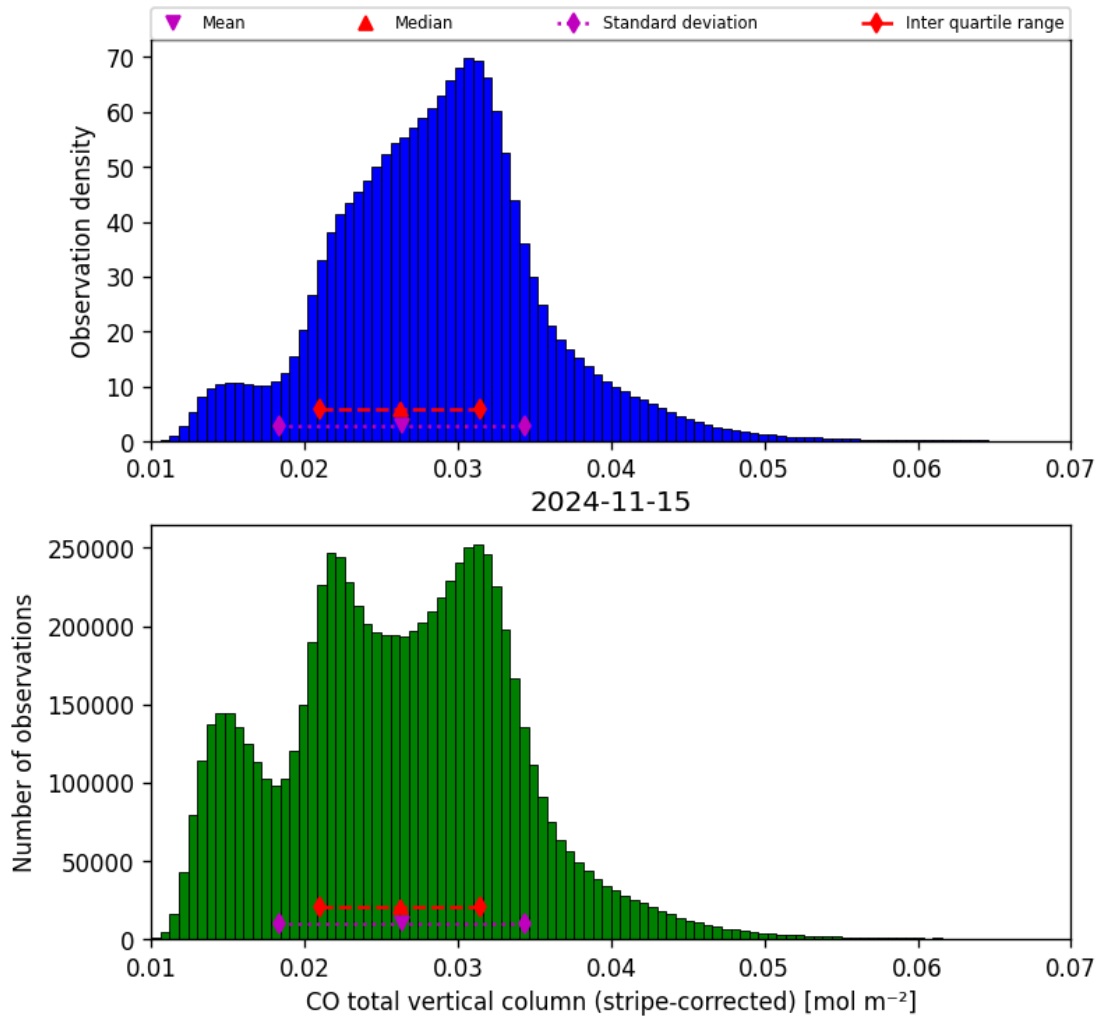
Figure 19: Histogram of “CO total vertical column (stripe-corrected)” for 2024-11-14 to 2024-11-16
