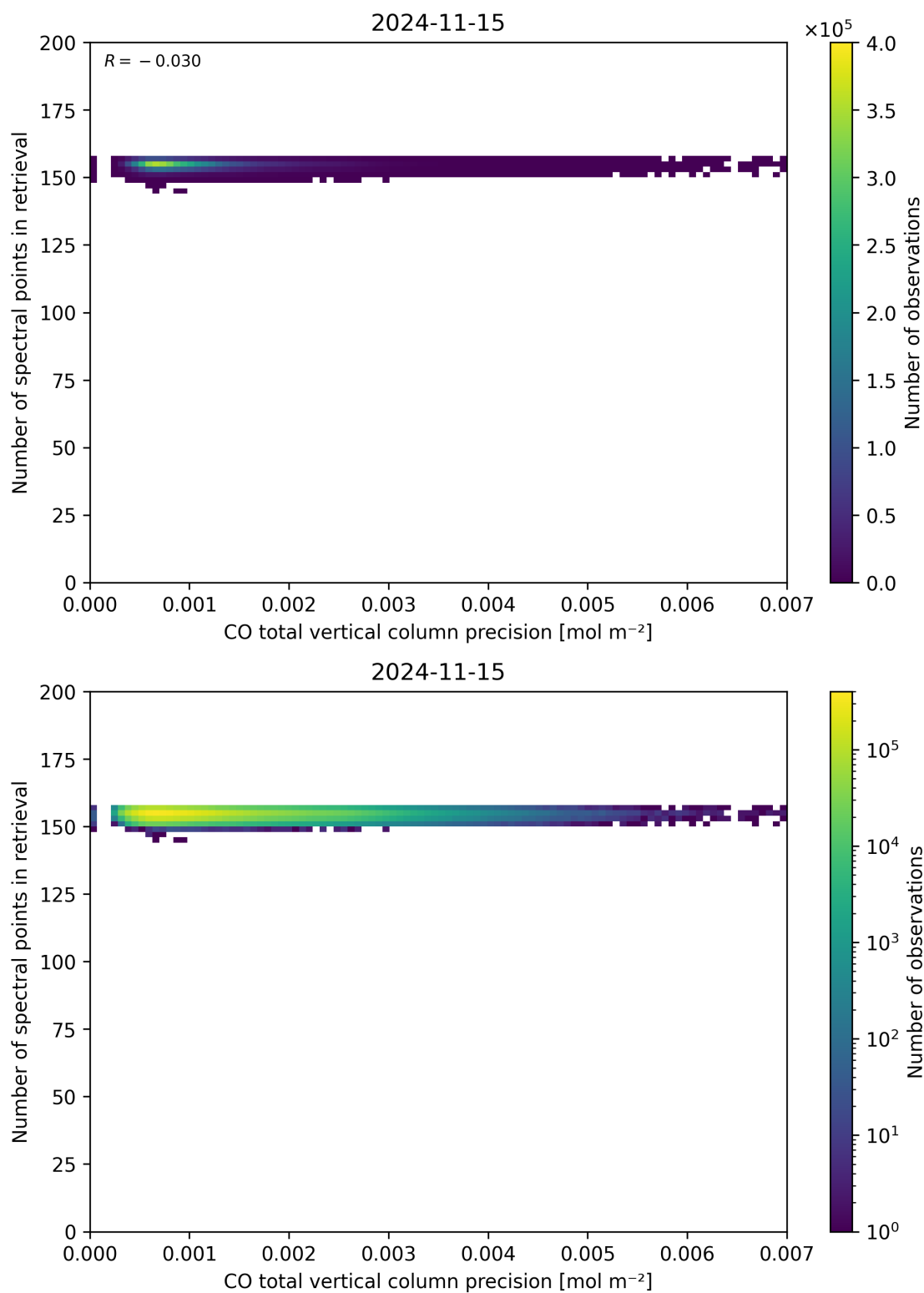
Figure 47: Scatter density plot of “CO total vertical column precision” against “Number of spectral points in retrieval” for 2024-11-14 to 2024-11-16.
