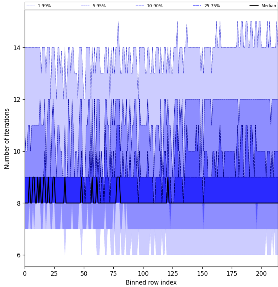
Figure 32: Along track statistics of “Number of iterations” for 2024-11-14 to 2024-11-16
