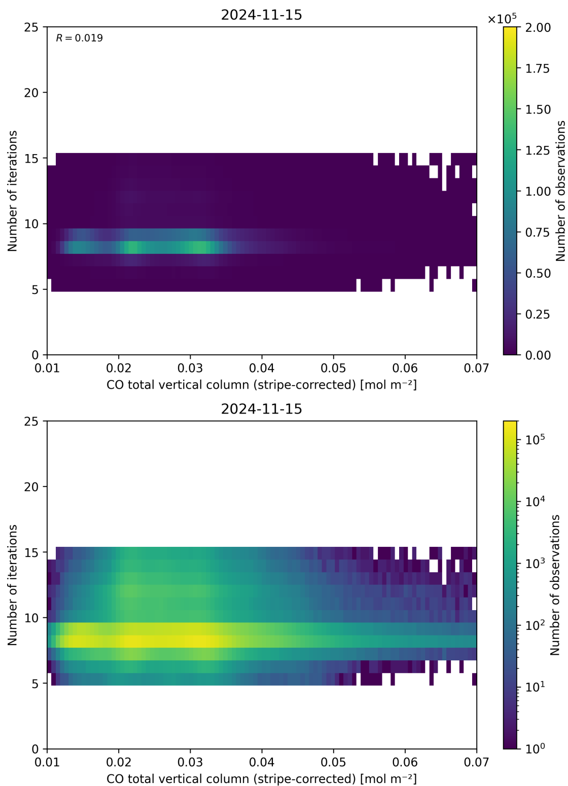
Figure 39: Scatter density plot of “CO total vertical column (stripe-corrected)” against “Number of iterations” for 2024-11-14 to 2024-11-16.
