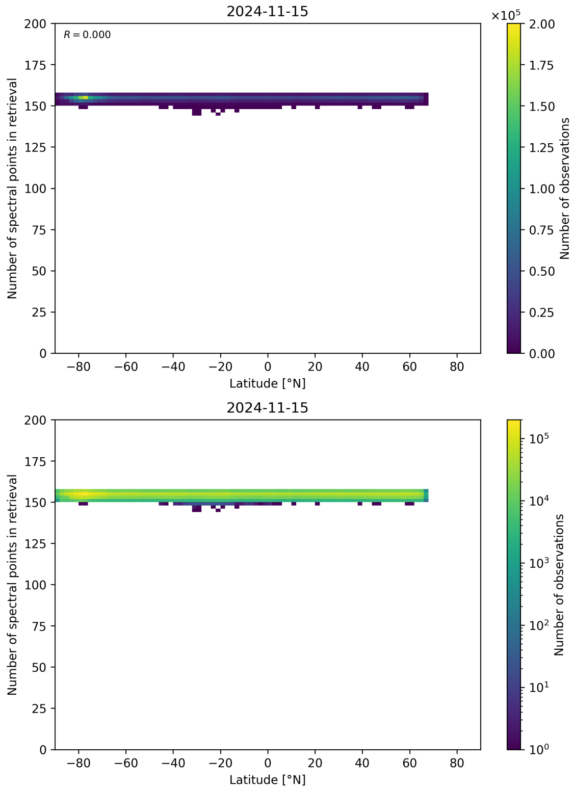
Figure 57: Scatter density plot of “Latitude” against “Number of spectral points in retrieval” for 2024-11-14 to 2024-11-16.
