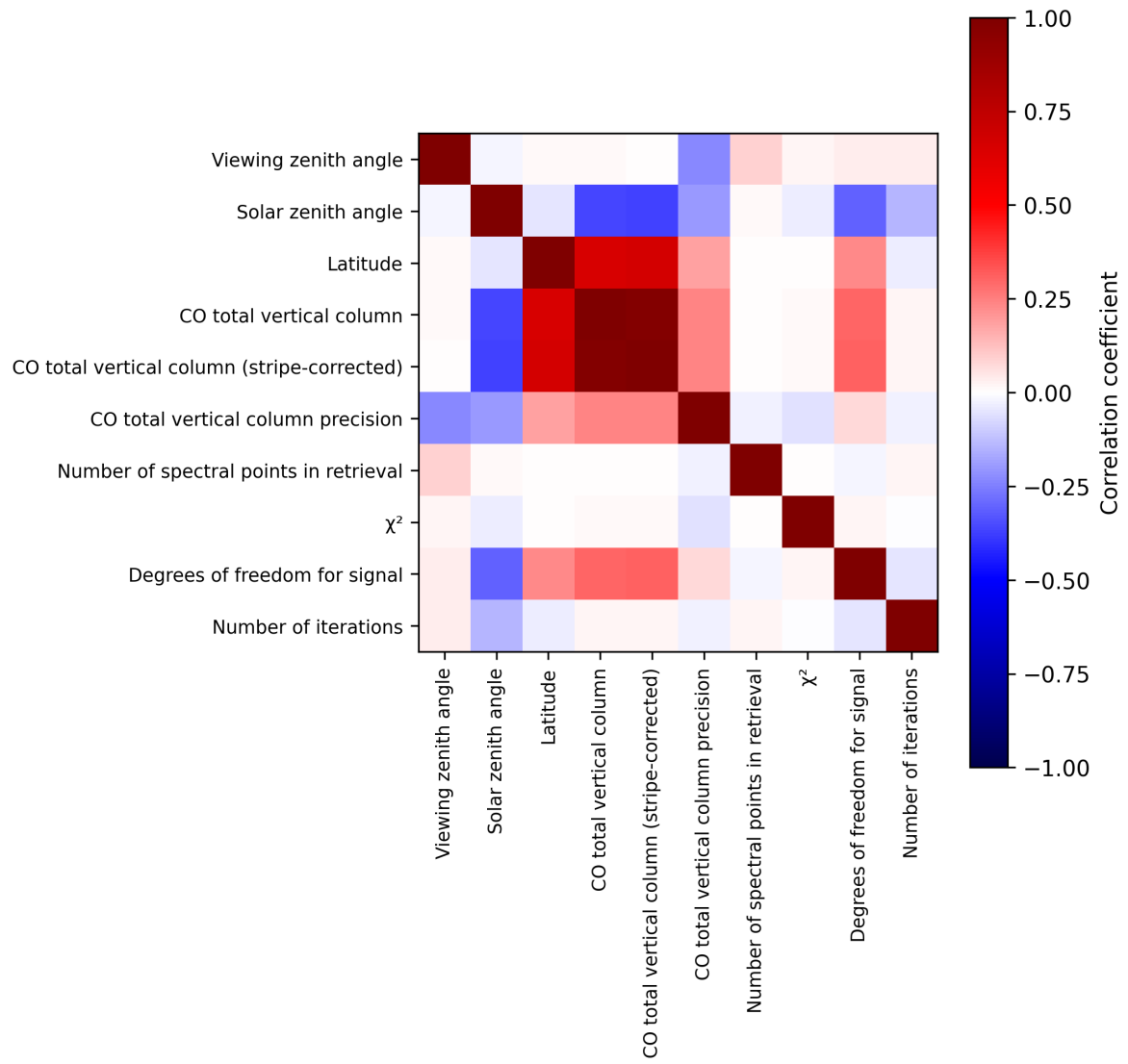
Figure 2: Map of correlation matrix for 2024-11-14 to 2024-11-16.
