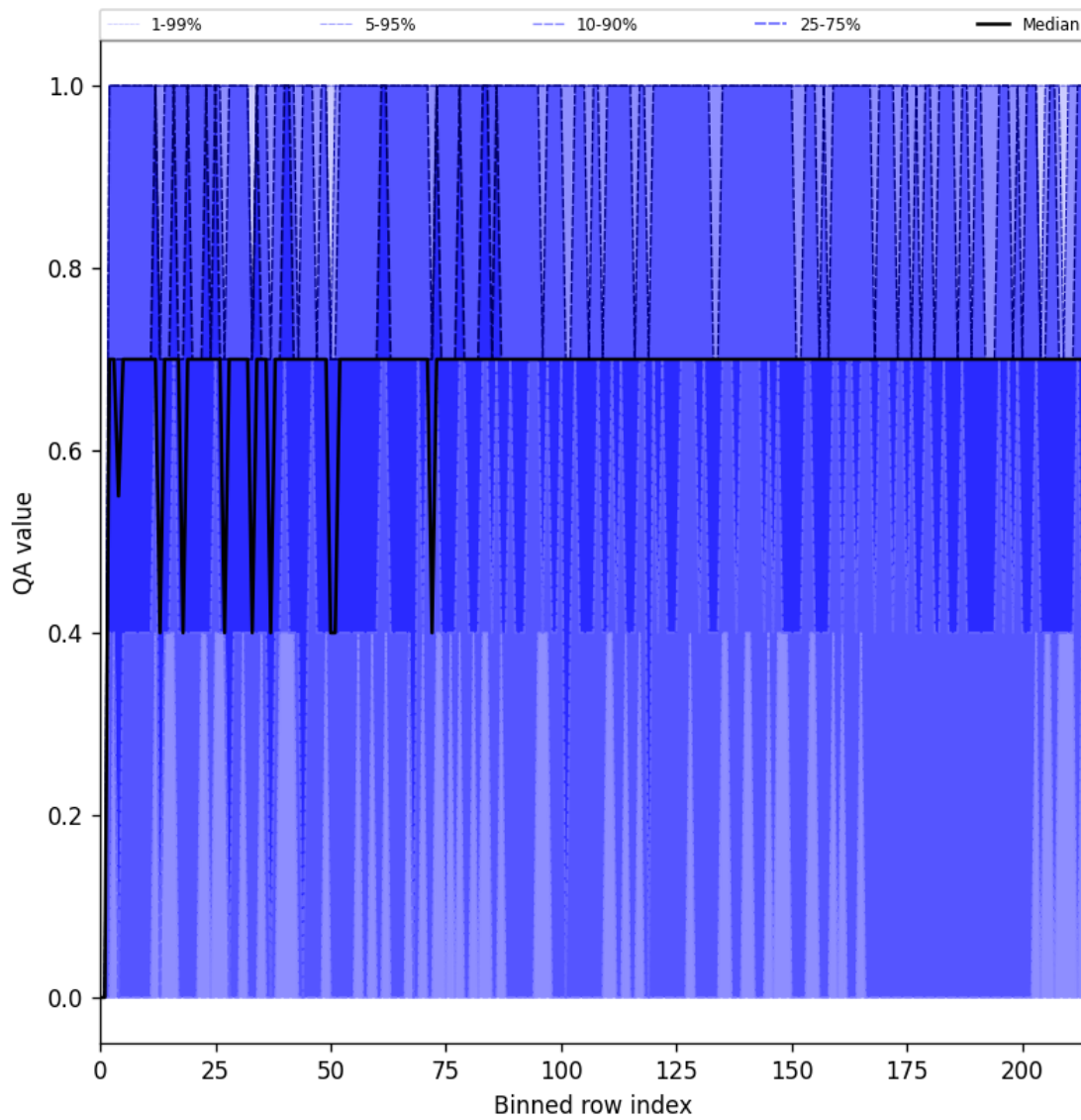
Figure 25: Along track statistics of “QA value” for 2024-11-14 to 2024-11-16
