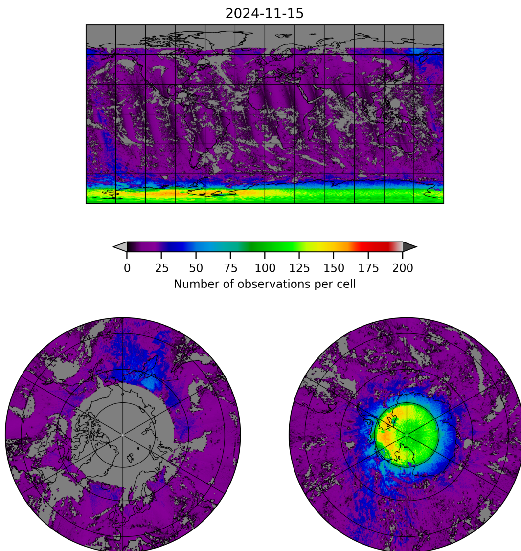
Figure 8: Map of the number of observations for 2024-11-14 to 2024-11-16
