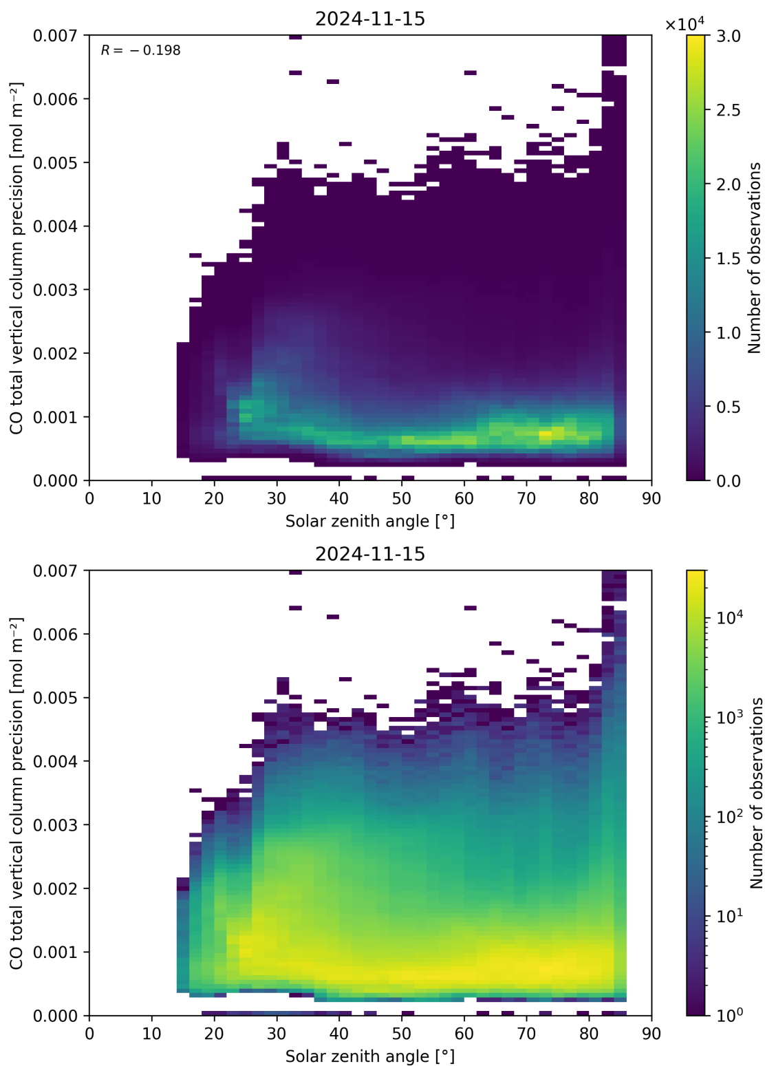
Figure 63: Scatter density plot of “Solar zenith angle” against “CO total vertical column precision” for 2024-11-14 to 2024-11-16.
