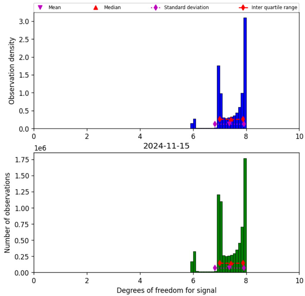
Figure 23: Histogram of “Degrees of freedom for signal” for 2024-11-14 to 2024-11-16
