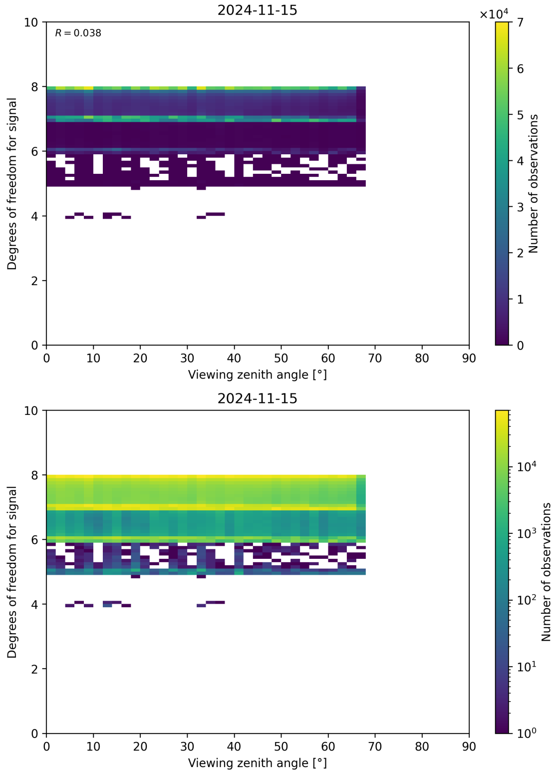
Figure 73: Scatter density plot of “Viewing zenith angle” against “Degrees of freedom for signal” for 2024-11-14 to 2024-11-16.
