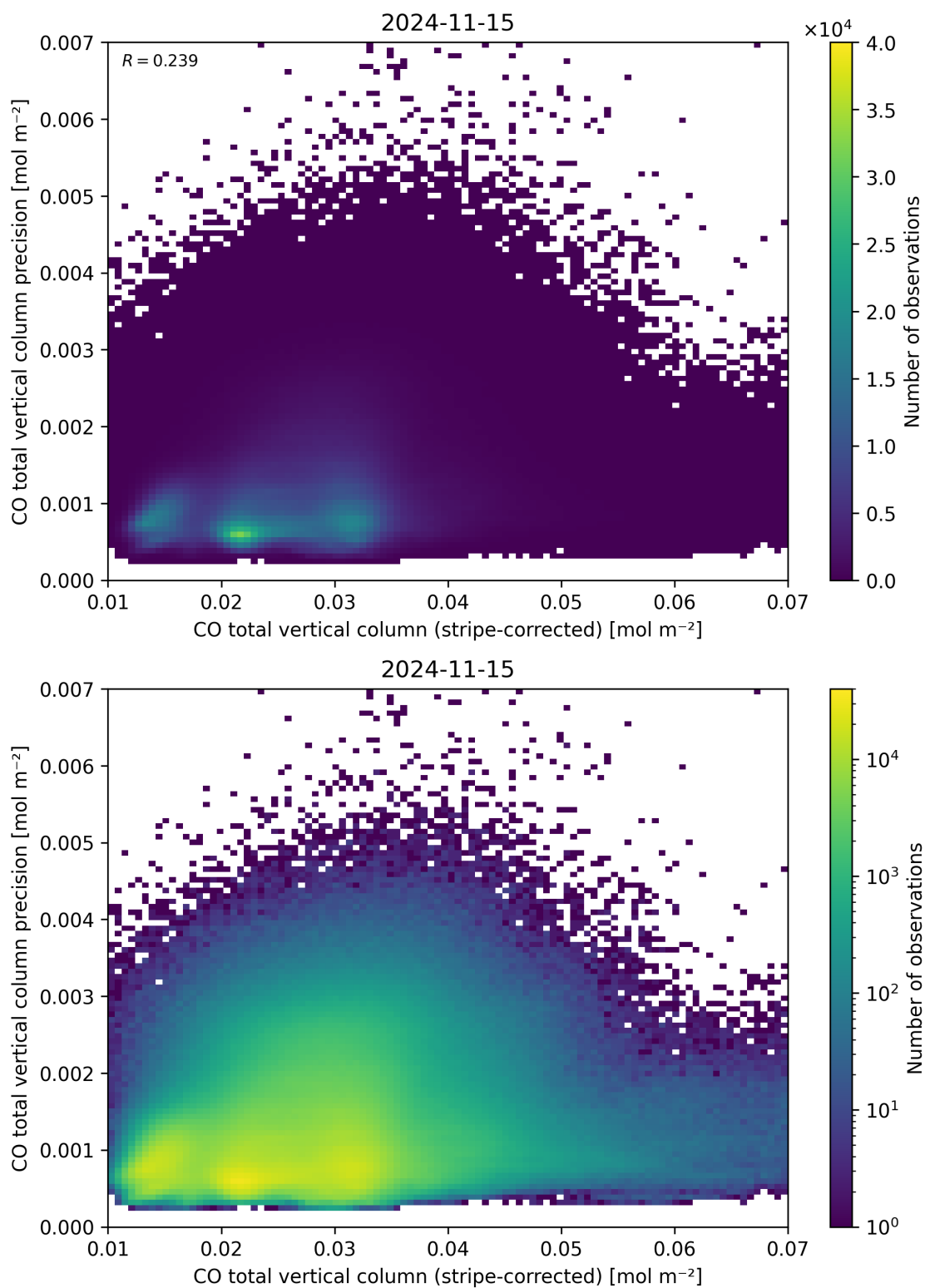
Figure 36: Scatter density plot of “CO total vertical column (stripe-corrected)” against “CO total vertical column precision” for 2024-11-14 to 2024-11-16.
