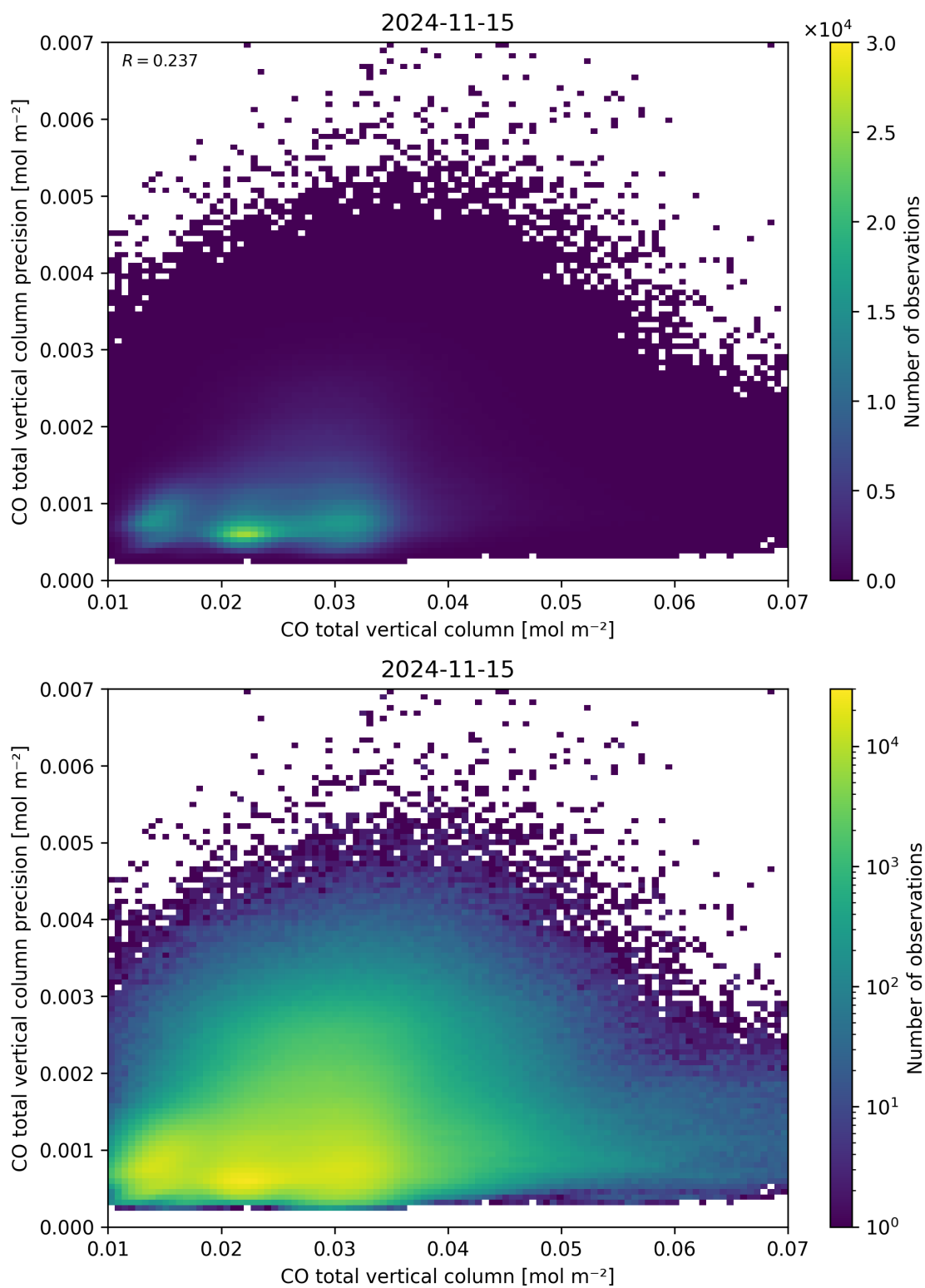
Figure 34: Scatter density plot of “CO total vertical column” against “CO total vertical column precision” for 2024-11-14 to 2024-11-16.
