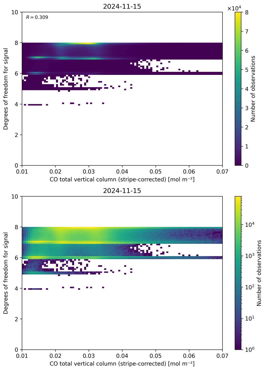
Figure 38: Scatter density plot of “CO total vertical column (stripe-corrected)” against “Degrees of freedom for signal” for 2024-11-14 to 2024-11-16.
