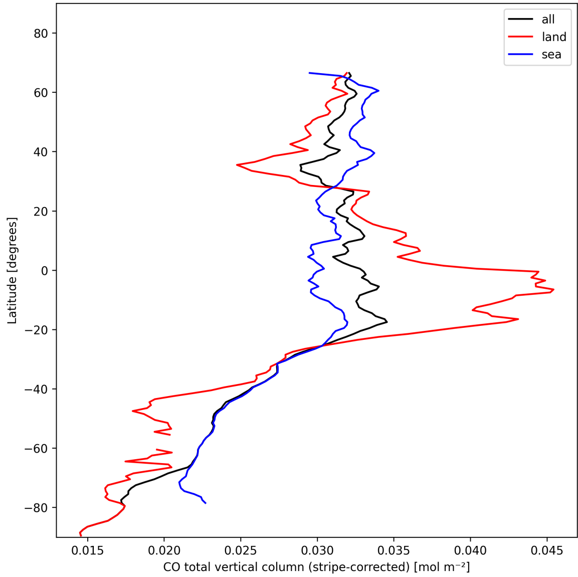
Figure 11: Zonal average of “CO total vertical column (stripe-corrected)” for 2024-11-14 to 2024-11-16.
