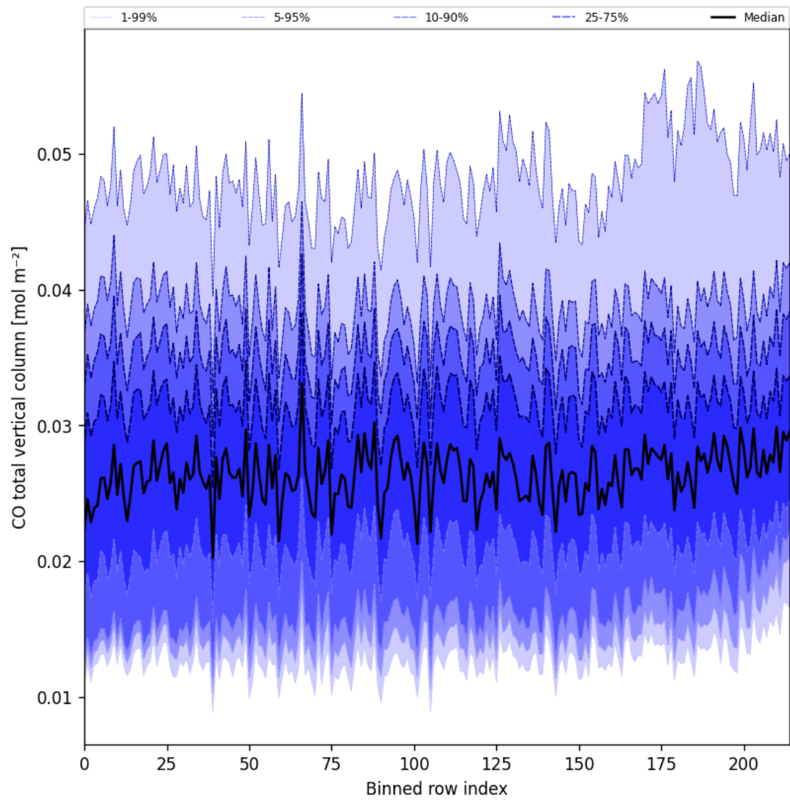
Figure 26: Along track statistics of “CO total vertical column” for 2024-11-14 to 2024-11-16
