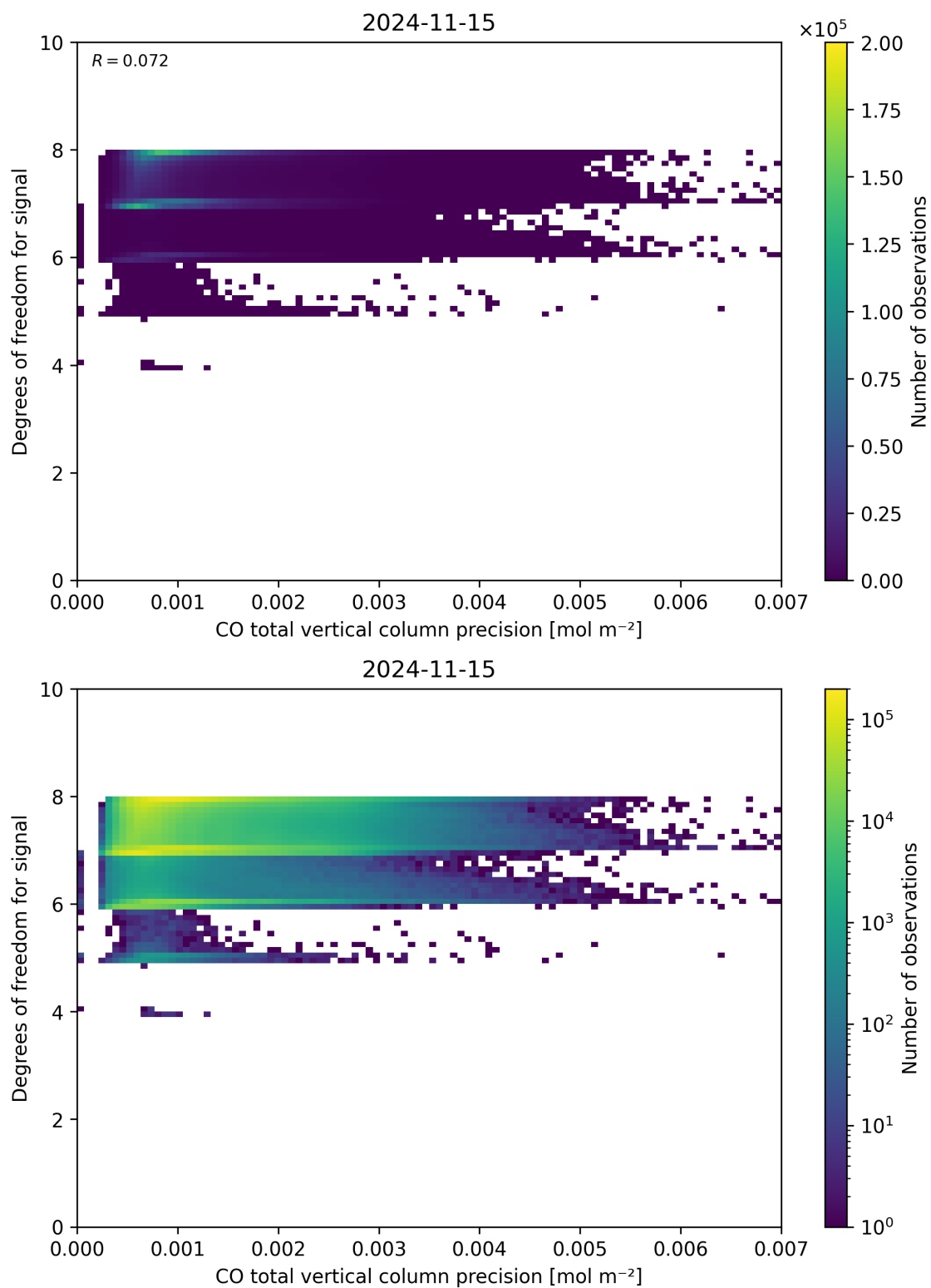
Figure 45: Scatter density plot of “CO total vertical column precision” against “Degrees of freedom for signal” for 2024-11-14 to 2024-11-16.
