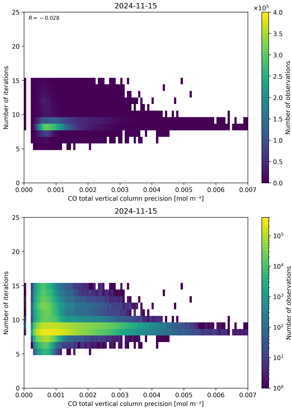
Figure 46: Scatter density plot of “CO total vertical column precision” against “Number of iterations” for 2024-11-14 to 2024-11-16.
