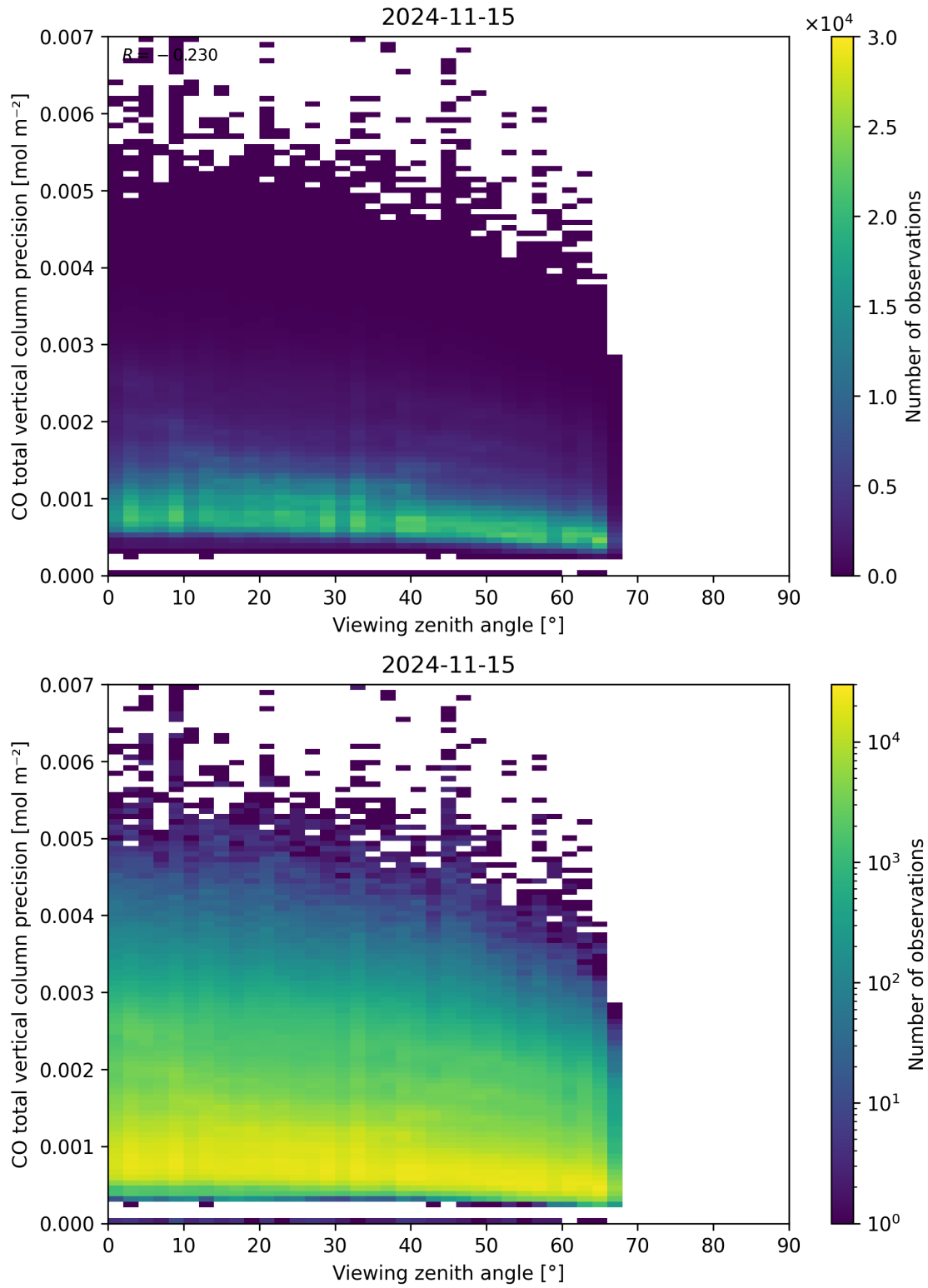
Figure 71: Scatter density plot of “Viewing zenith angle” against “CO total vertical column precision” for 2024-11-14 to 2024-11-16.
