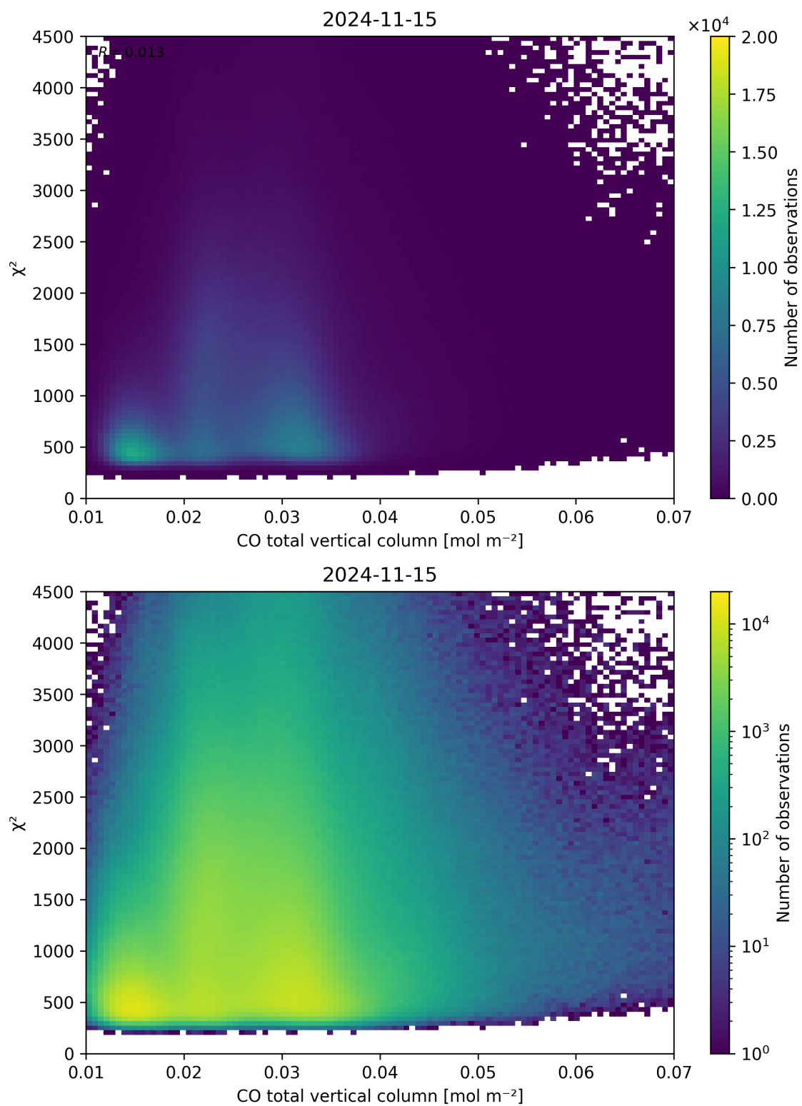
Figure 35: Scatter density plot of “CO total vertical column” against “ \chi^2 ” for 2024-11-14 to 2024-11-16.
