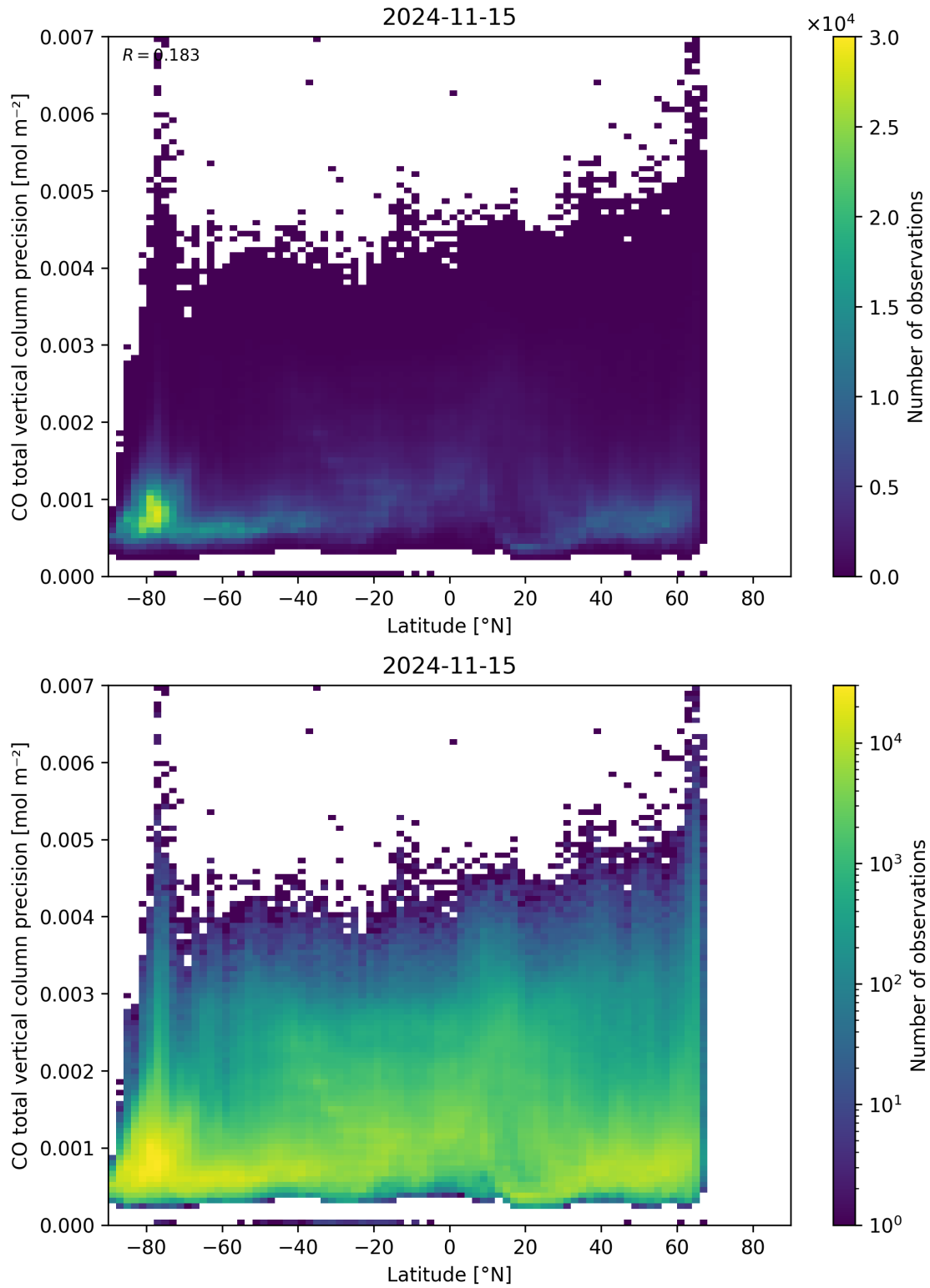
Figure 53: Scatter density plot of “Latitude” against “CO total vertical column precision” for 2024-11-14 to 2024-11-16.
