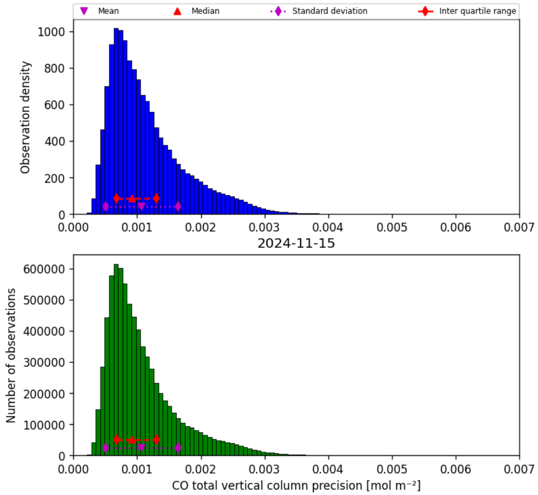
Figure 20: Histogram of “CO total vertical column precision” for 2024-11-14 to 2024-11-16
