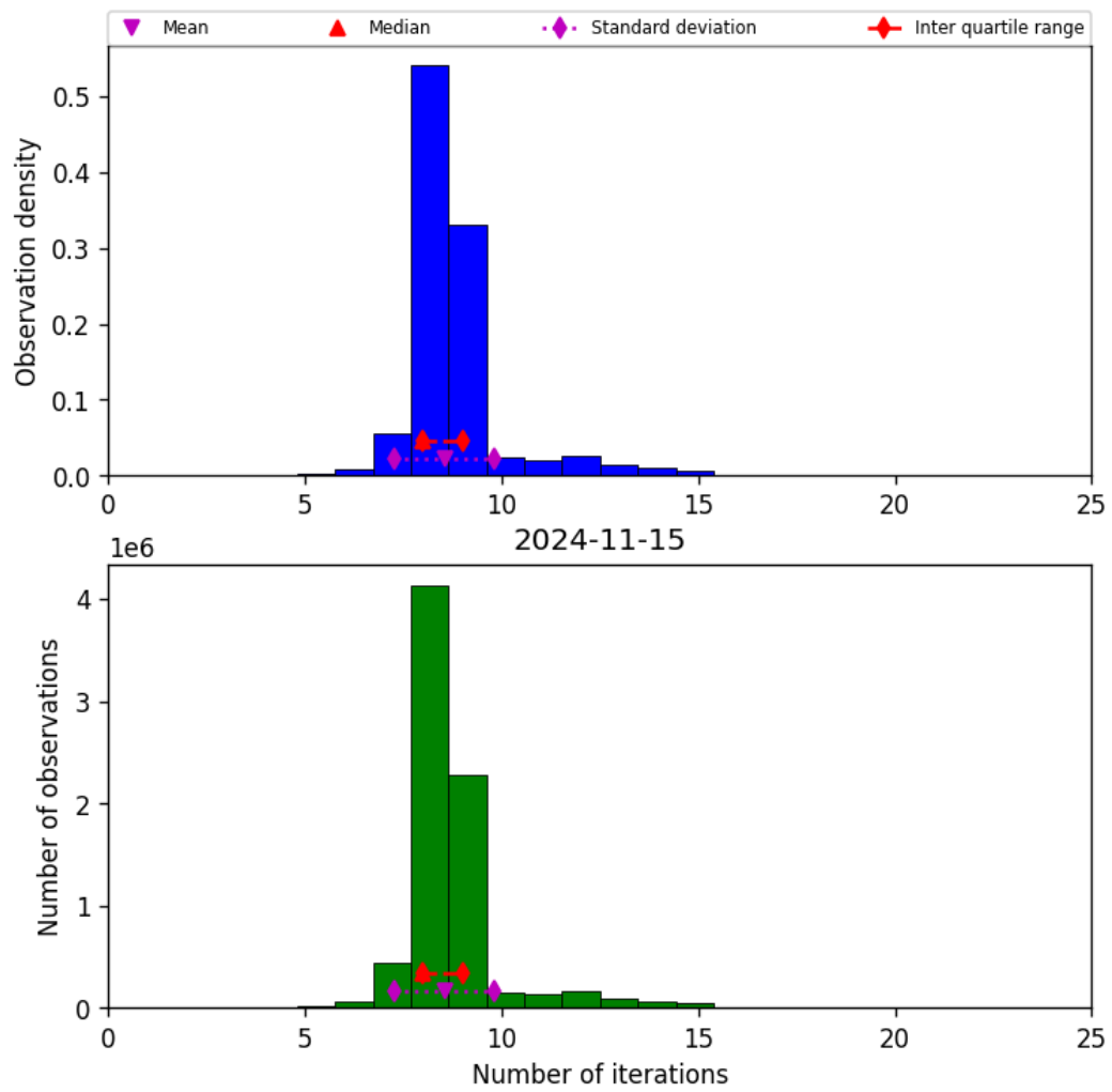
Figure 24: Histogram of “Number of iterations” for 2024-11-14 to 2024-11-16
