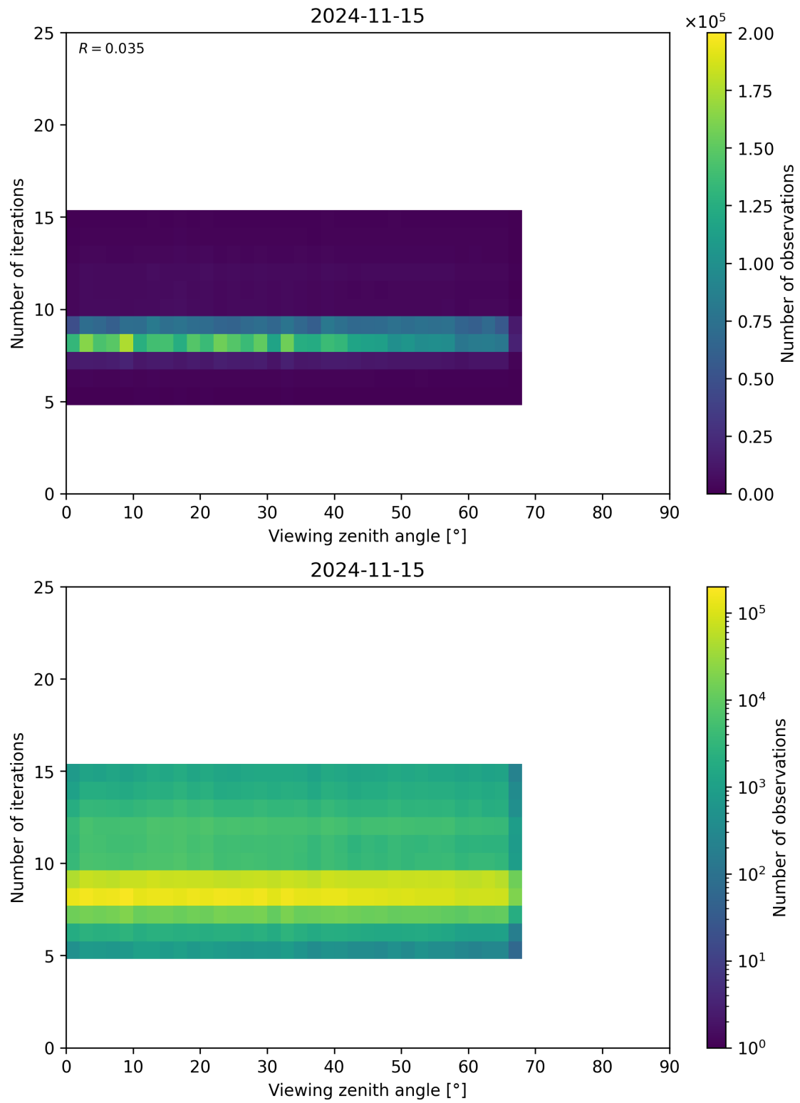
Figure 75: Scatter density plot of “Viewing zenith angle” against “Number of iterations” for 2024-11-14 to 2024-11-16.
