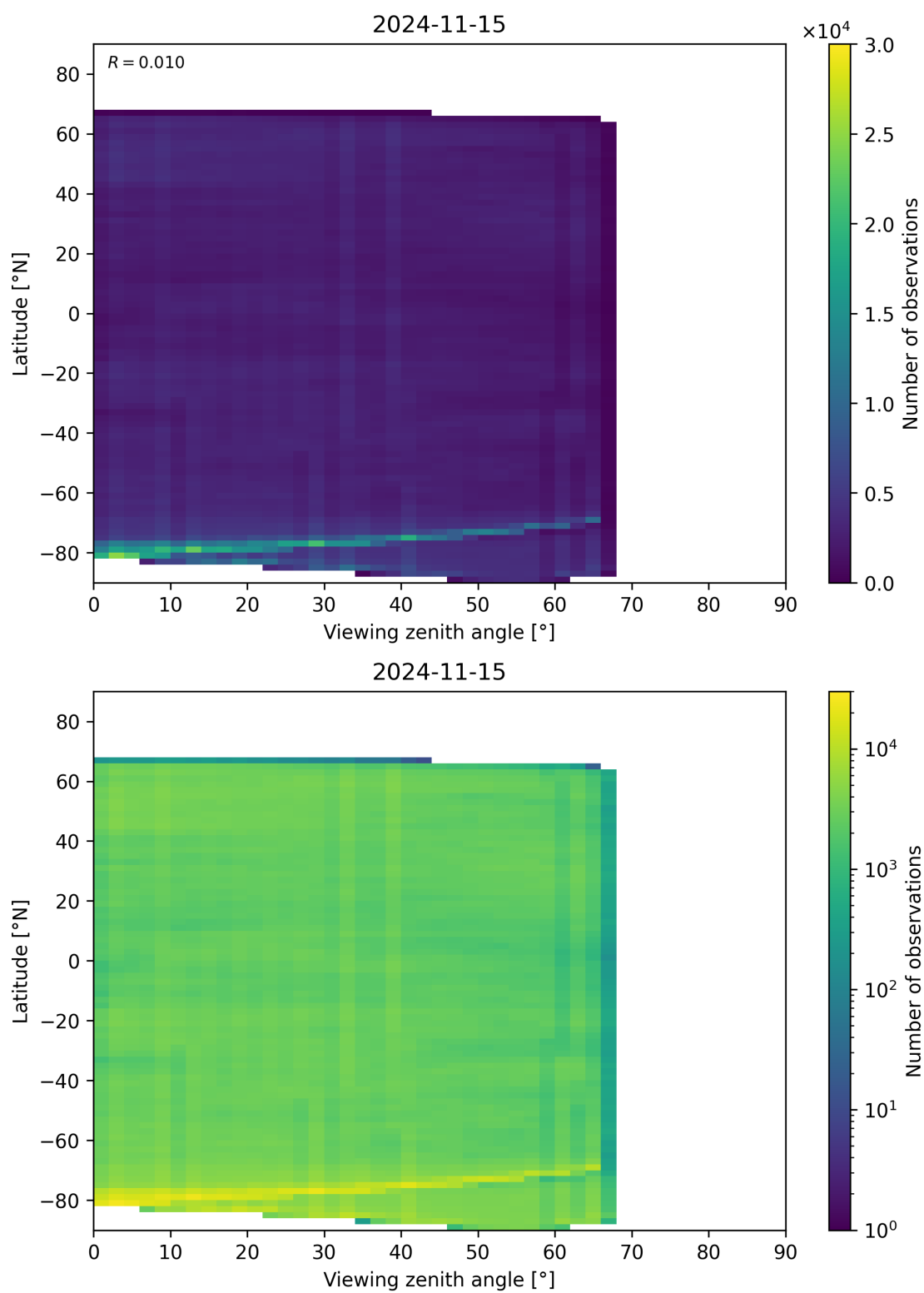
Figure 74: Scatter density plot of “Viewing zenith angle” against “Latitude” for 2024-11-14 to 2024-11-16.
