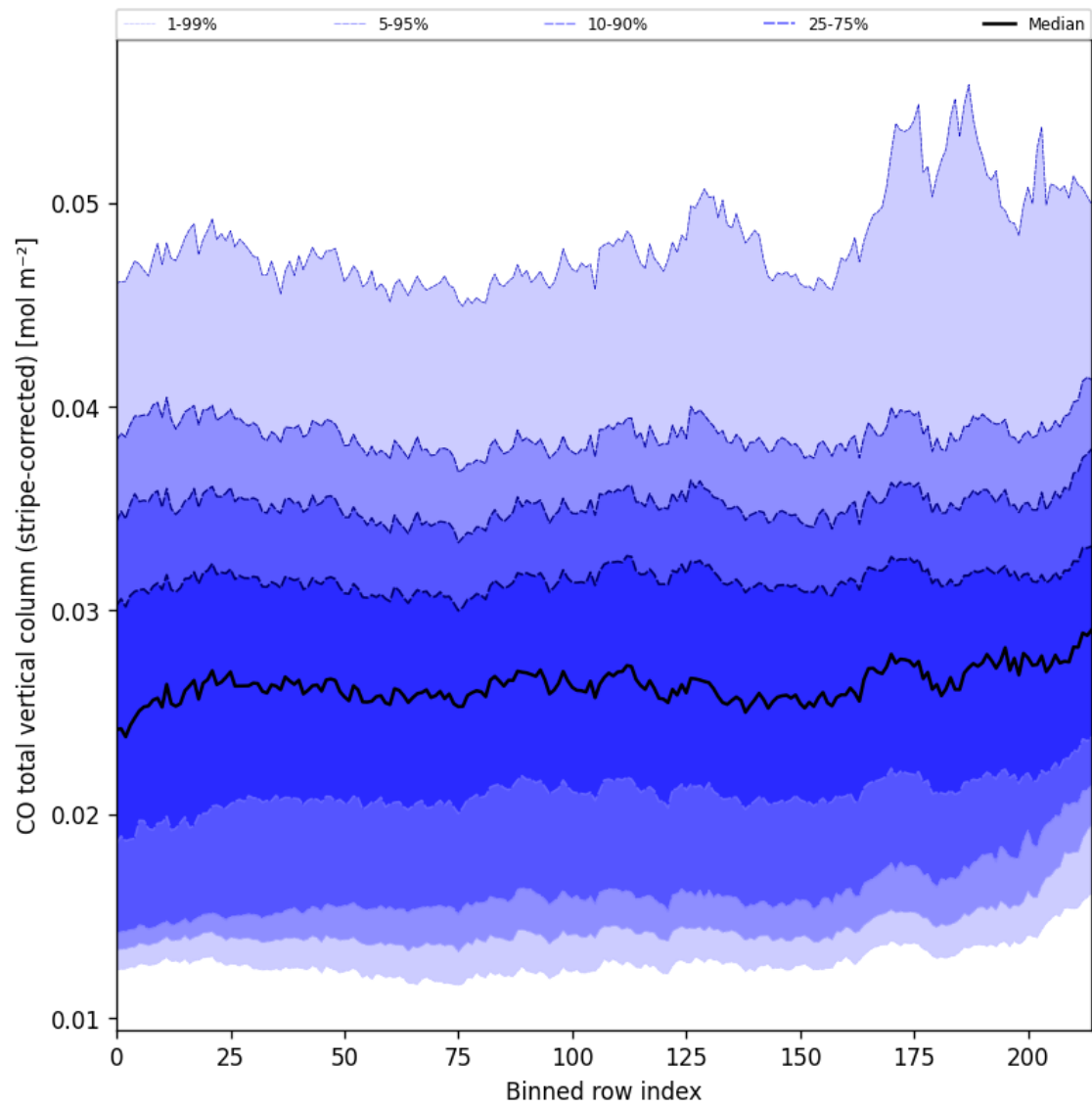
Figure 27: Along track statistics of “CO total vertical column (stripe-corrected)” for 2024-11-14 to 2024-11-16
