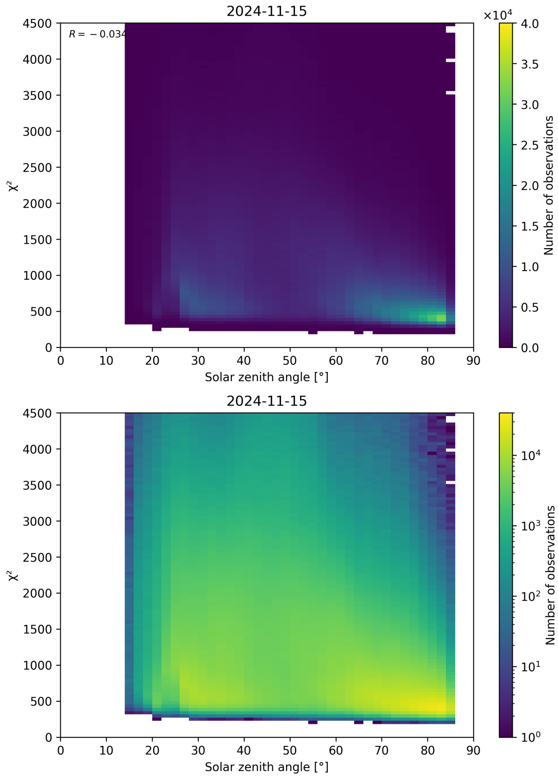
Figure 64: Scatter density plot of “Solar zenith angle” against “ \chi^2 ” for 2024-11-14 to 2024-11-16.
