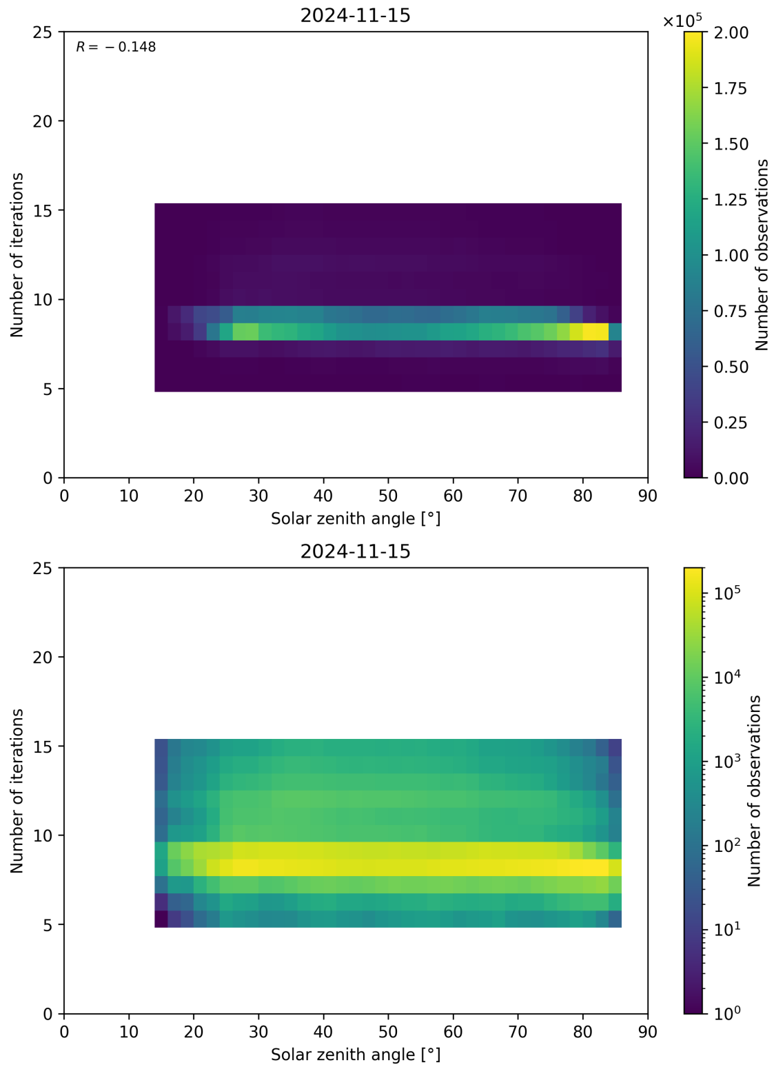
Figure 67: Scatter density plot of “Solar zenith angle” against “Number of iterations” for 2024-11-14 to 2024-11-16.
