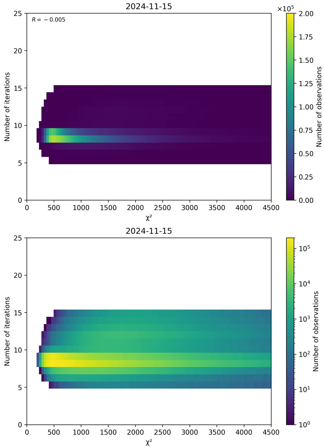
Figure 49: Scatter density plot of “ \chi^2 ” against “Number of iterations” for 2024-11-14 to 2024-11-16.
