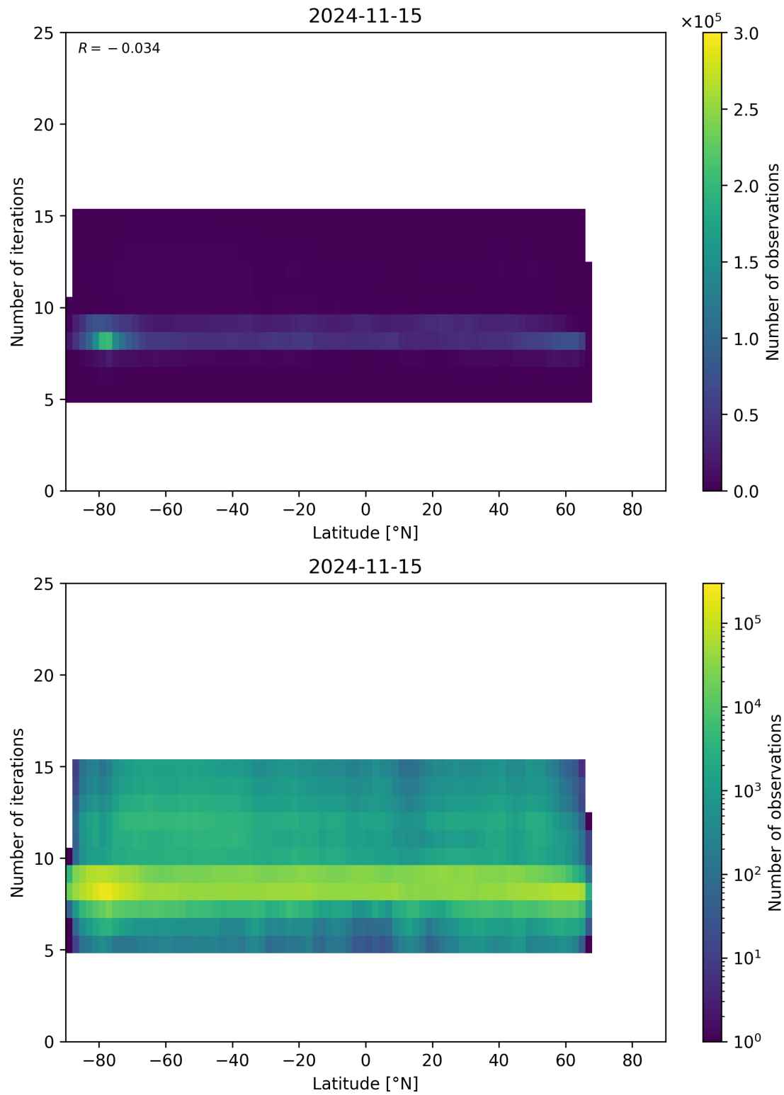
Figure 56: Scatter density plot of “Latitude” against “Number of iterations” for 2024-11-14 to 2024-11-16.
