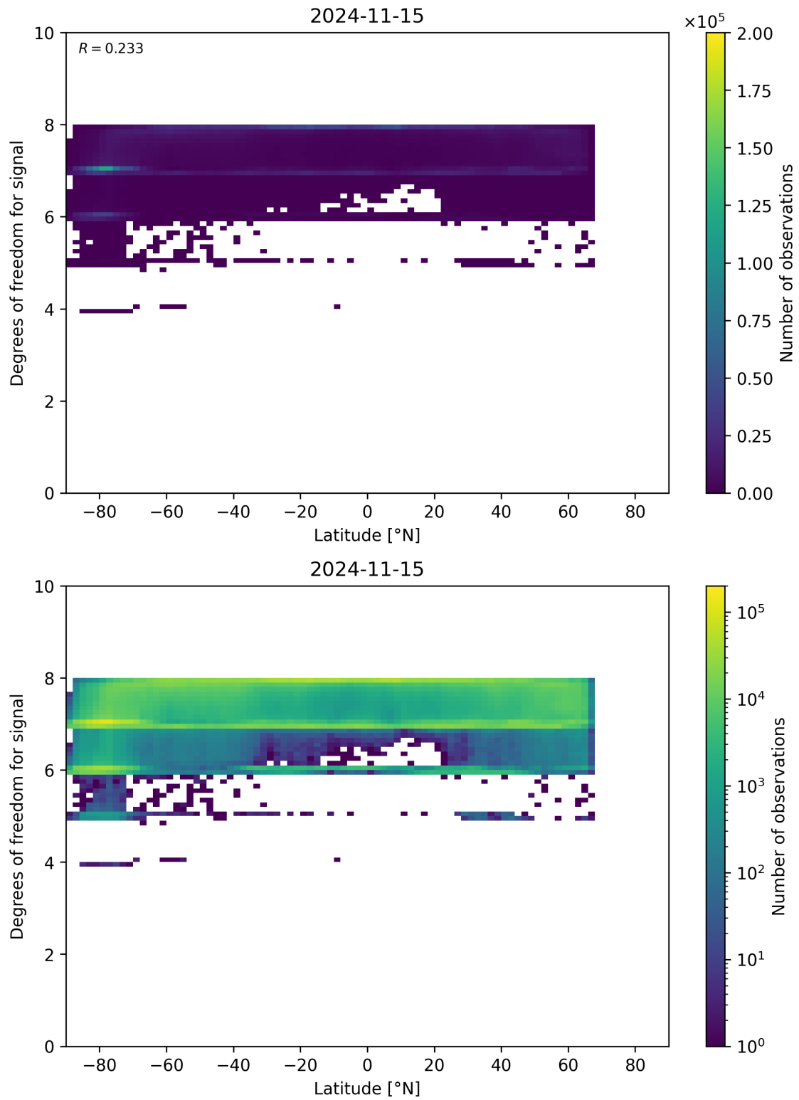
Figure 55: Scatter density plot of “Latitude” against “Degrees of freedom for signal” for 2024-11-14 to 2024-11-16.
