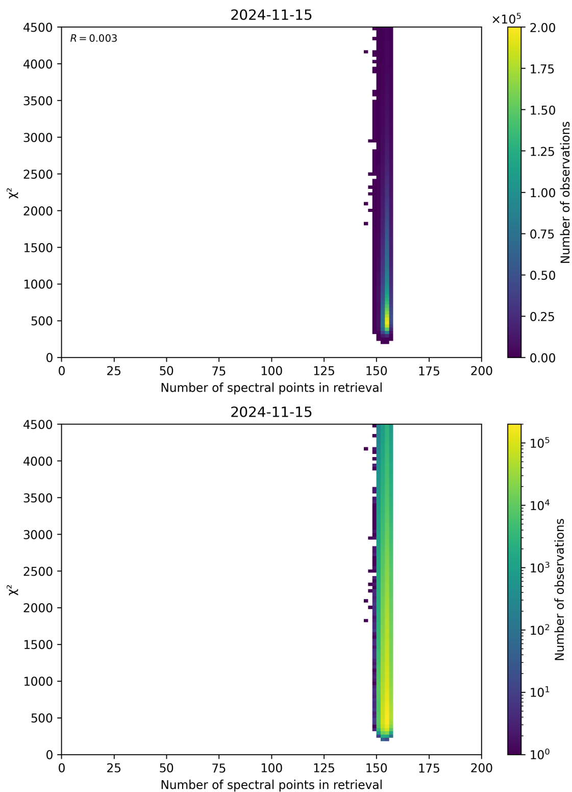
Figure 58: Scatter density plot of “Number of spectral points in retrieval” against “ \chi^2 ” for 2024-11-14 to 2024-11-16.
