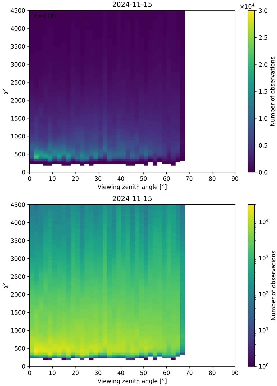
Figure 72: Scatter density plot of “Viewing zenith angle” against “ \chi^2 ” for 2024-11-14 to 2024-11-16.
