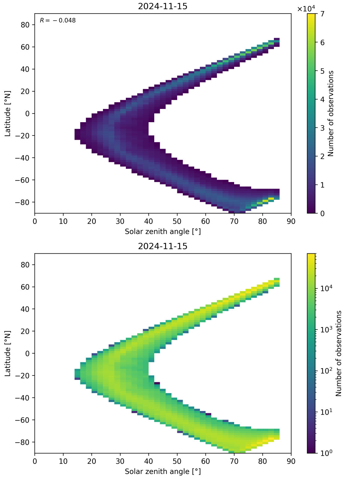
Figure 66: Scatter density plot of “Solar zenith angle” against “Latitude” for 2024-11-14 to 2024-11-16.
