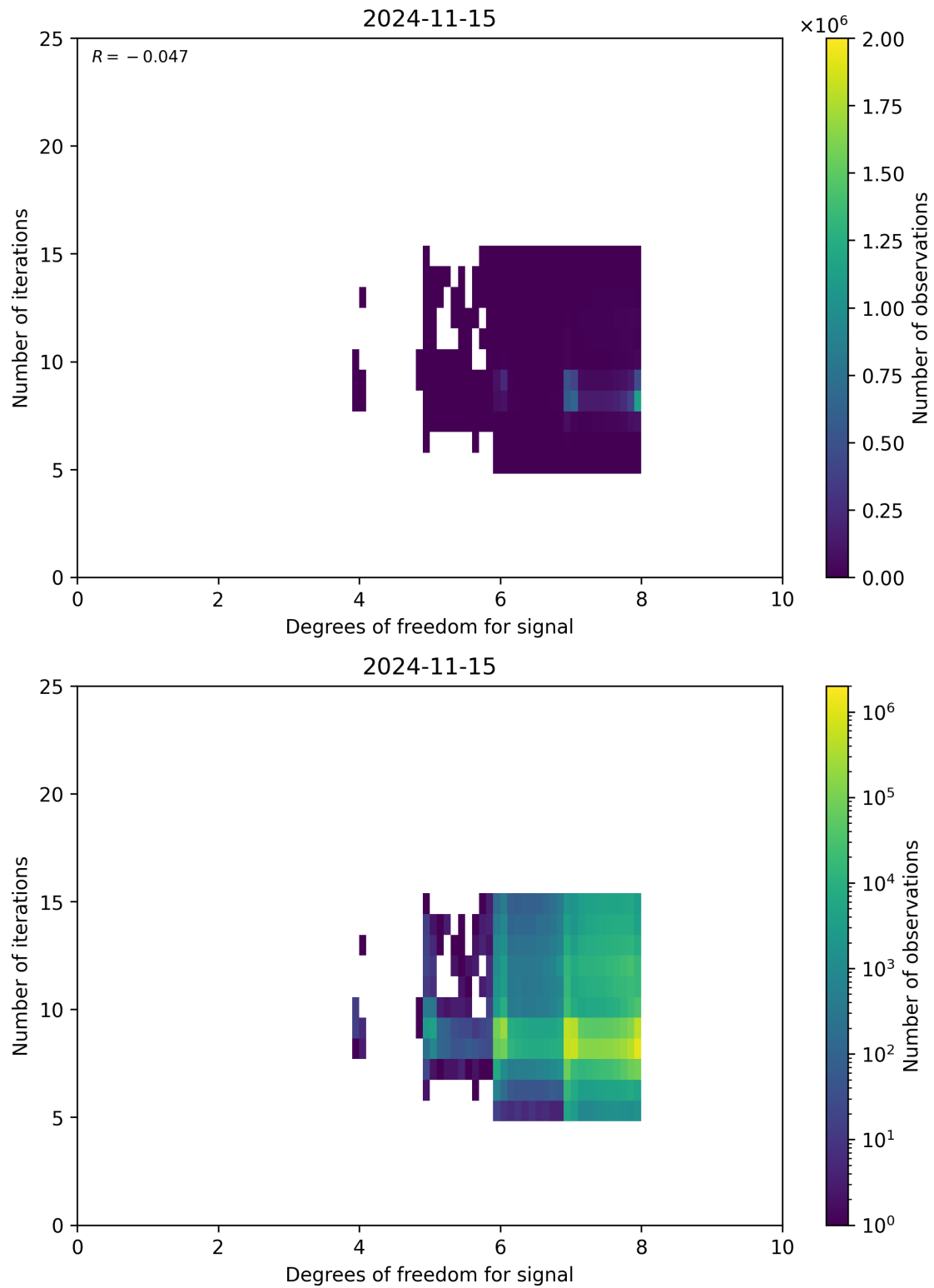
Figure 50: Scatter density plot of “Degrees of freedom for signal” against “Number of iterations” for 2024-11-14 to 2024-11-16.
