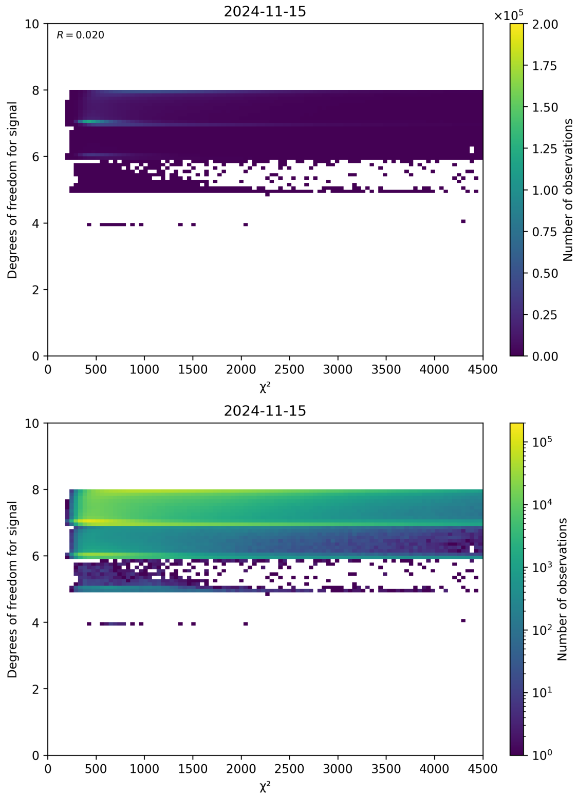
Figure 48: Scatter density plot of “ \chi^2 ” against “Degrees of freedom for signal” for 2024-11-14 to 2024-11-16.
