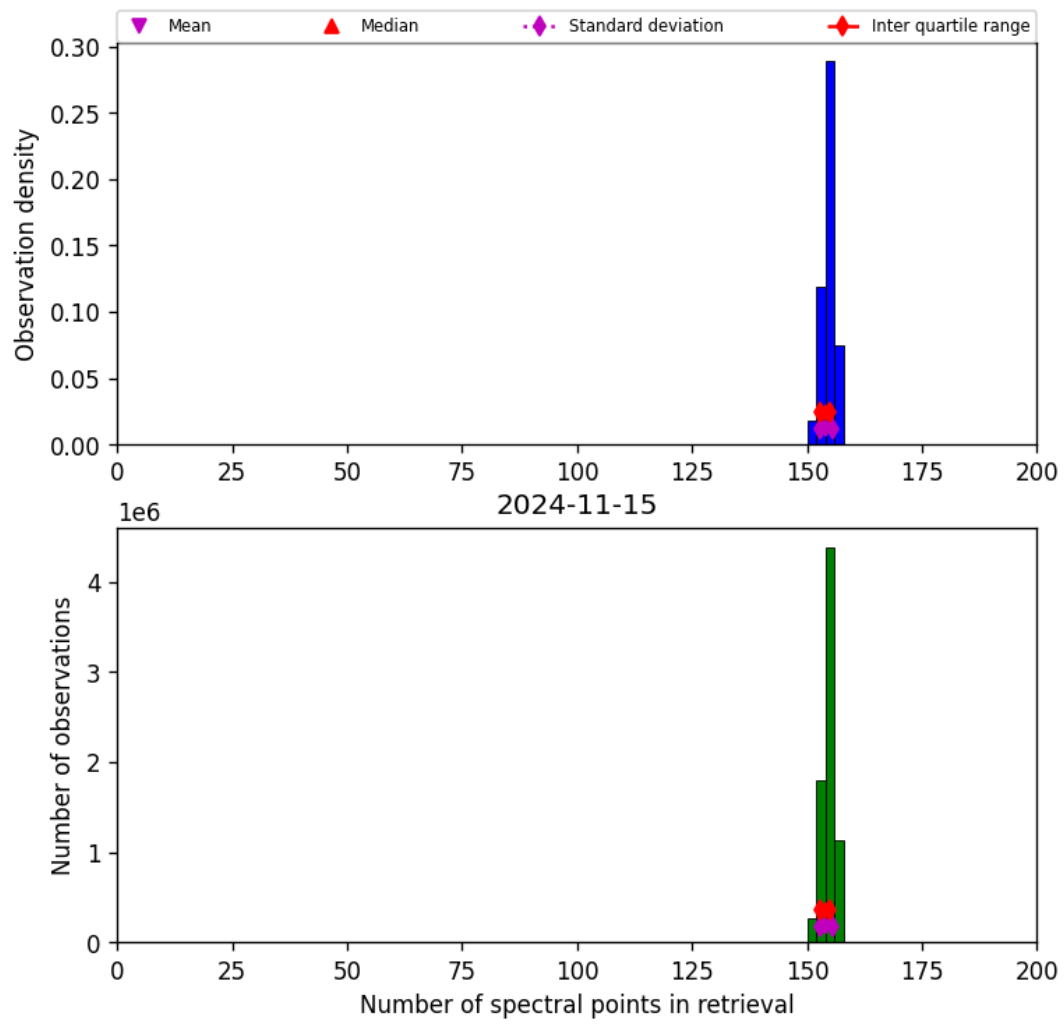
Figure 21: Histogram of “Number of spectral points in retrieval” for 2024-11-14 to 2024-11-16
