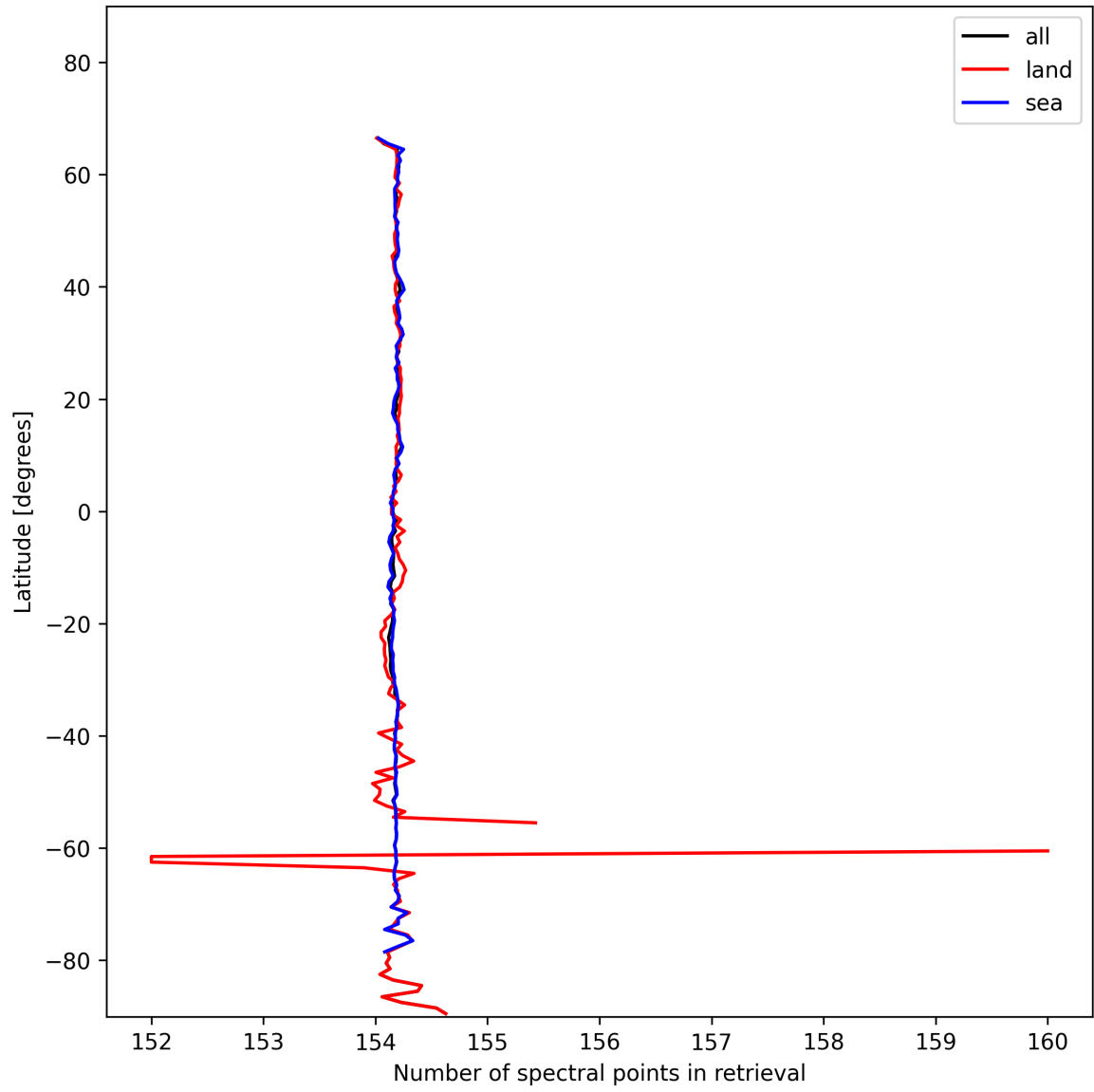
Figure 13: Zonal average of “Number of spectral points in retrieval” for 2024-11-14 to 2024-11-16.
