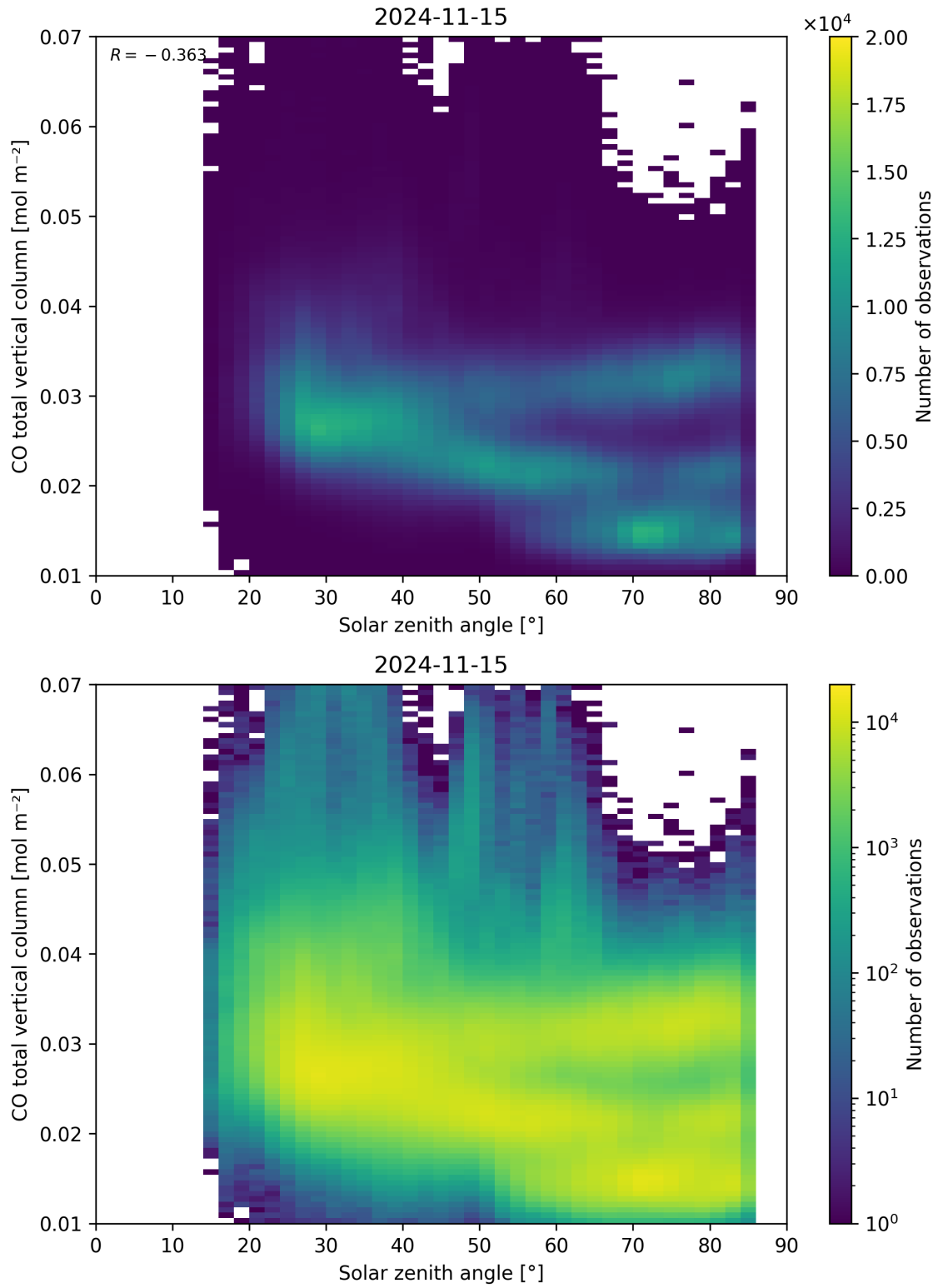
Figure 61: Scatter density plot of “Solar zenith angle” against “CO total vertical column” for 2024-11-14 to 2024-11-16.
