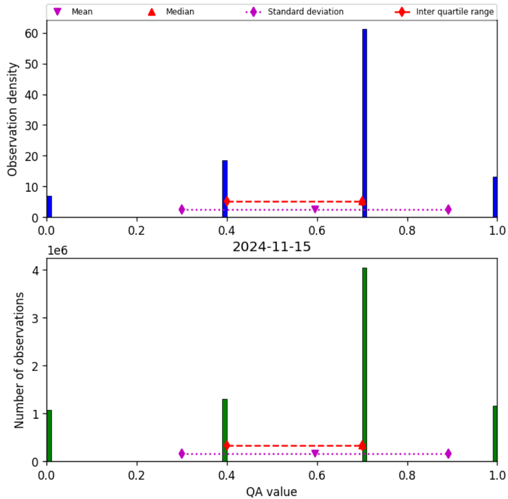
Figure 17: Histogram of “QA value” for 2024-11-14 to 2024-11-16
