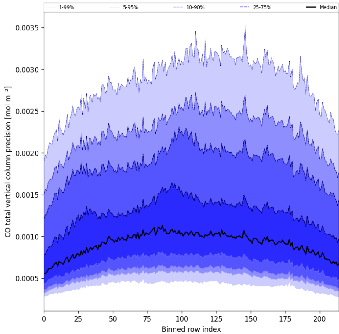
Figure 28: Along track statistics of “CO total vertical column precision” for 2024-11-14 to 2024-11-16
