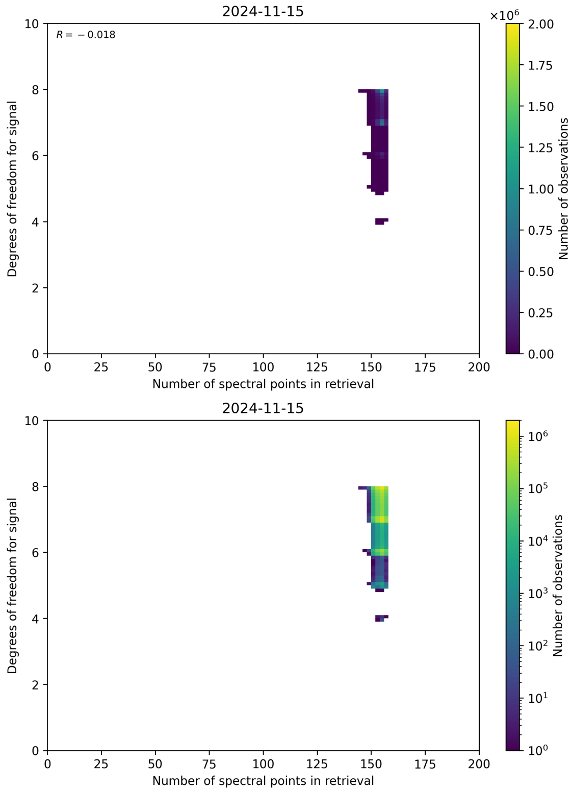
Figure 59: Scatter density plot of “Number of spectral points in retrieval” against “Degrees of freedom for signal” for 2024-11-14 to 2024-11-16.
