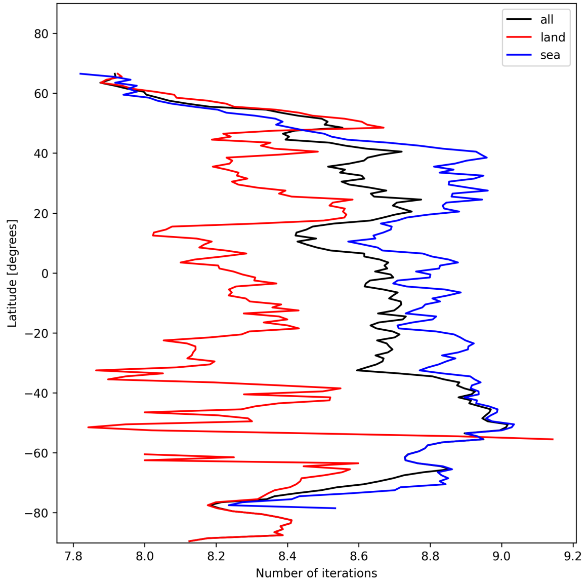
Figure 16: Zonal average of “Number of iterations” for 2024-11-14 to 2024-11-16.
