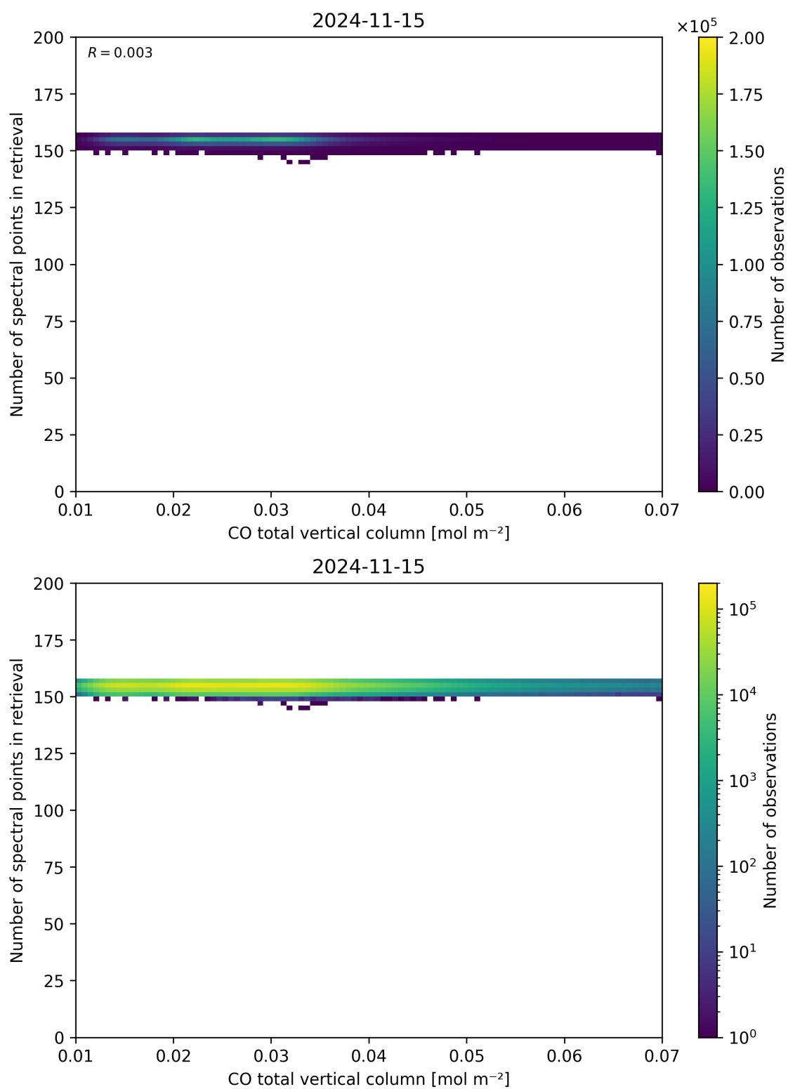
Figure 43: Scatter density plot of “CO total vertical column” against “Number of spectral points in retrieval” for 2024-11-14 to 2024-11-16.
