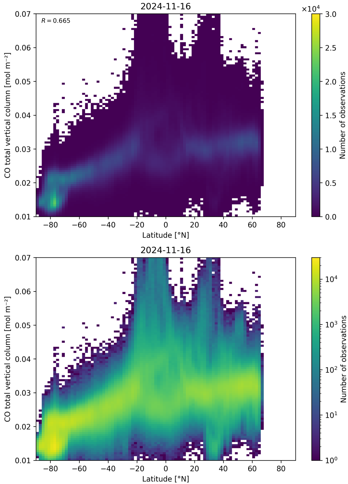
Figure 51: Scatter density plot of “Latitude” against “CO total vertical column” for 2024-11-15 to 2024-11-17.
