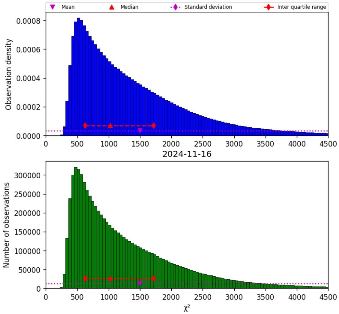
Figure 22: Histogram of “ \chi^2 ” for 2024-11-15 to 2024-11-17
