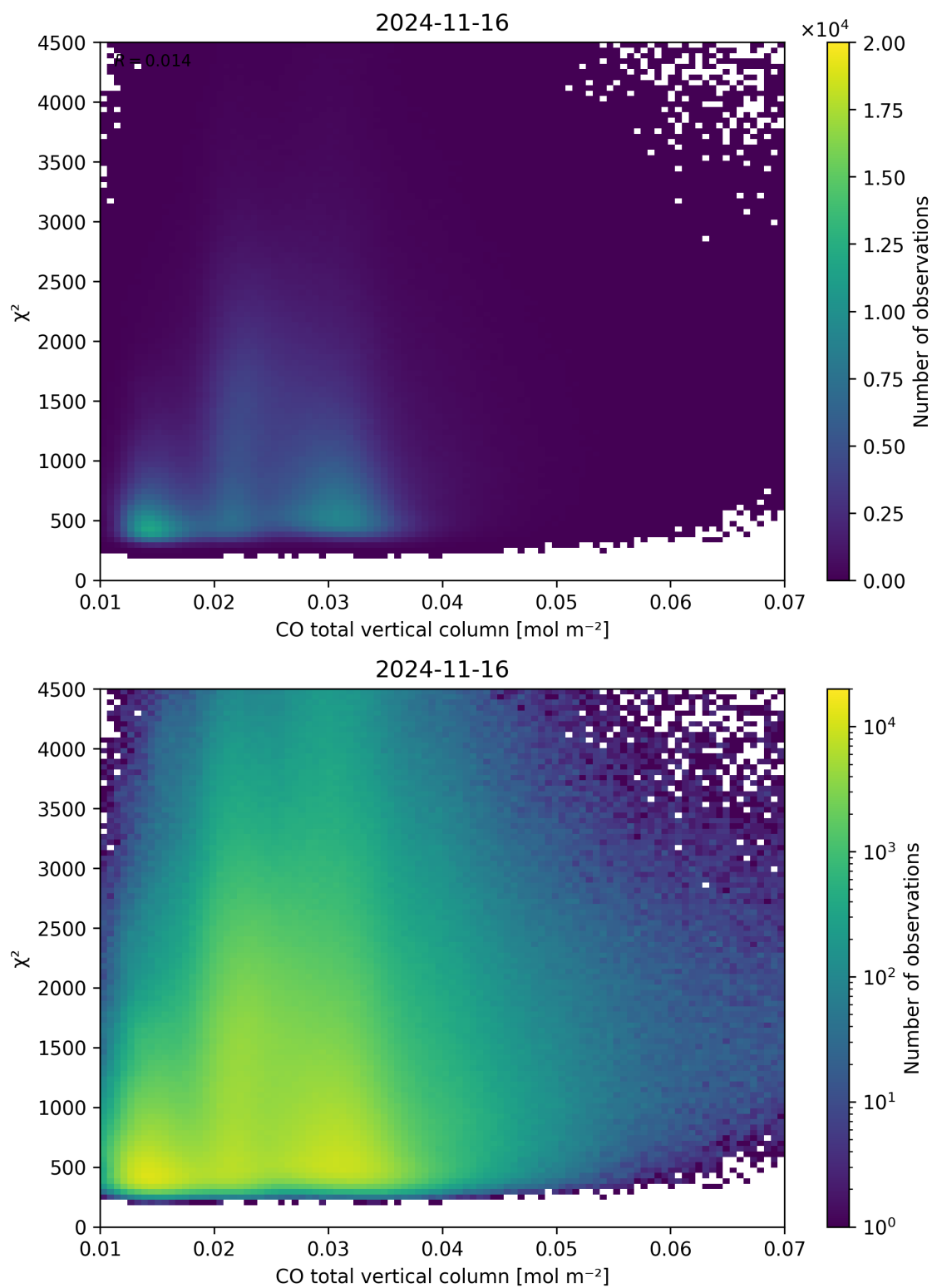
Figure 35: Scatter density plot of “CO total vertical column” against “ \chi^2 ” for 2024-11-15 to 2024-11-17.
