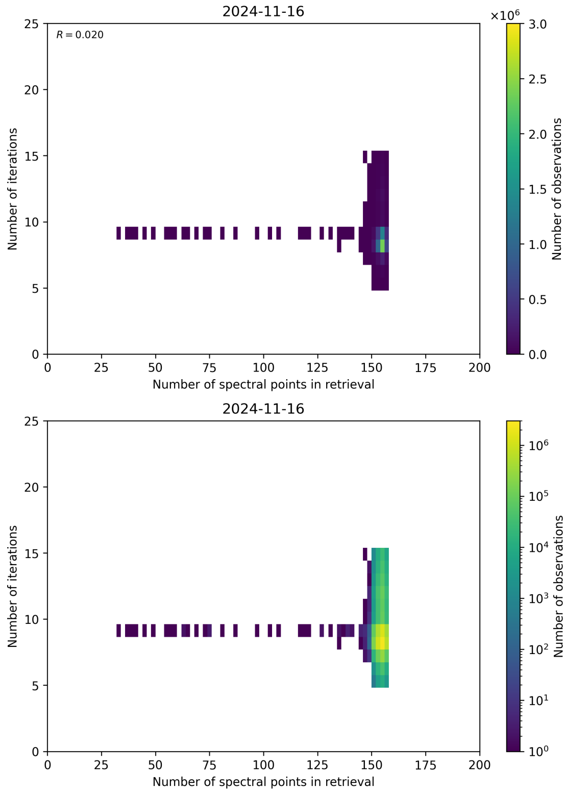
Figure 60: Scatter density plot of “Number of spectral points in retrieval” against “Number of iterations” for 2024-11-15 to 2024-11-17.
