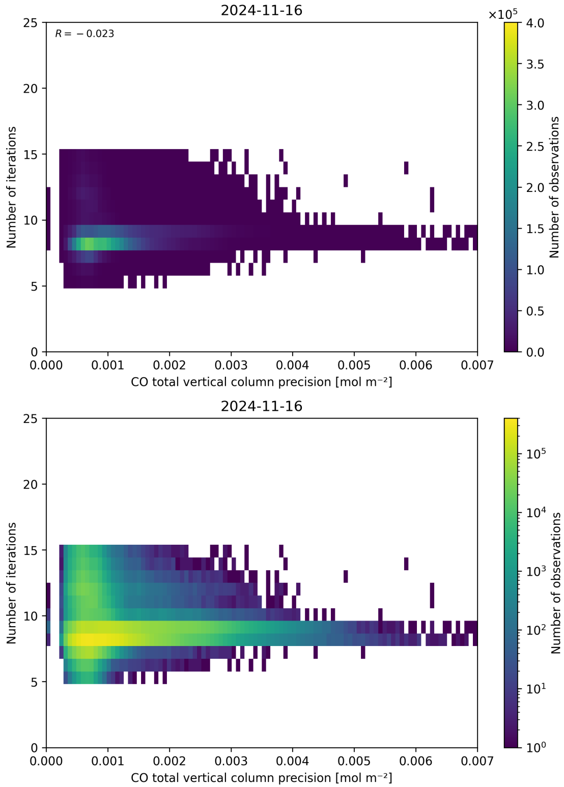
Figure 46: Scatter density plot of “CO total vertical column precision” against “Number of iterations” for 2024-11-15 to 2024-11-17.
