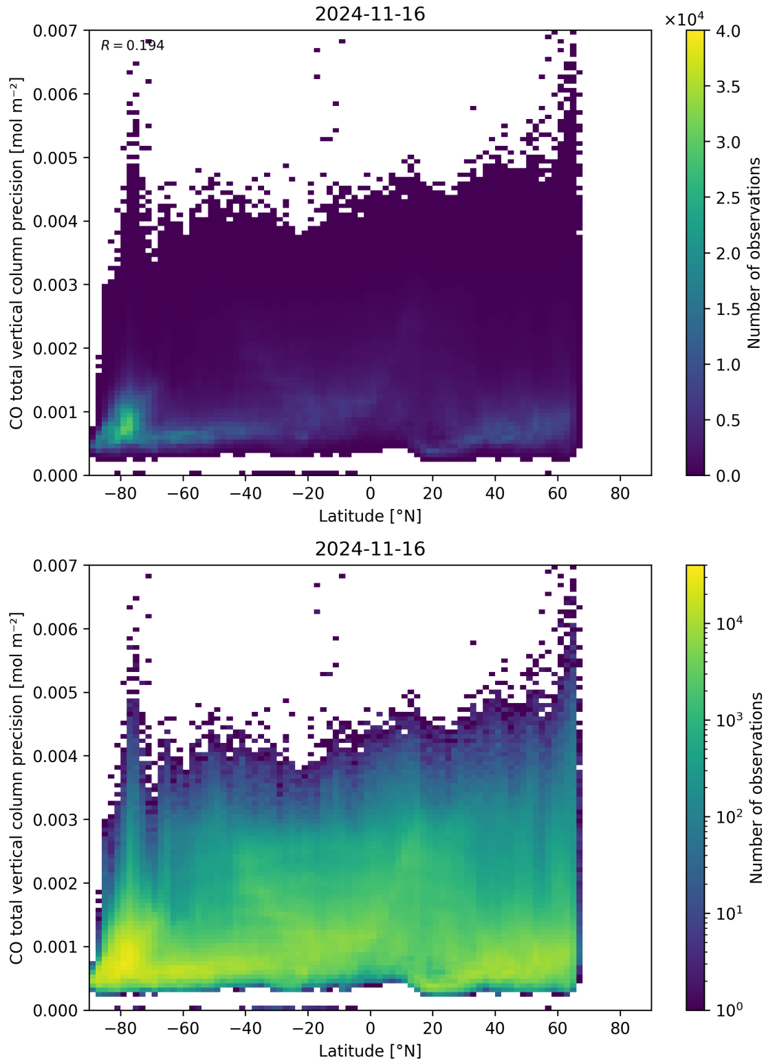
Figure 53: Scatter density plot of “Latitude” against “CO total vertical column precision” for 2024-11-15 to 2024-11-17.
