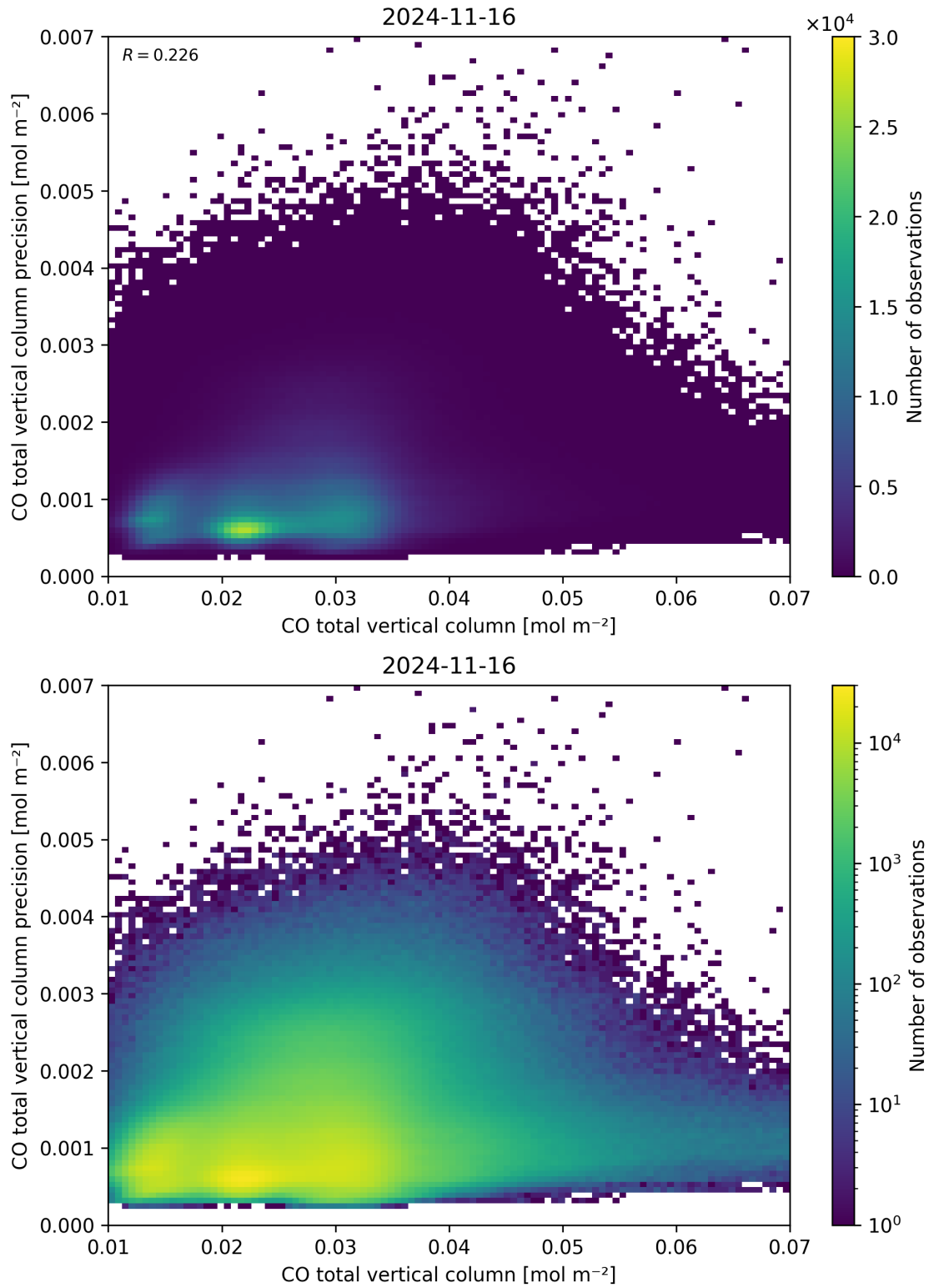
Figure 34: Scatter density plot of “CO total vertical column” against “CO total vertical column precision” for 2024-11-15 to 2024-11-17.
