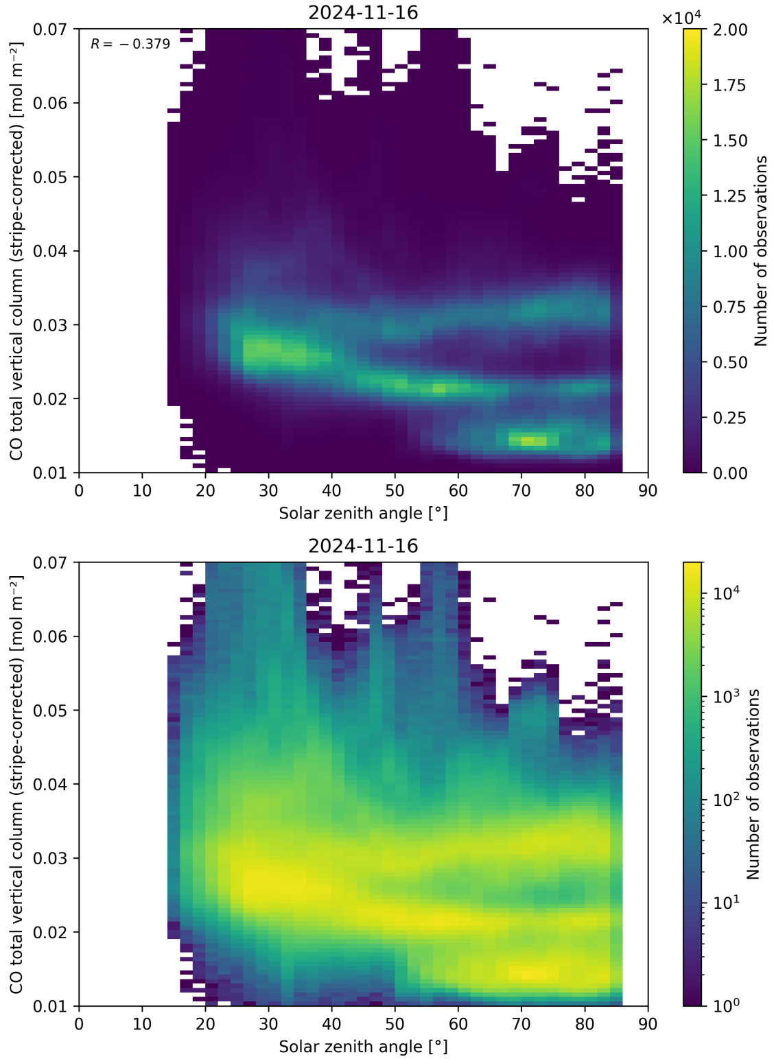
Figure 62: Scatter density plot of “Solar zenith angle” against “CO total vertical column (stripe-corrected)” for 2024-11-15 to 2024-11-17.
