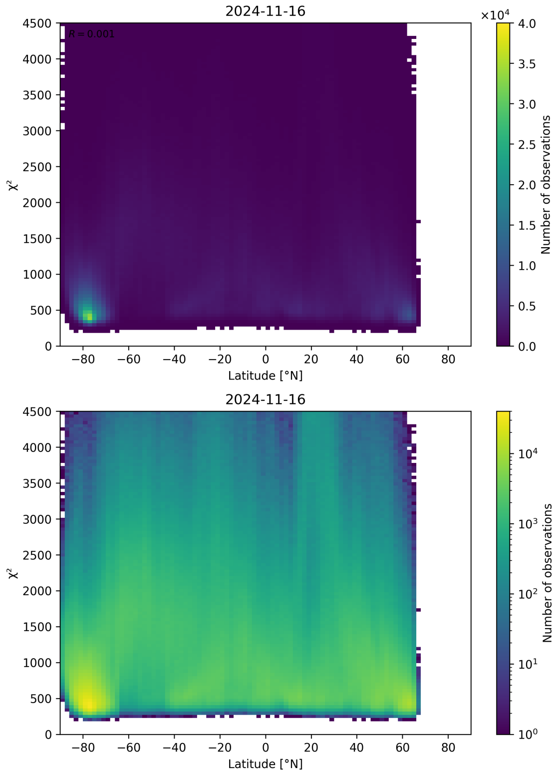
Figure 54: Scatter density plot of “Latitude” against “ \chi^2 ” for 2024-11-15 to 2024-11-17.
