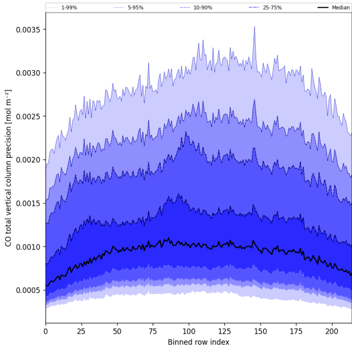
Figure 28: Along track statistics of “CO total vertical column precision” for 2024-11-15 to 2024-11-17
