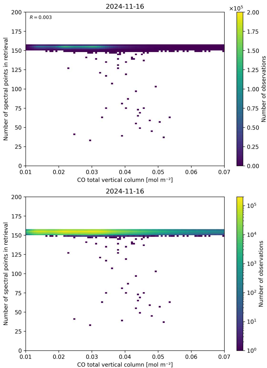
Figure 43: Scatter density plot of “CO total vertical column” against “Number of spectral points in retrieval” for 2024-11-15 to 2024-11-17.
