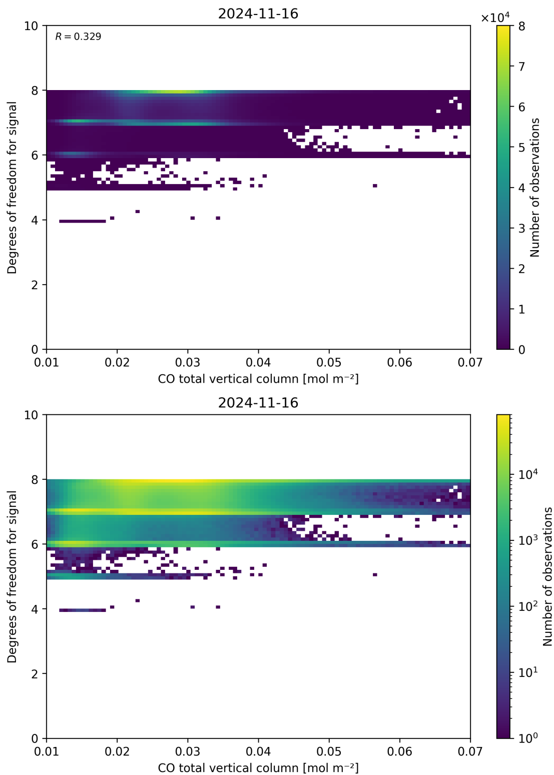
Figure 41: Scatter density plot of “CO total vertical column” against “Degrees of freedom for signal” for 2024-11-15 to 2024-11-17.
