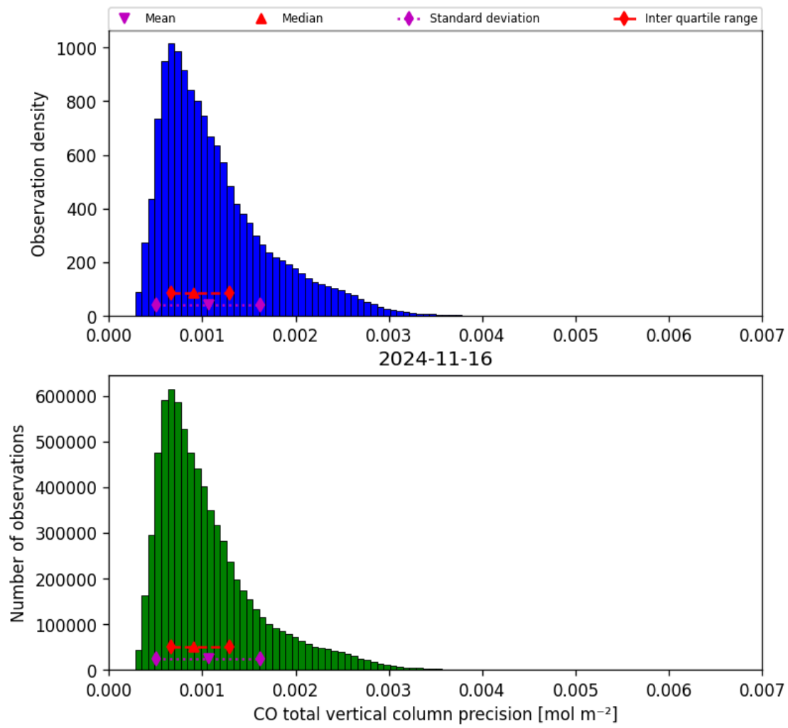
Figure 20: Histogram of “CO total vertical column precision” for 2024-11-15 to 2024-11-17
