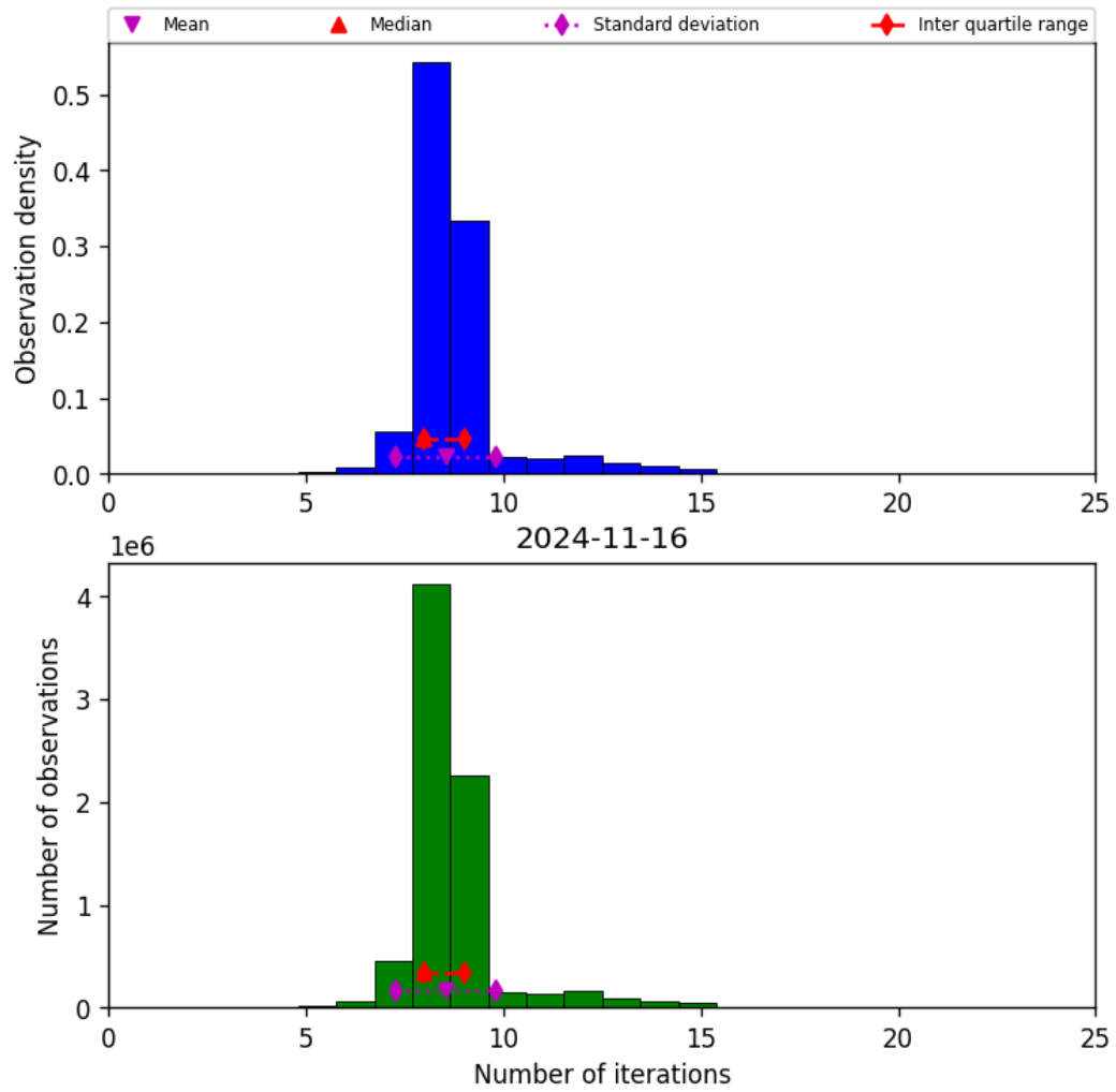
Figure 24: Histogram of “Number of iterations” for 2024-11-15 to 2024-11-17
