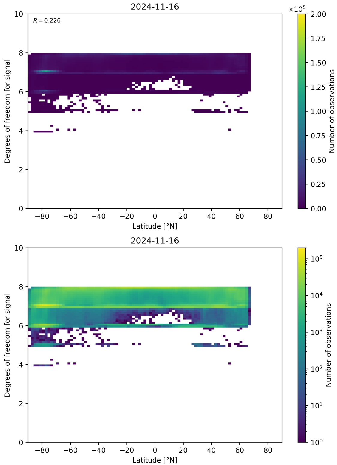
Figure 55: Scatter density plot of “Latitude” against “Degrees of freedom for signal” for 2024-11-15 to 2024-11-17.
