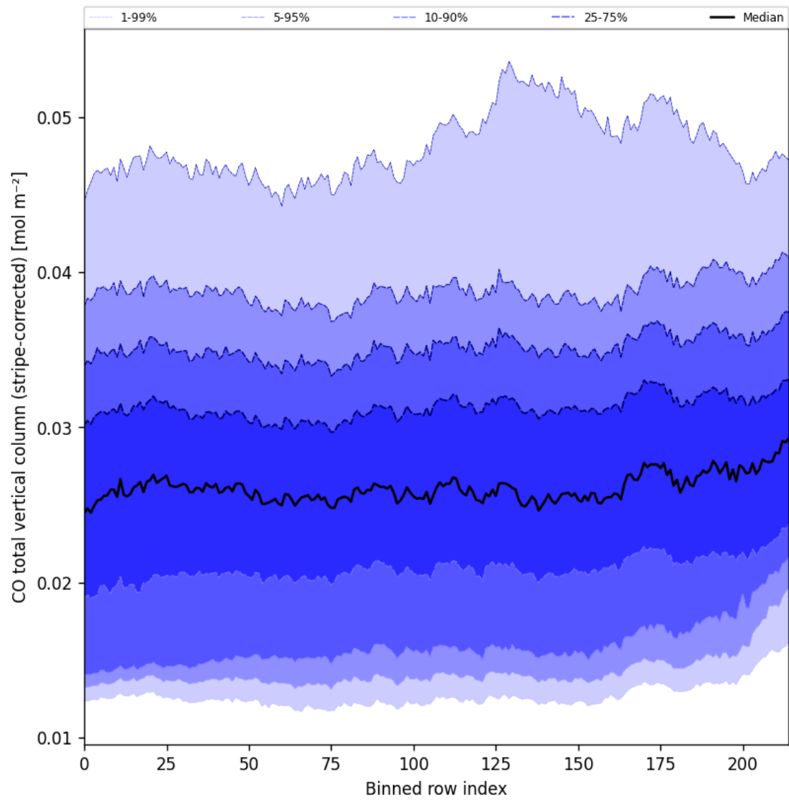
Figure 27: Along track statistics of “CO total vertical column (stripe-corrected)” for 2024-11-15 to 2024-11-17
