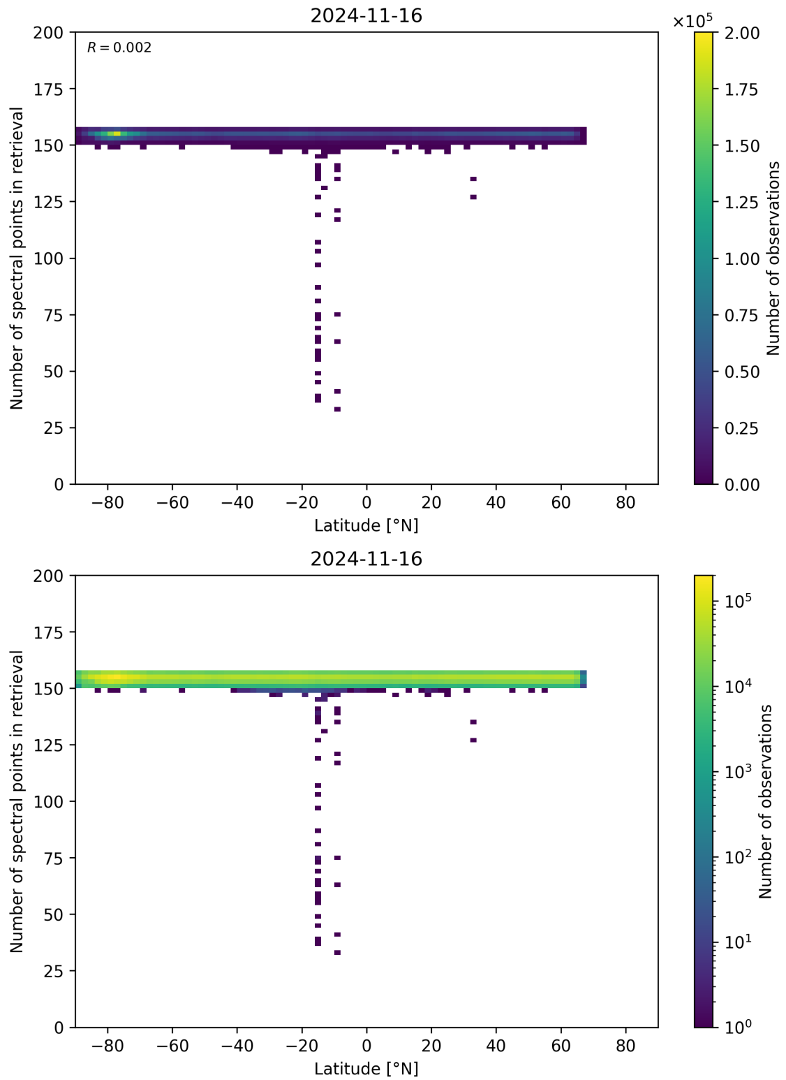
Figure 57: Scatter density plot of “Latitude” against “Number of spectral points in retrieval” for 2024-11-15 to 2024-11-17.
