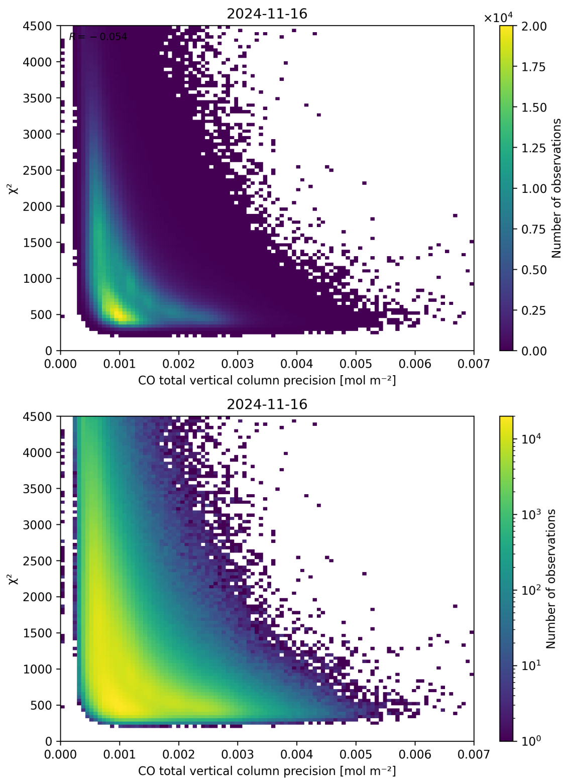
Figure 44: Scatter density plot of “CO total vertical column precision” against “ \chi^2 ” for 2024-11-15 to 2024-11-17.
