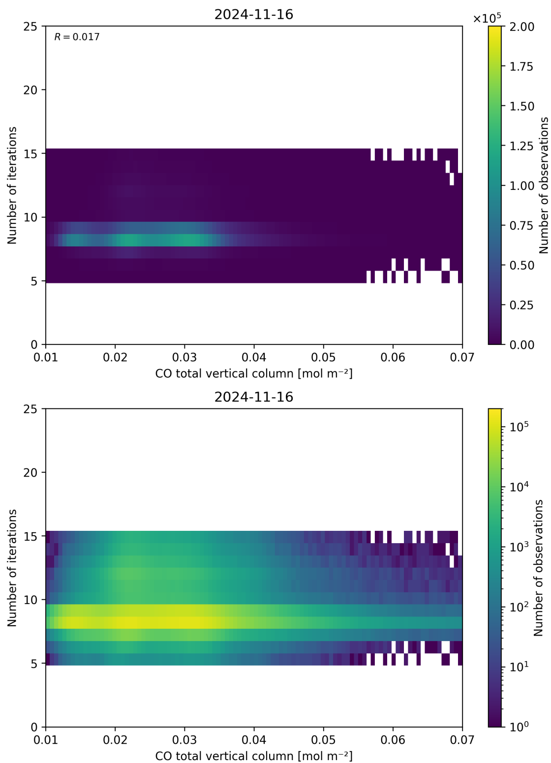
Figure 42: Scatter density plot of “CO total vertical column” against “Number of iterations” for 2024-11-15 to 2024-11-17.
