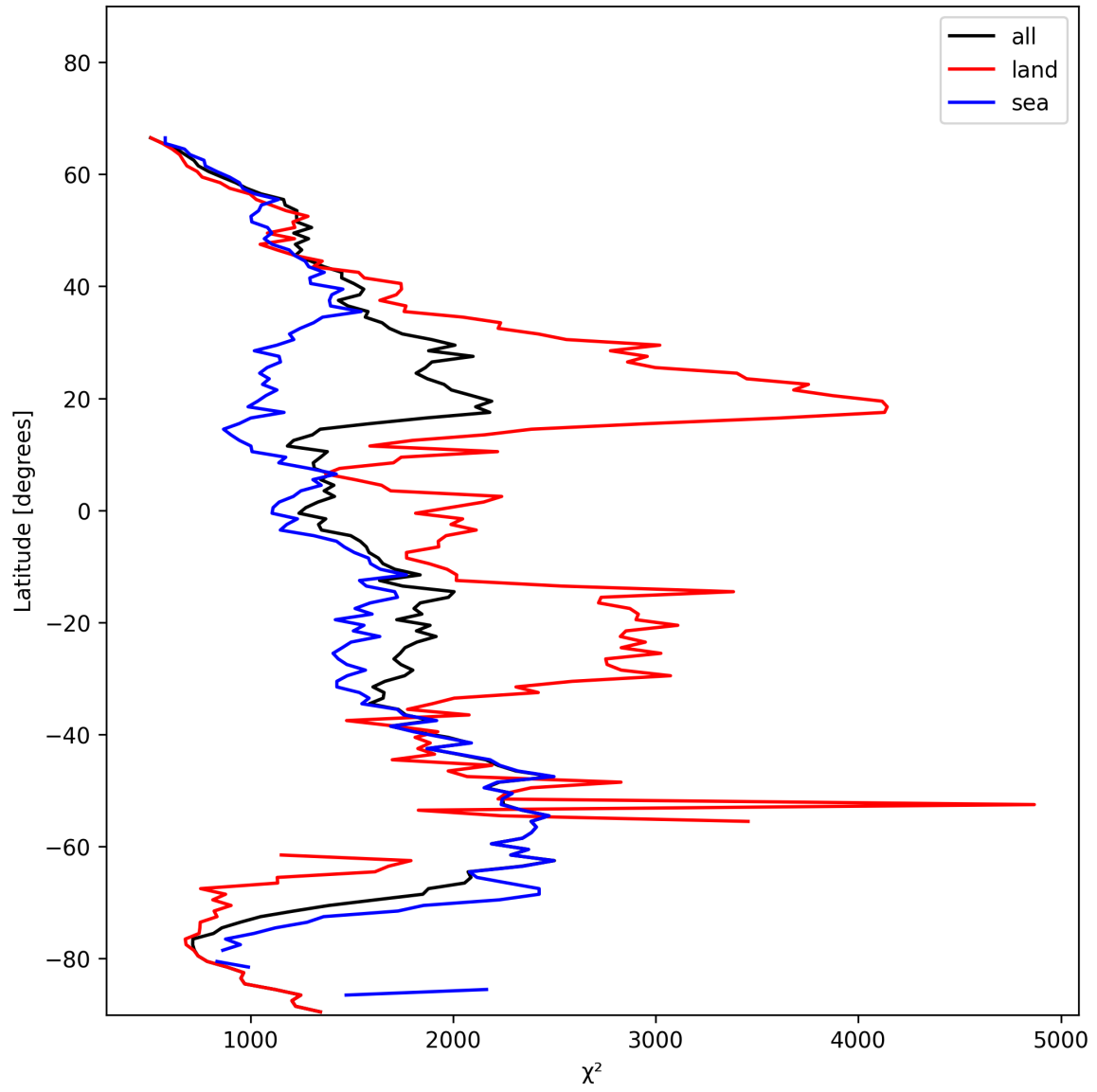
Figure 14: Zonal average of “ \chi^2 ” for 2024-11-15 to 2024-11-17.
