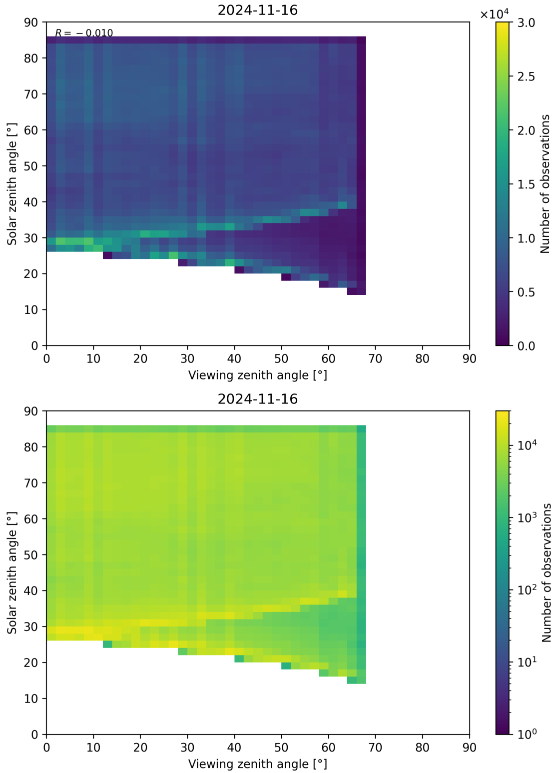
Figure 77: Scatter density plot of “Viewing zenith angle” against “Solar zenith angle” for 2024-11-15 to 2024-11-17.
