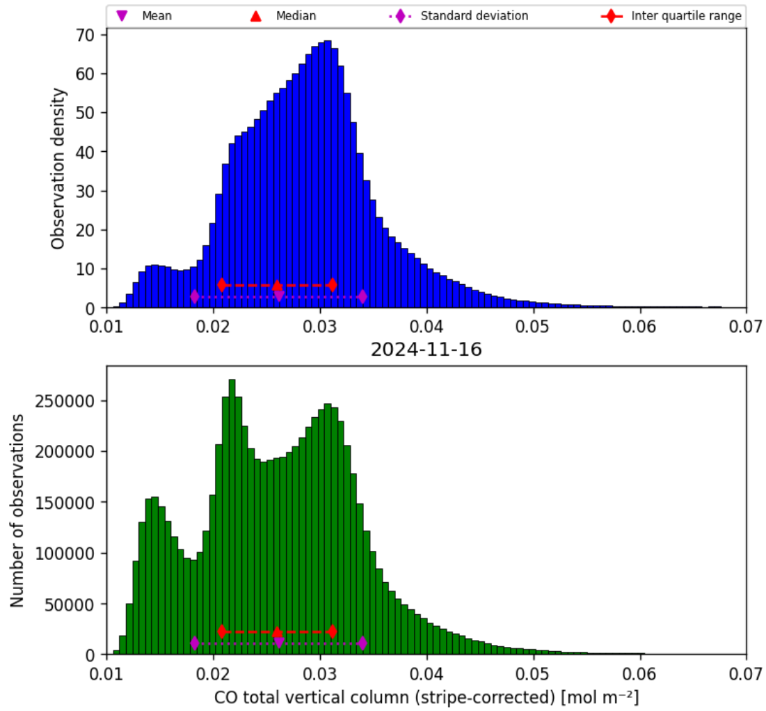
Figure 19: Histogram of “CO total vertical column (stripe-corrected)” for 2024-11-15 to 2024-11-17
