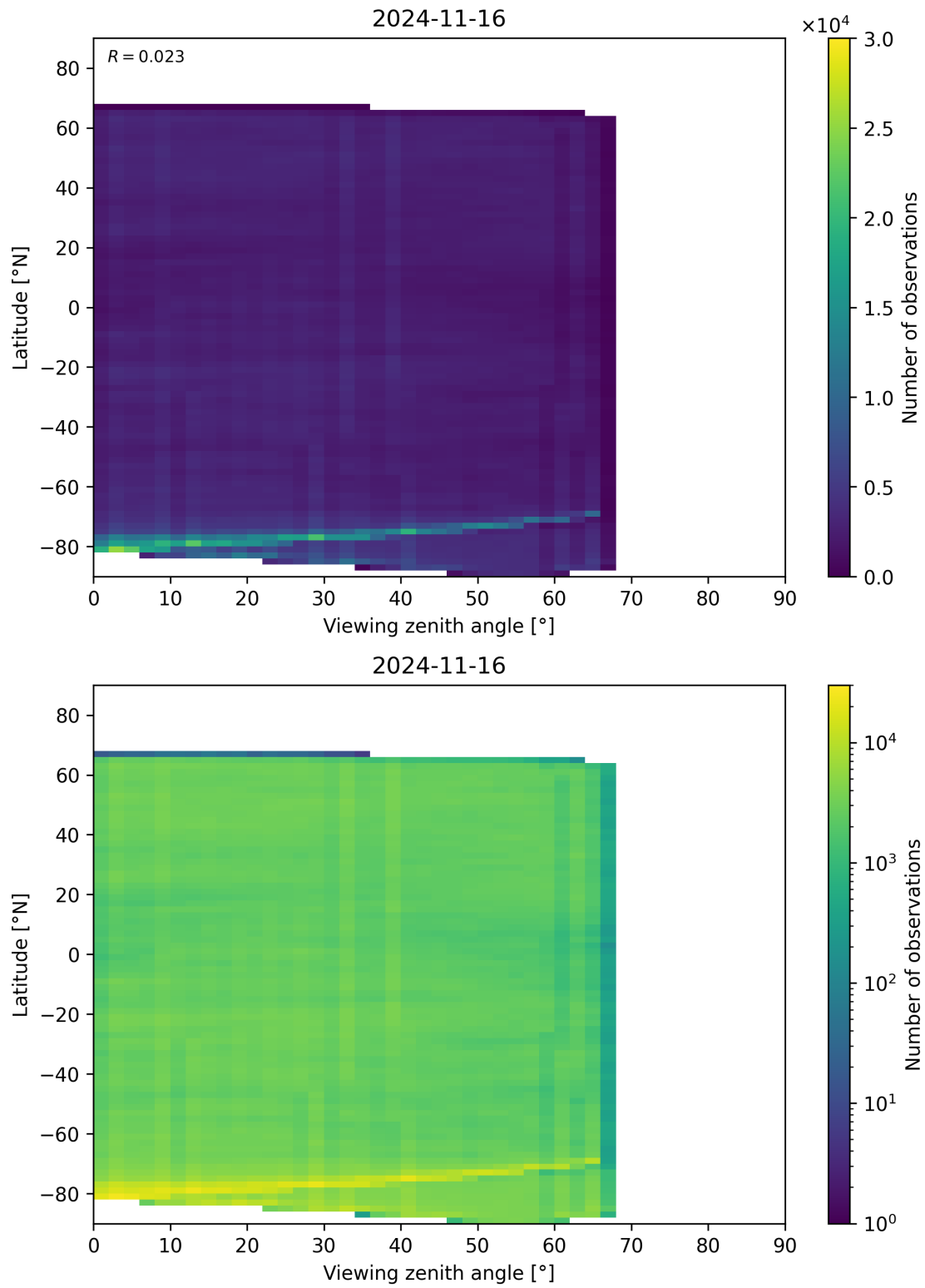
Figure 74: Scatter density plot of “Viewing zenith angle” against “Latitude” for 2024-11-15 to 2024-11-17.
