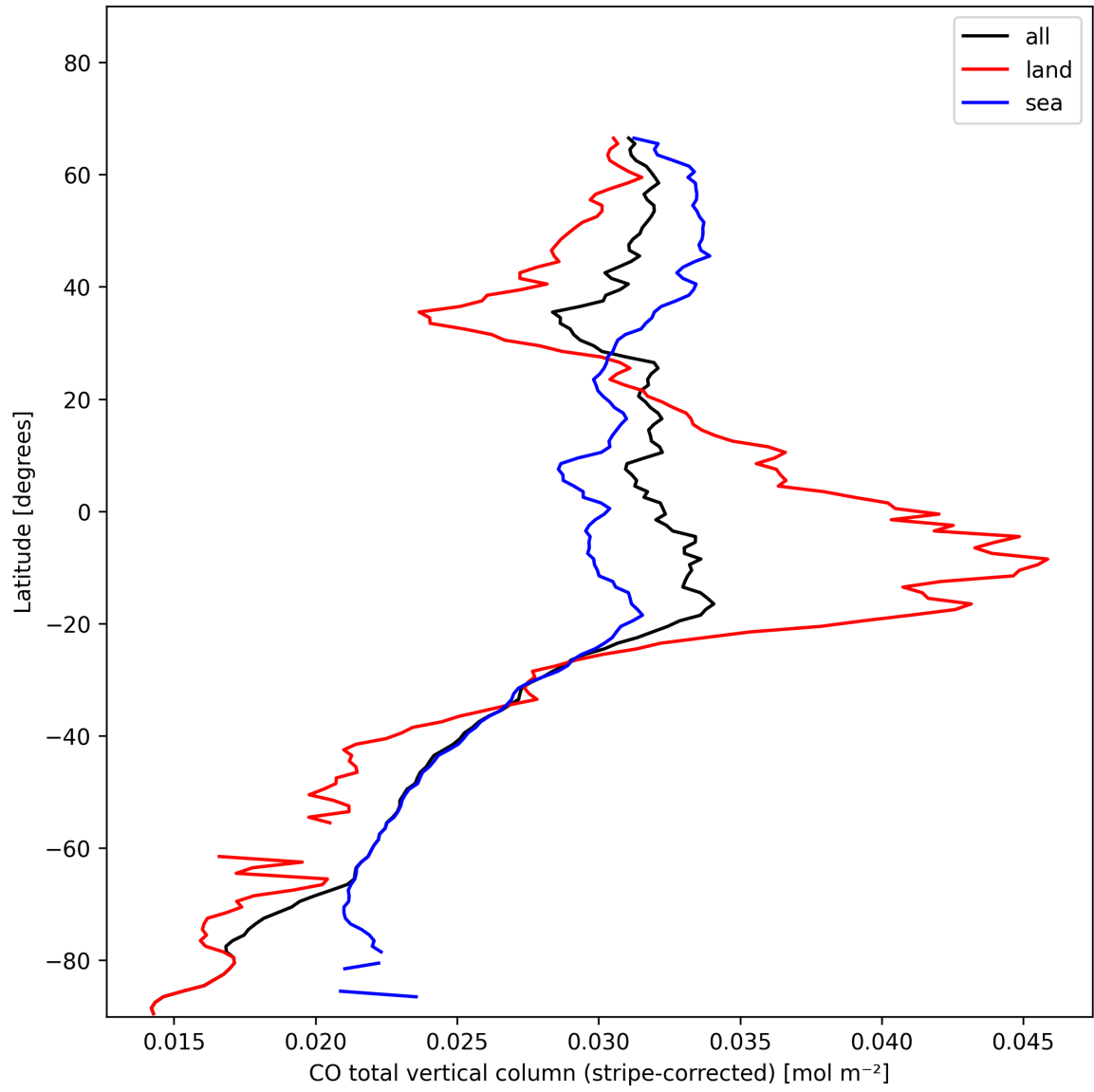
Figure 11: Zonal average of “CO total vertical column (stripe-corrected)” for 2024-11-15 to 2024-11-17.
