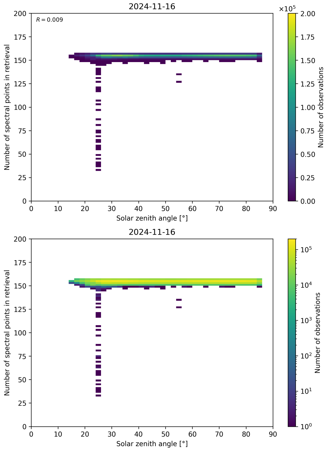
Figure 68: Scatter density plot of “Solar zenith angle” against “Number of spectral points in retrieval” for 2024-11-15 to 2024-11-17.
