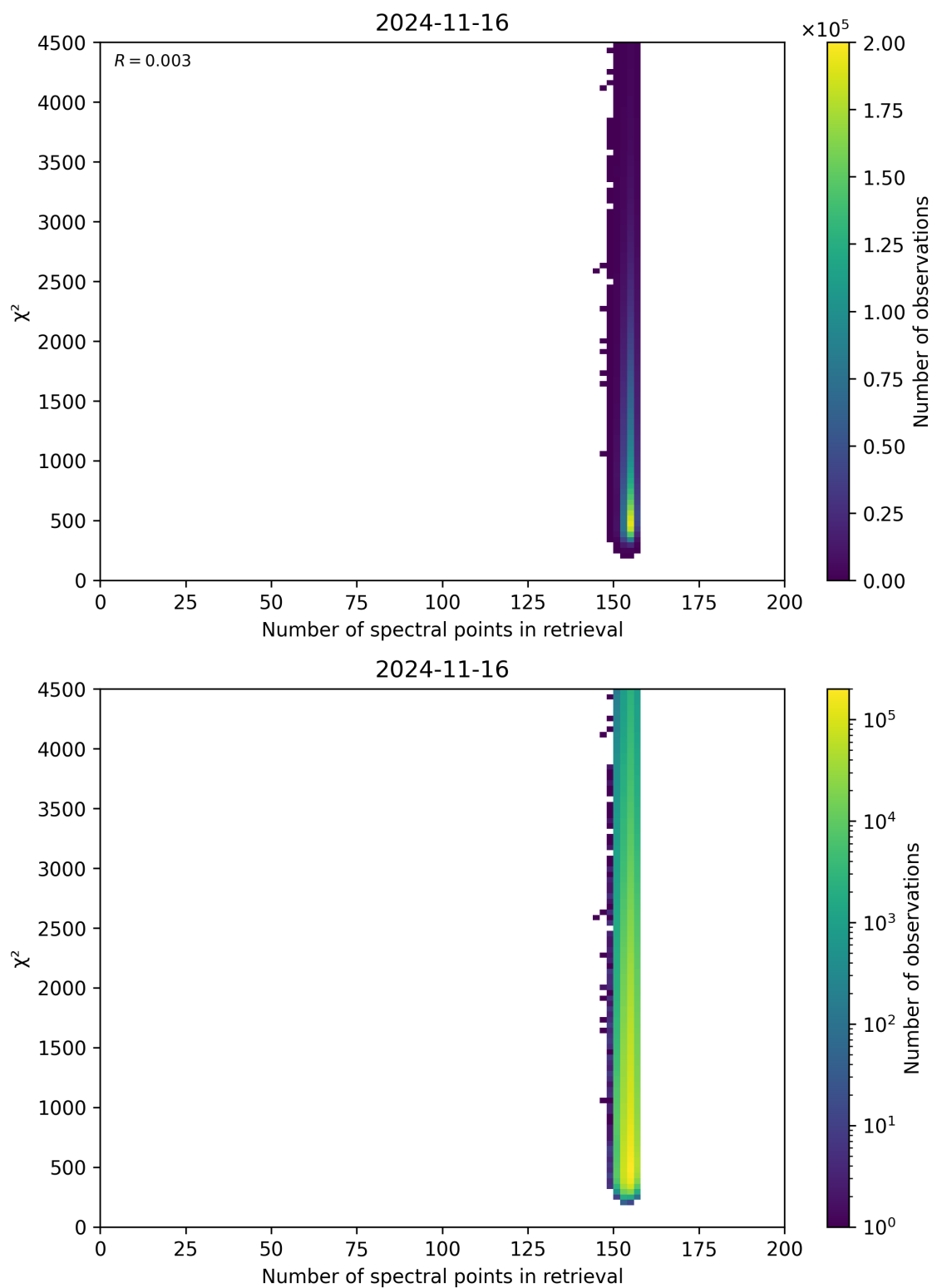
Figure 58: Scatter density plot of “Number of spectral points in retrieval” against “ \chi^2 ” for 2024-11-15 to 2024-11-17.
