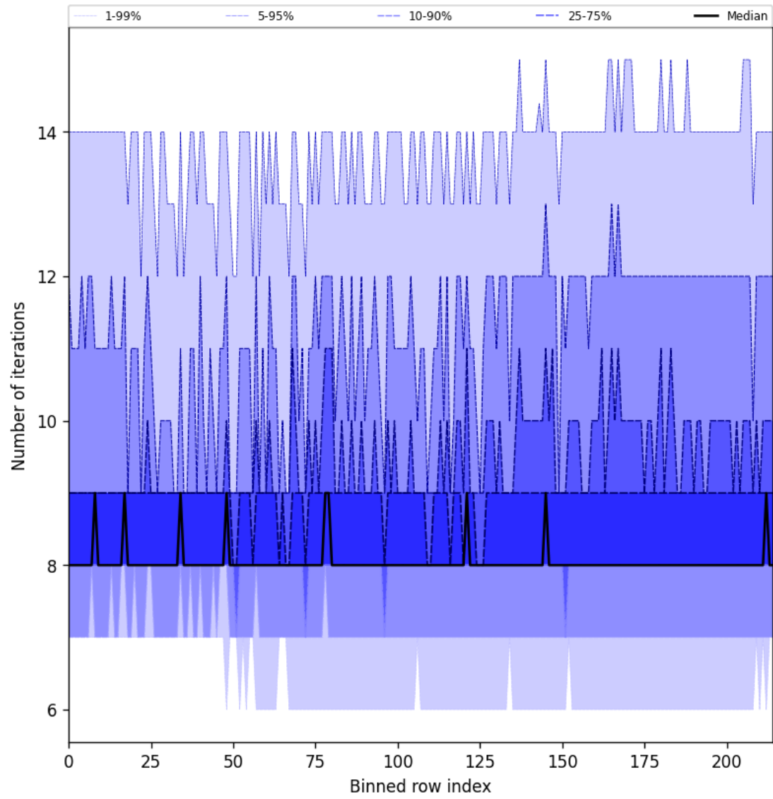
Figure 32: Along track statistics of “Number of iterations” for 2024-11-15 to 2024-11-17
