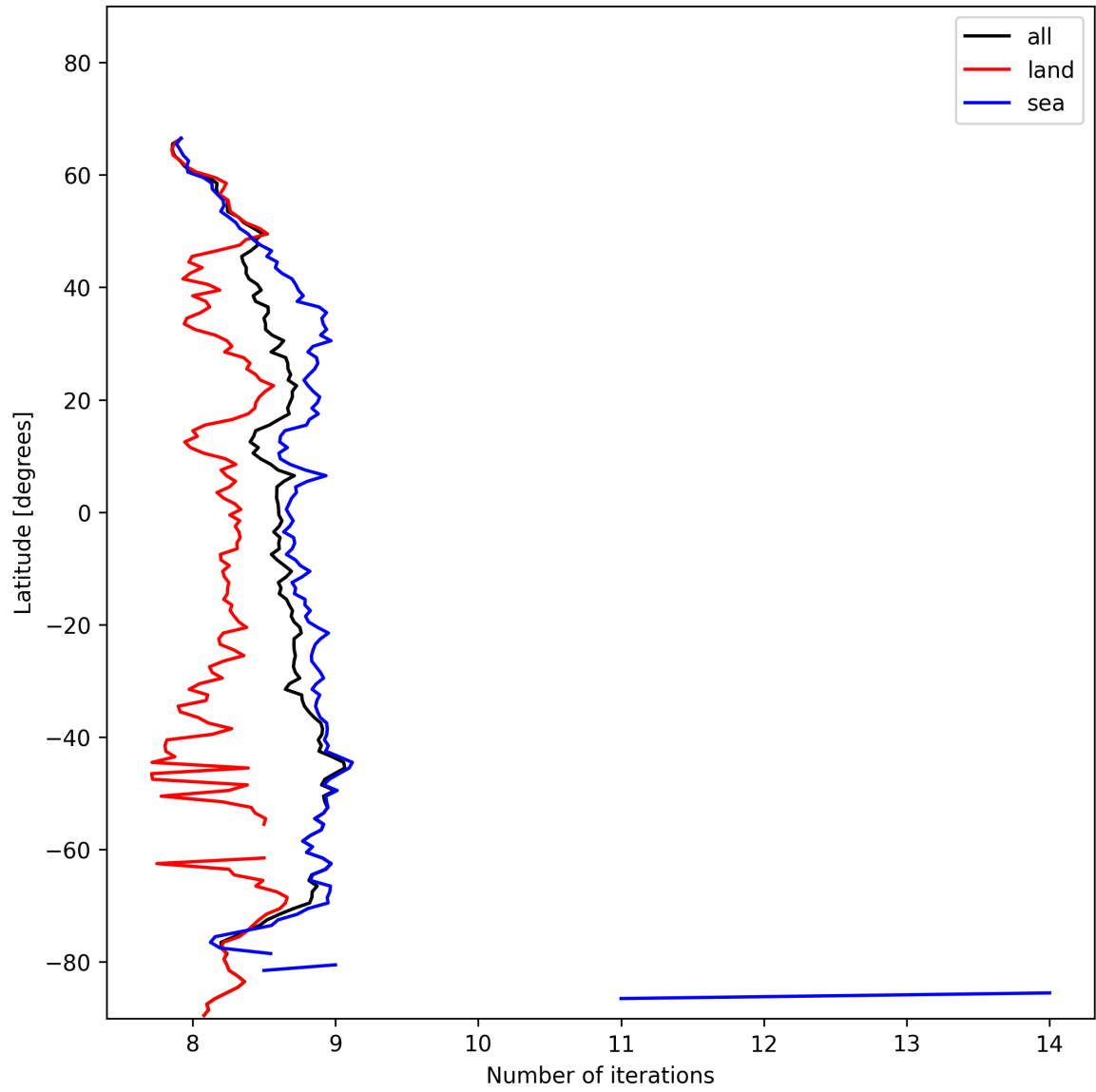
Figure 16: Zonal average of “Number of iterations” for 2024-11-15 to 2024-11-17.
