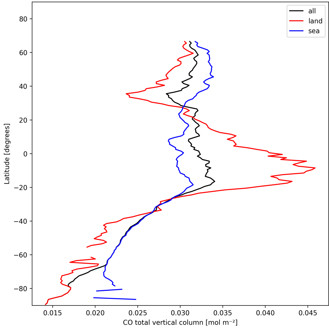
Figure 10: Zonal average of “CO total vertical column” for 2024-11-15 to 2024-11-17.
