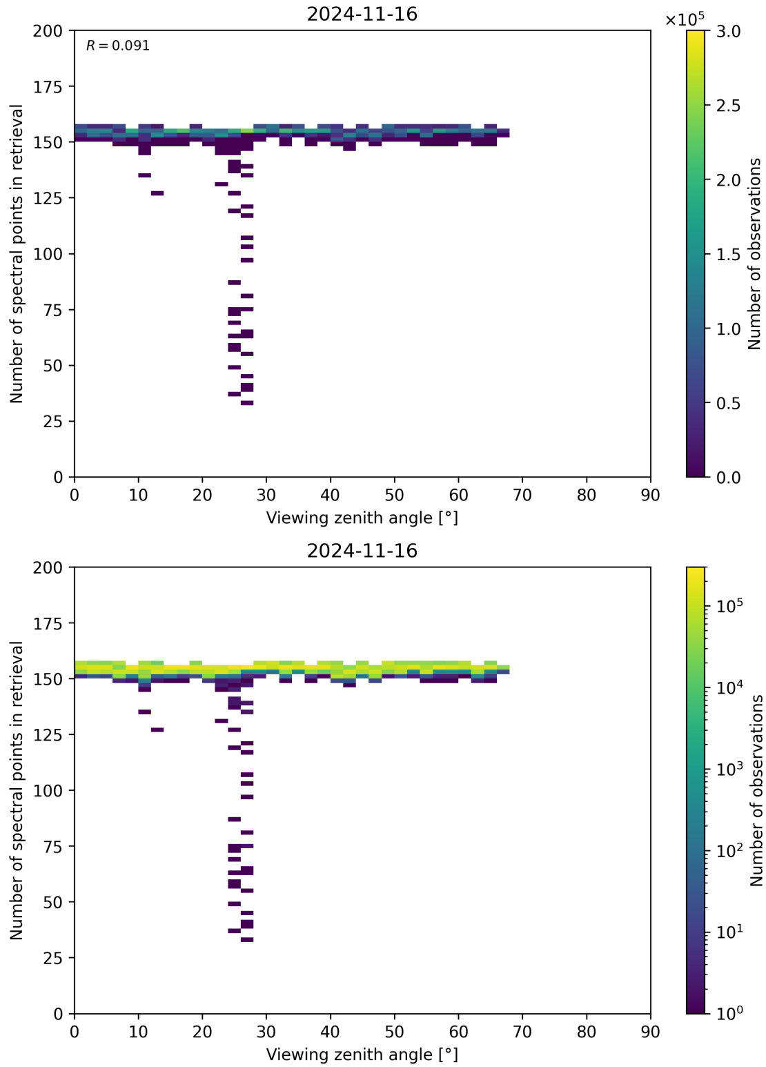
Figure 76: Scatter density plot of “Viewing zenith angle” against “Number of spectral points in retrieval” for 2024-11-15 to 2024-11-17.
