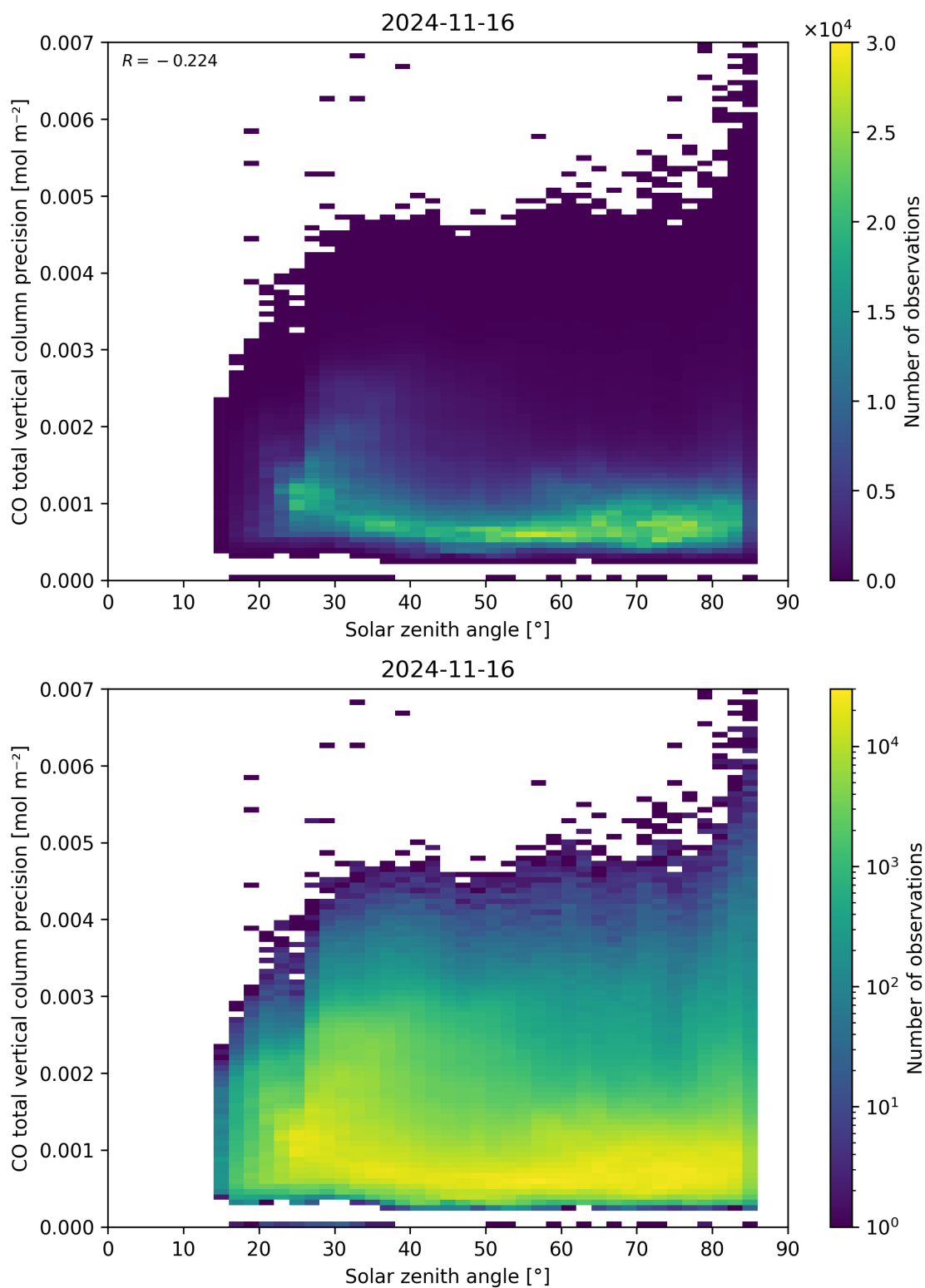
Figure 63: Scatter density plot of “Solar zenith angle” against “CO total vertical column precision” for 2024-11-15 to 2024-11-17.
