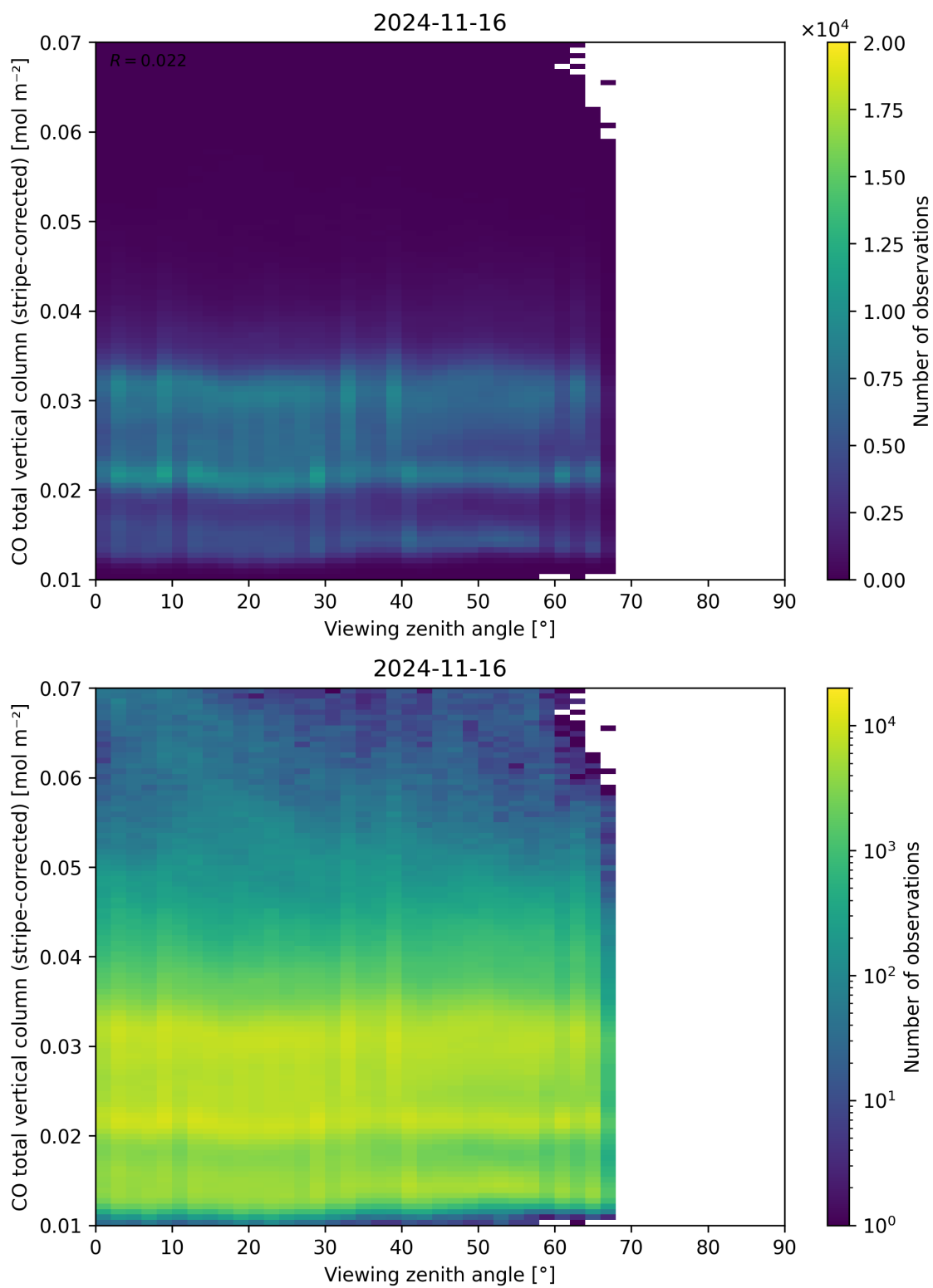
Figure 70: Scatter density plot of “Viewing zenith angle” against “CO total vertical column (stripe-corrected)” for 2024-11-15 to 2024-11-17.
