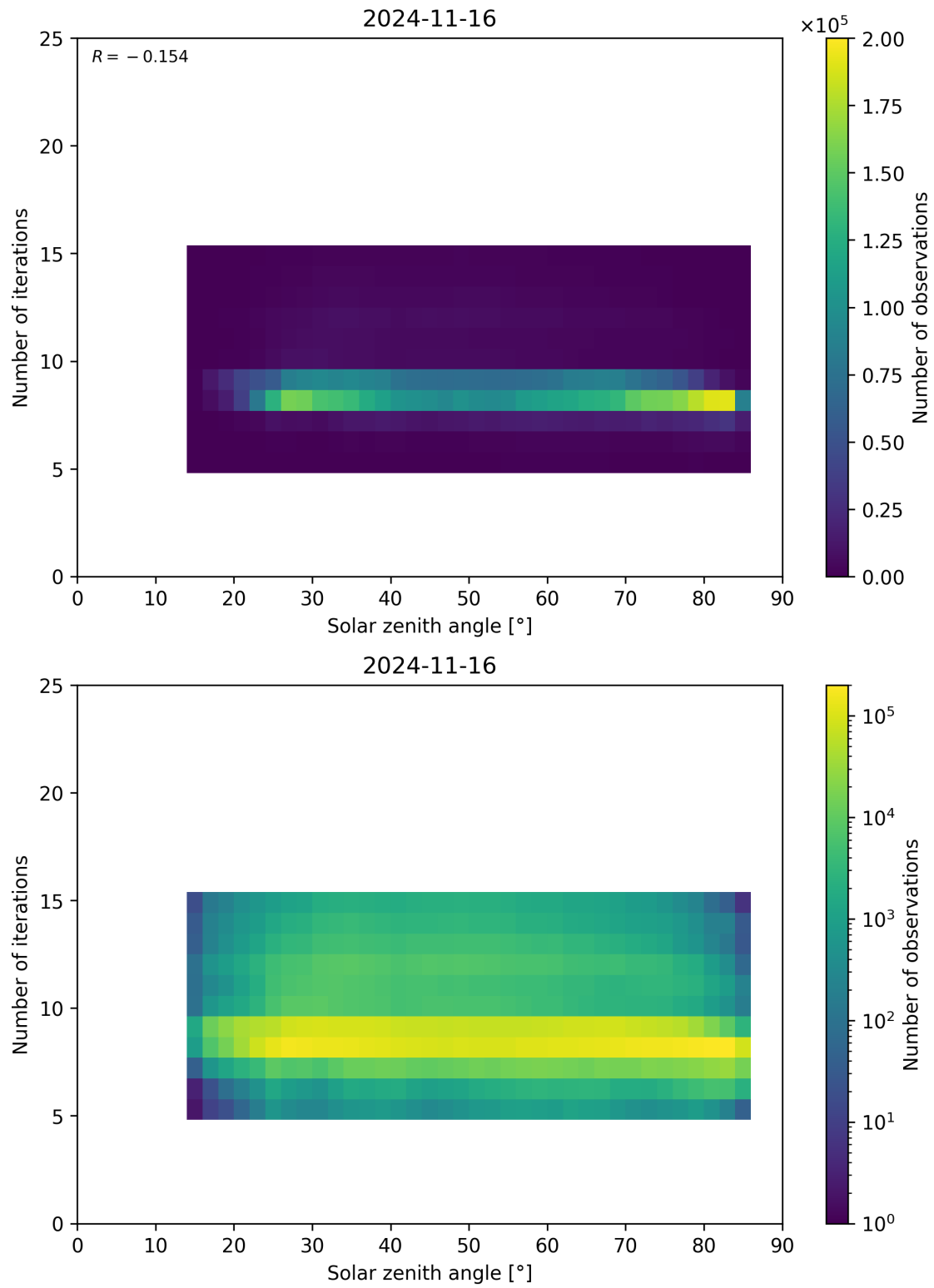
Figure 67: Scatter density plot of “Solar zenith angle” against “Number of iterations” for 2024-11-15 to 2024-11-17.
