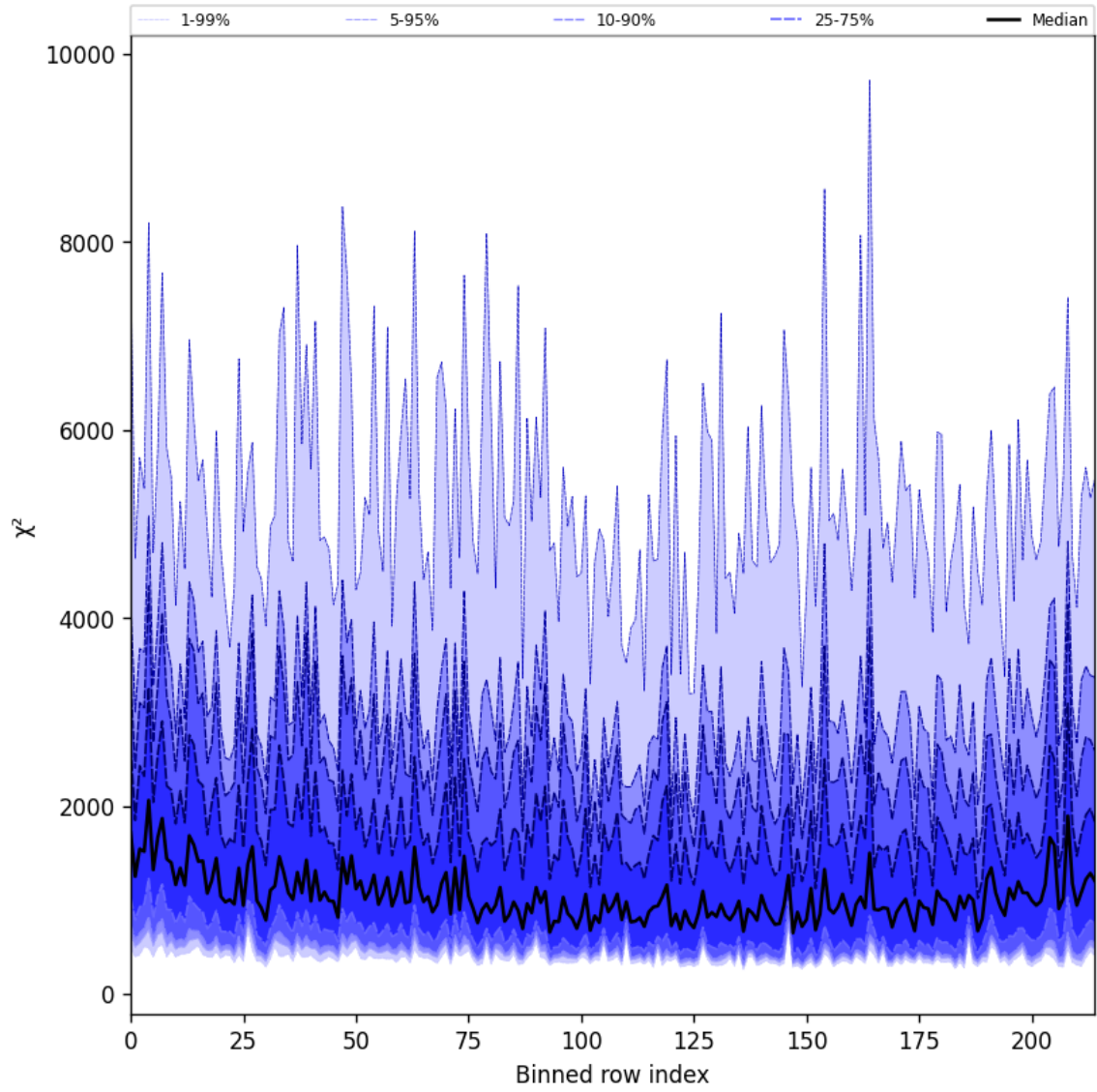
Figure 30: Along track statistics of “ \chi^2 ” for 2024-11-15 to 2024-11-17
