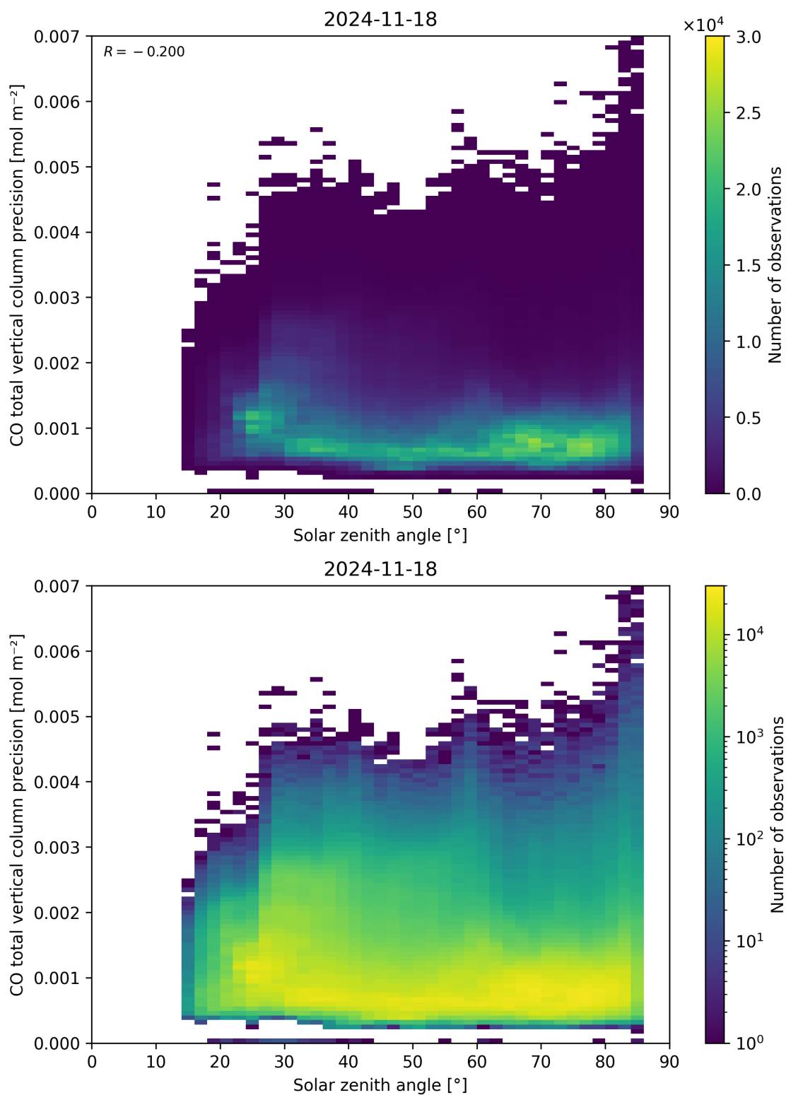
Figure 63: Scatter density plot of “Solar zenith angle” against “CO total vertical column precision” for 2024-11-17 to 2024-11-19.
