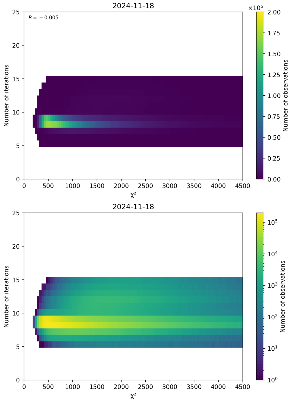
Figure 49: Scatter density plot of “ \chi^2 ” against “Number of iterations” for 2024-11-17 to 2024-11-19.
