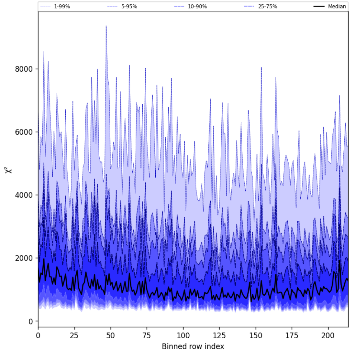
Figure 30: Along track statistics of “ \chi^2 ” for 2024-11-17 to 2024-11-19
