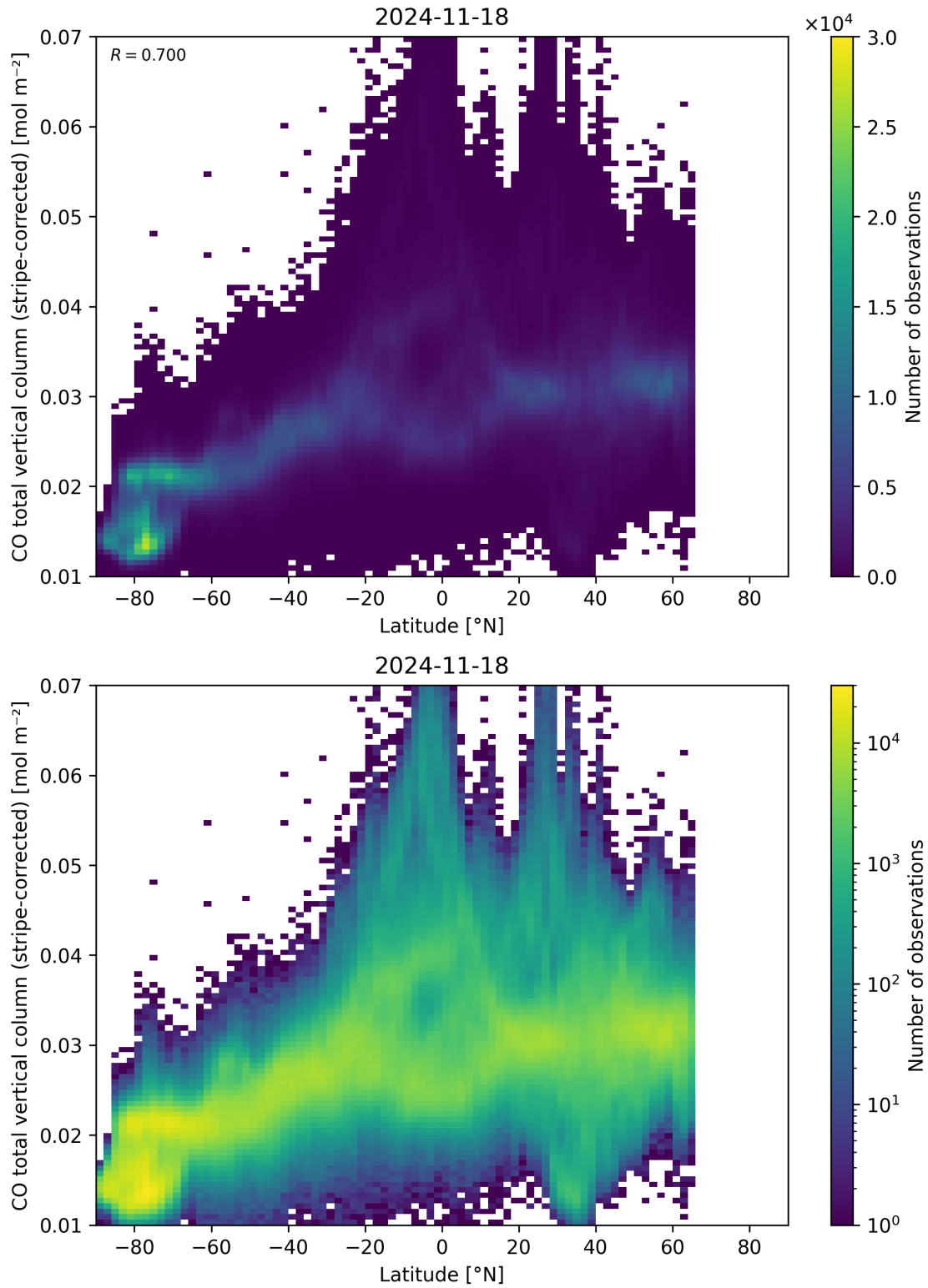
Figure 52: Scatter density plot of “Latitude” against “CO total vertical column (stripe-corrected)” for 2024-11-17 to 2024-11-19.
