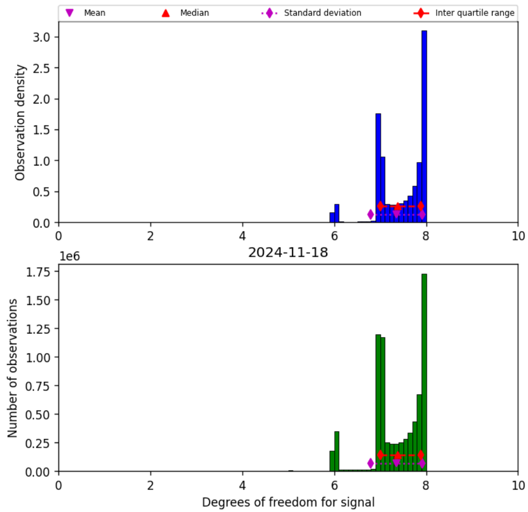
Figure 23: Histogram of “Degrees of freedom for signal” for 2024-11-17 to 2024-11-19
