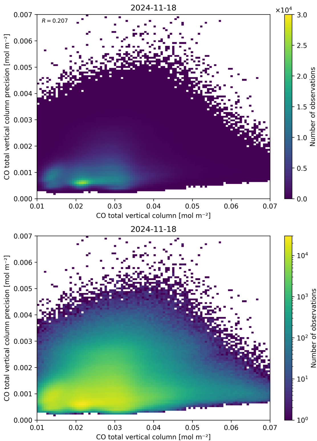
Figure 34: Scatter density plot of “CO total vertical column” against “CO total vertical column precision” for 2024-11-17 to 2024-11-19.
