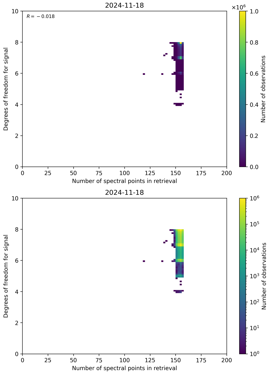
Figure 59: Scatter density plot of “Number of spectral points in retrieval” against “Degrees of freedom for signal” for 2024-11-17 to 2024-11-19.
