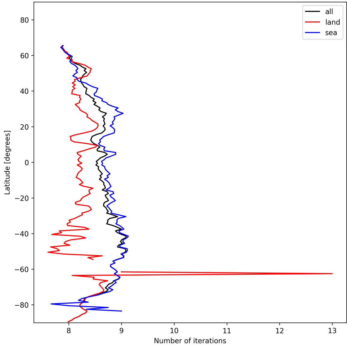
Figure 16: Zonal average of “Number of iterations” for 2024-11-17 to 2024-11-19.
