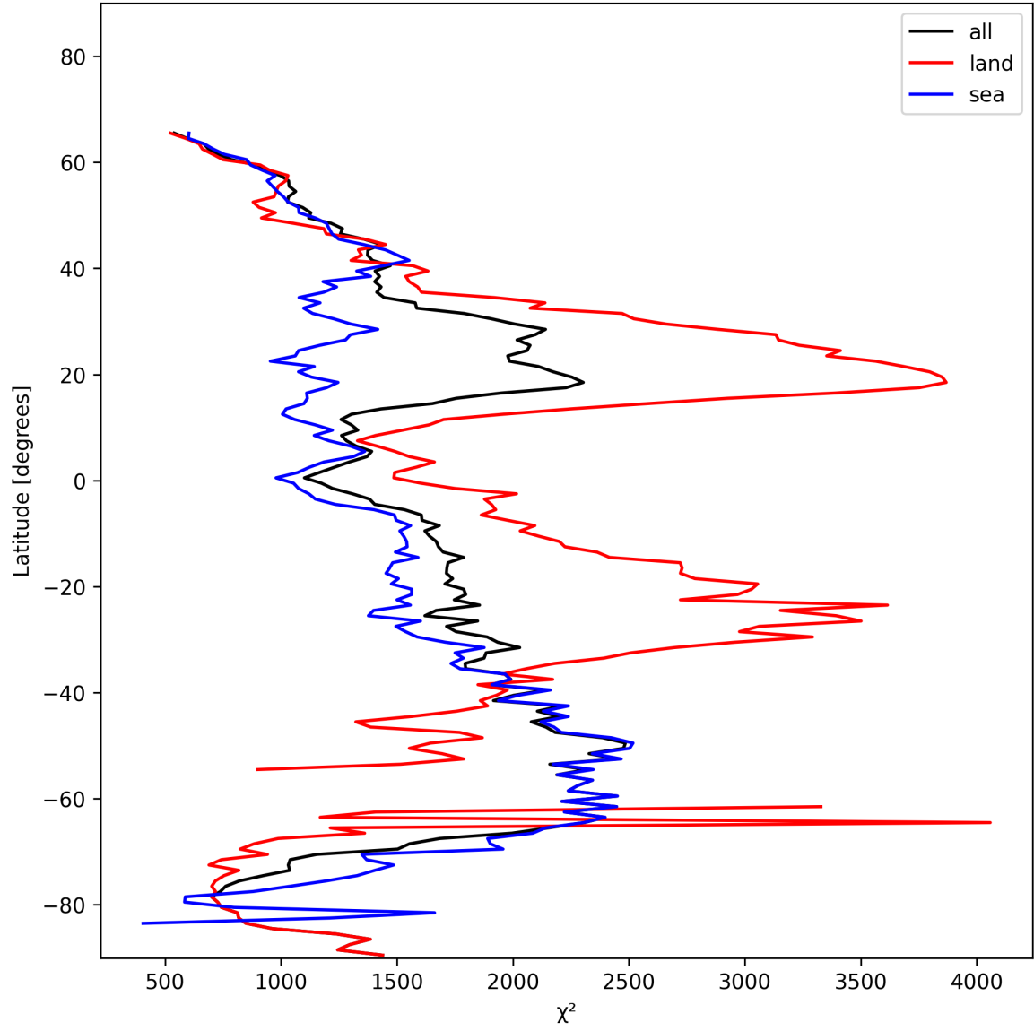
Figure 14: Zonal average of “ \chi^2 ” for 2024-11-17 to 2024-11-19.
