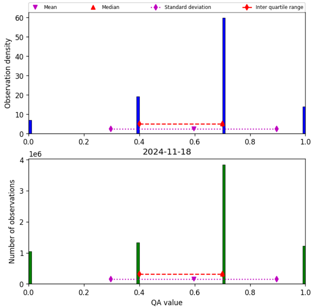
Figure 17: Histogram of “QA value” for 2024-11-17 to 2024-11-19
