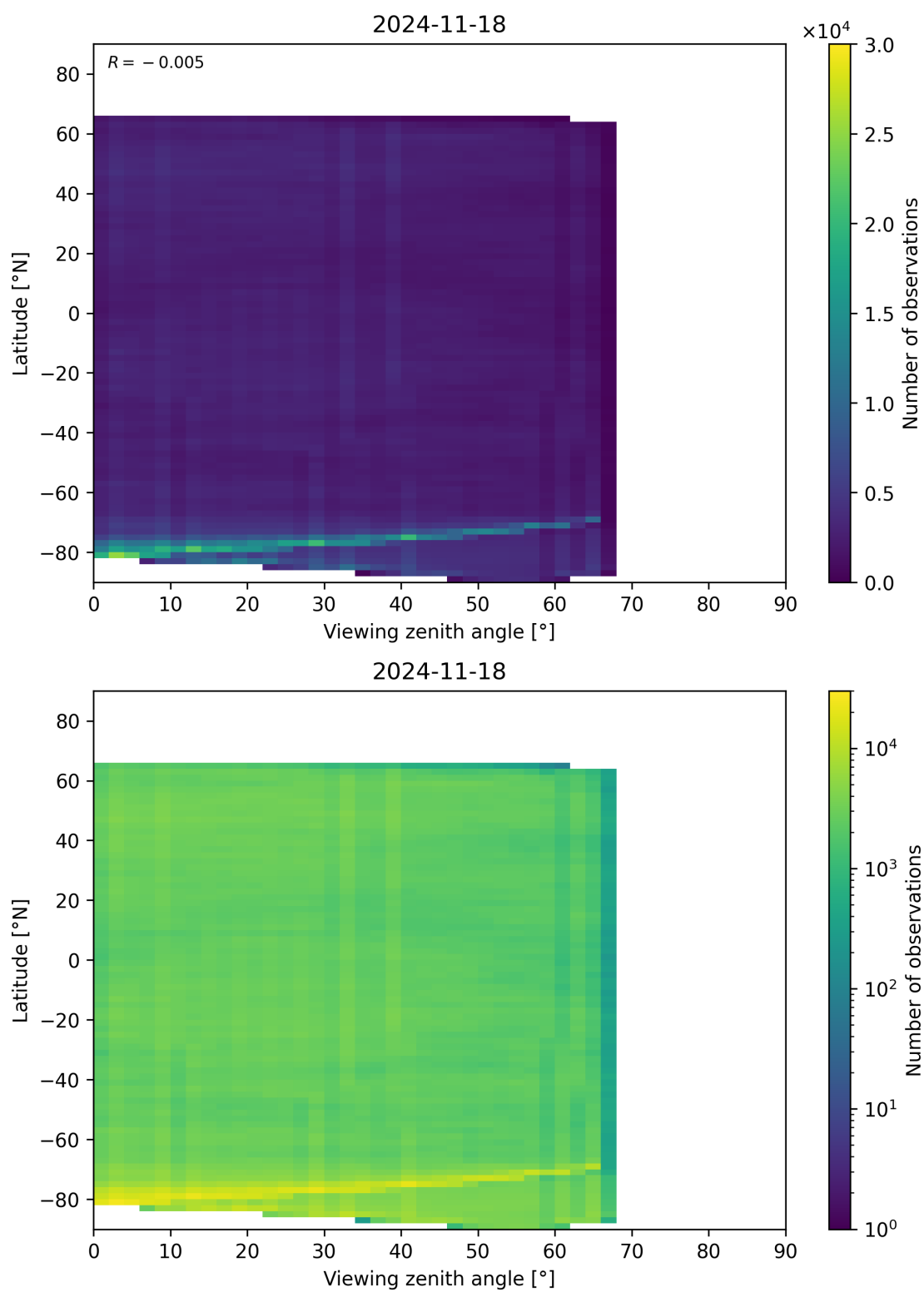
Figure 74: Scatter density plot of “Viewing zenith angle” against “Latitude” for 2024-11-17 to 2024-11-19.
