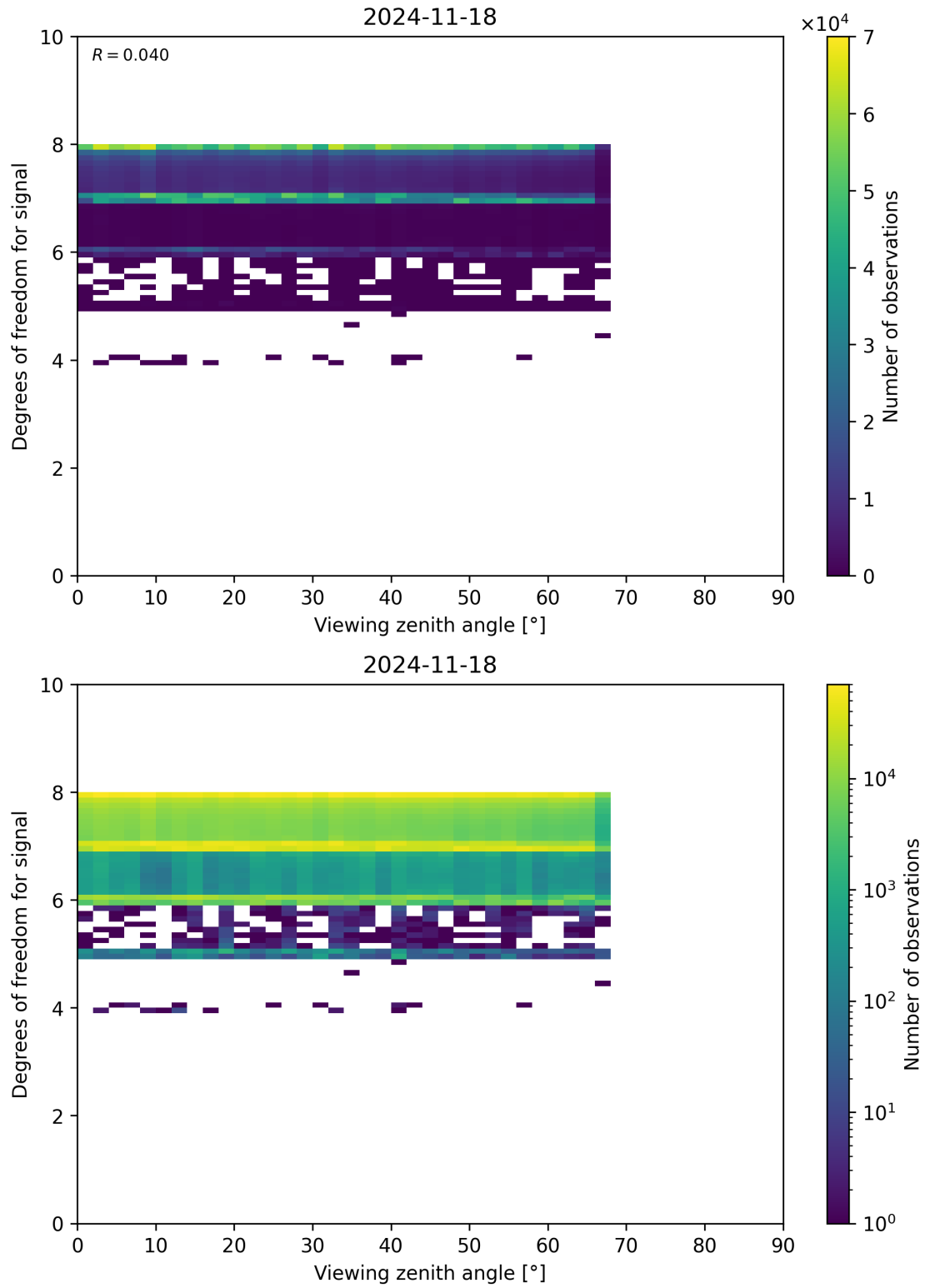
Figure 73: Scatter density plot of “Viewing zenith angle” against “Degrees of freedom for signal” for 2024-11-17 to 2024-11-19.
