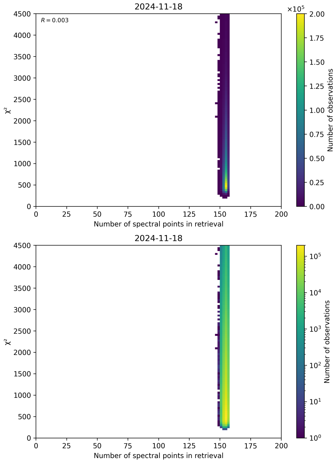
Figure 58: Scatter density plot of “Number of spectral points in retrieval” against “ \chi^2 ” for 2024-11-17 to 2024-11-19.
