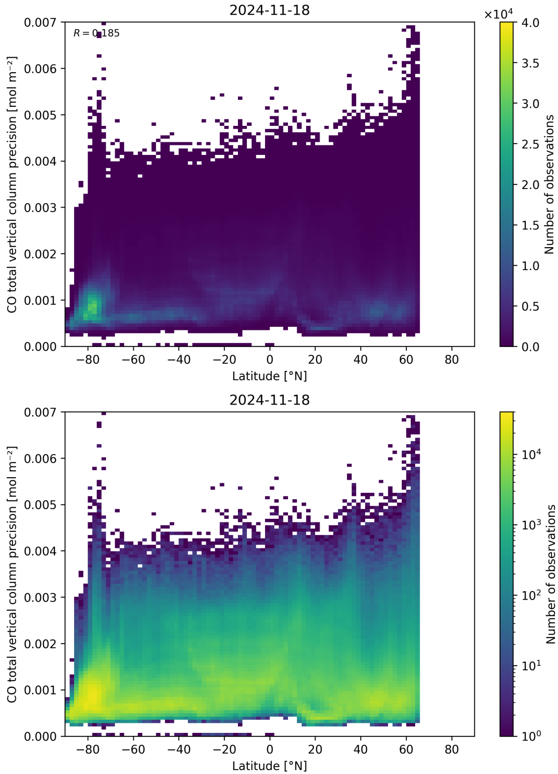
Figure 53: Scatter density plot of “Latitude” against “CO total vertical column precision” for 2024-11-17 to 2024-11-19.
