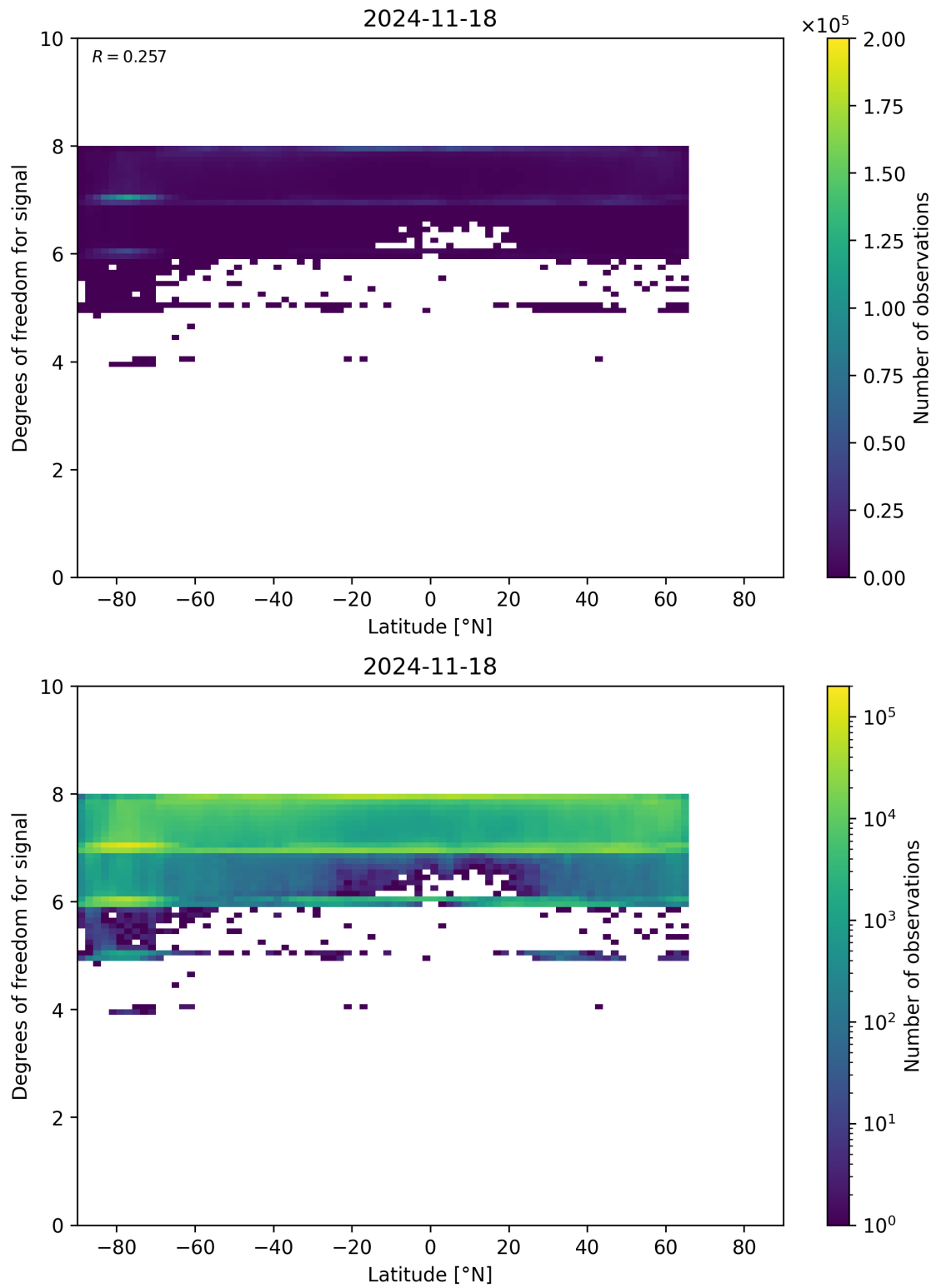
Figure 55: Scatter density plot of “Latitude” against “Degrees of freedom for signal” for 2024-11-17 to 2024-11-19.
