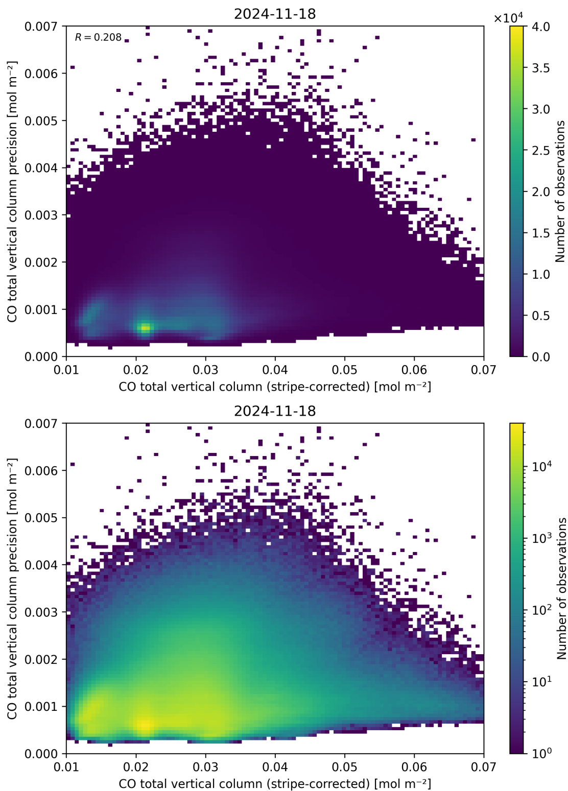
Figure 36: Scatter density plot of “CO total vertical column (stripe-corrected)” against “CO total vertical column precision” for 2024-11-17 to 2024-11-19.
