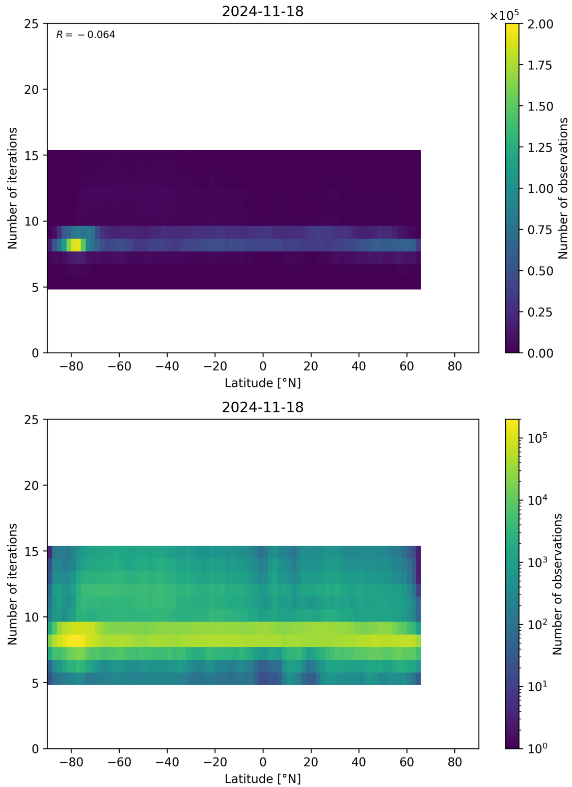
Figure 56: Scatter density plot of “Latitude” against “Number of iterations” for 2024-11-17 to 2024-11-19.
