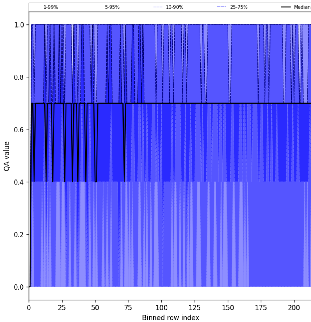
Figure 25: Along track statistics of “QA value” for 2024-11-17 to 2024-11-19
