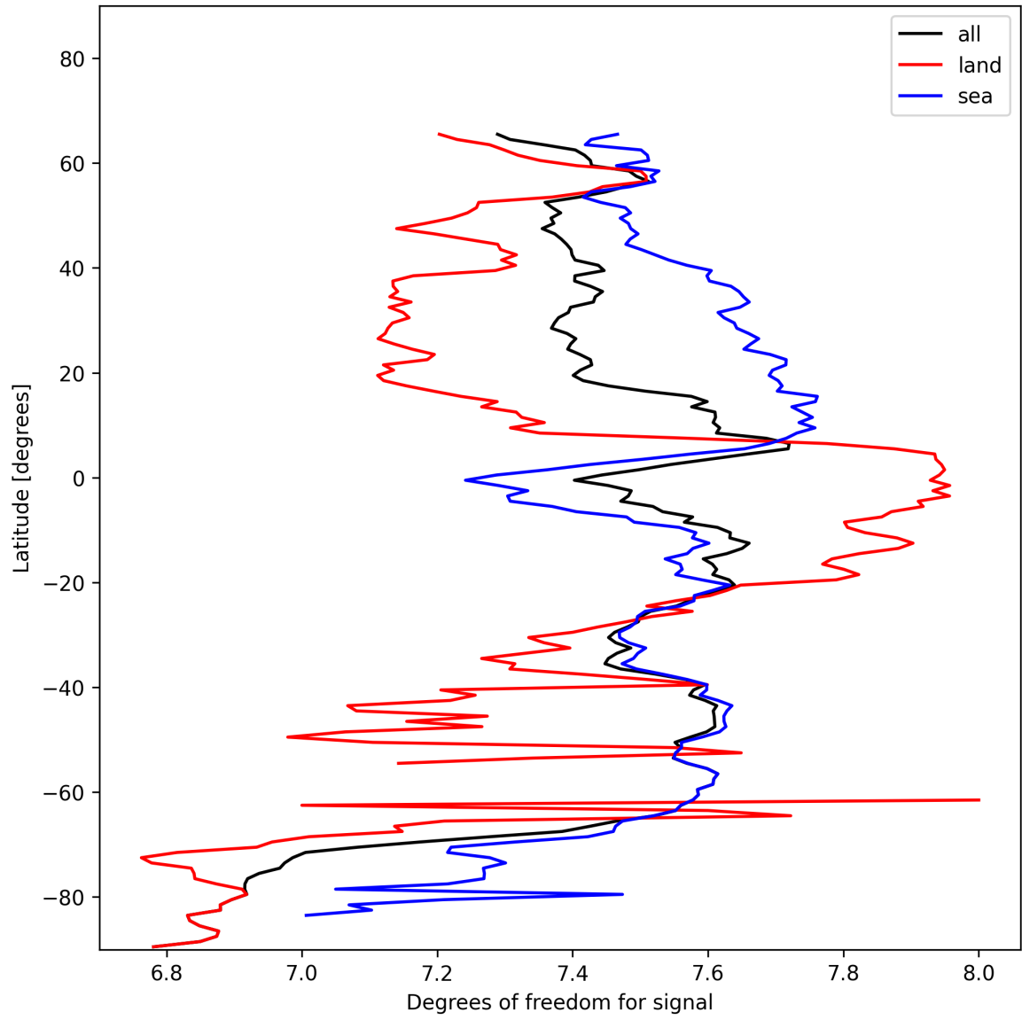
Figure 15: Zonal average of “Degrees of freedom for signal” for 2024-11-17 to 2024-11-19.
