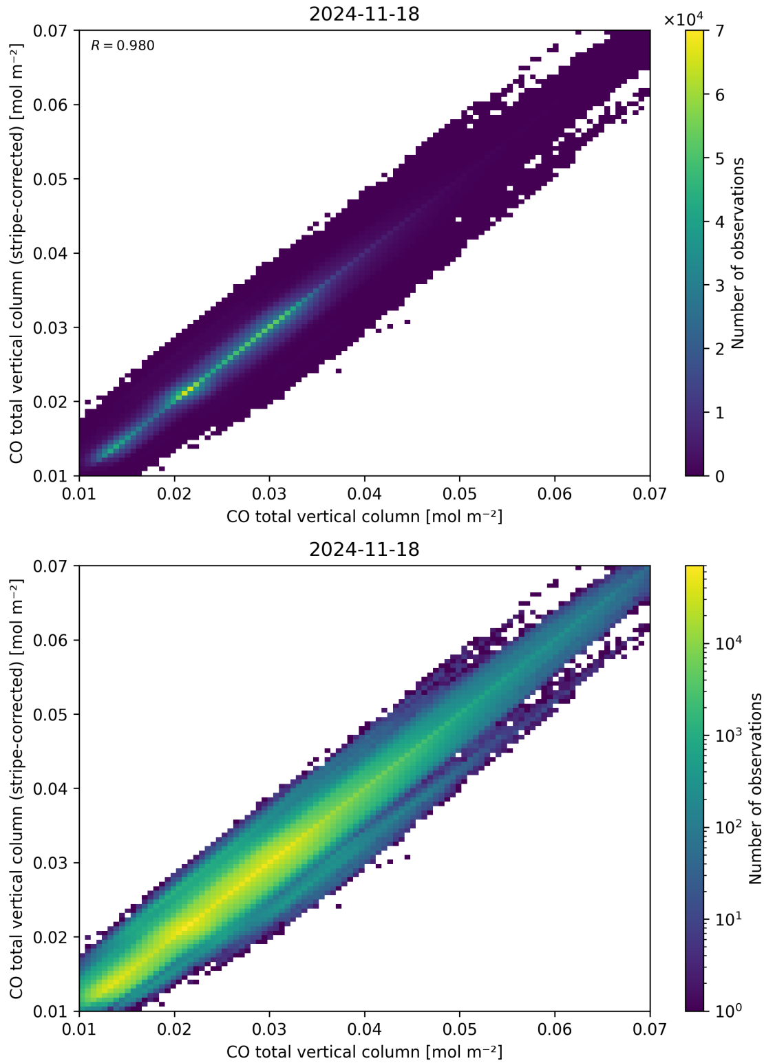
Figure 33: Scatter density plot of “CO total vertical column” against “CO total vertical column (stripe-corrected)” for 2024-11-17 to 2024-11-19.
