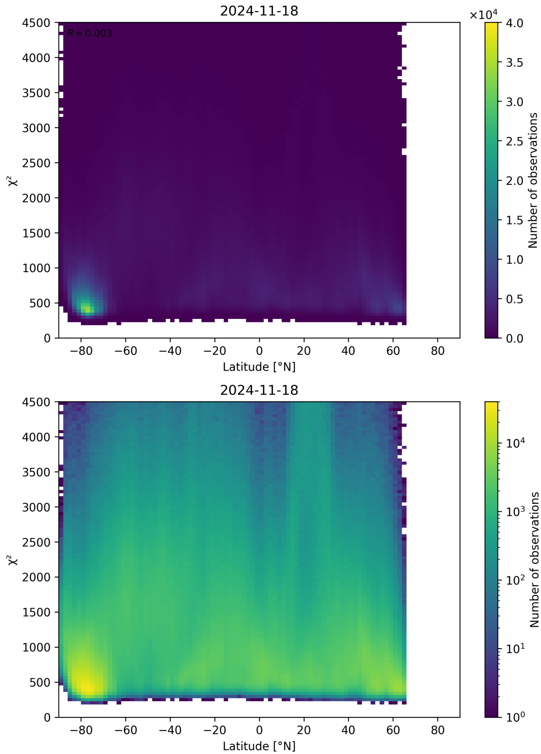
Figure 54: Scatter density plot of “Latitude” against “ \chi^2 ” for 2024-11-17 to 2024-11-19.
