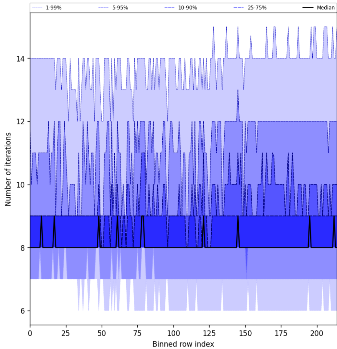
Figure 32: Along track statistics of “Number of iterations” for 2024-11-17 to 2024-11-19
