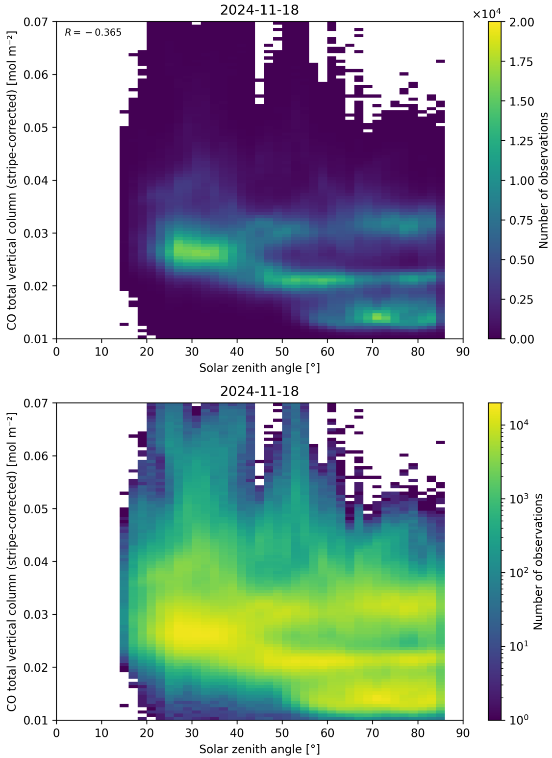
Figure 62: Scatter density plot of “Solar zenith angle” against “CO total vertical column (stripe-corrected)” for 2024-11-17 to 2024-11-19.
