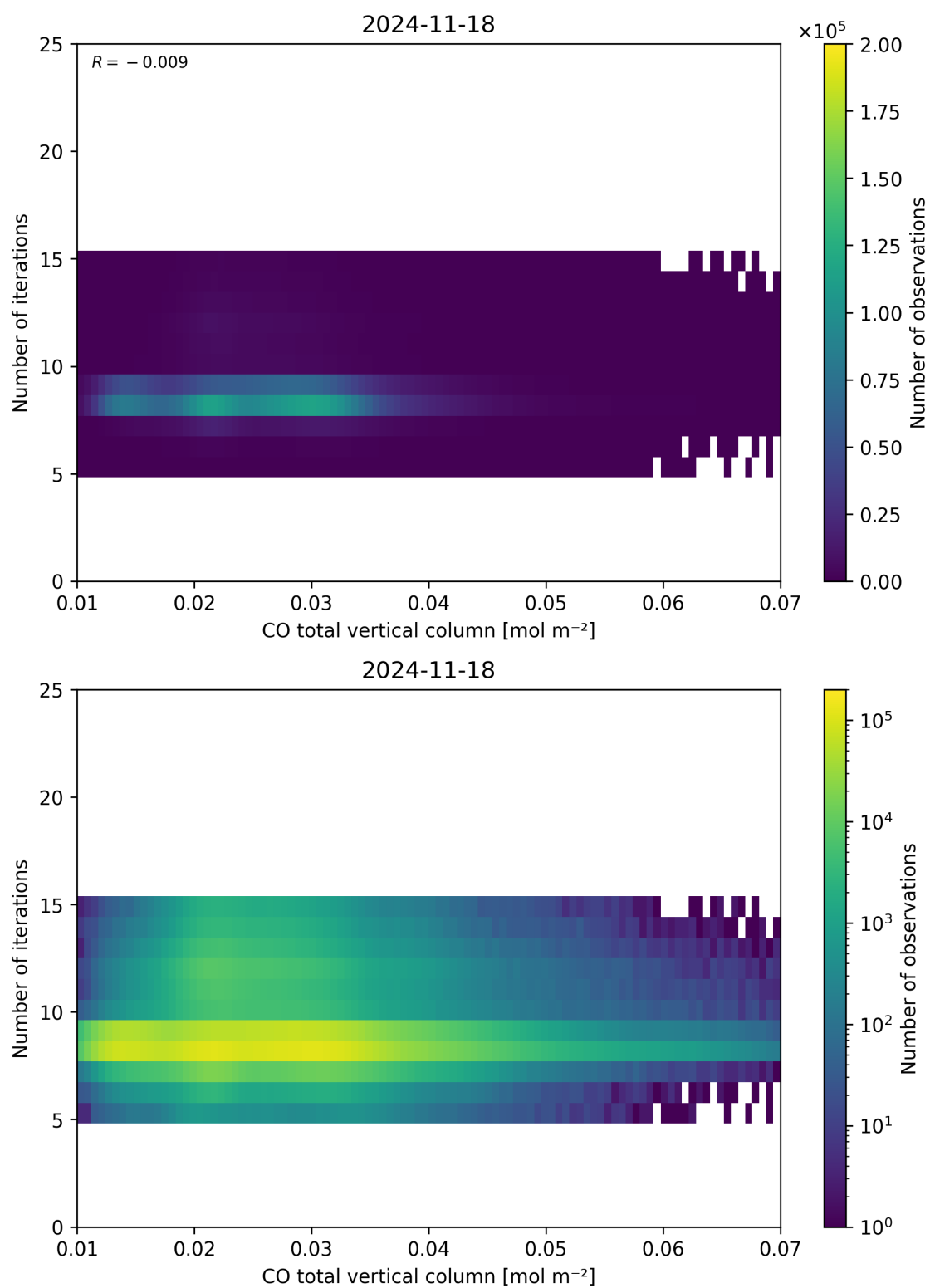
Figure 42: Scatter density plot of “CO total vertical column” against “Number of iterations” for 2024-11-17 to 2024-11-19.
