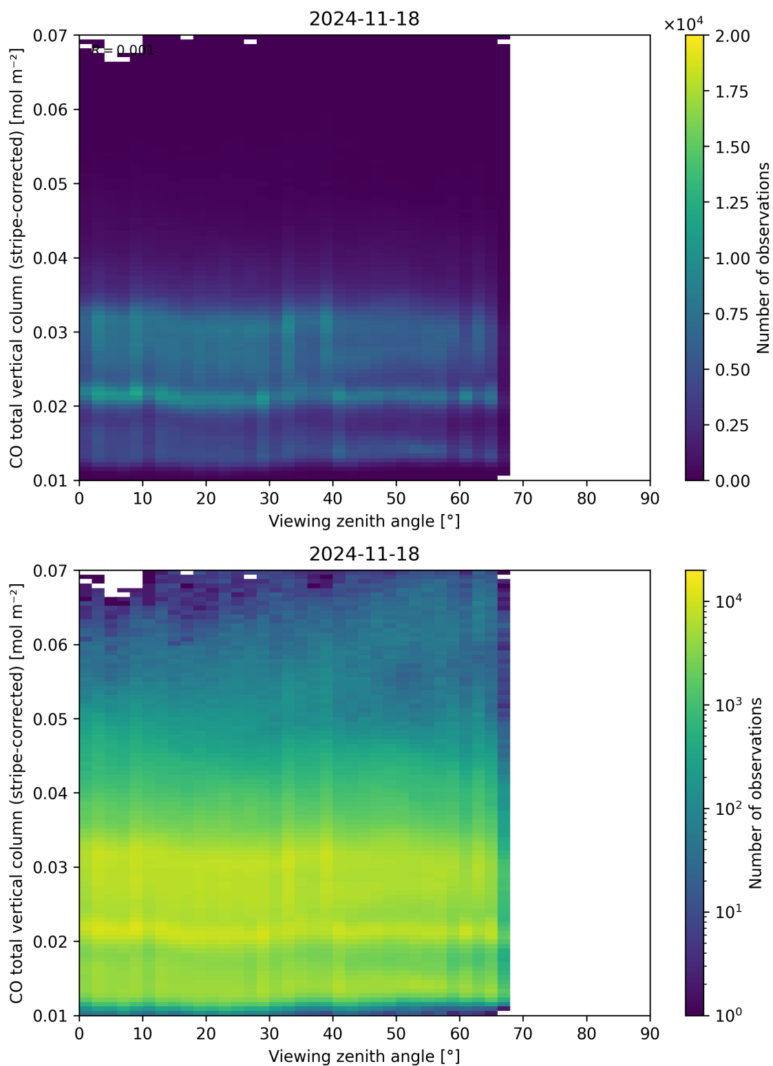
Figure 70: Scatter density plot of “Viewing zenith angle” against “CO total vertical column (stripe-corrected)” for 2024-11-17 to 2024-11-19.
