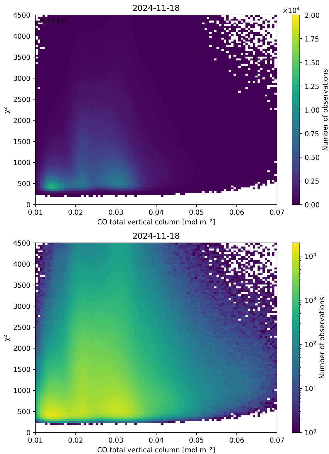
Figure 35: Scatter density plot of “CO total vertical column” against “ \chi^2 ” for 2024-11-17 to 2024-11-19.
