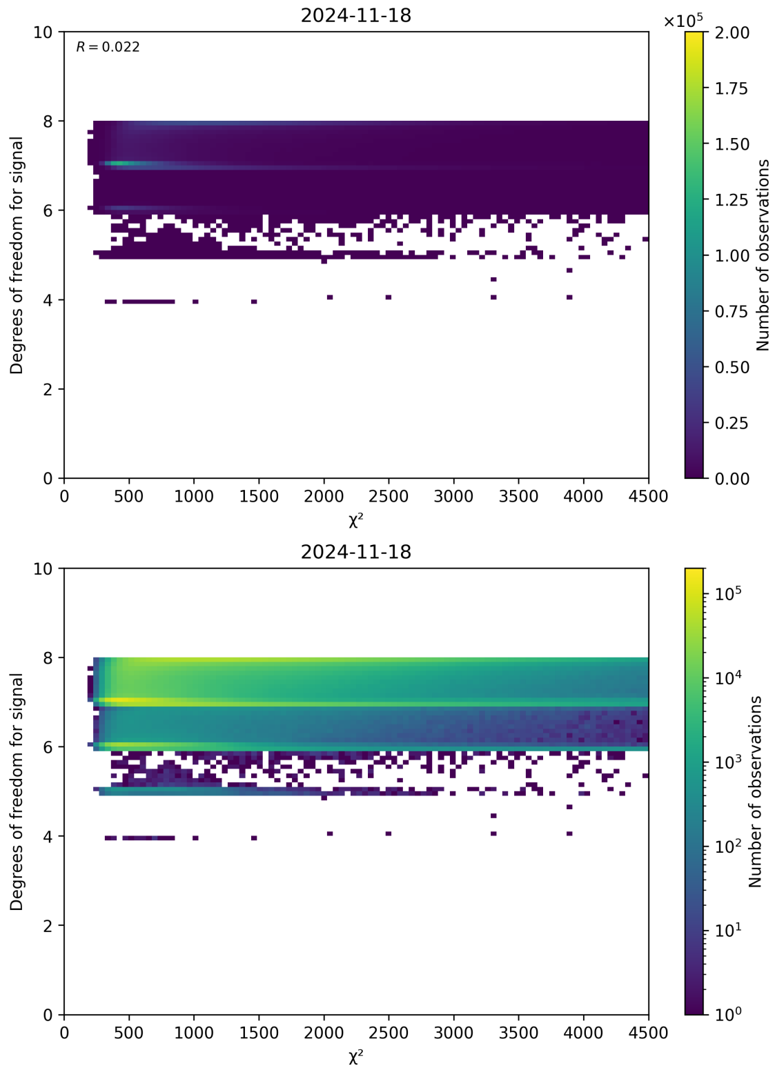
Figure 48: Scatter density plot of “ \chi^2 ” against “Degrees of freedom for signal” for 2024-11-17 to 2024-11-19.
