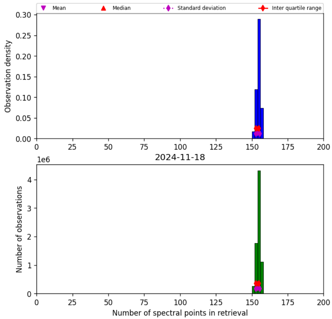
Figure 21: Histogram of “Number of spectral points in retrieval” for 2024-11-17 to 2024-11-19
