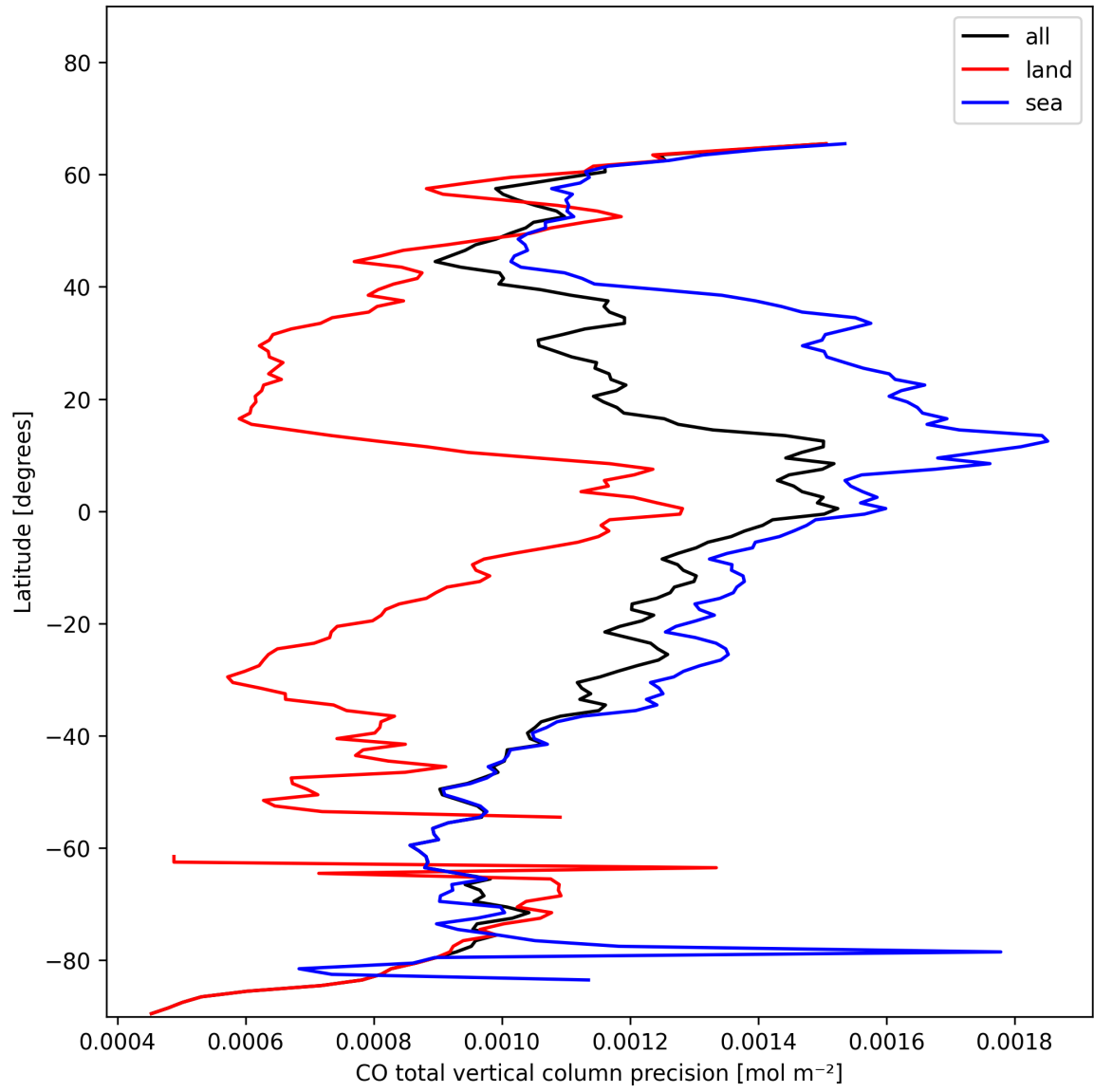
Figure 12: Zonal average of “CO total vertical column precision” for 2024-11-17 to 2024-11-19.
