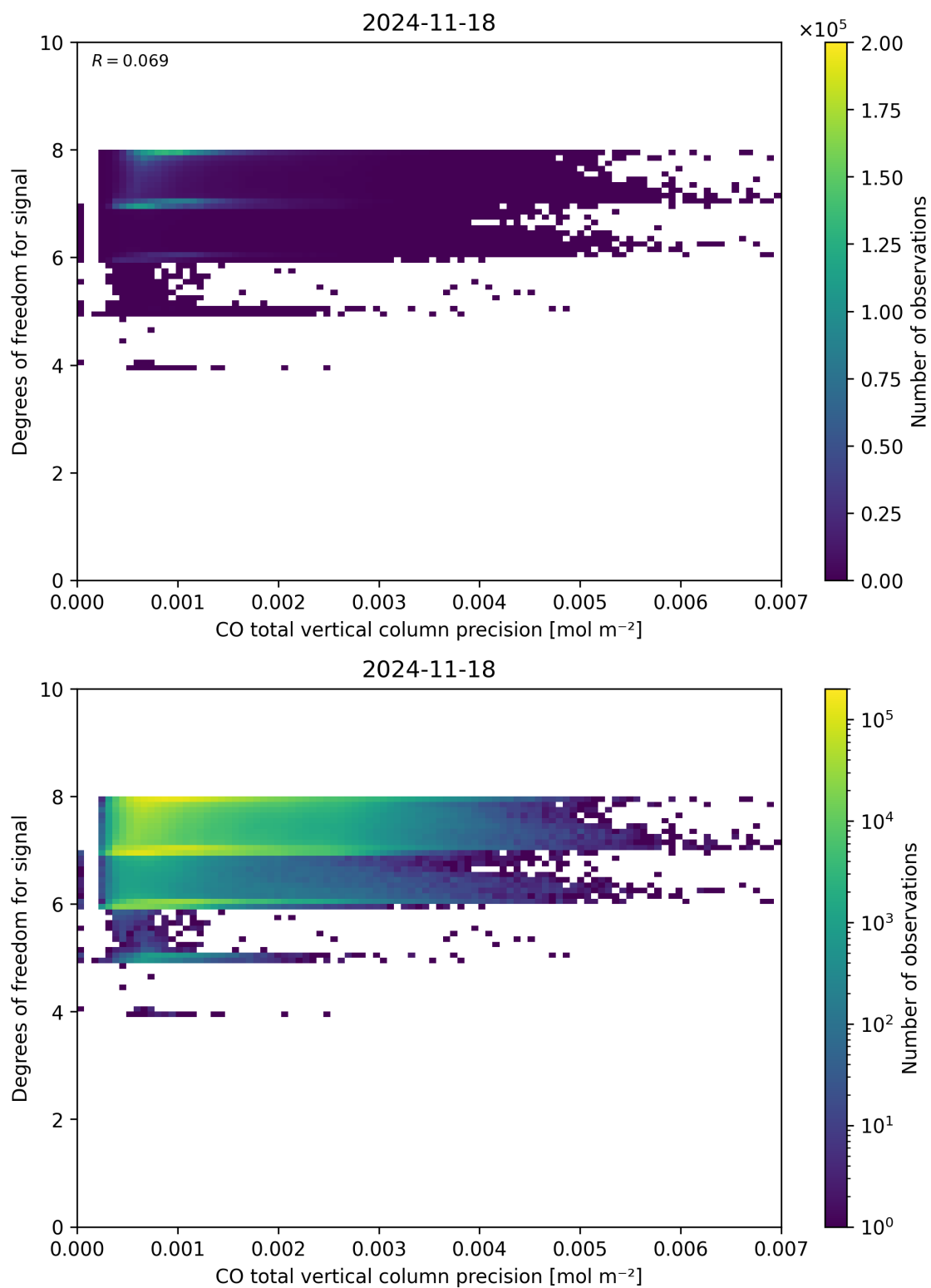
Figure 45: Scatter density plot of “CO total vertical column precision” against “Degrees of freedom for signal” for 2024-11-17 to 2024-11-19.
