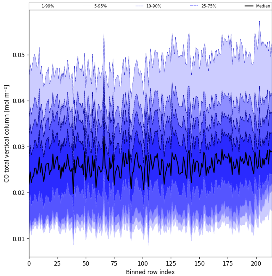
Figure 26: Along track statistics of “CO total vertical column” for 2024-11-17 to 2024-11-19
