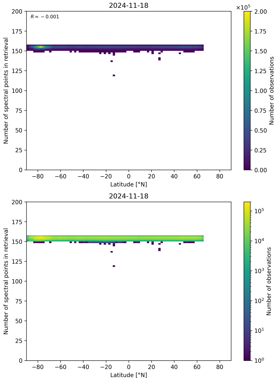
Figure 57: Scatter density plot of “Latitude” against “Number of spectral points in retrieval” for 2024-11-17 to 2024-11-19.
