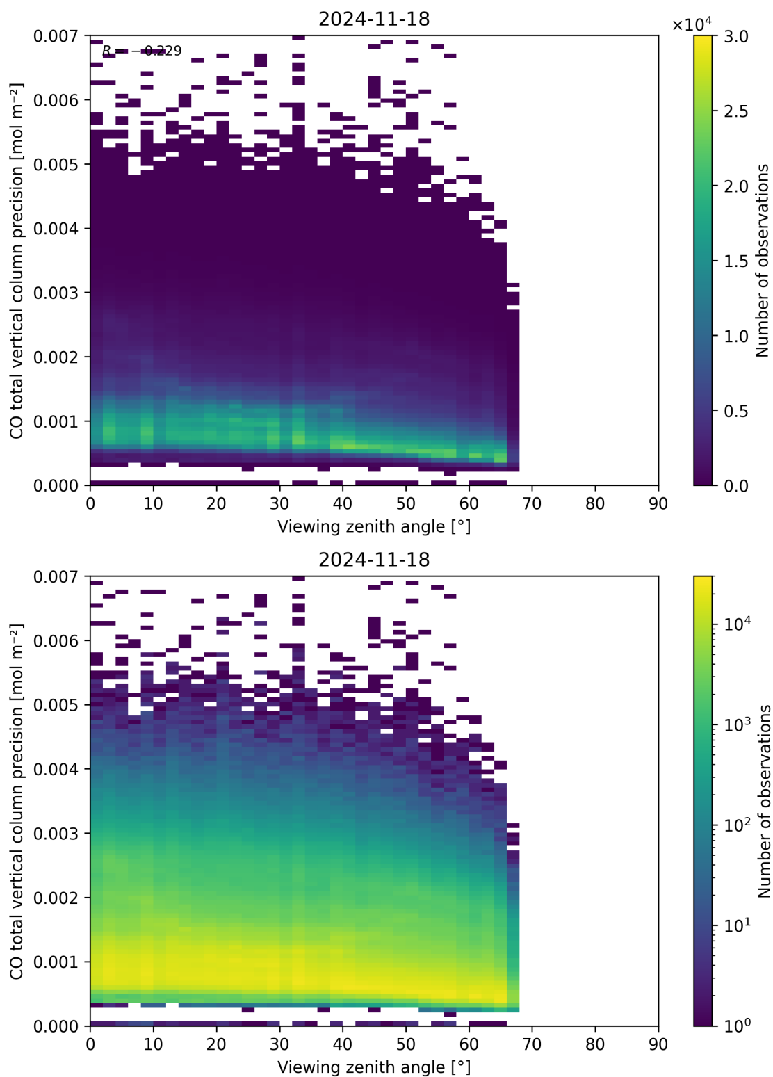
Figure 71: Scatter density plot of “Viewing zenith angle” against “CO total vertical column precision” for 2024-11-17 to 2024-11-19.
