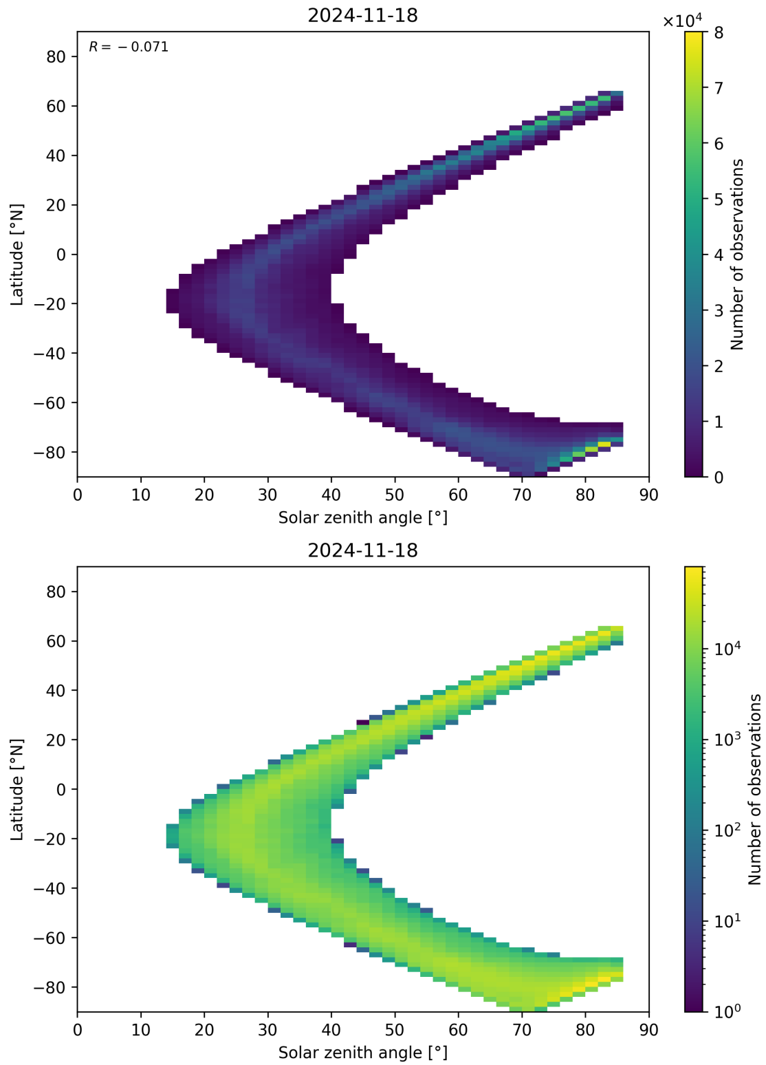
Figure 66: Scatter density plot of “Solar zenith angle” against “Latitude” for 2024-11-17 to 2024-11-19.
