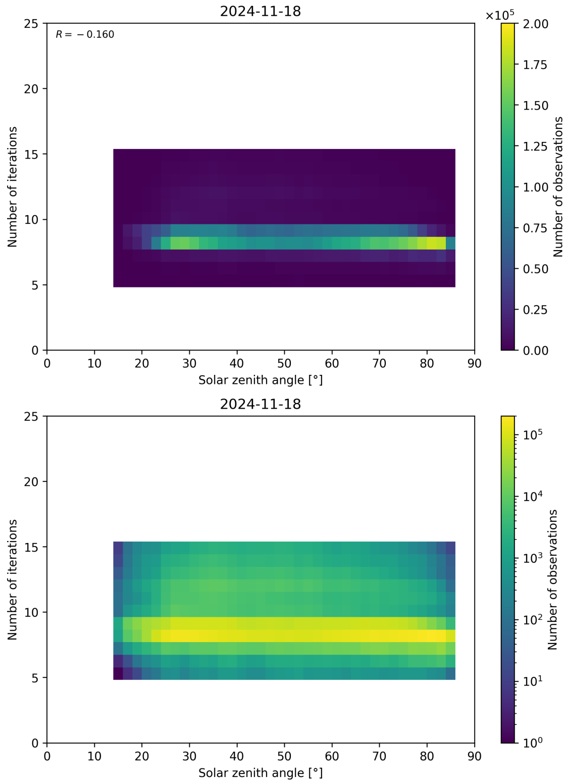
Figure 67: Scatter density plot of “Solar zenith angle” against “Number of iterations” for 2024-11-17 to 2024-11-19.
