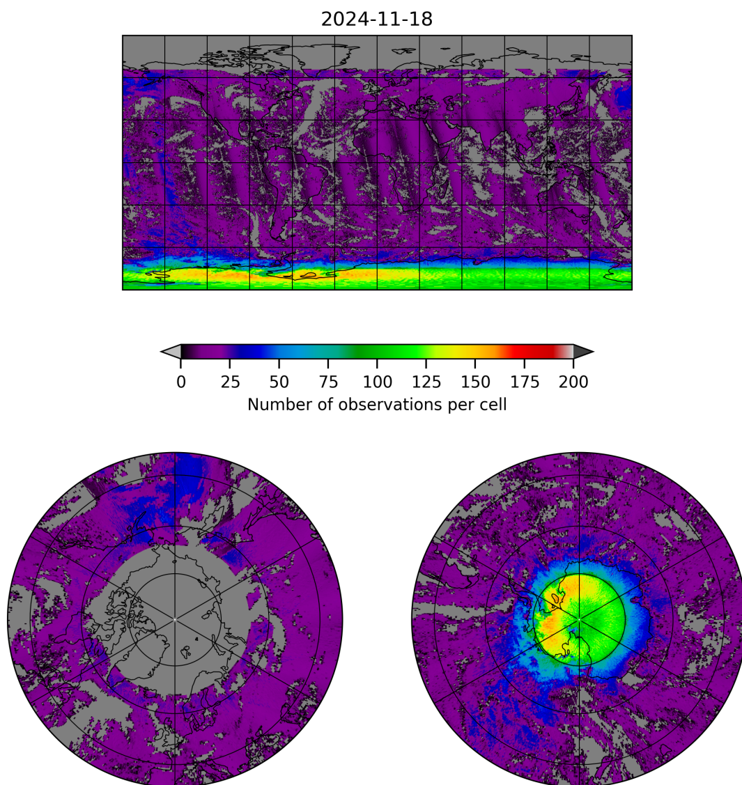
Figure 8: Map of the number of observations for 2024-11-17 to 2024-11-19
