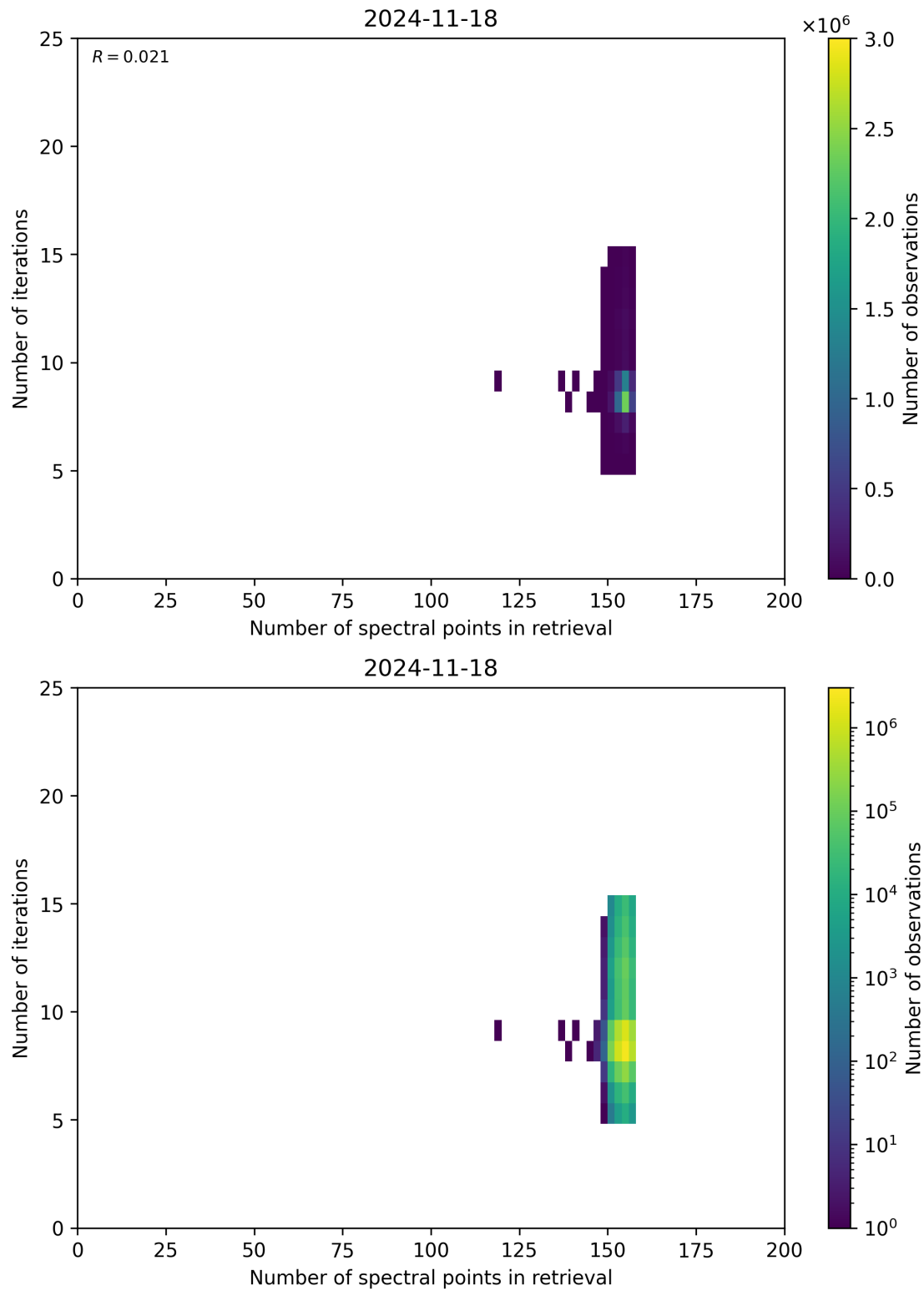
Figure 60: Scatter density plot of “Number of spectral points in retrieval” against “Number of iterations” for 2024-11-17 to 2024-11-19.
