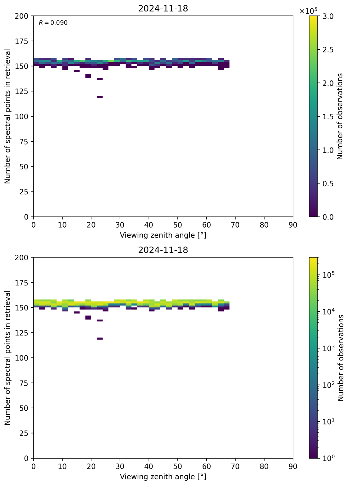
Figure 76: Scatter density plot of “Viewing zenith angle” against “Number of spectral points in retrieval” for 2024-11-17 to 2024-11-19.
