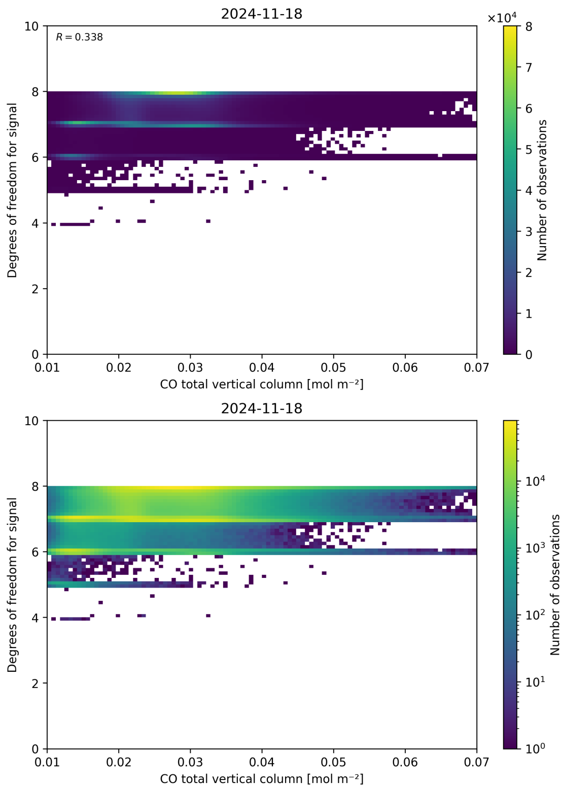
Figure 41: Scatter density plot of “CO total vertical column” against “Degrees of freedom for signal” for 2024-11-17 to 2024-11-19.
