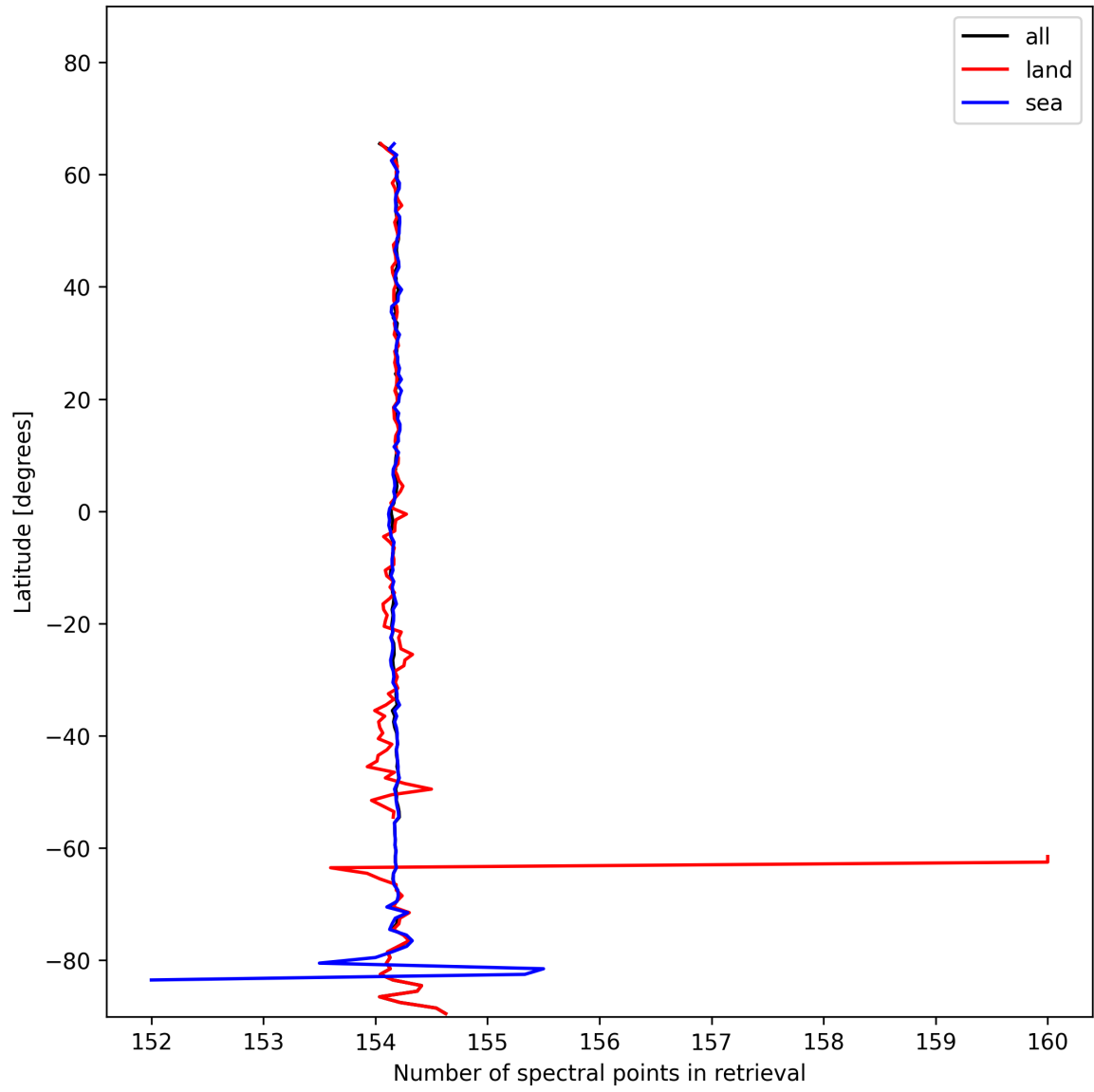
Figure 13: Zonal average of “Number of spectral points in retrieval” for 2024-11-17 to 2024-11-19.
