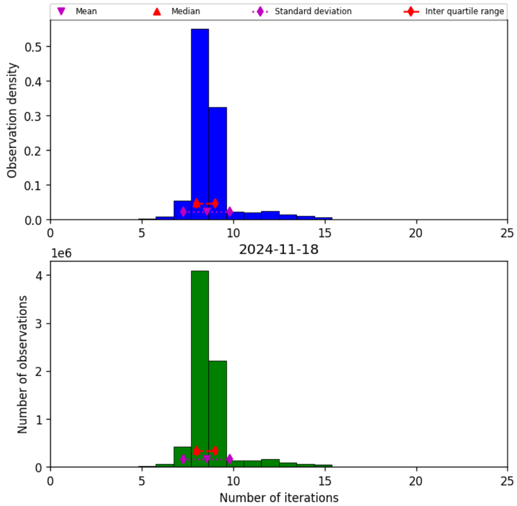
Figure 24: Histogram of “Number of iterations” for 2024-11-17 to 2024-11-19
