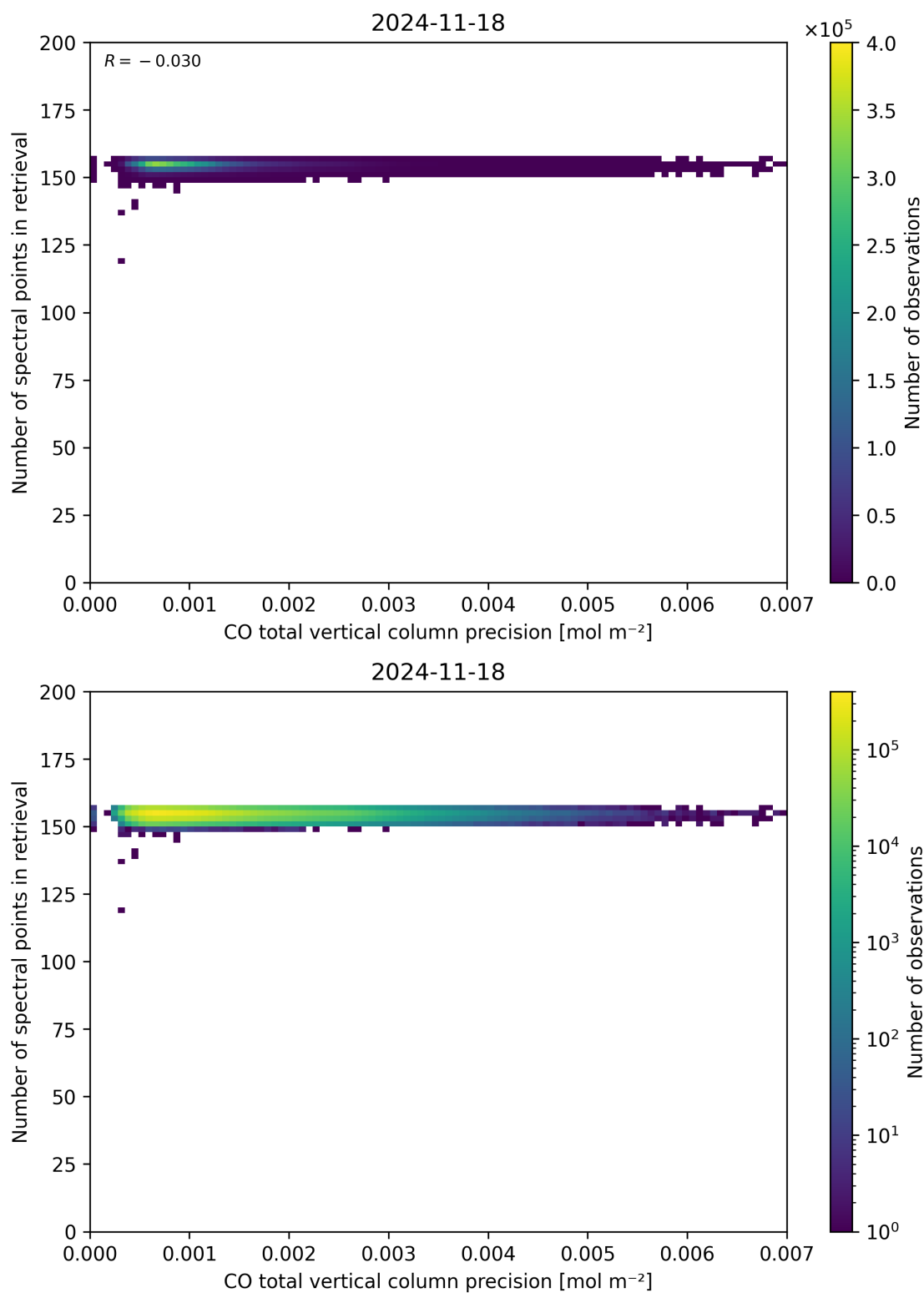
Figure 47: Scatter density plot of “CO total vertical column precision” against “Number of spectral points in retrieval” for 2024-11-17 to 2024-11-19.
