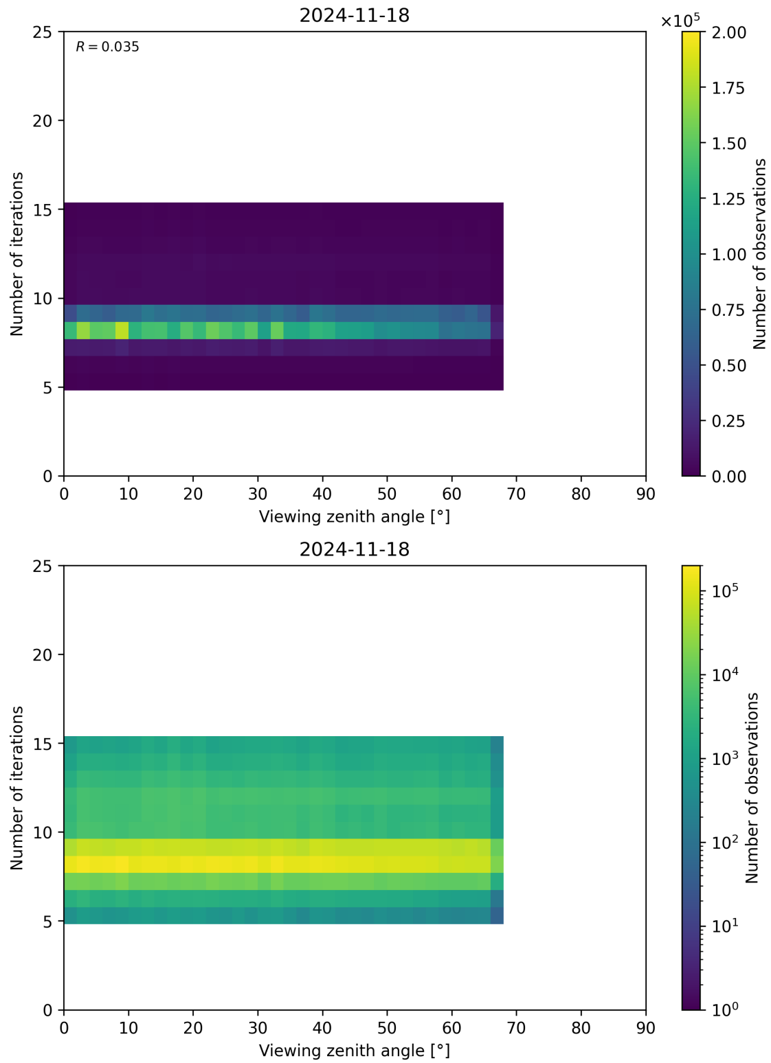
Figure 75: Scatter density plot of “Viewing zenith angle” against “Number of iterations” for 2024-11-17 to 2024-11-19.
