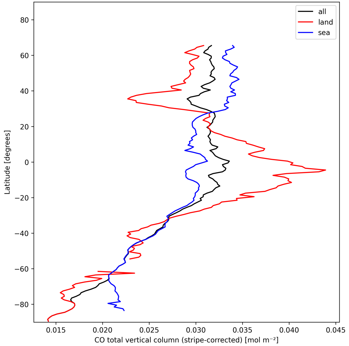
Figure 11: Zonal average of “CO total vertical column (stripe-corrected)” for 2024-11-17 to 2024-11-19.
