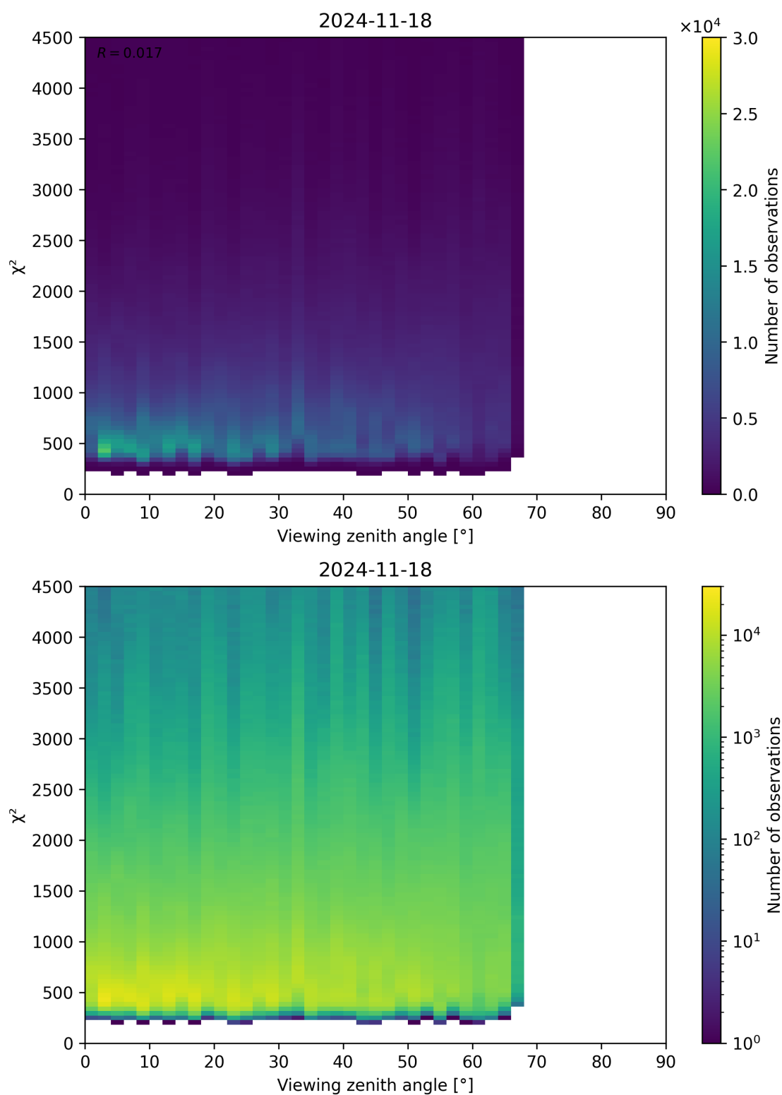
Figure 72: Scatter density plot of “Viewing zenith angle” against “ \chi^2 ” for 2024-11-17 to 2024-11-19.
