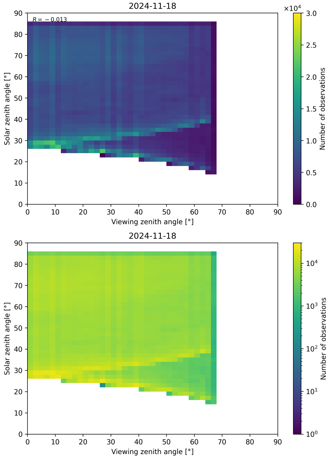
Figure 77: Scatter density plot of “Viewing zenith angle” against “Solar zenith angle” for 2024-11-17 to 2024-11-19.
