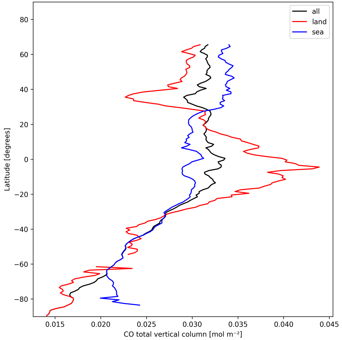
Figure 10: Zonal average of “CO total vertical column” for 2024-11-17 to 2024-11-19.
