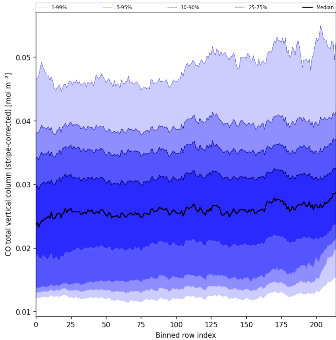
Figure 27: Along track statistics of “CO total vertical column (stripe-corrected)” for 2024-11-17 to 2024-11-19
