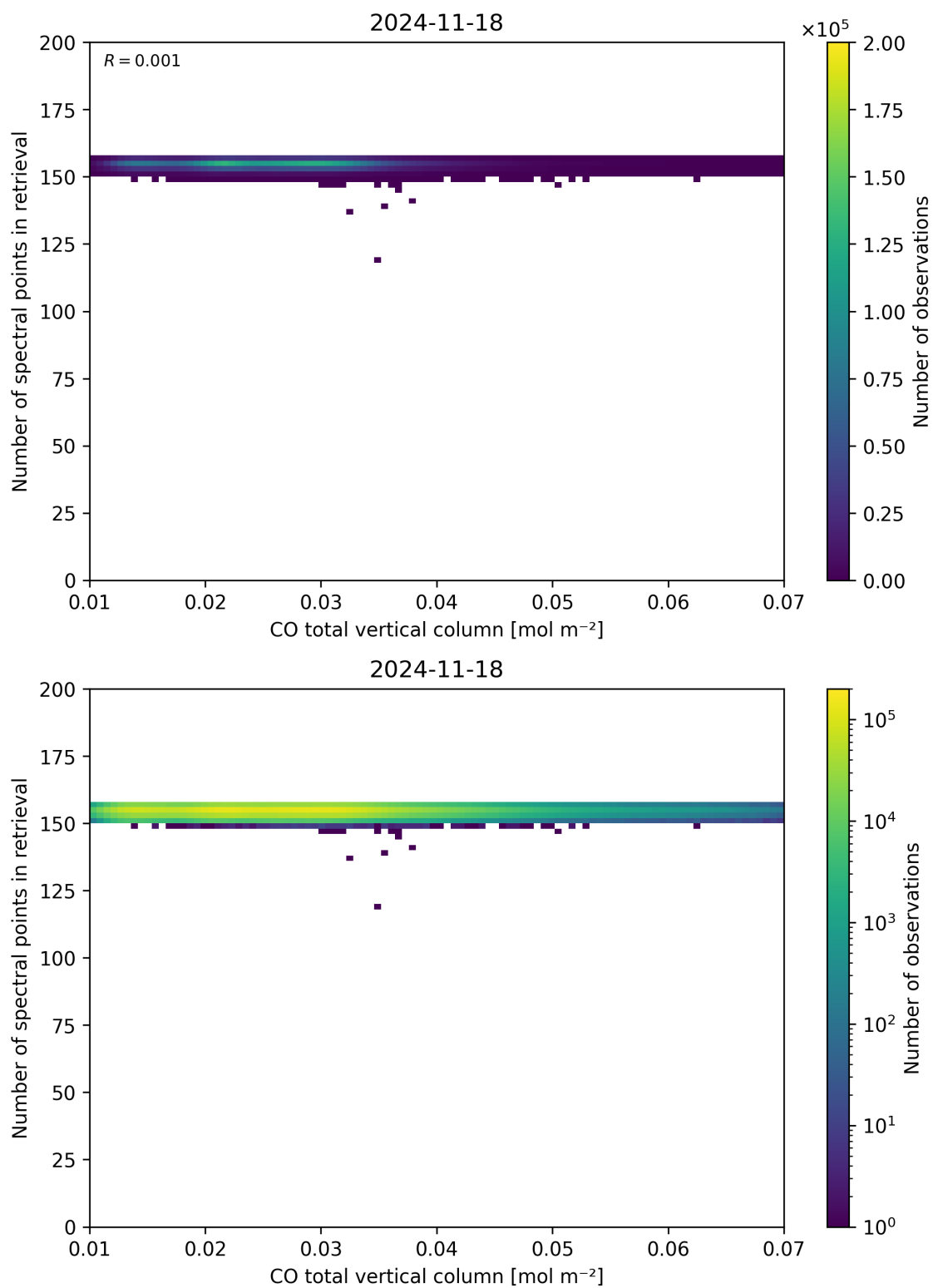
Figure 43: Scatter density plot of “CO total vertical column” against “Number of spectral points in retrieval” for 2024-11-17 to 2024-11-19.
