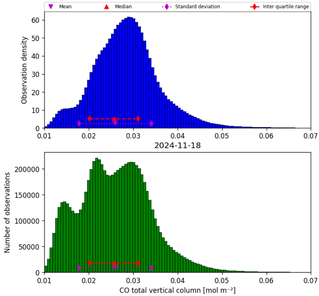
Figure 18: Histogram of “CO total vertical column” for 2024-11-17 to 2024-11-19
