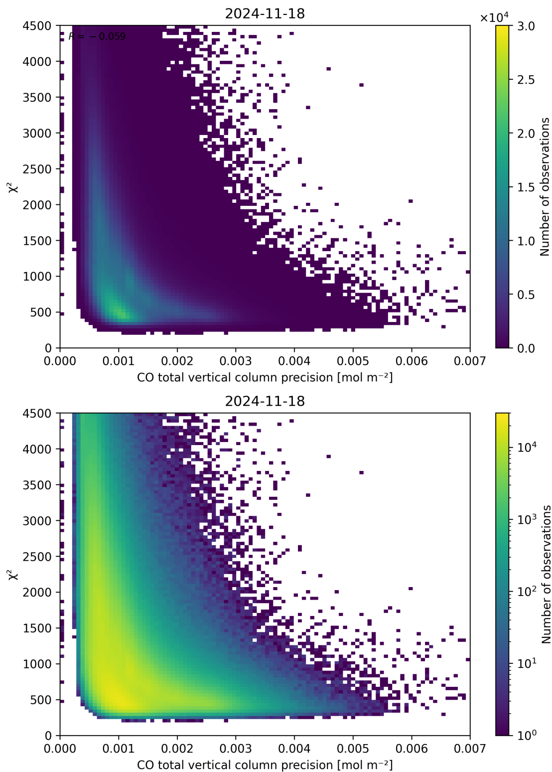
Figure 44: Scatter density plot of “CO total vertical column precision” against “ \chi^2 ” for 2024-11-17 to 2024-11-19.
