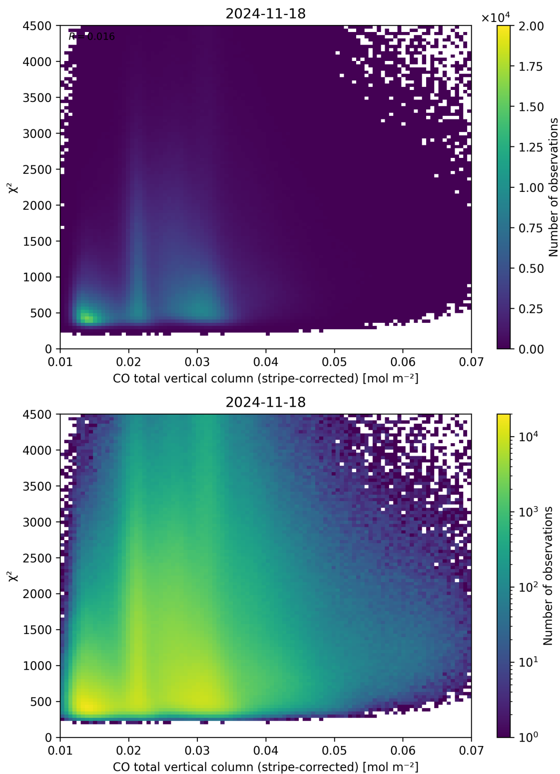
Figure 37: Scatter density plot of “CO total vertical column (stripe-corrected)” against “ \chi^2 ” for 2024-11-17 to 2024-11-19.
