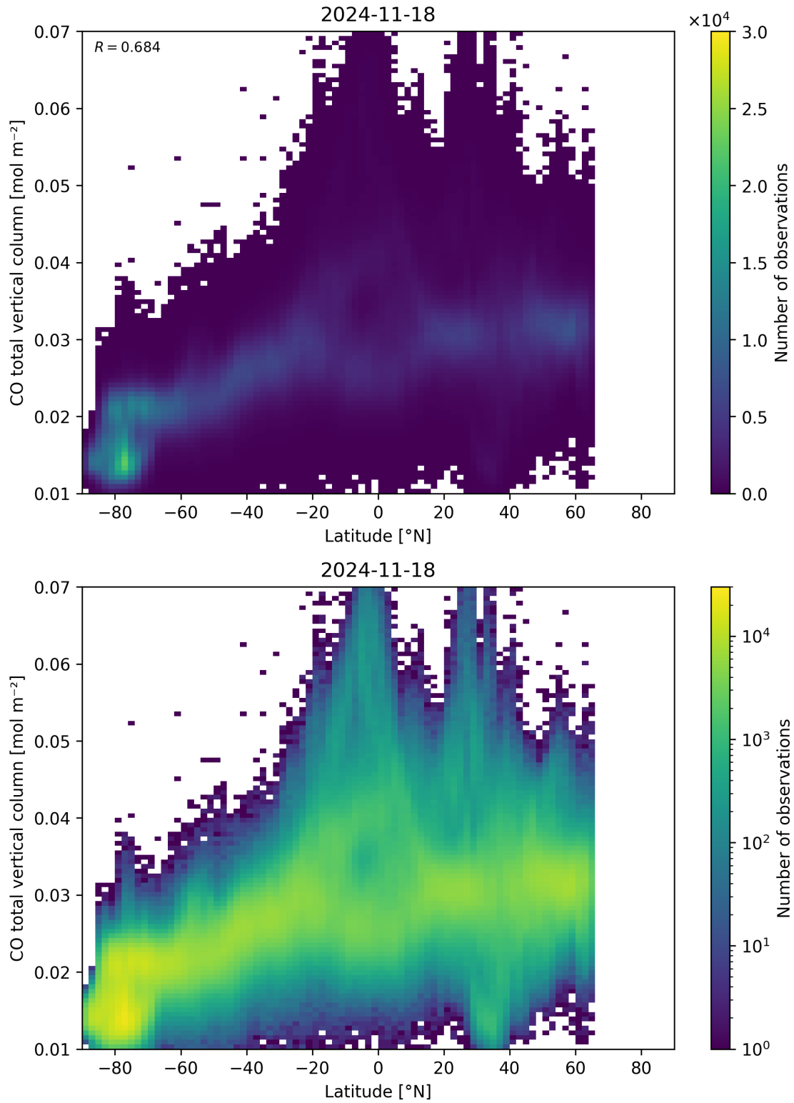
Figure 51: Scatter density plot of “Latitude” against “CO total vertical column” for 2024-11-17 to 2024-11-19.
