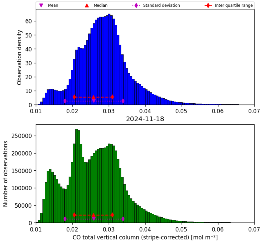
Figure 19: Histogram of “CO total vertical column (stripe-corrected)” for 2024-11-17 to 2024-11-19
