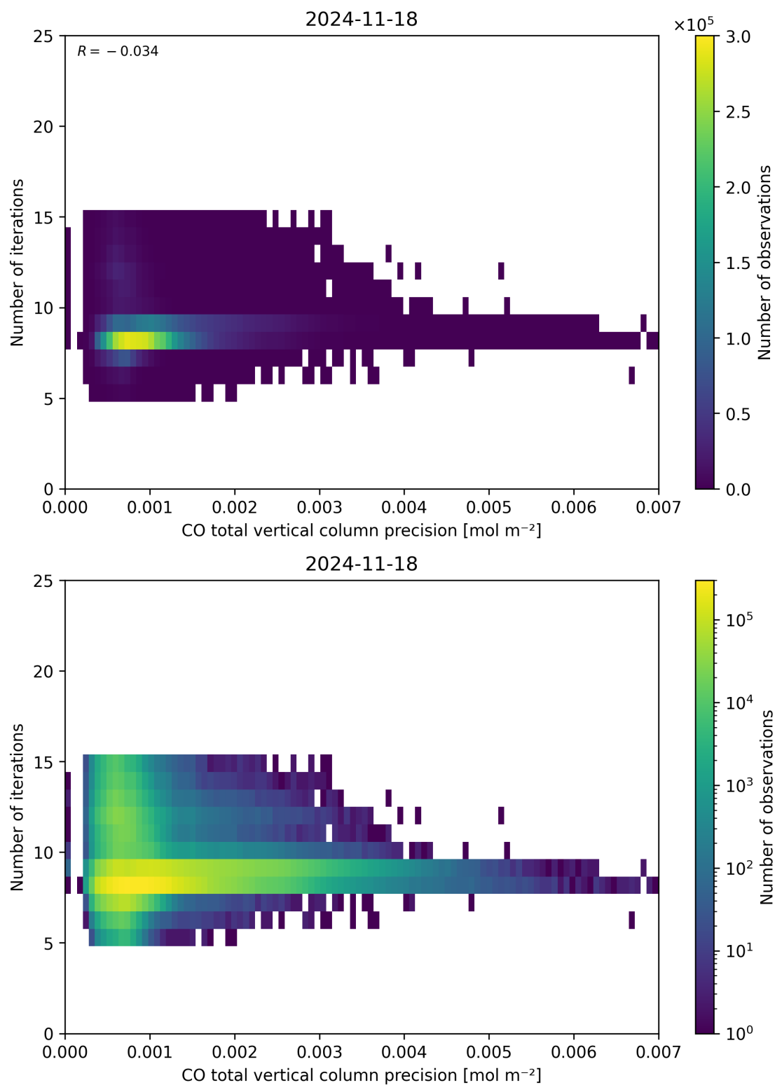
Figure 46: Scatter density plot of “CO total vertical column precision” against “Number of iterations” for 2024-11-17 to 2024-11-19.
