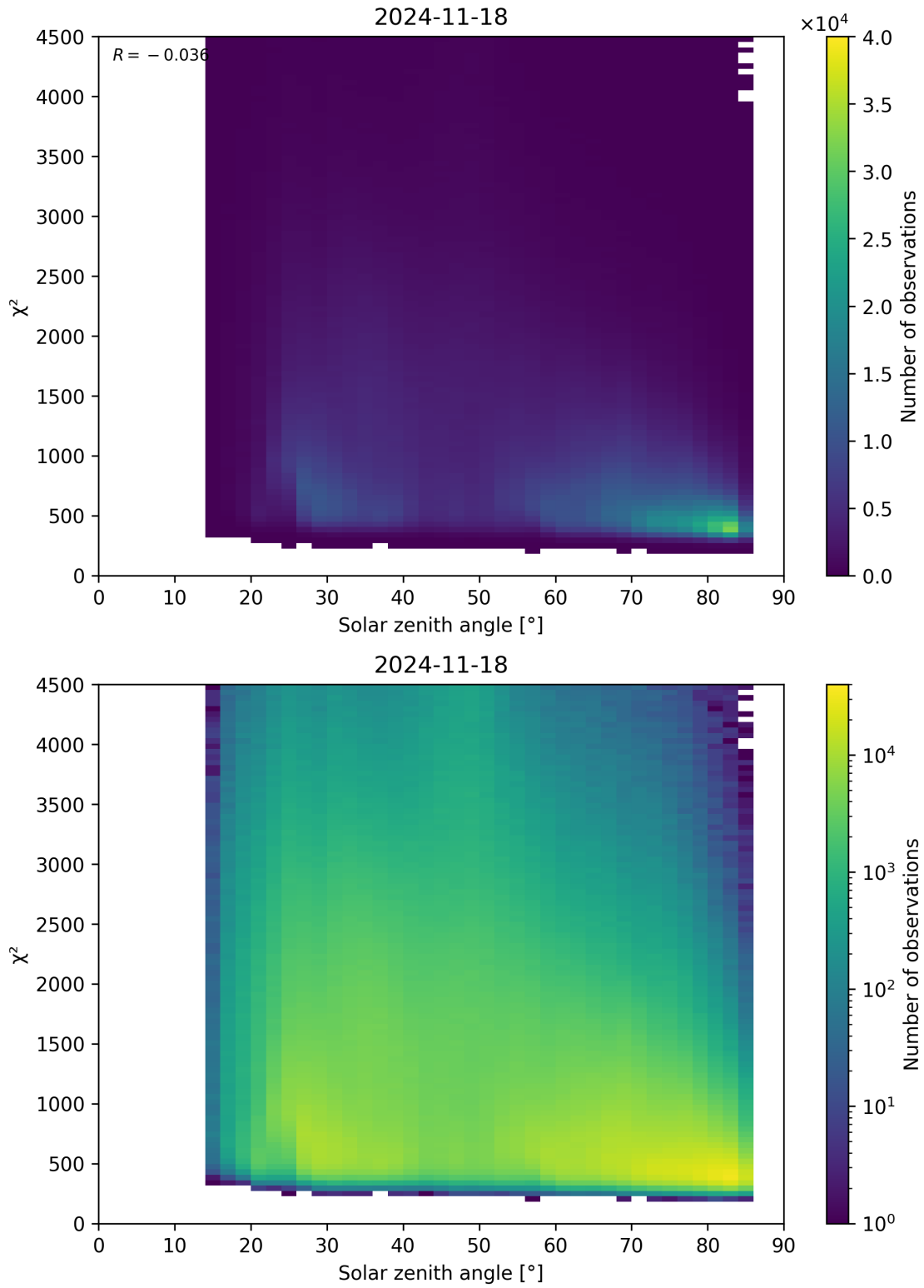
Figure 64: Scatter density plot of “Solar zenith angle” against “ \chi^2 ” for 2024-11-17 to 2024-11-19.
