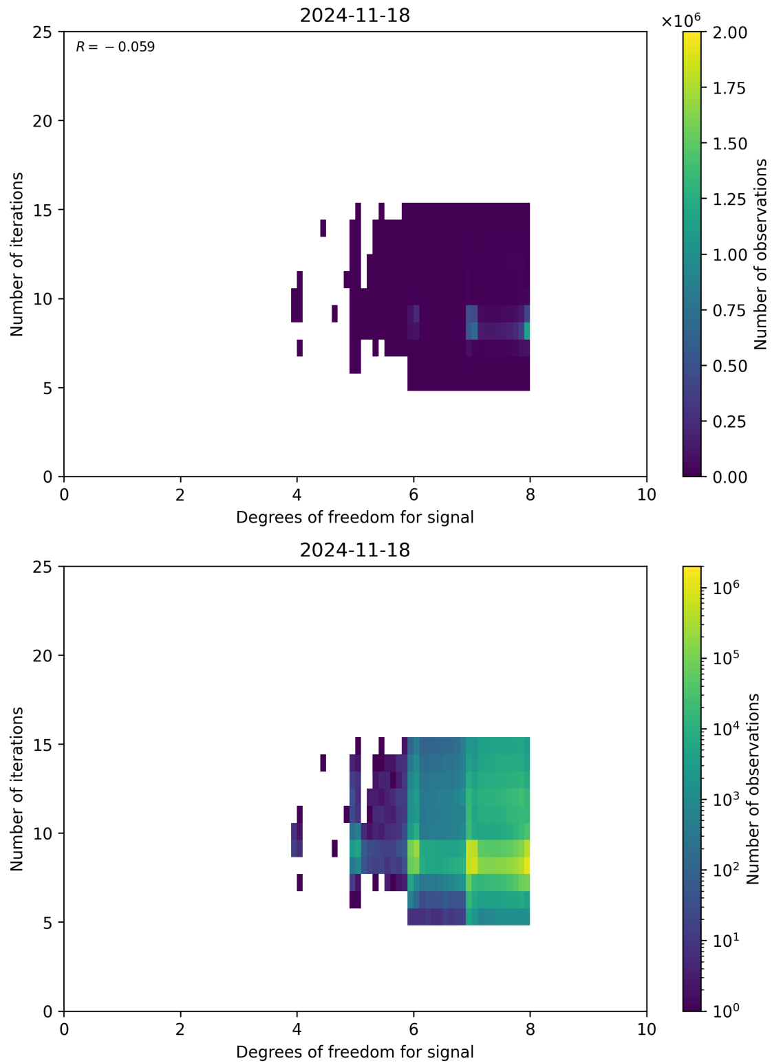
Figure 50: Scatter density plot of “Degrees of freedom for signal” against “Number of iterations” for 2024-11-17 to 2024-11-19.
