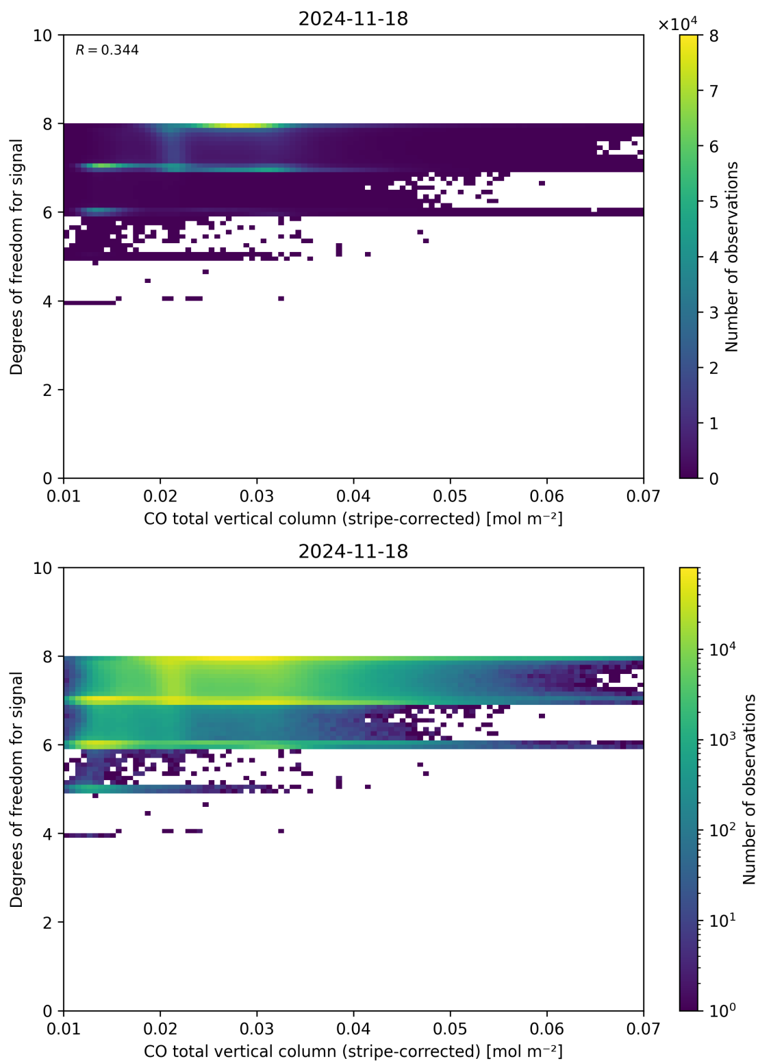
Figure 38: Scatter density plot of “CO total vertical column (stripe-corrected)” against “Degrees of freedom for signal” for 2024-11-17 to 2024-11-19.
