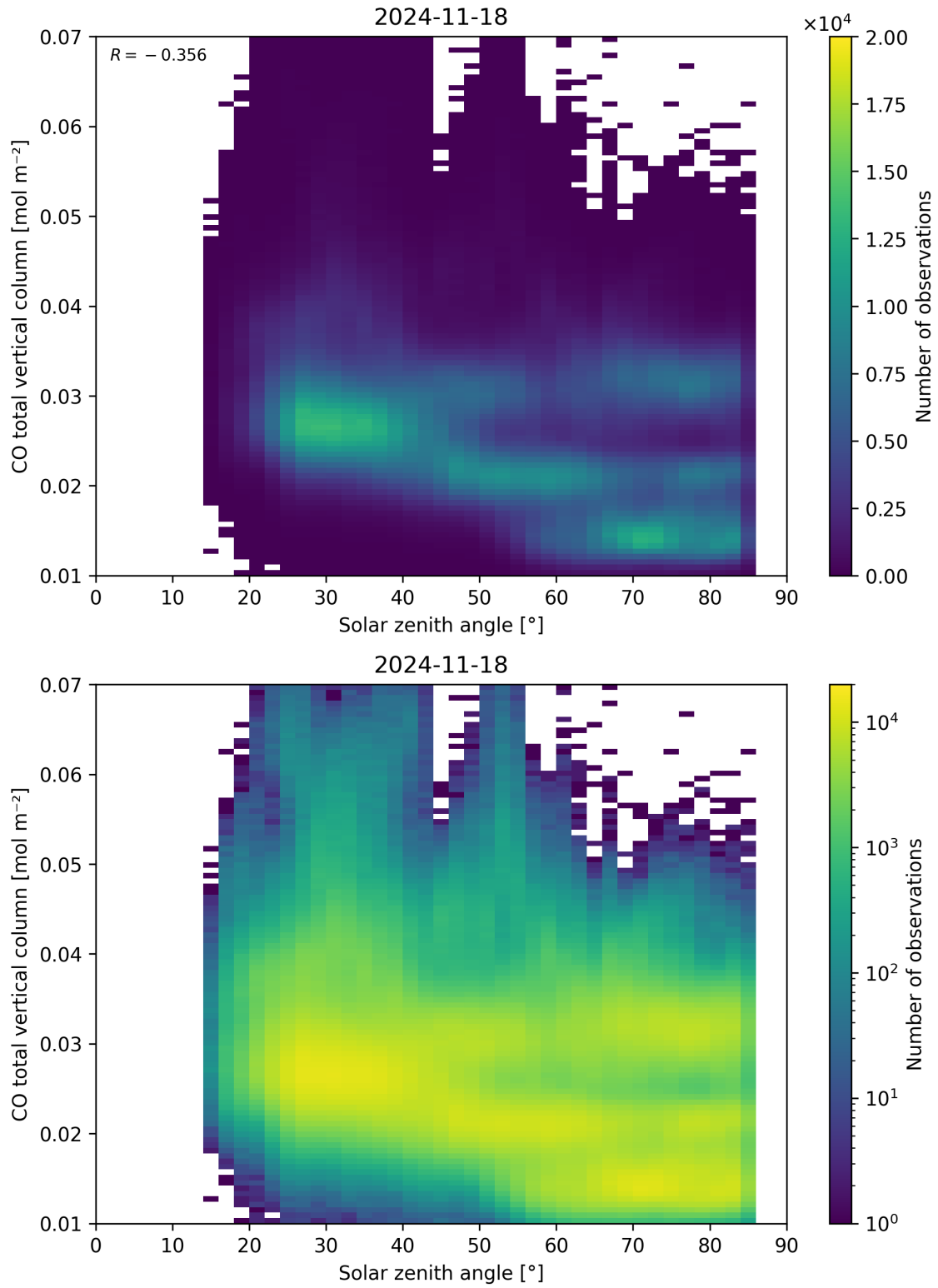
Figure 61: Scatter density plot of “Solar zenith angle” against “CO total vertical column” for 2024-11-17 to 2024-11-19.
