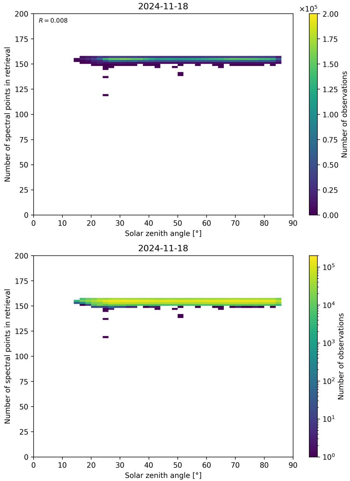
Figure 68: Scatter density plot of “Solar zenith angle” against “Number of spectral points in retrieval” for 2024-11-17 to 2024-11-19.
