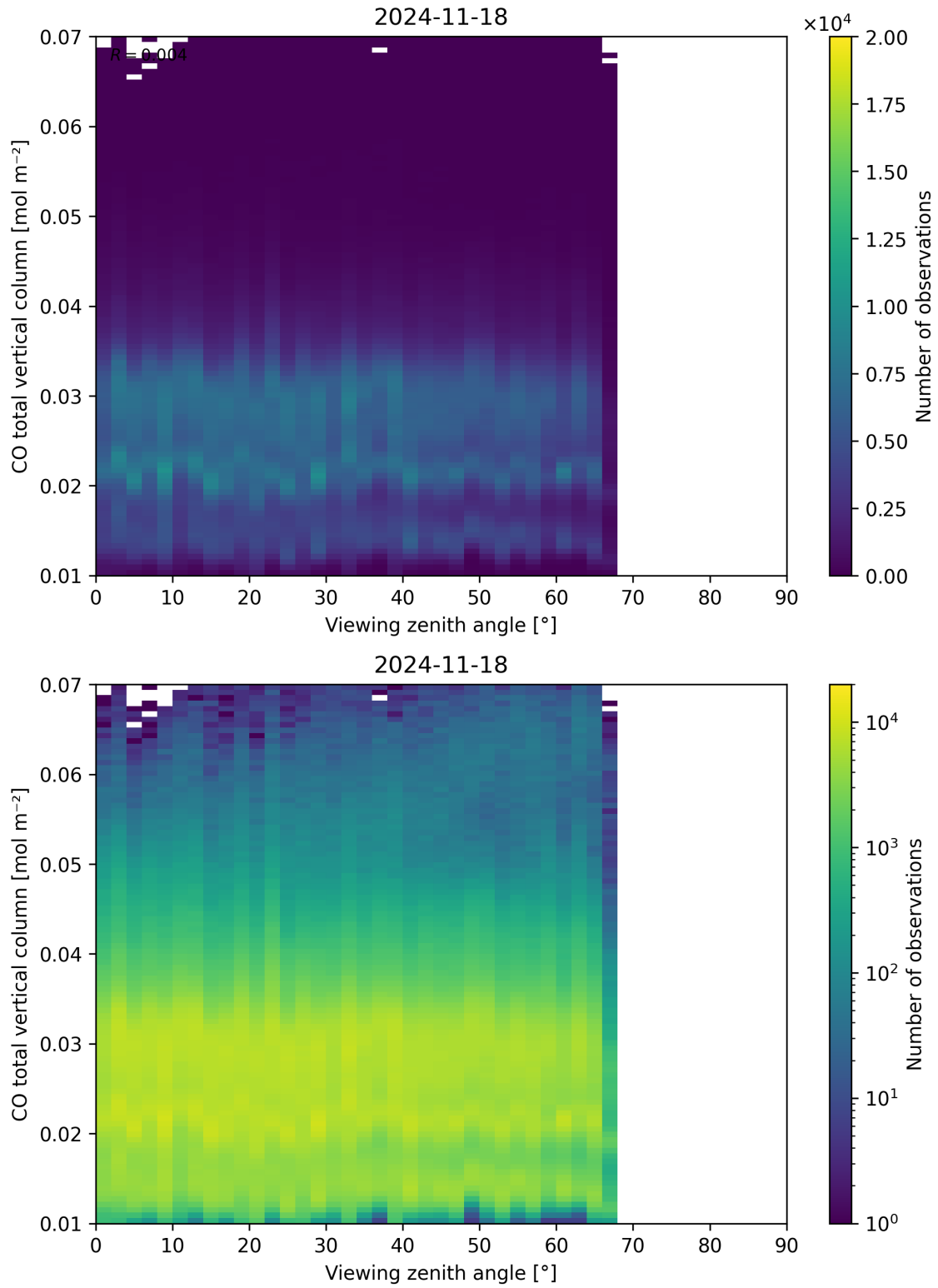
Figure 69: Scatter density plot of “Viewing zenith angle” against “CO total vertical column” for 2024-11-17 to 2024-11-19.
