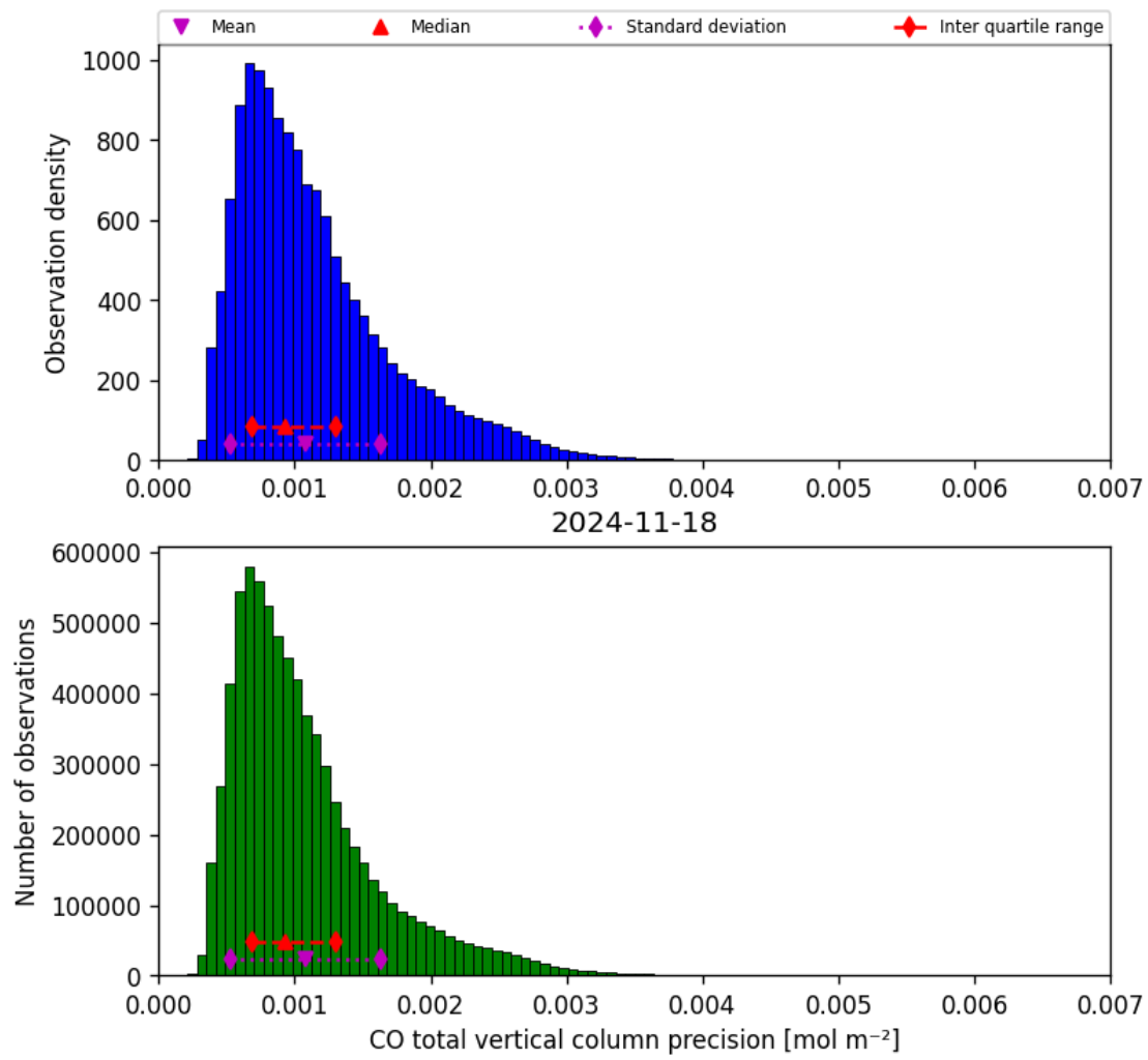
Figure 20: Histogram of “CO total vertical column precision” for 2024-11-17 to 2024-11-19
