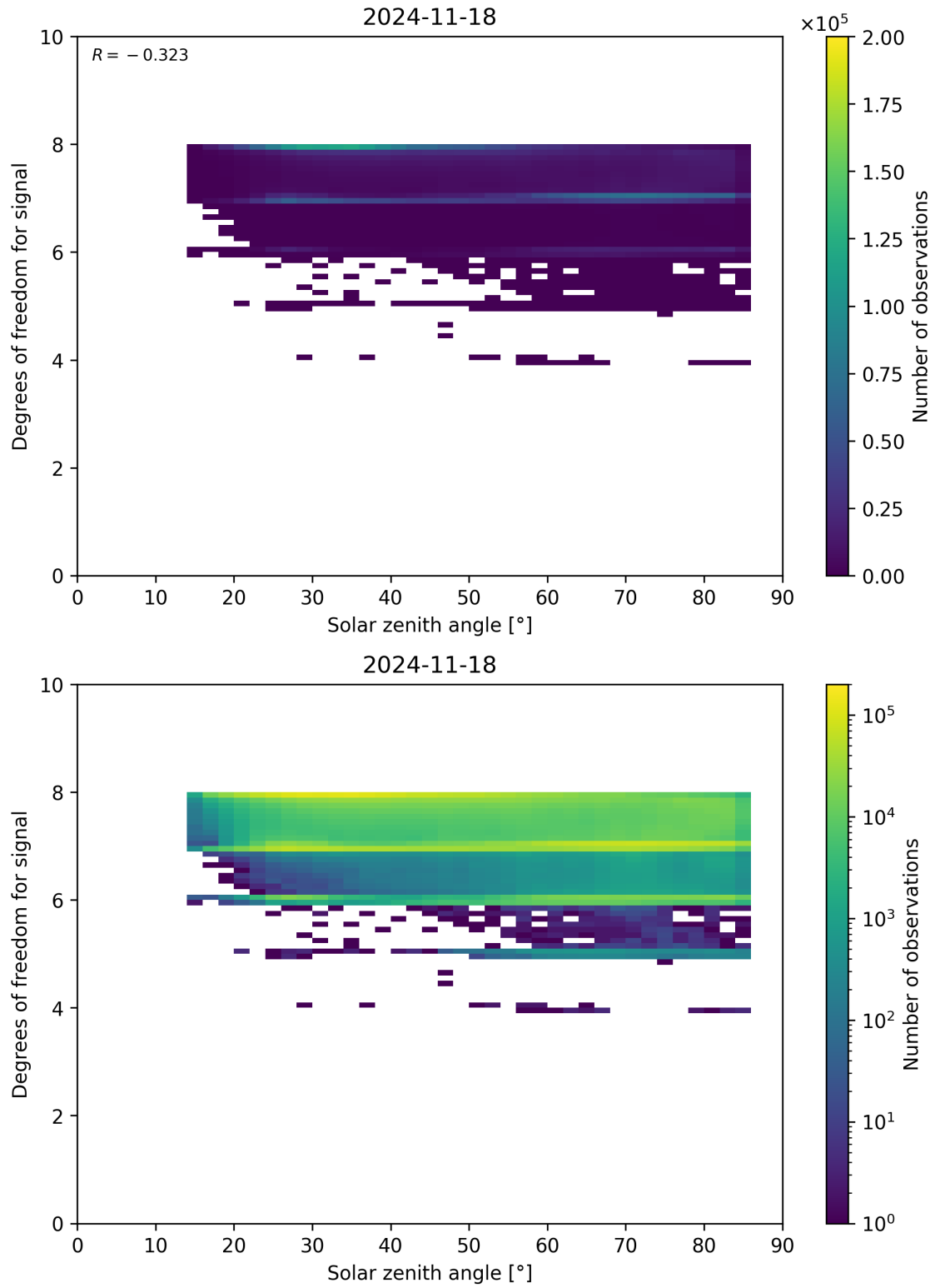
Figure 65: Scatter density plot of “Solar zenith angle” against “Degrees of freedom for signal” for 2024-11-17 to 2024-11-19.
