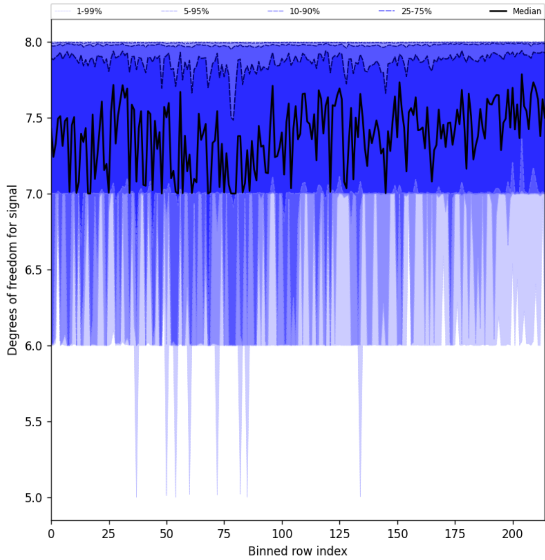
Figure 31: Along track statistics of “Degrees of freedom for signal” for 2024-11-17 to 2024-11-19
