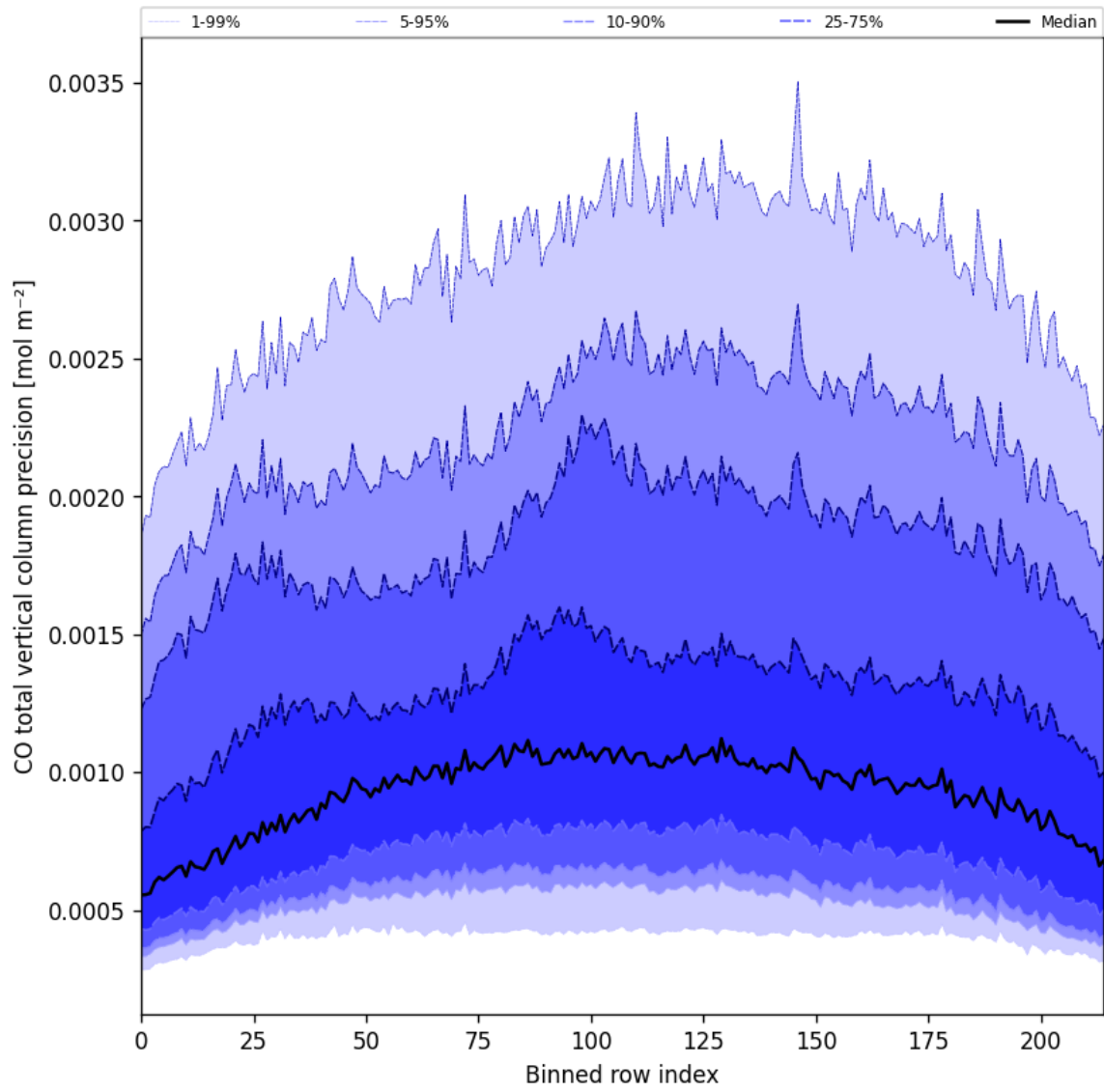
Figure 28: Along track statistics of “CO total vertical column precision” for 2024-11-17 to 2024-11-19
