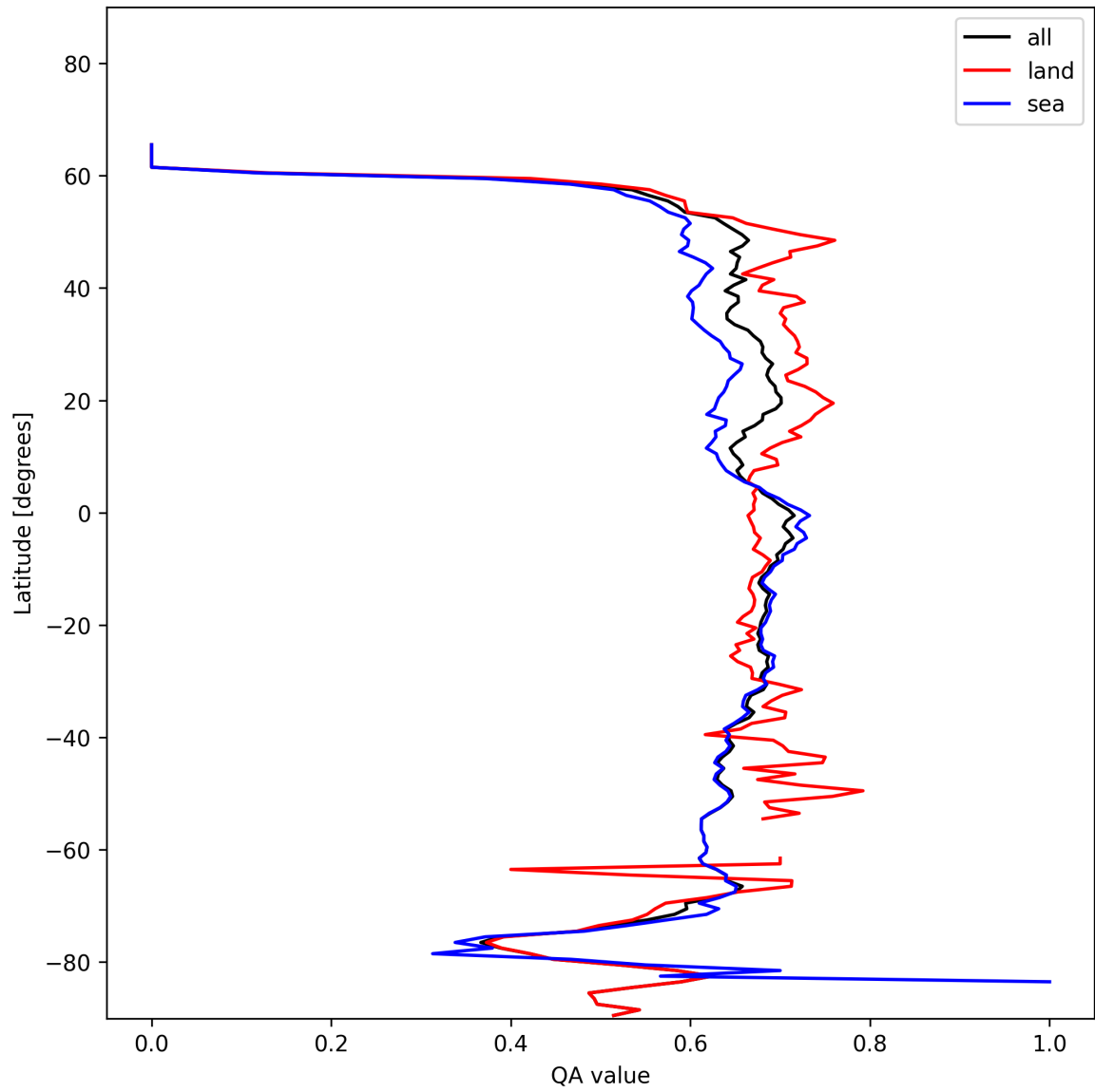
Figure 9: Zonal average of “QA value” for 2024-11-17 to 2024-11-19.
