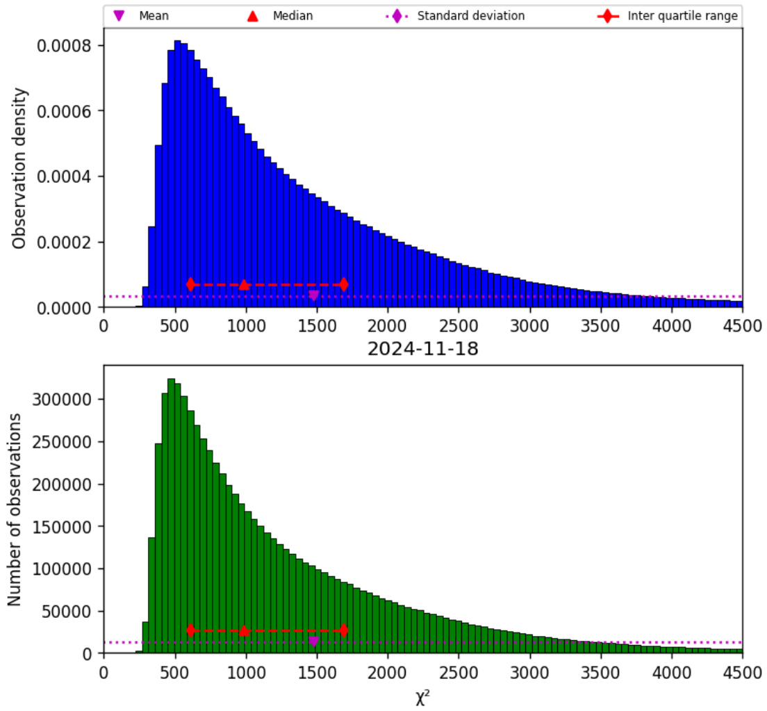
Figure 22: Histogram of “ \chi^2 ” for 2024-11-17 to 2024-11-19
