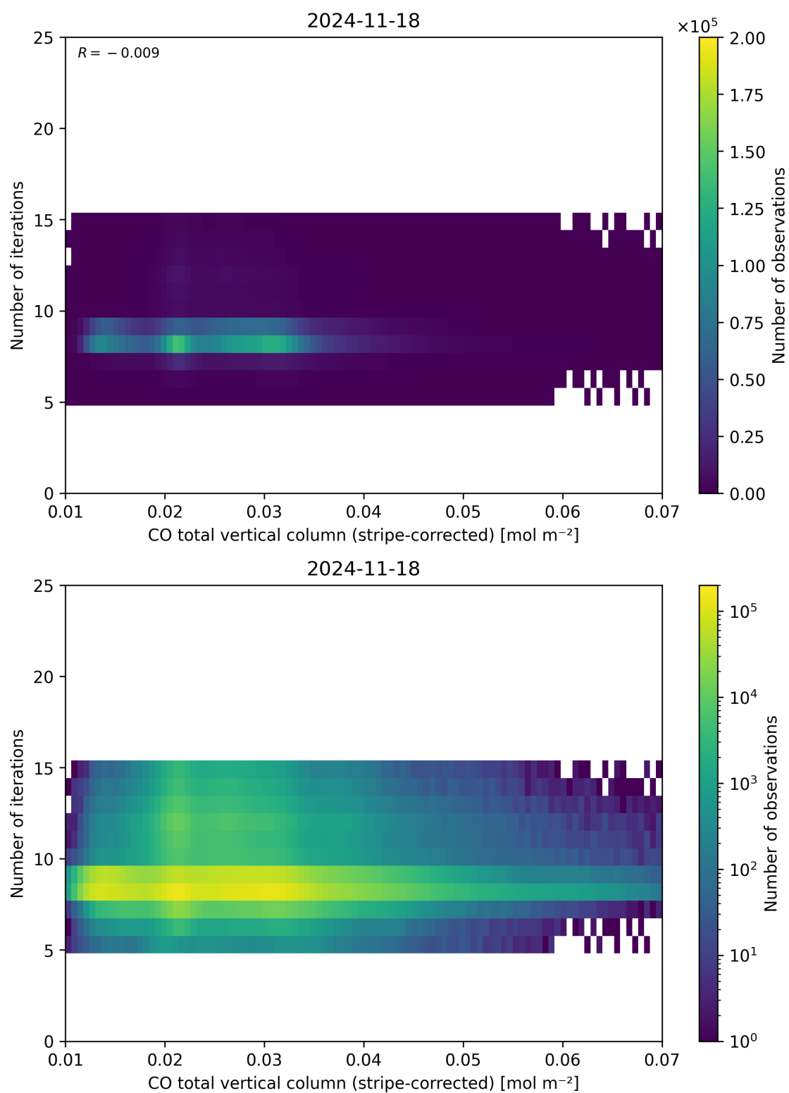
Figure 39: Scatter density plot of “CO total vertical column (stripe-corrected)” against “Number of iterations” for 2024-11-17 to 2024-11-19.
