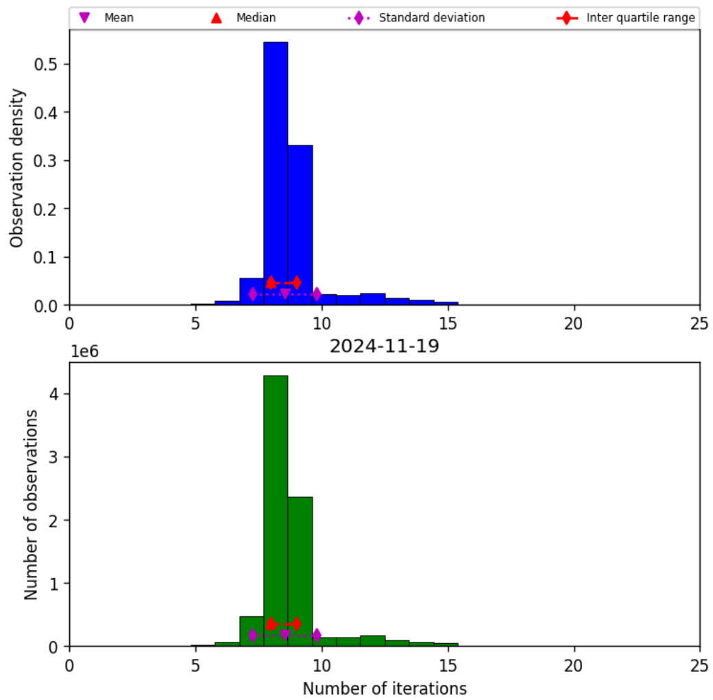
Figure 24: Histogram of “Number of iterations” for 2024-11-18 to 2024-11-20
