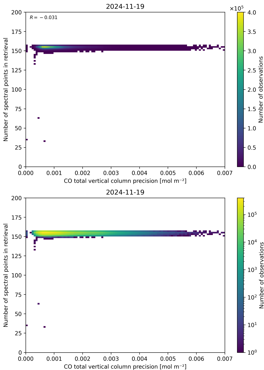
Figure 47: Scatter density plot of “CO total vertical column precision” against “Number of spectral points in retrieval” for 2024-11-18 to 2024-11-20.
