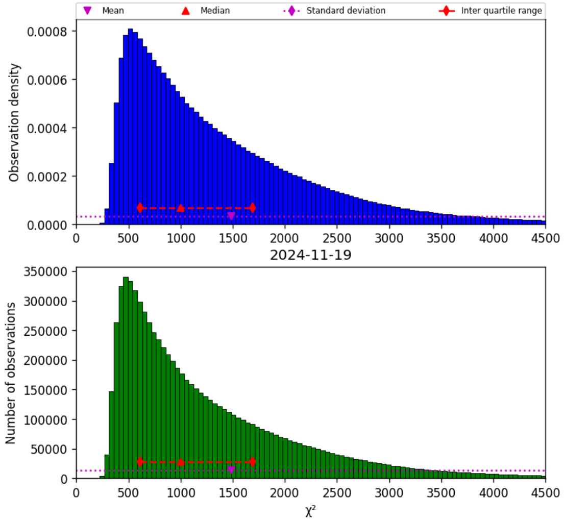
Figure 22: Histogram of “ \chi^2 ” for 2024-11-18 to 2024-11-20
