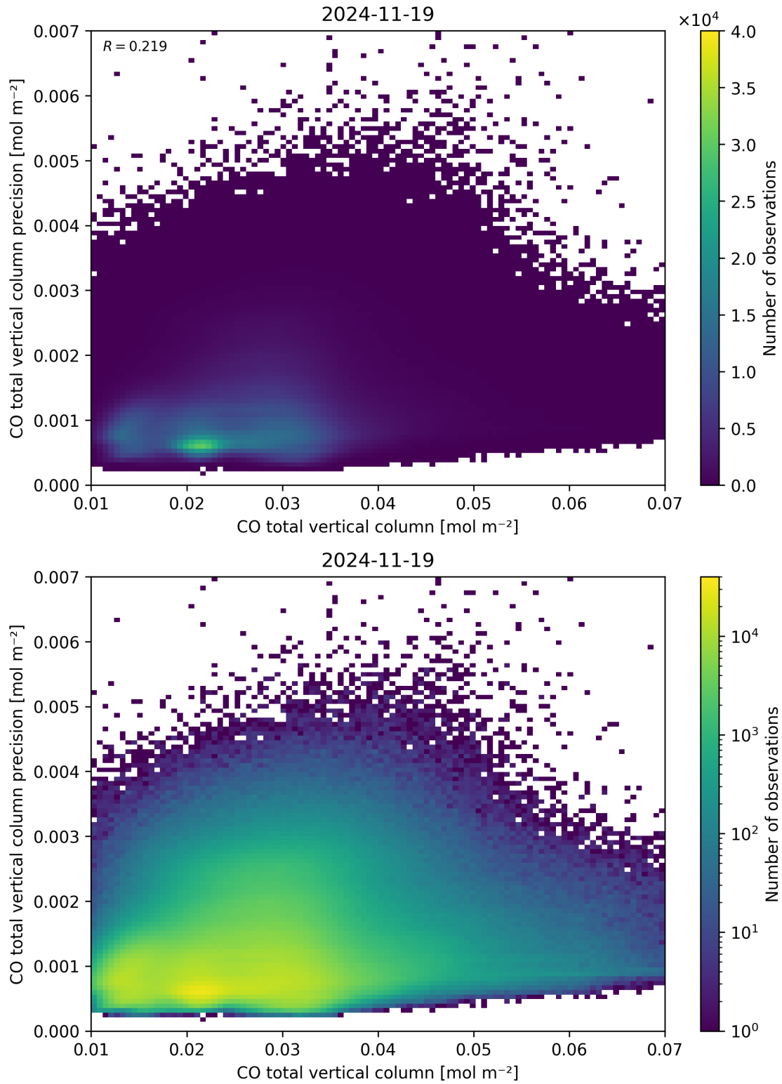
Figure 34: Scatter density plot of “CO total vertical column” against “CO total vertical column precision” for 2024-11-18 to 2024-11-20.
