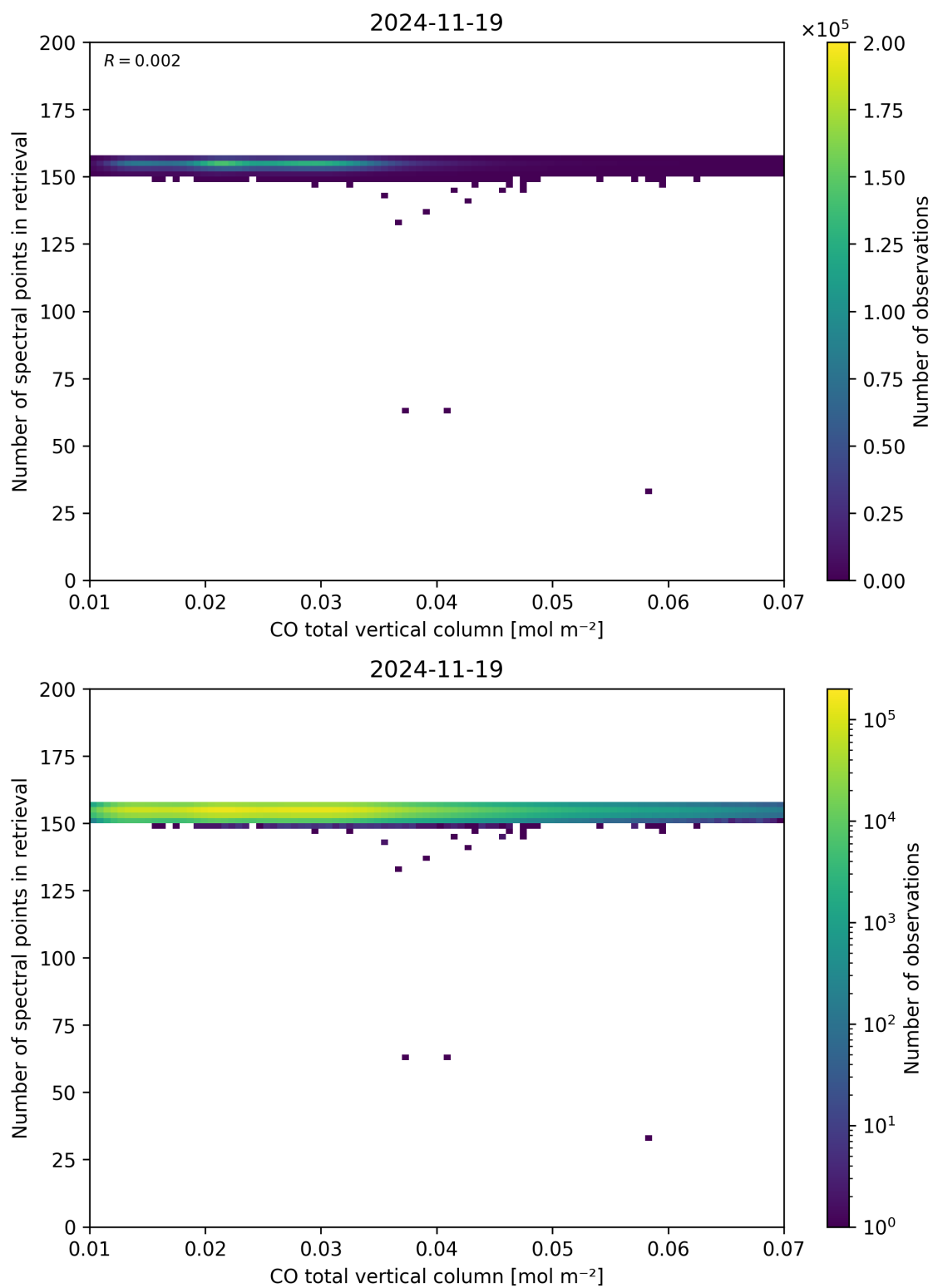
Figure 43: Scatter density plot of “CO total vertical column” against “Number of spectral points in retrieval” for 2024-11-18 to 2024-11-20.
