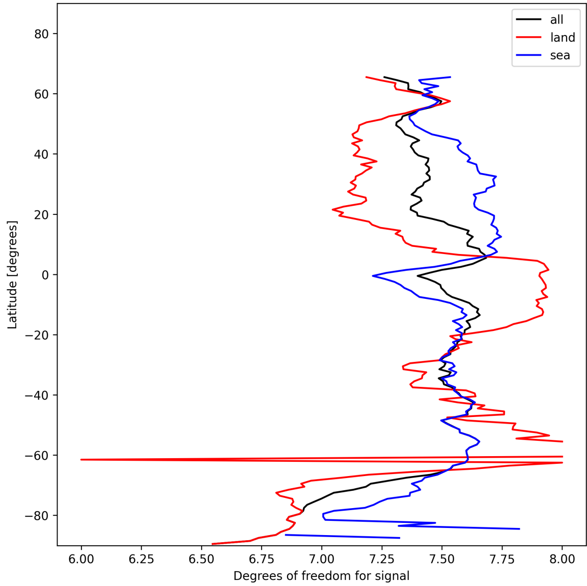
Figure 15: Zonal average of “Degrees of freedom for signal” for 2024-11-18 to 2024-11-20.
