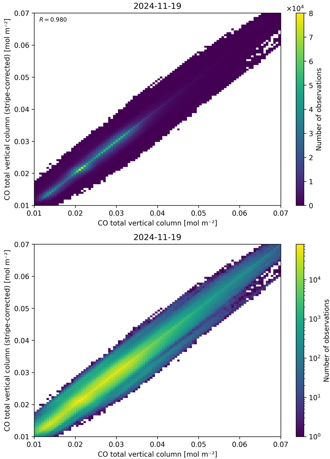
Figure 33: Scatter density plot of “CO total vertical column” against “CO total vertical column (stripe-corrected)” for 2024-11-18 to 2024-11-20.
