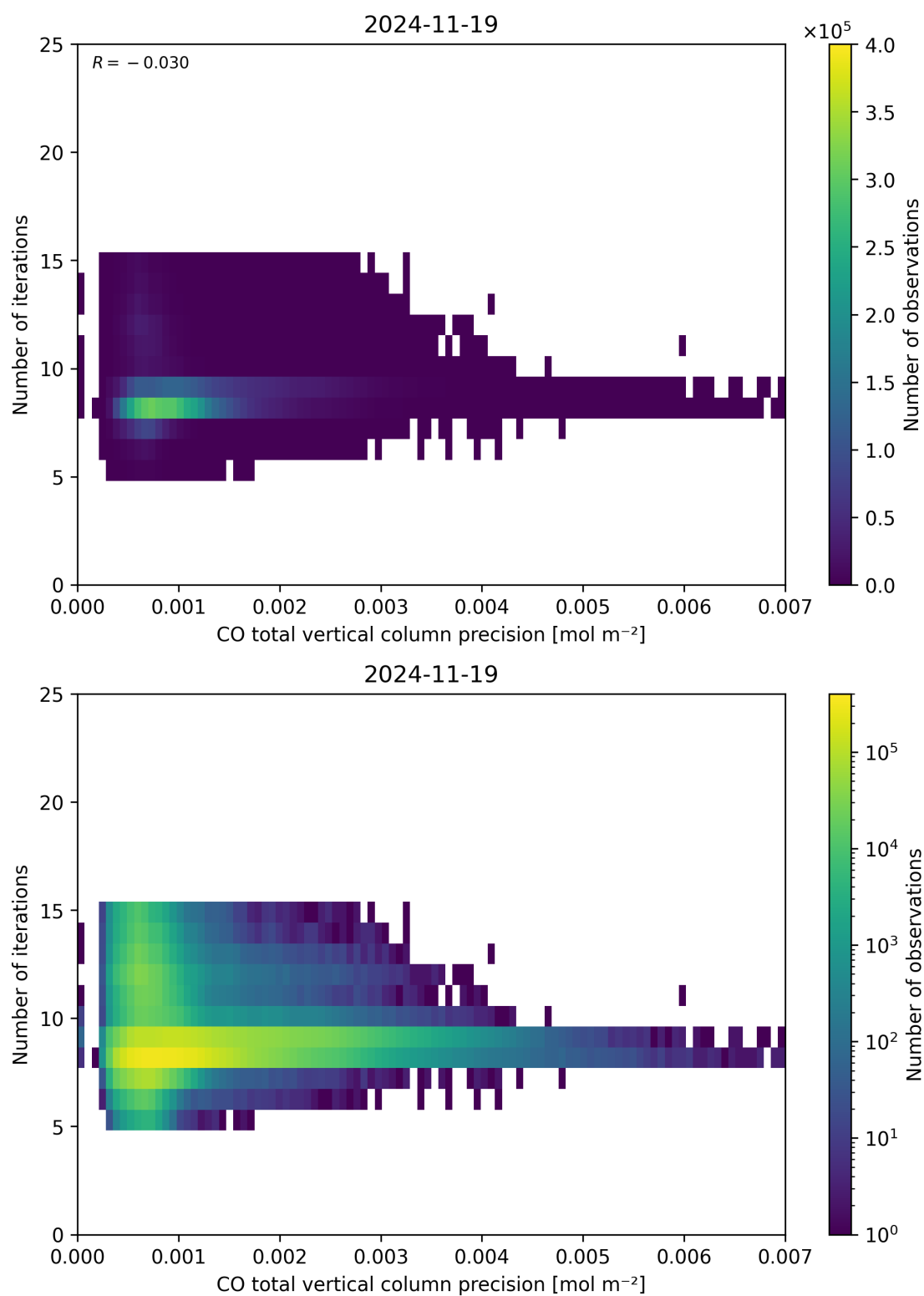
Figure 46: Scatter density plot of “CO total vertical column precision” against “Number of iterations” for 2024-11-18 to 2024-11-20.
