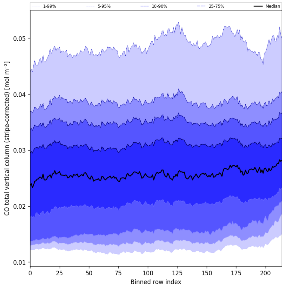
Figure 27: Along track statistics of “CO total vertical column (stripe-corrected)” for 2024-11-18 to 2024-11-20
