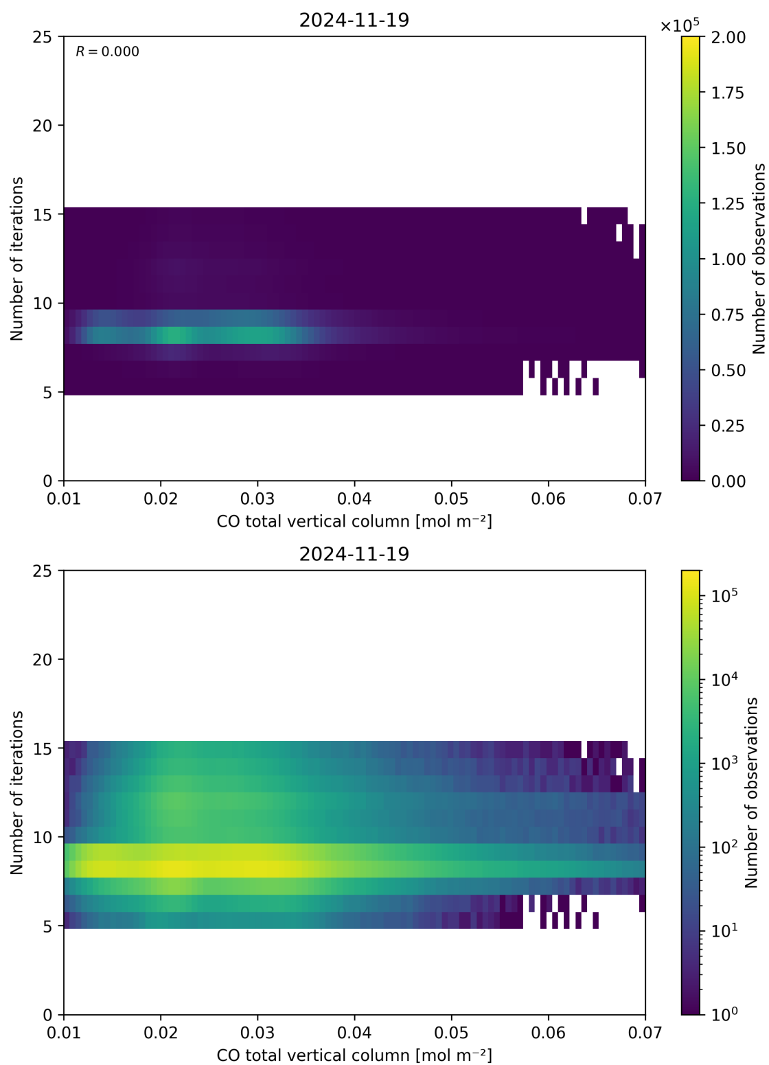
Figure 42: Scatter density plot of “CO total vertical column” against “Number of iterations” for 2024-11-18 to 2024-11-20.
