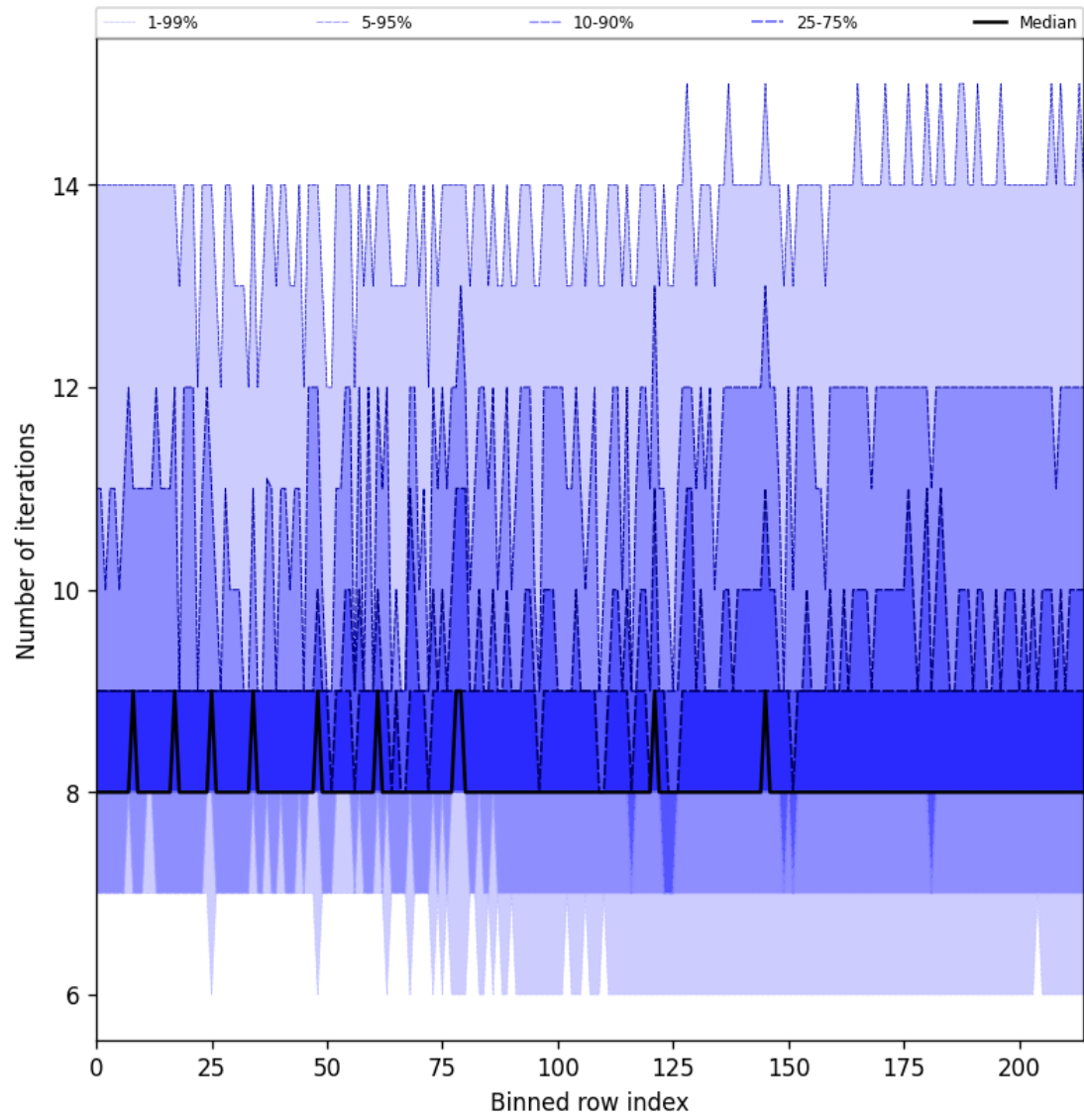
Figure 32: Along track statistics of “Number of iterations” for 2024-11-18 to 2024-11-20
