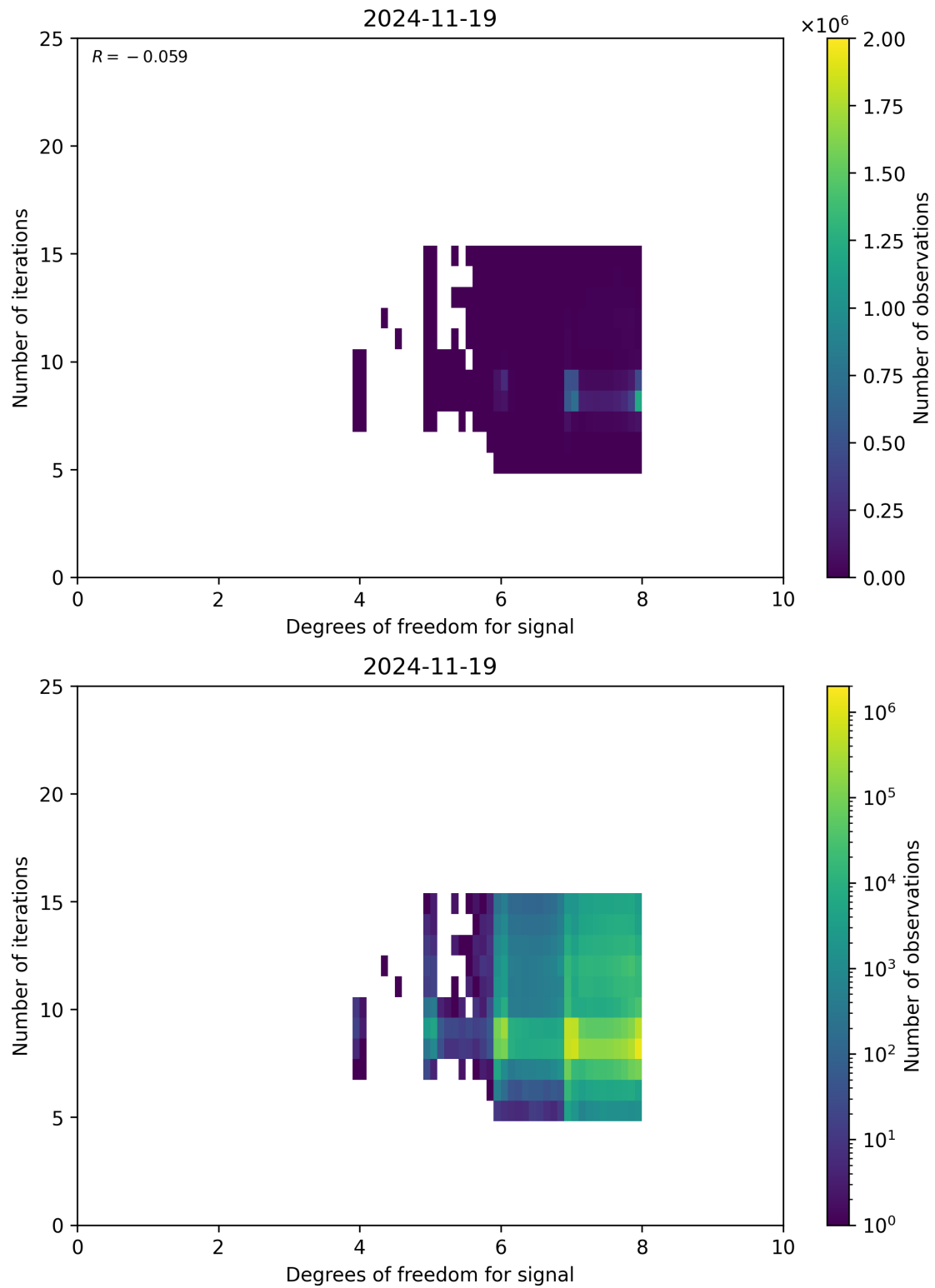
Figure 50: Scatter density plot of “Degrees of freedom for signal” against “Number of iterations” for 2024-11-18 to 2024-11-20.
