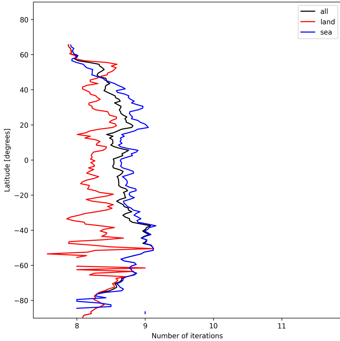
Figure 16: Zonal average of “Number of iterations” for 2024-11-18 to 2024-11-20.
