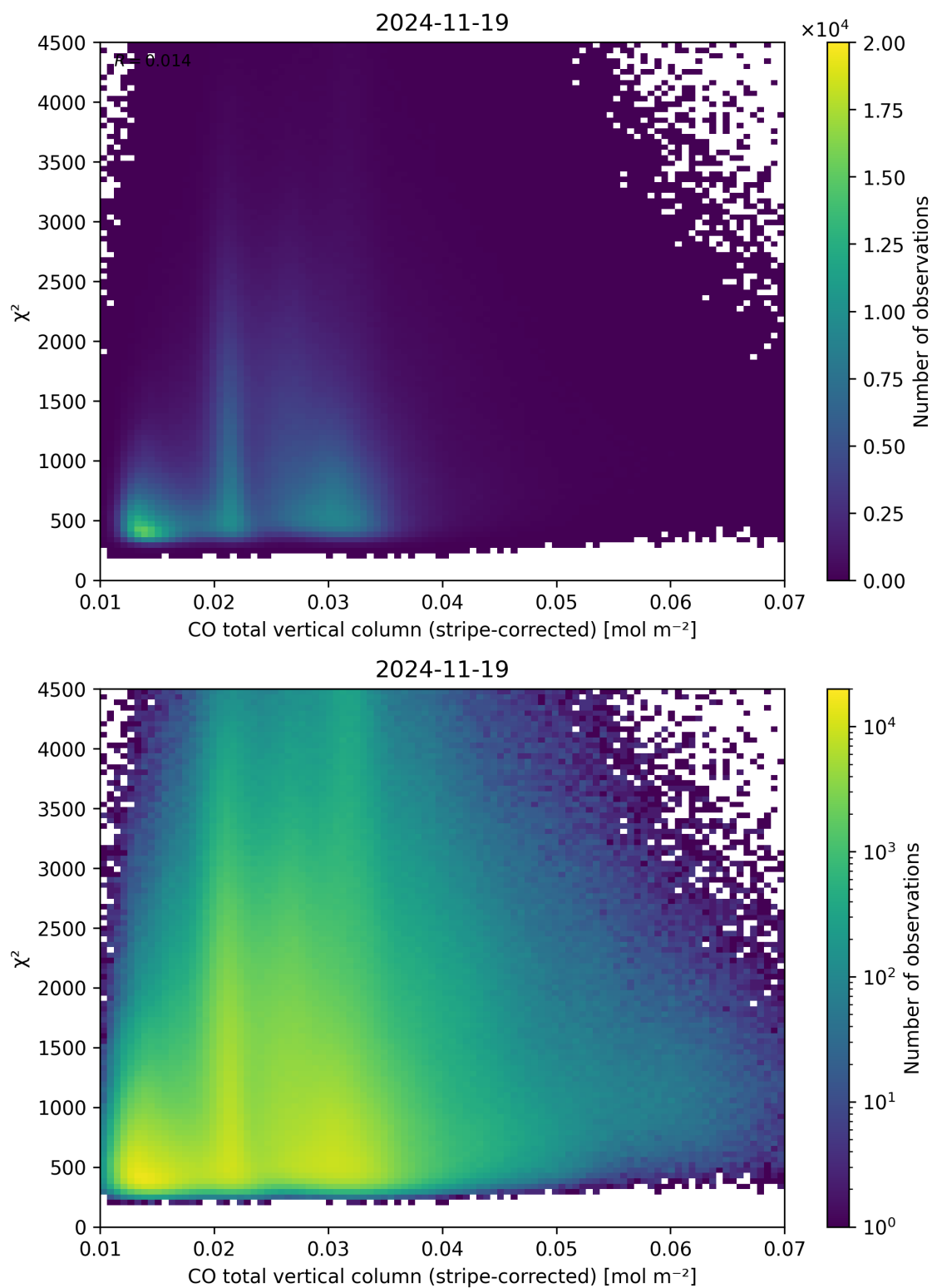
Figure 37: Scatter density plot of “CO total vertical column (stripe-corrected)” against “ \chi^2 ” for 2024-11-18 to 2024-11-20.
