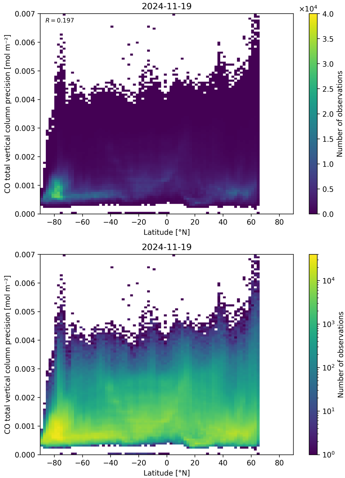
Figure 53: Scatter density plot of “Latitude” against “CO total vertical column precision” for 2024-11-18 to 2024-11-20.
