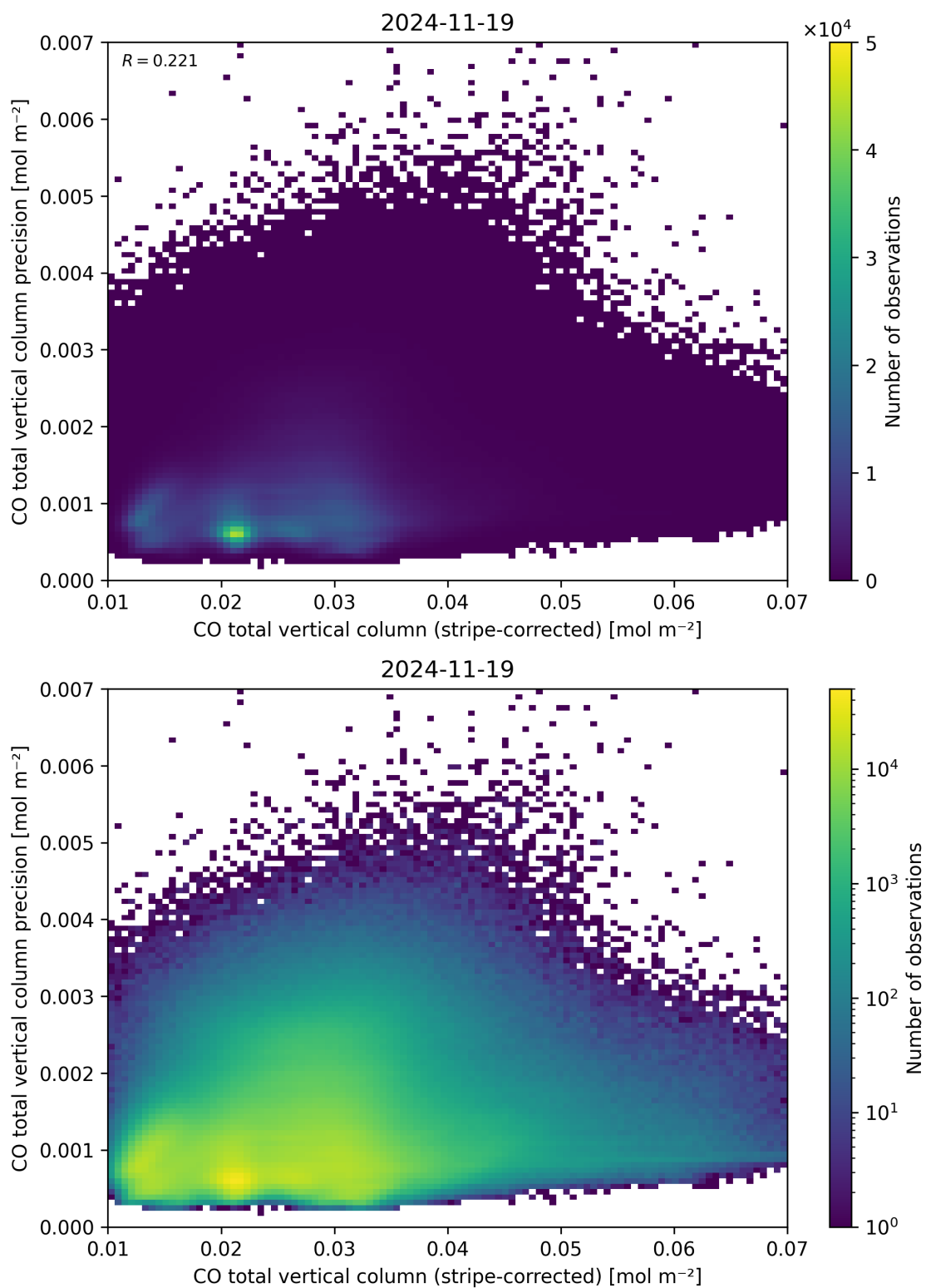
Figure 36: Scatter density plot of “CO total vertical column (stripe-corrected)” against “CO total vertical column precision” for 2024-11-18 to 2024-11-20.
