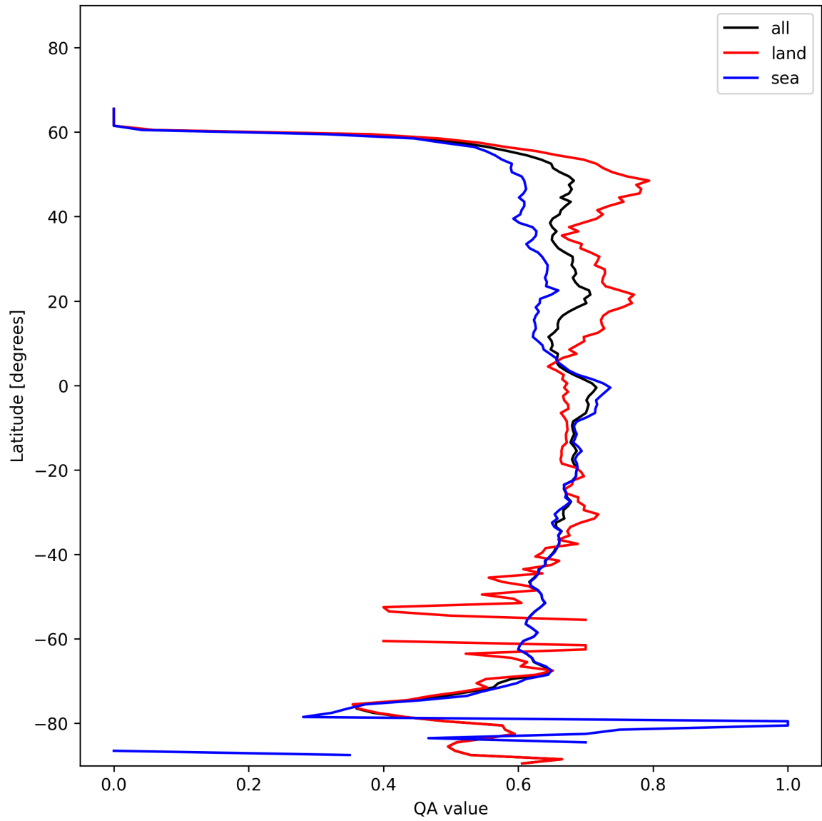
Figure 9: Zonal average of “QA value” for 2024-11-18 to 2024-11-20.
