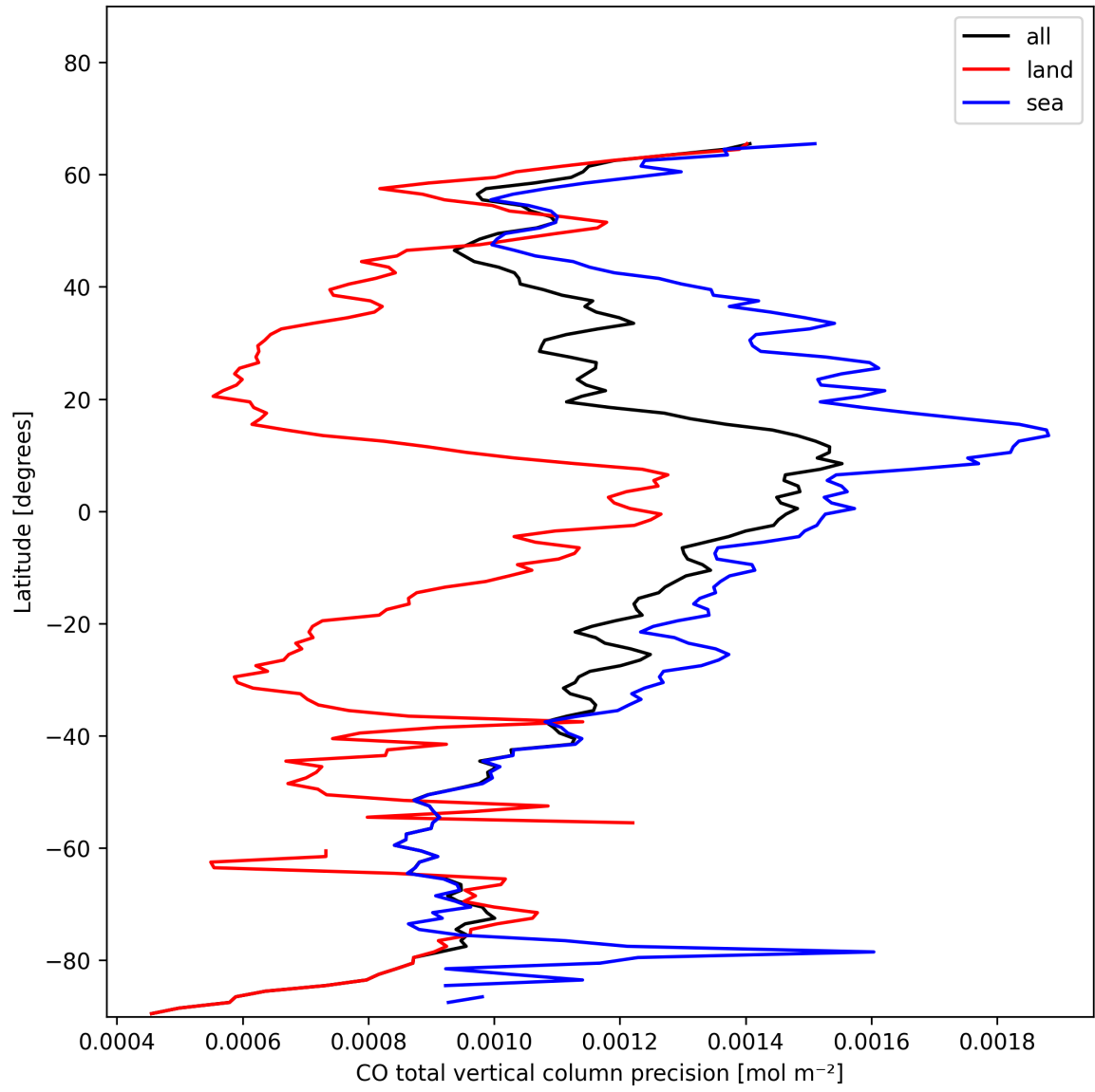
Figure 12: Zonal average of “CO total vertical column precision” for 2024-11-18 to 2024-11-20.
