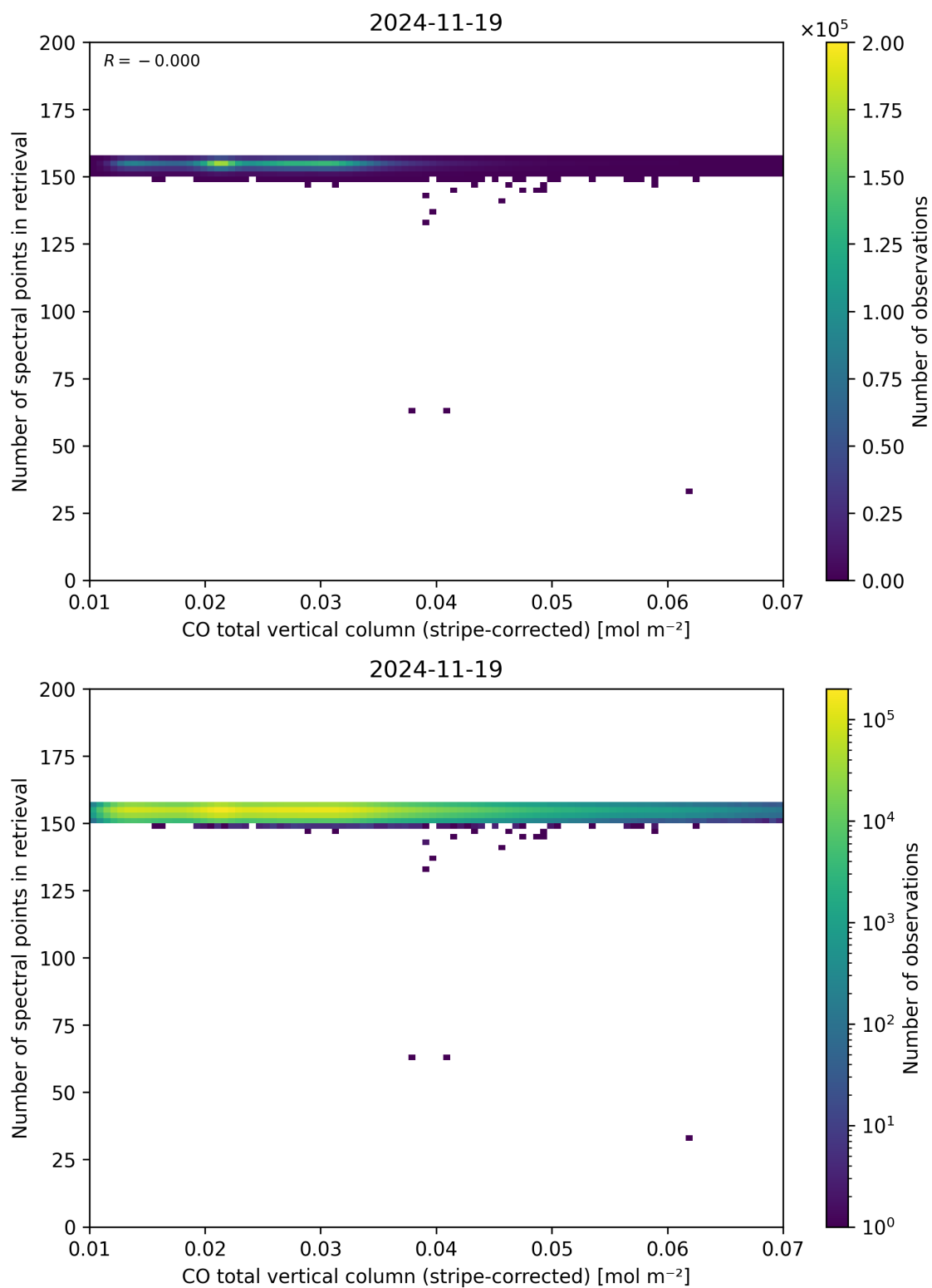
Figure 40: Scatter density plot of “CO total vertical column (stripe-corrected)” against “Number of spectral points in retrieval” for 2024-11-18 to 2024-11-20.
