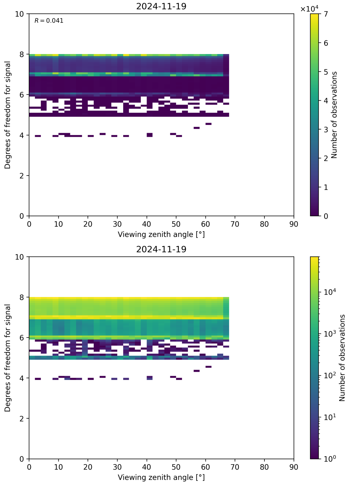
Figure 73: Scatter density plot of “Viewing zenith angle” against “Degrees of freedom for signal” for 2024-11-18 to 2024-11-20.
