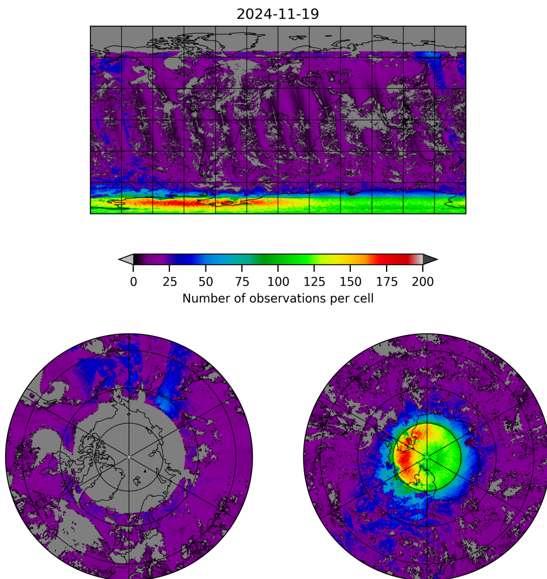
Figure 8: Map of the number of observations for 2024-11-18 to 2024-11-20
