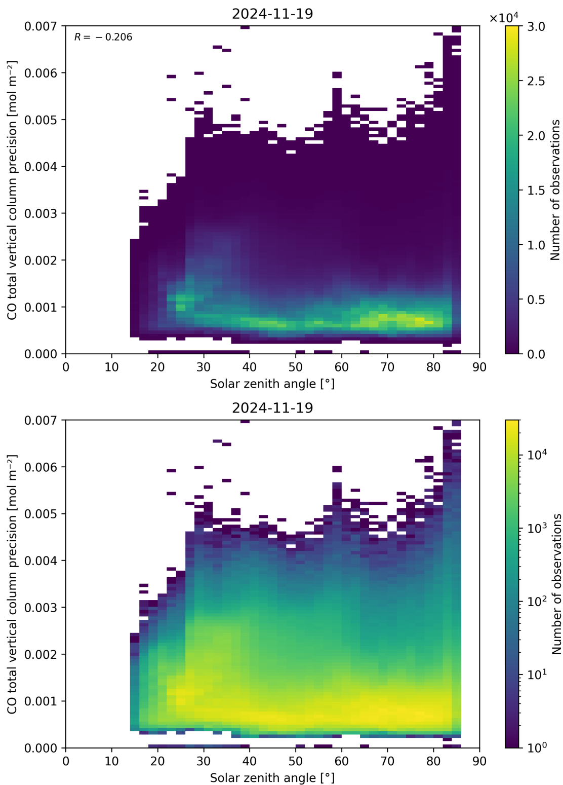
Figure 63: Scatter density plot of “Solar zenith angle” against “CO total vertical column precision” for 2024-11-18 to 2024-11-20.
