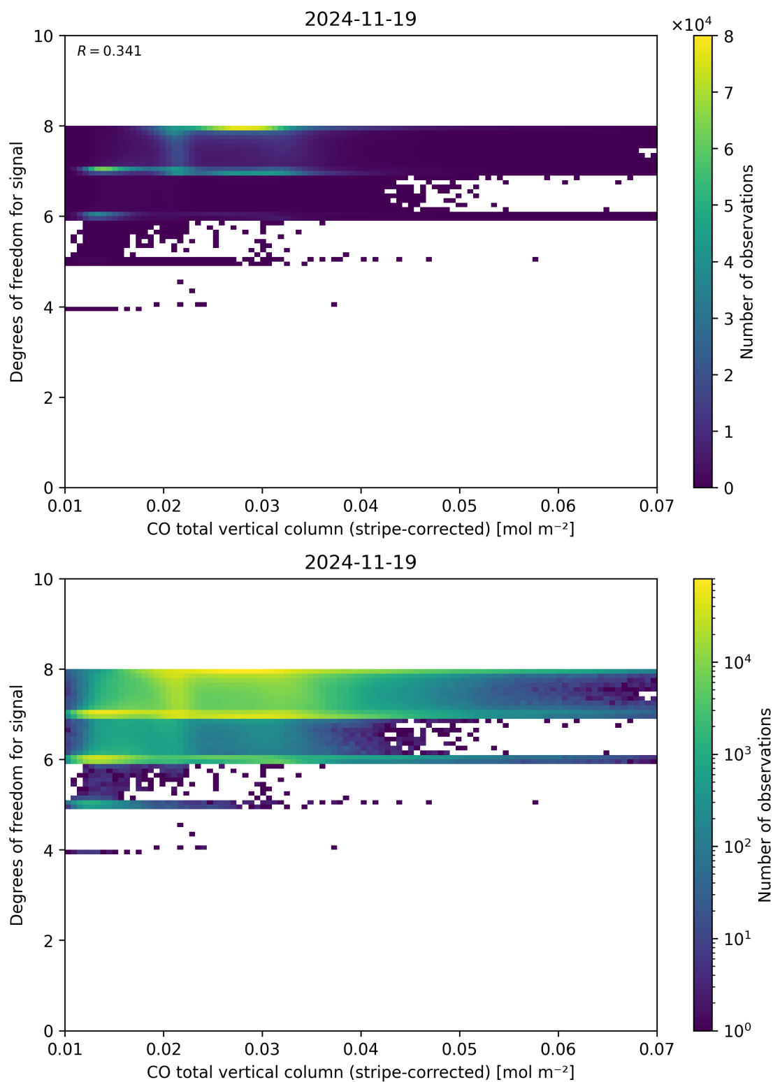
Figure 38: Scatter density plot of “CO total vertical column (stripe-corrected)” against “Degrees of freedom for signal” for 2024-11-18 to 2024-11-20.
