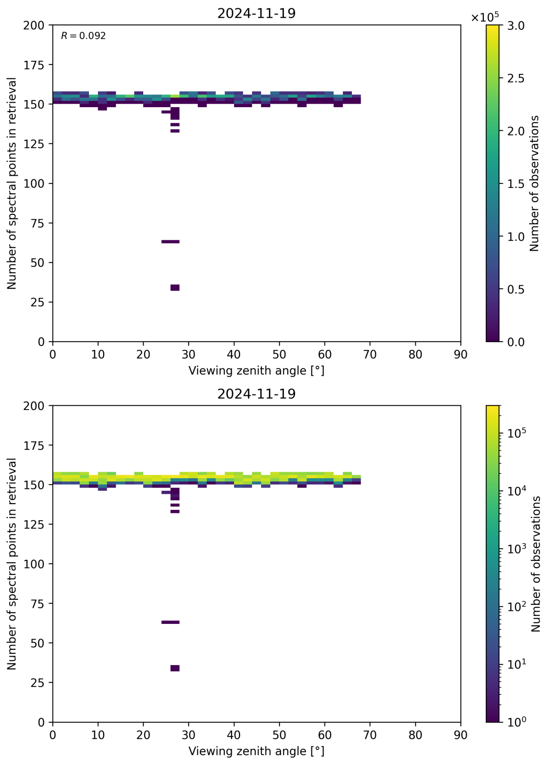
Figure 76: Scatter density plot of “Viewing zenith angle” against “Number of spectral points in retrieval” for 2024-11-18 to 2024-11-20.
