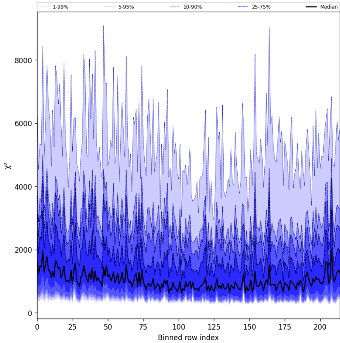
Figure 30: Along track statistics of “ \chi^2 ” for 2024-11-18 to 2024-11-20
