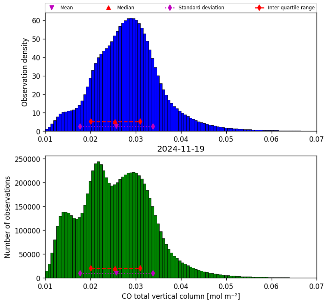
Figure 18: Histogram of “CO total vertical column” for 2024-11-18 to 2024-11-20
