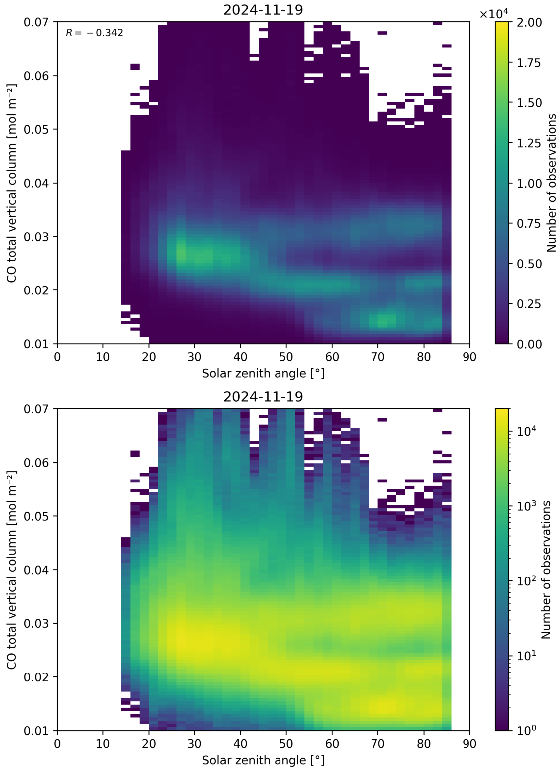
Figure 61: Scatter density plot of “Solar zenith angle” against “CO total vertical column” for 2024-11-18 to 2024-11-20.
