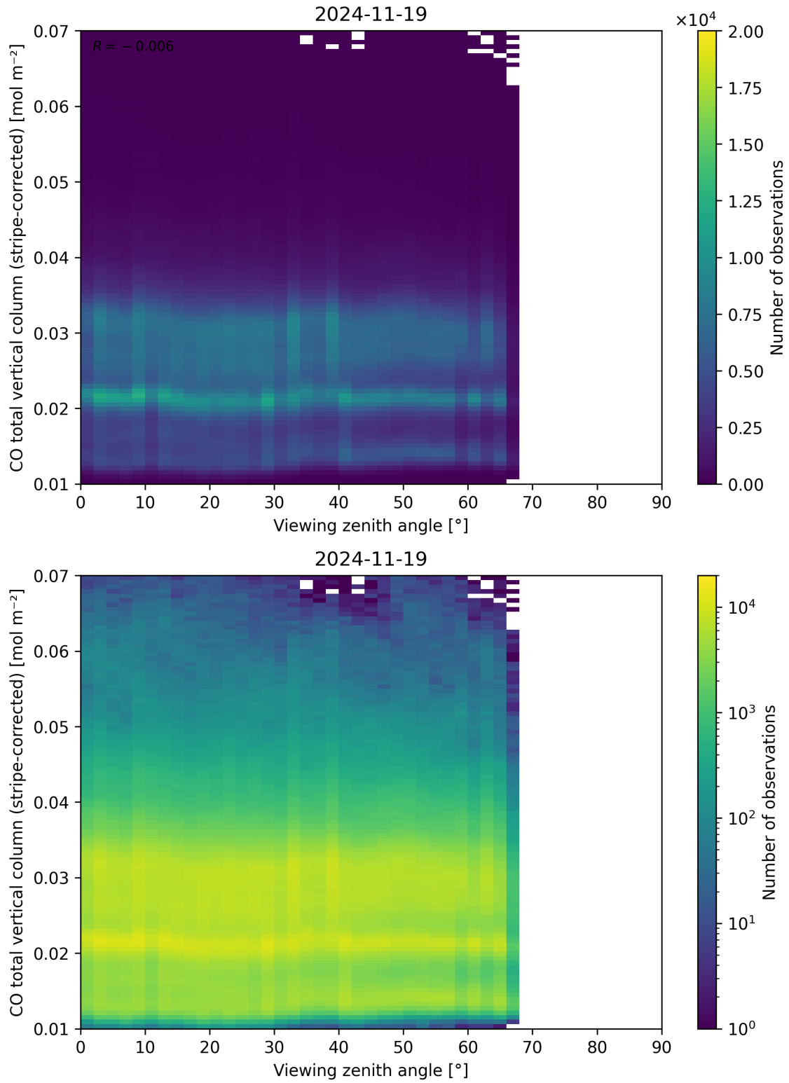
Figure 70: Scatter density plot of “Viewing zenith angle” against “CO total vertical column (stripe-corrected)” for 2024-11-18 to 2024-11-20.
