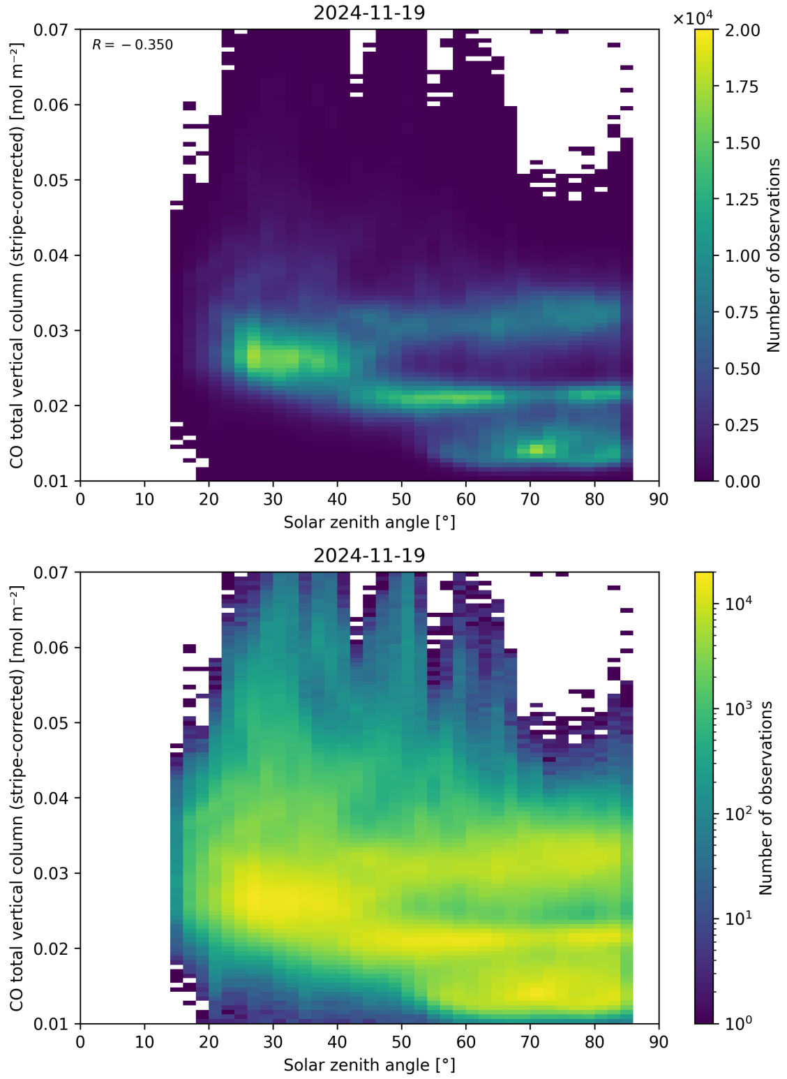
Figure 62: Scatter density plot of “Solar zenith angle” against “CO total vertical column (stripe-corrected)” for 2024-11-18 to 2024-11-20.
