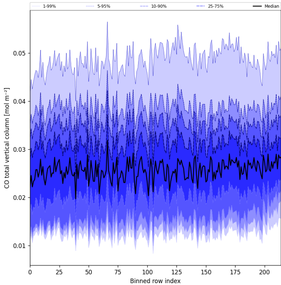
Figure 26: Along track statistics of “CO total vertical column” for 2024-11-18 to 2024-11-20
