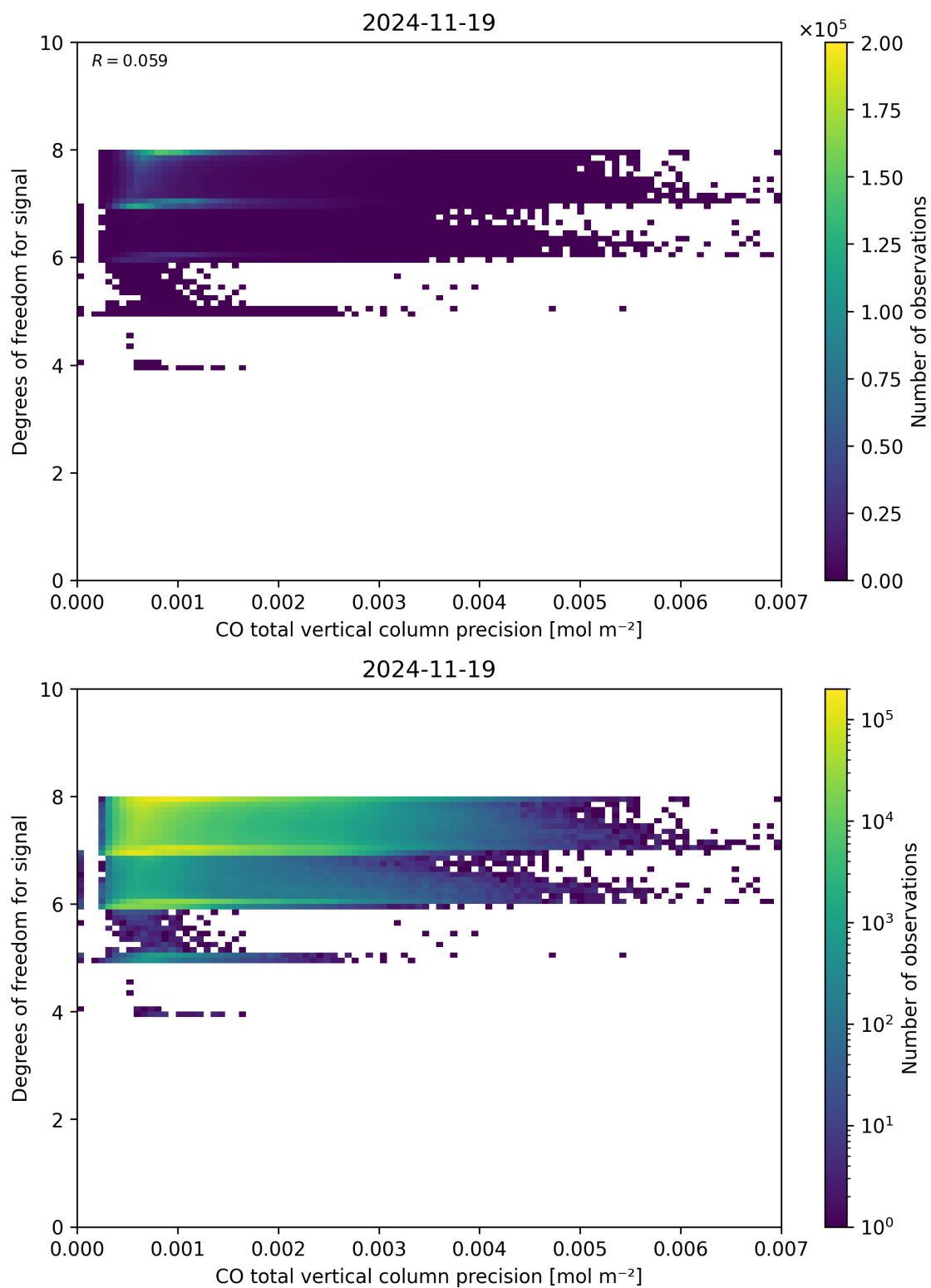
Figure 45: Scatter density plot of “CO total vertical column precision” against “Degrees of freedom for signal” for 2024-11-18 to 2024-11-20.
