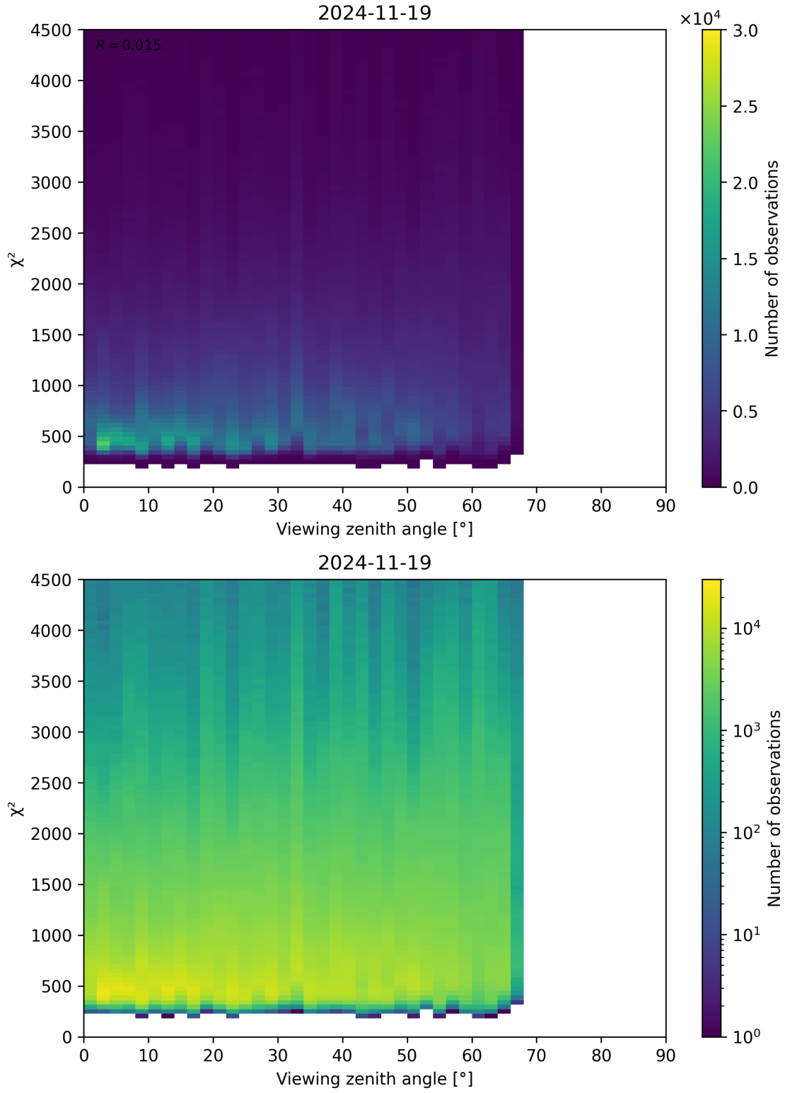
Figure 72: Scatter density plot of “Viewing zenith angle” against “ \chi^2 ” for 2024-11-18 to 2024-11-20.
