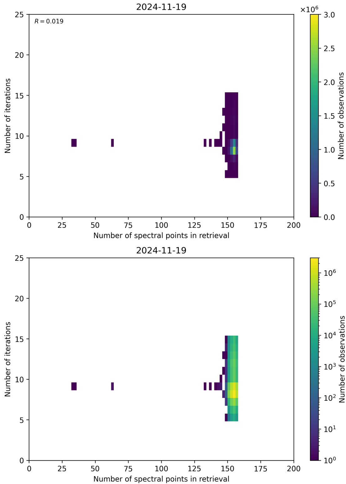
Figure 60: Scatter density plot of “Number of spectral points in retrieval” against “Number of iterations” for 2024-11-18 to 2024-11-20.
