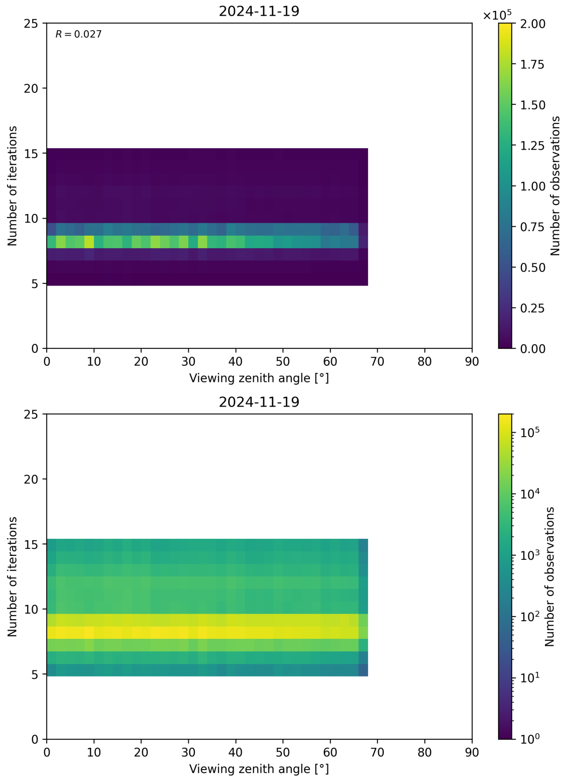
Figure 75: Scatter density plot of “Viewing zenith angle” against “Number of iterations” for 2024-11-18 to 2024-11-20.
