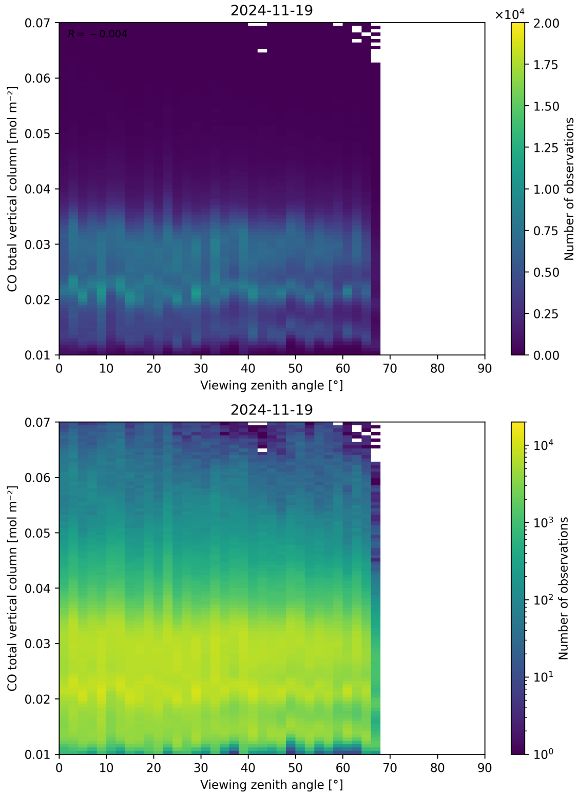
Figure 69: Scatter density plot of “Viewing zenith angle” against “CO total vertical column” for 2024-11-18 to 2024-11-20.
