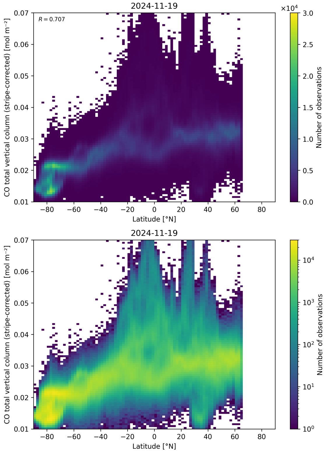
Figure 52: Scatter density plot of “Latitude” against “CO total vertical column (stripe-corrected)” for 2024-11-18 to 2024-11-20.
