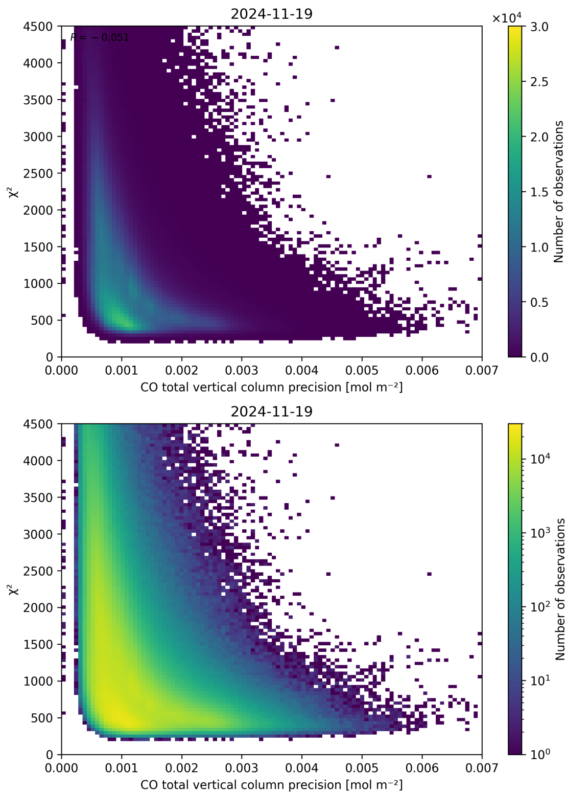
Figure 44: Scatter density plot of “CO total vertical column precision” against “ \chi^2 ” for 2024-11-18 to 2024-11-20.
