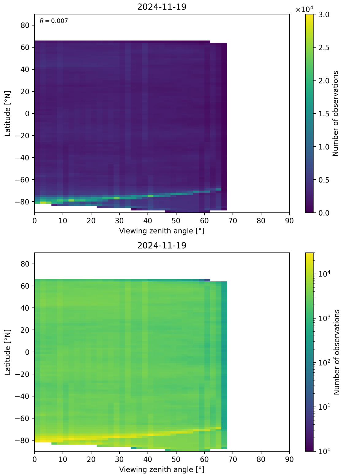
Figure 74: Scatter density plot of “Viewing zenith angle” against “Latitude” for 2024-11-18 to 2024-11-20.
