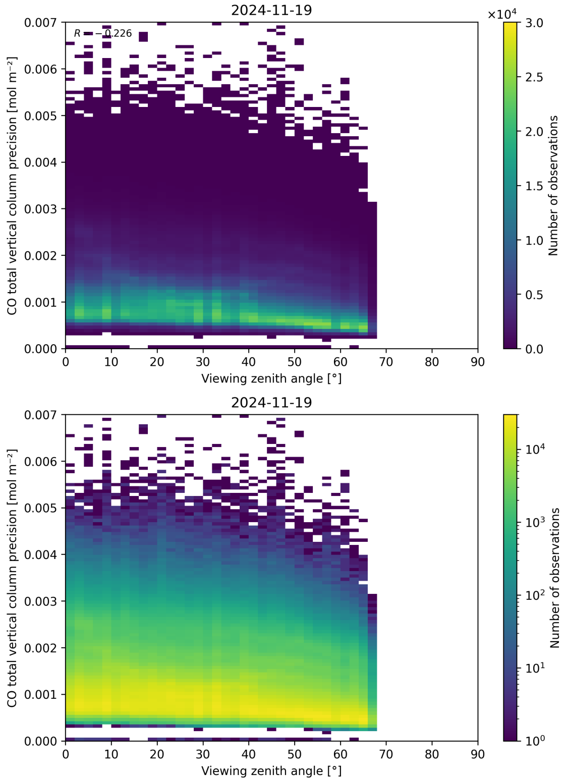
Figure 71: Scatter density plot of “Viewing zenith angle” against “CO total vertical column precision” for 2024-11-18 to 2024-11-20.
