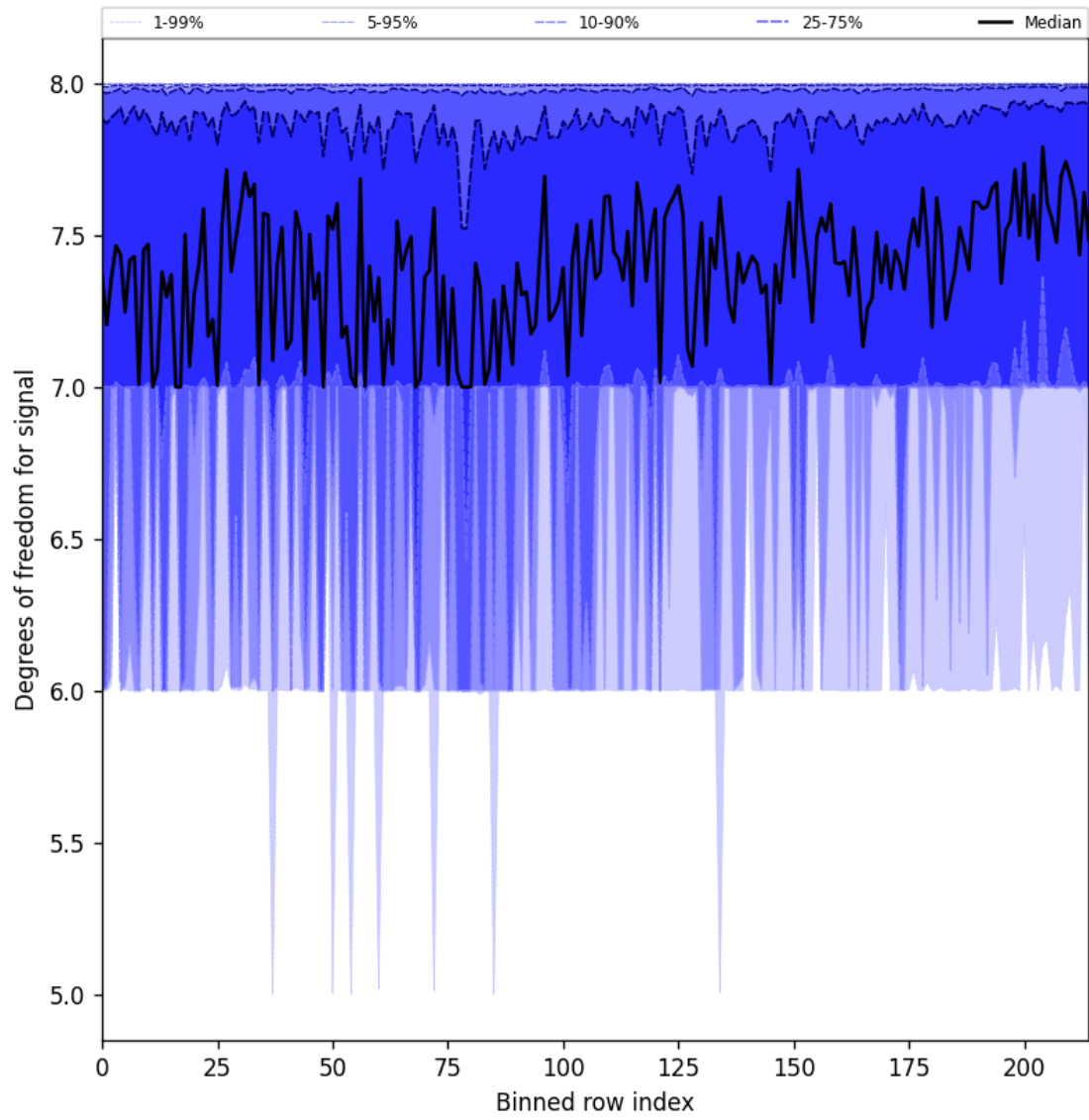
Figure 31: Along track statistics of “Degrees of freedom for signal” for 2024-11-18 to 2024-11-20
