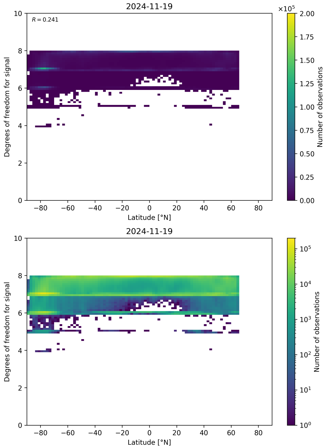
Figure 55: Scatter density plot of “Latitude” against “Degrees of freedom for signal” for 2024-11-18 to 2024-11-20.
