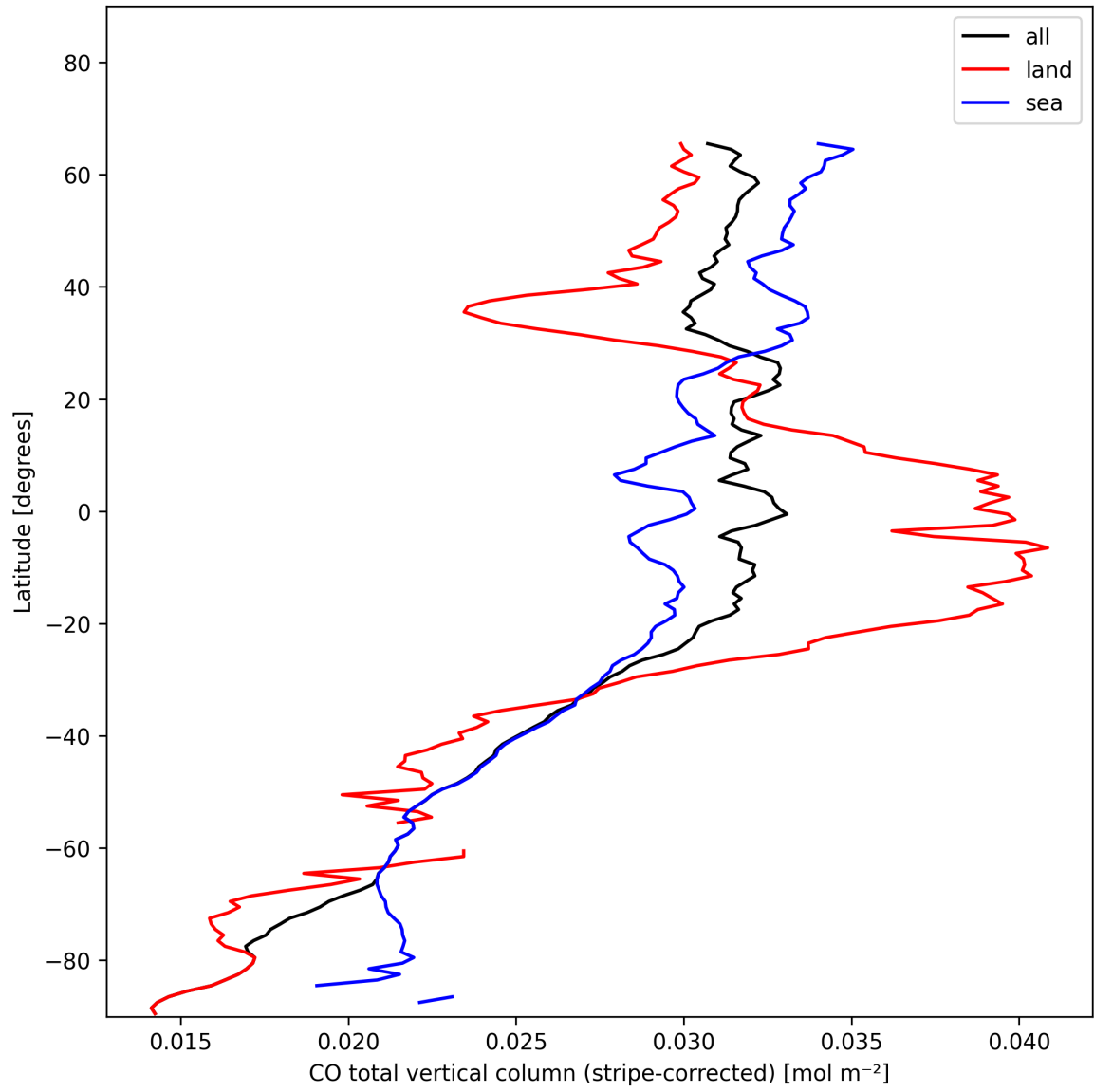
Figure 11: Zonal average of “CO total vertical column (stripe-corrected)” for 2024-11-18 to 2024-11-20.
