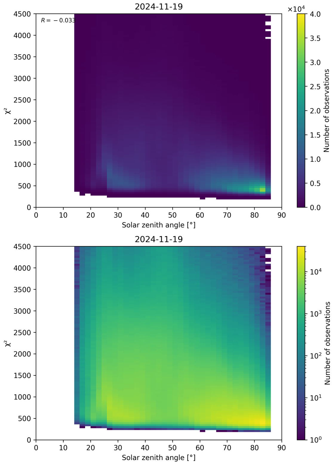
Figure 64: Scatter density plot of “Solar zenith angle” against “ \chi^2 ” for 2024-11-18 to 2024-11-20.
