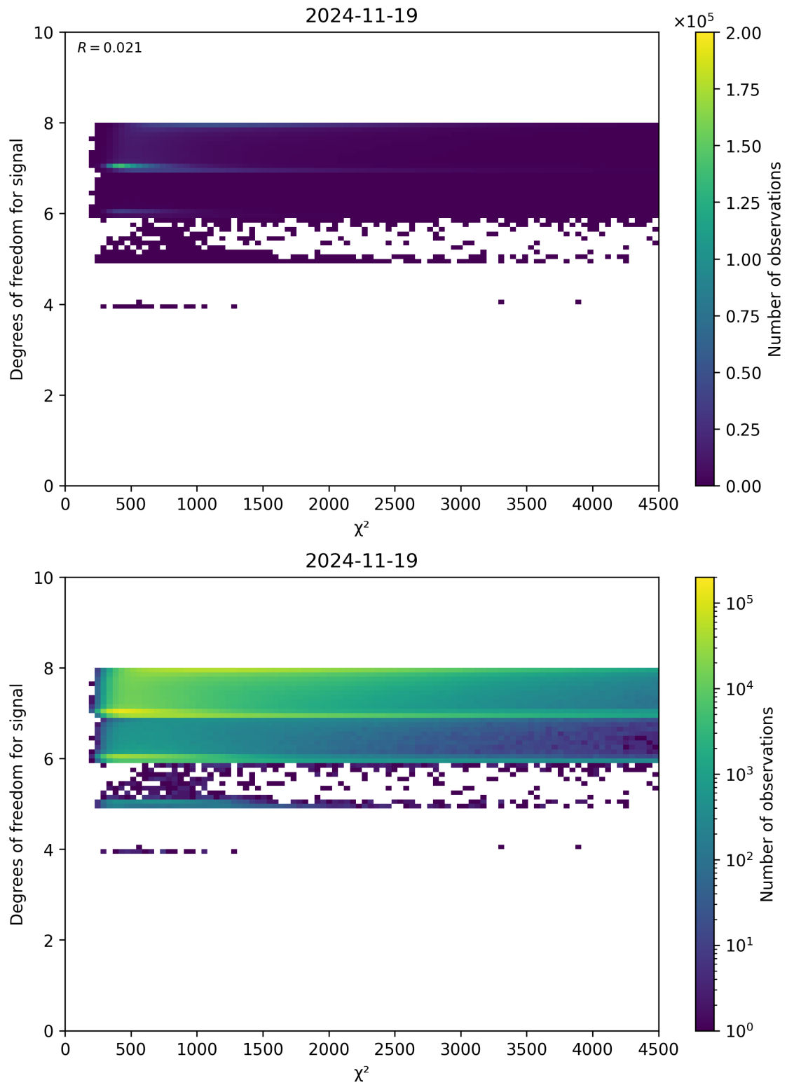
Figure 48: Scatter density plot of “ \chi^2 ” against “Degrees of freedom for signal” for 2024-11-18 to 2024-11-20.
