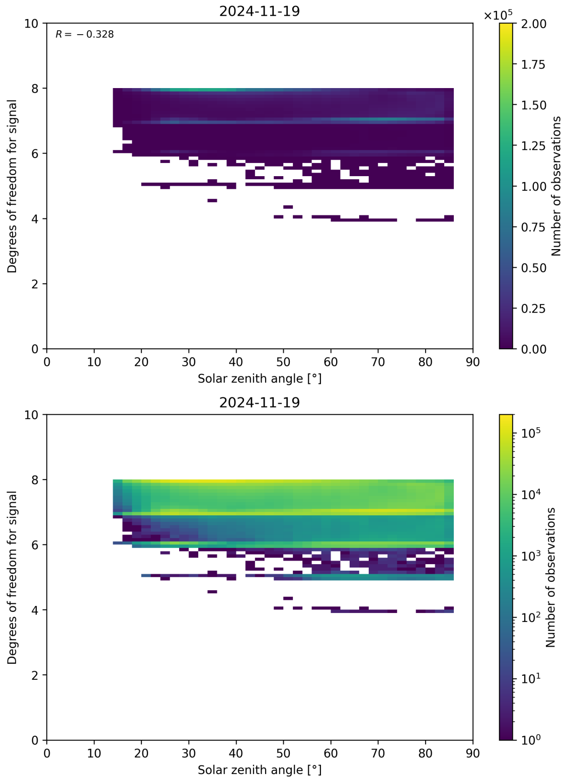
Figure 65: Scatter density plot of “Solar zenith angle” against “Degrees of freedom for signal” for 2024-11-18 to 2024-11-20.
