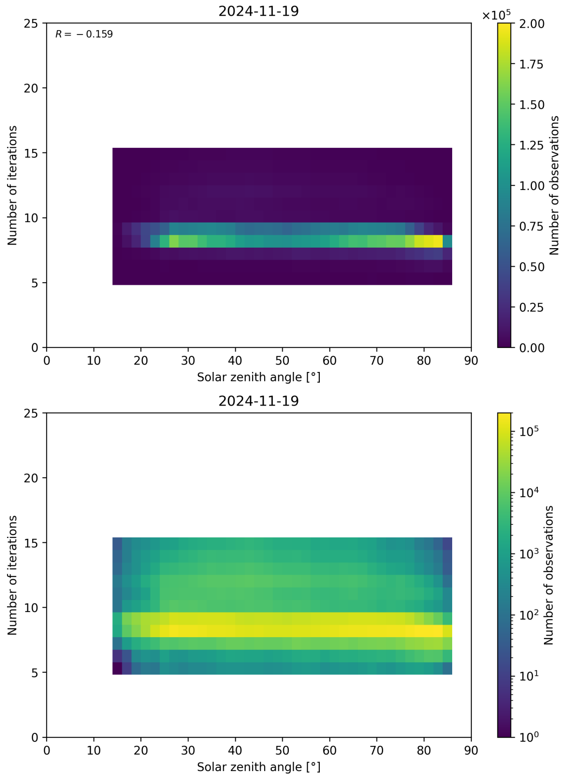
Figure 67: Scatter density plot of “Solar zenith angle” against “Number of iterations” for 2024-11-18 to 2024-11-20.
