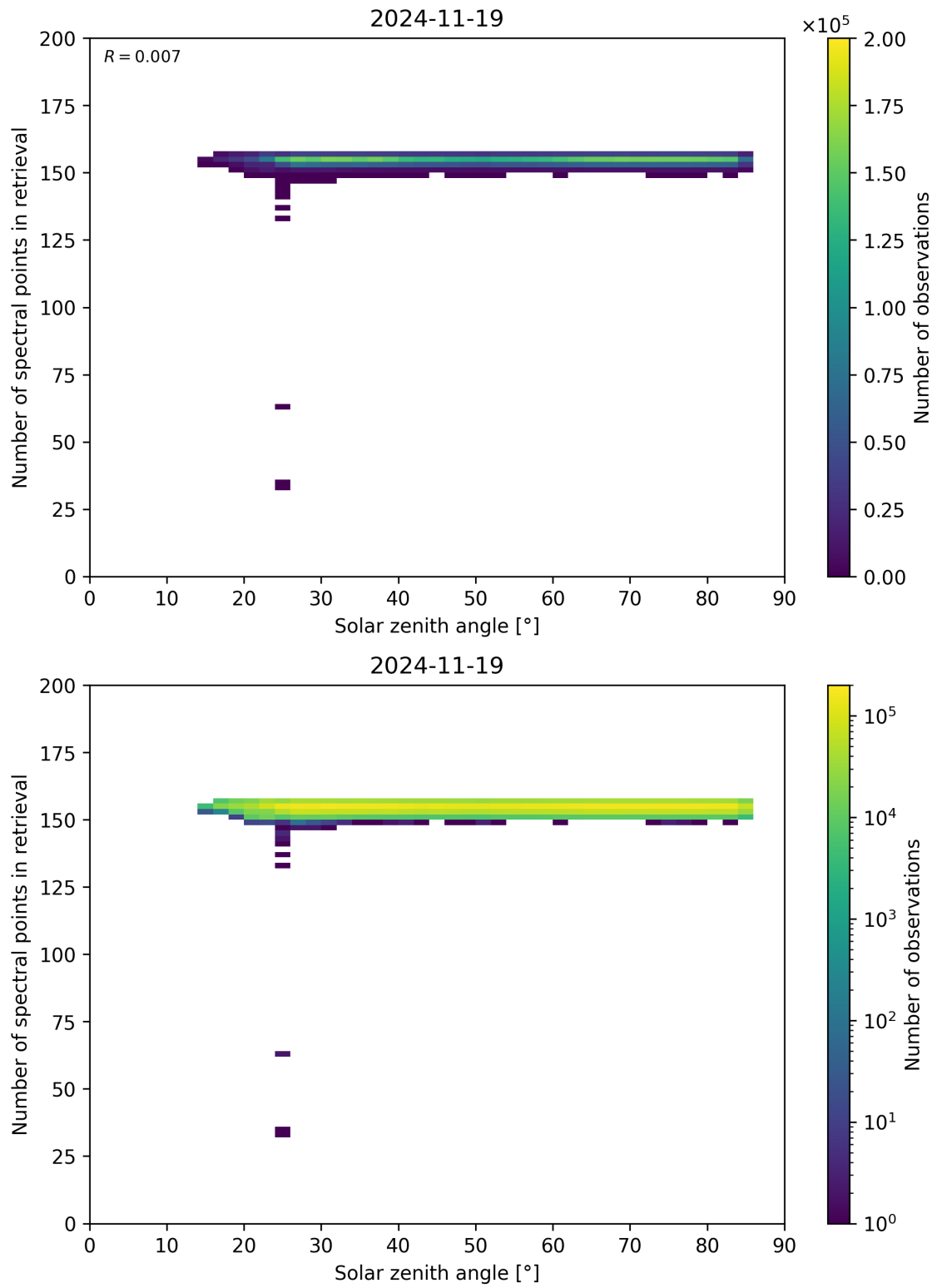
Figure 68: Scatter density plot of “Solar zenith angle” against “Number of spectral points in retrieval” for 2024-11-18 to 2024-11-20.
