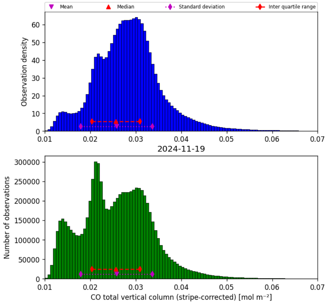
Figure 19: Histogram of “CO total vertical column (stripe-corrected)” for 2024-11-18 to 2024-11-20
