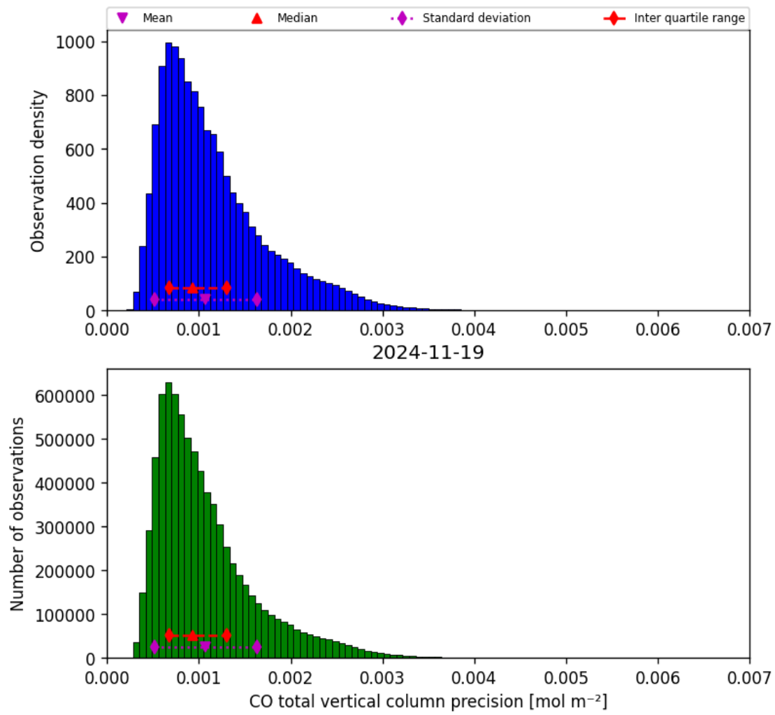
Figure 20: Histogram of “CO total vertical column precision” for 2024-11-18 to 2024-11-20
