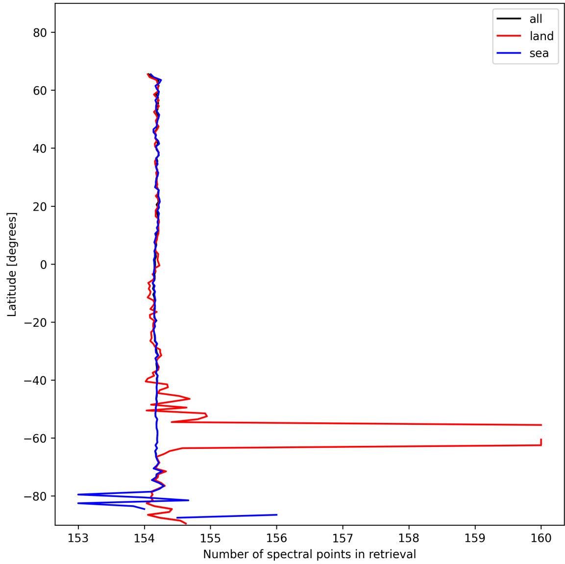
Figure 13: Zonal average of “Number of spectral points in retrieval” for 2024-11-18 to 2024-11-20.
