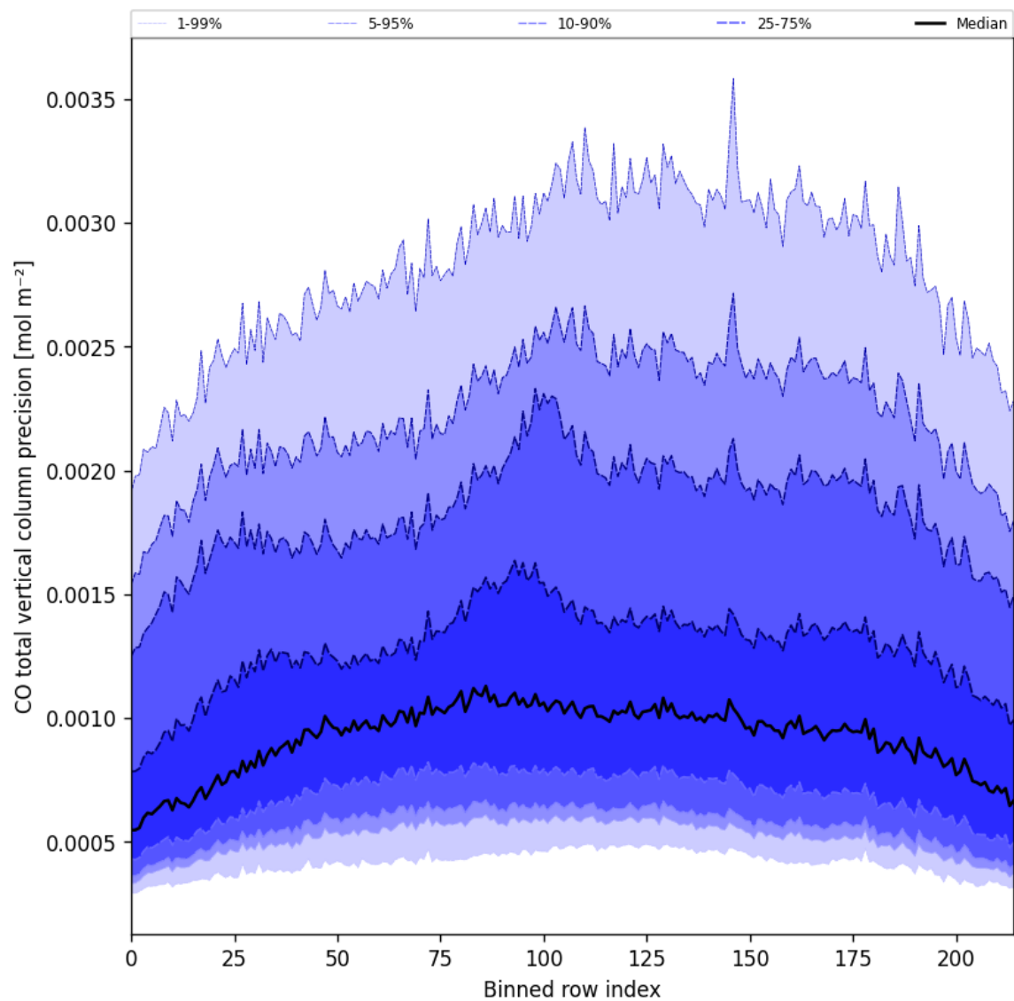
Figure 28: Along track statistics of “CO total vertical column precision” for 2024-11-18 to 2024-11-20
