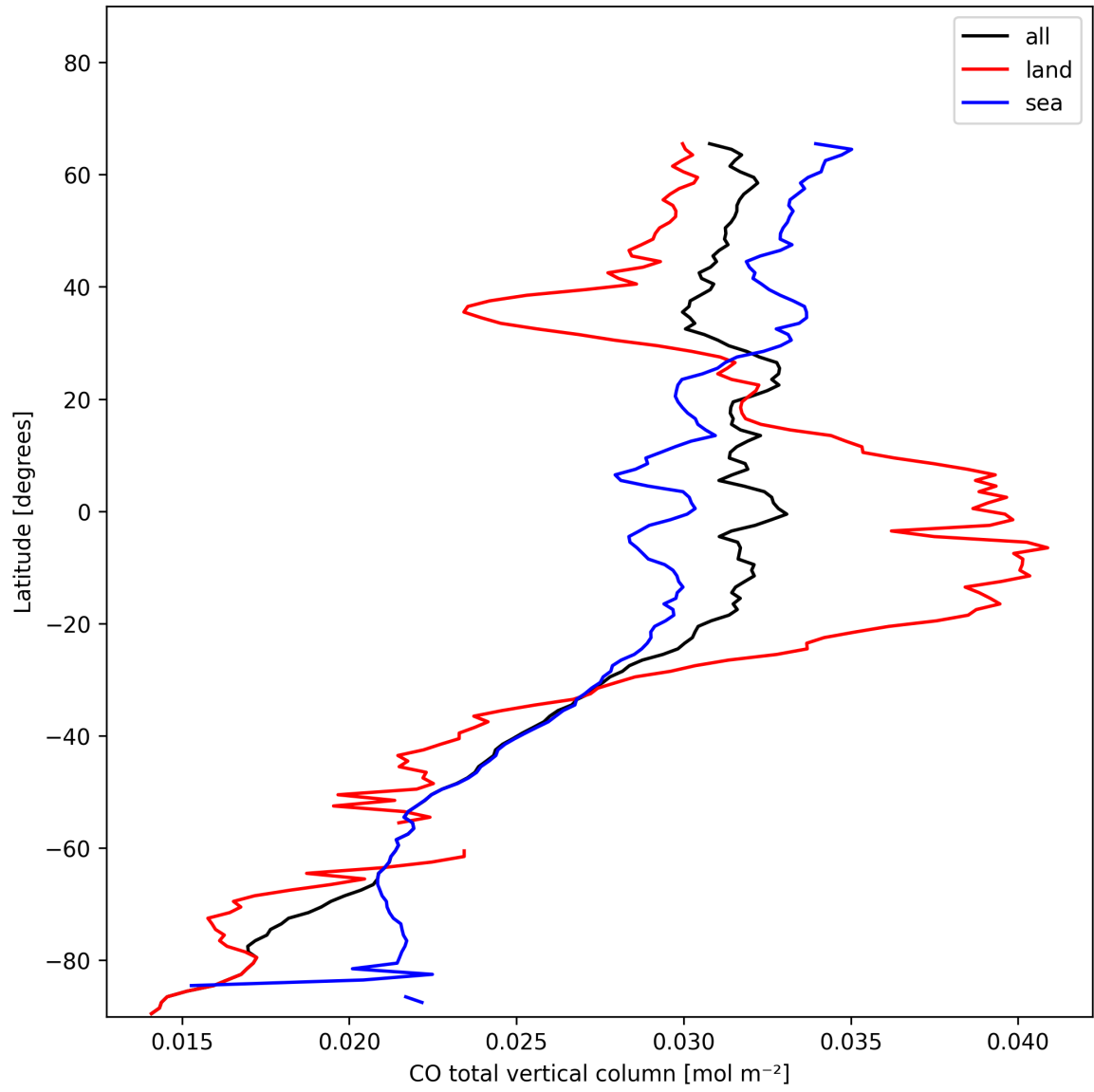
Figure 10: Zonal average of “CO total vertical column” for 2024-11-18 to 2024-11-20.
