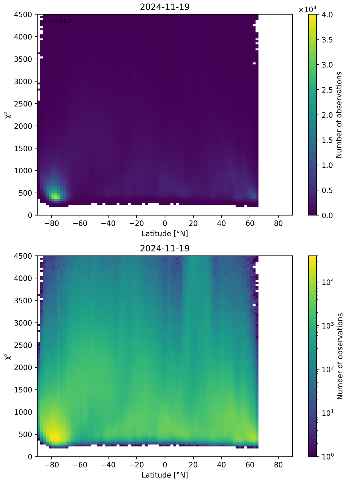
Figure 54: Scatter density plot of “Latitude” against “ \chi^2 ” for 2024-11-18 to 2024-11-20.
