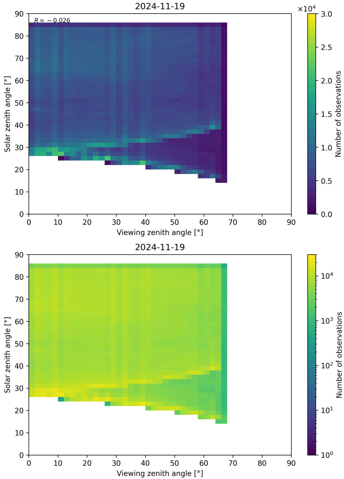
Figure 77: Scatter density plot of “Viewing zenith angle” against “Solar zenith angle” for 2024-11-18 to 2024-11-20.
