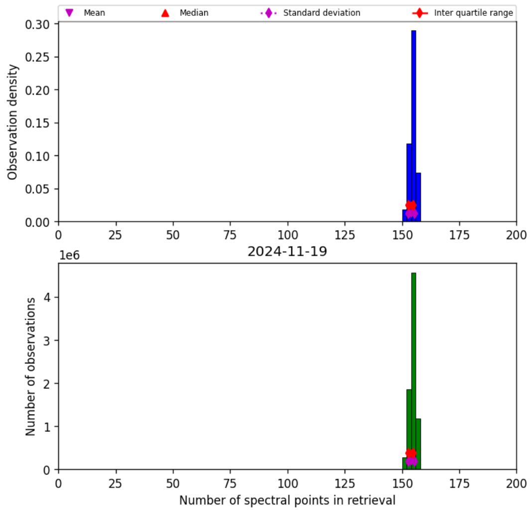
Figure 21: Histogram of “Number of spectral points in retrieval” for 2024-11-18 to 2024-11-20
