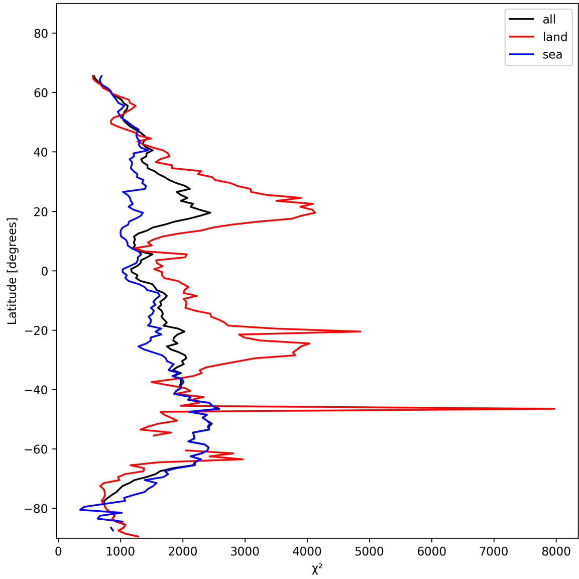
Figure 14: Zonal average of “ \chi^2 ” for 2024-11-18 to 2024-11-20.
