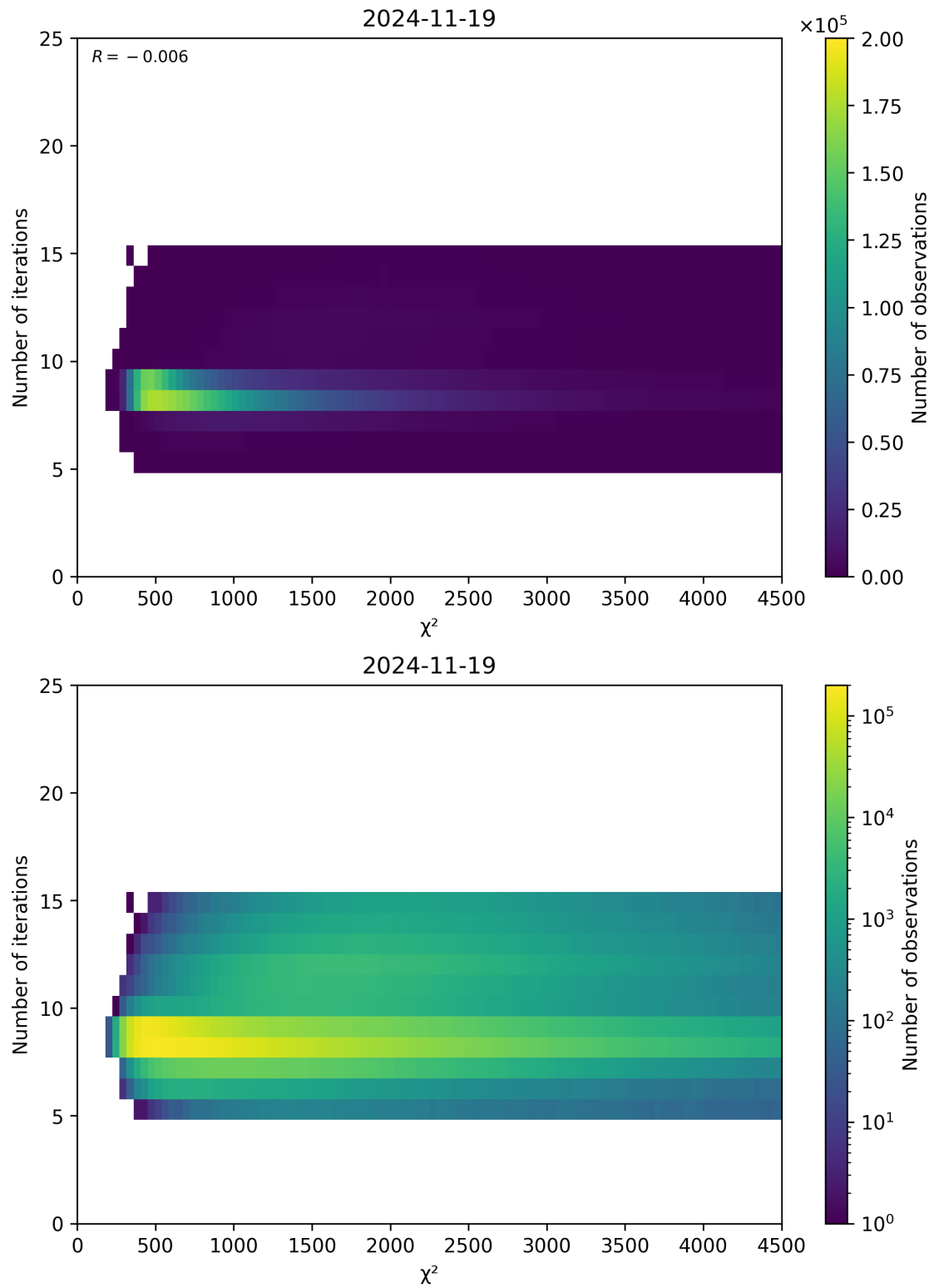
Figure 49: Scatter density plot of “ \chi^2 ” against “Number of iterations” for 2024-11-18 to 2024-11-20.
