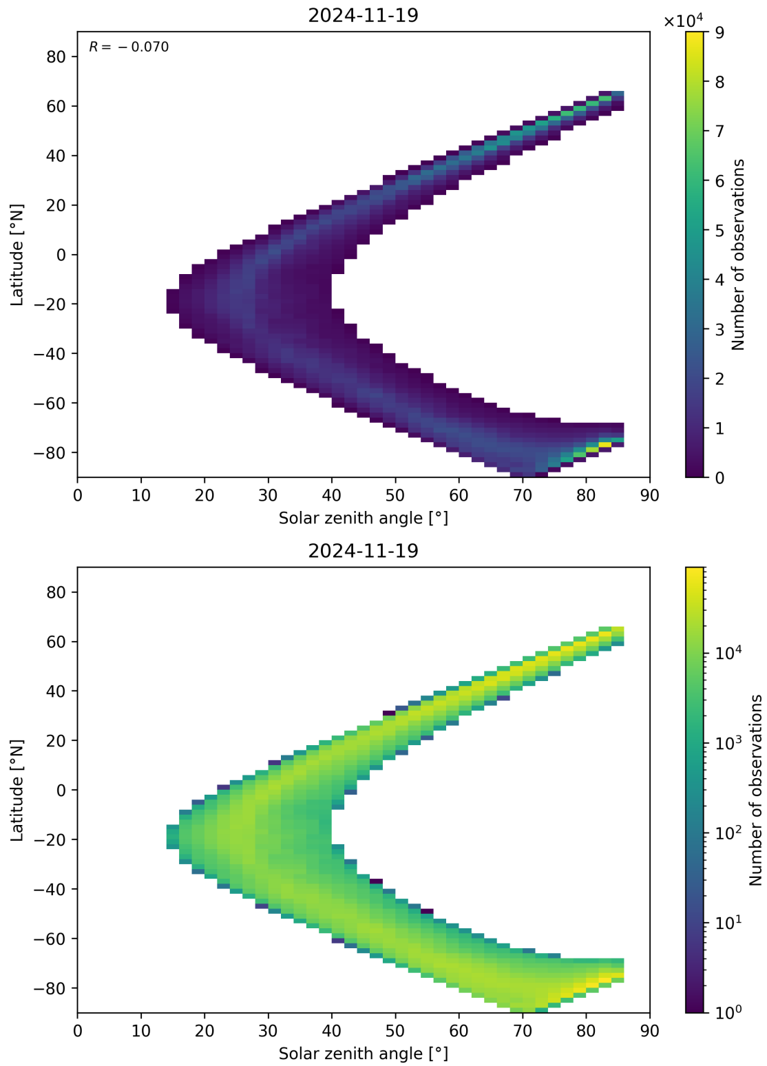
Figure 66: Scatter density plot of “Solar zenith angle” against “Latitude” for 2024-11-18 to 2024-11-20.
