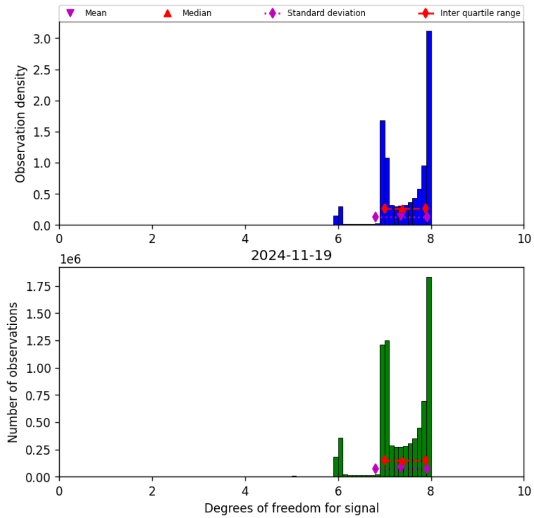
Figure 23: Histogram of “Degrees of freedom for signal” for 2024-11-18 to 2024-11-20
