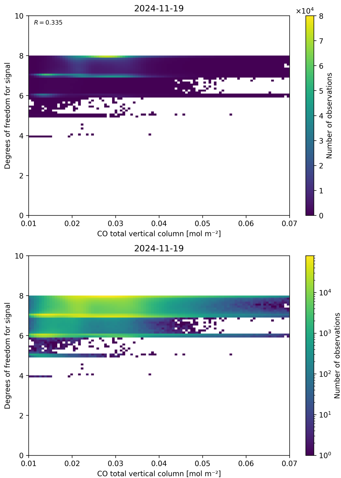
Figure 41: Scatter density plot of “CO total vertical column” against “Degrees of freedom for signal” for 2024-11-18 to 2024-11-20.
