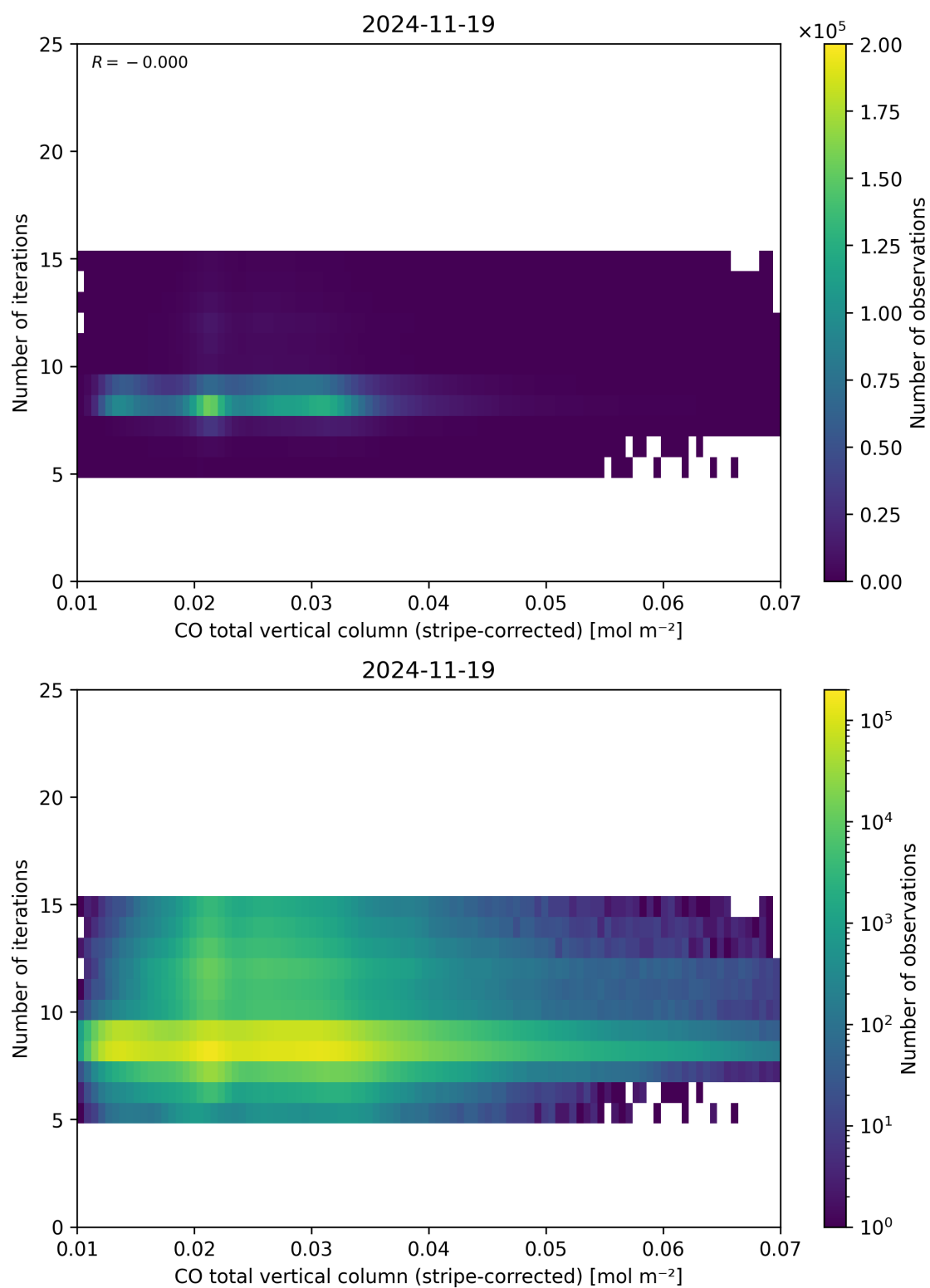
Figure 39: Scatter density plot of “CO total vertical column (stripe-corrected)” against “Number of iterations” for 2024-11-18 to 2024-11-20.
