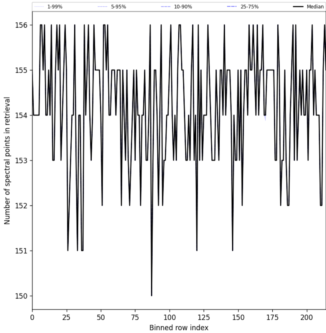
Figure 29: Along track statistics of “Number of spectral points in retrieval” for 2024-11-18 to 2024-11-20
