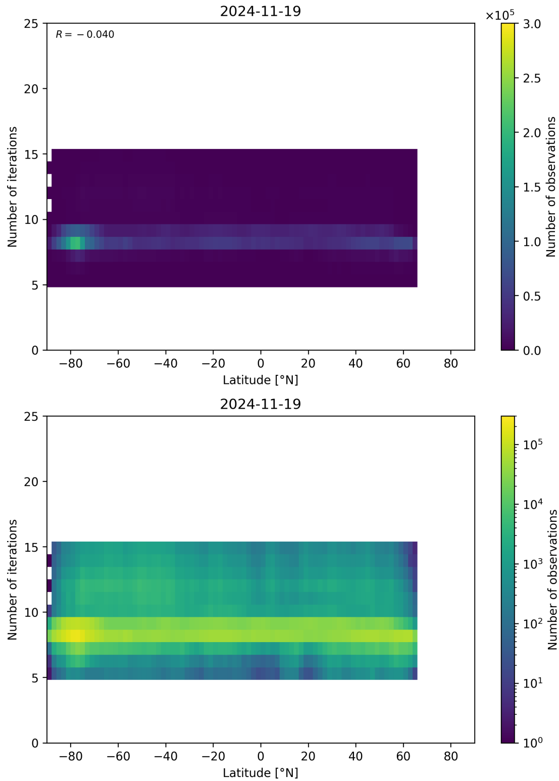
Figure 56: Scatter density plot of “Latitude” against “Number of iterations” for 2024-11-18 to 2024-11-20.
