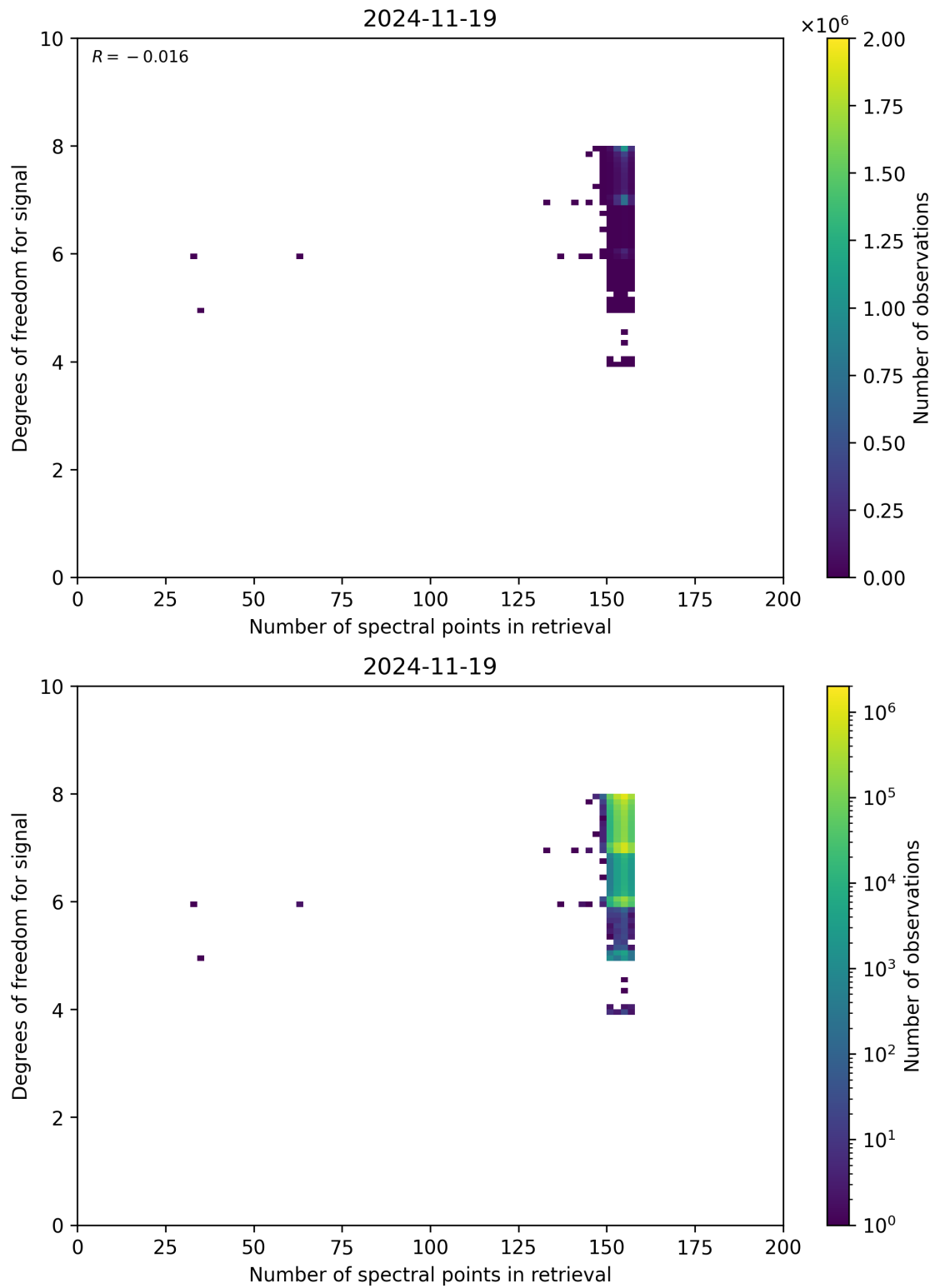
Figure 59: Scatter density plot of “Number of spectral points in retrieval” against “Degrees of freedom for signal” for 2024-11-18 to 2024-11-20.
