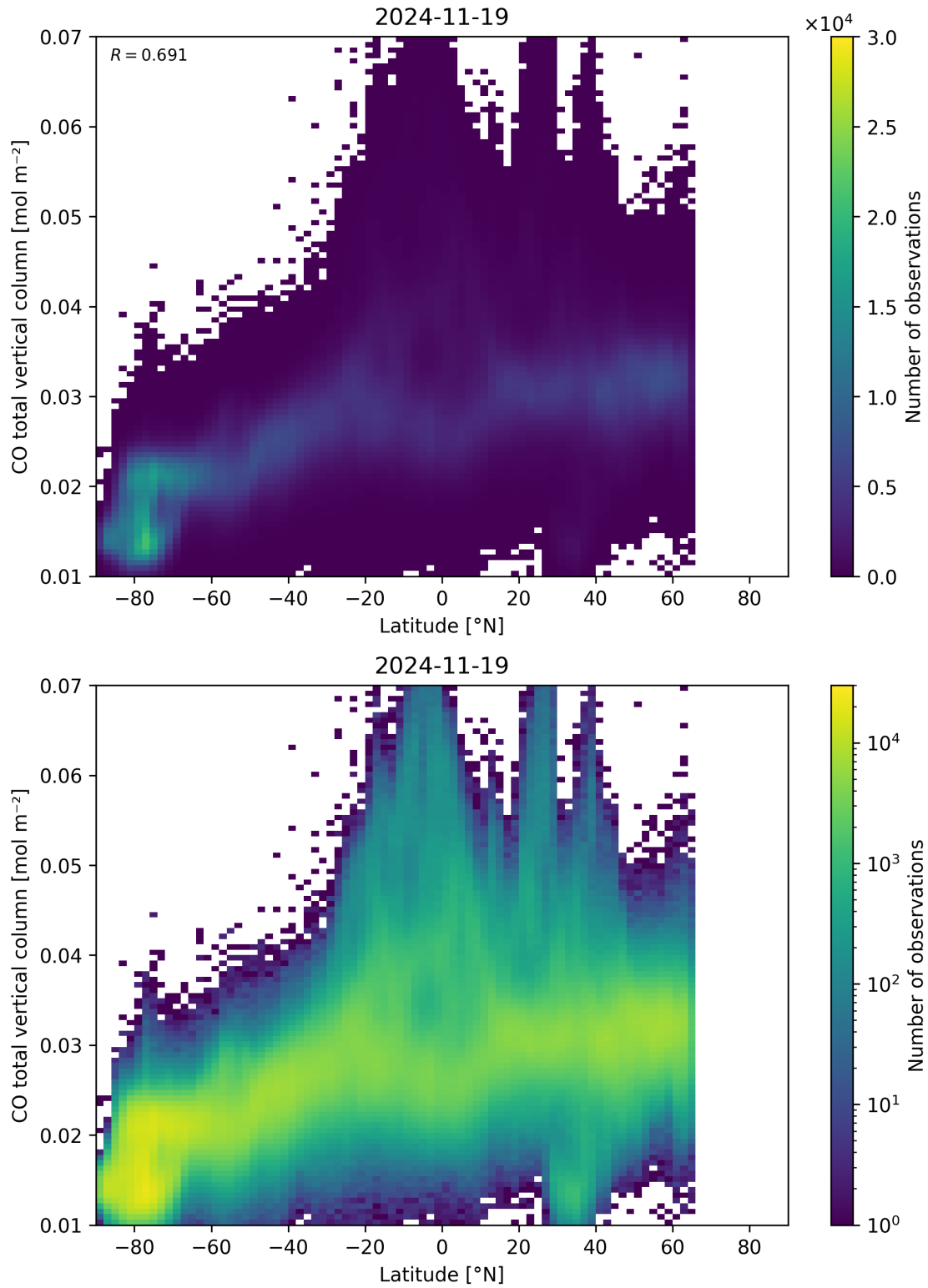
Figure 51: Scatter density plot of “Latitude” against “CO total vertical column” for 2024-11-18 to 2024-11-20.
