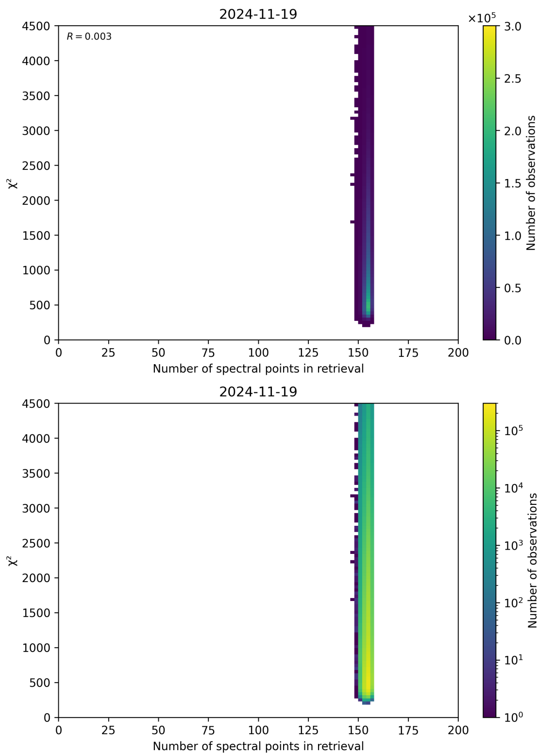
Figure 58: Scatter density plot of “Number of spectral points in retrieval” against “ \chi^2 ” for 2024-11-18 to 2024-11-20.
