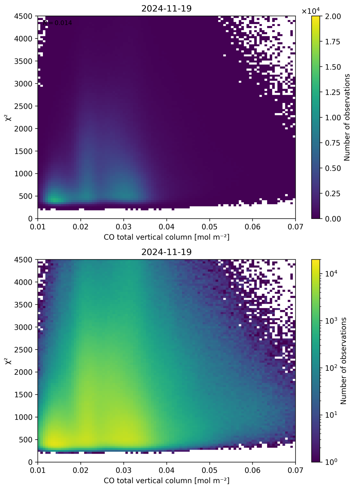
Figure 35: Scatter density plot of “CO total vertical column” against “ \chi^2 ” for 2024-11-18 to 2024-11-20.
