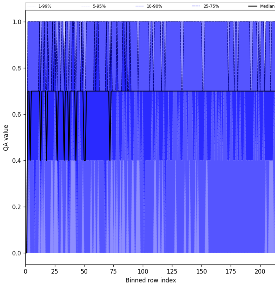
Figure 25: Along track statistics of “QA value” for 2024-11-18 to 2024-11-20
