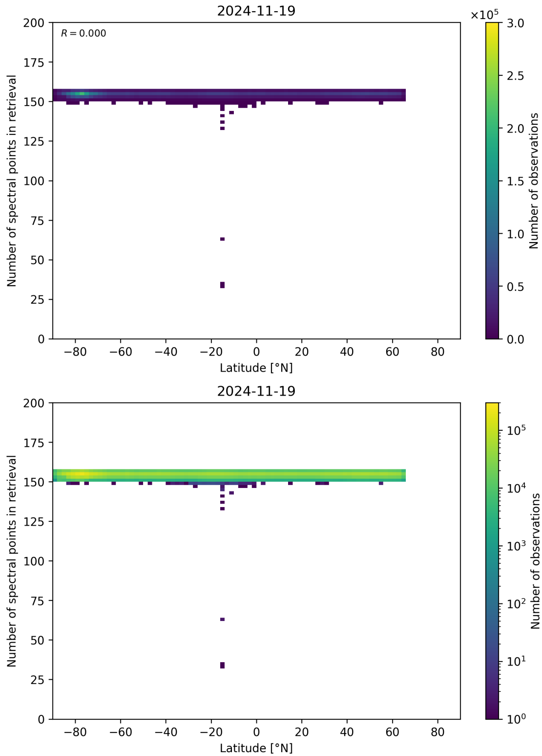
Figure 57: Scatter density plot of “Latitude” against “Number of spectral points in retrieval” for 2024-11-18 to 2024-11-20.
