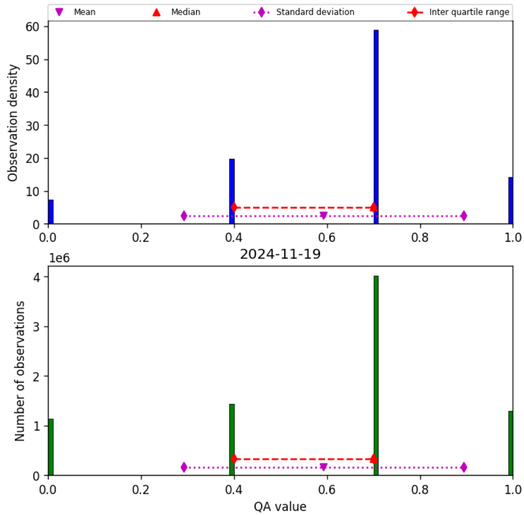
Figure 17: Histogram of “QA value” for 2024-11-18 to 2024-11-20
