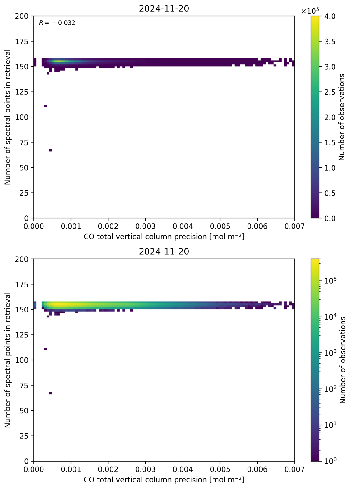
Figure 47: Scatter density plot of “CO total vertical column precision” against “Number of spectral points in retrieval” for 2024-11-20 to 2024-11-21.
