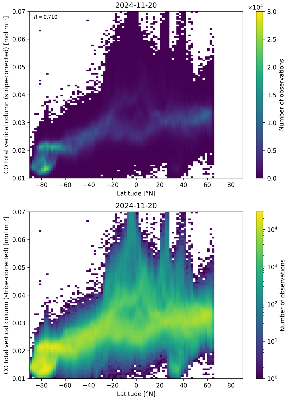
Figure 52: Scatter density plot of “Latitude” against “CO total vertical column (stripe-corrected)” for 2024-11-20 to 2024-11-21.
