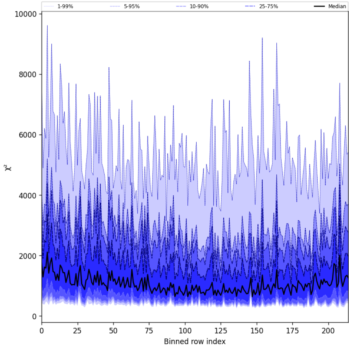
Figure 30: Along track statistics of “ \chi^2 ” for 2024-11-20 to 2024-11-21
