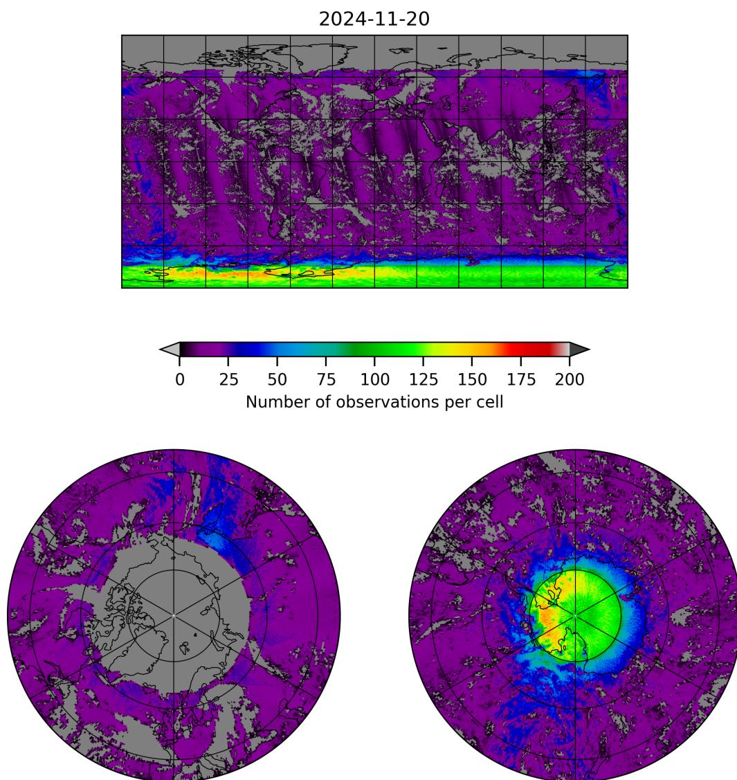
Figure 8: Map of the number of observations for 2024-11-20 to 2024-11-21
