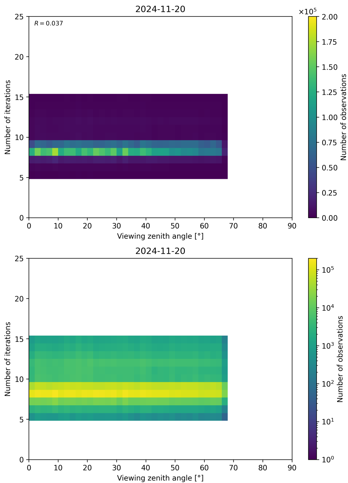
Figure 75: Scatter density plot of “Viewing zenith angle” against “Number of iterations” for 2024-11-20 to 2024-11-21.
