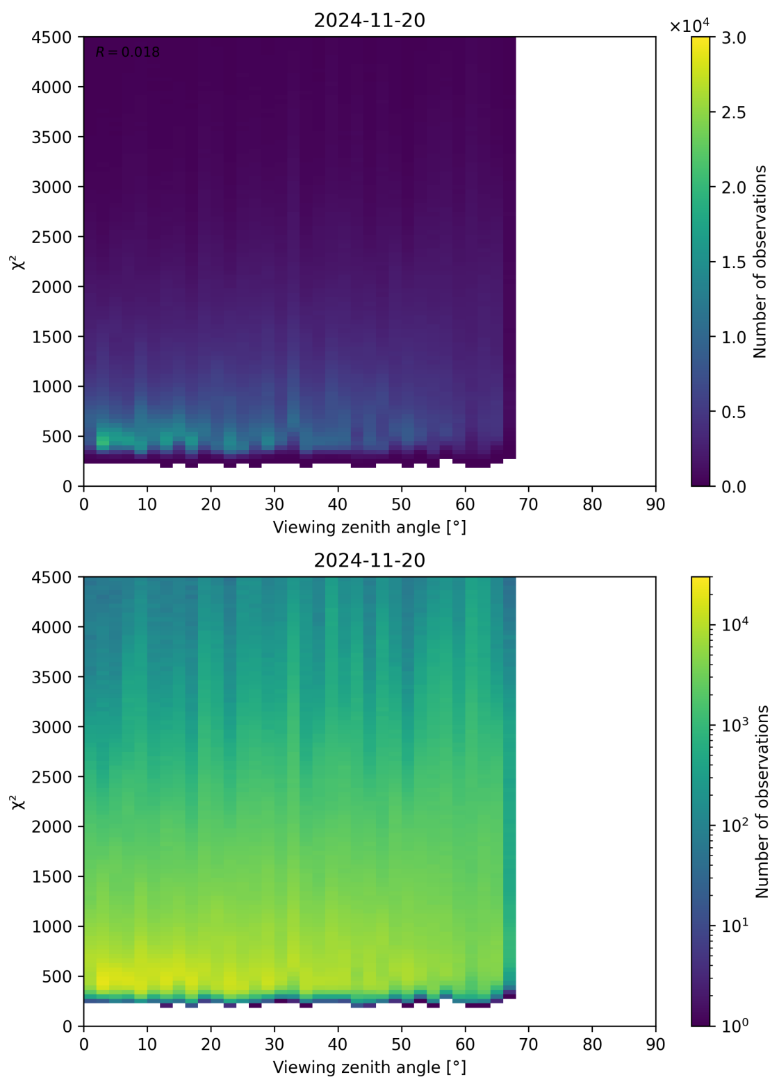
Figure 72: Scatter density plot of “Viewing zenith angle” against “ \chi^2 ” for 2024-11-20 to 2024-11-21.
