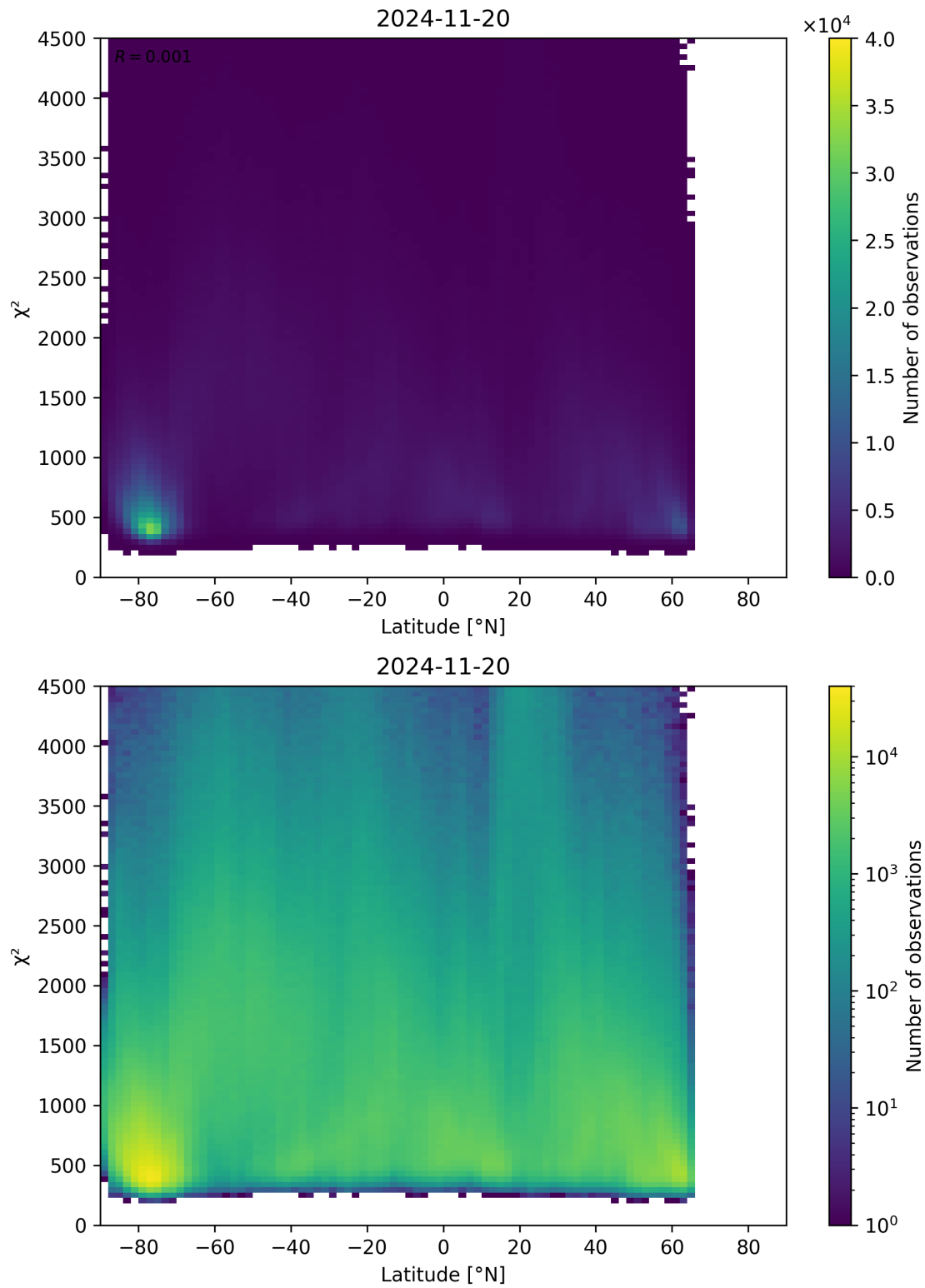
Figure 54: Scatter density plot of “Latitude” against “ \chi^2 ” for 2024-11-20 to 2024-11-21.
