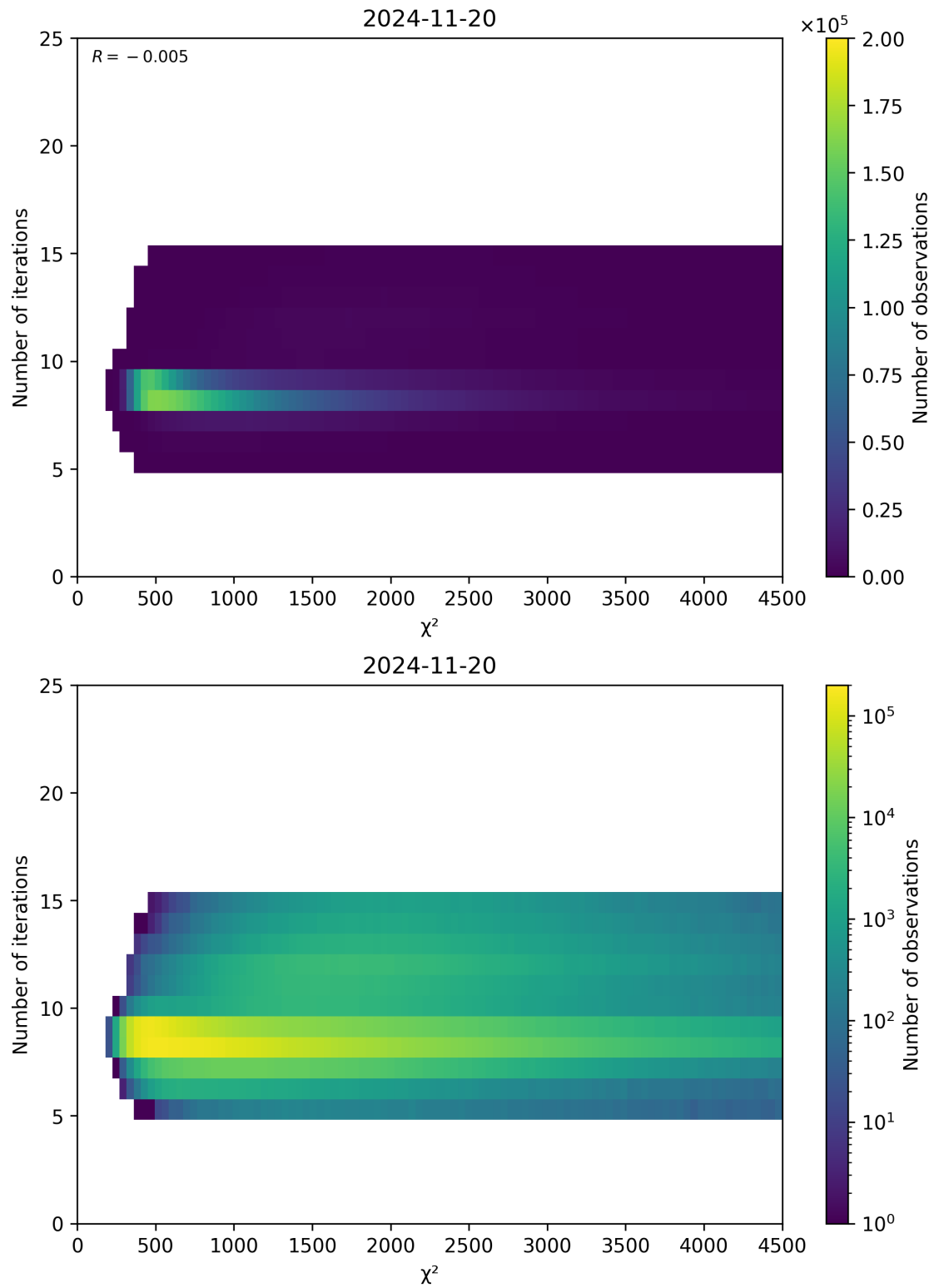
Figure 49: Scatter density plot of “ \chi^2 ” against “Number of iterations” for 2024-11-20 to 2024-11-21.
