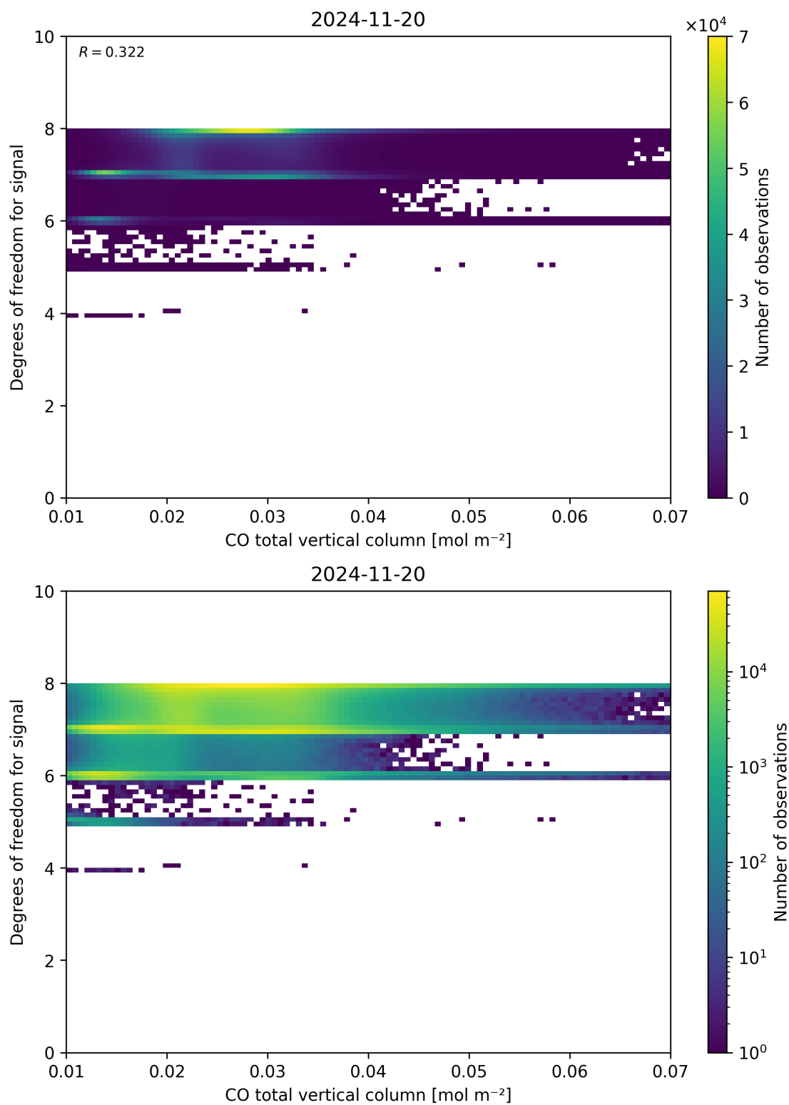
Figure 41: Scatter density plot of “CO total vertical column” against “Degrees of freedom for signal” for 2024-11-20 to 2024-11-21.
