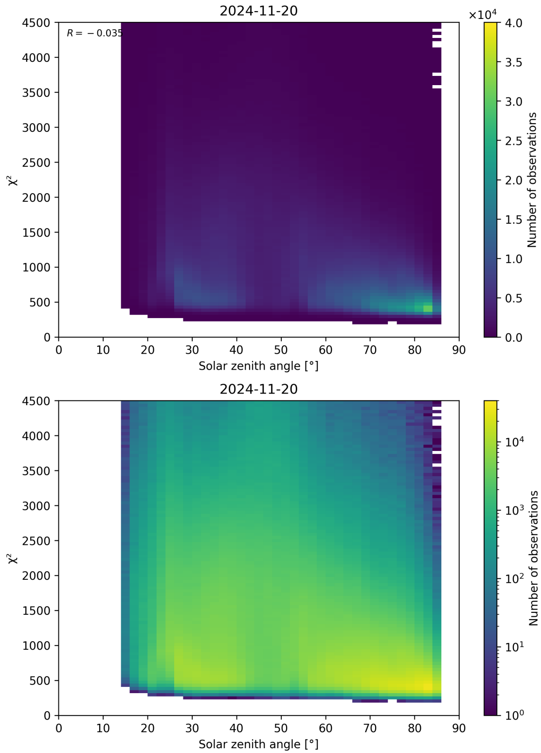
Figure 64: Scatter density plot of “Solar zenith angle” against “ \chi^2 ” for 2024-11-20 to 2024-11-21.
