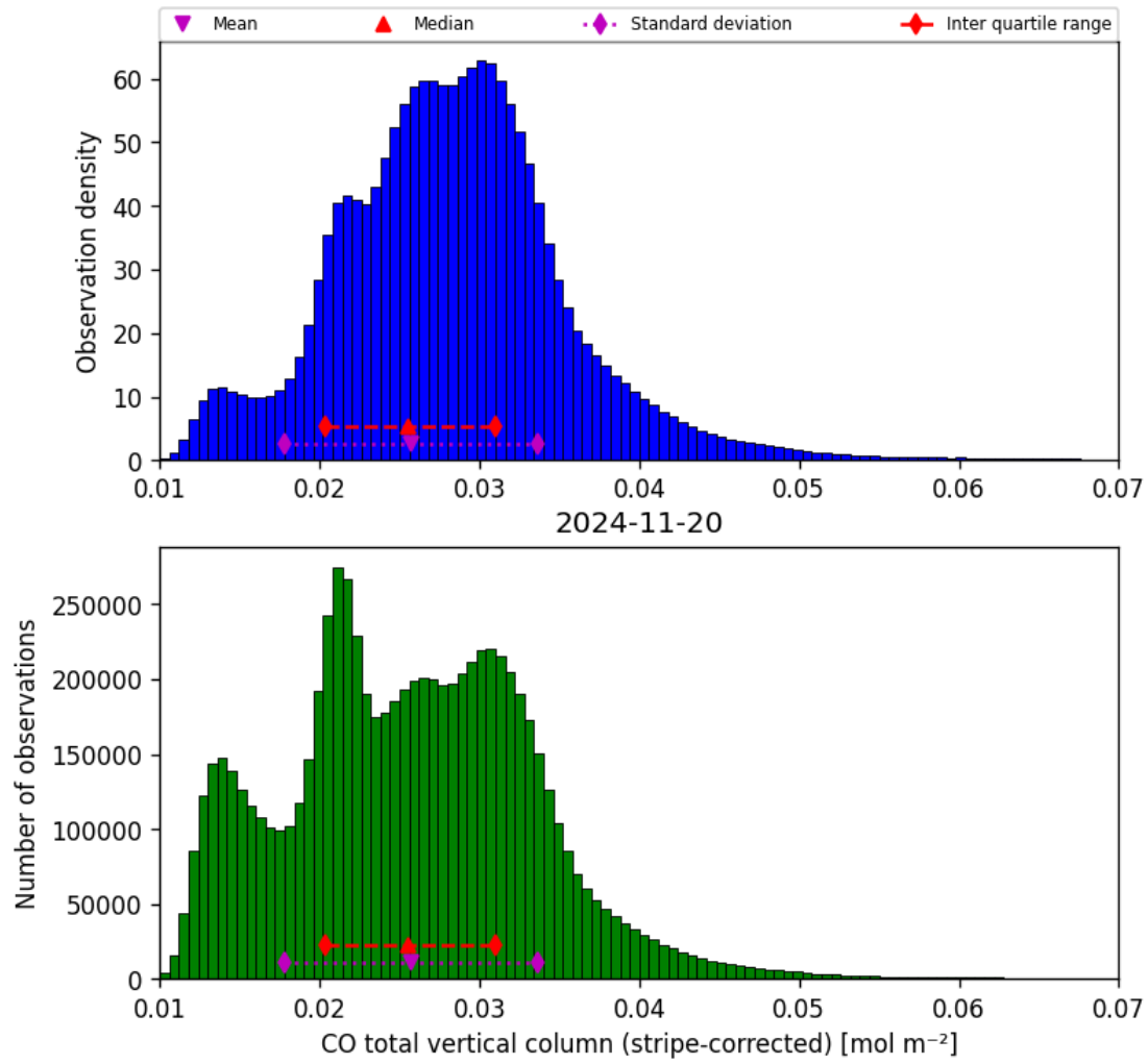
Figure 19: Histogram of “CO total vertical column (stripe-corrected)” for 2024-11-20 to 2024-11-21
