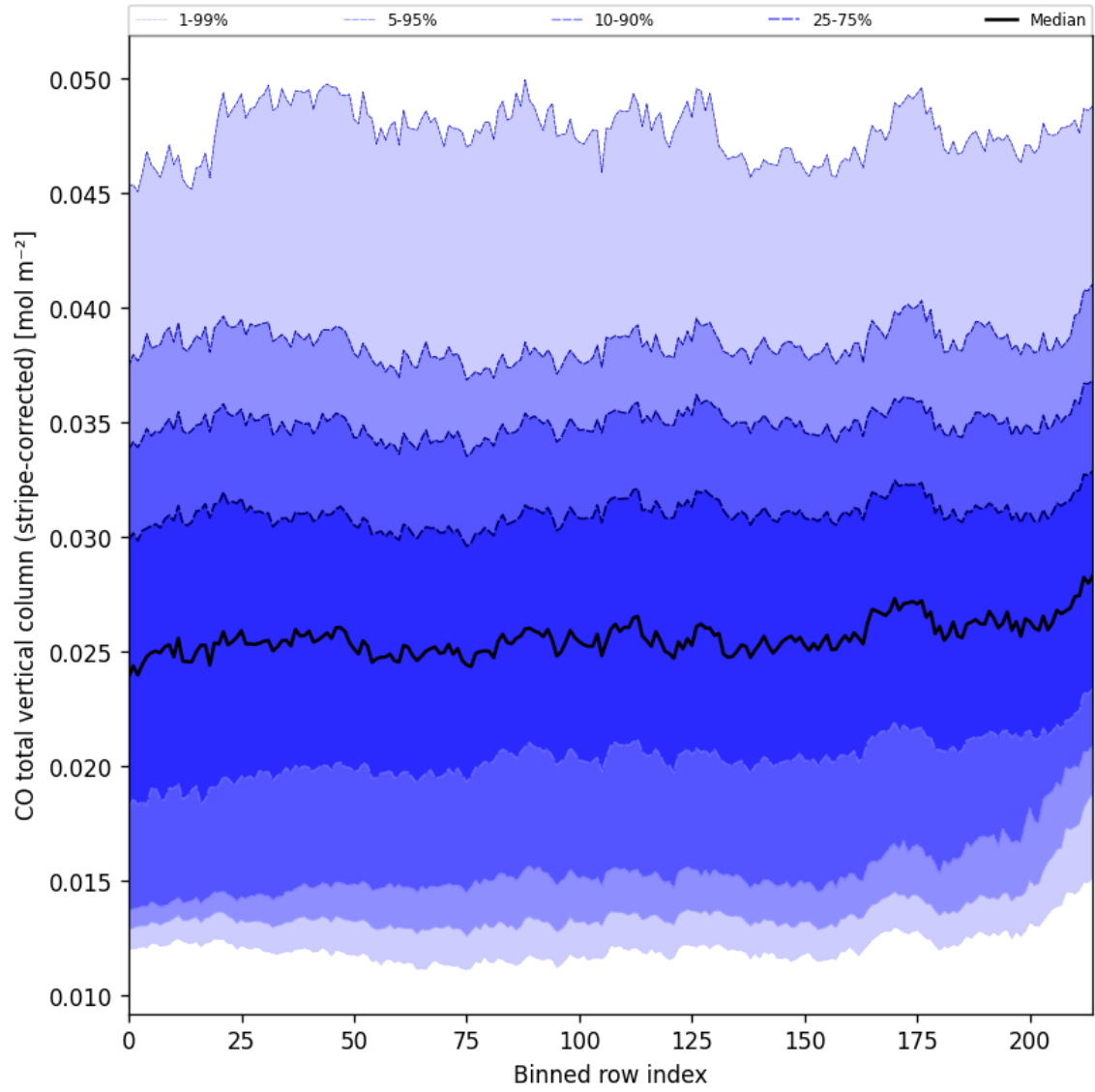
Figure 27: Along track statistics of “CO total vertical column (stripe-corrected)” for 2024-11-20 to 2024-11-21
