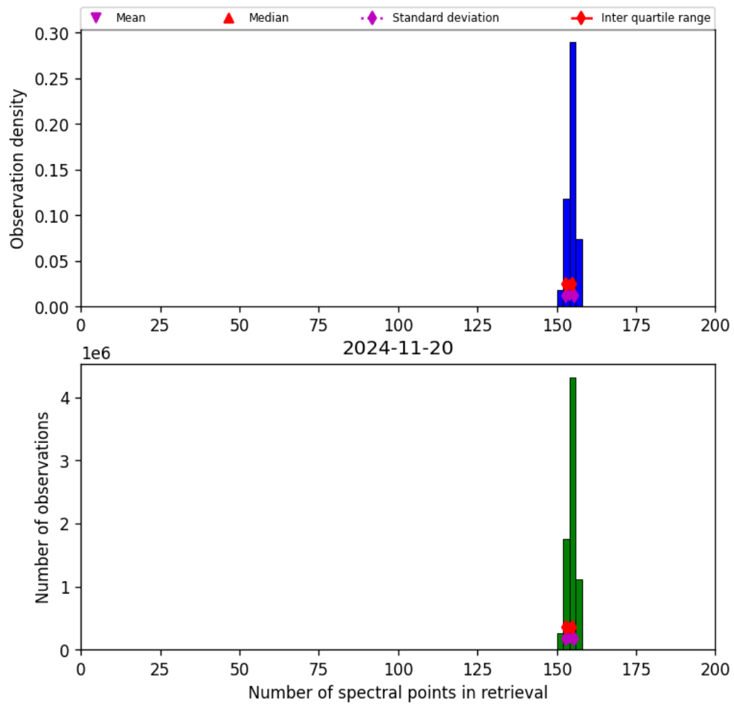
Figure 21: Histogram of “Number of spectral points in retrieval” for 2024-11-20 to 2024-11-21
