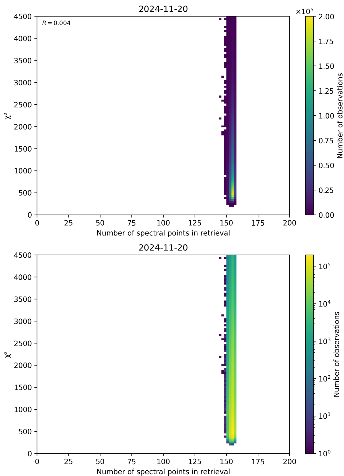
Figure 58: Scatter density plot of “Number of spectral points in retrieval” against “ \chi^2 ” for 2024-11-20 to 2024-11-21.
