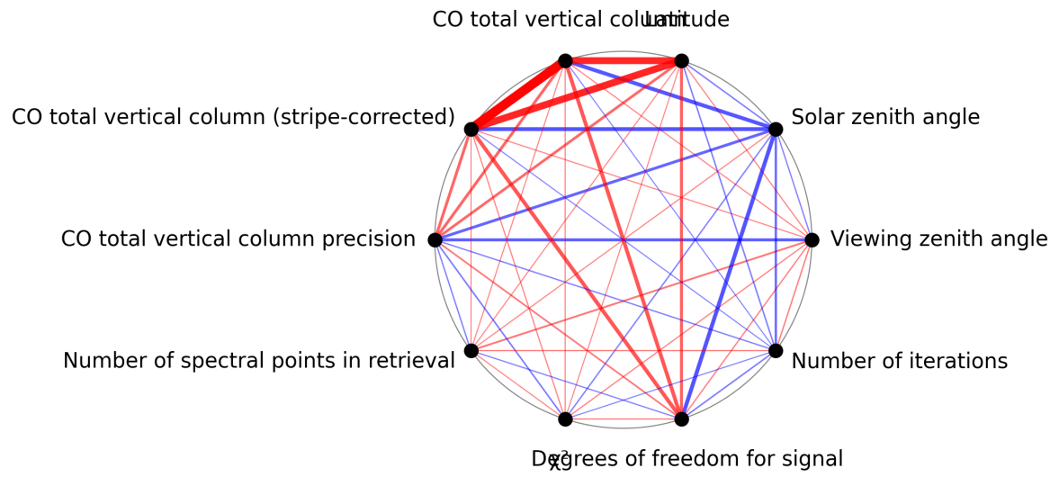
Figure 1: Map of correlation graph for 2024-11-20 to 2024-11-21.
