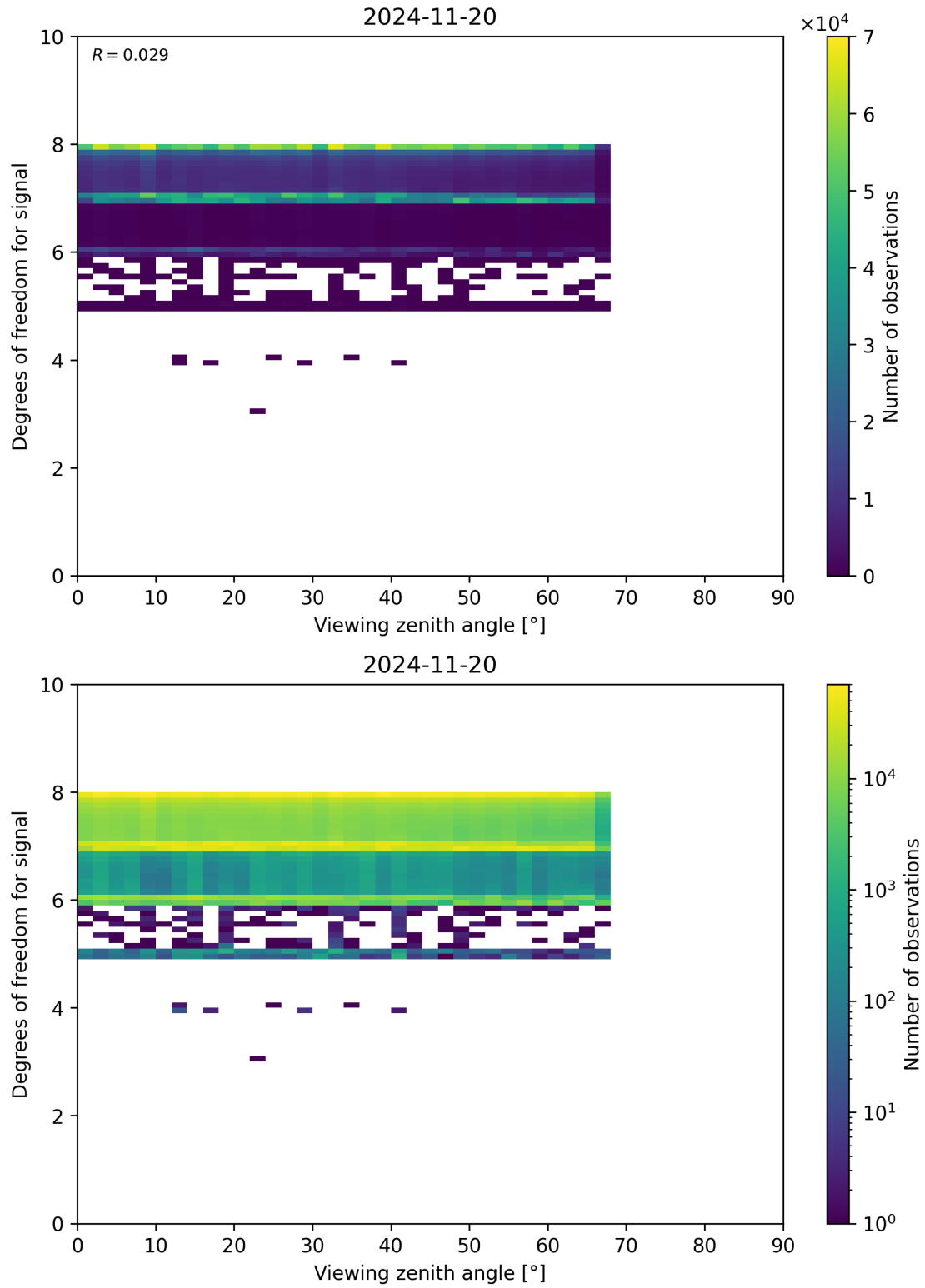
Figure 73: Scatter density plot of “Viewing zenith angle” against “Degrees of freedom for signal” for 2024-11-20 to 2024-11-21.
