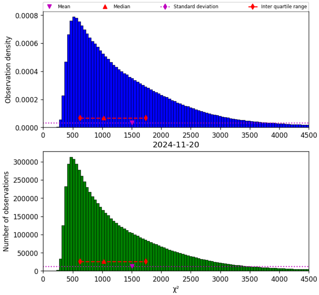
Figure 22: Histogram of “ \chi^2 ” for 2024-11-20 to 2024-11-21
