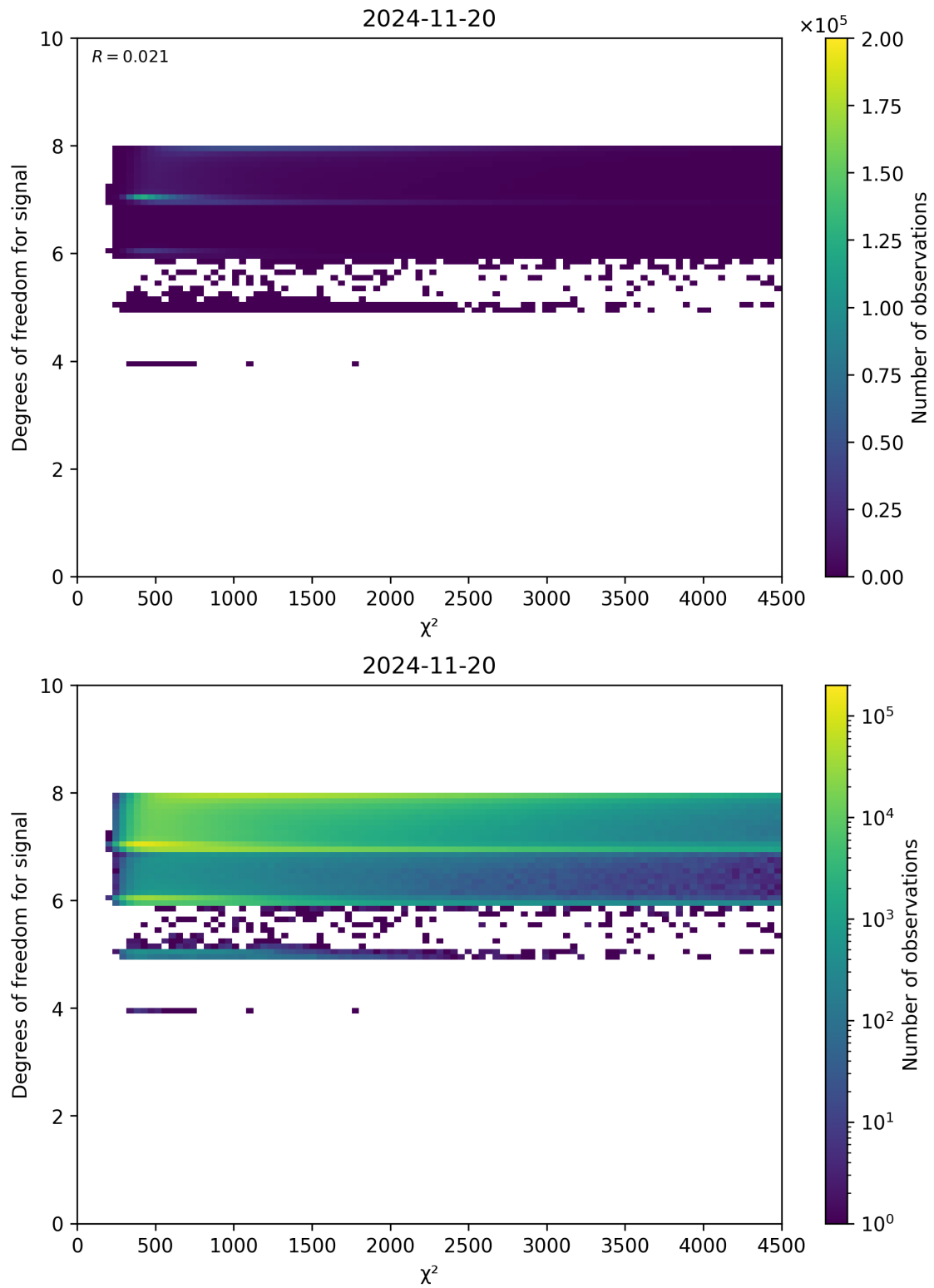
Figure 48: Scatter density plot of “ \chi^2 ” against “Degrees of freedom for signal” for 2024-11-20 to 2024-11-21.
