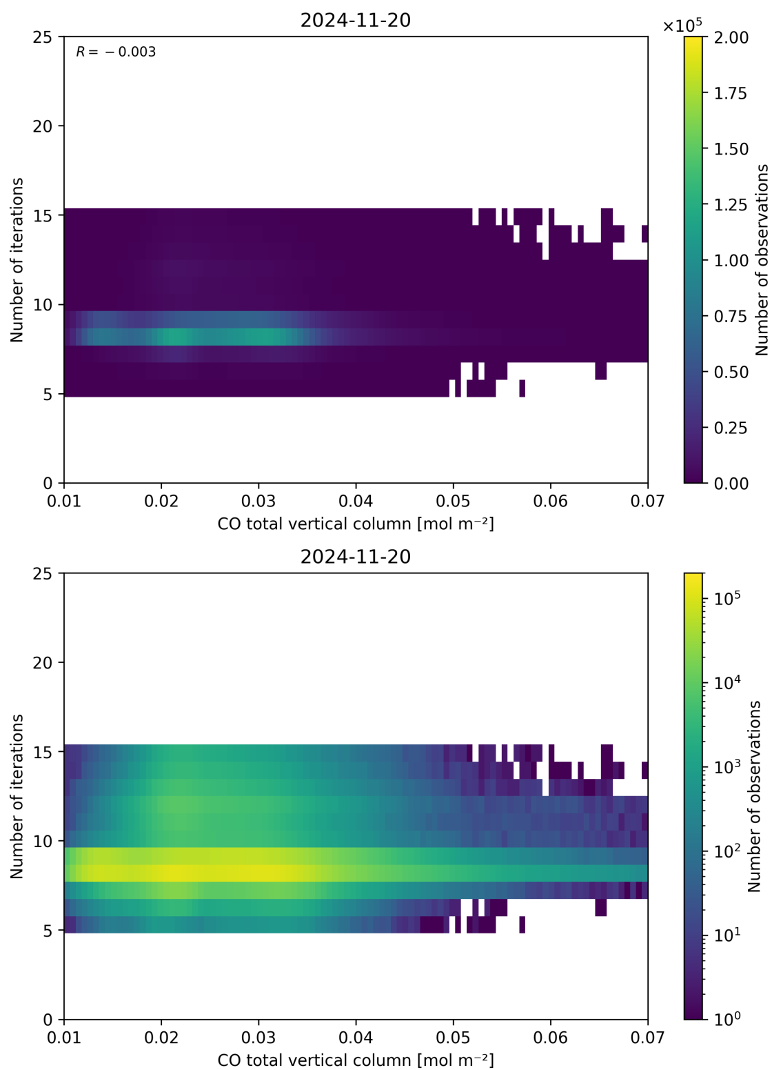
Figure 42: Scatter density plot of “CO total vertical column” against “Number of iterations” for 2024-11-20 to 2024-11-21.
