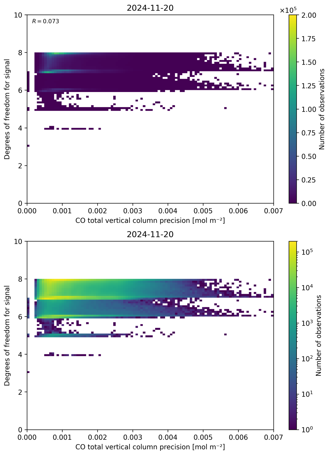
Figure 45: Scatter density plot of “CO total vertical column precision” against “Degrees of freedom for signal” for 2024-11-20 to 2024-11-21.
