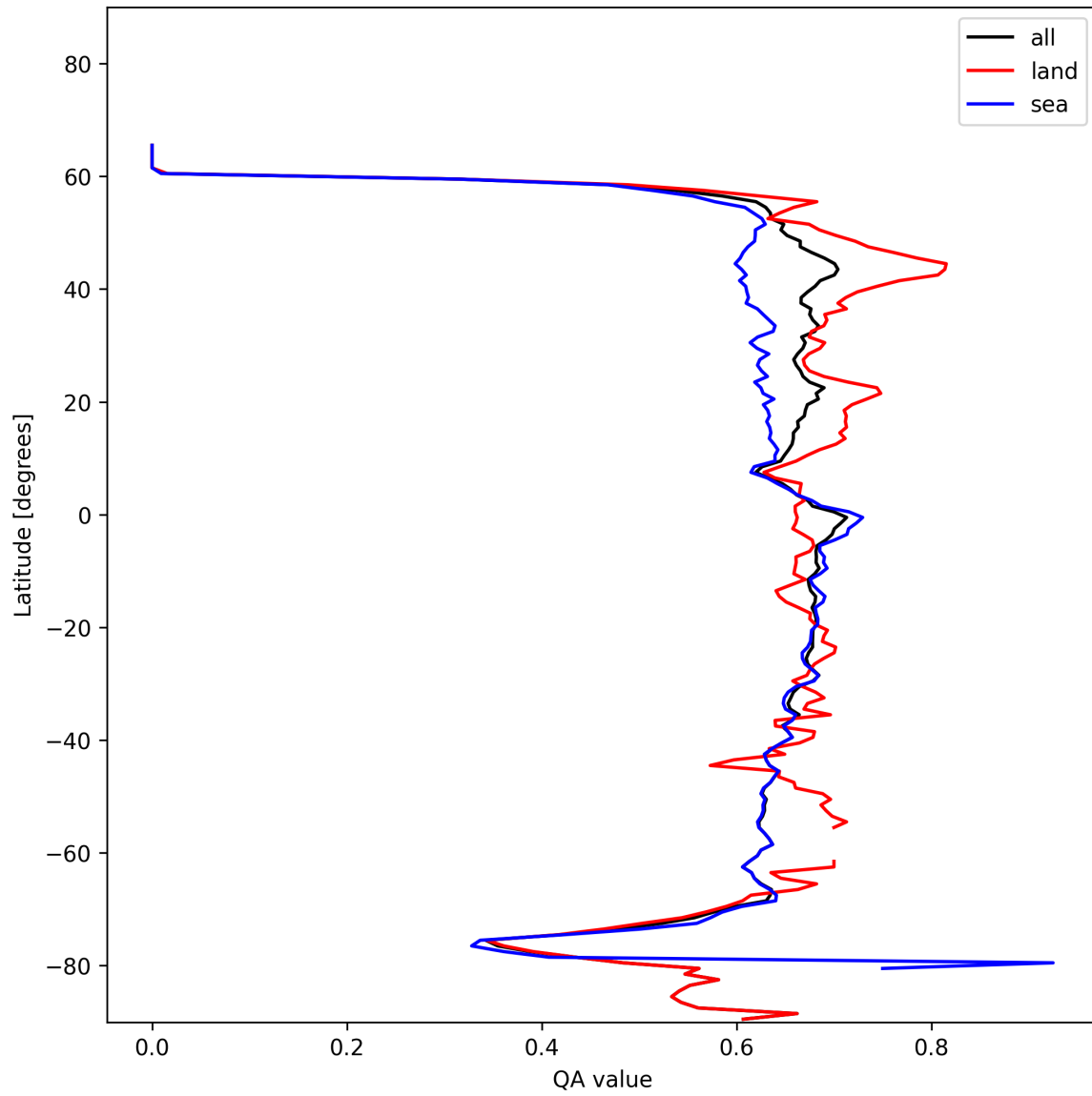
Figure 9: Zonal average of “QA value” for 2024-11-20 to 2024-11-21.
