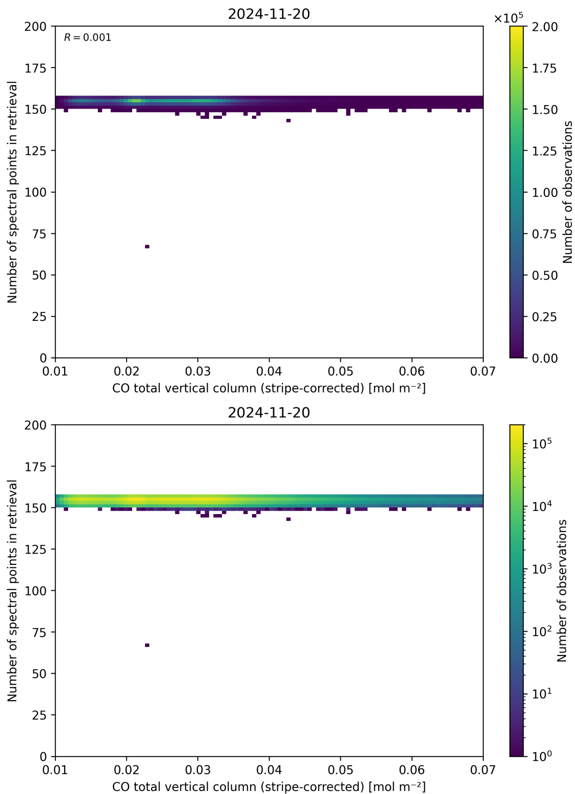
Figure 40: Scatter density plot of “CO total vertical column (stripe-corrected)” against “Number of spectral points in retrieval” for 2024-11-20 to 2024-11-21.
