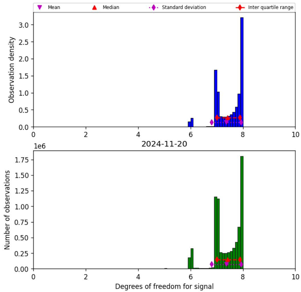
Figure 23: Histogram of “Degrees of freedom for signal” for 2024-11-20 to 2024-11-21
