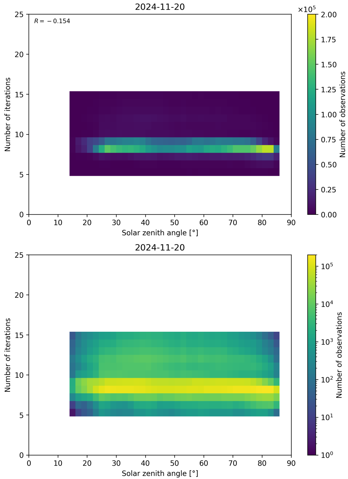
Figure 67: Scatter density plot of “Solar zenith angle” against “Number of iterations” for 2024-11-20 to 2024-11-21.
