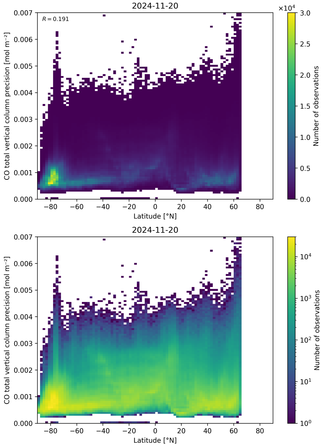
Figure 53: Scatter density plot of “Latitude” against “CO total vertical column precision” for 2024-11-20 to 2024-11-21.
