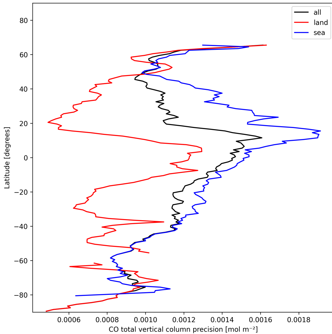
Figure 12: Zonal average of “CO total vertical column precision” for 2024-11-20 to 2024-11-21.
