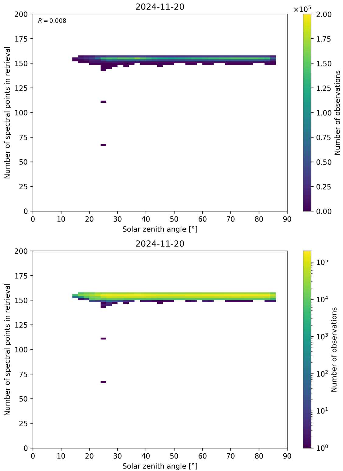
Figure 68: Scatter density plot of “Solar zenith angle” against “Number of spectral points in retrieval” for 2024-11-20 to 2024-11-21.
