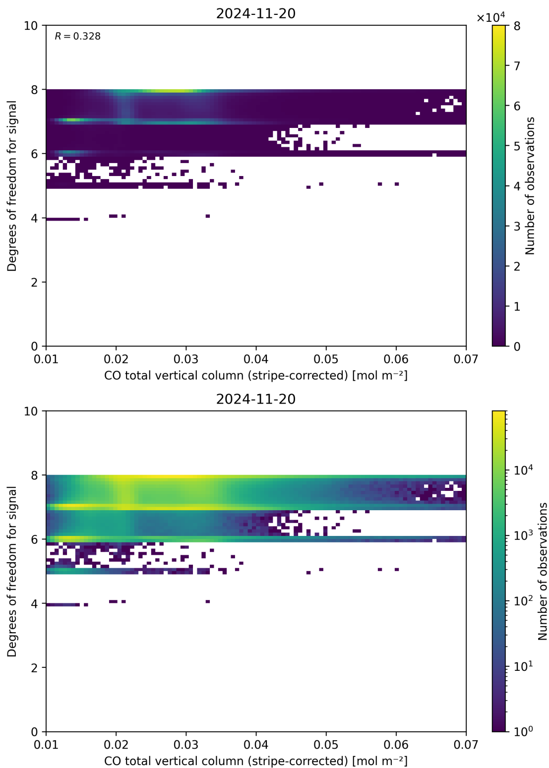
Figure 38: Scatter density plot of “CO total vertical column (stripe-corrected)” against “Degrees of freedom for signal” for 2024-11-20 to 2024-11-21.
