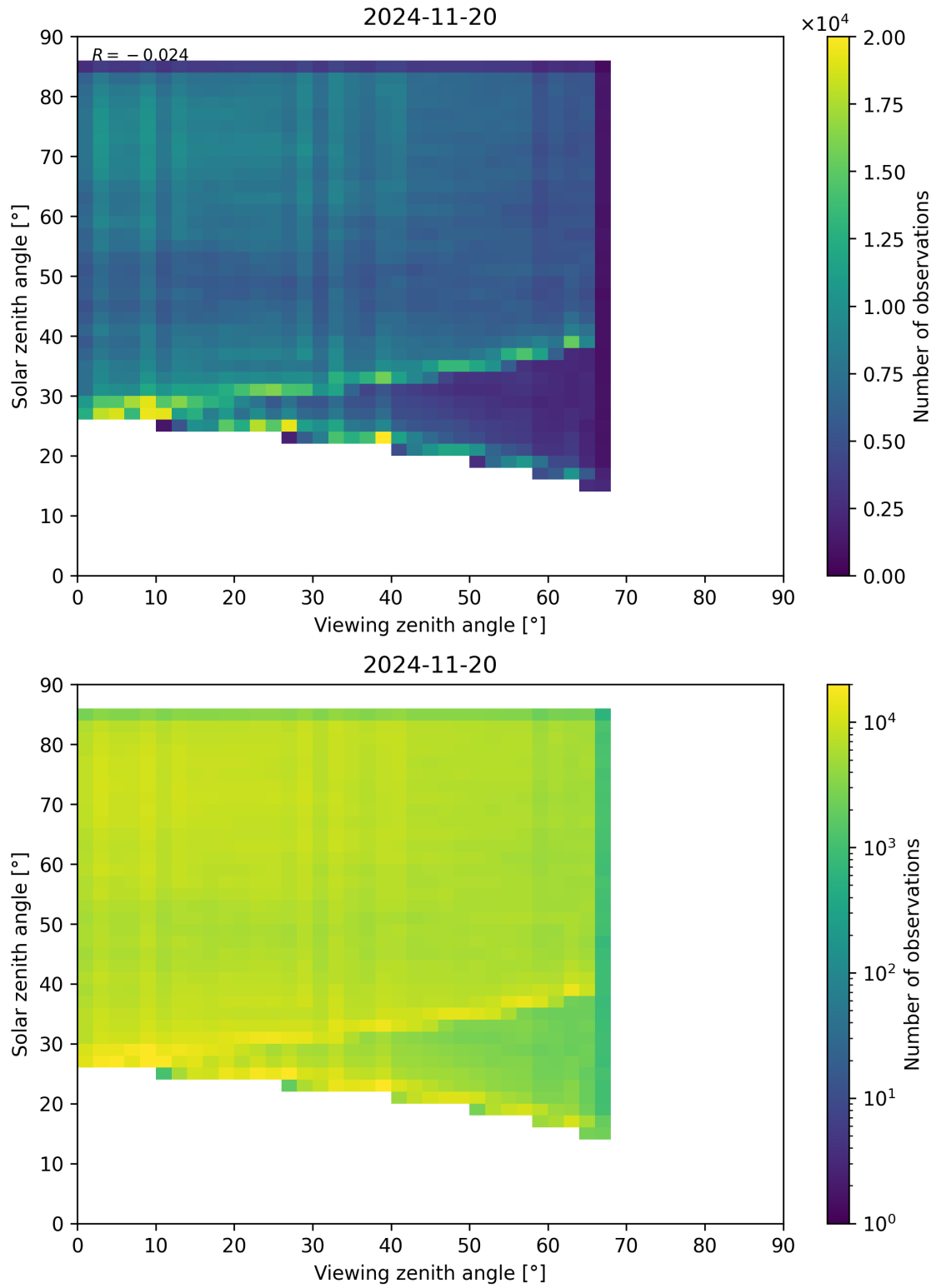
Figure 77: Scatter density plot of “Viewing zenith angle” against “Solar zenith angle” for 2024-11-20 to 2024-11-21.
