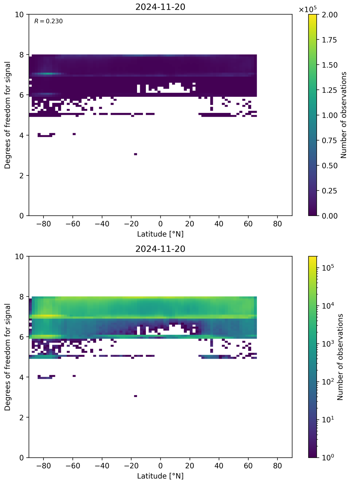
Figure 55: Scatter density plot of “Latitude” against “Degrees of freedom for signal” for 2024-11-20 to 2024-11-21.
