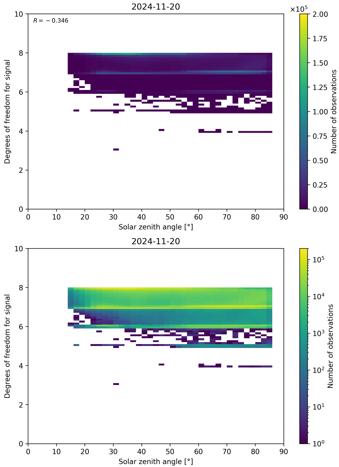
Figure 65: Scatter density plot of “Solar zenith angle” against “Degrees of freedom for signal” for 2024-11-20 to 2024-11-21.
