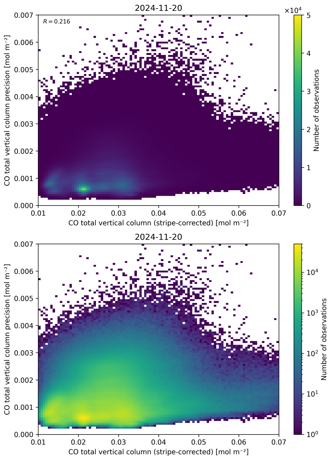
Figure 36: Scatter density plot of “CO total vertical column (stripe-corrected)” against “CO total vertical column precision” for 2024-11-20 to 2024-11-21.
