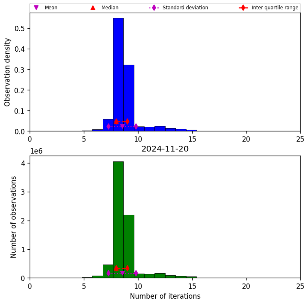
Figure 24: Histogram of “Number of iterations” for 2024-11-20 to 2024-11-21
