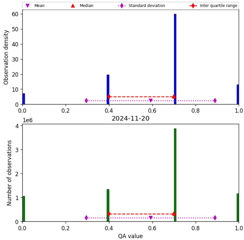
Figure 17: Histogram of “QA value” for 2024-11-20 to 2024-11-21
