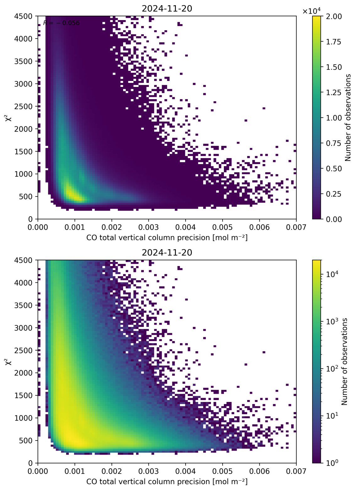
Figure 44: Scatter density plot of “CO total vertical column precision” against “ \chi^2 ” for 2024-11-20 to 2024-11-21.
