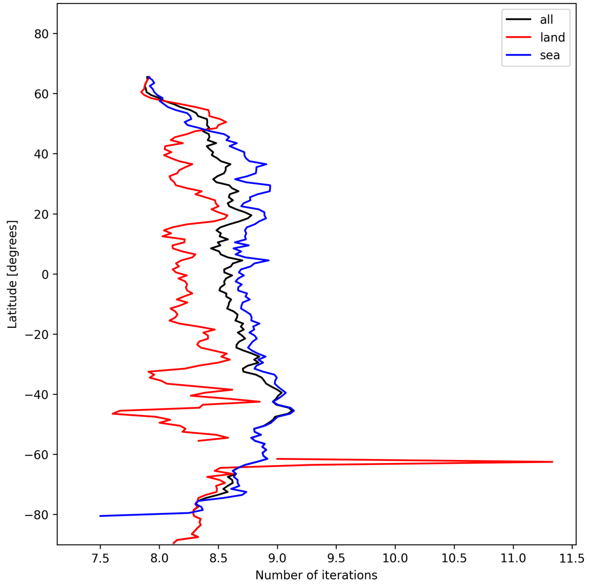
Figure 16: Zonal average of “Number of iterations” for 2024-11-20 to 2024-11-21.
