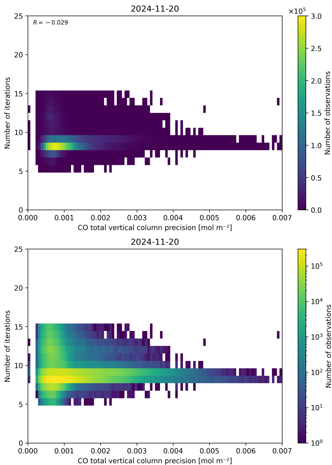
Figure 46: Scatter density plot of “CO total vertical column precision” against “Number of iterations” for 2024-11-20 to 2024-11-21.
