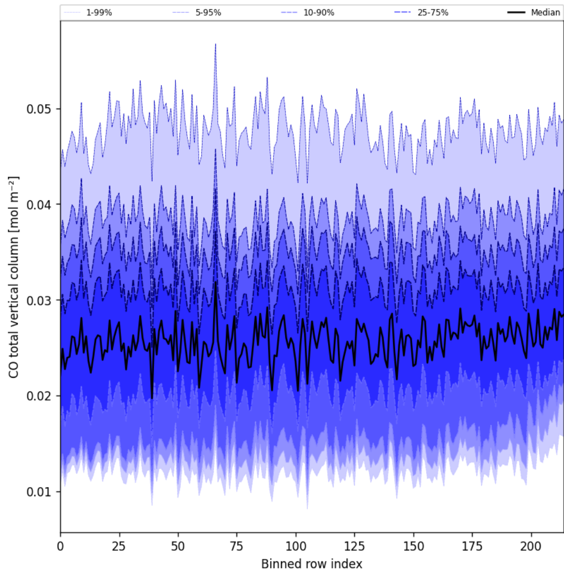
Figure 26: Along track statistics of “CO total vertical column” for 2024-11-20 to 2024-11-21
