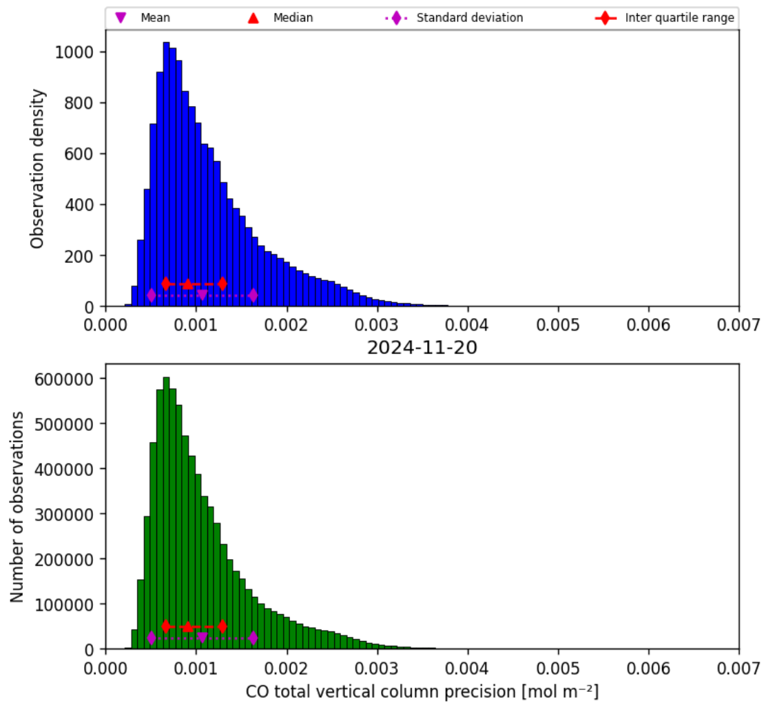
Figure 20: Histogram of “CO total vertical column precision” for 2024-11-20 to 2024-11-21
