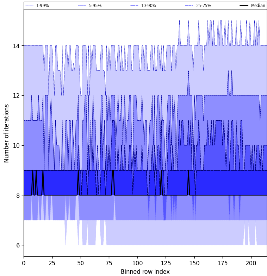
Figure 32: Along track statistics of “Number of iterations” for 2024-11-20 to 2024-11-21
