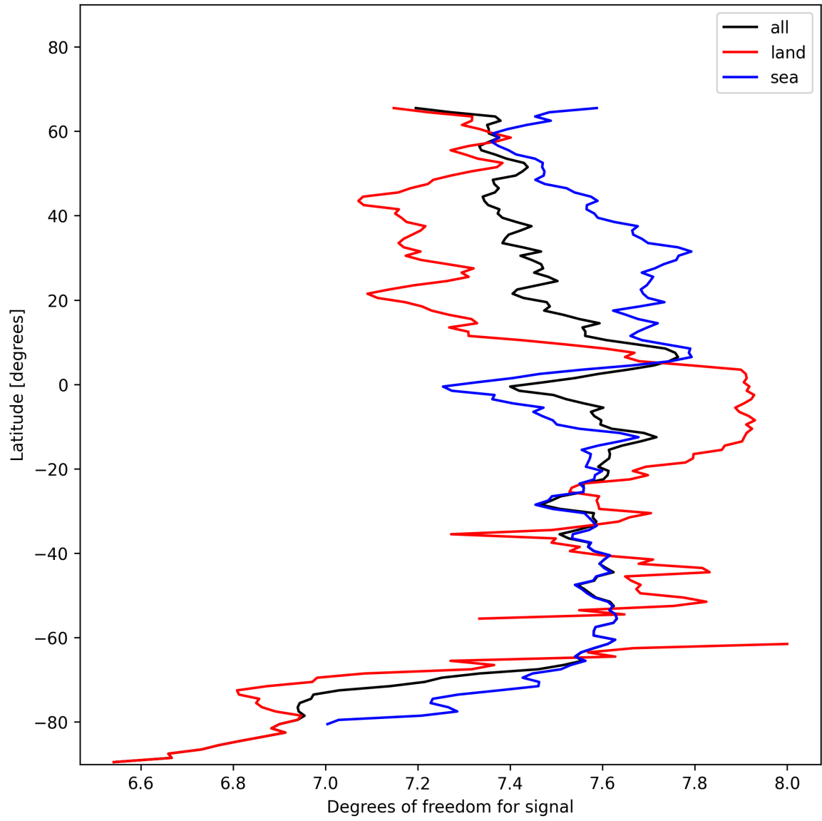
Figure 15: Zonal average of “Degrees of freedom for signal” for 2024-11-20 to 2024-11-21.
