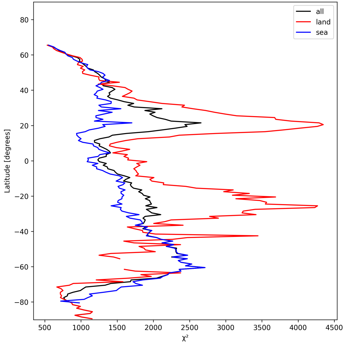
Figure 14: Zonal average of “ \chi^2 ” for 2024-11-20 to 2024-11-21.
