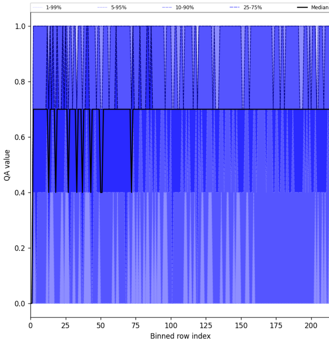
Figure 25: Along track statistics of “QA value” for 2024-11-20 to 2024-11-21
