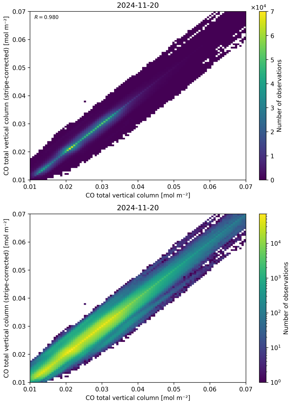
Figure 33: Scatter density plot of “CO total vertical column” against “CO total vertical column (stripe-corrected)” for 2024-11-20 to 2024-11-21.
