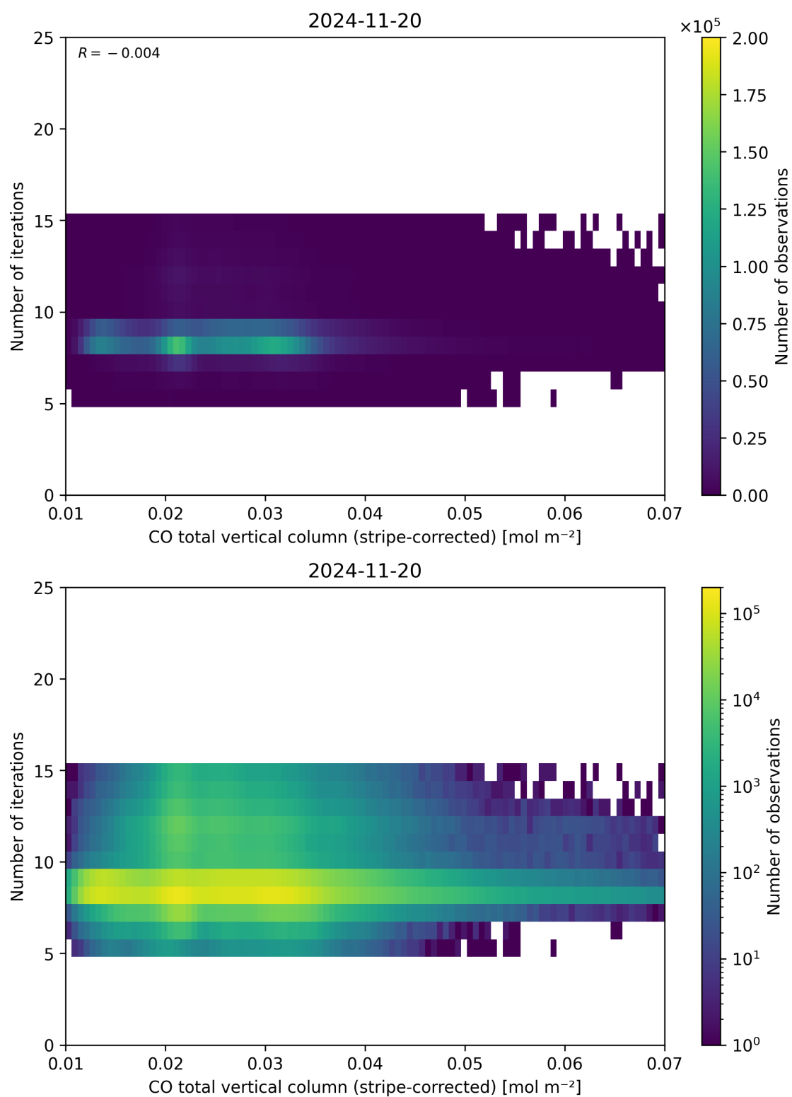
Figure 39: Scatter density plot of “CO total vertical column (stripe-corrected)” against “Number of iterations” for 2024-11-20 to 2024-11-21.
