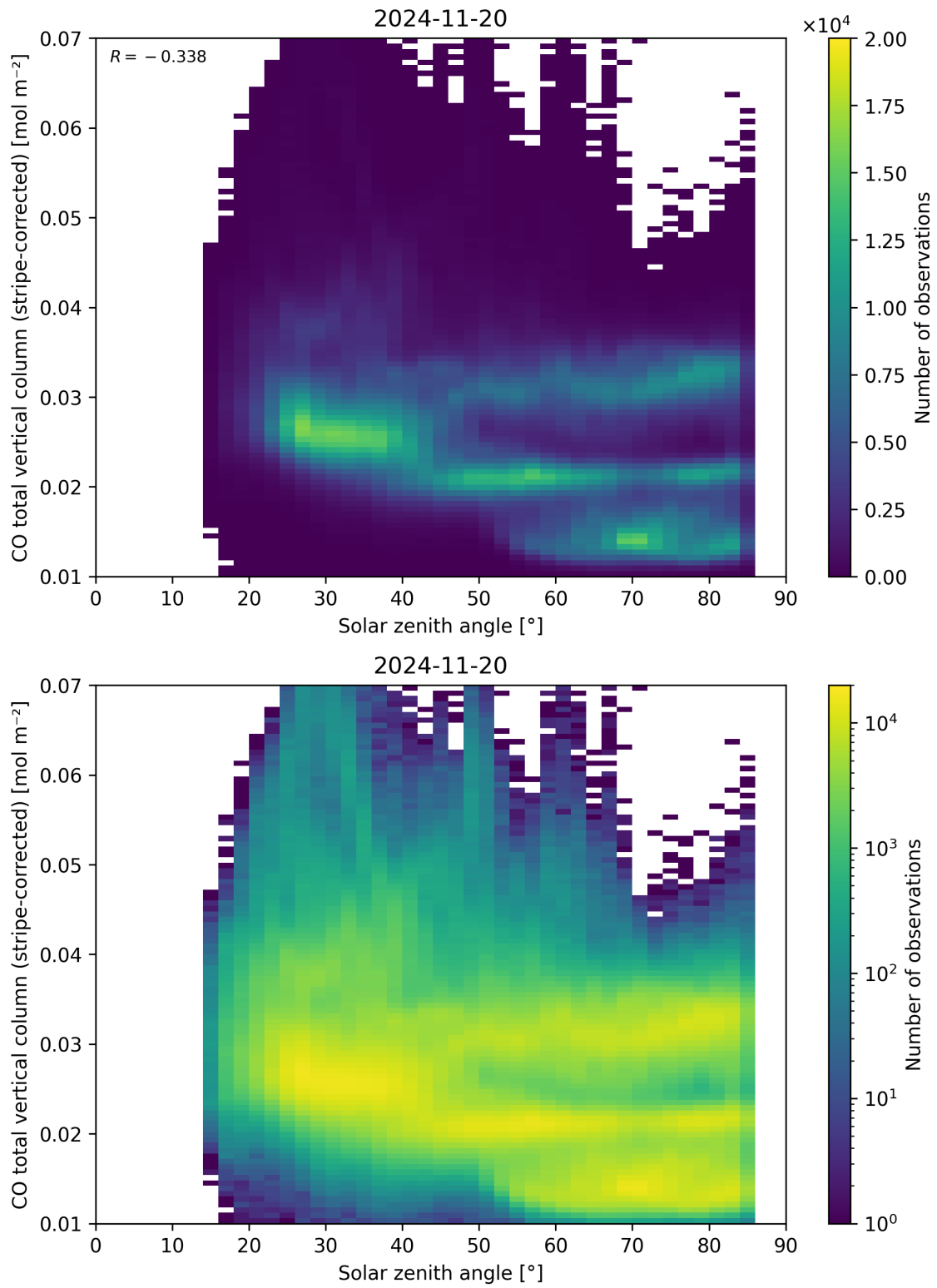
Figure 62: Scatter density plot of “Solar zenith angle” against “CO total vertical column (stripe-corrected)” for 2024-11-20 to 2024-11-21.
