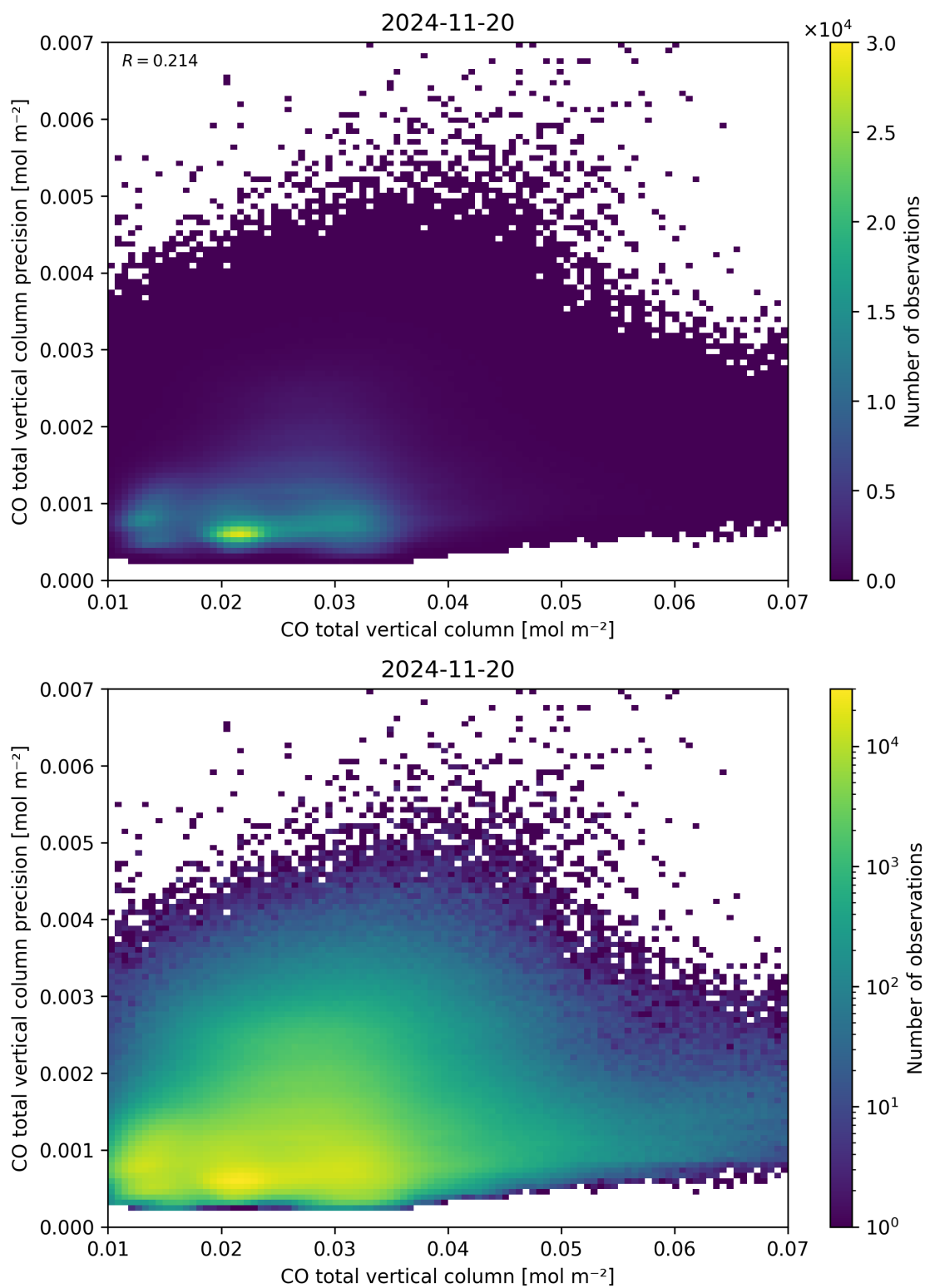
Figure 34: Scatter density plot of “CO total vertical column” against “CO total vertical column precision” for 2024-11-20 to 2024-11-21.
