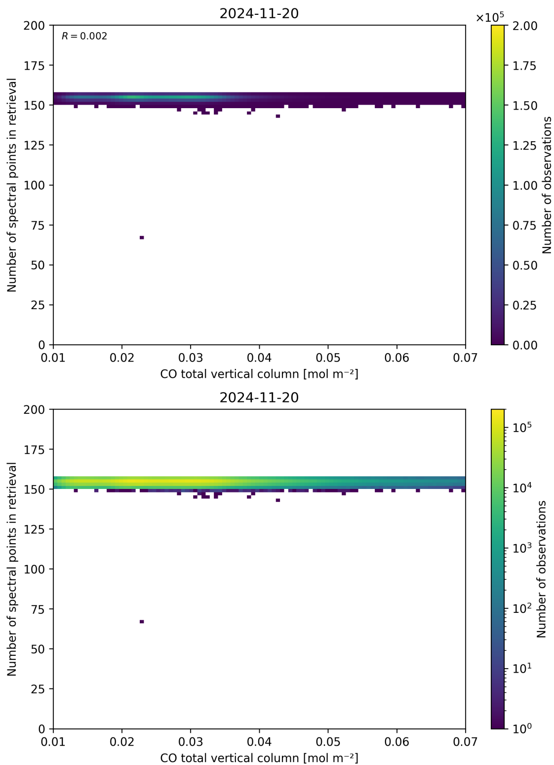
Figure 43: Scatter density plot of “CO total vertical column” against “Number of spectral points in retrieval” for 2024-11-20 to 2024-11-21.
