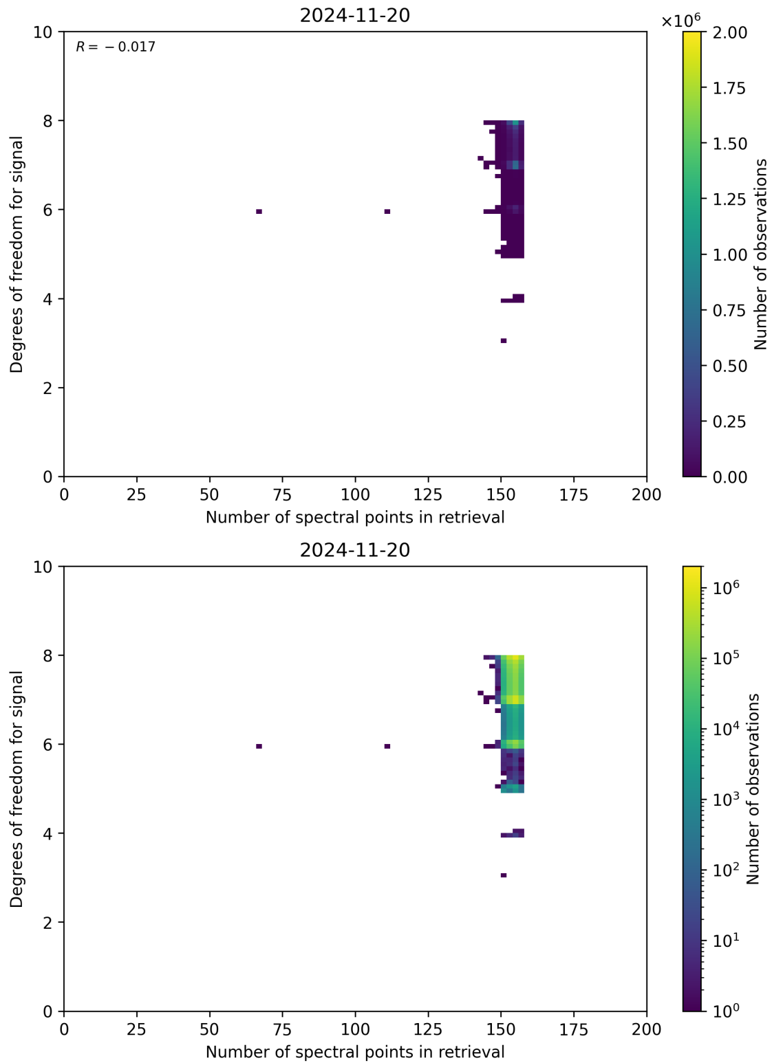
Figure 59: Scatter density plot of “Number of spectral points in retrieval” against “Degrees of freedom for signal” for 2024-11-20 to 2024-11-21.
