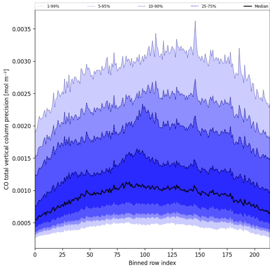
Figure 28: Along track statistics of “CO total vertical column precision” for 2024-11-20 to 2024-11-21
