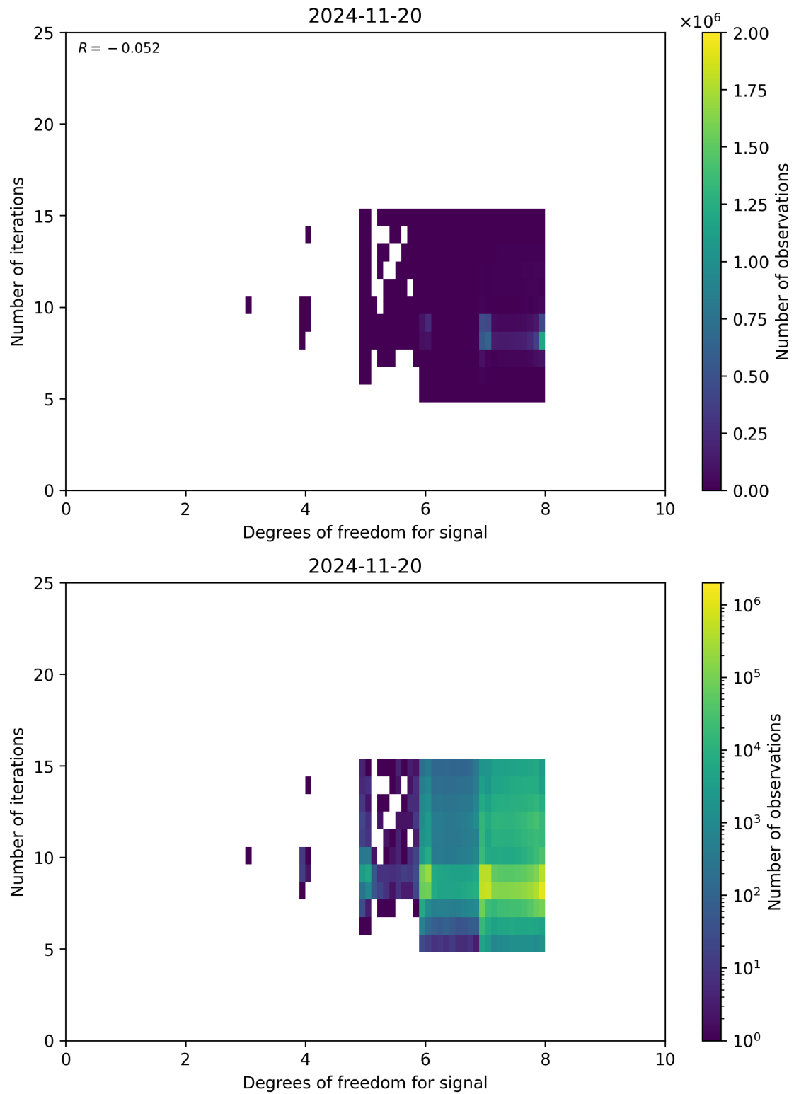
Figure 50: Scatter density plot of “Degrees of freedom for signal” against “Number of iterations” for 2024-11-20 to 2024-11-21.
