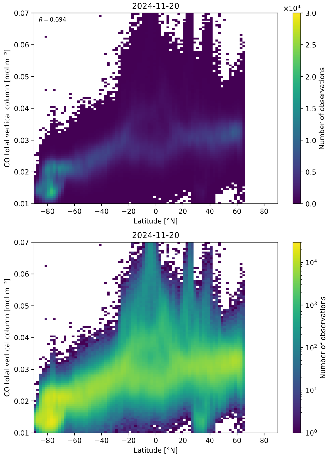
Figure 51: Scatter density plot of “Latitude” against “CO total vertical column” for 2024-11-20 to 2024-11-21.
