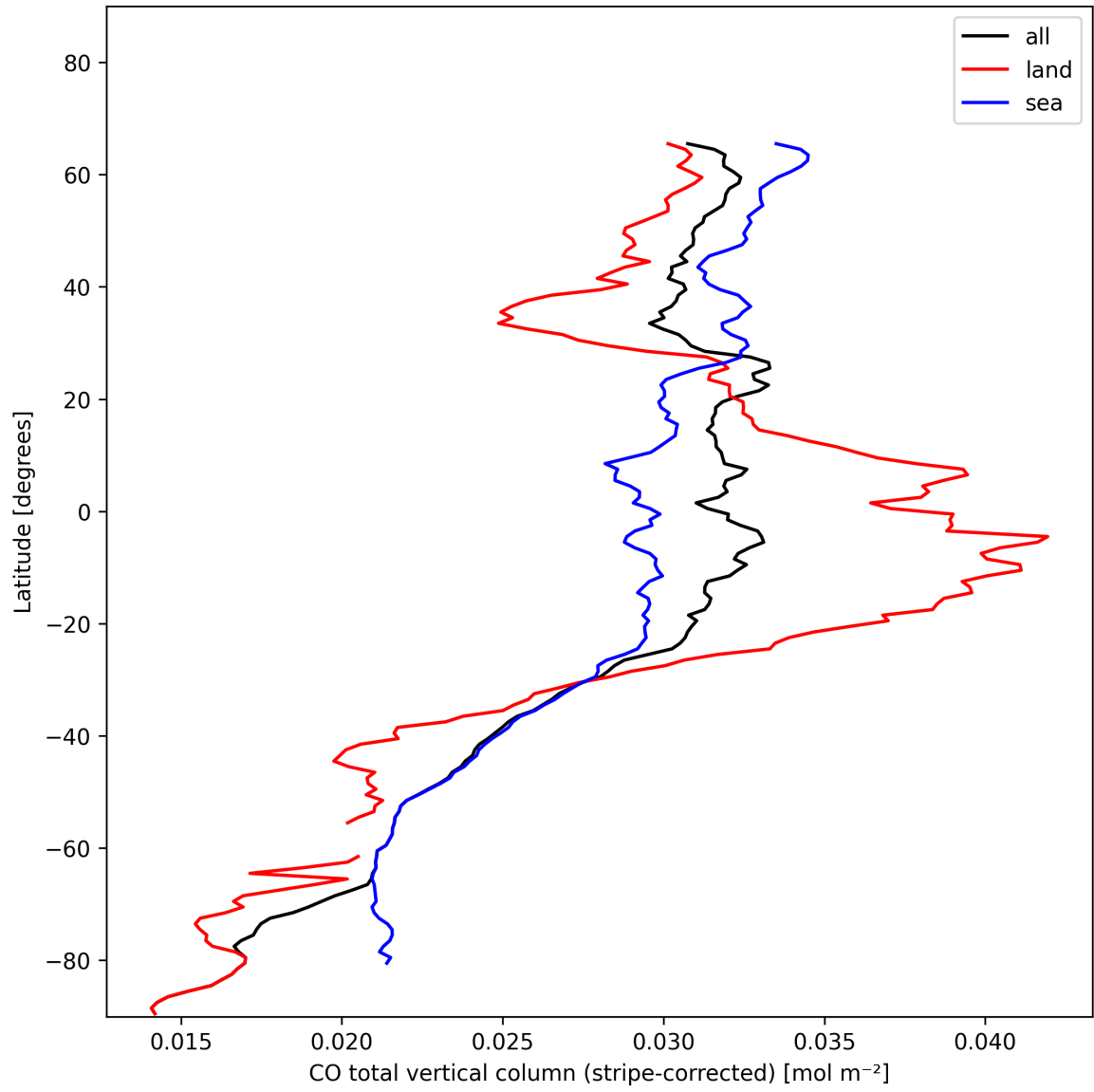
Figure 11: Zonal average of “CO total vertical column (stripe-corrected)” for 2024-11-20 to 2024-11-21.
