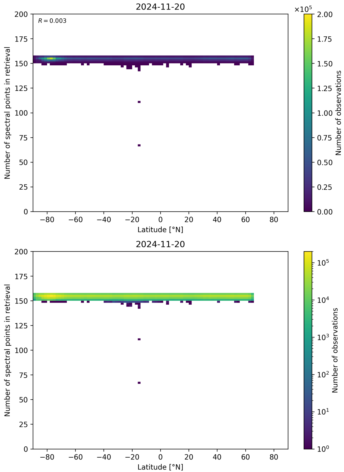
Figure 57: Scatter density plot of “Latitude” against “Number of spectral points in retrieval” for 2024-11-20 to 2024-11-21.
