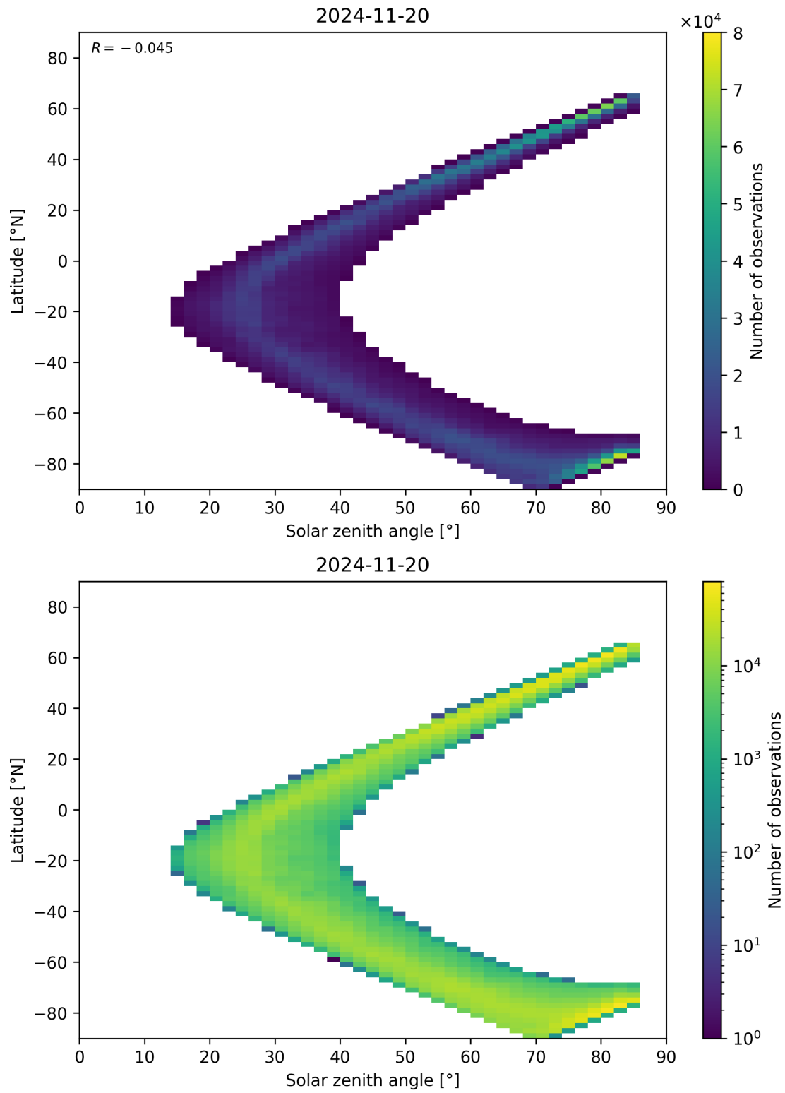
Figure 66: Scatter density plot of “Solar zenith angle” against “Latitude” for 2024-11-20 to 2024-11-21.
