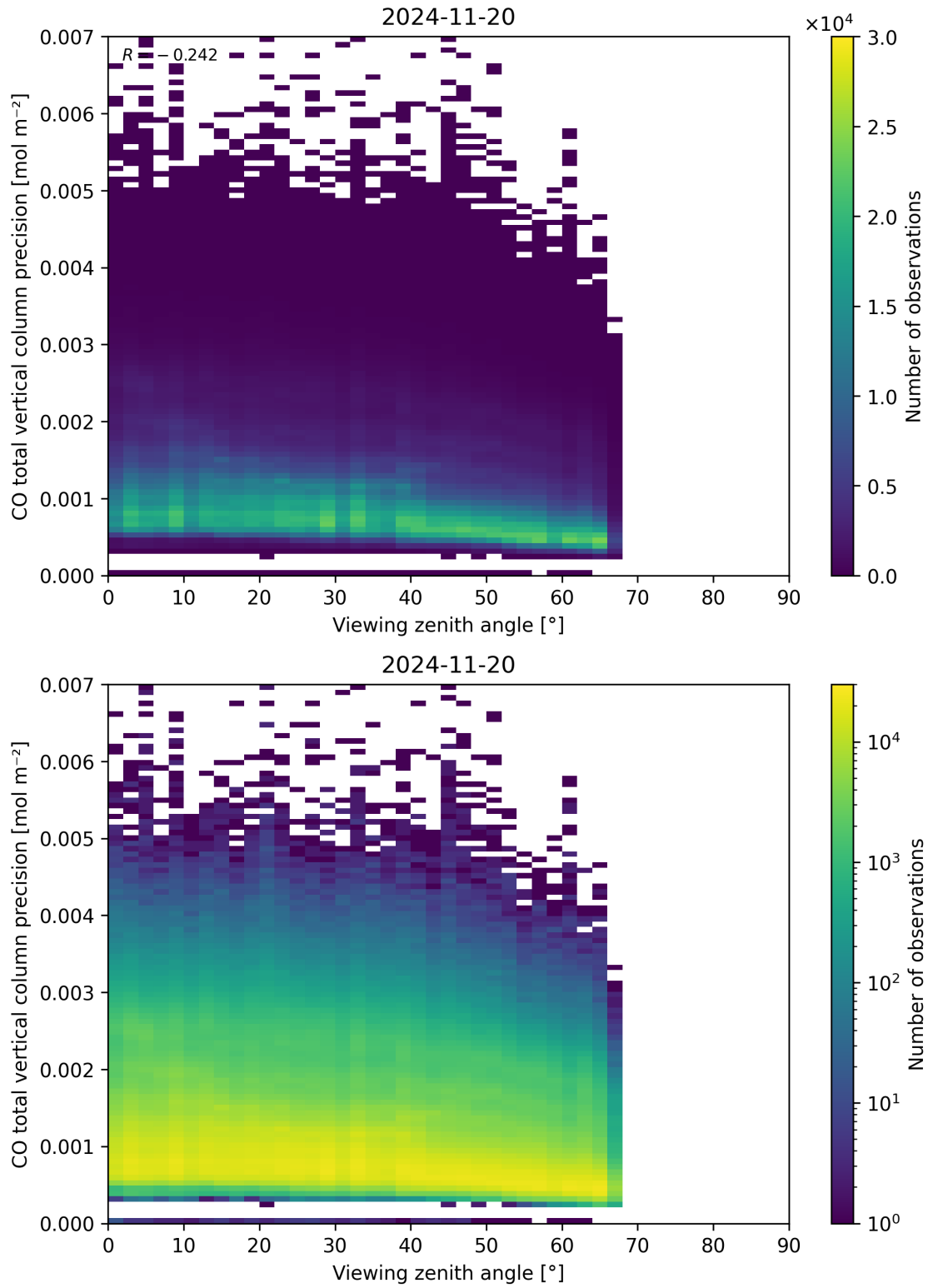
Figure 71: Scatter density plot of “Viewing zenith angle” against “CO total vertical column precision” for 2024-11-20 to 2024-11-21.
