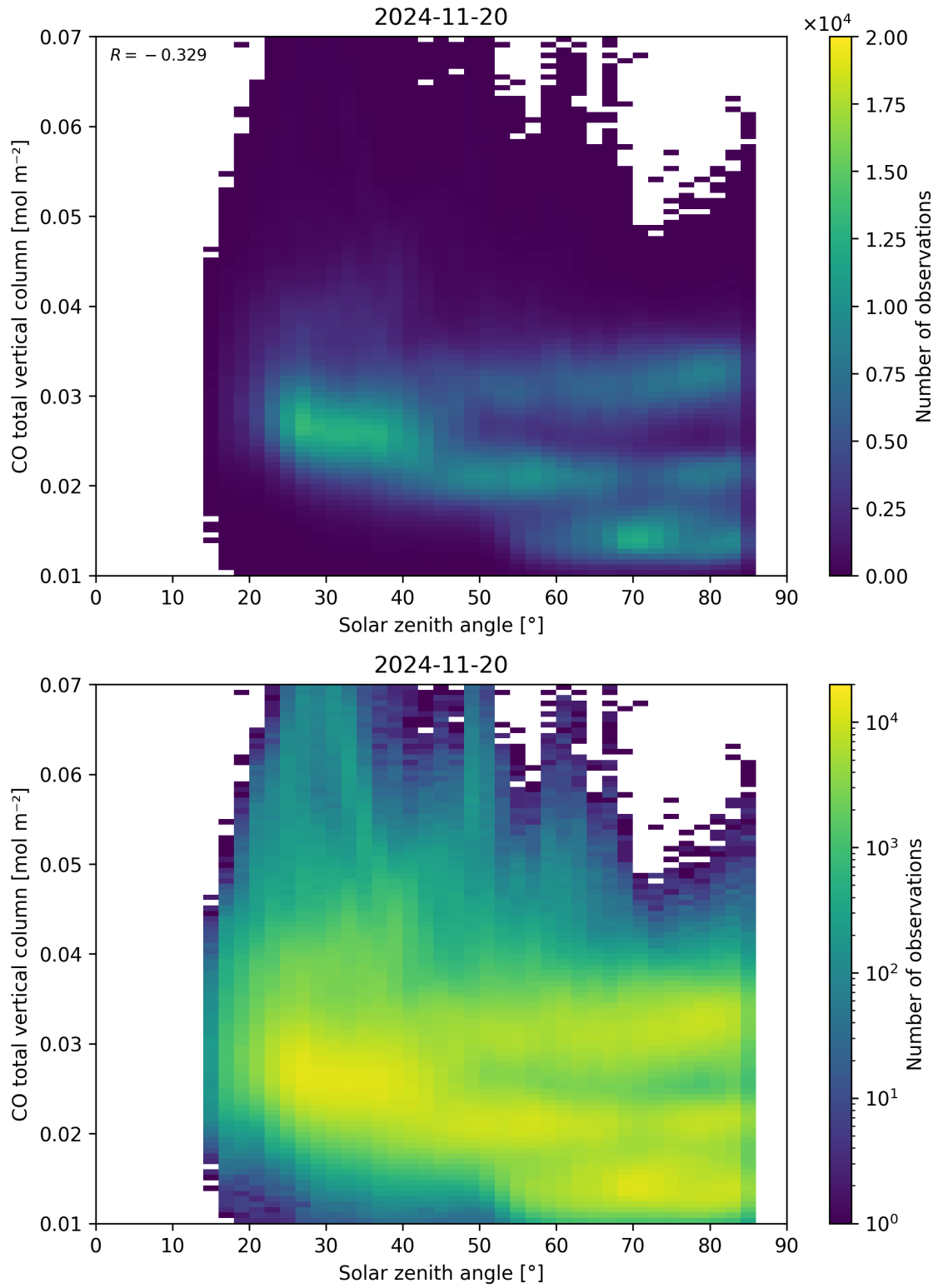
Figure 61: Scatter density plot of “Solar zenith angle” against “CO total vertical column” for 2024-11-20 to 2024-11-21.
