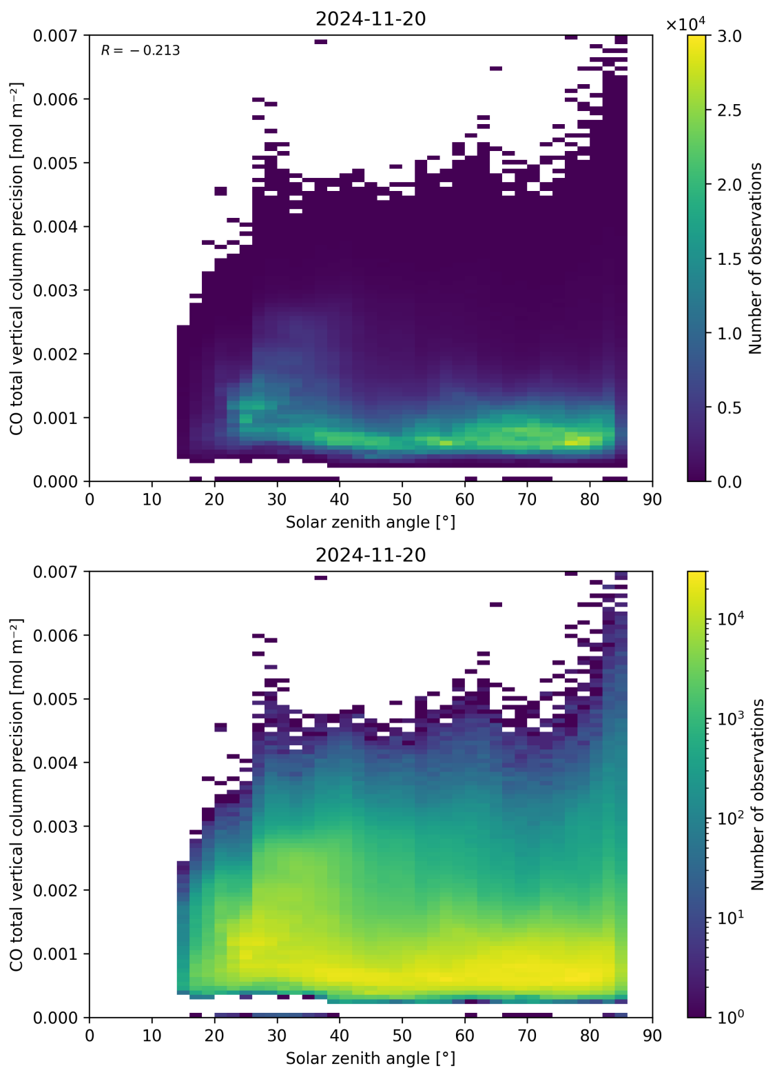
Figure 63: Scatter density plot of “Solar zenith angle” against “CO total vertical column precision” for 2024-11-20 to 2024-11-21.
