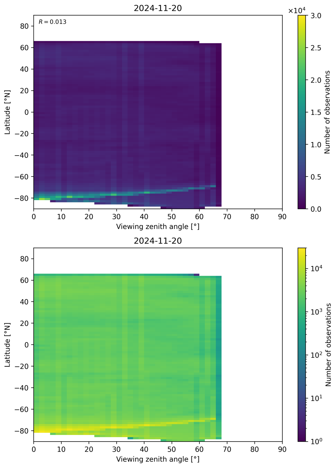
Figure 74: Scatter density plot of “Viewing zenith angle” against “Latitude” for 2024-11-20 to 2024-11-21.
