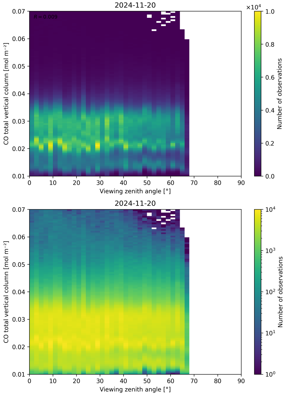
Figure 69: Scatter density plot of “Viewing zenith angle” against “CO total vertical column” for 2024-11-20 to 2024-11-21.
