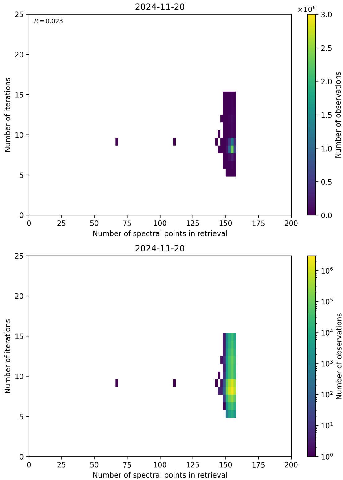
Figure 60: Scatter density plot of “Number of spectral points in retrieval” against “Number of iterations” for 2024-11-20 to 2024-11-21.
