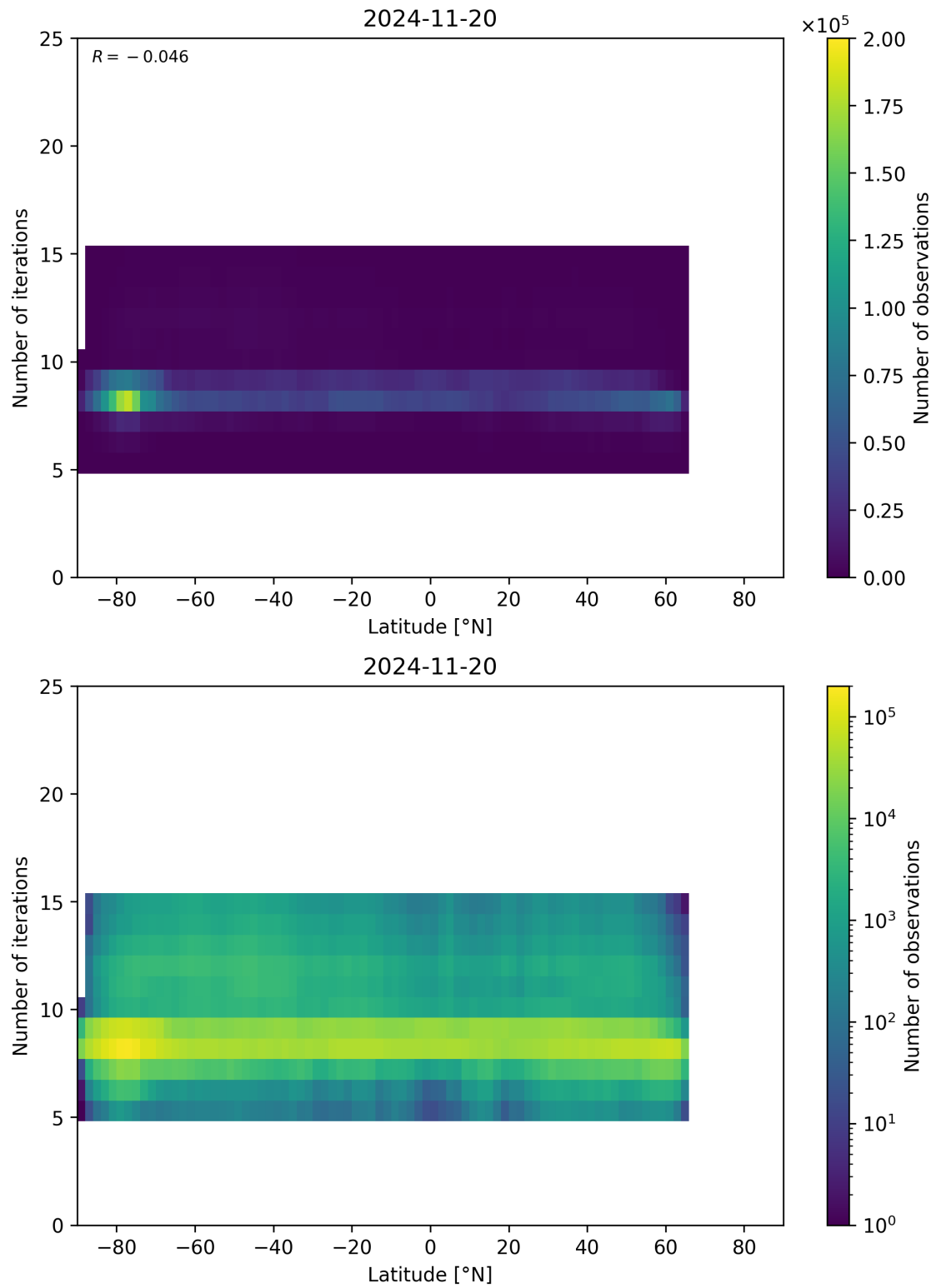
Figure 56: Scatter density plot of “Latitude” against “Number of iterations” for 2024-11-20 to 2024-11-21.
