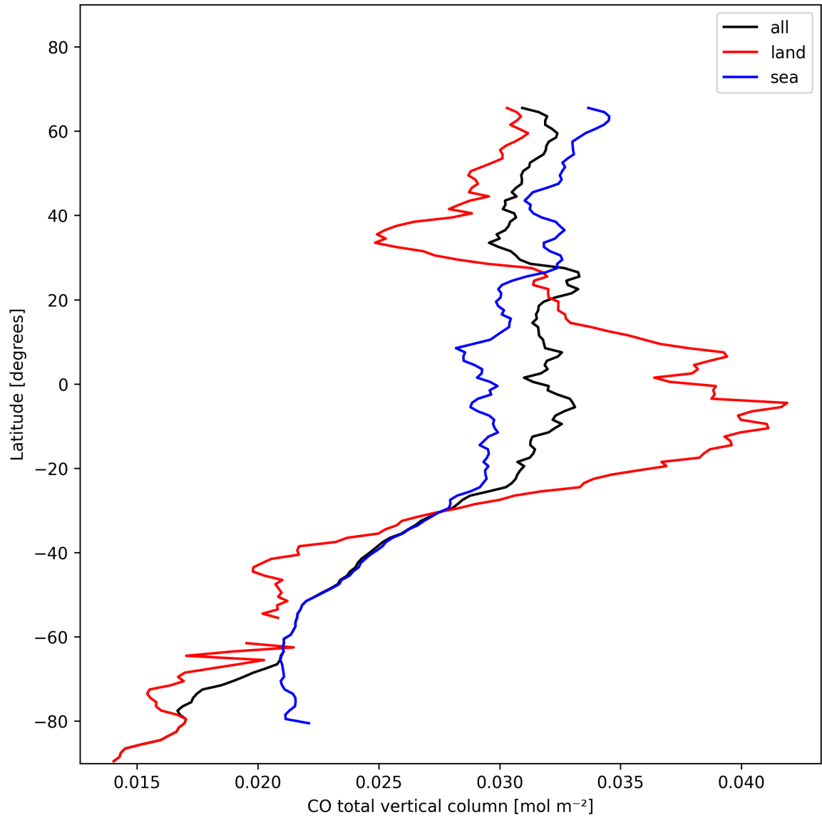
Figure 10: Zonal average of “CO total vertical column” for 2024-11-20 to 2024-11-21.
