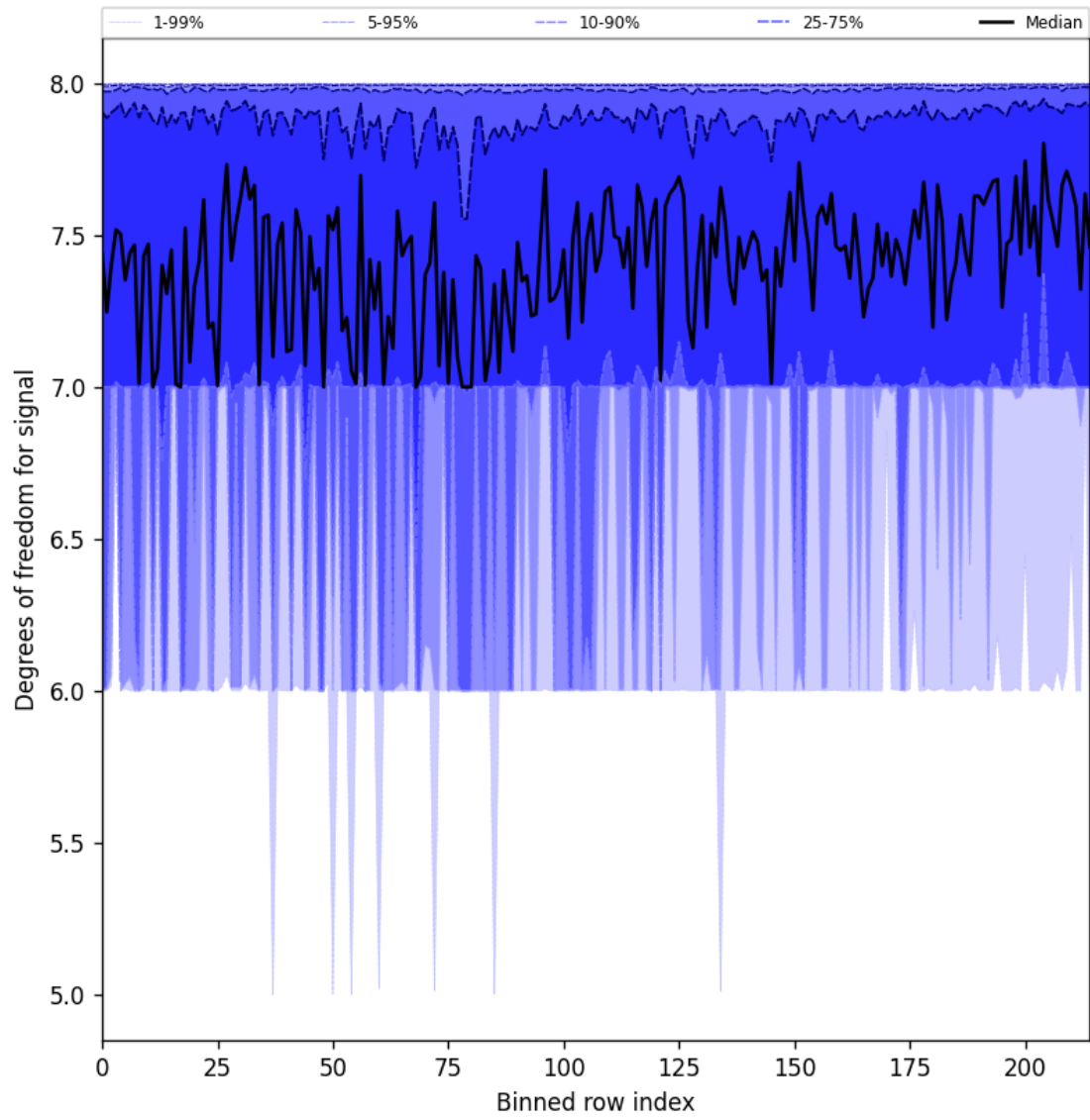
Figure 31: Along track statistics of “Degrees of freedom for signal” for 2024-11-20 to 2024-11-21
