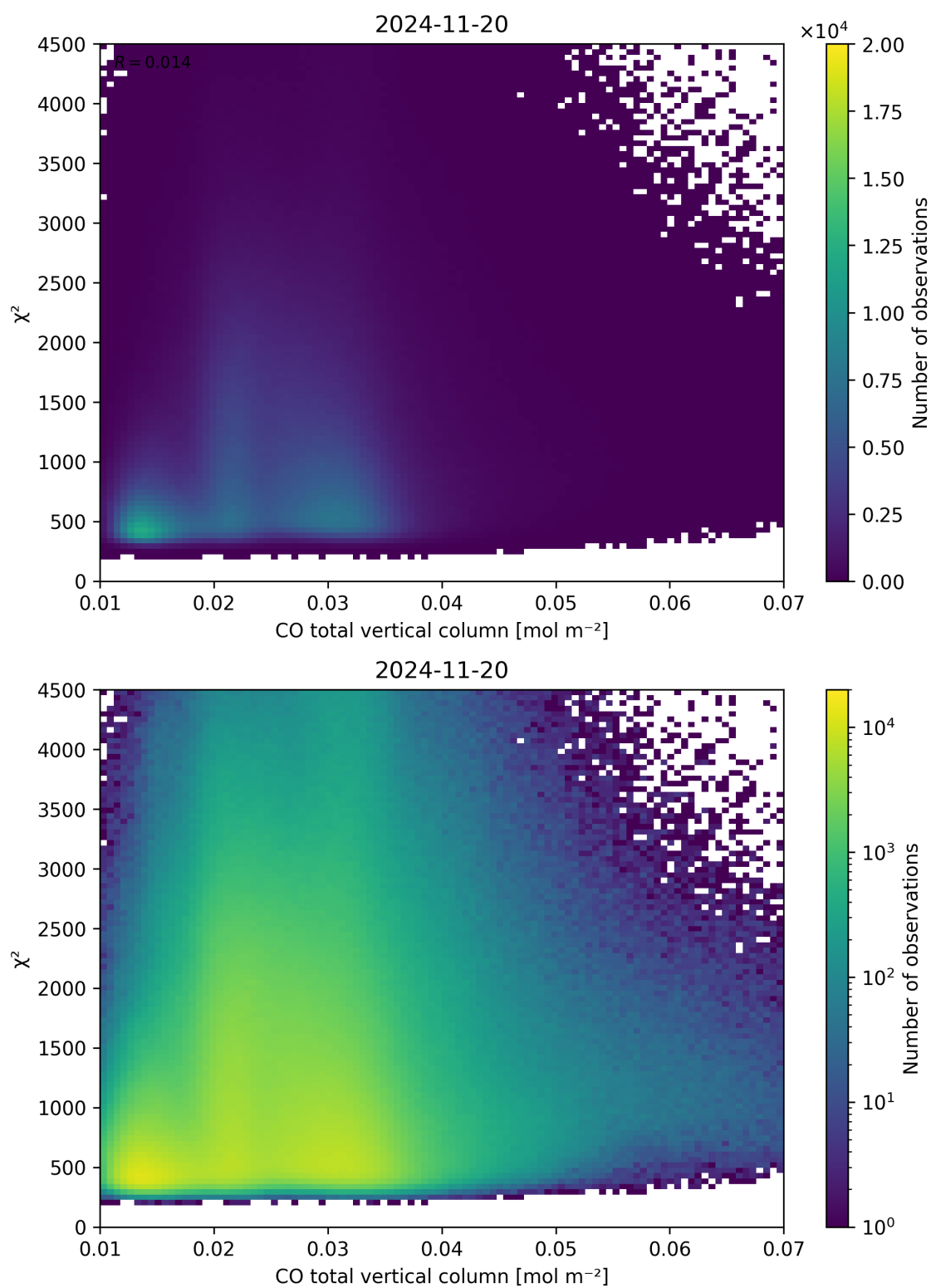
Figure 35: Scatter density plot of “CO total vertical column” against “ \chi^2 ” for 2024-11-20 to 2024-11-21.
