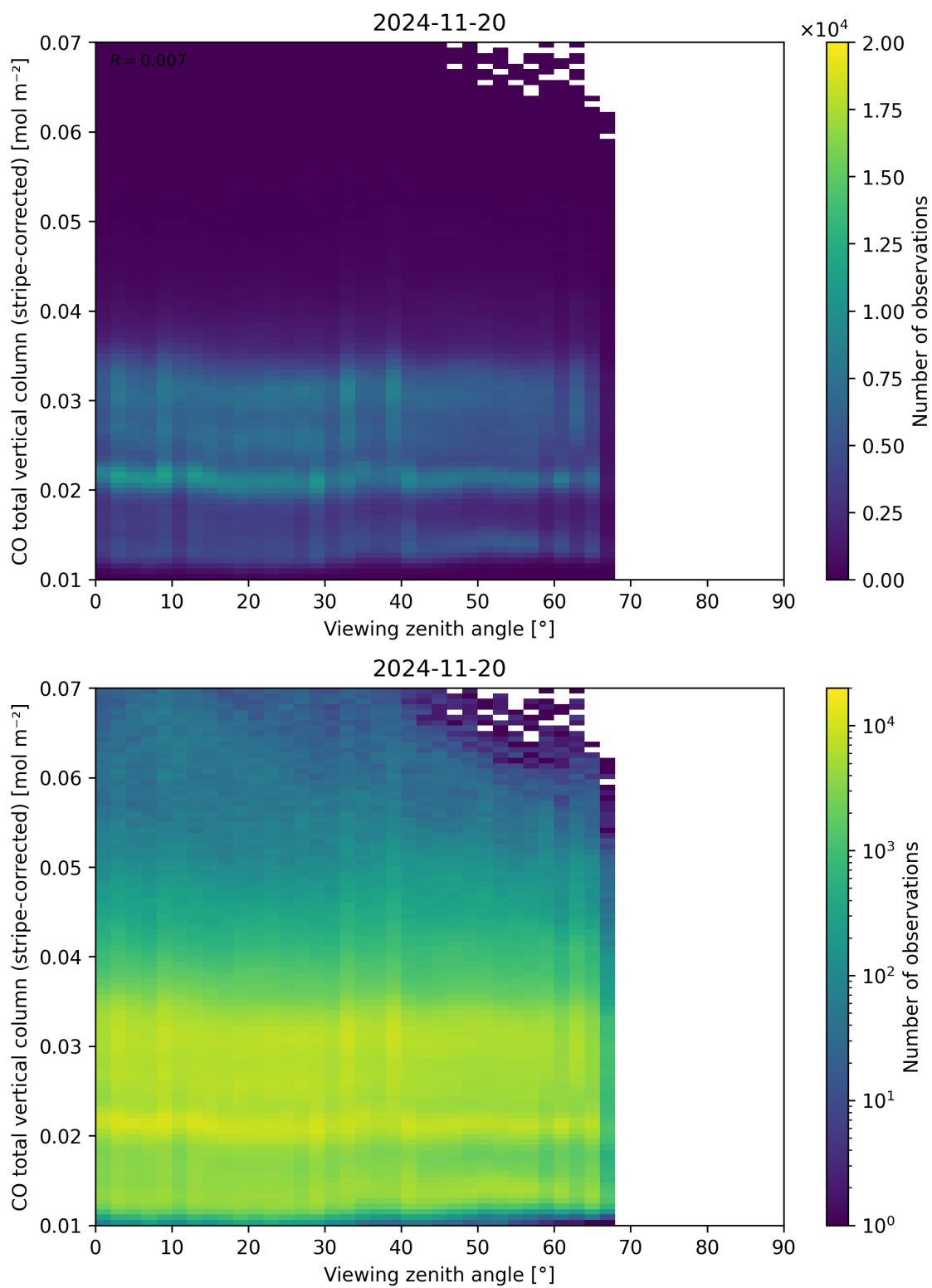
Figure 70: Scatter density plot of “Viewing zenith angle” against “CO total vertical column (stripe-corrected)” for 2024-11-20 to 2024-11-21.
