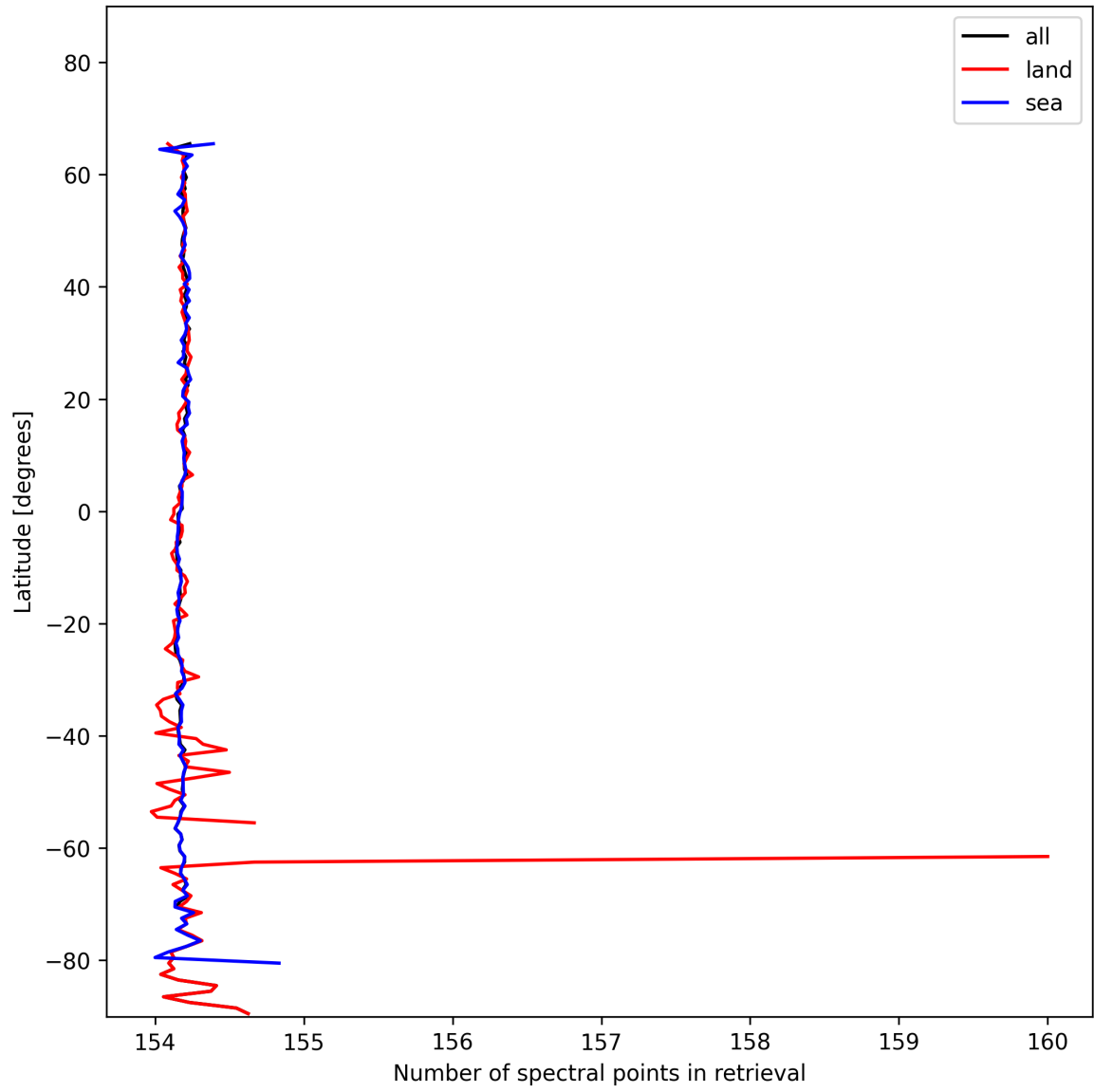
Figure 13: Zonal average of “Number of spectral points in retrieval” for 2024-11-20 to 2024-11-21.
