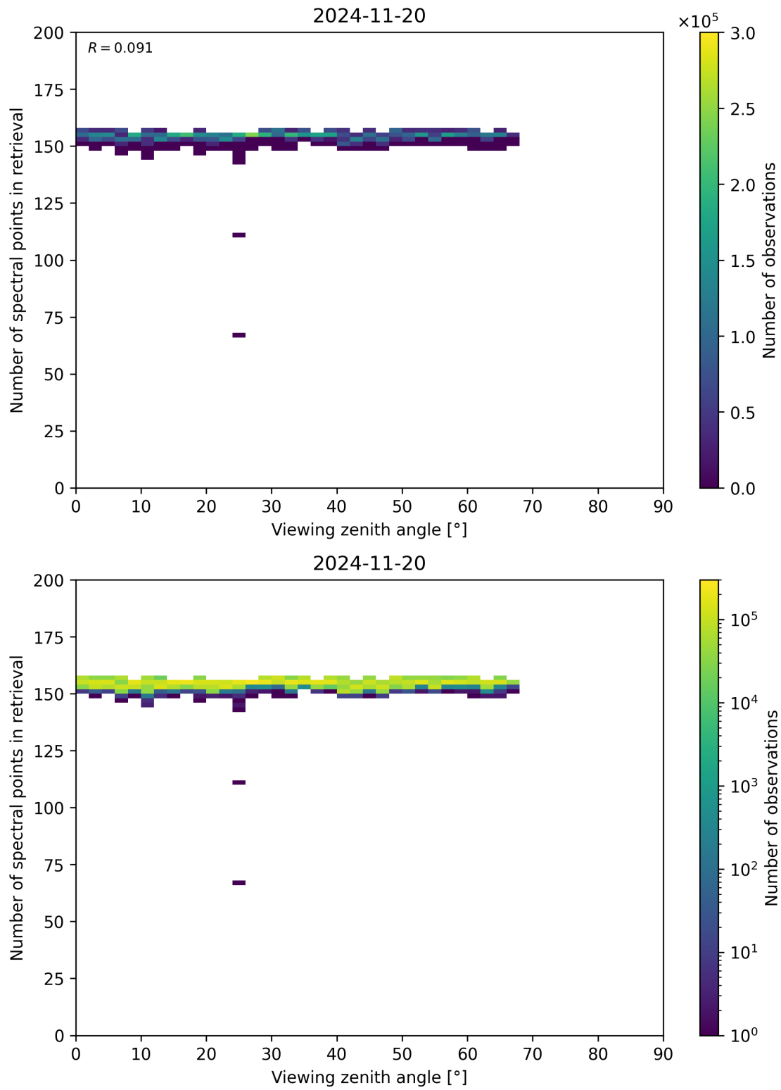
Figure 76: Scatter density plot of “Viewing zenith angle” against “Number of spectral points in retrieval” for 2024-11-20 to 2024-11-21.
