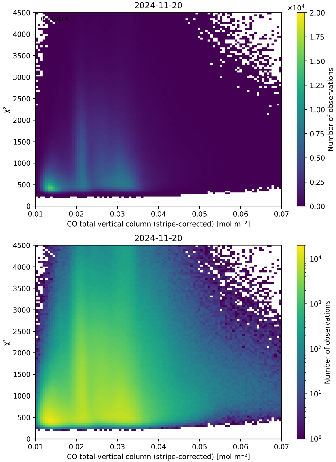
Figure 37: Scatter density plot of “CO total vertical column (stripe-corrected)” against “ \chi^2 ” for 2024-11-20 to 2024-11-21.
