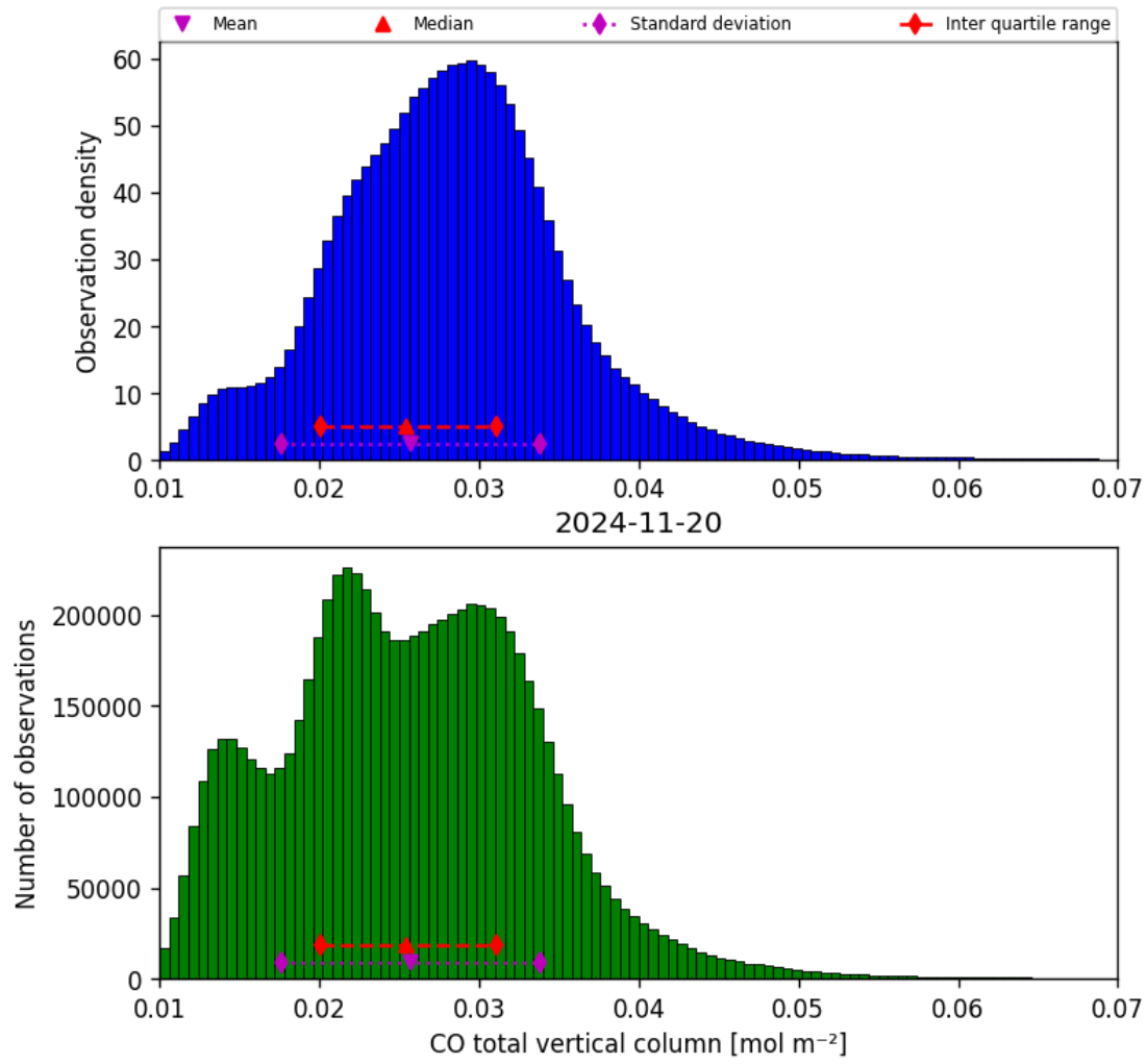
Figure 18: Histogram of “CO total vertical column” for 2024-11-20 to 2024-11-21
