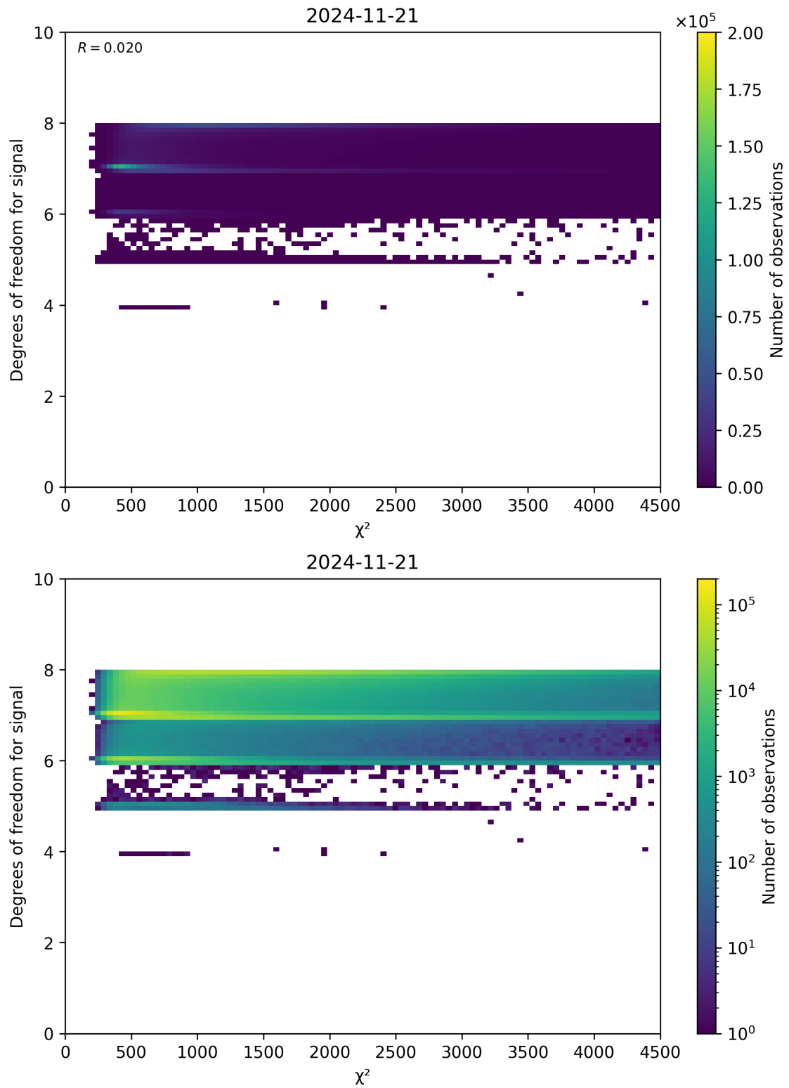
Figure 48: Scatter density plot of “ \chi^2 ” against “Degrees of freedom for signal” for 2024-11-20 to 2024-11-22.
