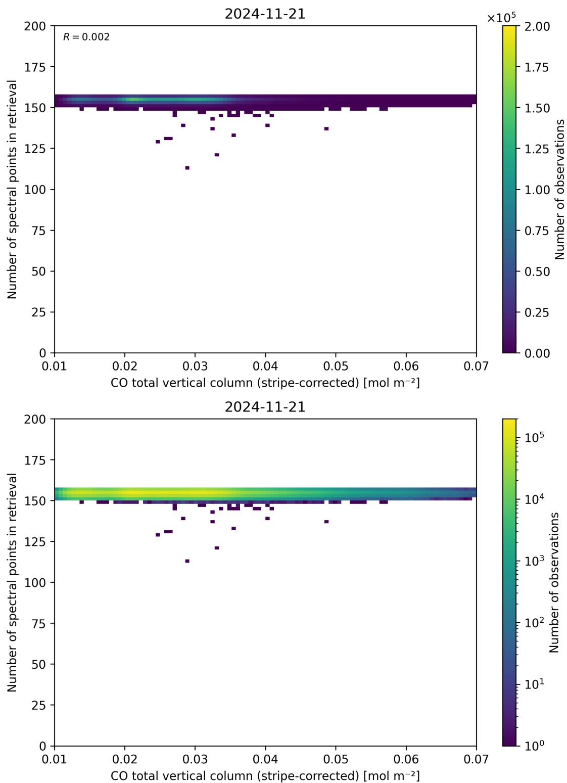
Figure 40: Scatter density plot of “CO total vertical column (stripe-corrected)” against “Number of spectral points in retrieval” for 2024-11-20 to 2024-11-22.
