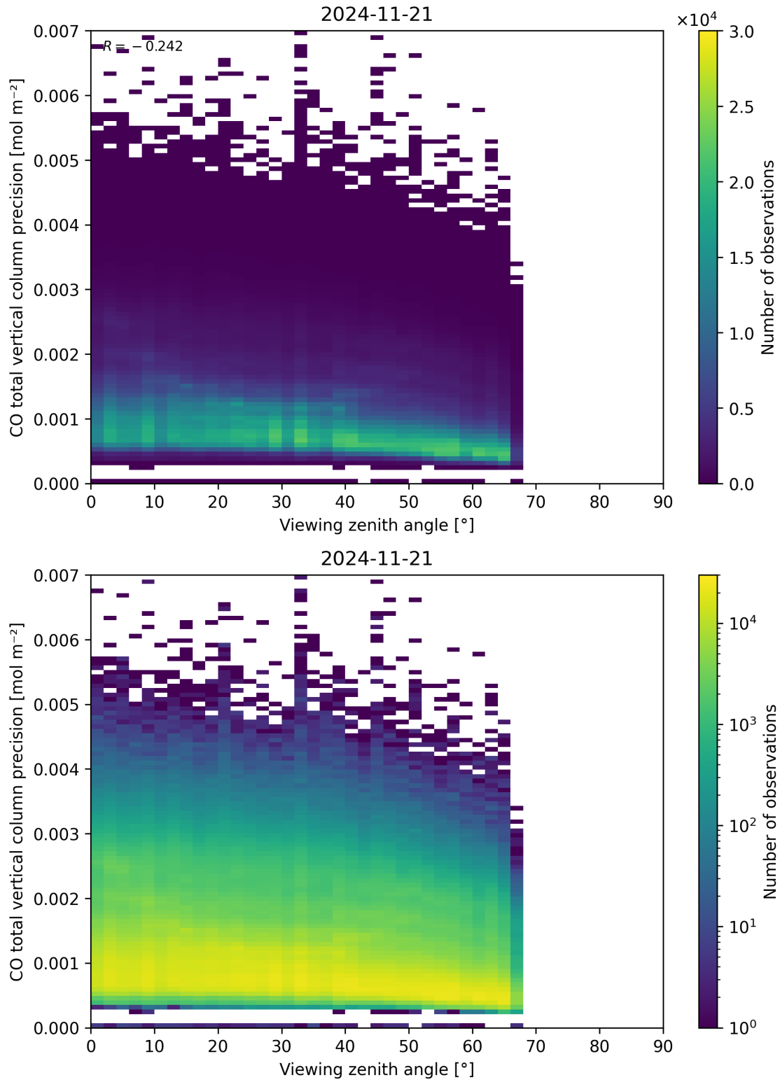
Figure 71: Scatter density plot of “Viewing zenith angle” against “CO total vertical column precision” for 2024-11-20 to 2024-11-22.
