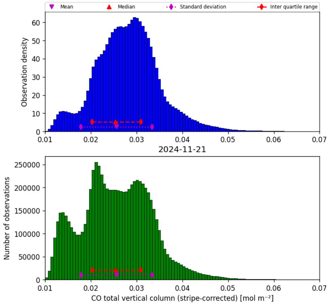
Figure 19: Histogram of “CO total vertical column (stripe-corrected)” for 2024-11-20 to 2024-11-22
