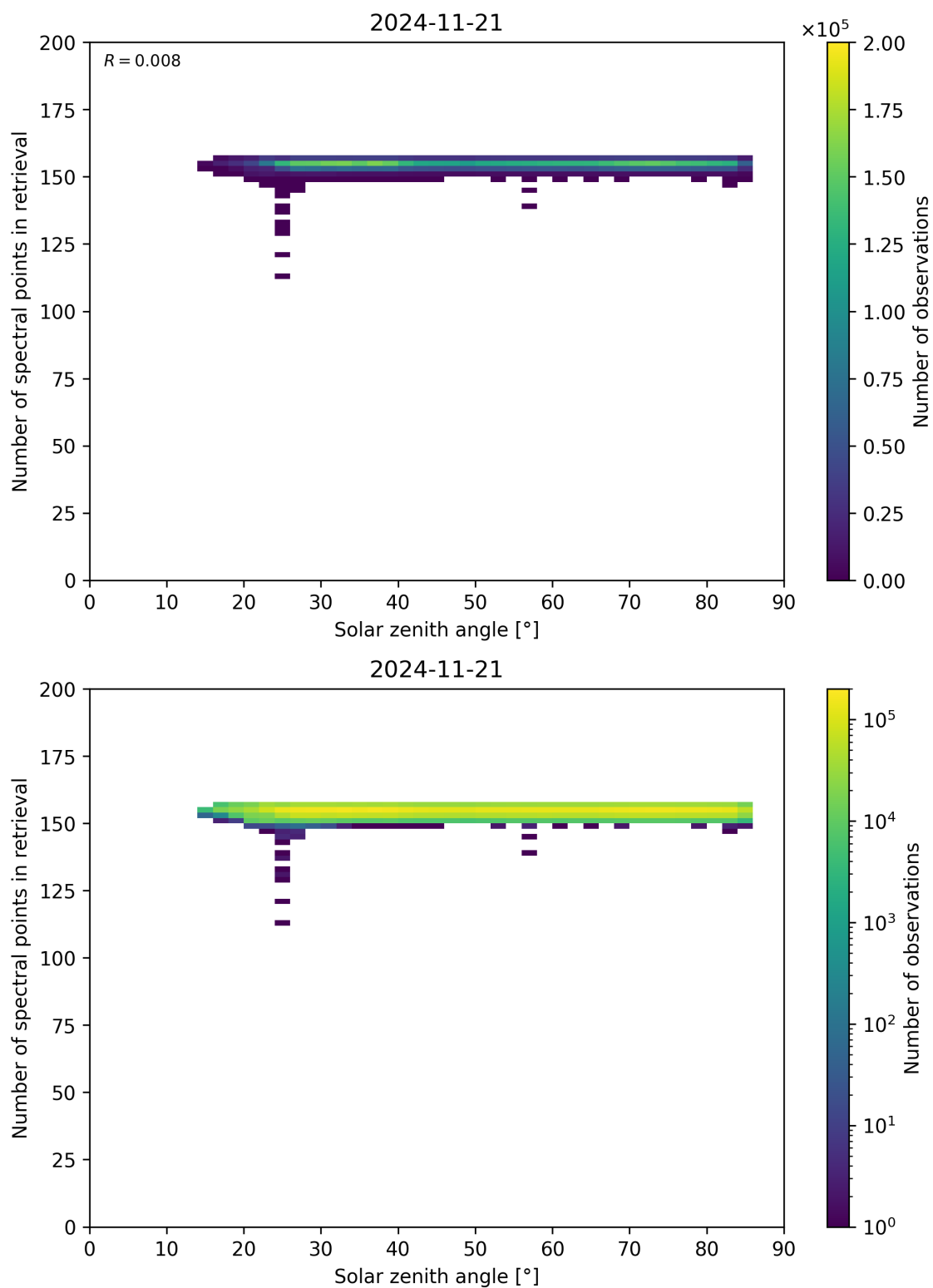
Figure 68: Scatter density plot of “Solar zenith angle” against “Number of spectral points in retrieval” for 2024-11-20 to 2024-11-22.
