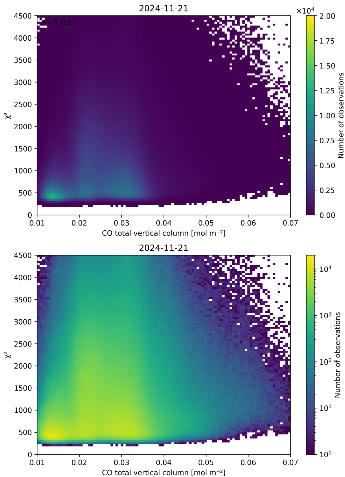
Figure 35: Scatter density plot of “CO total vertical column” against “ \chi^2 ” for 2024-11-20 to 2024-11-22.
