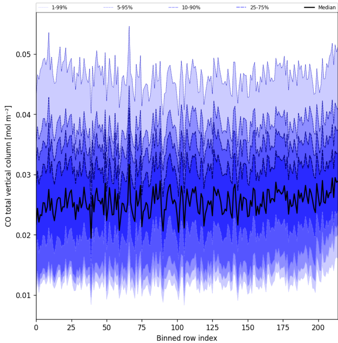
Figure 26: Along track statistics of “CO total vertical column” for 2024-11-20 to 2024-11-22
