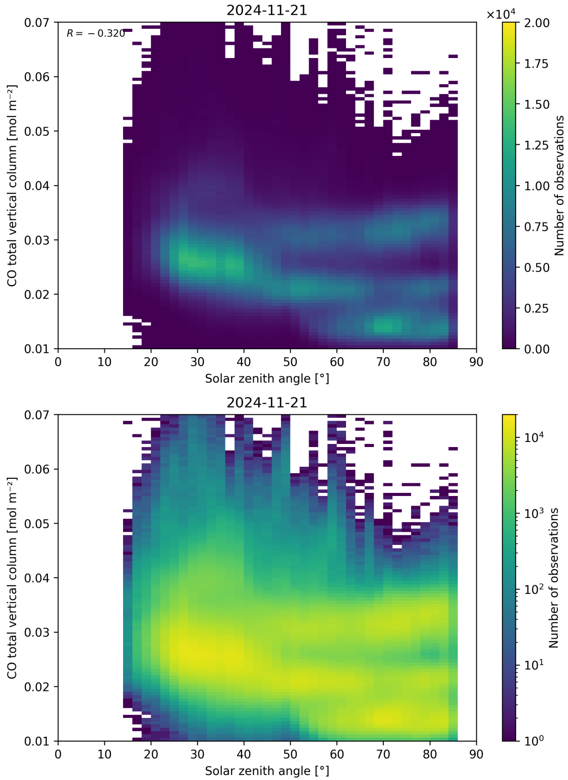
Figure 61: Scatter density plot of “Solar zenith angle” against “CO total vertical column” for 2024-11-20 to 2024-11-22.
