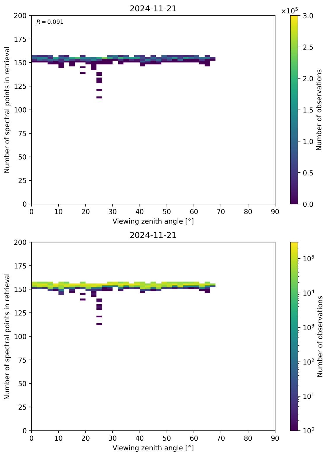
Figure 76: Scatter density plot of “Viewing zenith angle” against “Number of spectral points in retrieval” for 2024-11-20 to 2024-11-22.
