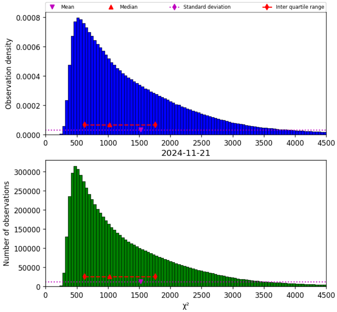
Figure 22: Histogram of “ \chi^2 ” for 2024-11-20 to 2024-11-22
