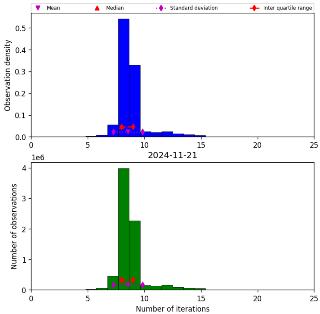
Figure 24: Histogram of “Number of iterations” for 2024-11-20 to 2024-11-22
