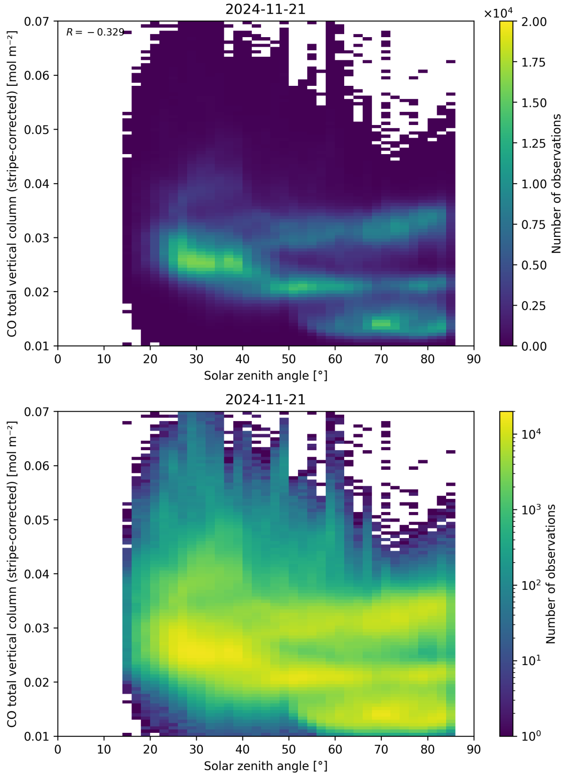
Figure 62: Scatter density plot of “Solar zenith angle” against “CO total vertical column (stripe-corrected)” for 2024-11-20 to 2024-11-22.
