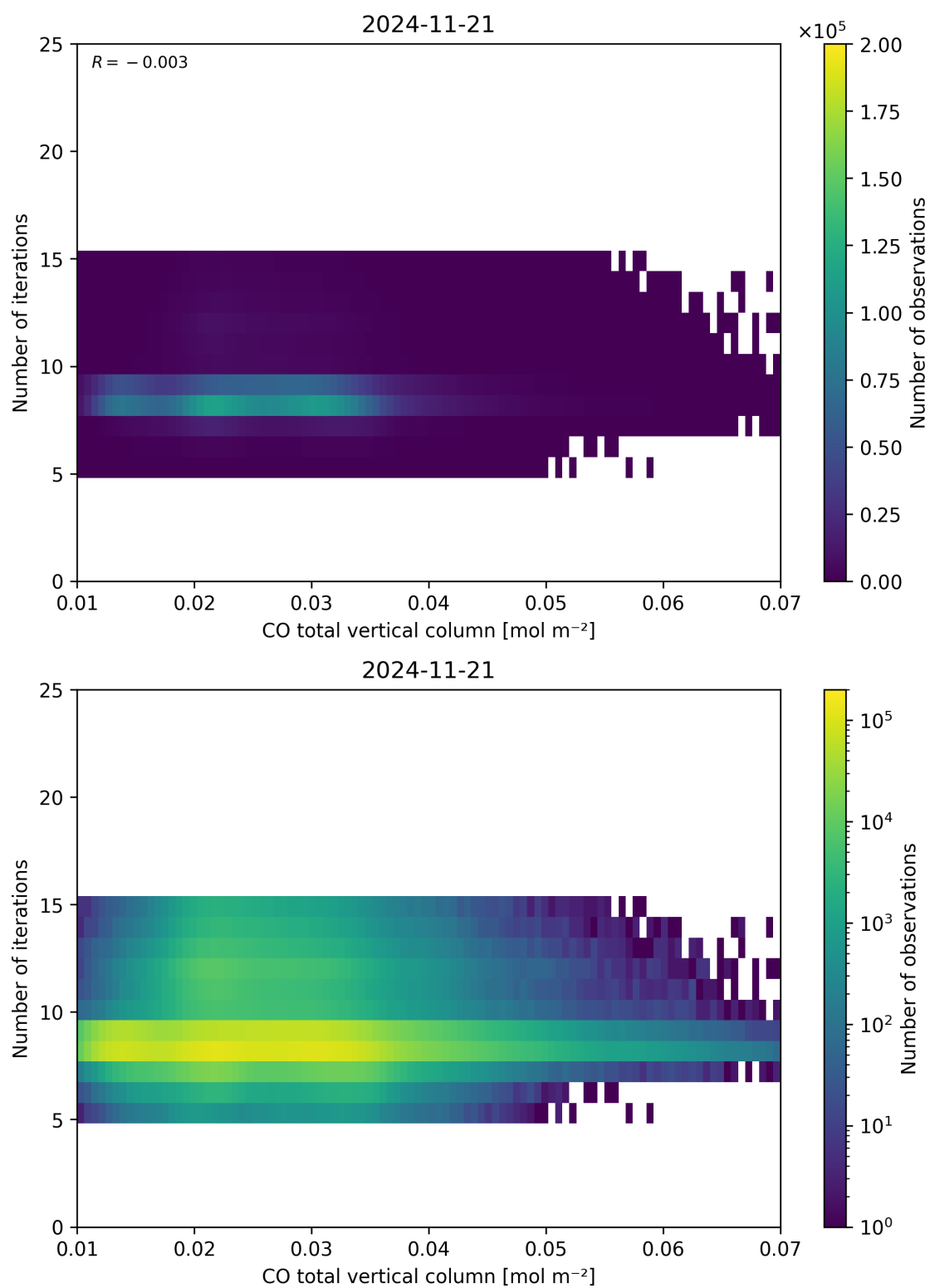
Figure 42: Scatter density plot of “CO total vertical column” against “Number of iterations” for 2024-11-20 to 2024-11-22.
