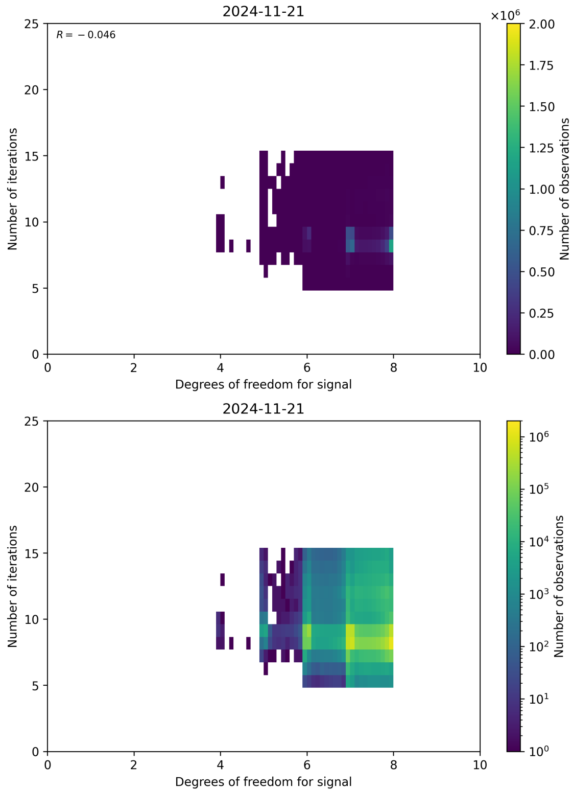
Figure 50: Scatter density plot of “Degrees of freedom for signal” against “Number of iterations” for 2024-11-20 to 2024-11-22.
