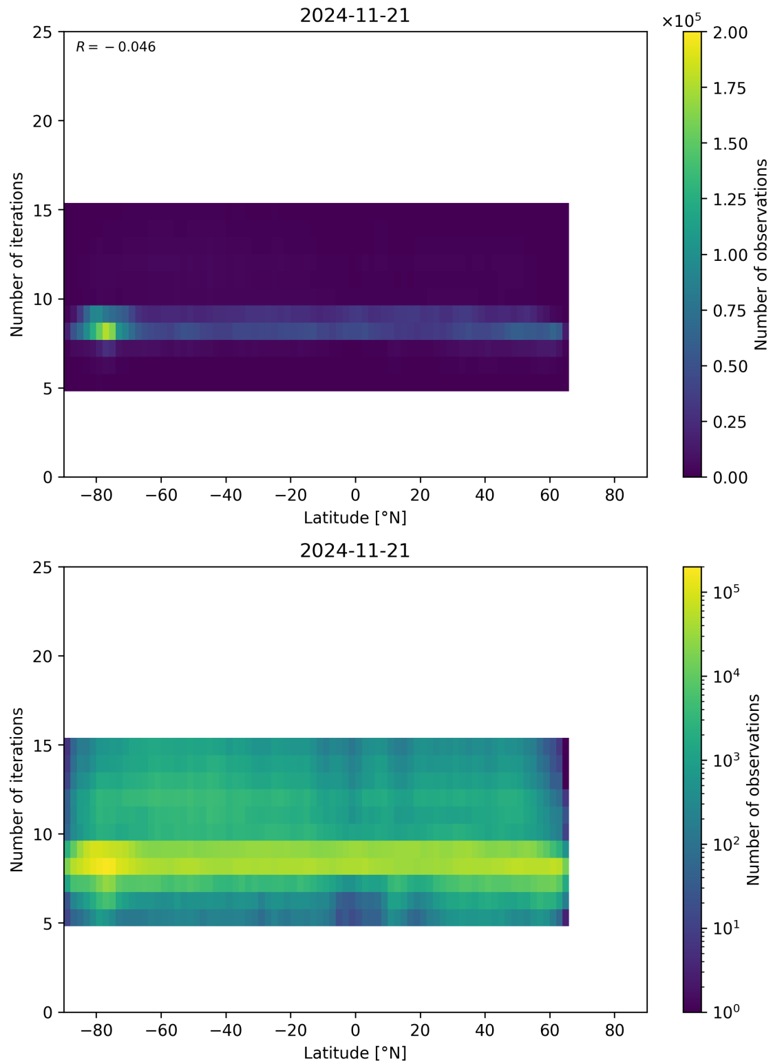
Figure 56: Scatter density plot of “Latitude” against “Number of iterations” for 2024-11-20 to 2024-11-22.
