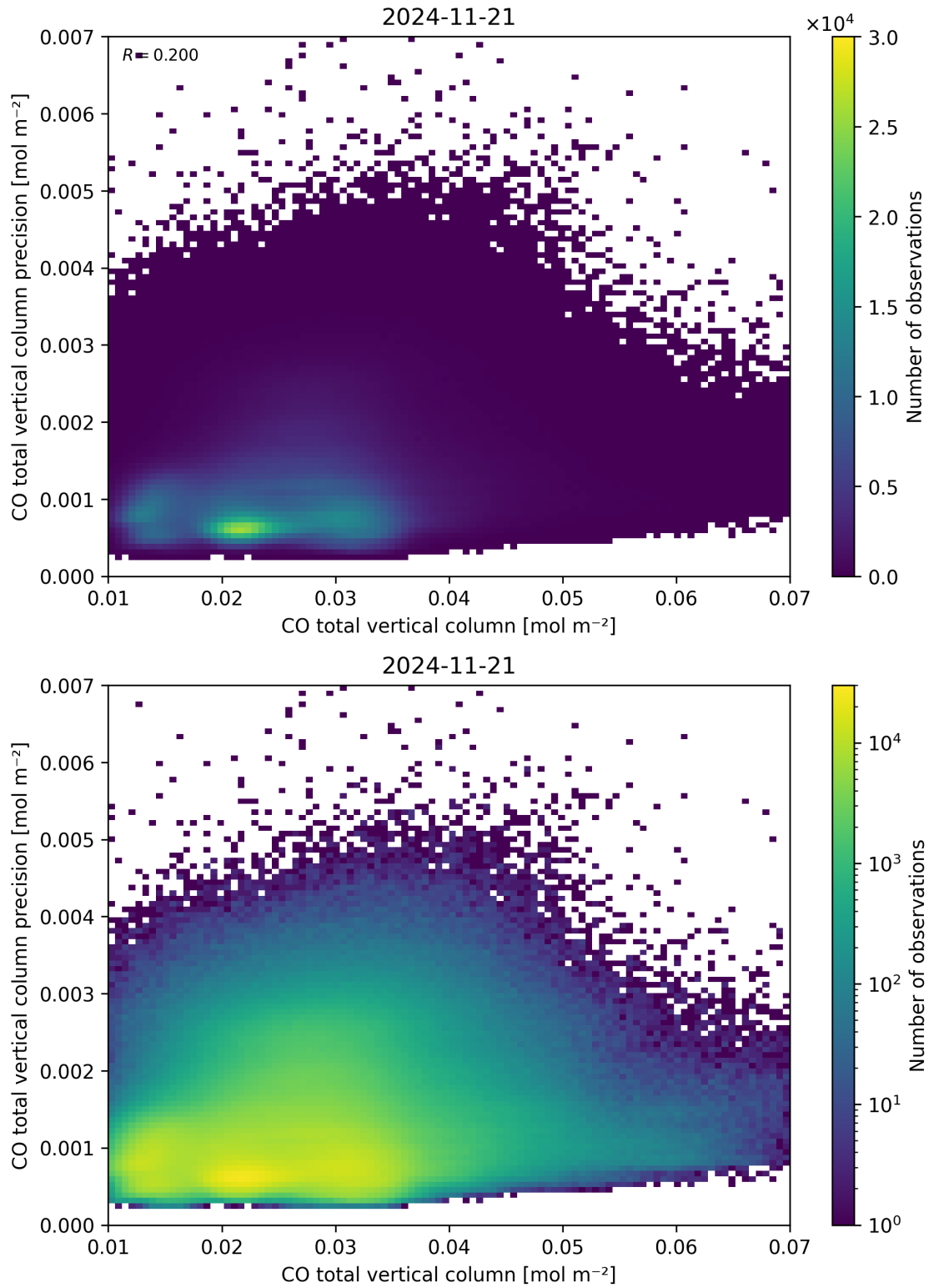
Figure 34: Scatter density plot of “CO total vertical column” against “CO total vertical column precision” for 2024-11-20 to 2024-11-22.
