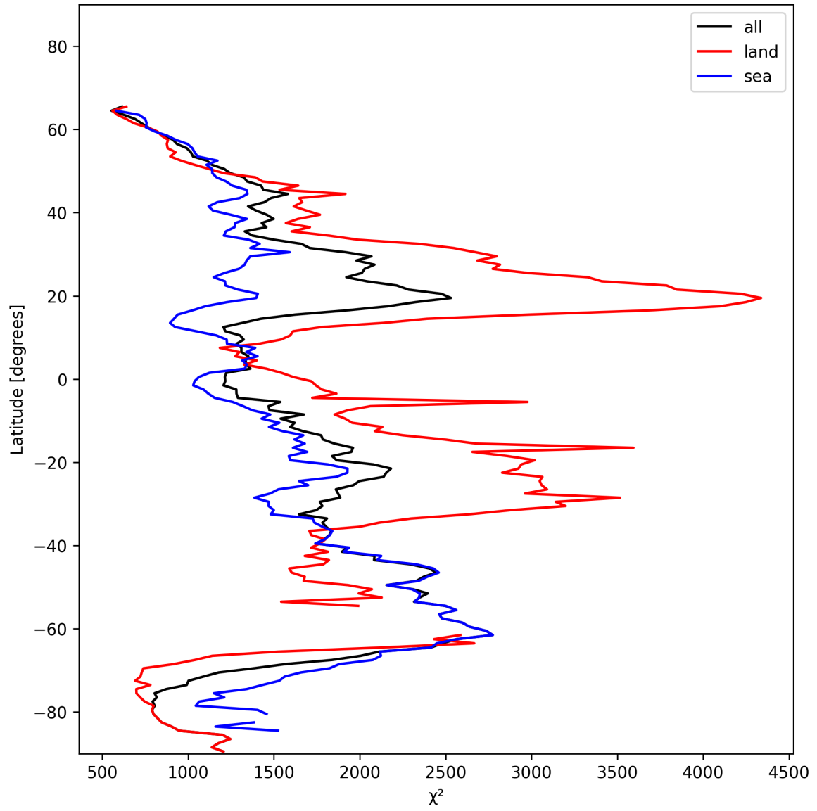
Figure 14: Zonal average of “ \chi^2 ” for 2024-11-20 to 2024-11-22.
