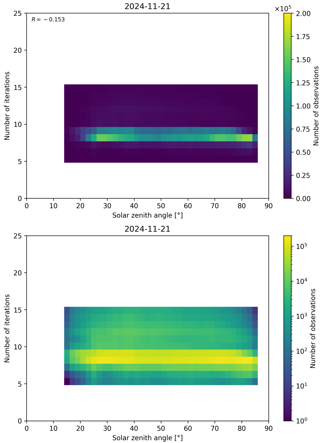
Figure 67: Scatter density plot of “Solar zenith angle” against “Number of iterations” for 2024-11-20 to 2024-11-22.
