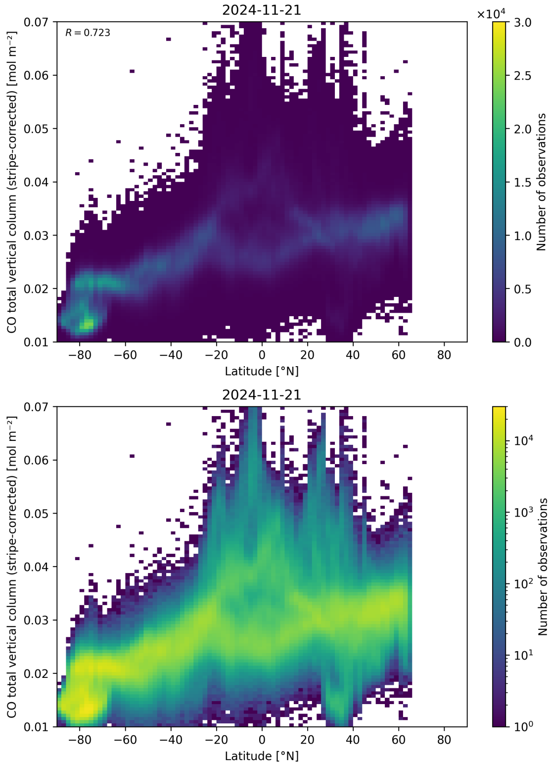
Figure 52: Scatter density plot of “Latitude” against “CO total vertical column (stripe-corrected)” for 2024-11-20 to 2024-11-22.
