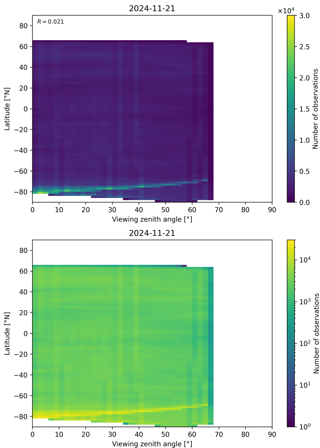
Figure 74: Scatter density plot of “Viewing zenith angle” against “Latitude” for 2024-11-20 to 2024-11-22.
