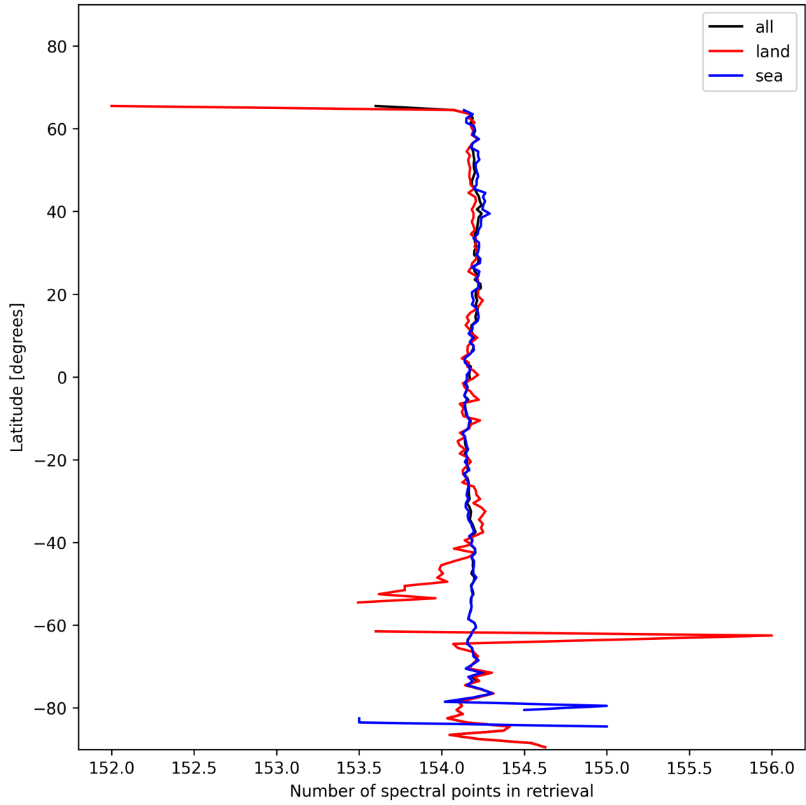
Figure 13: Zonal average of “Number of spectral points in retrieval” for 2024-11-20 to 2024-11-22.
