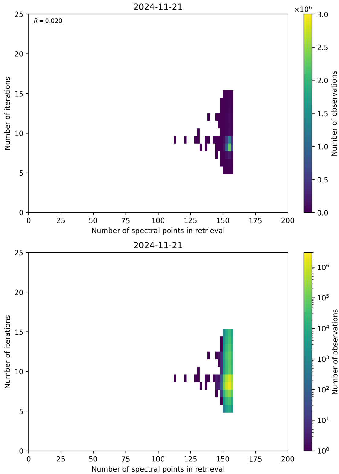
Figure 60: Scatter density plot of “Number of spectral points in retrieval” against “Number of iterations” for 2024-11-20 to 2024-11-22.
