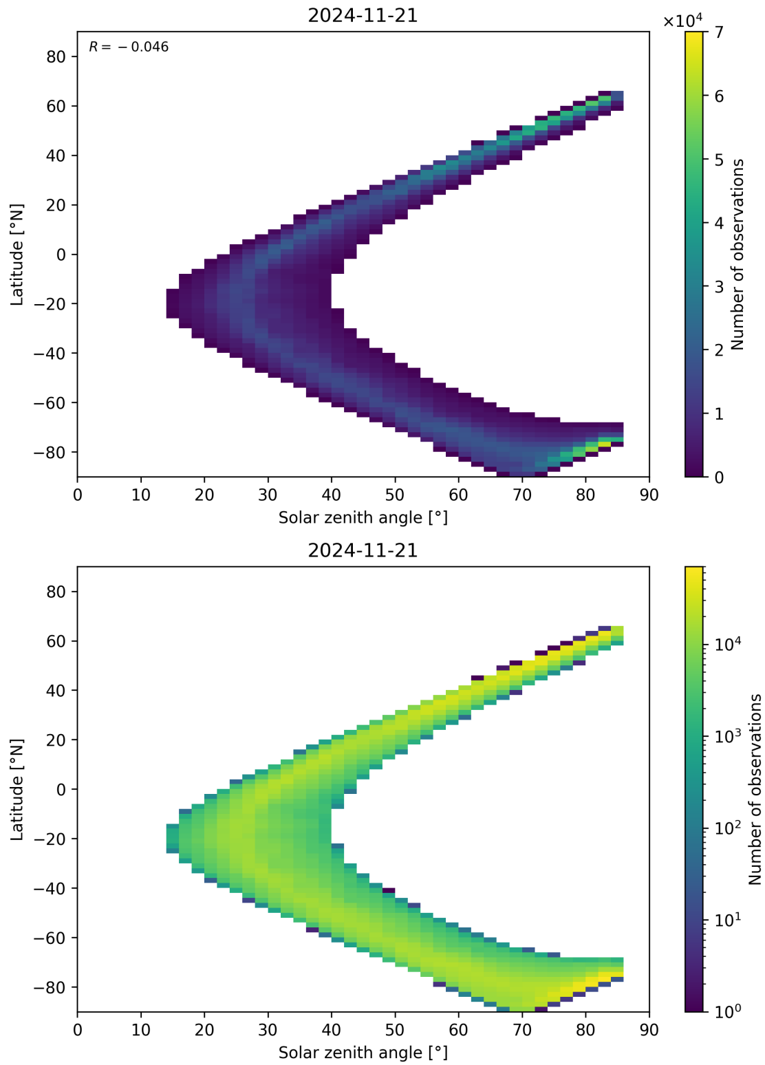
Figure 66: Scatter density plot of “Solar zenith angle” against “Latitude” for 2024-11-20 to 2024-11-22.
