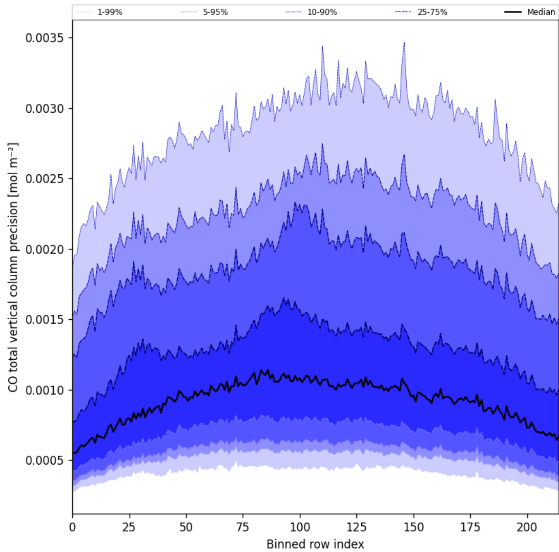
Figure 28: Along track statistics of “CO total vertical column precision” for 2024-11-20 to 2024-11-22
