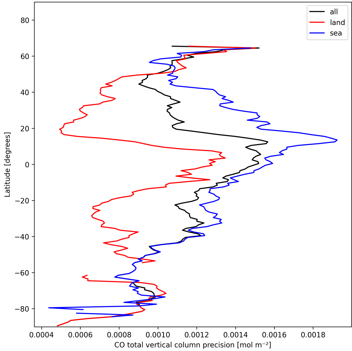
Figure 12: Zonal average of “CO total vertical column precision” for 2024-11-20 to 2024-11-22.
