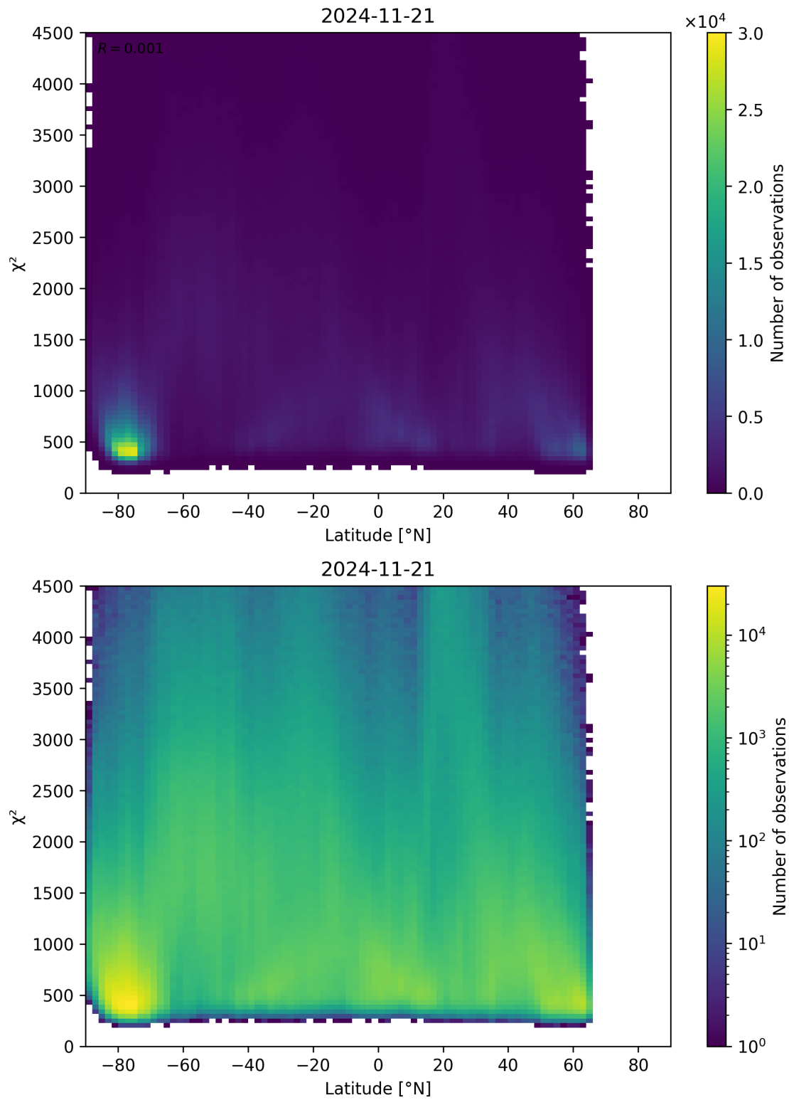
Figure 54: Scatter density plot of “Latitude” against “ \chi^2 ” for 2024-11-20 to 2024-11-22.
