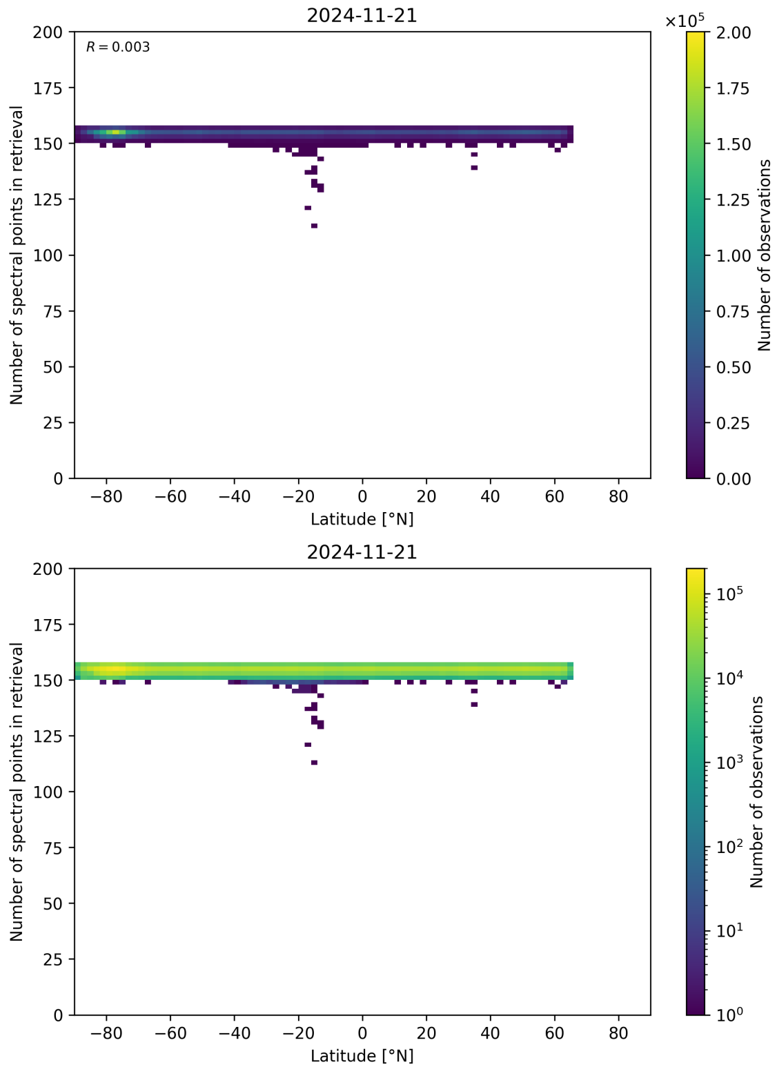
Figure 57: Scatter density plot of “Latitude” against “Number of spectral points in retrieval” for 2024-11-20 to 2024-11-22.
