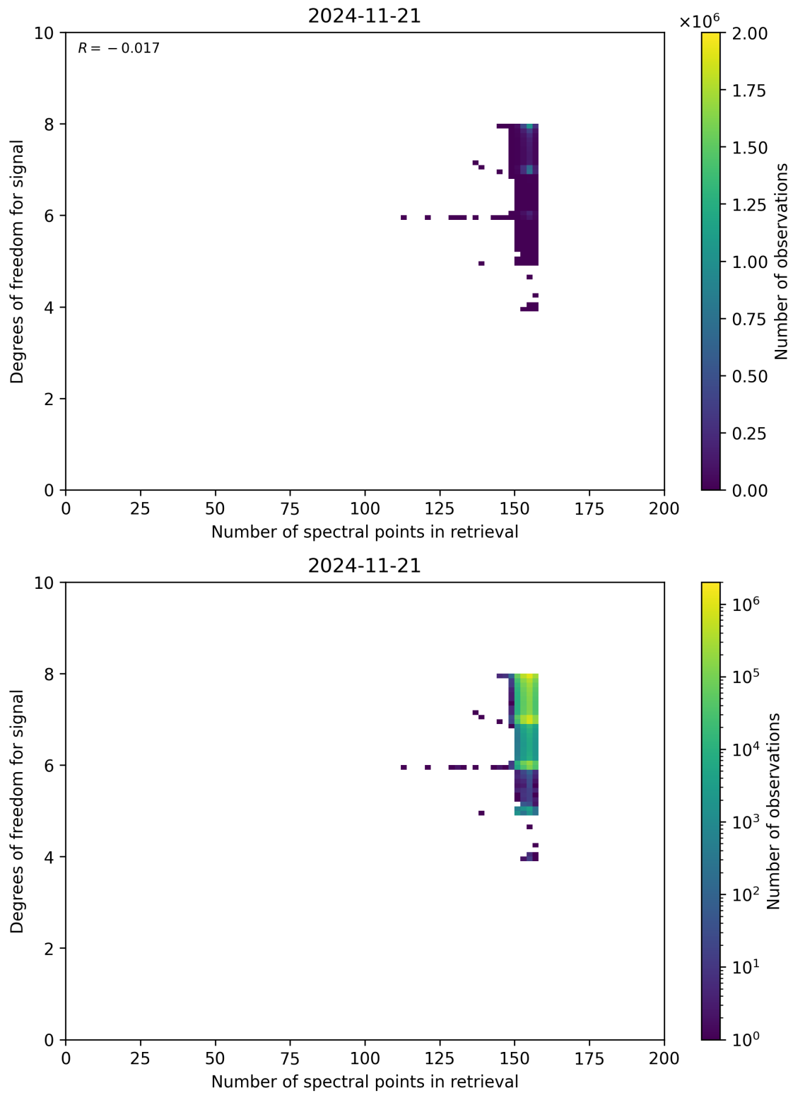
Figure 59: Scatter density plot of “Number of spectral points in retrieval” against “Degrees of freedom for signal” for 2024-11-20 to 2024-11-22.
