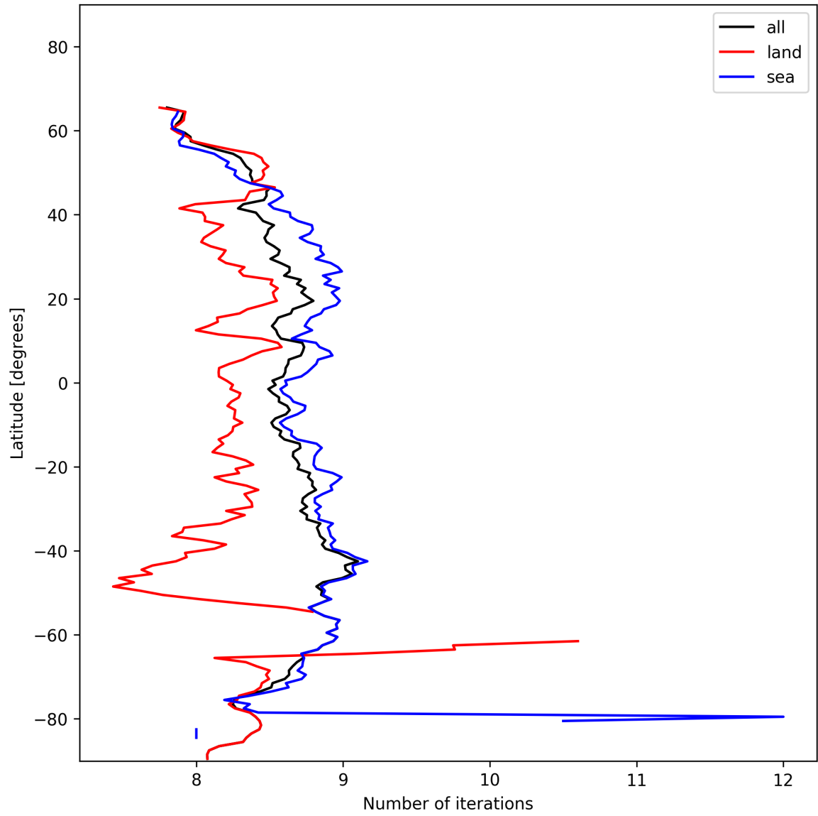
Figure 16: Zonal average of “Number of iterations” for 2024-11-20 to 2024-11-22.
