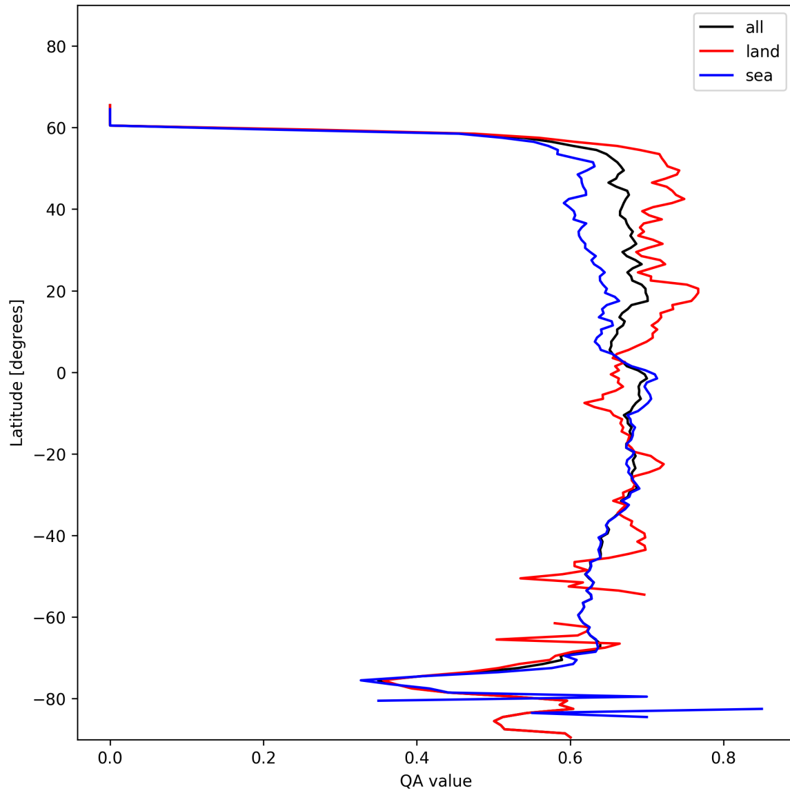
Figure 9: Zonal average of “QA value” for 2024-11-20 to 2024-11-22.
