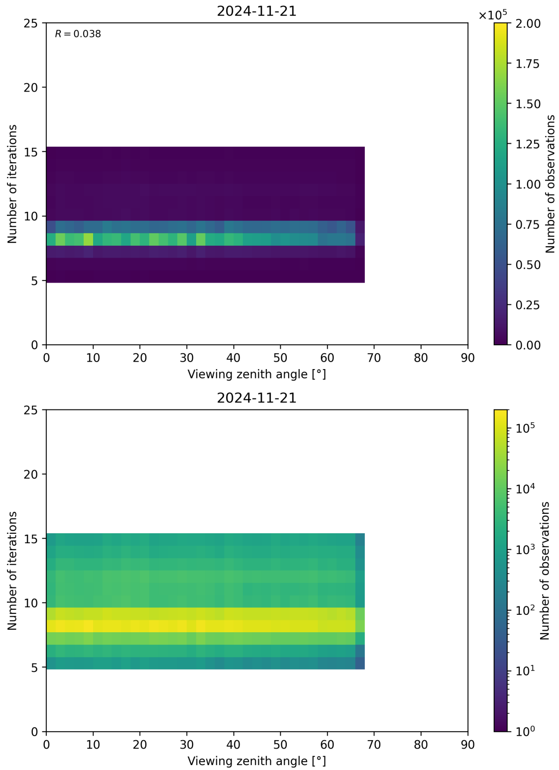
Figure 75: Scatter density plot of “Viewing zenith angle” against “Number of iterations” for 2024-11-20 to 2024-11-22.
