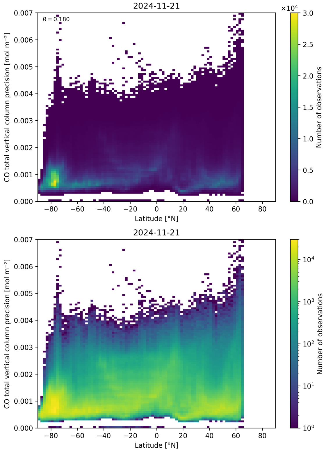
Figure 53: Scatter density plot of “Latitude” against “CO total vertical column precision” for 2024-11-20 to 2024-11-22.
