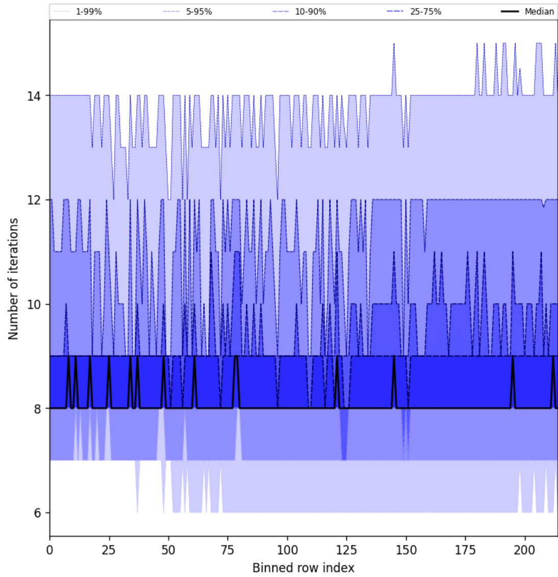
Figure 32: Along track statistics of “Number of iterations” for 2024-11-20 to 2024-11-22
