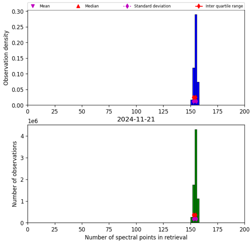
Figure 21: Histogram of “Number of spectral points in retrieval” for 2024-11-20 to 2024-11-22
