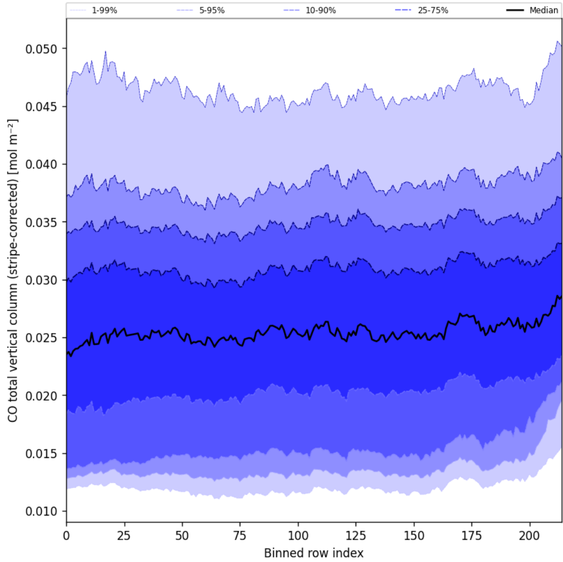
Figure 27: Along track statistics of “CO total vertical column (stripe-corrected)” for 2024-11-20 to 2024-11-22
