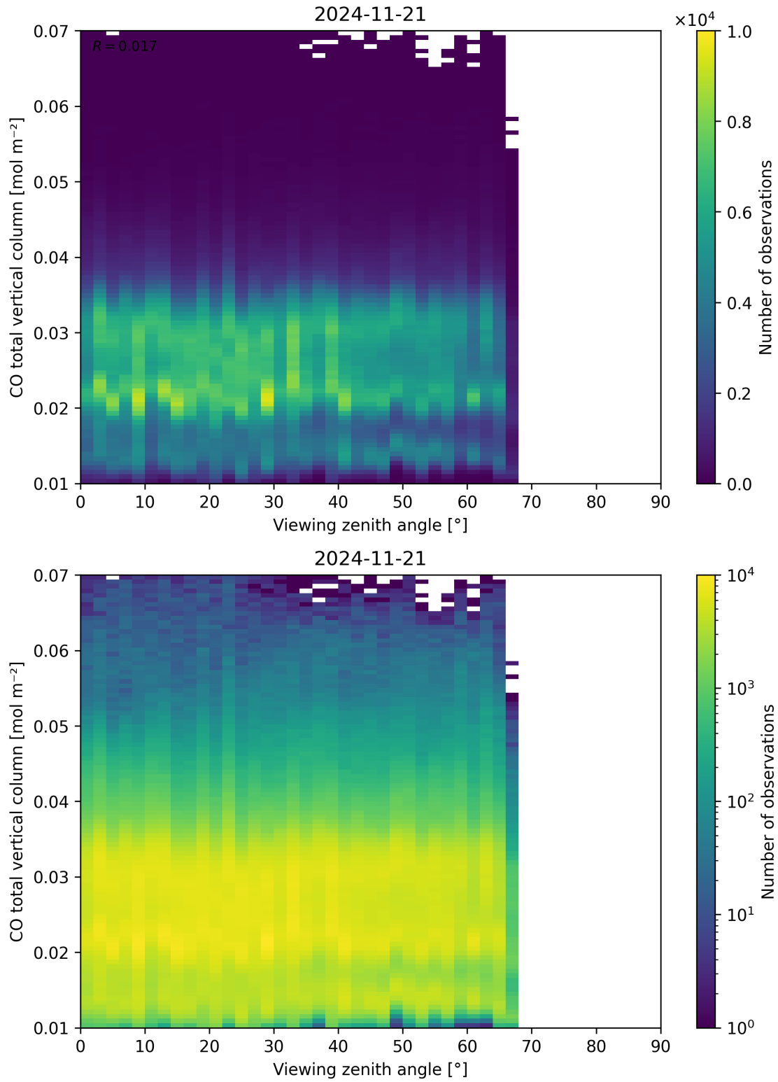
Figure 69: Scatter density plot of “Viewing zenith angle” against “CO total vertical column” for 2024-11-20 to 2024-11-22.
