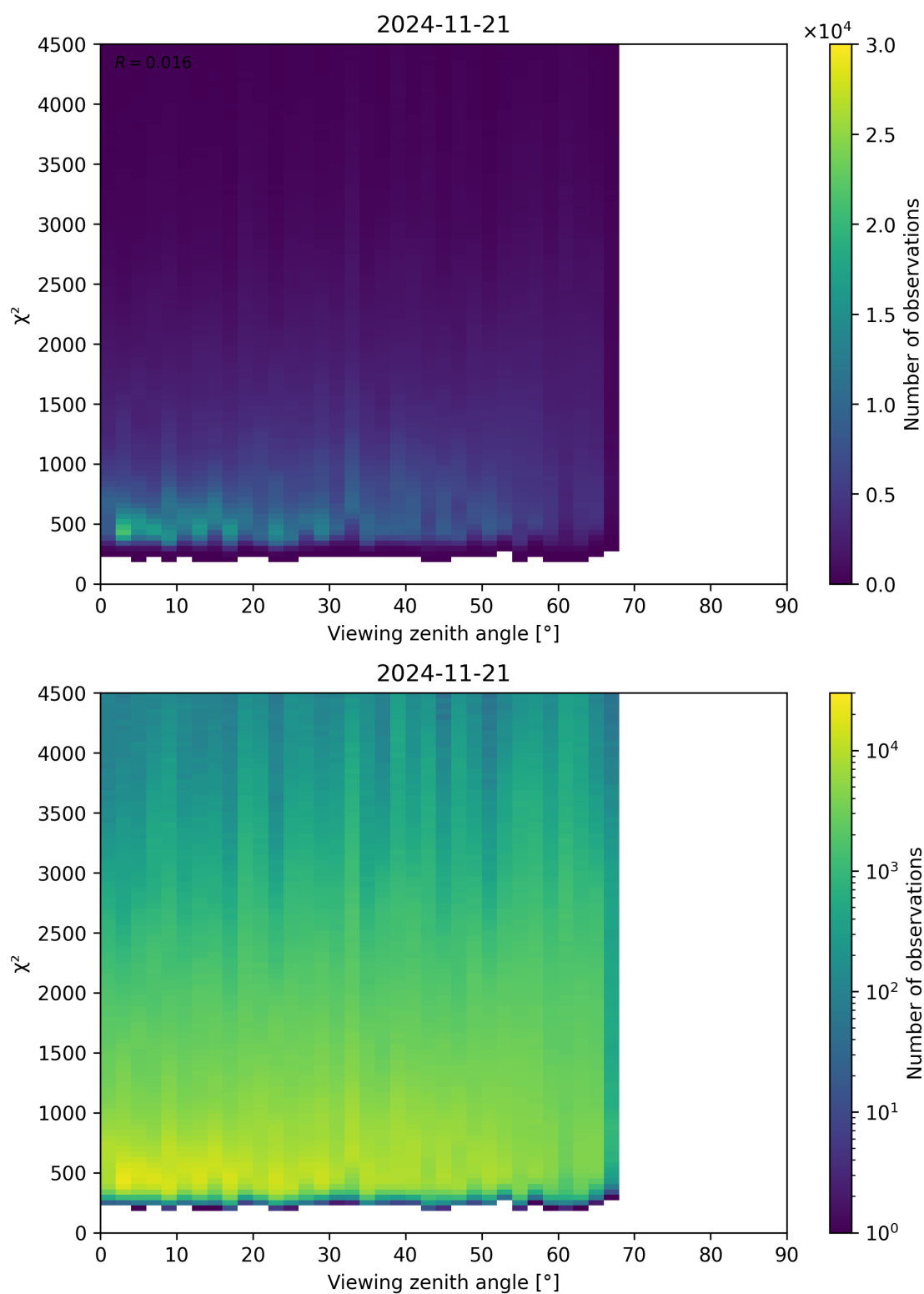
Figure 72: Scatter density plot of “Viewing zenith angle” against “ \chi^2 ” for 2024-11-20 to 2024-11-22.
