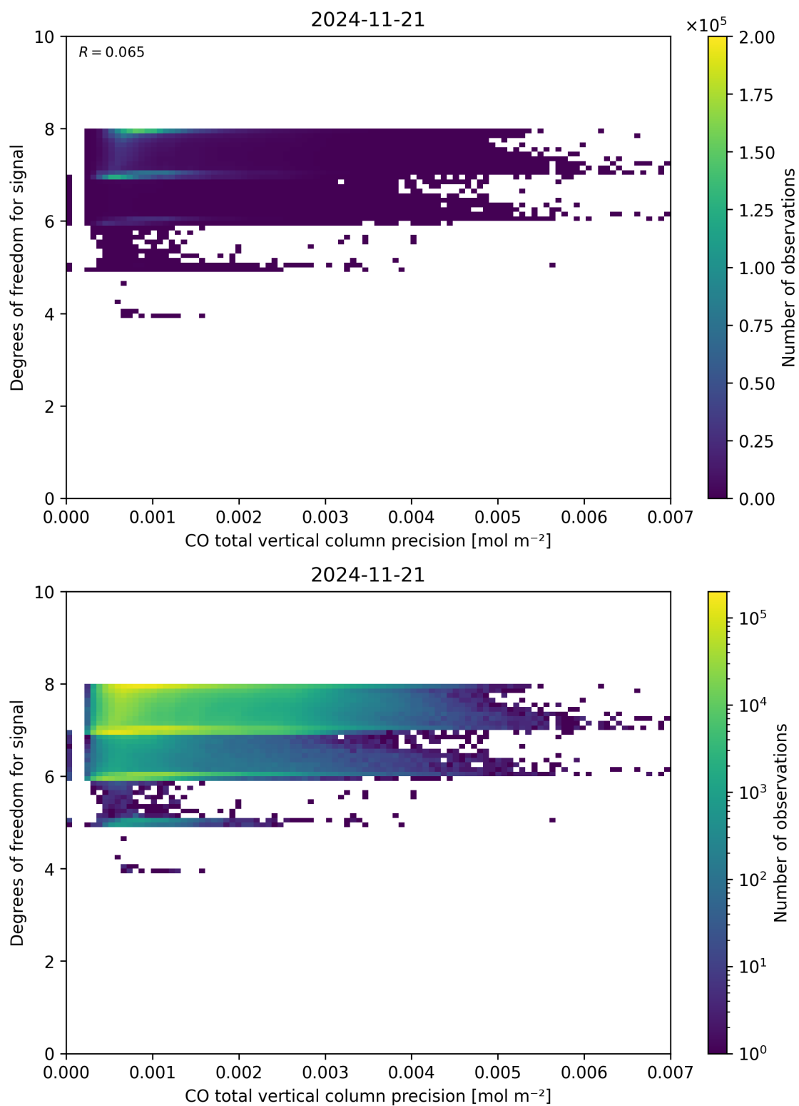
Figure 45: Scatter density plot of “CO total vertical column precision” against “Degrees of freedom for signal” for 2024-11-20 to 2024-11-22.
