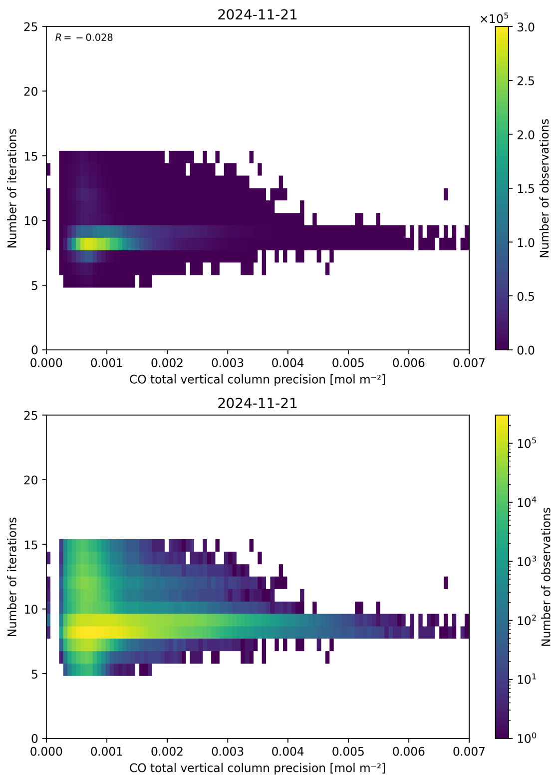
Figure 46: Scatter density plot of “CO total vertical column precision” against “Number of iterations” for 2024-11-20 to 2024-11-22.
