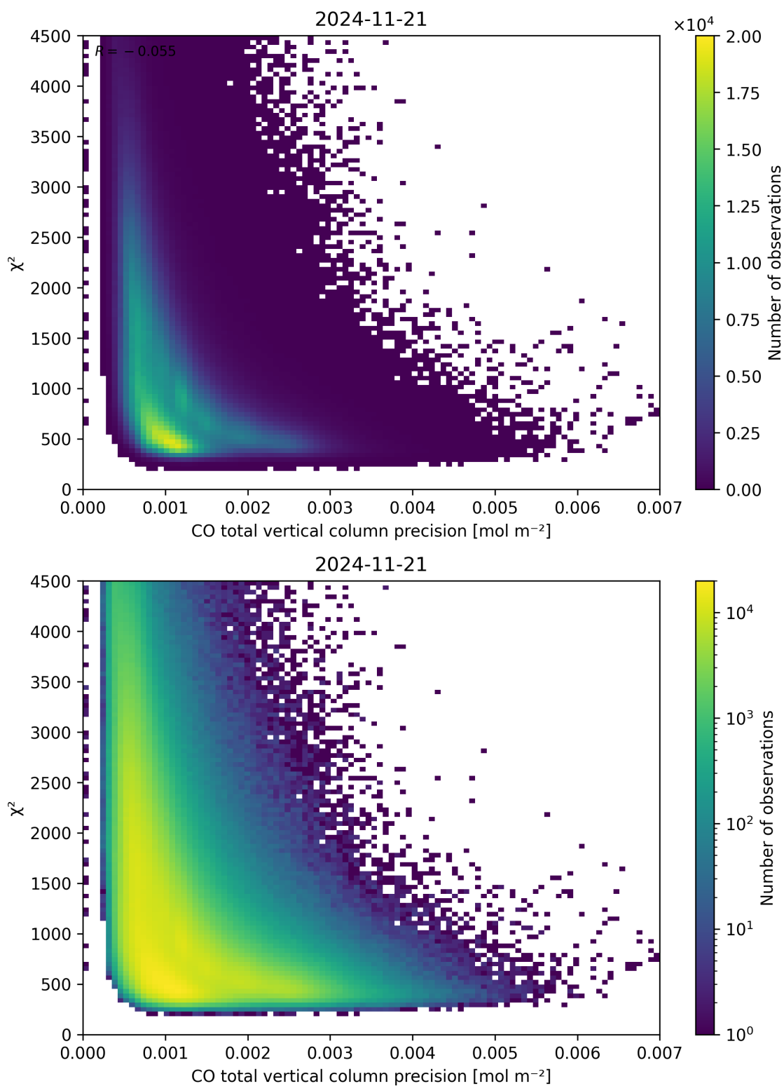
Figure 44: Scatter density plot of “CO total vertical column precision” against “ \chi^2 ” for 2024-11-20 to 2024-11-22.
