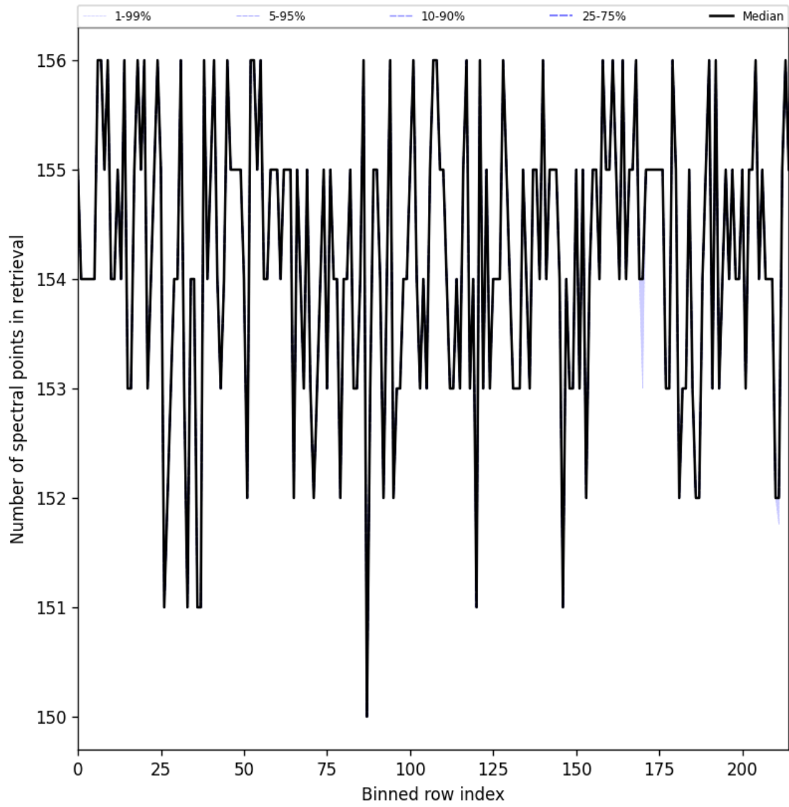
Figure 29: Along track statistics of “Number of spectral points in retrieval” for 2024-11-20 to 2024-11-22
