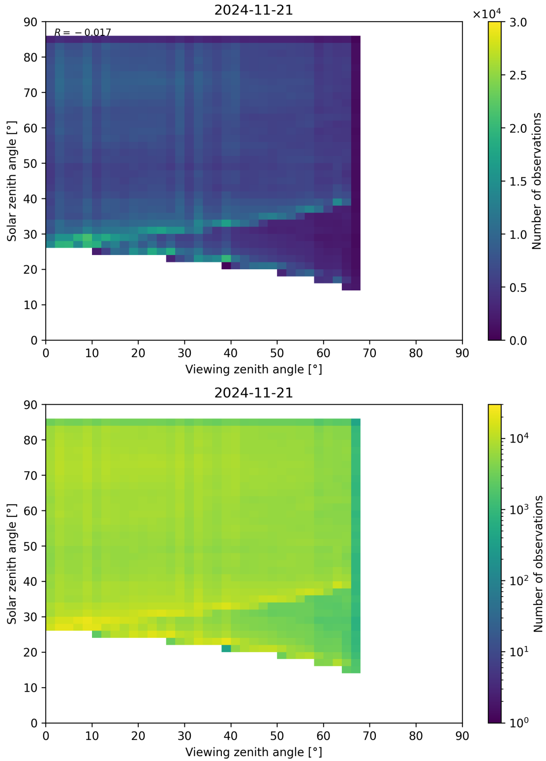
Figure 77: Scatter density plot of “Viewing zenith angle” against “Solar zenith angle” for 2024-11-20 to 2024-11-22.
