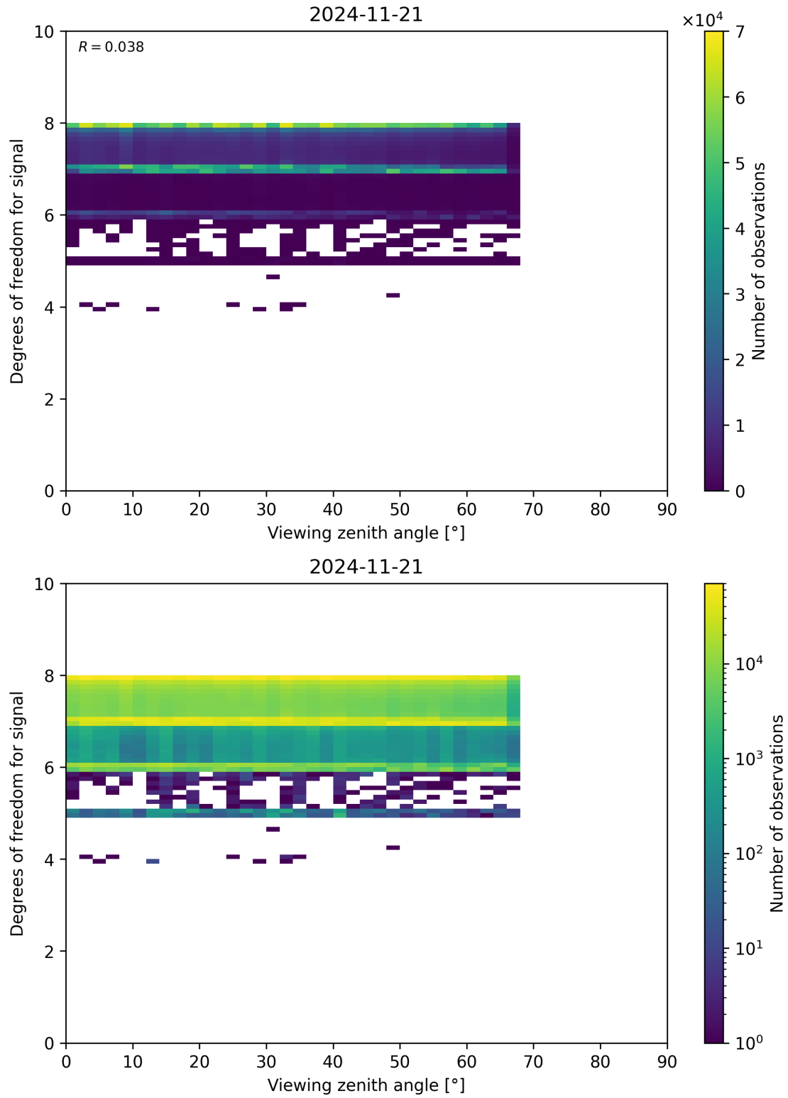
Figure 73: Scatter density plot of “Viewing zenith angle” against “Degrees of freedom for signal” for 2024-11-20 to 2024-11-22.
