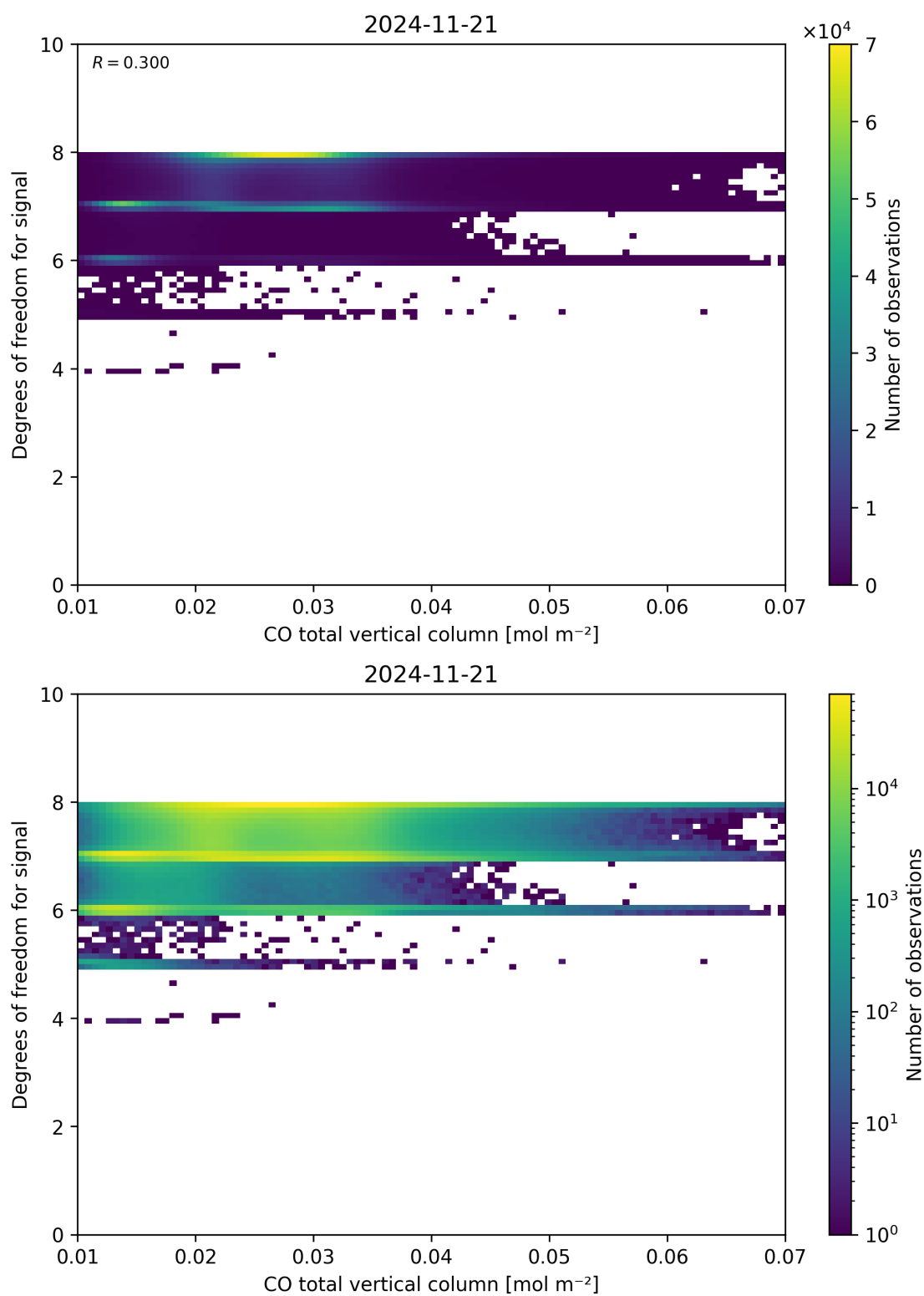
Figure 41: Scatter density plot of “CO total vertical column” against “Degrees of freedom for signal” for 2024-11-20 to 2024-11-22.
