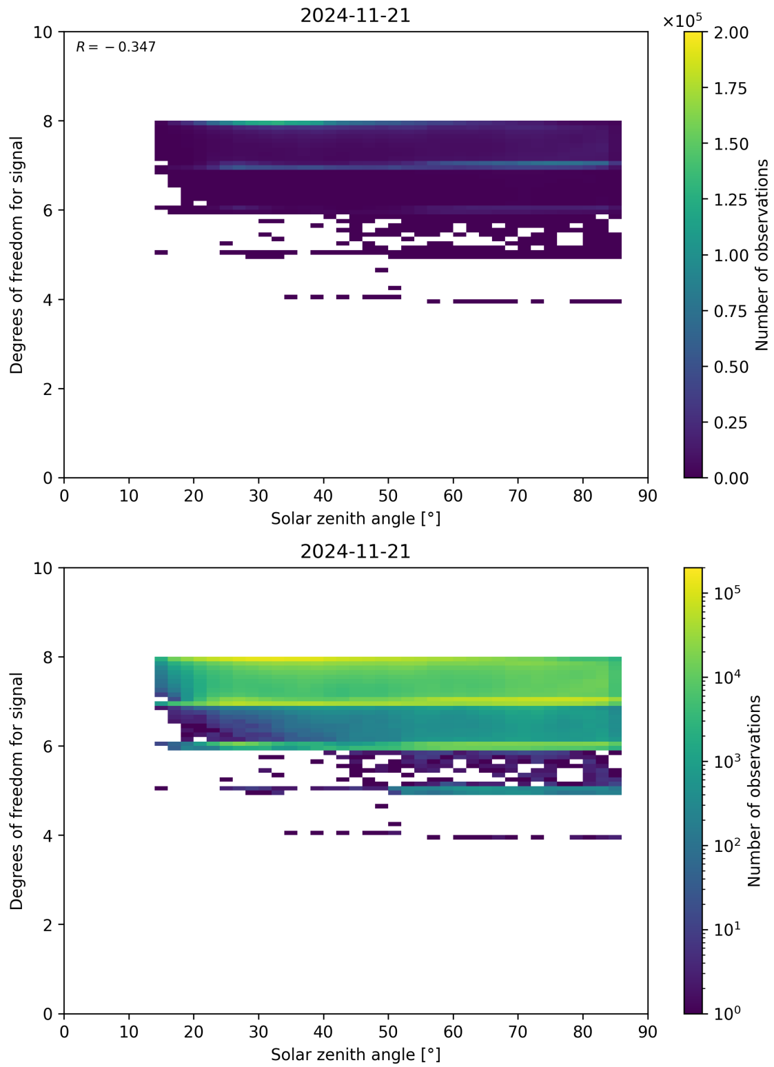
Figure 65: Scatter density plot of “Solar zenith angle” against “Degrees of freedom for signal” for 2024-11-20 to 2024-11-22.
