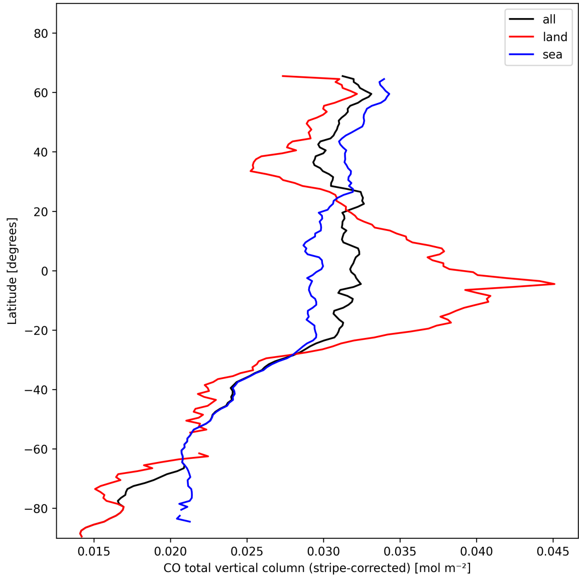
Figure 11: Zonal average of “CO total vertical column (stripe-corrected)” for 2024-11-20 to 2024-11-22.
