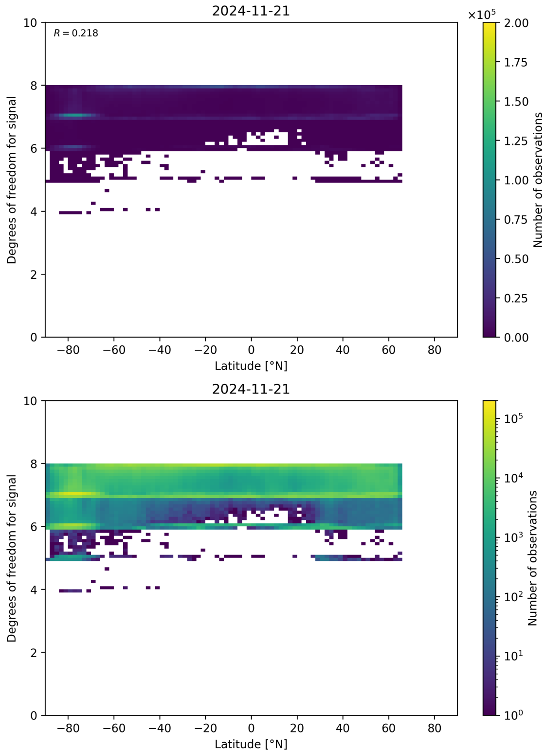
Figure 55: Scatter density plot of “Latitude” against “Degrees of freedom for signal” for 2024-11-20 to 2024-11-22.
