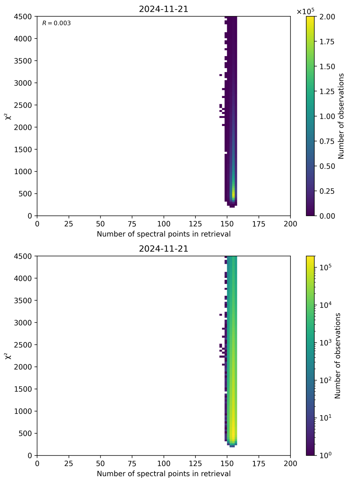
Figure 58: Scatter density plot of “Number of spectral points in retrieval” against “ \chi^2 ” for 2024-11-20 to 2024-11-22.
