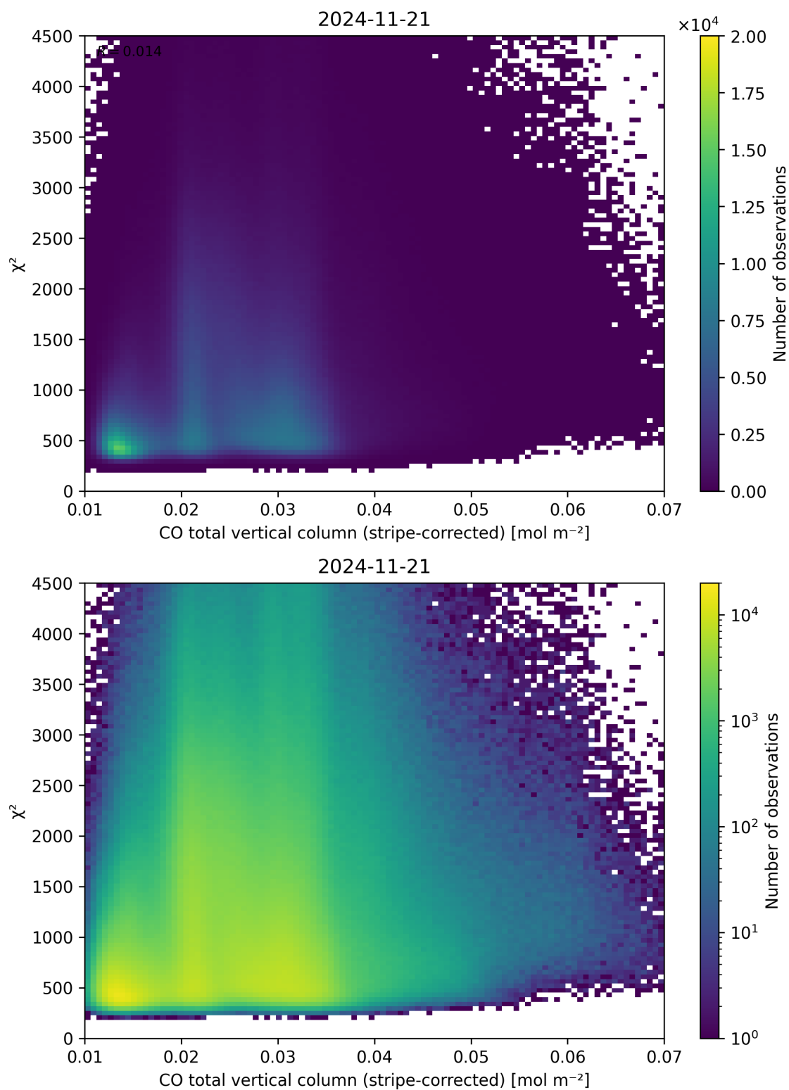
Figure 37: Scatter density plot of “CO total vertical column (stripe-corrected)” against “ \chi^2 ” for 2024-11-20 to 2024-11-22.
