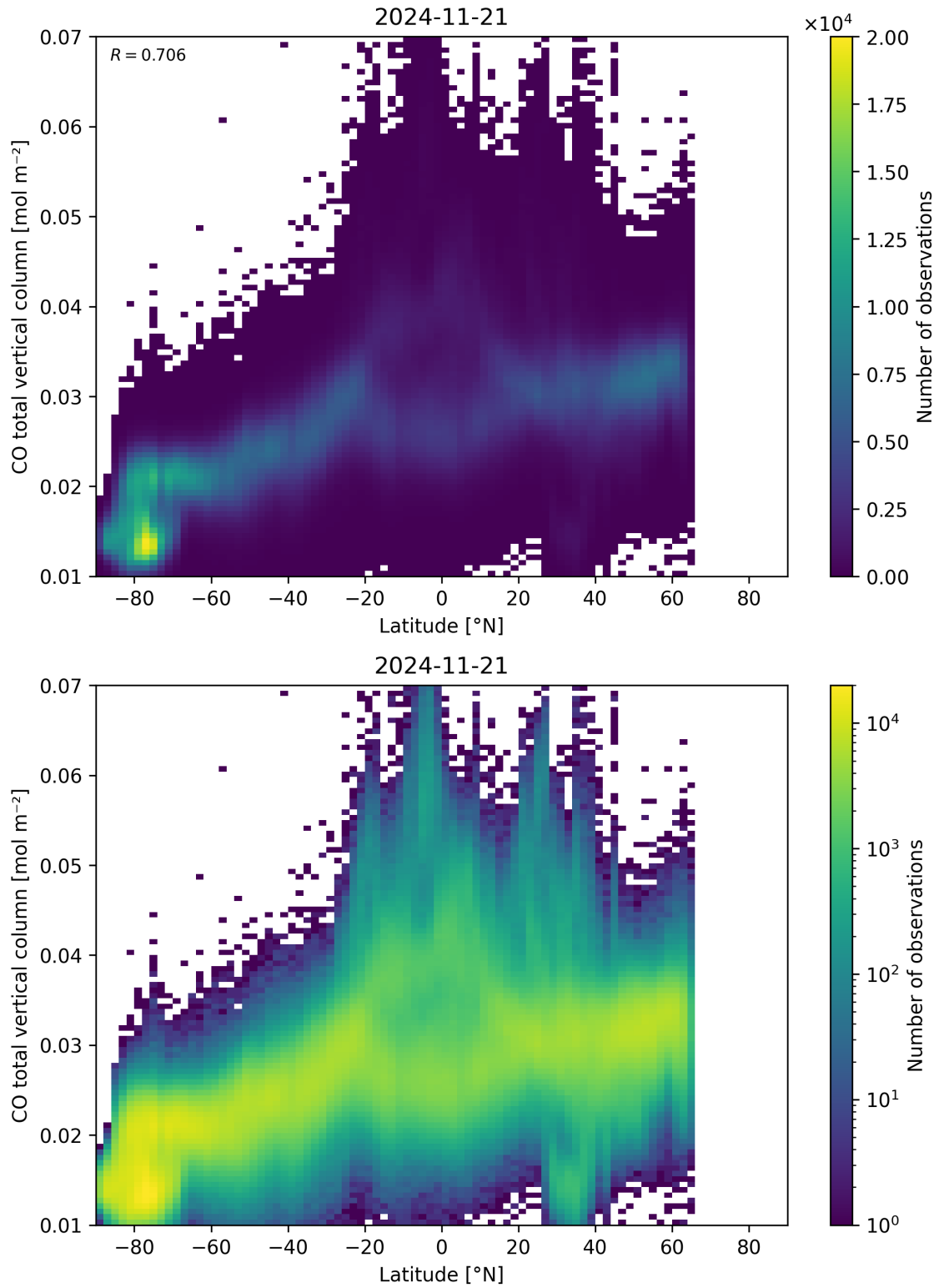
Figure 51: Scatter density plot of “Latitude” against “CO total vertical column” for 2024-11-20 to 2024-11-22.
