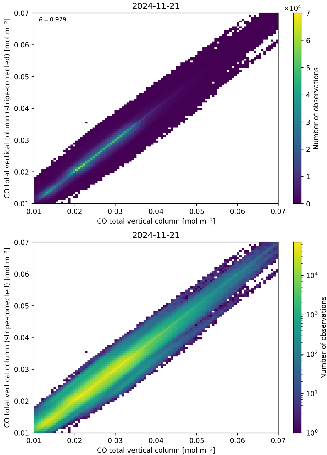
Figure 33: Scatter density plot of “CO total vertical column” against “CO total vertical column (stripe-corrected)” for 2024-11-20 to 2024-11-22.
