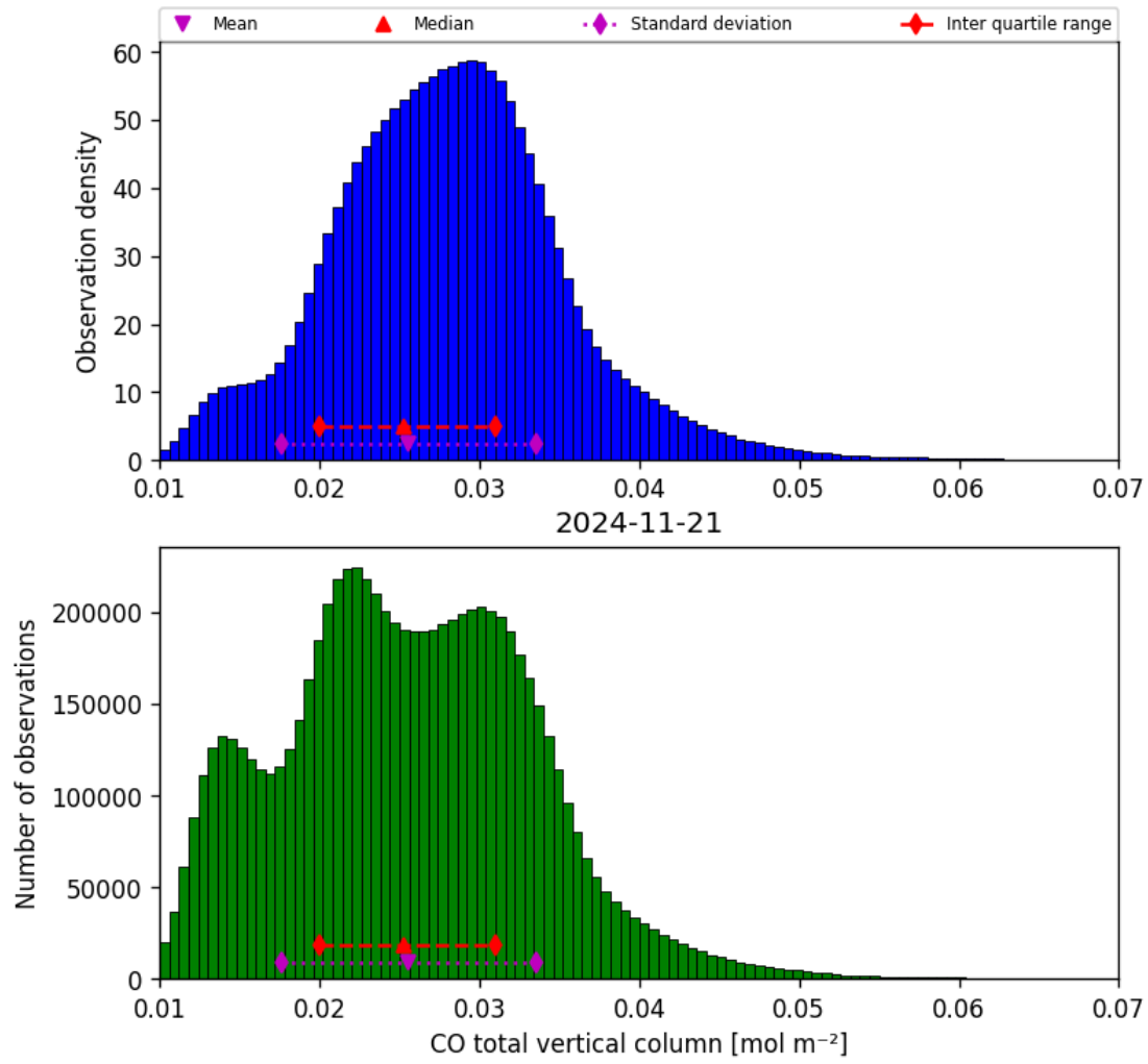
Figure 18: Histogram of “CO total vertical column” for 2024-11-20 to 2024-11-22
