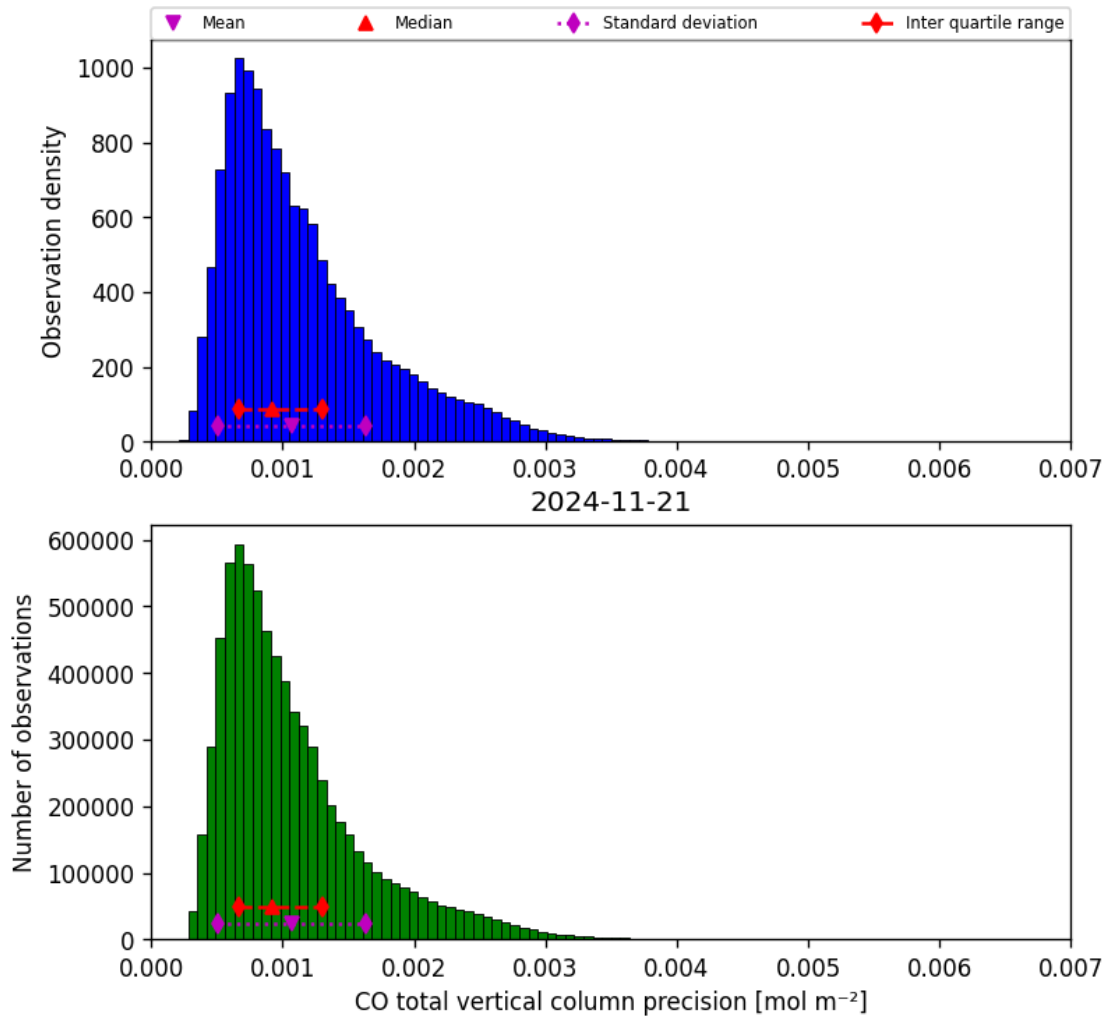
Figure 20: Histogram of “CO total vertical column precision” for 2024-11-20 to 2024-11-22
