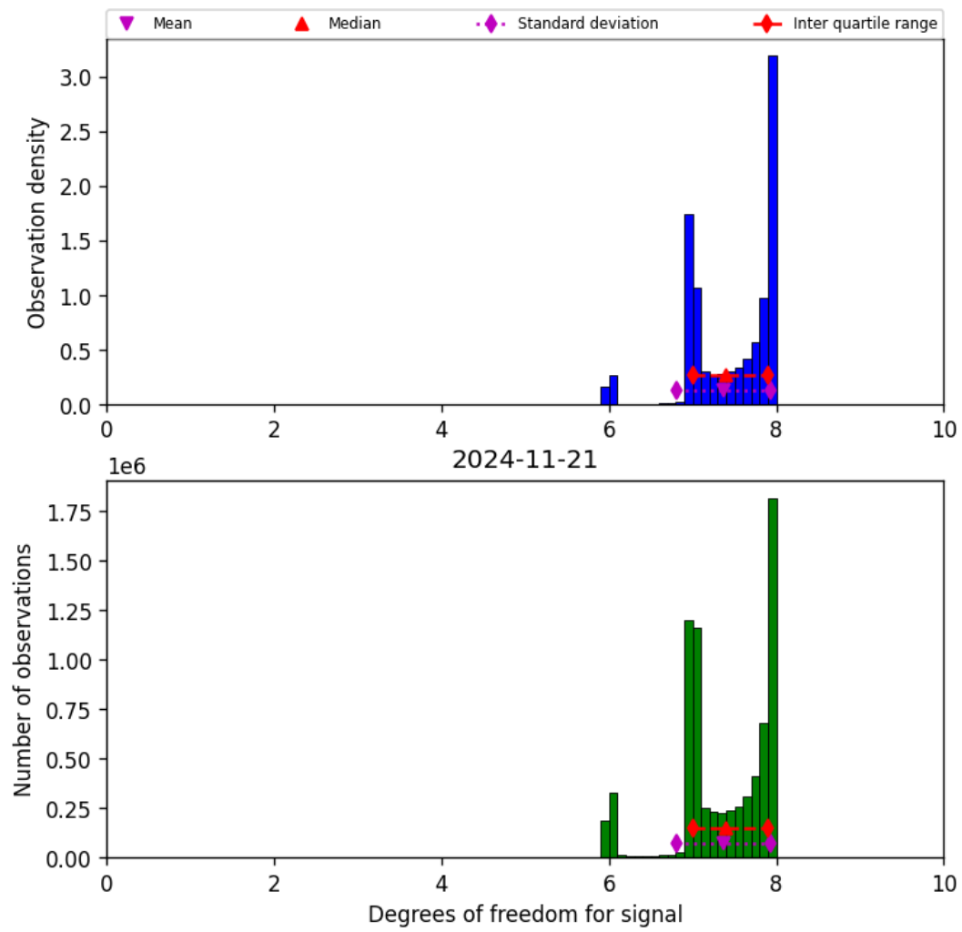
Figure 23: Histogram of “Degrees of freedom for signal” for 2024-11-20 to 2024-11-22
