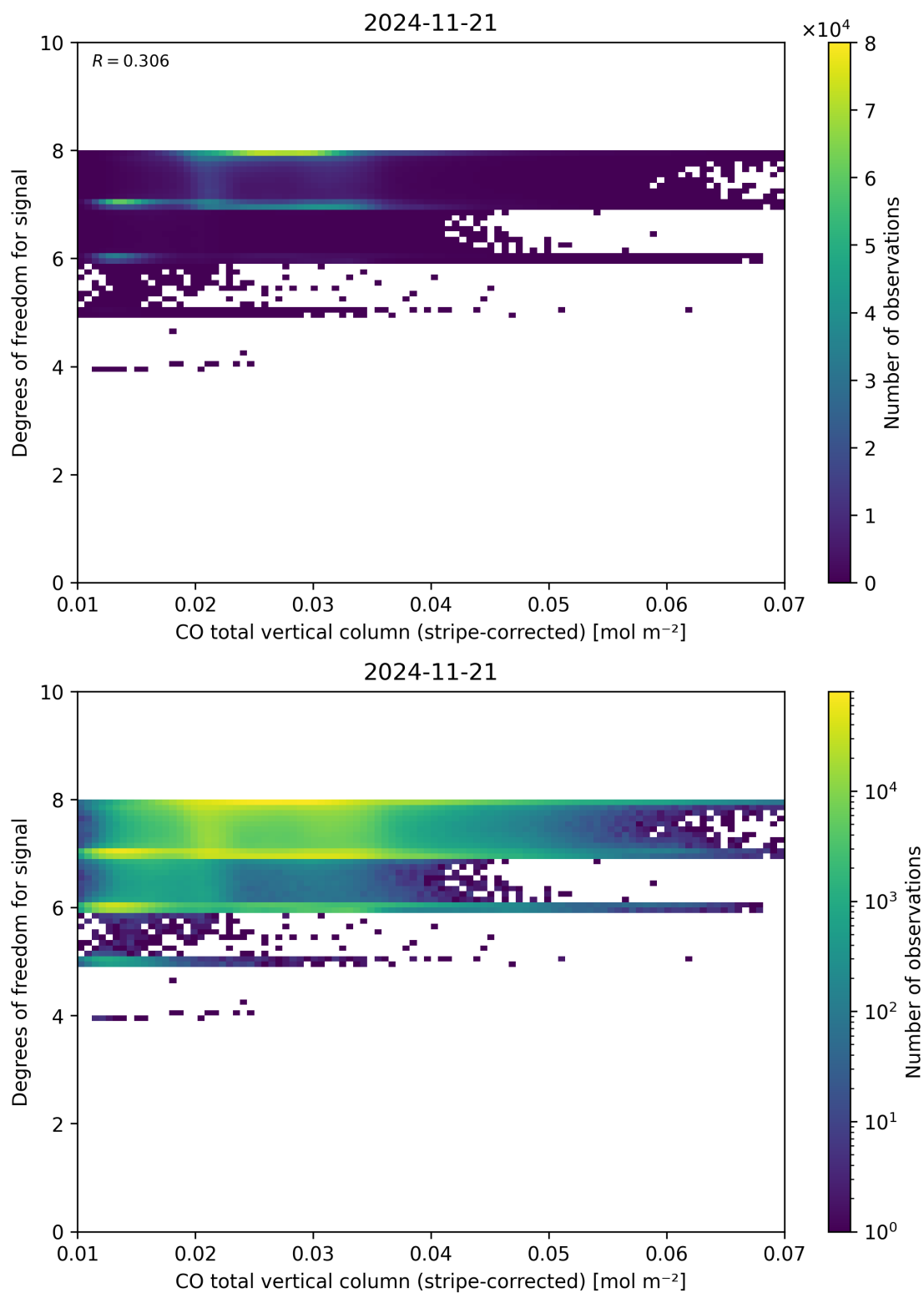
Figure 38: Scatter density plot of “CO total vertical column (stripe-corrected)” against “Degrees of freedom for signal” for 2024-11-20 to 2024-11-22.
