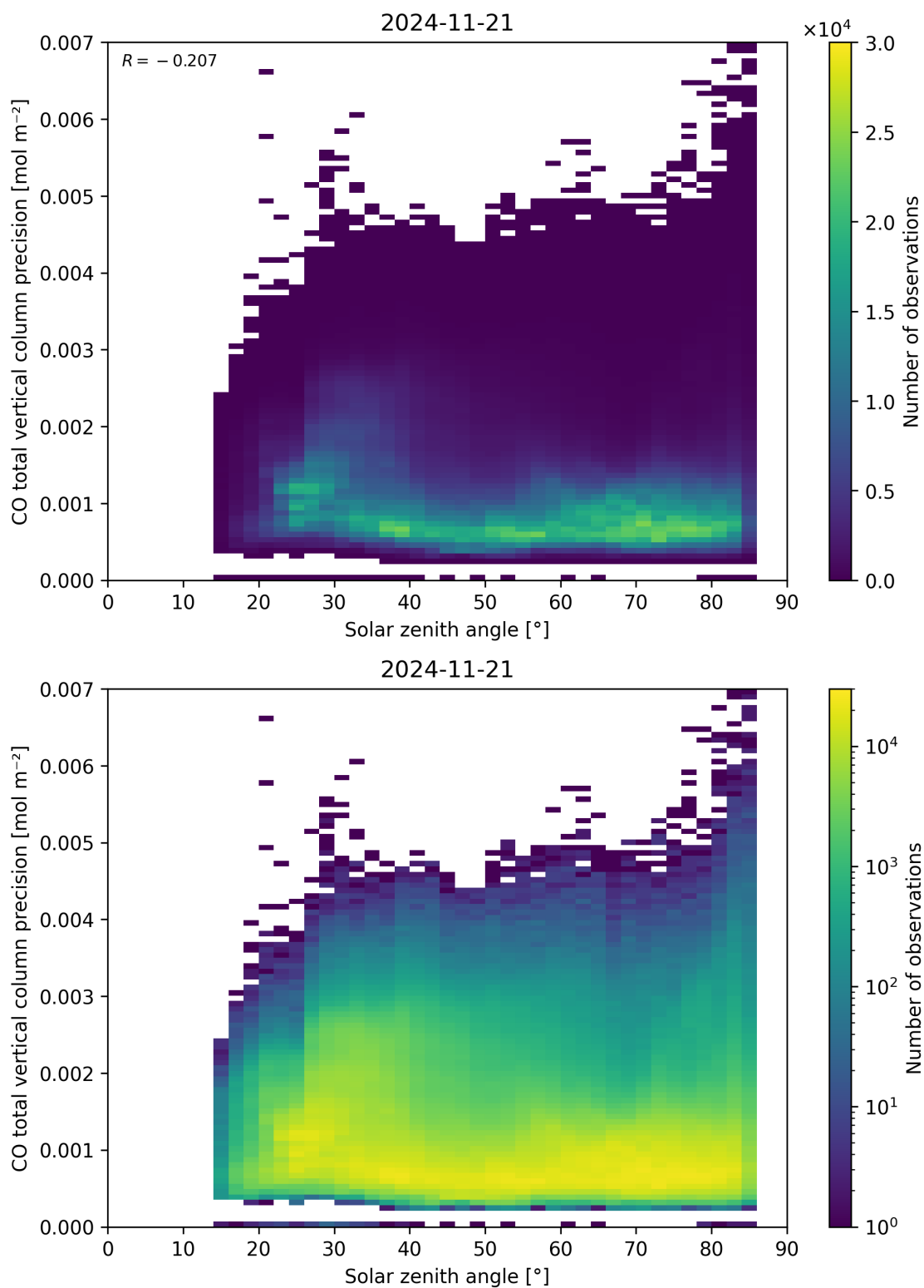
Figure 63: Scatter density plot of “Solar zenith angle” against “CO total vertical column precision” for 2024-11-20 to 2024-11-22.
