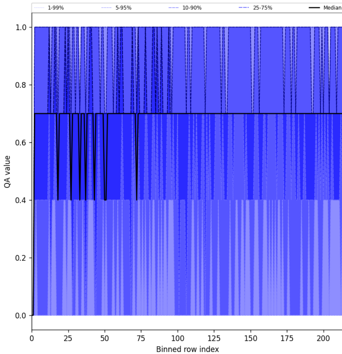
Figure 25: Along track statistics of “QA value” for 2024-11-20 to 2024-11-22
