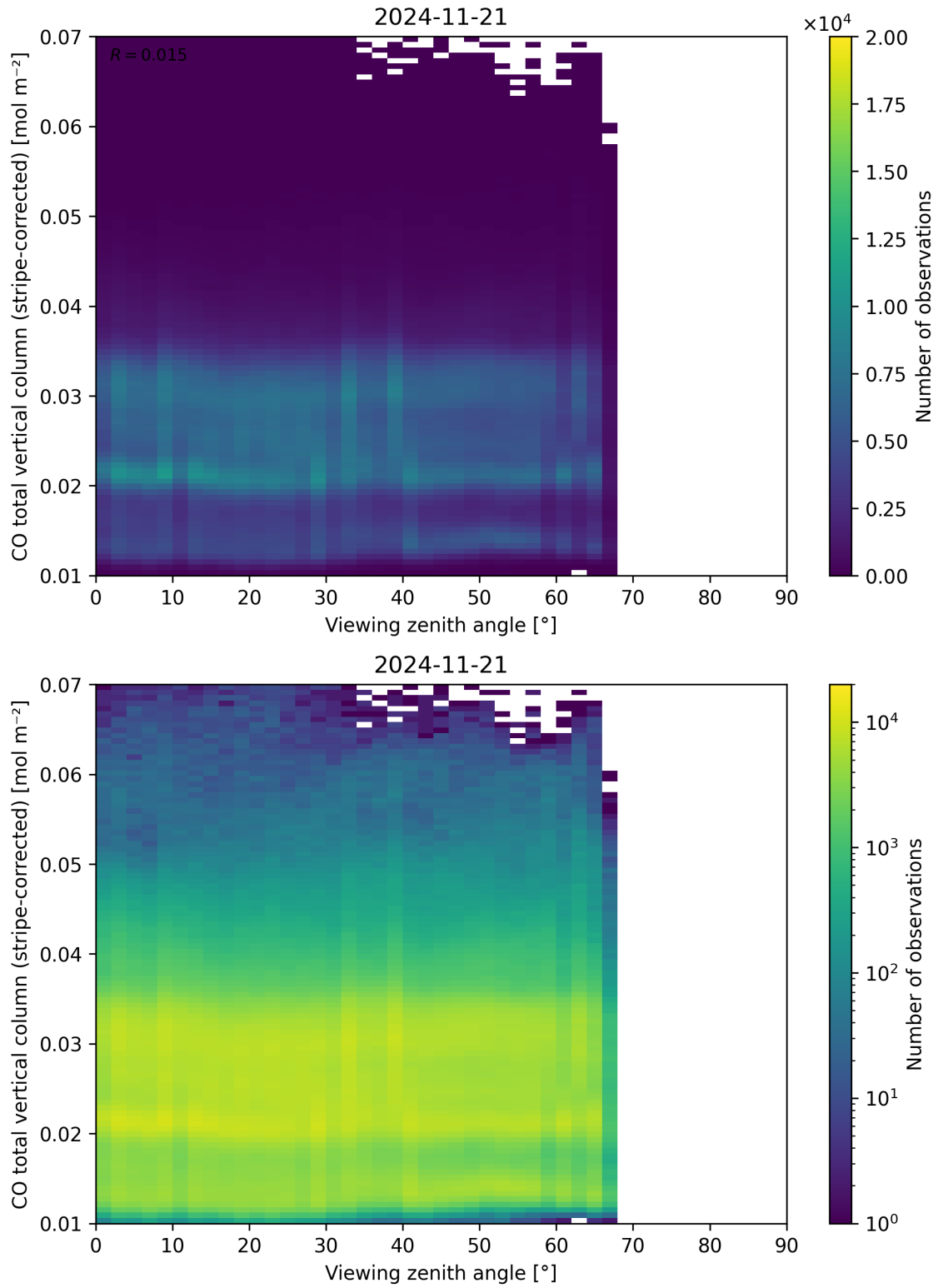
Figure 70: Scatter density plot of “Viewing zenith angle” against “CO total vertical column (stripe-corrected)” for 2024-11-20 to 2024-11-22.
