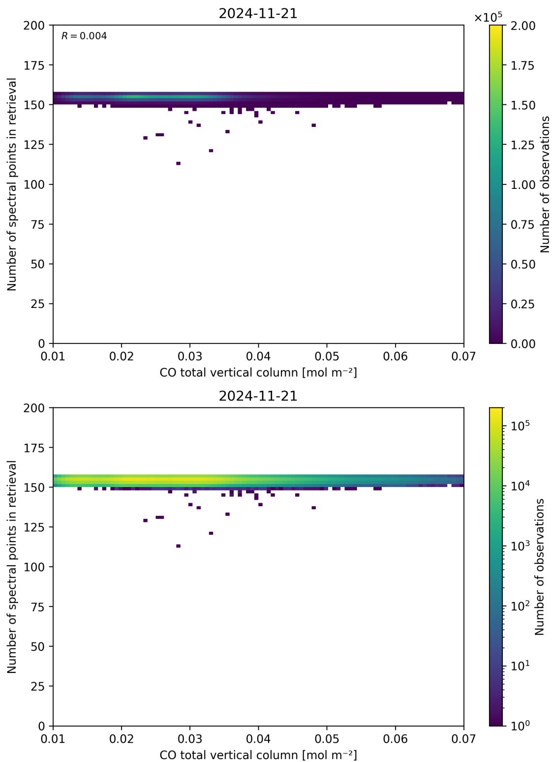
Figure 43: Scatter density plot of “CO total vertical column” against “Number of spectral points in retrieval” for 2024-11-20 to 2024-11-22.
