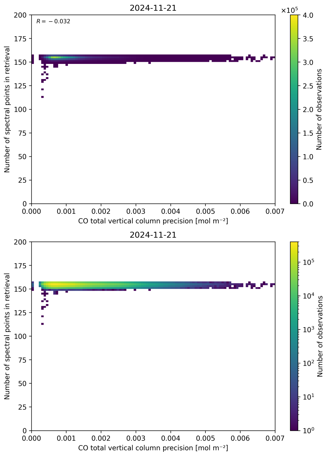
Figure 47: Scatter density plot of “CO total vertical column precision” against “Number of spectral points in retrieval” for 2024-11-20 to 2024-11-22.
