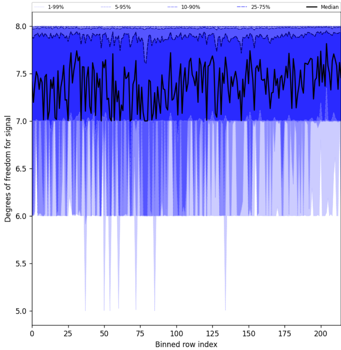
Figure 31: Along track statistics of “Degrees of freedom for signal” for 2024-11-20 to 2024-11-22
