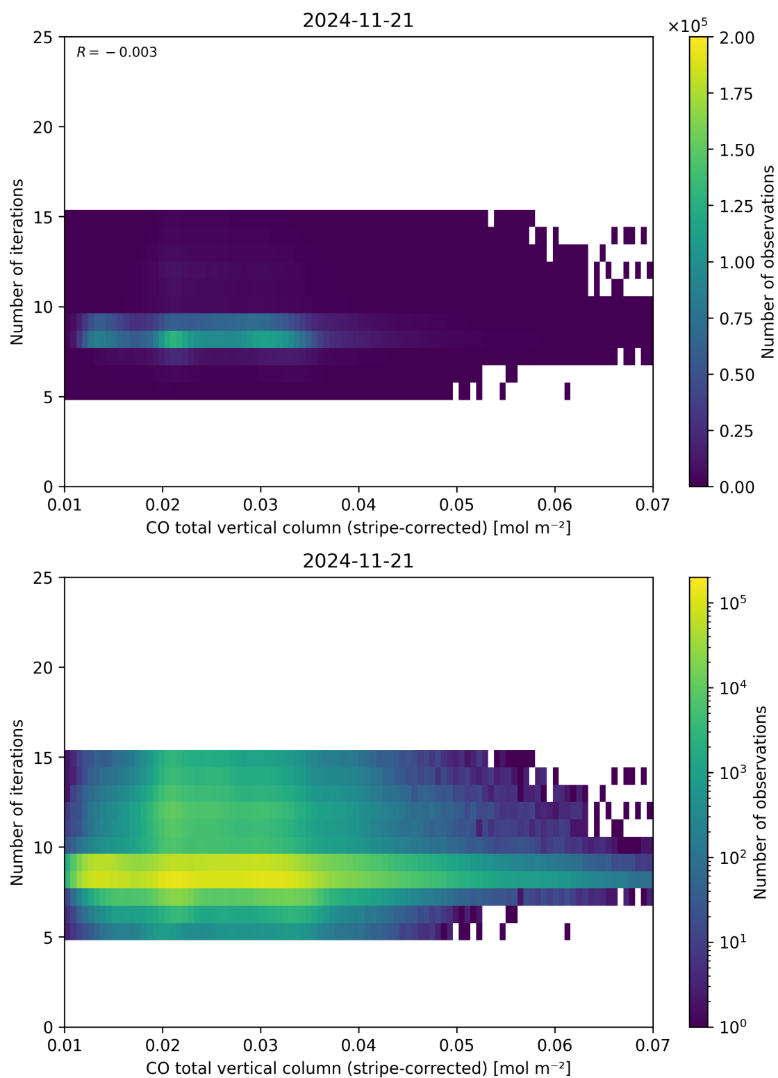
Figure 39: Scatter density plot of “CO total vertical column (stripe-corrected)” against “Number of iterations” for 2024-11-20 to 2024-11-22.
