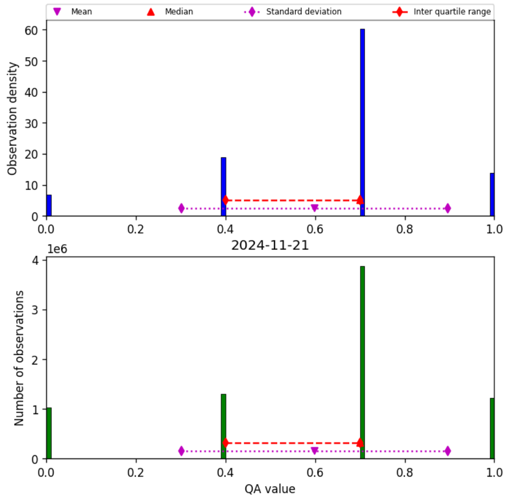
Figure 17: Histogram of “QA value” for 2024-11-20 to 2024-11-22
