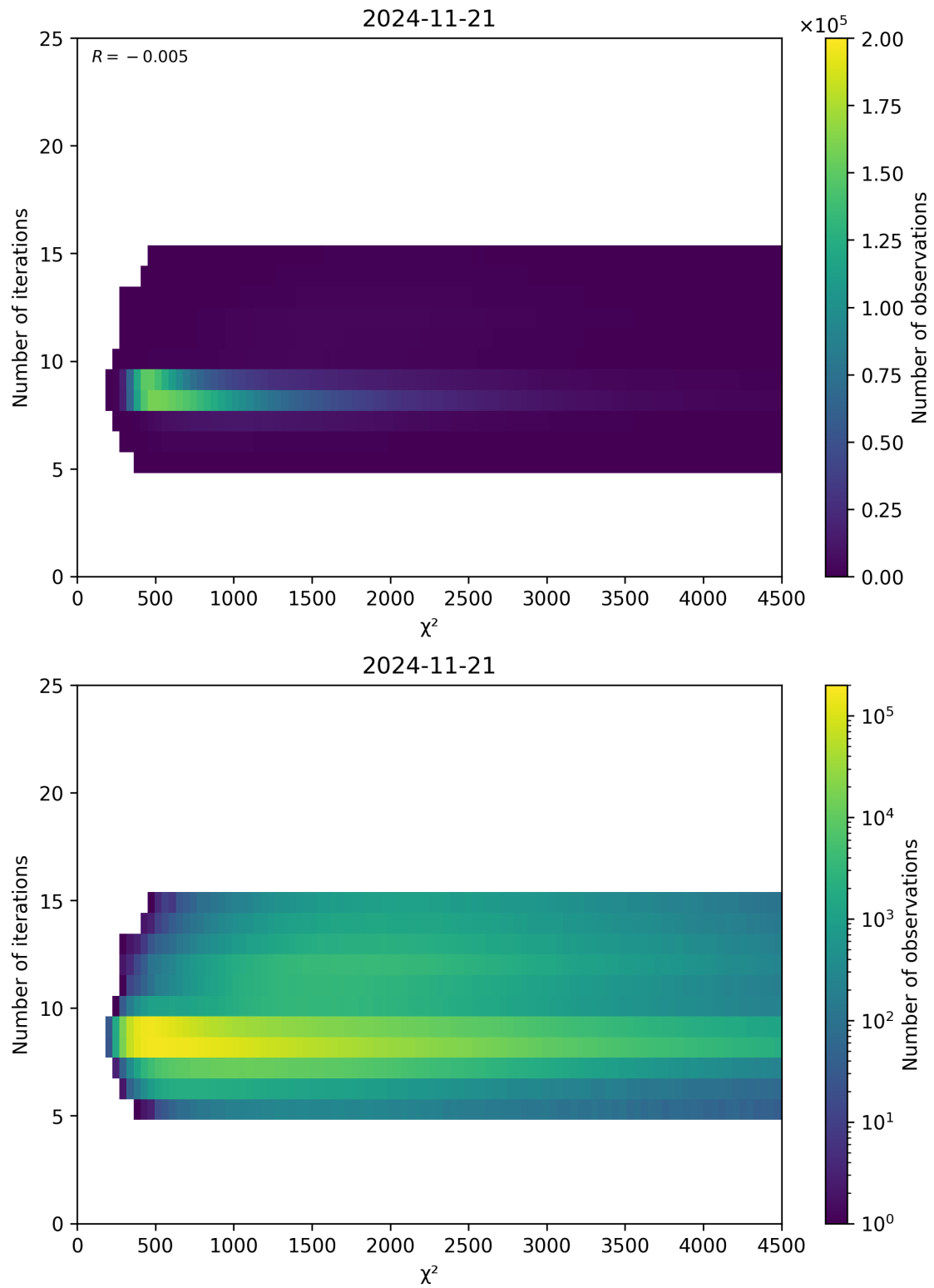
Figure 49: Scatter density plot of “ \chi^2 ” against “Number of iterations” for 2024-11-20 to 2024-11-22.
