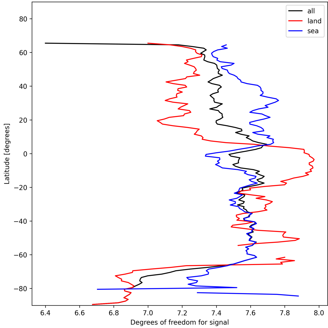
Figure 15: Zonal average of “Degrees of freedom for signal” for 2024-11-20 to 2024-11-22.
