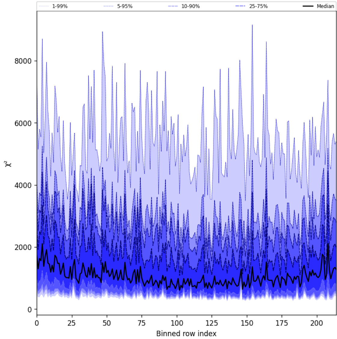
Figure 30: Along track statistics of “ \chi^2 ” for 2024-11-20 to 2024-11-22
