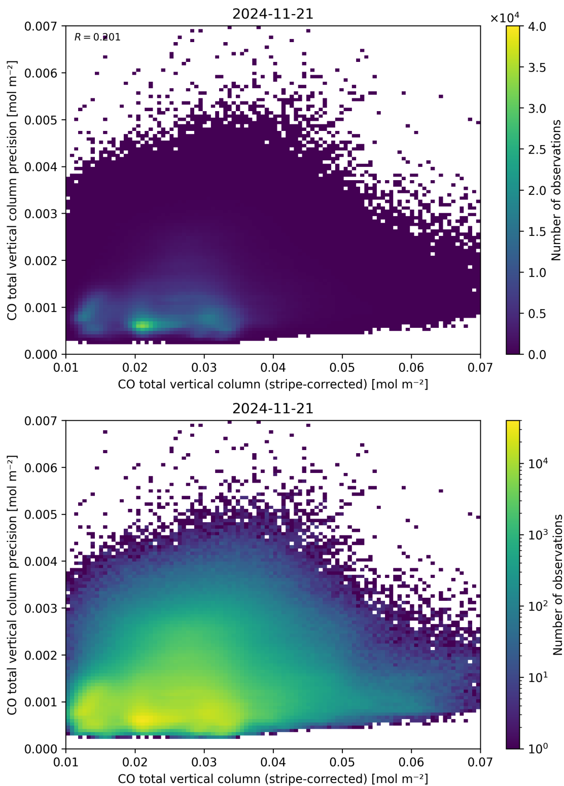
Figure 36: Scatter density plot of “CO total vertical column (stripe-corrected)” against “CO total vertical column precision” for 2024-11-20 to 2024-11-22.
