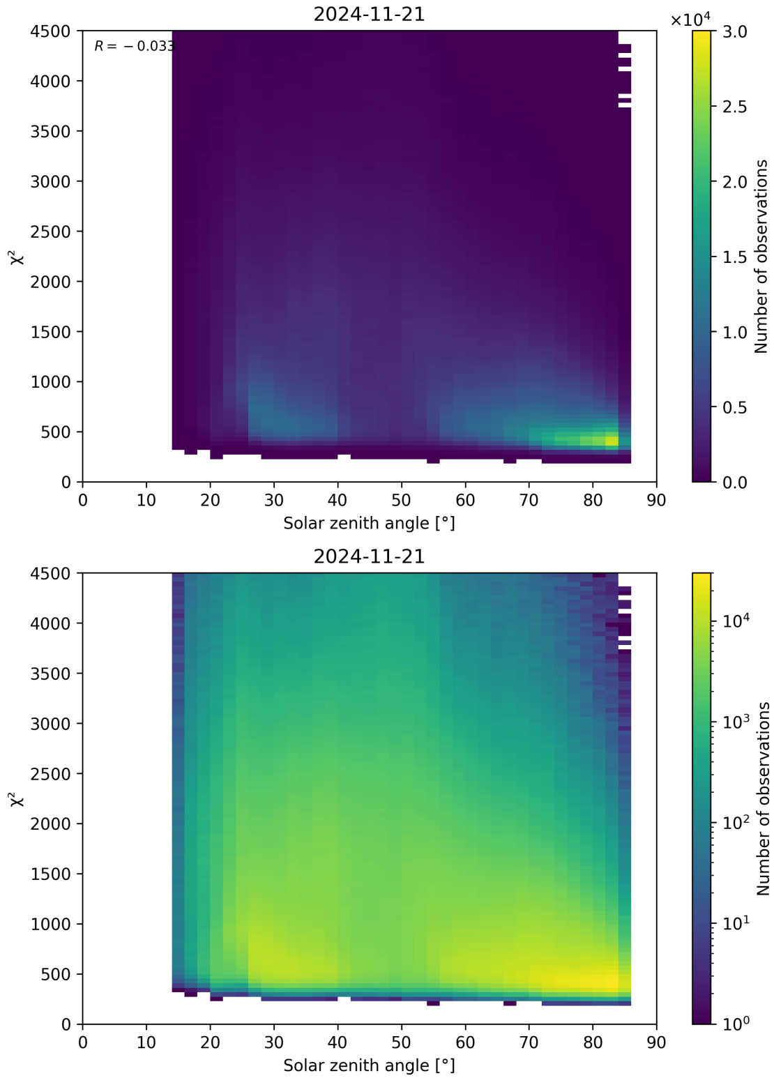
Figure 64: Scatter density plot of “Solar zenith angle” against “ \chi^2 ” for 2024-11-20 to 2024-11-22.
