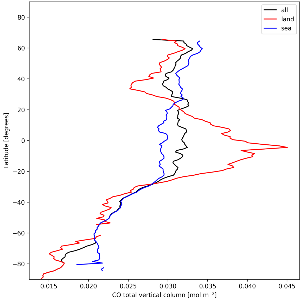
Figure 10: Zonal average of “CO total vertical column” for 2024-11-20 to 2024-11-22.
