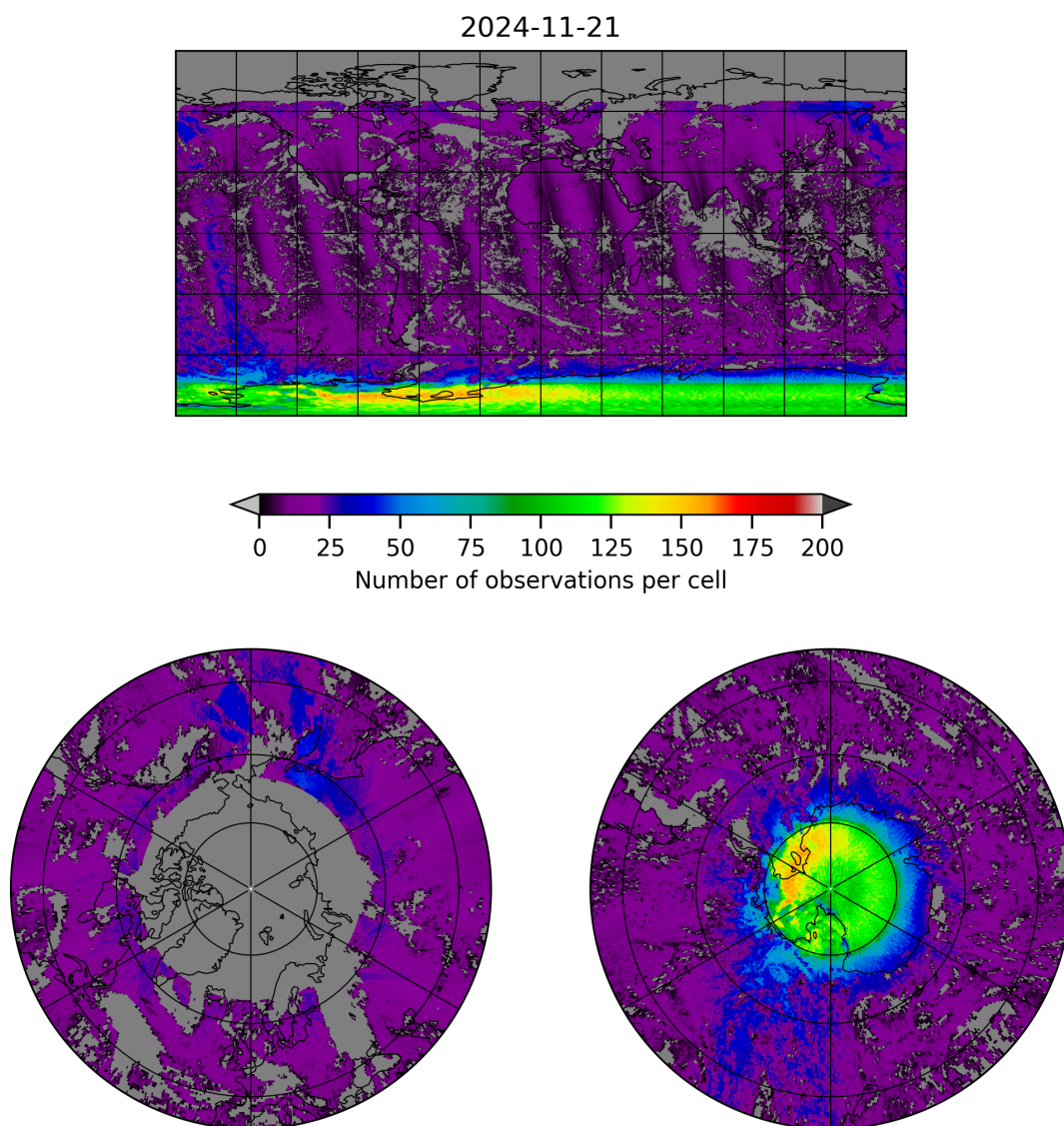
Figure 8: Map of the number of observations for 2024-11-20 to 2024-11-22
