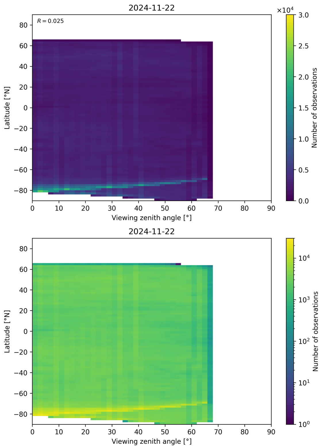
Figure 74: Scatter density plot of “Viewing zenith angle” against “Latitude” for 2024-11-21 to 2024-11-23.
