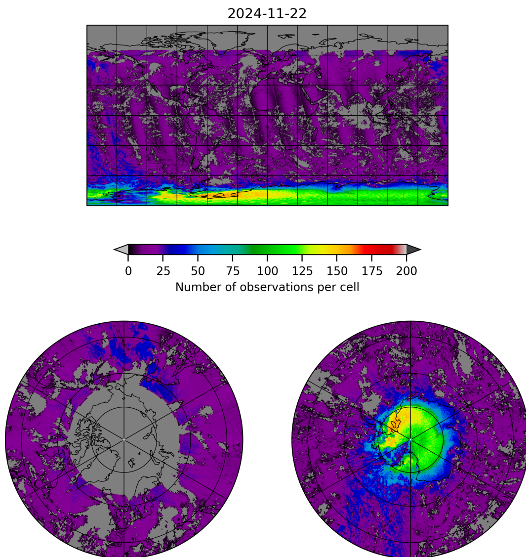
Figure 8: Map of the number of observations for 2024-11-21 to 2024-11-23
