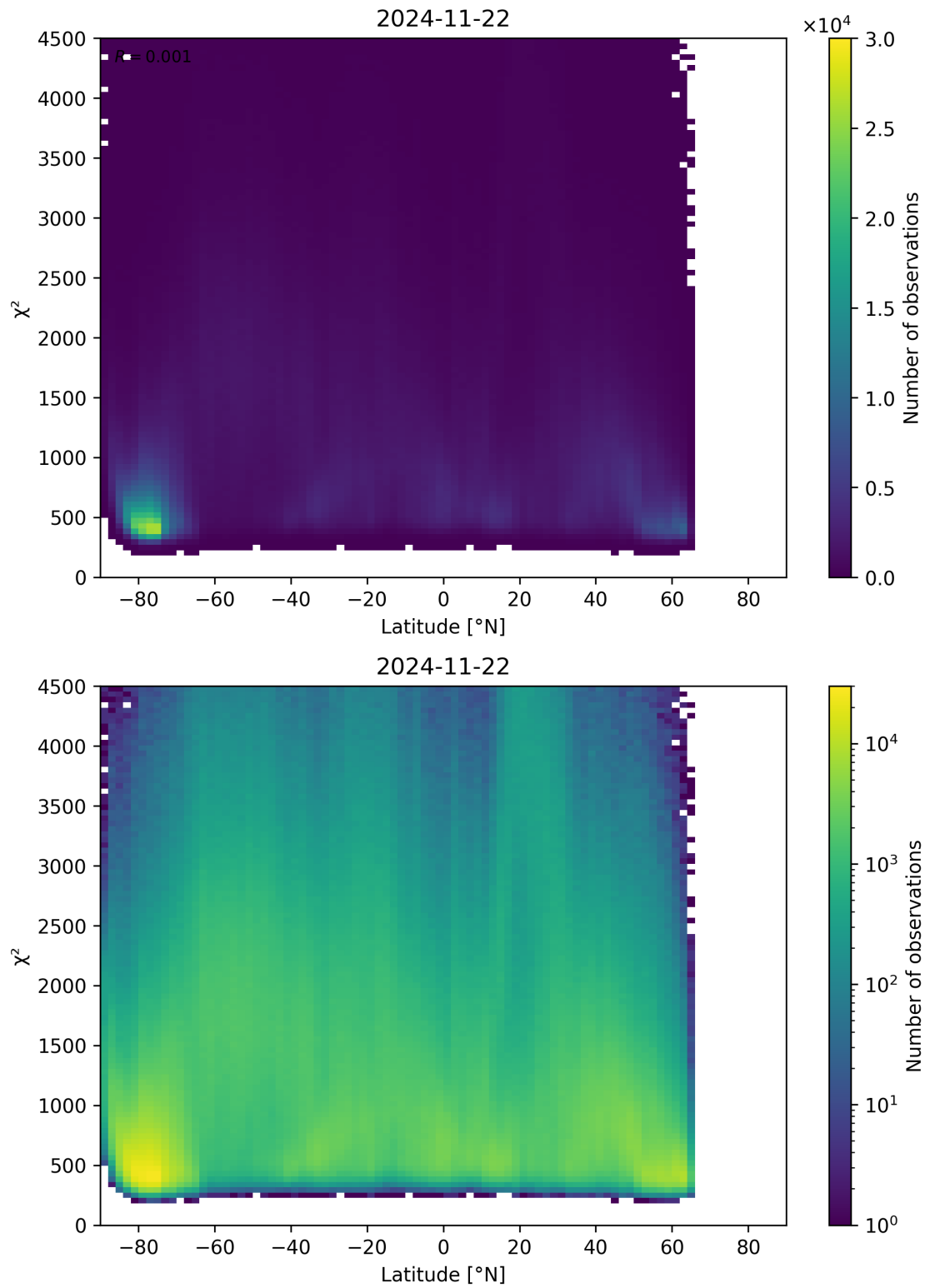
Figure 54: Scatter density plot of “Latitude” against “ \chi^2 ” for 2024-11-21 to 2024-11-23.
