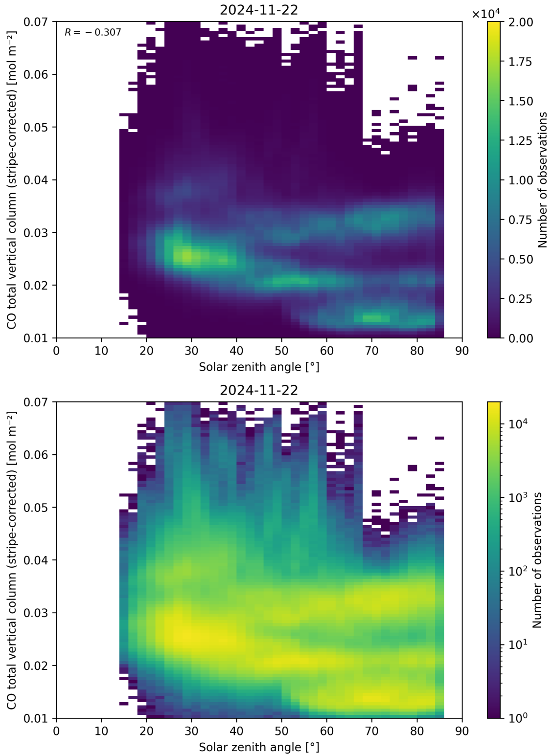
Figure 62: Scatter density plot of “Solar zenith angle” against “CO total vertical column (stripe-corrected)” for 2024-11-21 to 2024-11-23.
