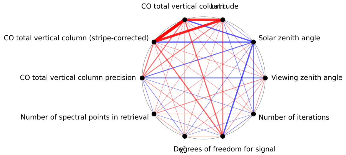
Figure 1: Map of correlation graph for 2024-11-21 to 2024-11-23.
