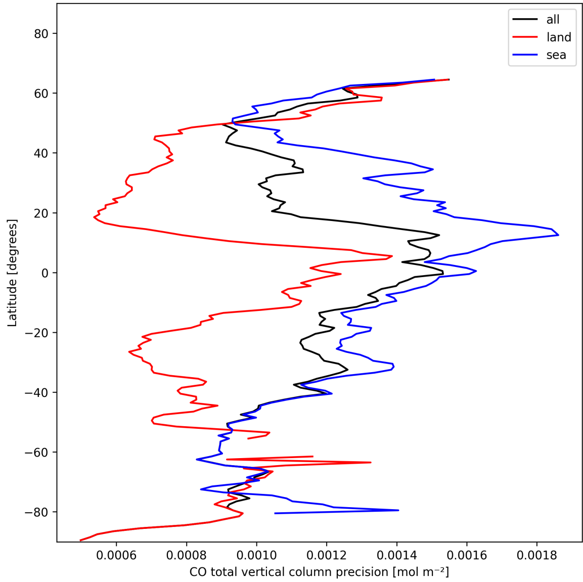
Figure 12: Zonal average of “CO total vertical column precision” for 2024-11-21 to 2024-11-23.
