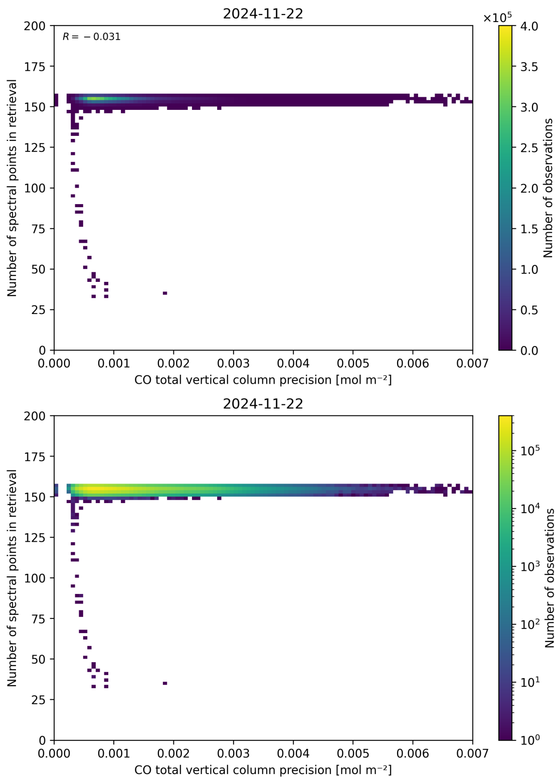
Figure 47: Scatter density plot of “CO total vertical column precision” against “Number of spectral points in retrieval” for 2024-11-21 to 2024-11-23.
