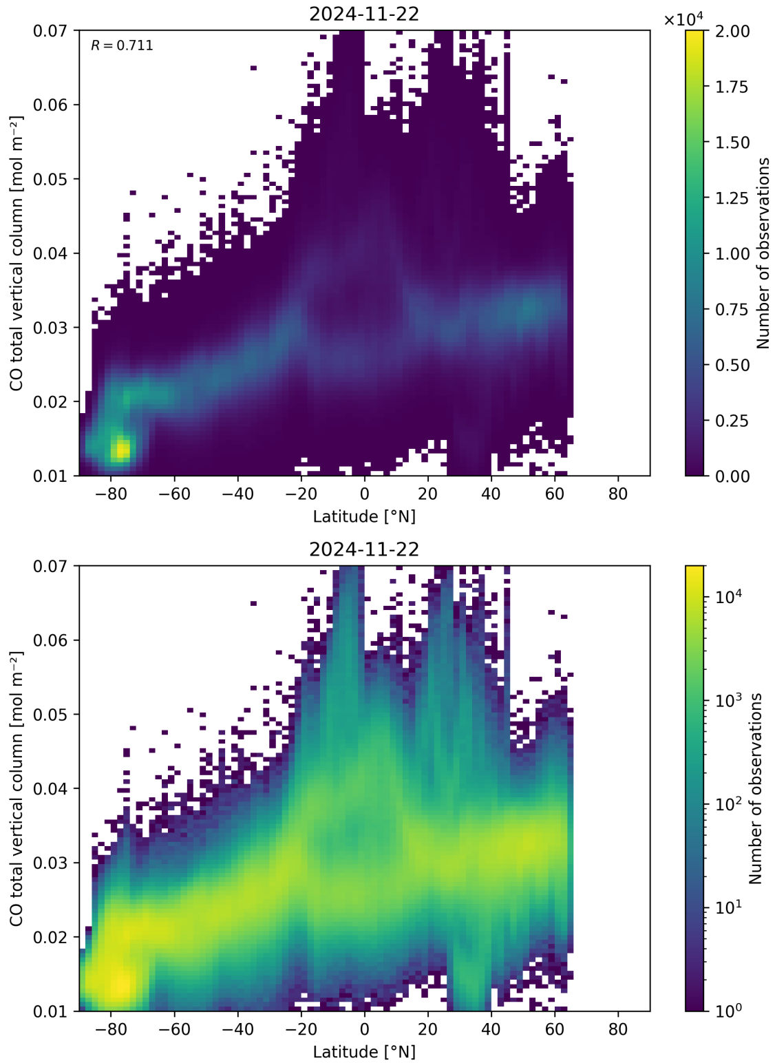
Figure 51: Scatter density plot of “Latitude” against “CO total vertical column” for 2024-11-21 to 2024-11-23.
