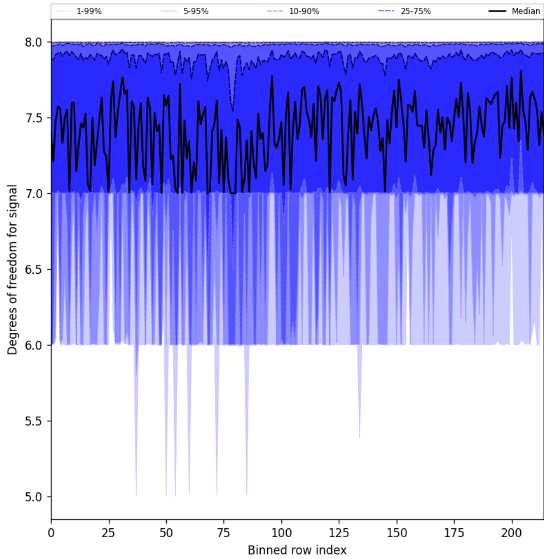
Figure 31: Along track statistics of “Degrees of freedom for signal” for 2024-11-21 to 2024-11-23
