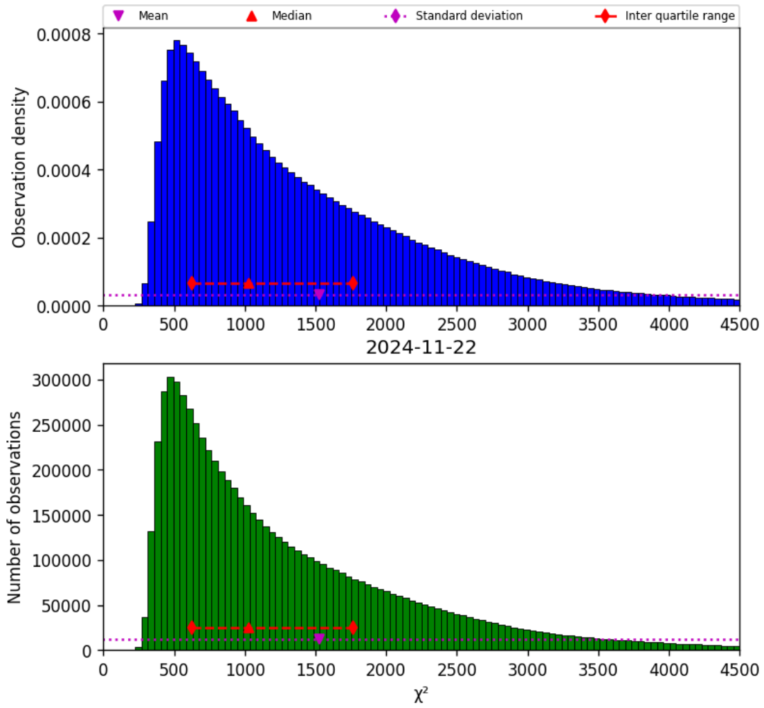
Figure 22: Histogram of “ \chi^2 ” for 2024-11-21 to 2024-11-23
