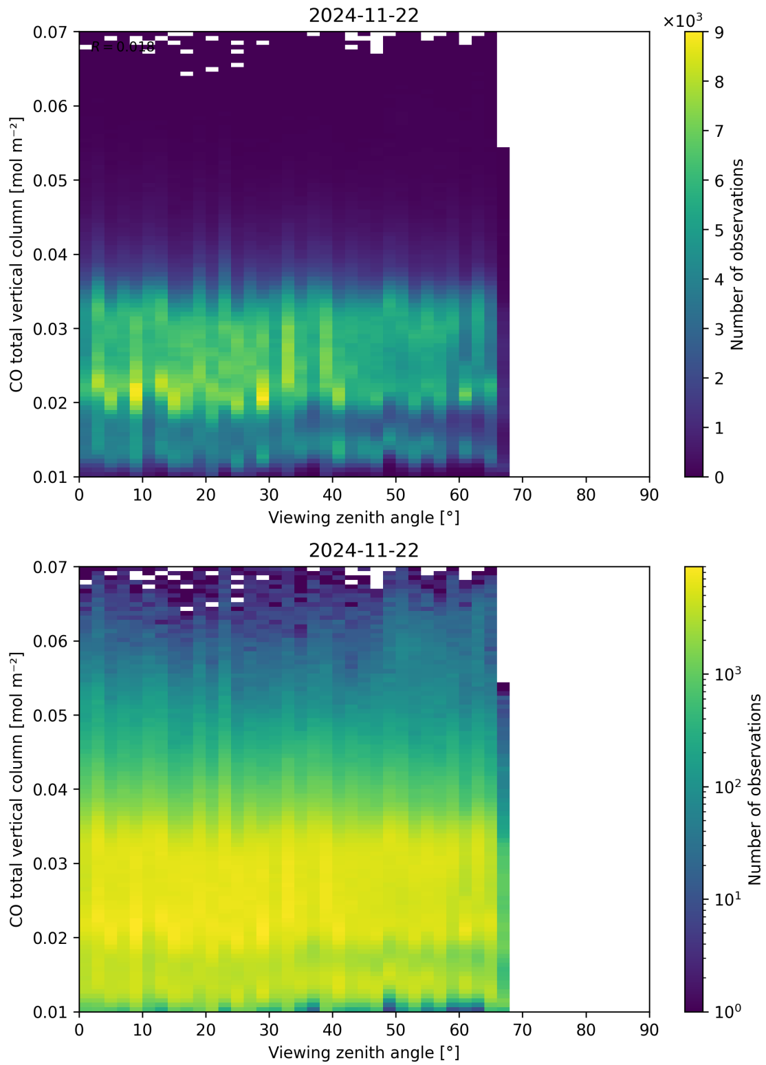
Figure 69: Scatter density plot of “Viewing zenith angle” against “CO total vertical column” for 2024-11-21 to 2024-11-23.
