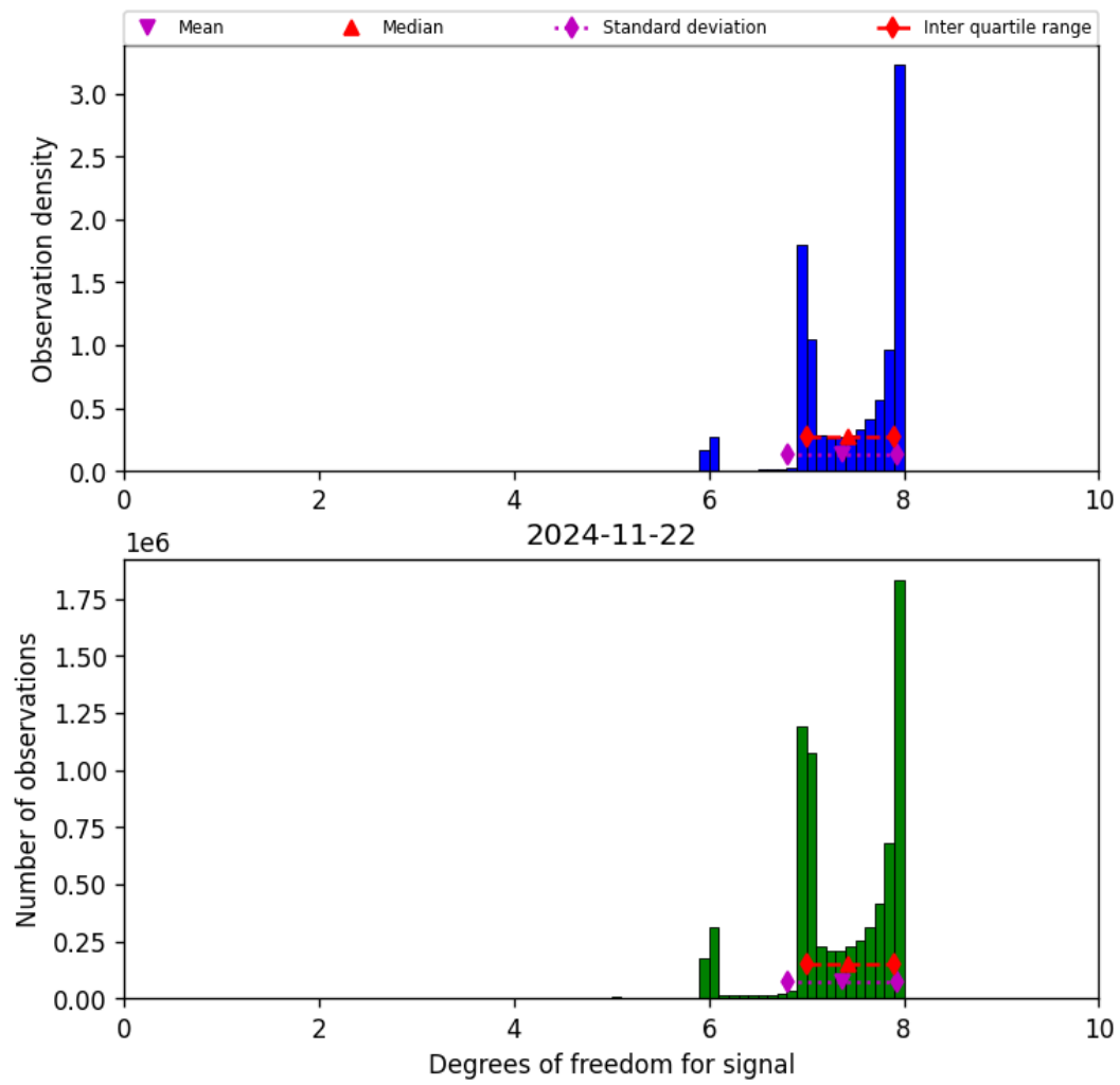
Figure 23: Histogram of “Degrees of freedom for signal” for 2024-11-21 to 2024-11-23
