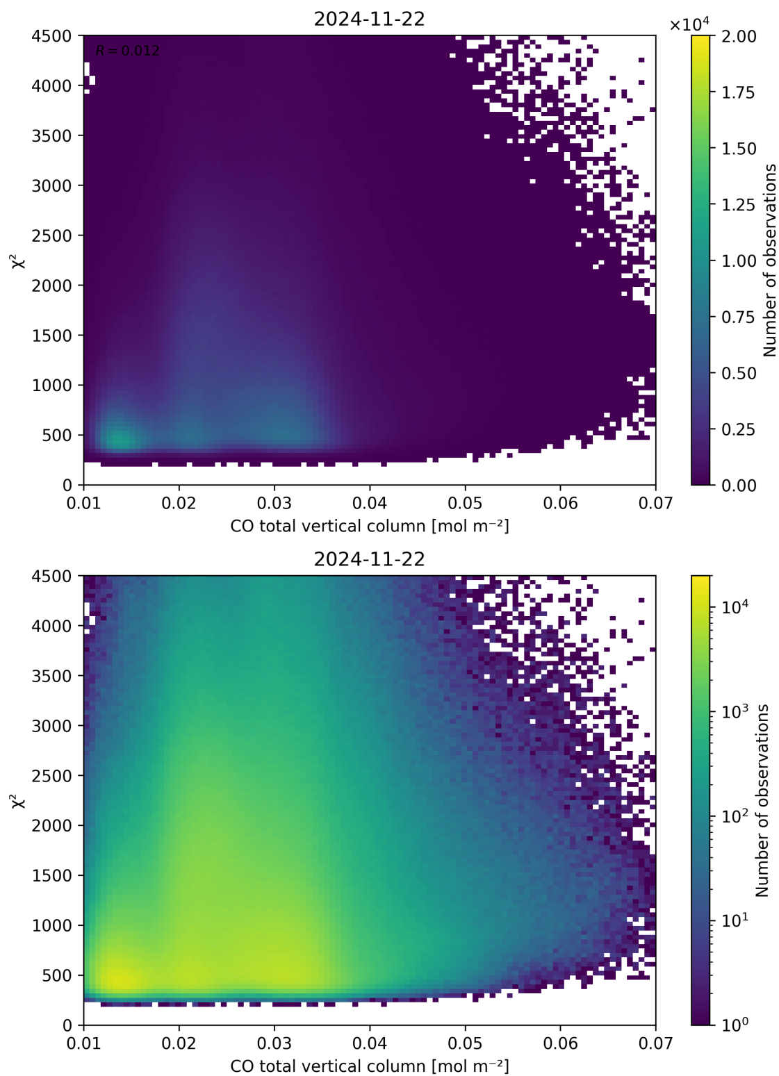
Figure 35: Scatter density plot of “CO total vertical column” against “ \chi^2 ” for 2024-11-21 to 2024-11-23.
