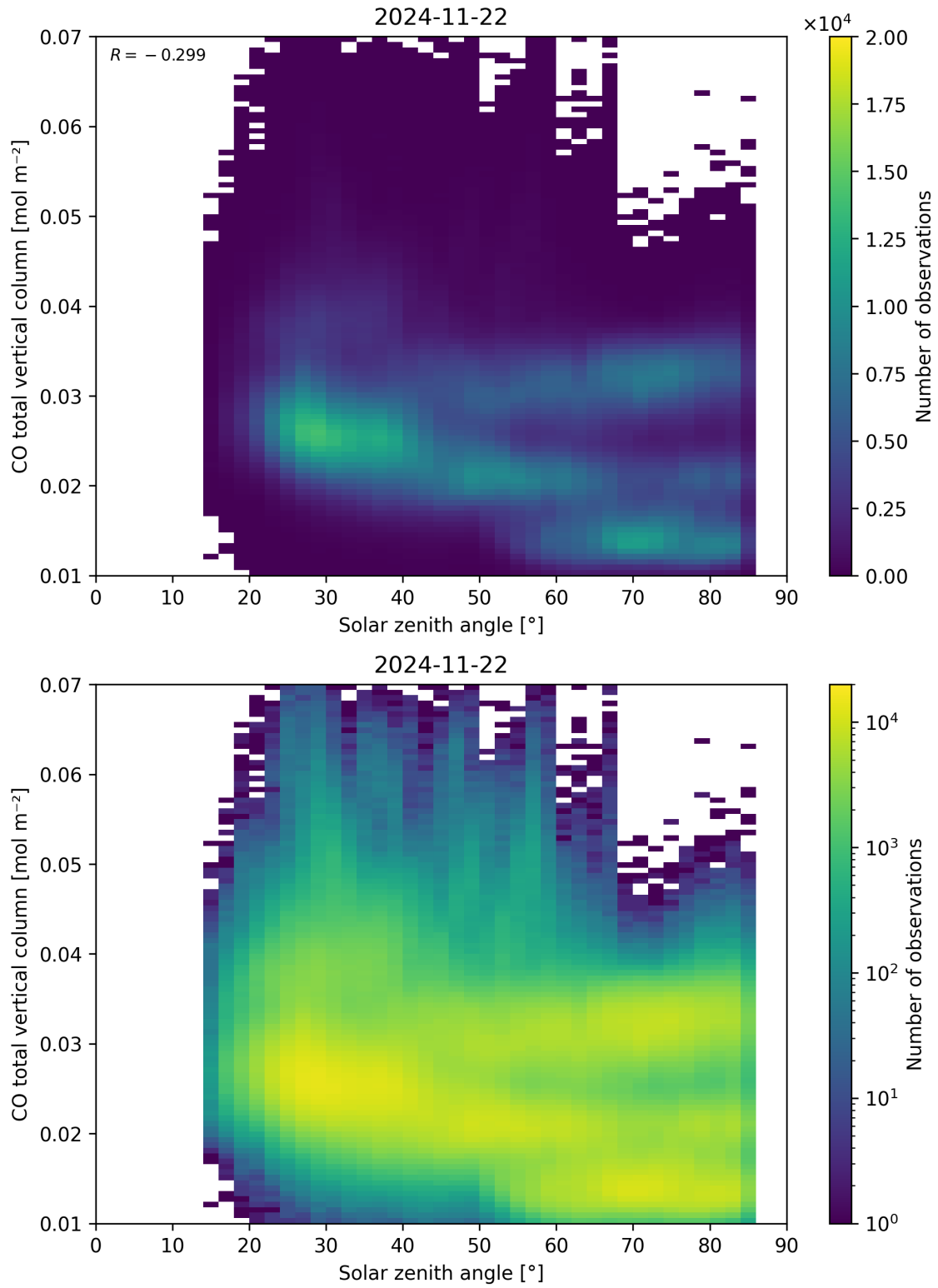
Figure 61: Scatter density plot of “Solar zenith angle” against “CO total vertical column” for 2024-11-21 to 2024-11-23.
