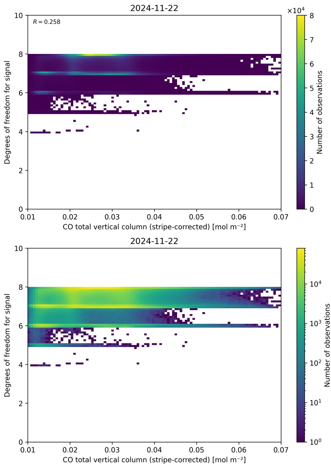
Figure 38: Scatter density plot of “CO total vertical column (stripe-corrected)” against “Degrees of freedom for signal” for 2024-11-21 to 2024-11-23.
