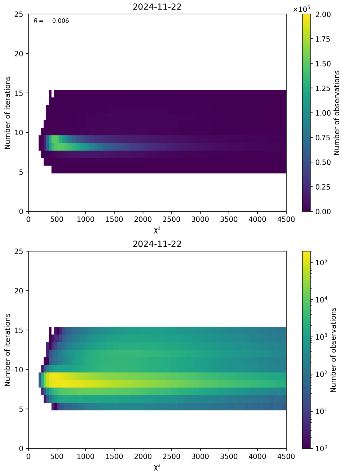
Figure 49: Scatter density plot of “ \chi^2 ” against “Number of iterations” for 2024-11-21 to 2024-11-23.
