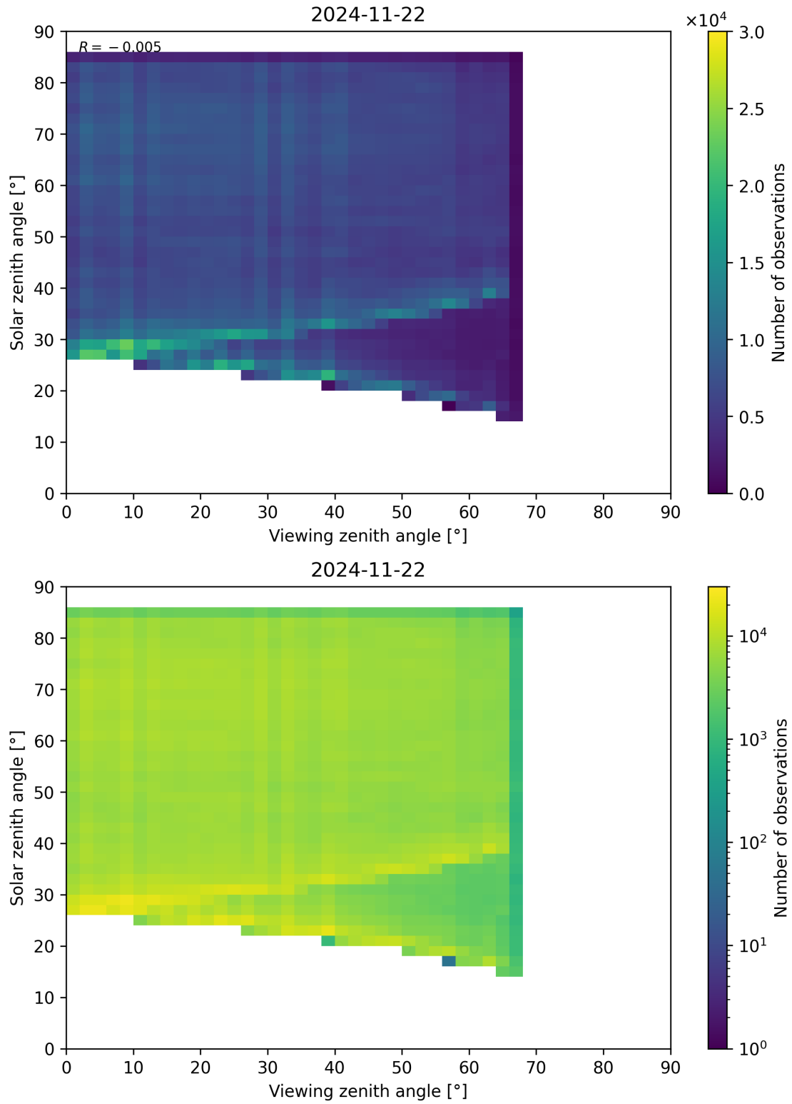
Figure 77: Scatter density plot of “Viewing zenith angle” against “Solar zenith angle” for 2024-11-21 to 2024-11-23.
