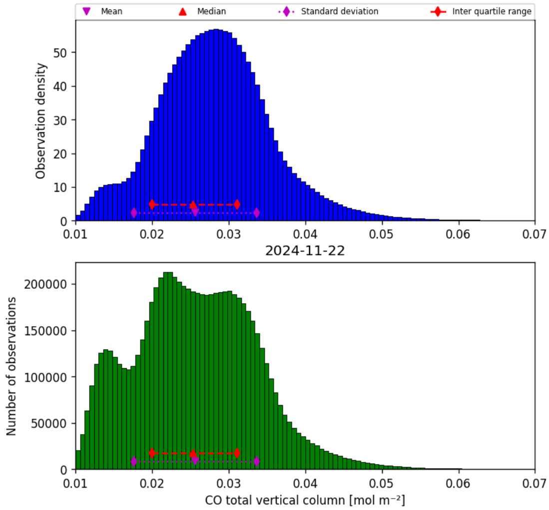
Figure 18: Histogram of “CO total vertical column” for 2024-11-21 to 2024-11-23
