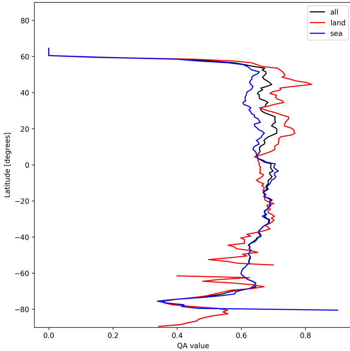
Figure 9: Zonal average of “QA value” for 2024-11-21 to 2024-11-23.
