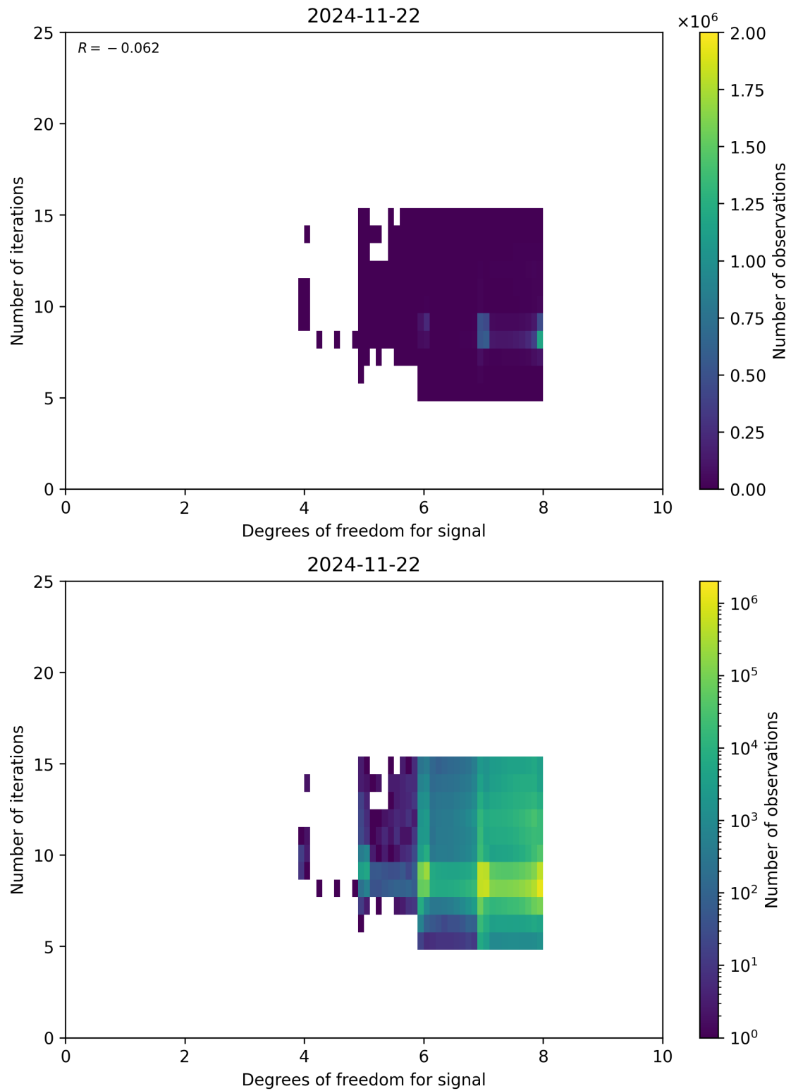
Figure 50: Scatter density plot of “Degrees of freedom for signal” against “Number of iterations” for 2024-11-21 to 2024-11-23.
