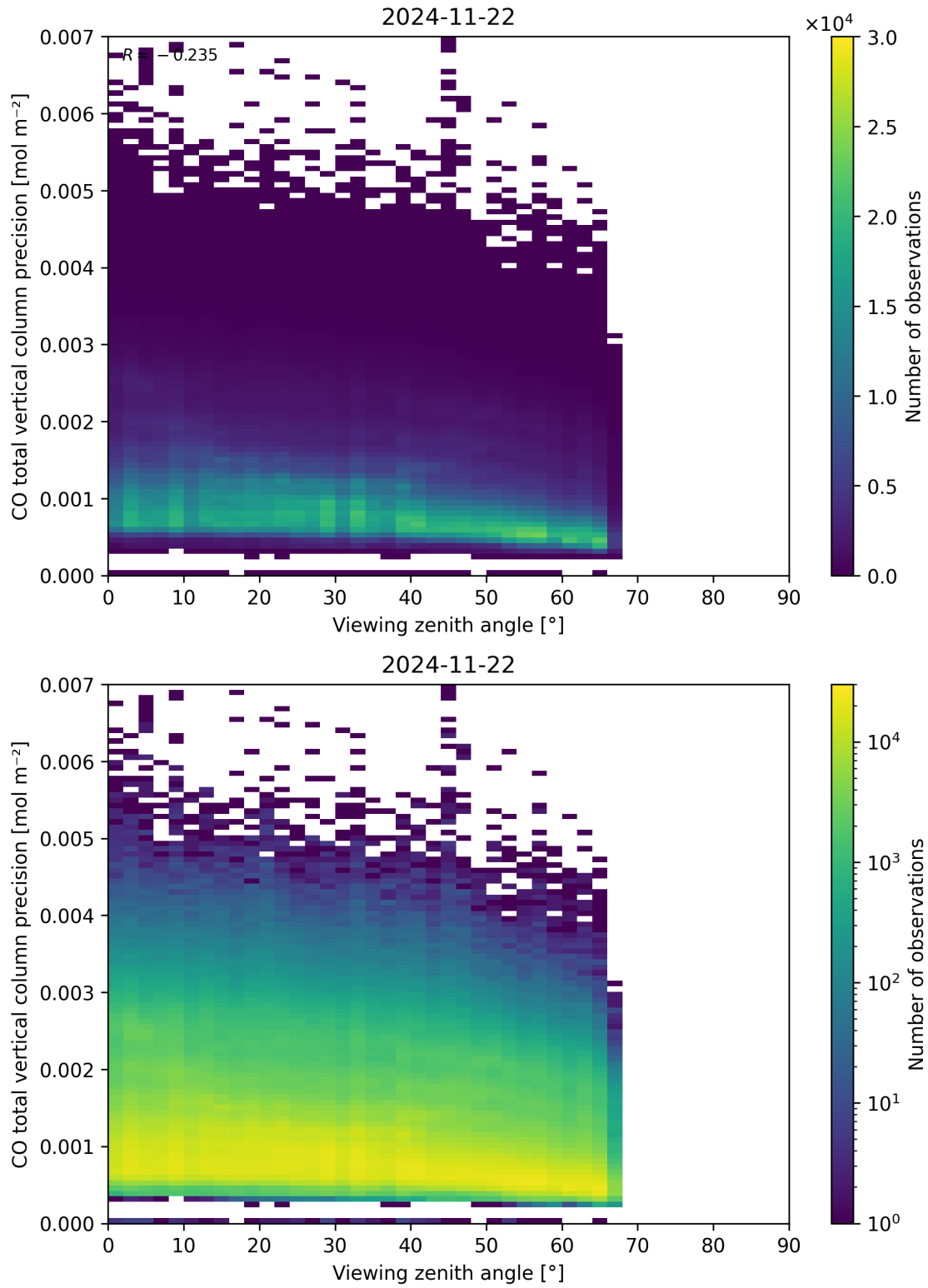
Figure 71: Scatter density plot of “Viewing zenith angle” against “CO total vertical column precision” for 2024-11-21 to 2024-11-23.
