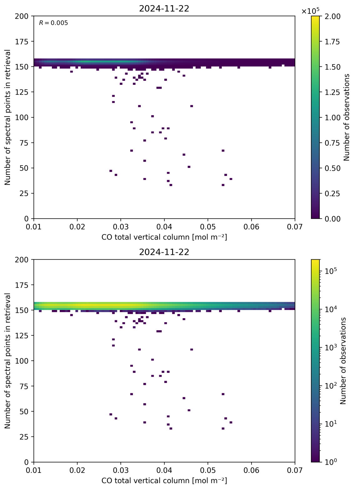
Figure 43: Scatter density plot of “CO total vertical column” against “Number of spectral points in retrieval” for 2024-11-21 to 2024-11-23.
