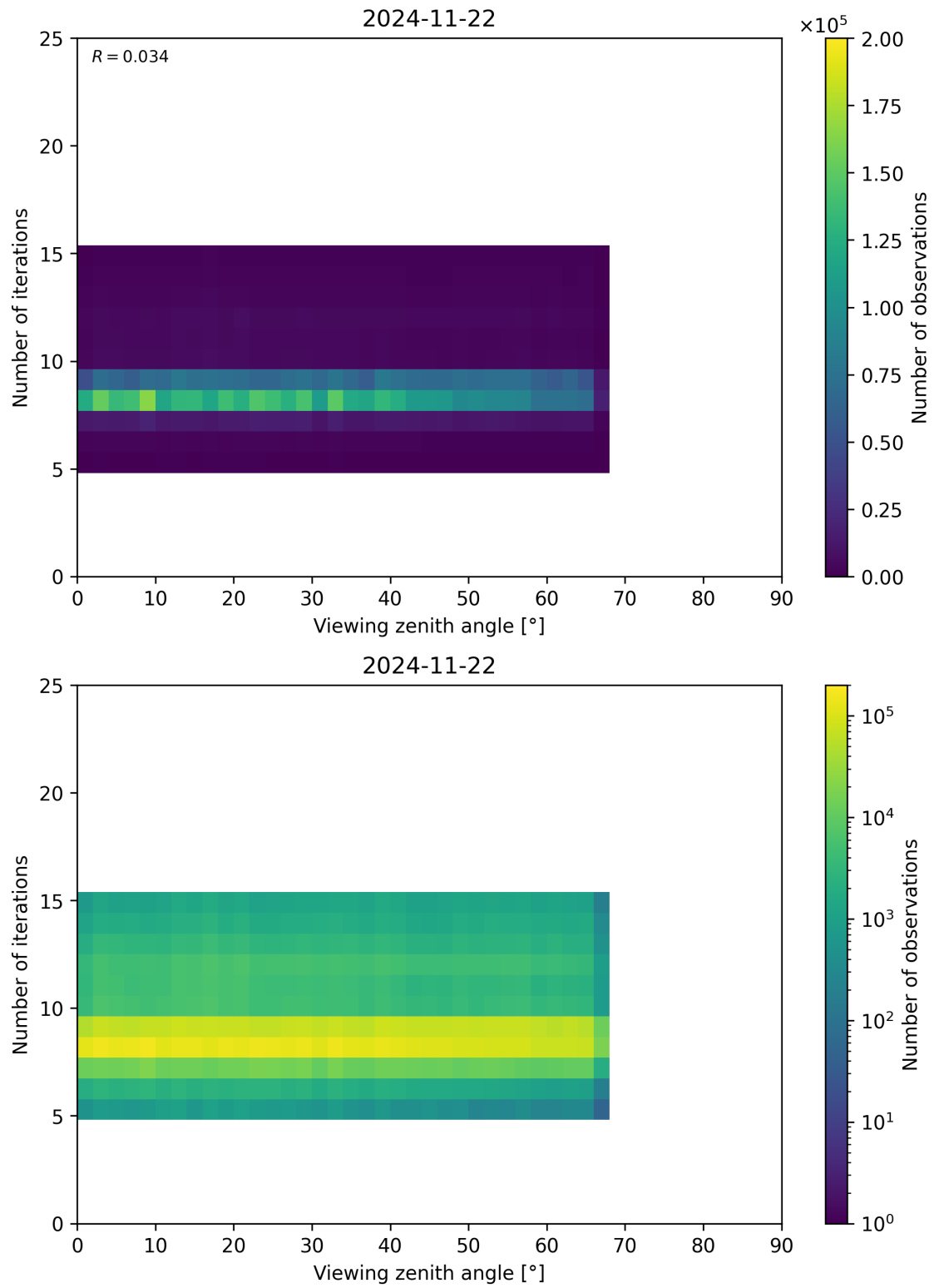
Figure 75: Scatter density plot of “Viewing zenith angle” against “Number of iterations” for 2024-11-21 to 2024-11-23.
