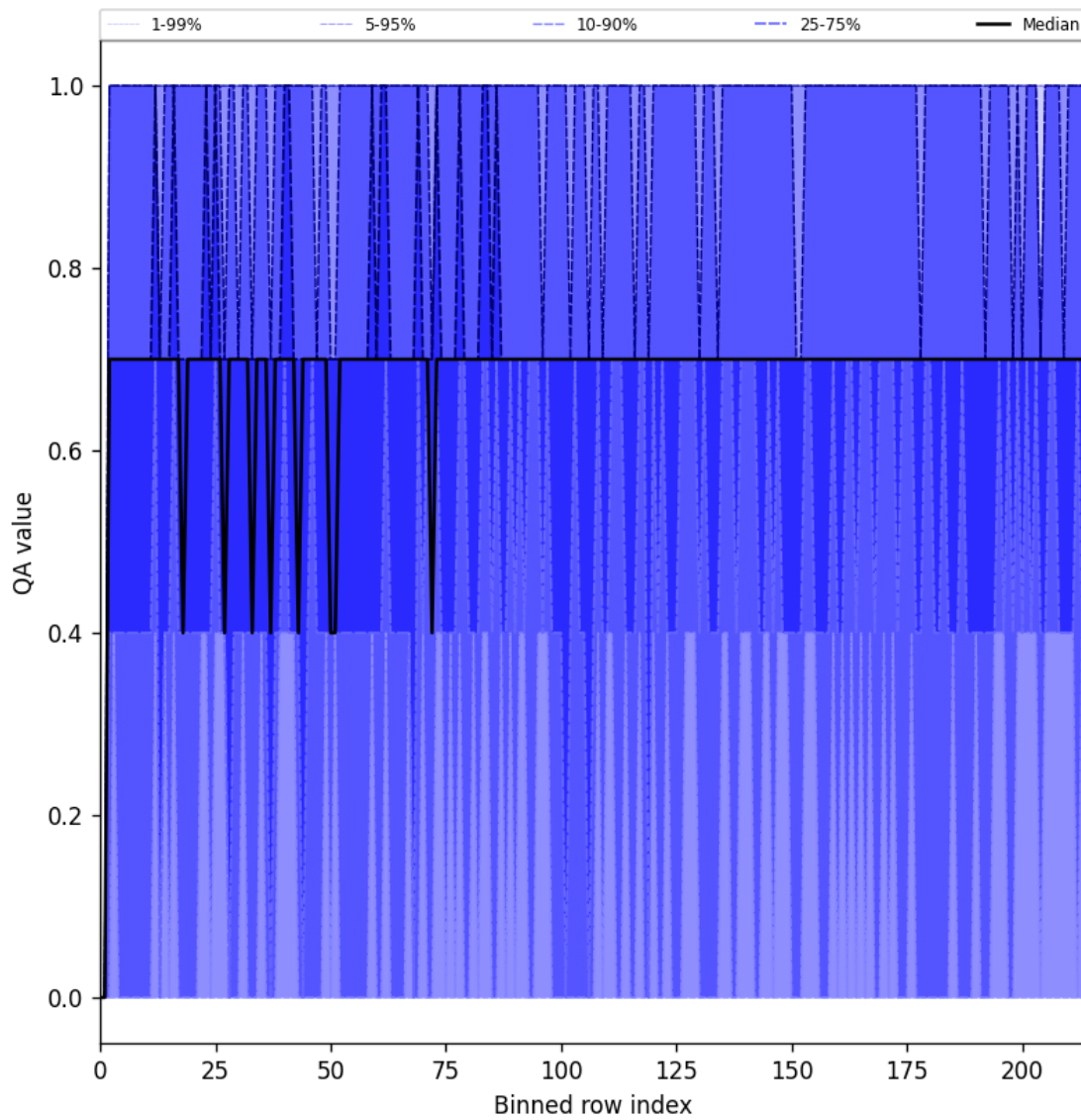
Figure 25: Along track statistics of “QA value” for 2024-11-21 to 2024-11-23
