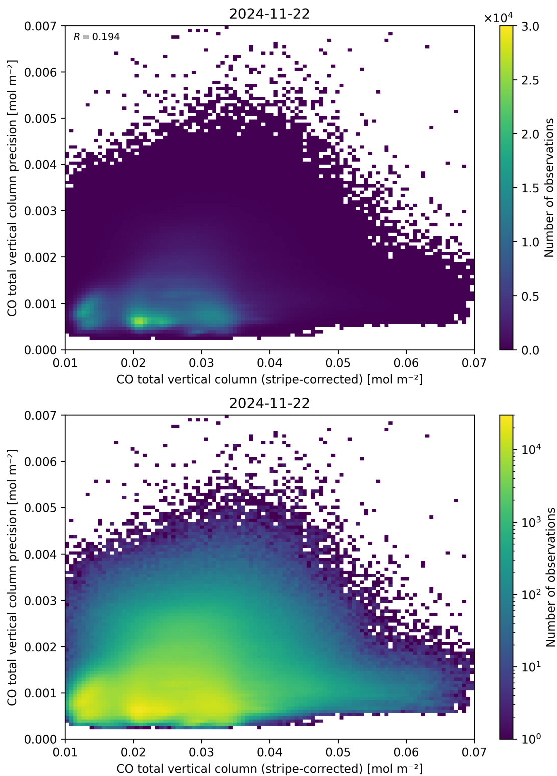
Figure 36: Scatter density plot of “CO total vertical column (stripe-corrected)” against “CO total vertical column precision” for 2024-11-21 to 2024-11-23.
