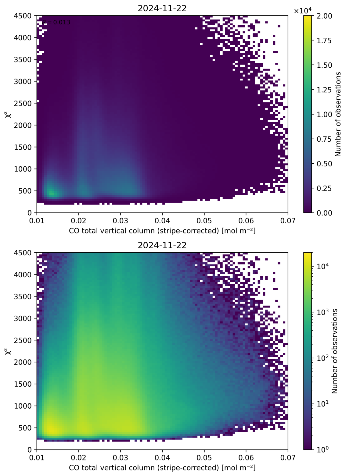
Figure 37: Scatter density plot of “CO total vertical column (stripe-corrected)” against “ \chi^2 ” for 2024-11-21 to 2024-11-23.
