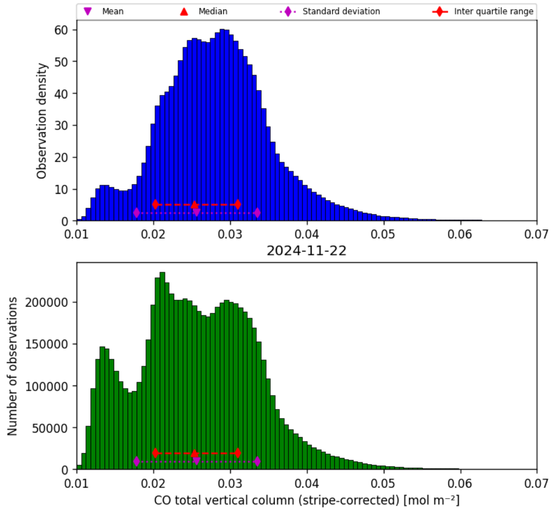
Figure 19: Histogram of “CO total vertical column (stripe-corrected)” for 2024-11-21 to 2024-11-23
