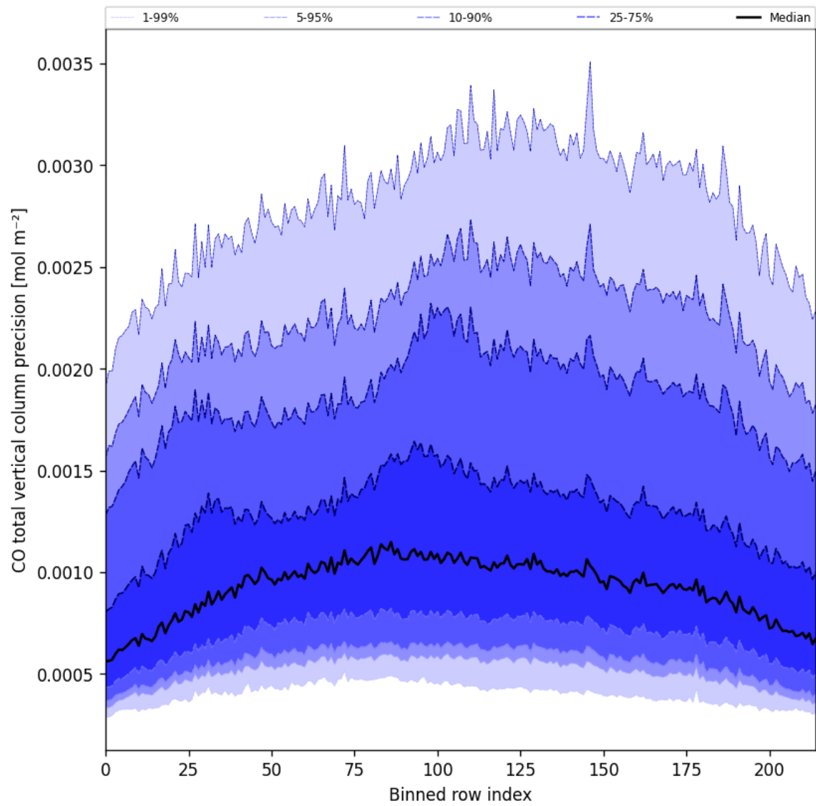
Figure 28: Along track statistics of “CO total vertical column precision” for 2024-11-21 to 2024-11-23
