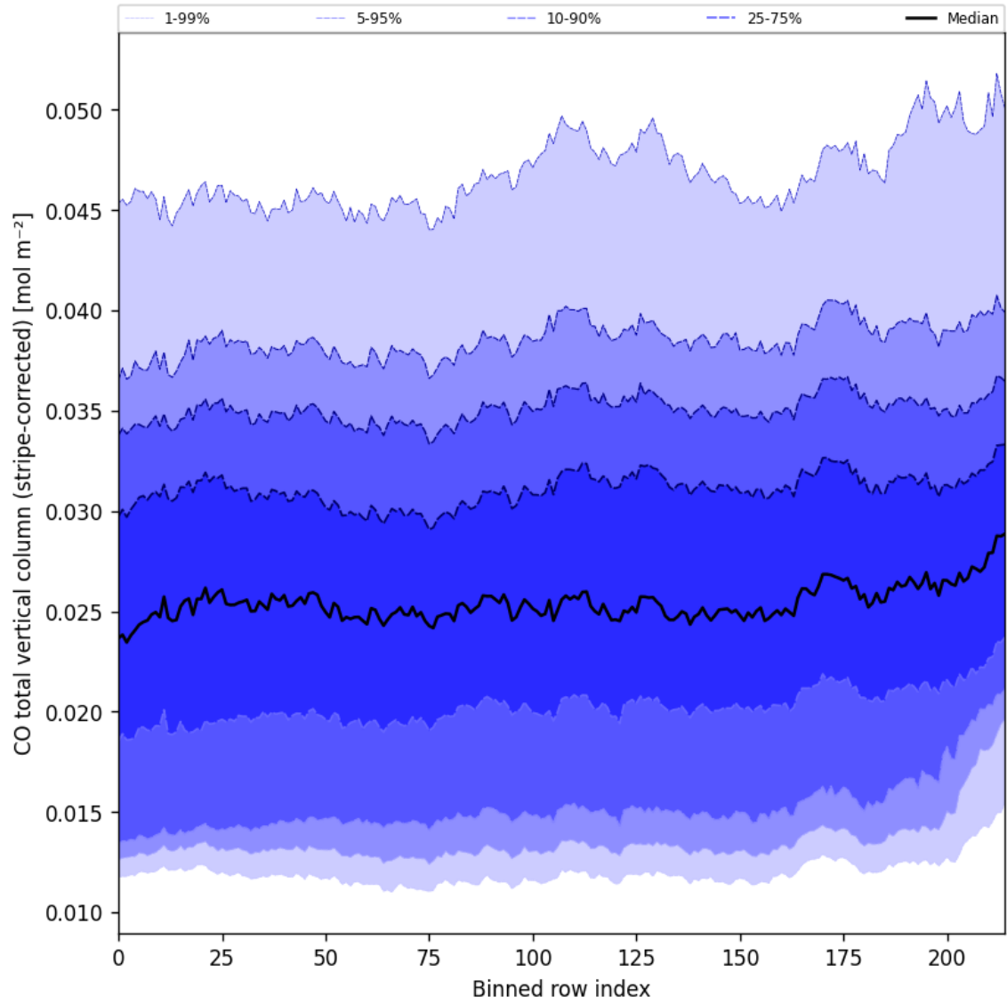
Figure 27: Along track statistics of “CO total vertical column (stripe-corrected)” for 2024-11-21 to 2024-11-23
