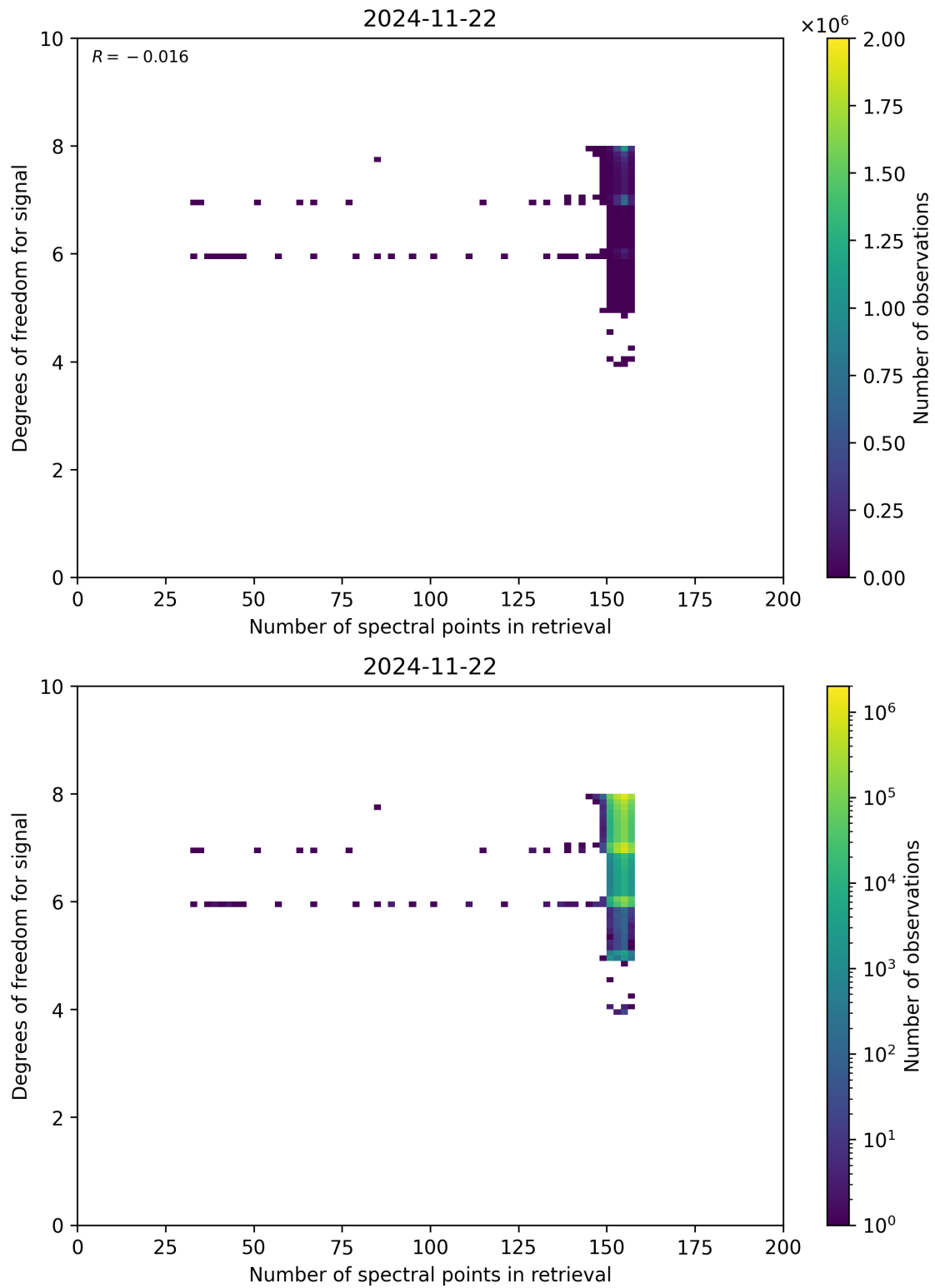
Figure 59: Scatter density plot of “Number of spectral points in retrieval” against “Degrees of freedom for signal” for 2024-11-21 to 2024-11-23.
