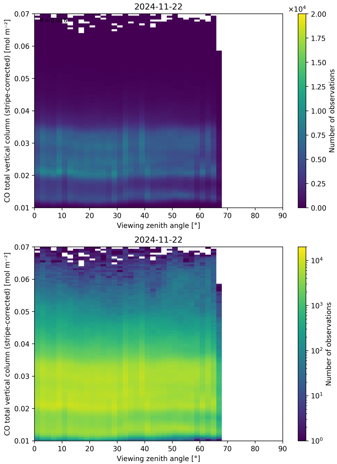
Figure 70: Scatter density plot of “Viewing zenith angle” against “CO total vertical column (stripe-corrected)” for 2024-11-21 to 2024-11-23.
