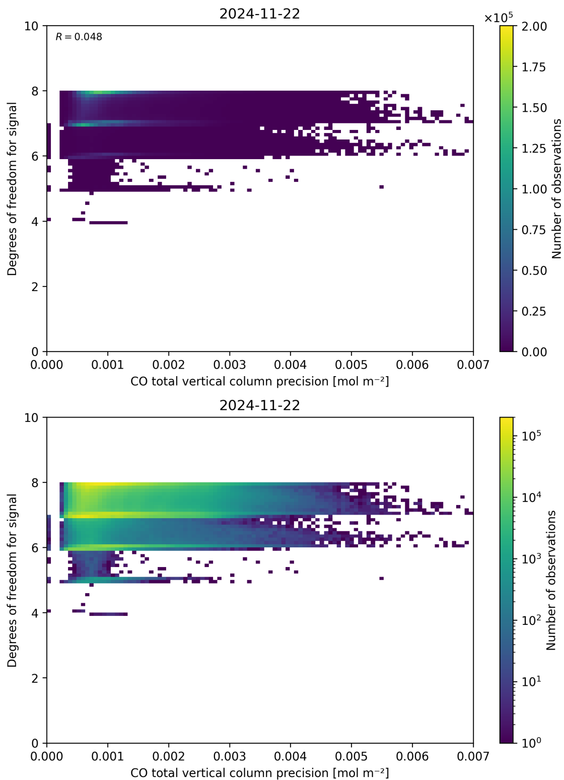
Figure 45: Scatter density plot of “CO total vertical column precision” against “Degrees of freedom for signal” for 2024-11-21 to 2024-11-23.
