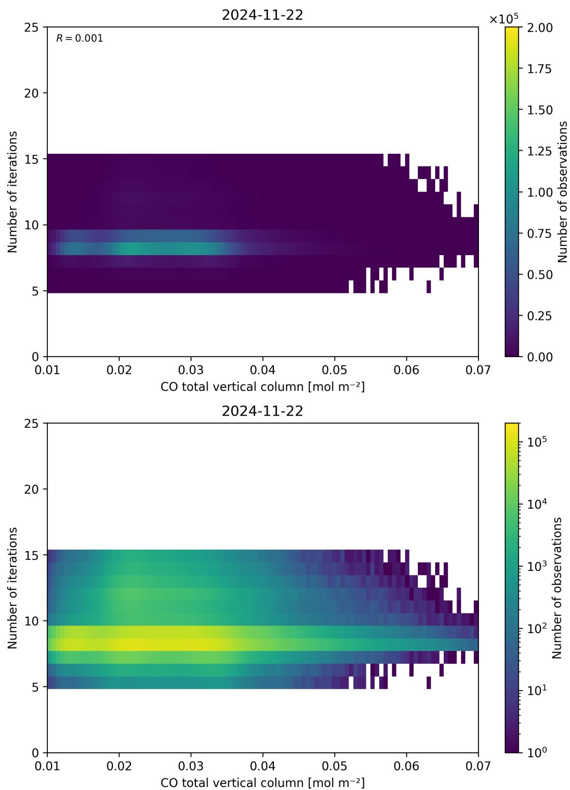
Figure 42: Scatter density plot of “CO total vertical column” against “Number of iterations” for 2024-11-21 to 2024-11-23.
