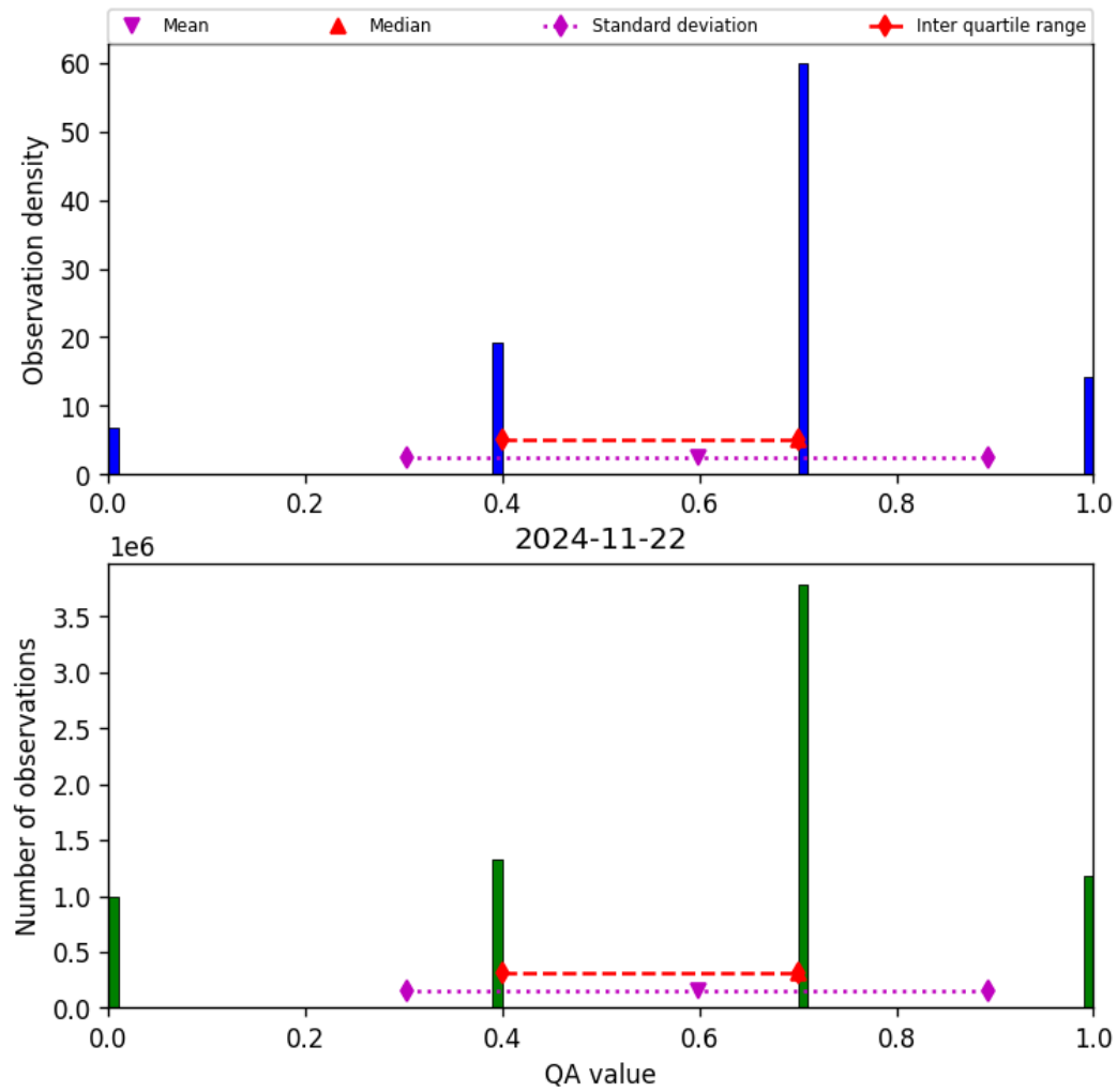
Figure 17: Histogram of “QA value” for 2024-11-21 to 2024-11-23
