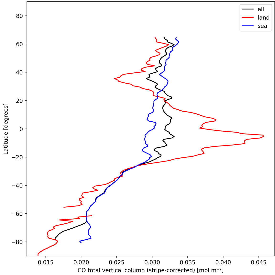
Figure 11: Zonal average of “CO total vertical column (stripe-corrected)” for 2024-11-21 to 2024-11-23.
