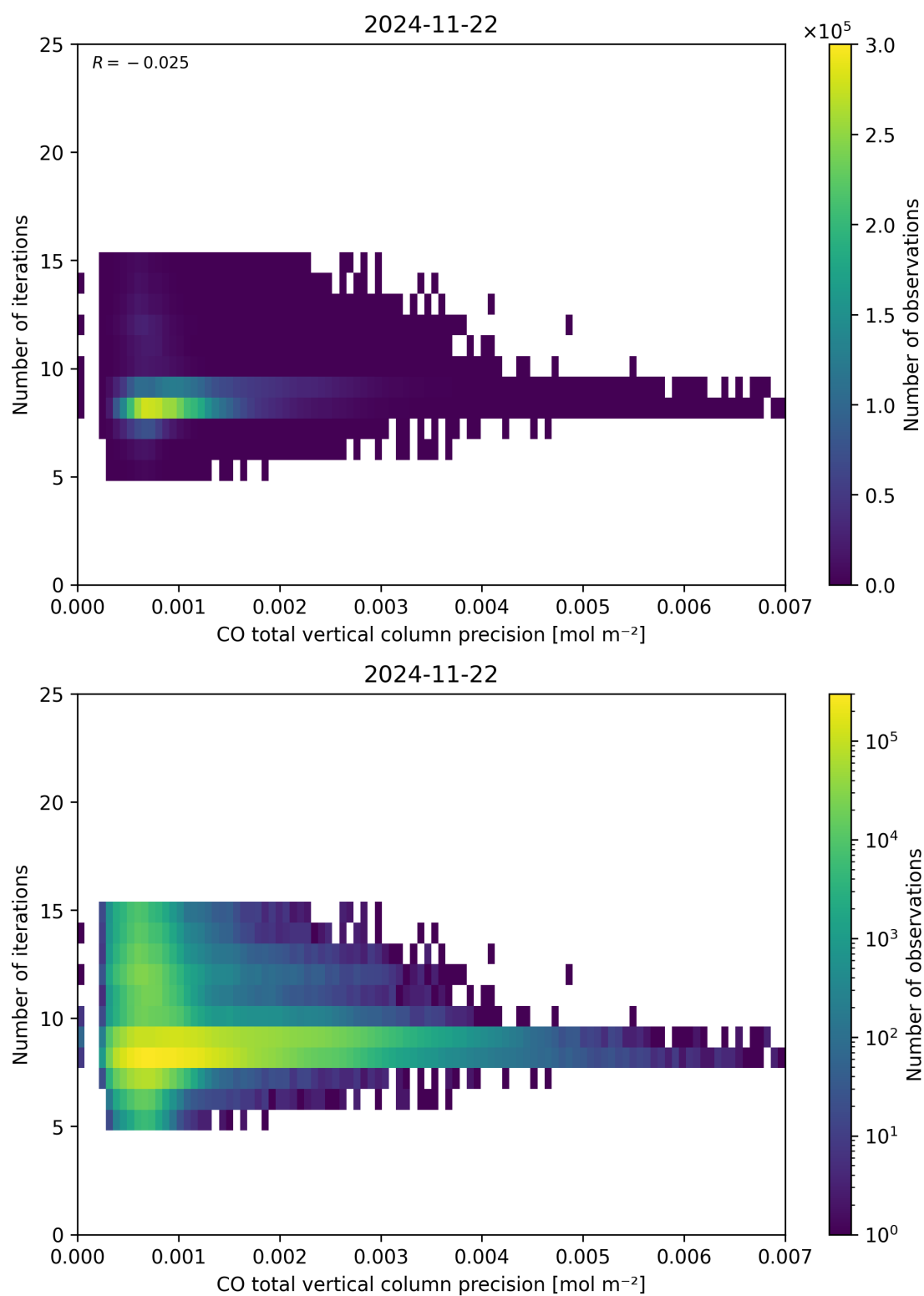
Figure 46: Scatter density plot of “CO total vertical column precision” against “Number of iterations” for 2024-11-21 to 2024-11-23.
