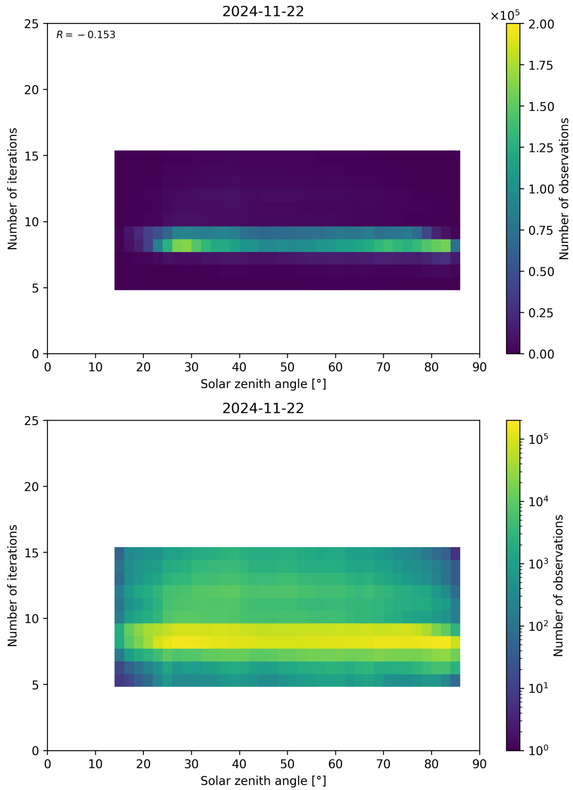
Figure 67: Scatter density plot of “Solar zenith angle” against “Number of iterations” for 2024-11-21 to 2024-11-23.
