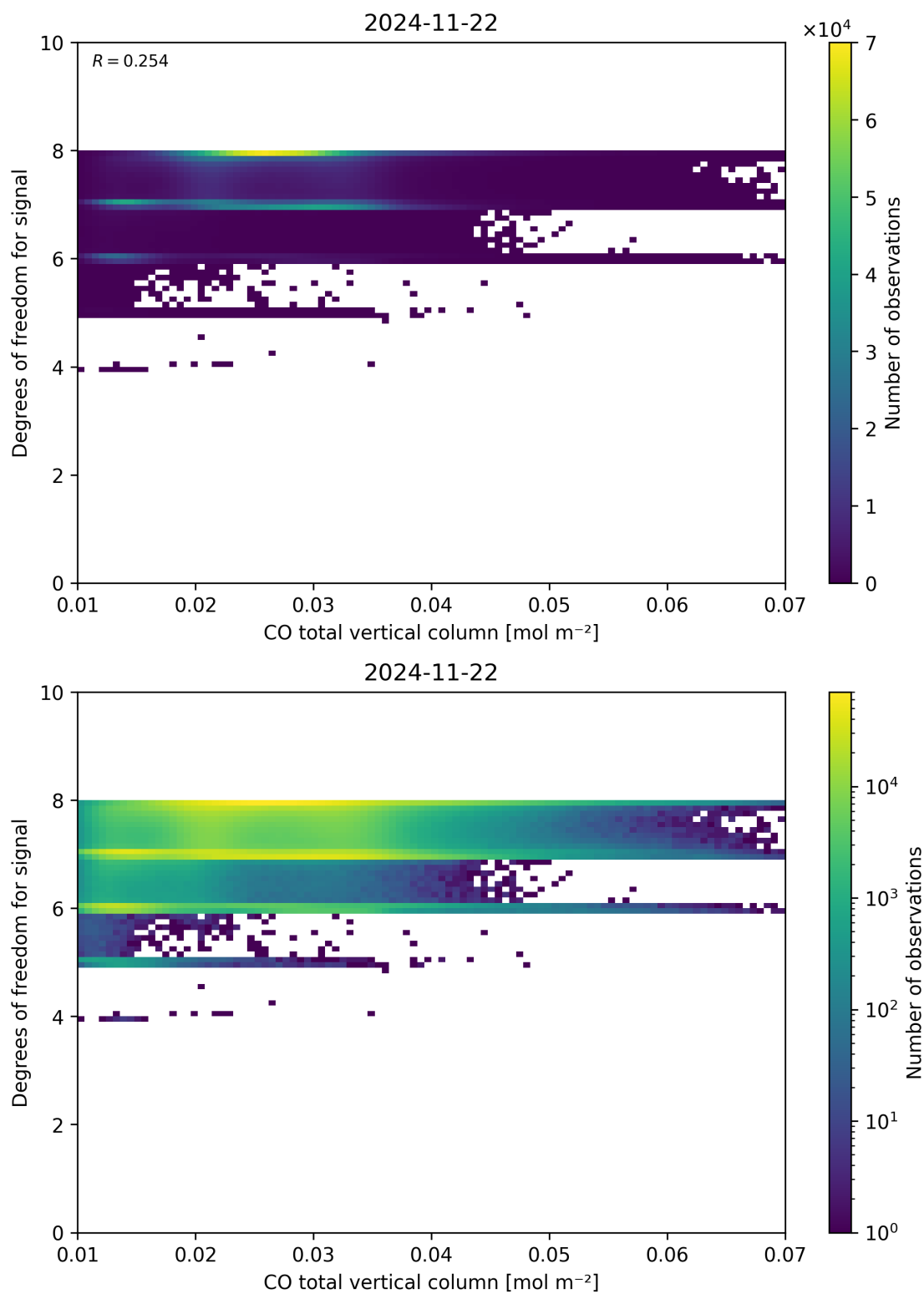
Figure 41: Scatter density plot of “CO total vertical column” against “Degrees of freedom for signal” for 2024-11-21 to 2024-11-23.
