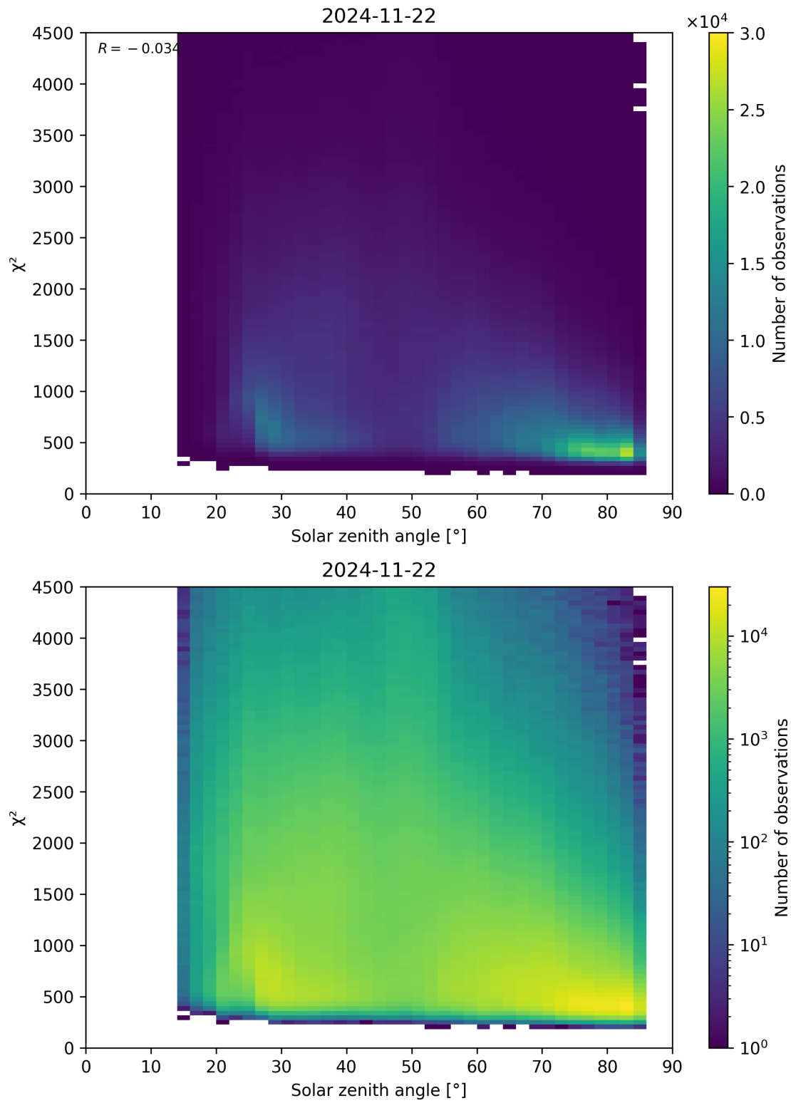
Figure 64: Scatter density plot of “Solar zenith angle” against “ \chi^2 ” for 2024-11-21 to 2024-11-23.
