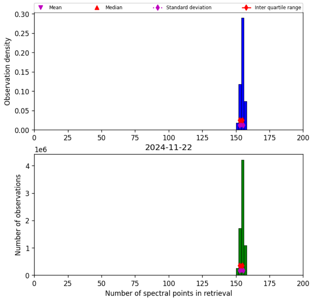
Figure 21: Histogram of “Number of spectral points in retrieval” for 2024-11-21 to 2024-11-23
