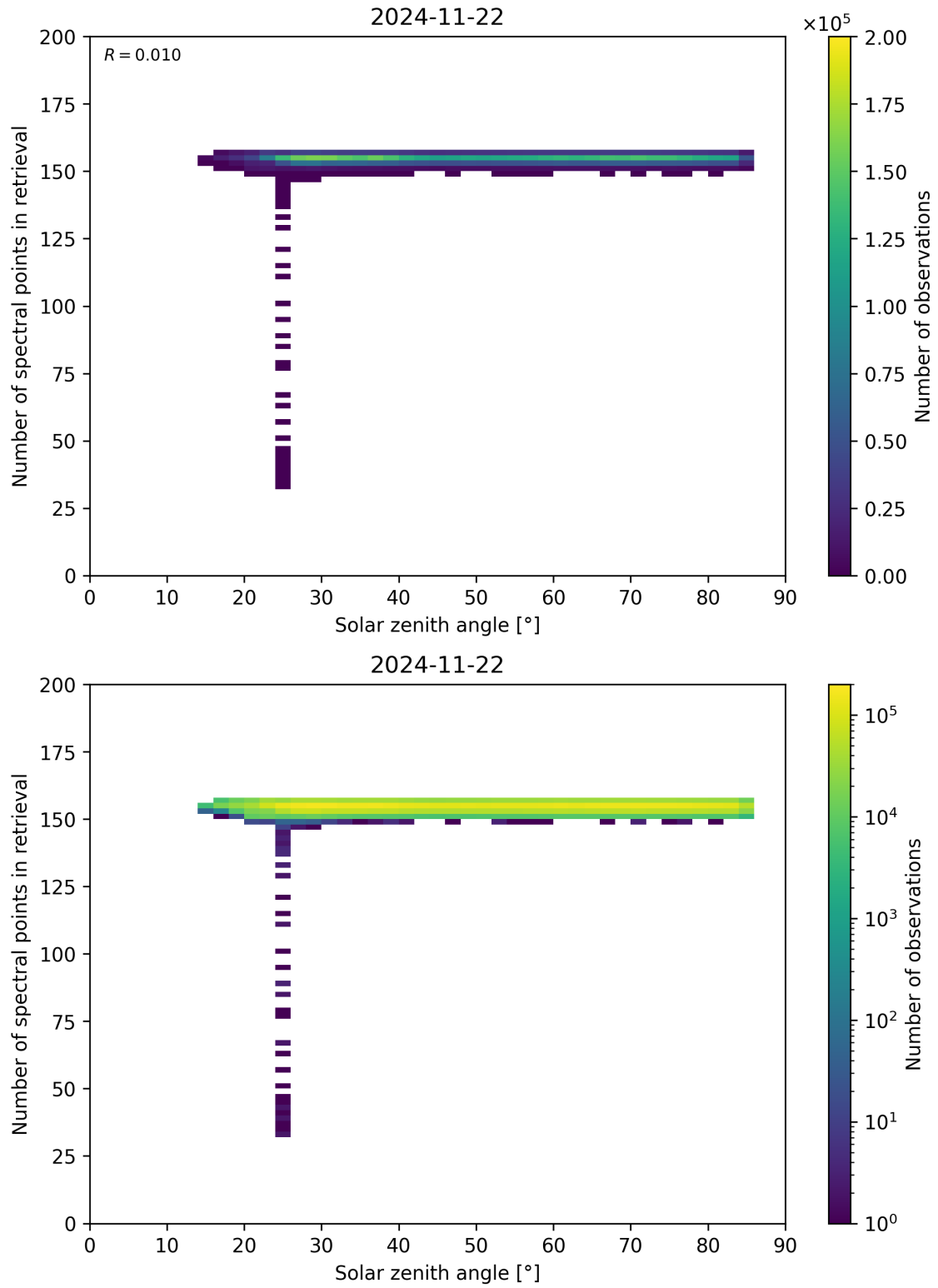
Figure 68: Scatter density plot of “Solar zenith angle” against “Number of spectral points in retrieval” for 2024-11-21 to 2024-11-23.
