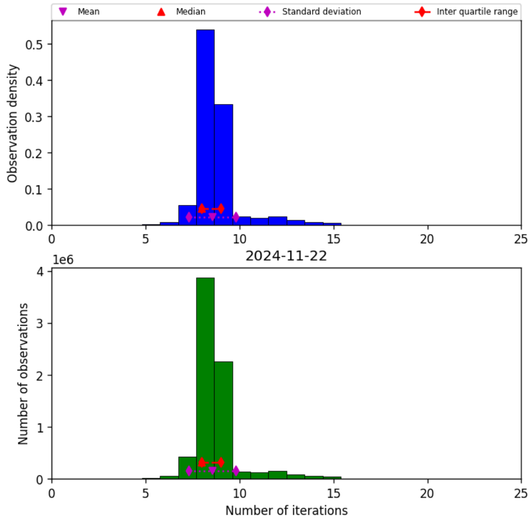
Figure 24: Histogram of “Number of iterations” for 2024-11-21 to 2024-11-23
