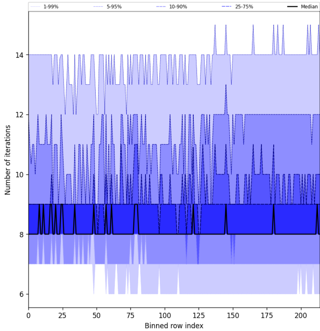
Figure 32: Along track statistics of “Number of iterations” for 2024-11-21 to 2024-11-23
