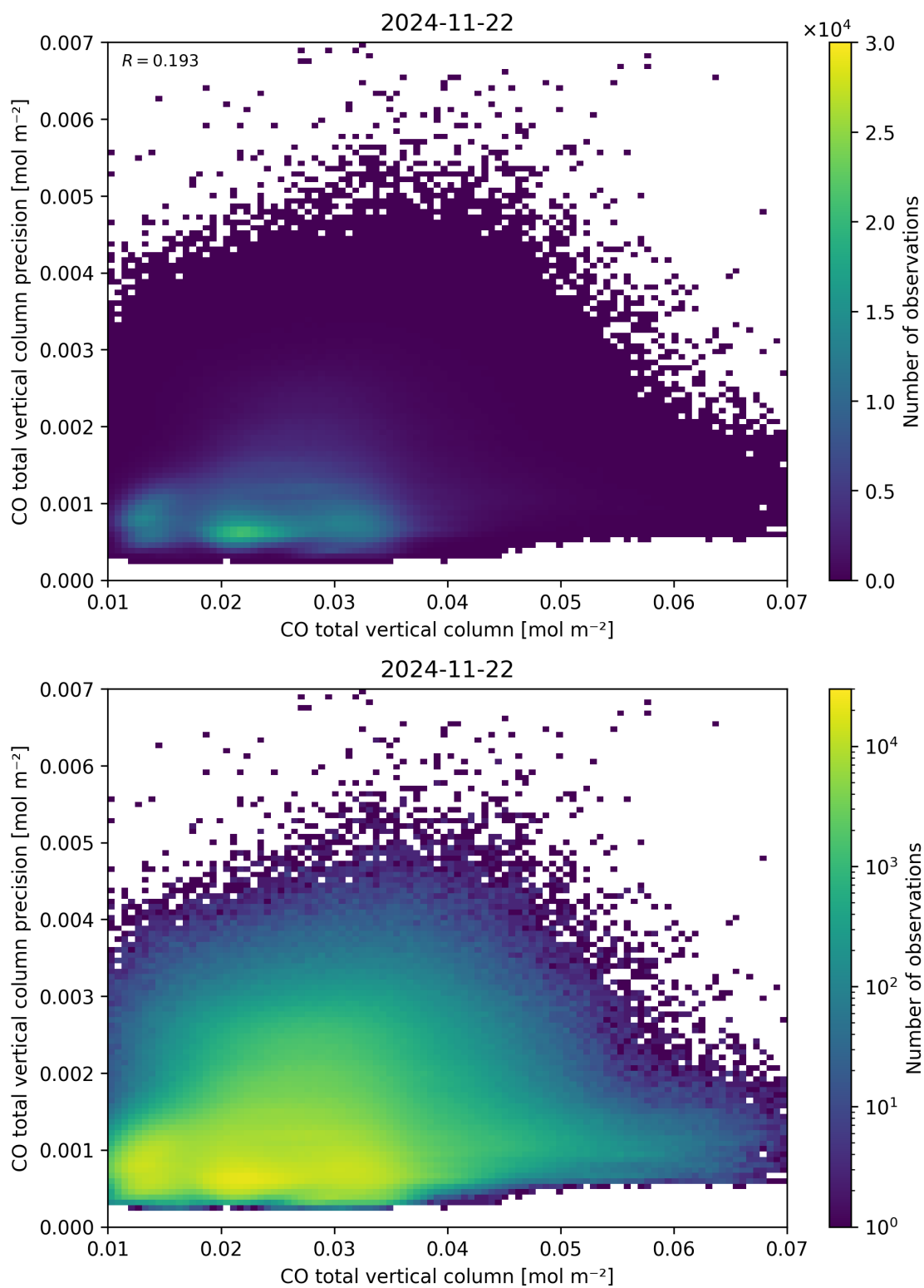
Figure 34: Scatter density plot of “CO total vertical column” against “CO total vertical column precision” for 2024-11-21 to 2024-11-23.
