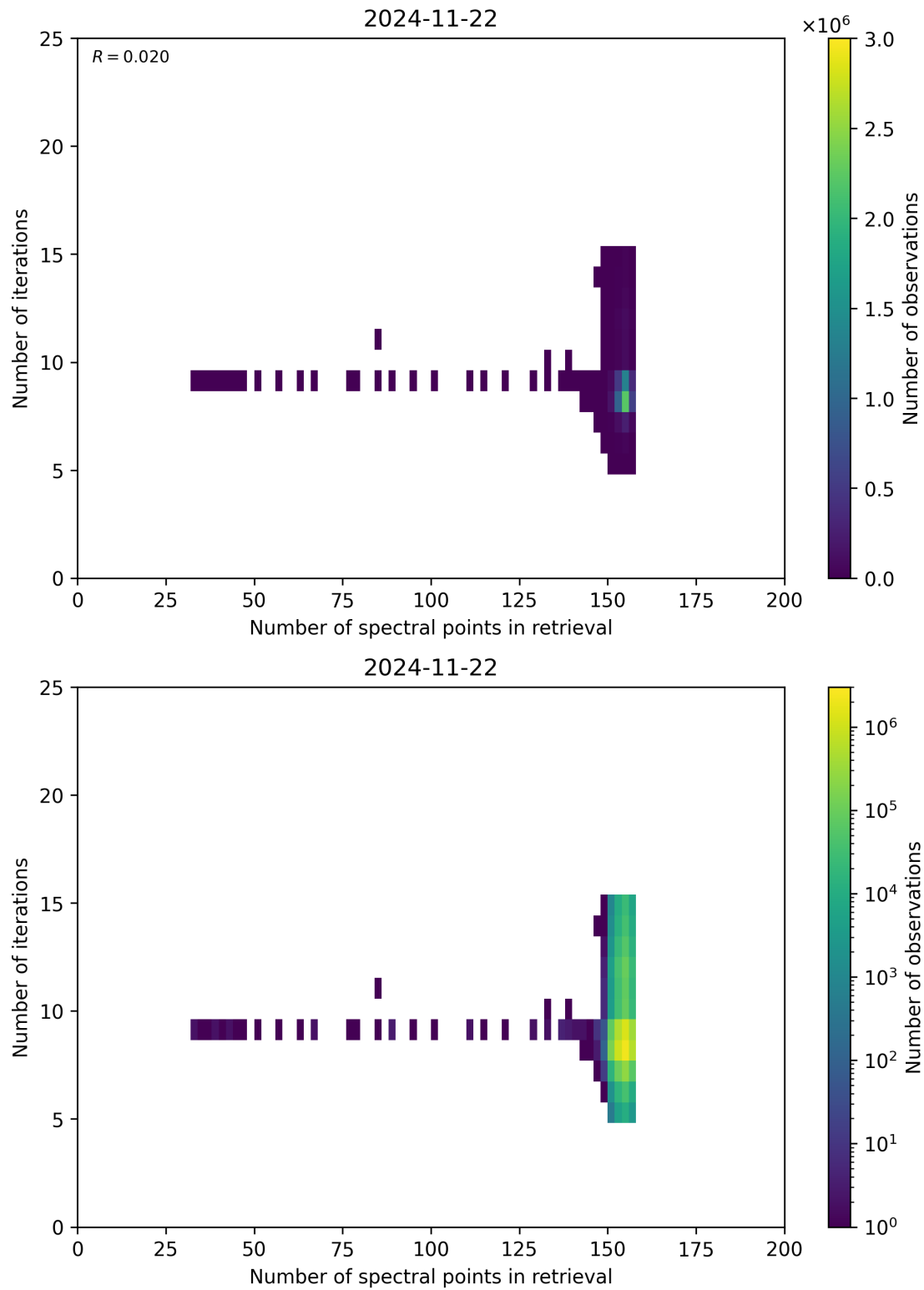
Figure 60: Scatter density plot of “Number of spectral points in retrieval” against “Number of iterations” for 2024-11-21 to 2024-11-23.
