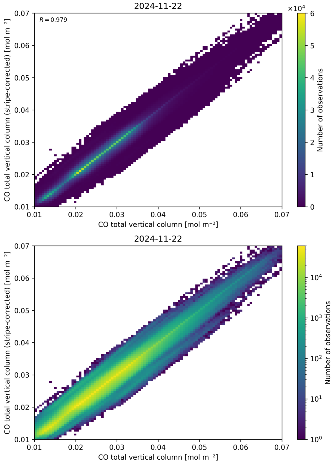
Figure 33: Scatter density plot of “CO total vertical column” against “CO total vertical column (stripe-corrected)” for 2024-11-21 to 2024-11-23.
