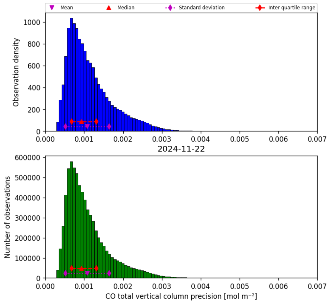
Figure 20: Histogram of “CO total vertical column precision” for 2024-11-21 to 2024-11-23
