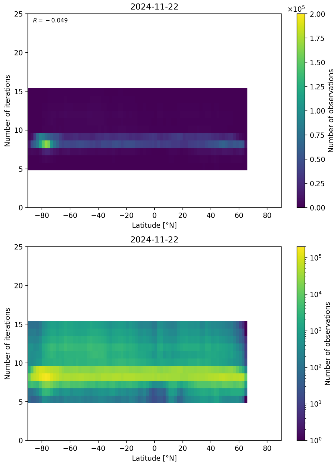
Figure 56: Scatter density plot of “Latitude” against “Number of iterations” for 2024-11-21 to 2024-11-23.
