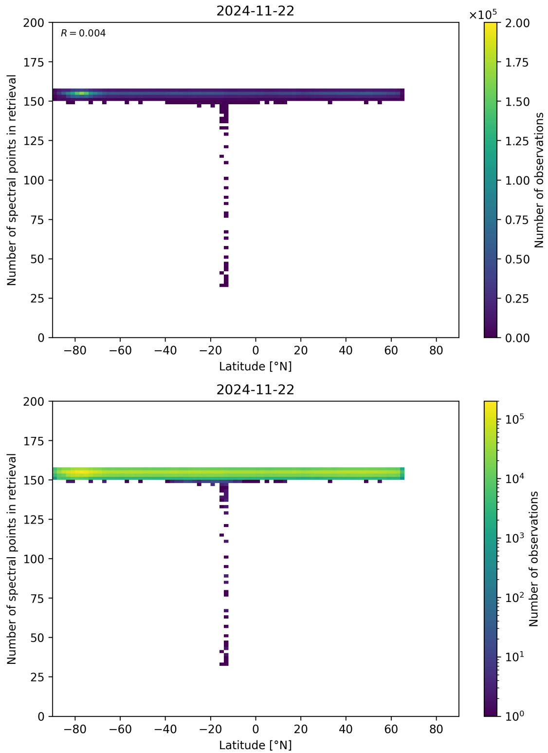
Figure 57: Scatter density plot of “Latitude” against “Number of spectral points in retrieval” for 2024-11-21 to 2024-11-23.
