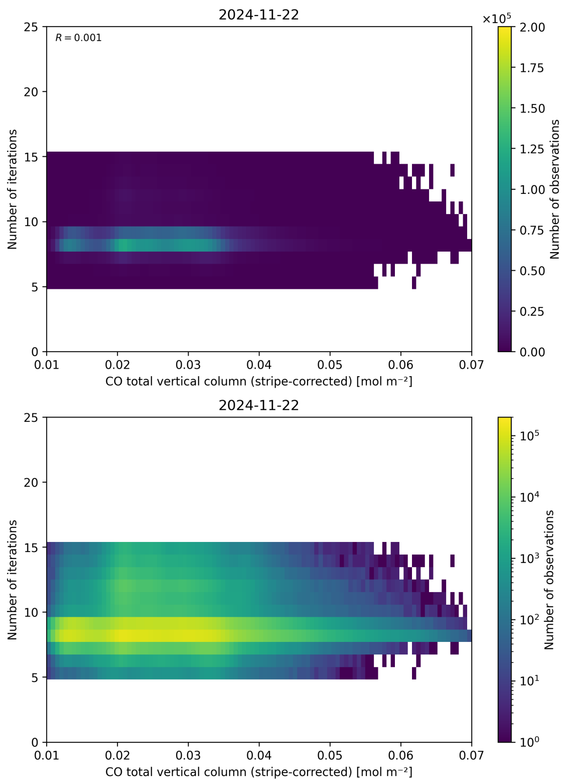
Figure 39: Scatter density plot of “CO total vertical column (stripe-corrected)” against “Number of iterations” for 2024-11-21 to 2024-11-23.
