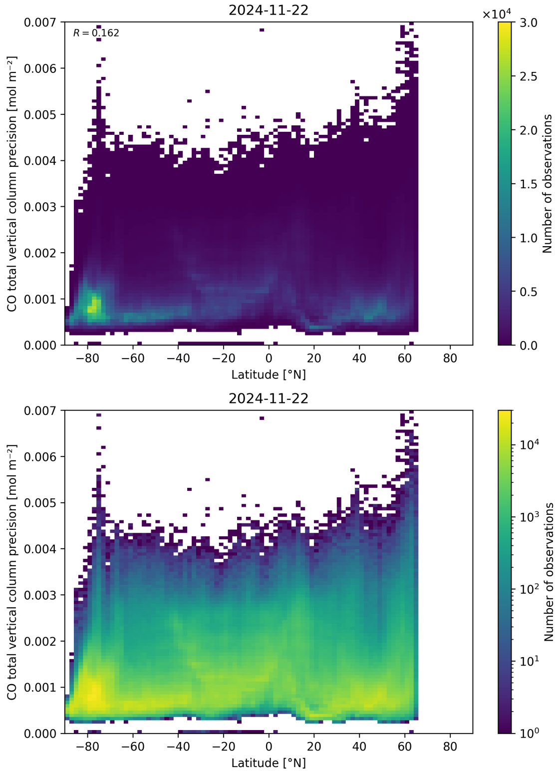
Figure 53: Scatter density plot of “Latitude” against “CO total vertical column precision” for 2024-11-21 to 2024-11-23.
