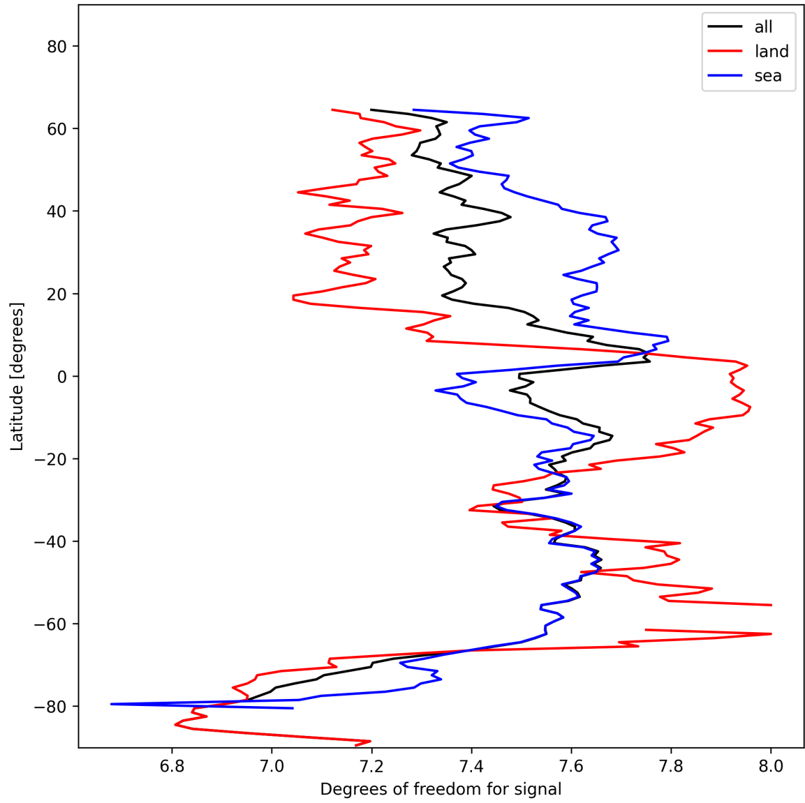
Figure 15: Zonal average of “Degrees of freedom for signal” for 2024-11-21 to 2024-11-23.
