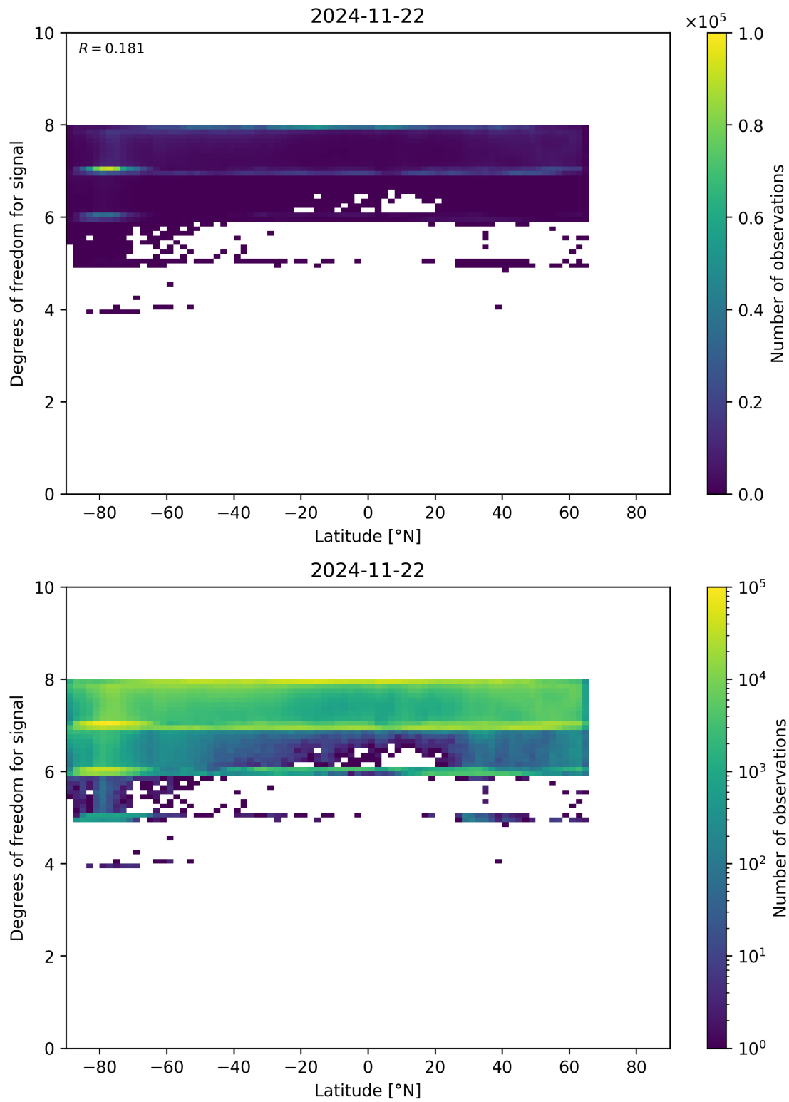
Figure 55: Scatter density plot of “Latitude” against “Degrees of freedom for signal” for 2024-11-21 to 2024-11-23.
