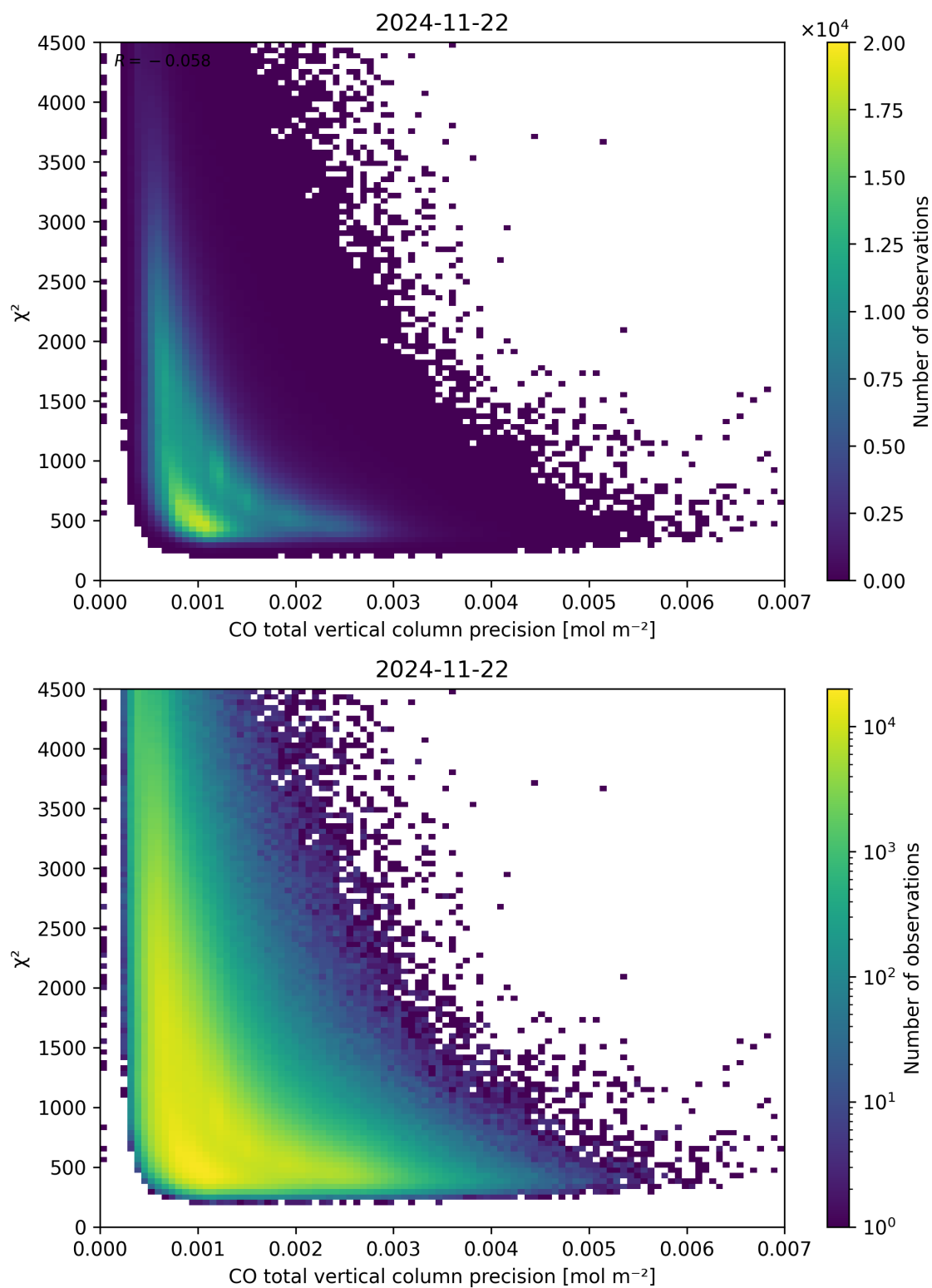
Figure 44: Scatter density plot of “CO total vertical column precision” against “ \chi^2 ” for 2024-11-21 to 2024-11-23.
