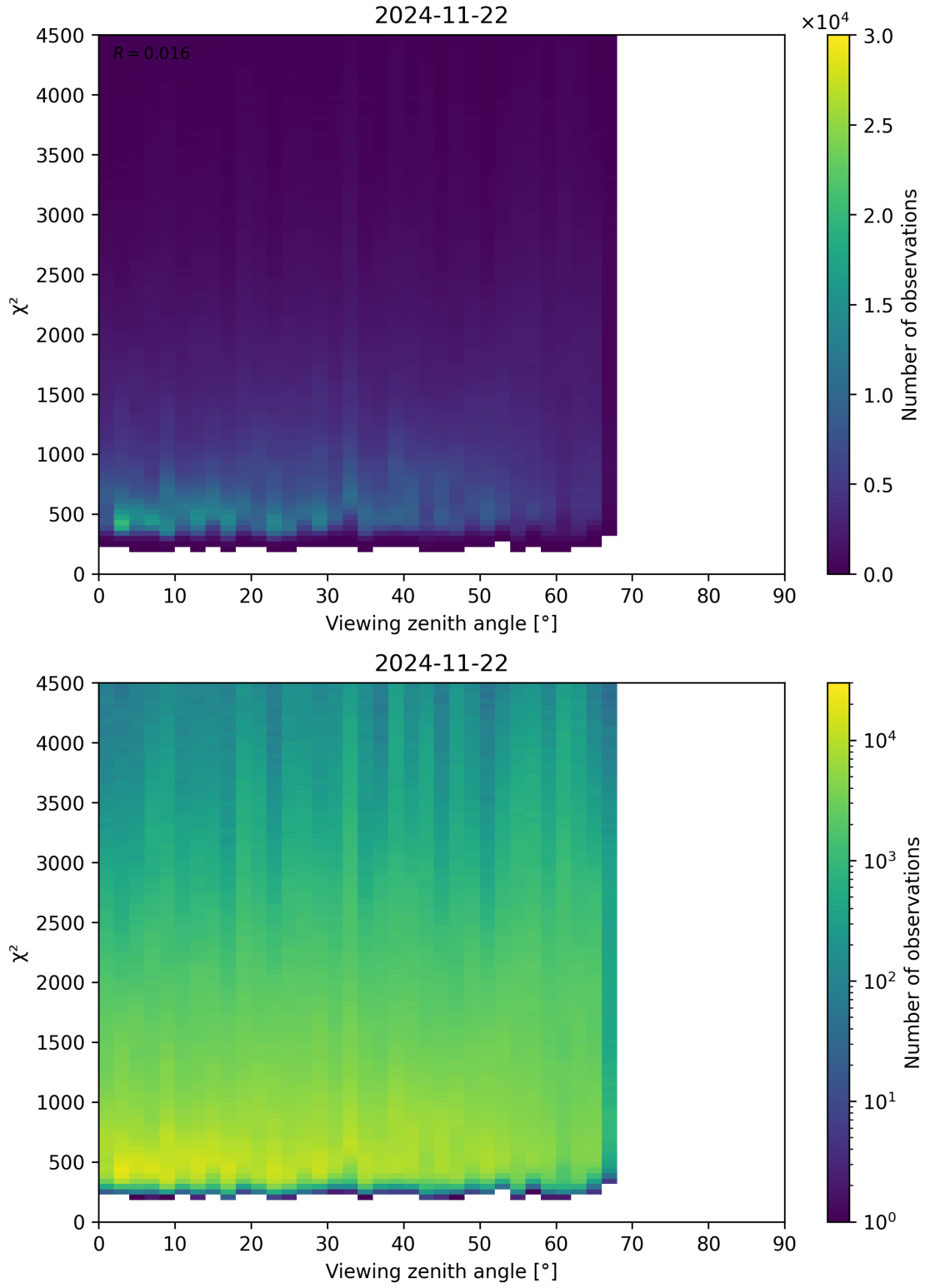
Figure 72: Scatter density plot of “Viewing zenith angle” against “ \chi^2 ” for 2024-11-21 to 2024-11-23.
