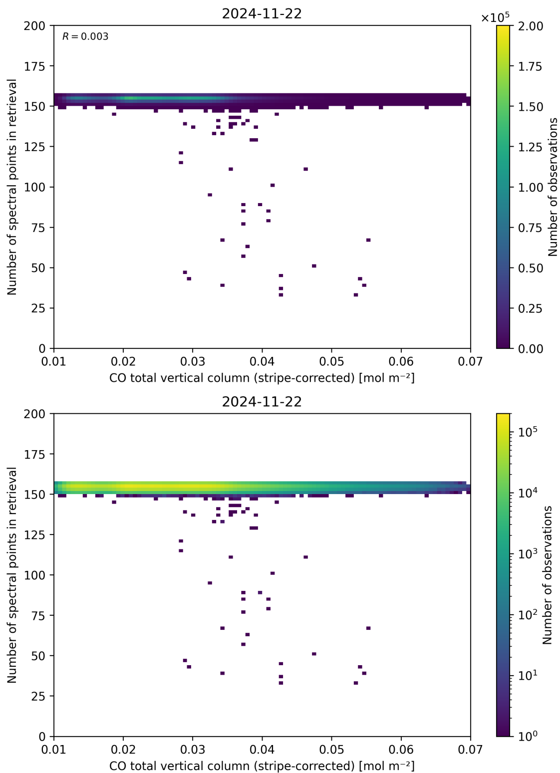
Figure 40: Scatter density plot of “CO total vertical column (stripe-corrected)” against “Number of spectral points in retrieval” for 2024-11-21 to 2024-11-23.
