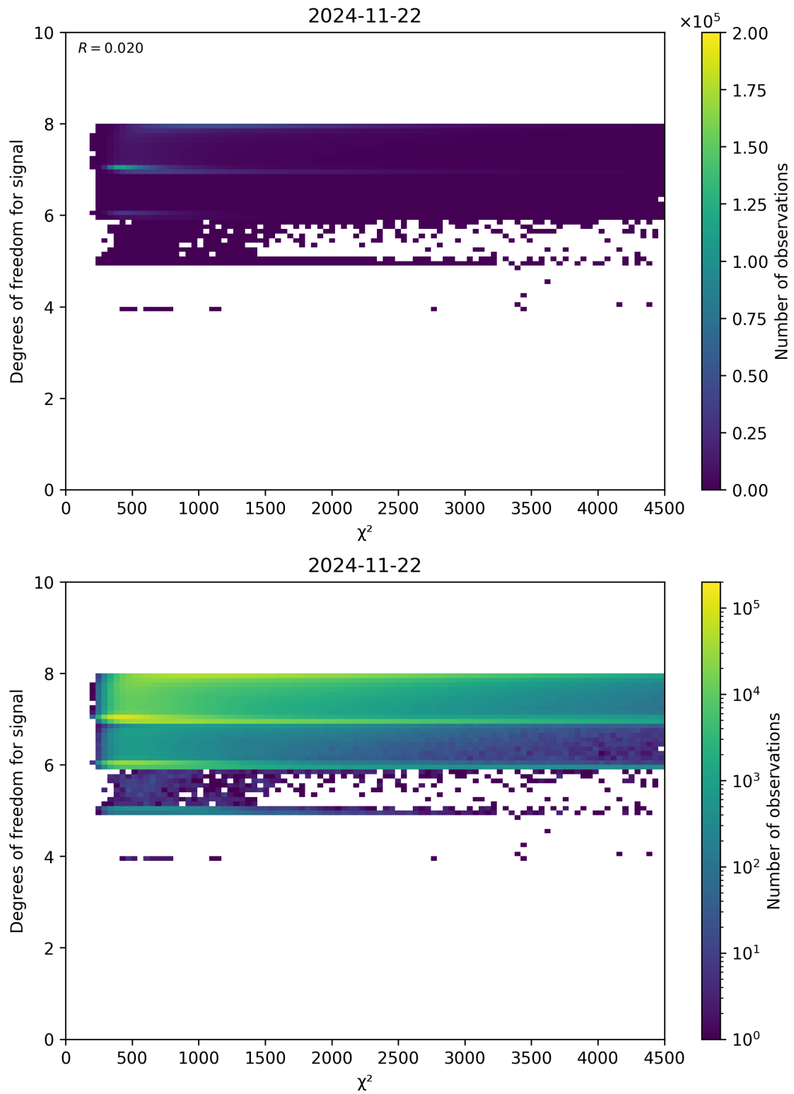
Figure 48: Scatter density plot of “ \chi^2 ” against “Degrees of freedom for signal” for 2024-11-21 to 2024-11-23.
