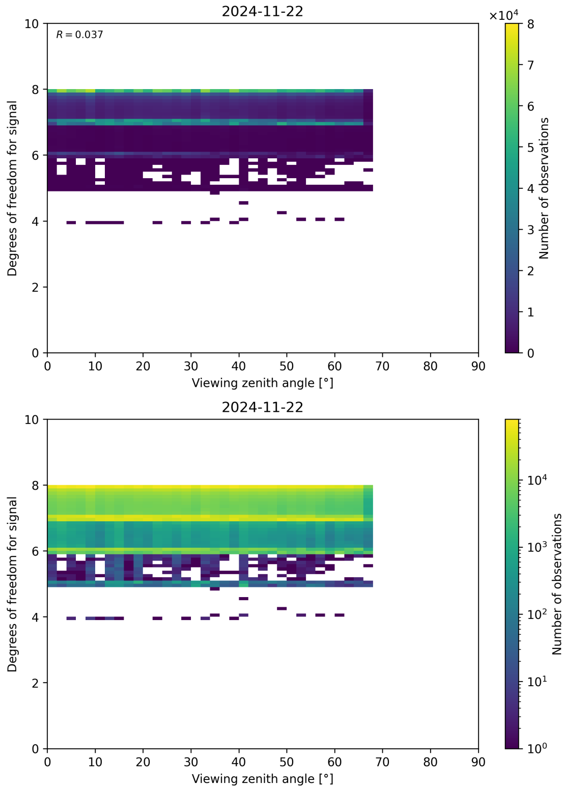
Figure 73: Scatter density plot of “Viewing zenith angle” against “Degrees of freedom for signal” for 2024-11-21 to 2024-11-23.
