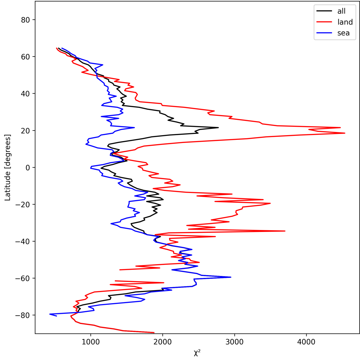
Figure 14: Zonal average of “ \chi^2 ” for 2024-11-21 to 2024-11-23.
