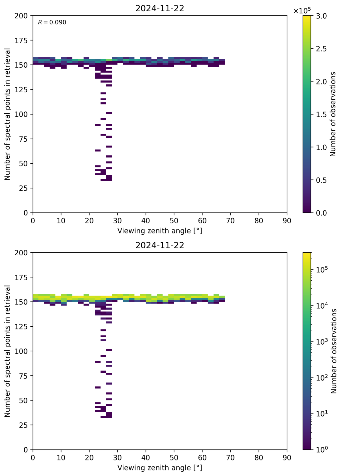
Figure 76: Scatter density plot of “Viewing zenith angle” against “Number of spectral points in retrieval” for 2024-11-21 to 2024-11-23.
