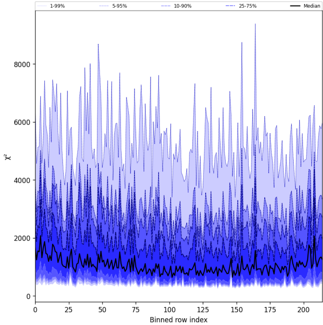
Figure 30: Along track statistics of “ \chi^2 ” for 2024-11-21 to 2024-11-23
