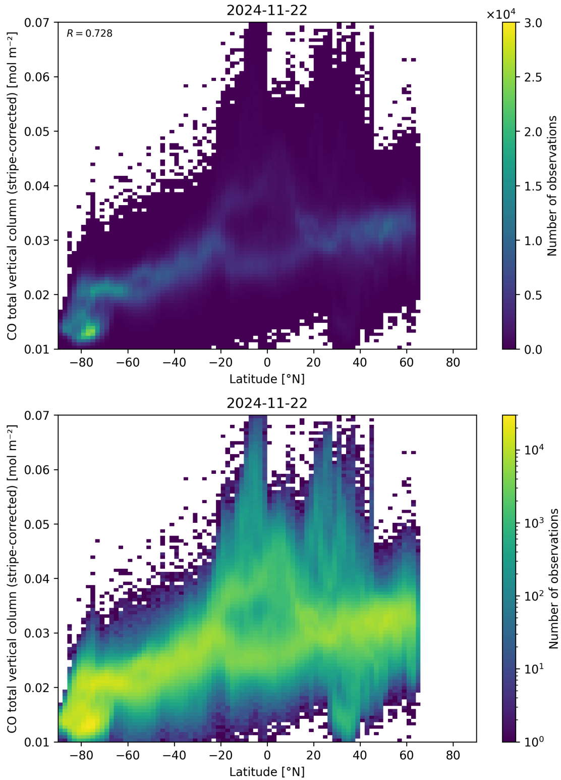
Figure 52: Scatter density plot of “Latitude” against “CO total vertical column (stripe-corrected)” for 2024-11-21 to 2024-11-23.
