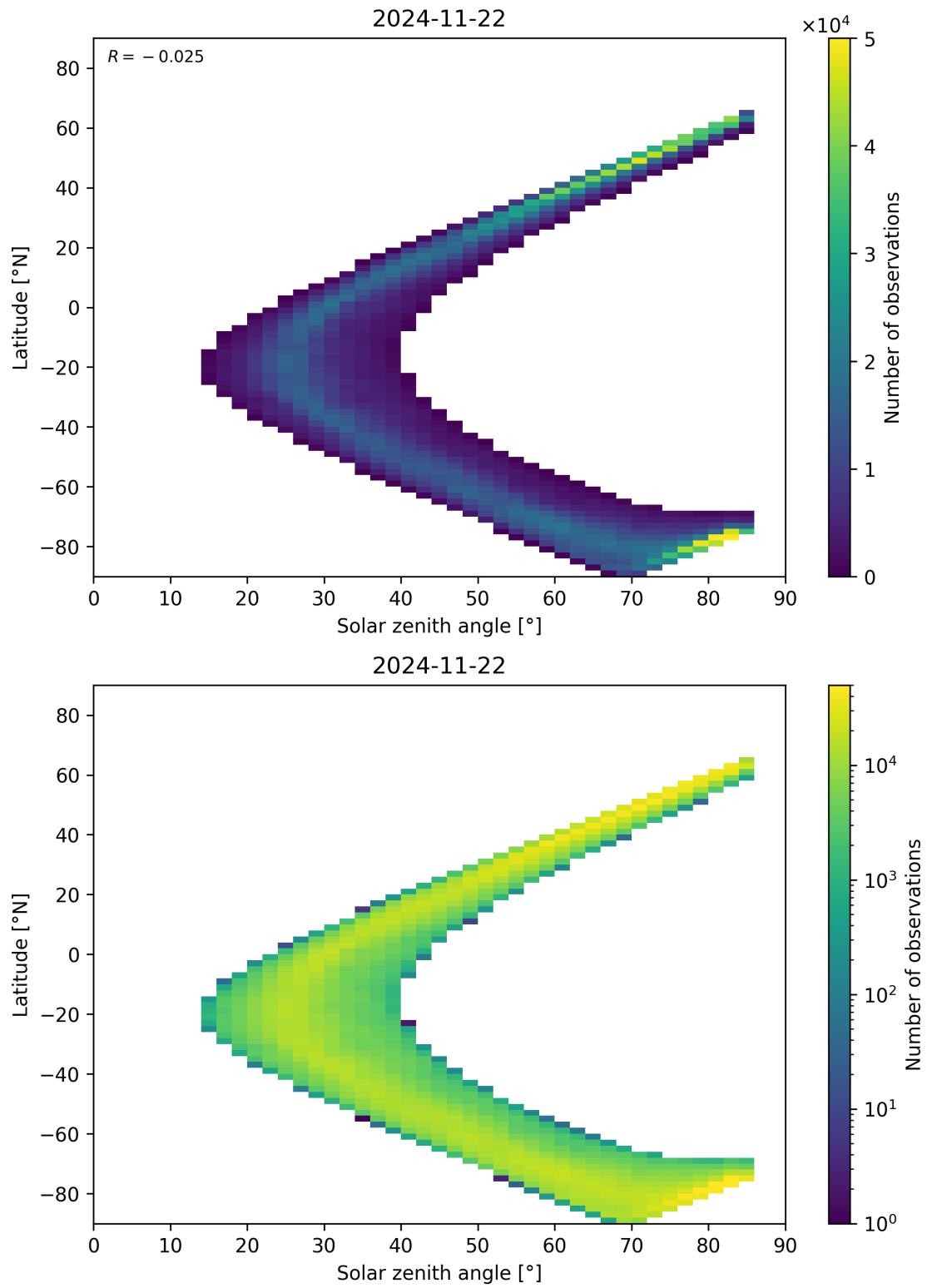
Figure 66: Scatter density plot of “Solar zenith angle” against “Latitude” for 2024-11-21 to 2024-11-23.
