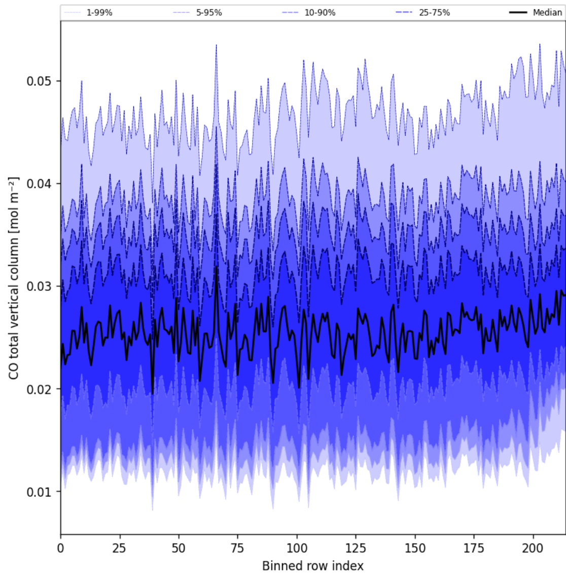
Figure 26: Along track statistics of “CO total vertical column” for 2024-11-21 to 2024-11-23
