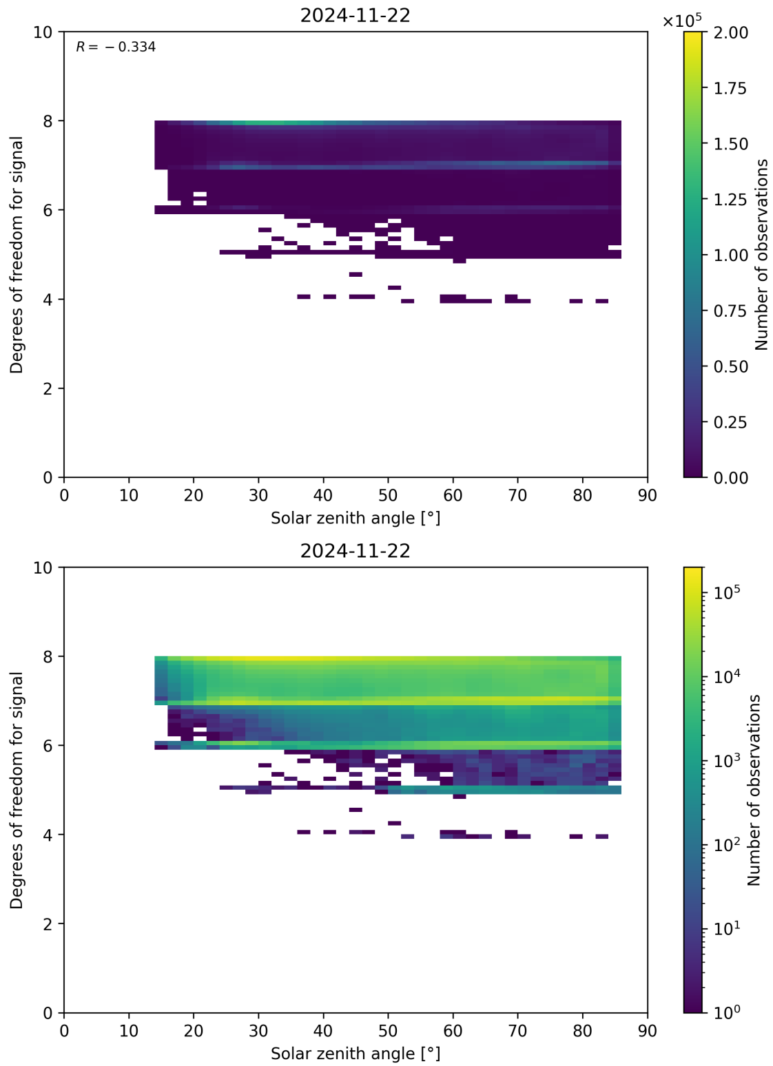
Figure 65: Scatter density plot of “Solar zenith angle” against “Degrees of freedom for signal” for 2024-11-21 to 2024-11-23.
