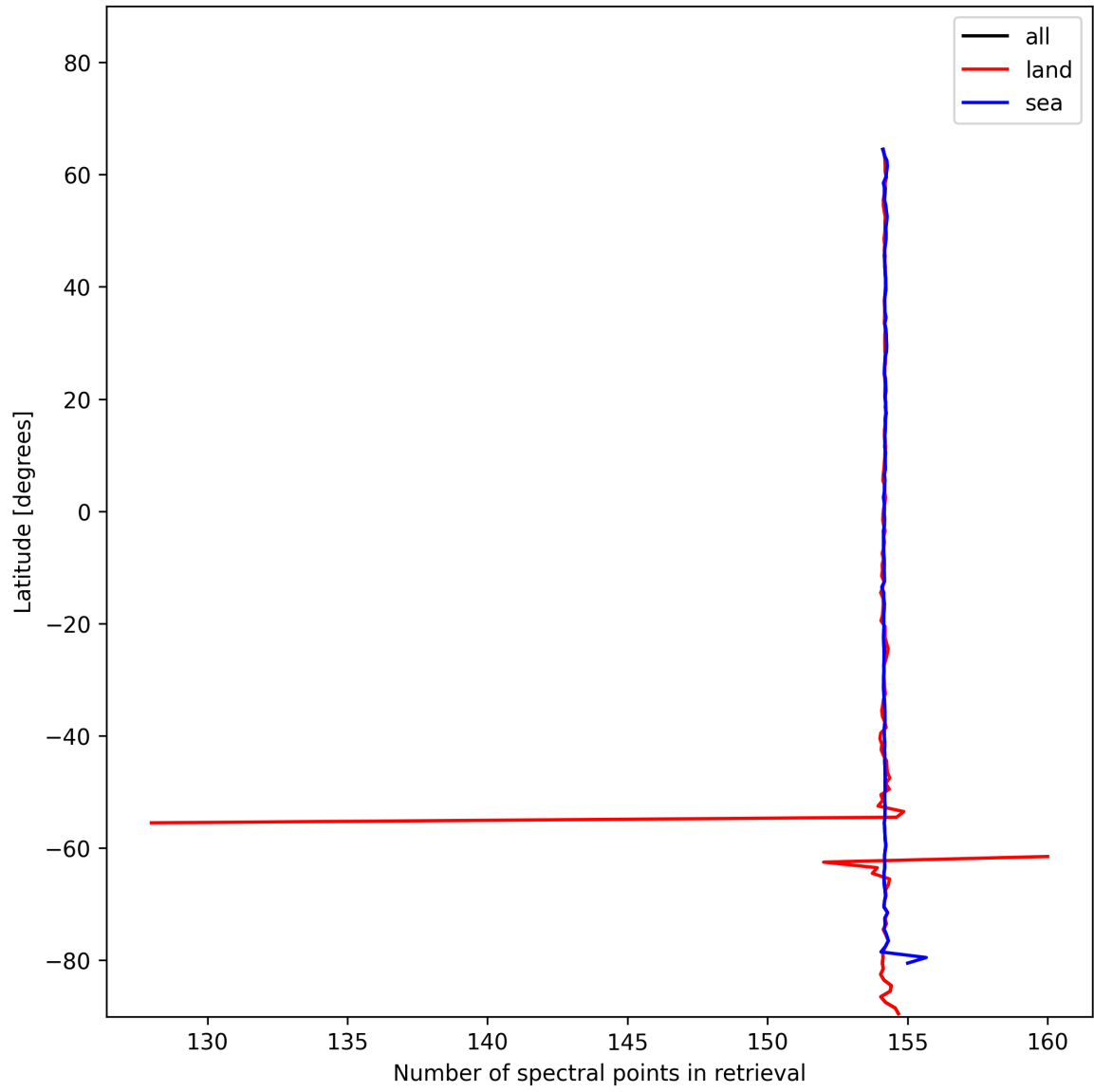
Figure 13: Zonal average of “Number of spectral points in retrieval” for 2024-11-21 to 2024-11-23.
