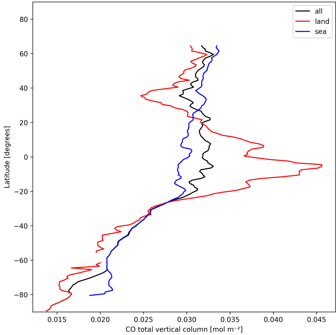
Figure 10: Zonal average of “CO total vertical column” for 2024-11-21 to 2024-11-23.
