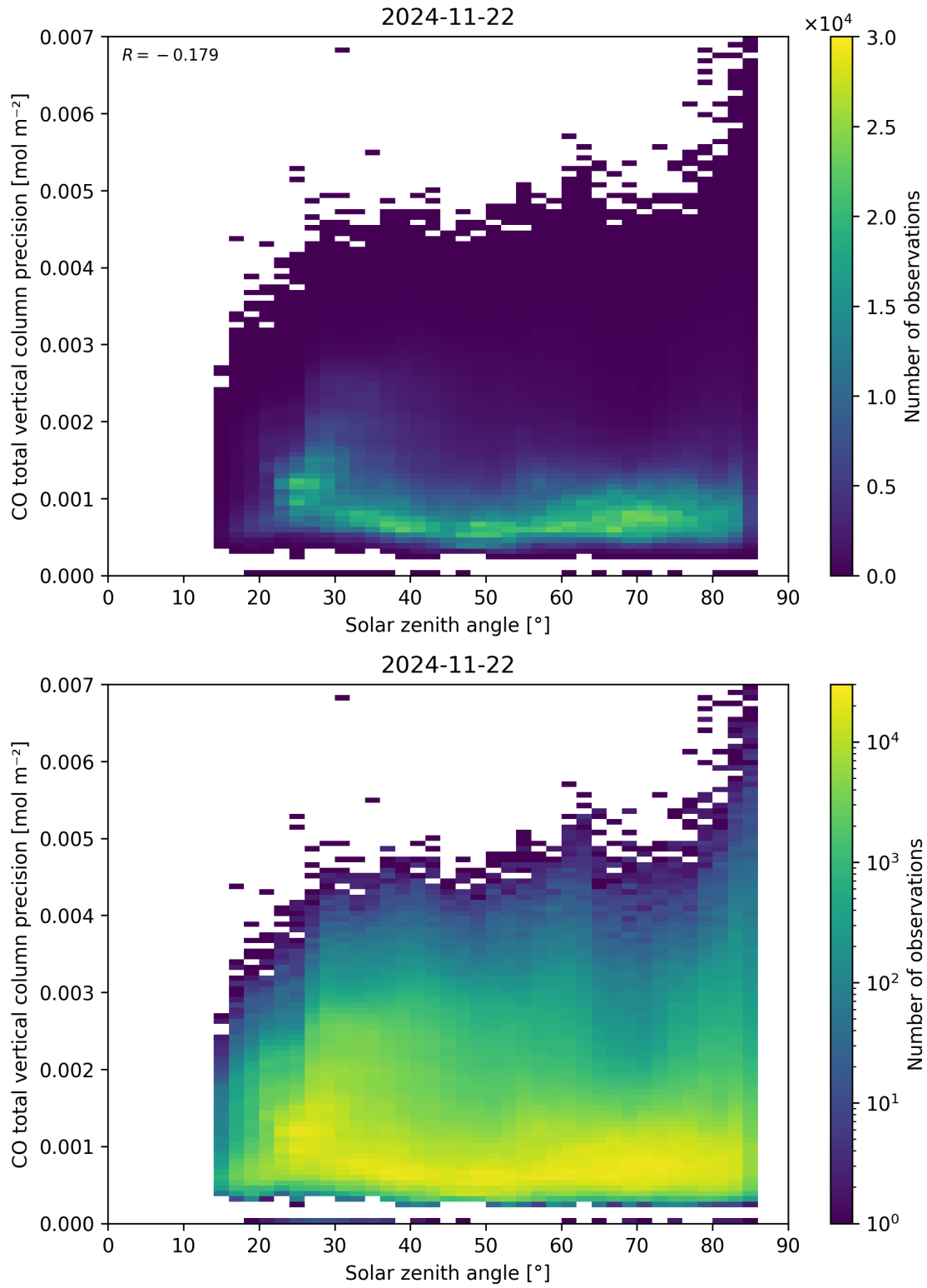
Figure 63: Scatter density plot of “Solar zenith angle” against “CO total vertical column precision” for 2024-11-21 to 2024-11-23.
