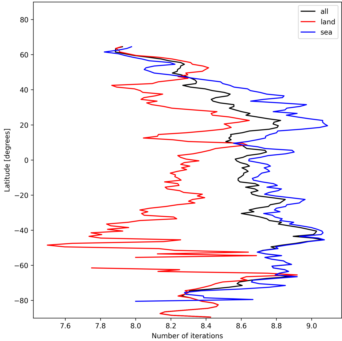
Figure 16: Zonal average of “Number of iterations” for 2024-11-21 to 2024-11-23.
