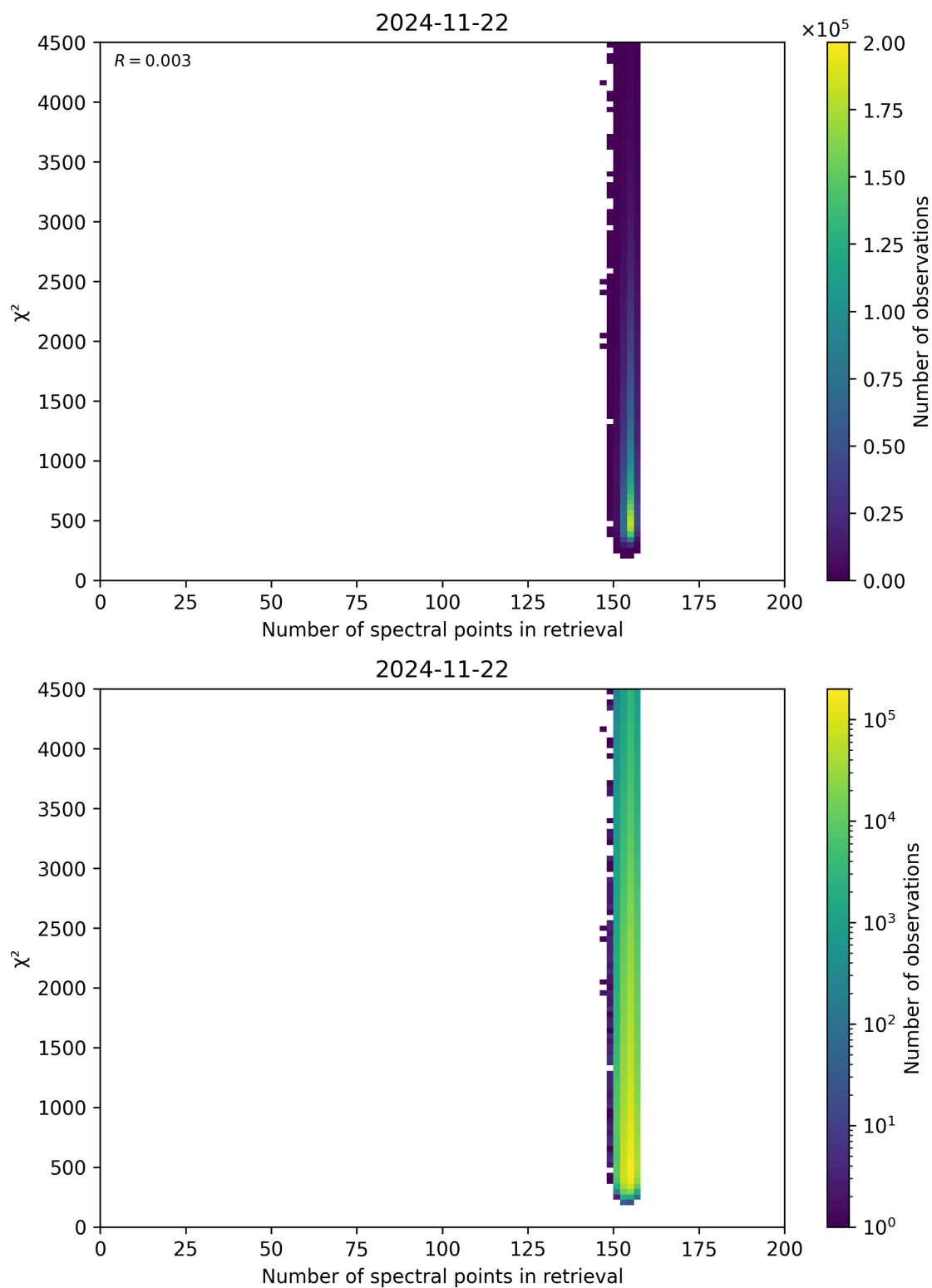
Figure 58: Scatter density plot of “Number of spectral points in retrieval” against “ \chi^2 ” for 2024-11-21 to 2024-11-23.
