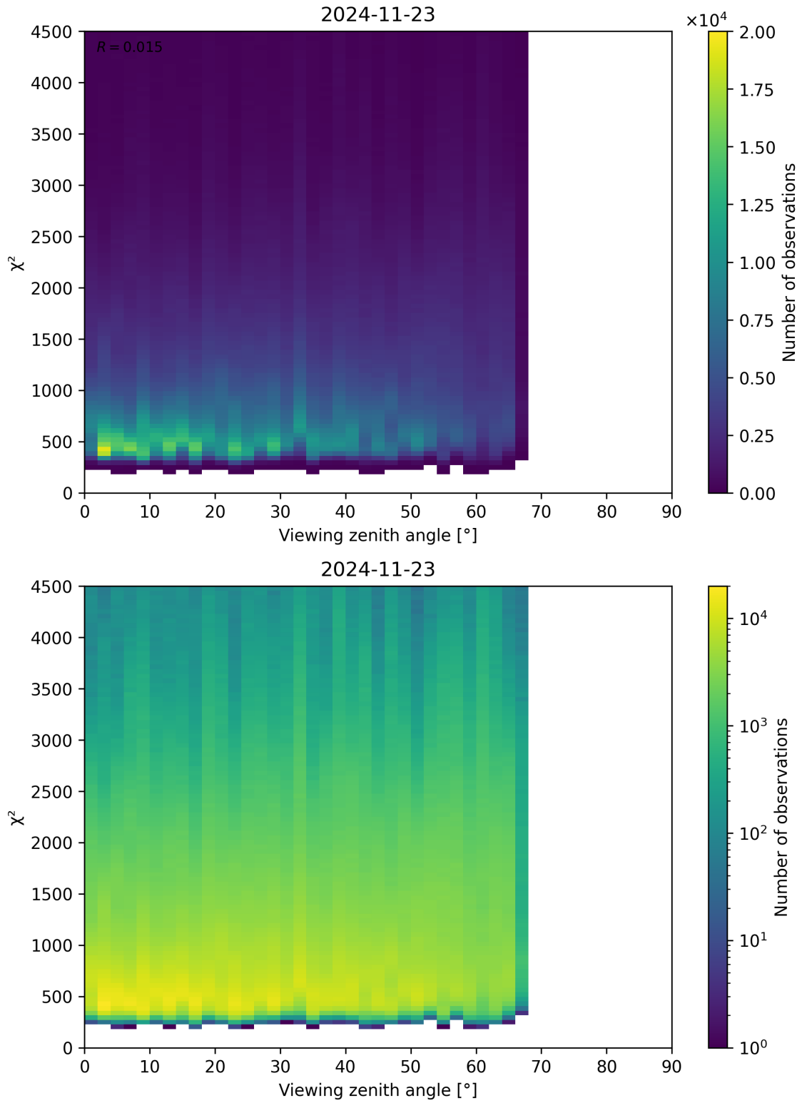
Figure 72: Scatter density plot of “Viewing zenith angle” against “ \chi^2 ” for 2024-11-22 to 2024-11-24.
