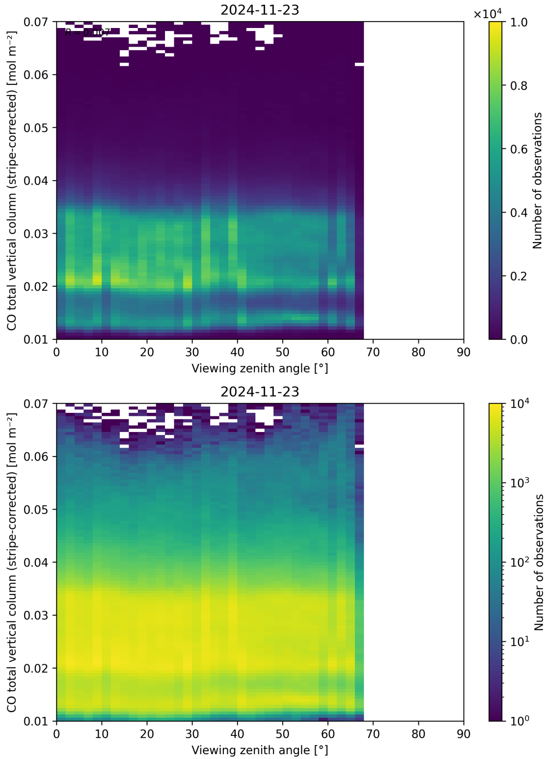
Figure 70: Scatter density plot of “Viewing zenith angle” against “CO total vertical column (stripe-corrected)” for 2024-11-22 to 2024-11-24.
