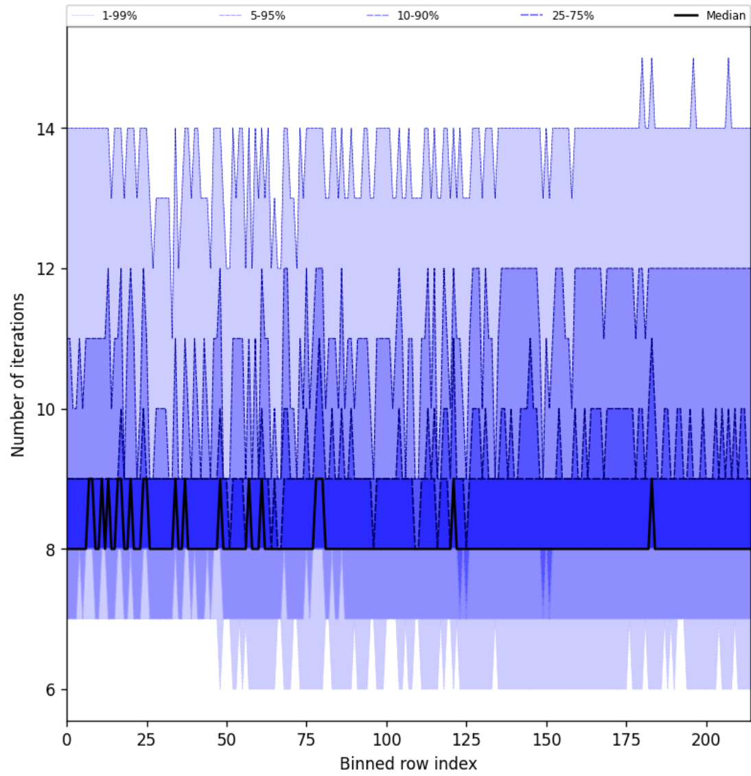
Figure 32: Along track statistics of “Number of iterations” for 2024-11-22 to 2024-11-24
