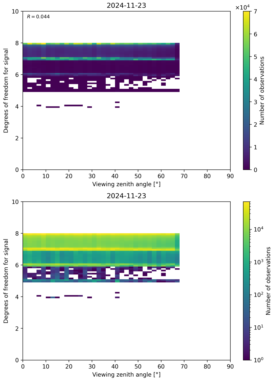
Figure 73: Scatter density plot of “Viewing zenith angle” against “Degrees of freedom for signal” for 2024-11-22 to 2024-11-24.
