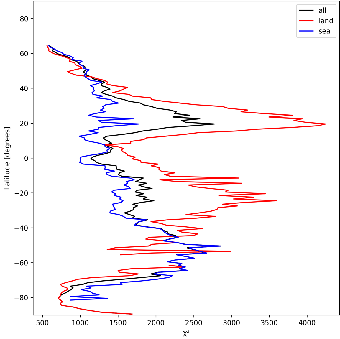
Figure 14: Zonal average of “ \chi^2 ” for 2024-11-22 to 2024-11-24.
