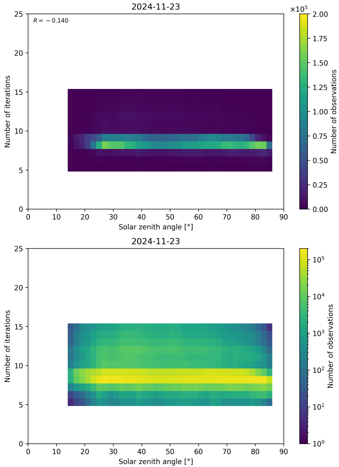
Figure 67: Scatter density plot of “Solar zenith angle” against “Number of iterations” for 2024-11-22 to 2024-11-24.
