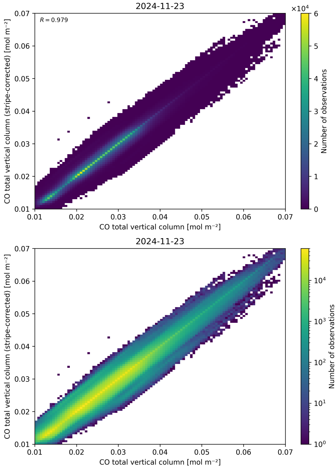
Figure 33: Scatter density plot of “CO total vertical column” against “CO total vertical column (stripe-corrected)” for 2024-11-22 to 2024-11-24.
