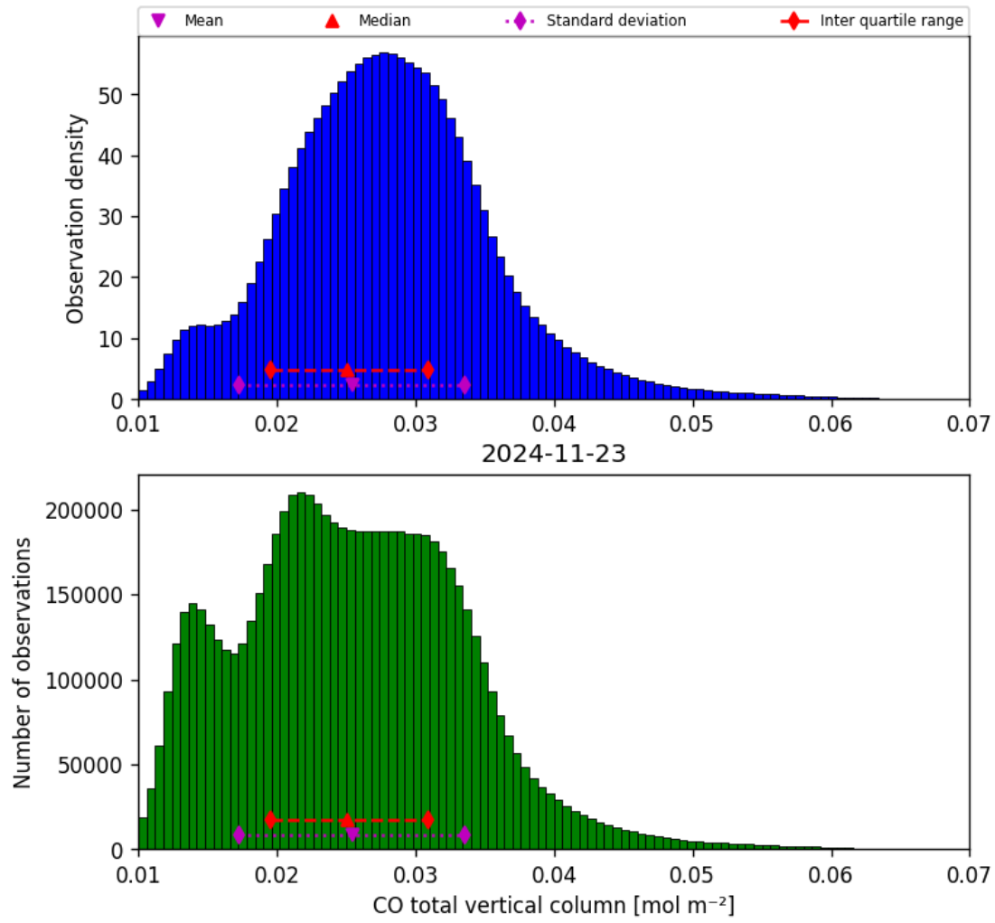
Figure 18: Histogram of “CO total vertical column” for 2024-11-22 to 2024-11-24
