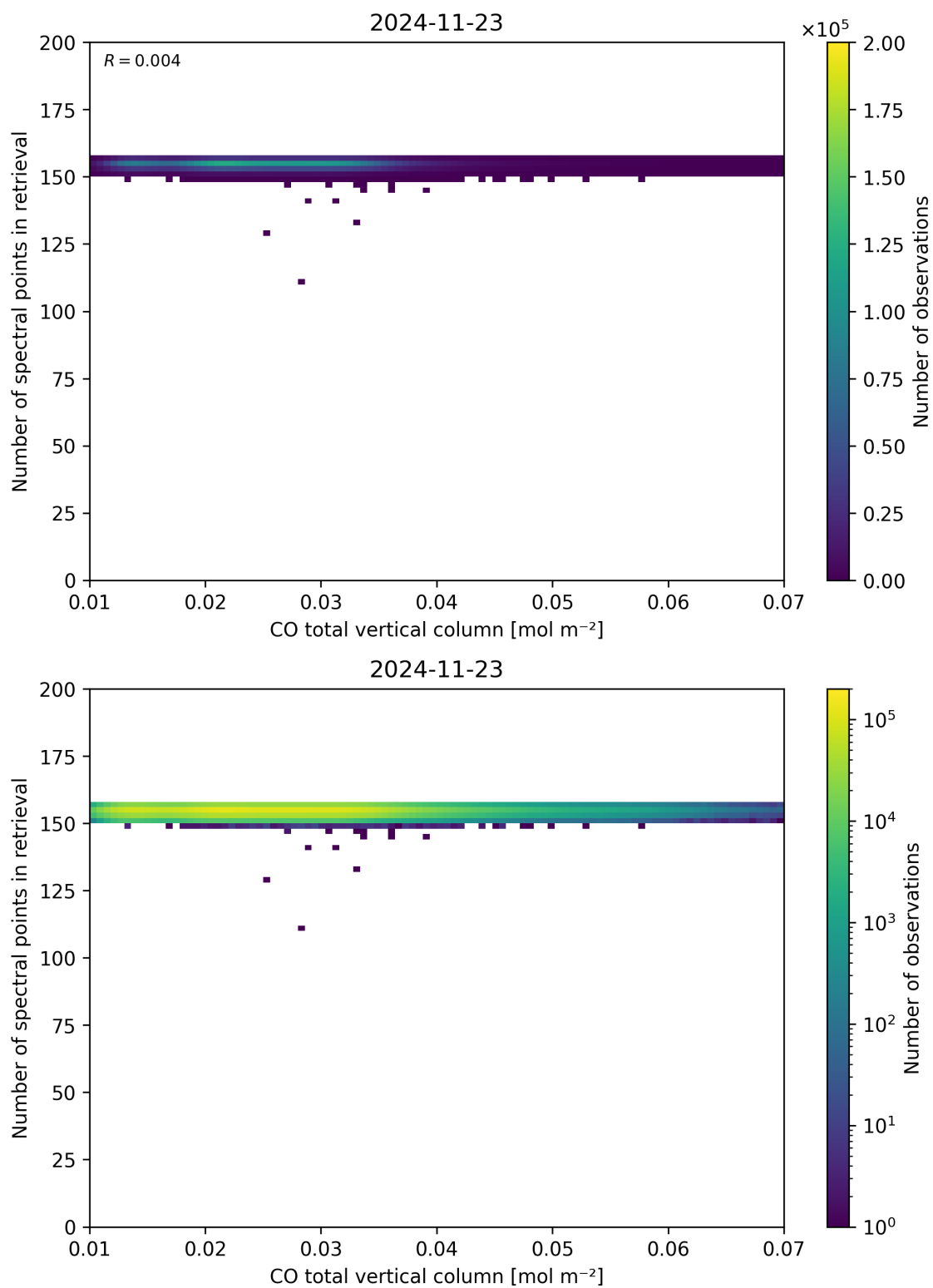
Figure 43: Scatter density plot of “CO total vertical column” against “Number of spectral points in retrieval” for 2024-11-22 to 2024-11-24.
