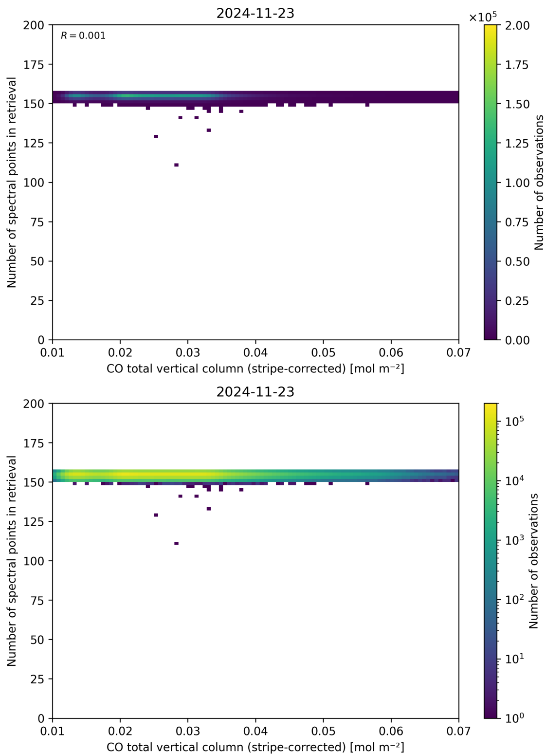
Figure 40: Scatter density plot of “CO total vertical column (stripe-corrected)” against “Number of spectral points in retrieval” for 2024-11-22 to 2024-11-24.
