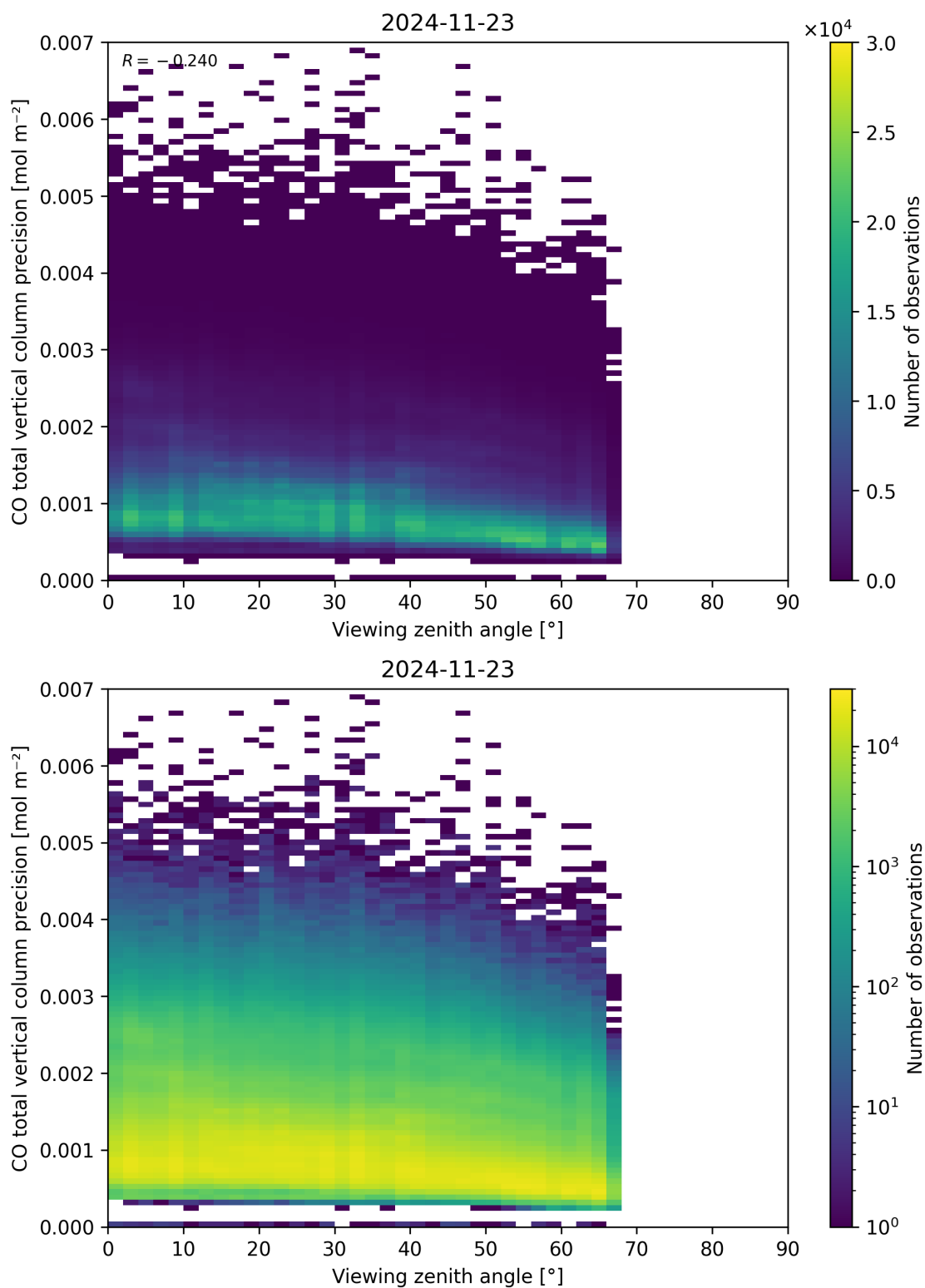
Figure 71: Scatter density plot of “Viewing zenith angle” against “CO total vertical column precision” for 2024-11-22 to 2024-11-24.
