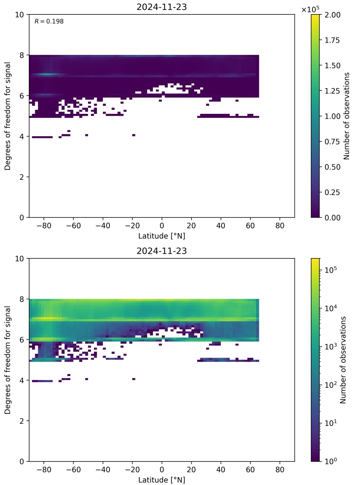
Figure 55: Scatter density plot of “Latitude” against “Degrees of freedom for signal” for 2024-11-22 to 2024-11-24.
