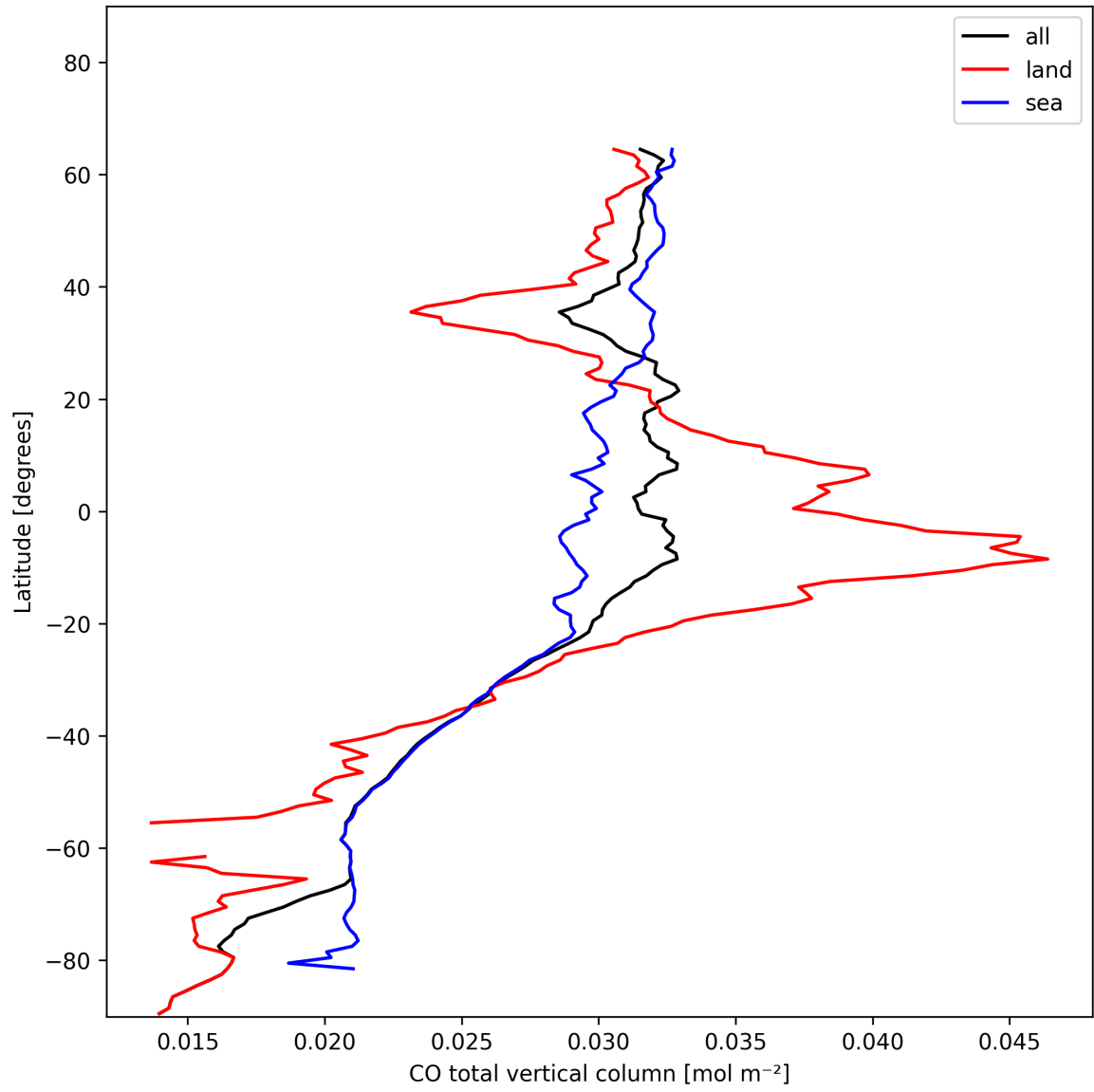
Figure 10: Zonal average of “CO total vertical column” for 2024-11-22 to 2024-11-24.
