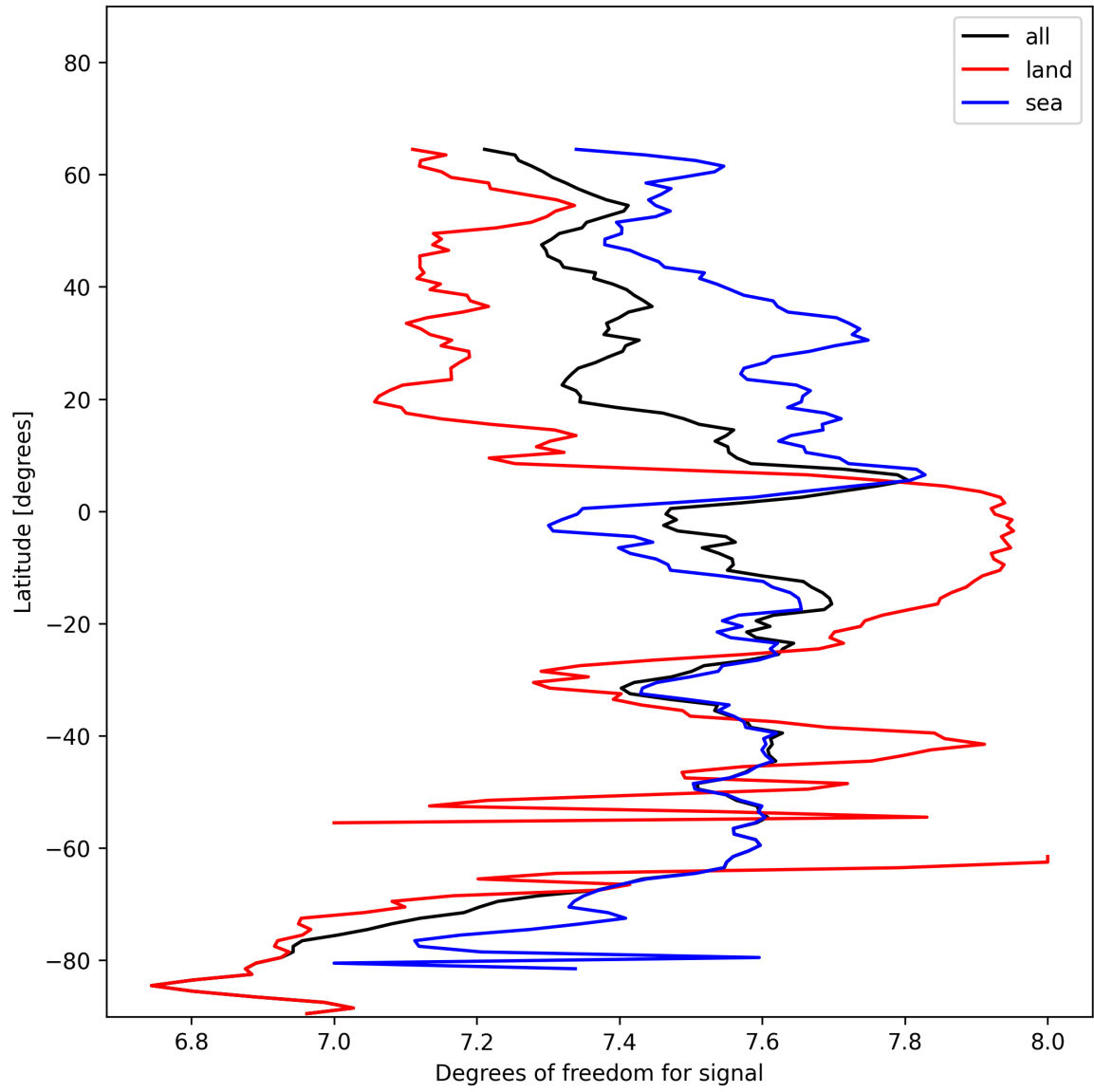
Figure 15: Zonal average of “Degrees of freedom for signal” for 2024-11-22 to 2024-11-24.
