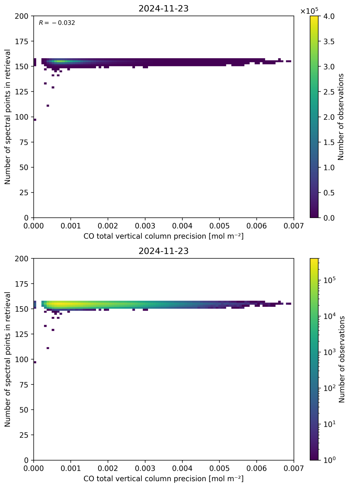
Figure 47: Scatter density plot of “CO total vertical column precision” against “Number of spectral points in retrieval” for 2024-11-22 to 2024-11-24.
