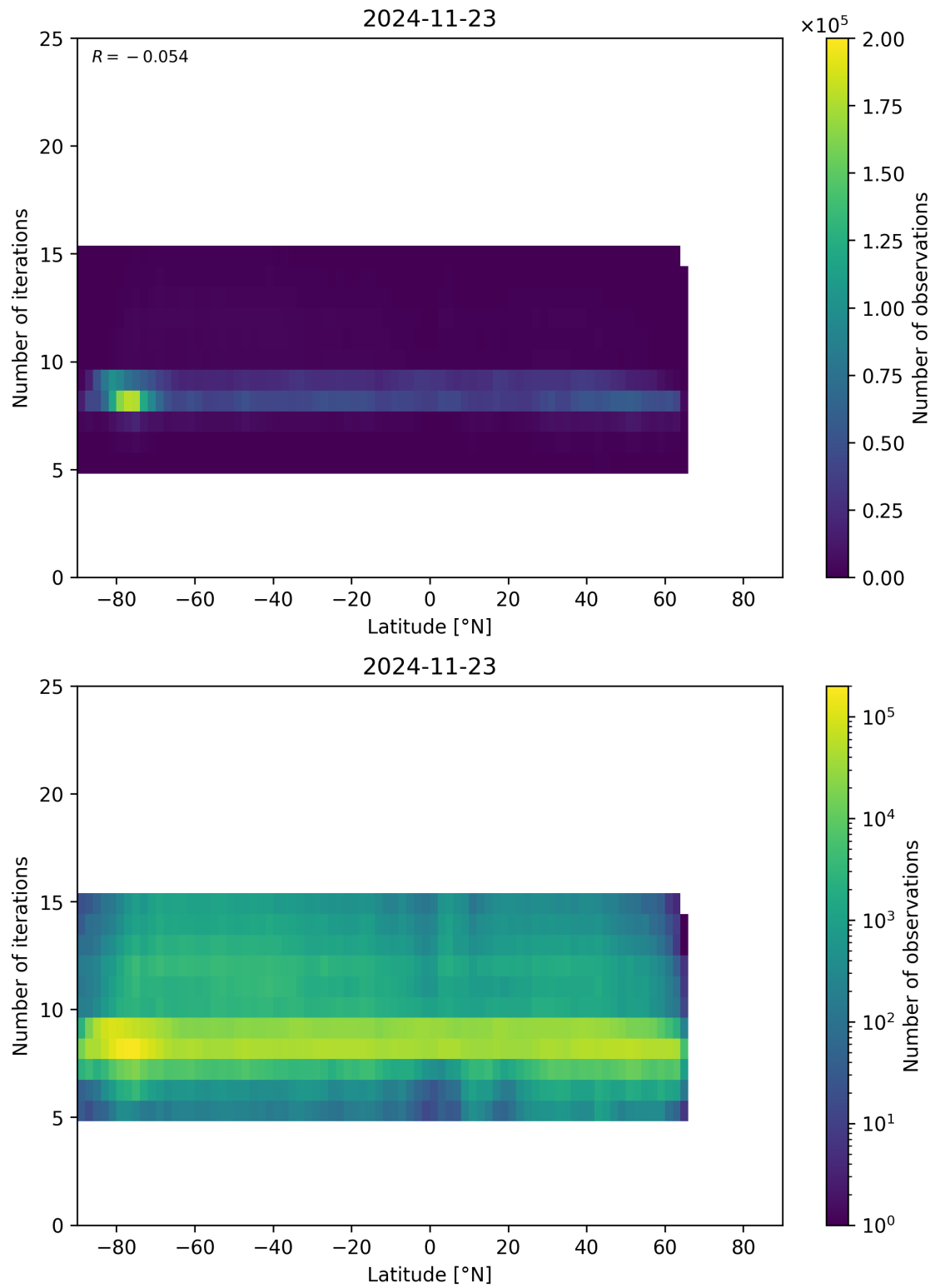
Figure 56: Scatter density plot of “Latitude” against “Number of iterations” for 2024-11-22 to 2024-11-24.
