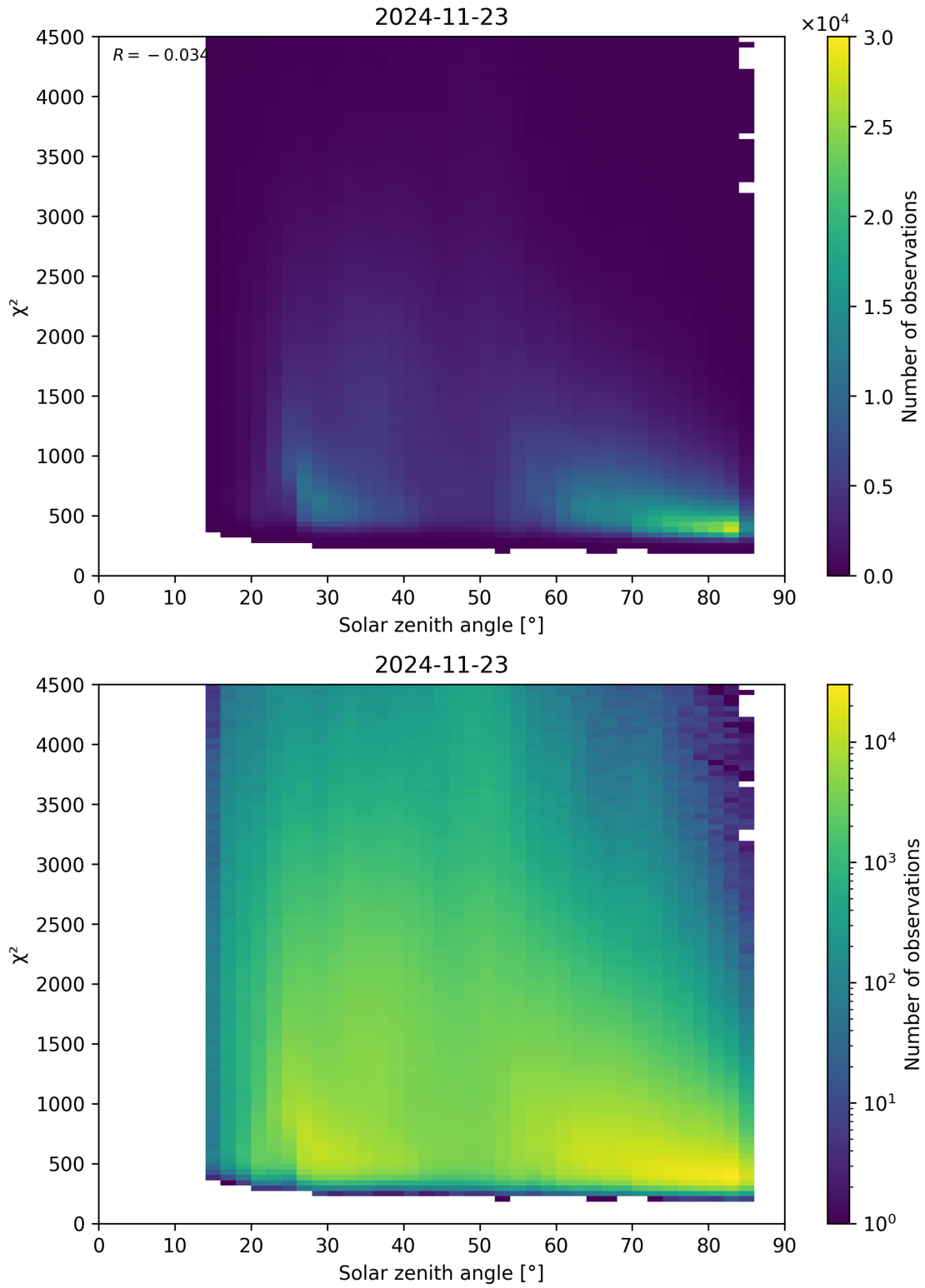
Figure 64: Scatter density plot of “Solar zenith angle” against “ \chi^2 ” for 2024-11-22 to 2024-11-24.
