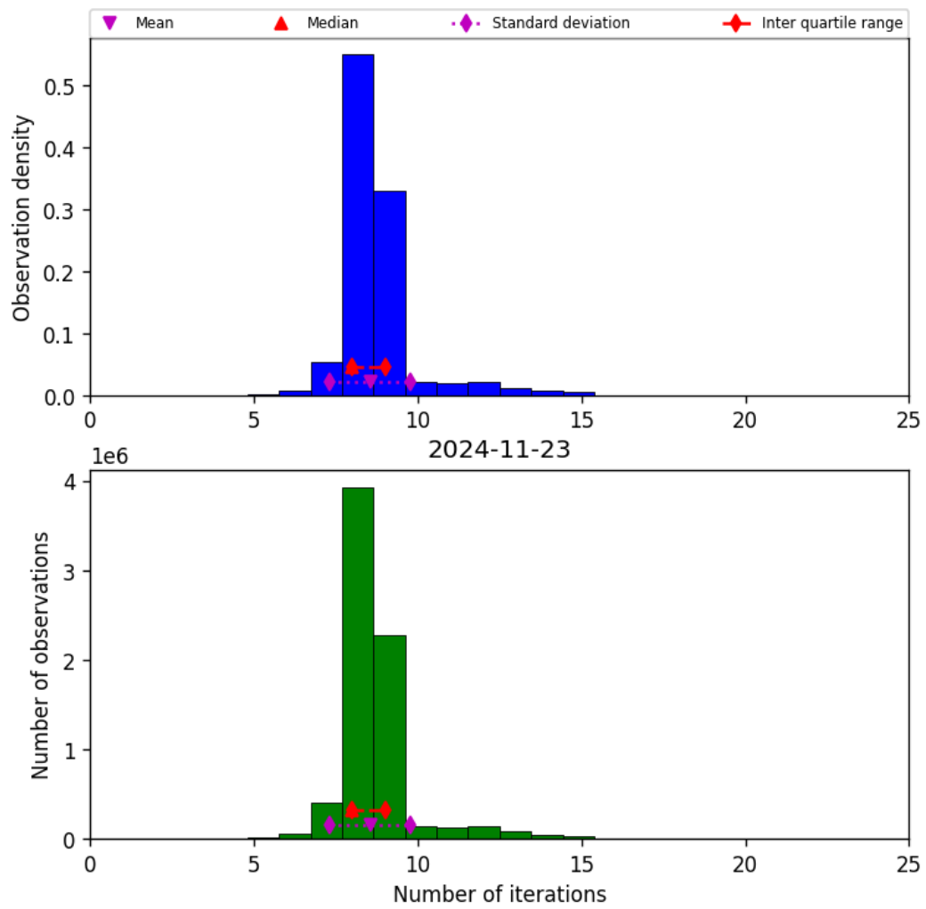
Figure 24: Histogram of “Number of iterations” for 2024-11-22 to 2024-11-24
