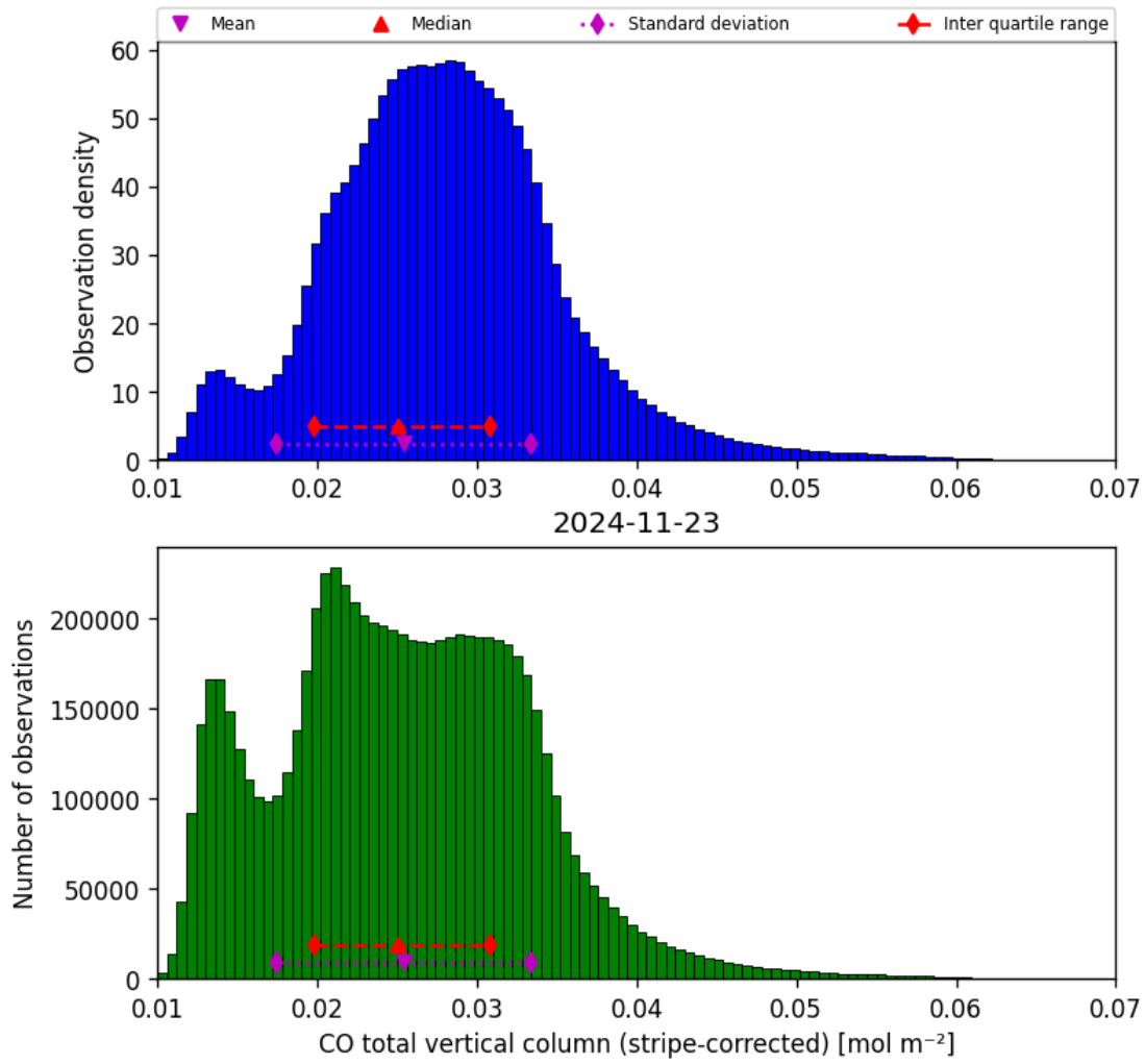
Figure 19: Histogram of “CO total vertical column (stripe-corrected)” for 2024-11-22 to 2024-11-24
