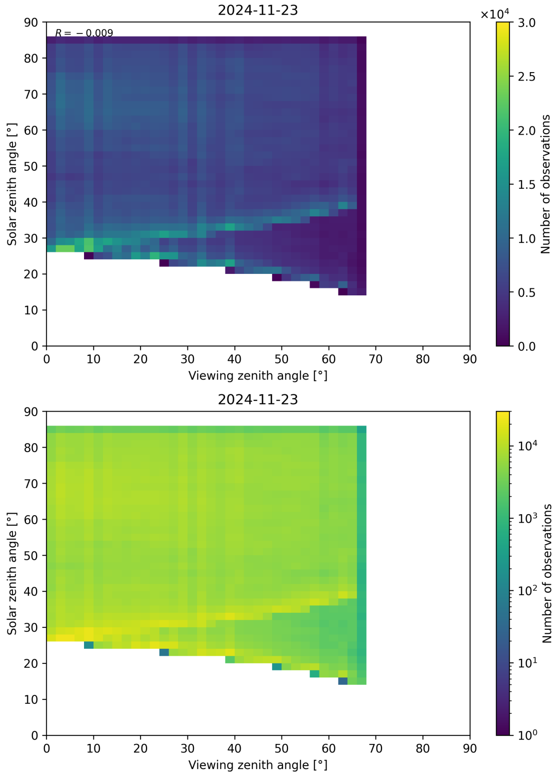
Figure 77: Scatter density plot of “Viewing zenith angle” against “Solar zenith angle” for 2024-11-22 to 2024-11-24.
