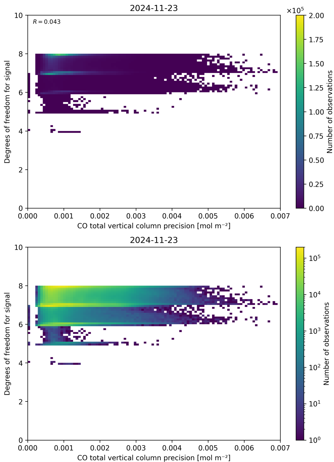
Figure 45: Scatter density plot of “CO total vertical column precision” against “Degrees of freedom for signal” for 2024-11-22 to 2024-11-24.
