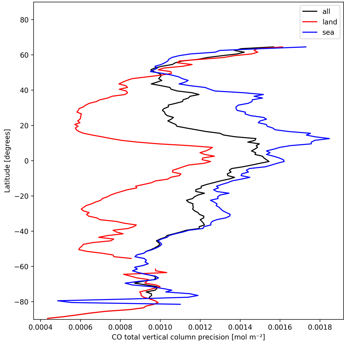
Figure 12: Zonal average of "CO total vertical column precision" for 2024-11-22 to 2024-11-24.
