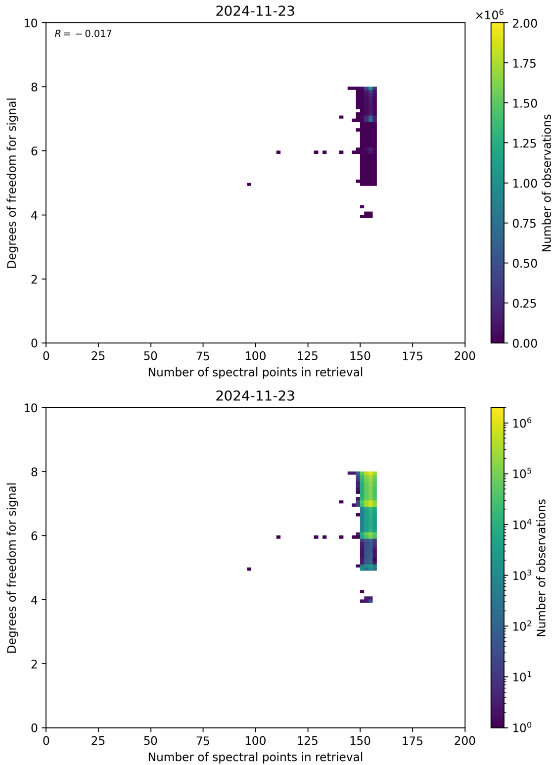
Figure 59: Scatter density plot of “Number of spectral points in retrieval” against “Degrees of freedom for signal” for 2024-11-22 to 2024-11-24.
