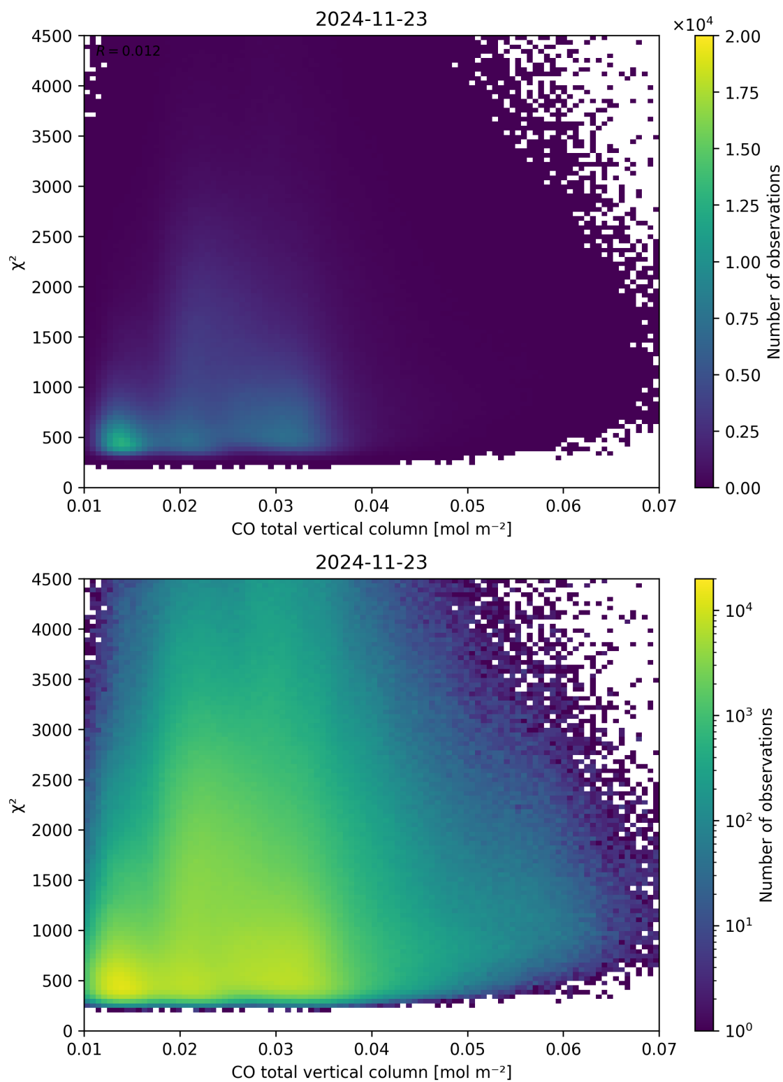
Figure 35: Scatter density plot of “CO total vertical column” against “ \chi^2 ” for 2024-11-22 to 2024-11-24.
