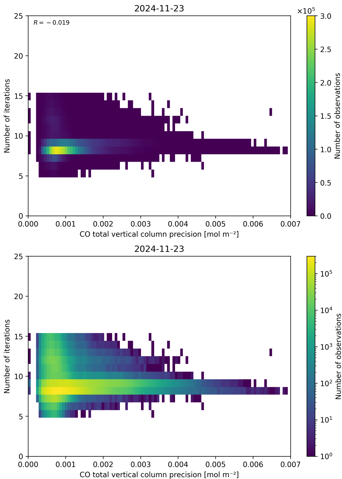
Figure 46: Scatter density plot of “CO total vertical column precision” against “Number of iterations” for 2024-11-22 to 2024-11-24.
