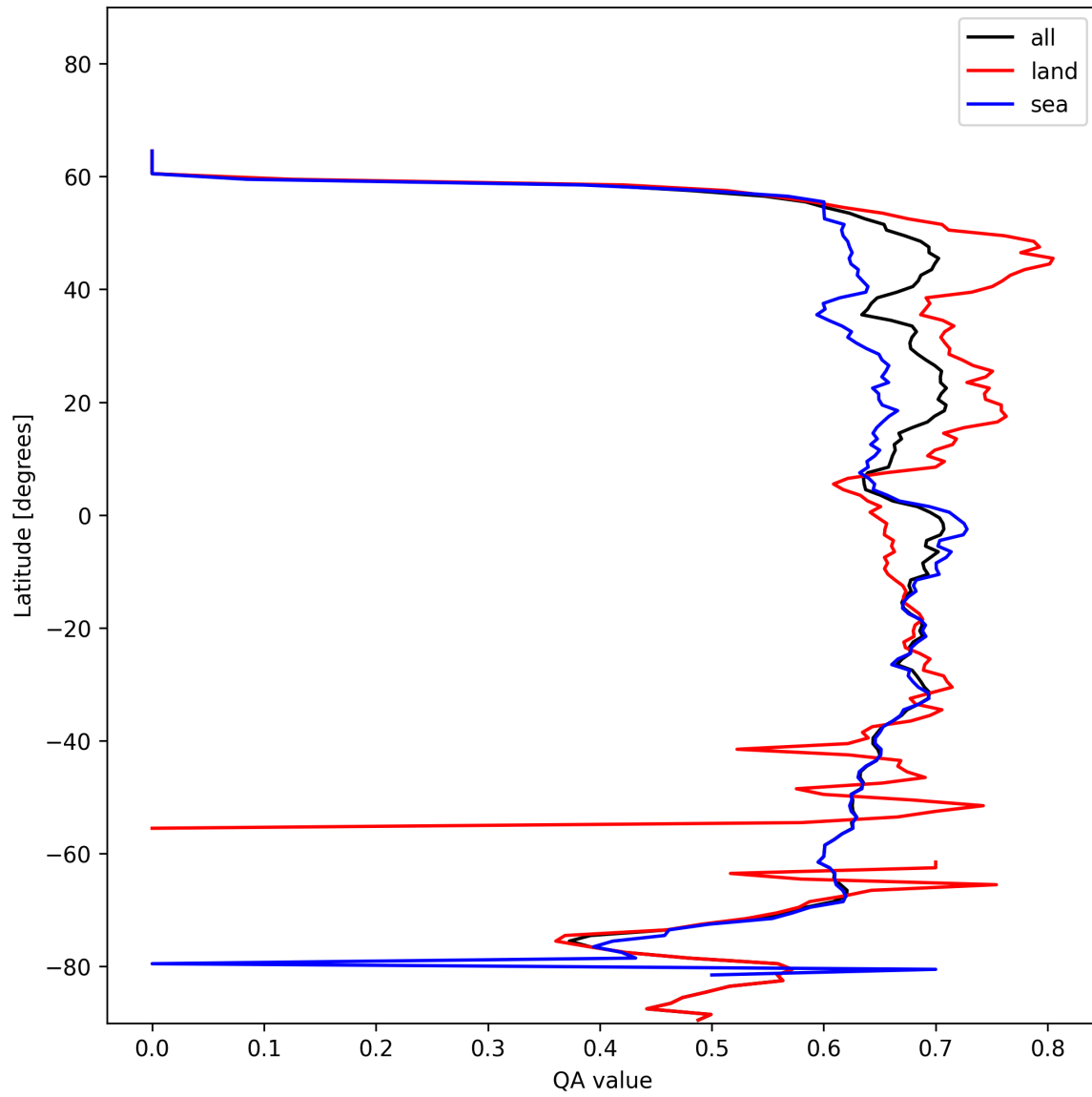
Figure 9: Zonal average of “QA value” for 2024-11-22 to 2024-11-24.
