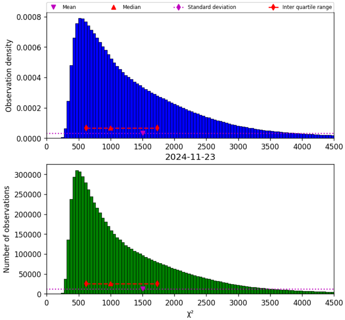
Figure 22: Histogram of “ \chi^2 ” for 2024-11-22 to 2024-11-24
