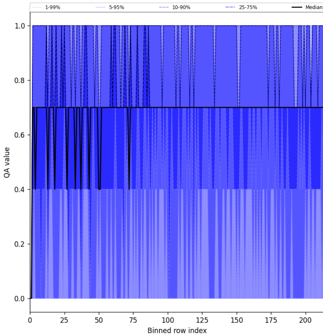
Figure 25: Along track statistics of “QA value” for 2024-11-22 to 2024-11-24
