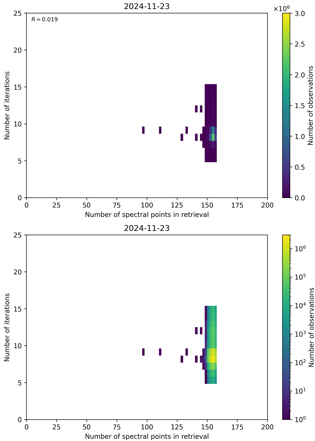
Figure 60: Scatter density plot of “Number of spectral points in retrieval” against “Number of iterations” for 2024-11-22 to 2024-11-24.
