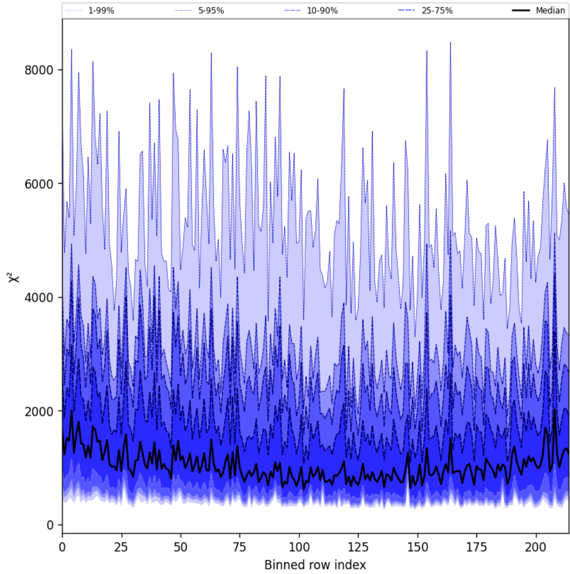
Figure 30: Along track statistics of “ \chi^2 ” for 2024-11-22 to 2024-11-24
