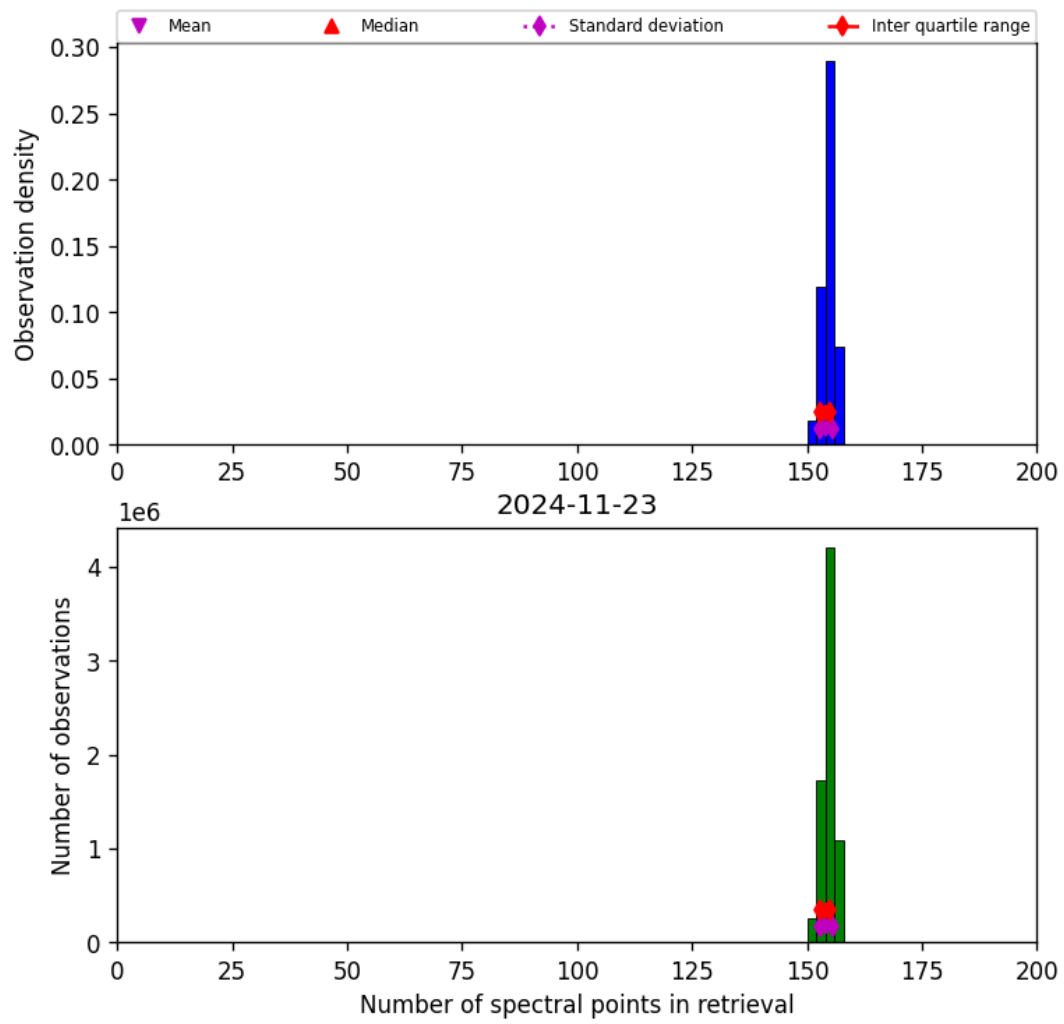
Figure 21: Histogram of “Number of spectral points in retrieval” for 2024-11-22 to 2024-11-24
