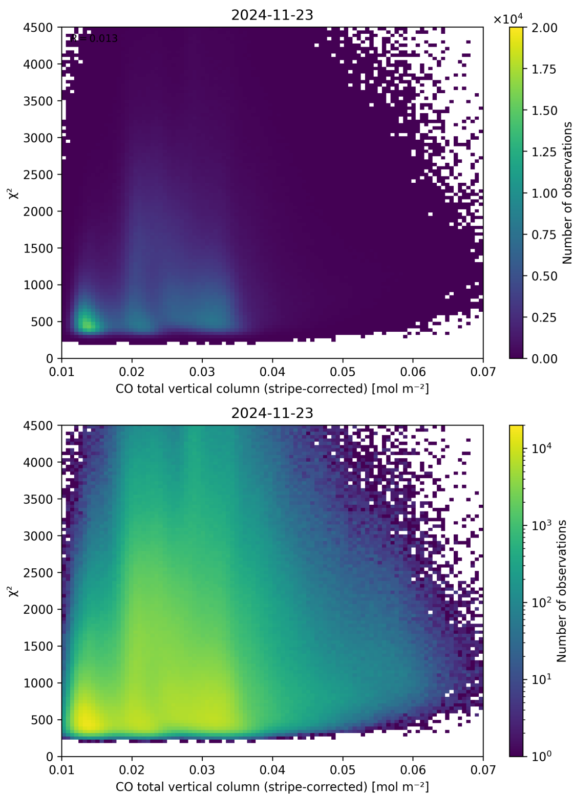
Figure 37: Scatter density plot of “CO total vertical column (stripe-corrected)” against “ \chi^2 ” for 2024-11-22 to 2024-11-24.
