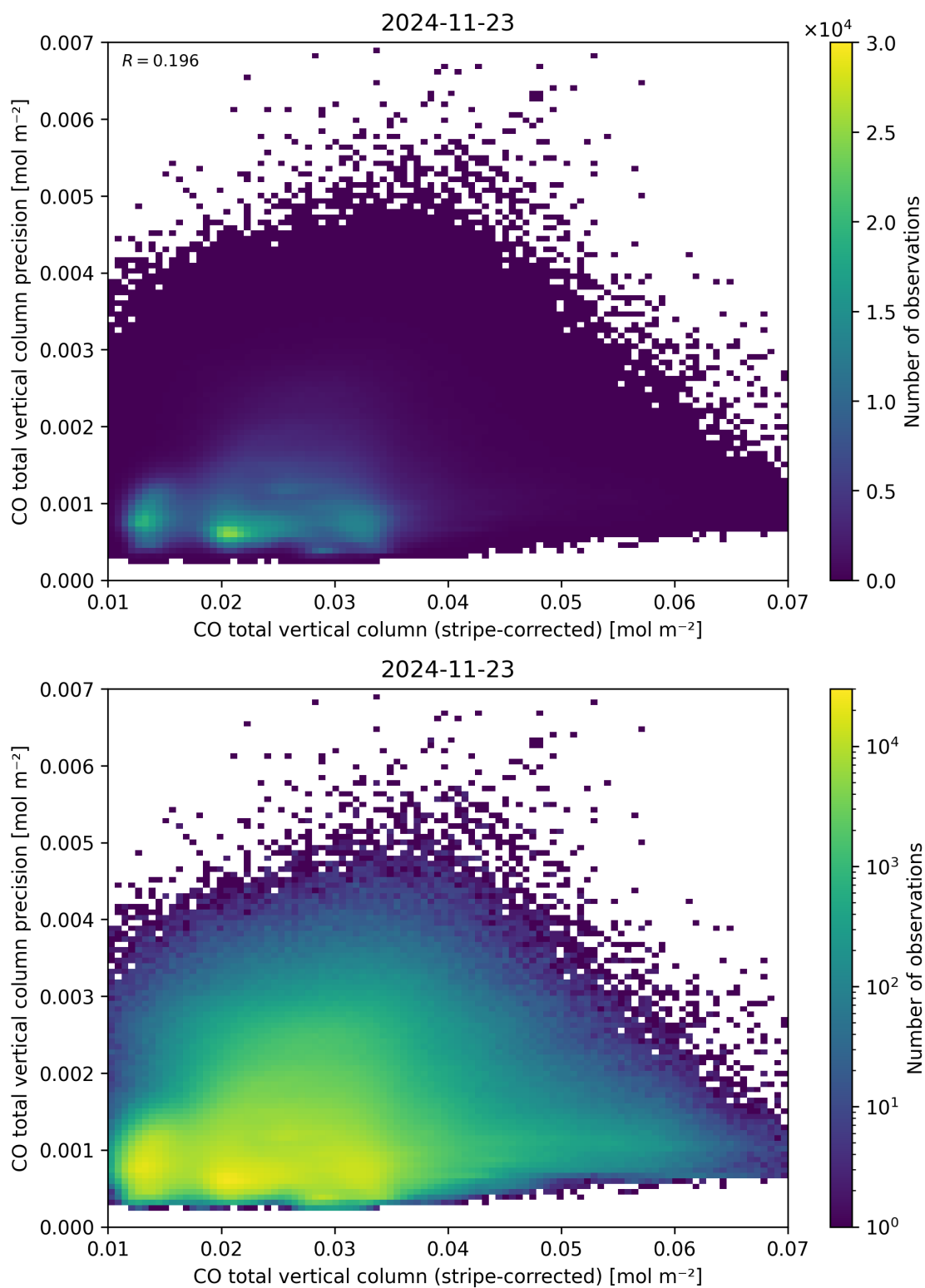
Figure 36: Scatter density plot of “CO total vertical column (stripe-corrected)” against “CO total vertical column precision” for 2024-11-22 to 2024-11-24.
