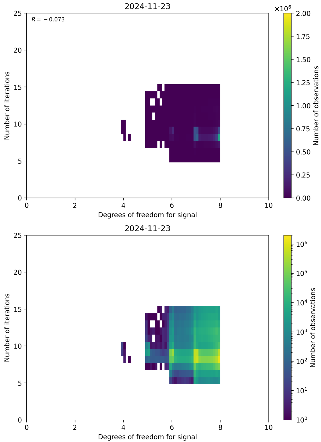
Figure 50: Scatter density plot of “Degrees of freedom for signal” against “Number of iterations” for 2024-11-22 to 2024-11-24.
