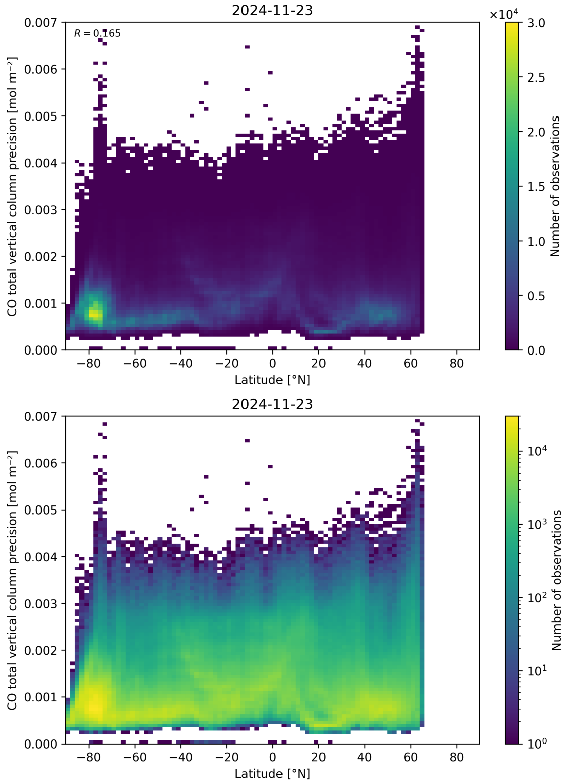
Figure 53: Scatter density plot of “Latitude” against “CO total vertical column precision” for 2024-11-22 to 2024-11-24.
