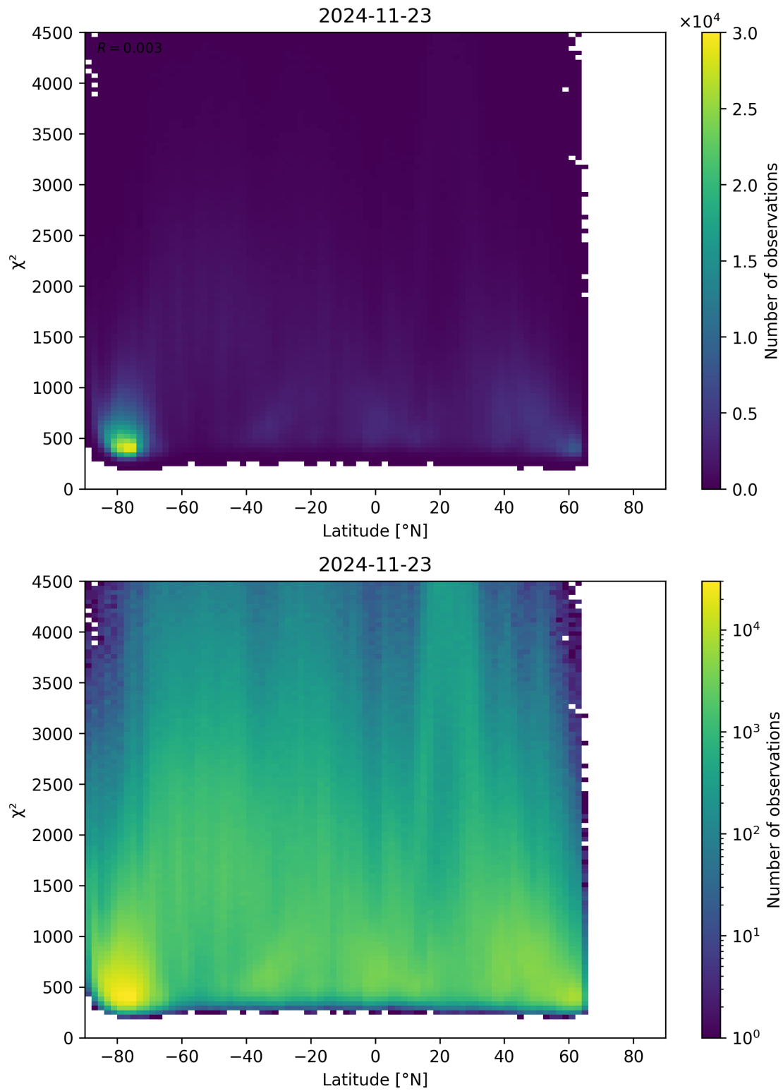
Figure 54: Scatter density plot of “Latitude” against “ \chi^2 ” for 2024-11-22 to 2024-11-24.
