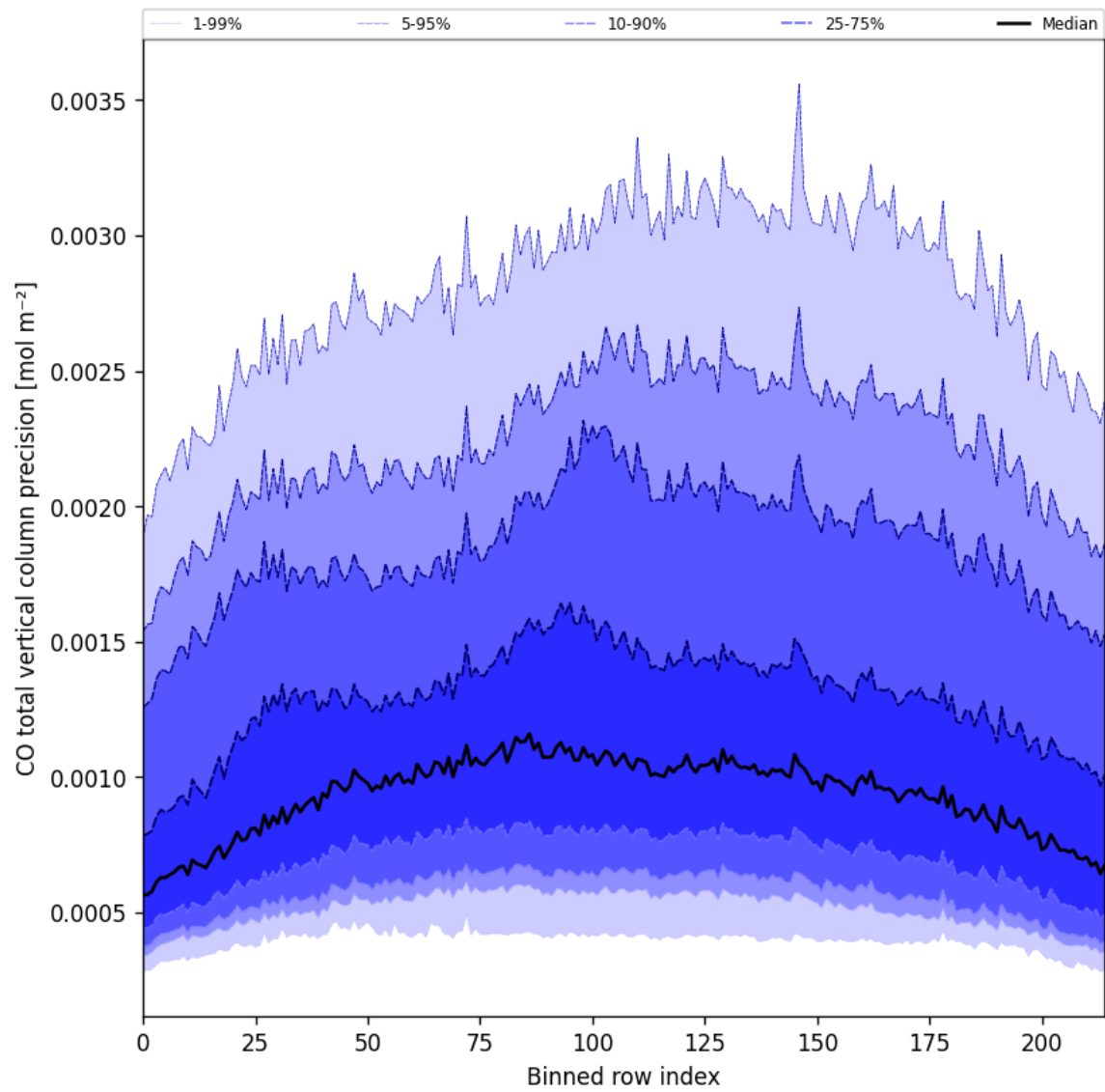
Figure 28: Along track statistics of “CO total vertical column precision” for 2024-11-22 to 2024-11-24
