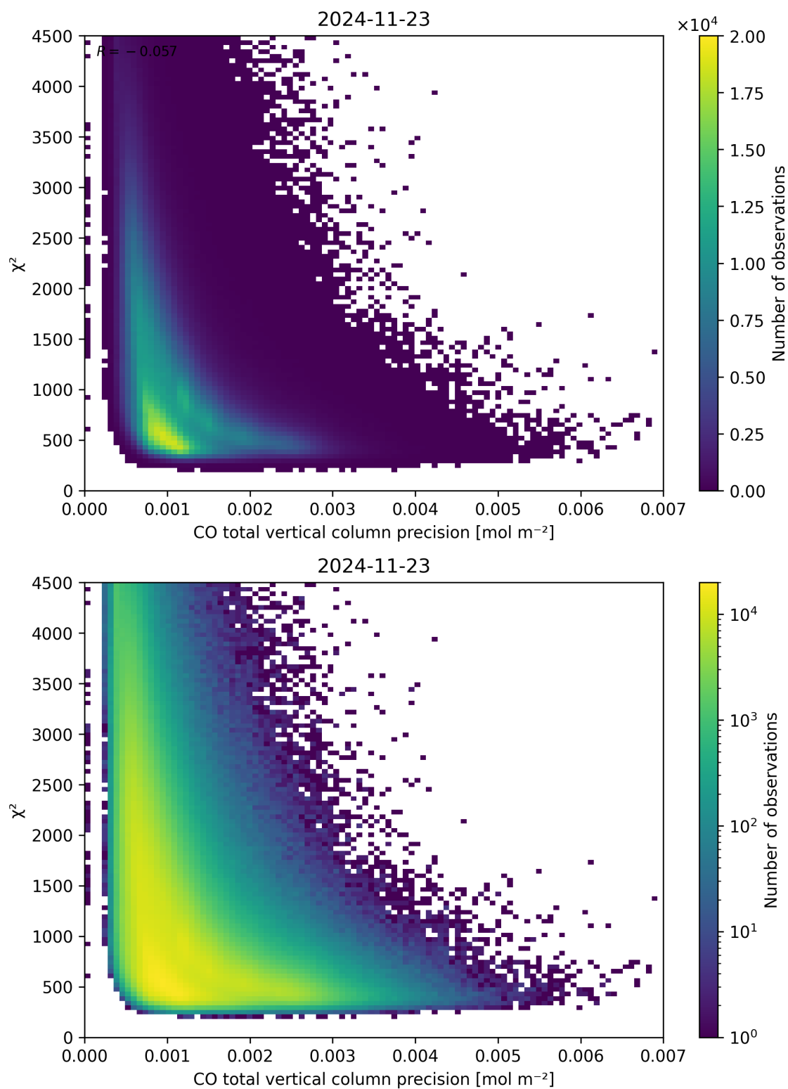
Figure 44: Scatter density plot of “CO total vertical column precision” against “ \chi^2 ” for 2024-11-22 to 2024-11-24.
