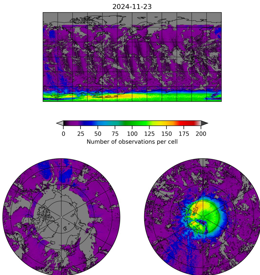
Figure 8: Map of the number of observations for 2024-11-22 to 2024-11-24
