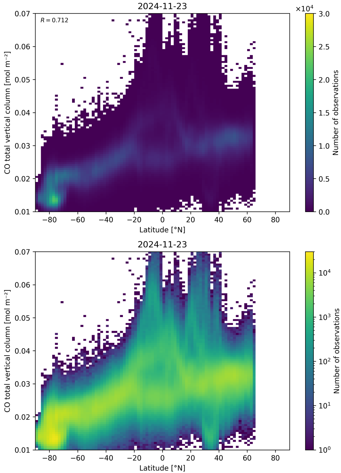
Figure 51: Scatter density plot of “Latitude” against “CO total vertical column” for 2024-11-22 to 2024-11-24.
