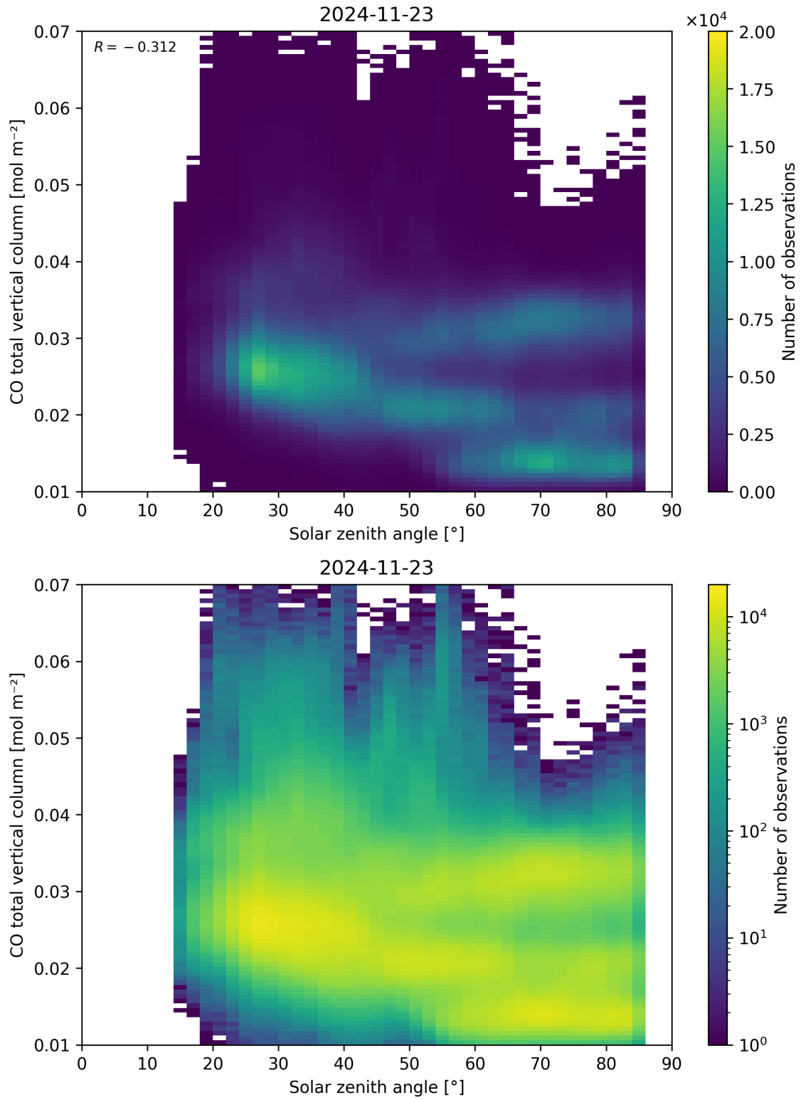
Figure 61: Scatter density plot of “Solar zenith angle” against “CO total vertical column” for 2024-11-22 to 2024-11-24.
