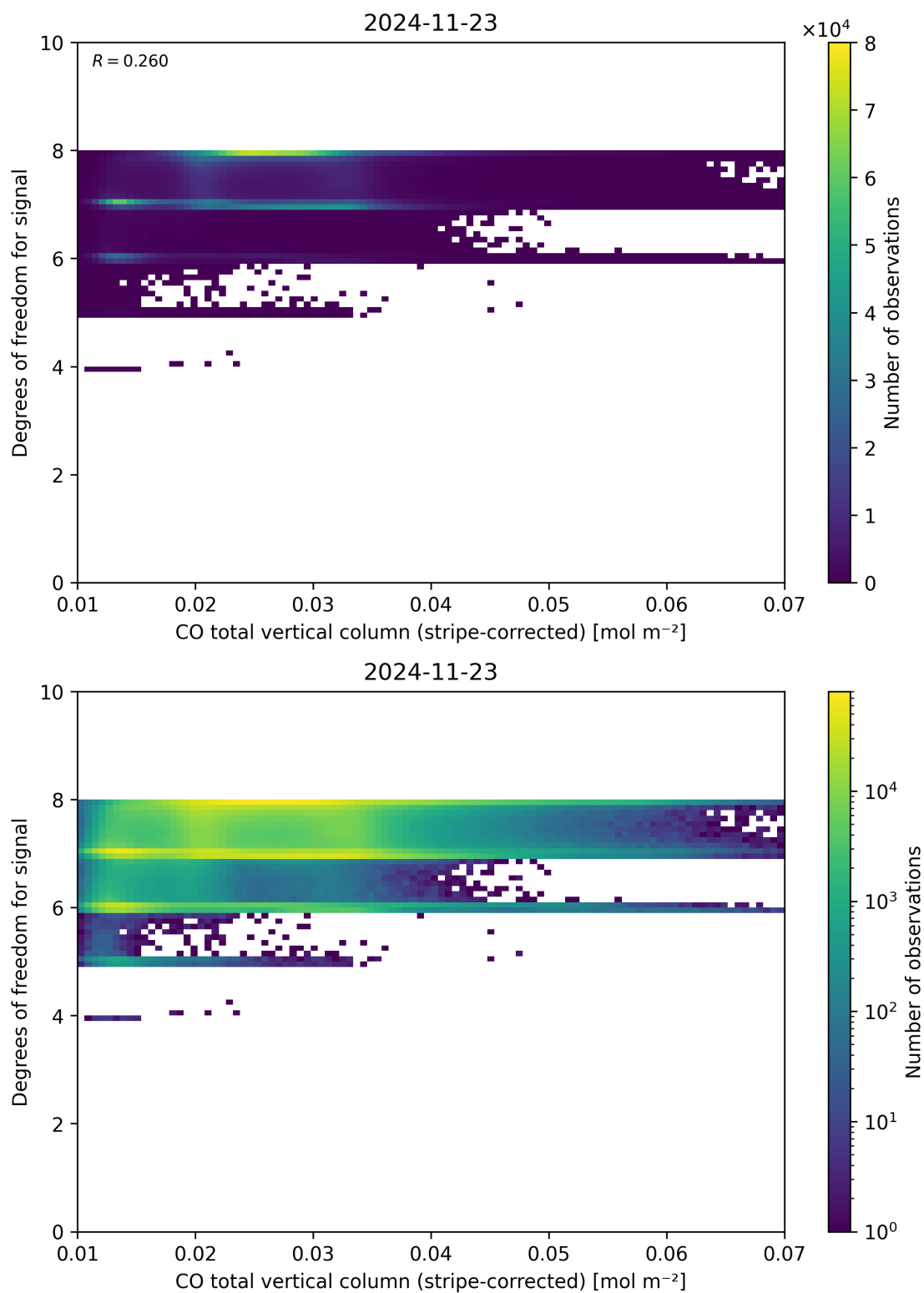
Figure 38: Scatter density plot of “CO total vertical column (stripe-corrected)” against “Degrees of freedom for signal” for 2024-11-22 to 2024-11-24.
