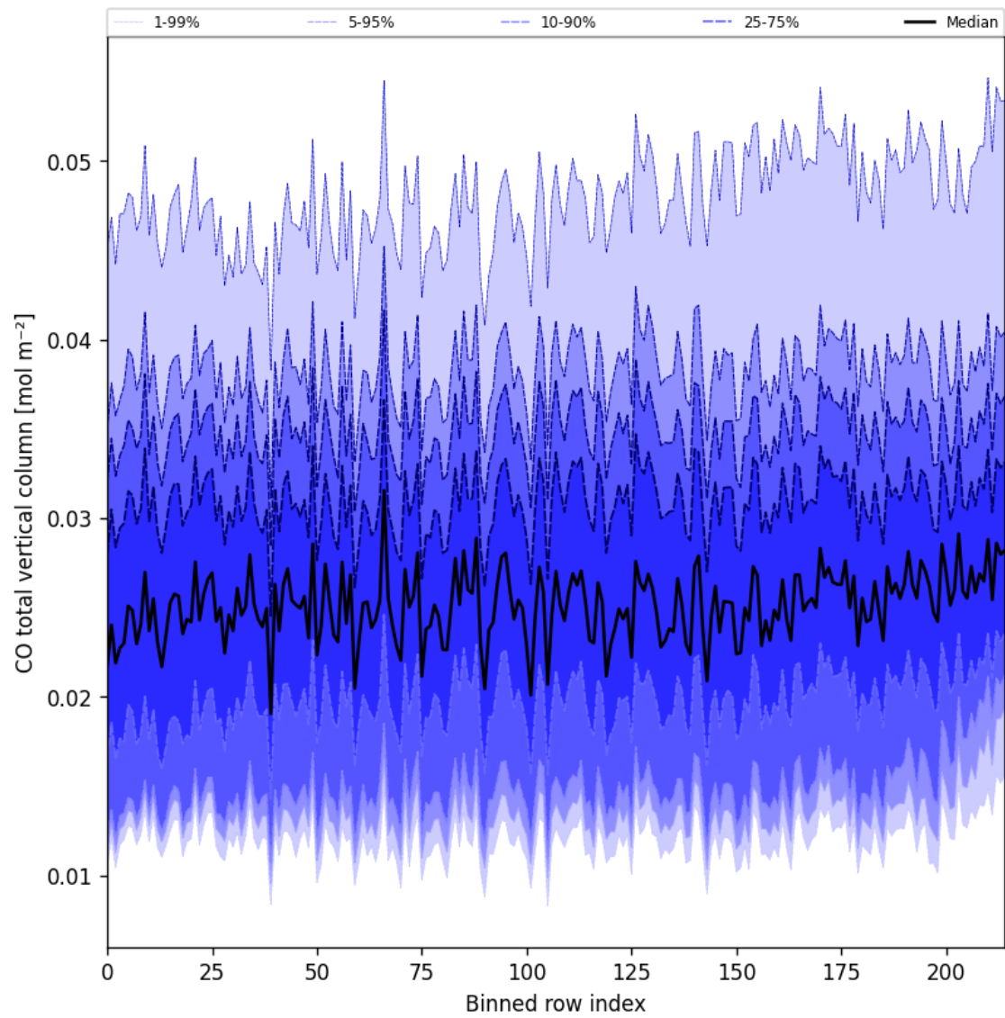
Figure 26: Along track statistics of “CO total vertical column” for 2024-11-22 to 2024-11-24
