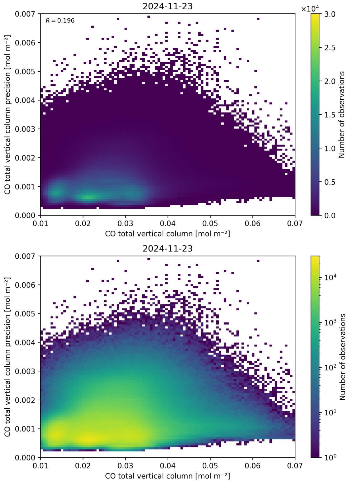
Figure 34: Scatter density plot of “CO total vertical column” against “CO total vertical column precision” for 2024-11-22 to 2024-11-24.
