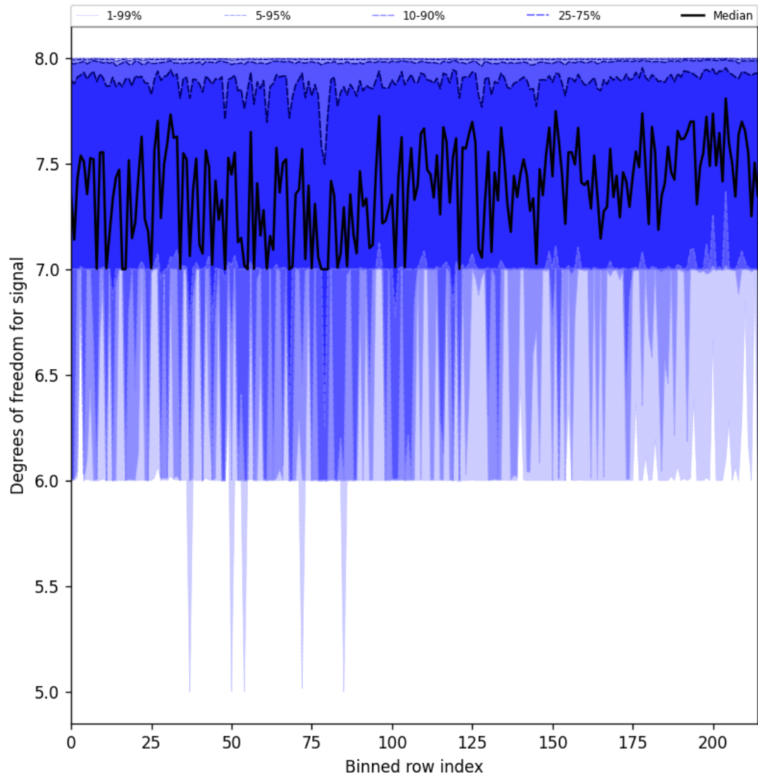
Figure 31: Along track statistics of “Degrees of freedom for signal” for 2024-11-22 to 2024-11-24
