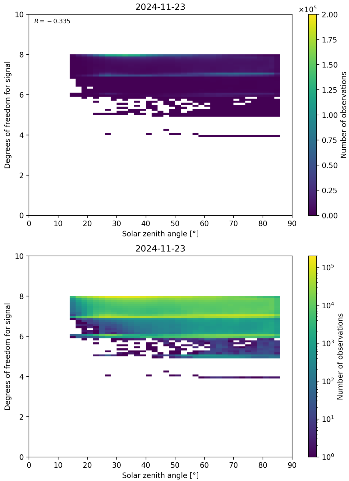
Figure 65: Scatter density plot of “Solar zenith angle” against “Degrees of freedom for signal” for 2024-11-22 to 2024-11-24.
