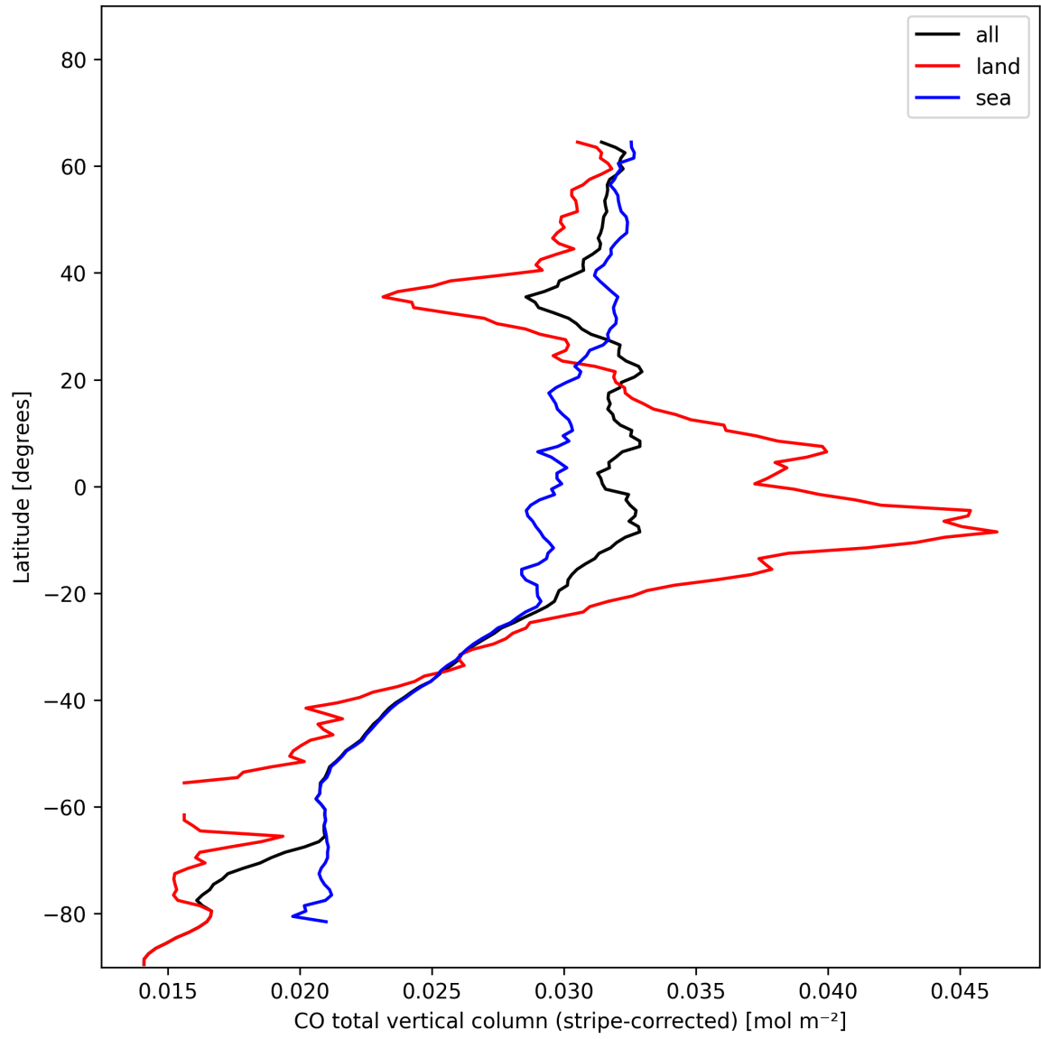
Figure 11: Zonal average of “CO total vertical column (stripe-corrected)” for 2024-11-22 to 2024-11-24.
