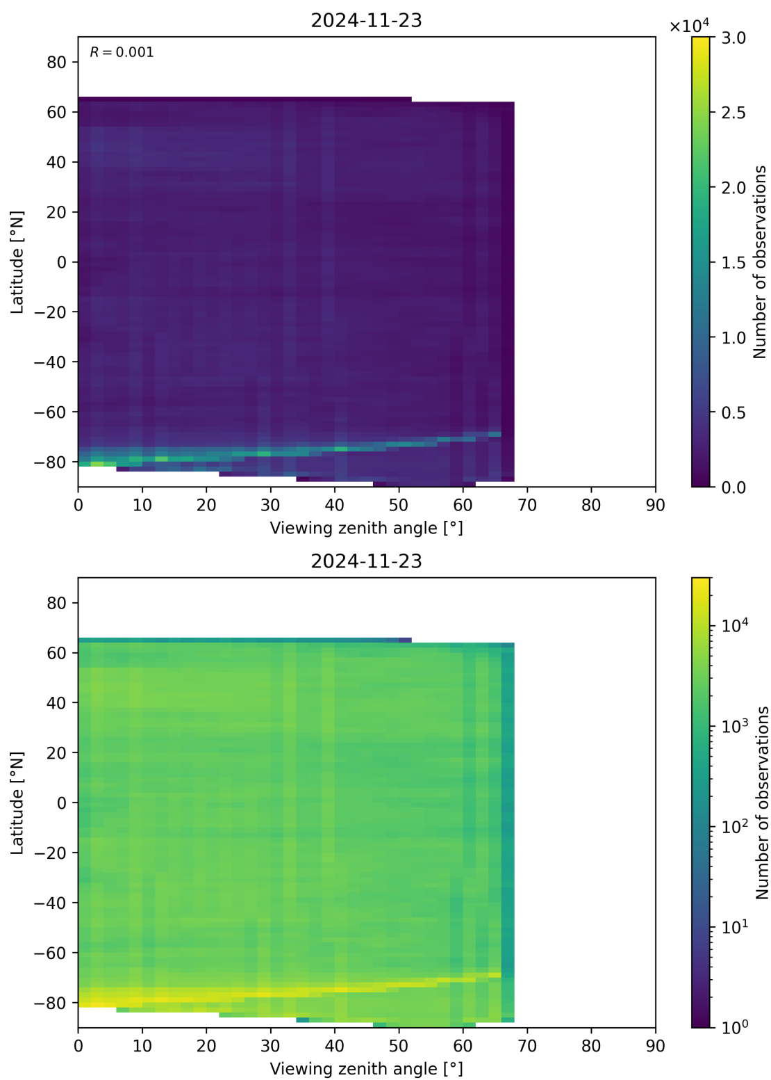
Figure 74: Scatter density plot of “Viewing zenith angle” against “Latitude” for 2024-11-22 to 2024-11-24.
