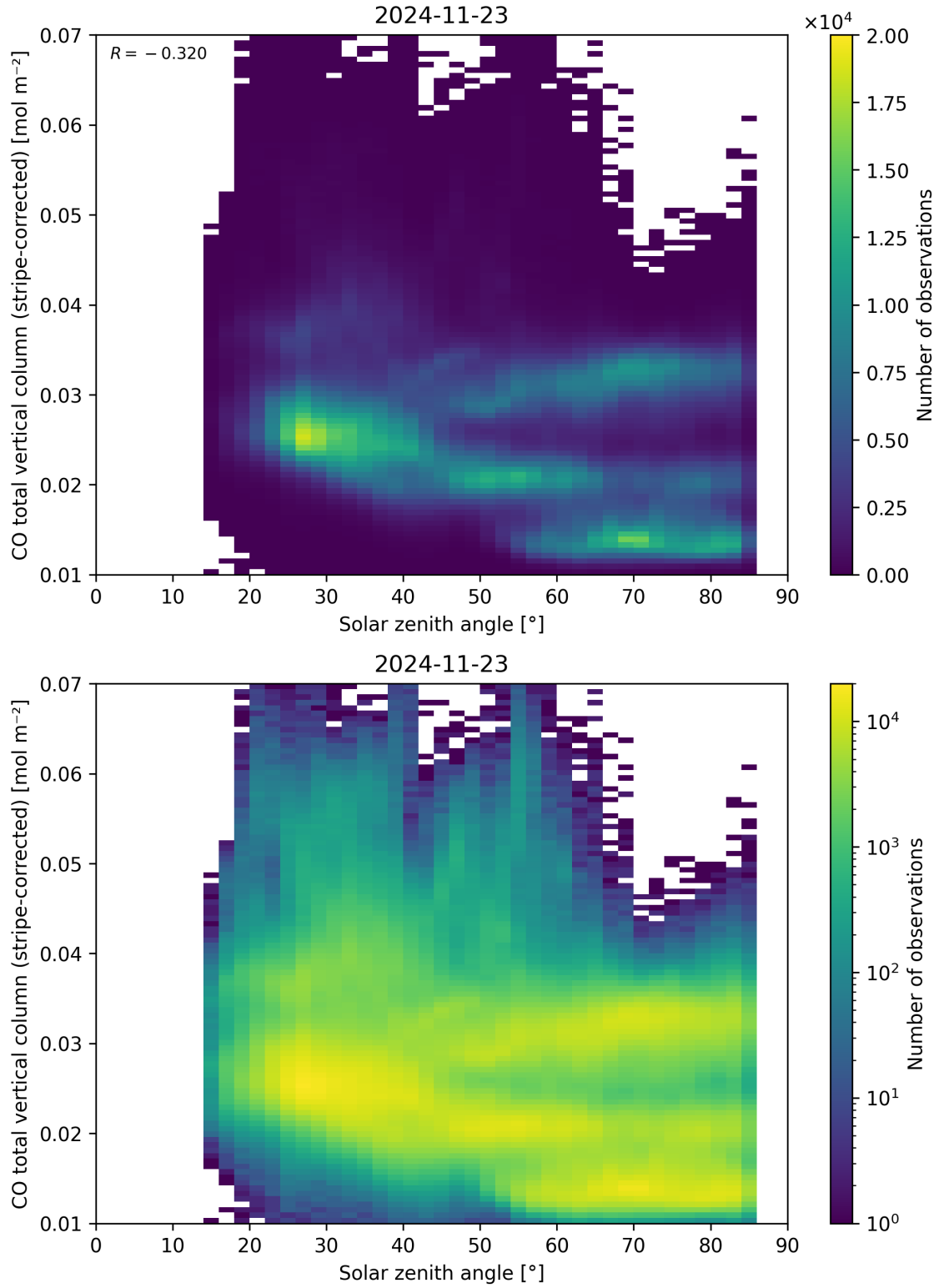
Figure 62: Scatter density plot of “Solar zenith angle” against “CO total vertical column (stripe-corrected)” for 2024-11-22 to 2024-11-24.
