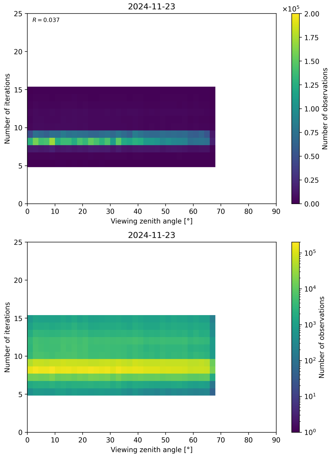
Figure 75: Scatter density plot of “Viewing zenith angle” against “Number of iterations” for 2024-11-22 to 2024-11-24.
