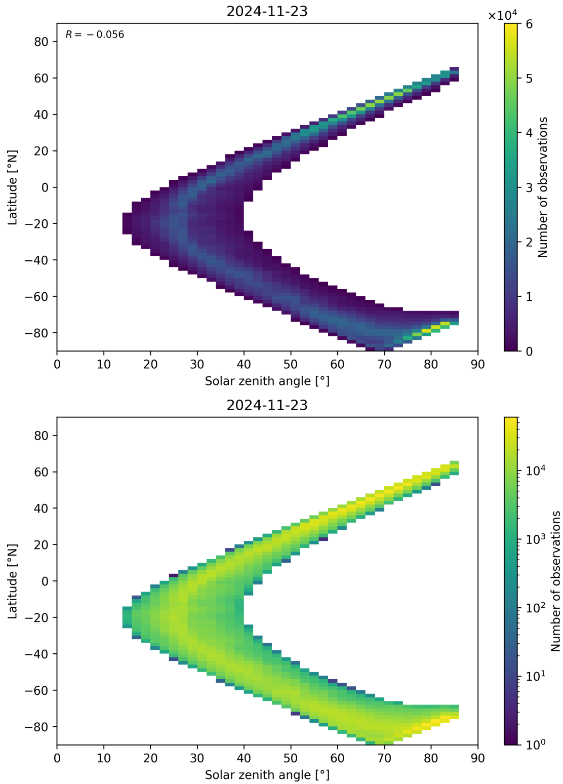
Figure 66: Scatter density plot of “Solar zenith angle” against “Latitude” for 2024-11-22 to 2024-11-24.
