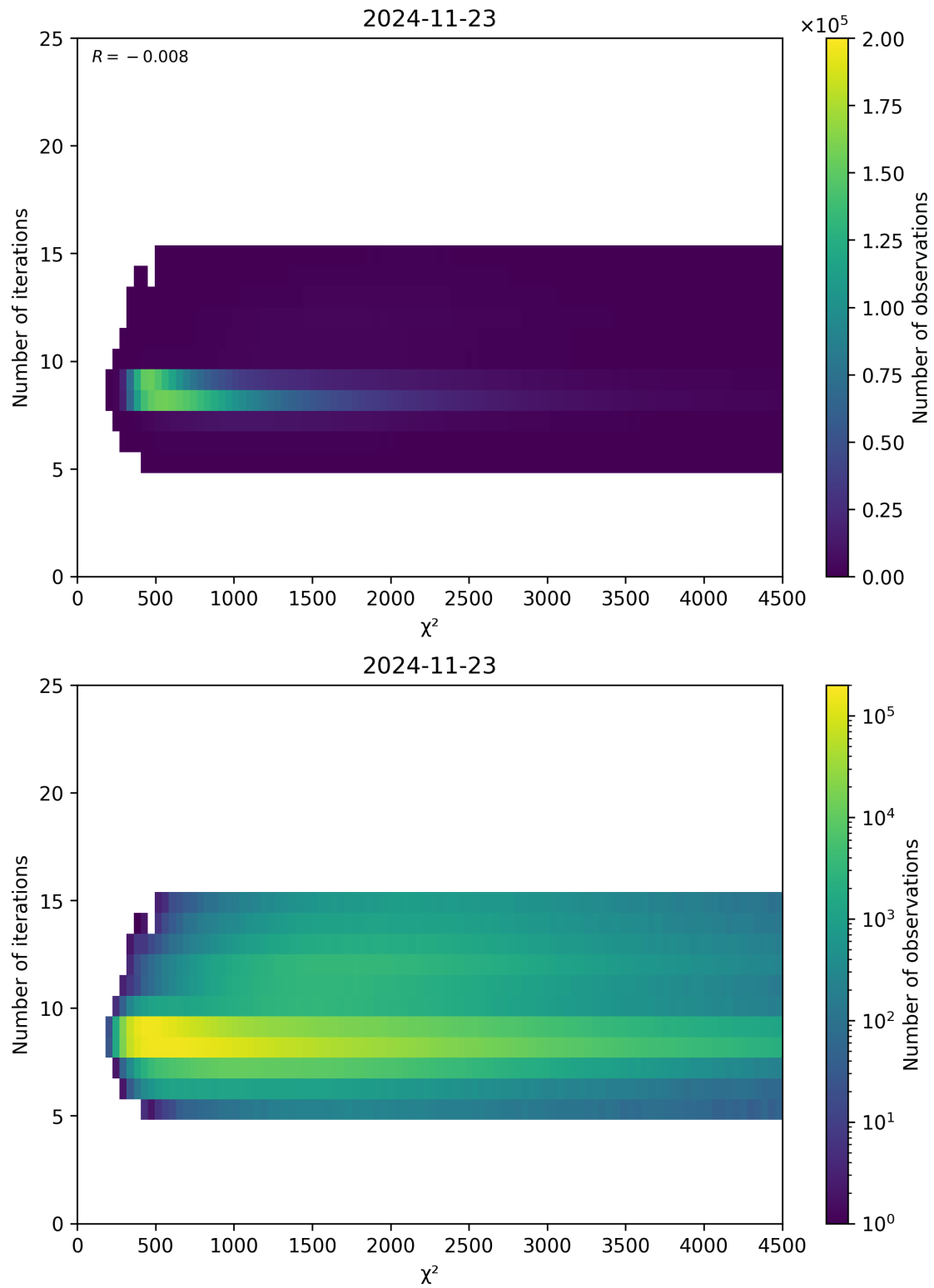
Figure 49: Scatter density plot of “ \chi^2 ” against “Number of iterations” for 2024-11-22 to 2024-11-24.
