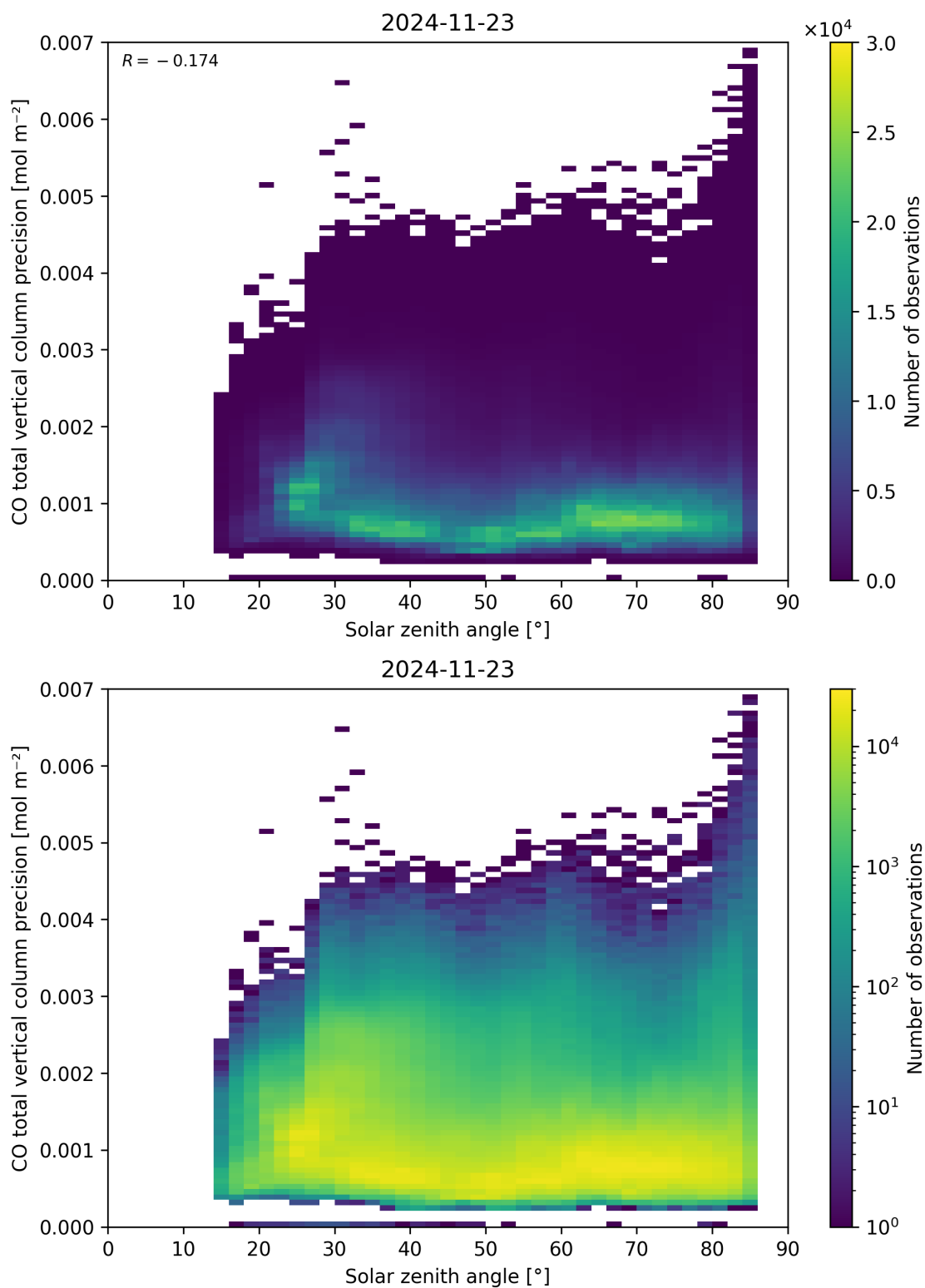
Figure 63: Scatter density plot of “Solar zenith angle” against “CO total vertical column precision” for 2024-11-22 to 2024-11-24.
