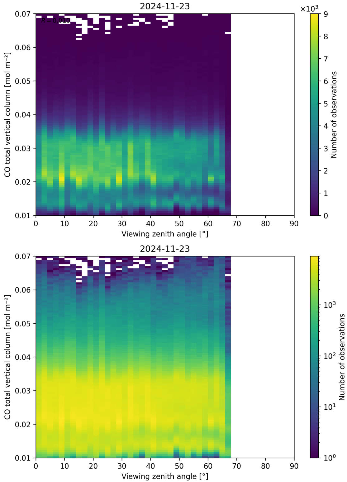
Figure 69: Scatter density plot of “Viewing zenith angle” against “CO total vertical column” for 2024-11-22 to 2024-11-24.
