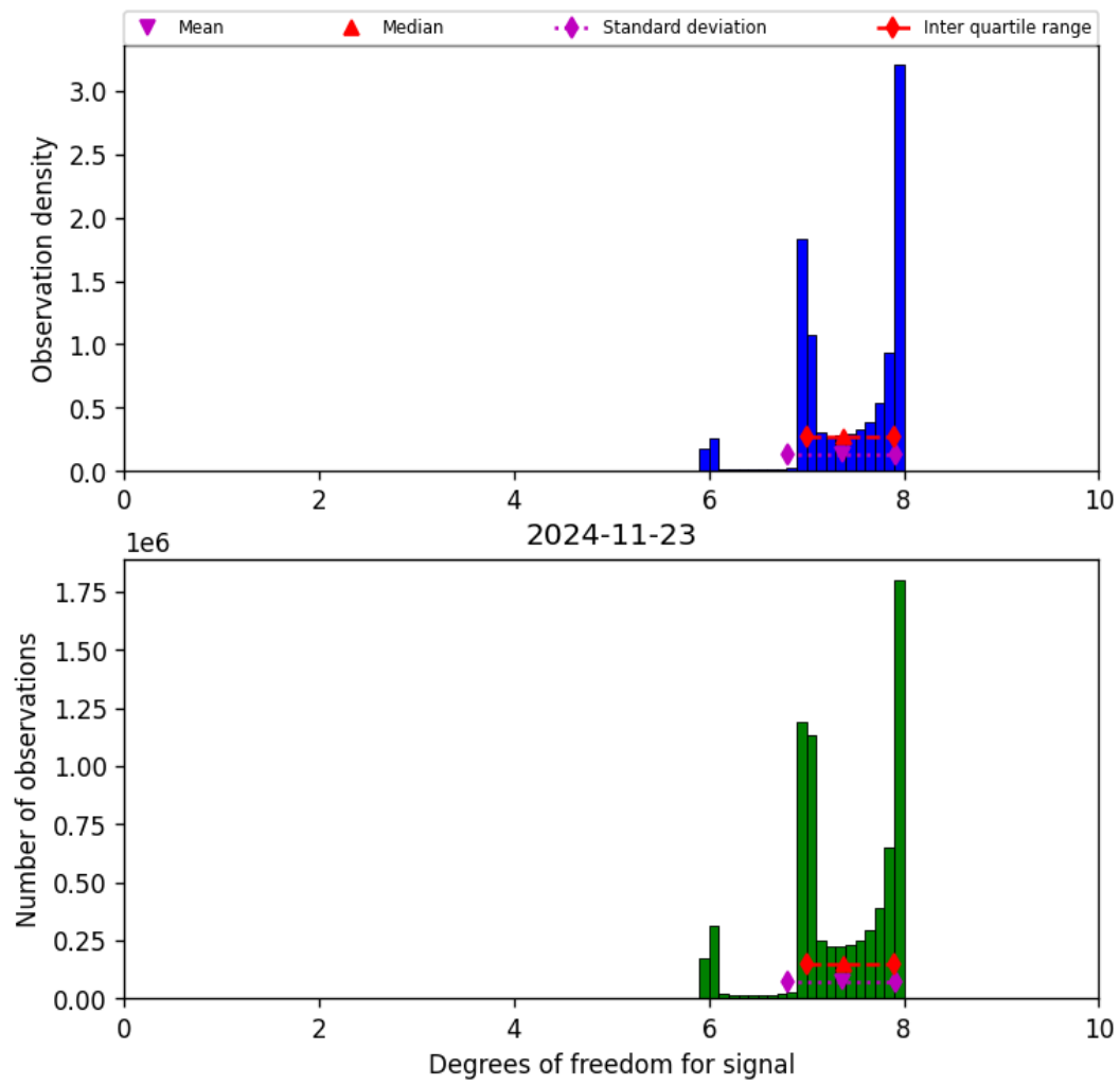
Figure 23: Histogram of “Degrees of freedom for signal” for 2024-11-22 to 2024-11-24
