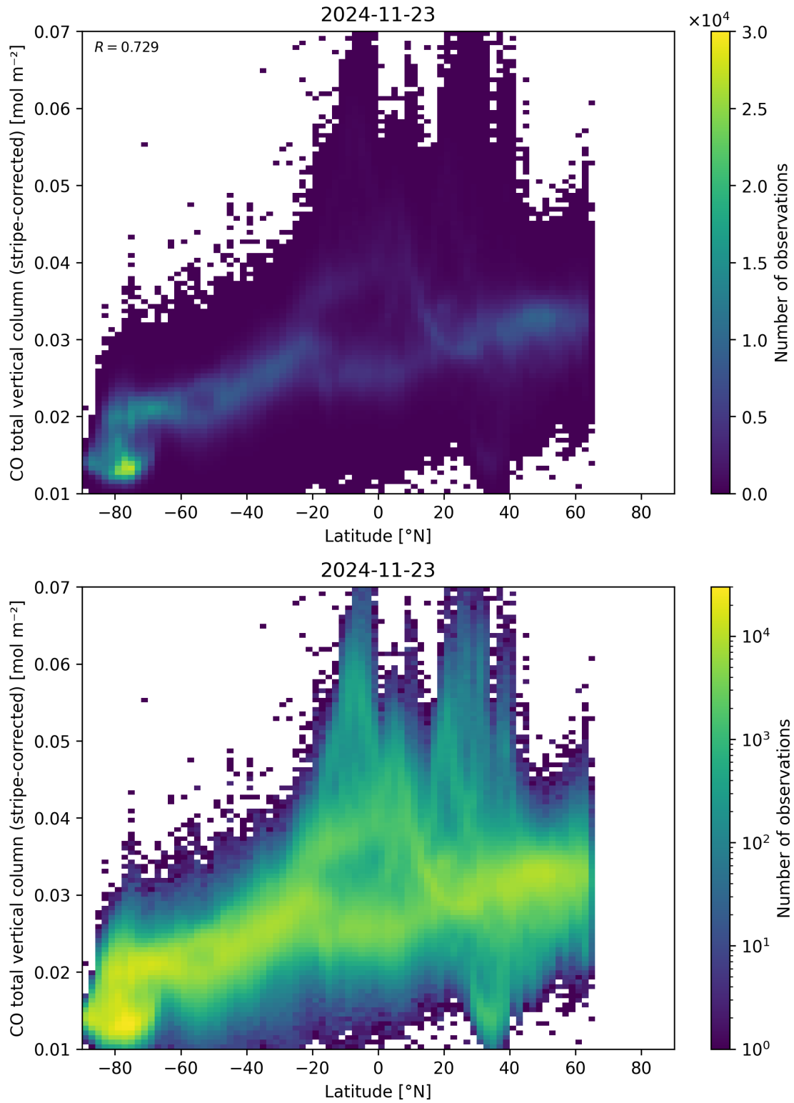
Figure 52: Scatter density plot of “Latitude” against “CO total vertical column (stripe-corrected)” for 2024-11-22 to 2024-11-24.
