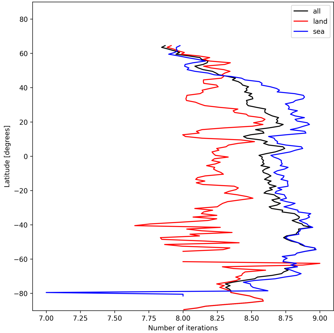
Figure 16: Zonal average of “Number of iterations” for 2024-11-22 to 2024-11-24.
