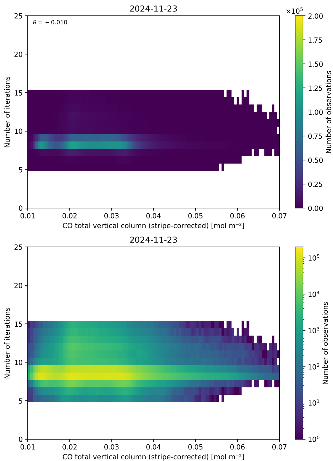
Figure 39: Scatter density plot of “CO total vertical column (stripe-corrected)” against “Number of iterations” for 2024-11-22 to 2024-11-24.
