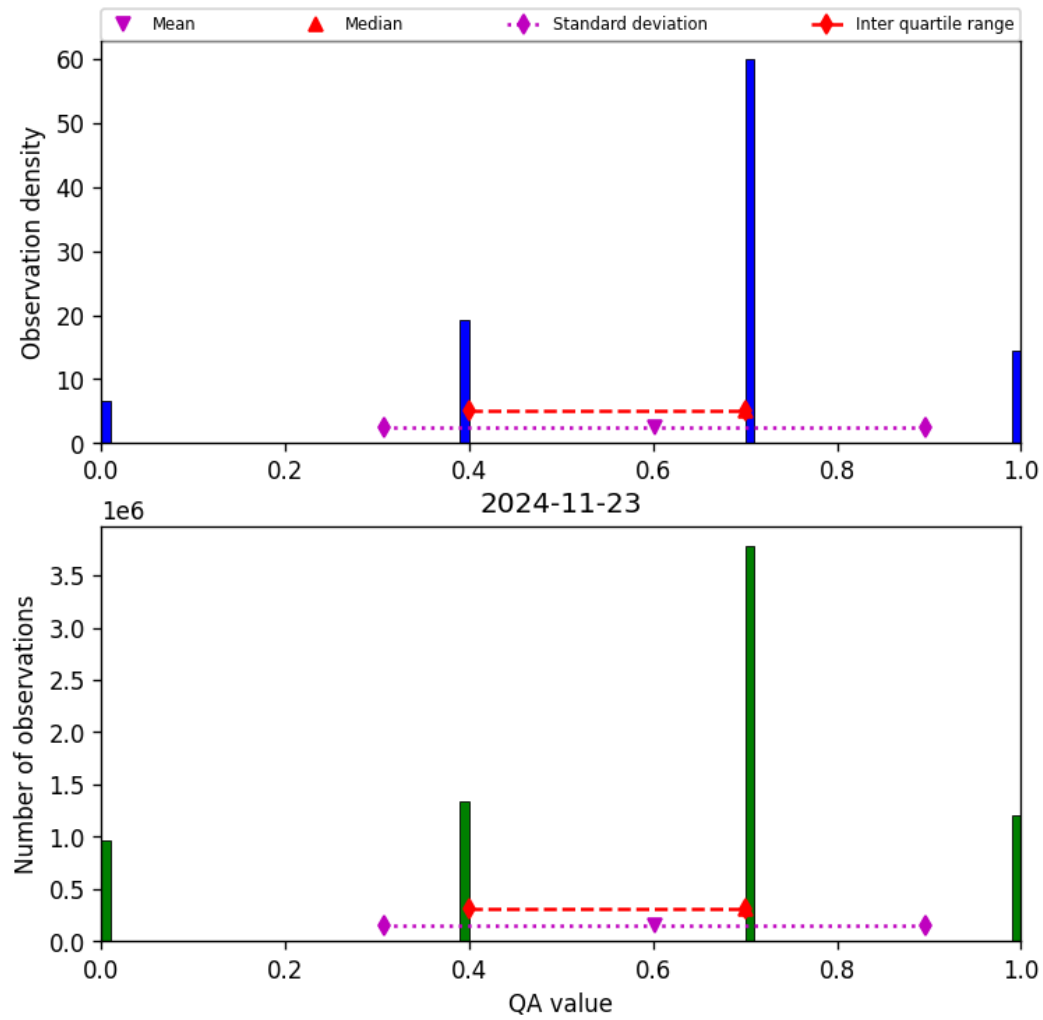
Figure 17: Histogram of “QA value” for 2024-11-22 to 2024-11-24
