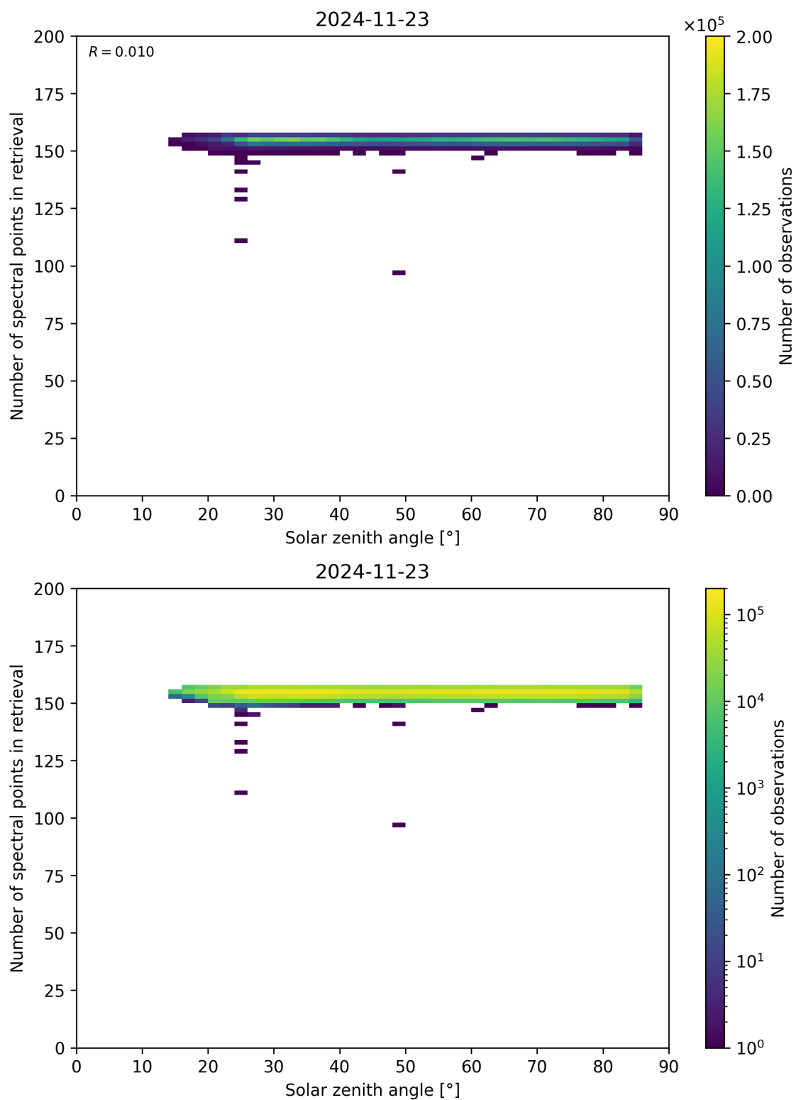
Figure 68: Scatter density plot of “Solar zenith angle” against “Number of spectral points in retrieval” for 2024-11-22 to 2024-11-24.
