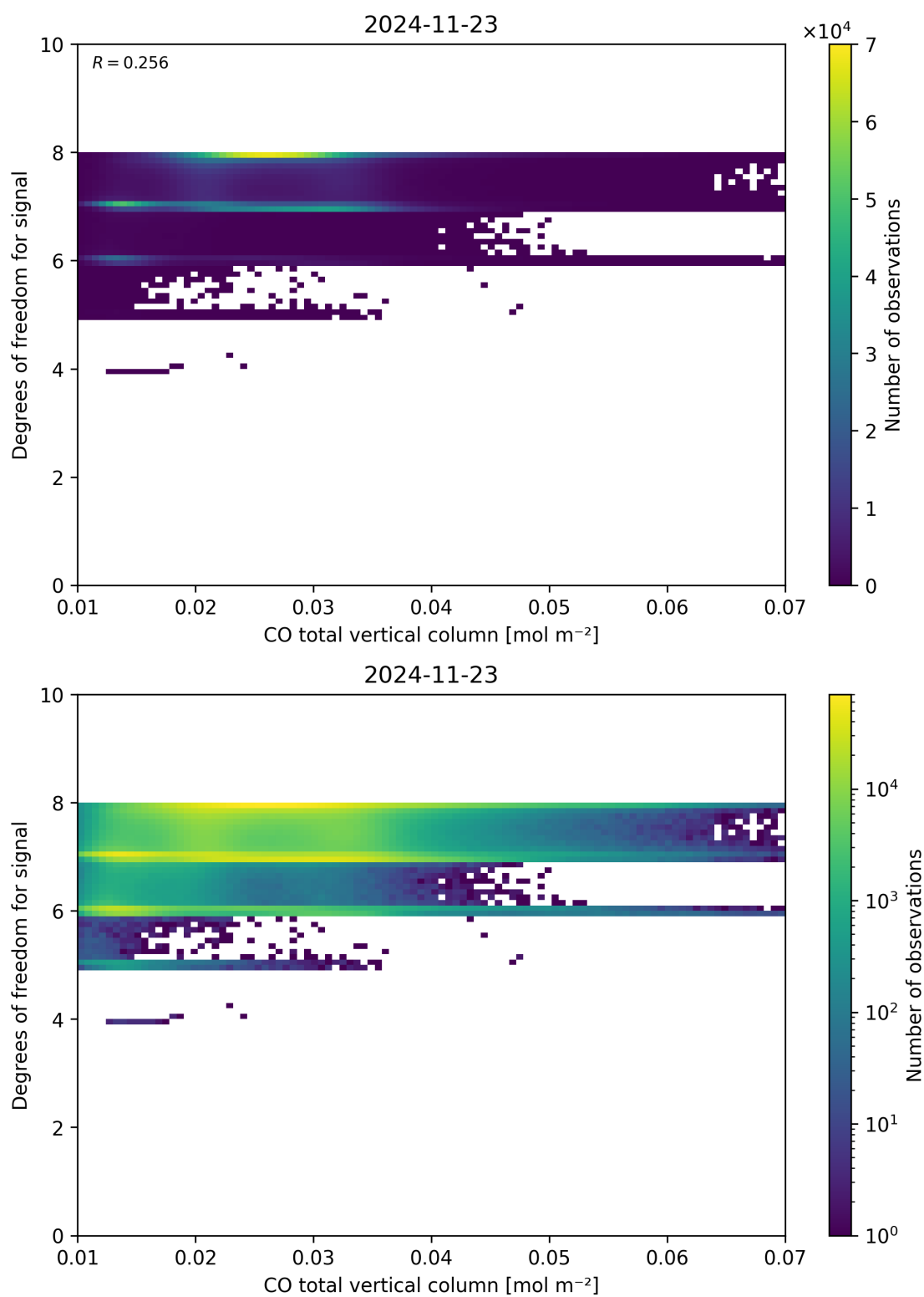
Figure 41: Scatter density plot of “CO total vertical column” against “Degrees of freedom for signal” for 2024-11-22 to 2024-11-24.
