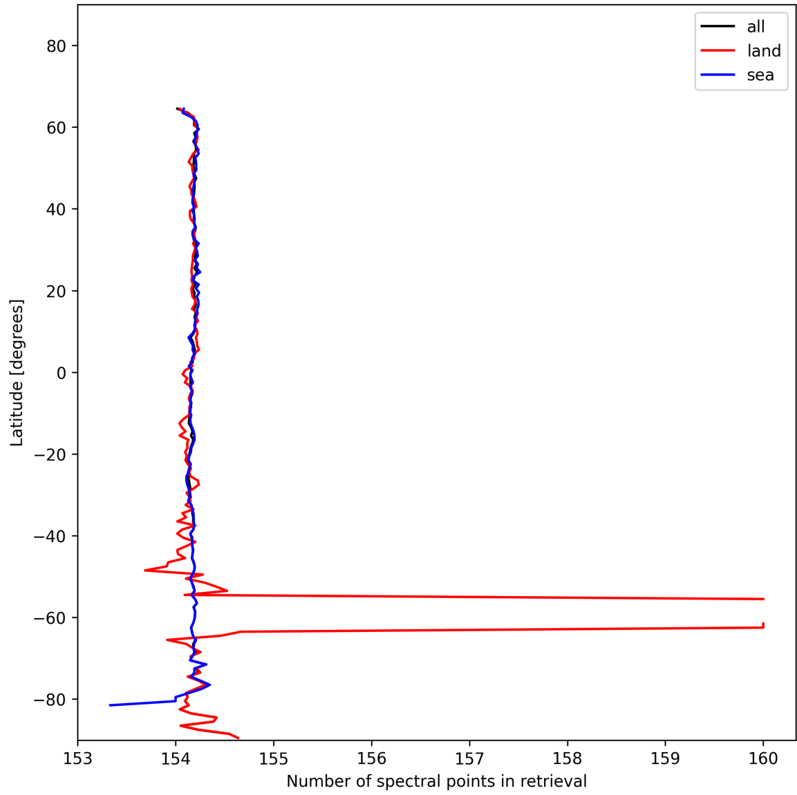
Figure 13: Zonal average of “Number of spectral points in retrieval” for 2024-11-22 to 2024-11-24.
