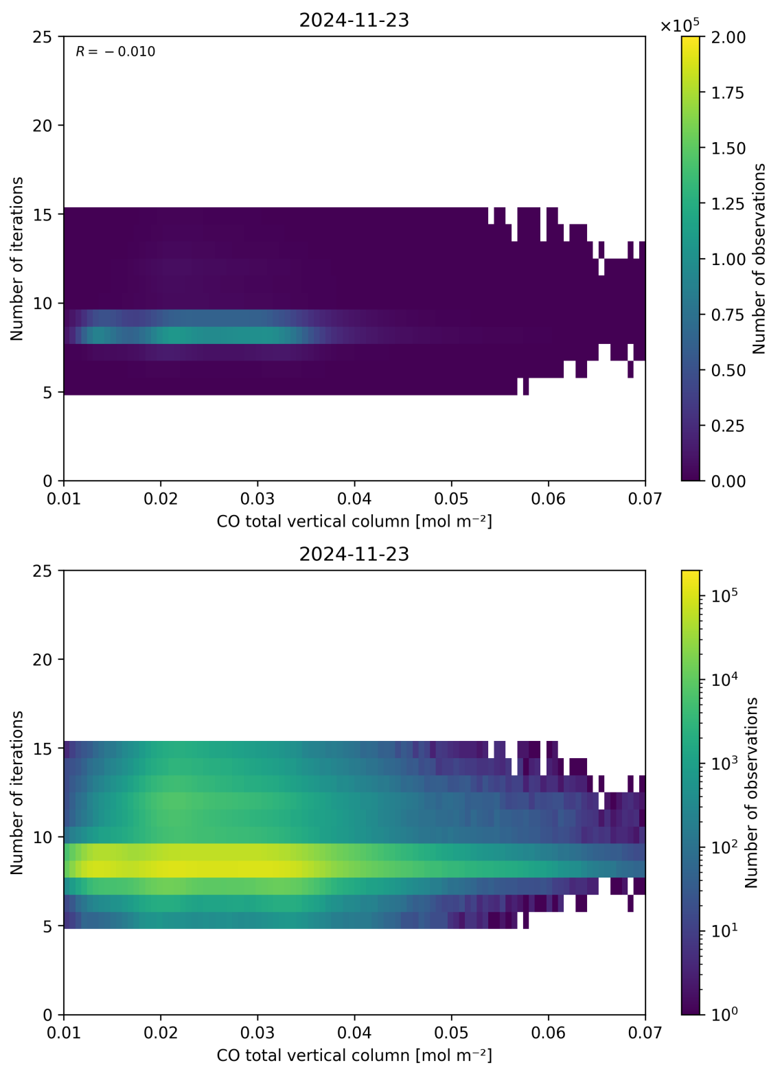
Figure 42: Scatter density plot of “CO total vertical column” against “Number of iterations” for 2024-11-22 to 2024-11-24.
