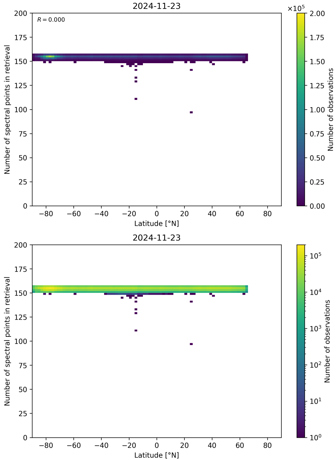
Figure 57: Scatter density plot of “Latitude” against “Number of spectral points in retrieval” for 2024-11-22 to 2024-11-24.
