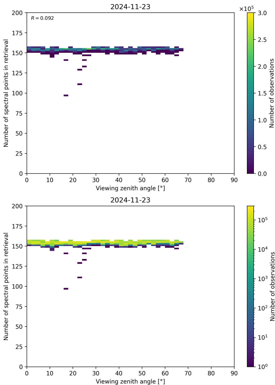
Figure 76: Scatter density plot of “Viewing zenith angle” against “Number of spectral points in retrieval” for 2024-11-22 to 2024-11-24.
