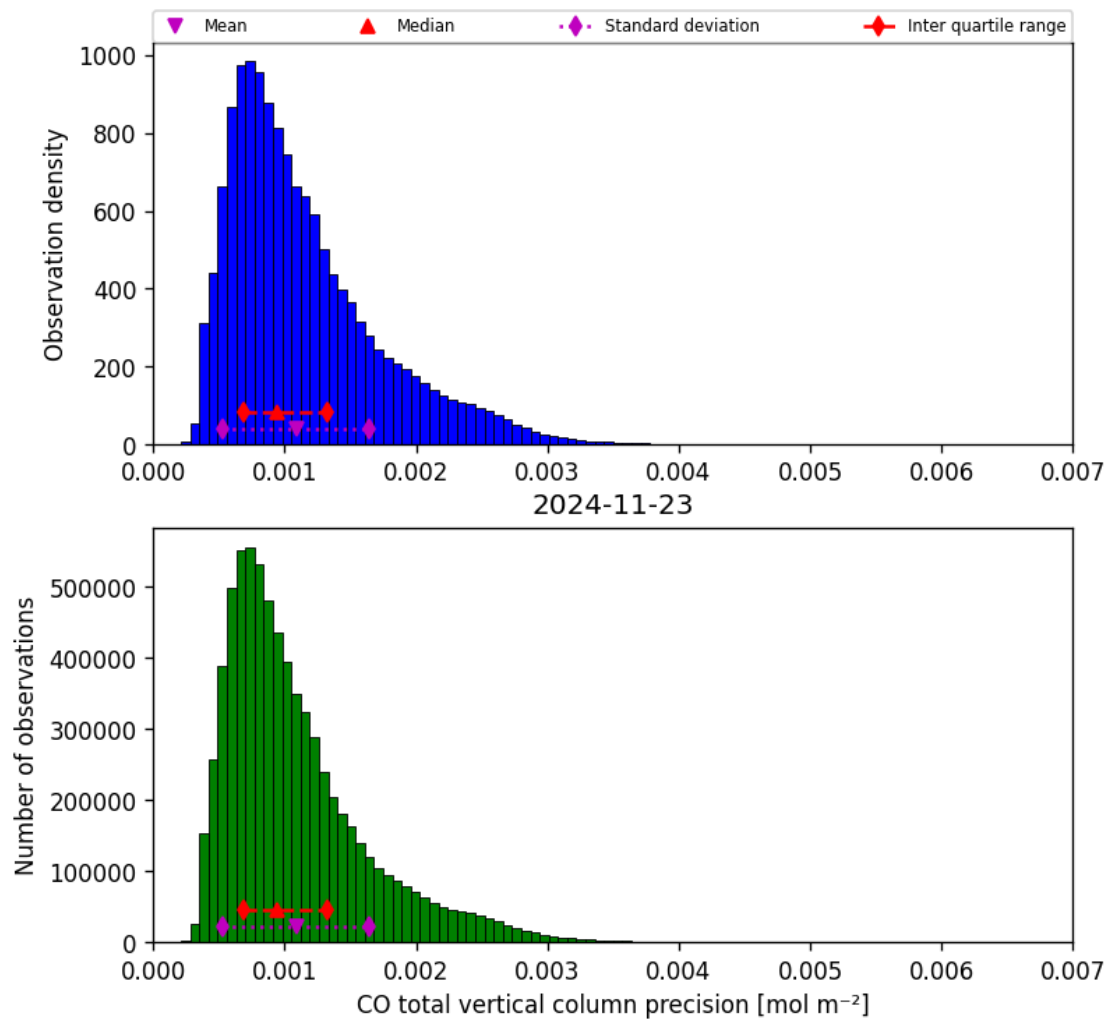
Figure 20: Histogram of “CO total vertical column precision” for 2024-11-22 to 2024-11-24
