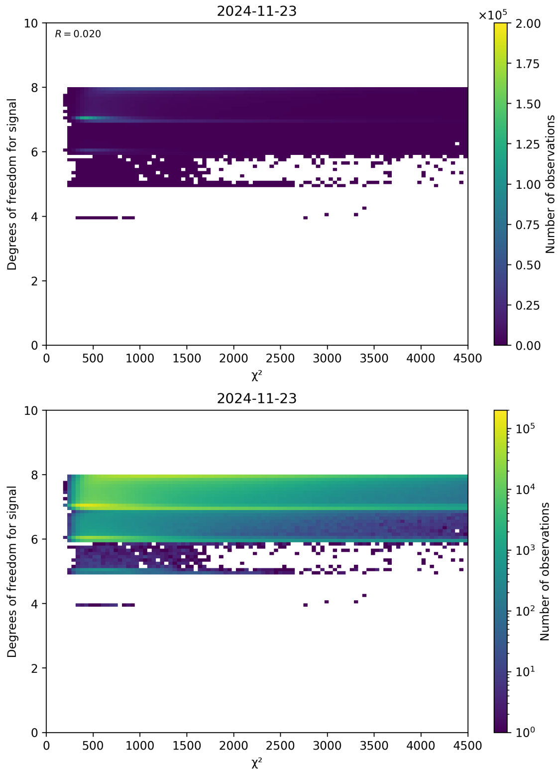
Figure 48: Scatter density plot of “ \chi^2 ” against “Degrees of freedom for signal” for 2024-11-22 to 2024-11-24.
