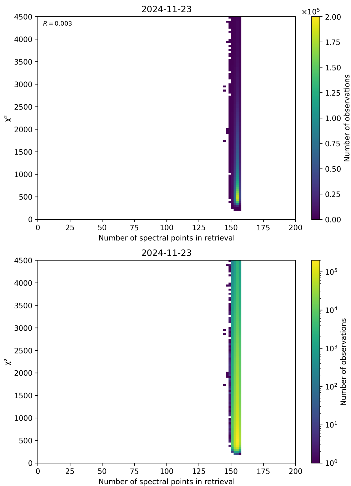
Figure 58: Scatter density plot of “Number of spectral points in retrieval” against “ \chi^2 ” for 2024-11-22 to 2024-11-24.
