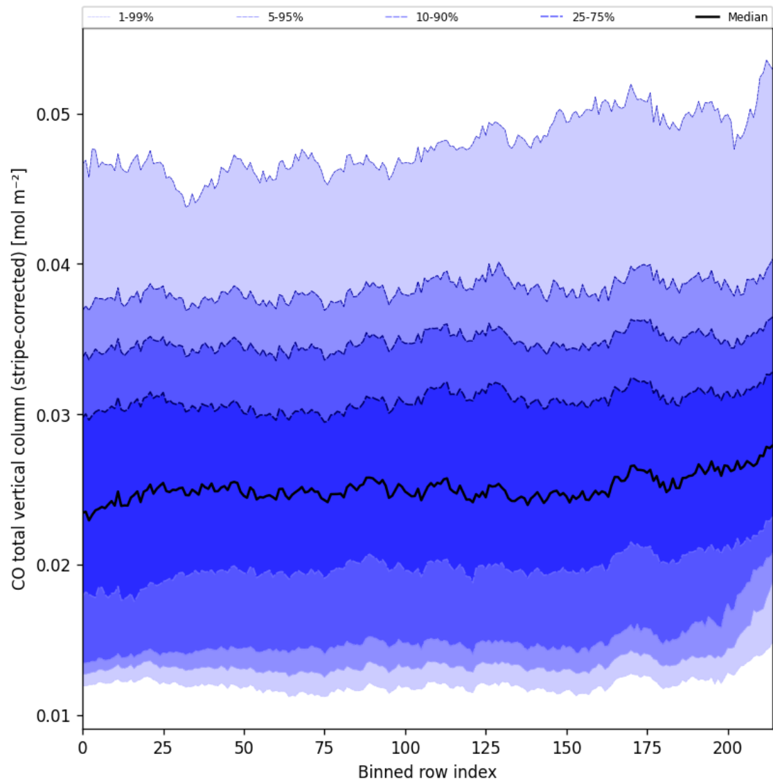
Figure 27: Along track statistics of "CO total vertical column (stripe-corrected)" for 2024-11-22 to 2024-11-24
